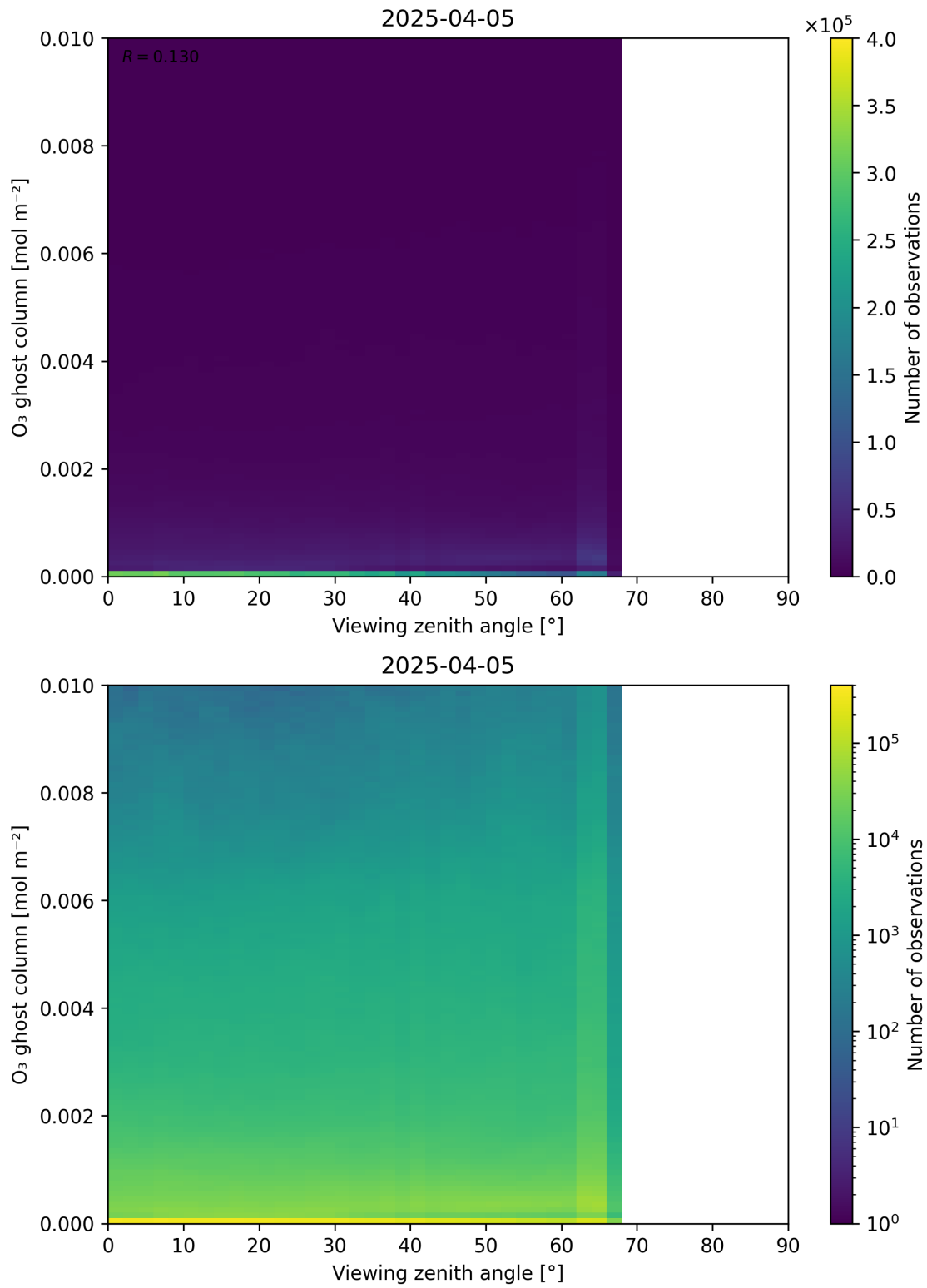
Figure 51: Scatter density plot of “Viewing zenith angle” against “O 3 ghost column” for 2025-04-04 to 2025-04-06.
