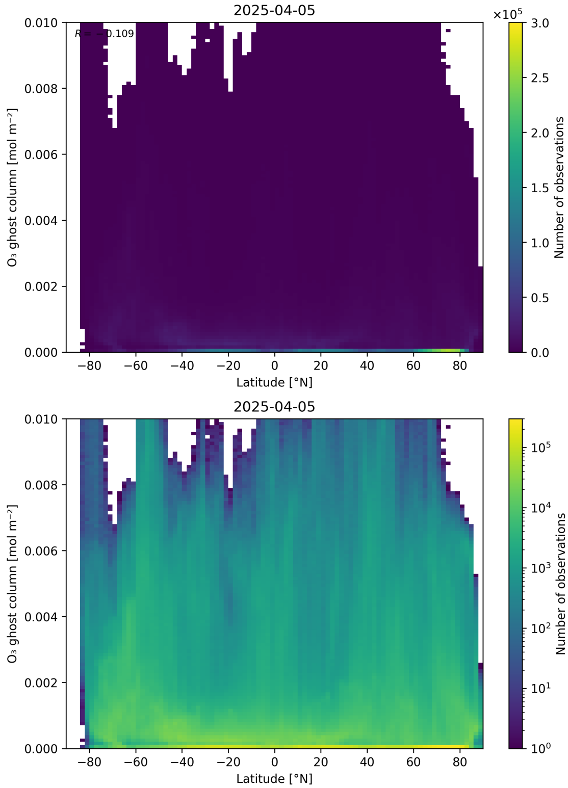
Figure 35: Scatter density plot of “Latitude” against “O 3 ghost column” for 2025-04-04 to 2025-04-06.
