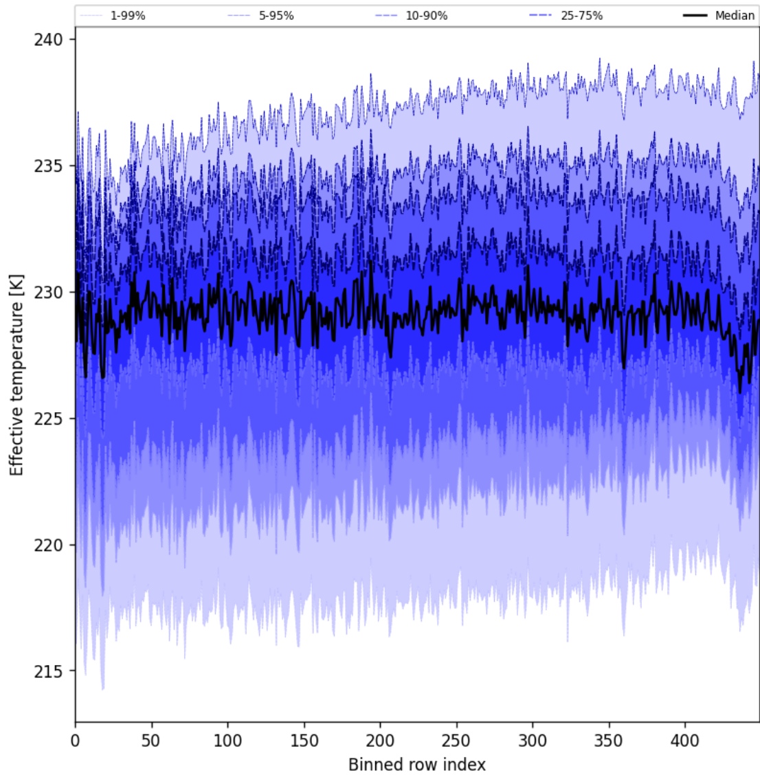
Figure 31: Along track statistics of “Effective temperature” for 2025-04-04 to 2025-04-06
