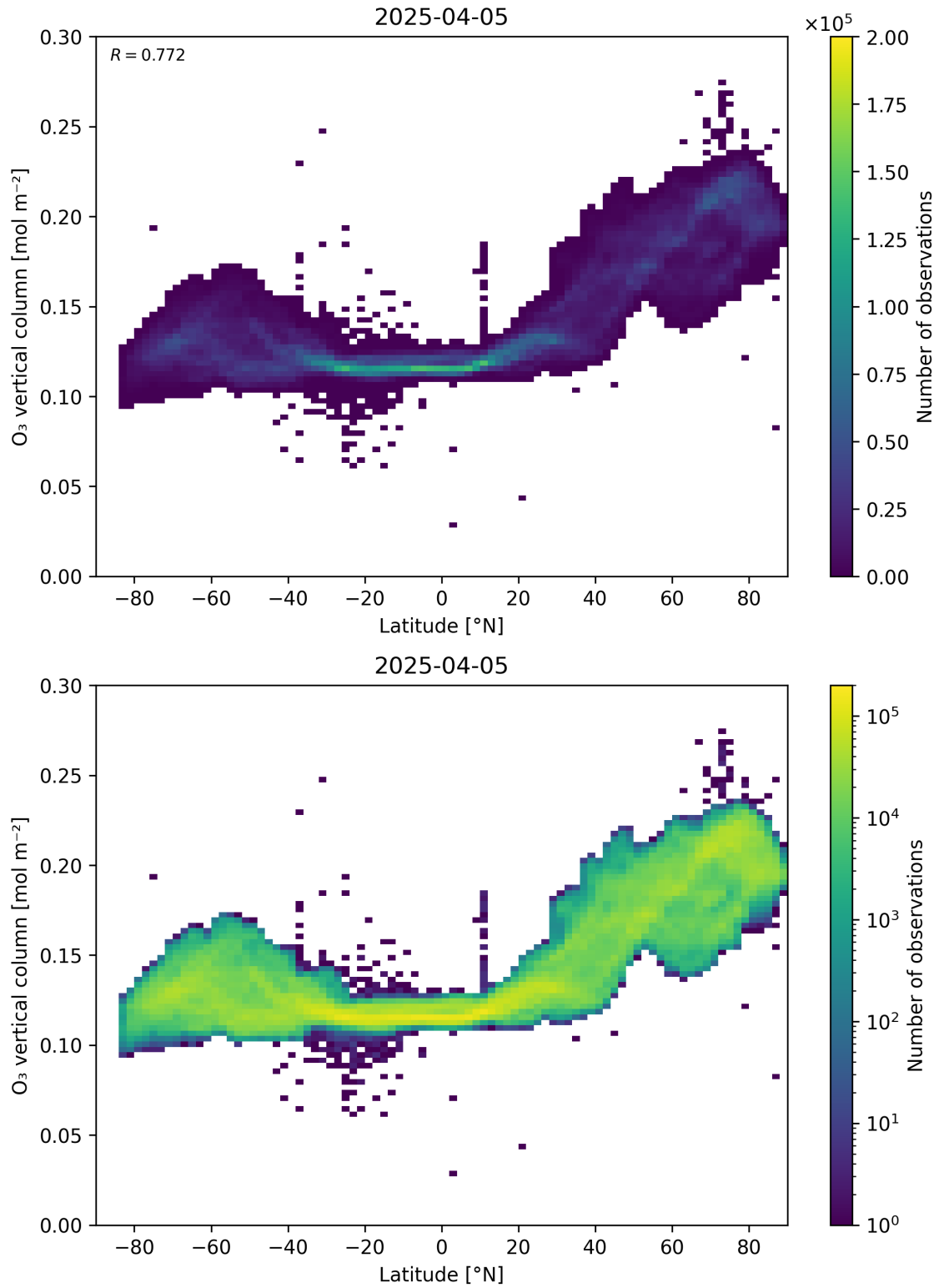
Figure 36: Scatter density plot of “Latitude” against “O 3 vertical column” for 2025-04-04 to 2025-04-06.
