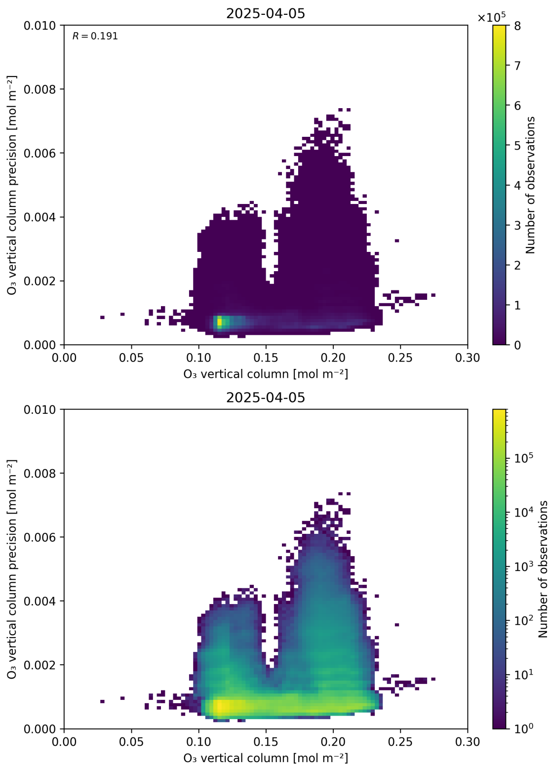
Figure 41: Scatter density plot of “O 3 vertical column” against “O 3 vertical column precision” for 2025-04-04 to 2025-04-06.
