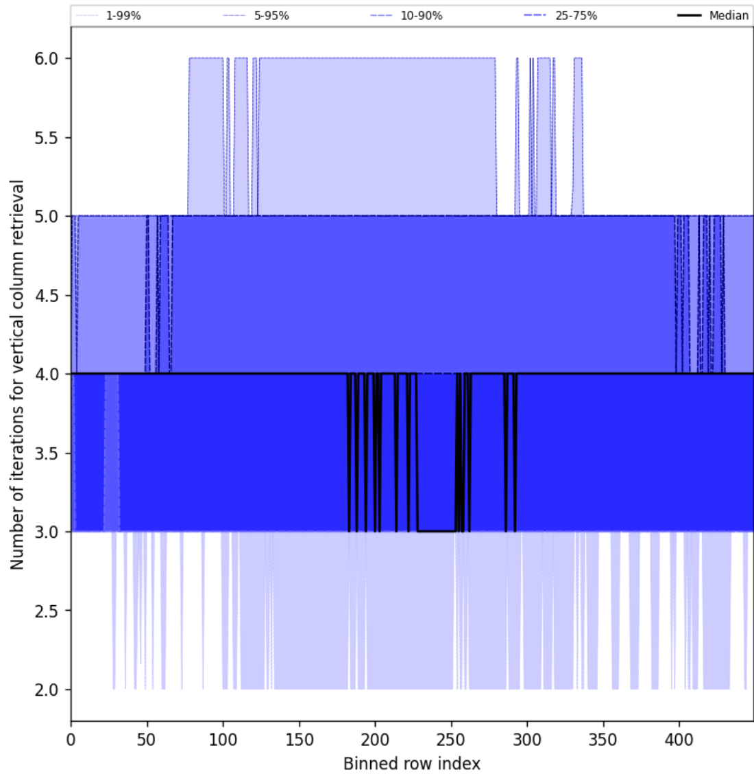
Figure 33: Along track statistics of “Number of iterations for vertical column retrieval” for 2025-04-04 to 2025-04-06
