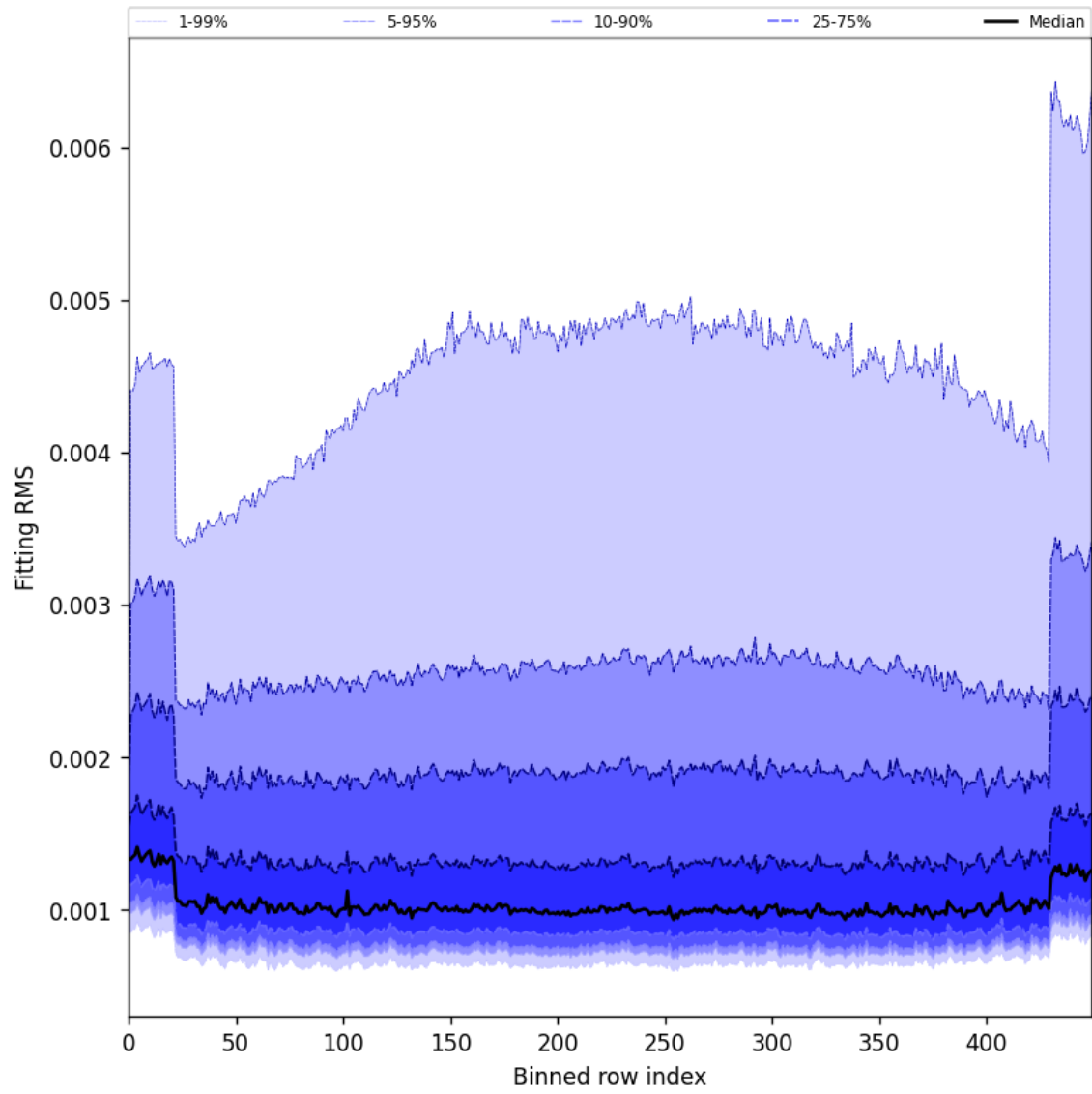
Figure 30: Along track statistics of “Fitting RMS” for 2025-04-04 to 2025-04-06
