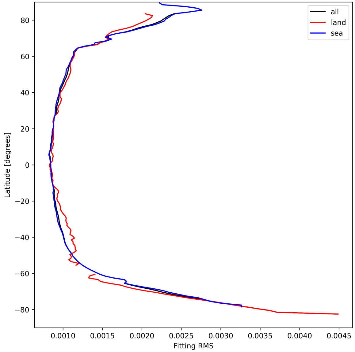
Figure 16: Zonal average of “Fitting RMS” for 2025-04-04 to 2025-04-06.
