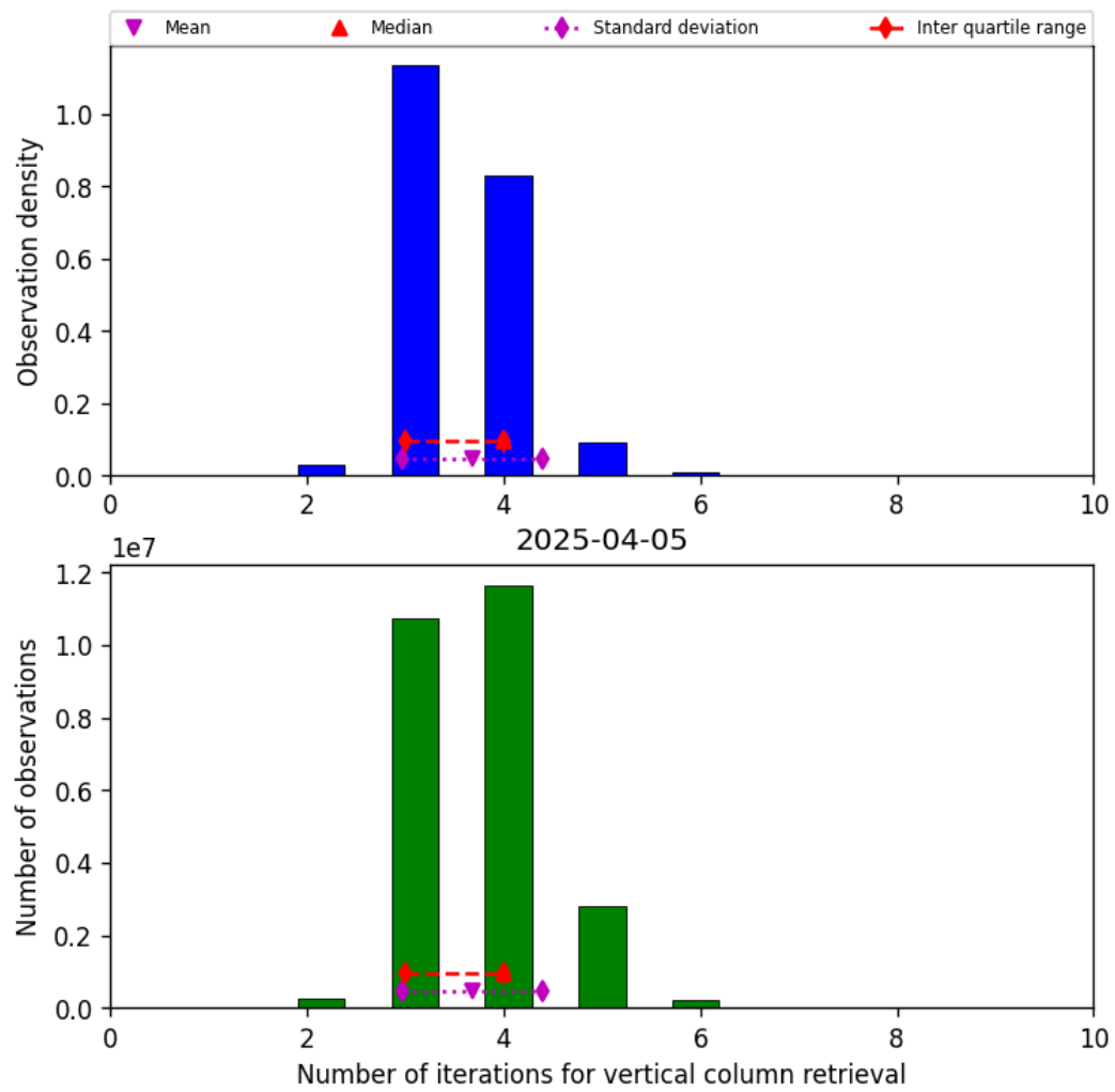
Figure 26: Histogram of “Number of iterations for vertical column retrieval” for 2025-04-04 to 2025-04-06
