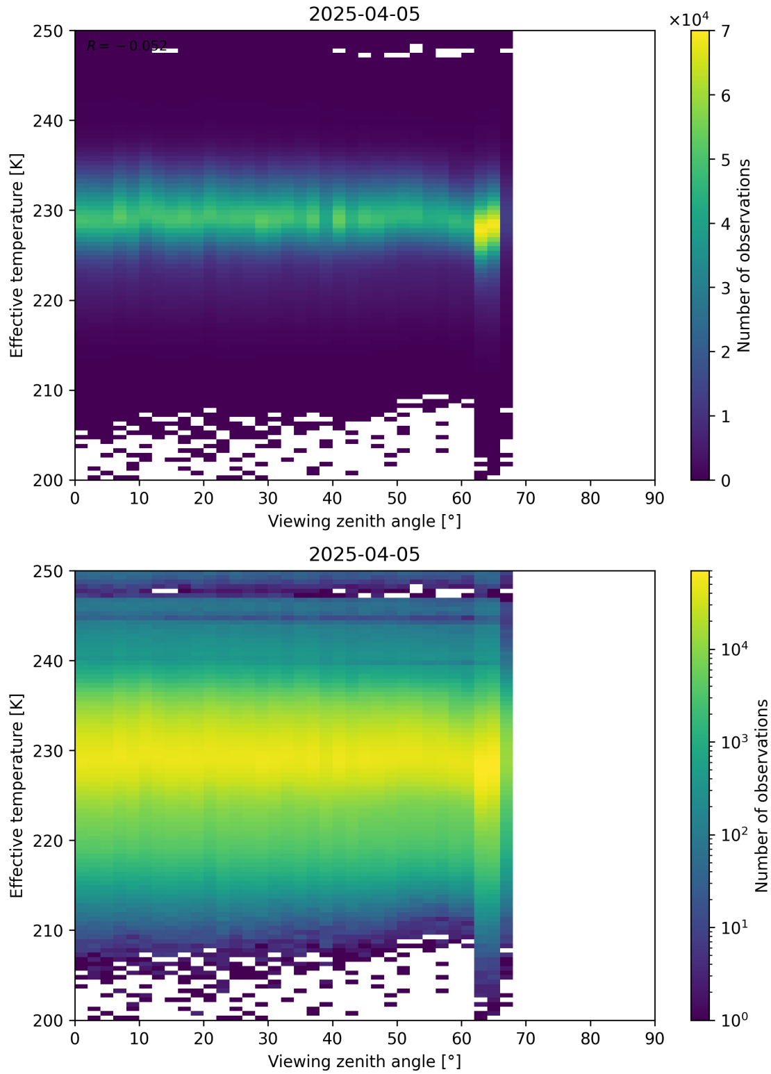
Figure 50: Scatter density plot of “Viewing zenith angle” against “Effective temperature” for 2025-04-04 to 2025-04-06.
