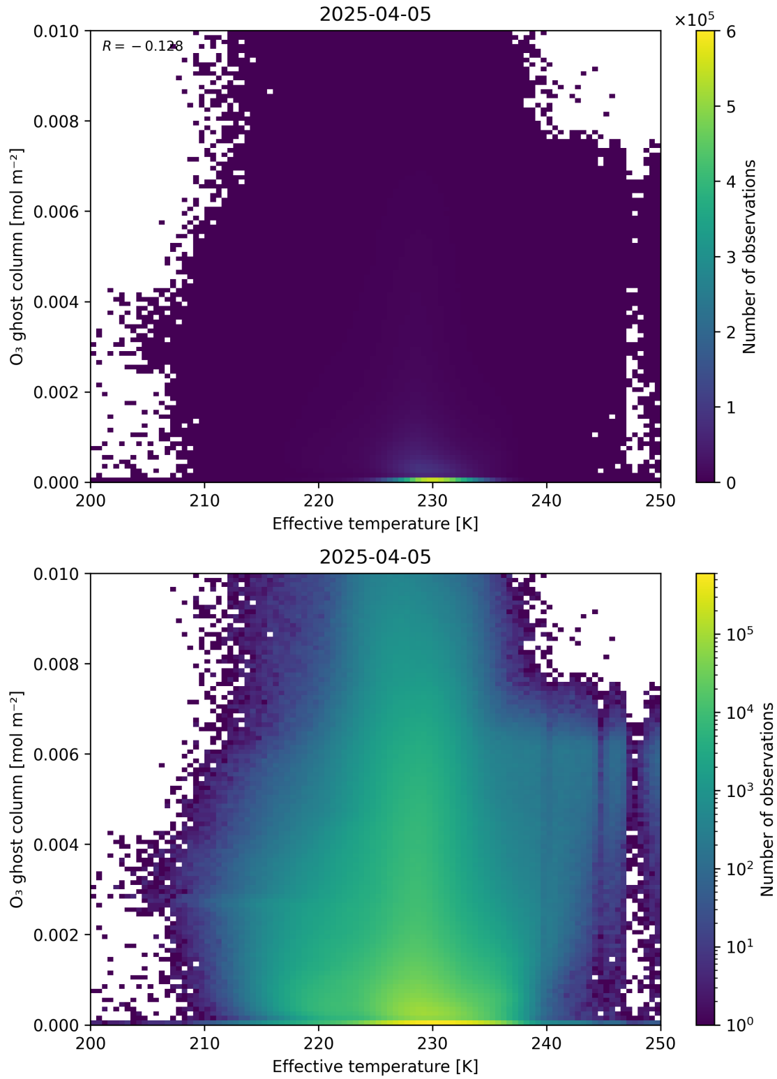
Figure 38: Scatter density plot of “Effective temperature” against “O 3 ghost column” for 2025-04-04 to 2025-04-06.
