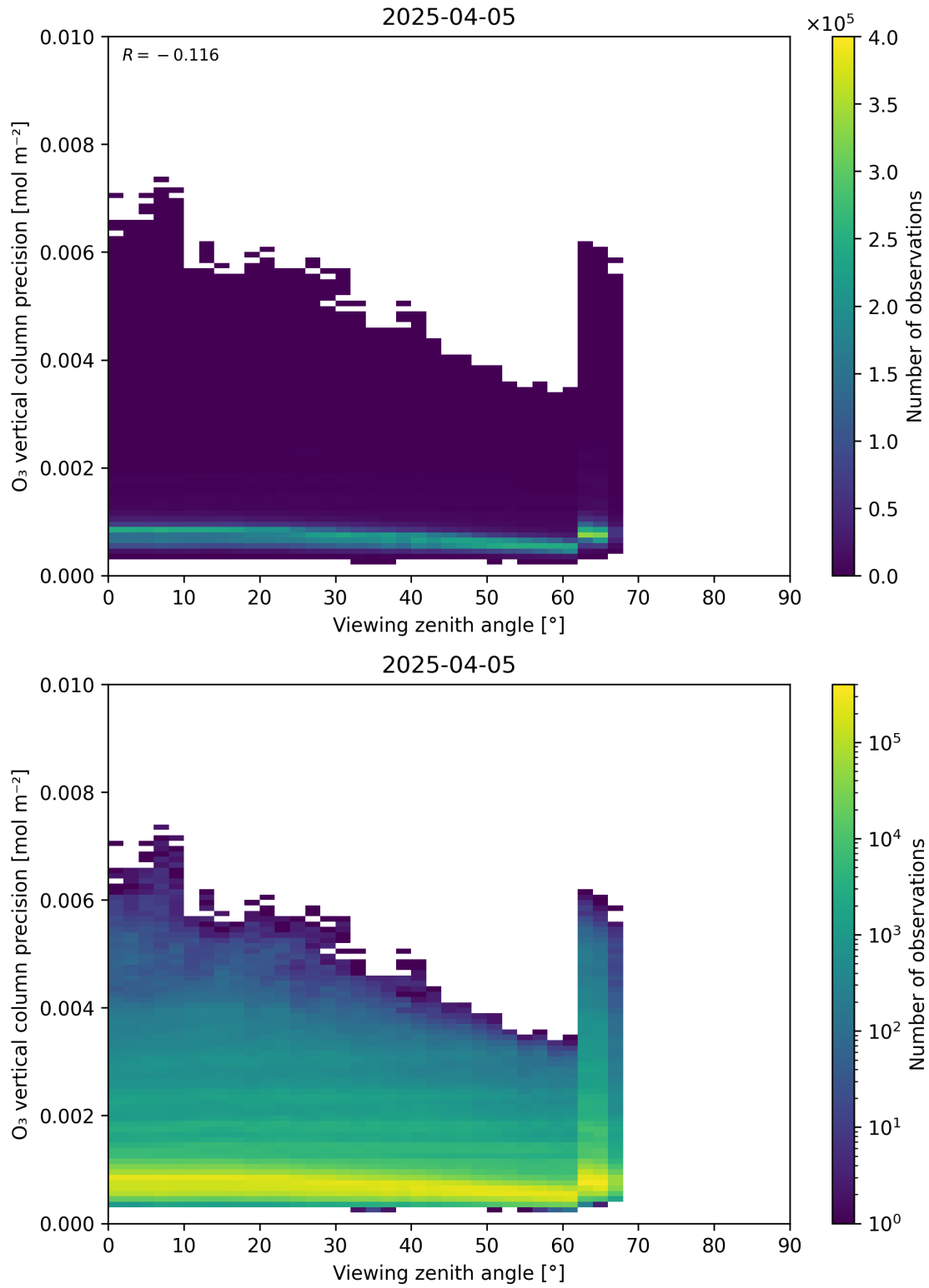
Figure 53: Scatter density plot of “Viewing zenith angle” against “O 3 vertical column precision” for 2025-04-04 to 2025-04-06.
