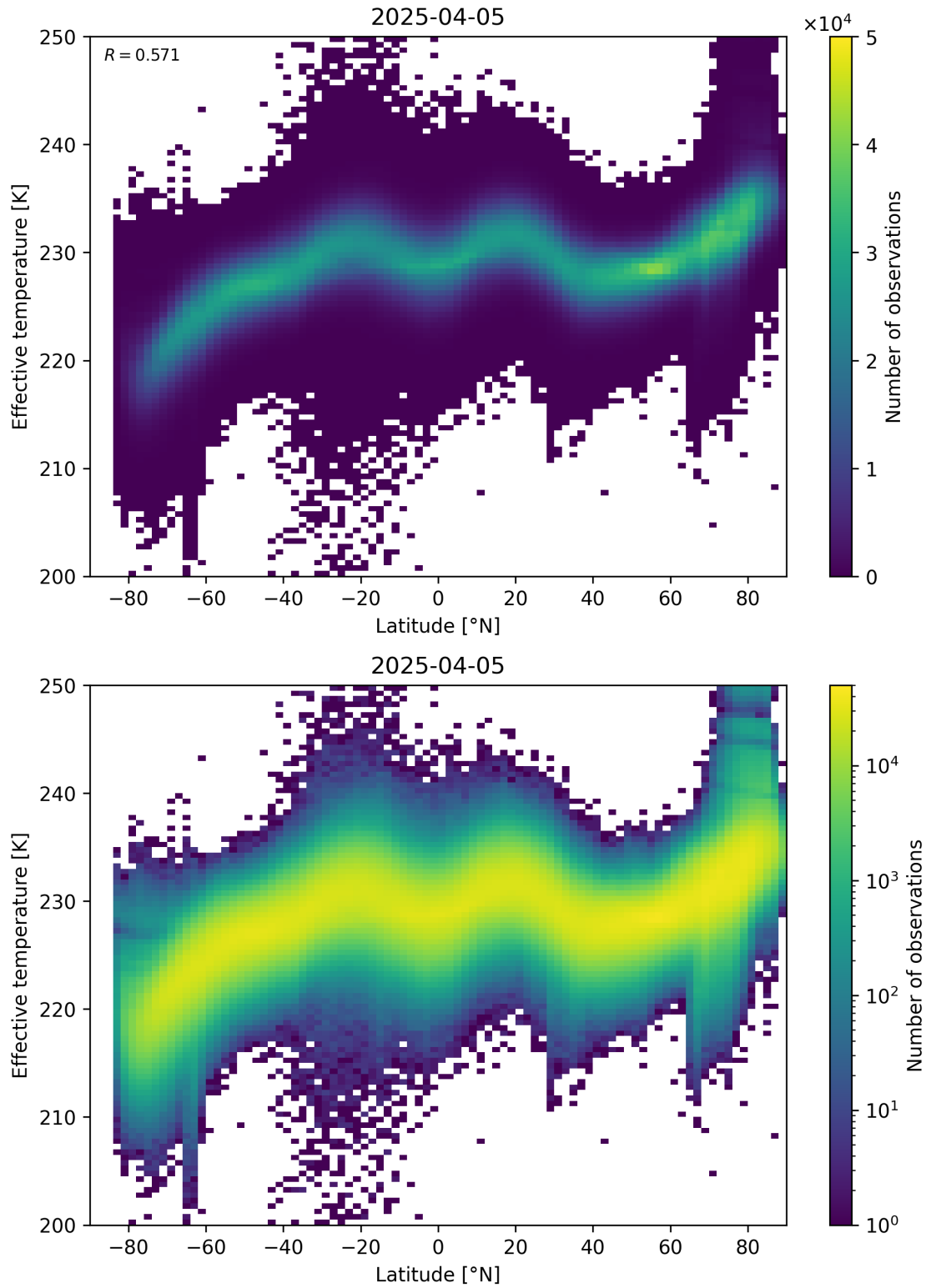
Figure 34: Scatter density plot of “Latitude” against “Effective temperature” for 2025-04-04 to 2025-04-06.
