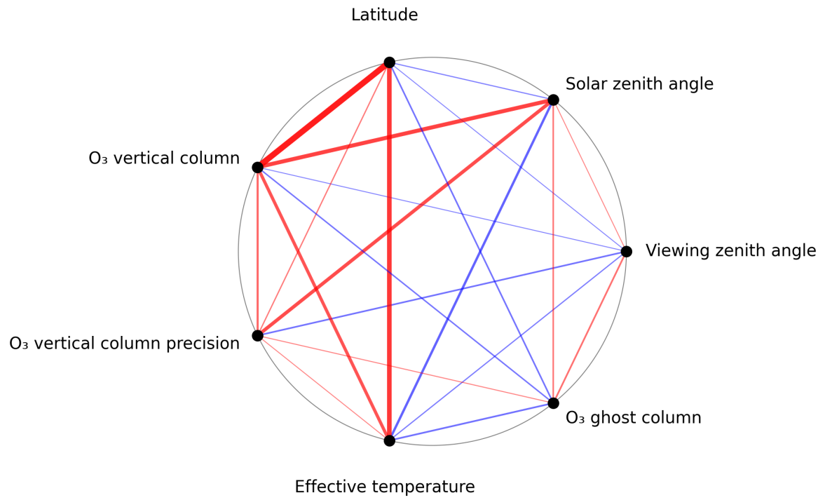
Figure 1: Map of correlation graph for 2025-04-04 to 2025-04-06.
