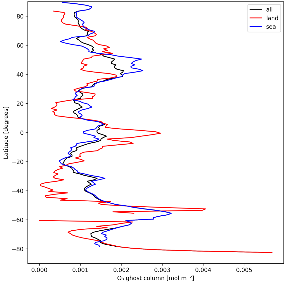
Figure 18: Zonal average of "O 3 ghost column" for 2025-04-04 to 2025-04-06.
