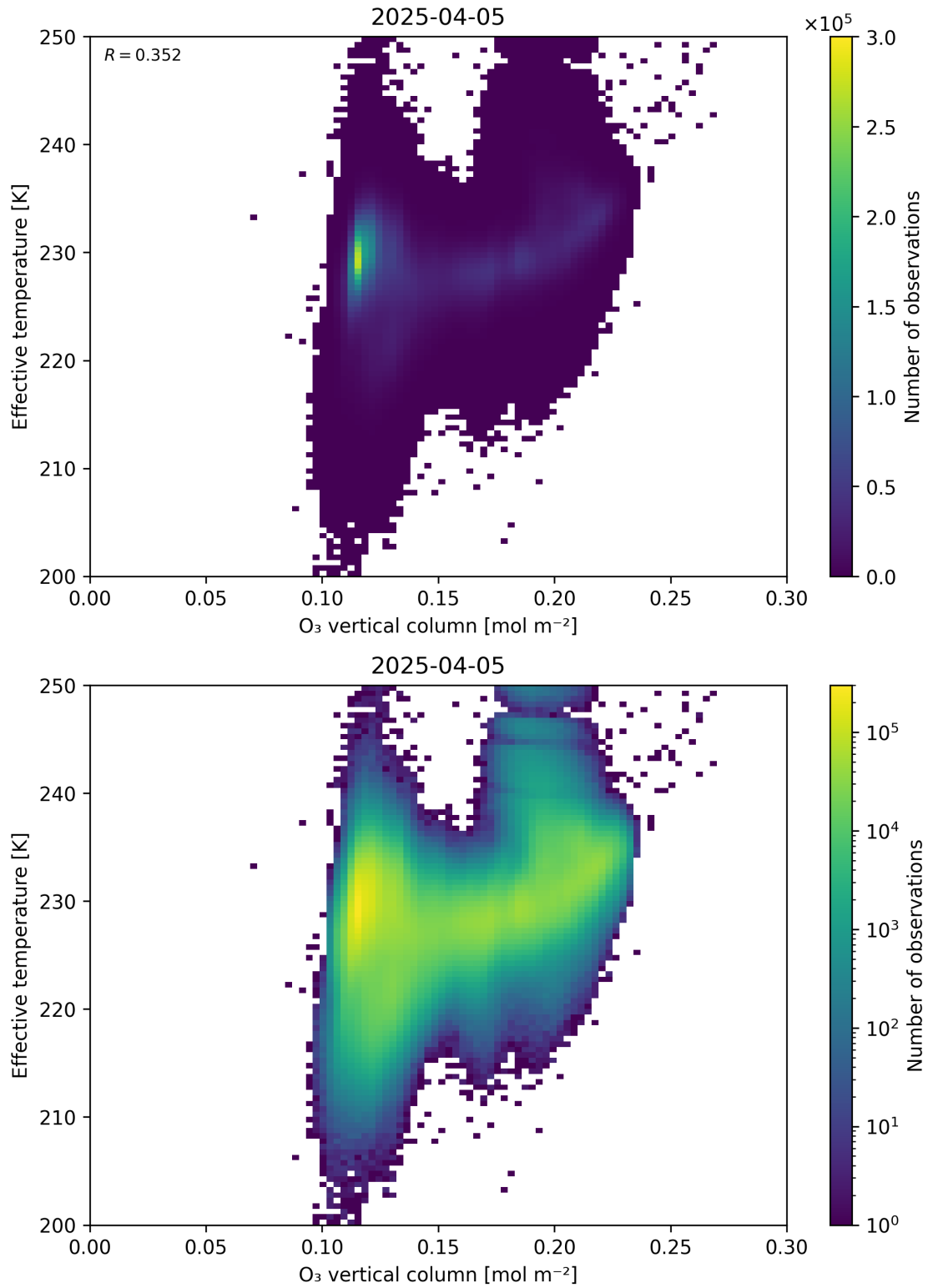
Figure 39: Scatter density plot of “O 3 vertical column” against “Effective temperature” for 2025-04-04 to 2025-04-06.
