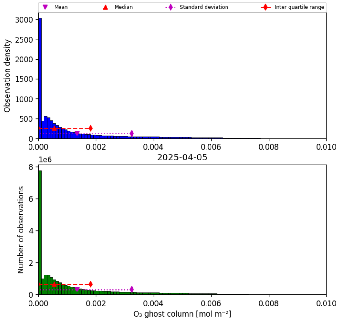
Figure 25: Histogram of “O 3 ghost column” for 2025-04-04 to 2025-04-06
