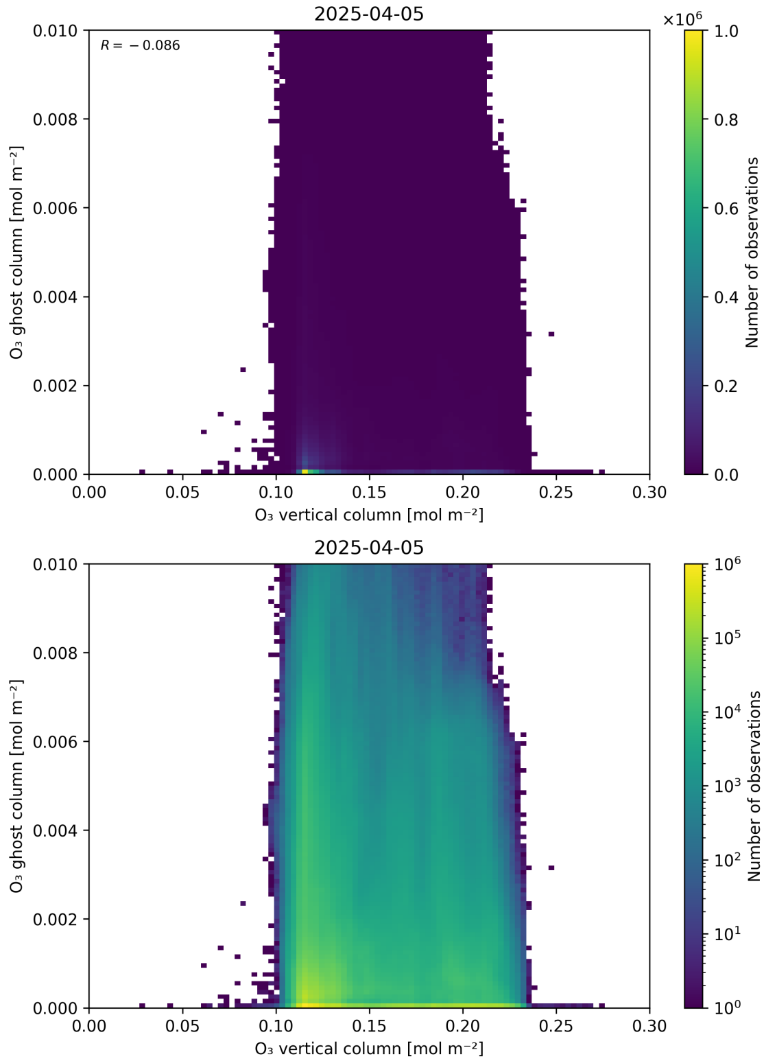
Figure 40: Scatter density plot of “O 3 vertical column” against “O 3 ghost column” for 2025-04-04 to 2025-04-06.
