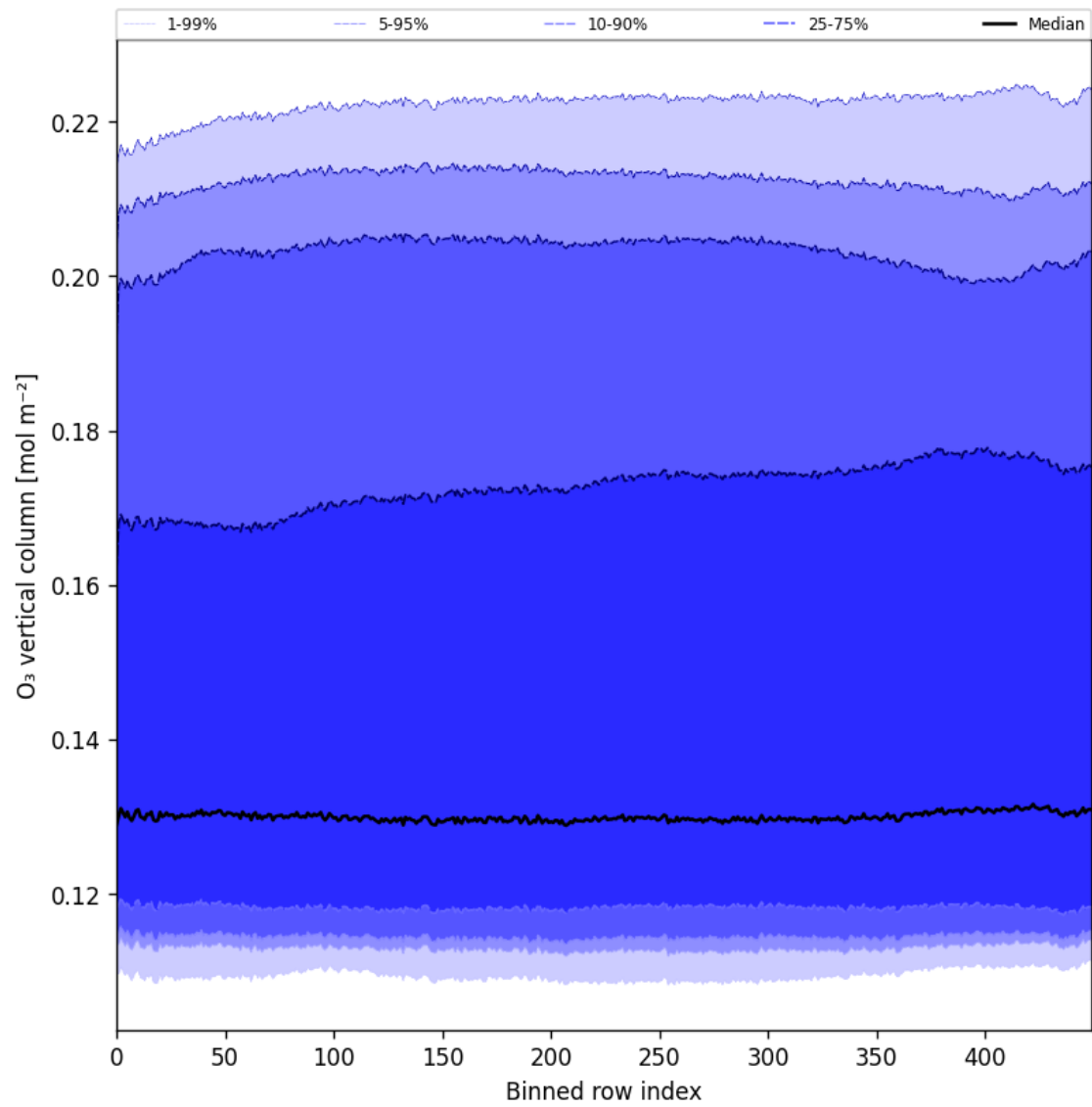
Figure 28: Along track statistics of “O 3 vertical column” for 2025-04-04 to 2025-04-06
