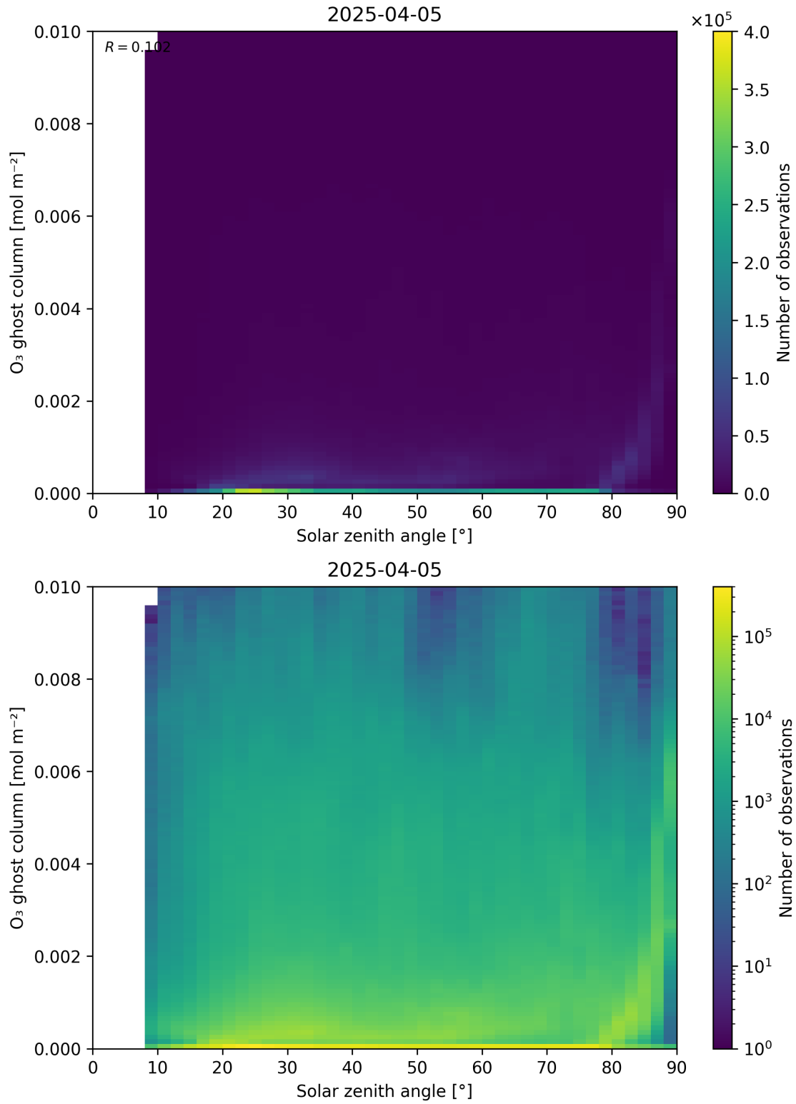
Figure 46: Scatter density plot of “Solar zenith angle” against “O 3 ghost column” for 2025-04-04 to 2025-04-06.
