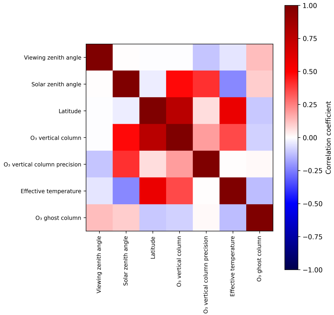
Figure 2: Map of correlation matrix for 2025-04-04 to 2025-04-06.
