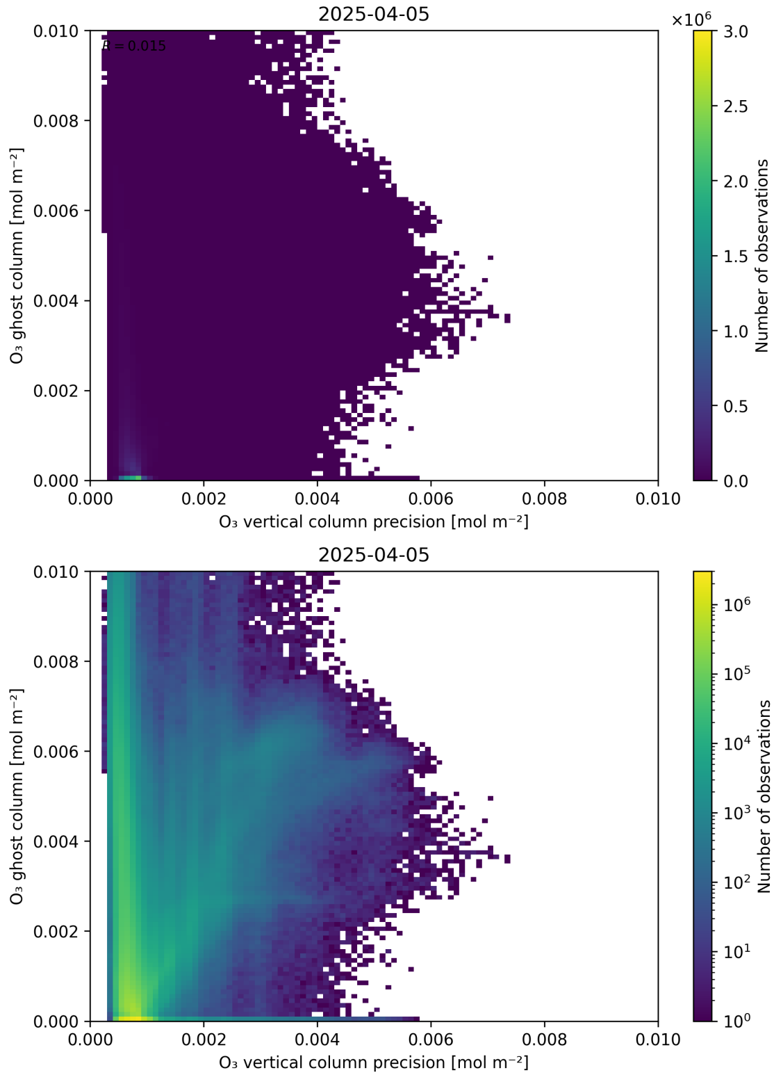
Figure 43: Scatter density plot of “O 3 vertical column precision” against “O 3 ghost column” for 2025-04-04 to 2025-04-06.
