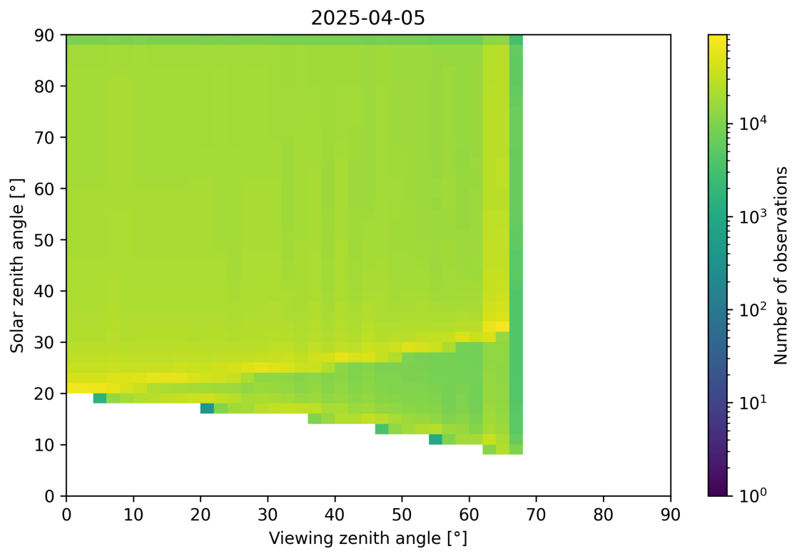
Figure 54: Scatter density plot of “Viewing zenith angle” against “Solar zenith angle” for 2025-04-04 to 2025-04-06.
