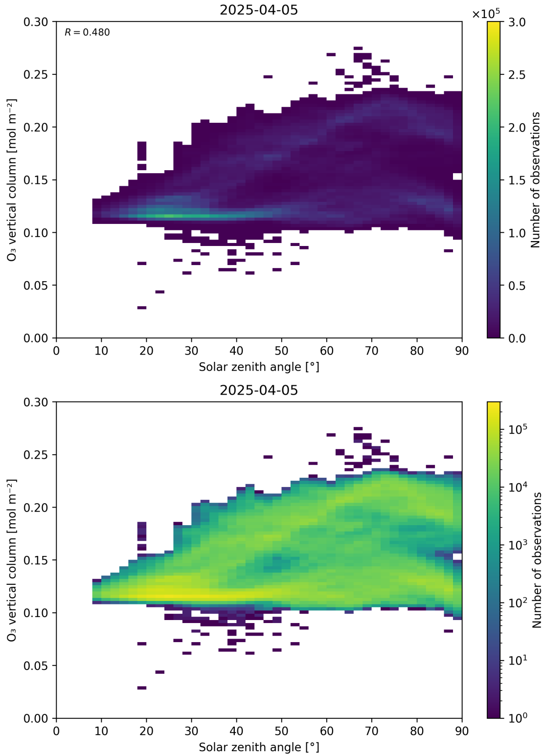
Figure 47: Scatter density plot of “Solar zenith angle” against “O 3 vertical column” for 2025-04-04 to 2025-04-06.
