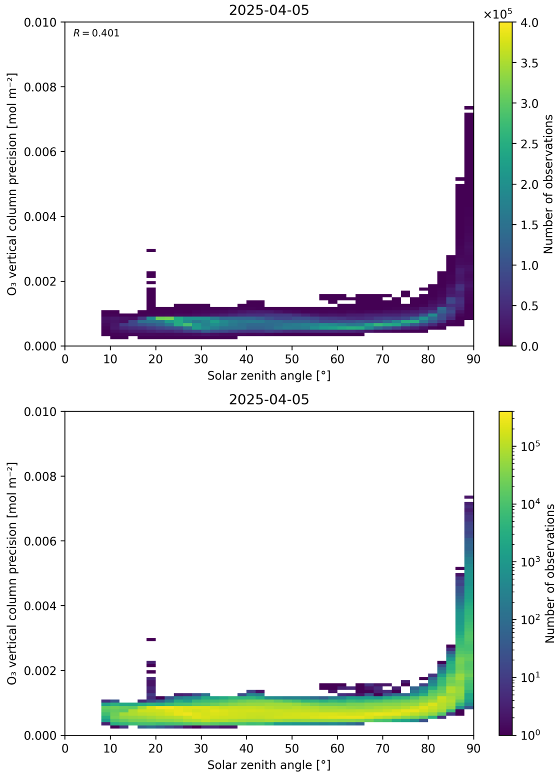
Figure 48: Scatter density plot of “Solar zenith angle” against “O 3 vertical column precision” for 2025-04-04 to 2025-04-06.
