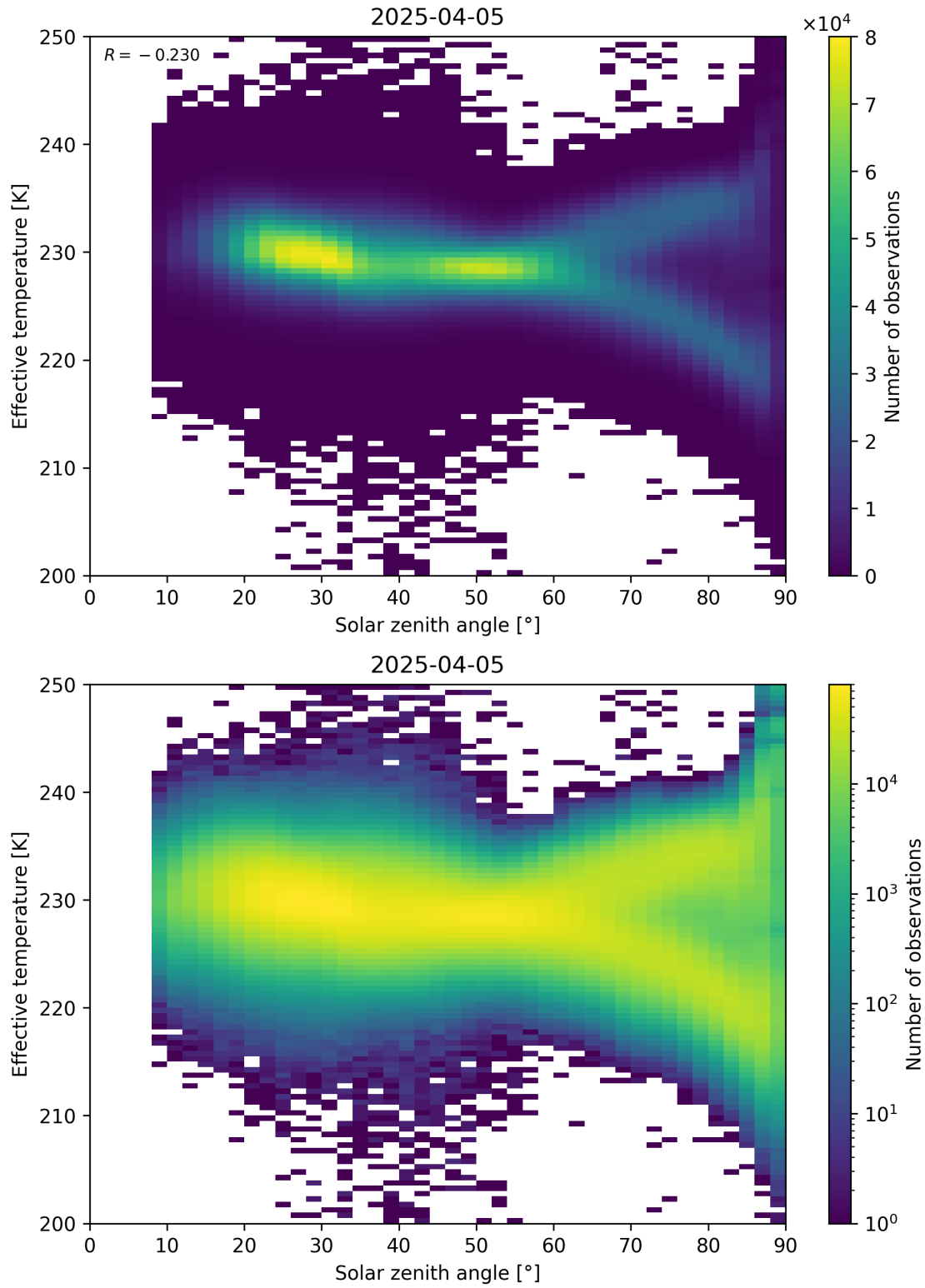
Figure 45: Scatter density plot of “Solar zenith angle” against “Effective temperature” for 2025-04-04 to 2025-04-06.
