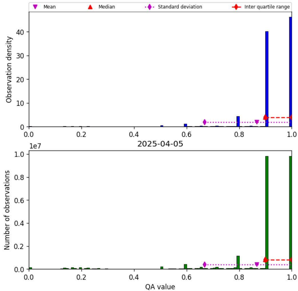
Figure 20: Histogram of “QA value” for 2025-04-04 to 2025-04-06
