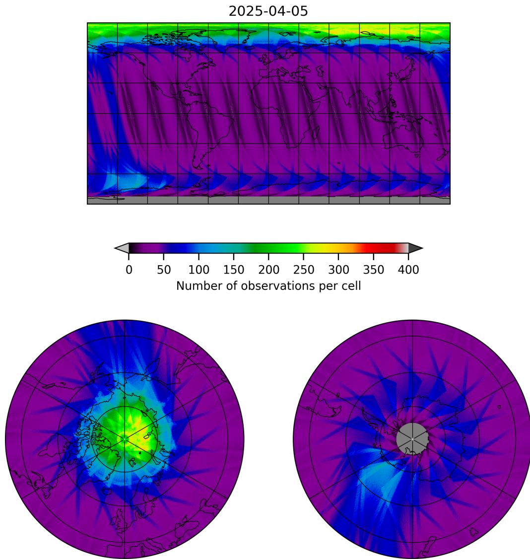
Figure 12: Map of the number of observations for 2025-04-04 to 2025-04-06
