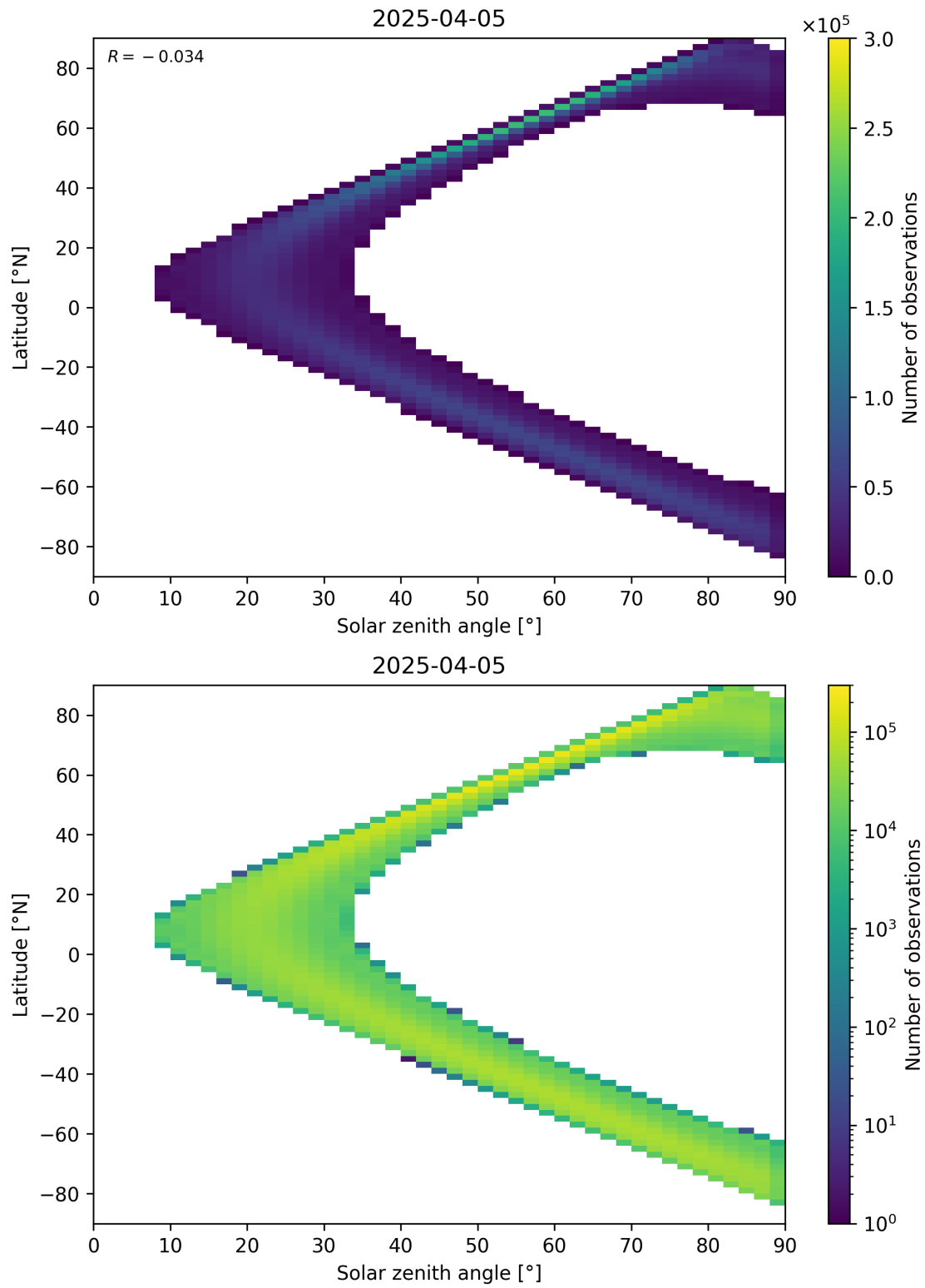
Figure 44: Scatter density plot of “Solar zenith angle” against “Latitude” for 2025-04-04 to 2025-04-06.
