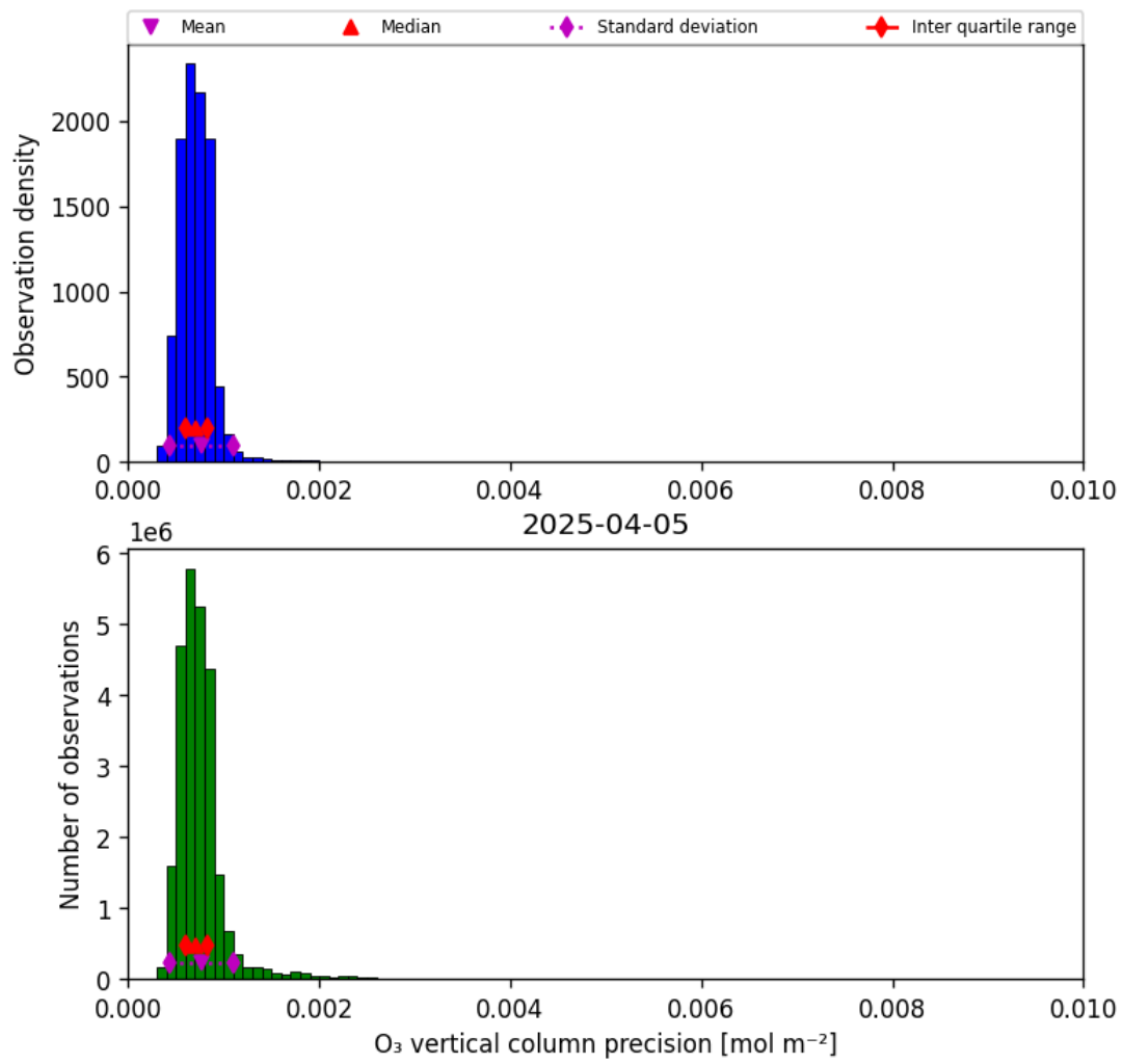
Figure 22: Histogram of “O 3 vertical column precision” for 2025-04-04 to 2025-04-06
