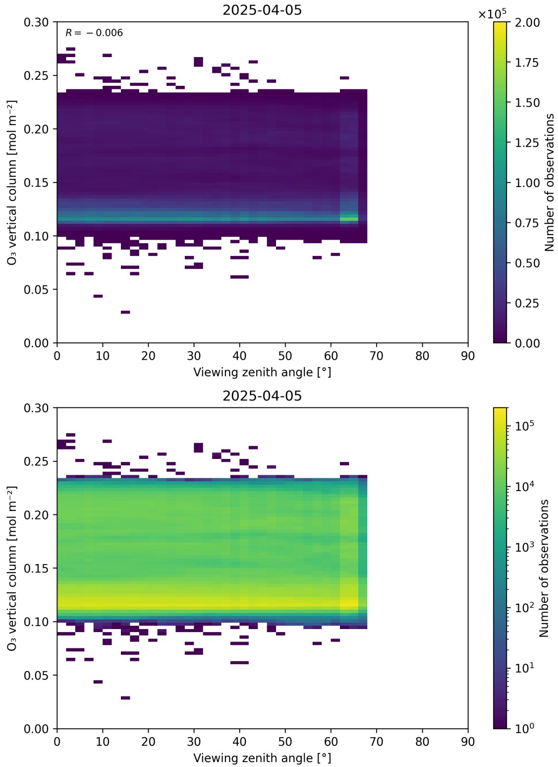
Figure 52: Scatter density plot of “Viewing zenith angle” against “O 3 vertical column” for 2025-04-04 to 2025-04-06.
