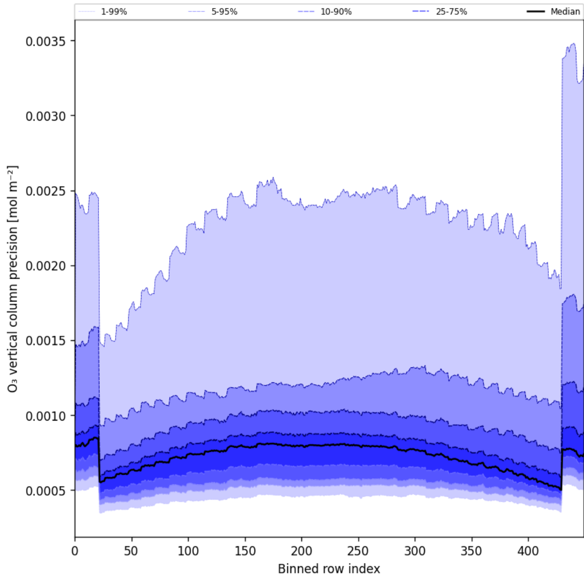
Figure 29: Along track statistics of “O 3 vertical column precision” for 2025-04-04 to 2025-04-06
