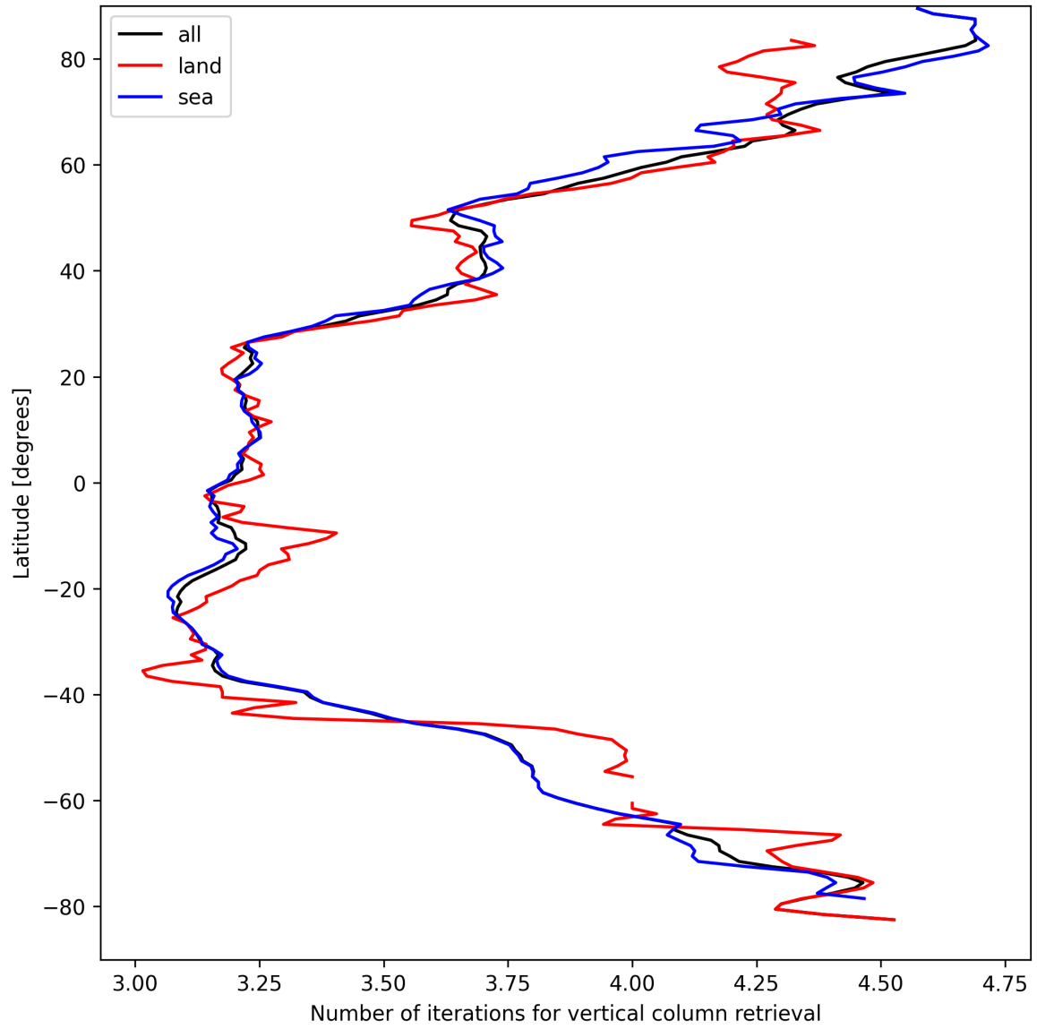
Figure 19: Zonal average of “Number of iterations for vertical column retrieval” for 2025-04-04 to 2025-04-06.
