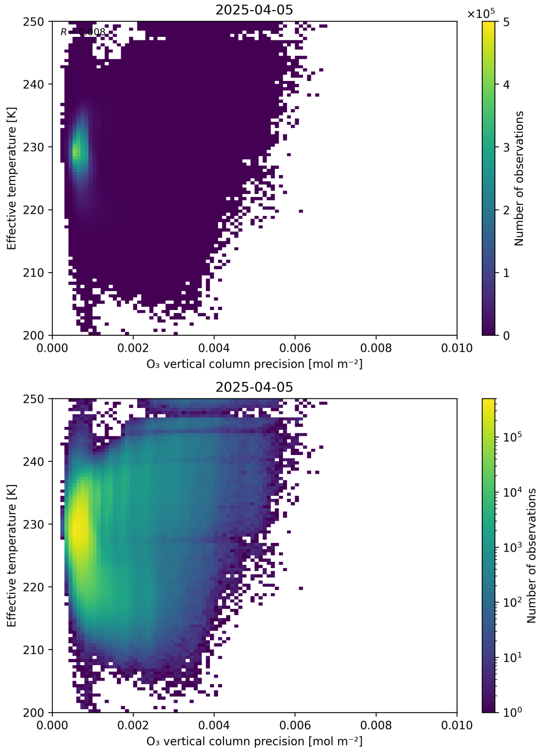
Figure 42: Scatter density plot of “ O_3 vertical column precision” against “Effective temperature” for 2025-04-04 to 2025-04-06.
