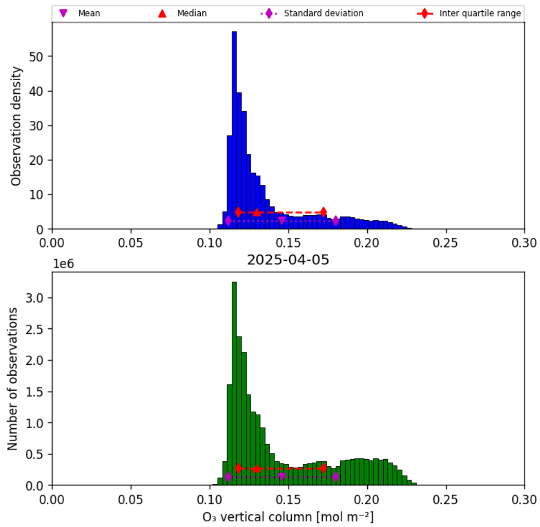
Figure 21: Histogram of “O 3 vertical column” for 2025-04-04 to 2025-04-06
