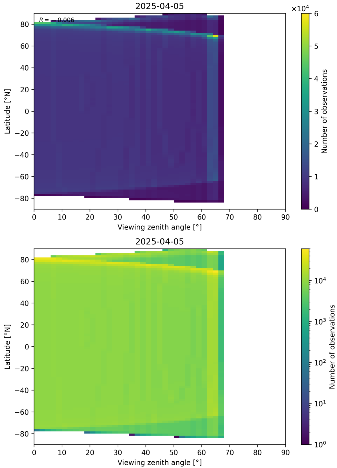
Figure 49: Scatter density plot of “Viewing zenith angle” against “Latitude” for 2025-04-04 to 2025-04-06.
