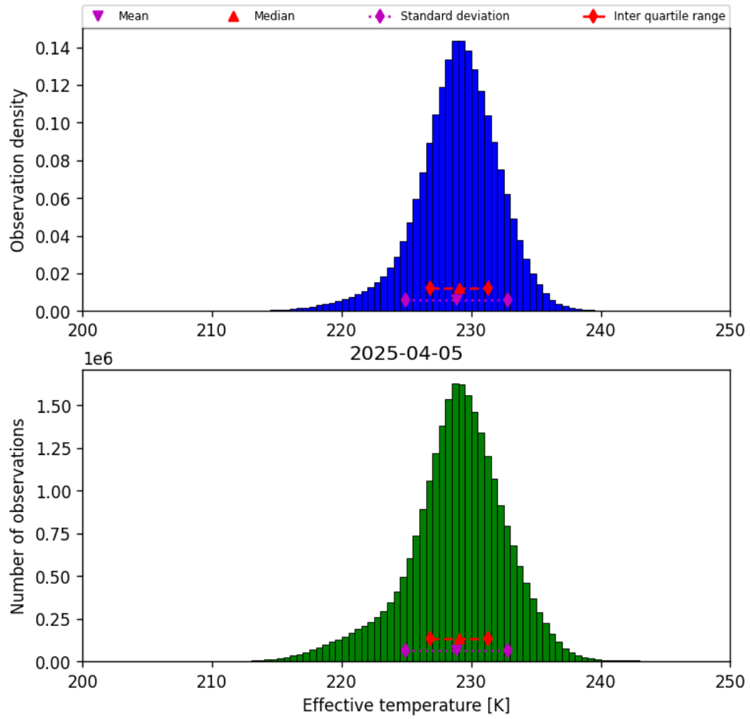
Figure 24: Histogram of “Effective temperature” for 2025-04-04 to 2025-04-06
