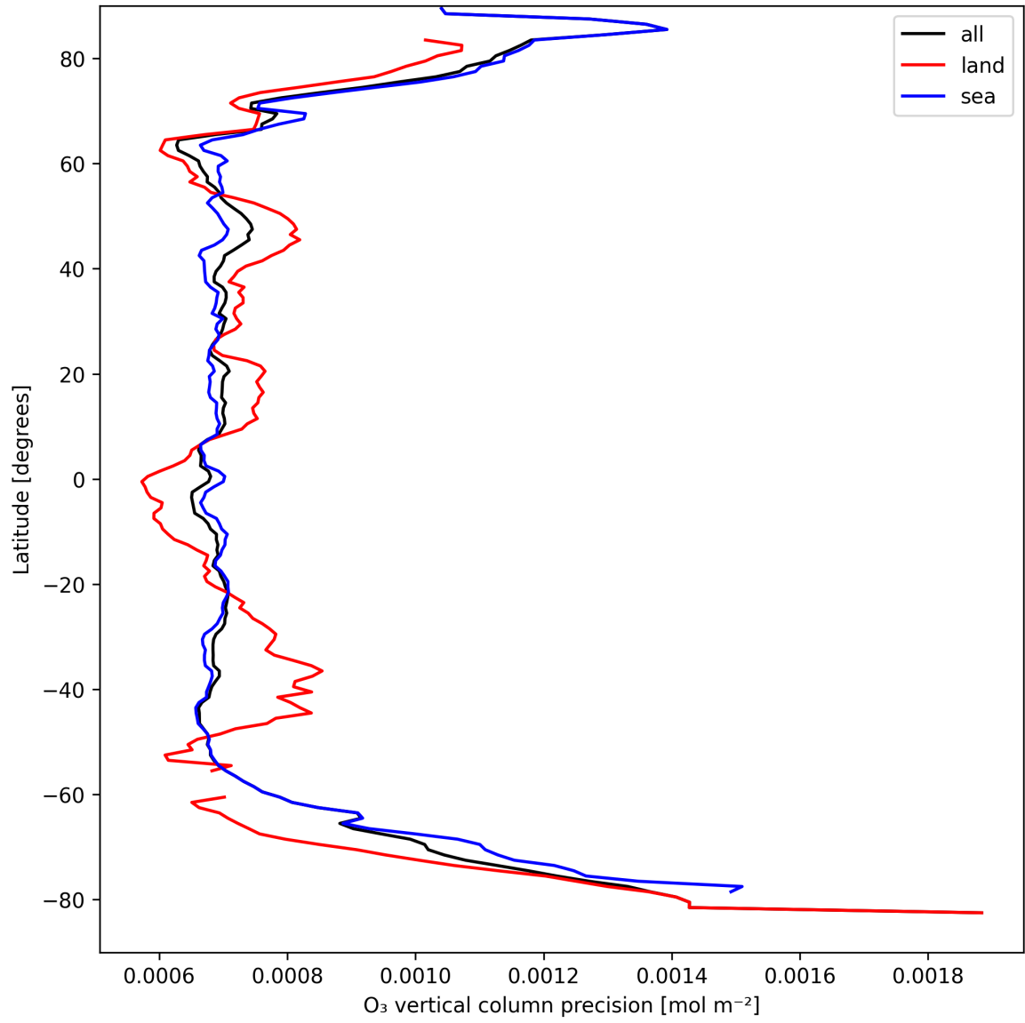
Figure 15: Zonal average of “O 3 vertical column precision” for 2025-04-04 to 2025-04-06.
