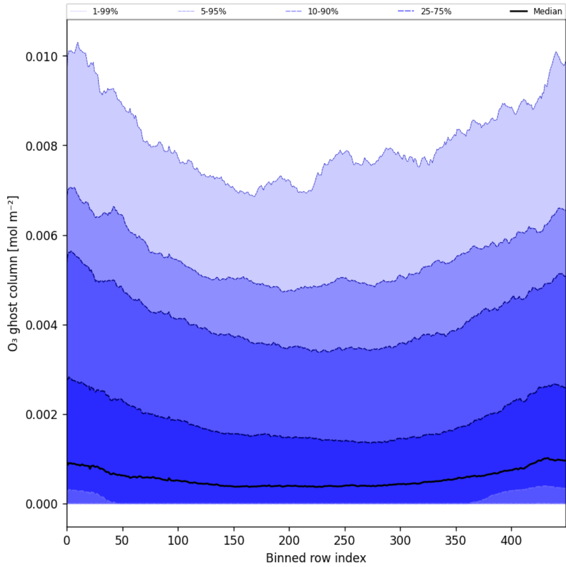
Figure 32: Along track statistics of “O 3 ghost column” for 2025-04-04 to 2025-04-06
