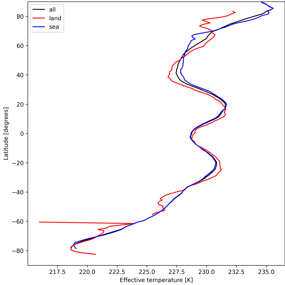
Figure 17: Zonal average of “Effective temperature” for 2025-04-04 to 2025-04-06.
