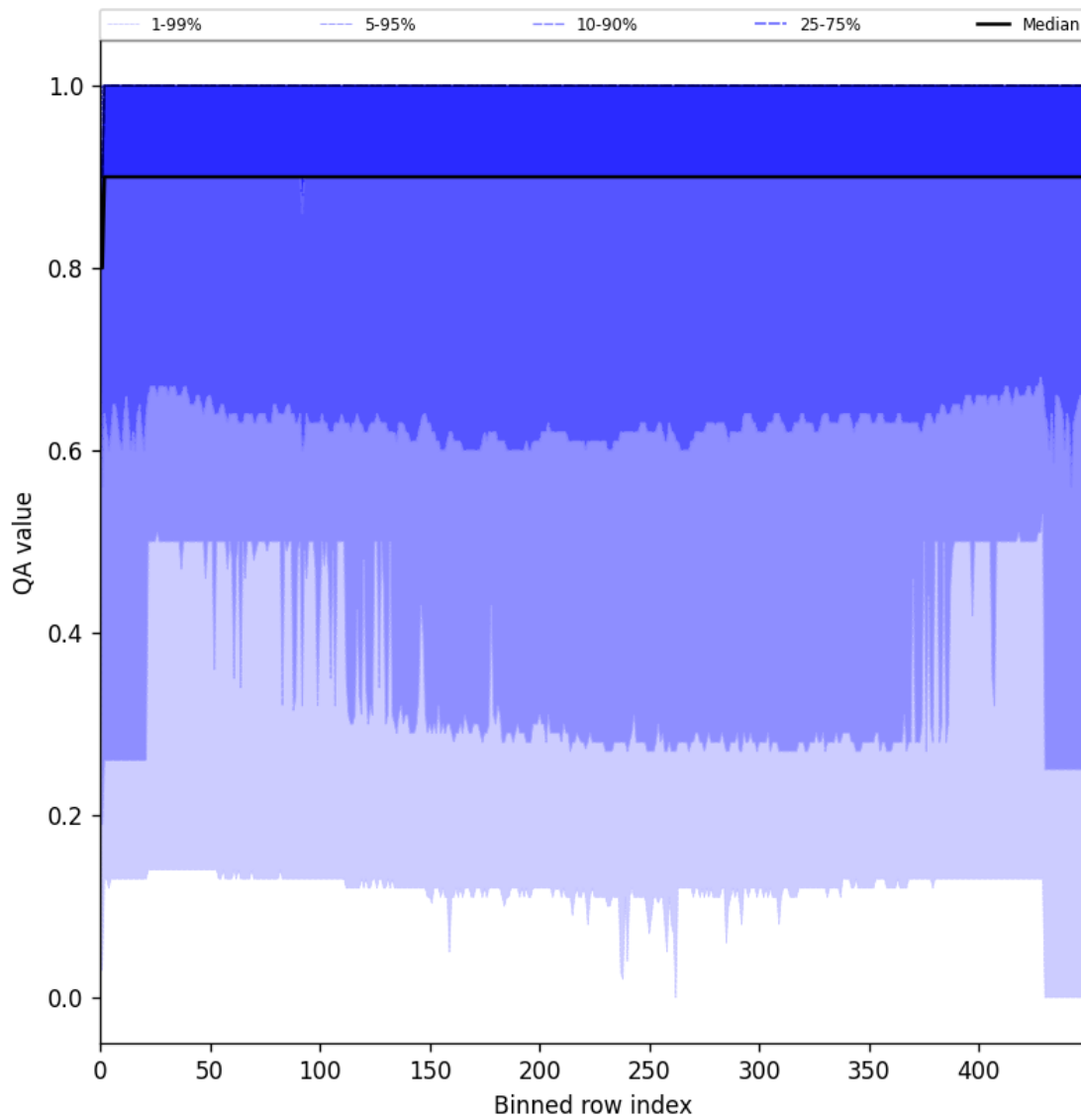
Figure 27: Along track statistics of “QA value” for 2025-04-04 to 2025-04-06
