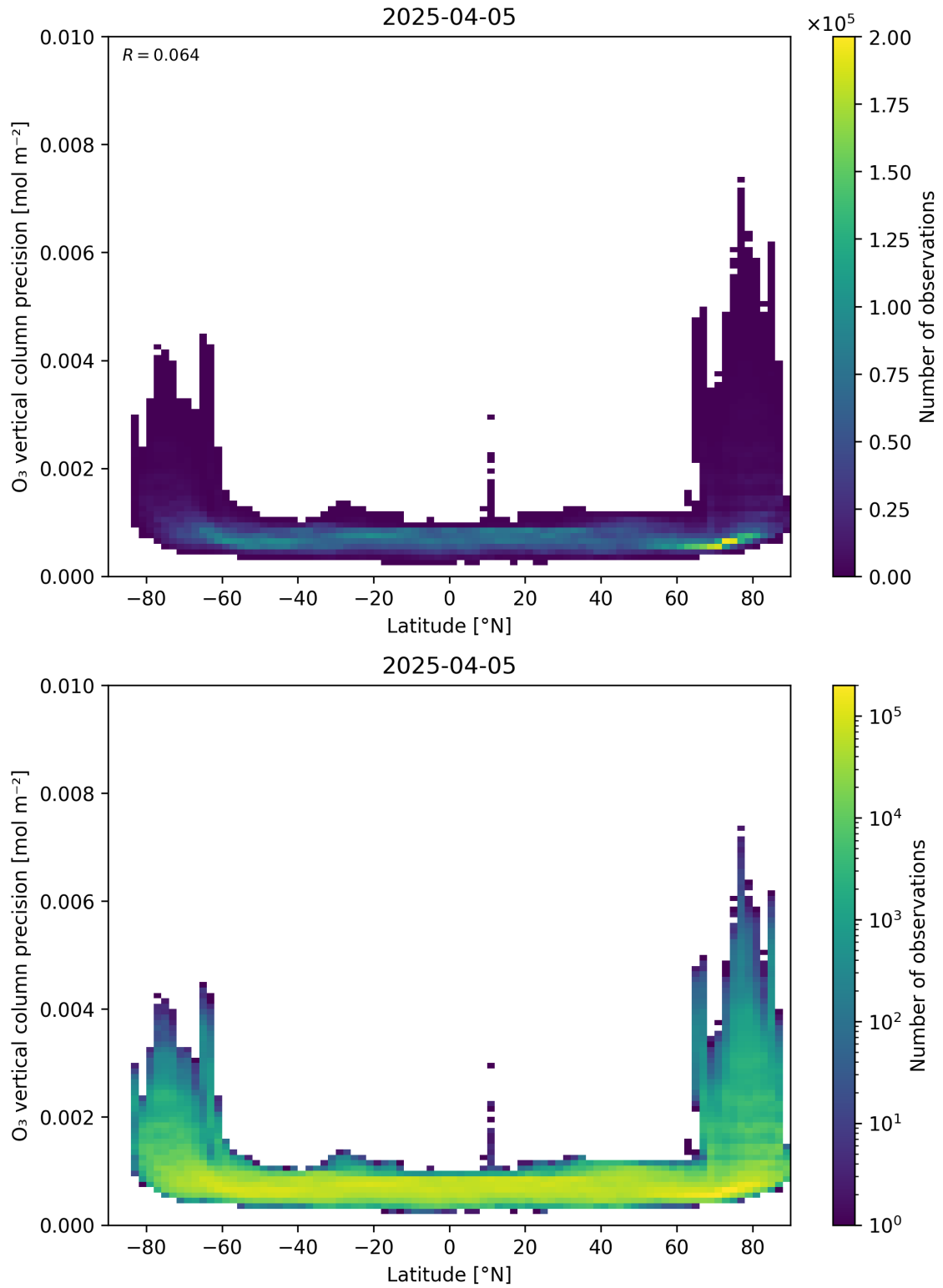
Figure 37: Scatter density plot of “Latitude” against “O 3 vertical column precision” for 2025-04-04 to 2025-04-06.
