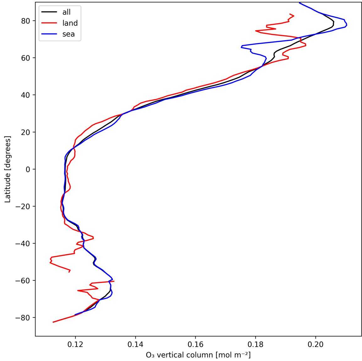
Figure 14: Zonal average of “O 3 vertical column” for 2025-04-04 to 2025-04-06.
