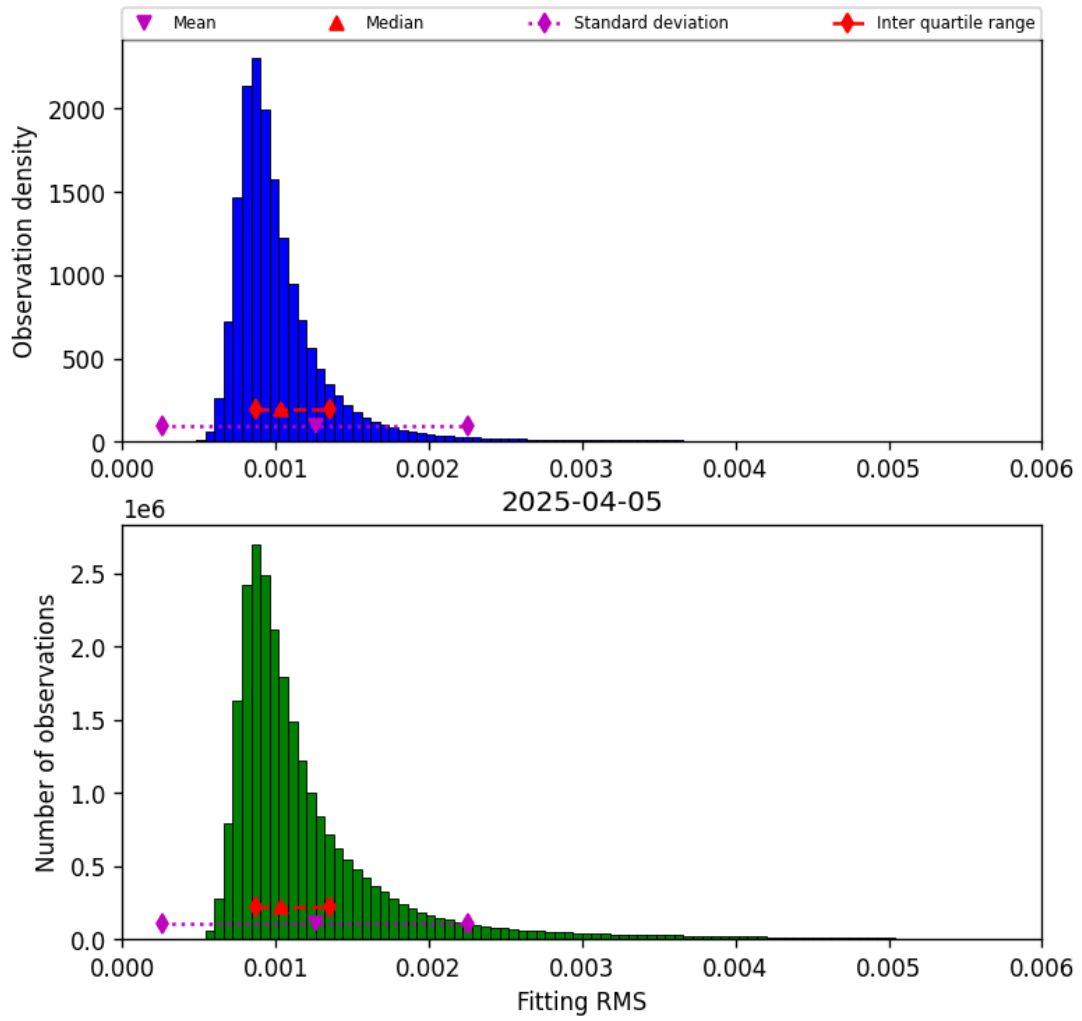
Figure 23: Histogram of “Fitting RMS” for 2025-04-04 to 2025-04-06
