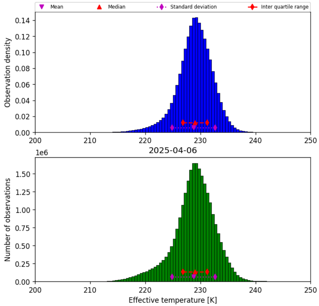
Figure 24: Histogram of “Effective temperature” for 2025-04-05 to 2025-04-07
