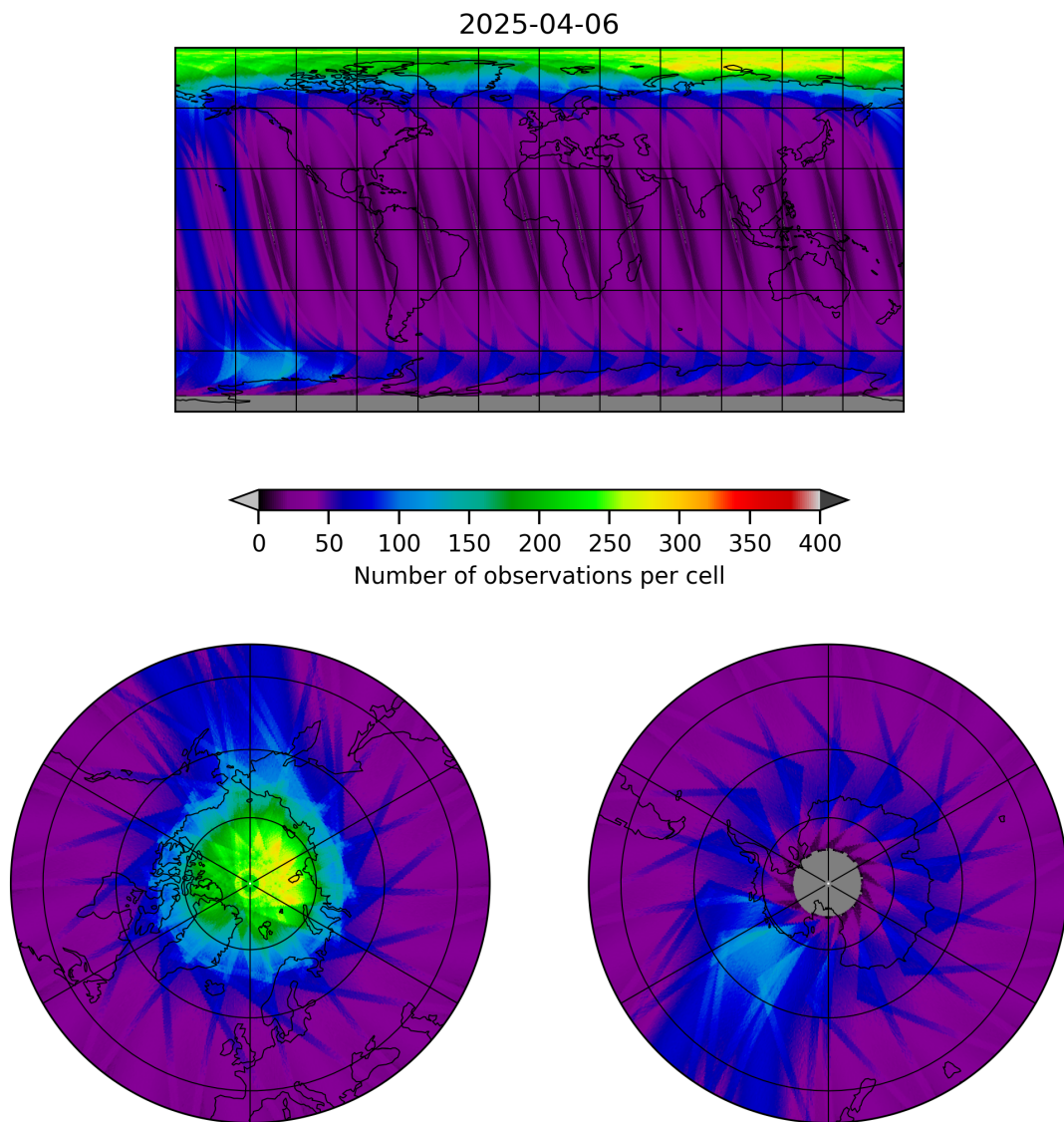
Figure 12: Map of the number of observations for 2025-04-05 to 2025-04-07
