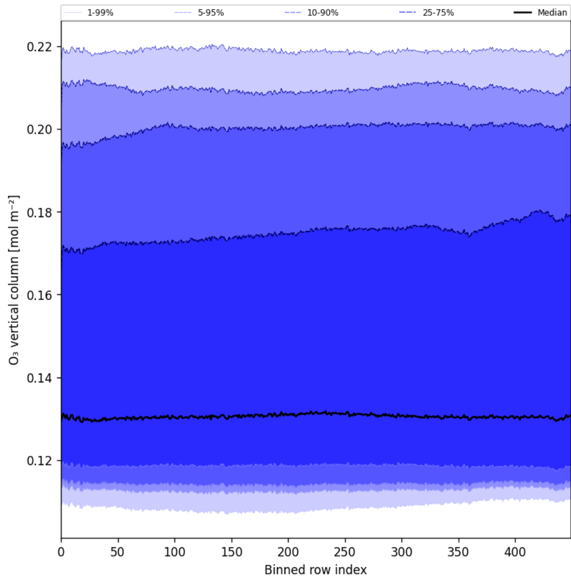
Figure 28: Along track statistics of “O 3 vertical column” for 2025-04-05 to 2025-04-07
