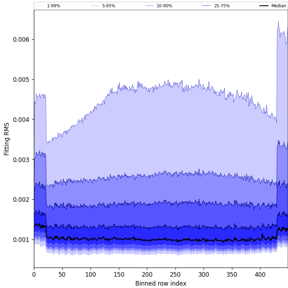
Figure 30: Along track statistics of “Fitting RMS” for 2025-04-05 to 2025-04-07
