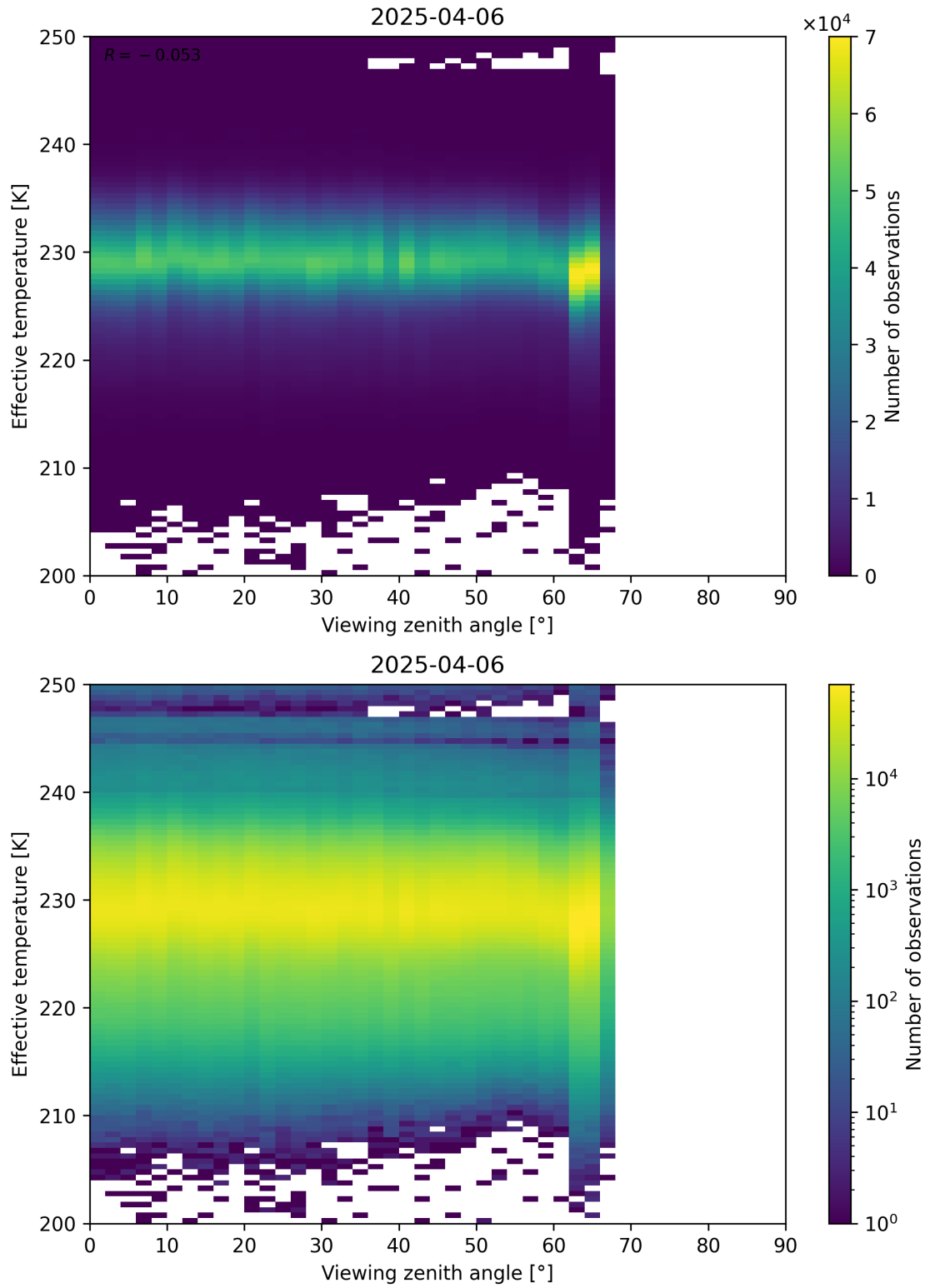
Figure 50: Scatter density plot of “Viewing zenith angle” against “Effective temperature” for 2025-04-05 to 2025-04-07.
