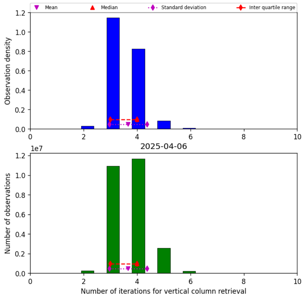
Figure 26: Histogram of “Number of iterations for vertical column retrieval” for 2025-04-05 to 2025-04-07
