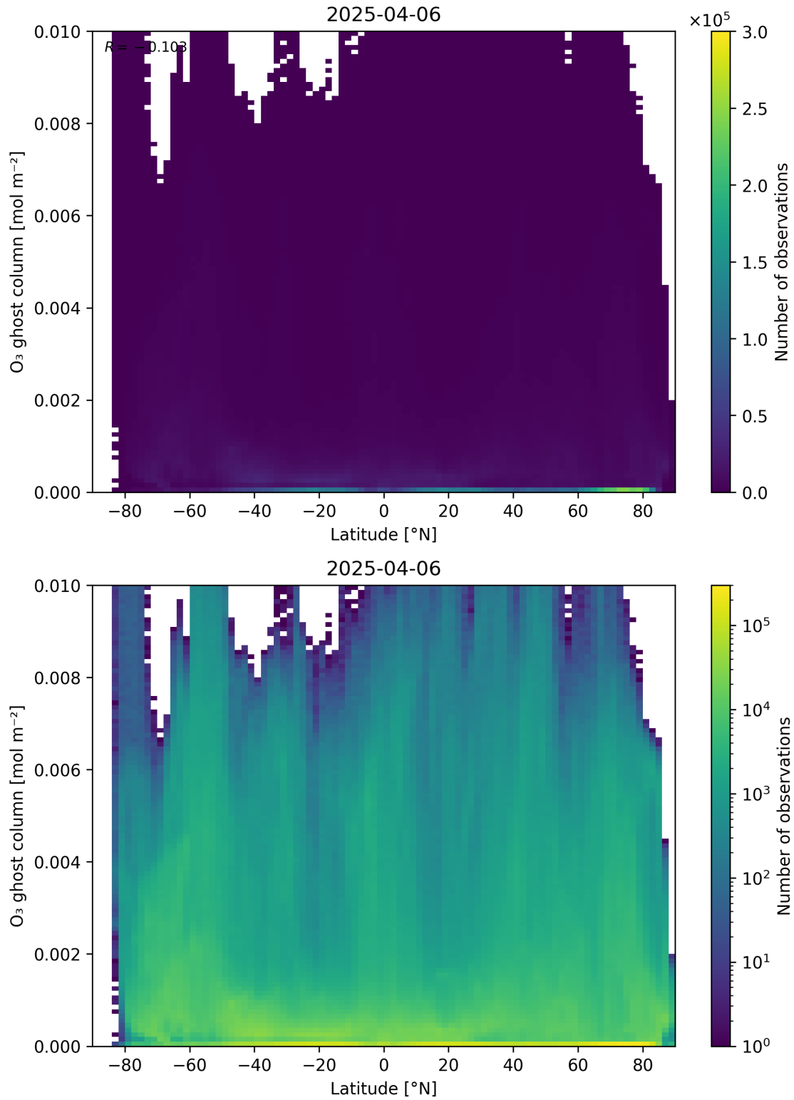
Figure 35: Scatter density plot of “Latitude” against “O 3 ghost column” for 2025-04-05 to 2025-04-07.
