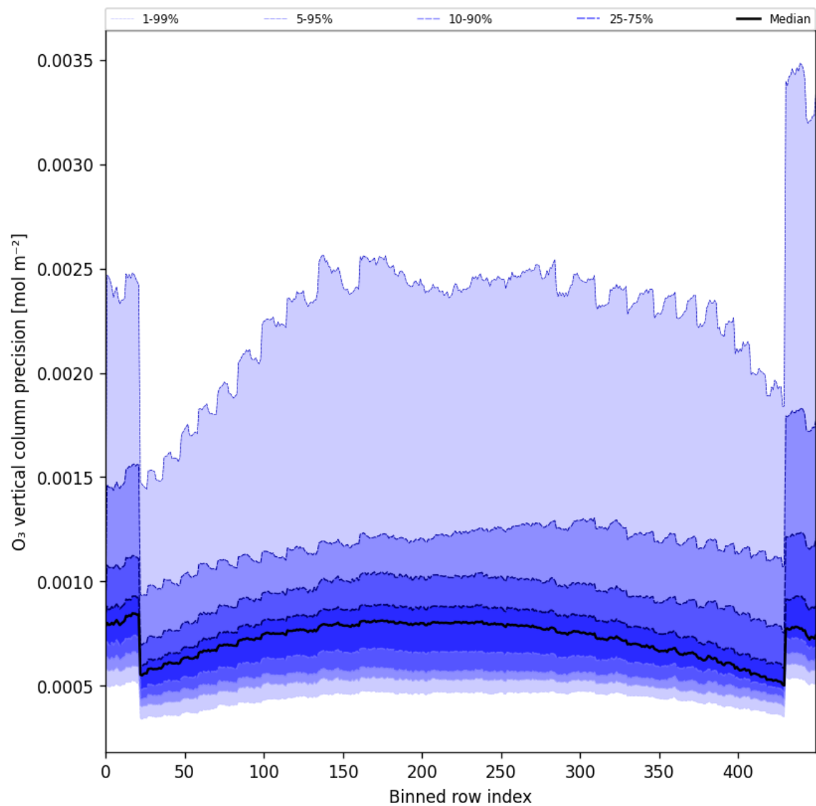
Figure 29: Along track statistics of “O 3 vertical column precision” for 2025-04-05 to 2025-04-07
