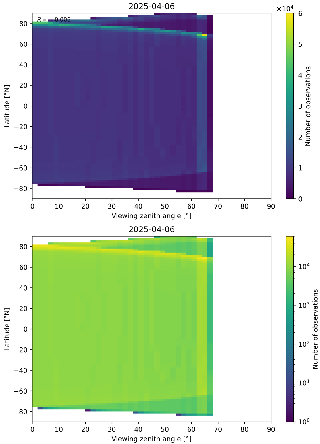
Figure 49: Scatter density plot of “Viewing zenith angle” against “Latitude” for 2025-04-05 to 2025-04-07.
