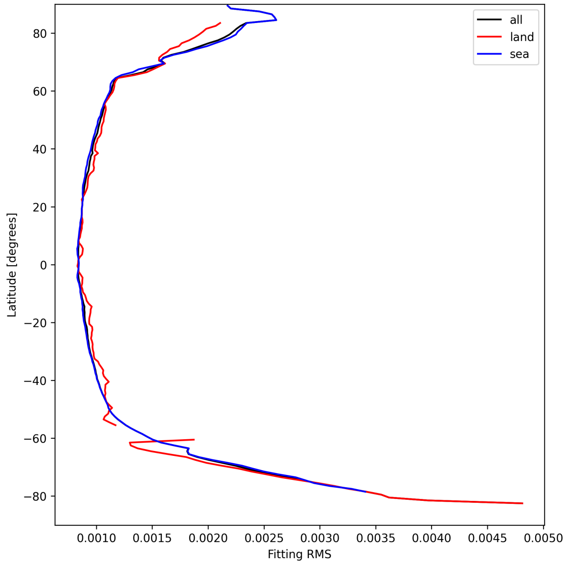
Figure 16: Zonal average of “Fitting RMS” for 2025-04-05 to 2025-04-07.
