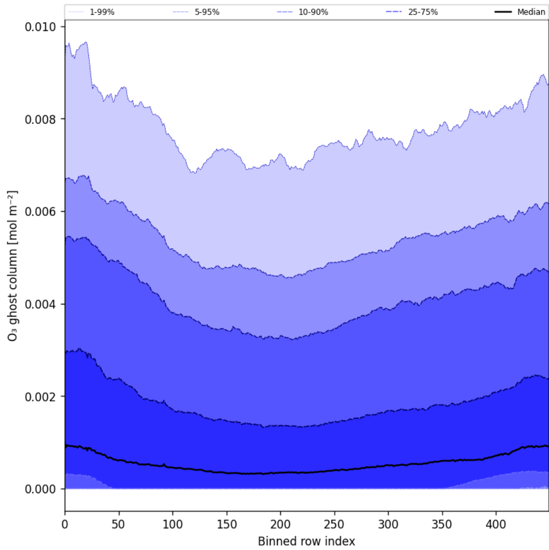
Figure 32: Along track statistics of “O 3 ghost column” for 2025-04-05 to 2025-04-07
