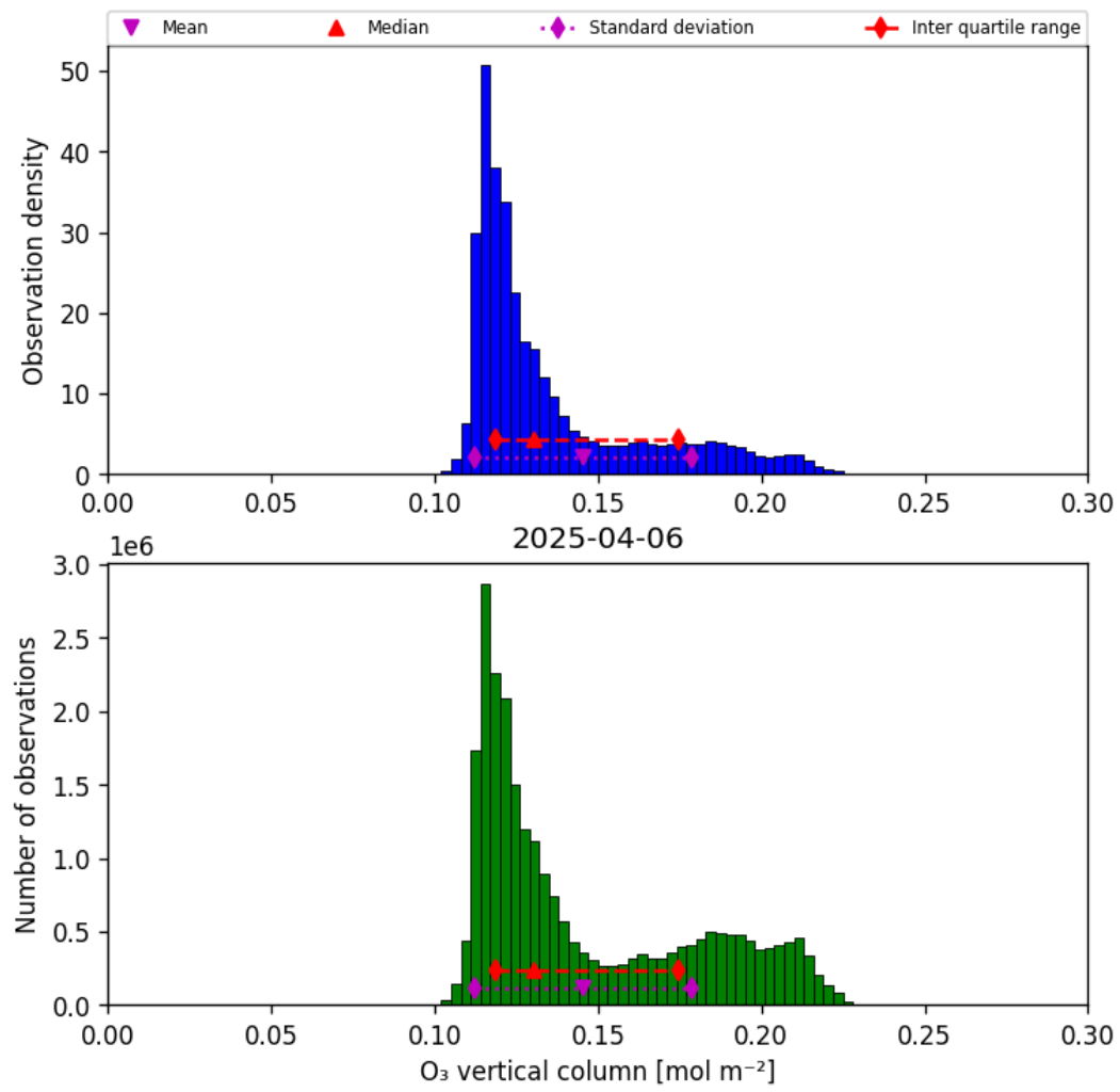
Figure 21: Histogram of “O 3 vertical column” for 2025-04-05 to 2025-04-07
