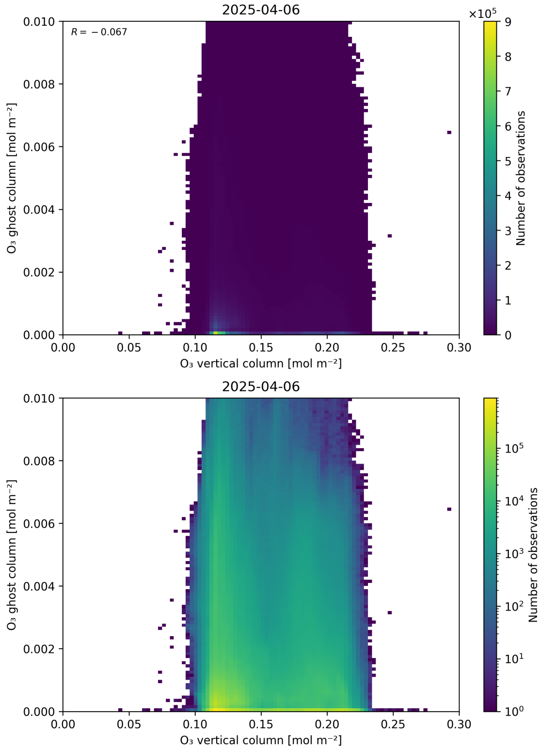
Figure 40: Scatter density plot of “O 3 vertical column” against “O 3 ghost column” for 2025-04-05 to 2025-04-07.
