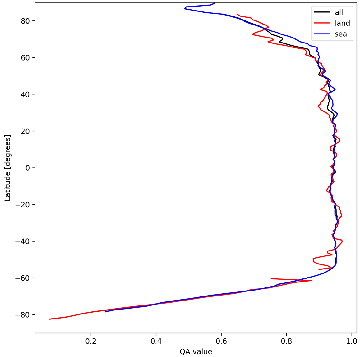
Figure 13: Zonal average of “QA value” for 2025-04-05 to 2025-04-07.
