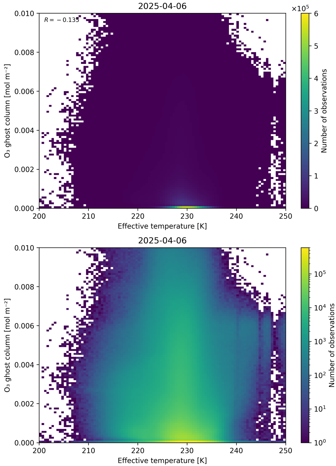
Figure 38: Scatter density plot of “Effective temperature” against “O 3 ghost column” for 2025-04-05 to 2025-04-07.
