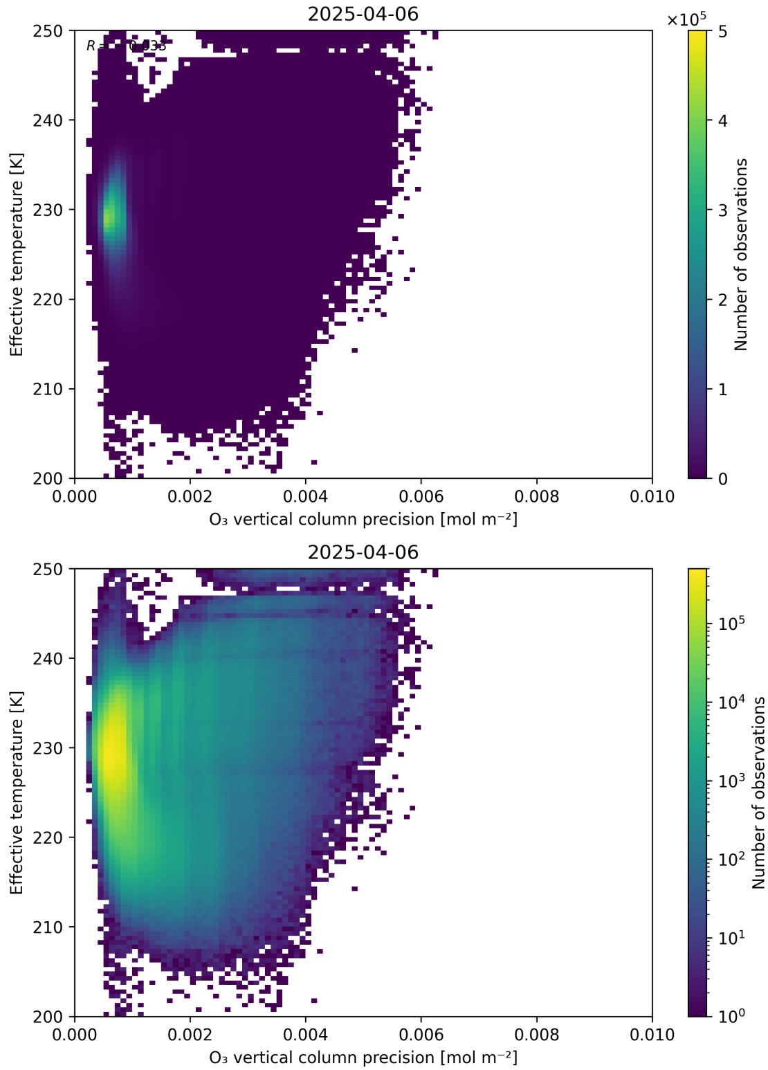
Figure 42: Scatter density plot of “O 3 vertical column precision” against “Effective temperature” for 2025-04-05 to 2025-04-07.
