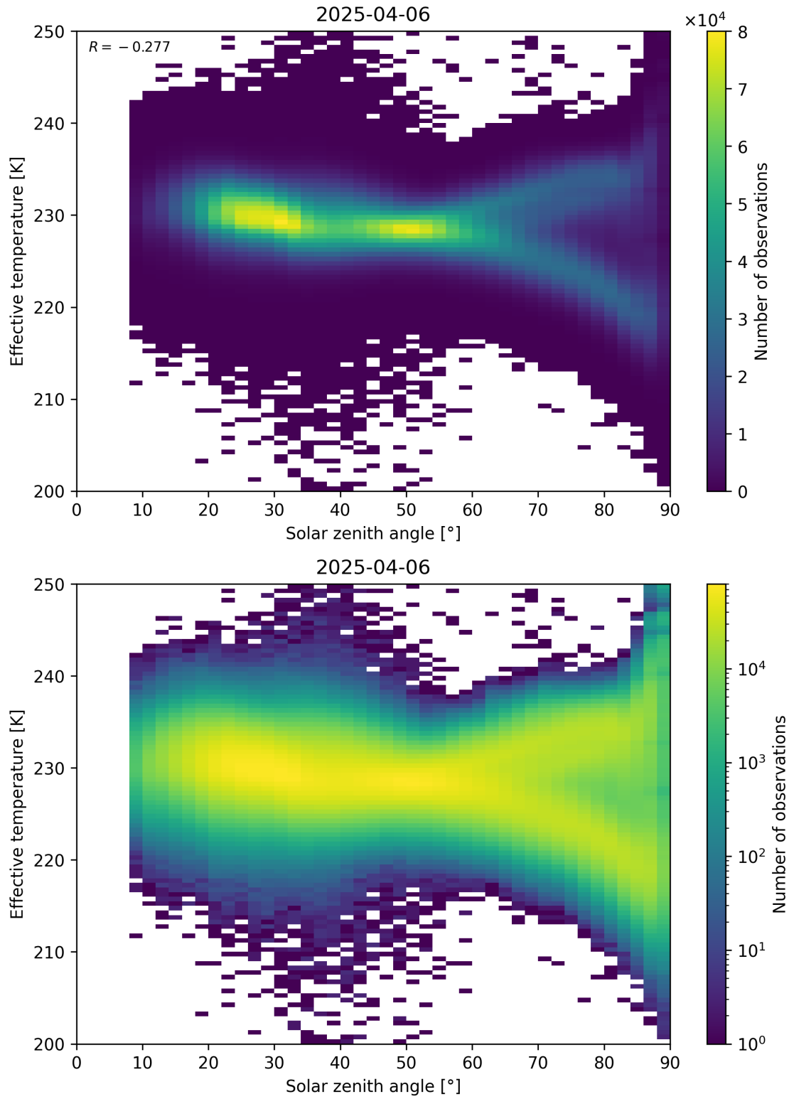
Figure 45: Scatter density plot of “Solar zenith angle” against “Effective temperature” for 2025-04-05 to 2025-04-07.
