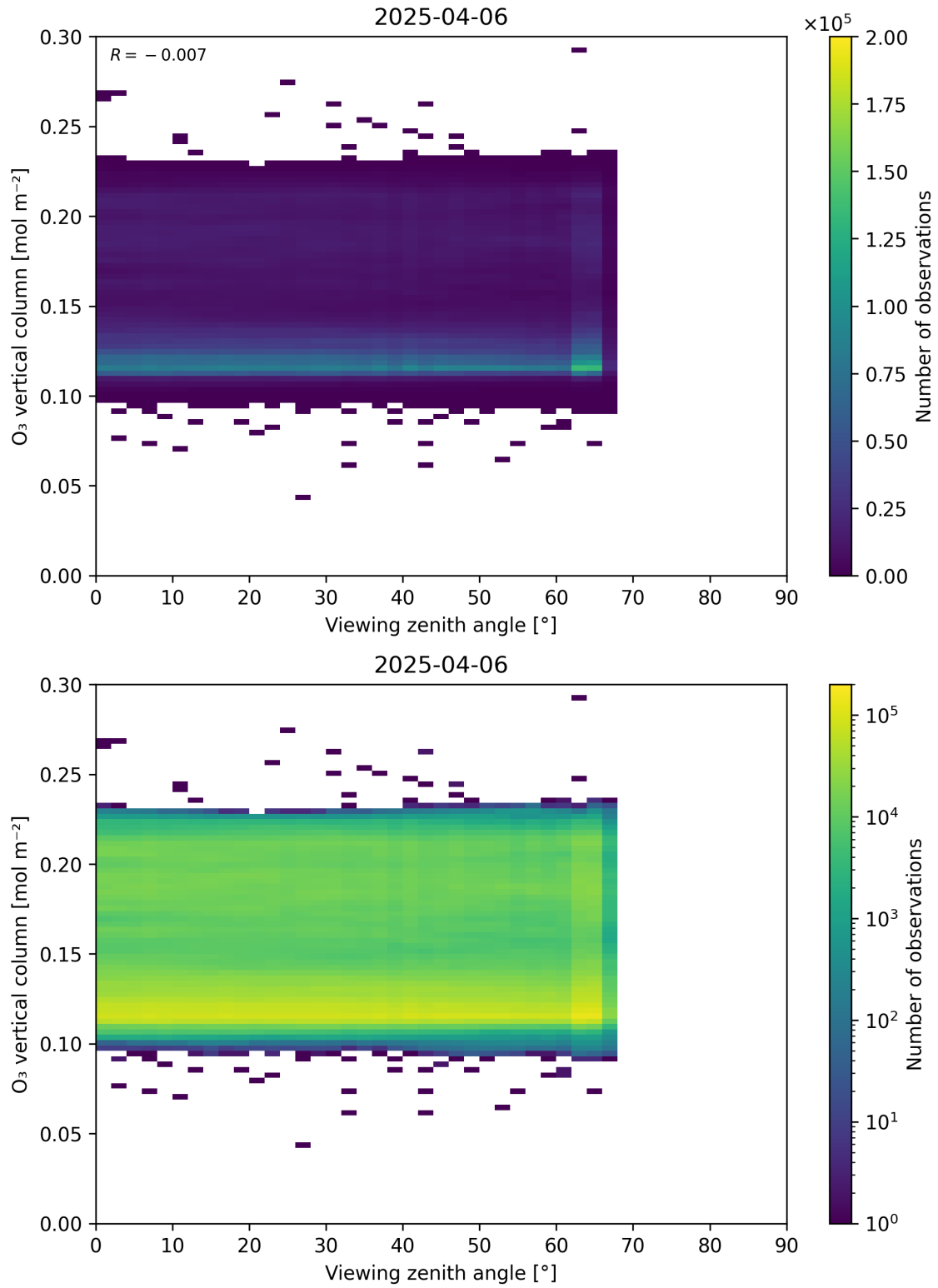
Figure 52: Scatter density plot of “Viewing zenith angle” against “O 3 vertical column” for 2025-04-05 to 2025-04-07.
