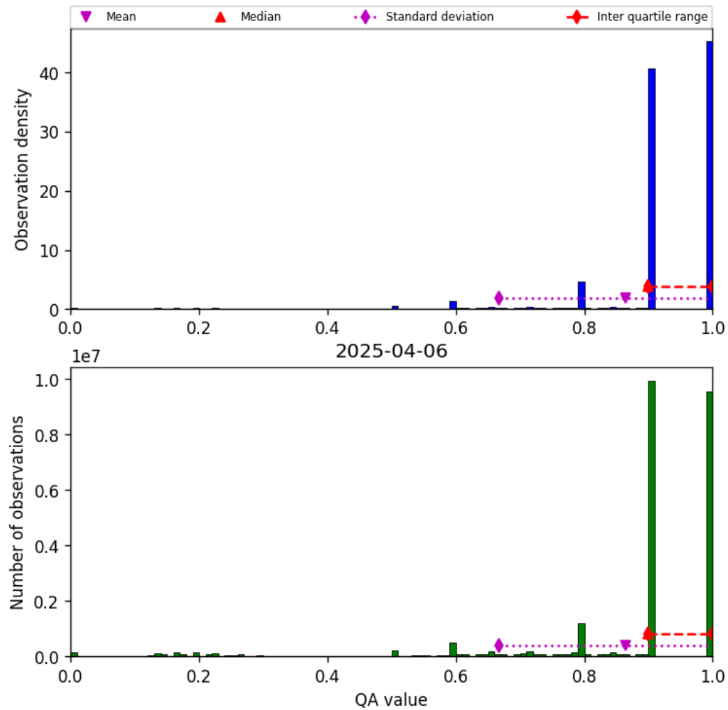
Figure 20: Histogram of “QA value” for 2025-04-05 to 2025-04-07
