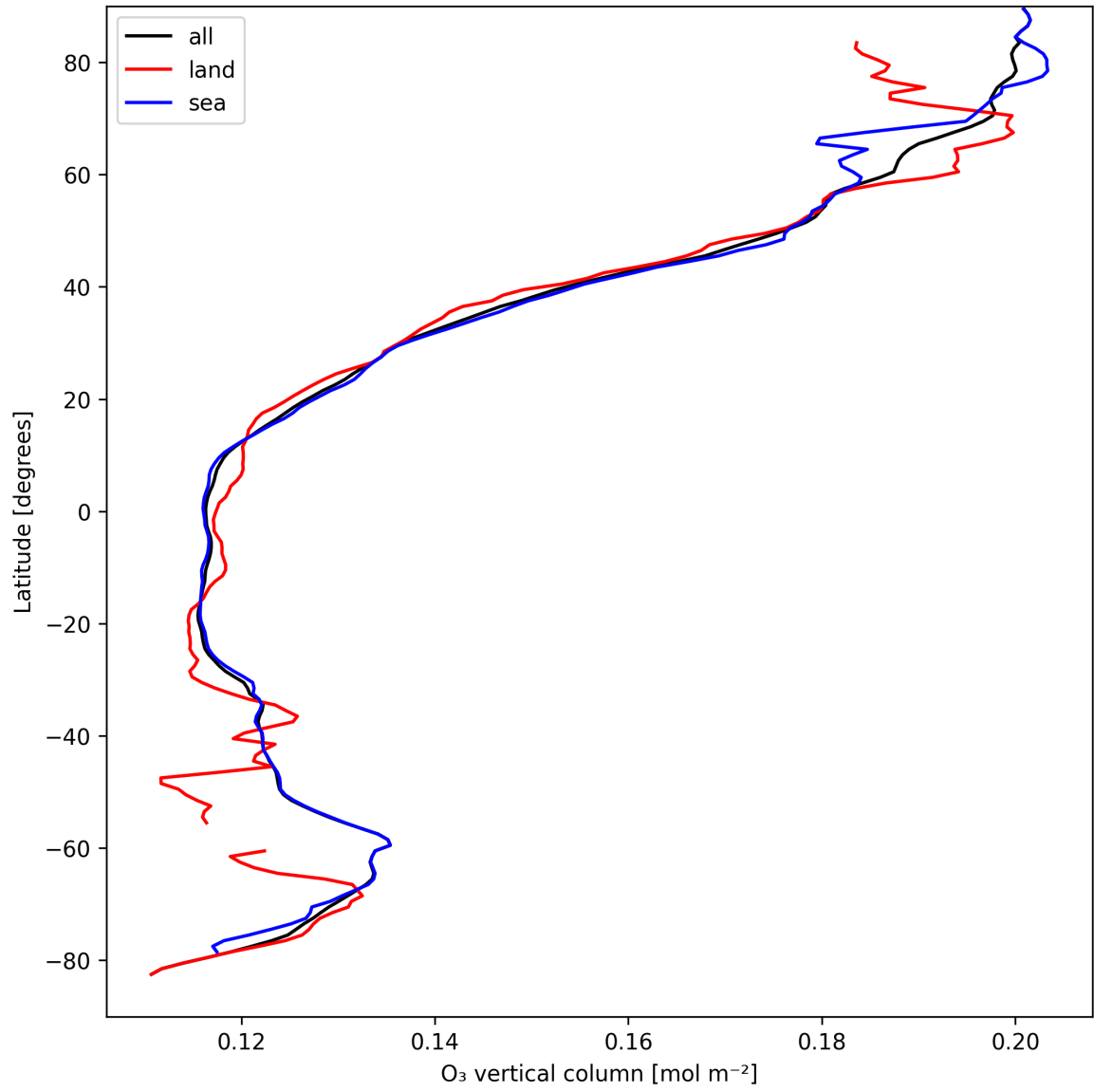
Figure 14: Zonal average of “O 3 vertical column” for 2025-04-05 to 2025-04-07.
