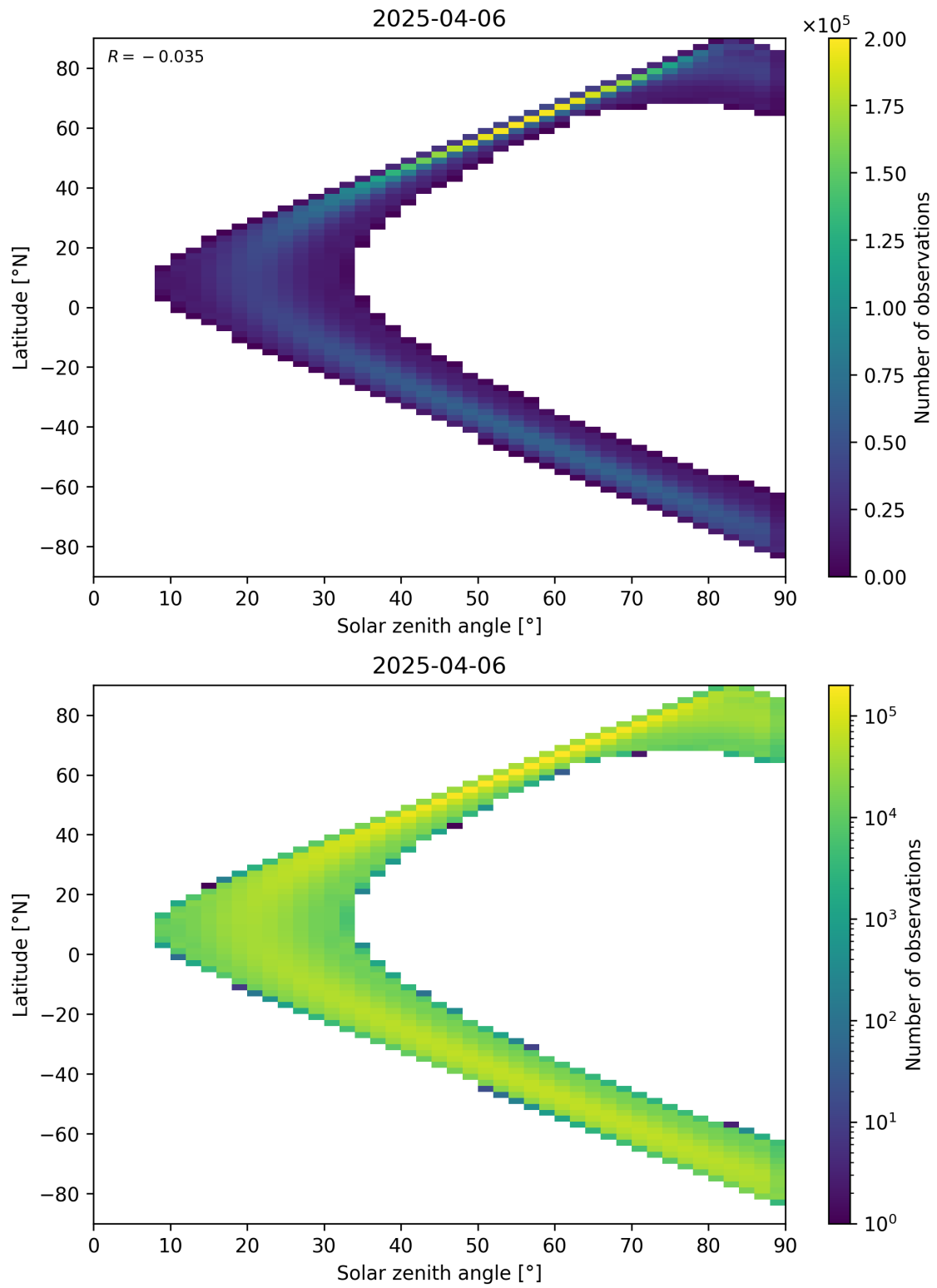
Figure 44: Scatter density plot of “Solar zenith angle” against “Latitude” for 2025-04-05 to 2025-04-07.
