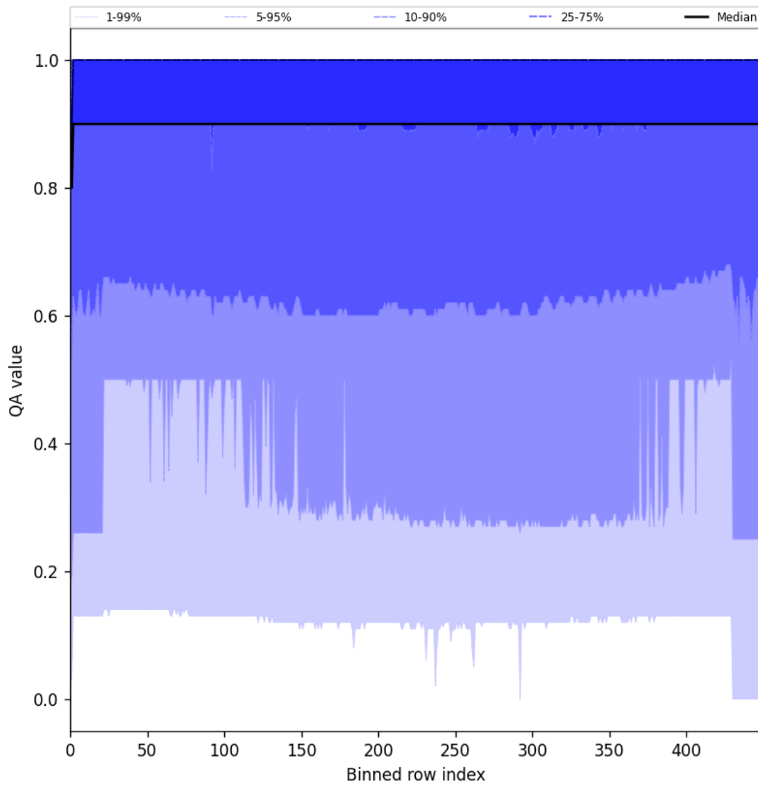
Figure 27: Along track statistics of “QA value” for 2025-04-05 to 2025-04-07
