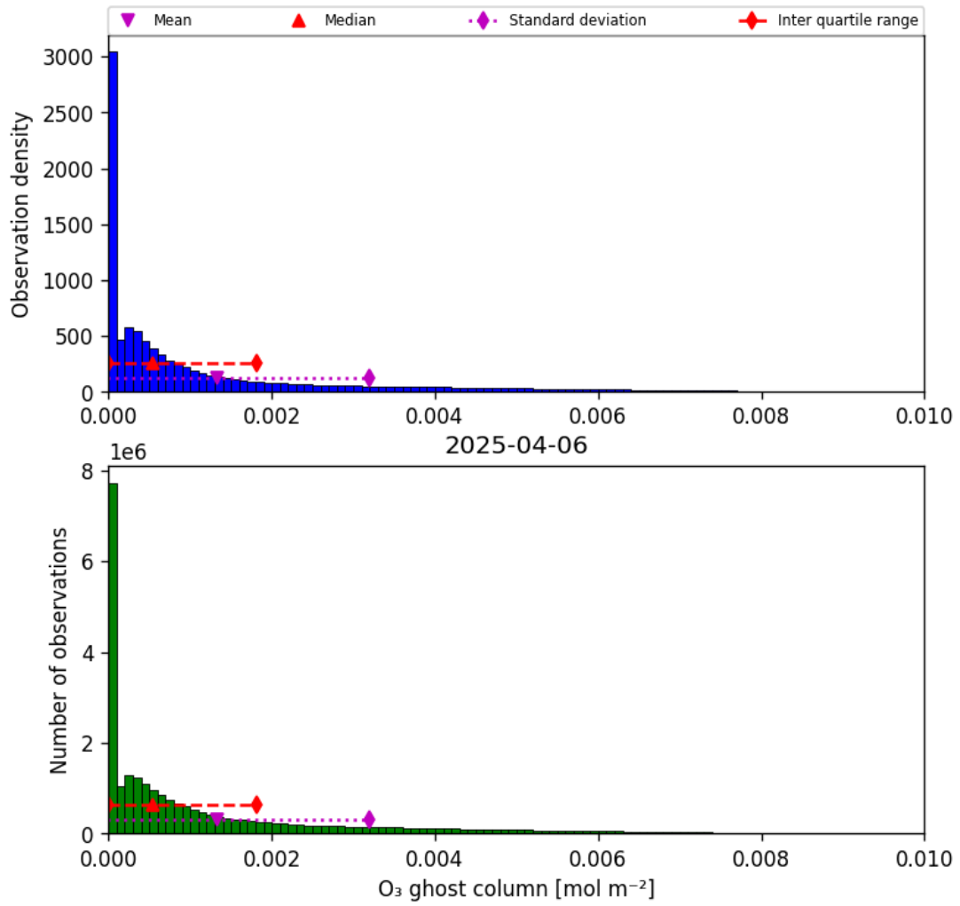
Figure 25: Histogram of “O 3 ghost column” for 2025-04-05 to 2025-04-07
