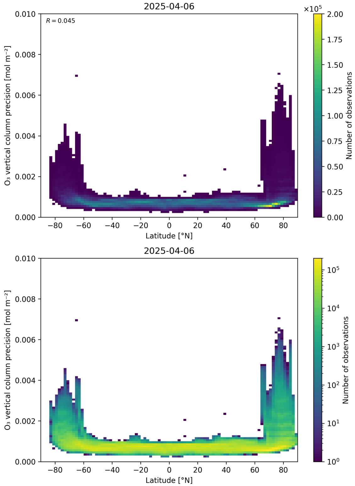
Figure 37: Scatter density plot of “Latitude” against “O 3 vertical column precision” for 2025-04-05 to 2025-04-07.
