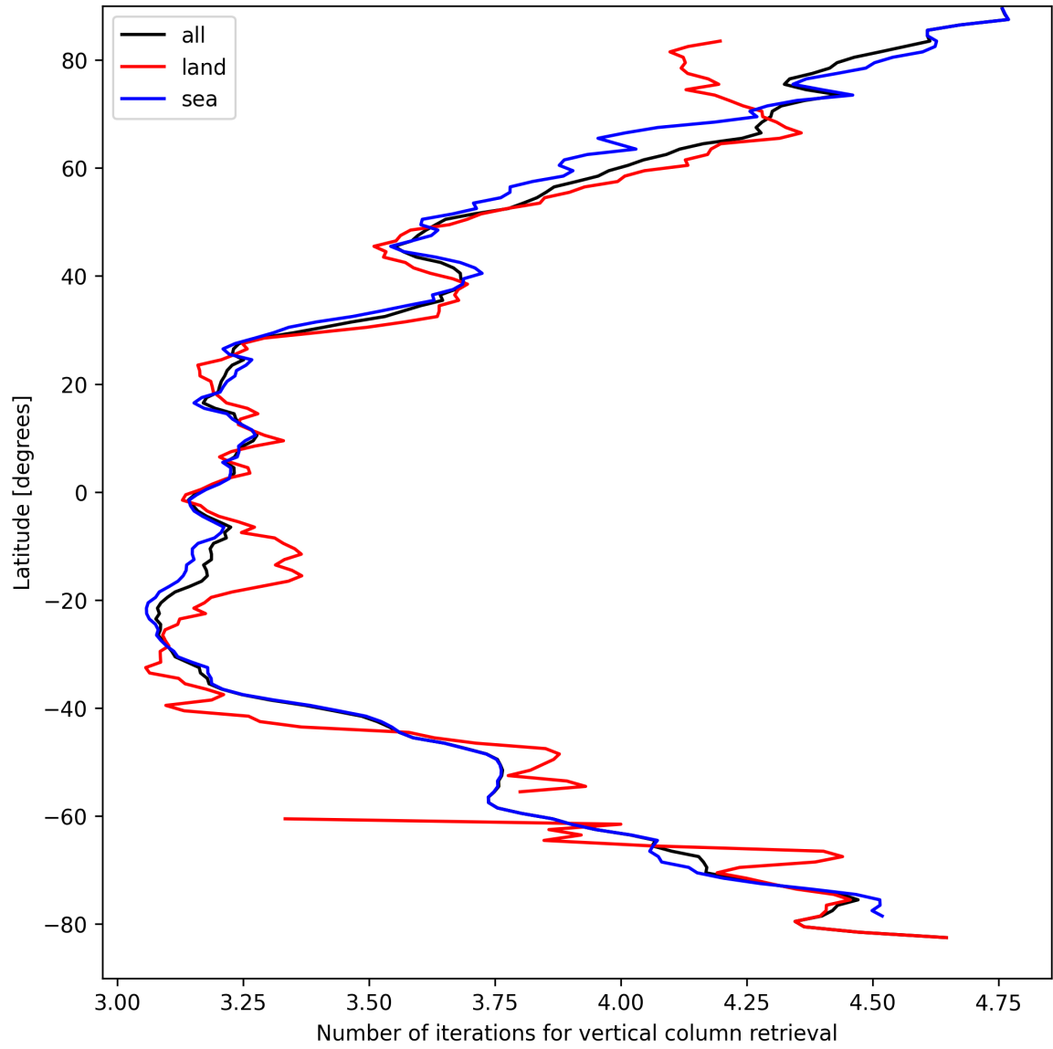
Figure 19: Zonal average of “Number of iterations for vertical column retrieval” for 2025-04-05 to 2025-04-07.
