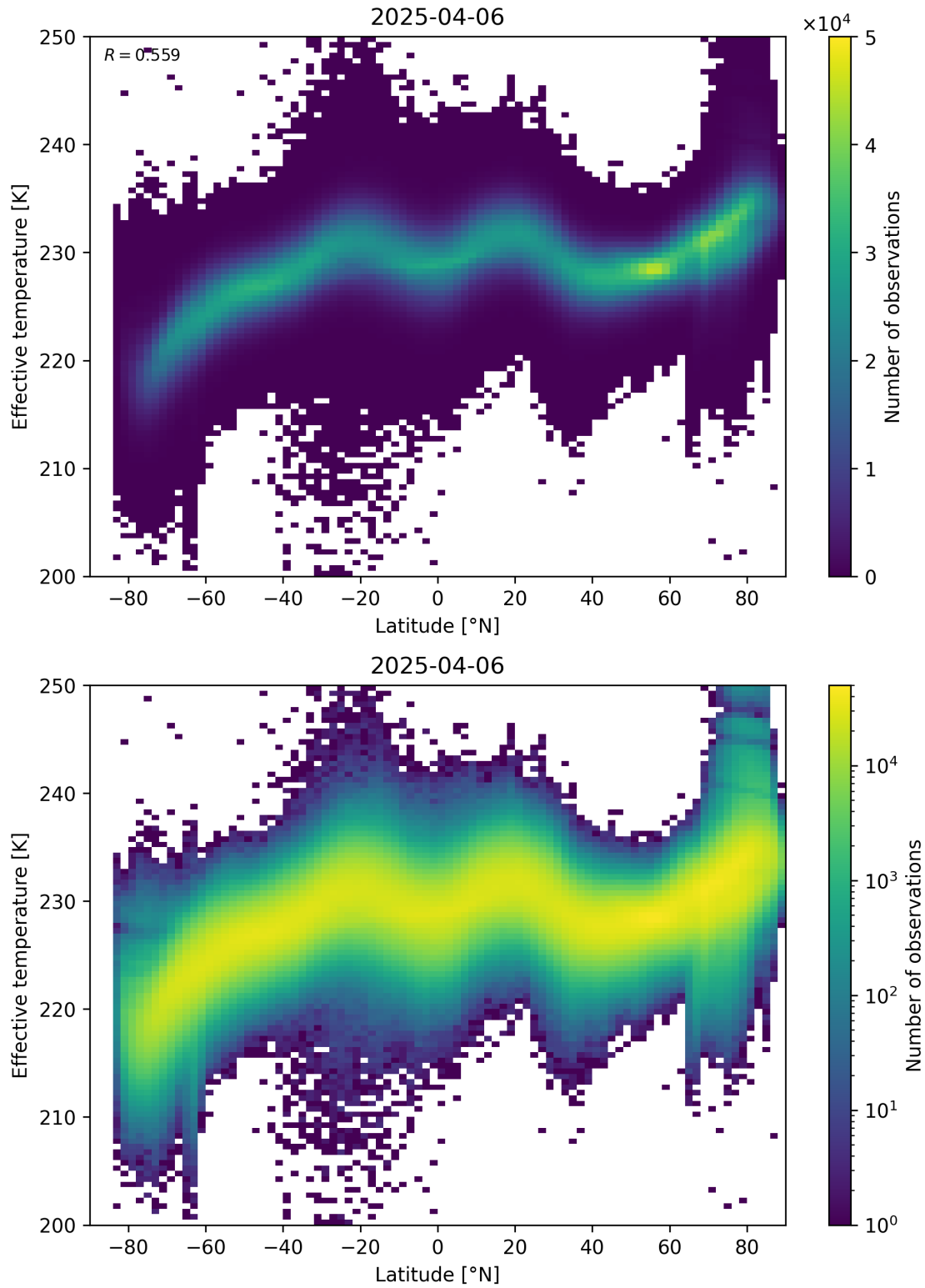
Figure 34: Scatter density plot of “Latitude” against “Effective temperature” for 2025-04-05 to 2025-04-07.
