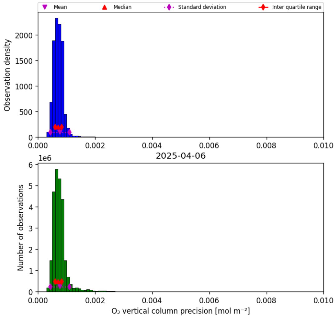
Figure 22: Histogram of “O 3 vertical column precision” for 2025-04-05 to 2025-04-07
