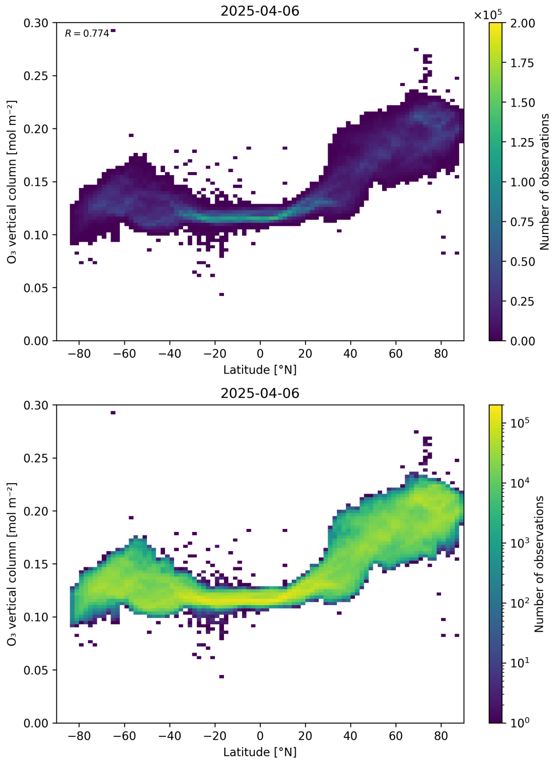
Figure 36: Scatter density plot of “Latitude” against “O 3 vertical column” for 2025-04-05 to 2025-04-07.
