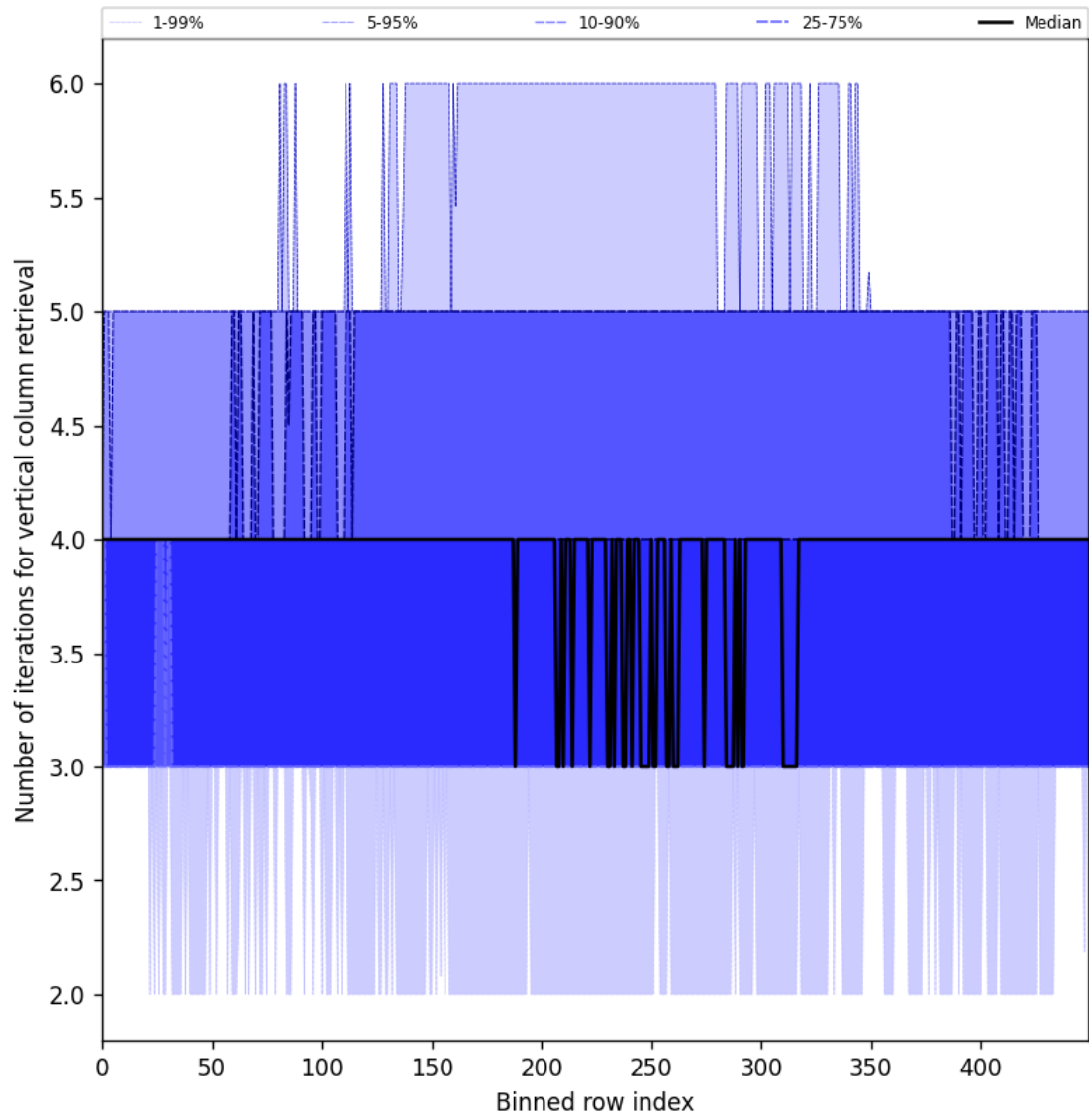
Figure 33: Along track statistics of “Number of iterations for vertical column retrieval” for 2025-04-05 to 2025-04-07
