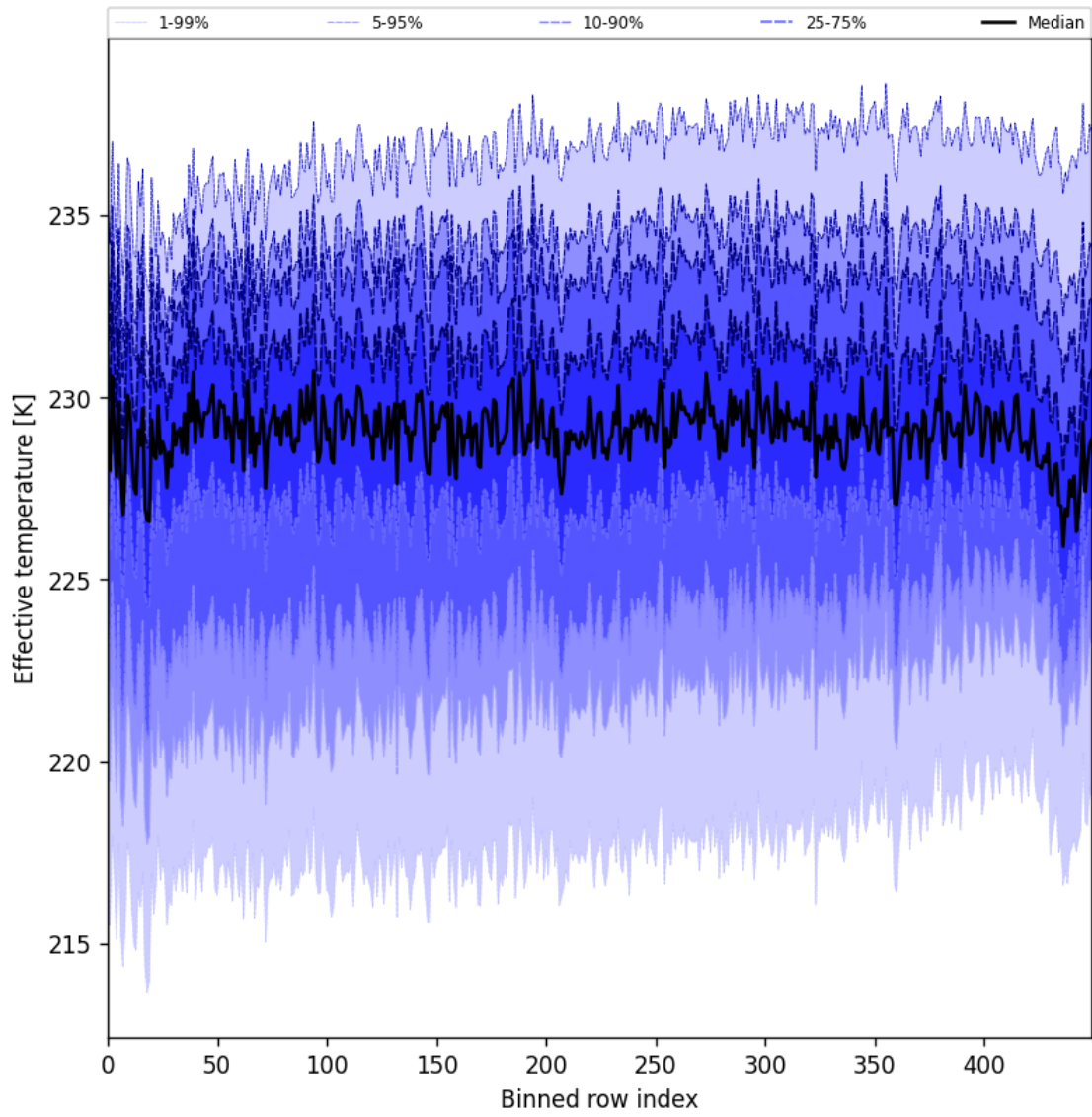
Figure 31: Along track statistics of “Effective temperature” for 2025-04-05 to 2025-04-07
