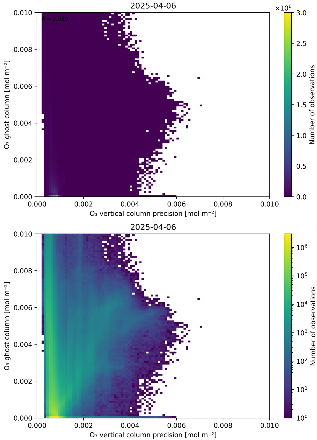
Figure 43: Scatter density plot of “O 3 vertical column precision” against “O 3 ghost column” for 2025-04-05 to 2025-04-07.
