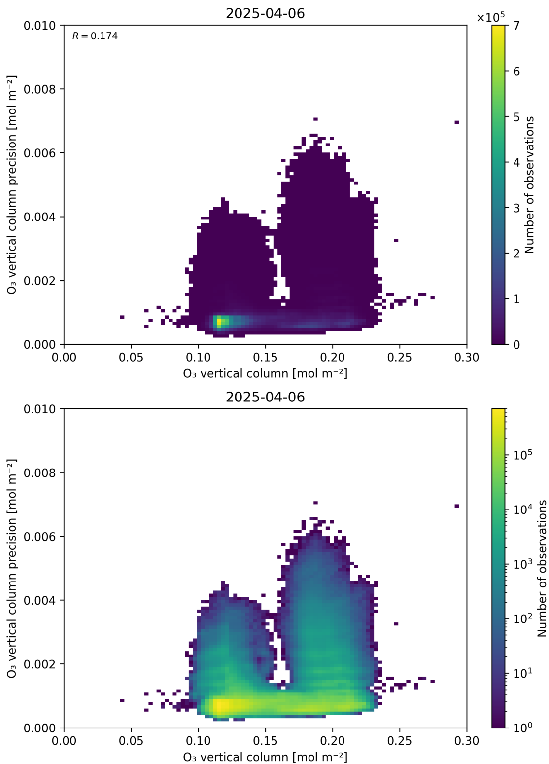
Figure 41: Scatter density plot of “O 3 vertical column” against “O 3 vertical column precision” for 2025-04-05 to 2025-04-07.
