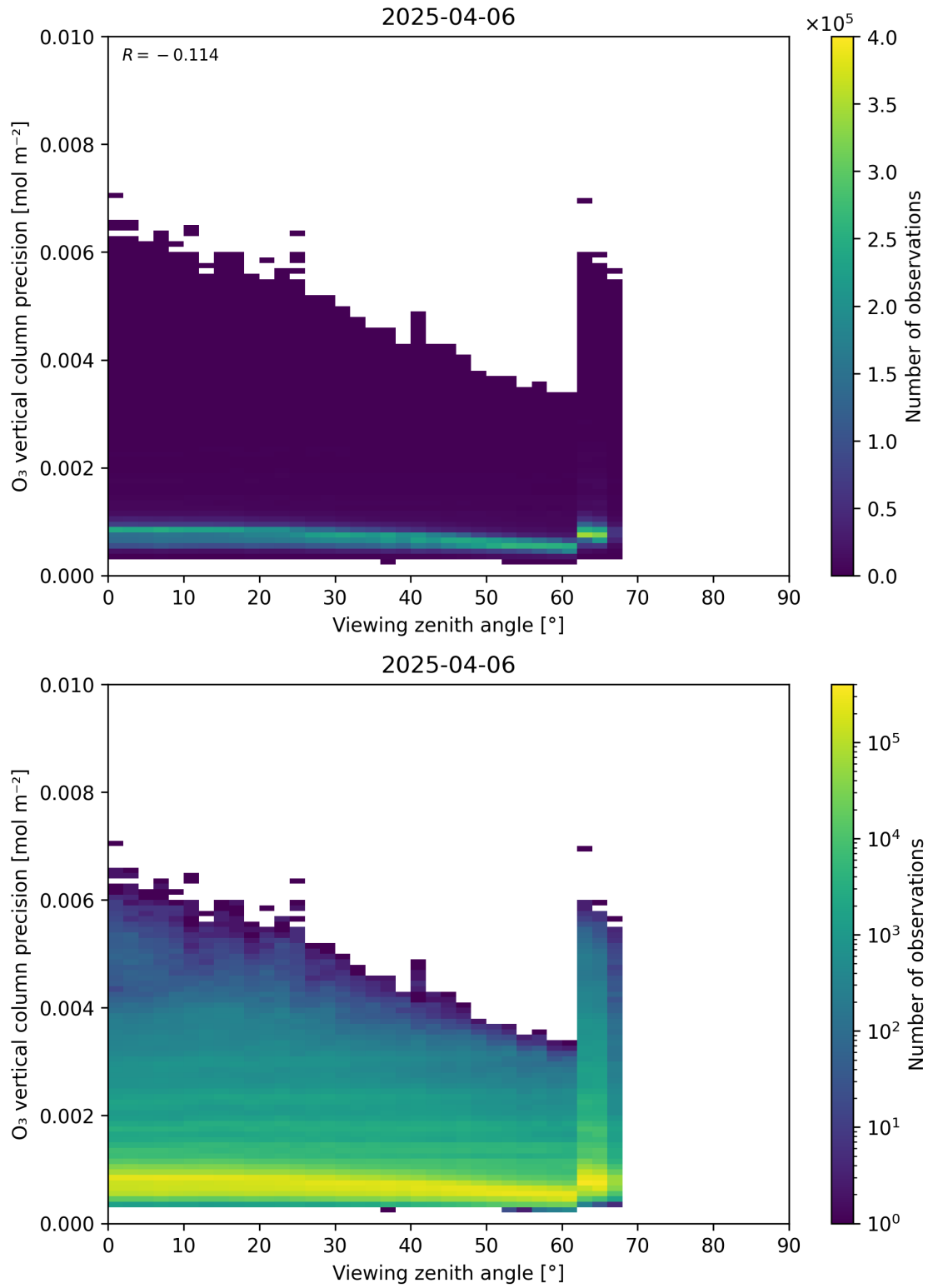
Figure 53: Scatter density plot of “Viewing zenith angle” against “O 3 vertical column precision” for 2025-04-05 to 2025-04-07.
