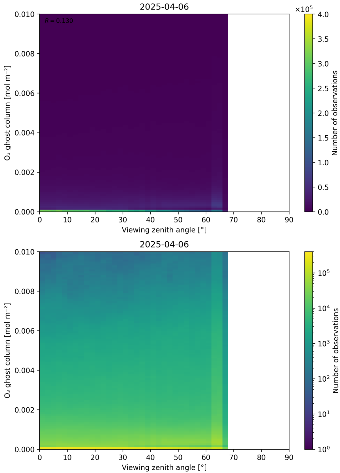
Figure 51: Scatter density plot of “Viewing zenith angle” against “O 3 ghost column” for 2025-04-05 to 2025-04-07.
