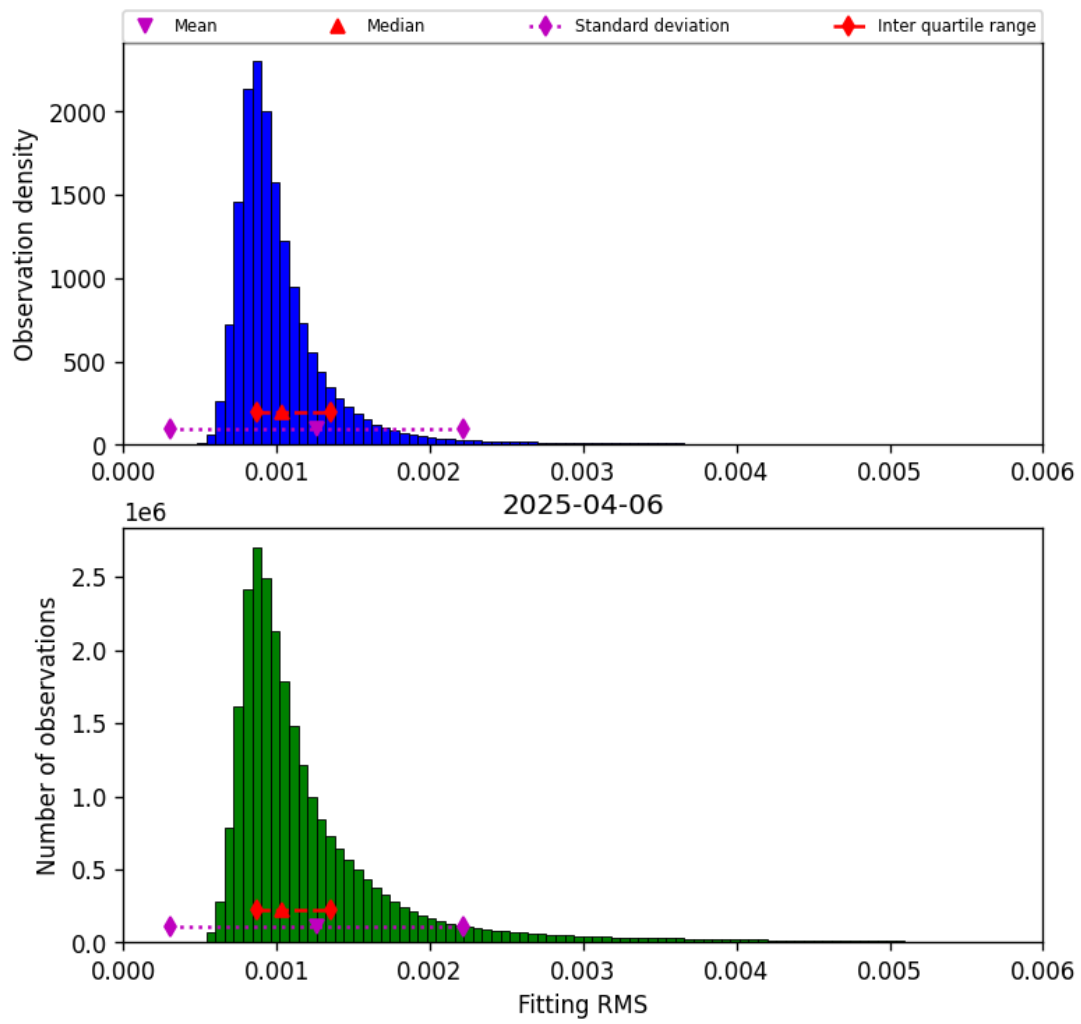
Figure 23: Histogram of “Fitting RMS” for 2025-04-05 to 2025-04-07
