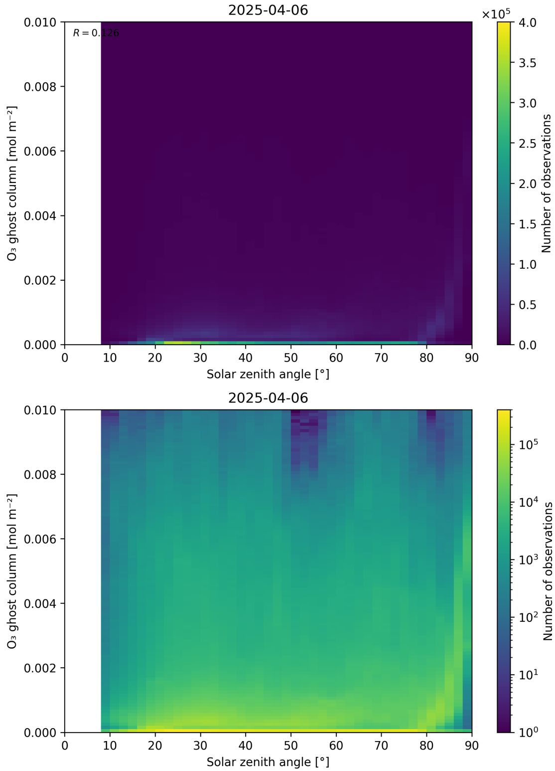
Figure 46: Scatter density plot of “Solar zenith angle” against “O 3 ghost column” for 2025-04-05 to 2025-04-07.
