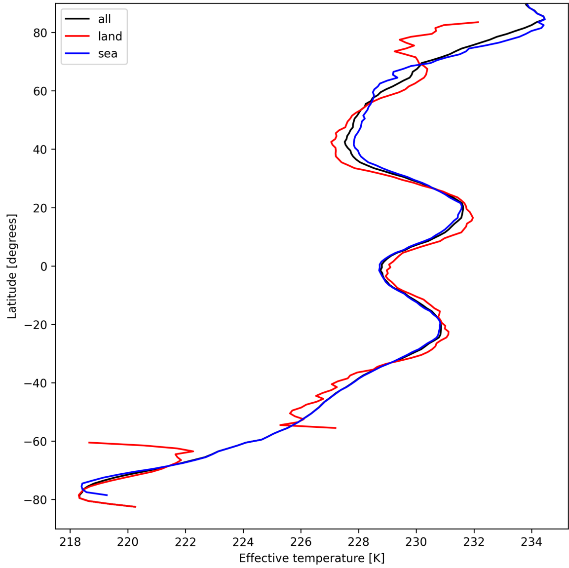
Figure 17: Zonal average of "Effective temperature" for 2025-04-05 to 2025-04-07.
