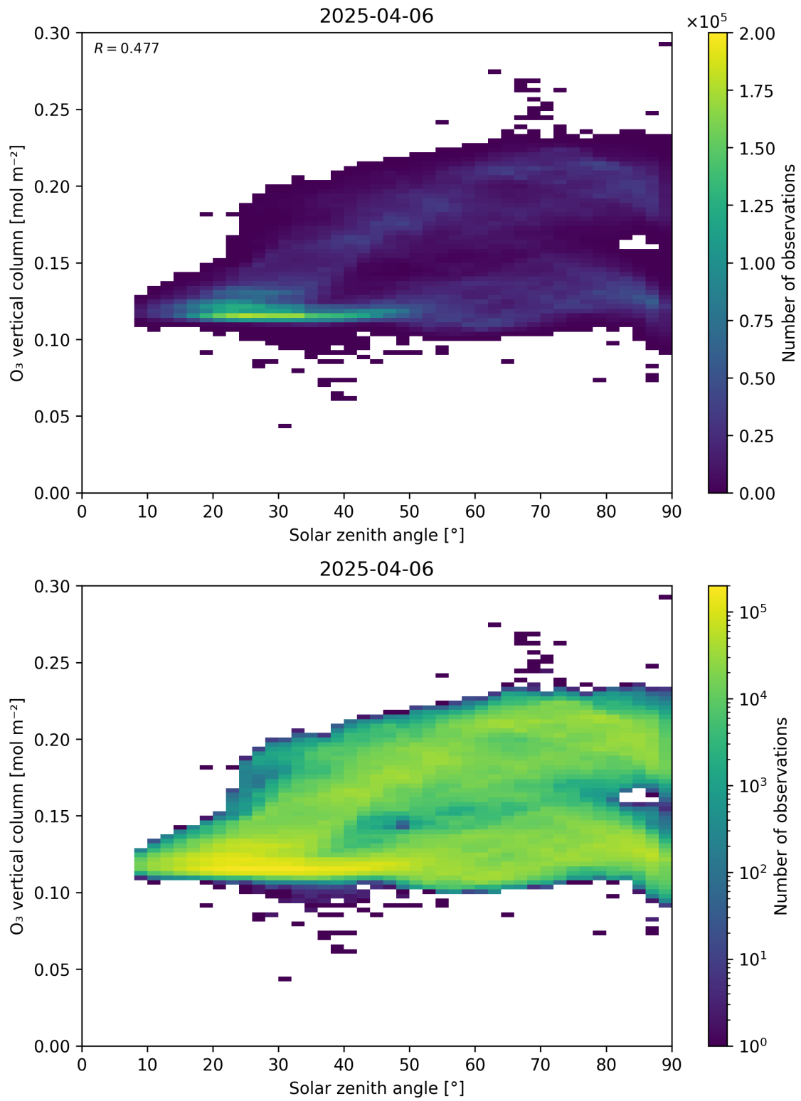
Figure 47: Scatter density plot of “Solar zenith angle” against “O 3 vertical column” for 2025-04-05 to 2025-04-07.
