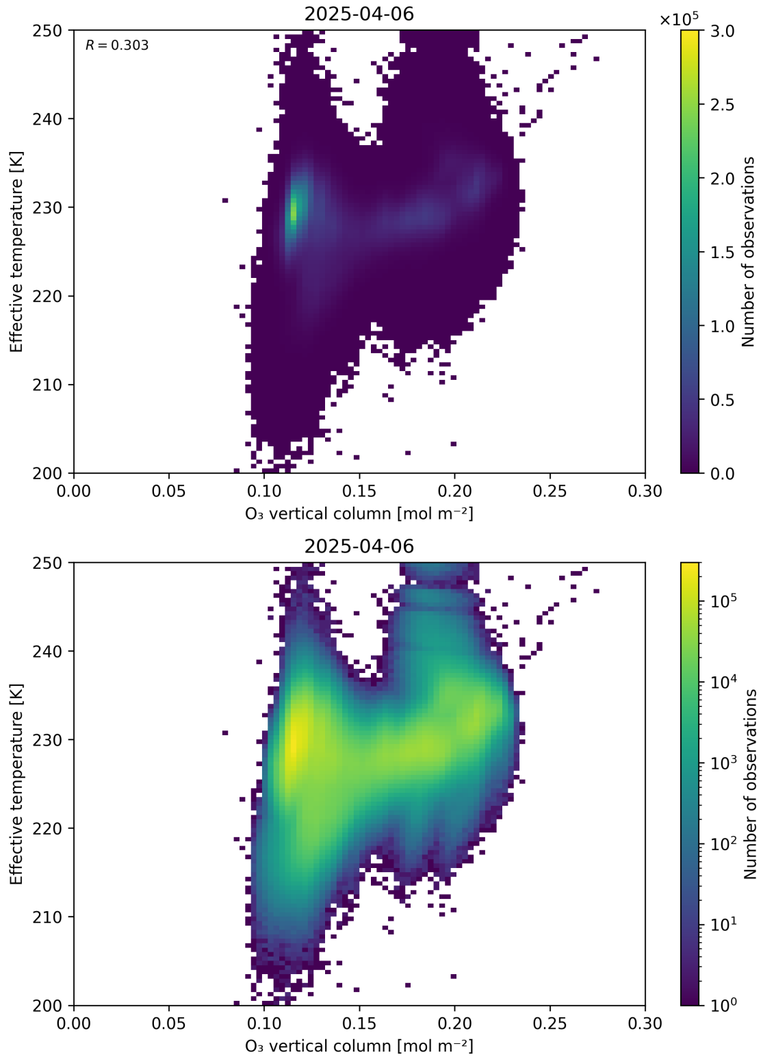
Figure 39: Scatter density plot of “O 3 vertical column” against “Effective temperature” for 2025-04-05 to 2025-04-07.
