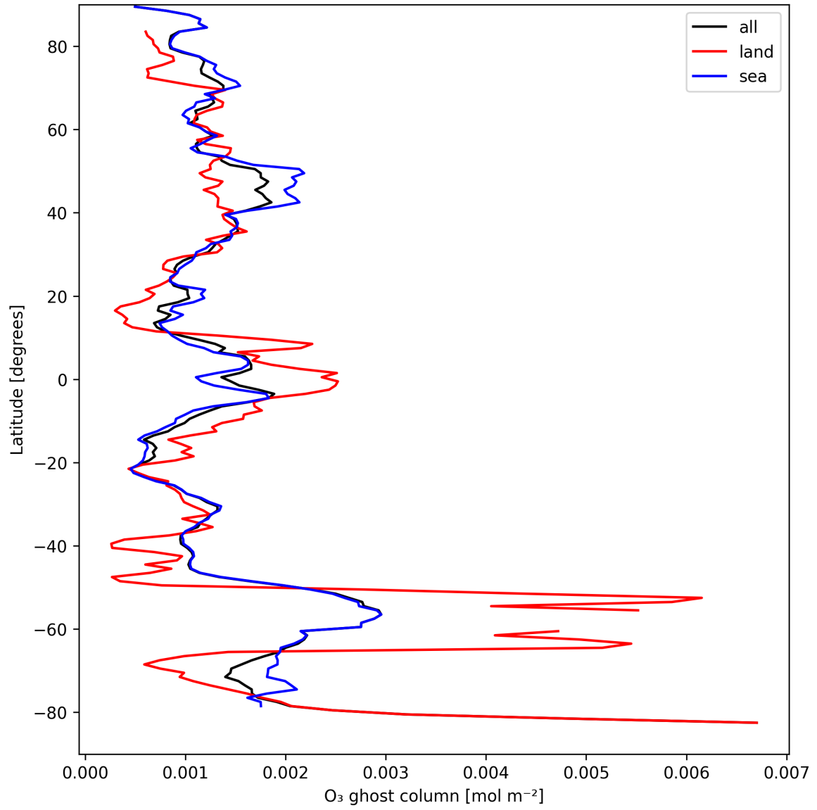
Figure 18: Zonal average of “O 3 ghost column” for 2025-04-05 to 2025-04-07.
