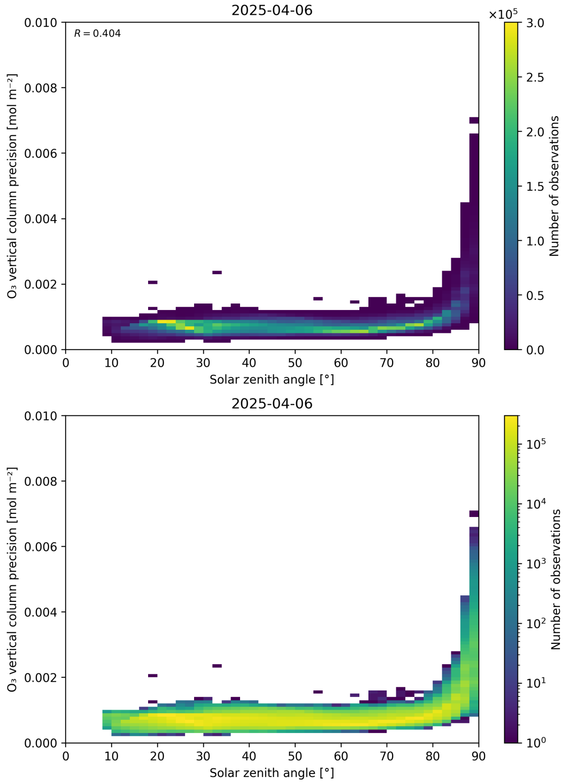
Figure 48: Scatter density plot of “Solar zenith angle” against “O 3 vertical column precision” for 2025-04-05 to 2025-04-07.
