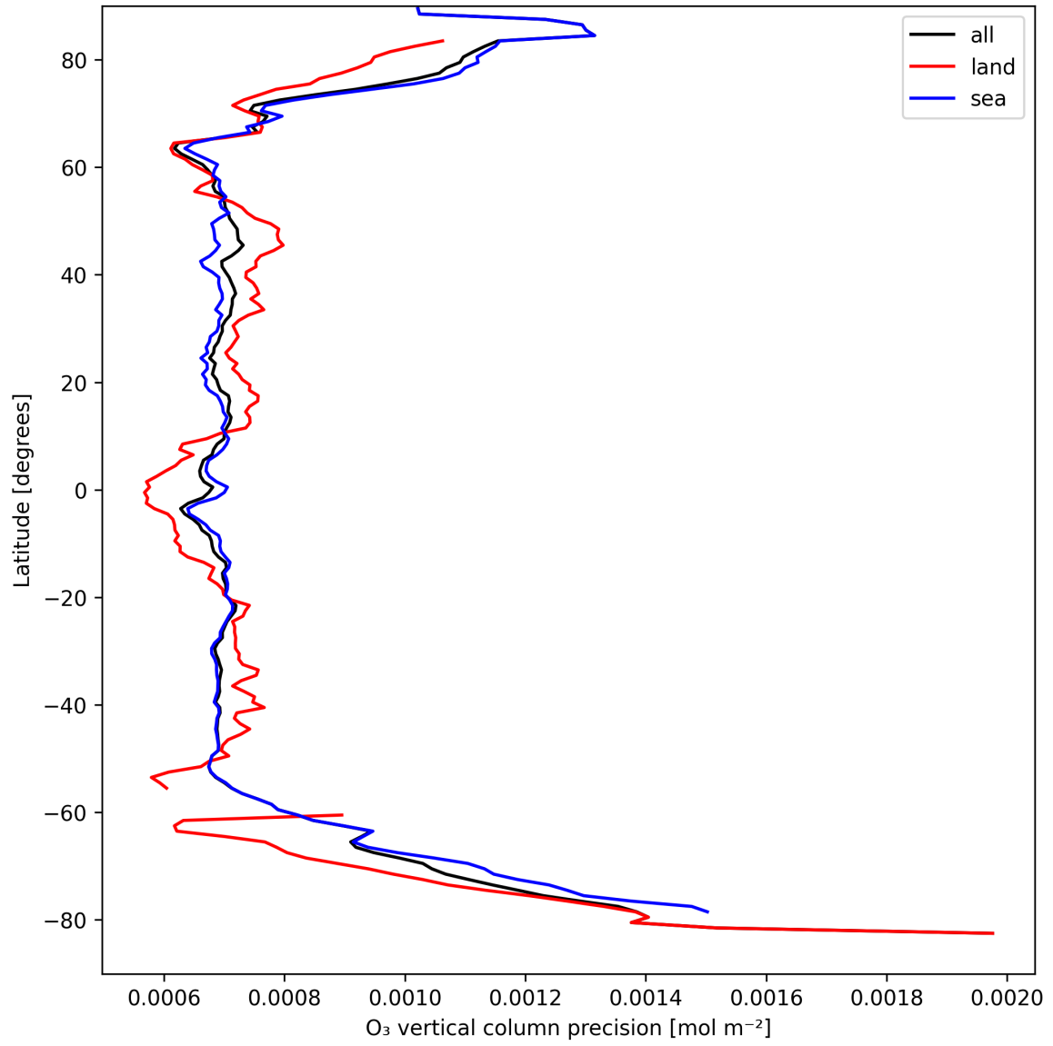
Figure 15: Zonal average of “O 3 vertical column precision” for 2025-04-05 to 2025-04-07.
