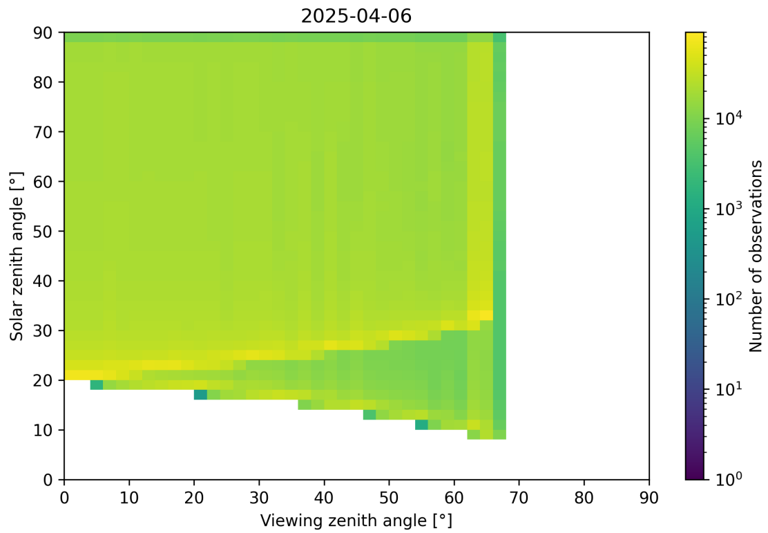
Figure 54: Scatter density plot of “Viewing zenith angle” against “Solar zenith angle” for 2025-04-05 to 2025-04-07.
