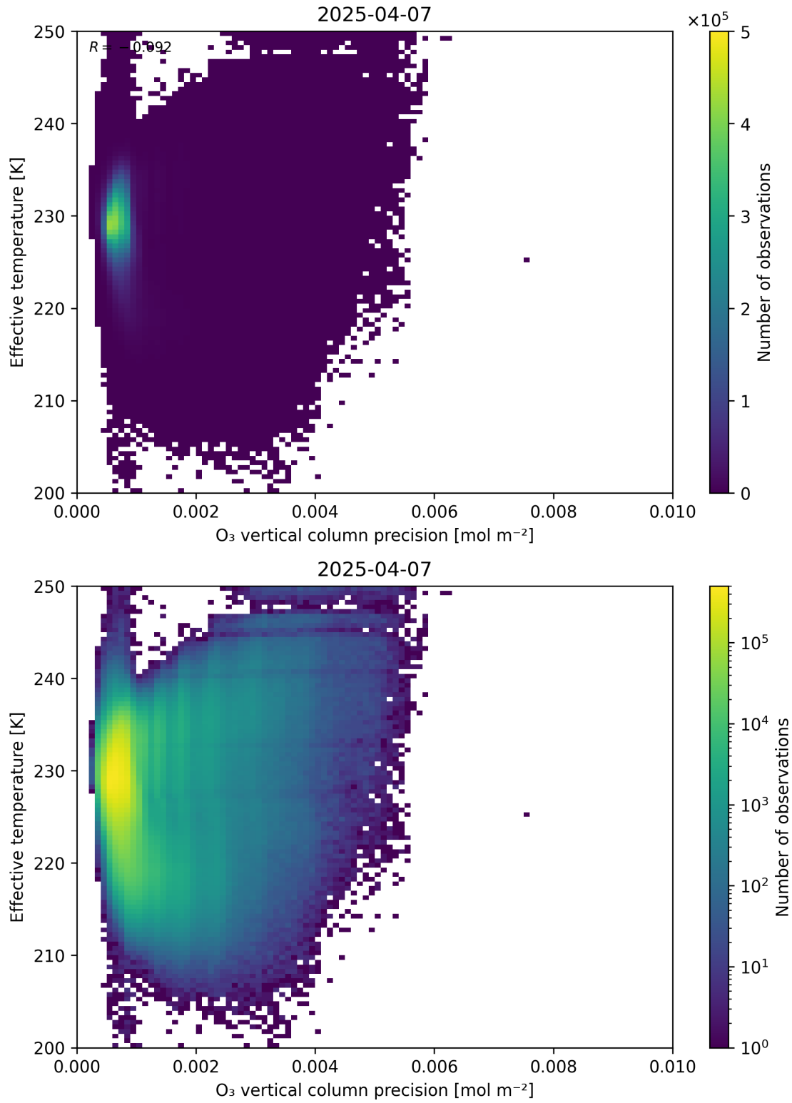
Figure 42: Scatter density plot of “ O_3 vertical column precision” against “Effective temperature” for 2025-04-06 to 2025-04-08.
