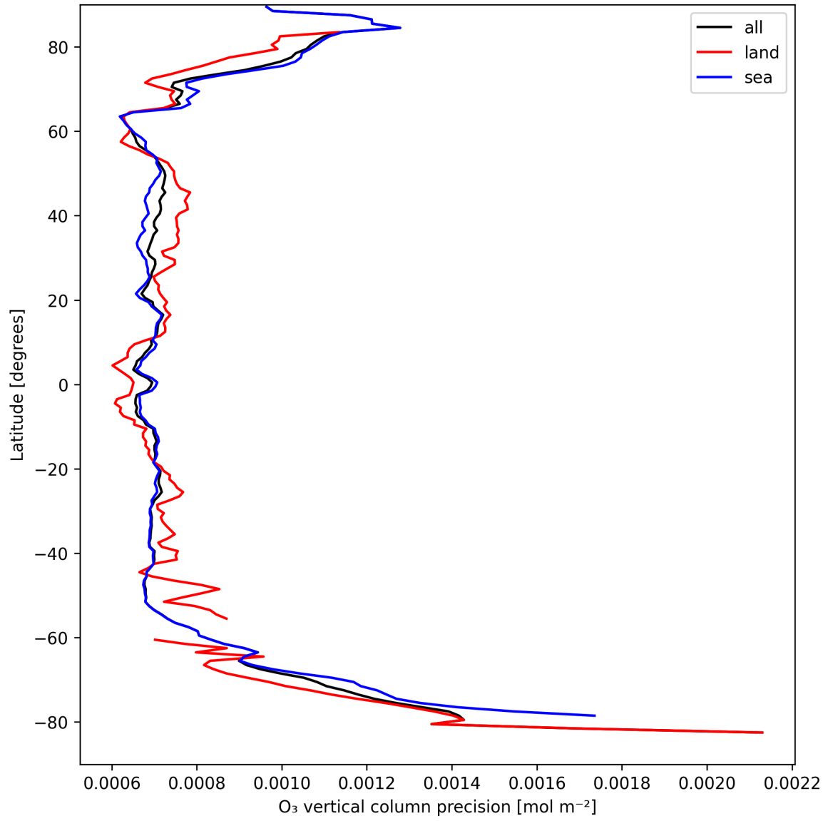
Figure 15: Zonal average of “O 3 vertical column precision” for 2025-04-06 to 2025-04-08.
