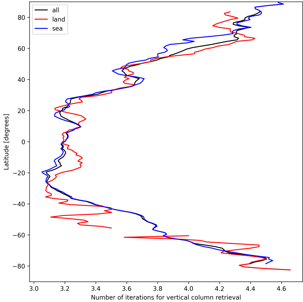
Figure 19: Zonal average of “Number of iterations for vertical column retrieval” for 2025-04-06 to 2025-04-08.
