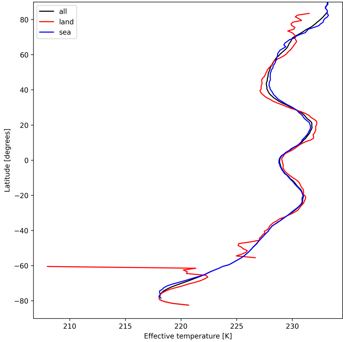
Figure 17: Zonal average of “Effective temperature” for 2025-04-06 to 2025-04-08.
