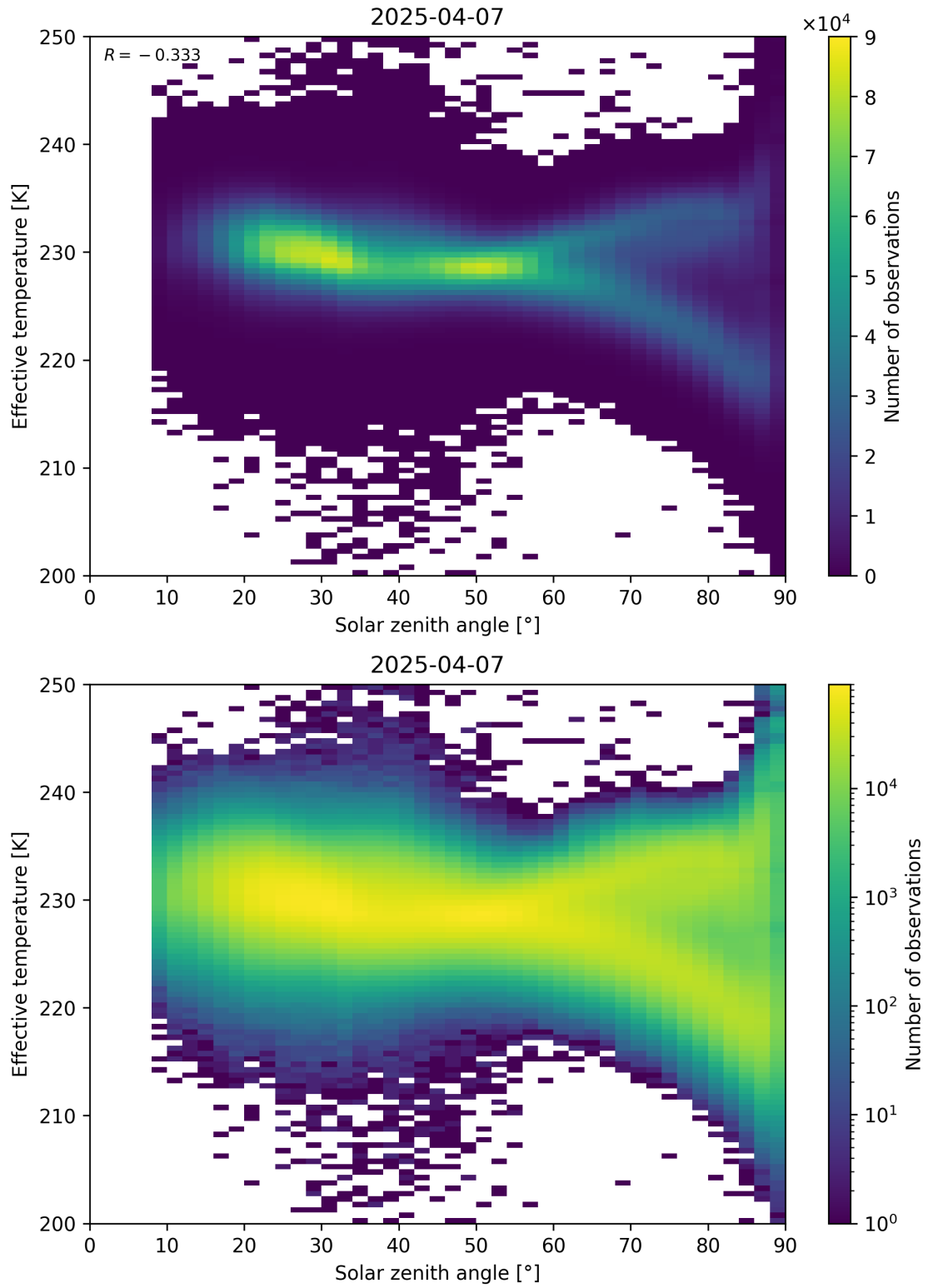
Figure 45: Scatter density plot of “Solar zenith angle” against “Effective temperature” for 2025-04-06 to 2025-04-08.
