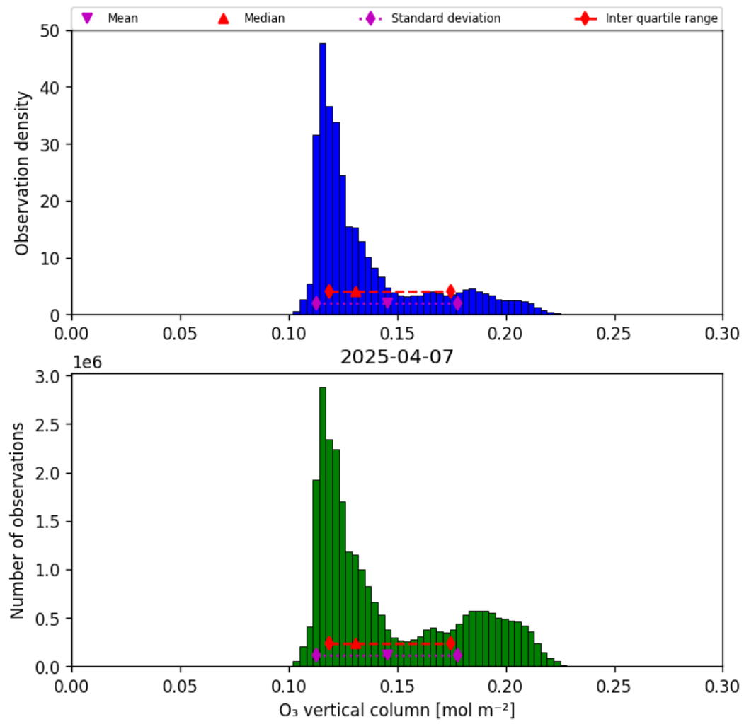
Figure 21: Histogram of “O 3 vertical column” for 2025-04-06 to 2025-04-08
