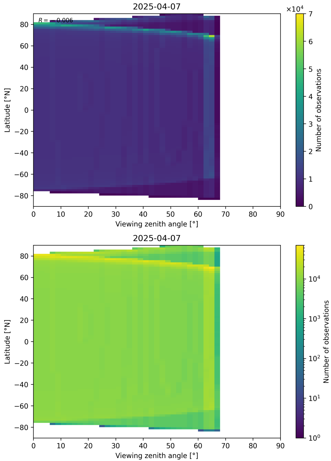
Figure 49: Scatter density plot of “Viewing zenith angle” against “Latitude” for 2025-04-06 to 2025-04-08.
