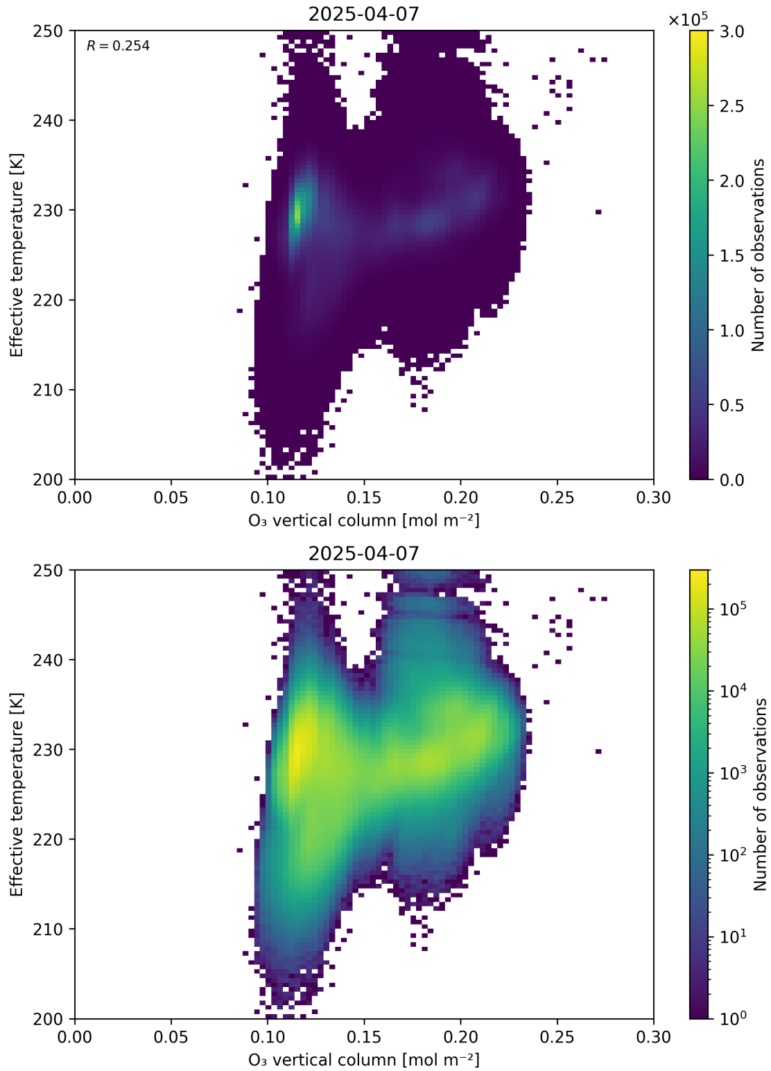
Figure 39: Scatter density plot of “O 3 vertical column” against “Effective temperature” for 2025-04-06 to 2025-04-08.
