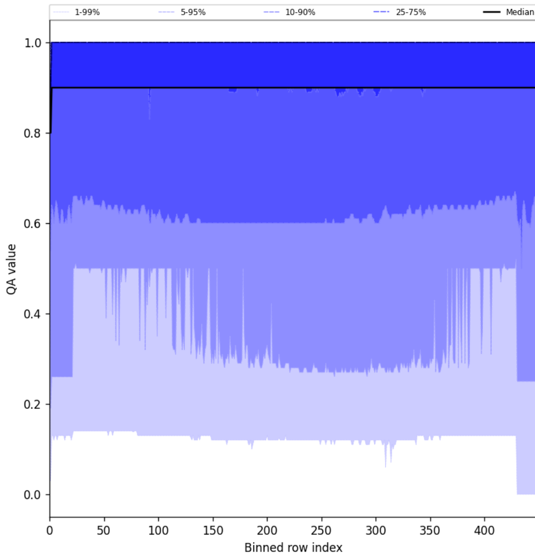
Figure 27: Along track statistics of “QA value” for 2025-04-06 to 2025-04-08
