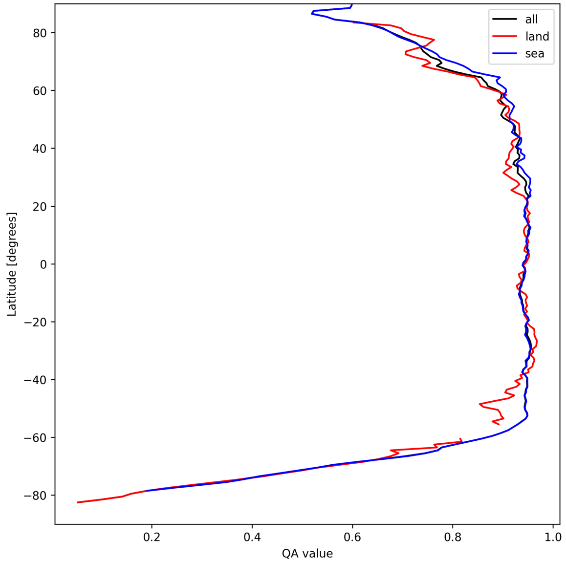
Figure 13: Zonal average of “QA value” for 2025-04-06 to 2025-04-08.
