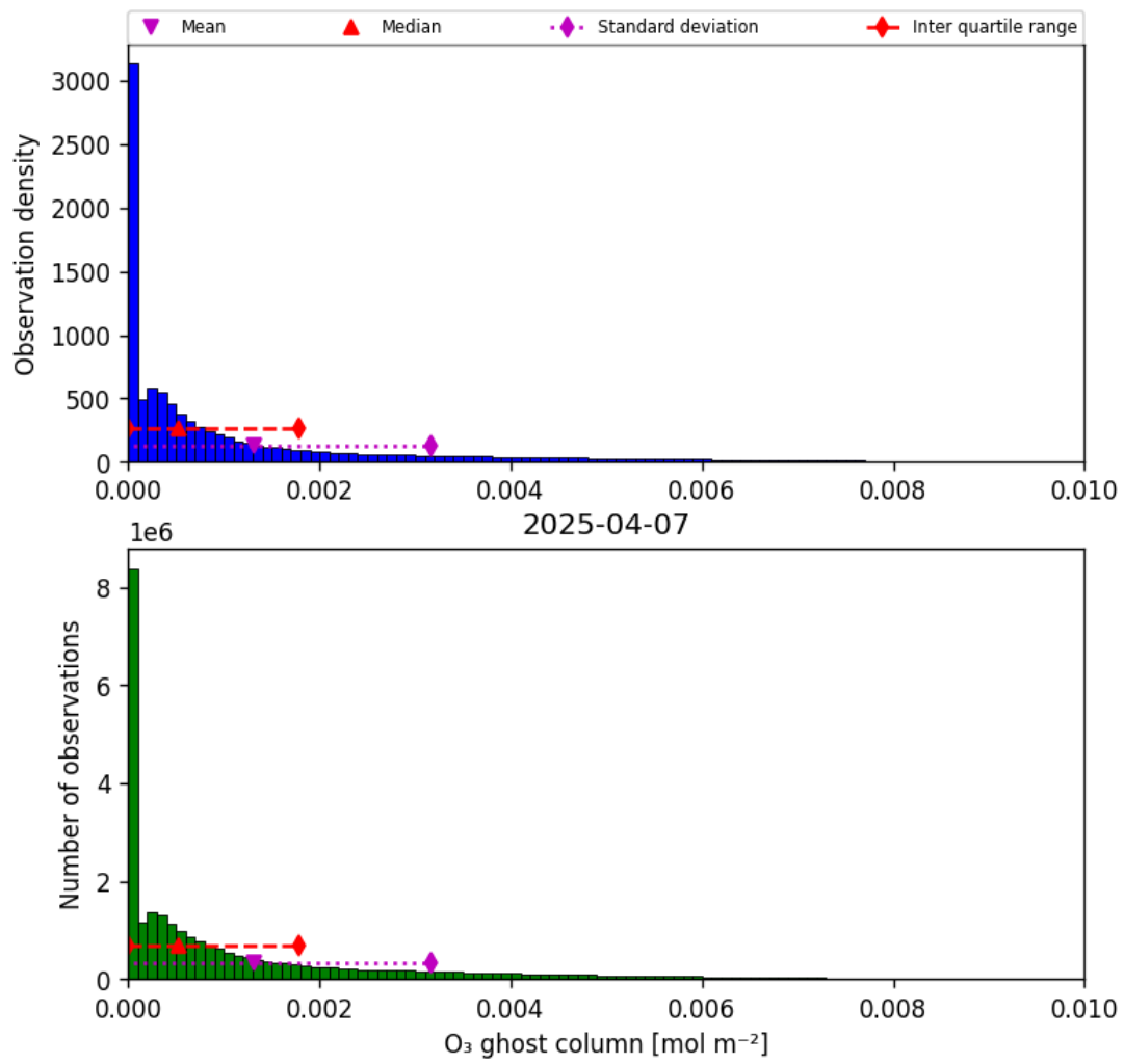
Figure 25: Histogram of “O 3 ghost column” for 2025-04-06 to 2025-04-08
