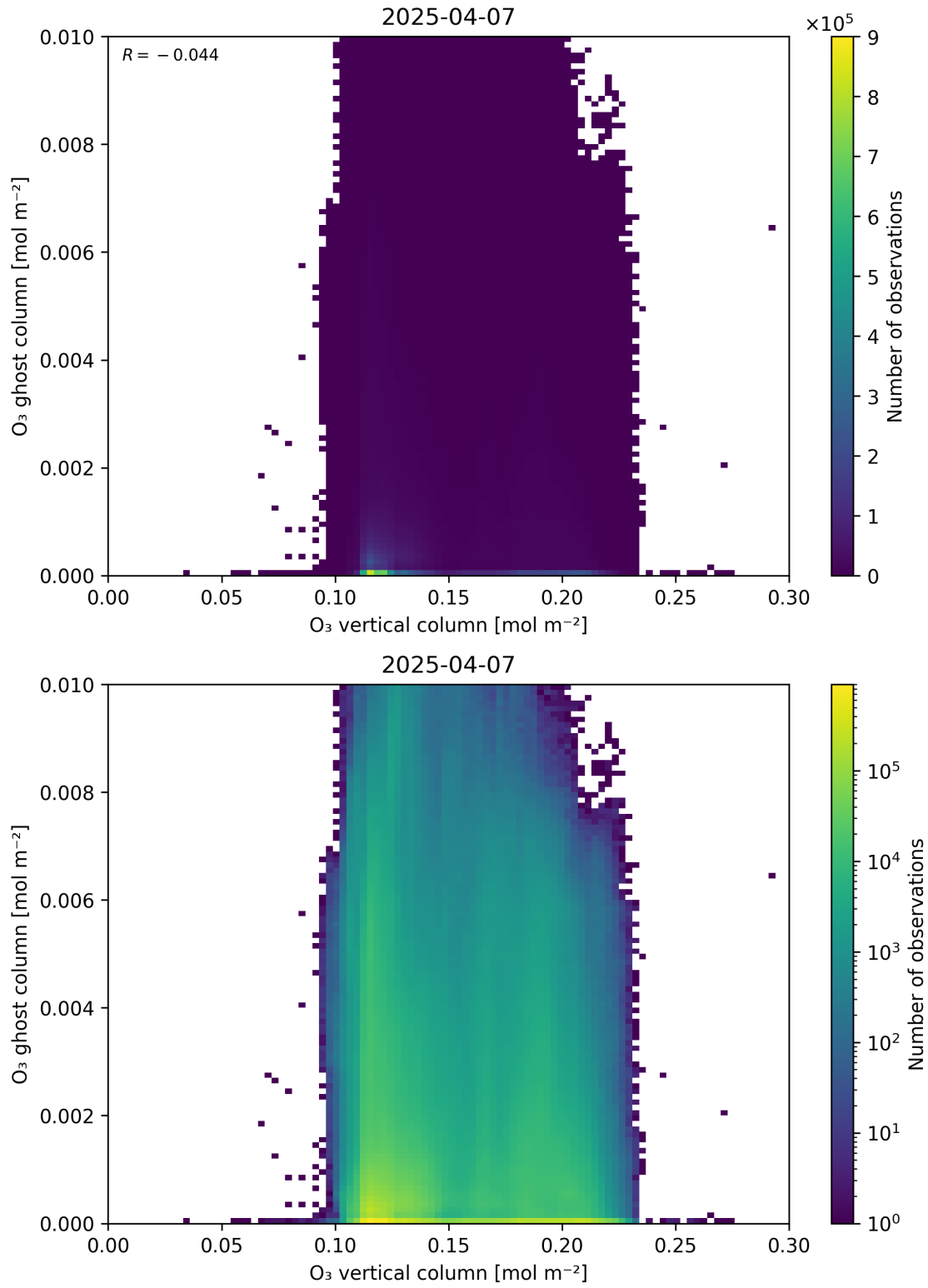
Figure 40: Scatter density plot of “O 3 vertical column” against “O 3 ghost column” for 2025-04-06 to 2025-04-08.
