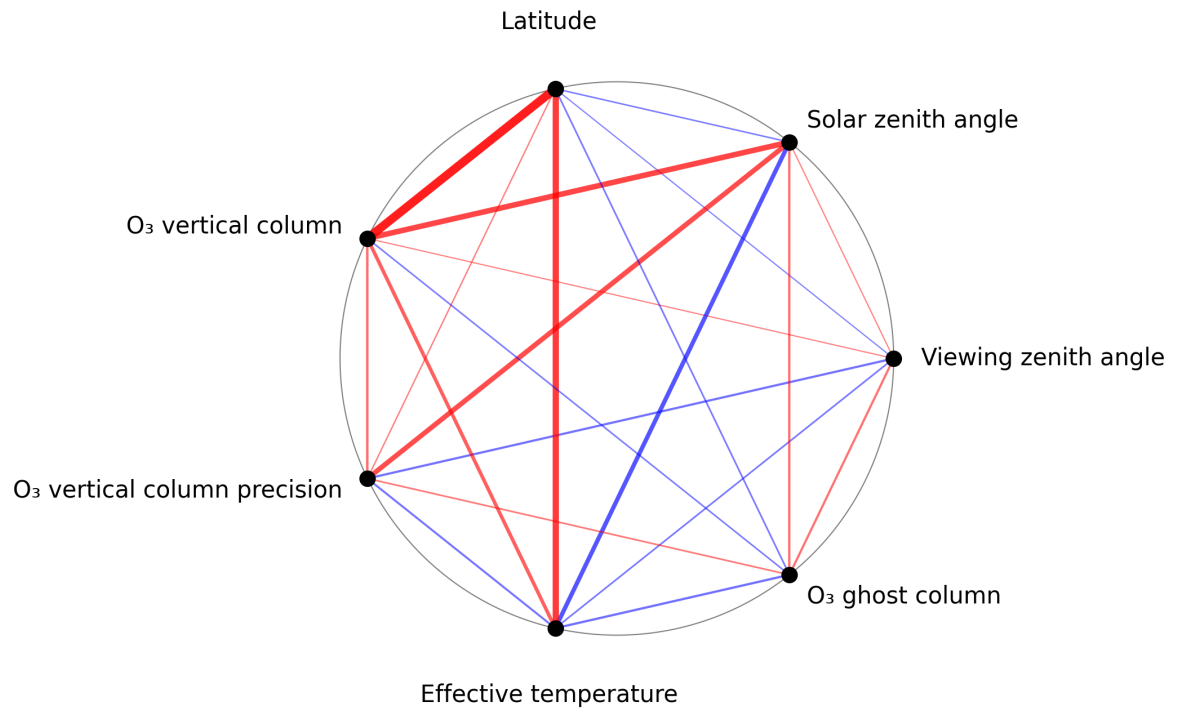
Figure 1: Map of correlation graph for 2025-04-06 to 2025-04-08.
