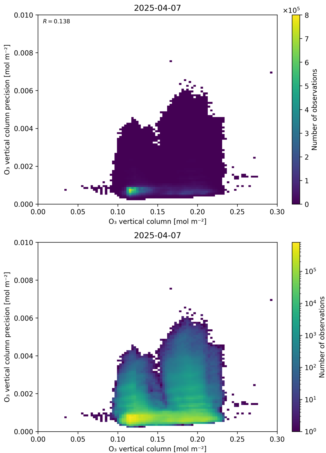
Figure 41: Scatter density plot of “O 3 vertical column” against “O 3 vertical column precision” for 2025-04-06 to 2025-04-08.
