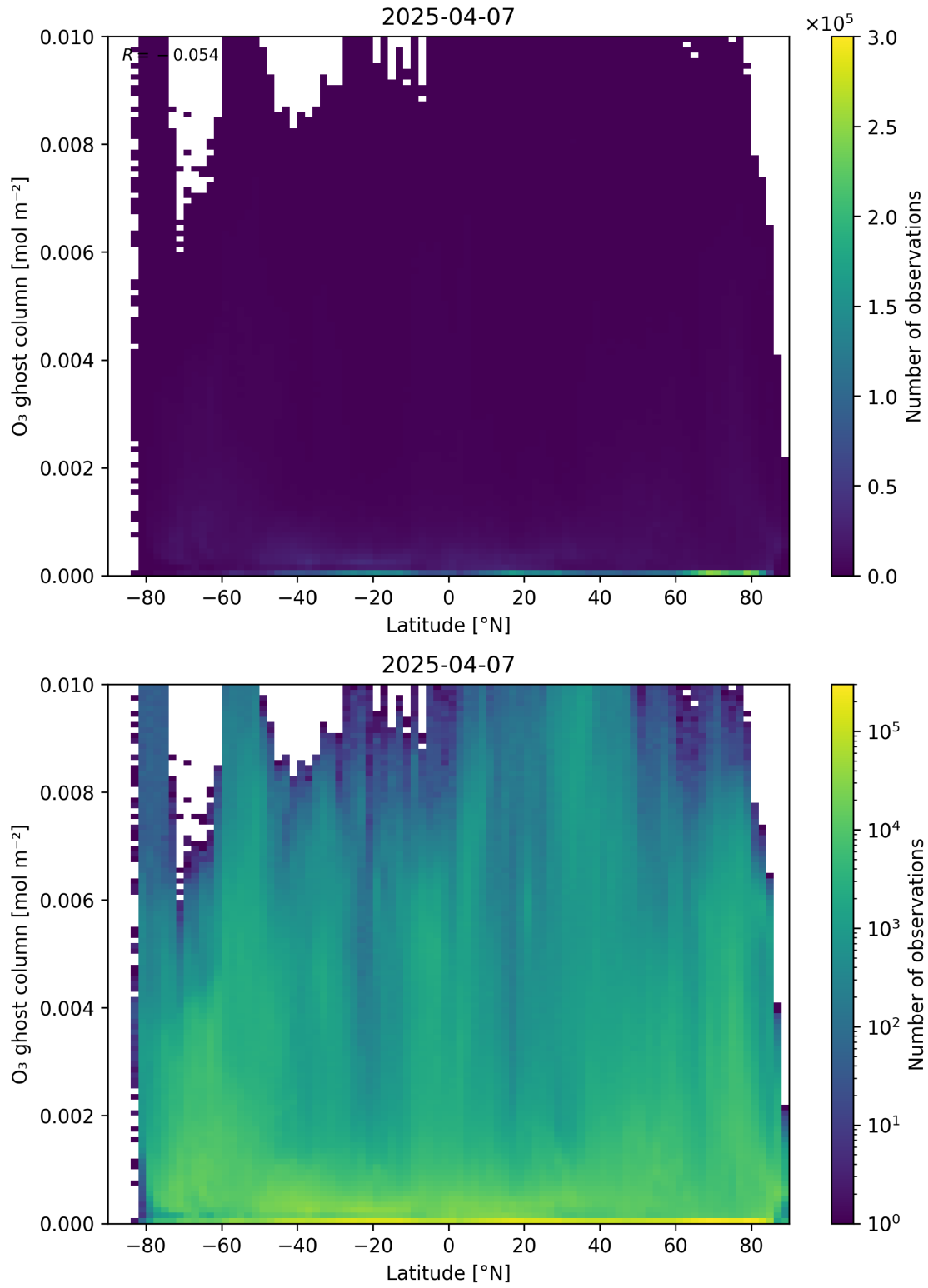
Figure 35: Scatter density plot of “Latitude” against “O 3 ghost column” for 2025-04-06 to 2025-04-08.
