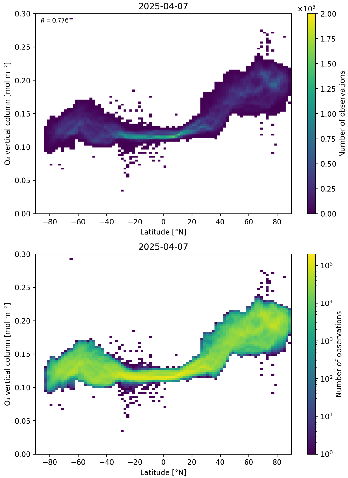
Figure 36: Scatter density plot of “Latitude” against “O 3 vertical column” for 2025-04-06 to 2025-04-08.
