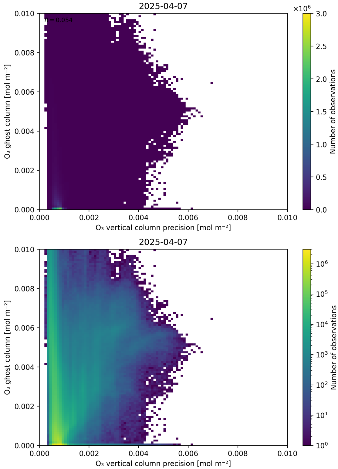
Figure 43: Scatter density plot of “O 3 vertical column precision” against “O 3 ghost column” for 2025-04-06 to 2025-04-08.
