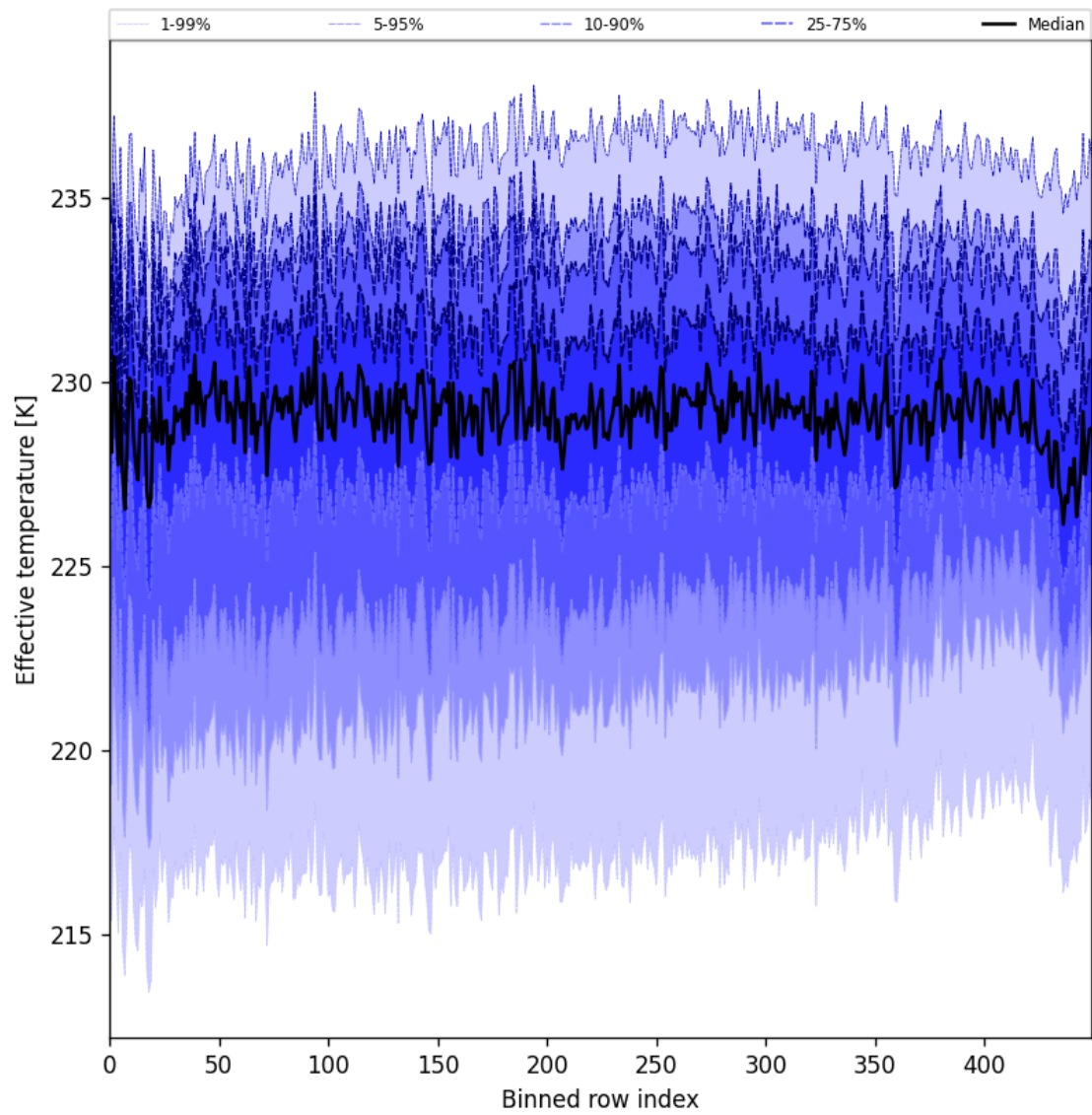
Figure 31: Along track statistics of “Effective temperature” for 2025-04-06 to 2025-04-08
