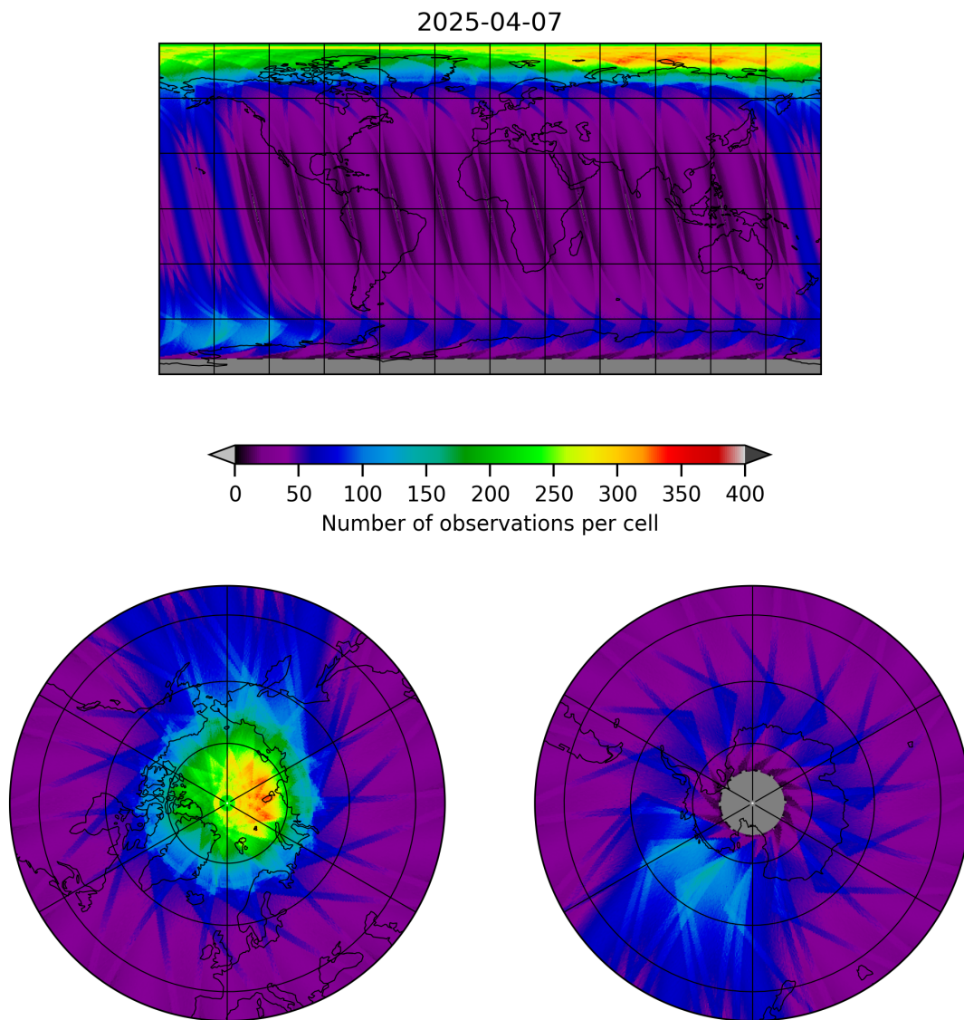
Figure 12: Map of the number of observations for 2025-04-06 to 2025-04-08
