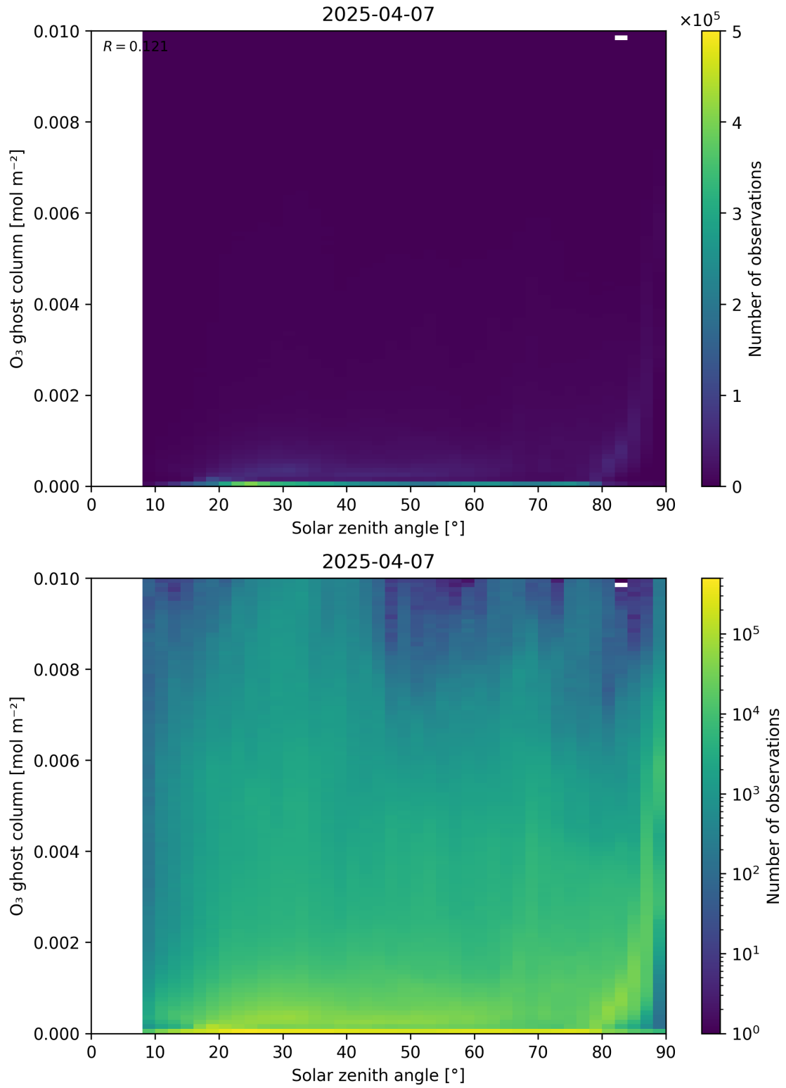
Figure 46: Scatter density plot of “Solar zenith angle” against “O 3 ghost column” for 2025-04-06 to 2025-04-08.
