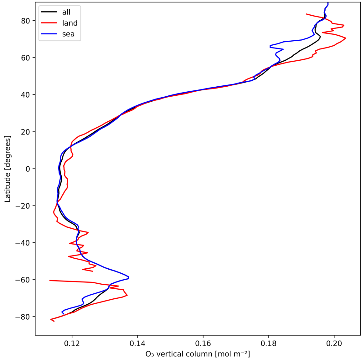
Figure 14: Zonal average of “O 3 vertical column” for 2025-04-06 to 2025-04-08.
