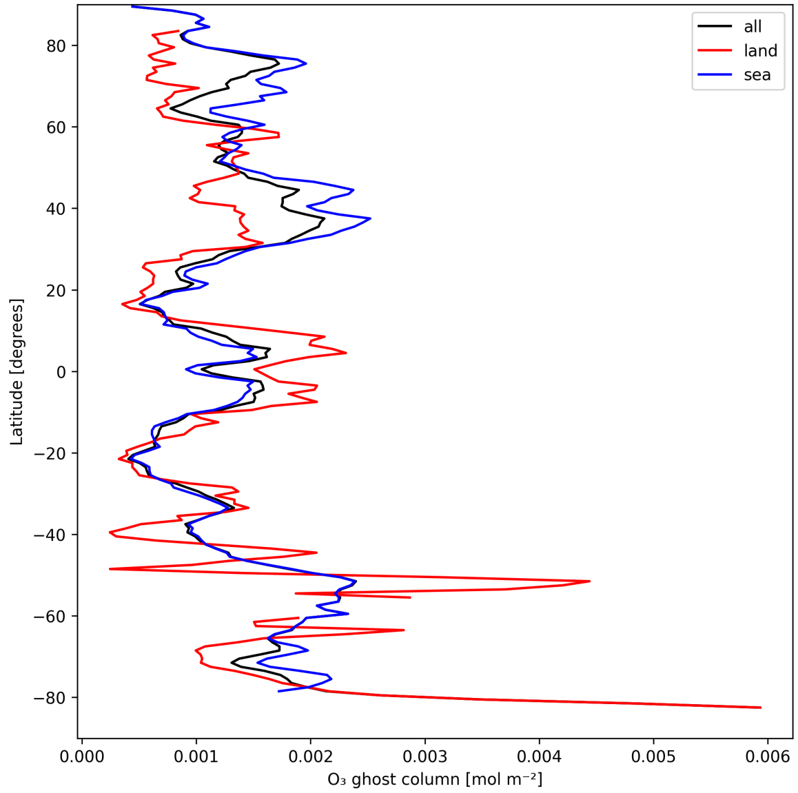
Figure 18: Zonal average of “O 3 ghost column” for 2025-04-06 to 2025-04-08.
