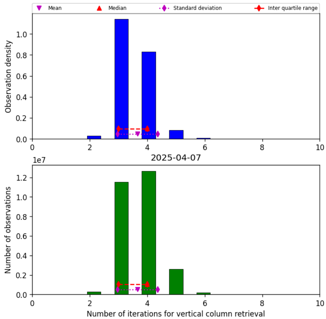
Figure 26: Histogram of “Number of iterations for vertical column retrieval” for 2025-04-06 to 2025-04-08
