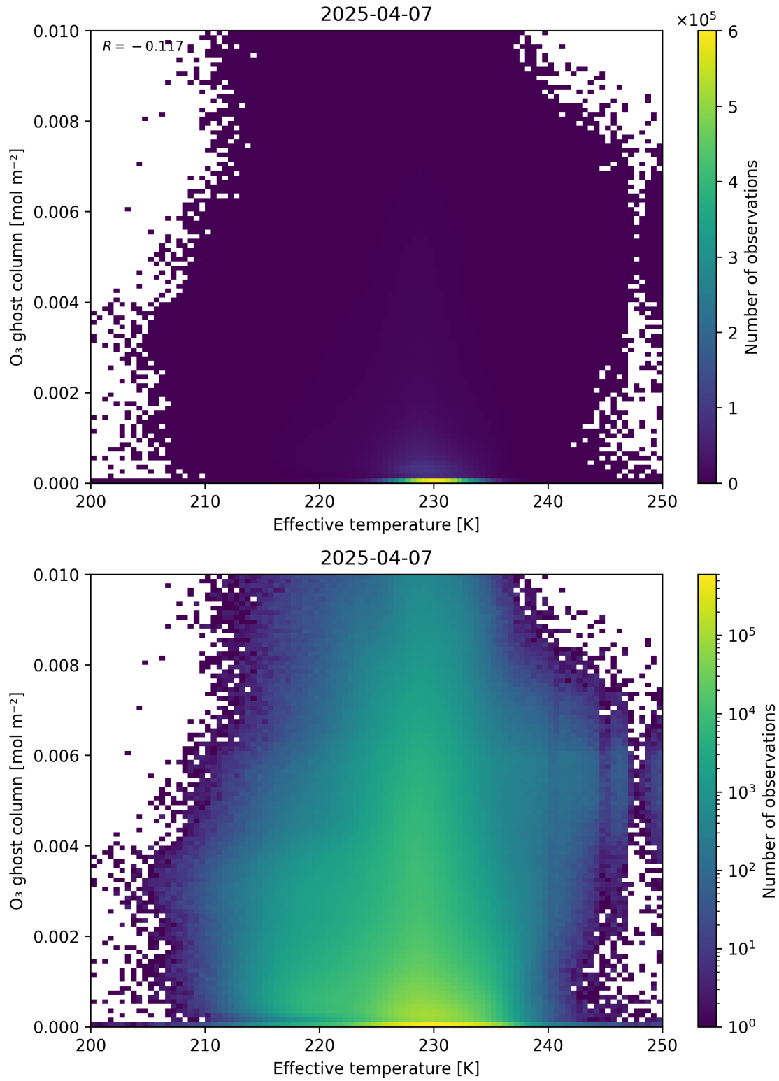
Figure 38: Scatter density plot of “Effective temperature” against “O 3 ghost column” for 2025-04-06 to 2025-04-08.
