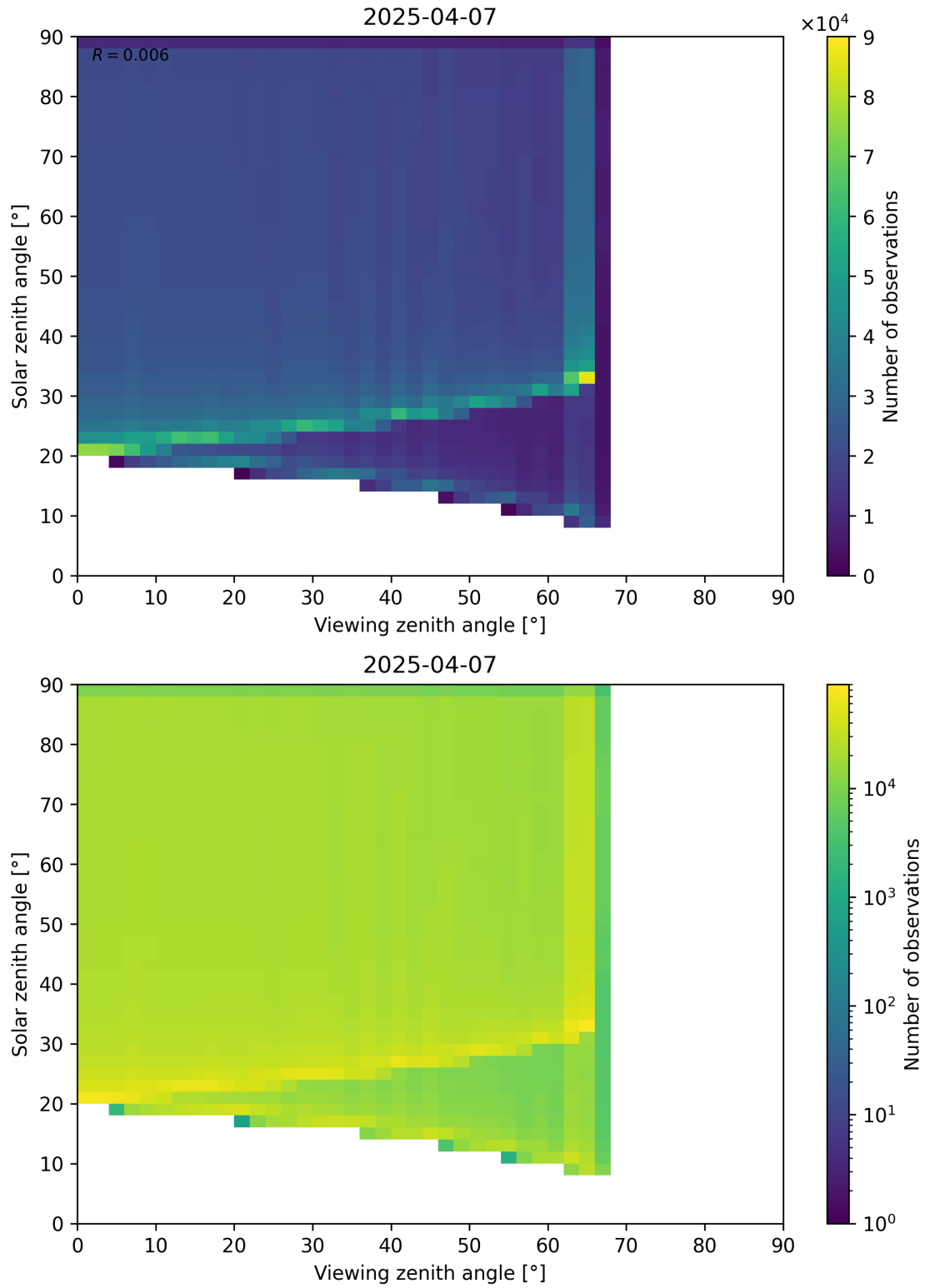
Figure 54: Scatter density plot of “Viewing zenith angle” against “Solar zenith angle” for 2025-04-06 to 2025-04-08.
