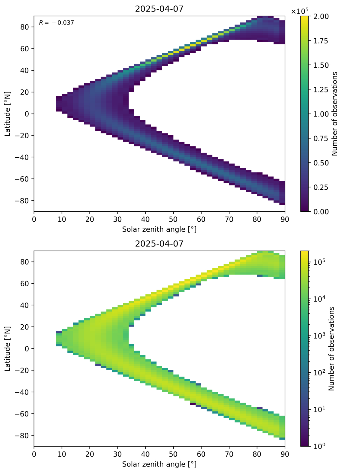
Figure 44: Scatter density plot of “Solar zenith angle” against “Latitude” for 2025-04-06 to 2025-04-08.
