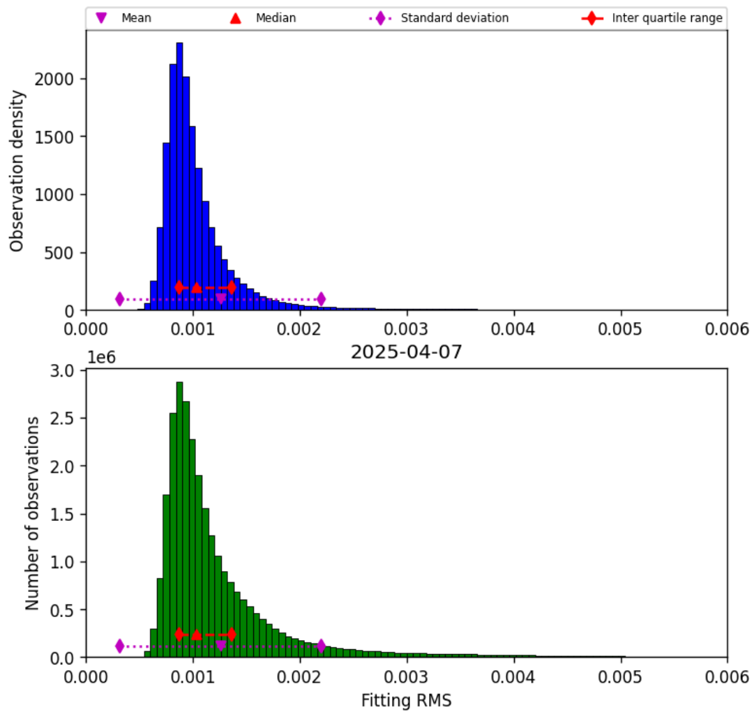
Figure 23: Histogram of “Fitting RMS” for 2025-04-06 to 2025-04-08
