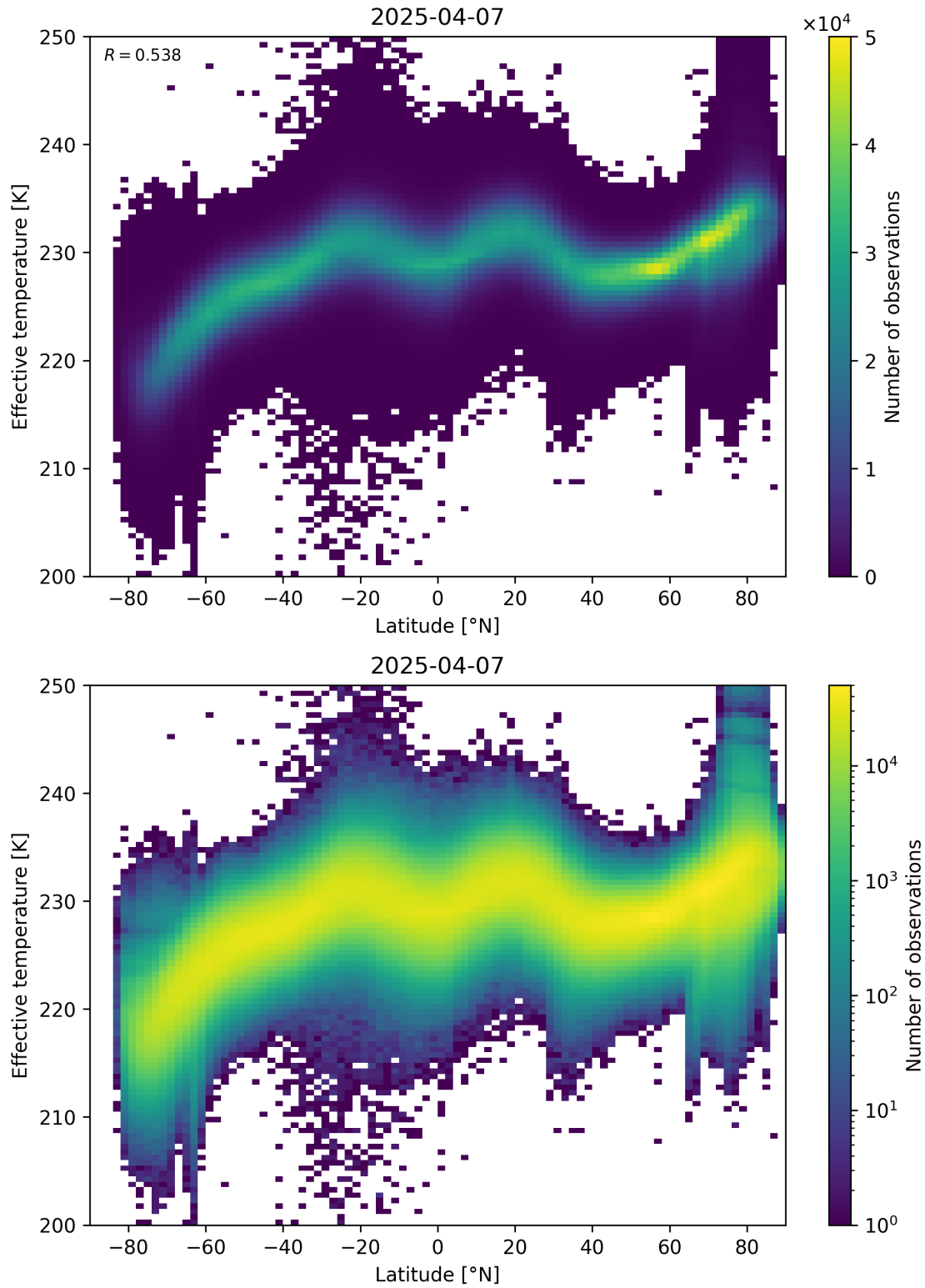
Figure 34: Scatter density plot of “Latitude” against “Effective temperature” for 2025-04-06 to 2025-04-08.
