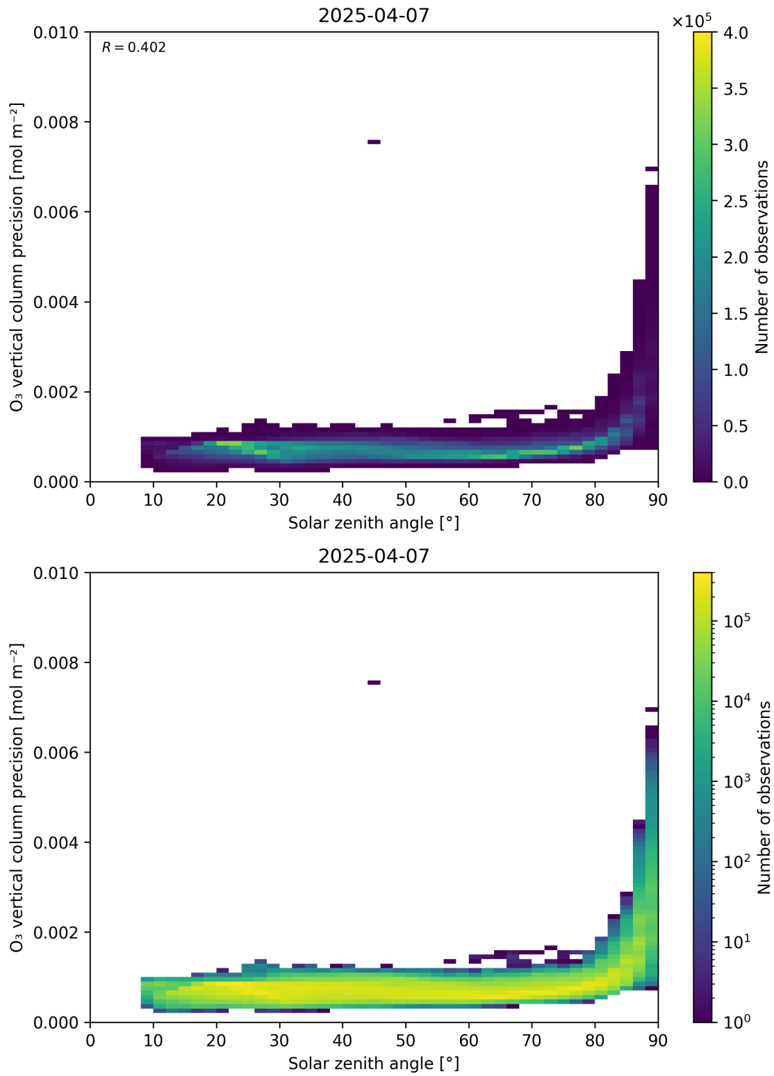
Figure 48: Scatter density plot of “Solar zenith angle” against “O 3 vertical column precision” for 2025-04-06 to 2025-04-08.
