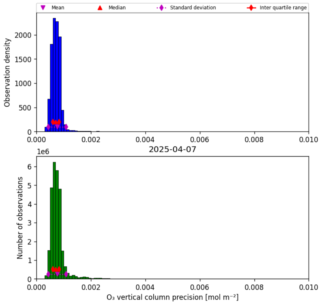
Figure 22: Histogram of “O 3 vertical column precision” for 2025-04-06 to 2025-04-08
