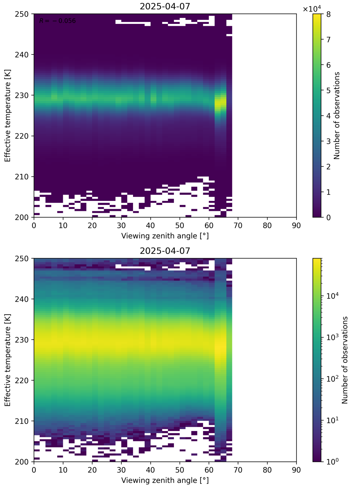
Figure 50: Scatter density plot of “Viewing zenith angle” against “Effective temperature” for 2025-04-06 to 2025-04-08.
