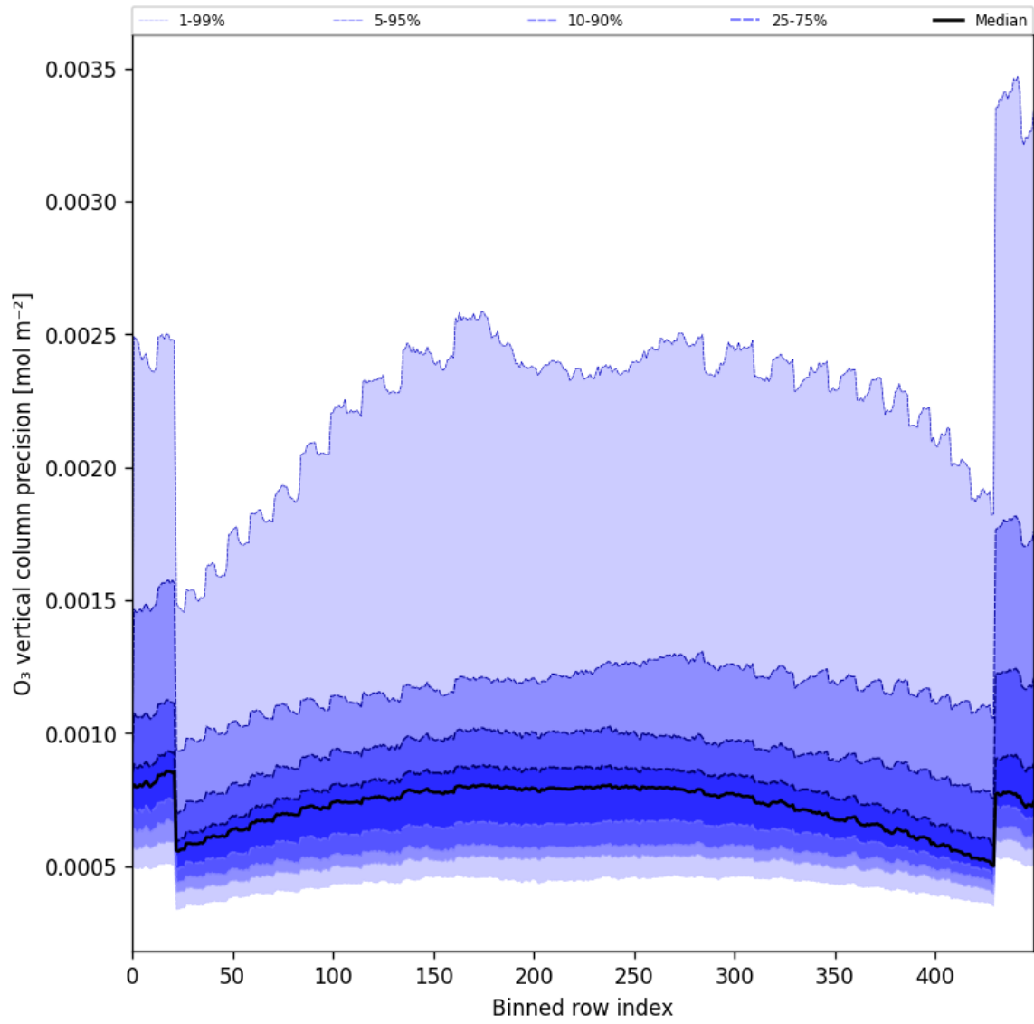
Figure 29: Along track statistics of “O 3 vertical column precision” for 2025-04-06 to 2025-04-08
