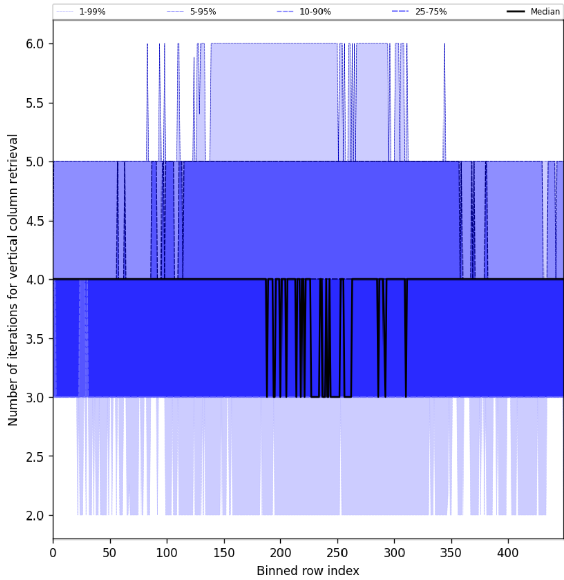
Figure 33: Along track statistics of “Number of iterations for vertical column retrieval” for 2025-04-06 to 2025-04-08
