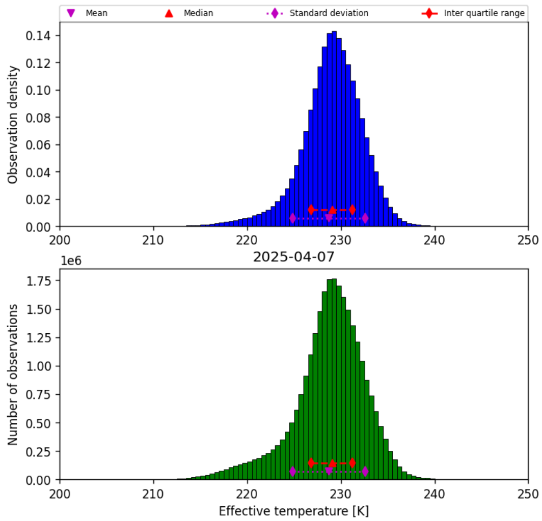
Figure 24: Histogram of “Effective temperature” for 2025-04-06 to 2025-04-08
