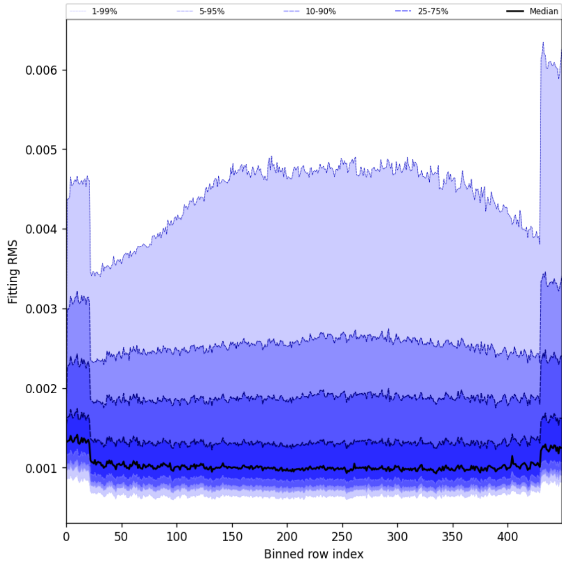
Figure 30: Along track statistics of “Fitting RMS” for 2025-04-06 to 2025-04-08
