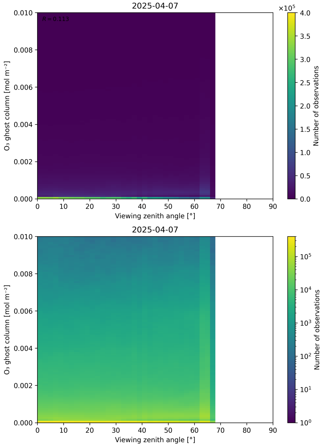
Figure 51: Scatter density plot of “Viewing zenith angle” against “O 3 ghost column” for 2025-04-06 to 2025-04-08.
