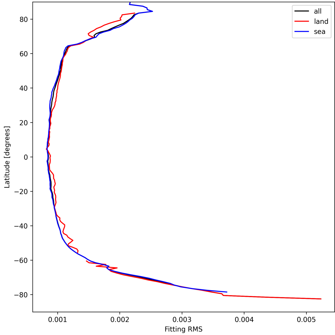
Figure 16: Zonal average of “Fitting RMS” for 2025-04-06 to 2025-04-08.
