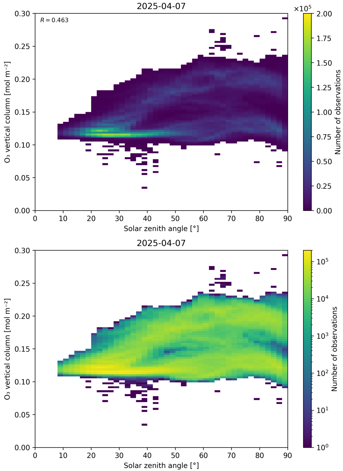
Figure 47: Scatter density plot of “Solar zenith angle” against “O 3 vertical column” for 2025-04-06 to 2025-04-08.
