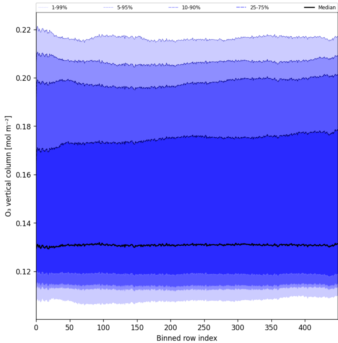
Figure 28: Along track statistics of “O 3 vertical column” for 2025-04-06 to 2025-04-08
