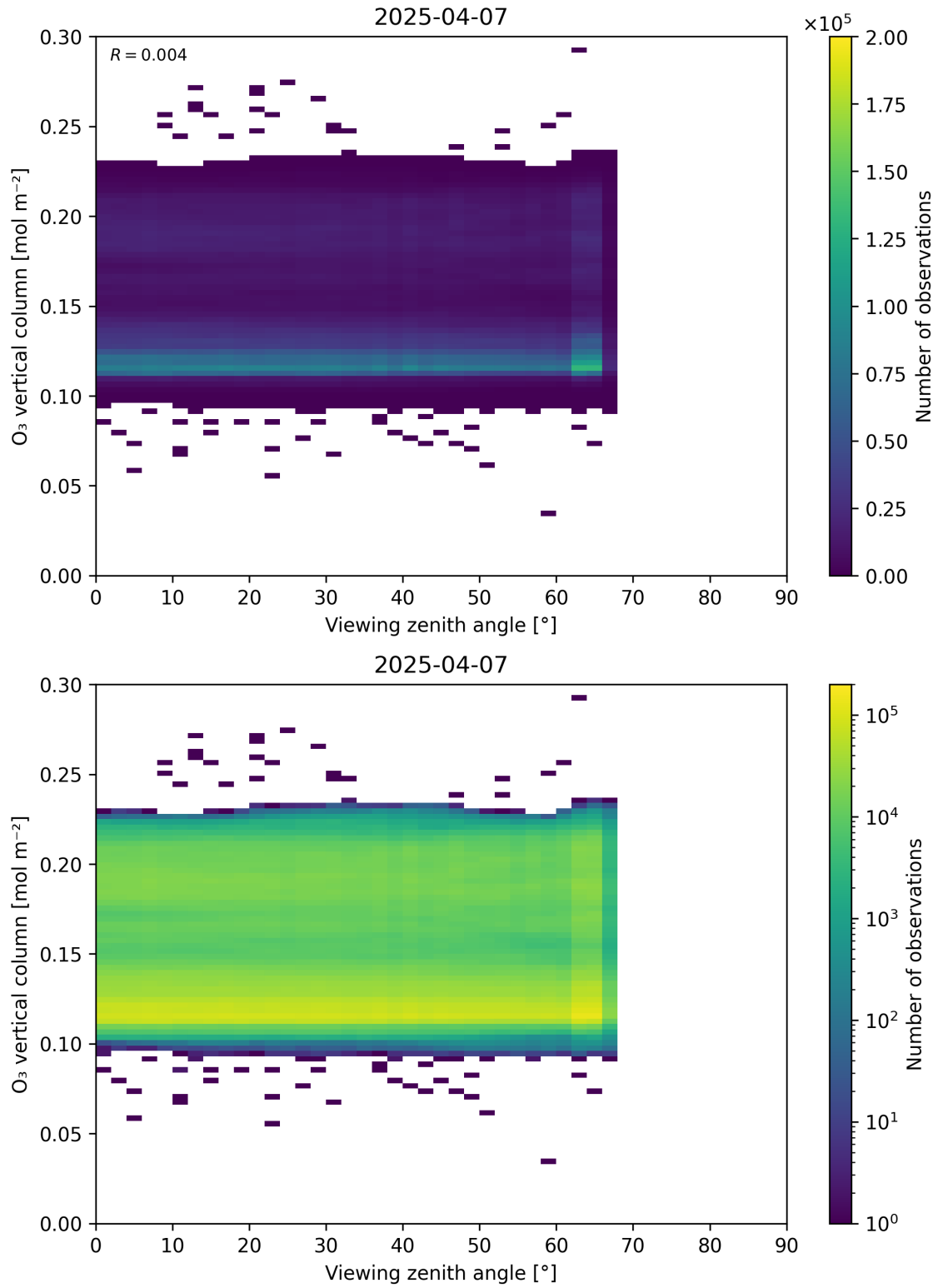
Figure 52: Scatter density plot of “Viewing zenith angle” against “O 3 vertical column” for 2025-04-06 to 2025-04-08.
