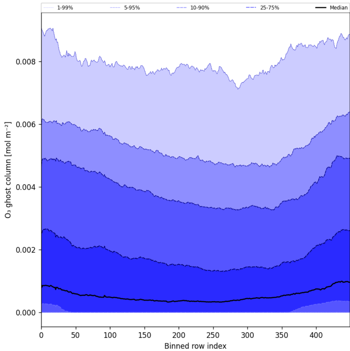
Figure 32: Along track statistics of “O 3 ghost column” for 2025-04-06 to 2025-04-08
