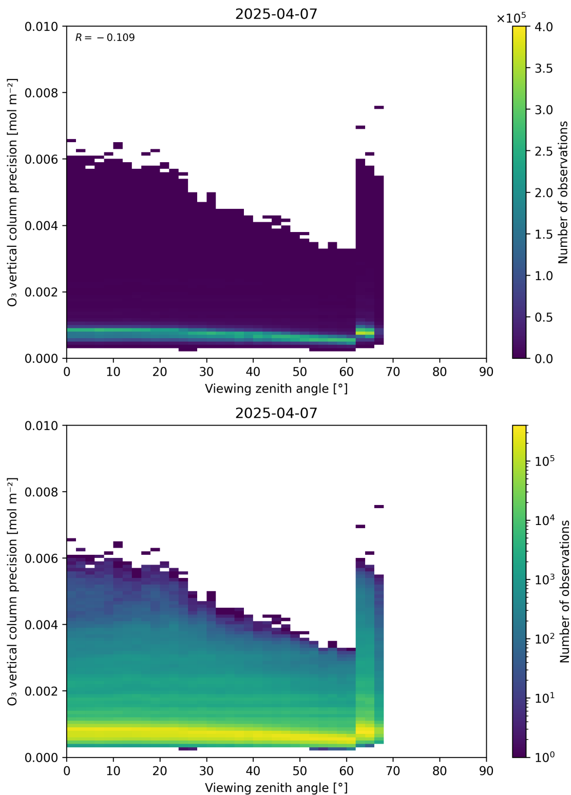
Figure 53: Scatter density plot of “Viewing zenith angle” against “O 3 vertical column precision” for 2025-04-06 to 2025-04-08.
