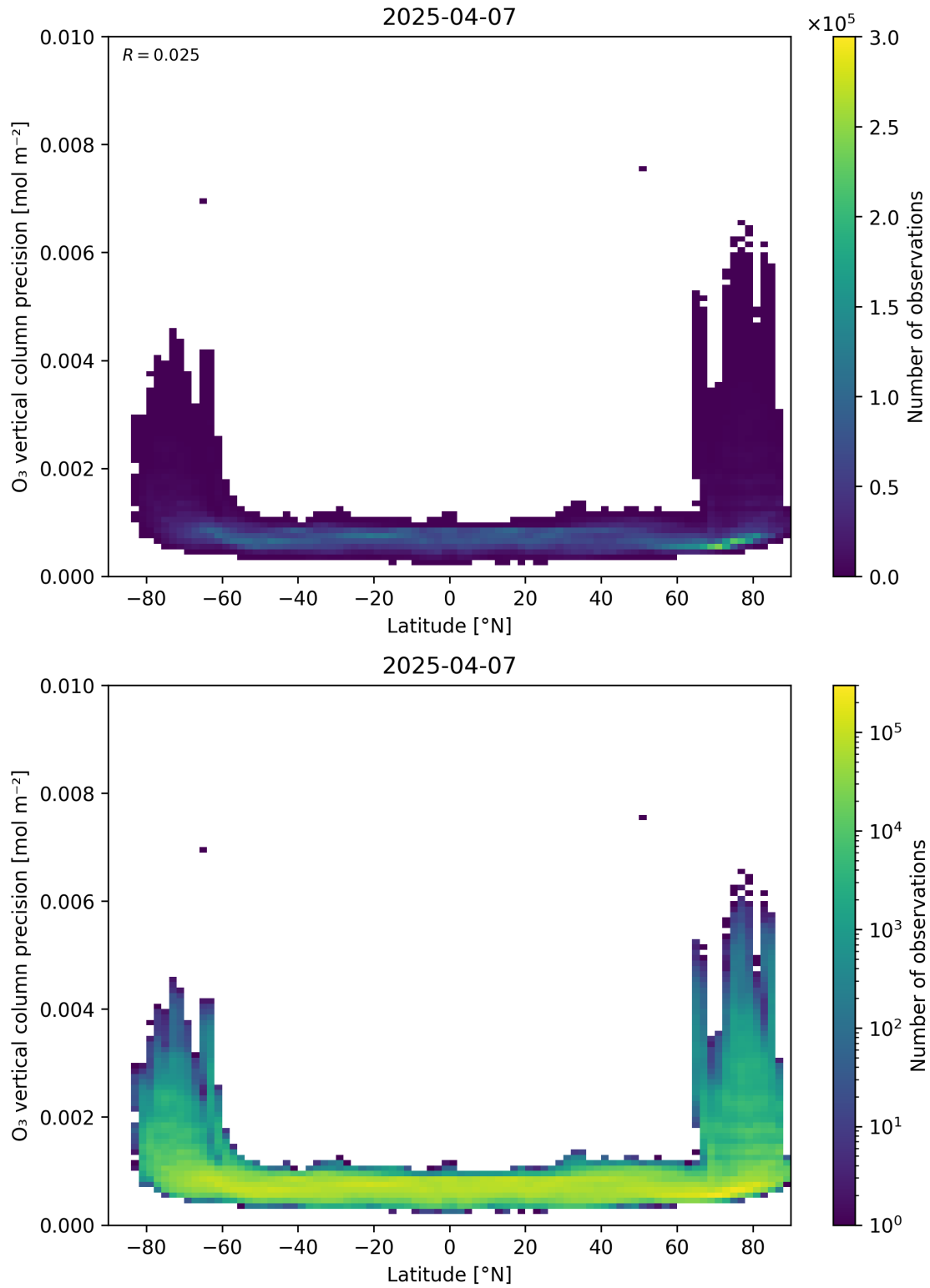
Figure 37: Scatter density plot of “Latitude” against “O 3 vertical column precision” for 2025-04-06 to 2025-04-08.
