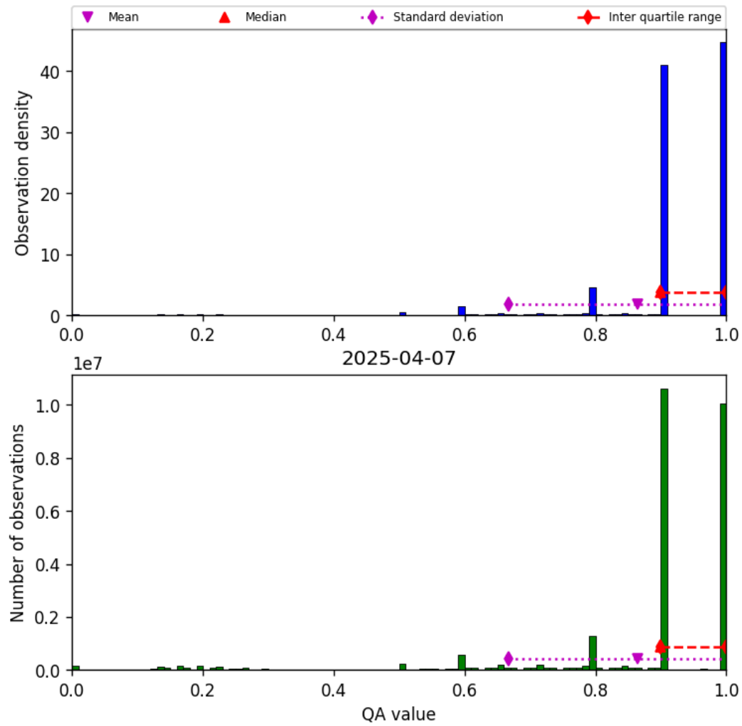
Figure 20: Histogram of “QA value” for 2025-04-06 to 2025-04-08
