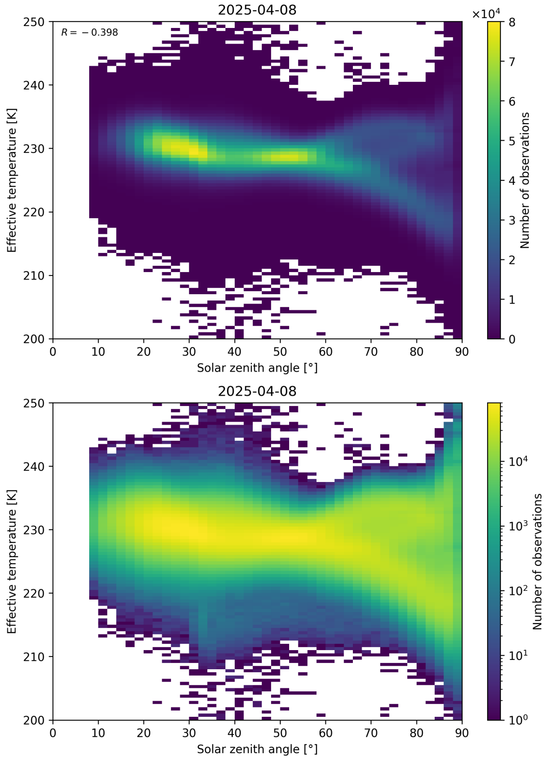
Figure 45: Scatter density plot of “Solar zenith angle” against “Effective temperature” for 2025-04-08 to 2025-04-09.
