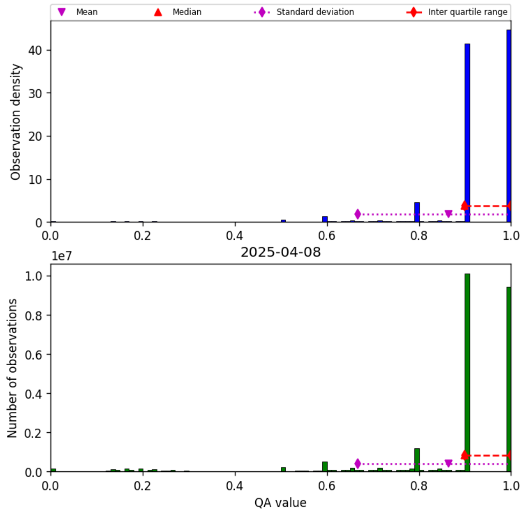
Figure 20: Histogram of “QA value” for 2025-04-08 to 2025-04-09
