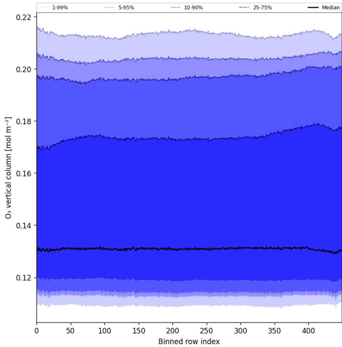
Figure 28: Along track statistics of “O 3 vertical column” for 2025-04-08 to 2025-04-09
