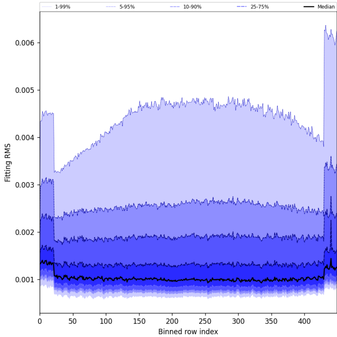
Figure 30: Along track statistics of “Fitting RMS” for 2025-04-08 to 2025-04-09
