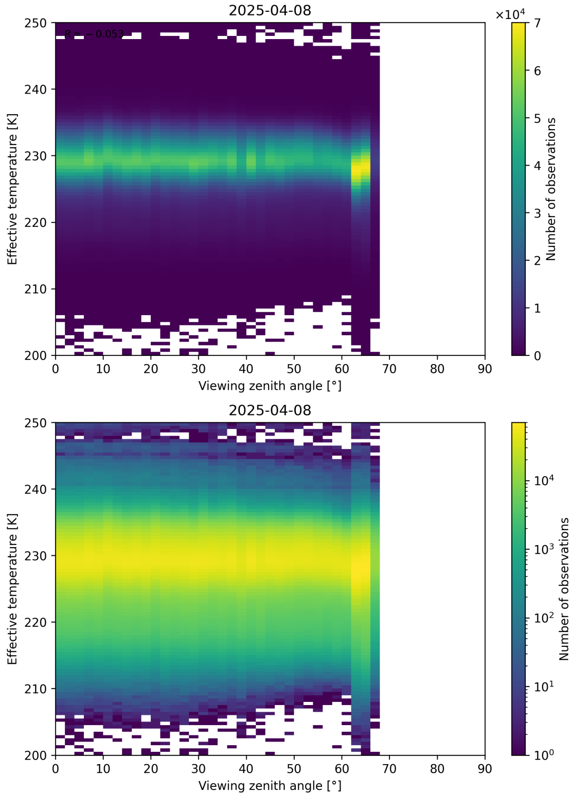
Figure 50: Scatter density plot of “Viewing zenith angle” against “Effective temperature” for 2025-04-08 to 2025-04-09.
