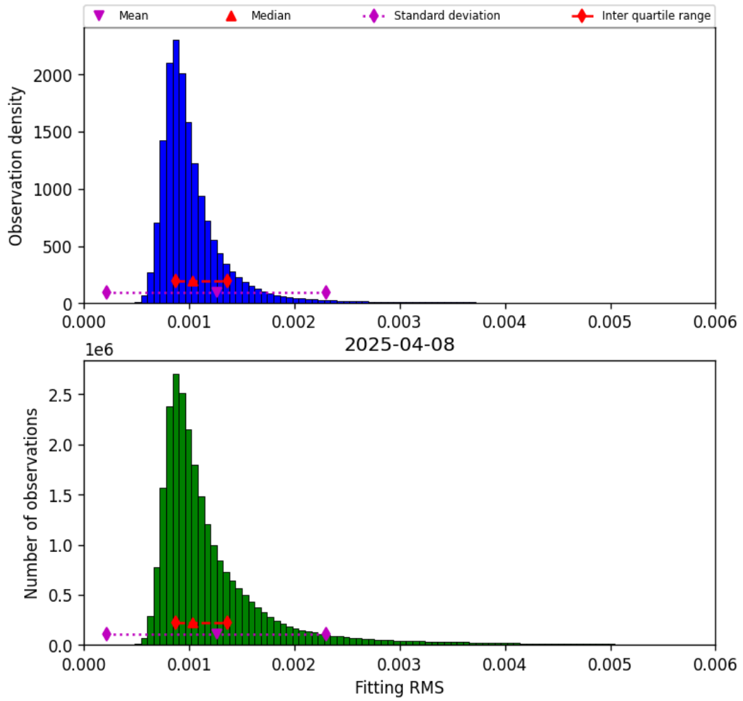
Figure 23: Histogram of “Fitting RMS” for 2025-04-08 to 2025-04-09
