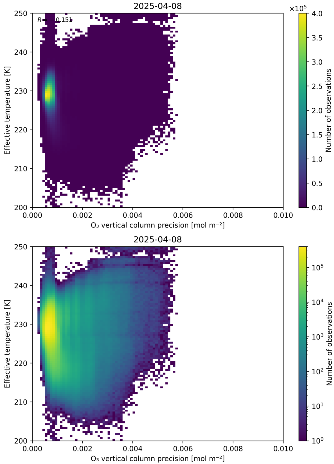
Figure 42: Scatter density plot of “O 3 vertical column precision” against “Effective temperature” for 2025-04-08 to 2025-04-09.
