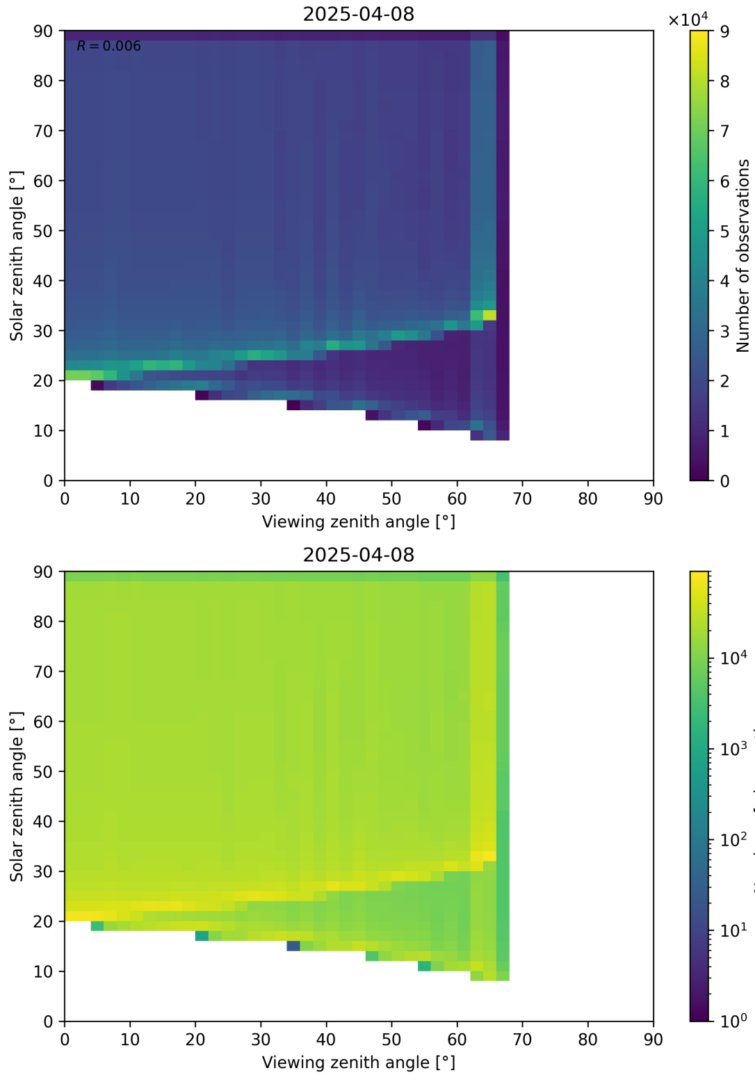
Figure 54: Scatter density plot of “Viewing zenith angle” against “Solar zenith angle” for 2025-04-08 to 2025-04-09.
