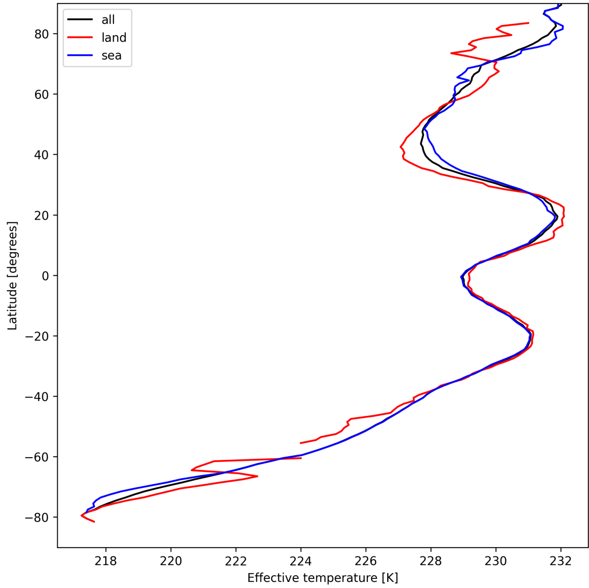
Figure 17: Zonal average of "Effective temperature" for 2025-04-08 to 2025-04-09.
