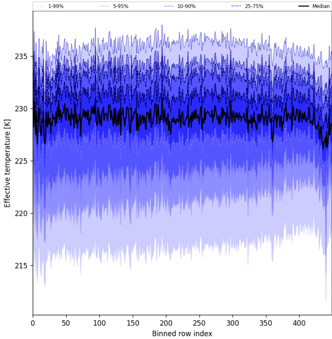
Figure 31: Along track statistics of “Effective temperature” for 2025-04-08 to 2025-04-09
