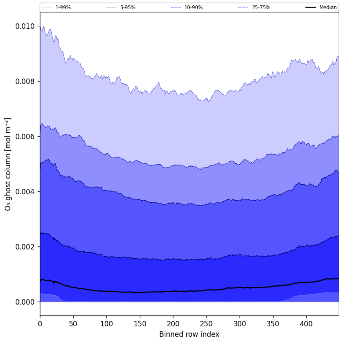
Figure 32: Along track statistics of “O 3 ghost column” for 2025-04-08 to 2025-04-09
