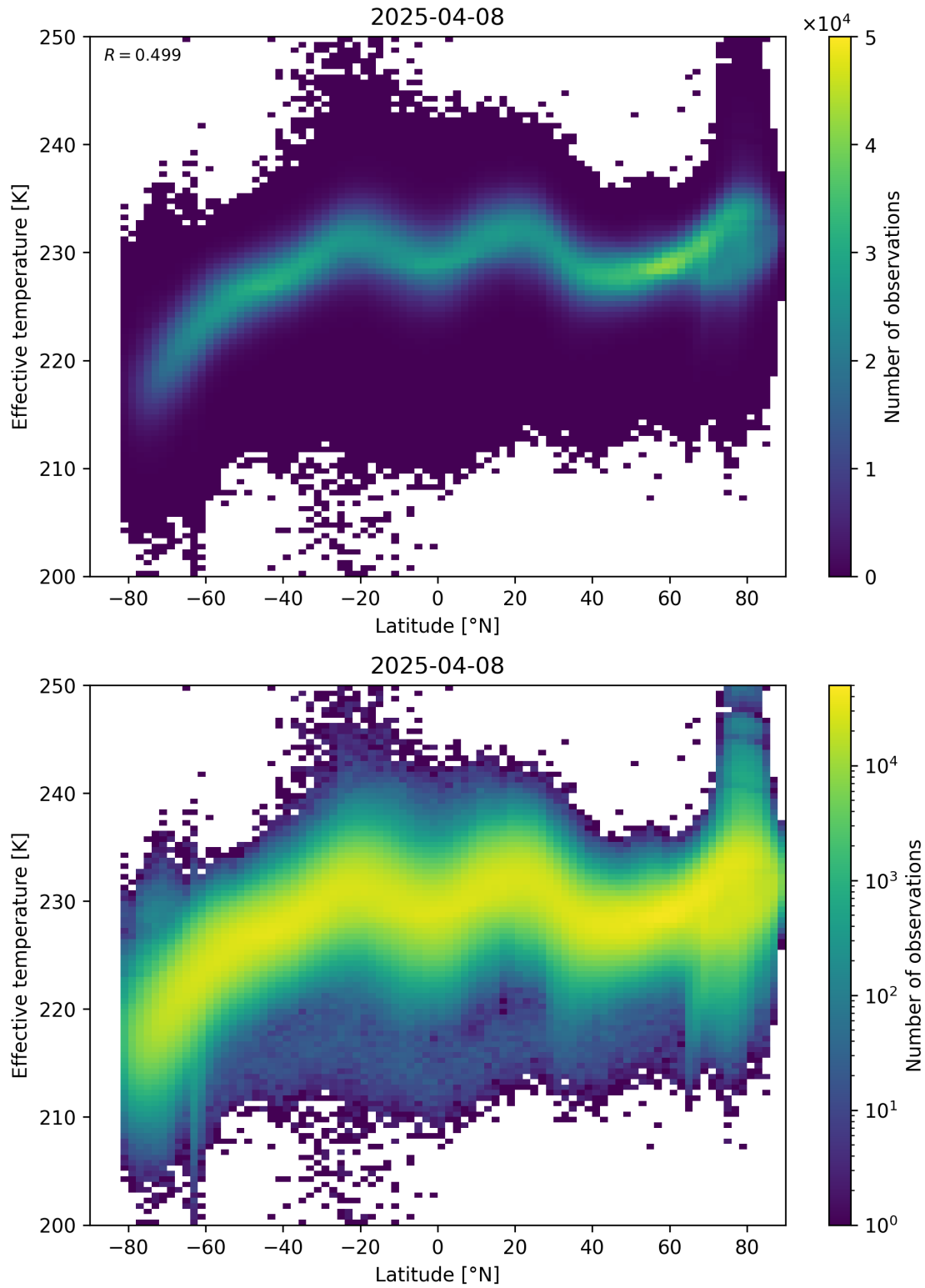
Figure 34: Scatter density plot of “Latitude” against “Effective temperature” for 2025-04-08 to 2025-04-09.
