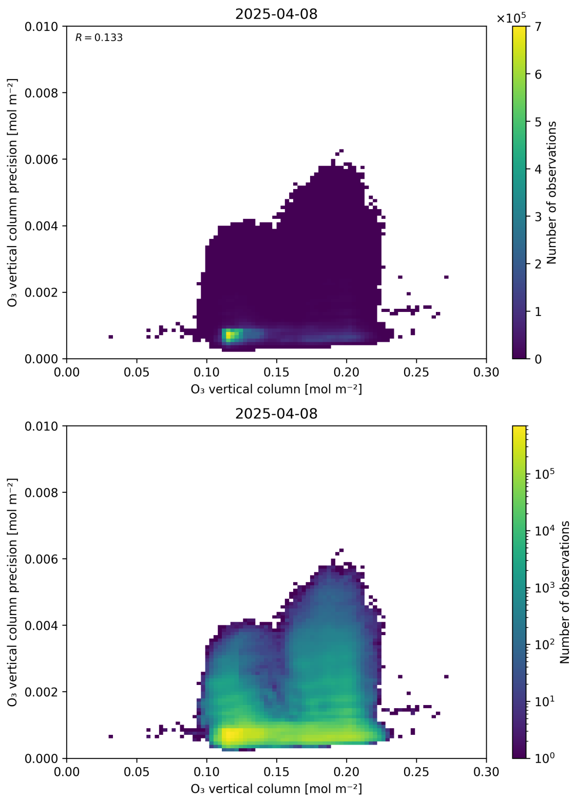
Figure 41: Scatter density plot of “O 3 vertical column” against “O 3 vertical column precision” for 2025-04-08 to 2025-04-09.
