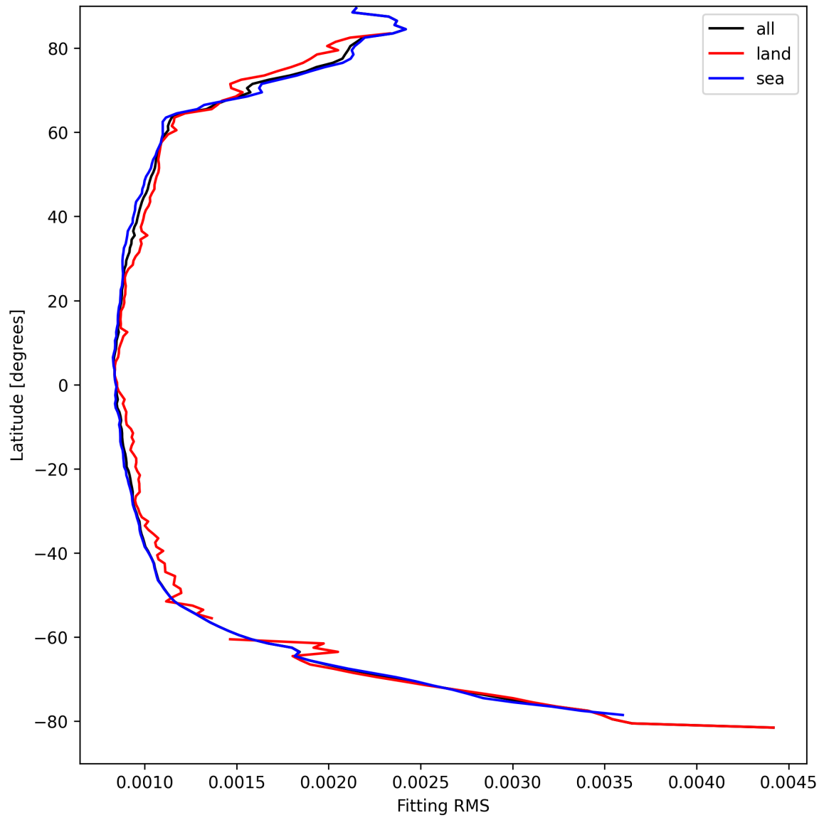
Figure 16: Zonal average of “Fitting RMS” for 2025-04-08 to 2025-04-09.
