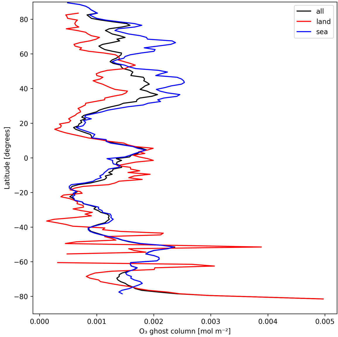
Figure 18: Zonal average of "O 3 ghost column" for 2025-04-08 to 2025-04-09.
