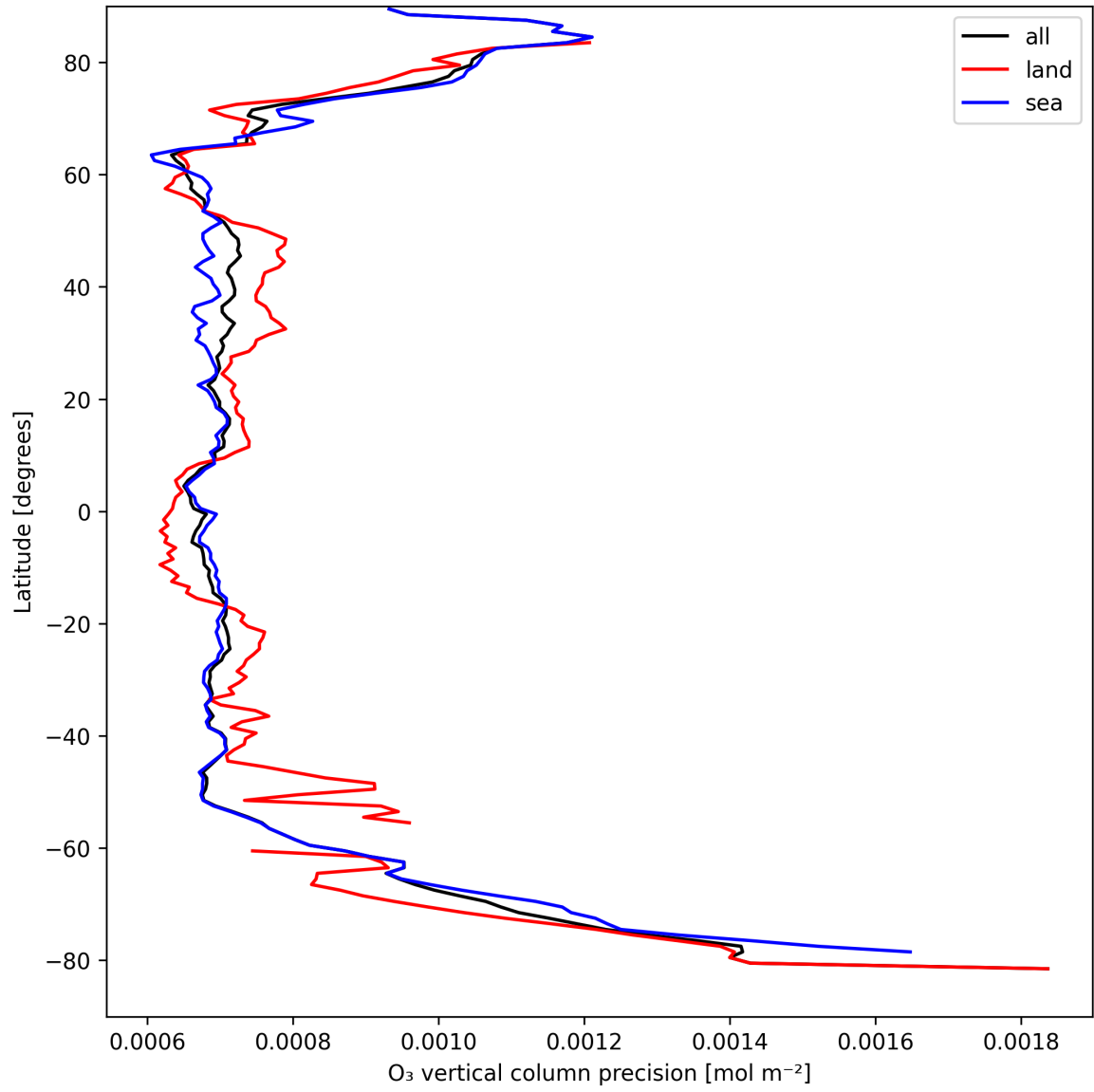
Figure 15: Zonal average of "O 3 vertical column precision" for 2025-04-08 to 2025-04-09.
