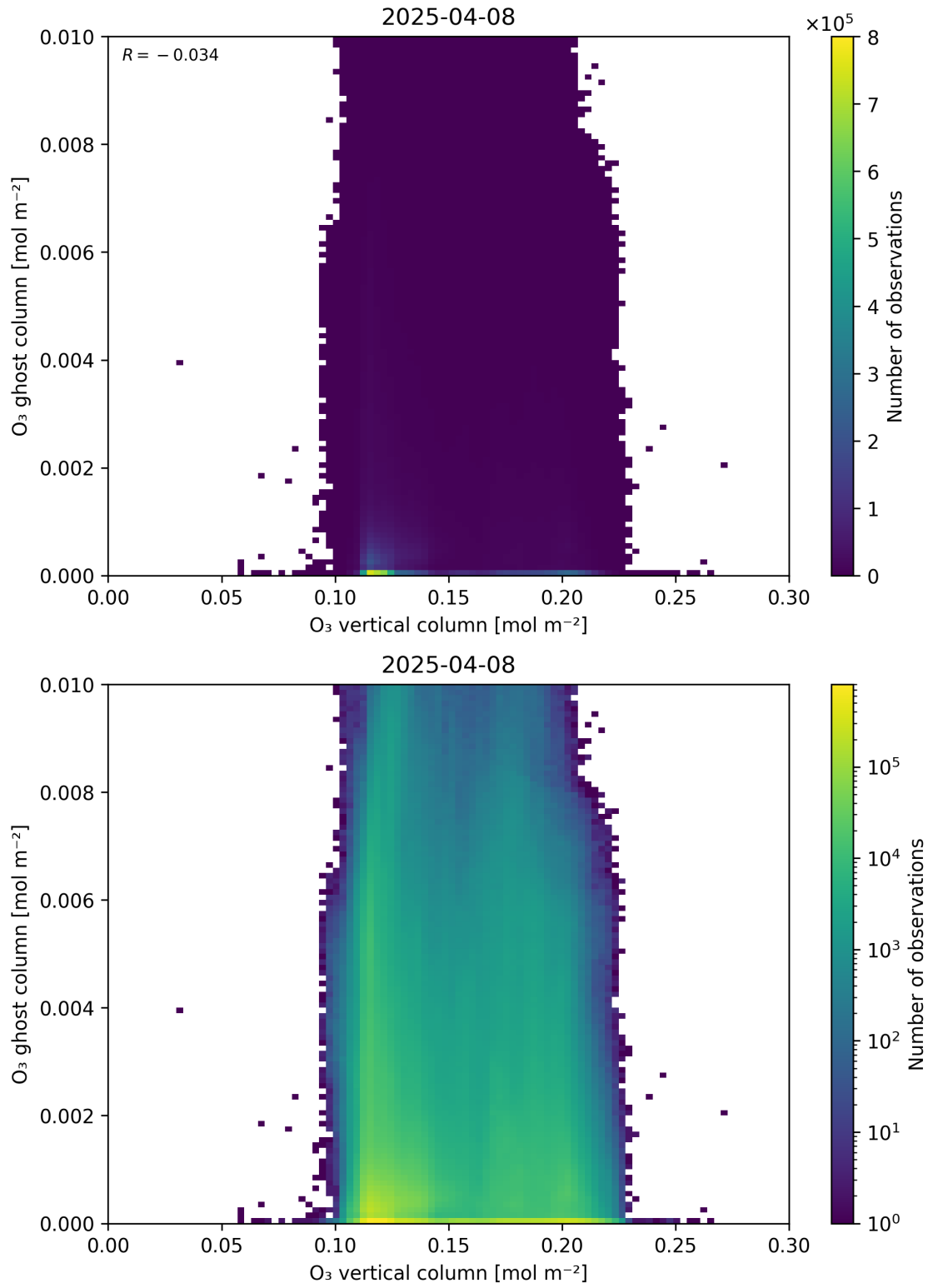
Figure 40: Scatter density plot of “O 3 vertical column” against “O 3 ghost column” for 2025-04-08 to 2025-04-09.
