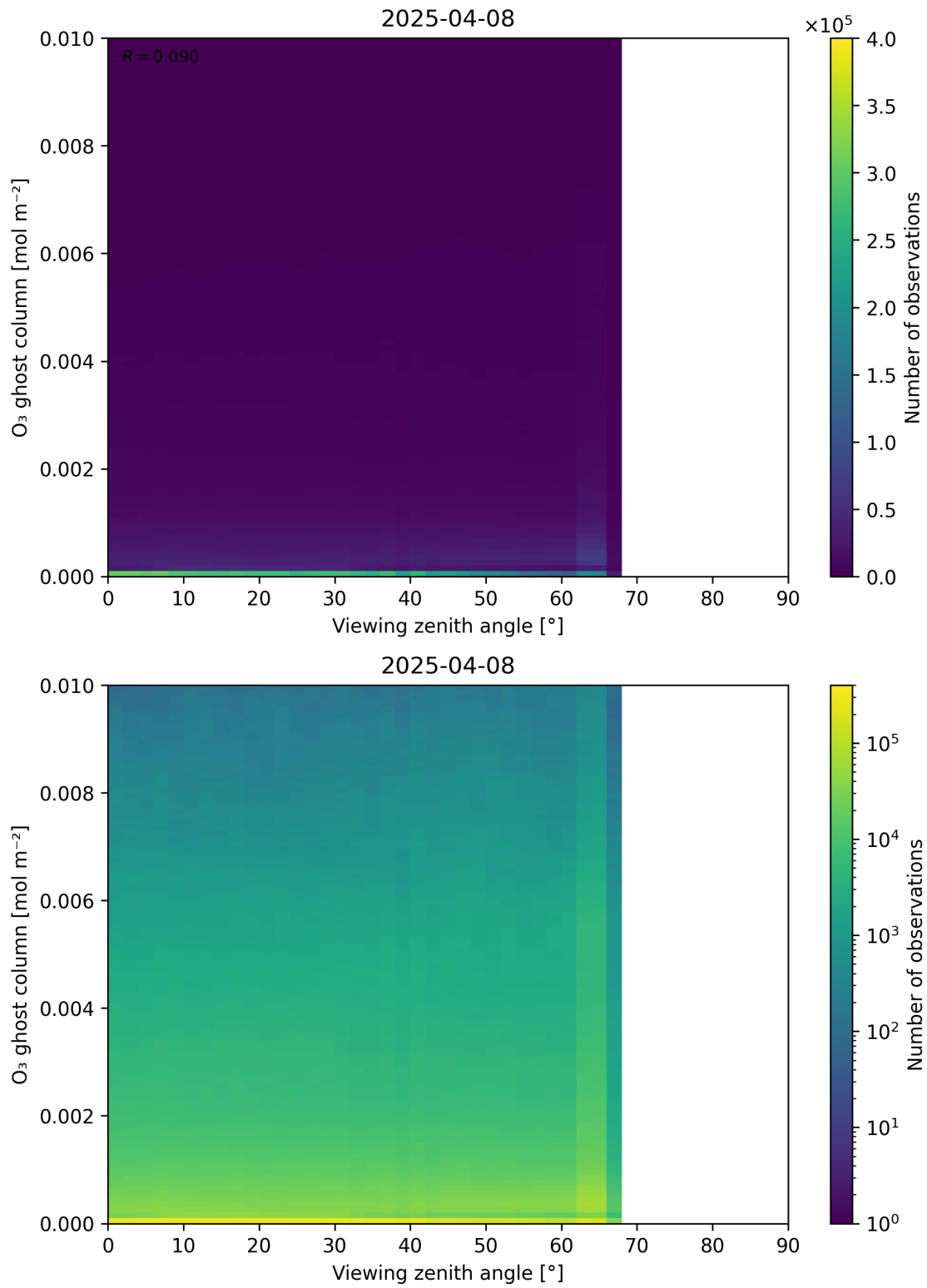
Figure 51: Scatter density plot of “Viewing zenith angle” against “O 3 ghost column” for 2025-04-08 to 2025-04-09.
