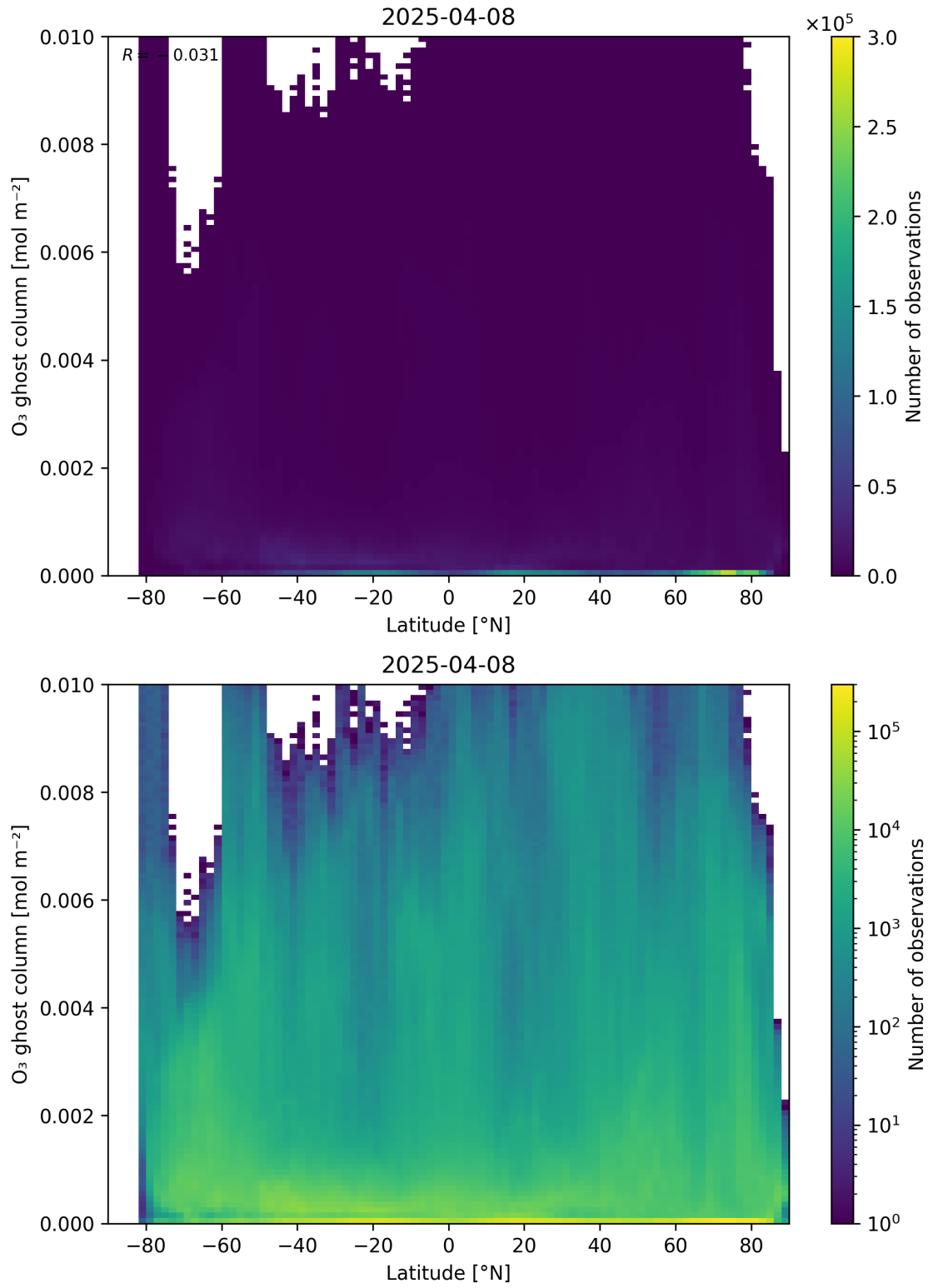
Figure 35: Scatter density plot of “Latitude” against “O 3 ghost column” for 2025-04-08 to 2025-04-09.
