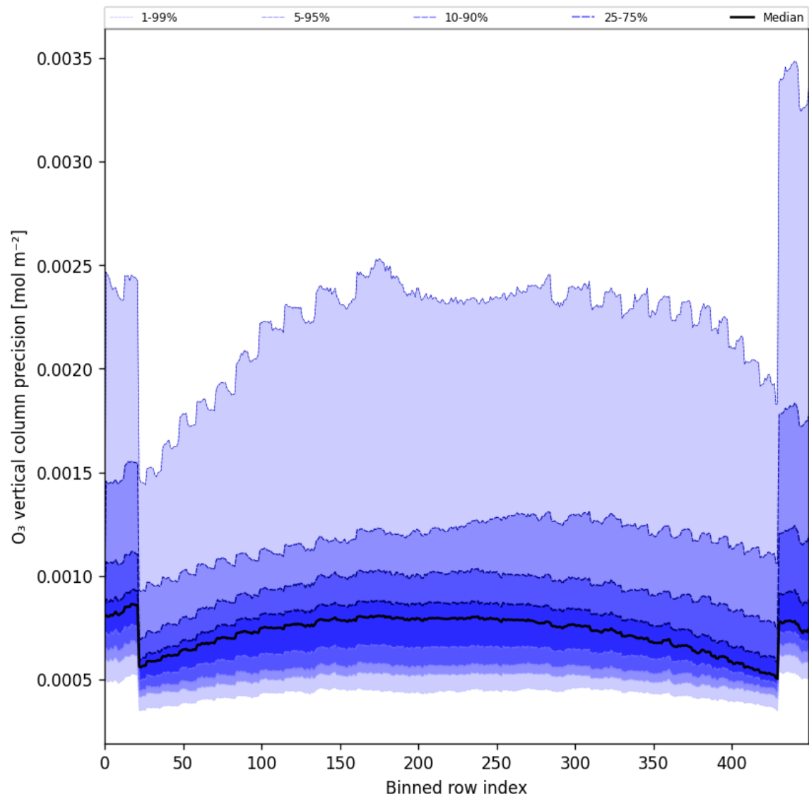
Figure 29: Along track statistics of “O 3 vertical column precision” for 2025-04-08 to 2025-04-09
