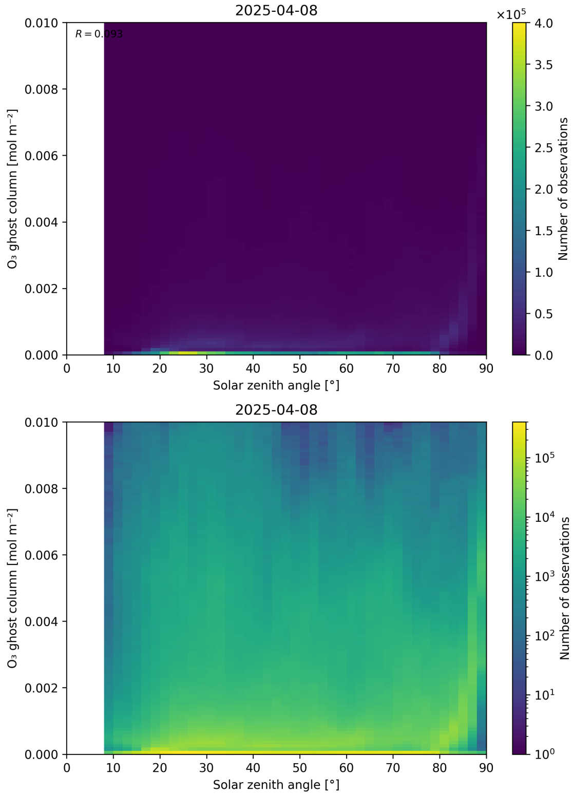
Figure 46: Scatter density plot of “Solar zenith angle” against “O 3 ghost column” for 2025-04-08 to 2025-04-09.
