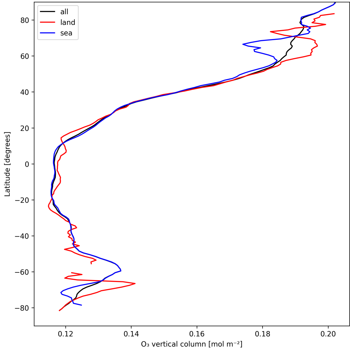
Figure 14: Zonal average of “O 3 vertical column” for 2025-04-08 to 2025-04-09.
