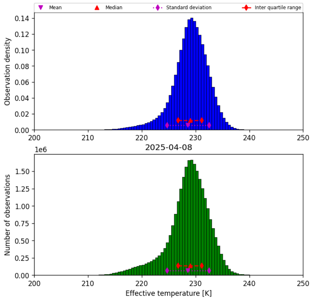
Figure 24: Histogram of “Effective temperature” for 2025-04-08 to 2025-04-09
