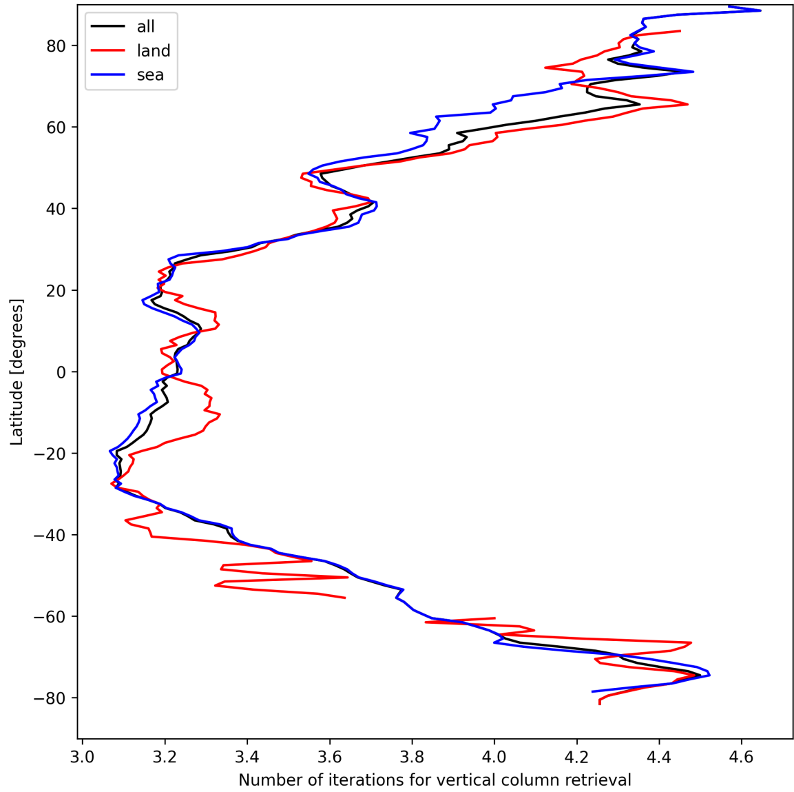
Figure 19: Zonal average of “Number of iterations for vertical column retrieval” for 2025-04-08 to 2025-04-09.
