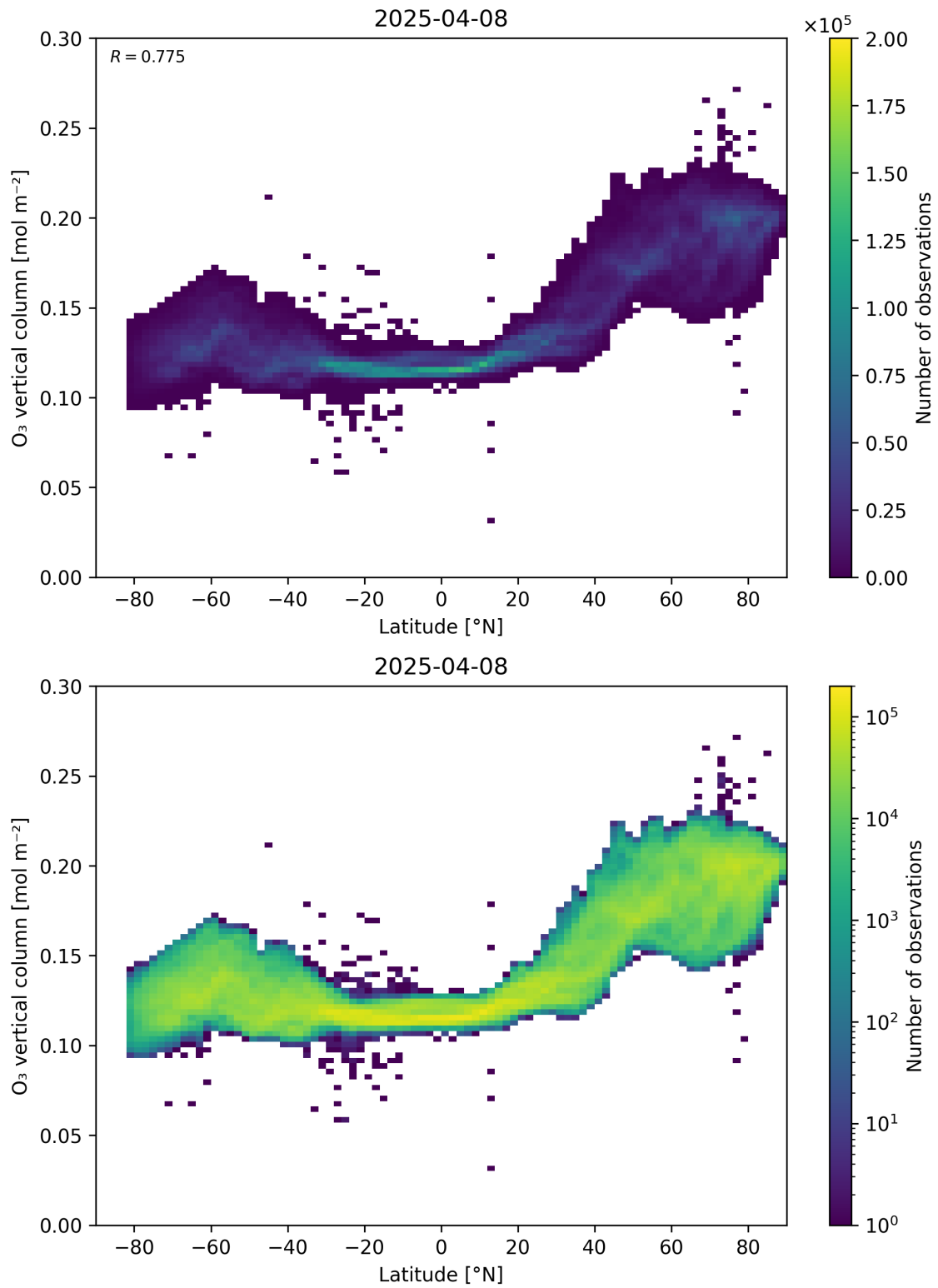
Figure 36: Scatter density plot of “Latitude” against “O 3 vertical column” for 2025-04-08 to 2025-04-09.
