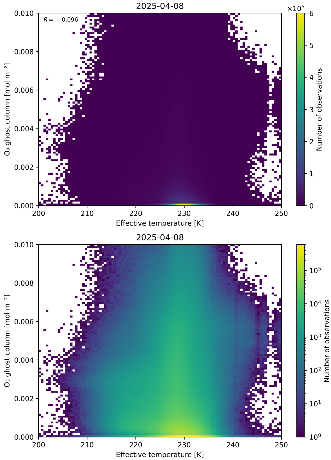
Figure 38: Scatter density plot of “Effective temperature” against “O 3 ghost column” for 2025-04-08 to 2025-04-09.
