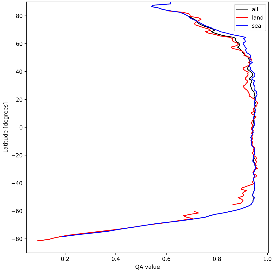
Figure 13: Zonal average of “QA value” for 2025-04-08 to 2025-04-09.
