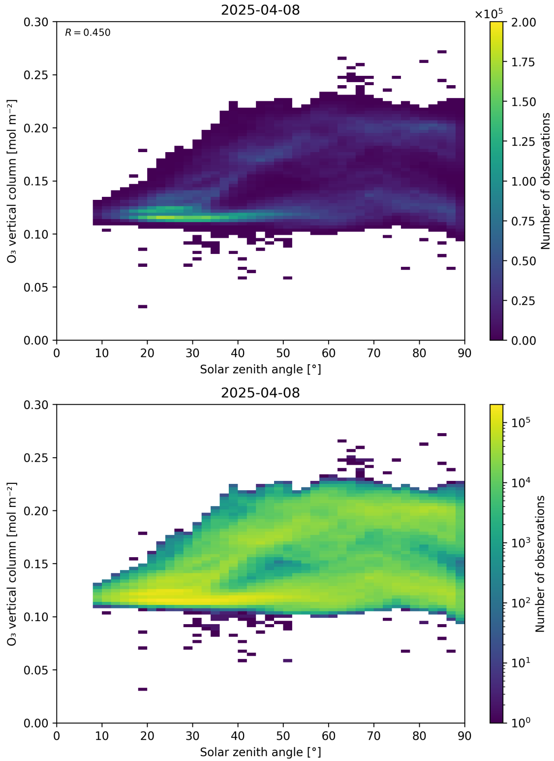
Figure 47: Scatter density plot of “Solar zenith angle” against “O 3 vertical column” for 2025-04-08 to 2025-04-09.
