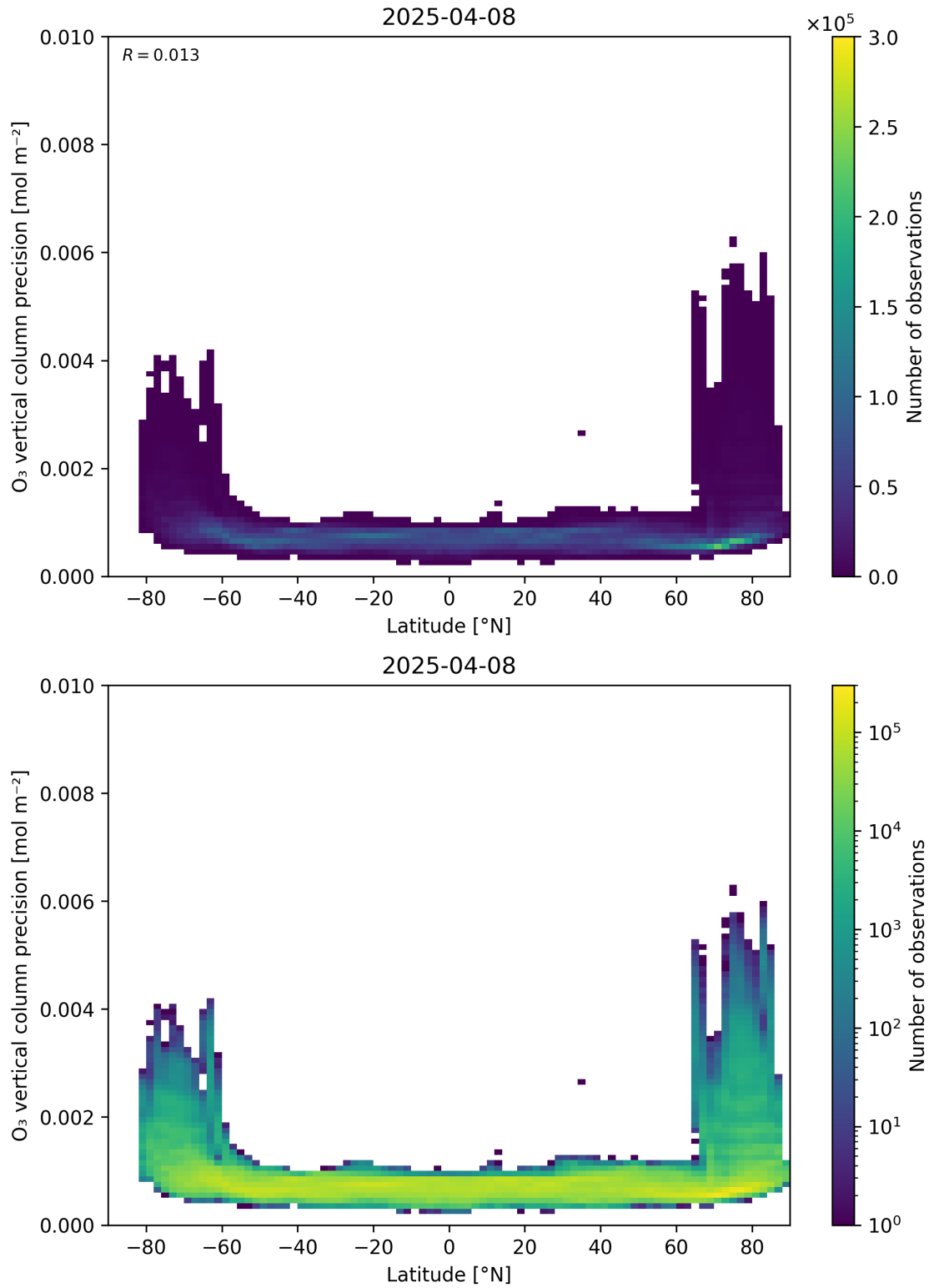
Figure 37: Scatter density plot of “Latitude” against “O 3 vertical column precision” for 2025-04-08 to 2025-04-09.
