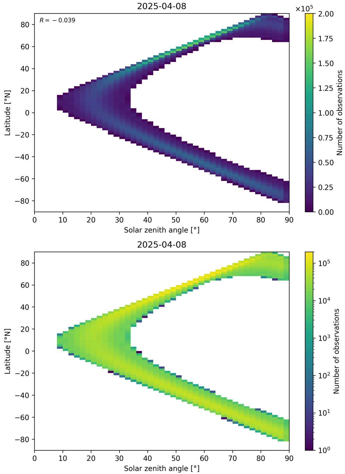
Figure 44: Scatter density plot of “Solar zenith angle” against “Latitude” for 2025-04-08 to 2025-04-09.
