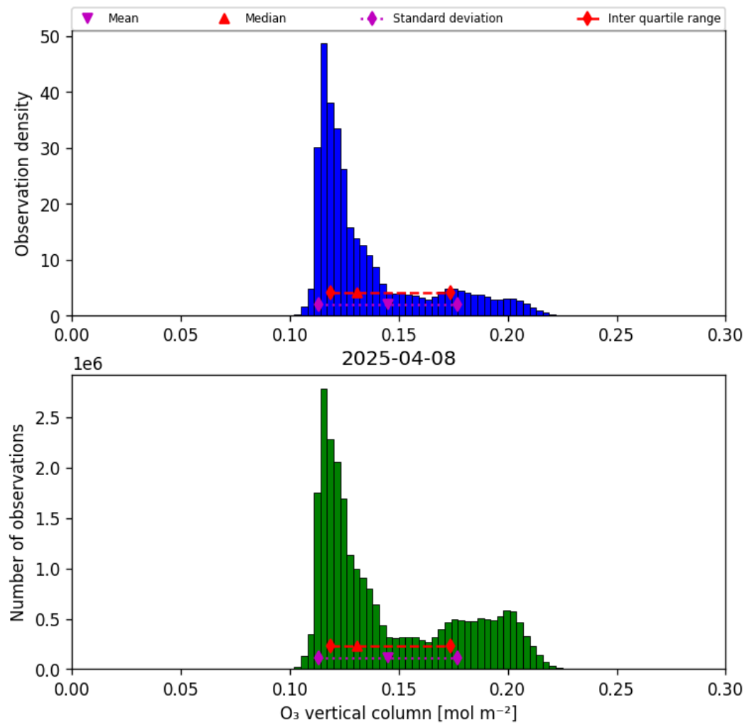
Figure 21: Histogram of “O 3 vertical column” for 2025-04-08 to 2025-04-09
