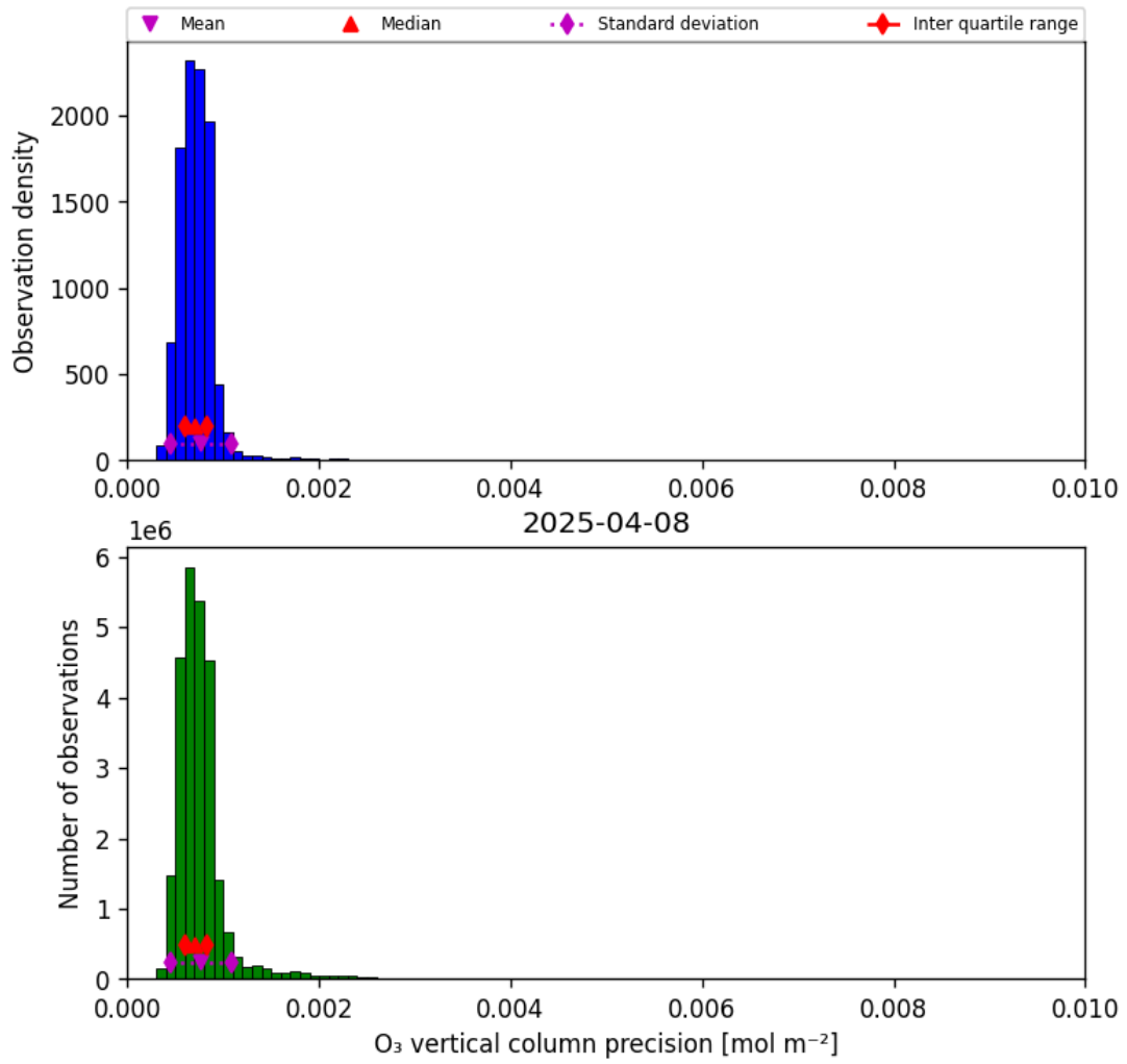
Figure 22: Histogram of “O 3 vertical column precision” for 2025-04-08 to 2025-04-09
