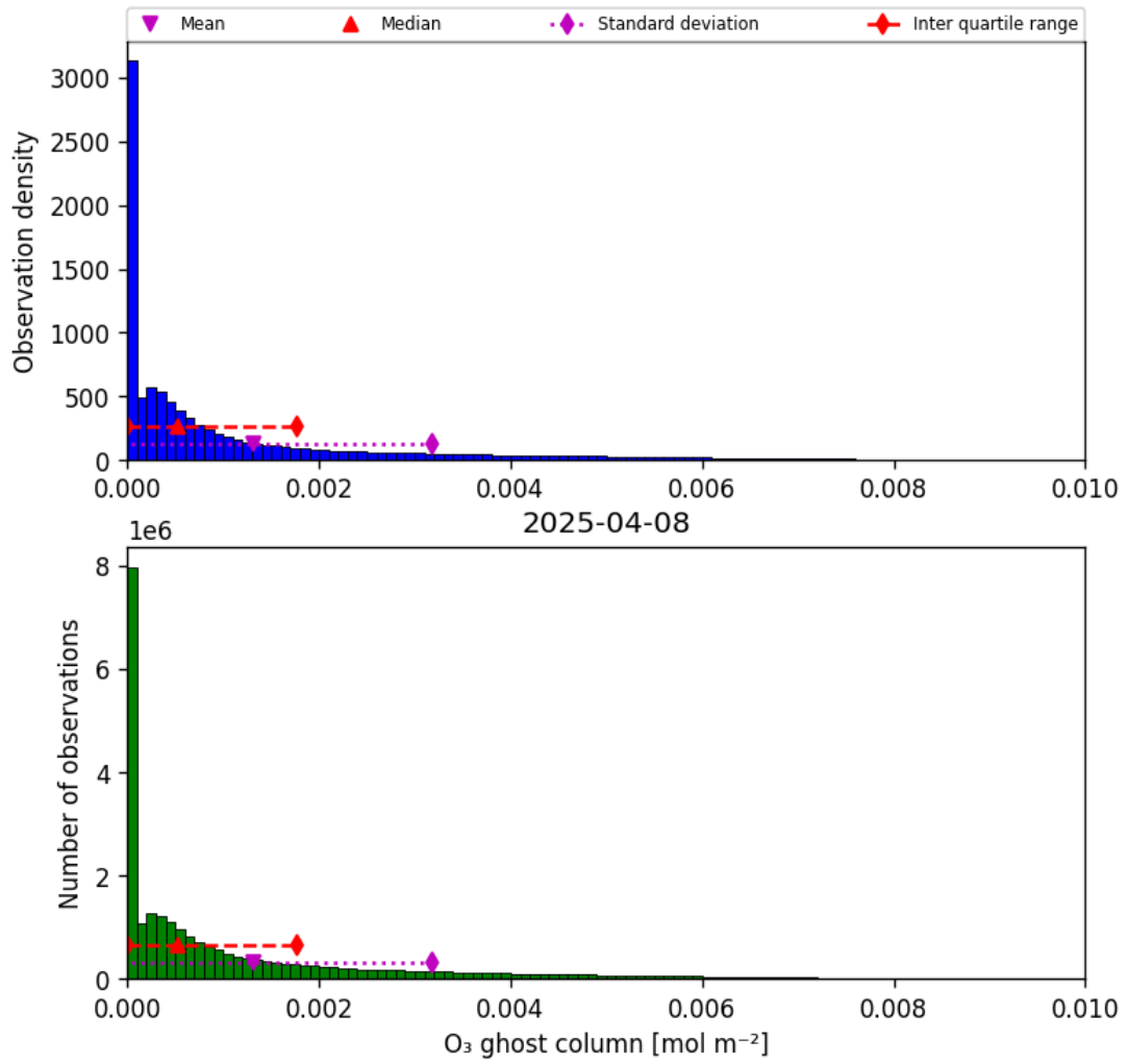
Figure 25: Histogram of “O 3 ghost column” for 2025-04-08 to 2025-04-09
