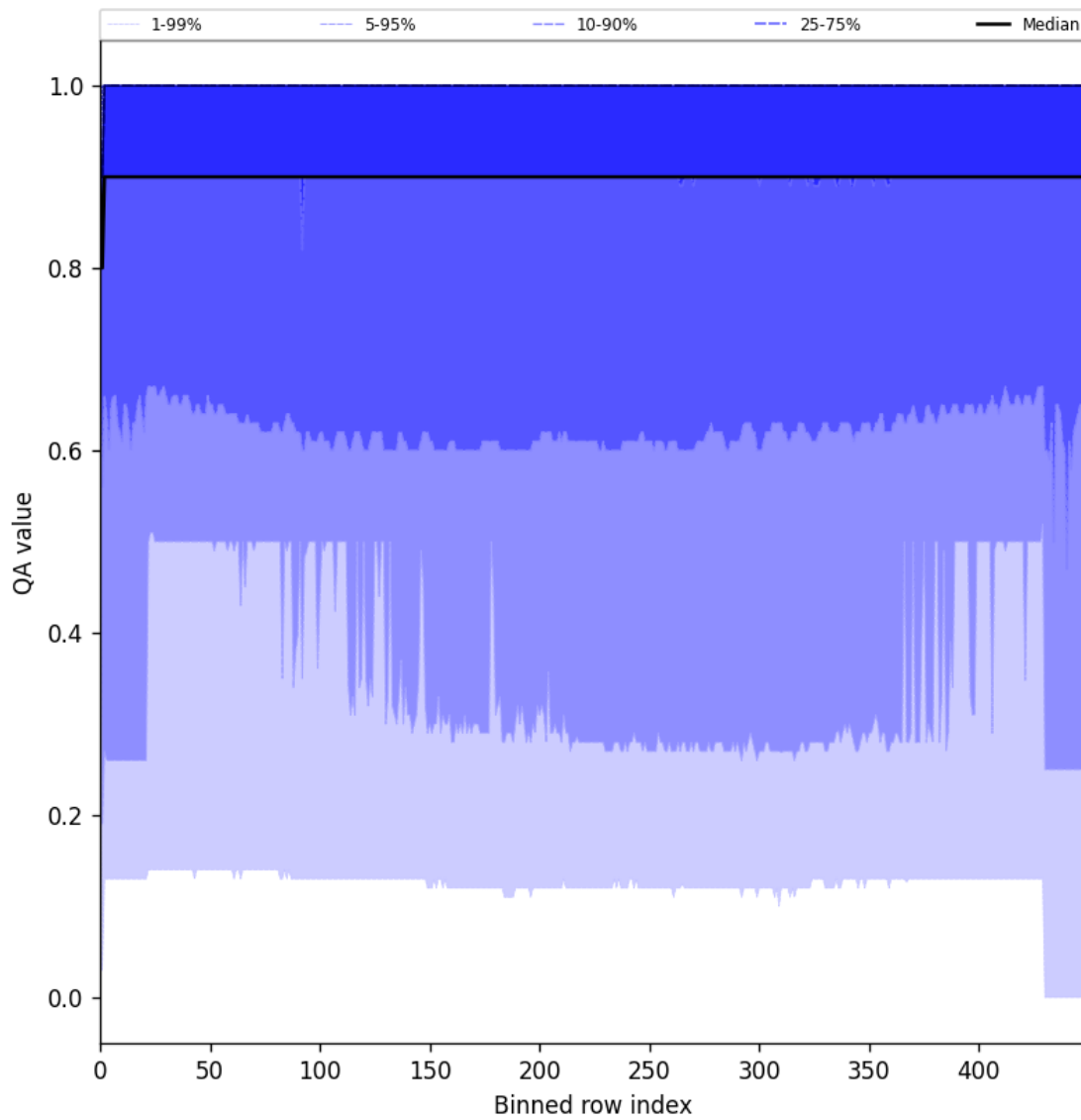
Figure 27: Along track statistics of “QA value” for 2025-04-08 to 2025-04-09
