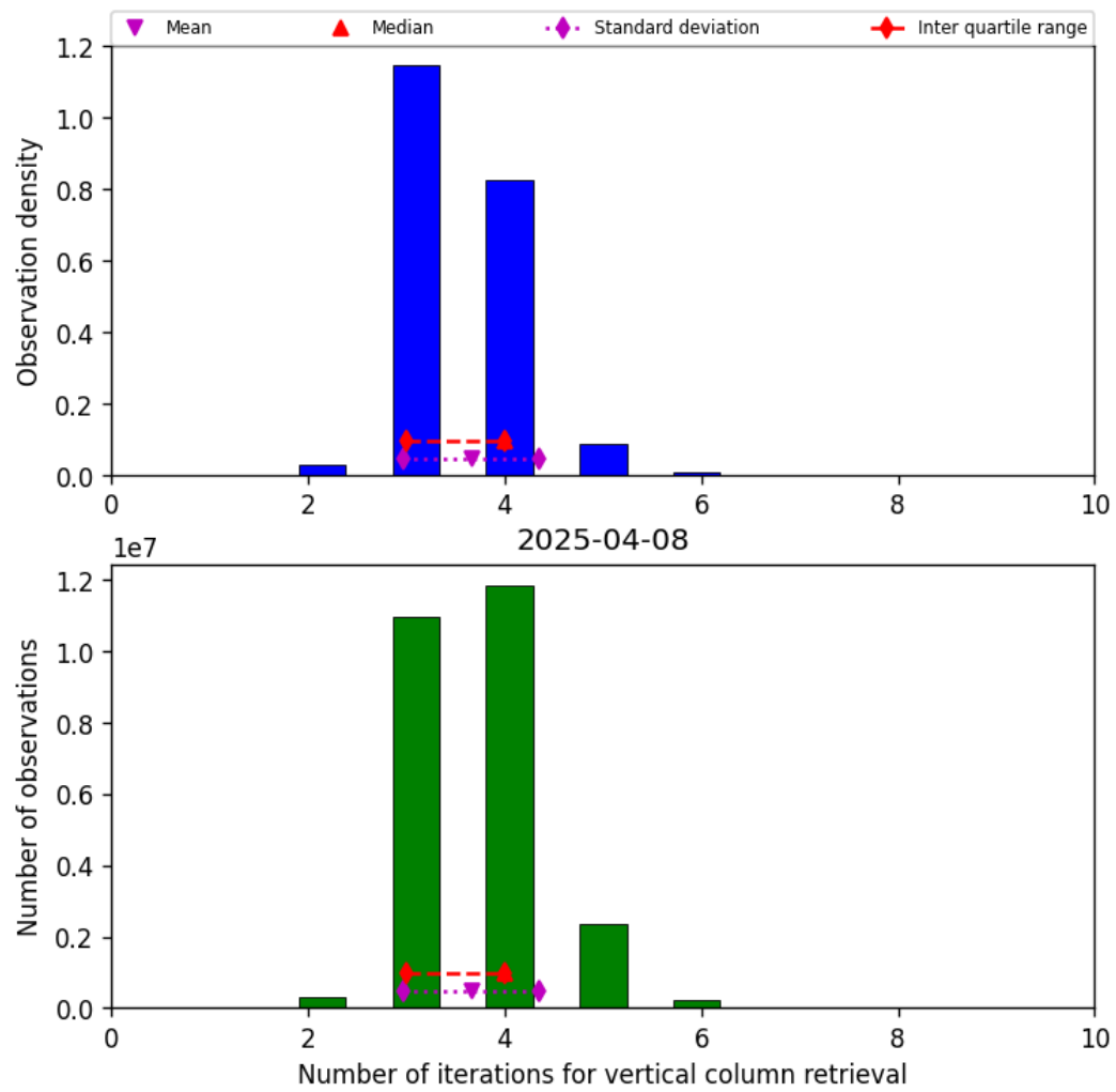
Figure 26: Histogram of “Number of iterations for vertical column retrieval” for 2025-04-08 to 2025-04-09
