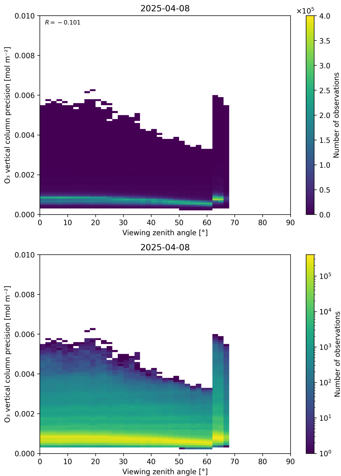
Figure 53: Scatter density plot of “Viewing zenith angle” against “O 3 vertical column precision” for 2025-04-08 to 2025-04-09.
