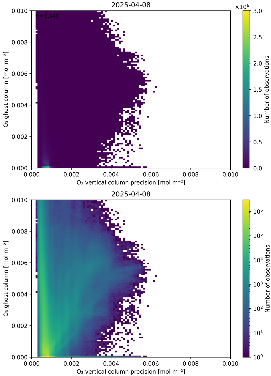
Figure 43: Scatter density plot of “O 3 vertical column precision” against “O 3 ghost column” for 2025-04-08 to 2025-04-09.
