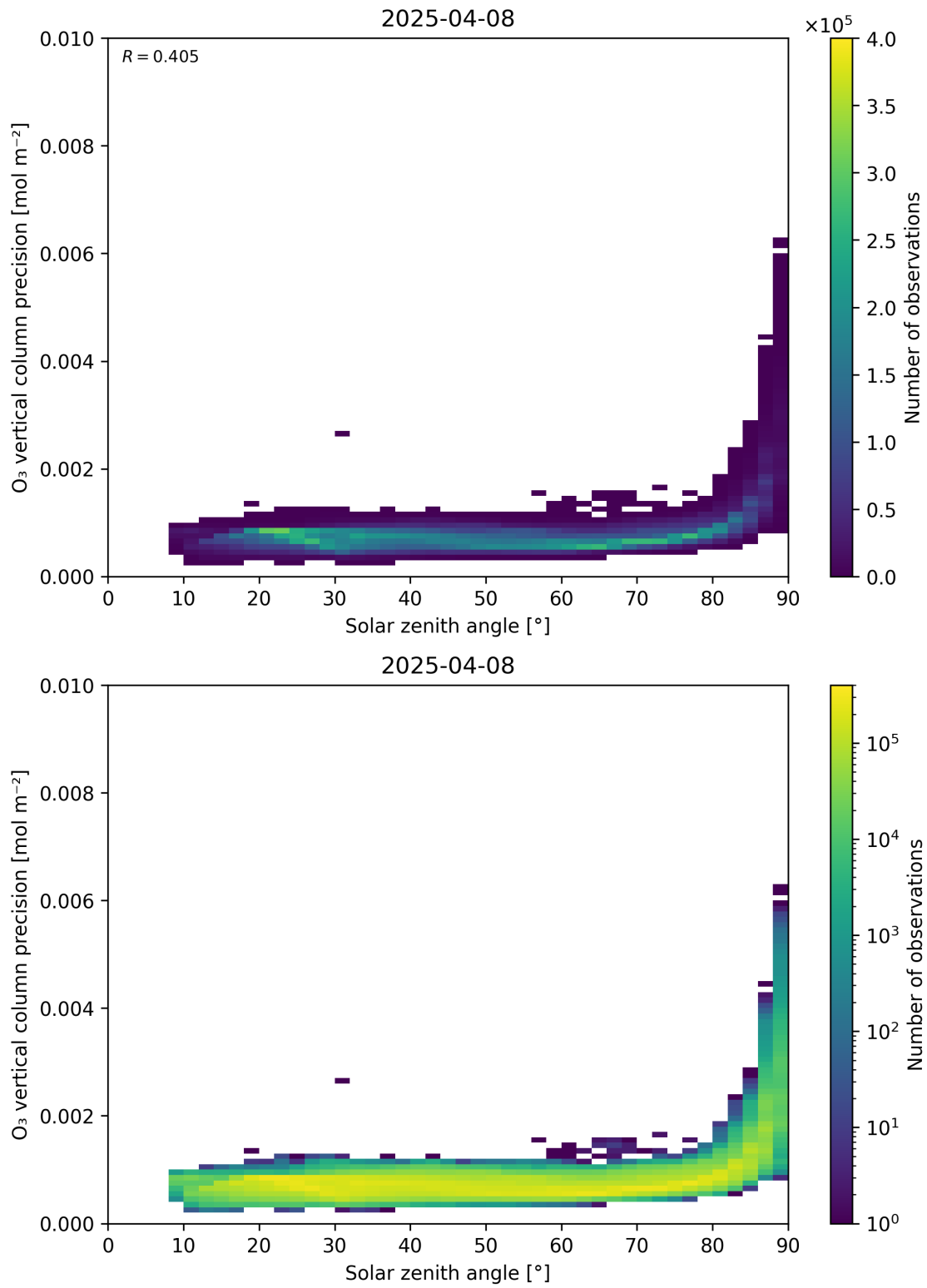
Figure 48: Scatter density plot of “Solar zenith angle” against “O 3 vertical column precision” for 2025-04-08 to 2025-04-09.
