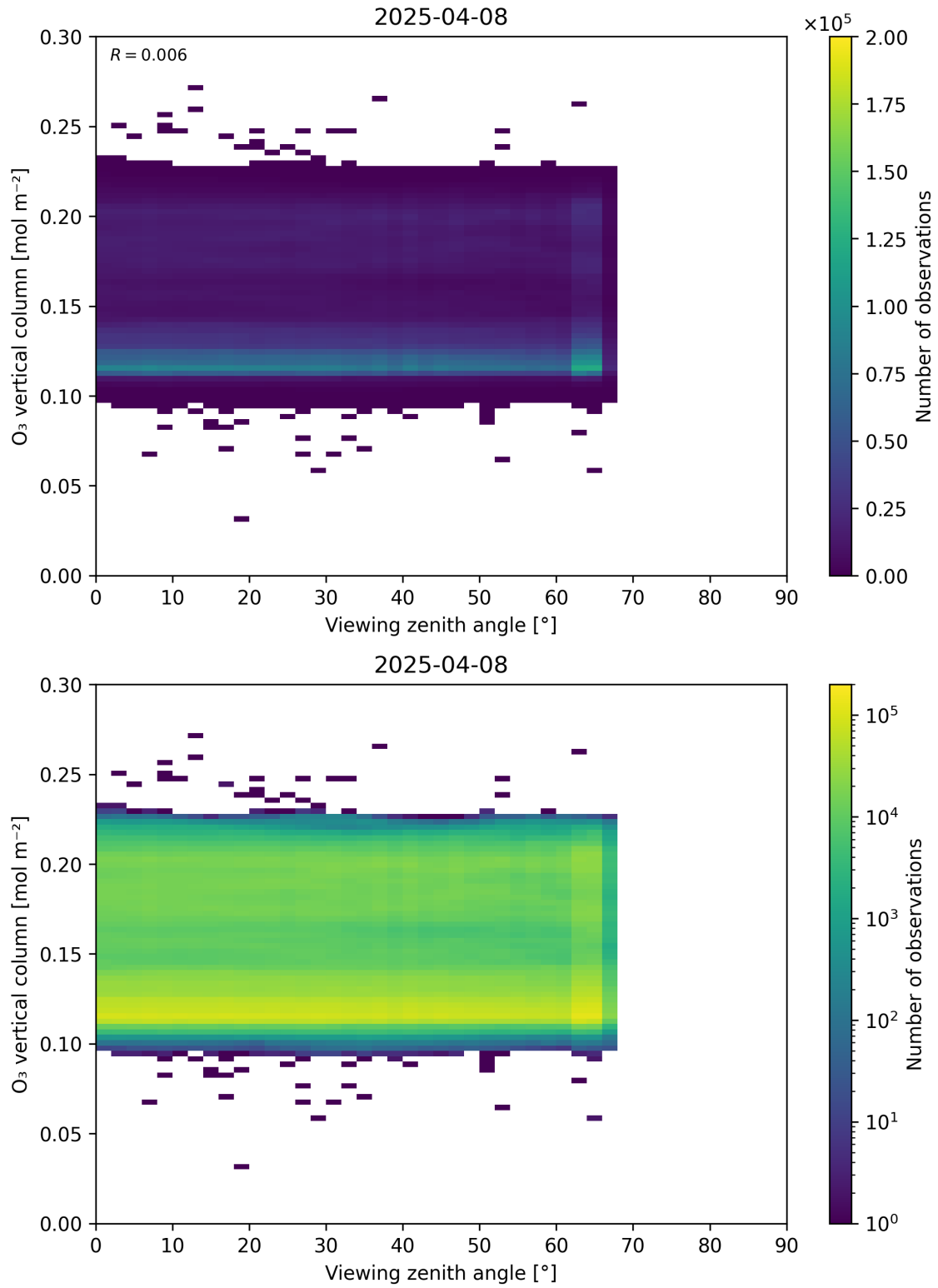
Figure 52: Scatter density plot of “Viewing zenith angle” against “O 3 vertical column” for 2025-04-08 to 2025-04-09.
