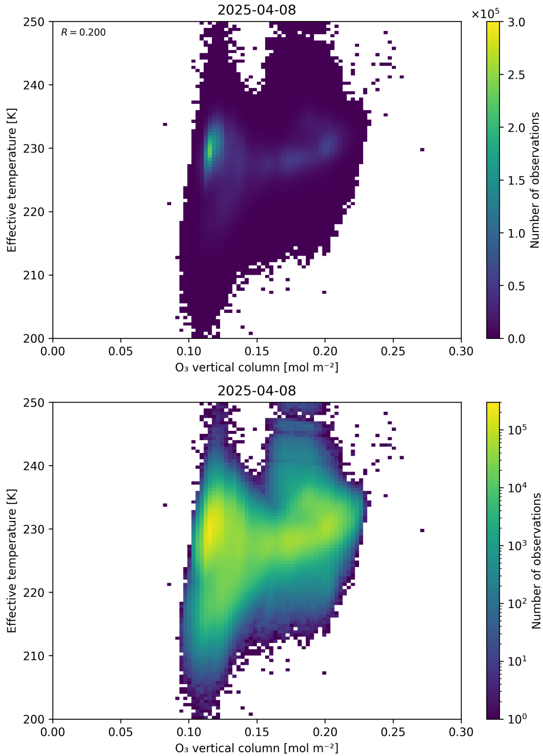
Figure 39: Scatter density plot of “O 3 vertical column” against “Effective temperature” for 2025-04-08 to 2025-04-09.
