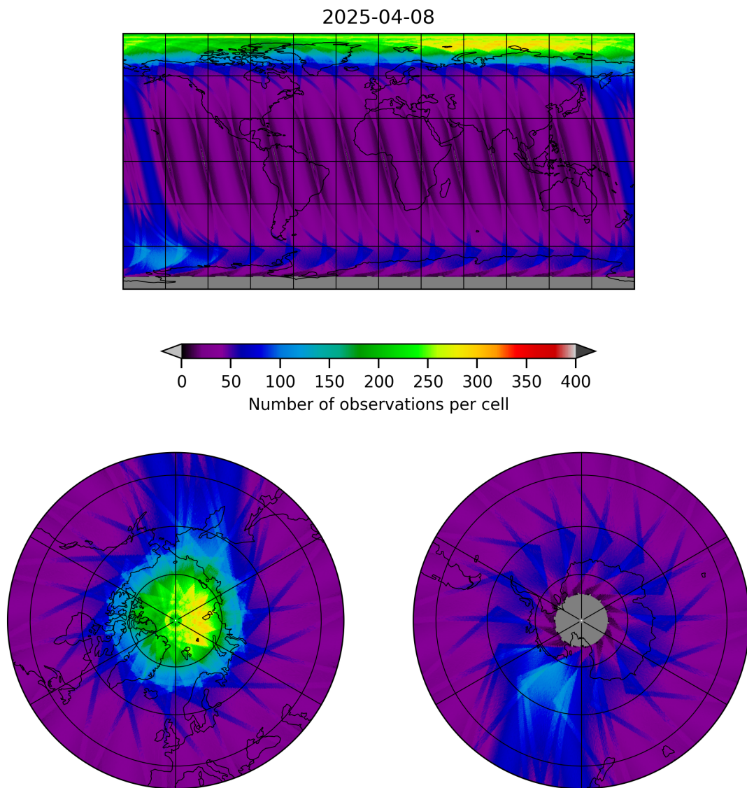
Figure 12: Map of the number of observations for 2025-04-08 to 2025-04-09
