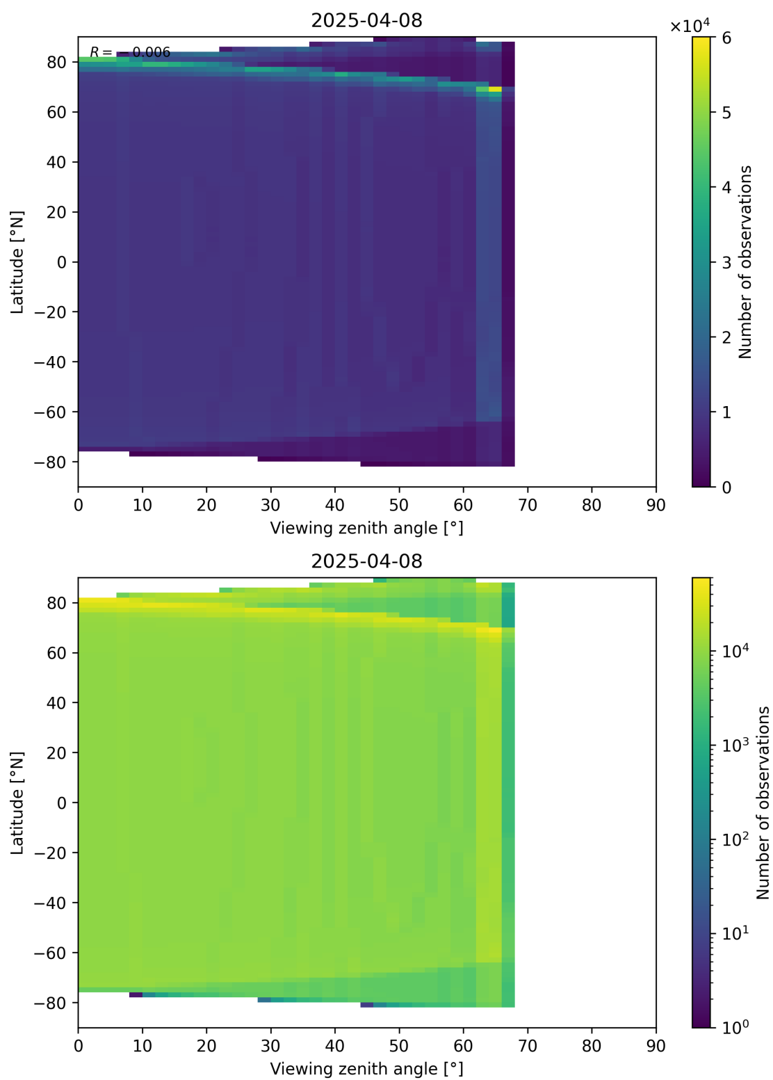
Figure 49: Scatter density plot of “Viewing zenith angle” against “Latitude” for 2025-04-08 to 2025-04-09.
