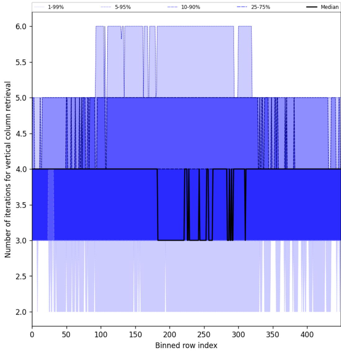
Figure 33: Along track statistics of “Number of iterations for vertical column retrieval” for 2025-04-08 to 2025-04-09
