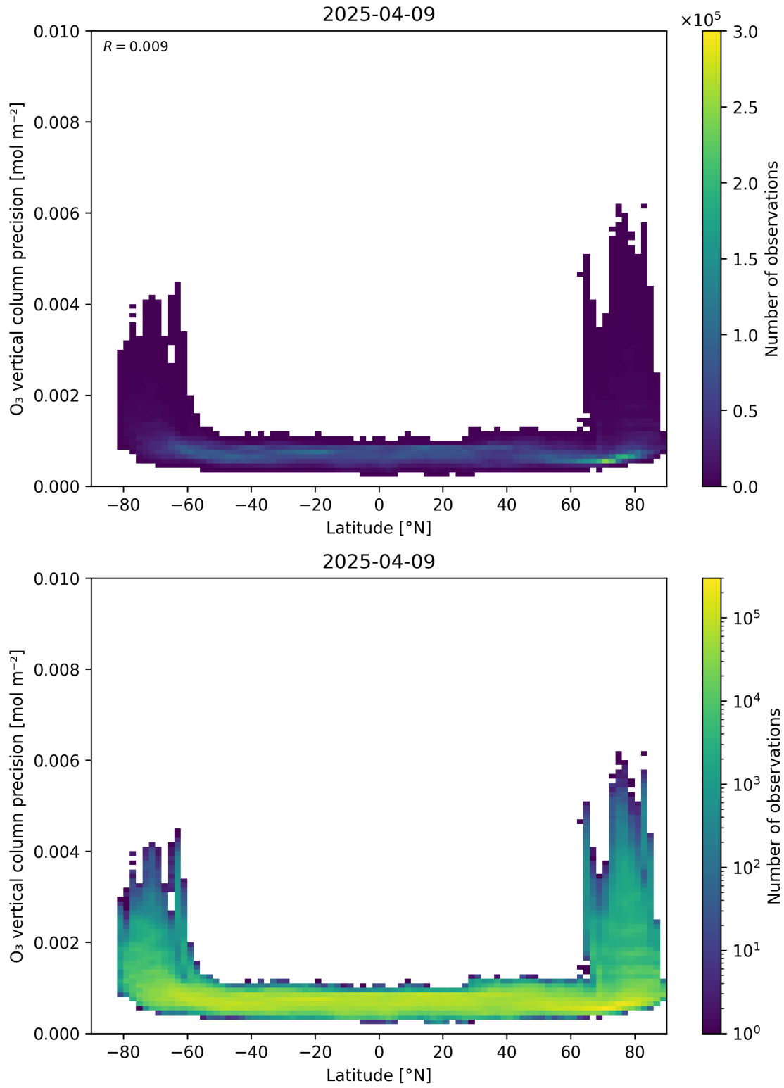
Figure 37: Scatter density plot of “Latitude” against “O 3 vertical column precision” for 2025-04-08 to 2025-04-10.
