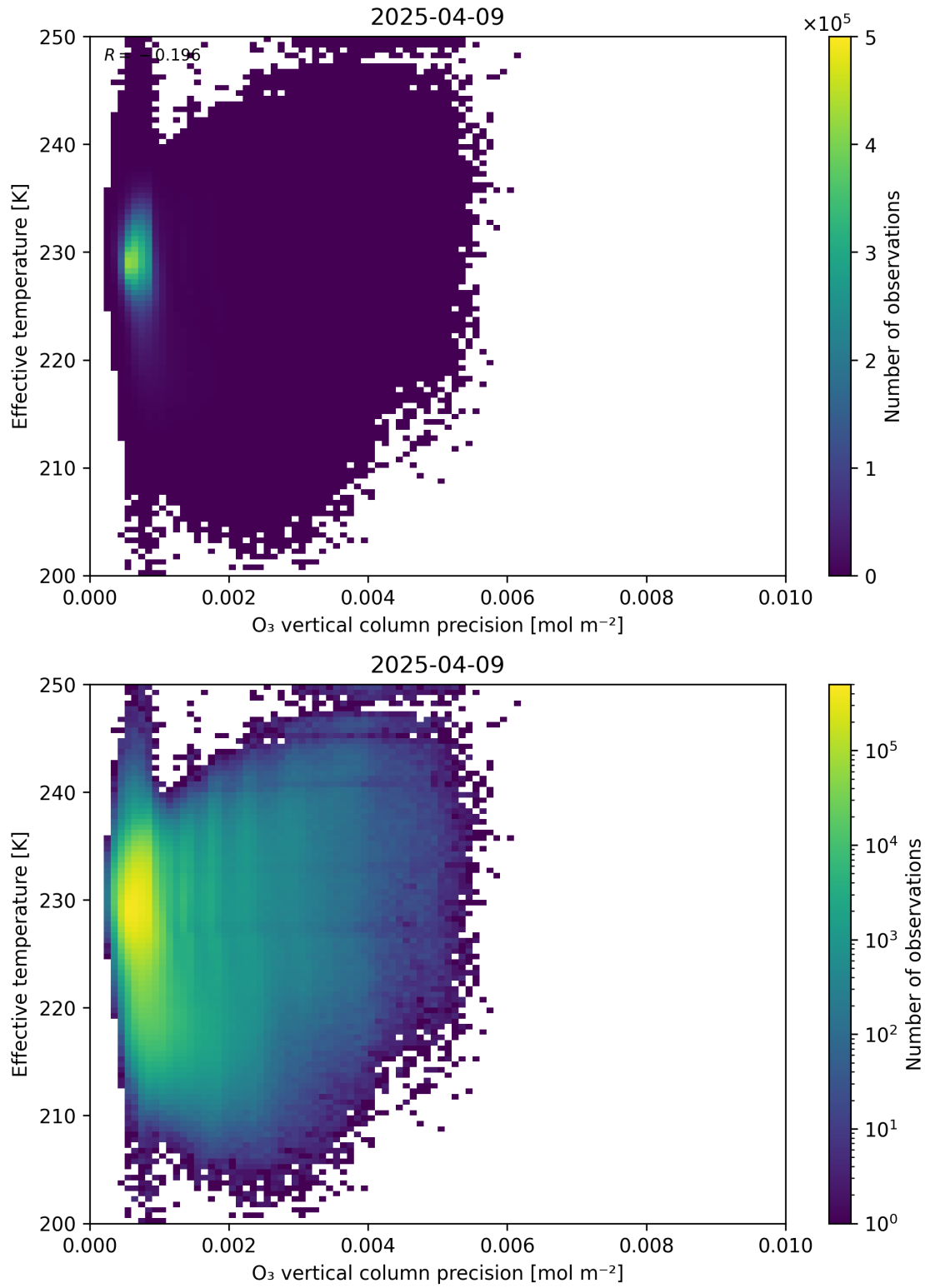
Figure 42: Scatter density plot of “O 3 vertical column precision” against “Effective temperature” for 2025-04-08 to 2025-04-10.
