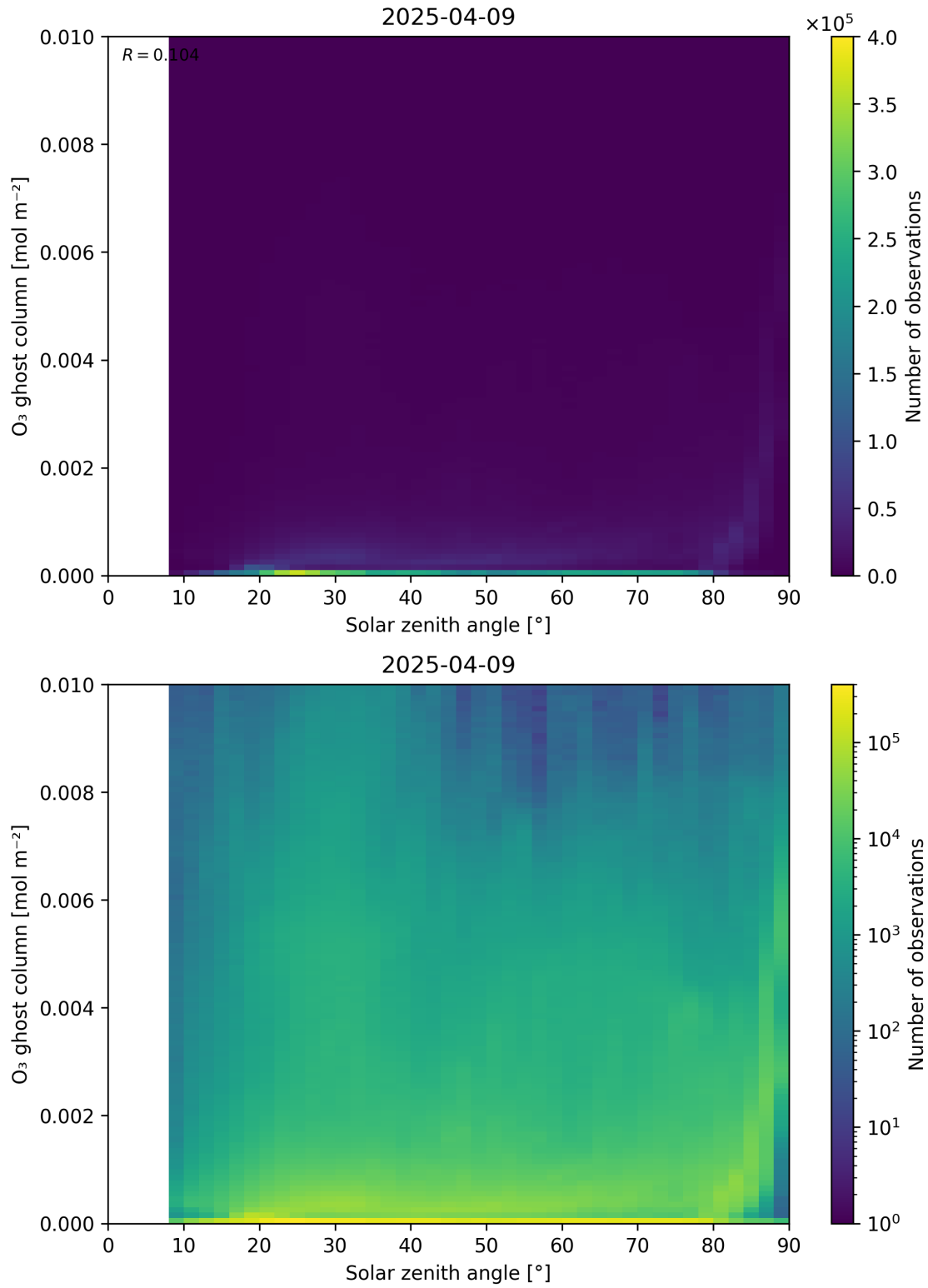
Figure 46: Scatter density plot of “Solar zenith angle” against “O 3 ghost column” for 2025-04-08 to 2025-04-10.
