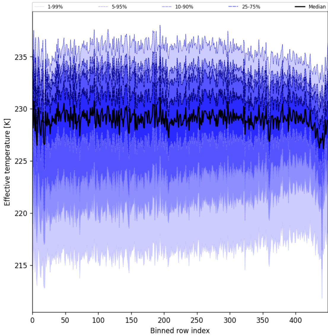
Figure 31: Along track statistics of “Effective temperature” for 2025-04-08 to 2025-04-10
