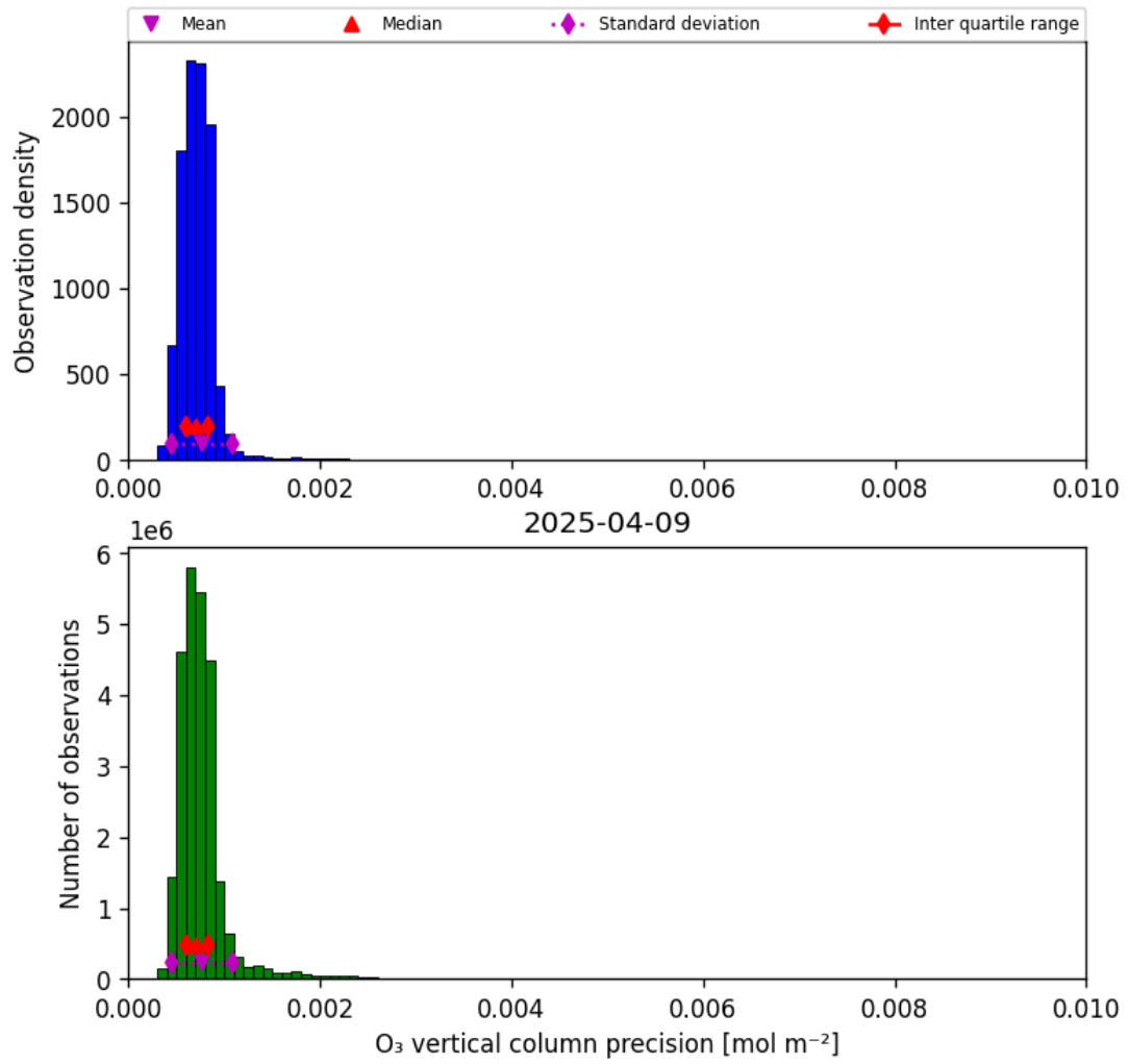
Figure 22: Histogram of “O 3 vertical column precision” for 2025-04-08 to 2025-04-10
