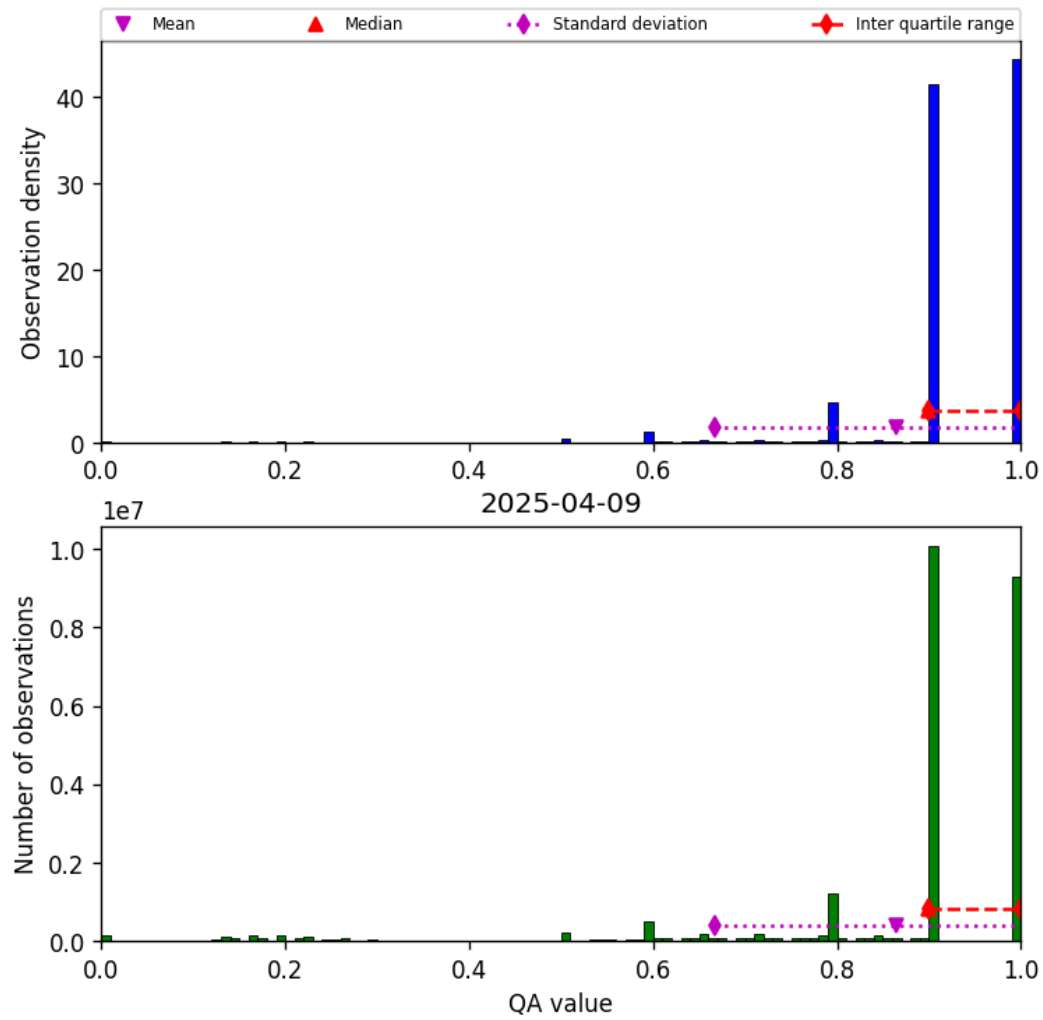
Figure 20: Histogram of “QA value” for 2025-04-08 to 2025-04-10
