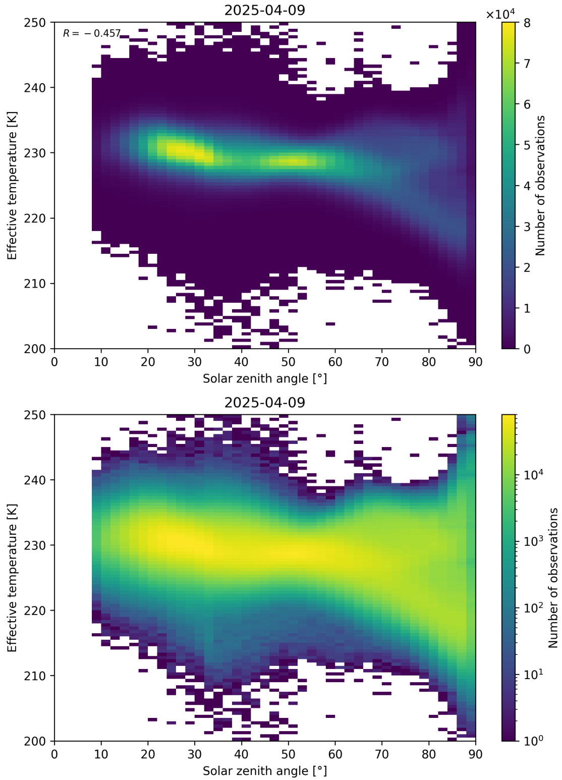
Figure 45: Scatter density plot of “Solar zenith angle” against “Effective temperature” for 2025-04-08 to 2025-04-10.
