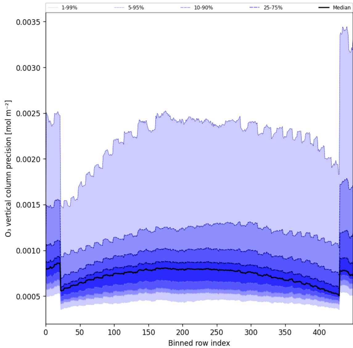
Figure 29: Along track statistics of “O 3 vertical column precision” for 2025-04-08 to 2025-04-10
