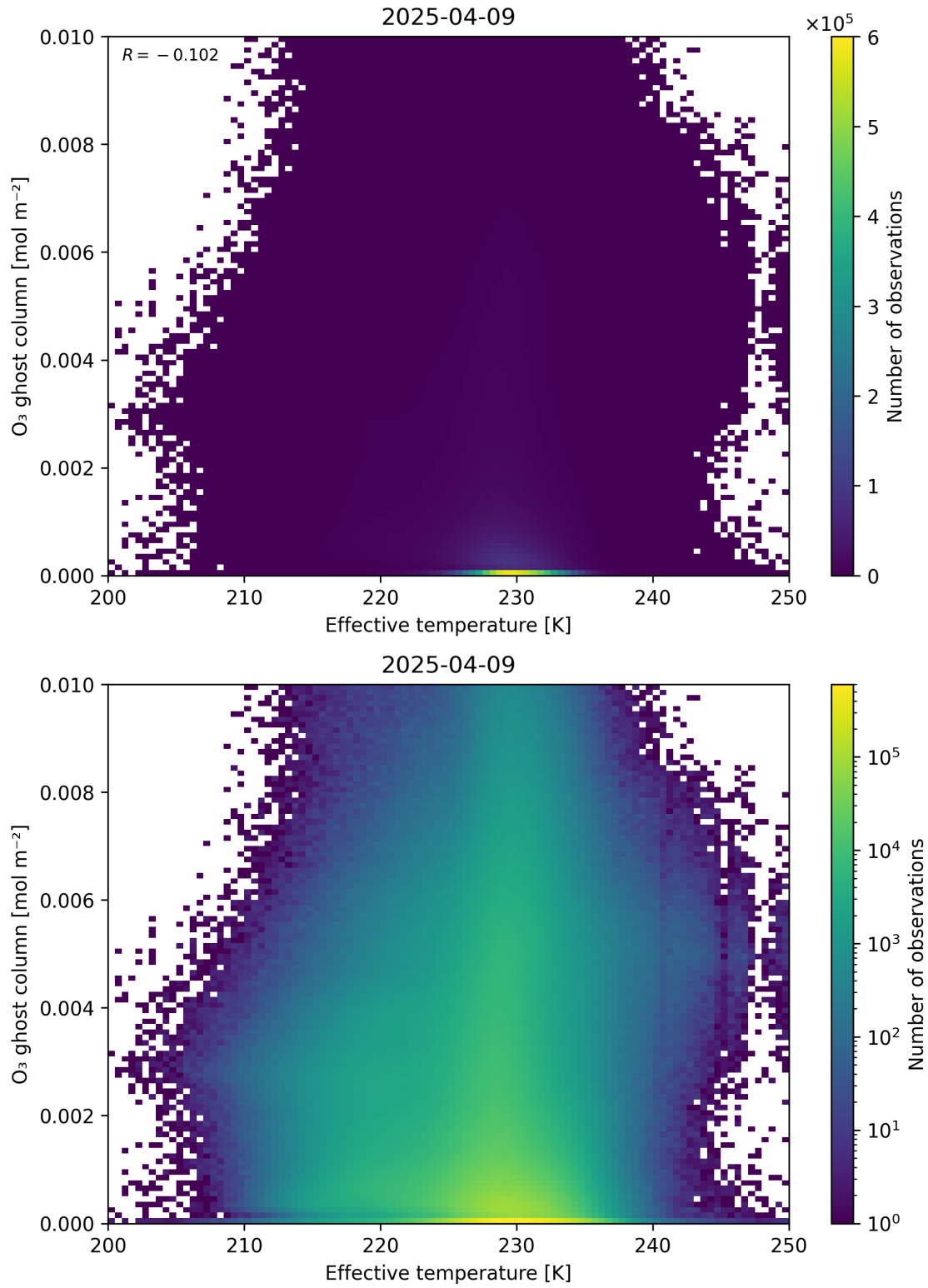
Figure 38: Scatter density plot of “Effective temperature” against “O 3 ghost column” for 2025-04-08 to 2025-04-10.
