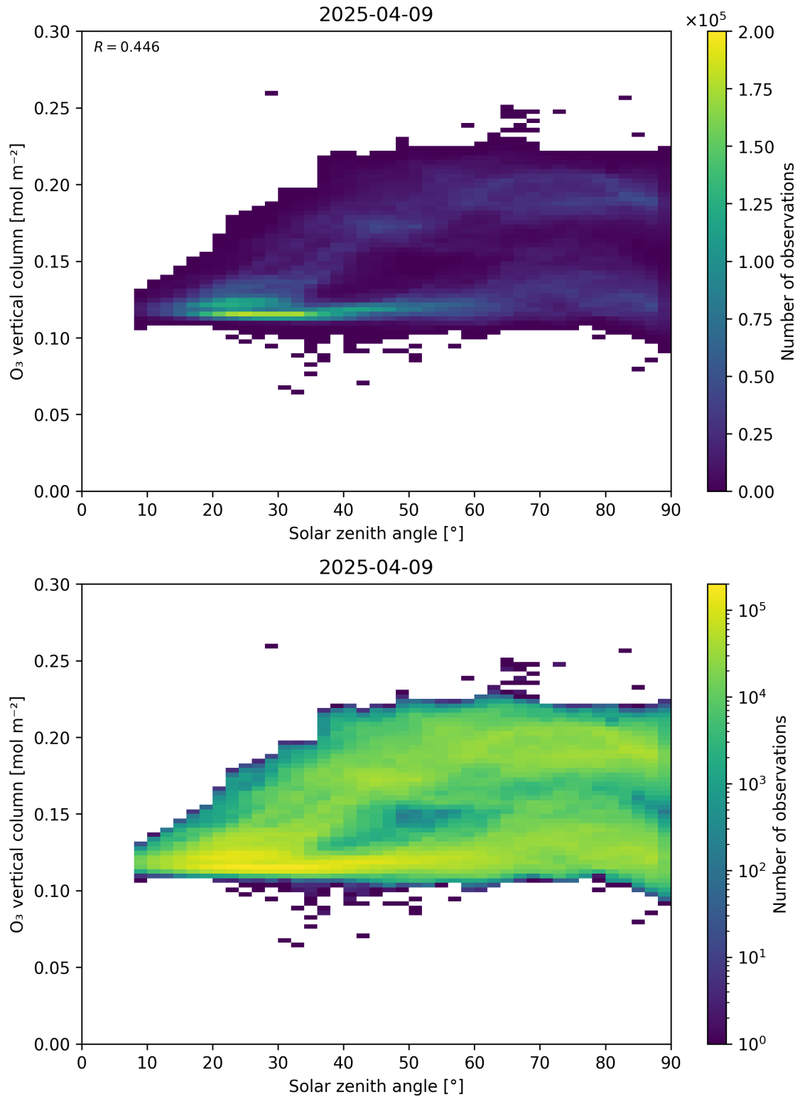
Figure 47: Scatter density plot of “Solar zenith angle” against “O 3 vertical column” for 2025-04-08 to 2025-04-10.
