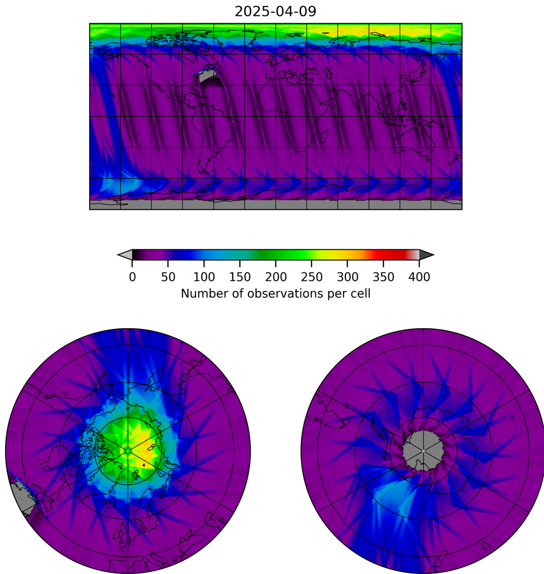
Figure 12: Map of the number of observations for 2025-04-08 to 2025-04-10
