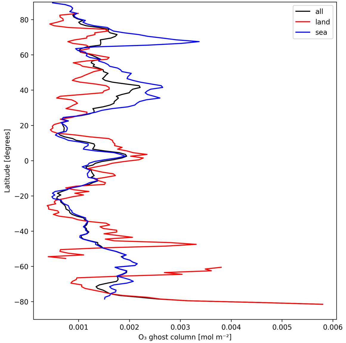
Figure 18: Zonal average of "O 3 ghost column" for 2025-04-08 to 2025-04-10.
