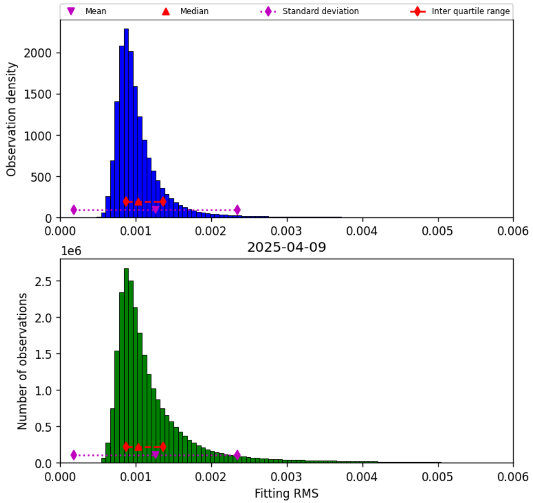
Figure 23: Histogram of “Fitting RMS” for 2025-04-08 to 2025-04-10
