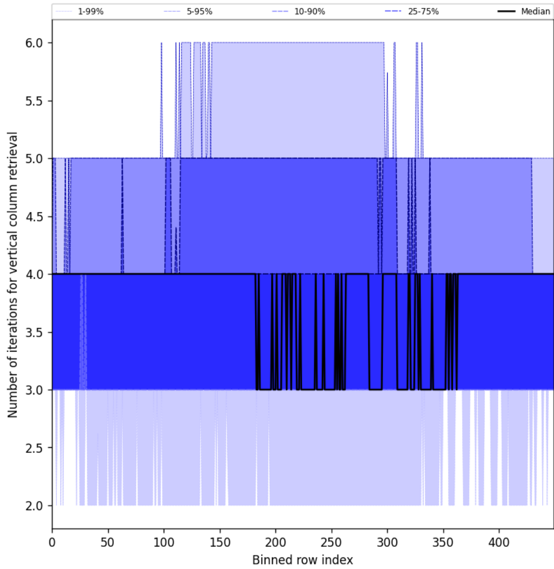
Figure 33: Along track statistics of “Number of iterations for vertical column retrieval” for 2025-04-08 to 2025-04-10
