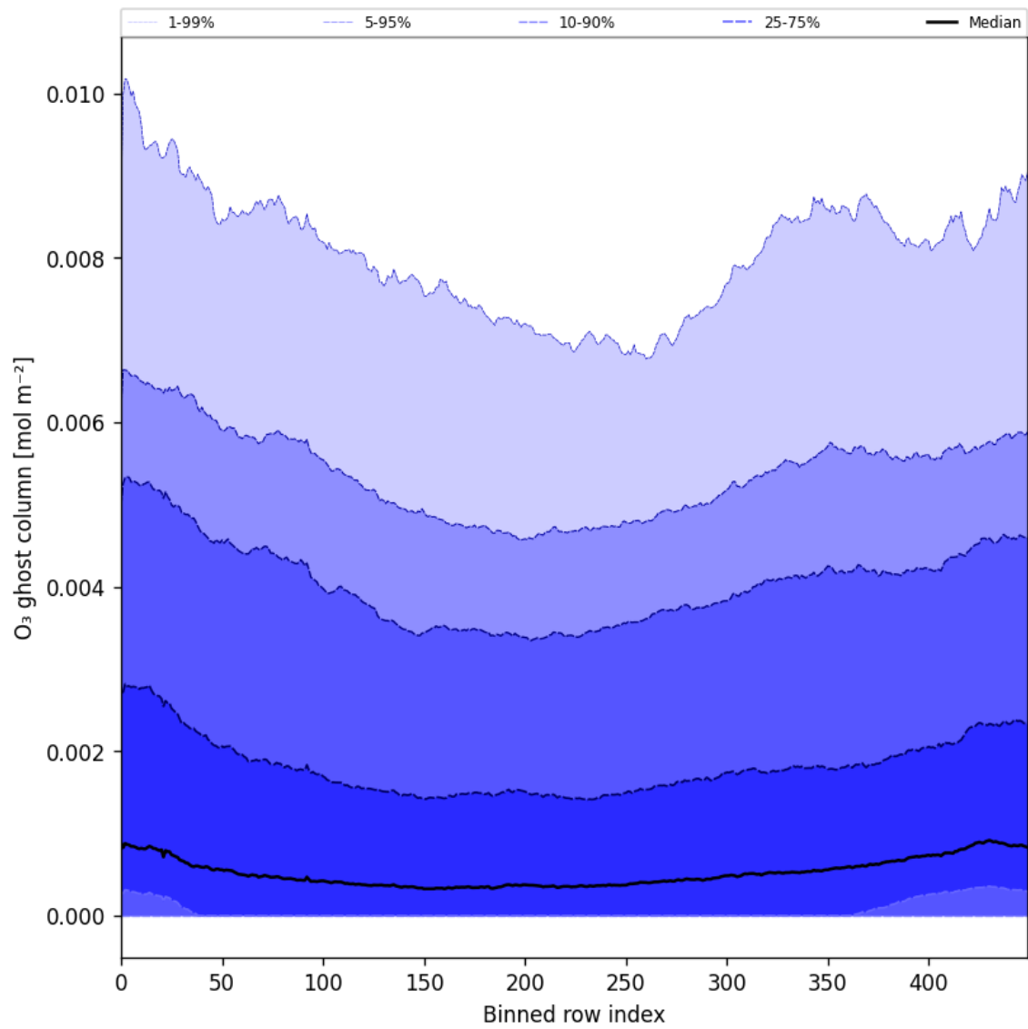
Figure 32: Along track statistics of “O 3 ghost column” for 2025-04-08 to 2025-04-10
