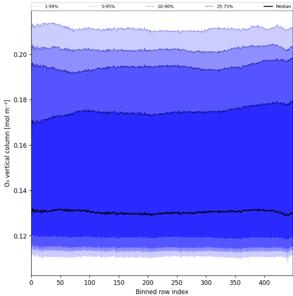
Figure 28: Along track statistics of “O 3 vertical column” for 2025-04-08 to 2025-04-10
