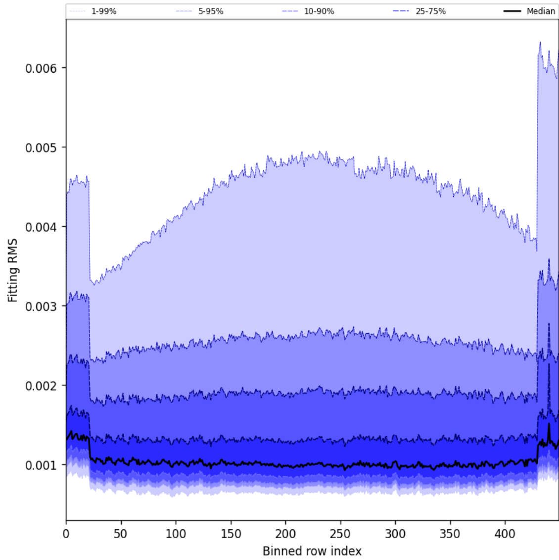
Figure 30: Along track statistics of “Fitting RMS” for 2025-04-08 to 2025-04-10
