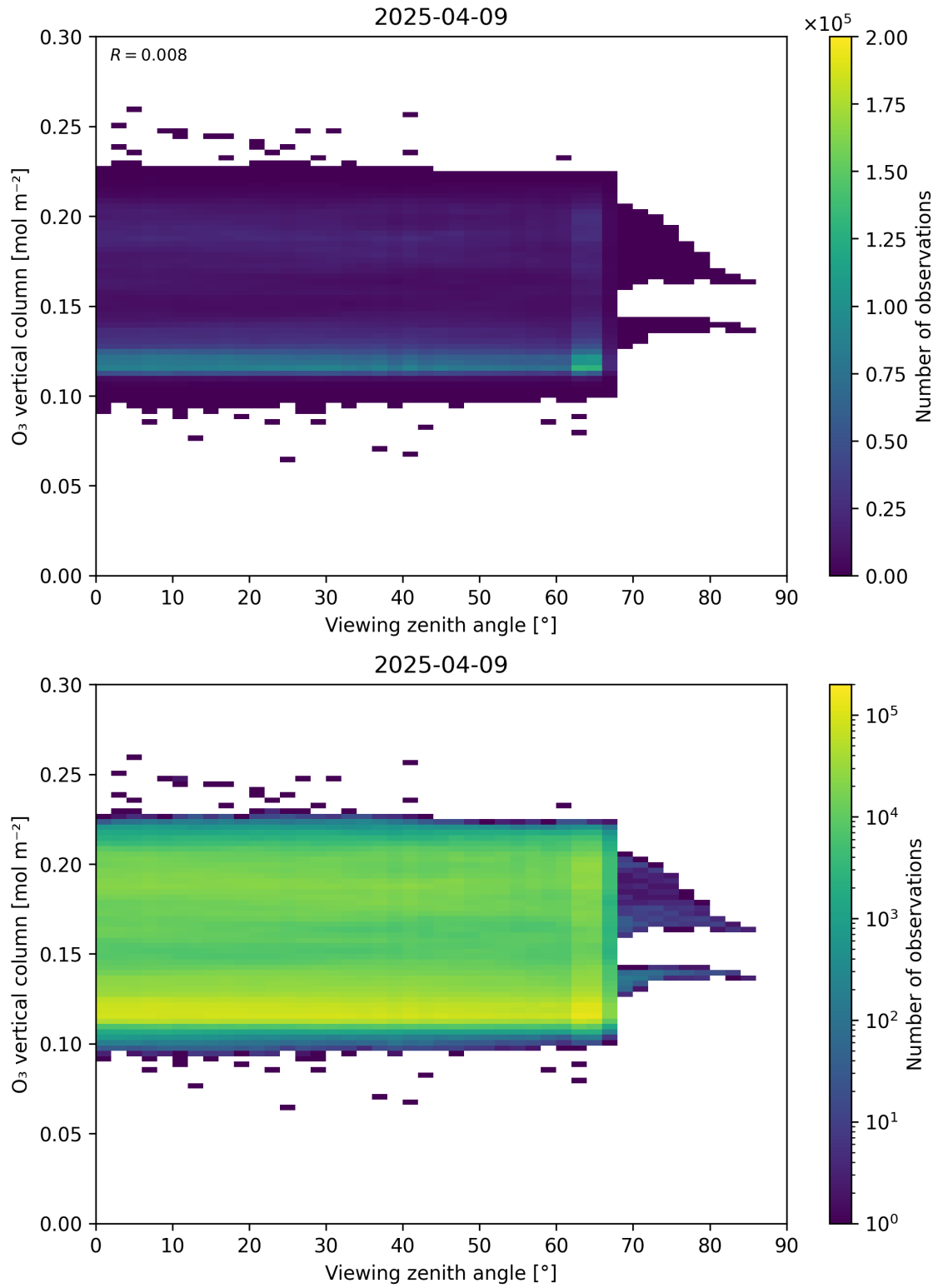
Figure 52: Scatter density plot of “Viewing zenith angle” against “O 3 vertical column” for 2025-04-08 to 2025-04-10.
