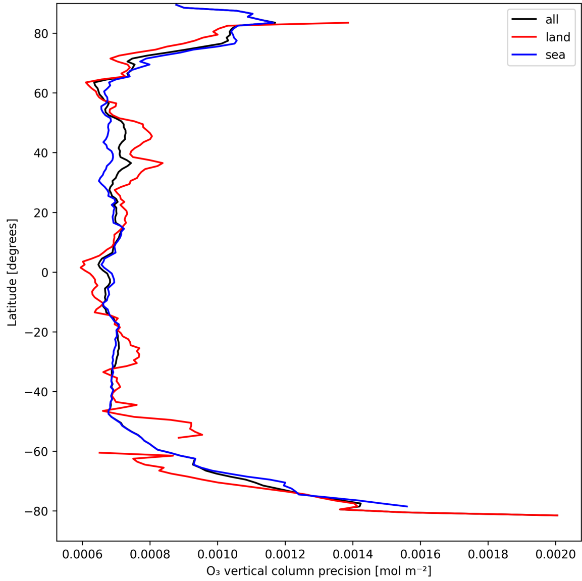
Figure 15: Zonal average of “O 3 vertical column precision” for 2025-04-08 to 2025-04-10.
