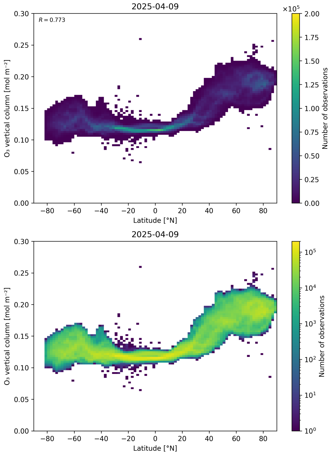
Figure 36: Scatter density plot of “Latitude” against “O 3 vertical column” for 2025-04-08 to 2025-04-10.
