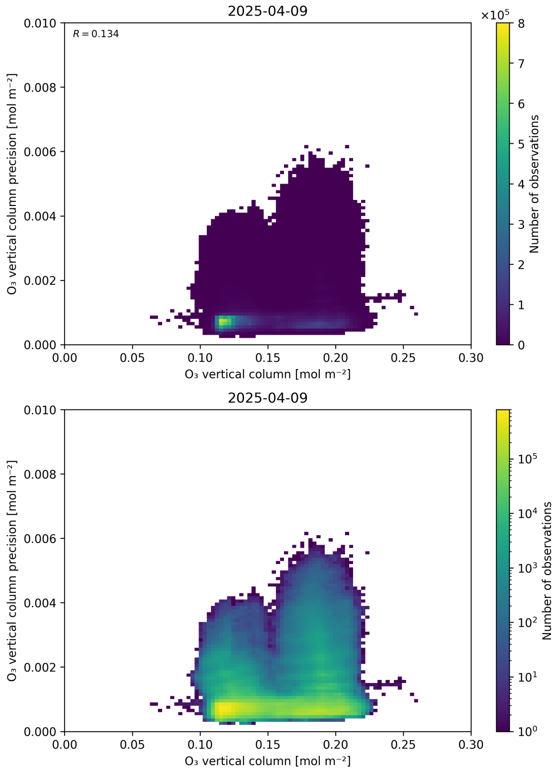
Figure 41: Scatter density plot of “O 3 vertical column” against “O 3 vertical column precision” for 2025-04-08 to 2025-04-10.
