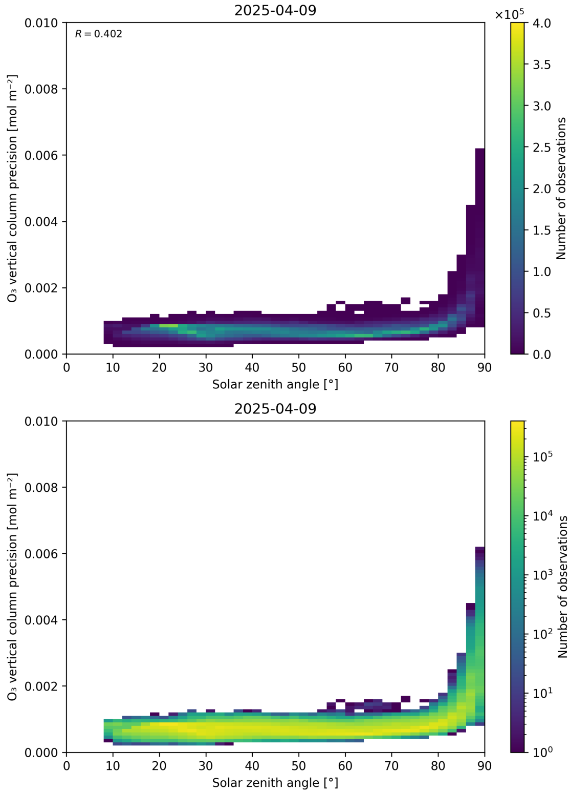
Figure 48: Scatter density plot of “Solar zenith angle” against “O 3 vertical column precision” for 2025-04-08 to 2025-04-10.
