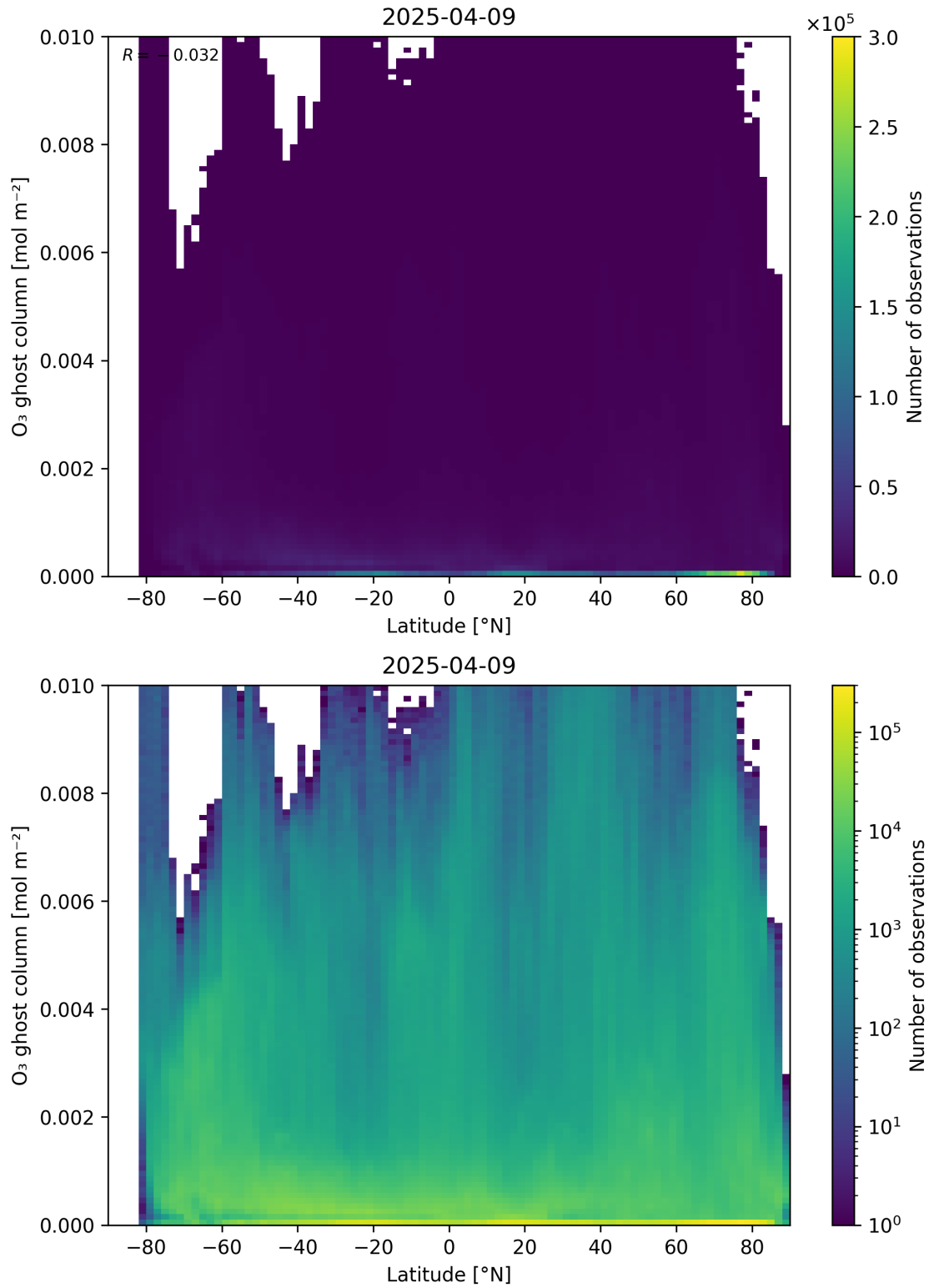
Figure 35: Scatter density plot of “Latitude” against “O 3 ghost column” for 2025-04-08 to 2025-04-10.
