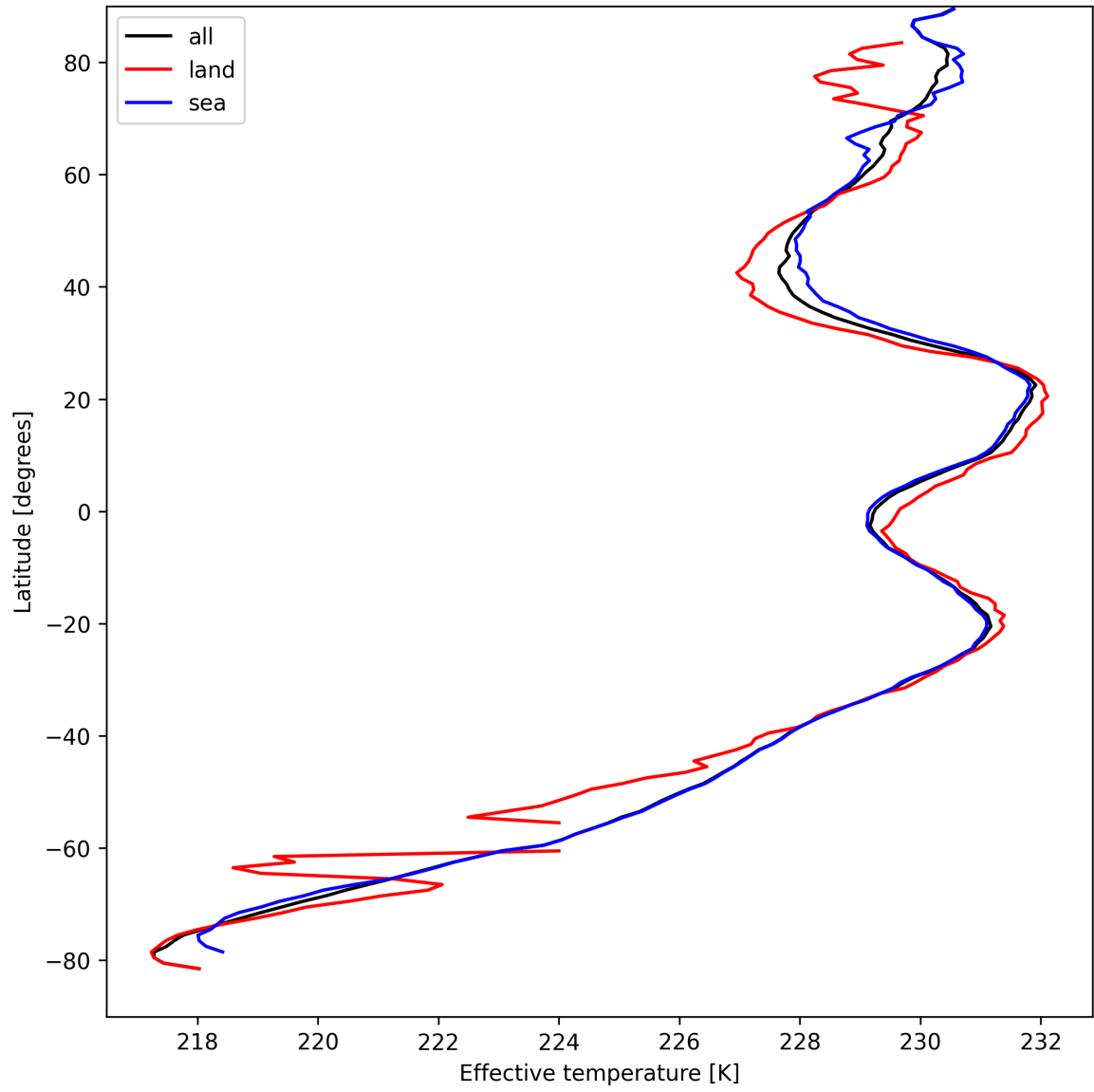
Figure 17: Zonal average of “Effective temperature” for 2025-04-08 to 2025-04-10.
