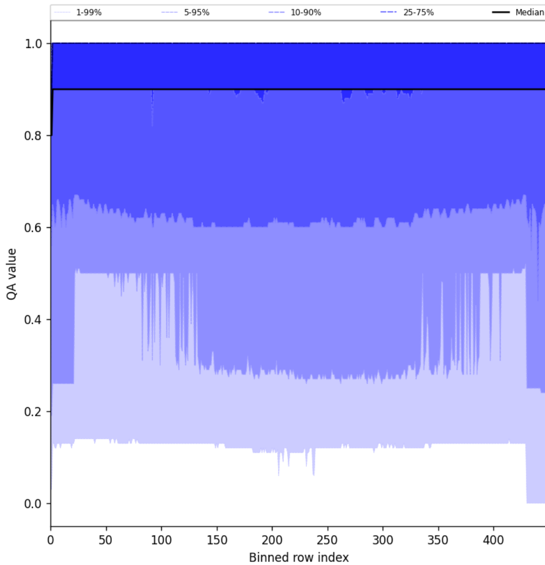
Figure 27: Along track statistics of “QA value” for 2025-04-08 to 2025-04-10
