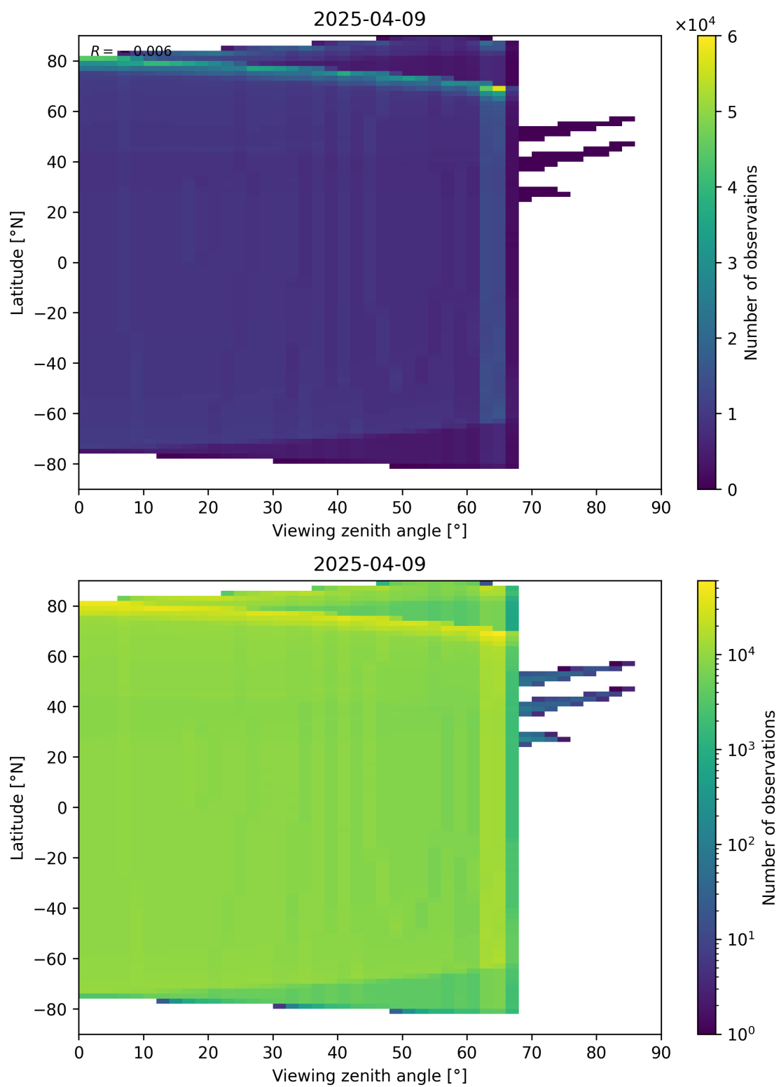
Figure 49: Scatter density plot of “Viewing zenith angle” against “Latitude” for 2025-04-08 to 2025-04-10.
