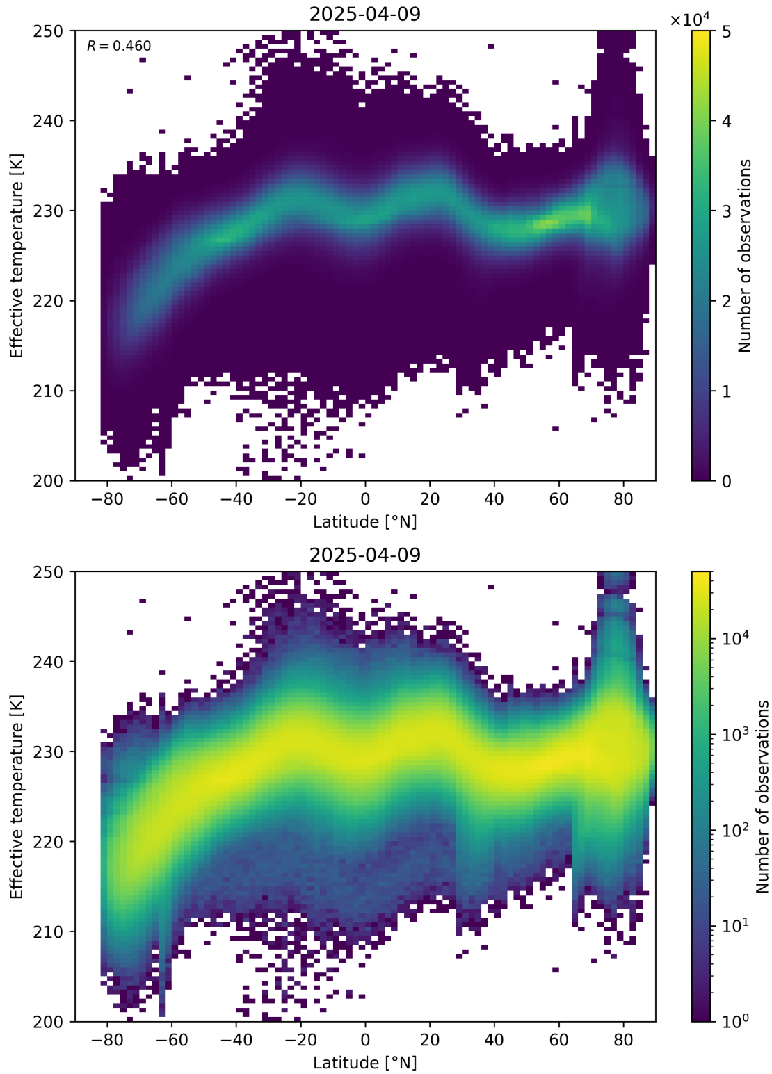
Figure 34: Scatter density plot of “Latitude” against “Effective temperature” for 2025-04-08 to 2025-04-10.
