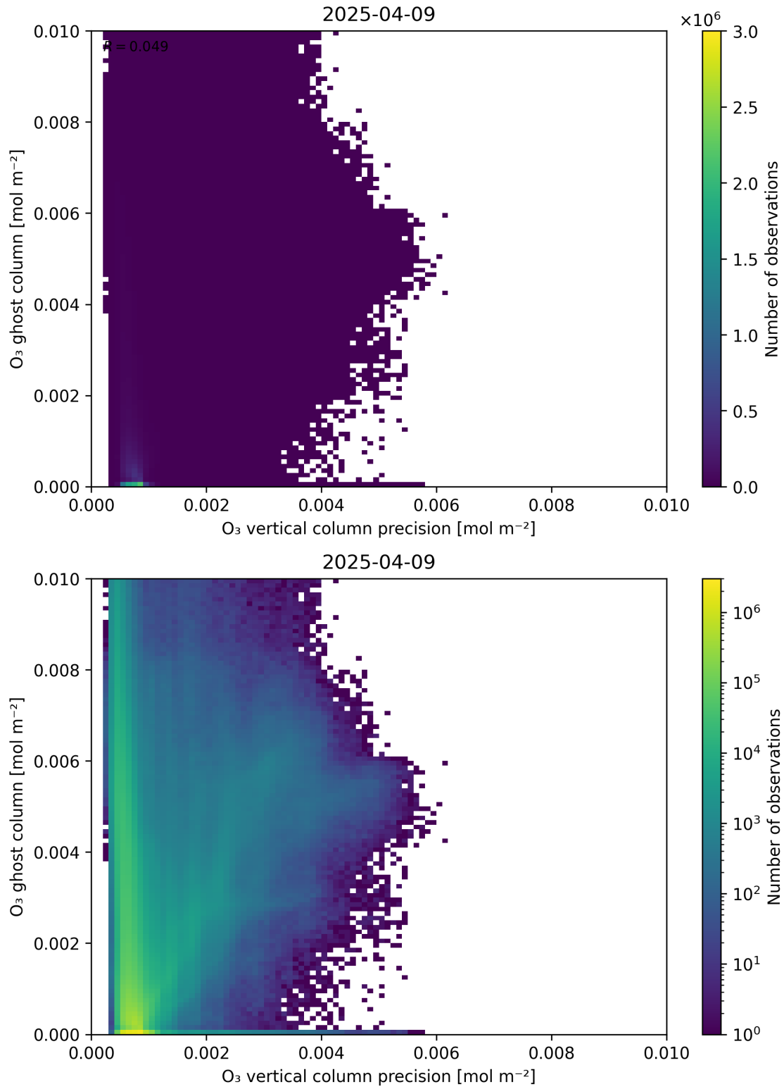
Figure 43: Scatter density plot of “O 3 vertical column precision” against “O 3 ghost column” for 2025-04-08 to 2025-04-10.
