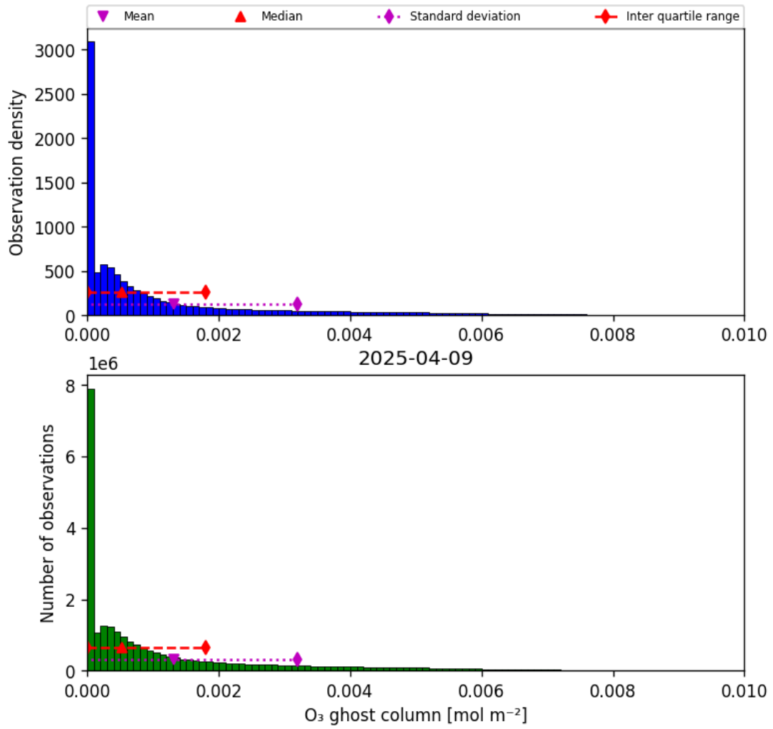
Figure 25: Histogram of “O 3 ghost column” for 2025-04-08 to 2025-04-10
