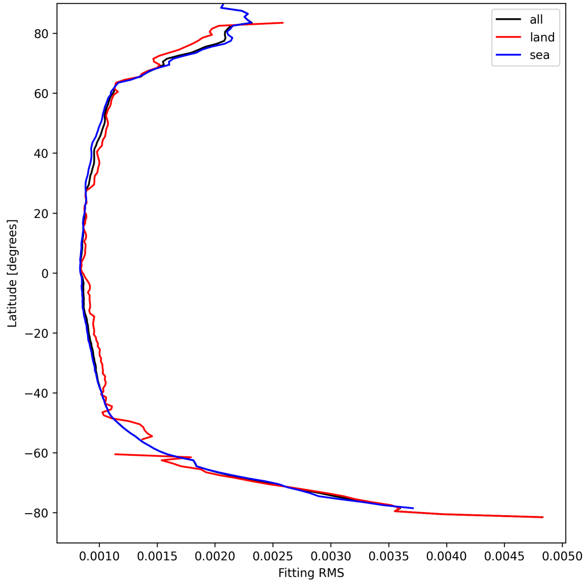
Figure 16: Zonal average of “Fitting RMS” for 2025-04-08 to 2025-04-10.
