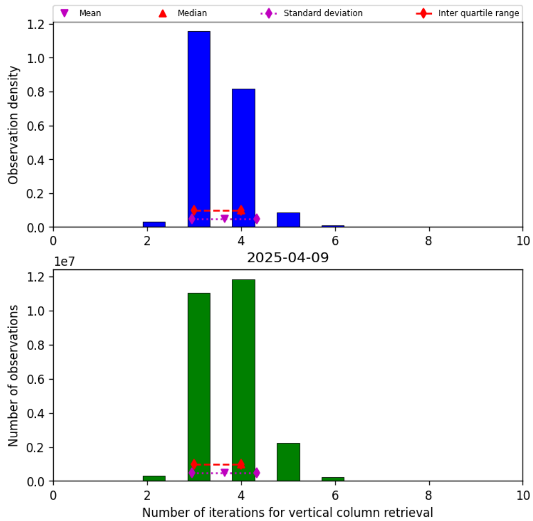
Figure 26: Histogram of “Number of iterations for vertical column retrieval” for 2025-04-08 to 2025-04-10
