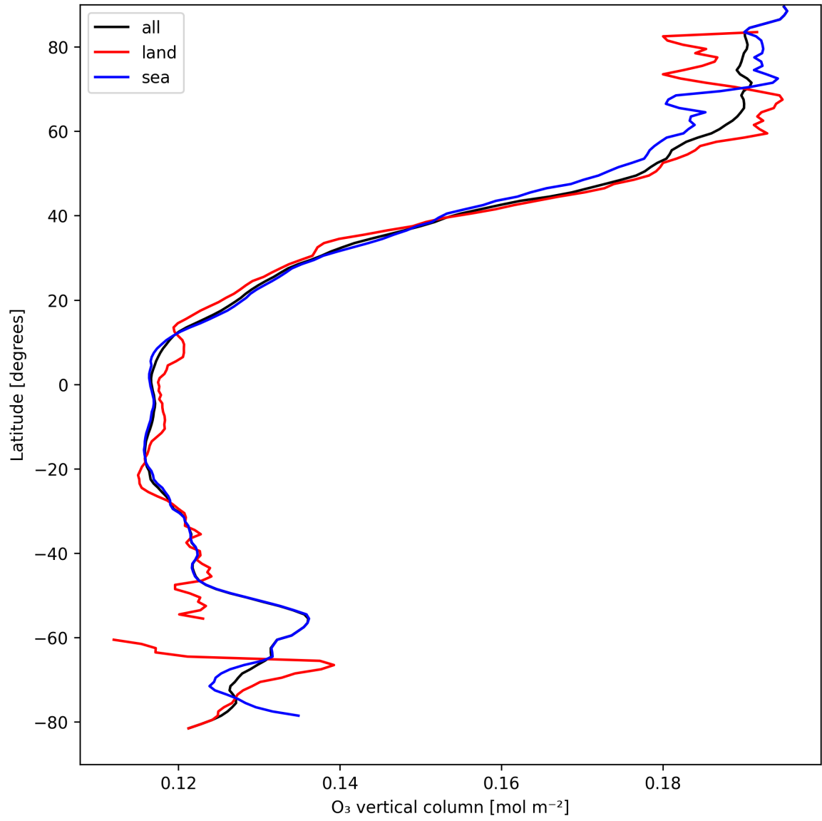
Figure 14: Zonal average of “O 3 vertical column” for 2025-04-08 to 2025-04-10.
