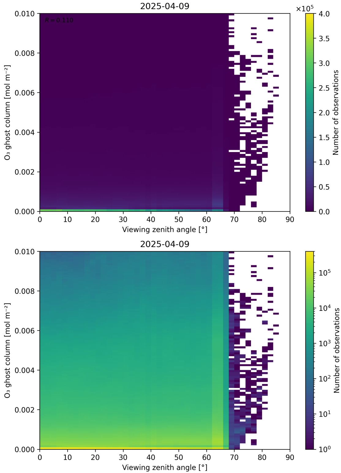
Figure 51: Scatter density plot of “Viewing zenith angle” against “O 3 ghost column” for 2025-04-08 to 2025-04-10.
