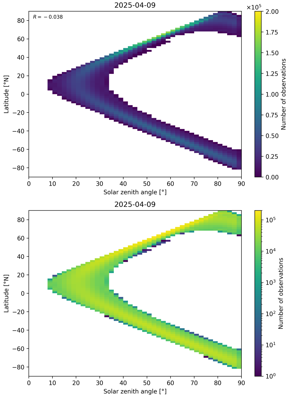
Figure 44: Scatter density plot of “Solar zenith angle” against “Latitude” for 2025-04-08 to 2025-04-10.
