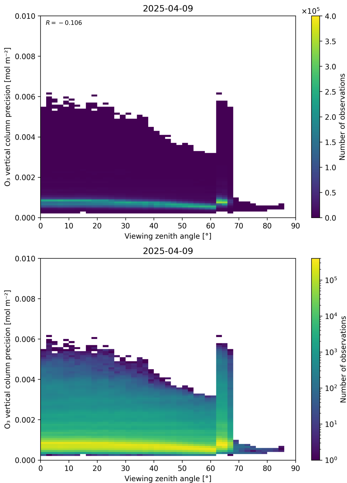
Figure 53: Scatter density plot of “Viewing zenith angle” against “O 3 vertical column precision” for 2025-04-08 to 2025-04-10.
