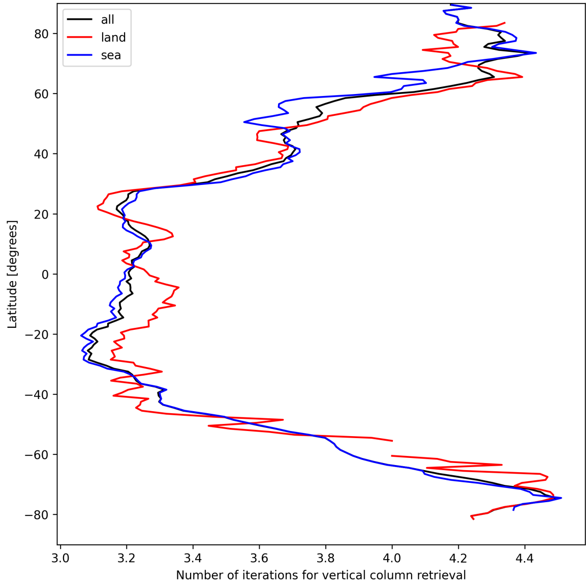
Figure 19: Zonal average of “Number of iterations for vertical column retrieval” for 2025-04-08 to 2025-04-10.
