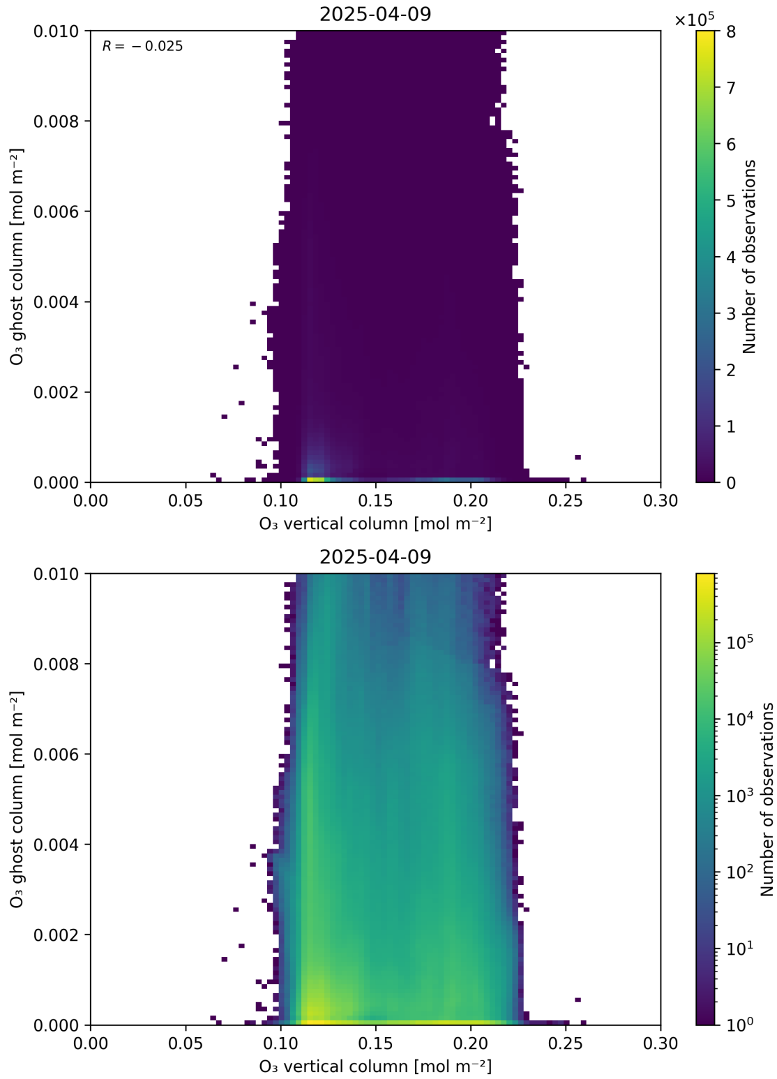
Figure 40: Scatter density plot of “O 3 vertical column” against “O 3 ghost column” for 2025-04-08 to 2025-04-10.
