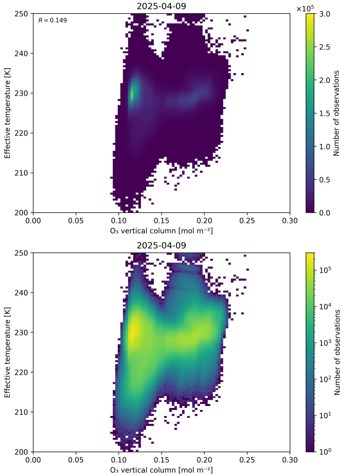
Figure 39: Scatter density plot of “O 3 vertical column” against “Effective temperature” for 2025-04-08 to 2025-04-10.
