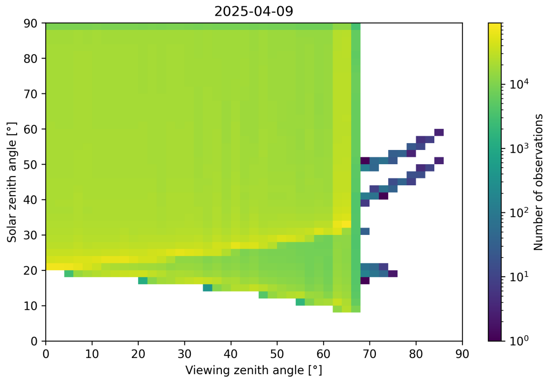
Figure 54: Scatter density plot of “Viewing zenith angle” against “Solar zenith angle” for 2025-04-08 to 2025-04-10.
