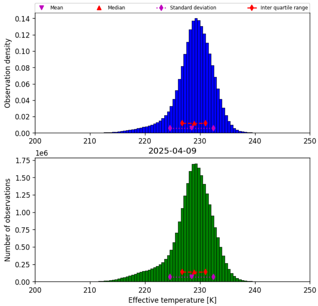
Figure 24: Histogram of “Effective temperature” for 2025-04-08 to 2025-04-10
