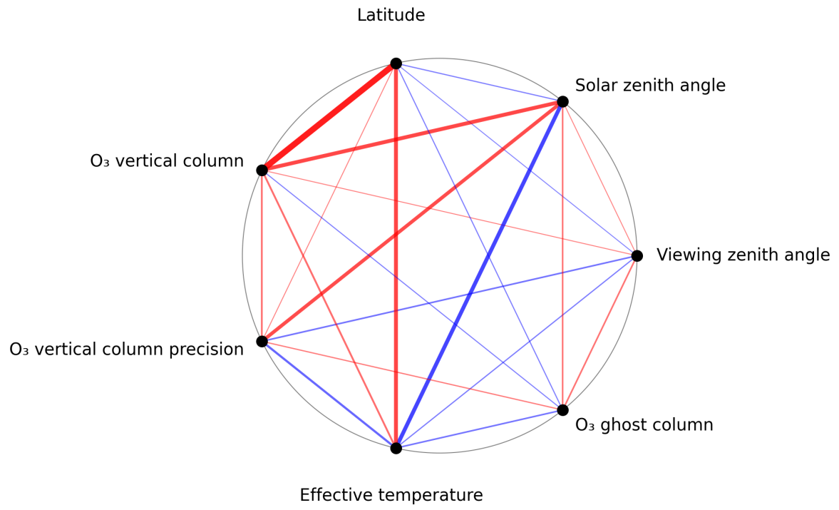
Figure 1: Map of correlation graph for 2025-04-08 to 2025-04-10.
