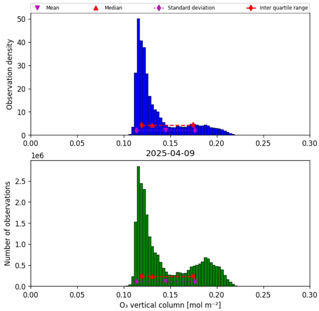
Figure 21: Histogram of “O 3 vertical column” for 2025-04-08 to 2025-04-10
