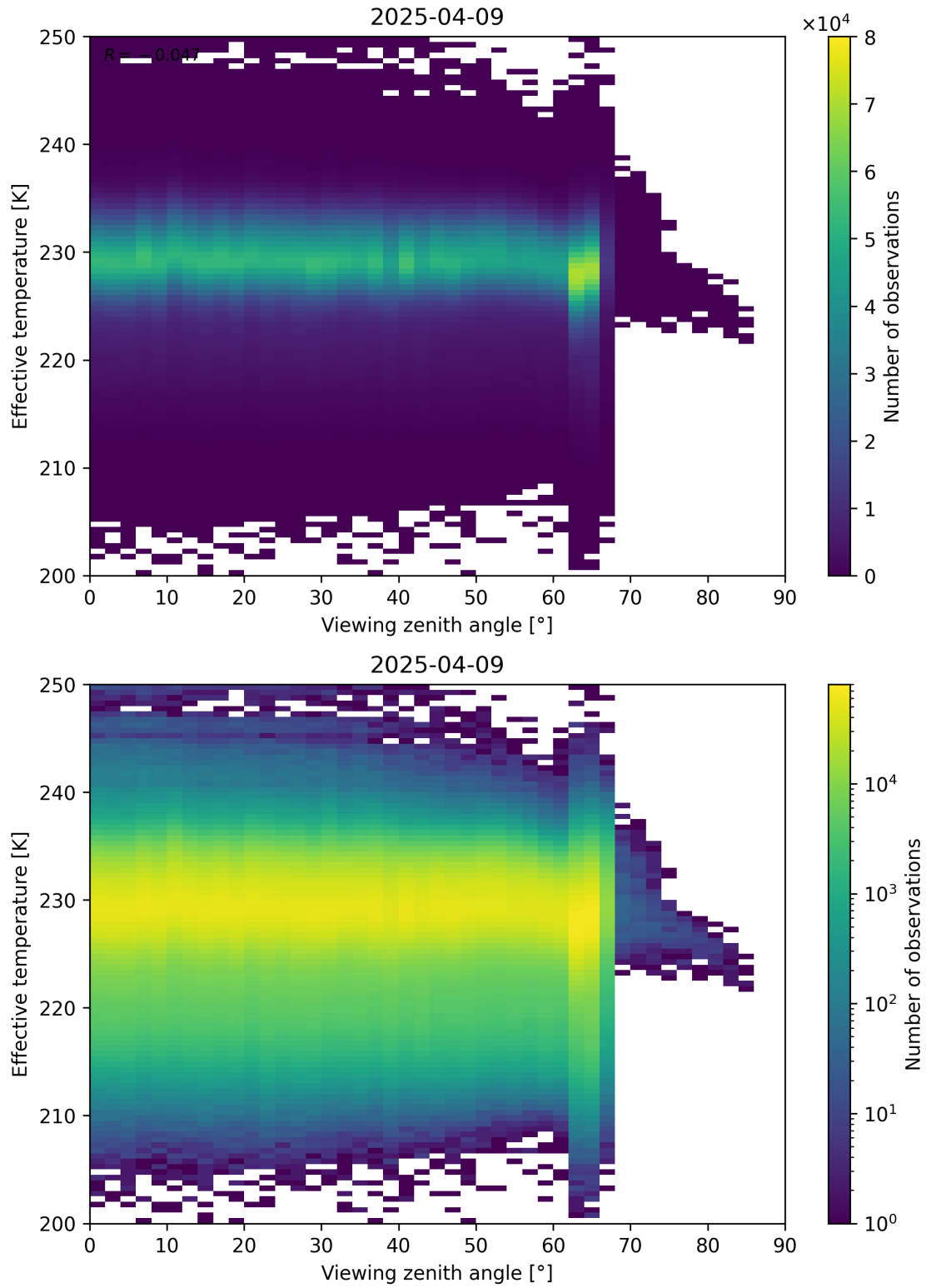
Figure 50: Scatter density plot of “Viewing zenith angle” against “Effective temperature” for 2025-04-08 to 2025-04-10.
