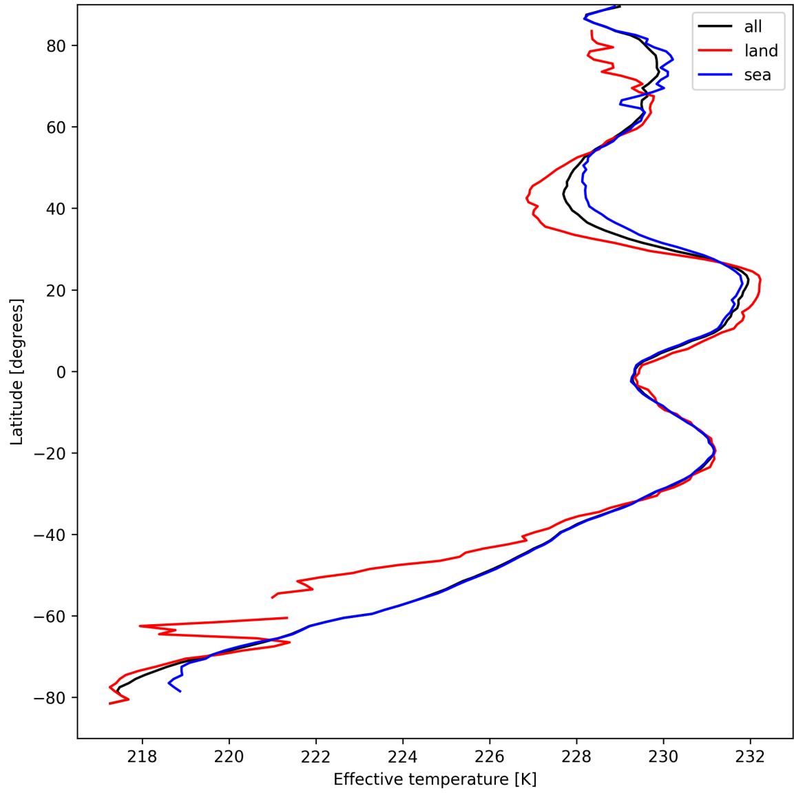
Figure 17: Zonal average of "Effective temperature" for 2025-04-09 to 2025-04-11.
