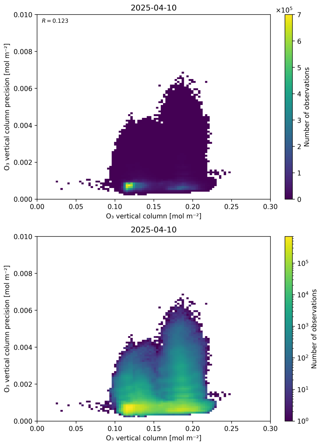
Figure 41: Scatter density plot of “O 3 vertical column” against “O 3 vertical column precision” for 2025-04-09 to 2025-04-11.
