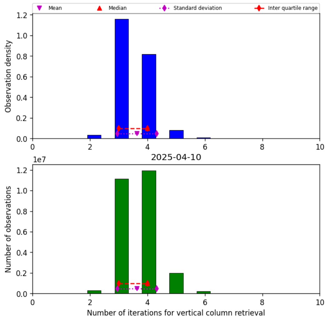
Figure 26: Histogram of “Number of iterations for vertical column retrieval” for 2025-04-09 to 2025-04-11
