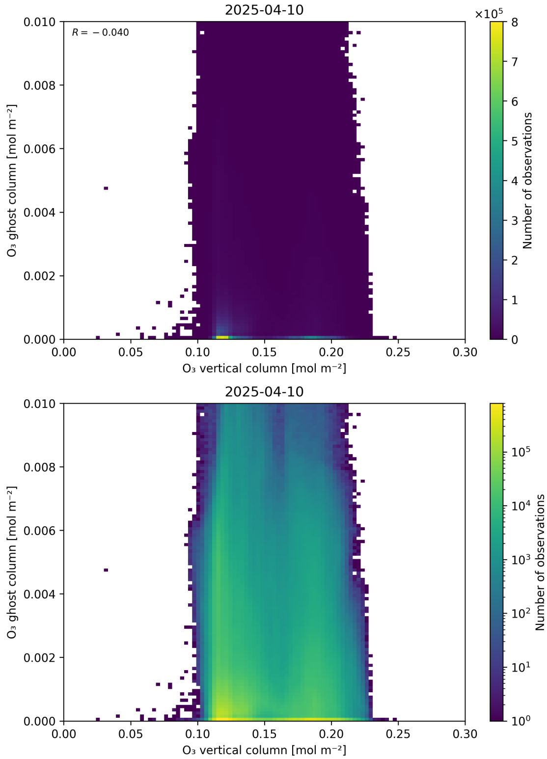
Figure 40: Scatter density plot of “O 3 vertical column” against “O 3 ghost column” for 2025-04-09 to 2025-04-11.
