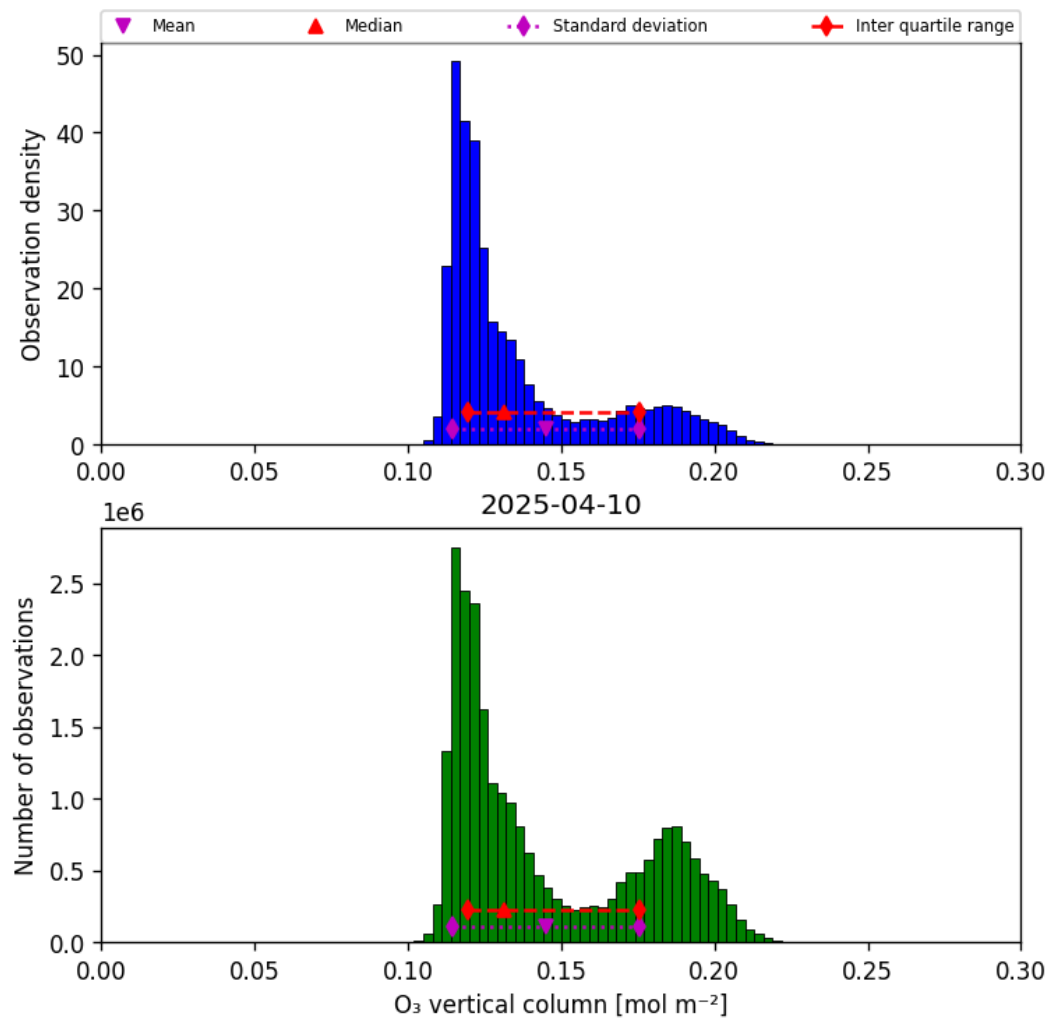
Figure 21: Histogram of “O 3 vertical column” for 2025-04-09 to 2025-04-11
