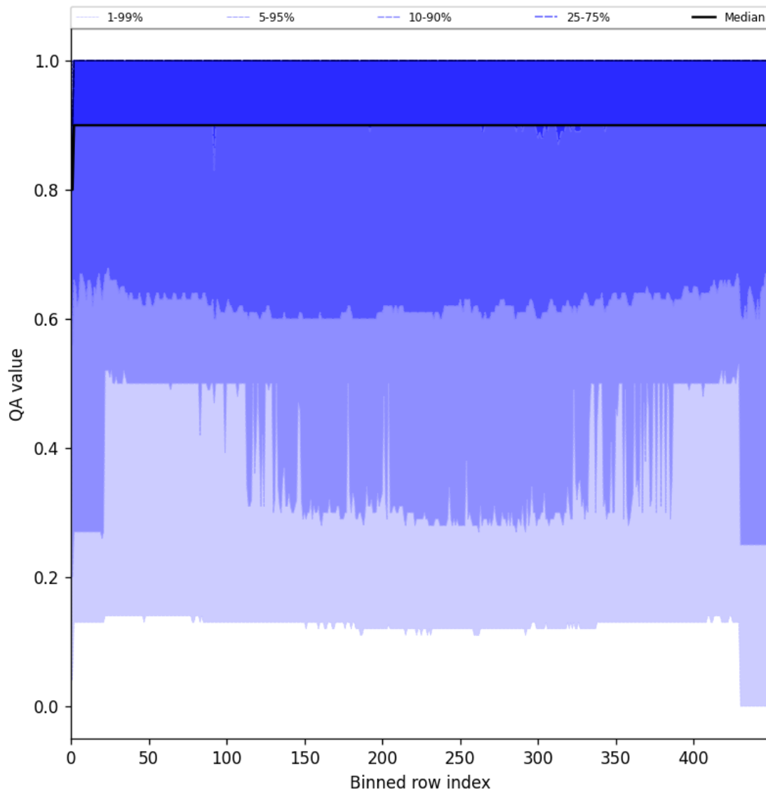
Figure 27: Along track statistics of “QA value” for 2025-04-09 to 2025-04-11
