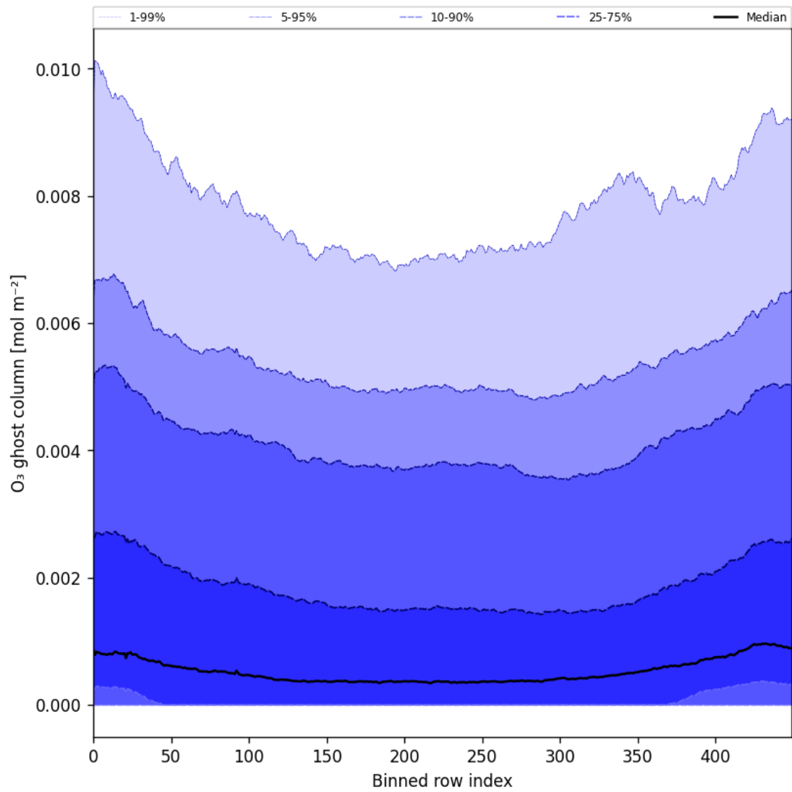
Figure 32: Along track statistics of “O 3 ghost column” for 2025-04-09 to 2025-04-11
