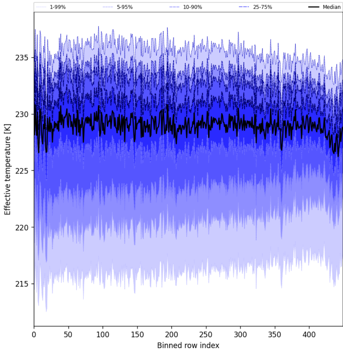
Figure 31: Along track statistics of “Effective temperature” for 2025-04-09 to 2025-04-11
