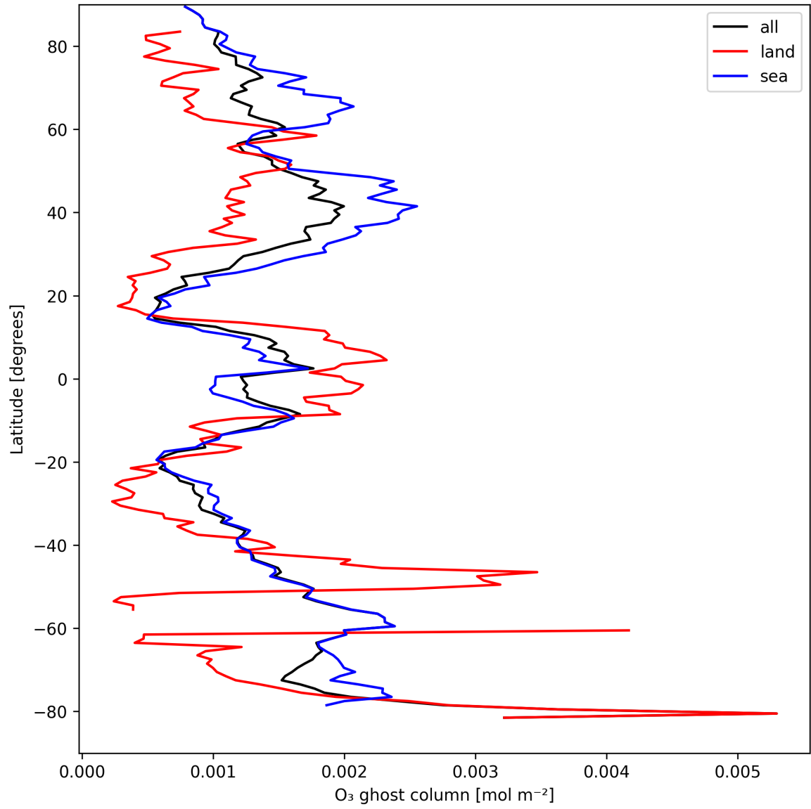
Figure 18: Zonal average of "O 3 ghost column" for 2025-04-09 to 2025-04-11.
