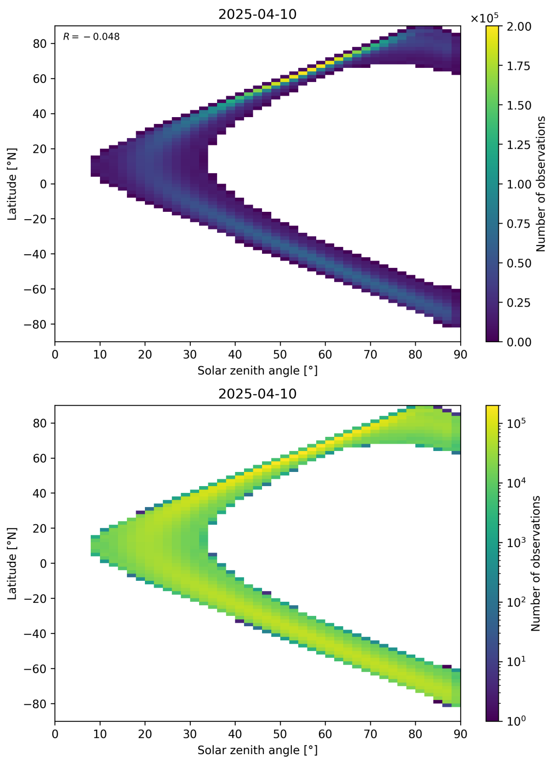
Figure 44: Scatter density plot of “Solar zenith angle” against “Latitude” for 2025-04-09 to 2025-04-11.
