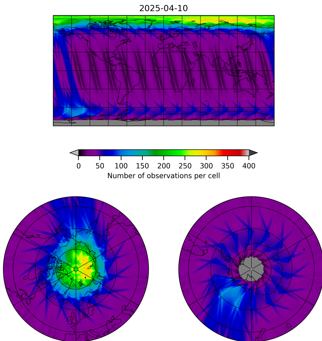
Figure 12: Map of the number of observations for 2025-04-09 to 2025-04-11
