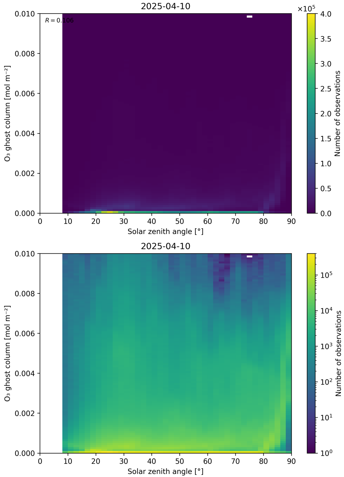
Figure 46: Scatter density plot of “Solar zenith angle” against “O 3 ghost column” for 2025-04-09 to 2025-04-11.
