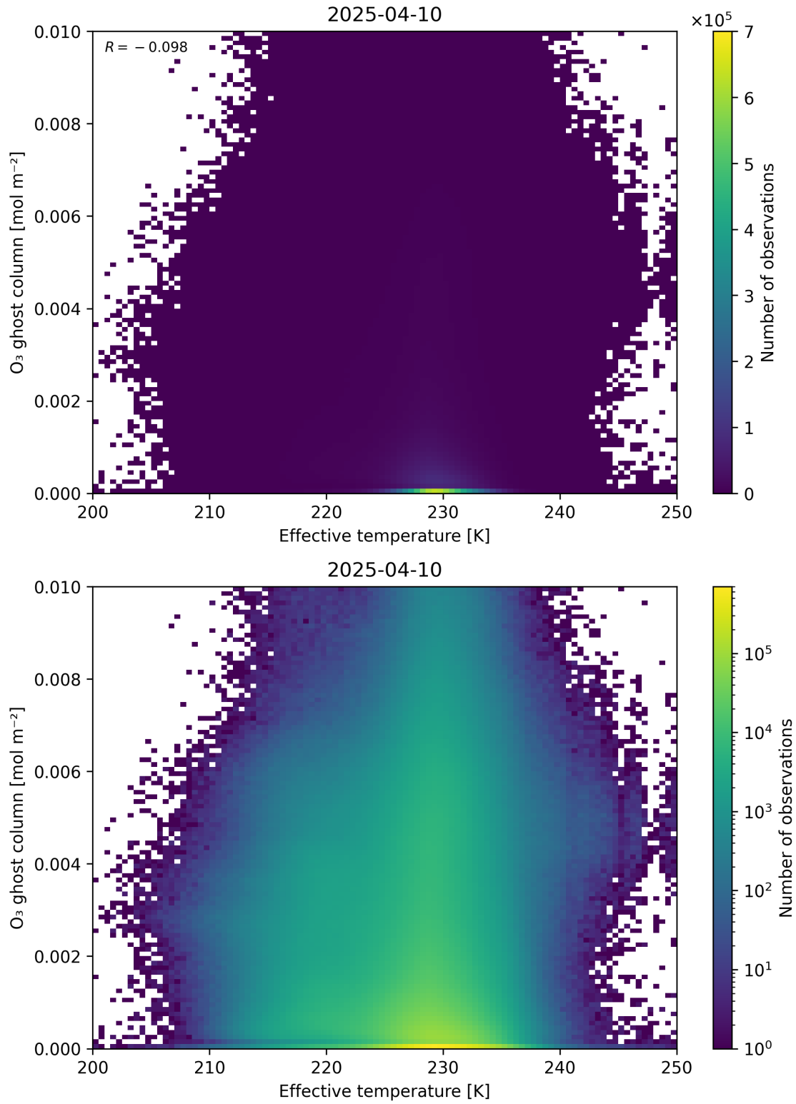
Figure 38: Scatter density plot of “Effective temperature” against “O 3 ghost column” for 2025-04-09 to 2025-04-11.
