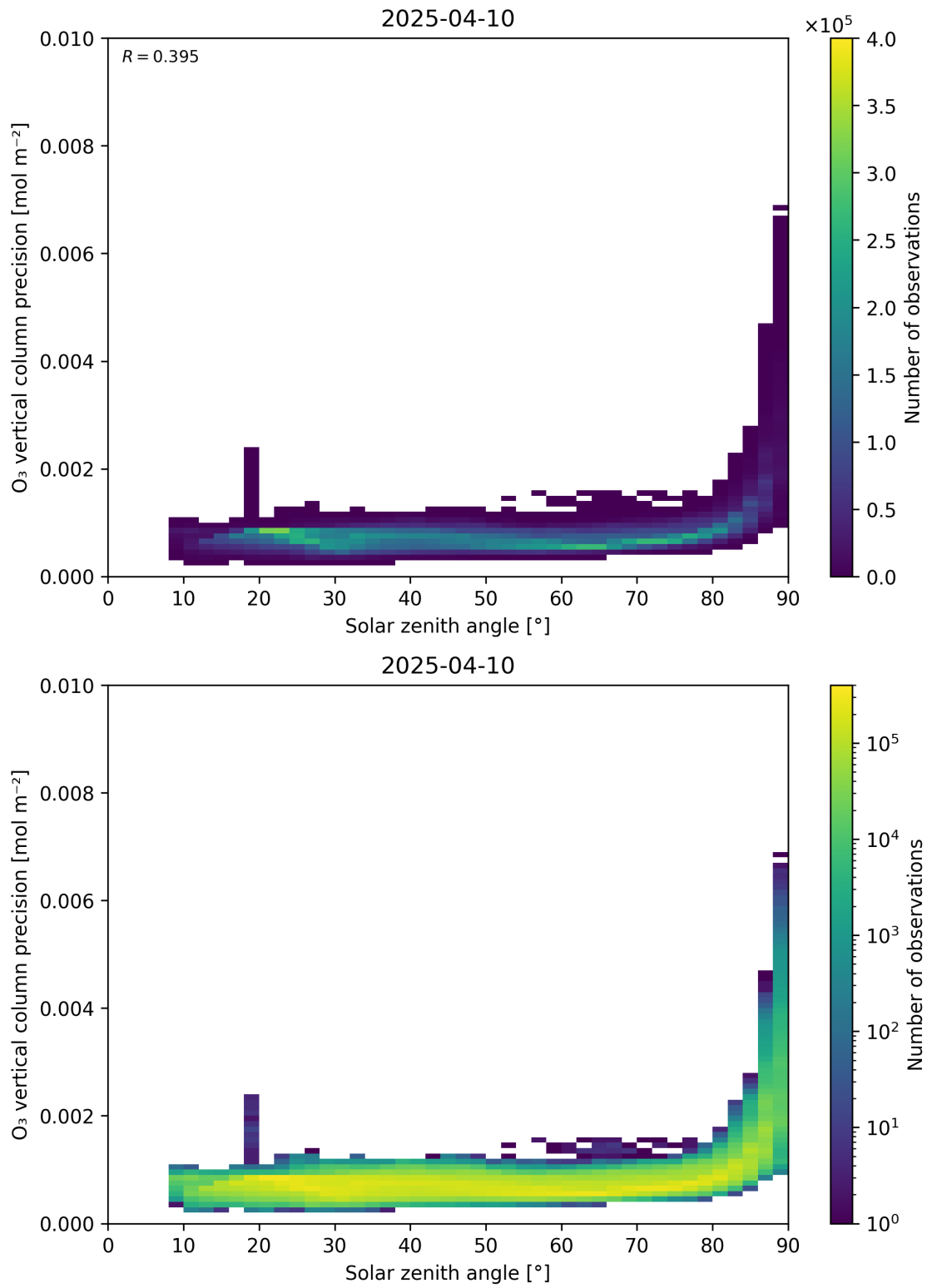
Figure 48: Scatter density plot of “Solar zenith angle” against “O 3 vertical column precision” for 2025-04-09 to 2025-04-11.
