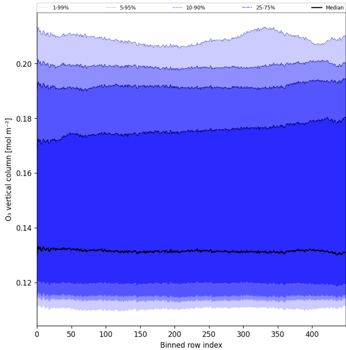
Figure 28: Along track statistics of “O 3 vertical column” for 2025-04-09 to 2025-04-11
