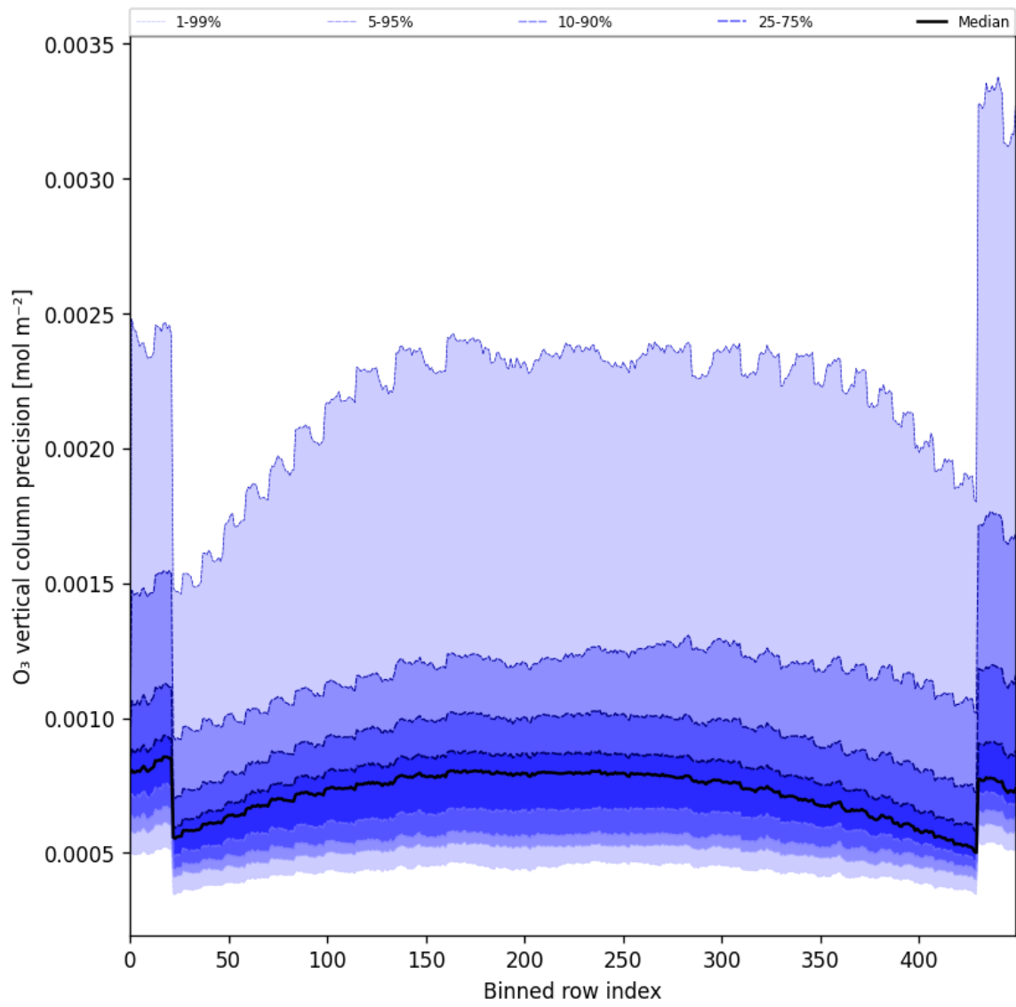
Figure 29: Along track statistics of “O 3 vertical column precision” for 2025-04-09 to 2025-04-11
