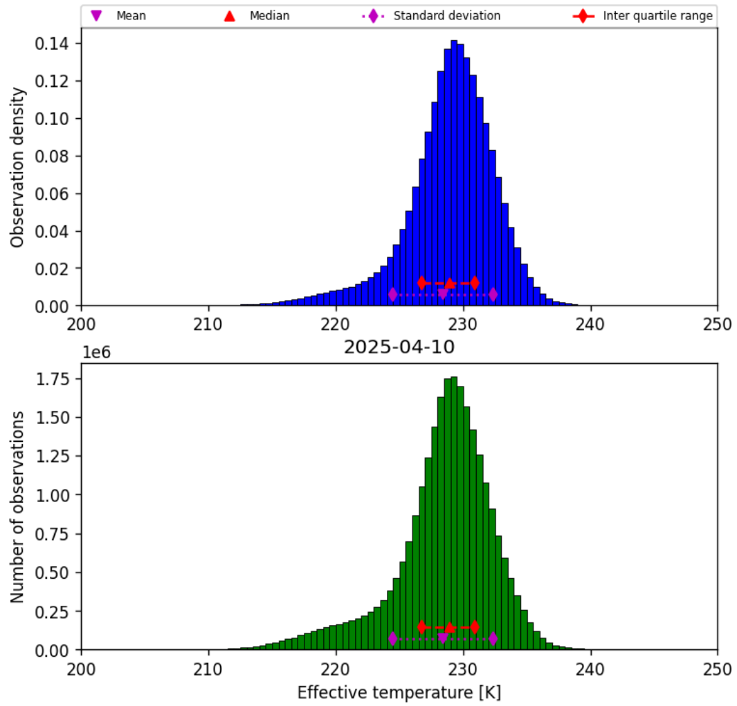
Figure 24: Histogram of “Effective temperature” for 2025-04-09 to 2025-04-11
