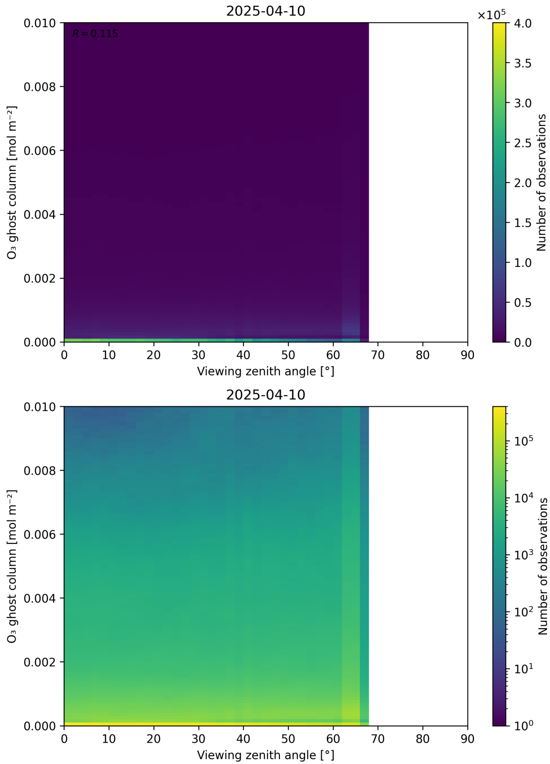
Figure 51: Scatter density plot of “Viewing zenith angle” against “O 3 ghost column” for 2025-04-09 to 2025-04-11.
