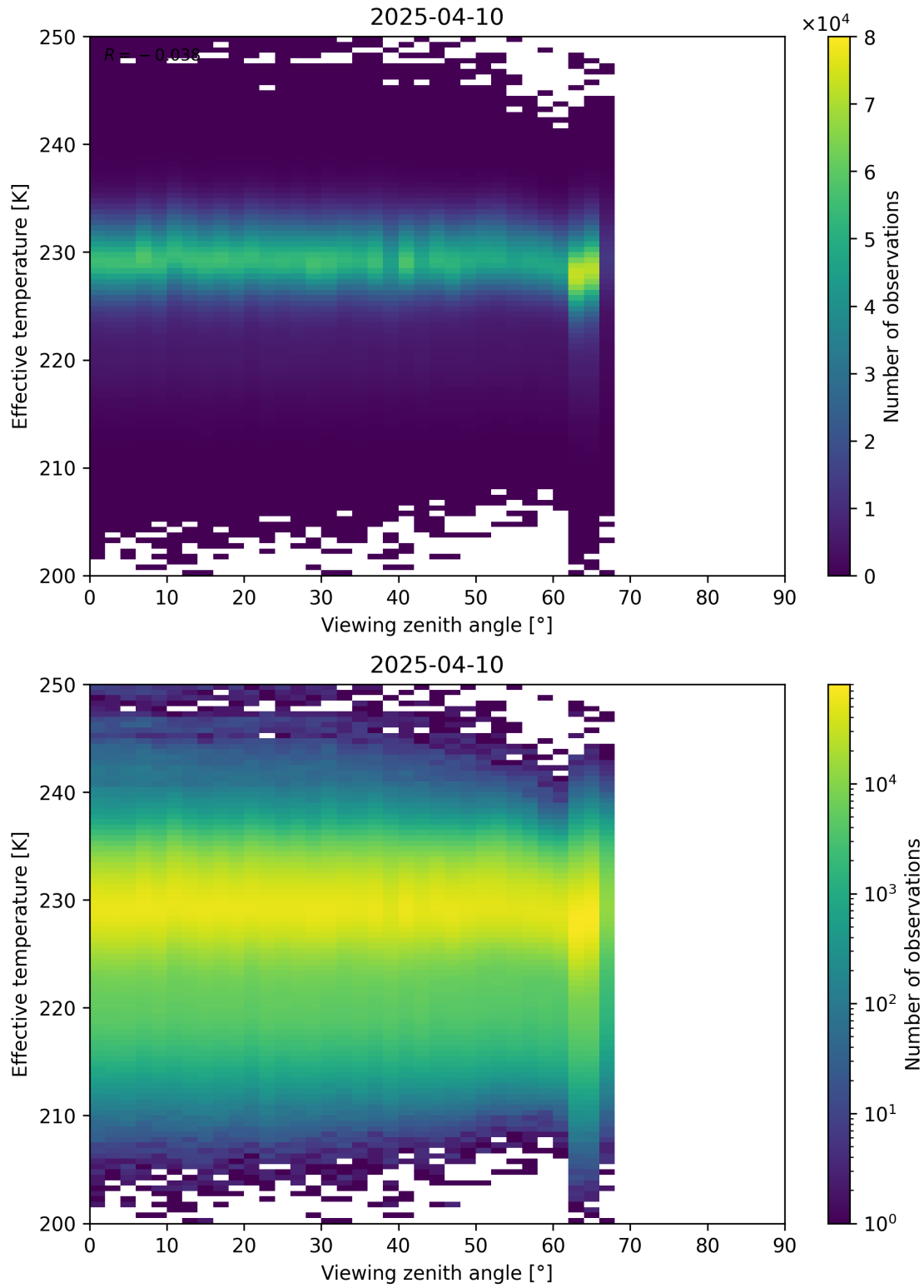
Figure 50: Scatter density plot of “Viewing zenith angle” against “Effective temperature” for 2025-04-09 to 2025-04-11.
