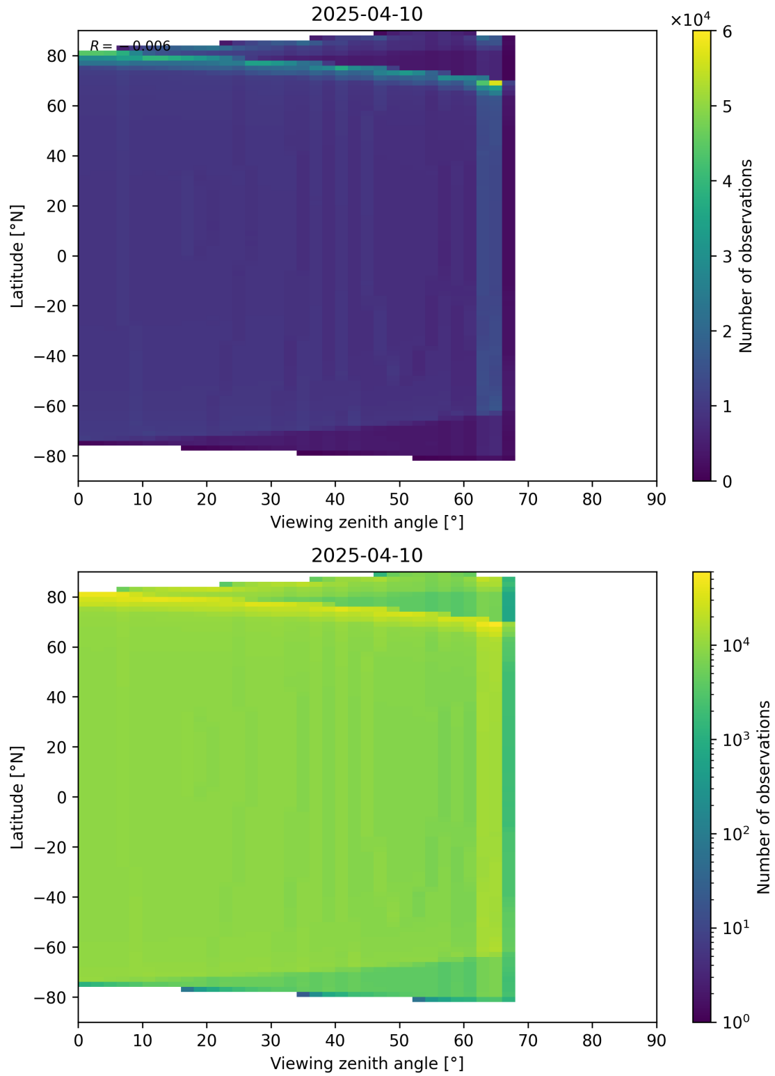
Figure 49: Scatter density plot of “Viewing zenith angle” against “Latitude” for 2025-04-09 to 2025-04-11.
