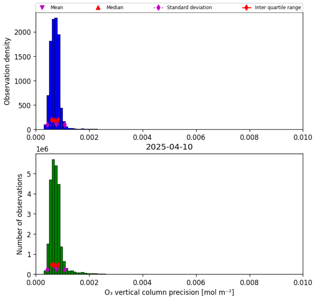
Figure 22: Histogram of "O 3 vertical column precision" for 2025-04-09 to 2025-04-11
