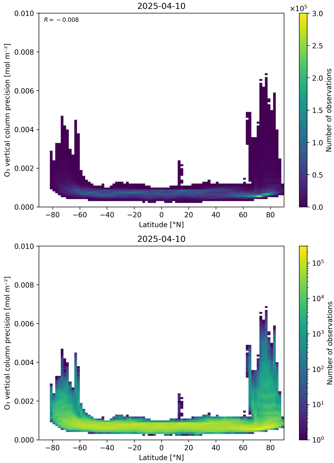
Figure 37: Scatter density plot of “Latitude” against “O 3 vertical column precision” for 2025-04-09 to 2025-04-11.
