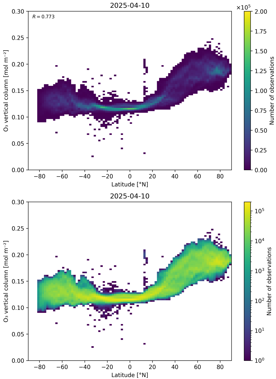
Figure 36: Scatter density plot of “Latitude” against “O 3 vertical column” for 2025-04-09 to 2025-04-11.
