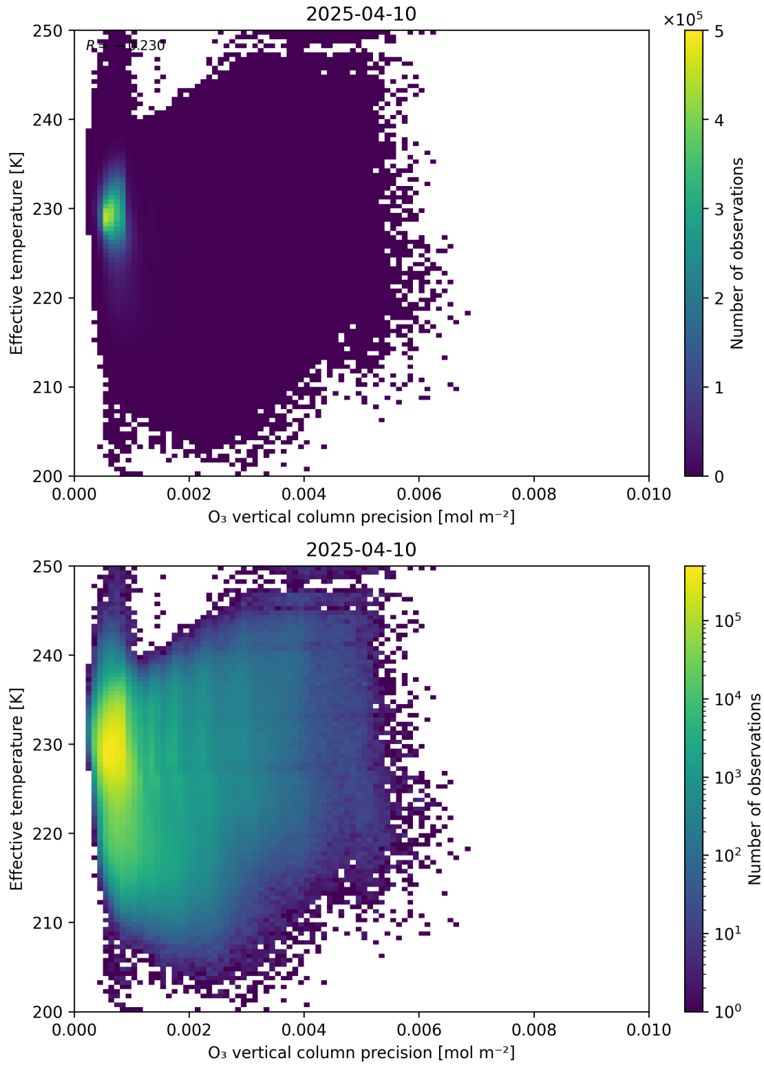
Figure 42: Scatter density plot of “O 3 vertical column precision” against “Effective temperature” for 2025-04-09 to 2025-04-11.
