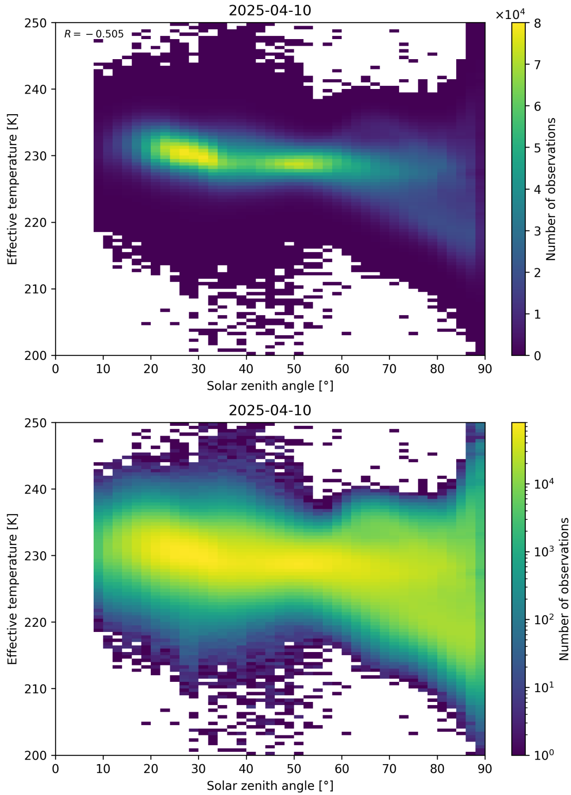
Figure 45: Scatter density plot of “Solar zenith angle” against “Effective temperature” for 2025-04-09 to 2025-04-11.
