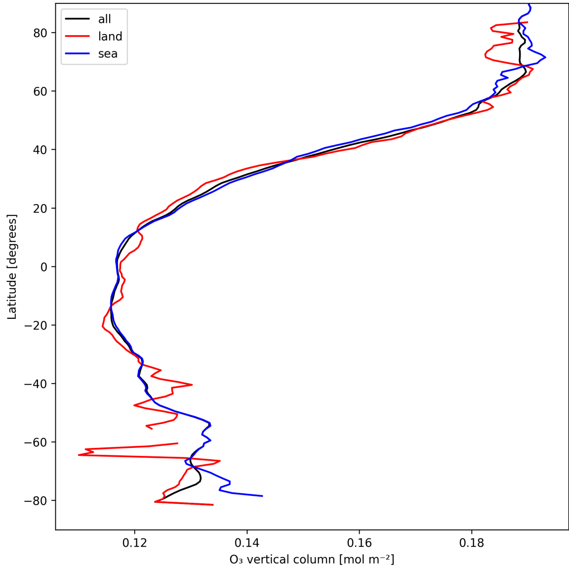
Figure 14: Zonal average of “O 3 vertical column” for 2025-04-09 to 2025-04-11.
