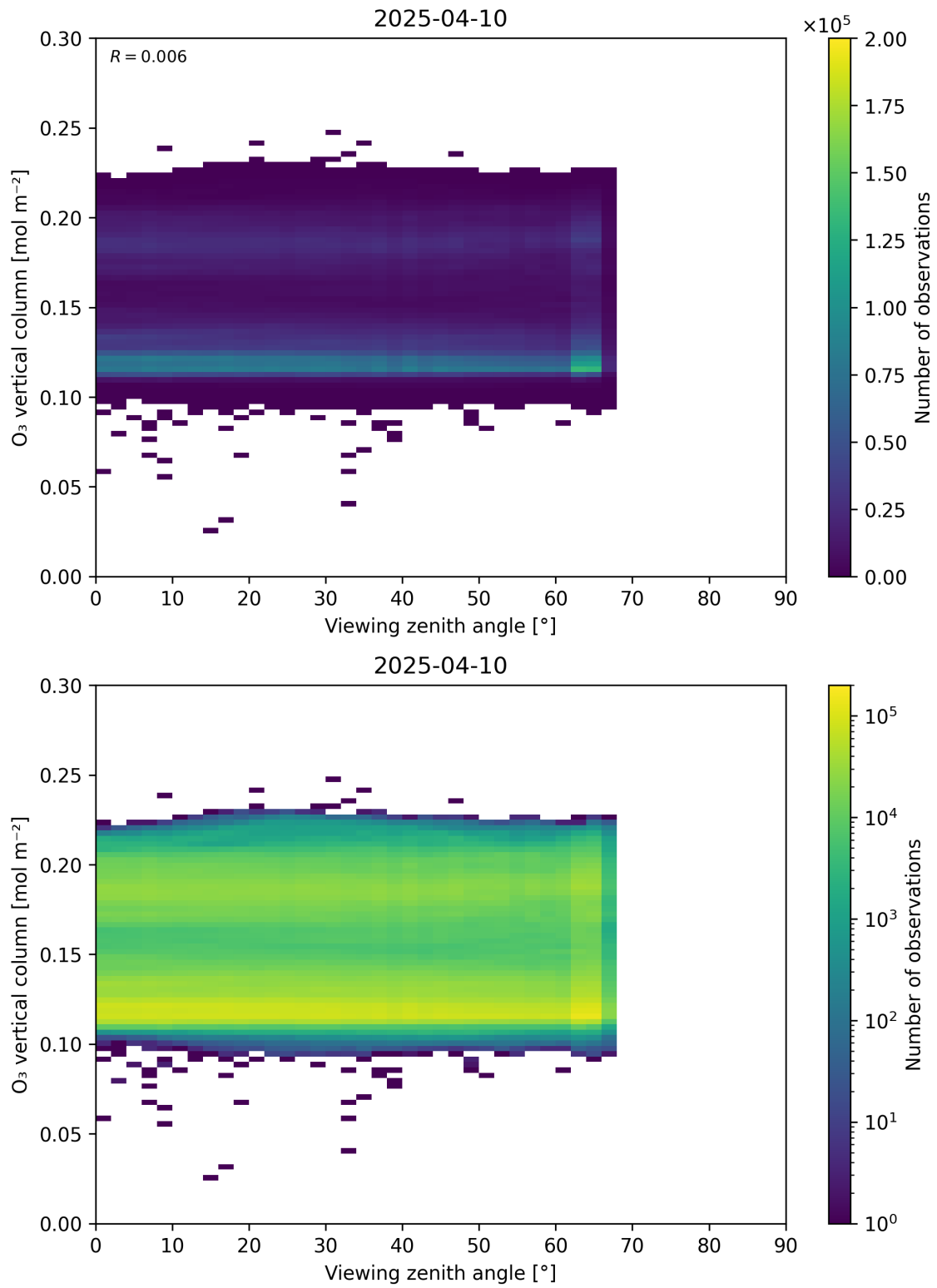
Figure 52: Scatter density plot of “Viewing zenith angle” against “O 3 vertical column” for 2025-04-09 to 2025-04-11.
