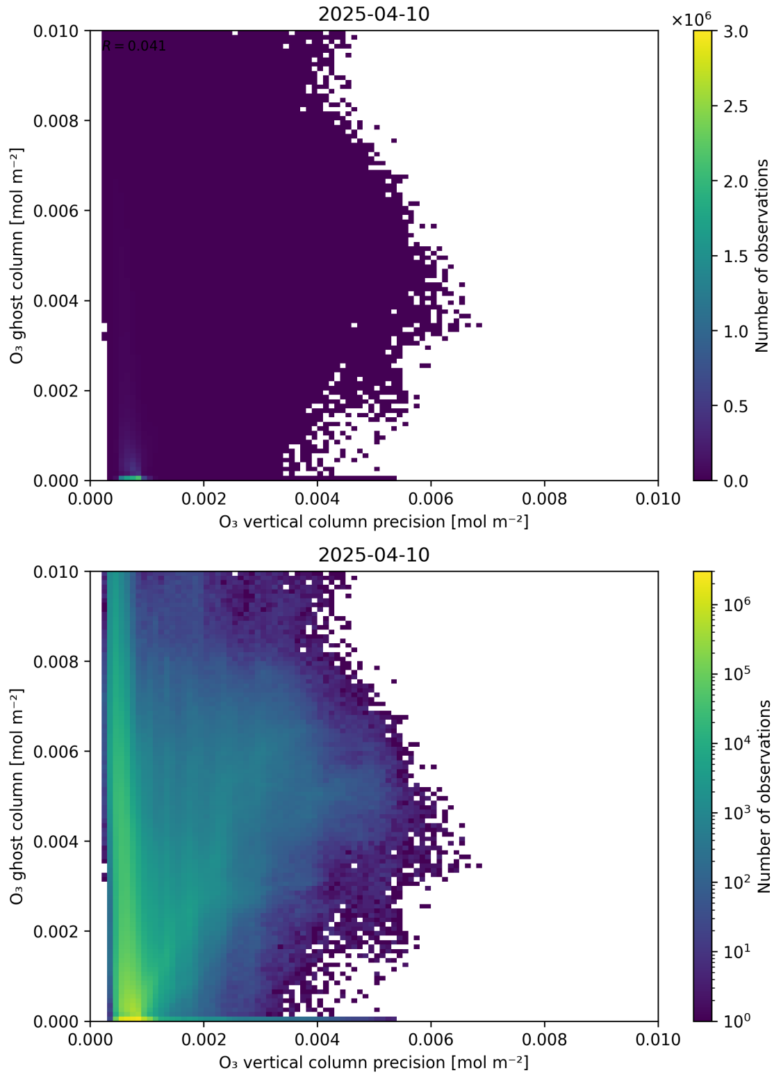
Figure 43: Scatter density plot of “O 3 vertical column precision” against “O 3 ghost column” for 2025-04-09 to 2025-04-11.
