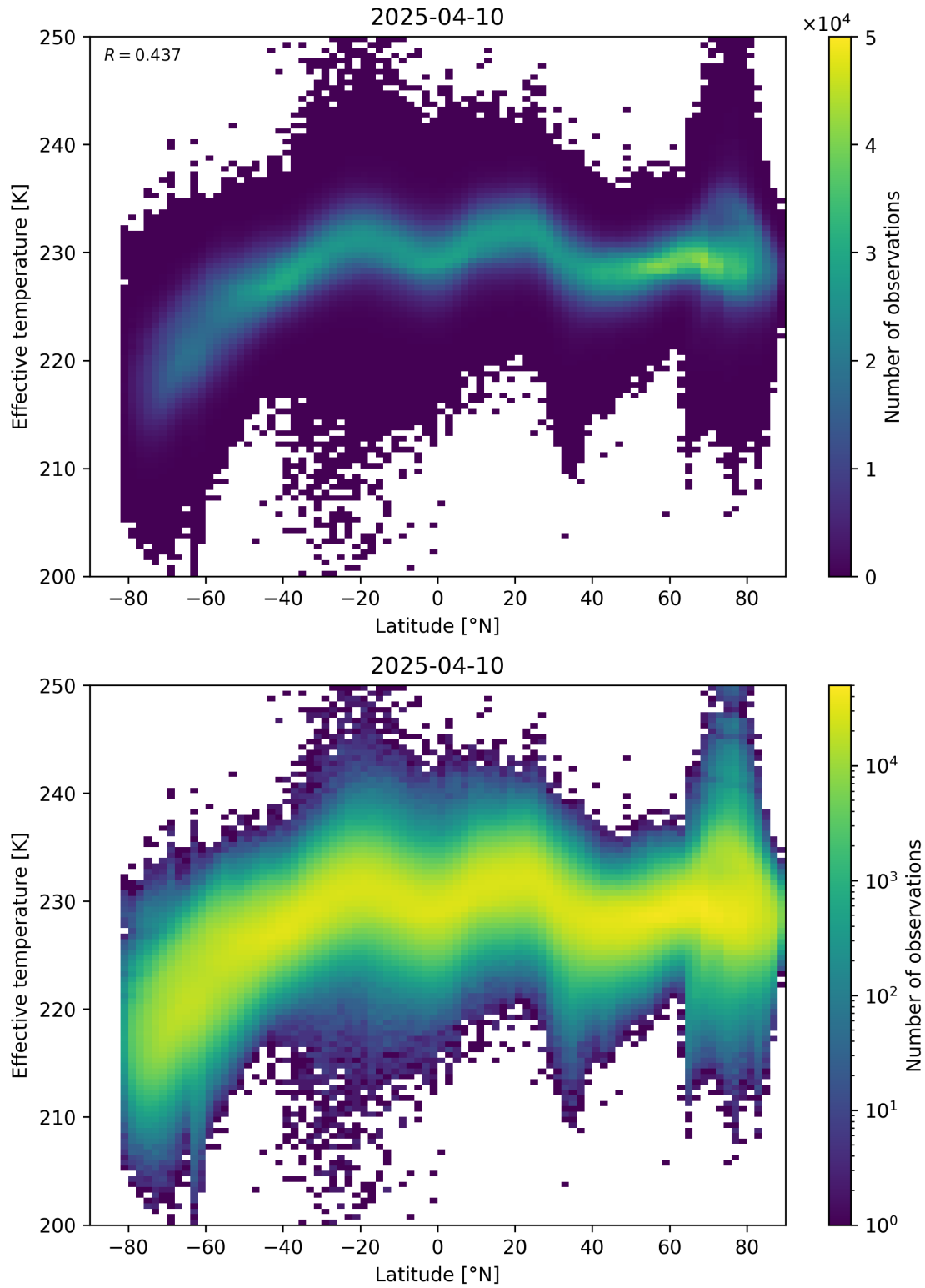
Figure 34: Scatter density plot of “Latitude” against “Effective temperature” for 2025-04-09 to 2025-04-11.
