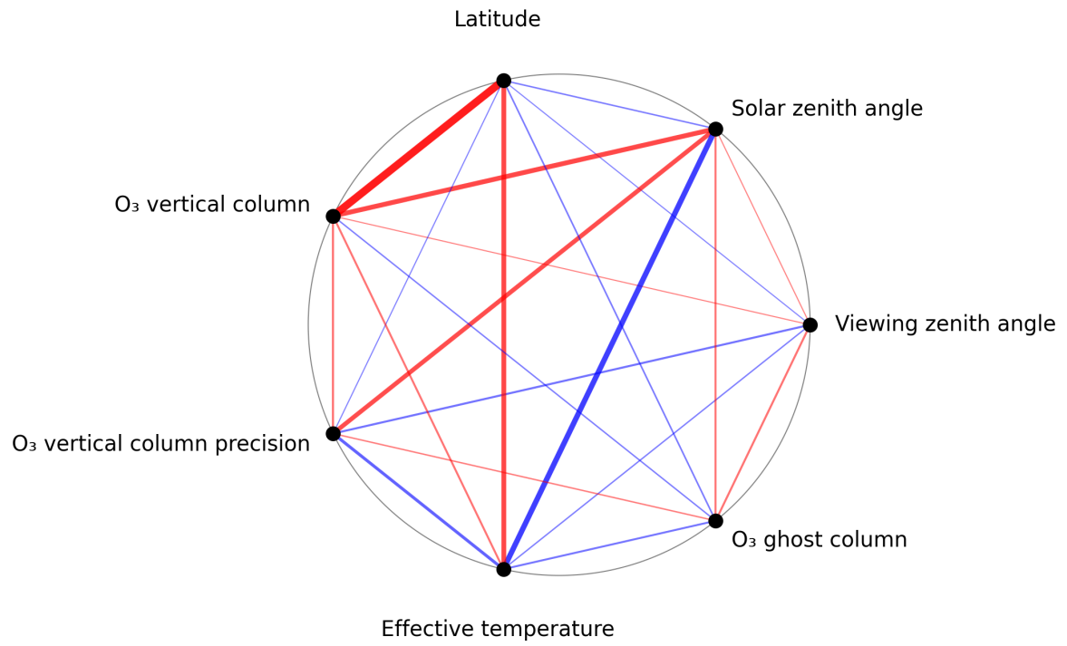
Figure 1: Map of correlation graph for 2025-04-09 to 2025-04-11.
