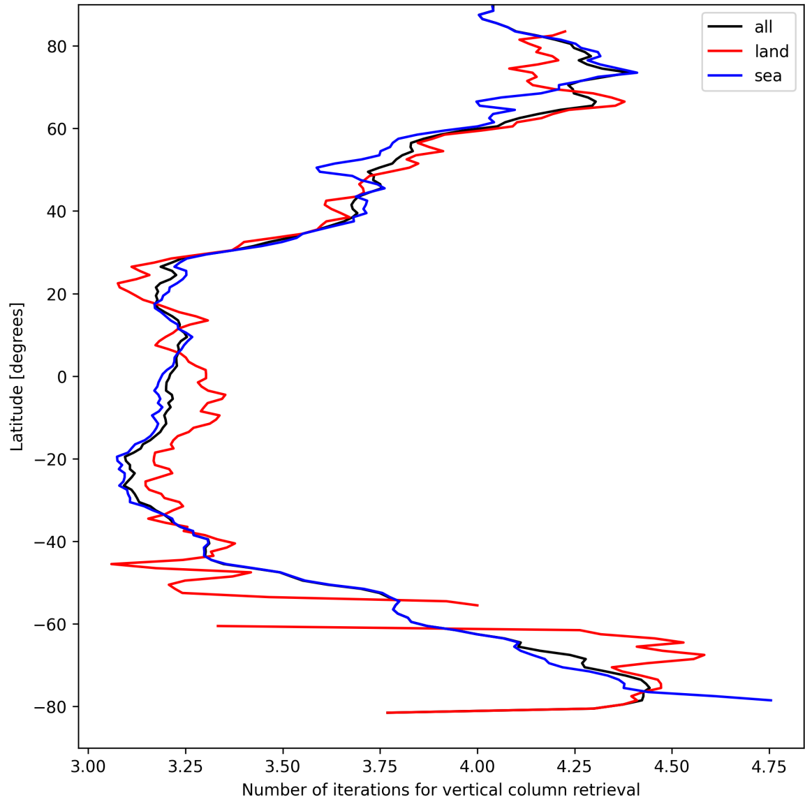
Figure 19: Zonal average of “Number of iterations for vertical column retrieval” for 2025-04-09 to 2025-04-11.
