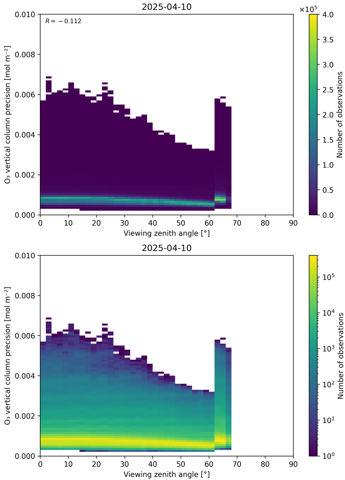
Figure 53: Scatter density plot of “Viewing zenith angle” against “O 3 vertical column precision” for 2025-04-09 to 2025-04-11.
