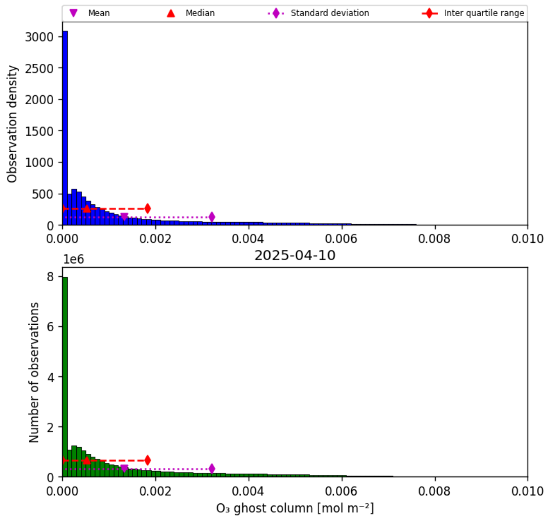
Figure 25: Histogram of “O 3 ghost column” for 2025-04-09 to 2025-04-11
