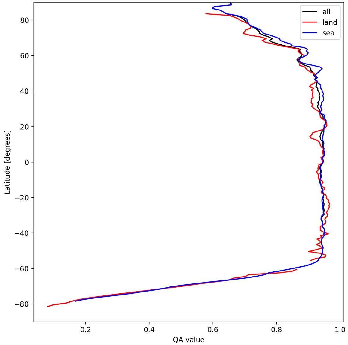
Figure 13: Zonal average of “QA value” for 2025-04-09 to 2025-04-11.
