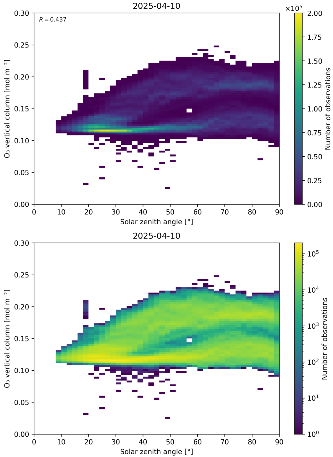
Figure 47: Scatter density plot of “Solar zenith angle” against “O 3 vertical column” for 2025-04-09 to 2025-04-11.
