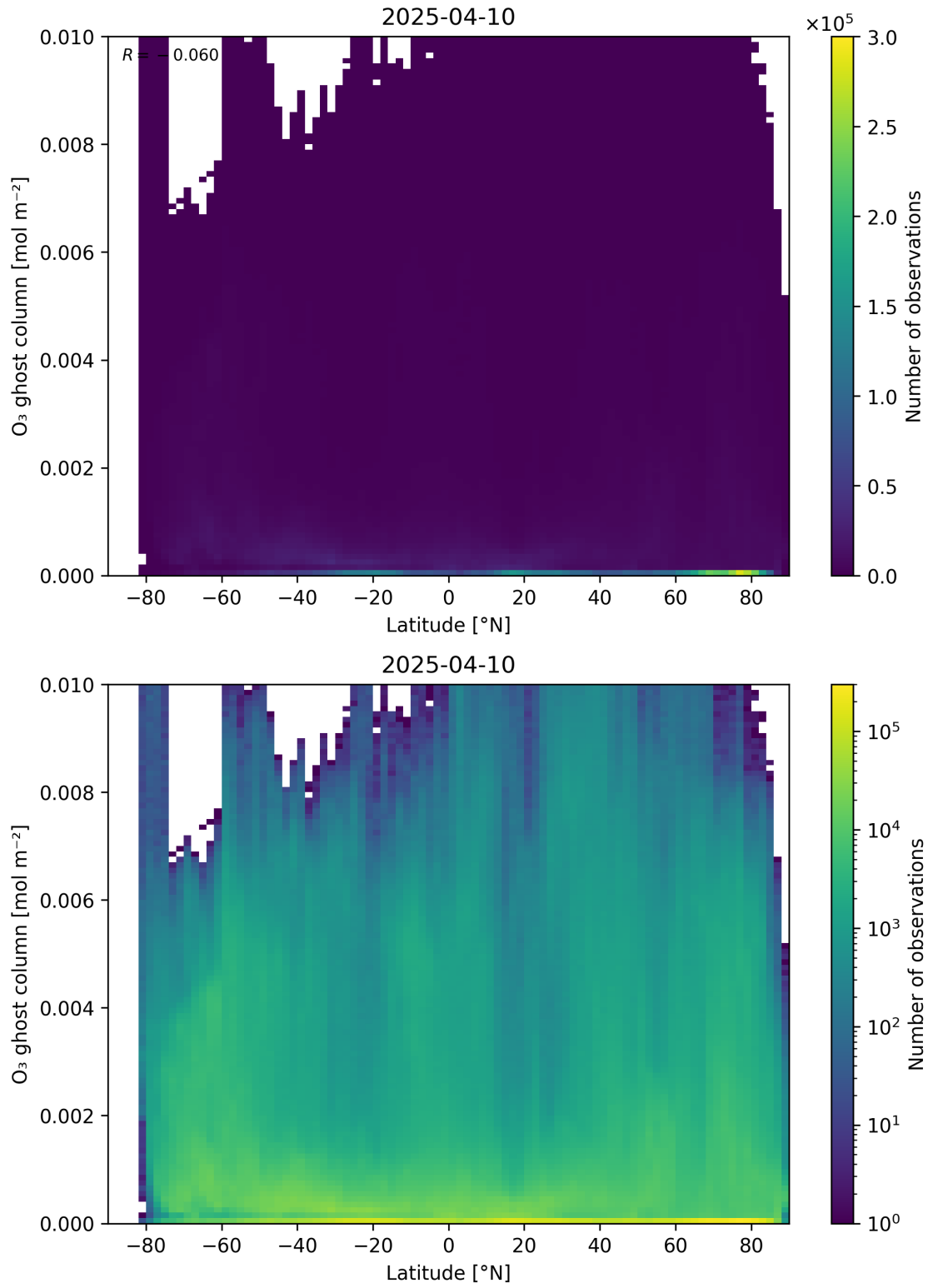
Figure 35: Scatter density plot of “Latitude” against “O 3 ghost column” for 2025-04-09 to 2025-04-11.
