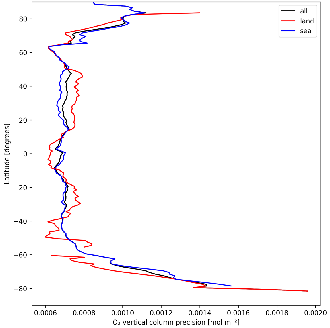
Figure 15: Zonal average of “O 3 vertical column precision” for 2025-04-09 to 2025-04-11.
