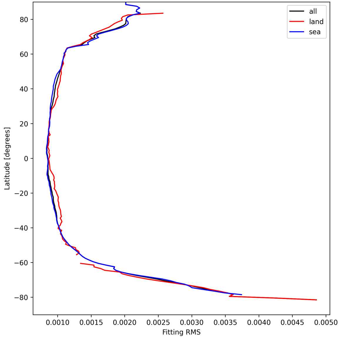
Figure 16: Zonal average of “Fitting RMS” for 2025-04-09 to 2025-04-11.
