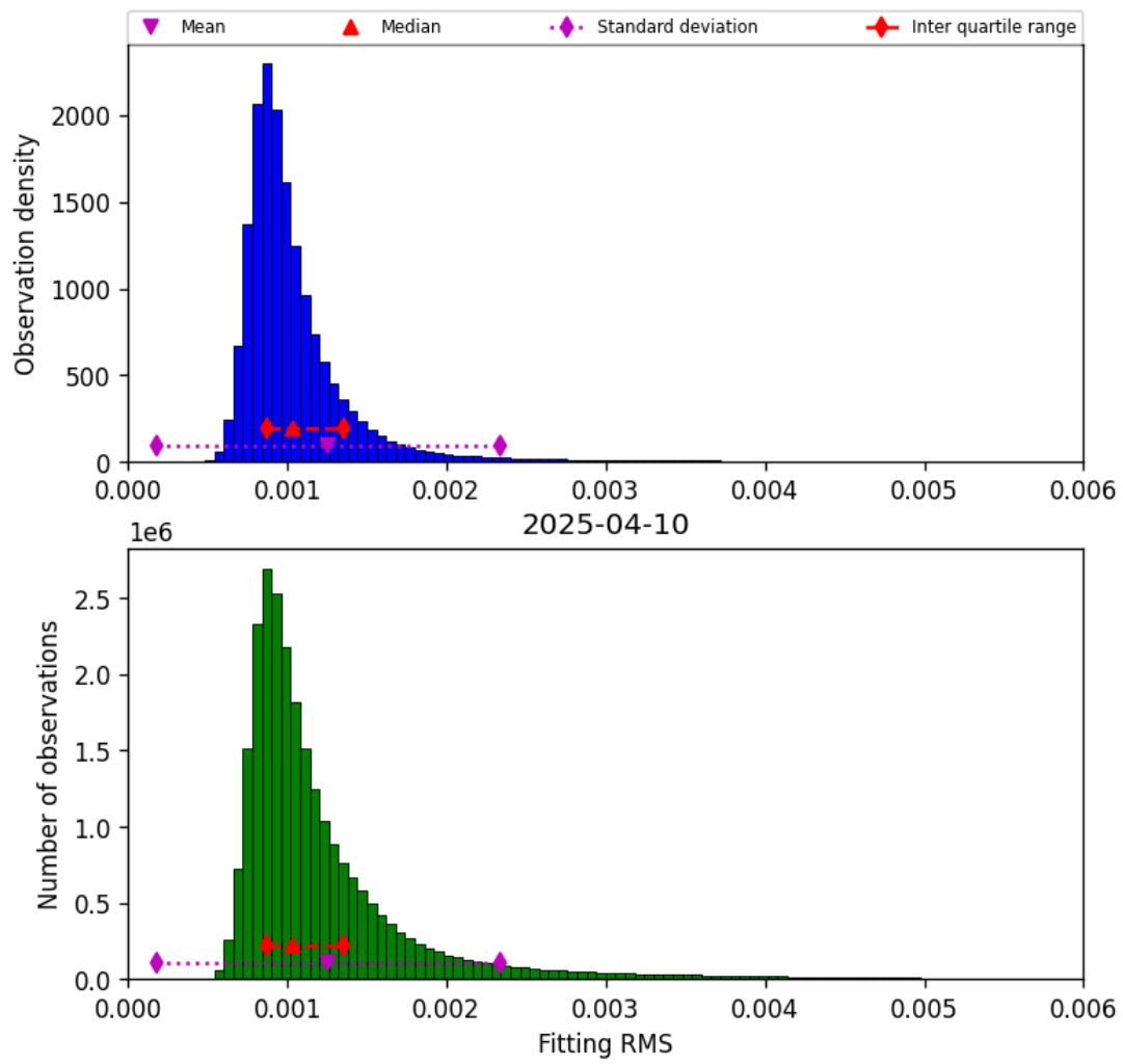
Figure 23: Histogram of “Fitting RMS” for 2025-04-09 to 2025-04-11
