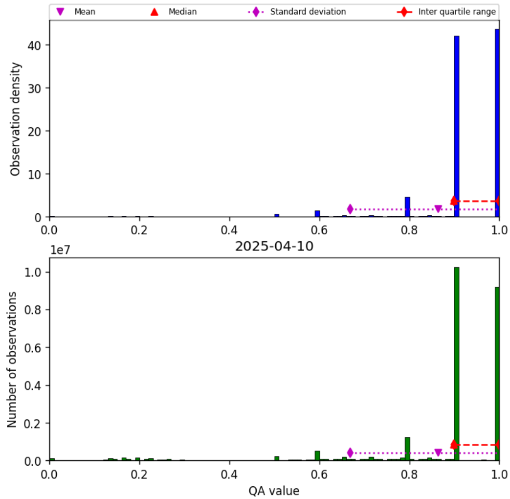
Figure 20: Histogram of “QA value” for 2025-04-09 to 2025-04-11
