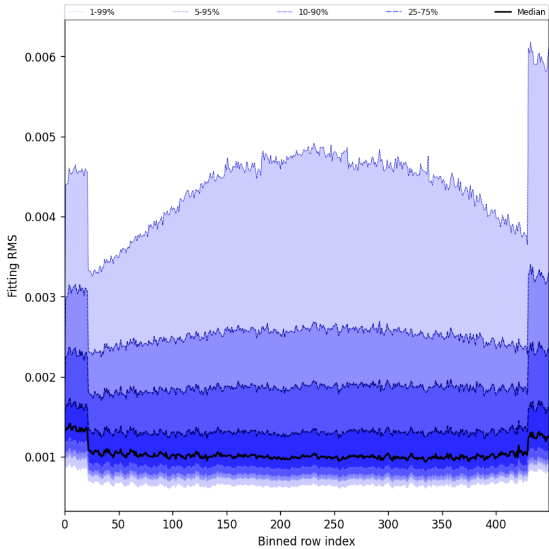
Figure 30: Along track statistics of “Fitting RMS” for 2025-04-09 to 2025-04-11
