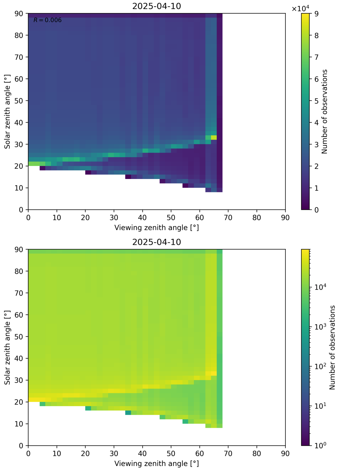
Figure 54: Scatter density plot of “Viewing zenith angle” against “Solar zenith angle” for 2025-04-09 to 2025-04-11.
