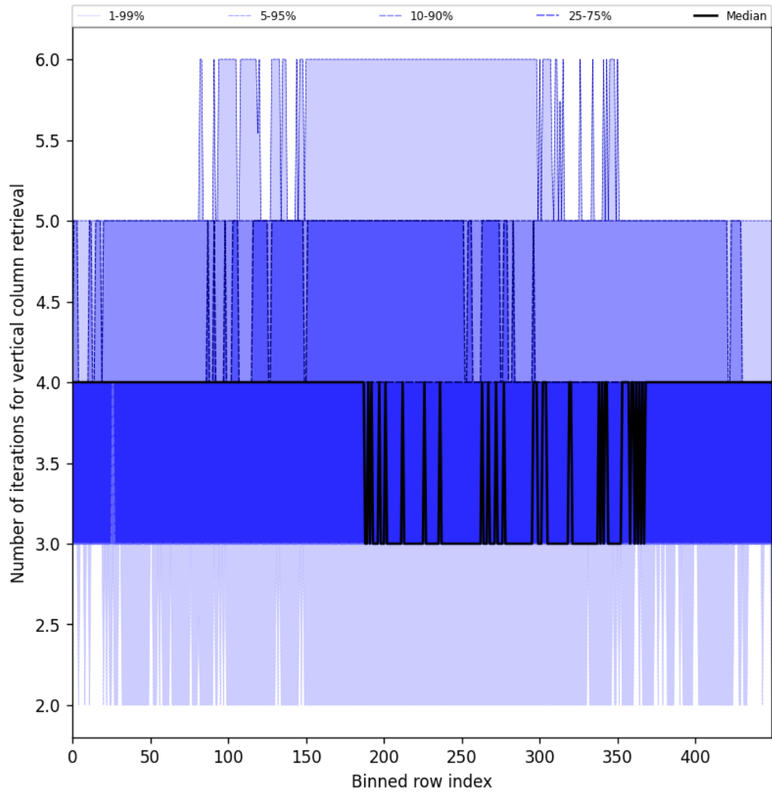
Figure 33: Along track statistics of “Number of iterations for vertical column retrieval” for 2025-04-09 to 2025-04-11
