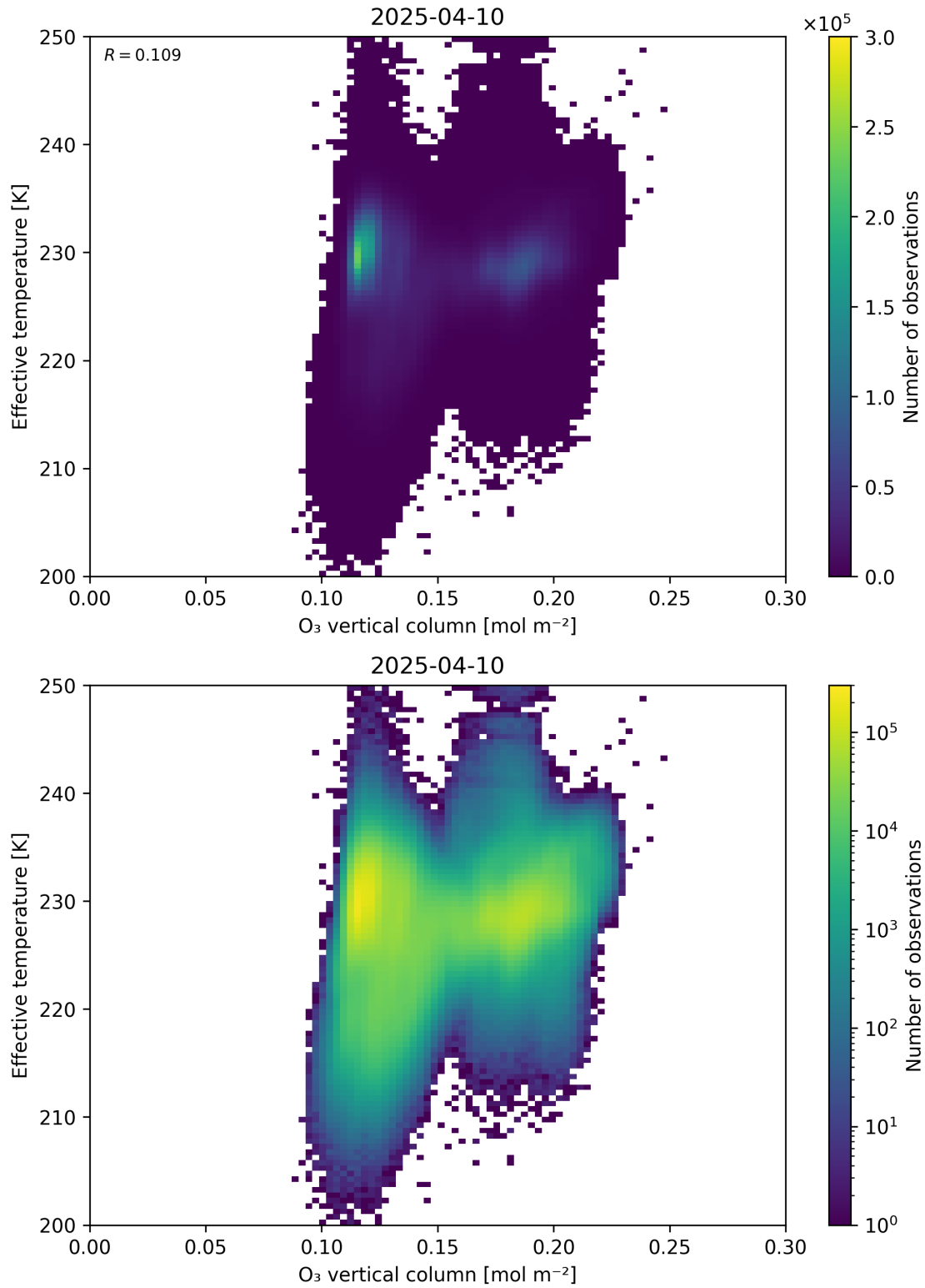
Figure 39: Scatter density plot of “O 3 vertical column” against “Effective temperature” for 2025-04-09 to 2025-04-11.
