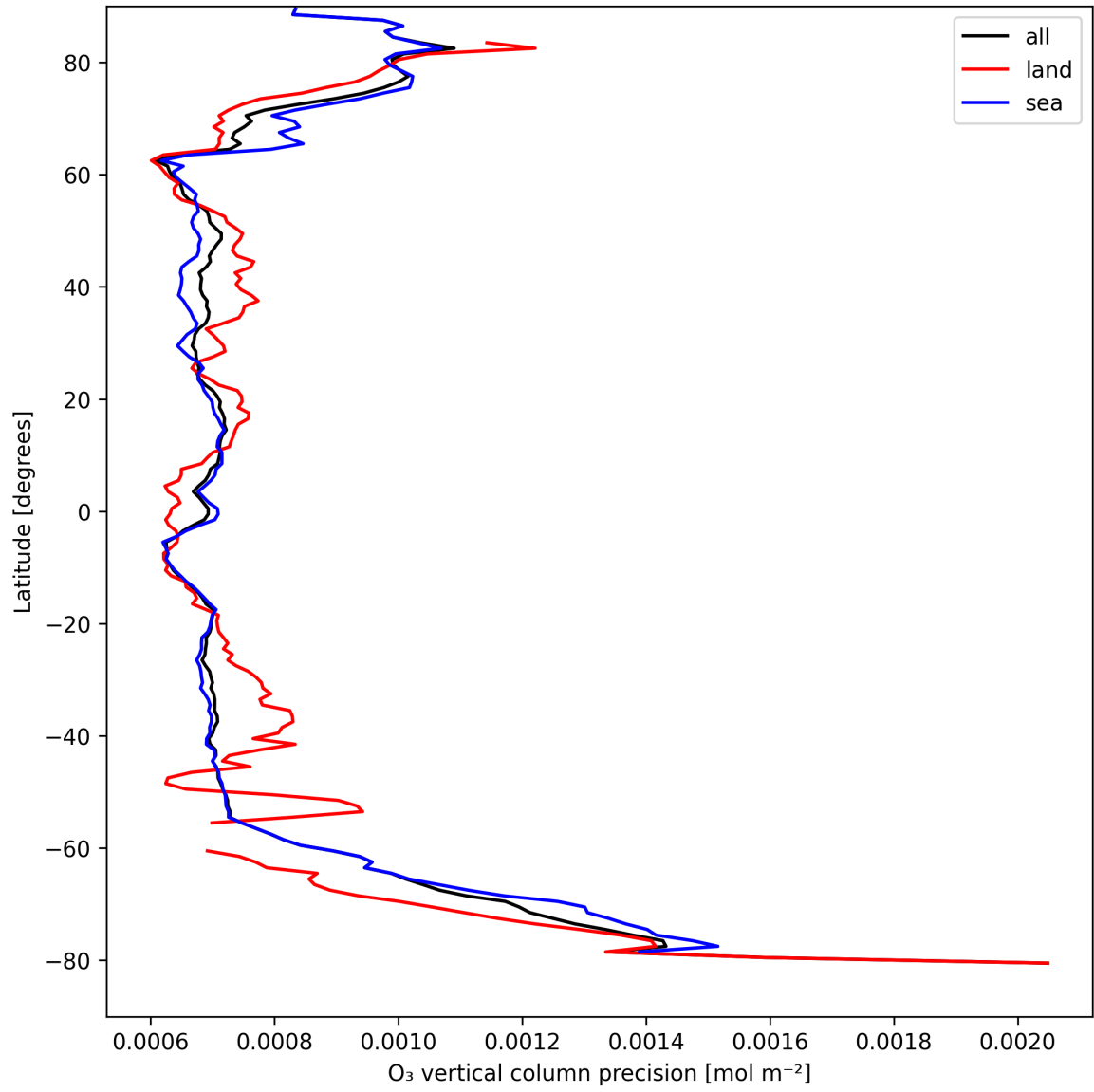
Figure 15: Zonal average of “O 3 vertical column precision” for 2025-04-11 to 2025-04-13.
