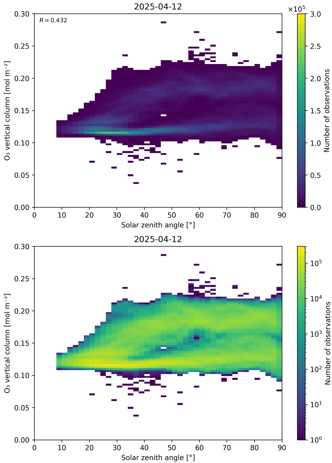
Figure 47: Scatter density plot of “Solar zenith angle” against “O 3 vertical column” for 2025-04-11 to 2025-04-13.
