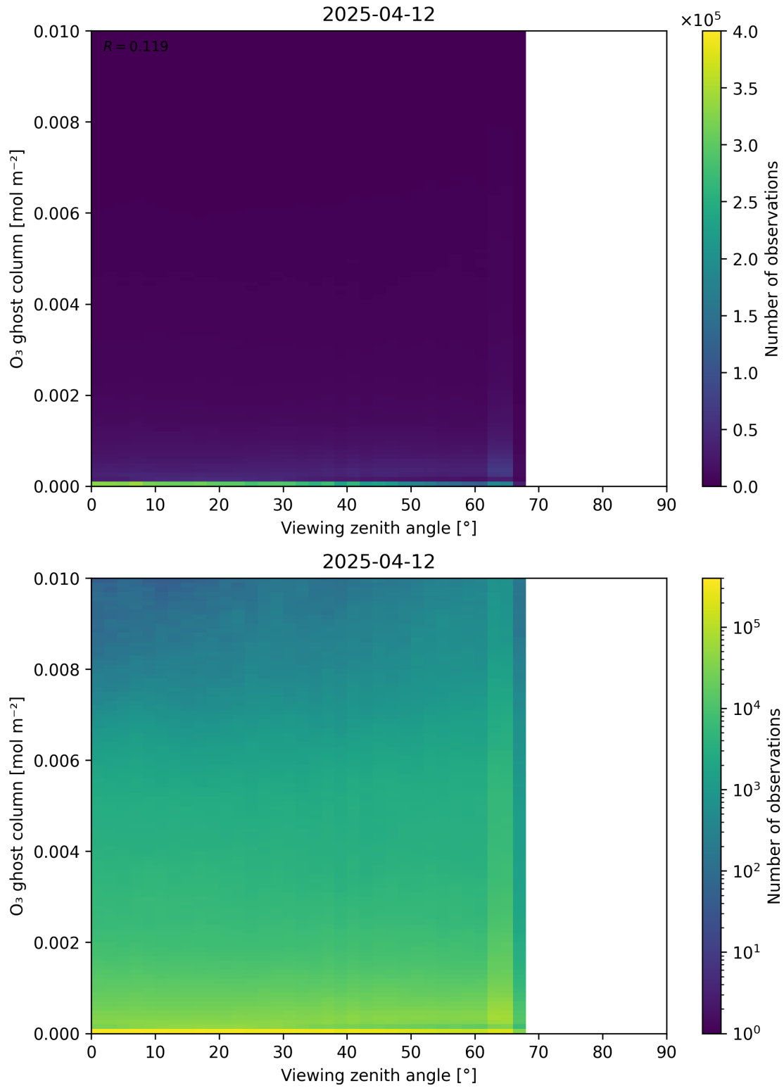
Figure 51: Scatter density plot of “Viewing zenith angle” against “O 3 ghost column” for 2025-04-11 to 2025-04-13.
