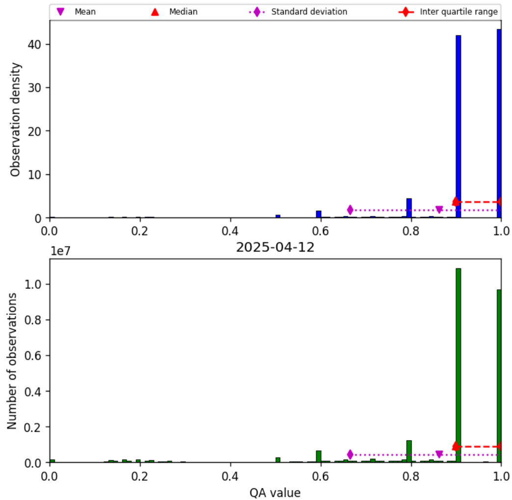
Figure 20: Histogram of “QA value” for 2025-04-11 to 2025-04-13
