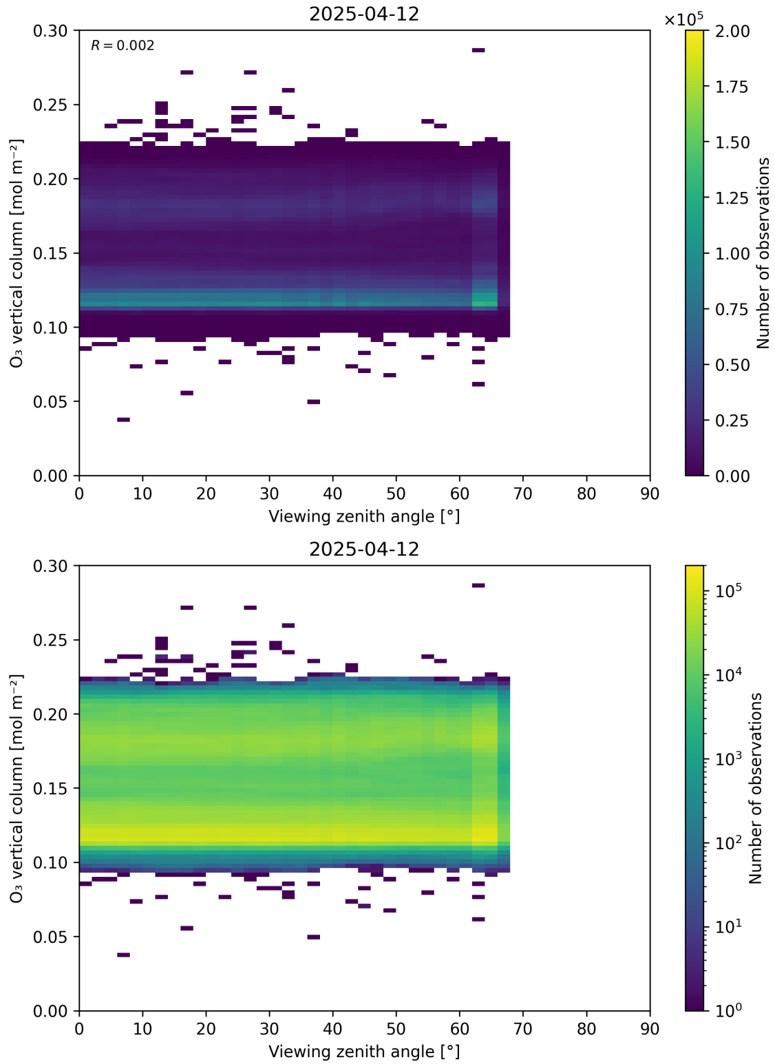
Figure 52: Scatter density plot of “Viewing zenith angle” against “O 3 vertical column” for 2025-04-11 to 2025-04-13.
