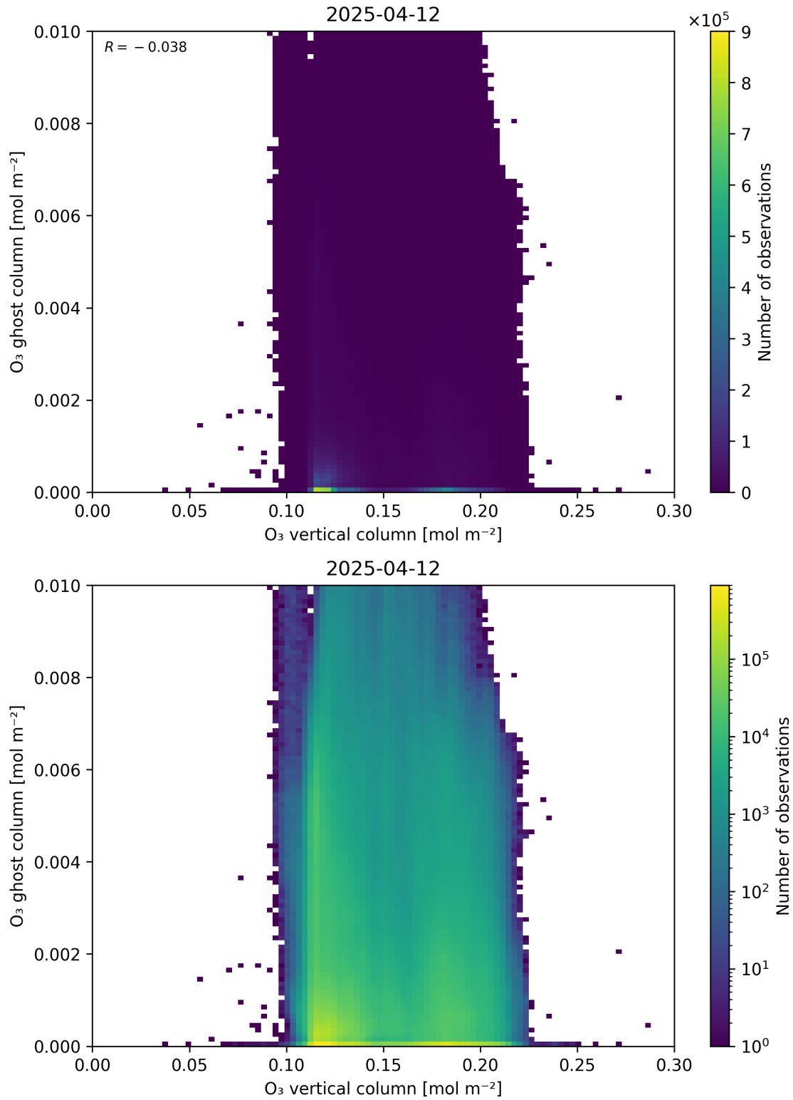
Figure 40: Scatter density plot of “ O_3 vertical column” against “ O_3 ghost column” for 2025-04-11 to 2025-04-13.
