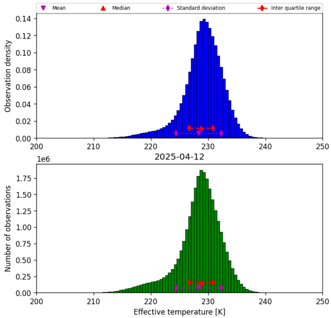
Figure 24: Histogram of “Effective temperature” for 2025-04-11 to 2025-04-13
