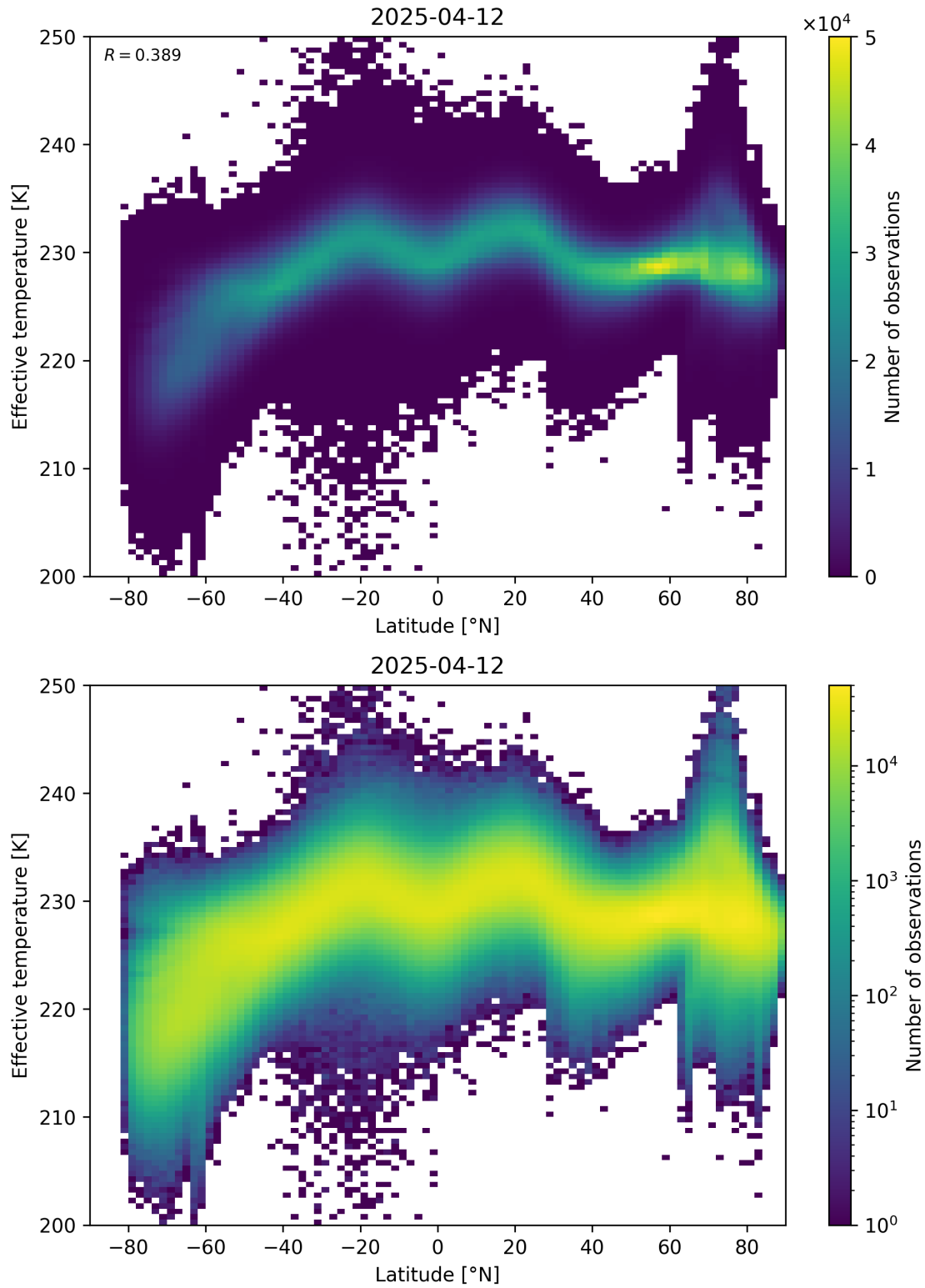
Figure 34: Scatter density plot of “Latitude” against “Effective temperature” for 2025-04-11 to 2025-04-13.
