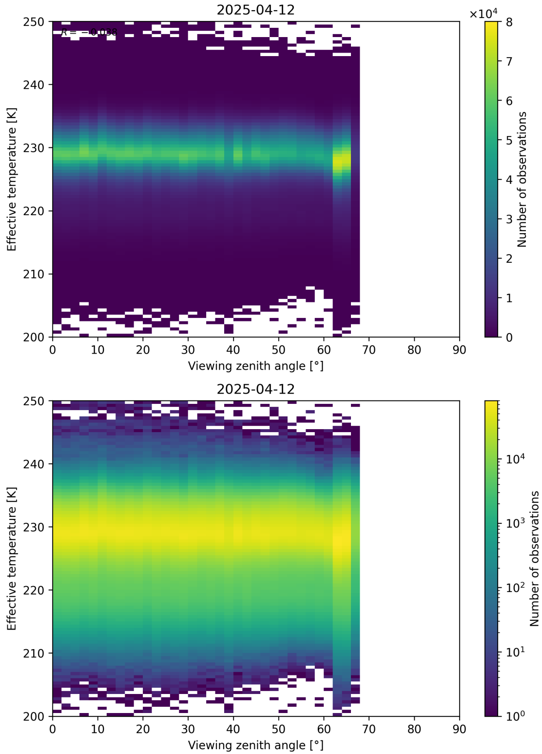
Figure 50: Scatter density plot of “Viewing zenith angle” against “Effective temperature” for 2025-04-11 to 2025-04-13.
