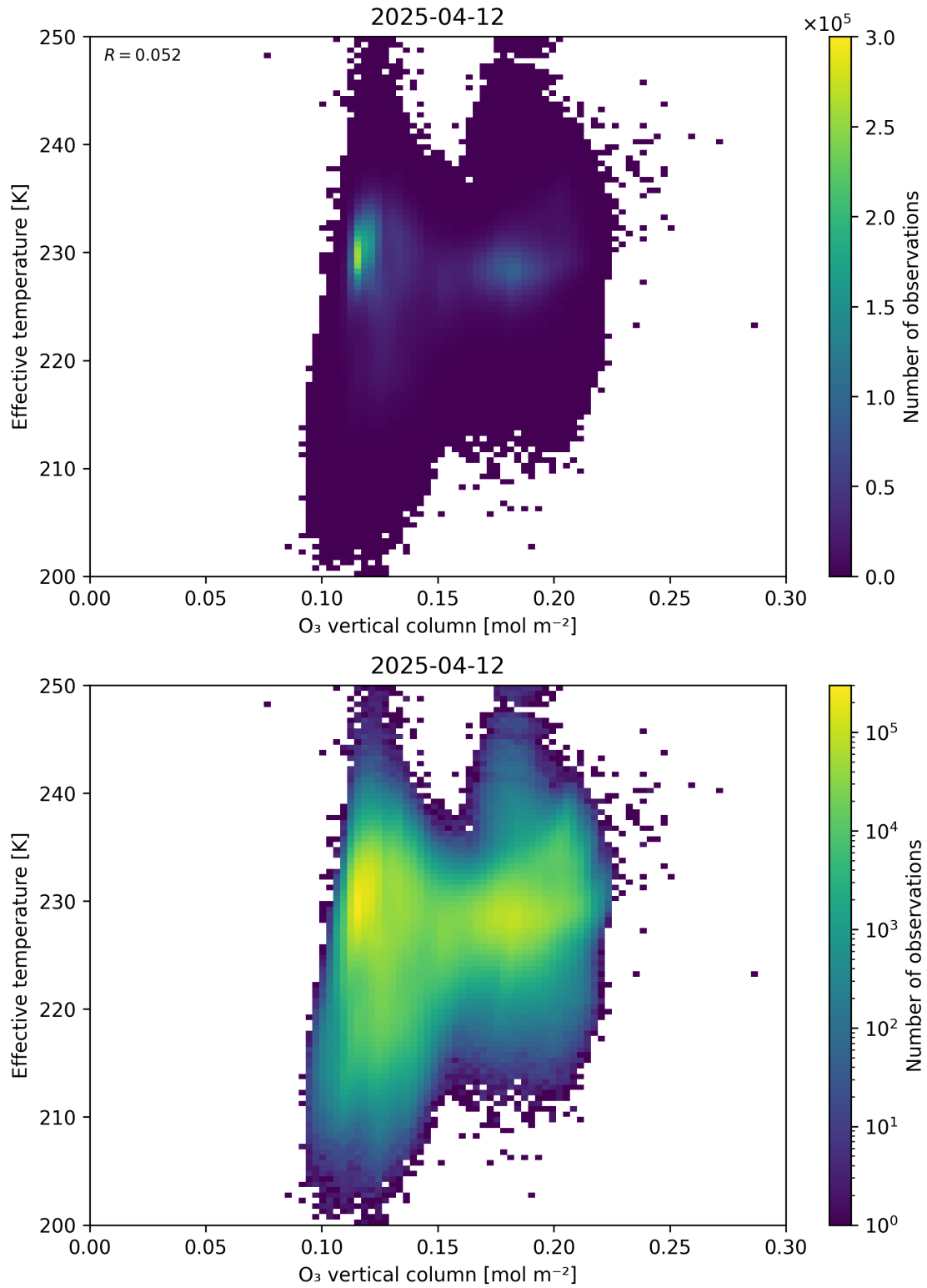
Figure 39: Scatter density plot of “O 3 vertical column” against “Effective temperature” for 2025-04-11 to 2025-04-13.
