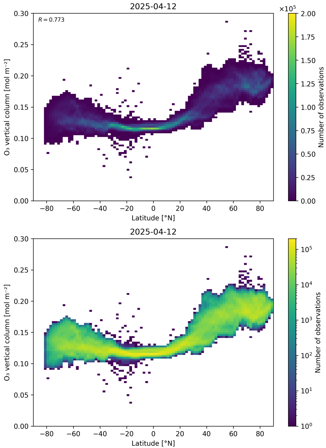
Figure 36: Scatter density plot of “Latitude” against “O 3 vertical column” for 2025-04-11 to 2025-04-13.
