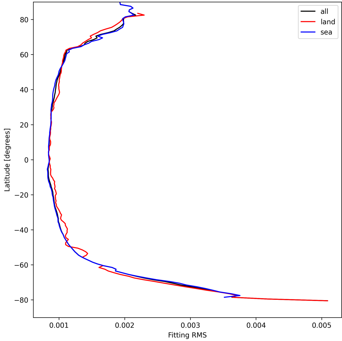
Figure 16: Zonal average of “Fitting RMS” for 2025-04-11 to 2025-04-13.
