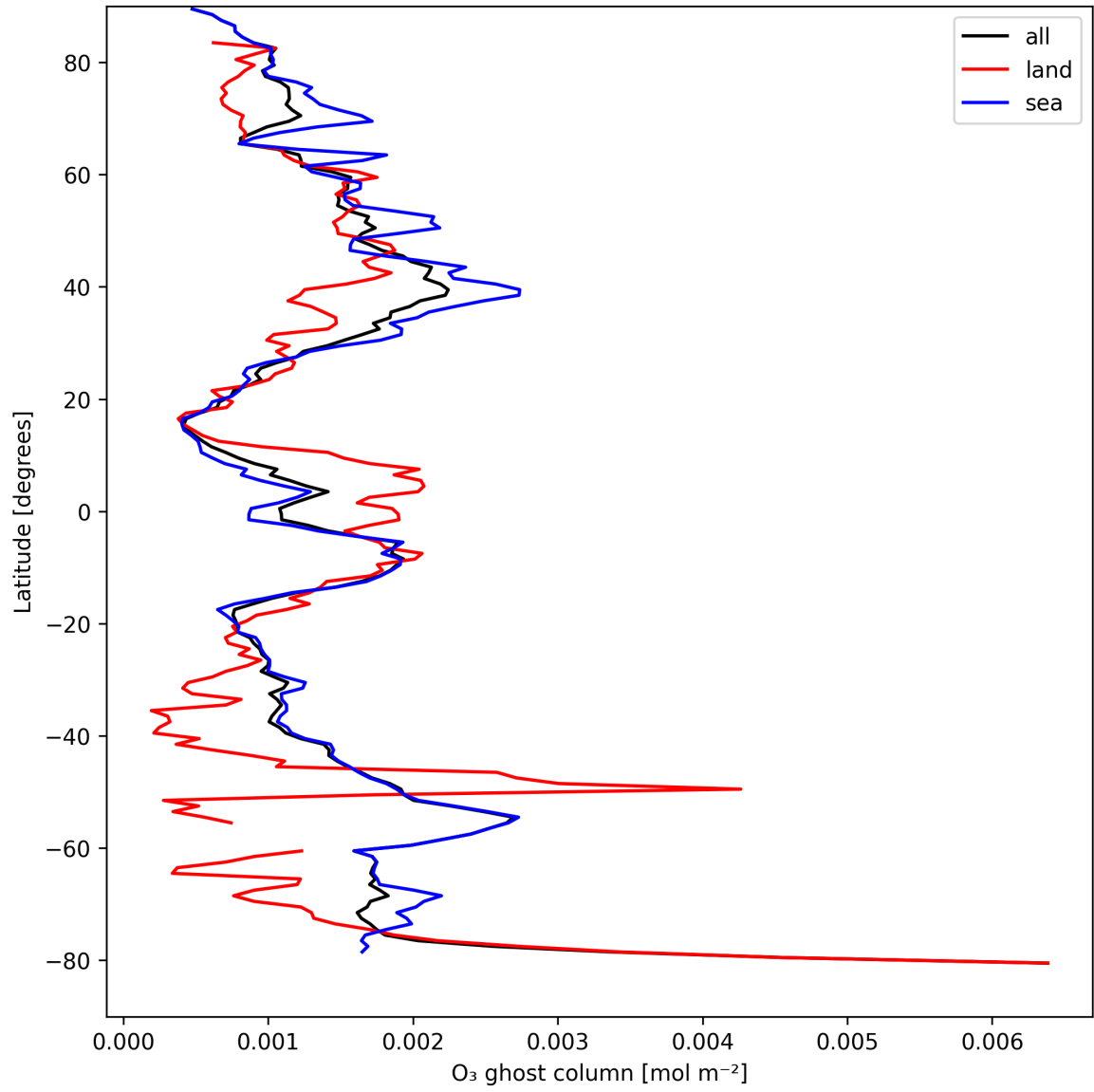
Figure 18: Zonal average of “O 3 ghost column” for 2025-04-11 to 2025-04-13.
