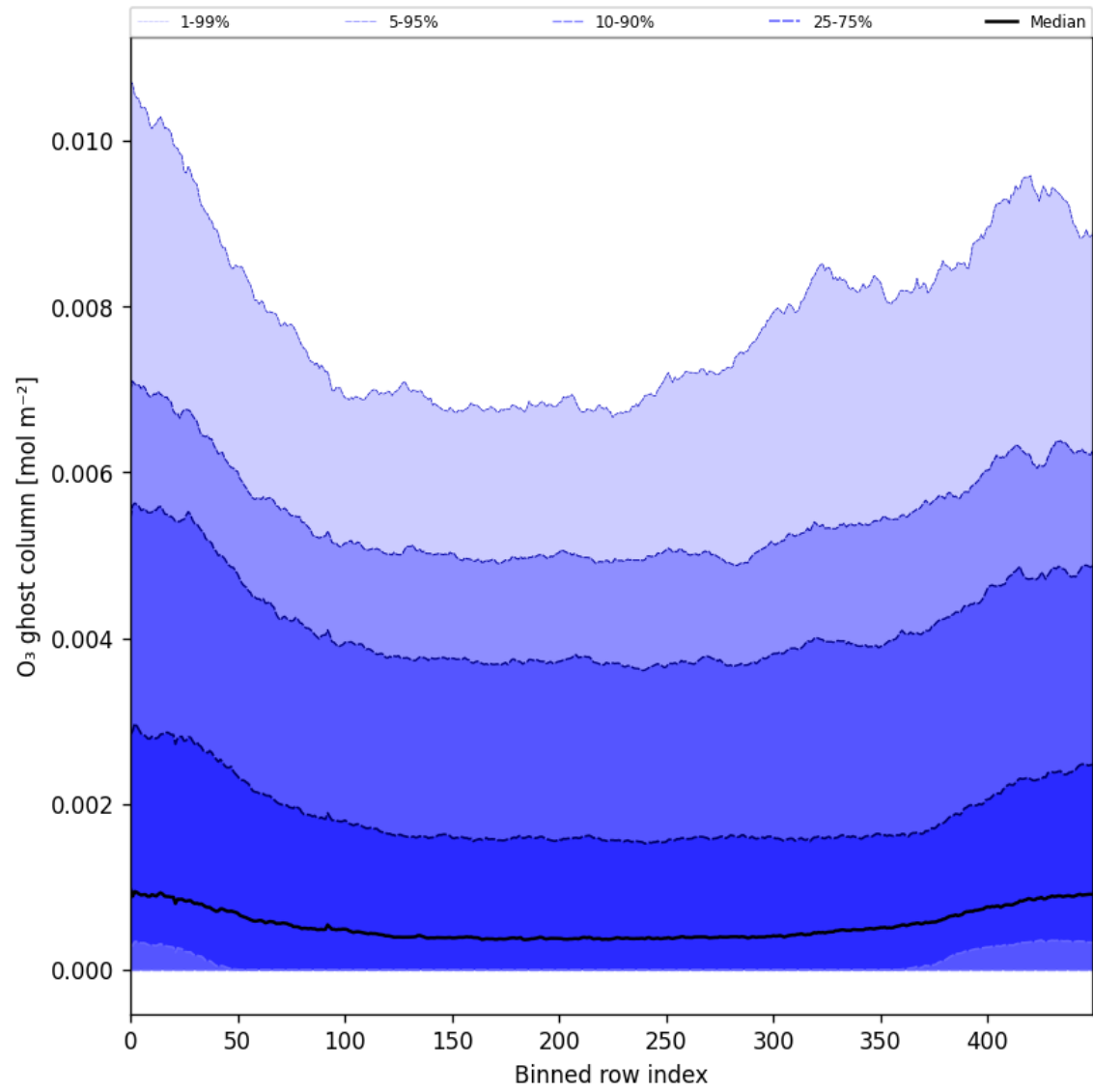
Figure 32: Along track statistics of “O 3 ghost column” for 2025-04-11 to 2025-04-13
