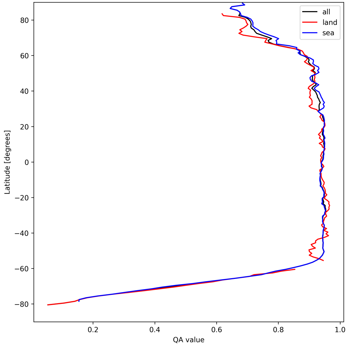
Figure 13: Zonal average of “QA value” for 2025-04-11 to 2025-04-13.
