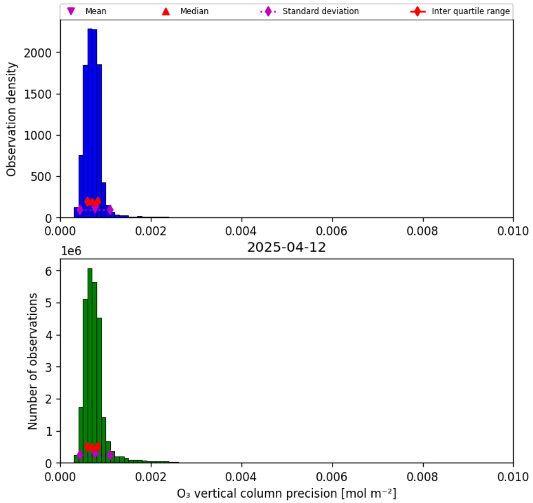
Figure 22: Histogram of “O 3 vertical column precision” for 2025-04-11 to 2025-04-13
