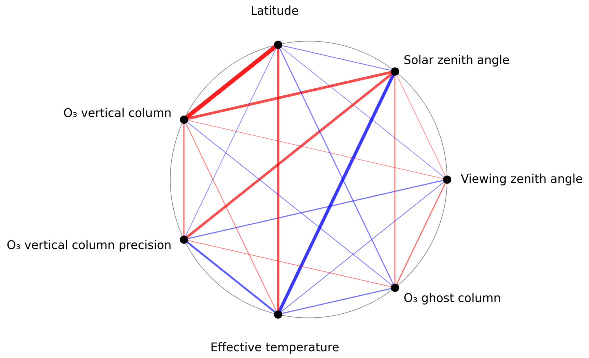
Figure 1: Map of correlation graph for 2025-04-11 to 2025-04-13.
