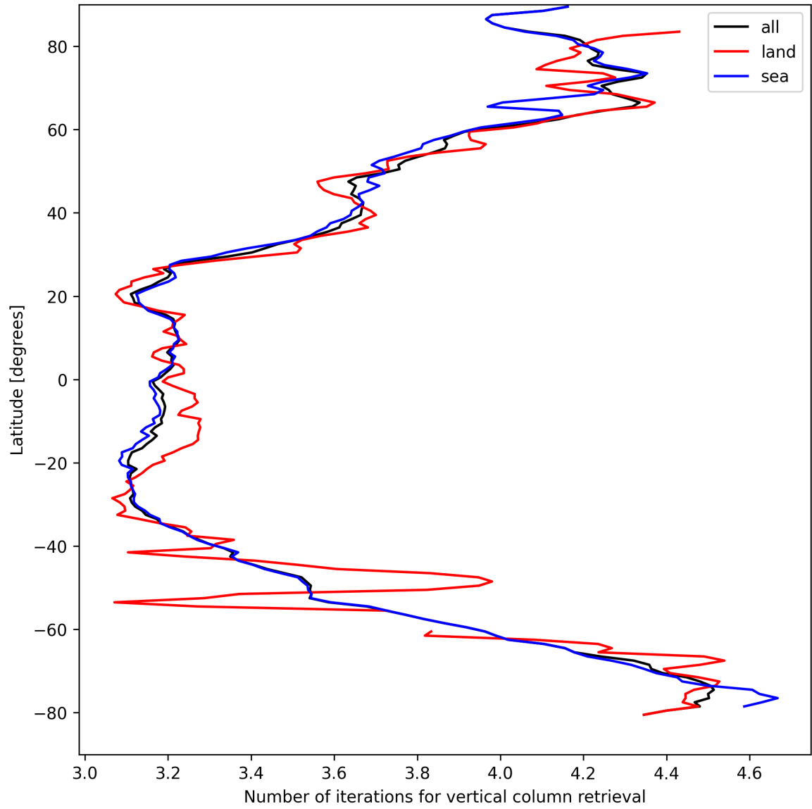
Figure 19: Zonal average of “Number of iterations for vertical column retrieval” for 2025-04-11 to 2025-04-13.
