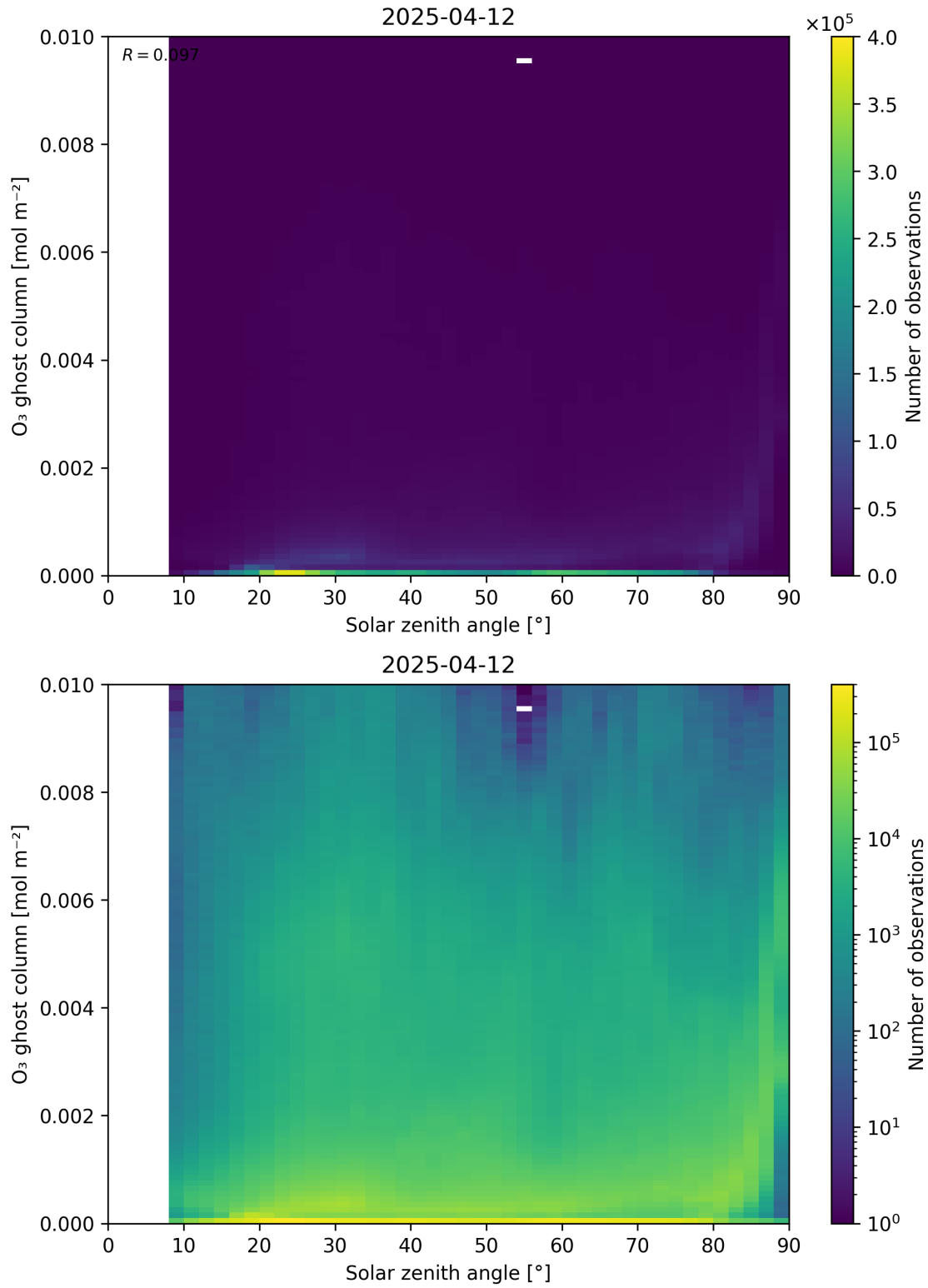
Figure 46: Scatter density plot of “Solar zenith angle” against “O 3 ghost column” for 2025-04-11 to 2025-04-13.
