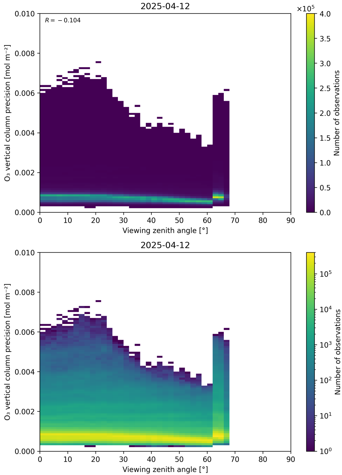
Figure 53: Scatter density plot of “Viewing zenith angle” against “O 3 vertical column precision” for 2025-04-11 to 2025-04-13.
