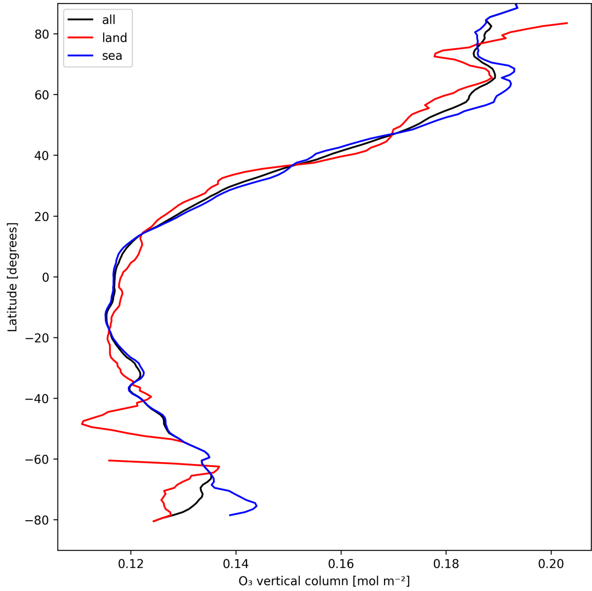
Figure 14: Zonal average of “O 3 vertical column” for 2025-04-11 to 2025-04-13.
