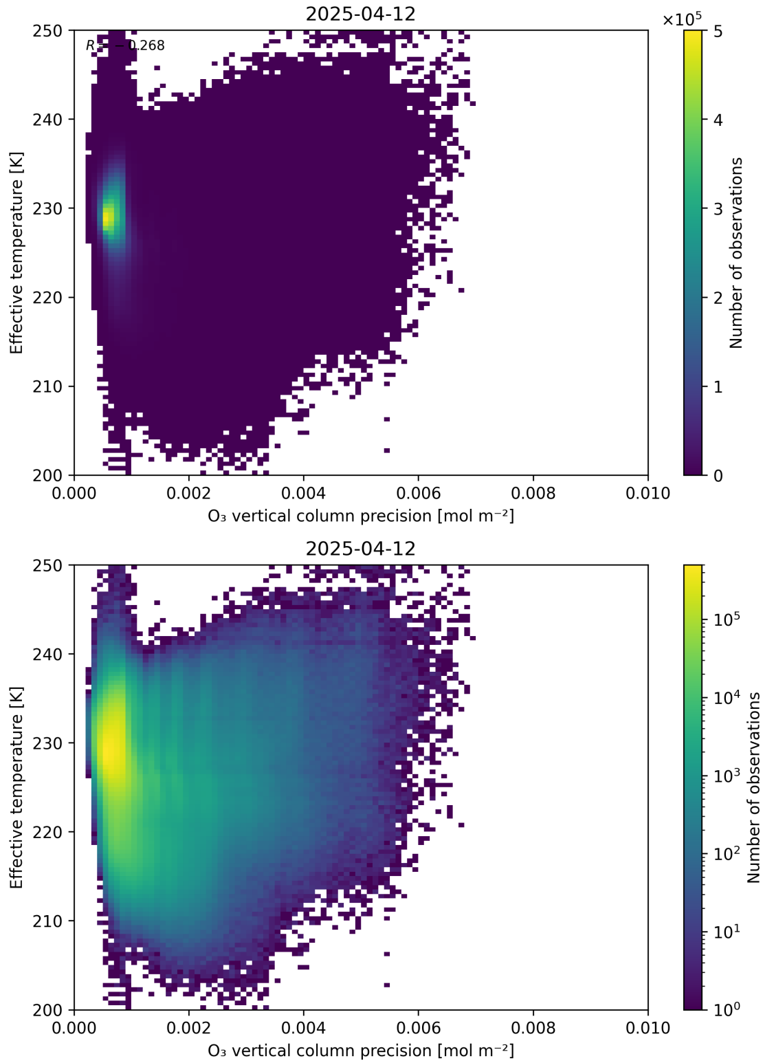
Figure 42: Scatter density plot of “O 3 vertical column precision” against “Effective temperature” for 2025-04-11 to 2025-04-13.
