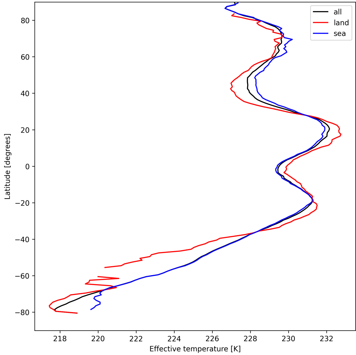
Figure 17: Zonal average of "Effective temperature" for 2025-04-11 to 2025-04-13.
