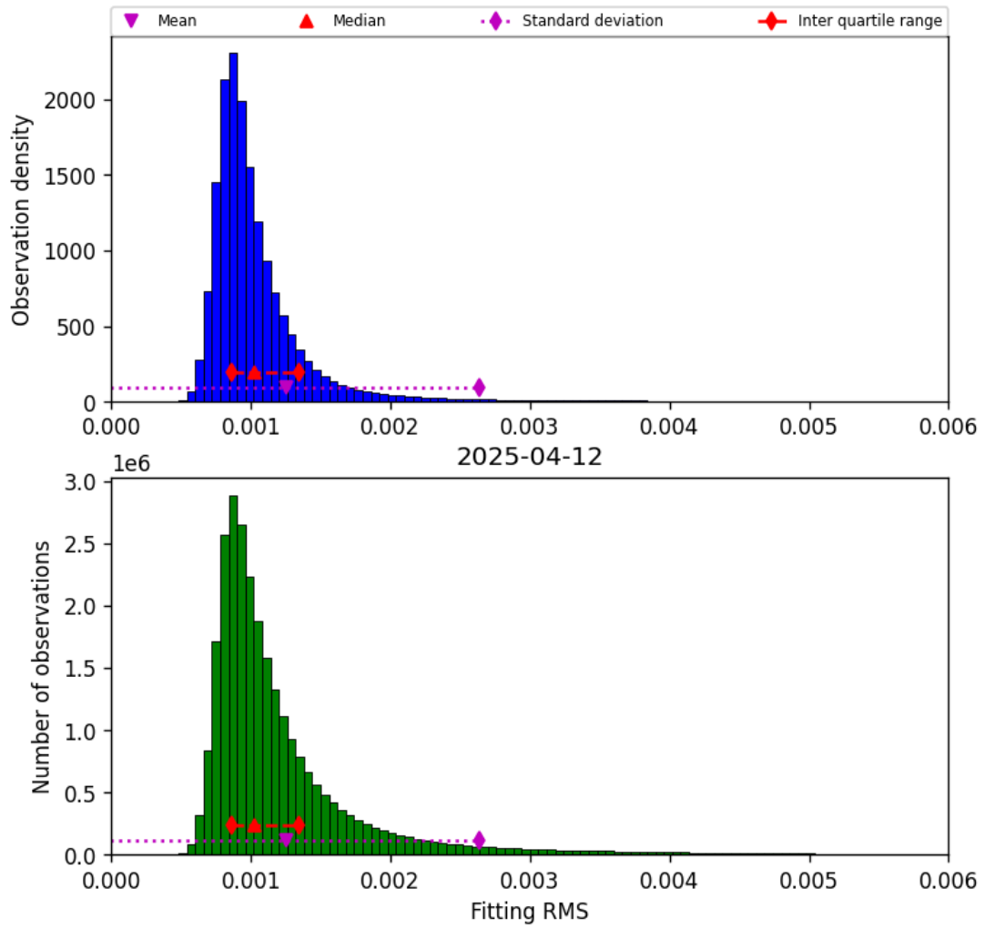
Figure 23: Histogram of “Fitting RMS” for 2025-04-11 to 2025-04-13
