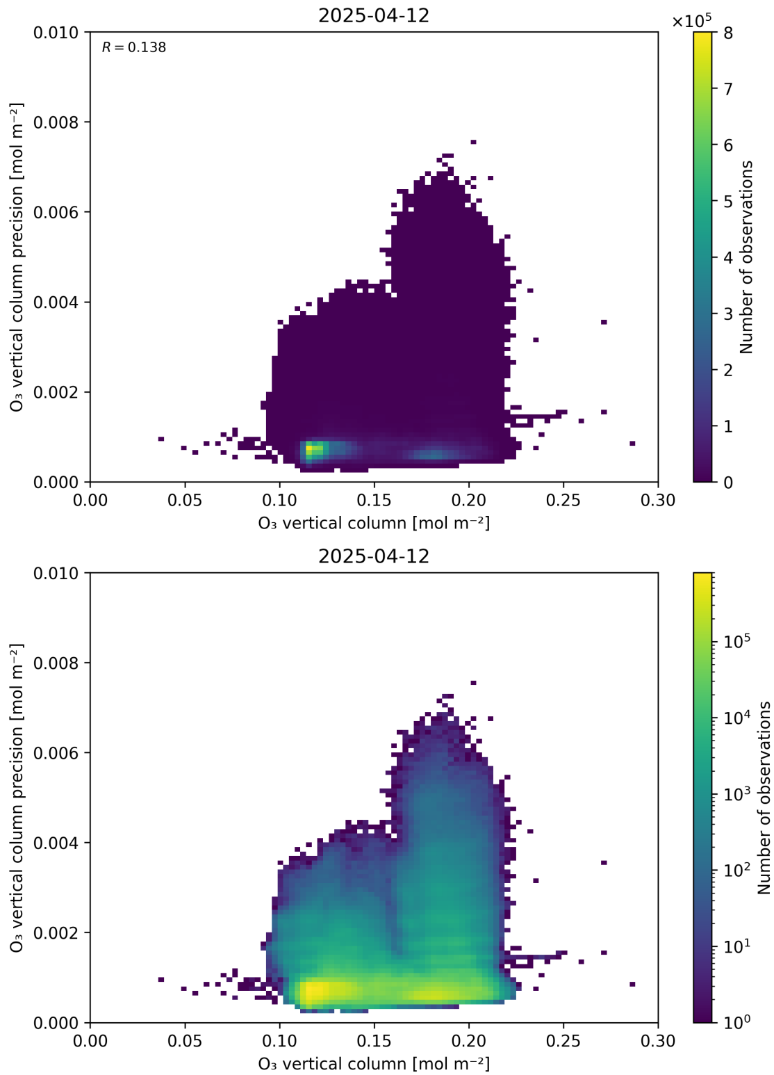
Figure 41: Scatter density plot of “O 3 vertical column” against “O 3 vertical column precision” for 2025-04-11 to 2025-04-13.
