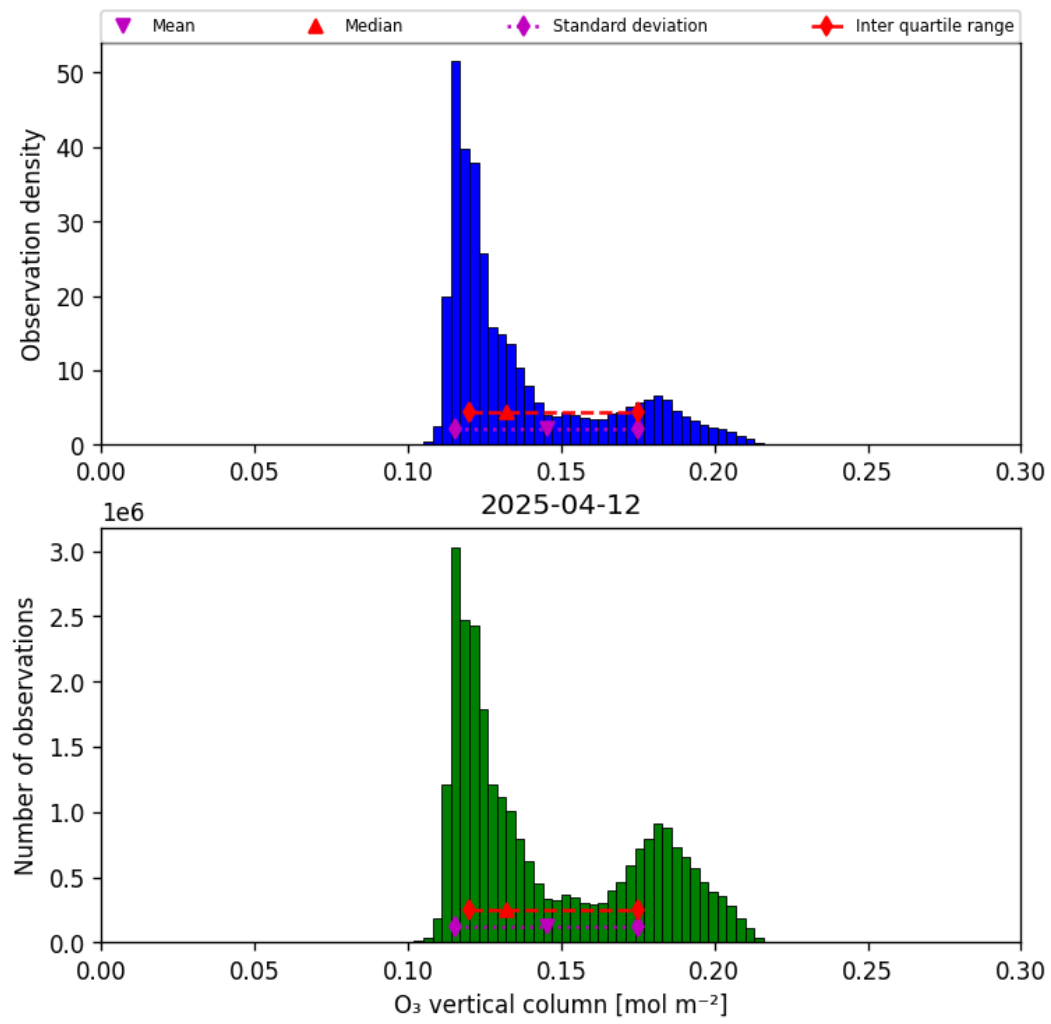
Figure 21: Histogram of “O 3 vertical column” for 2025-04-11 to 2025-04-13
