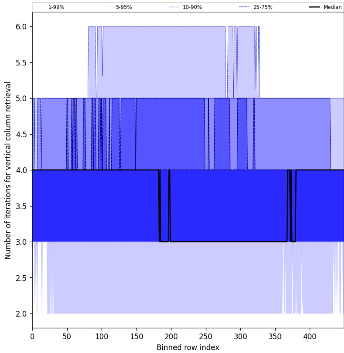
Figure 33: Along track statistics of “Number of iterations for vertical column retrieval” for 2025-04-11 to 2025-04-13
