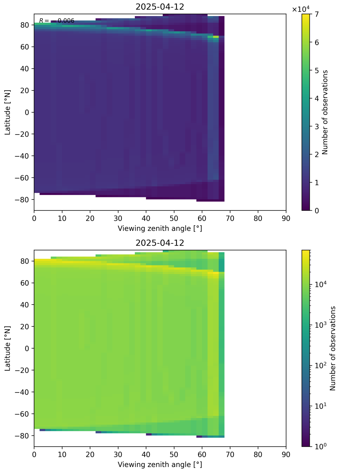
Figure 49: Scatter density plot of “Viewing zenith angle” against “Latitude” for 2025-04-11 to 2025-04-13.
