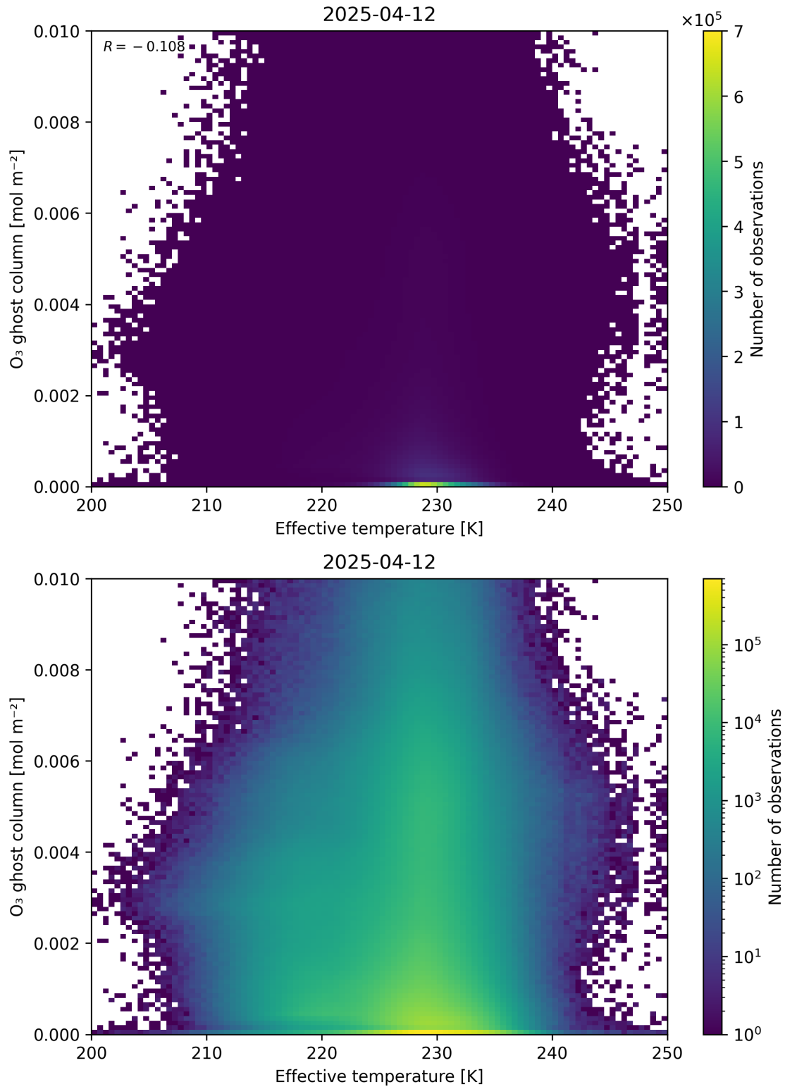
Figure 38: Scatter density plot of “Effective temperature” against “O 3 ghost column” for 2025-04-11 to 2025-04-13.
