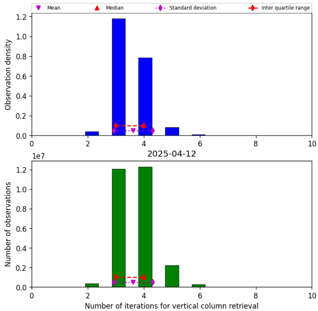
Figure 26: Histogram of “Number of iterations for vertical column retrieval” for 2025-04-11 to 2025-04-13
