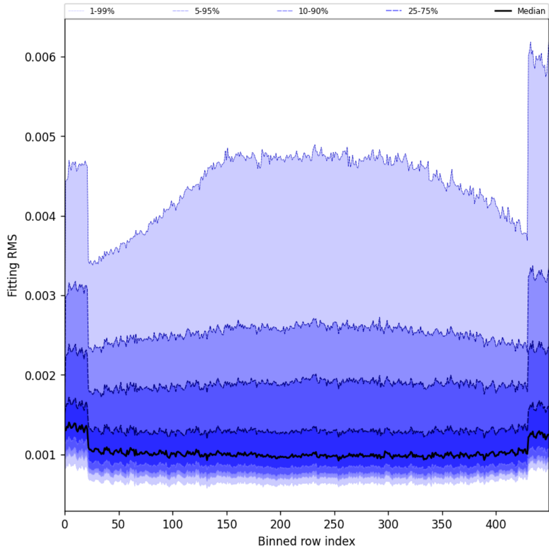
Figure 30: Along track statistics of “Fitting RMS” for 2025-04-11 to 2025-04-13
