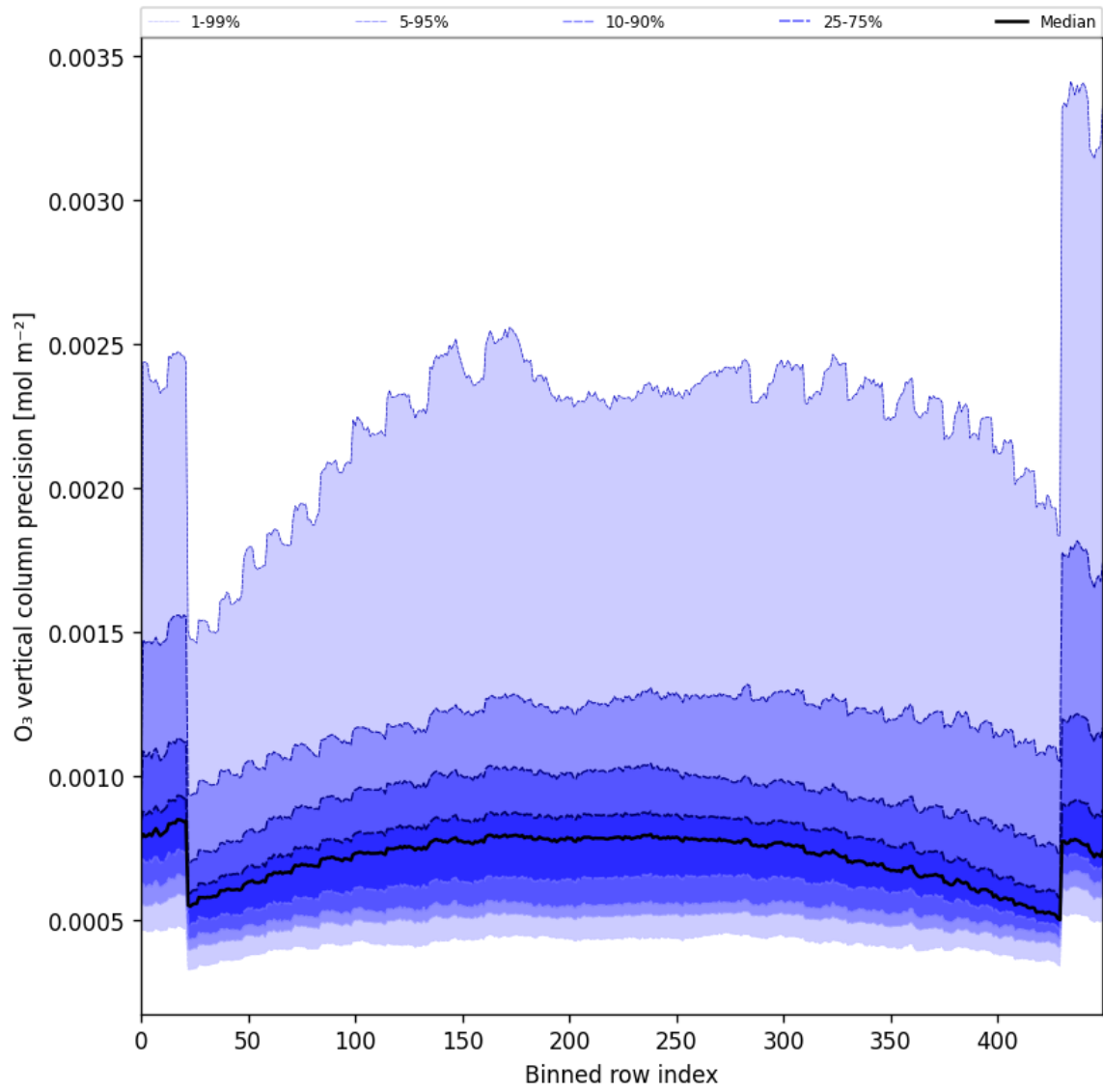
Figure 29: Along track statistics of “O 3 vertical column precision” for 2025-04-11 to 2025-04-13
