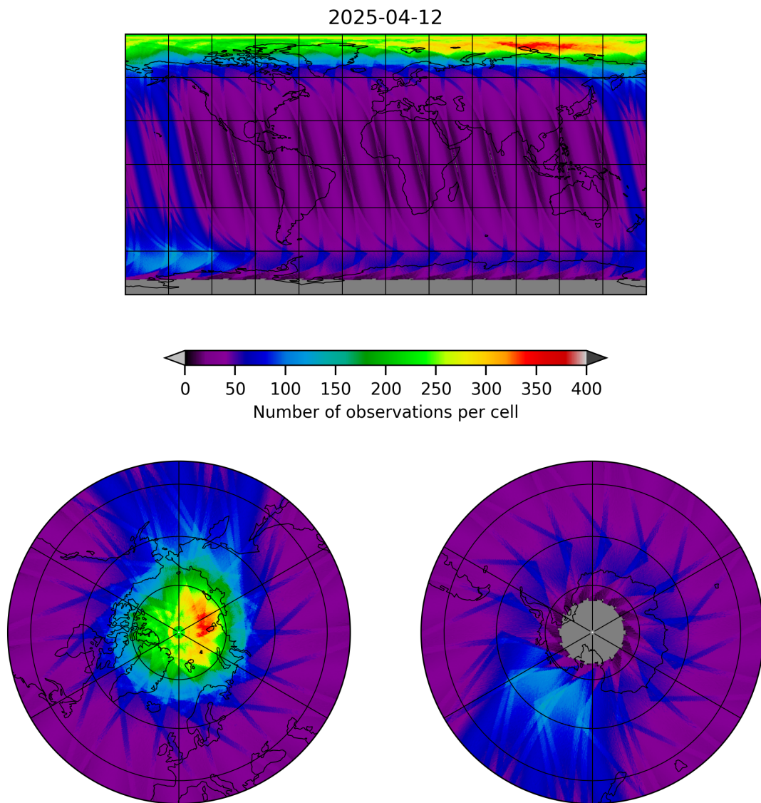
Figure 12: Map of the number of observations for 2025-04-11 to 2025-04-13
