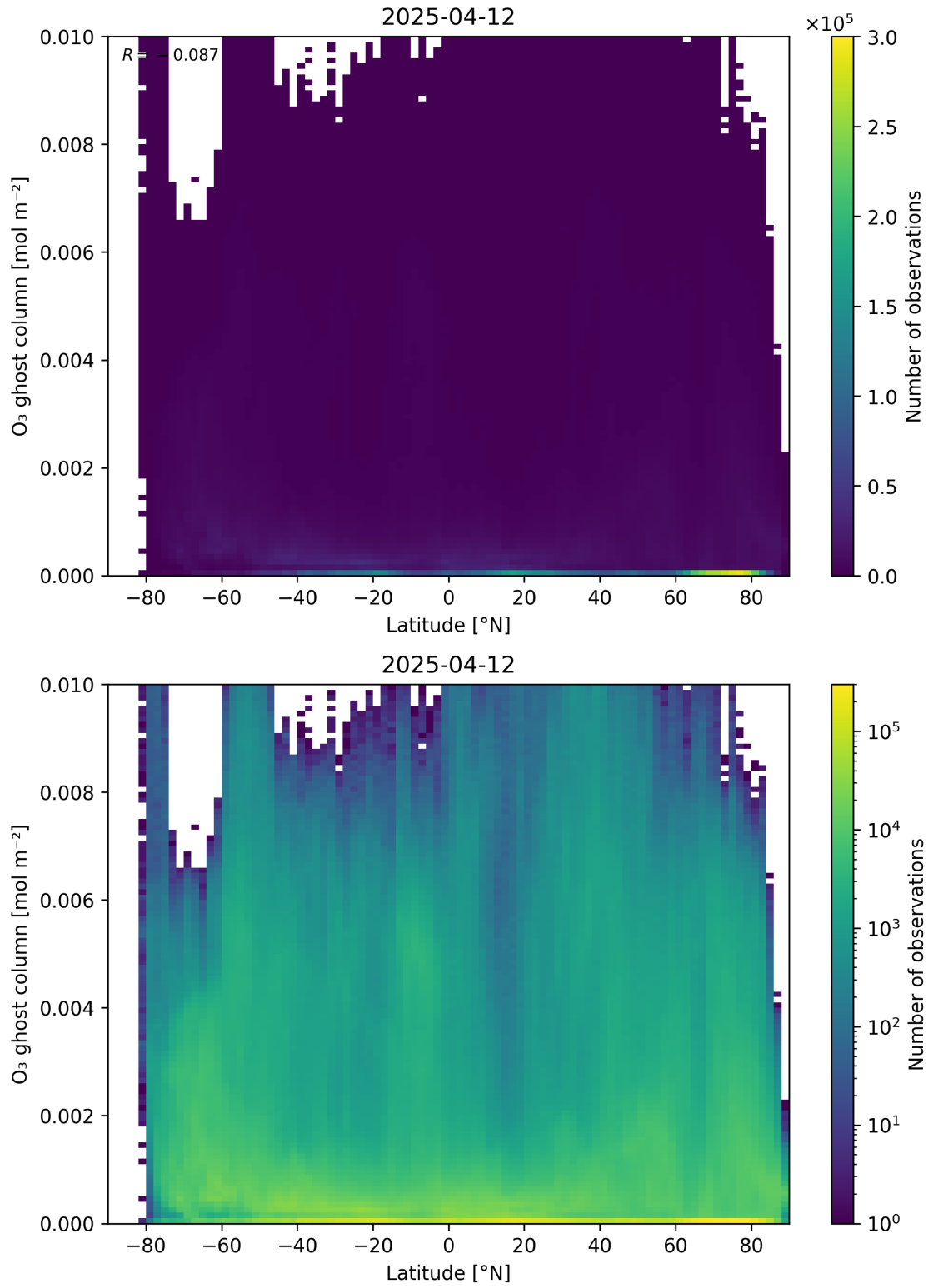
Figure 35: Scatter density plot of “Latitude” against “O 3 ghost column” for 2025-04-11 to 2025-04-13.
