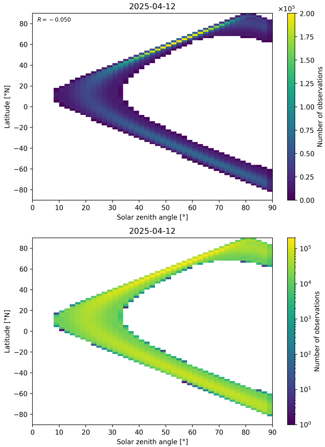
Figure 44: Scatter density plot of “Solar zenith angle” against “Latitude” for 2025-04-11 to 2025-04-13.
