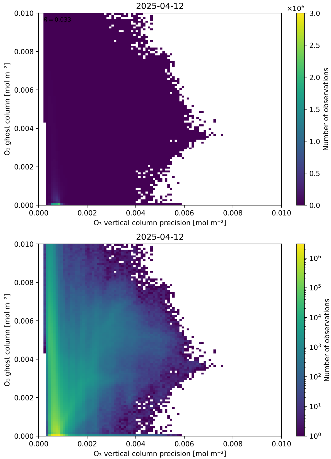
Figure 43: Scatter density plot of “O 3 vertical column precision” against “O 3 ghost column” for 2025-04-11 to 2025-04-13.
