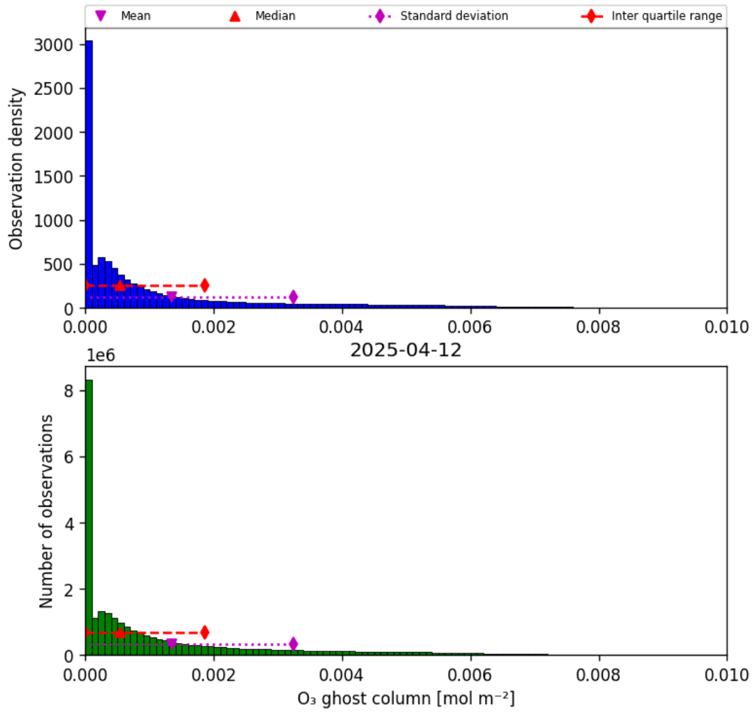
Figure 25: Histogram of “O 3 ghost column” for 2025-04-11 to 2025-04-13
