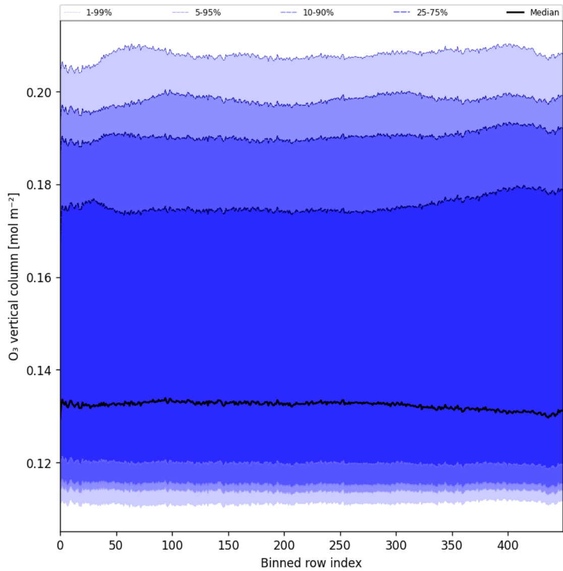
Figure 28: Along track statistics of “O 3 vertical column” for 2025-04-11 to 2025-04-13
