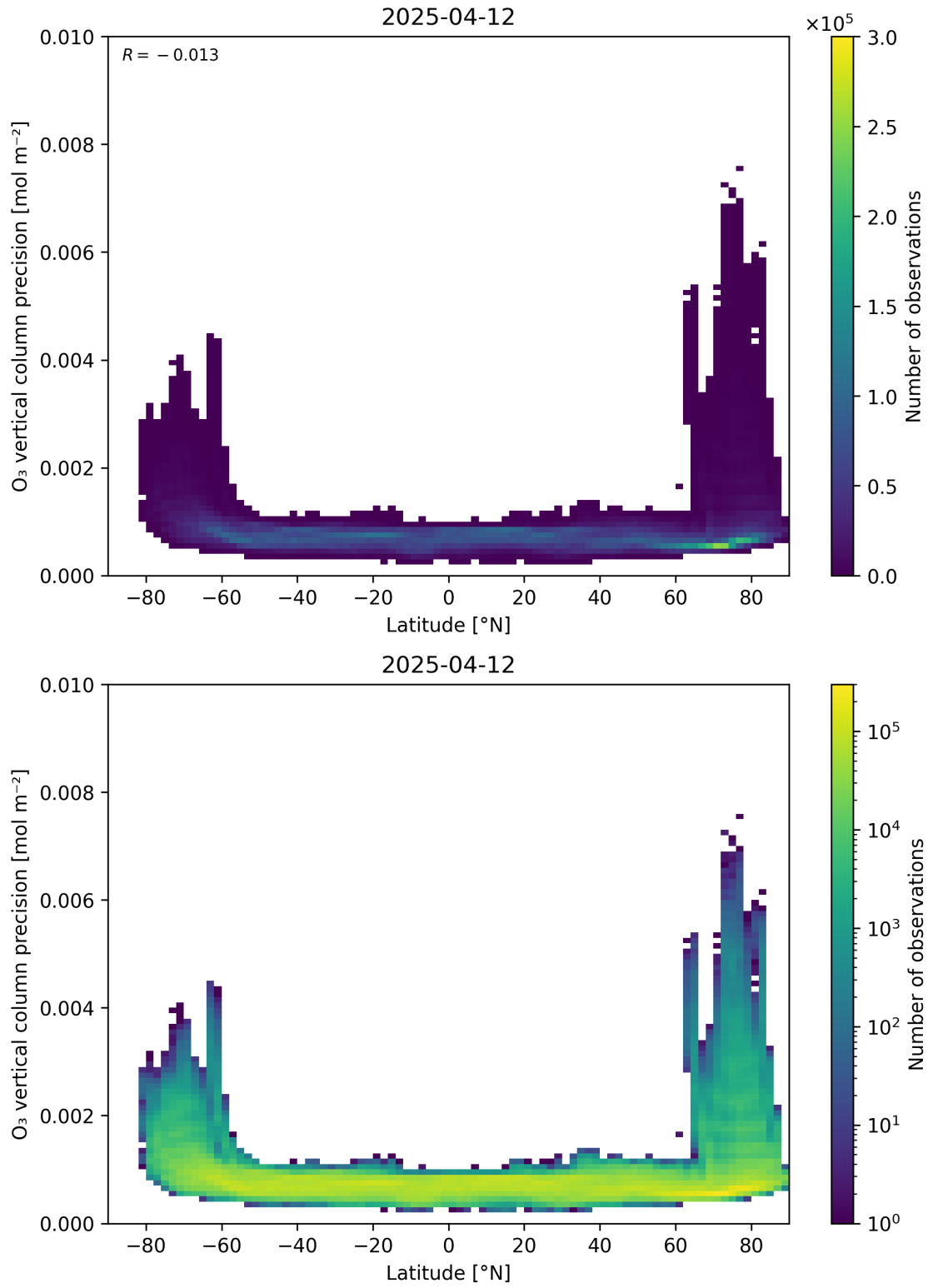
Figure 37: Scatter density plot of “Latitude” against “O 3 vertical column precision” for 2025-04-11 to 2025-04-13.
