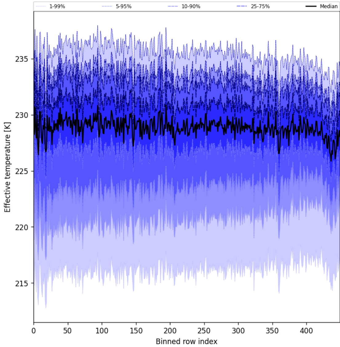
Figure 31: Along track statistics of “Effective temperature” for 2025-04-11 to 2025-04-13
