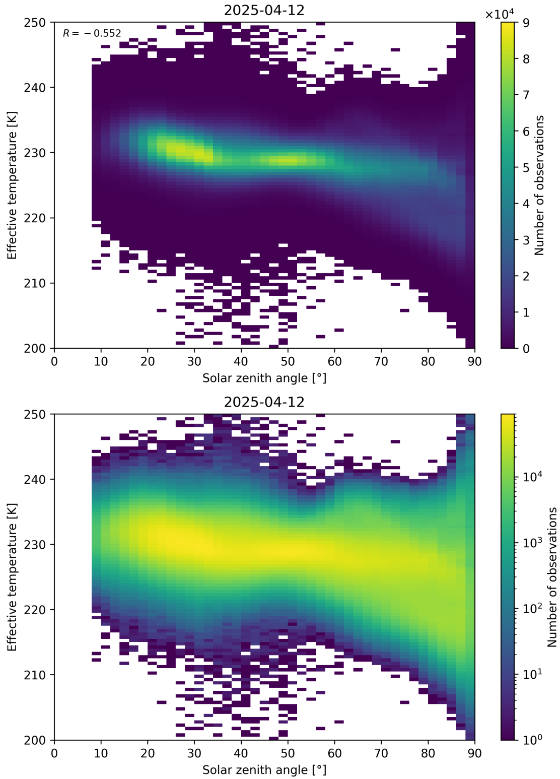
Figure 45: Scatter density plot of “Solar zenith angle” against “Effective temperature” for 2025-04-11 to 2025-04-13.
