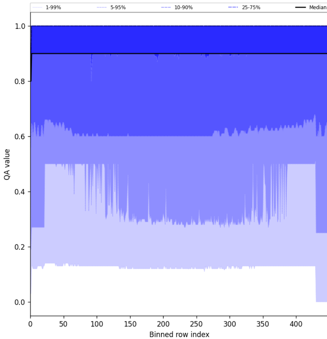
Figure 27: Along track statistics of “QA value” for 2025-04-11 to 2025-04-13
