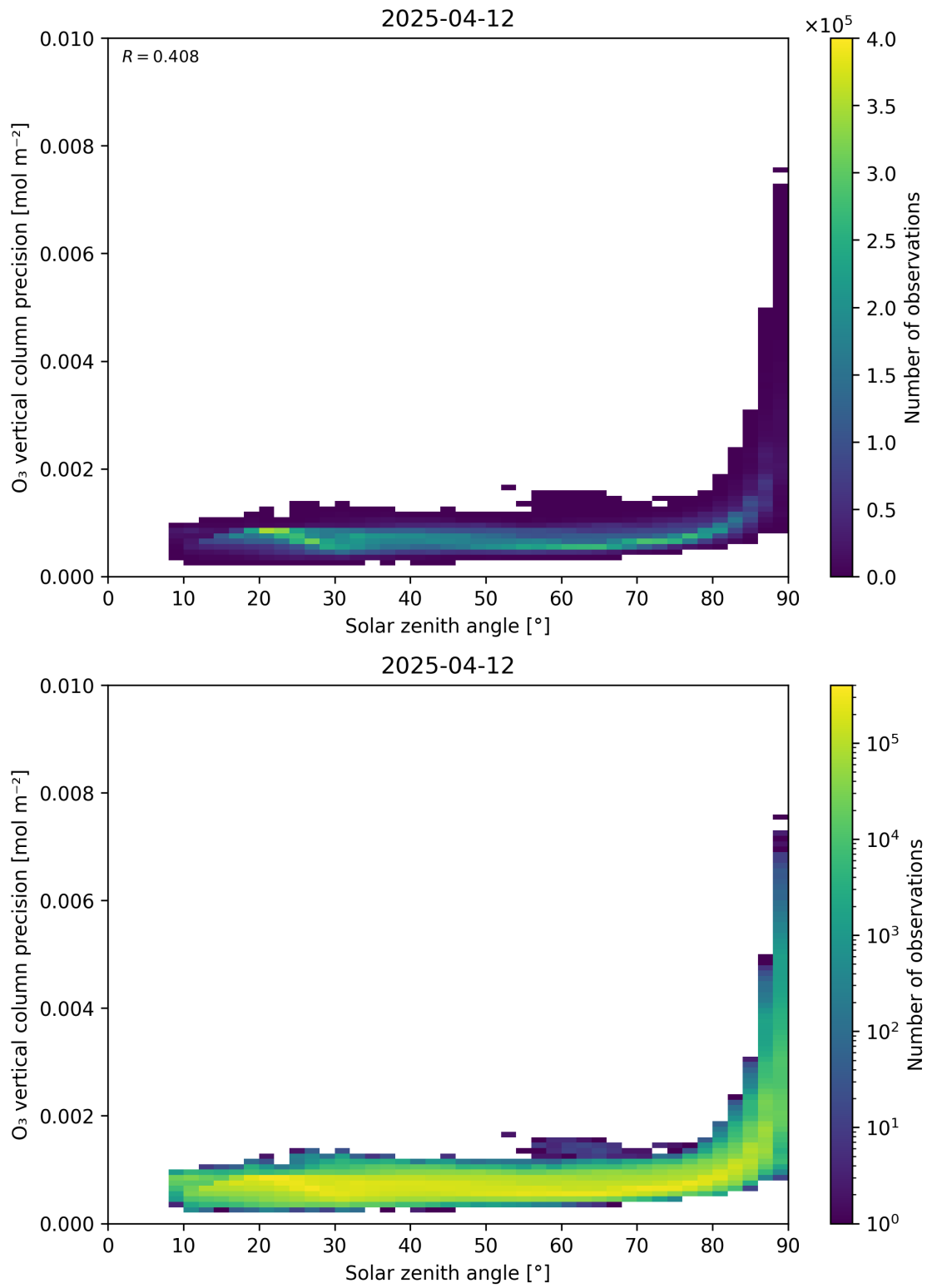
Figure 48: Scatter density plot of “Solar zenith angle” against “O 3 vertical column precision” for 2025-04-11 to 2025-04-13.
