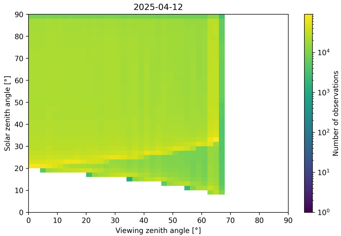
Figure 54: Scatter density plot of “Viewing zenith angle” against “Solar zenith angle” for 2025-04-11 to 2025-04-13.
