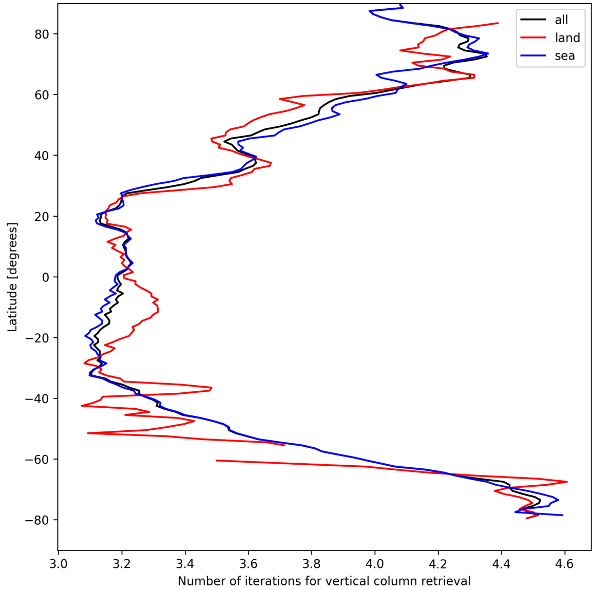
Figure 19: Zonal average of “Number of iterations for vertical column retrieval” for 2025-04-13 to 2025-04-14.
