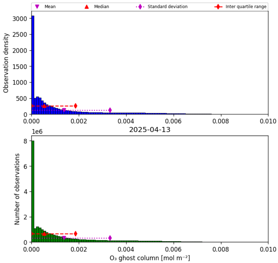
Figure 25: Histogram of “O 3 ghost column” for 2025-04-13 to 2025-04-14
