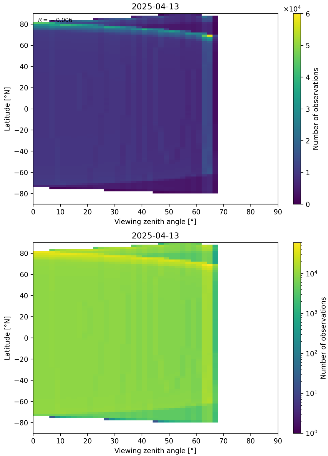
Figure 49: Scatter density plot of “Viewing zenith angle” against “Latitude” for 2025-04-13 to 2025-04-14.
