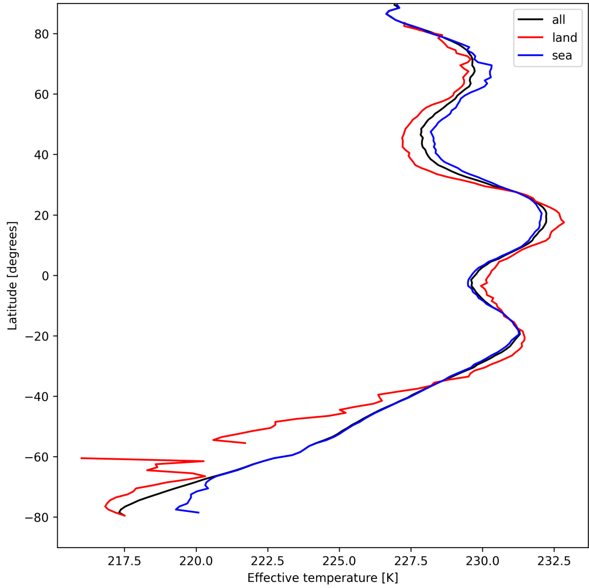
Figure 17: Zonal average of “Effective temperature” for 2025-04-13 to 2025-04-14.
