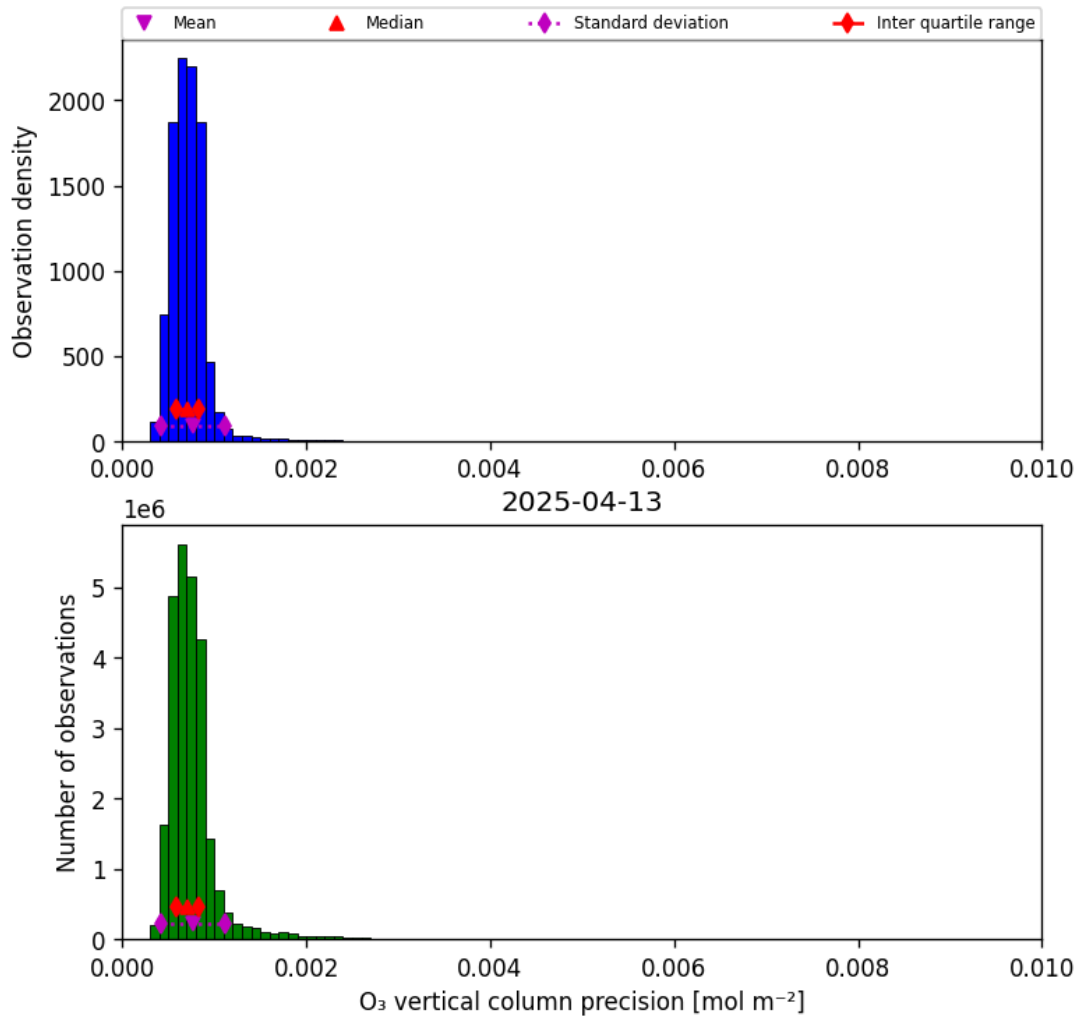
Figure 22: Histogram of “O 3 vertical column precision” for 2025-04-13 to 2025-04-14
