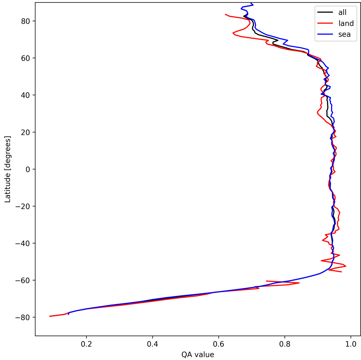
Figure 13: Zonal average of “QA value” for 2025-04-13 to 2025-04-14.
