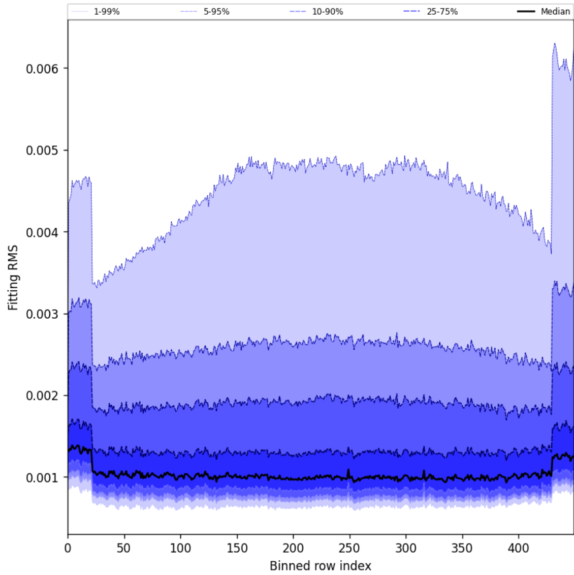
Figure 30: Along track statistics of “Fitting RMS” for 2025-04-13 to 2025-04-14
