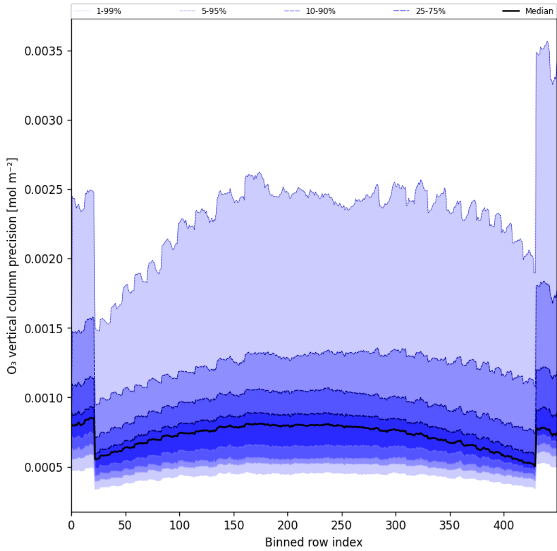
Figure 29: Along track statistics of “O 3 vertical column precision” for 2025-04-13 to 2025-04-14
