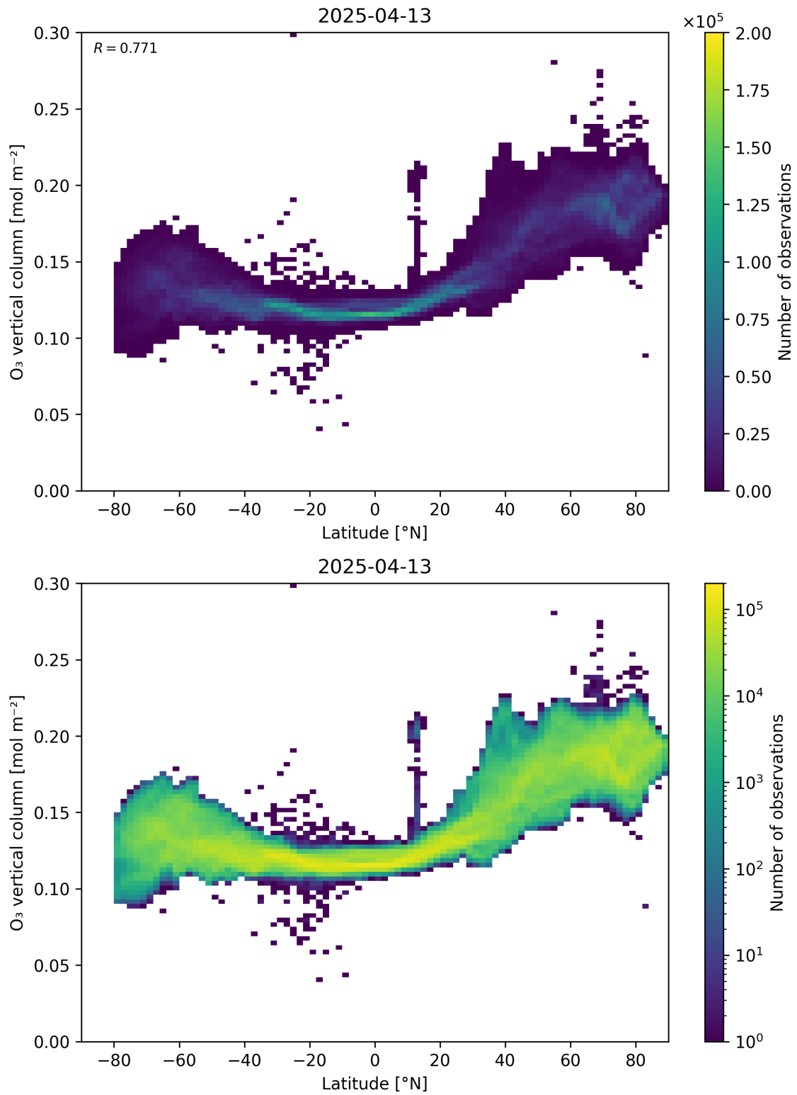
Figure 36: Scatter density plot of “Latitude” against “O 3 vertical column” for 2025-04-13 to 2025-04-14.
