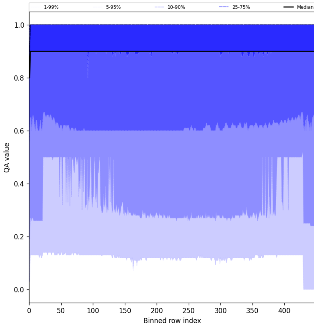
Figure 27: Along track statistics of “QA value” for 2025-04-13 to 2025-04-14
