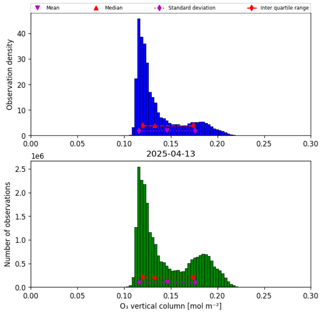
Figure 21: Histogram of “O 3 vertical column” for 2025-04-13 to 2025-04-14
