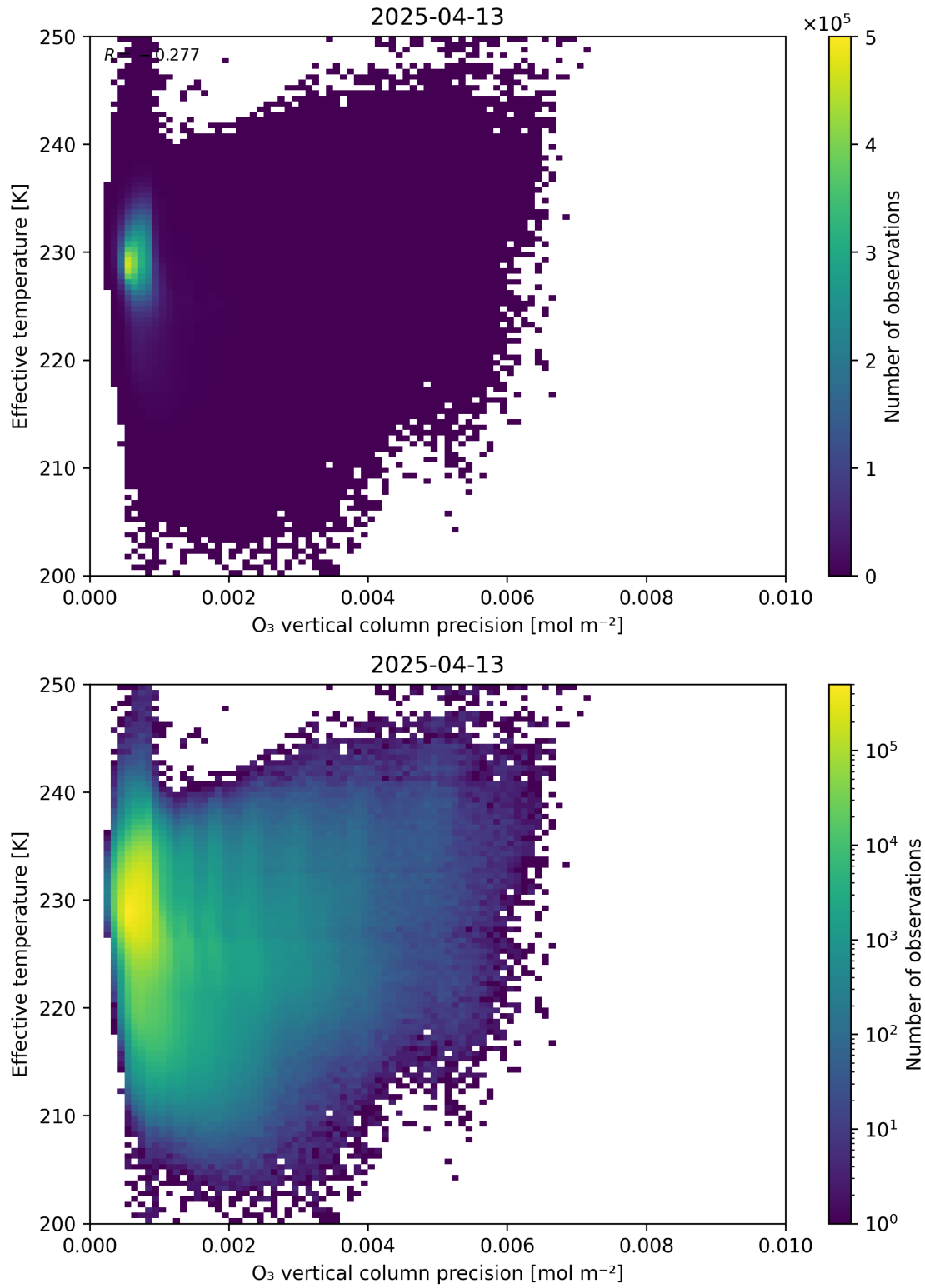
Figure 42: Scatter density plot of “ O_3 vertical column precision” against “Effective temperature” for 2025-04-13 to 2025-04-14.
