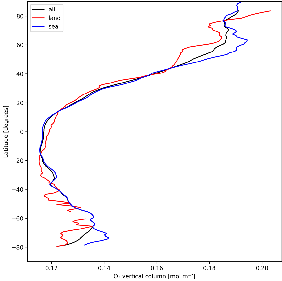
Figure 14: Zonal average of “O 3 vertical column” for 2025-04-13 to 2025-04-14.
