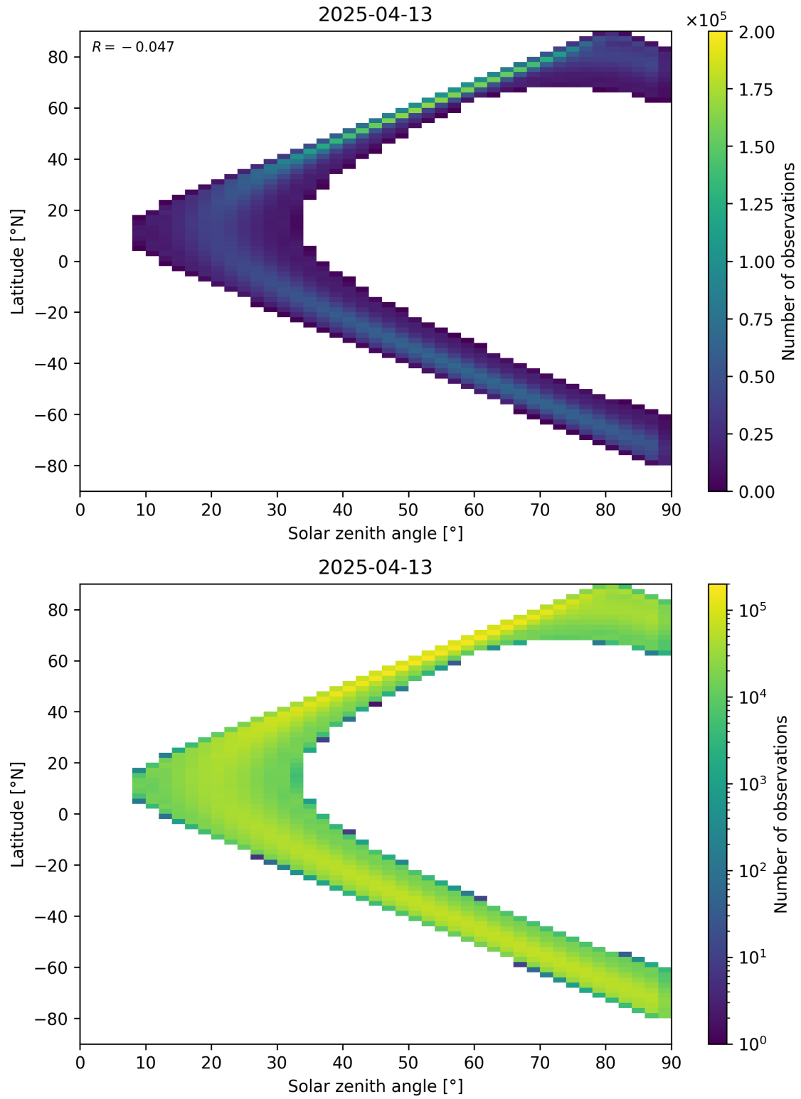
Figure 44: Scatter density plot of “Solar zenith angle” against “Latitude” for 2025-04-13 to 2025-04-14.
