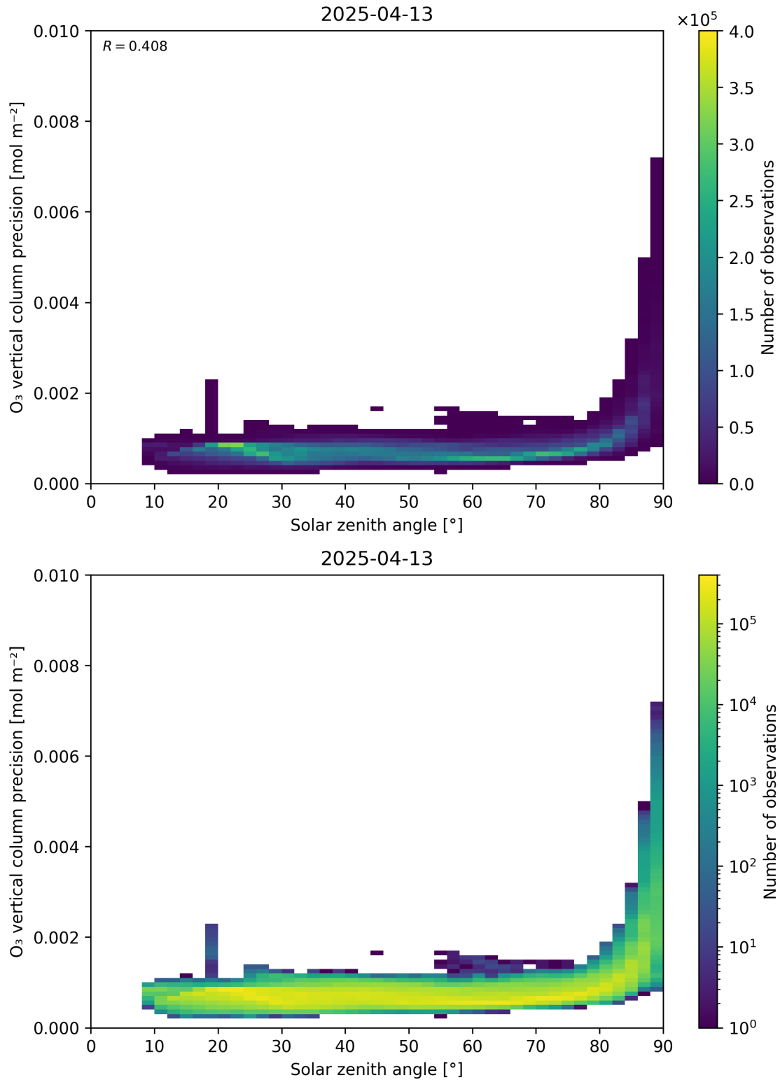
Figure 48: Scatter density plot of “Solar zenith angle” against “O 3 vertical column precision” for 2025-04-13 to 2025-04-14.
