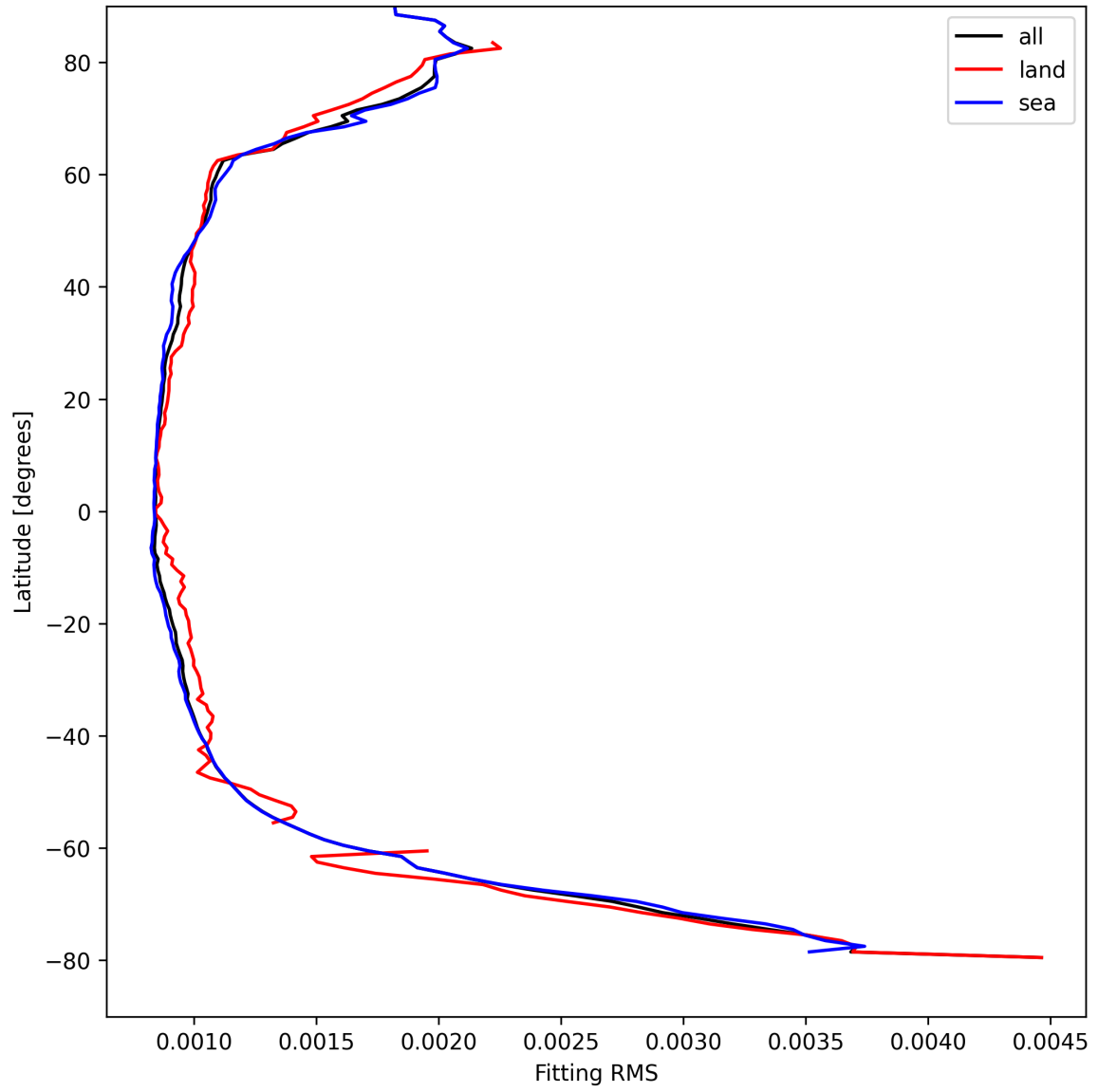
Figure 16: Zonal average of “Fitting RMS” for 2025-04-13 to 2025-04-14.
