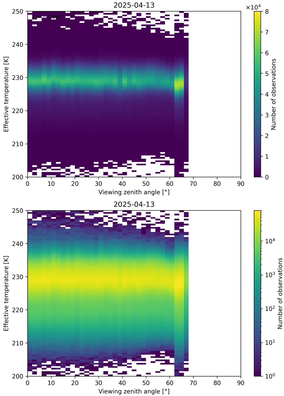
Figure 50: Scatter density plot of “Viewing zenith angle” against “Effective temperature” for 2025-04-13 to 2025-04-14.
