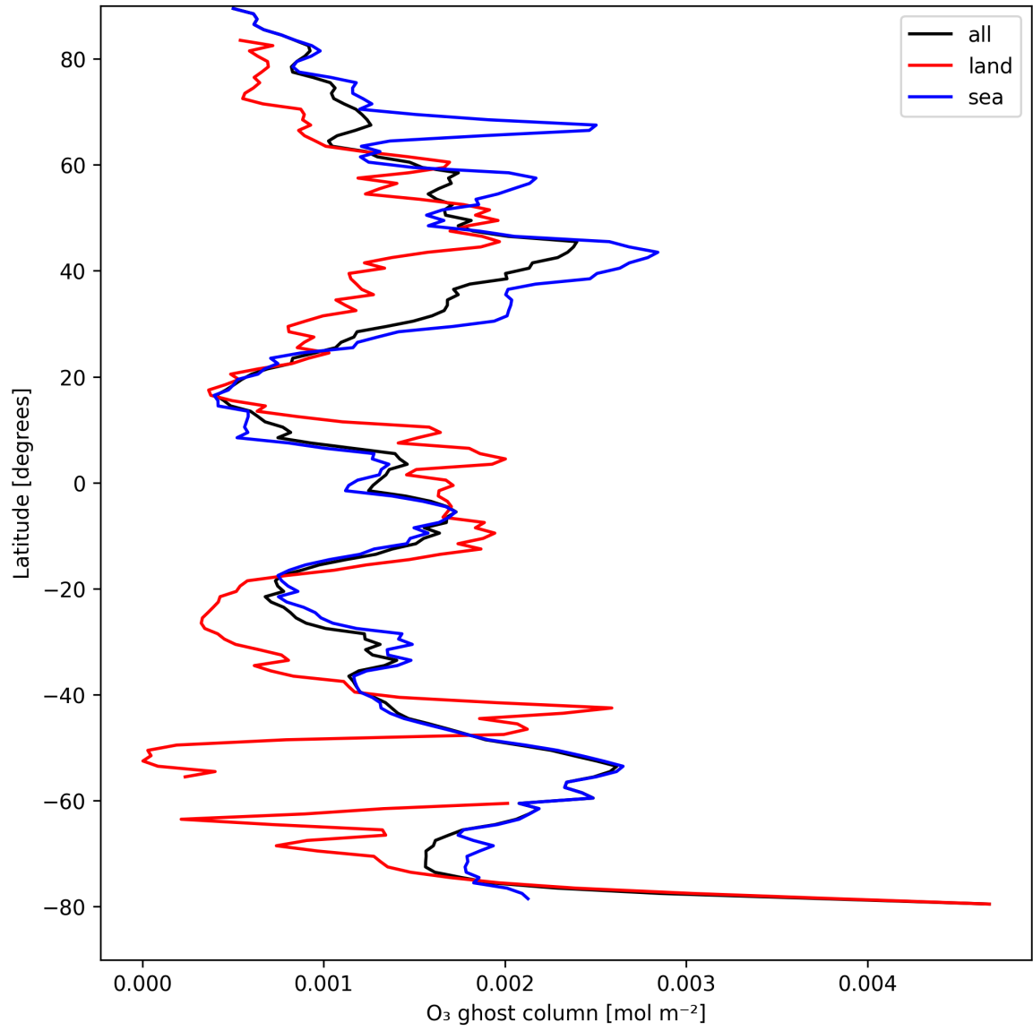
Figure 18: Zonal average of “O 3 ghost column” for 2025-04-13 to 2025-04-14.
