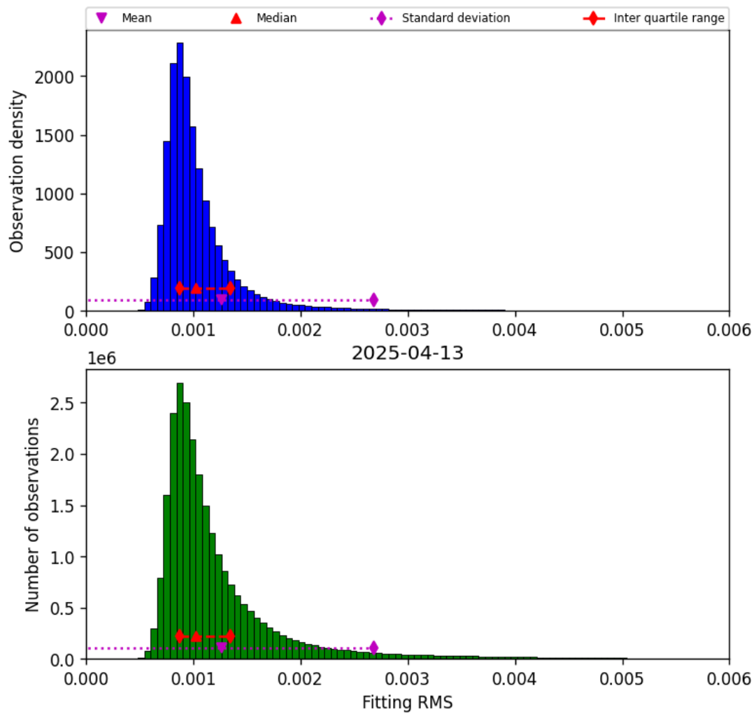
Figure 23: Histogram of “Fitting RMS” for 2025-04-13 to 2025-04-14
