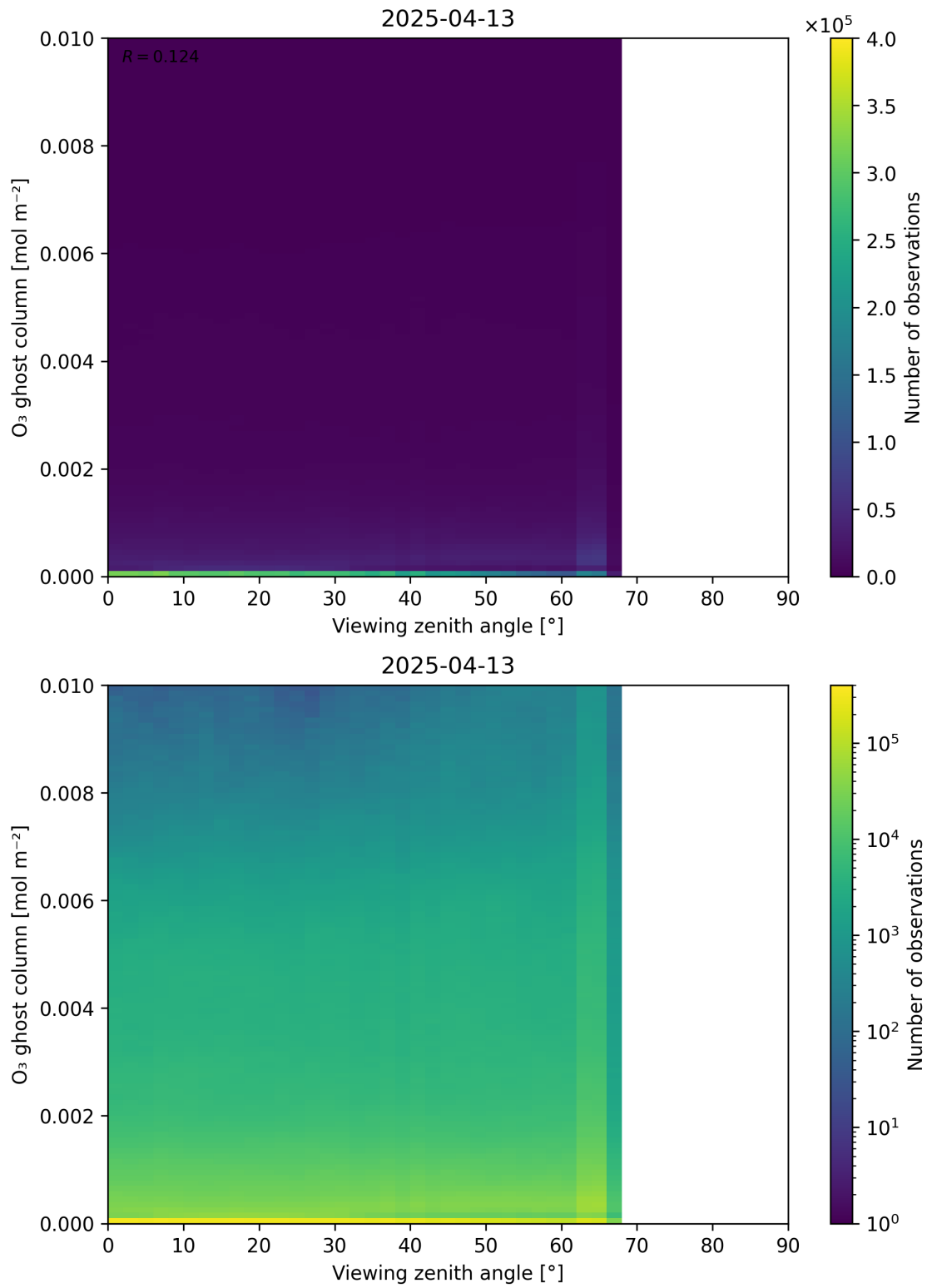
Figure 51: Scatter density plot of “Viewing zenith angle” against “O 3 ghost column” for 2025-04-13 to 2025-04-14.
