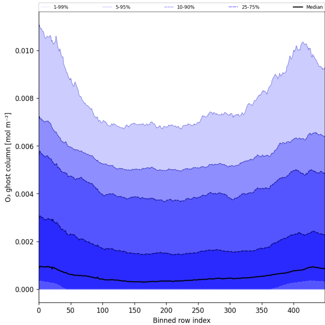
Figure 32: Along track statistics of “O 3 ghost column” for 2025-04-13 to 2025-04-14
