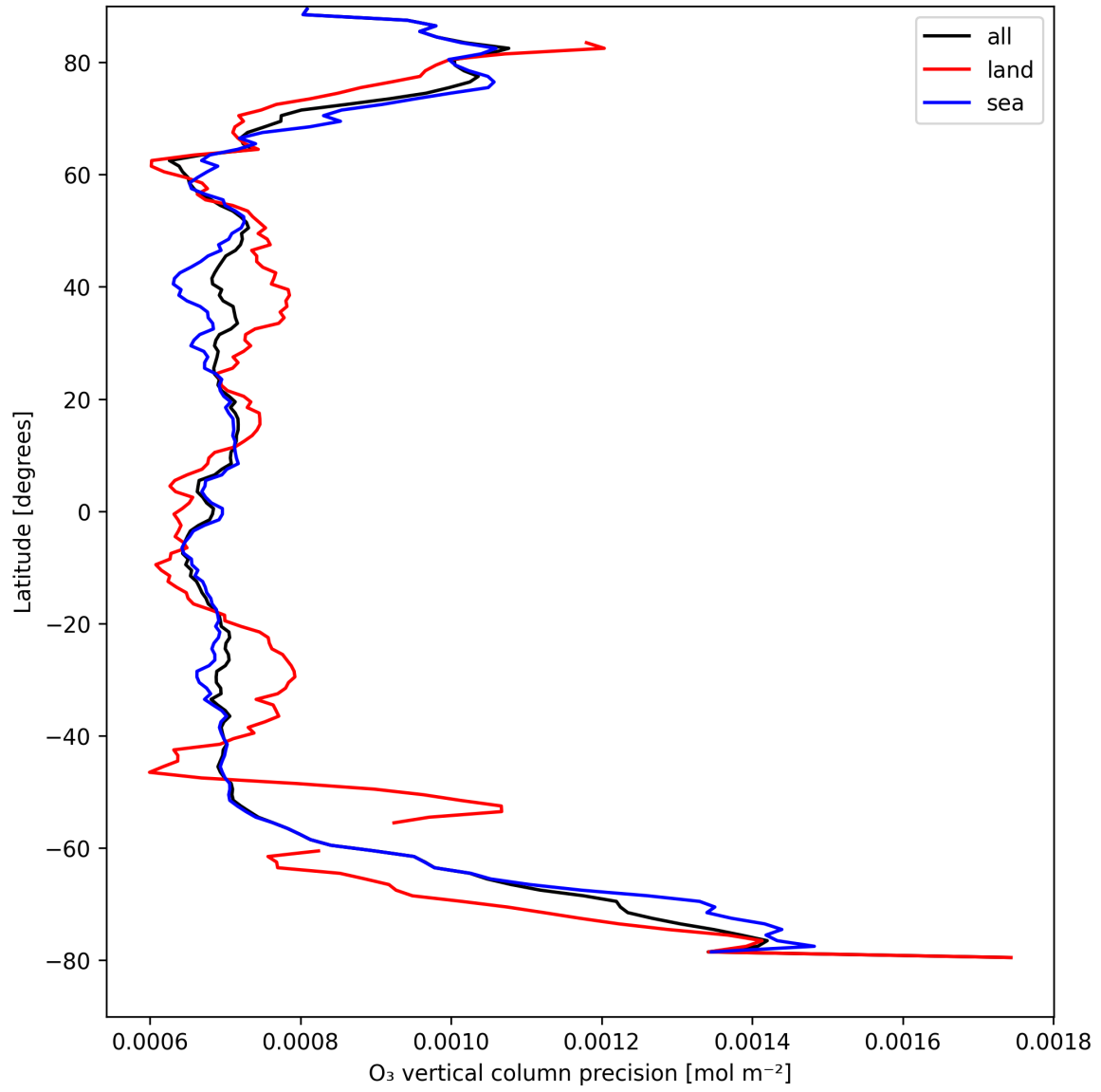
Figure 15: Zonal average of “O 3 vertical column precision” for 2025-04-13 to 2025-04-14.
