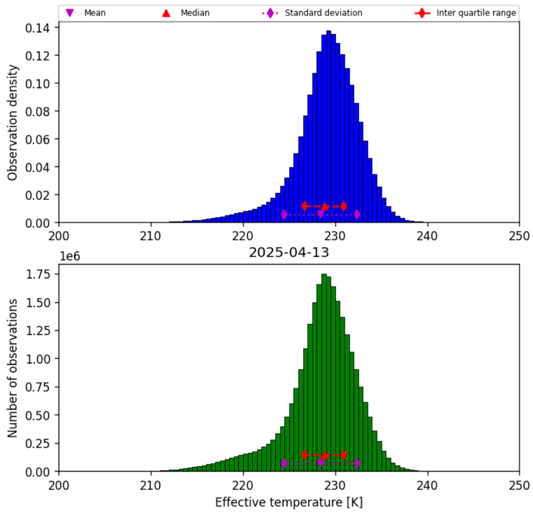
Figure 24: Histogram of “Effective temperature” for 2025-04-13 to 2025-04-14
