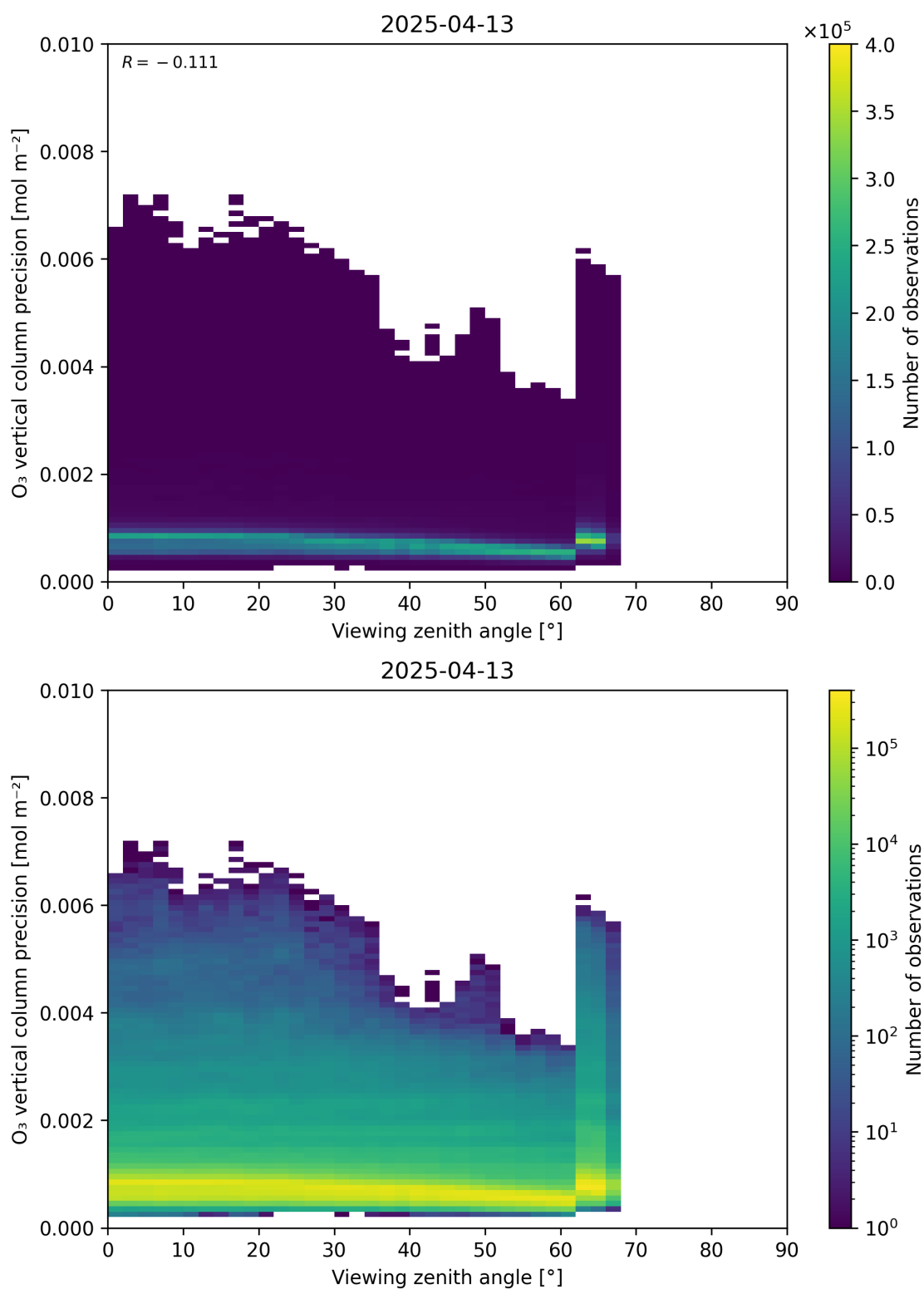
Figure 53: Scatter density plot of “Viewing zenith angle” against “O 3 vertical column precision” for 2025-04-13 to 2025-04-14.
