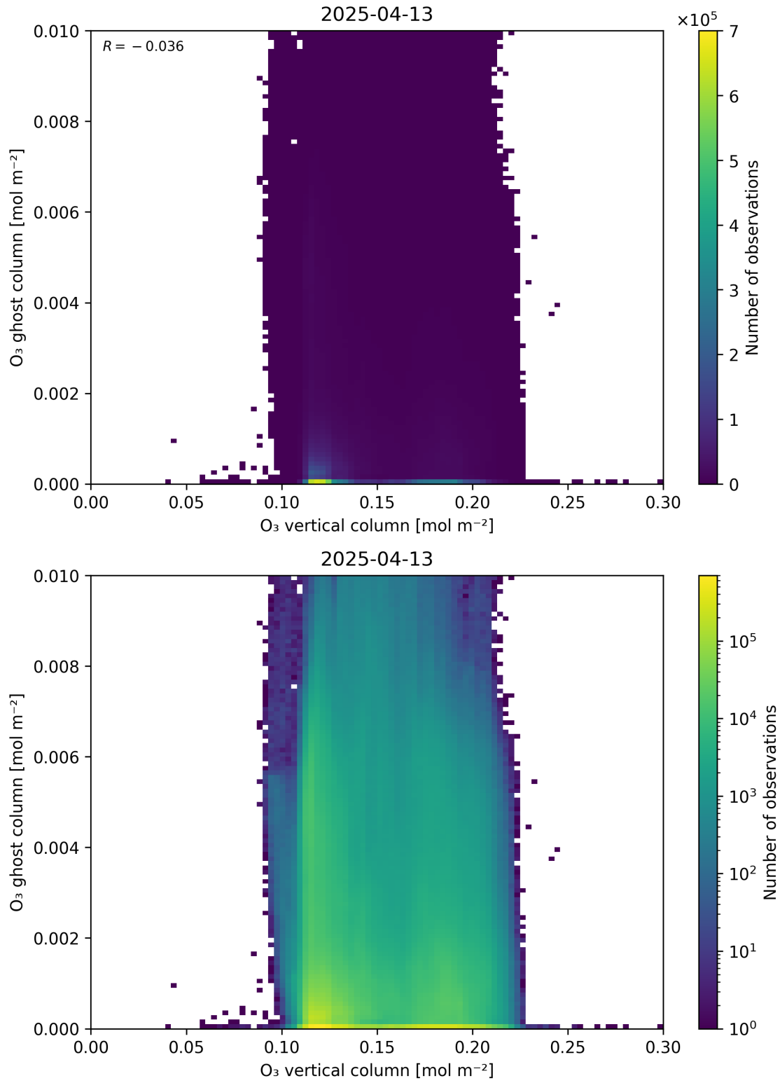
Figure 40: Scatter density plot of “O 3 vertical column” against “O 3 ghost column” for 2025-04-13 to 2025-04-14.
