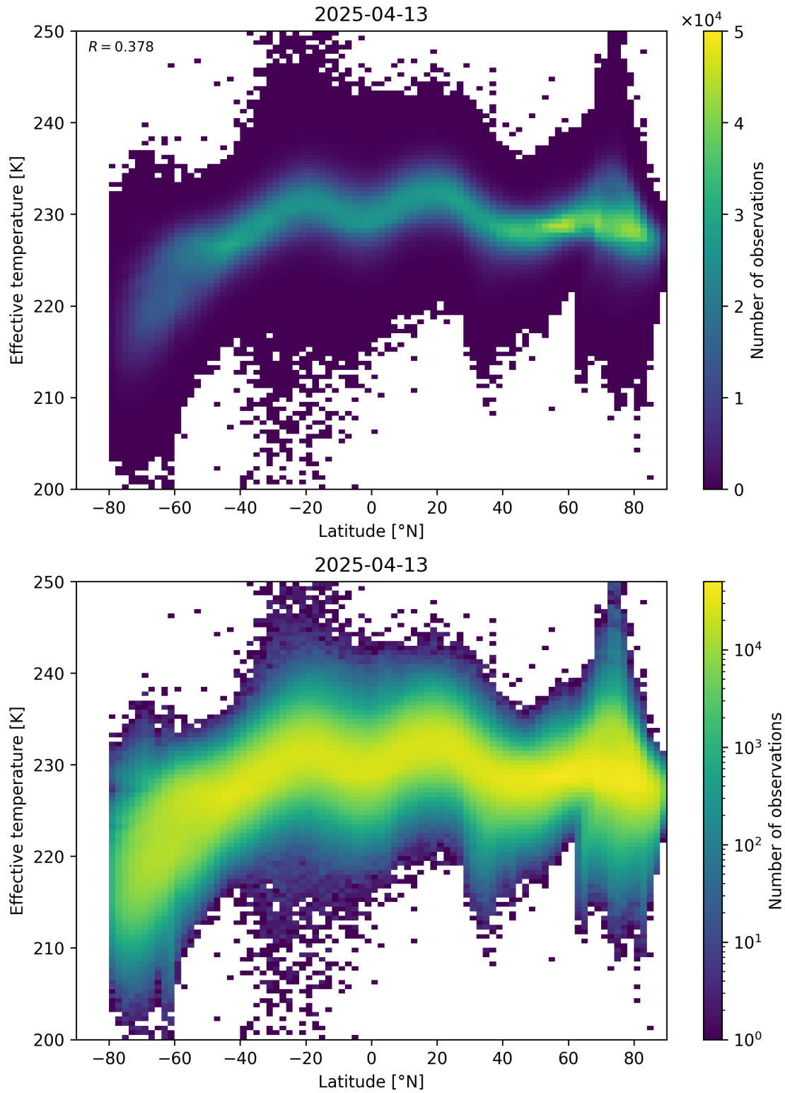
Figure 34: Scatter density plot of “Latitude” against “Effective temperature” for 2025-04-13 to 2025-04-14.
