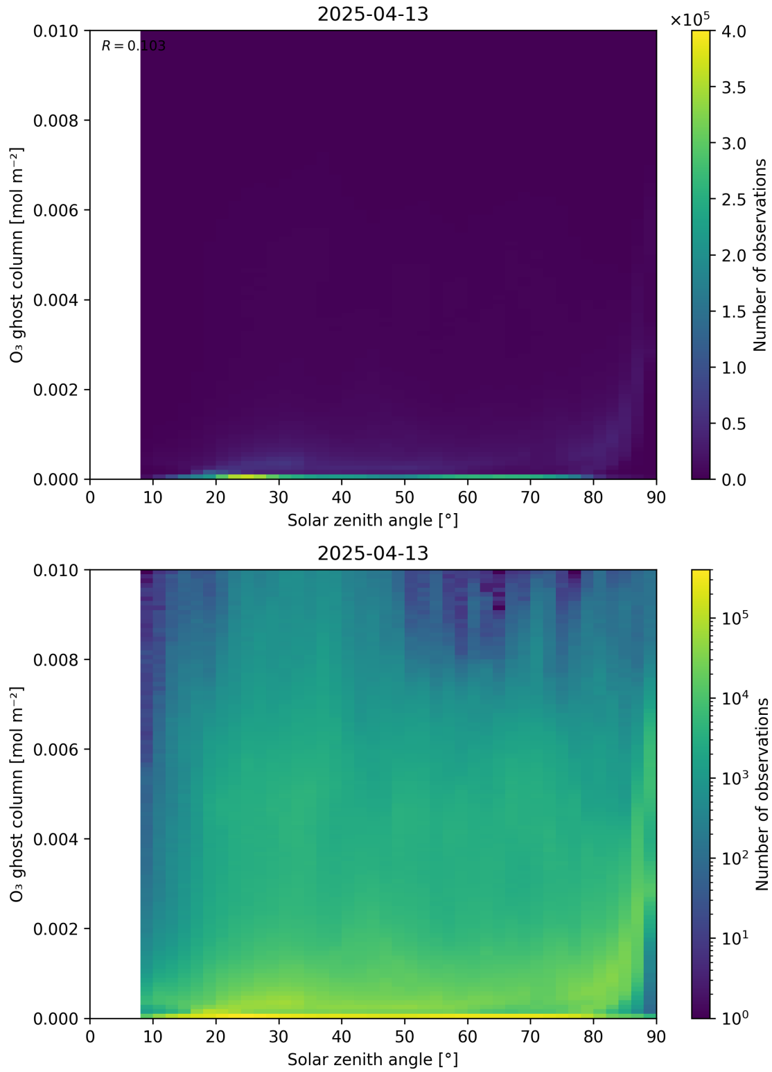
Figure 46: Scatter density plot of “Solar zenith angle” against “O 3 ghost column” for 2025-04-13 to 2025-04-14.
