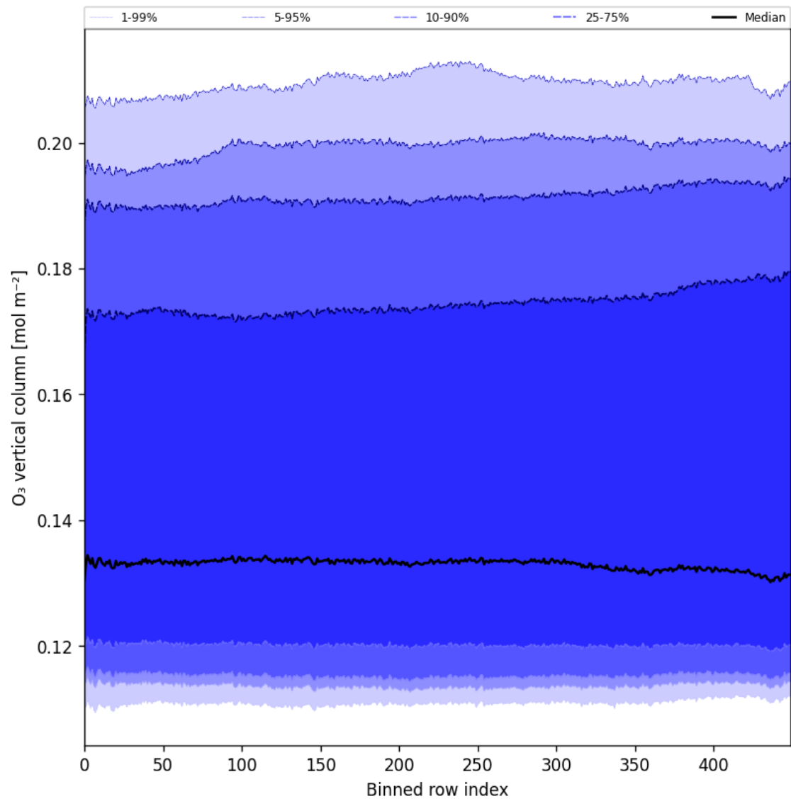
Figure 28: Along track statistics of “O 3 vertical column” for 2025-04-13 to 2025-04-14
