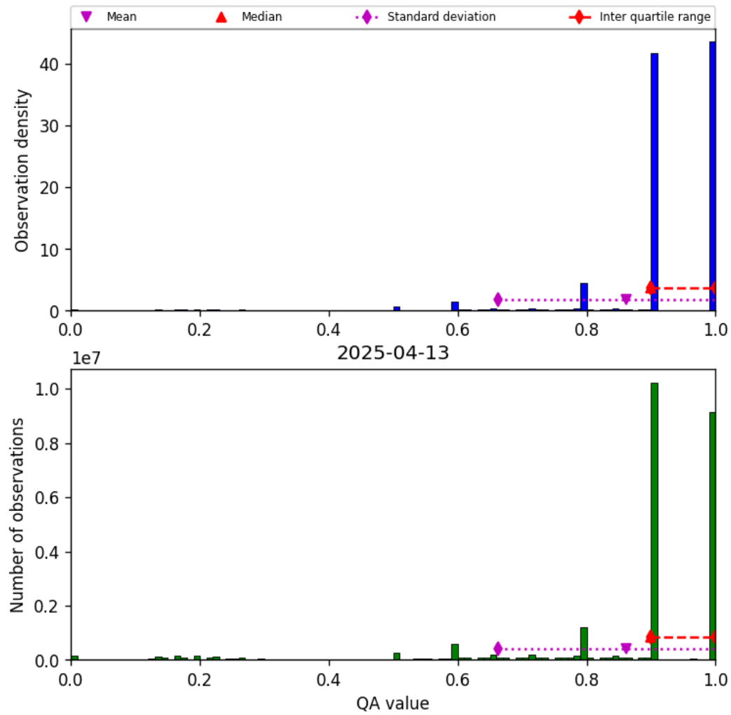
Figure 20: Histogram of “QA value” for 2025-04-13 to 2025-04-14
