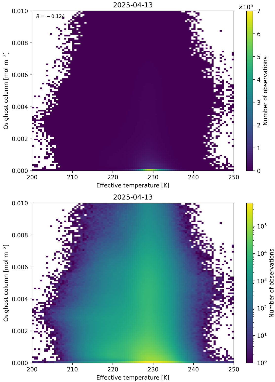
Figure 38: Scatter density plot of “Effective temperature” against “O 3 ghost column” for 2025-04-13 to 2025-04-14.
