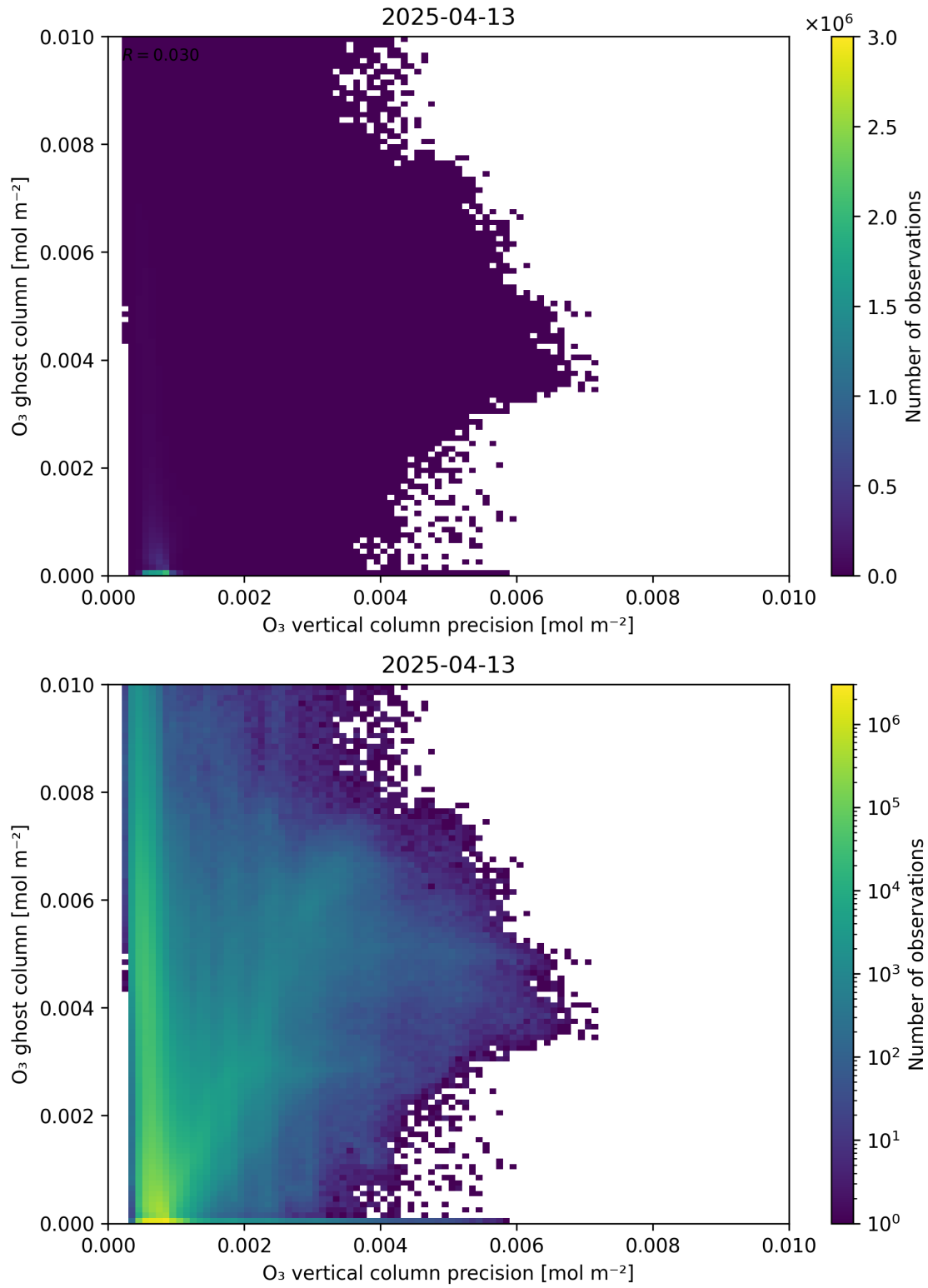
Figure 43: Scatter density plot of “ \text{O}_3 vertical column precision” against “ \text{O}_3 ghost column” for 2025-04-13 to 2025-04-14.
