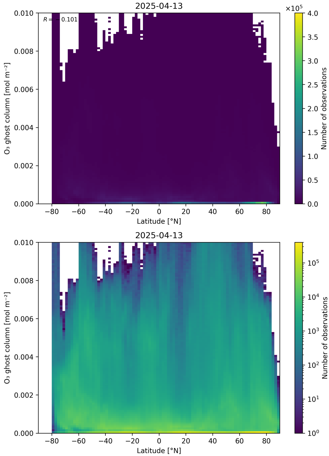
Figure 35: Scatter density plot of “Latitude” against “O 3 ghost column” for 2025-04-13 to 2025-04-14.
