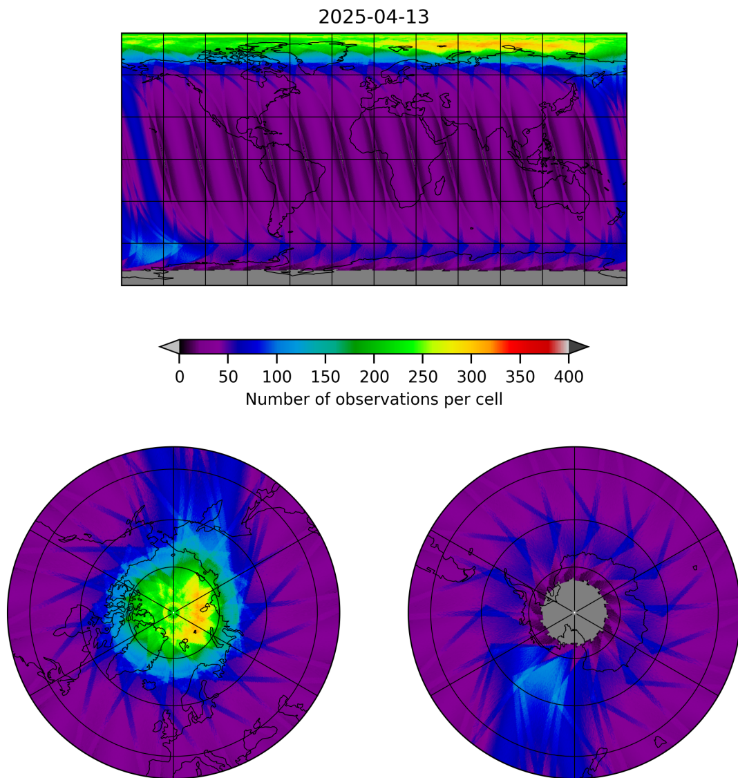
Figure 12: Map of the number of observations for 2025-04-13 to 2025-04-14
