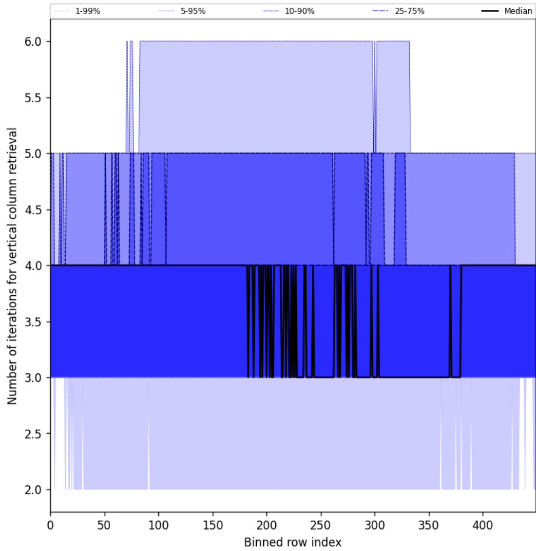
Figure 33: Along track statistics of “Number of iterations for vertical column retrieval” for 2025-04-13 to 2025-04-14
