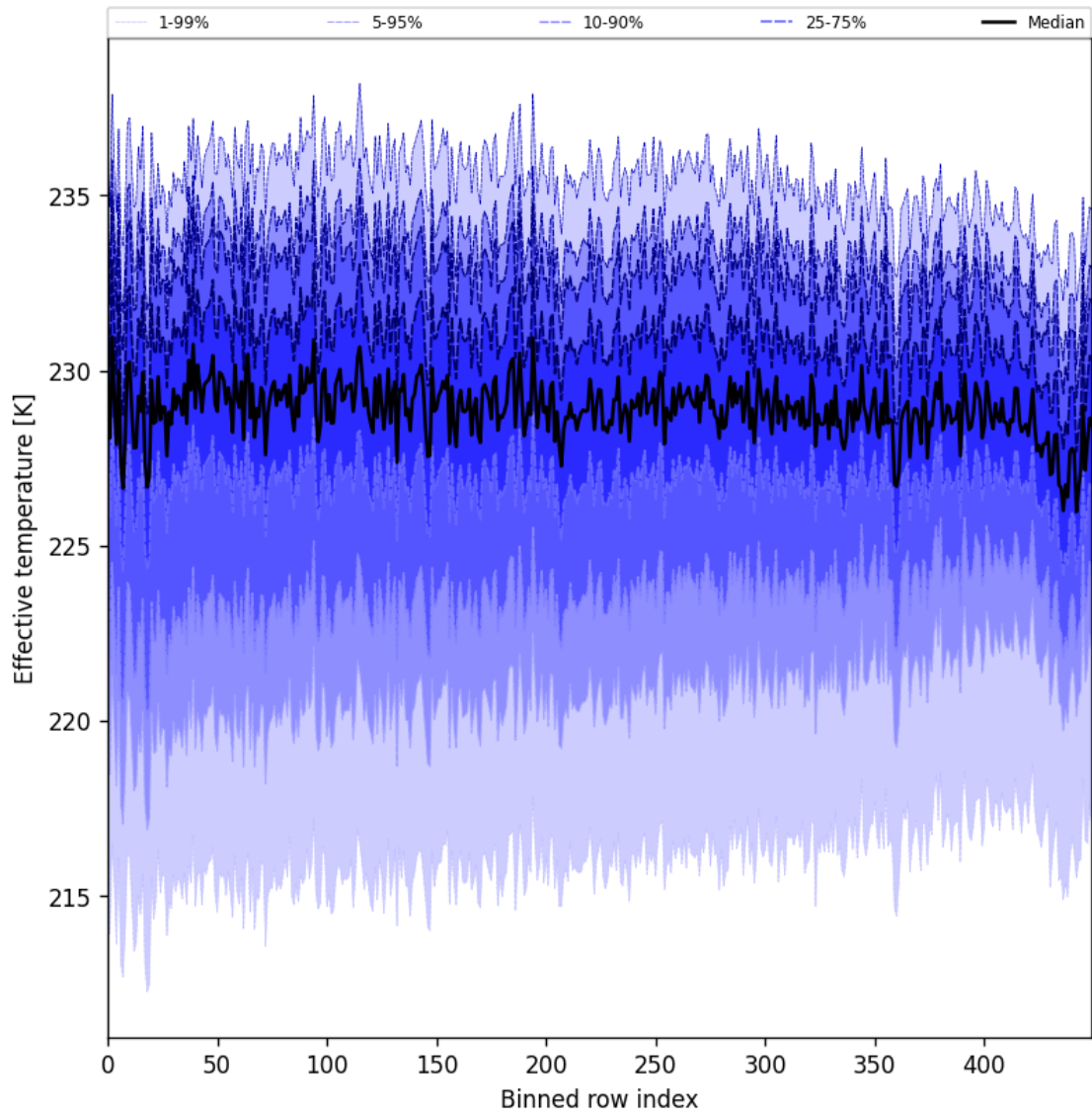
Figure 31: Along track statistics of “Effective temperature” for 2025-04-13 to 2025-04-14
