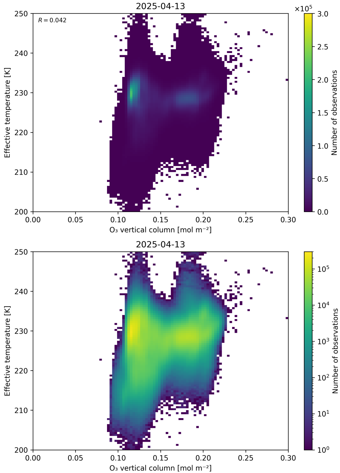
Figure 39: Scatter density plot of “O 3 vertical column” against “Effective temperature” for 2025-04-13 to 2025-04-14.
