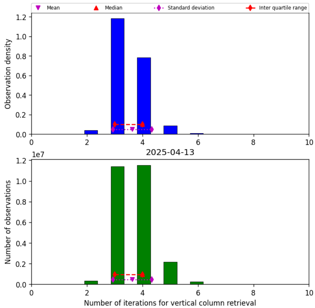
Figure 26: Histogram of “Number of iterations for vertical column retrieval” for 2025-04-13 to 2025-04-14
