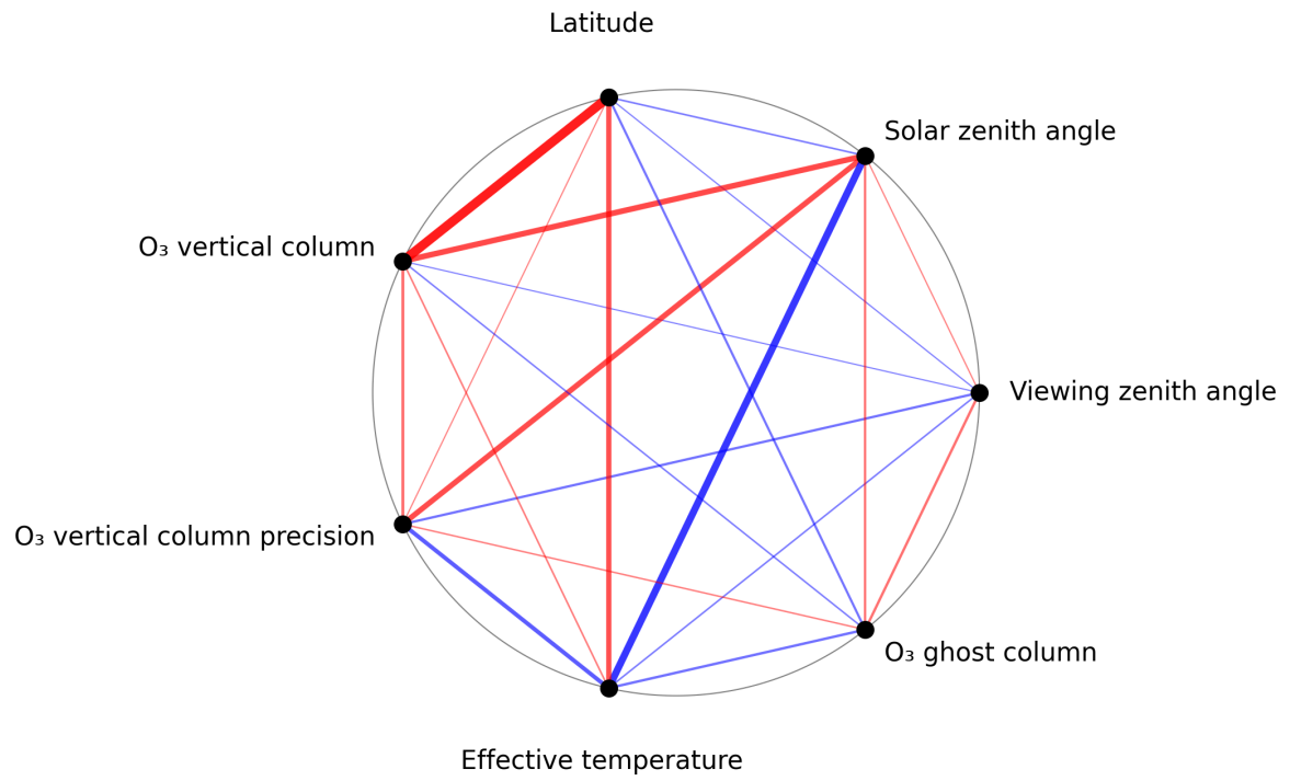
Figure 1: Map of correlation graph for 2025-04-13 to 2025-04-14.
