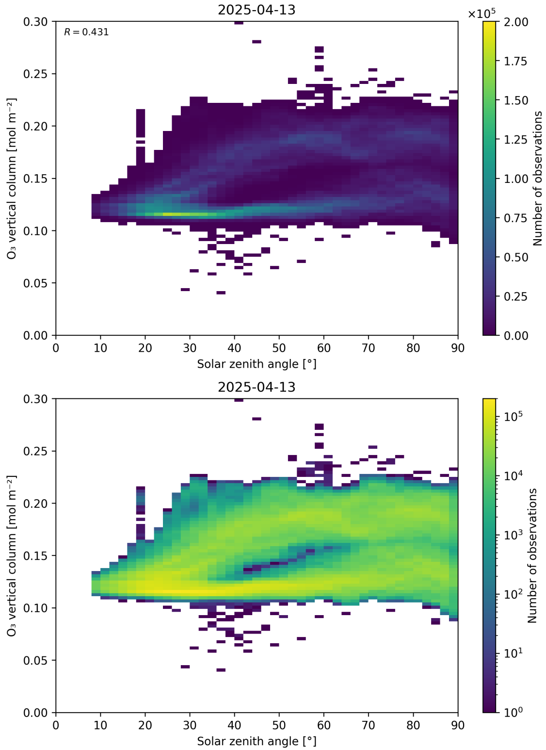
Figure 47: Scatter density plot of “Solar zenith angle” against “O 3 vertical column” for 2025-04-13 to 2025-04-14.
