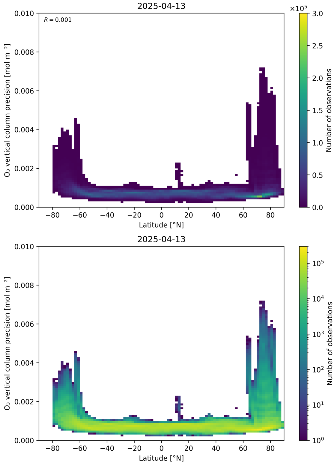
Figure 37: Scatter density plot of “Latitude” against “O 3 vertical column precision” for 2025-04-13 to 2025-04-14.
