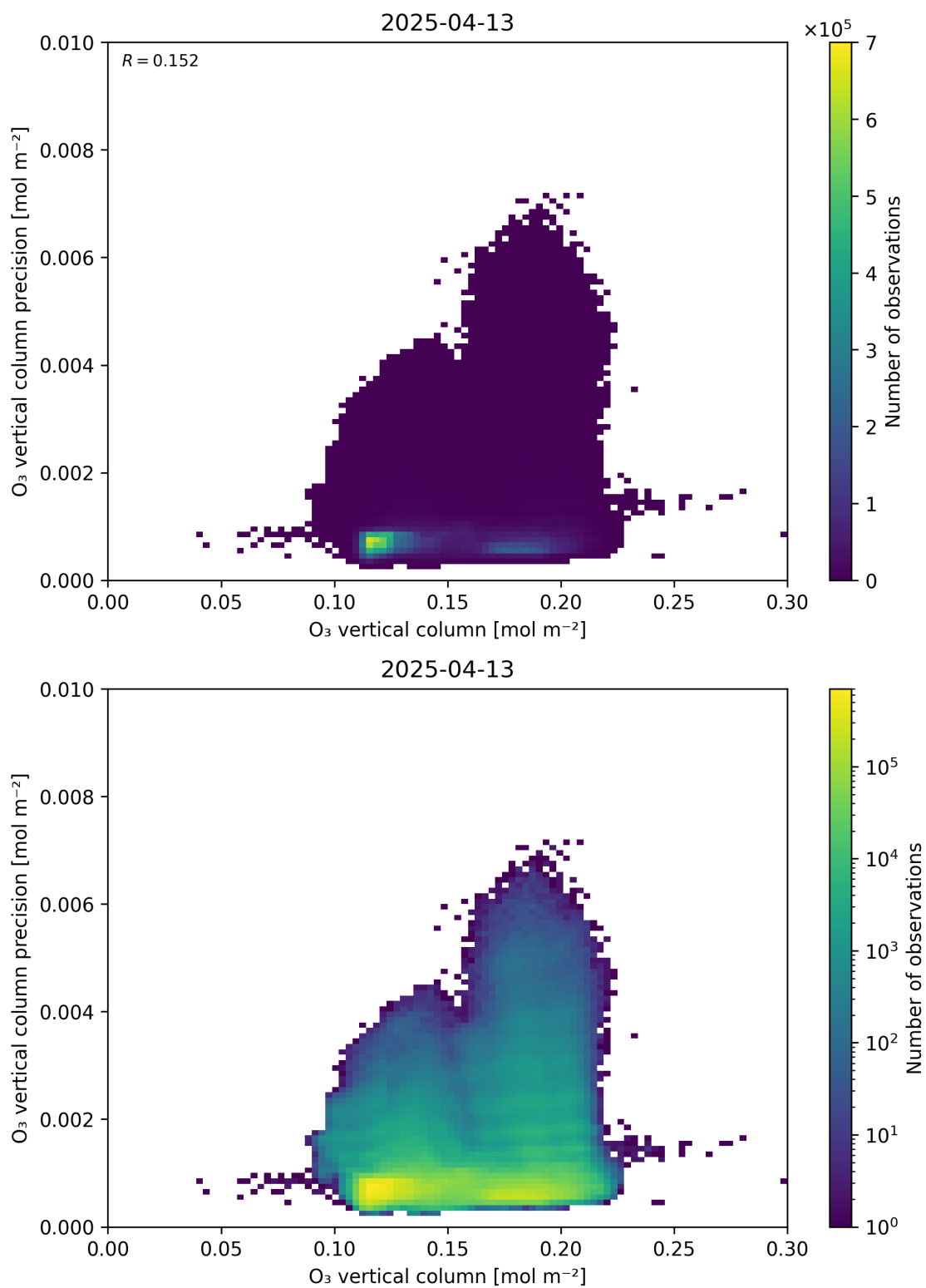
Figure 41: Scatter density plot of “O 3 vertical column” against “O 3 vertical column precision” for 2025-04-13 to 2025-04-14.
