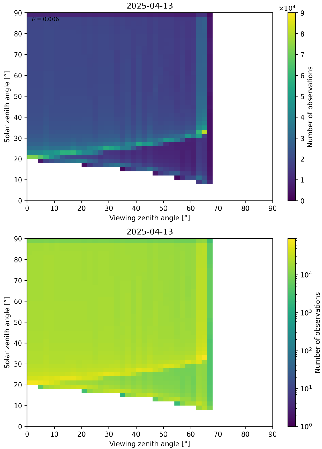
Figure 54: Scatter density plot of “Viewing zenith angle” against “Solar zenith angle” for 2025-04-13 to 2025-04-14.
