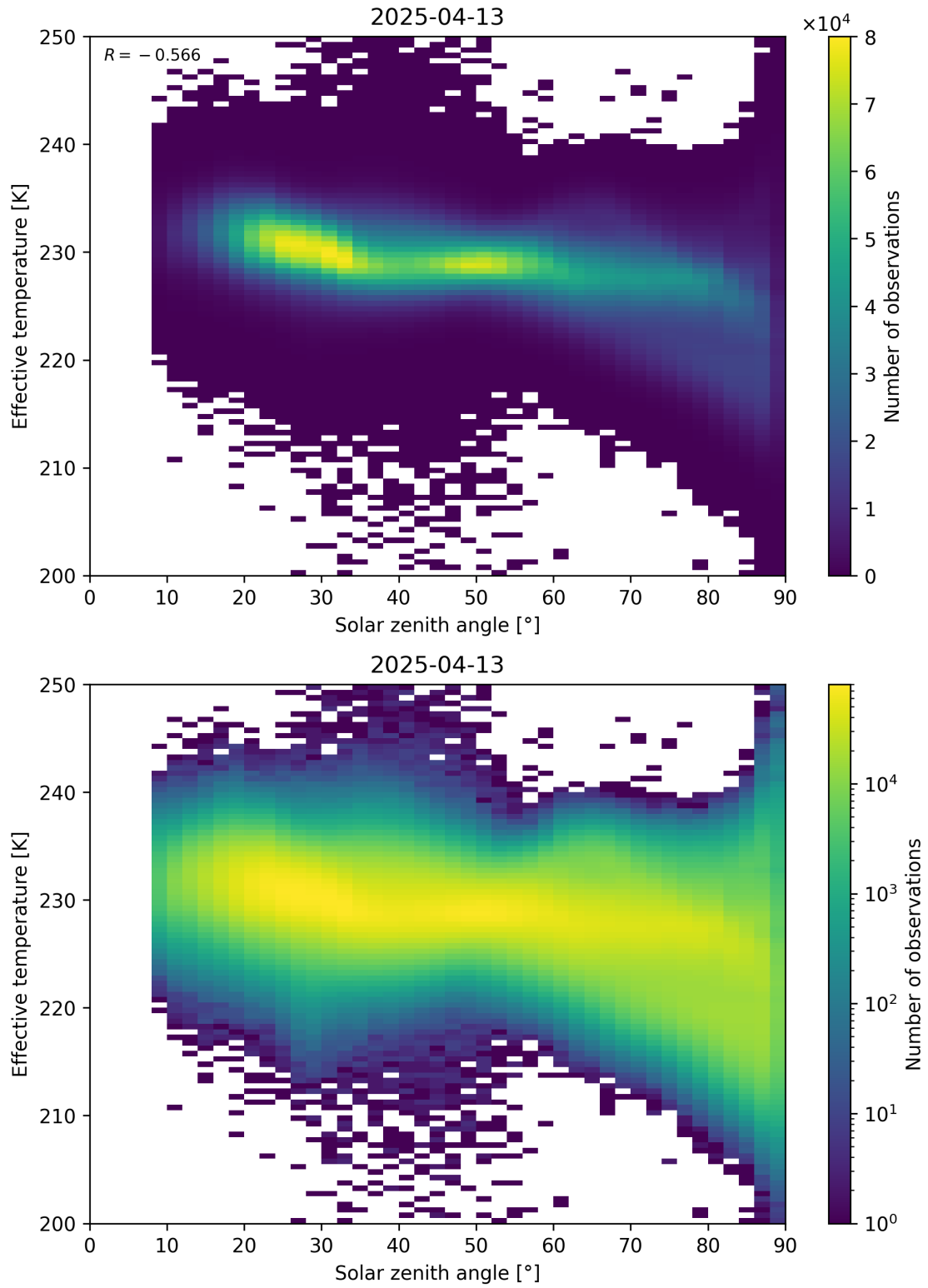
Figure 45: Scatter density plot of “Solar zenith angle” against “Effective temperature” for 2025-04-13 to 2025-04-14.
