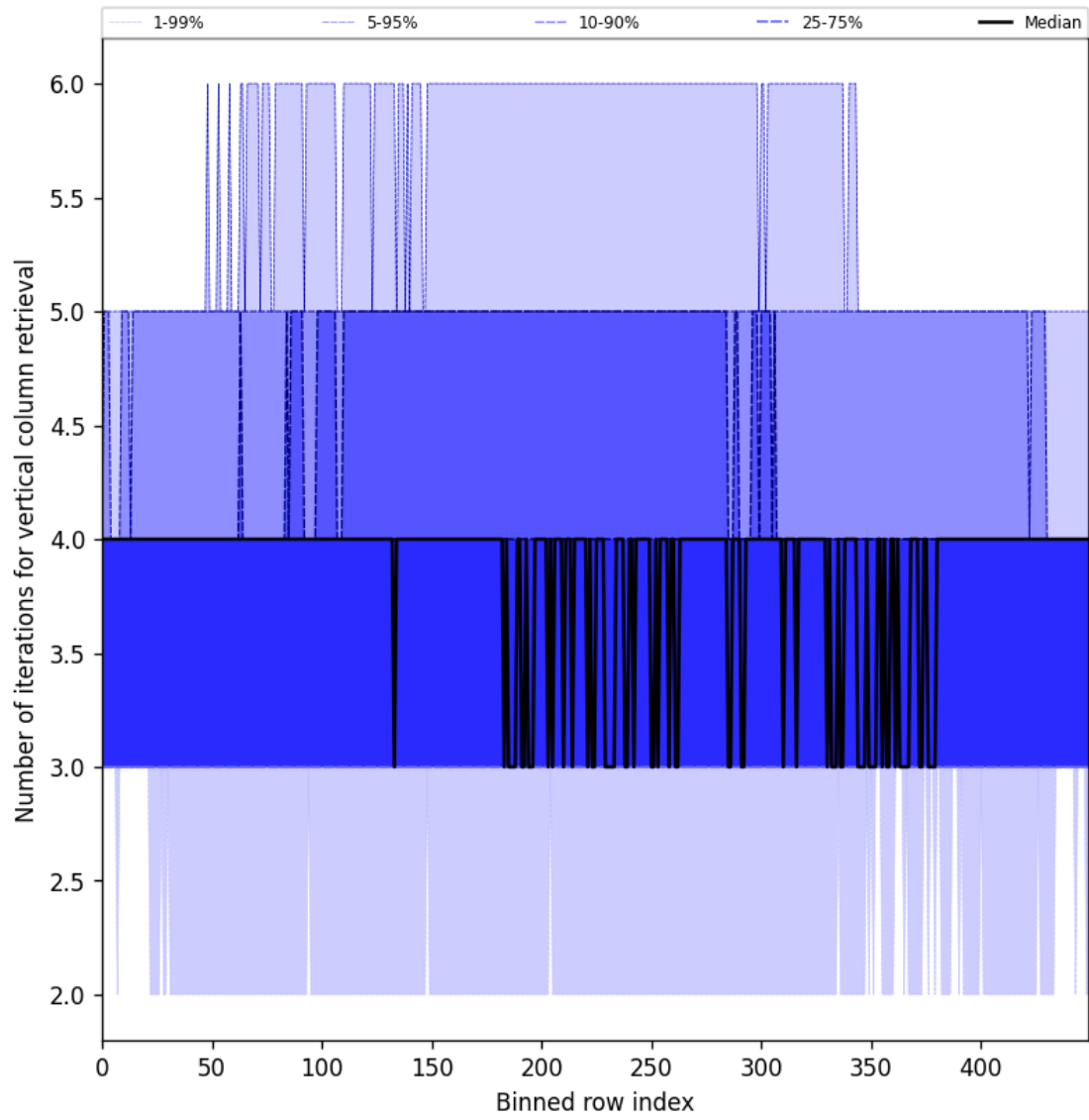
Figure 33: Along track statistics of “Number of iterations for vertical column retrieval” for 2025-04-13 to 2025-04-15
