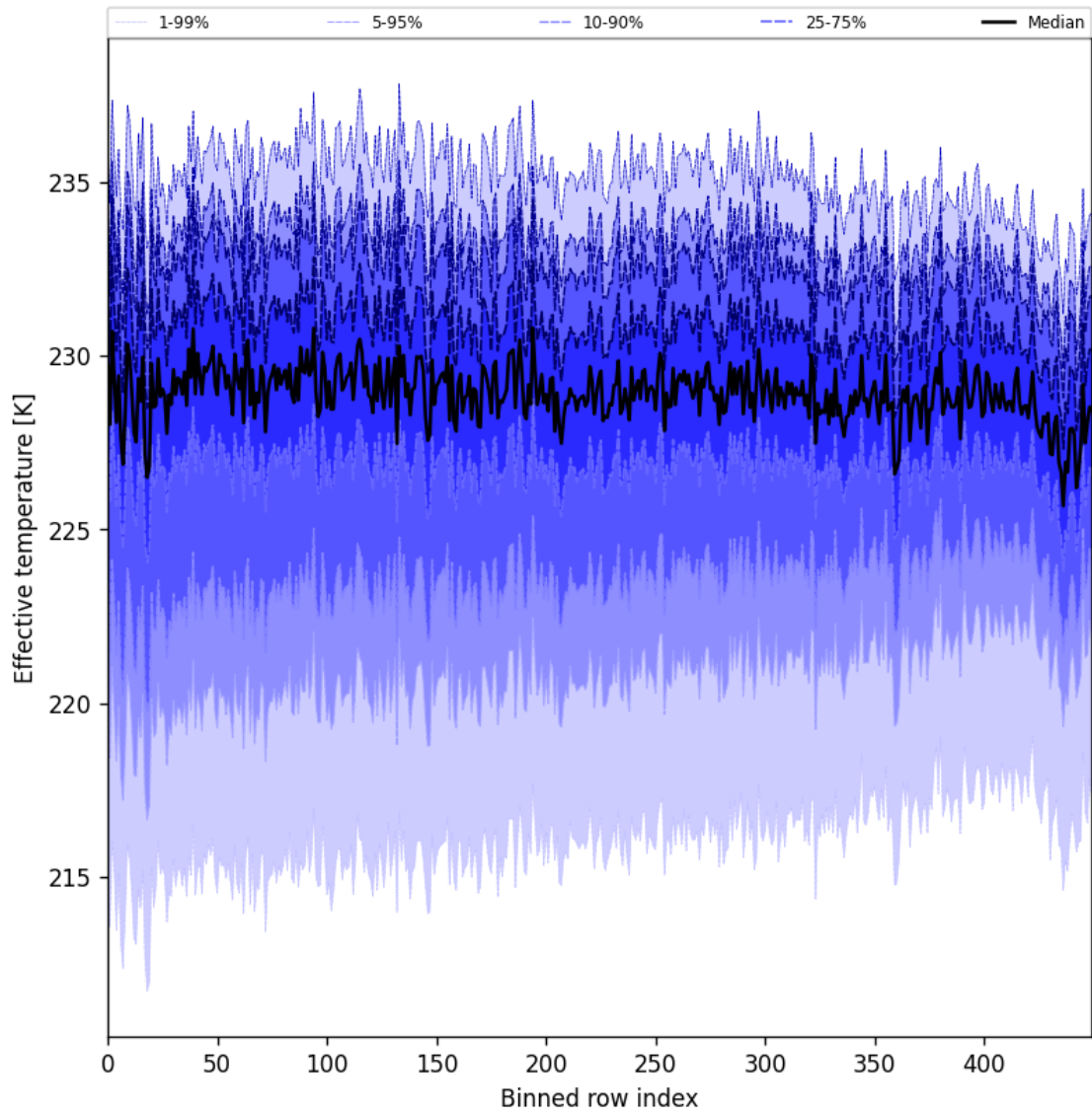
Figure 31: Along track statistics of “Effective temperature” for 2025-04-13 to 2025-04-15
