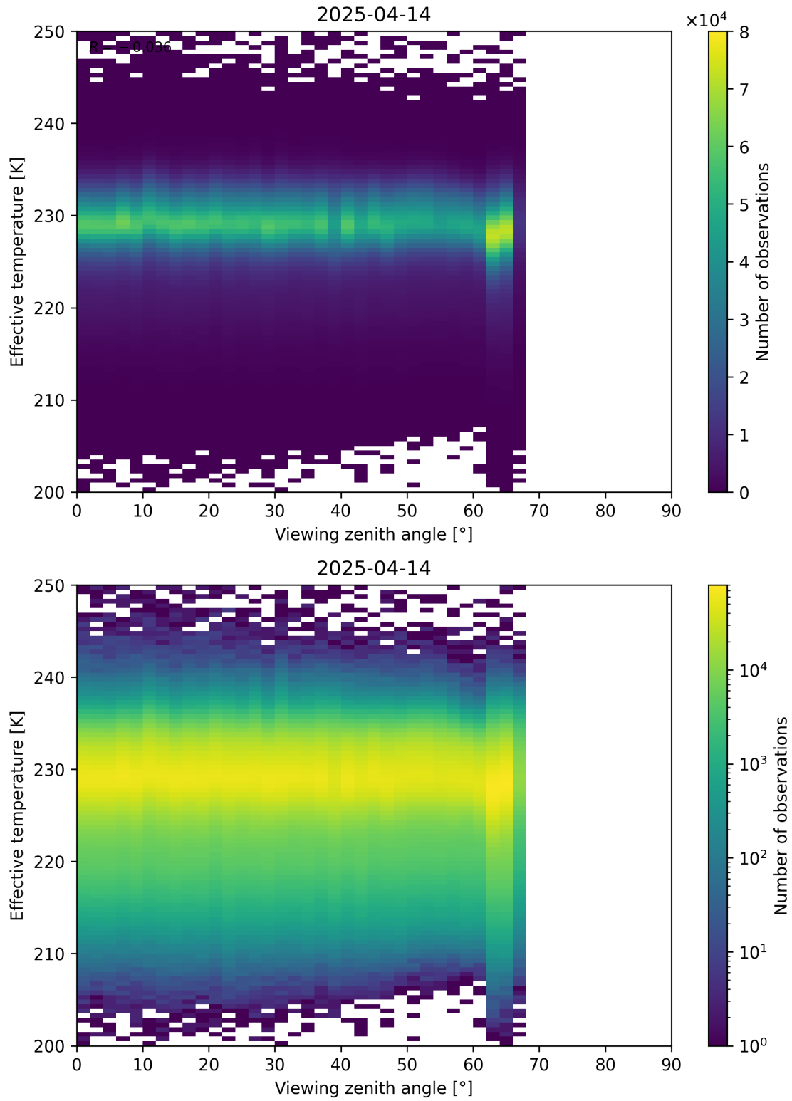
Figure 50: Scatter density plot of “Viewing zenith angle” against “Effective temperature” for 2025-04-13 to 2025-04-15.
