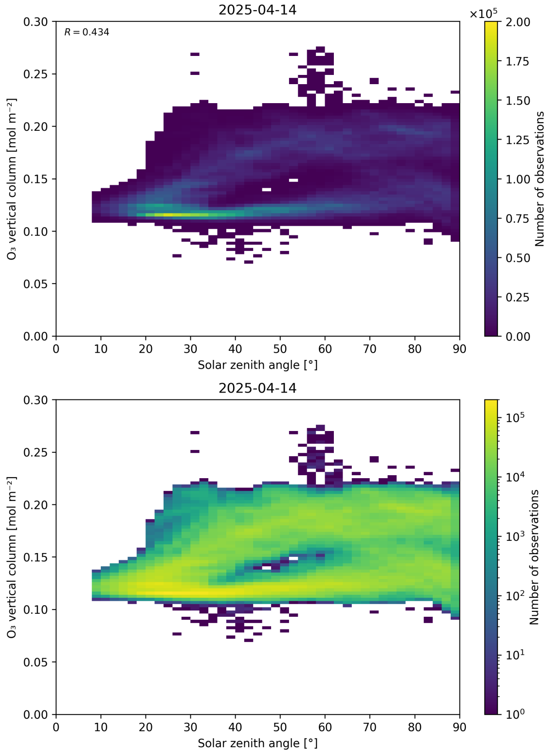
Figure 47: Scatter density plot of “Solar zenith angle” against “O 3 vertical column” for 2025-04-13 to 2025-04-15.
