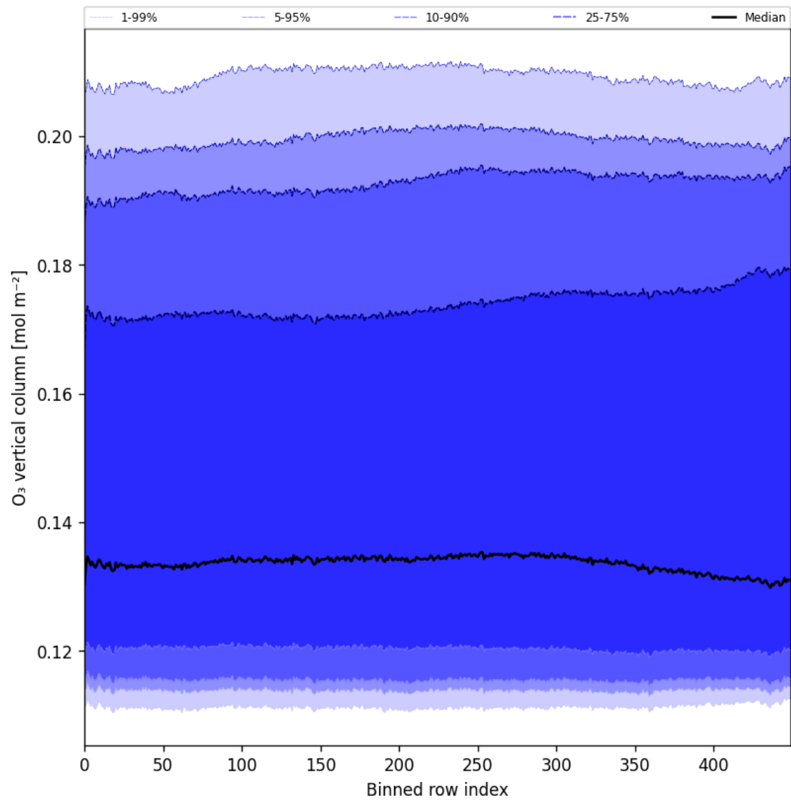
Figure 28: Along track statistics of “O 3 vertical column” for 2025-04-13 to 2025-04-15
