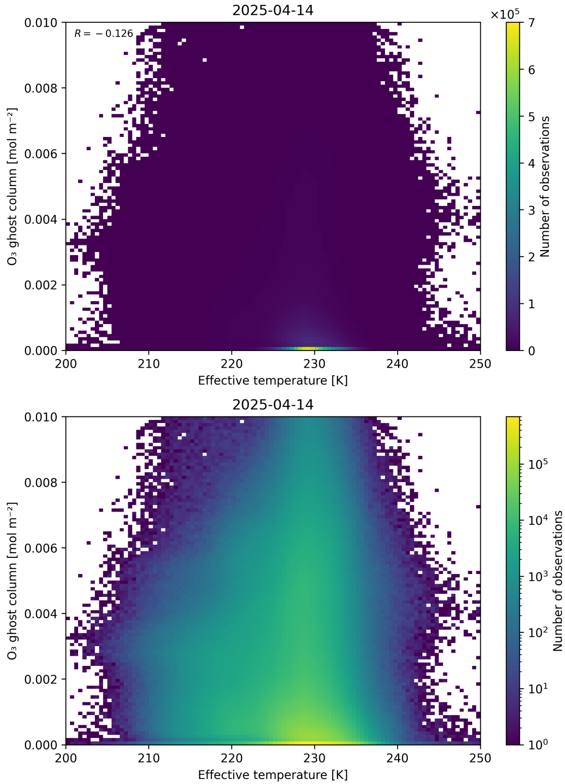
Figure 38: Scatter density plot of “Effective temperature” against “O 3 ghost column” for 2025-04-13 to 2025-04-15.
