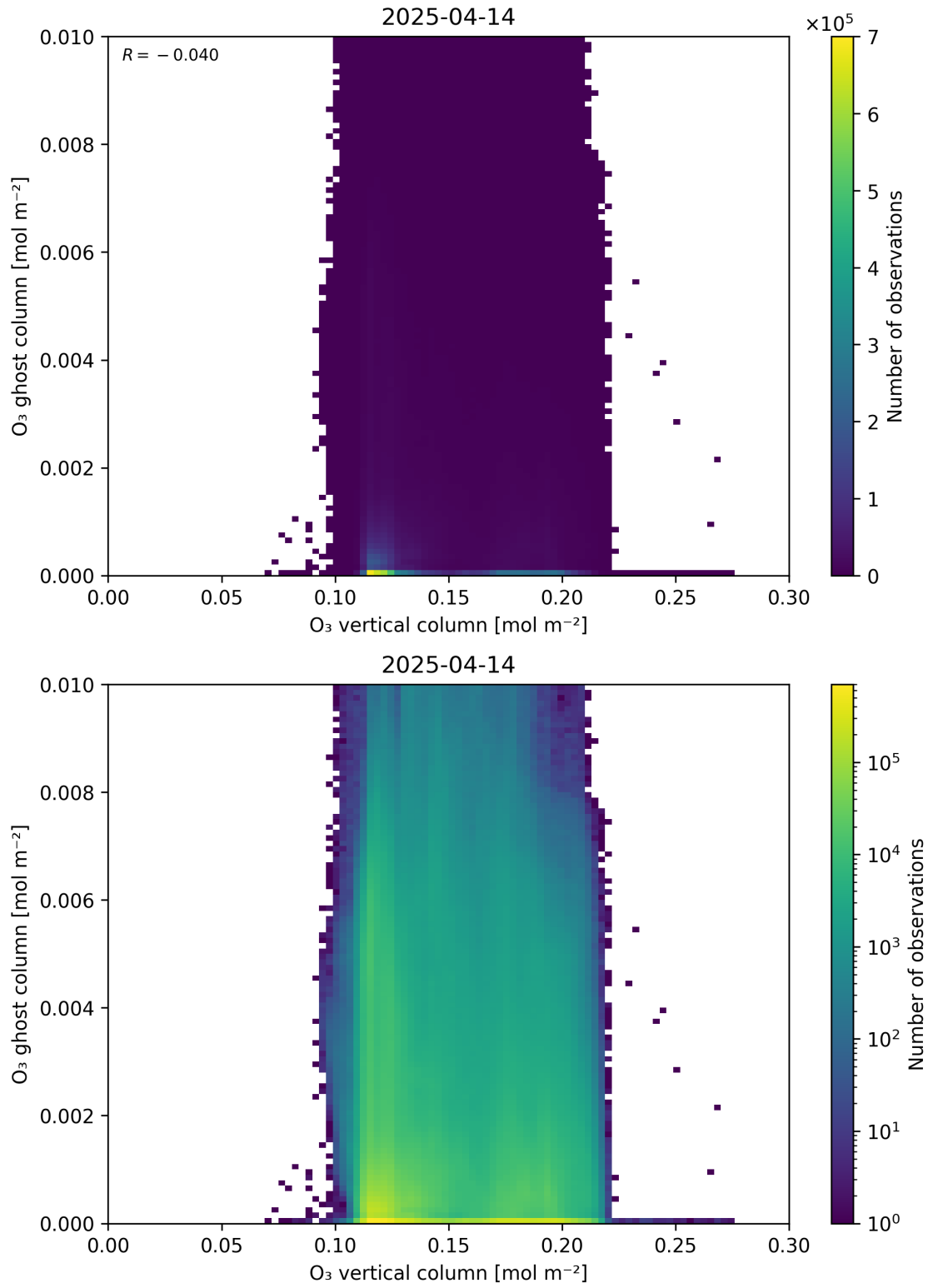
Figure 40: Scatter density plot of “O 3 vertical column” against “O 3 ghost column” for 2025-04-13 to 2025-04-15.
