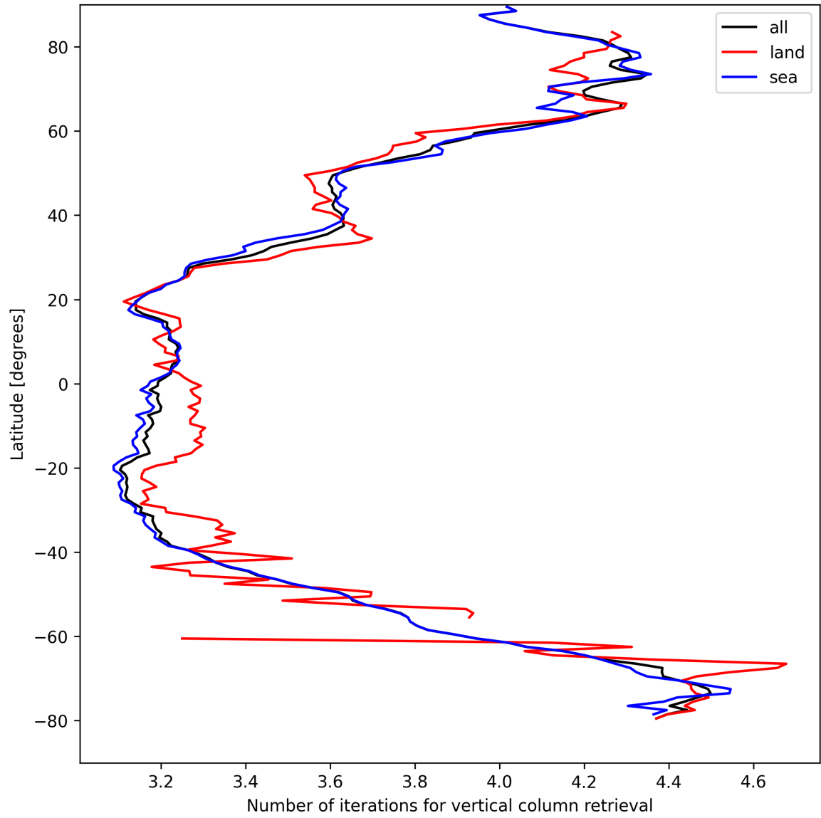
Figure 19: Zonal average of “Number of iterations for vertical column retrieval” for 2025-04-13 to 2025-04-15.
