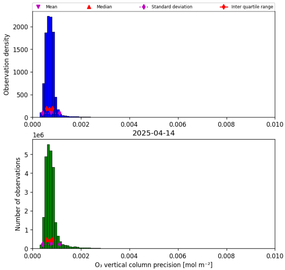
Figure 22: Histogram of “O 3 vertical column precision” for 2025-04-13 to 2025-04-15
