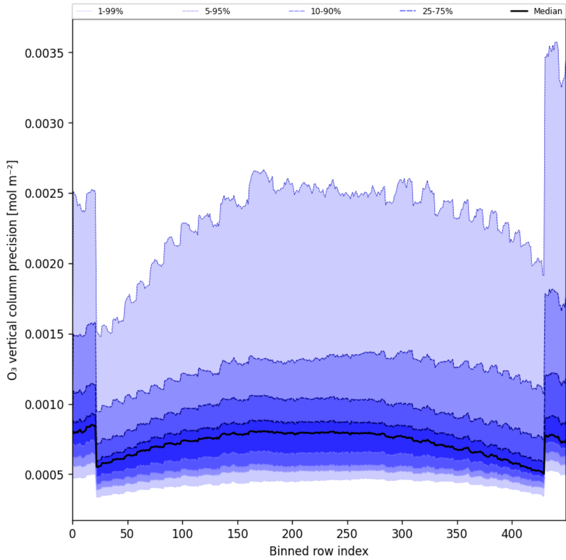
Figure 29: Along track statistics of “O 3 vertical column precision” for 2025-04-13 to 2025-04-15
