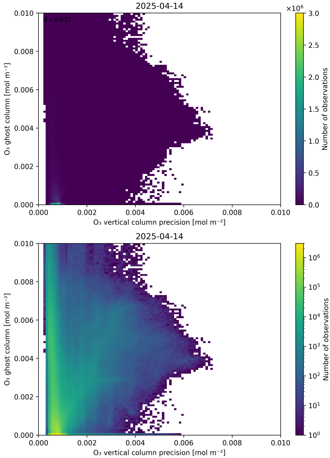
Figure 43: Scatter density plot of “O 3 vertical column precision” against “O 3 ghost column” for 2025-04-13 to 2025-04-15.
