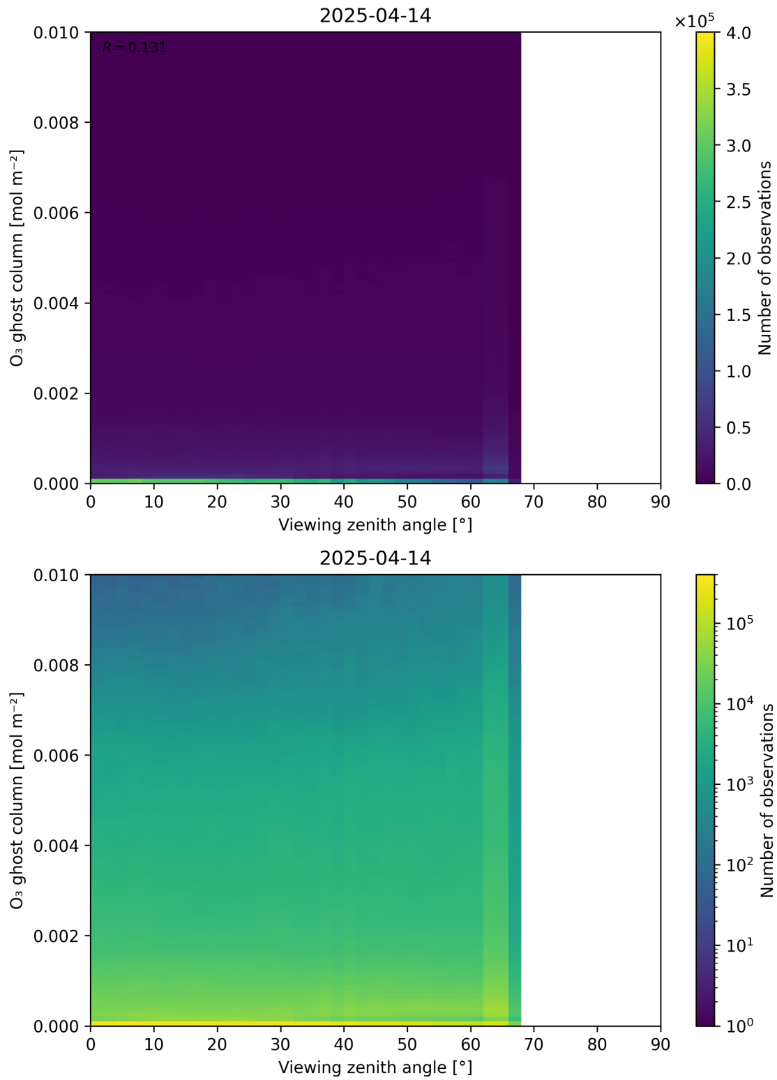
Figure 51: Scatter density plot of “Viewing zenith angle” against “O 3 ghost column” for 2025-04-13 to 2025-04-15.
