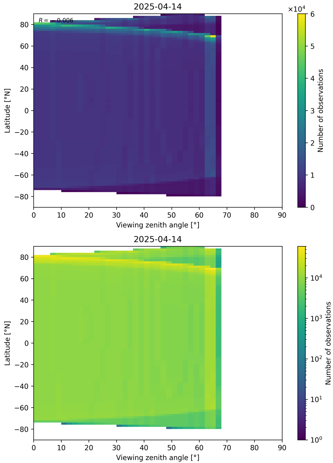
Figure 49: Scatter density plot of “Viewing zenith angle” against “Latitude” for 2025-04-13 to 2025-04-15.
