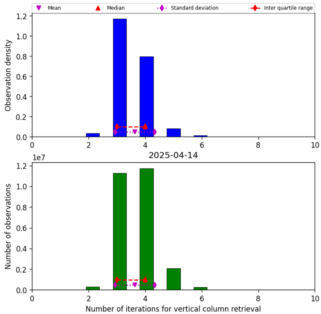
Figure 26: Histogram of “Number of iterations for vertical column retrieval” for 2025-04-13 to 2025-04-15
