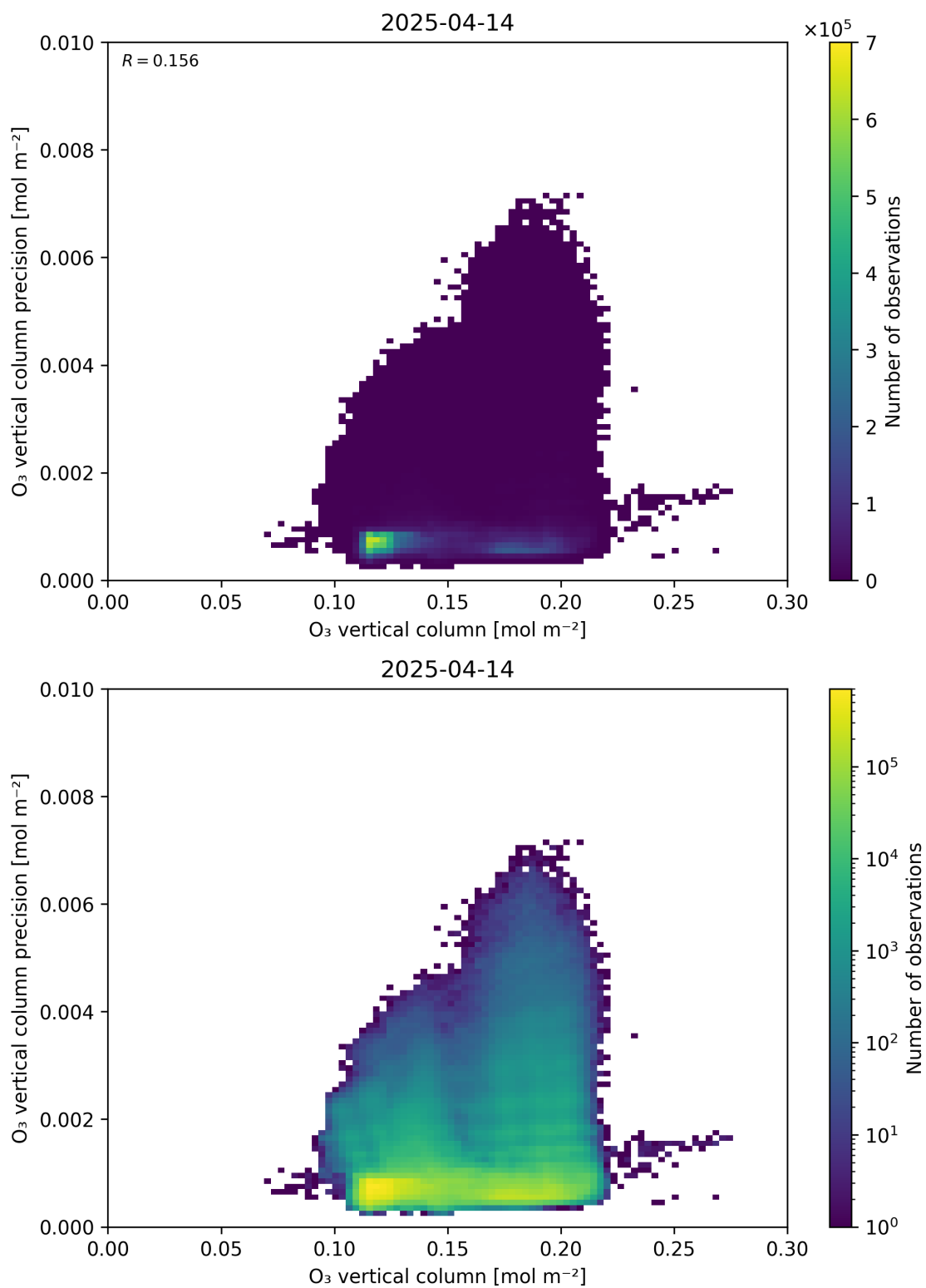
Figure 41: Scatter density plot of “O 3 vertical column” against “O 3 vertical column precision” for 2025-04-13 to 2025-04-15.
