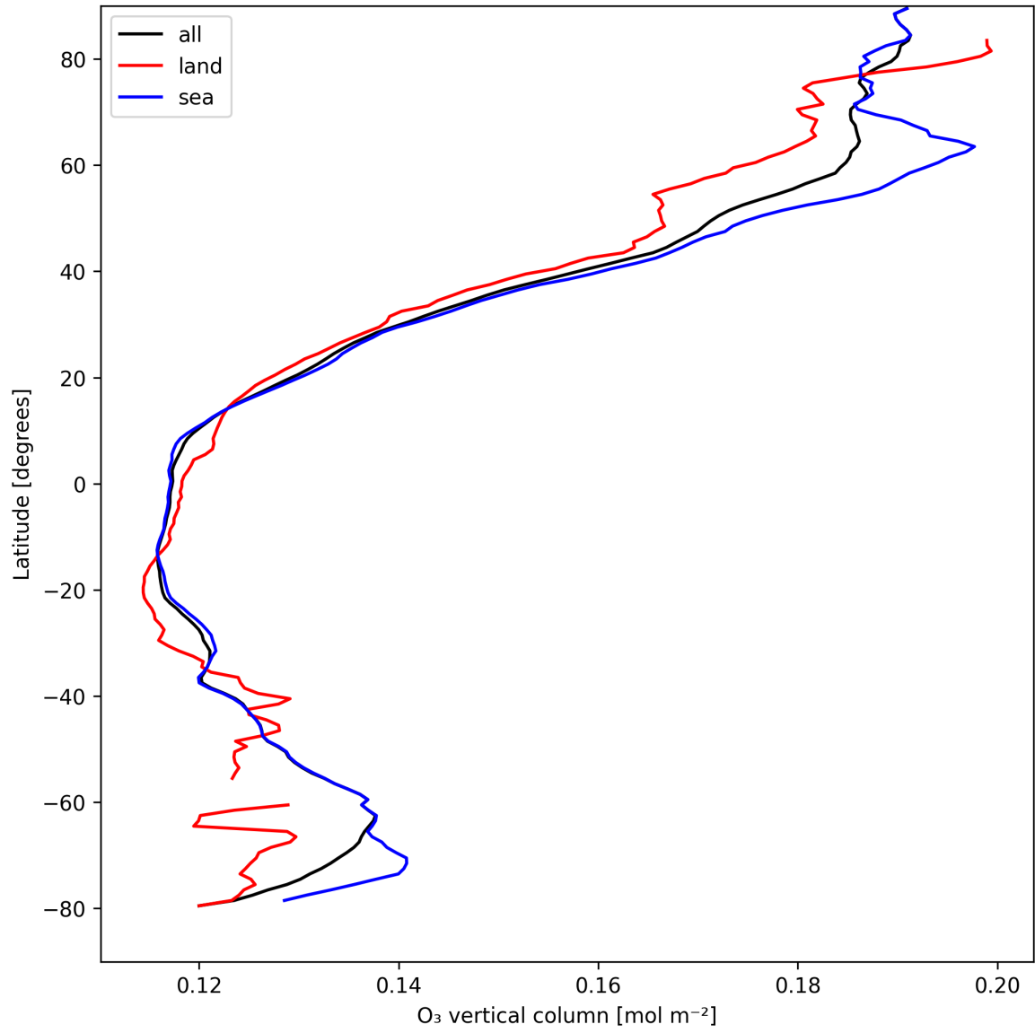
Figure 14: Zonal average of “O 3 vertical column” for 2025-04-13 to 2025-04-15.
