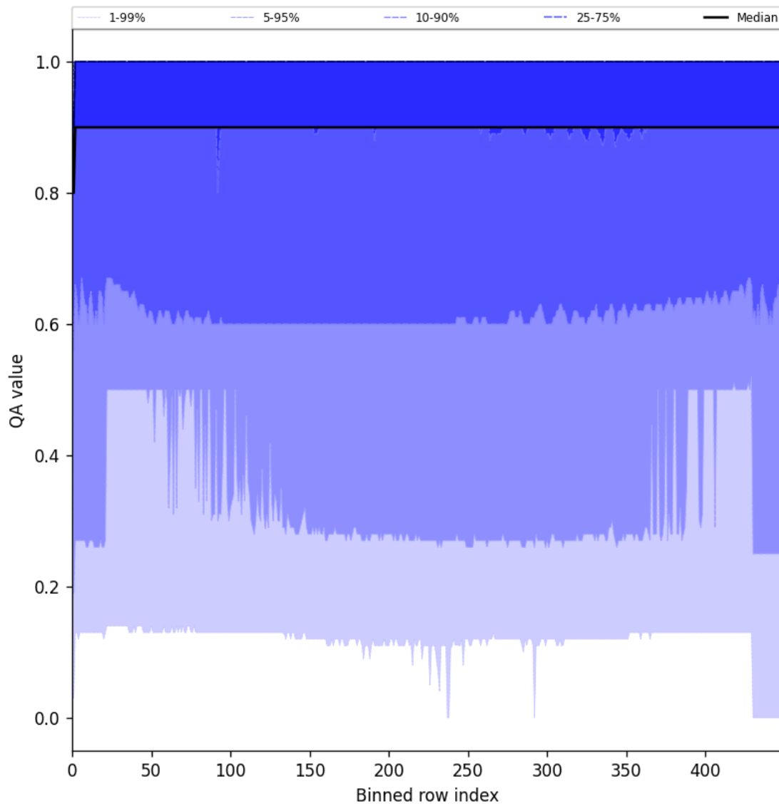
Figure 27: Along track statistics of “QA value” for 2025-04-13 to 2025-04-15
