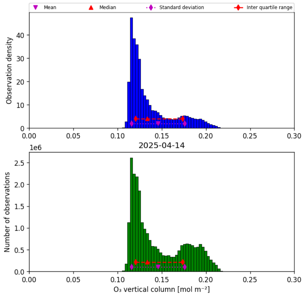
Figure 21: Histogram of “O 3 vertical column” for 2025-04-13 to 2025-04-15
