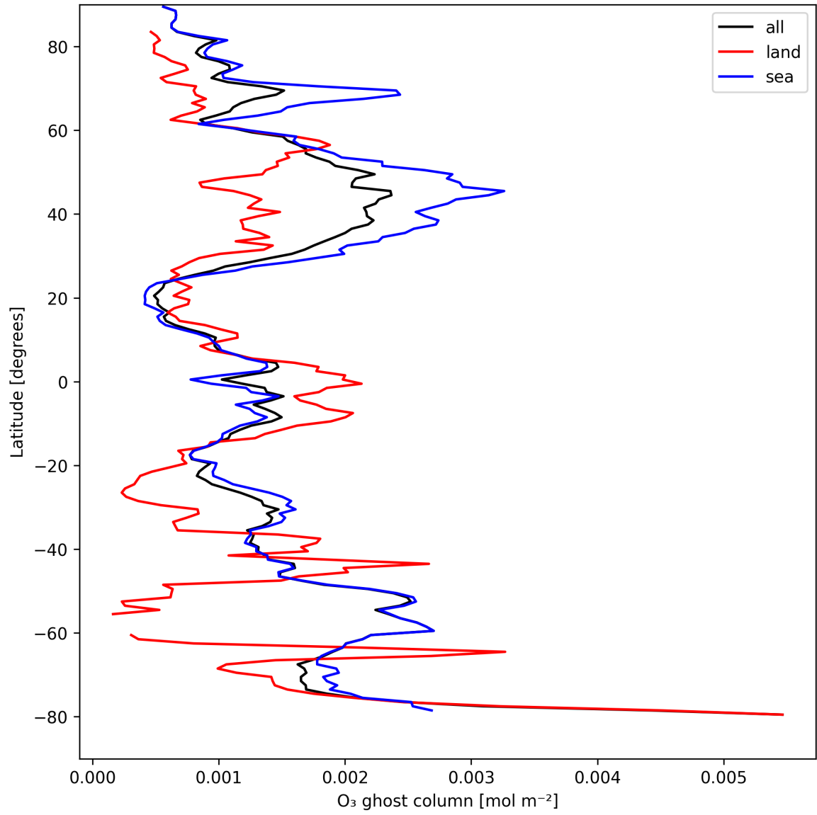
Figure 18: Zonal average of “O 3 ghost column” for 2025-04-13 to 2025-04-15.
