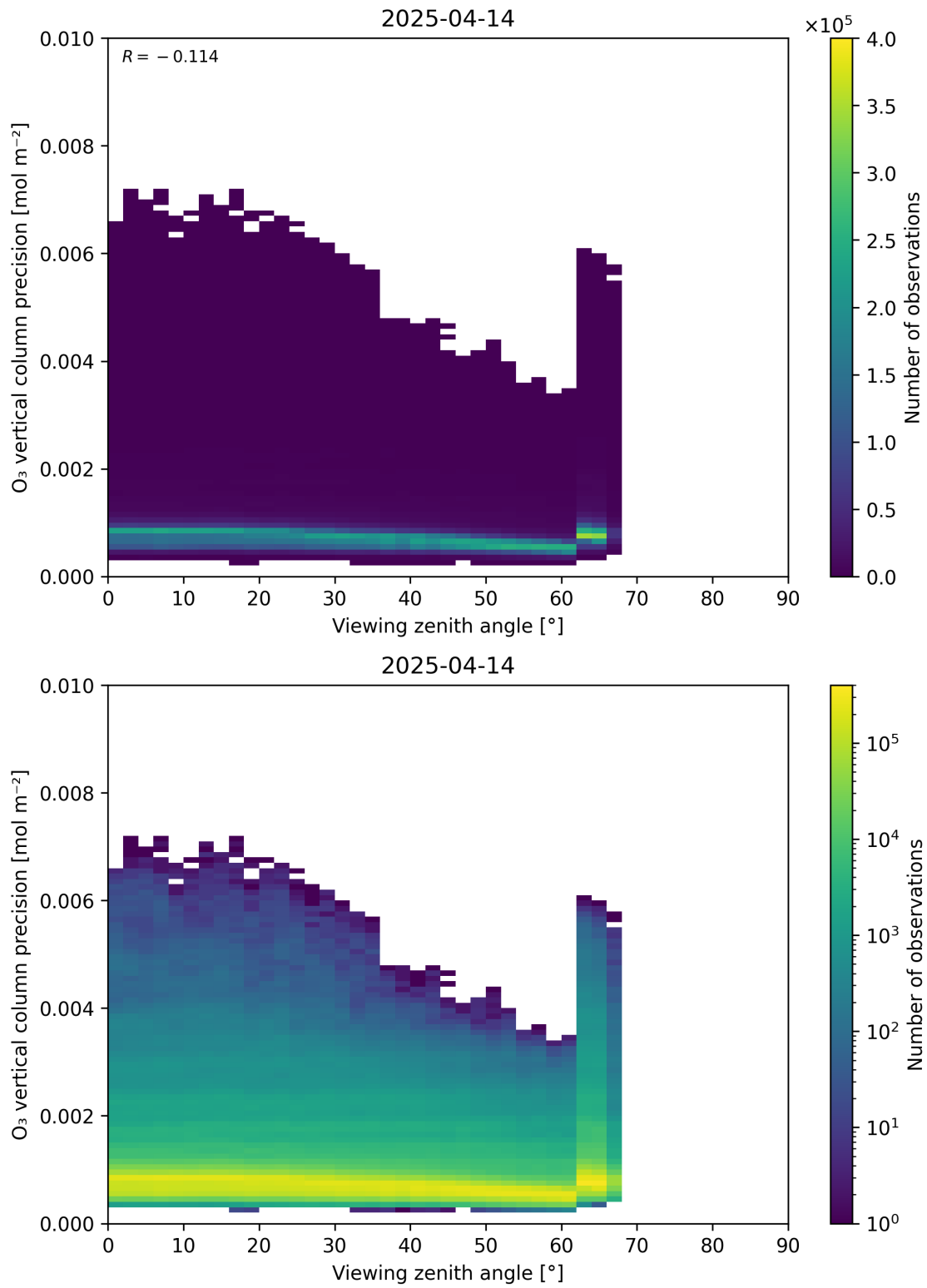
Figure 53: Scatter density plot of “Viewing zenith angle” against “O 3 vertical column precision” for 2025-04-13 to 2025-04-15.
