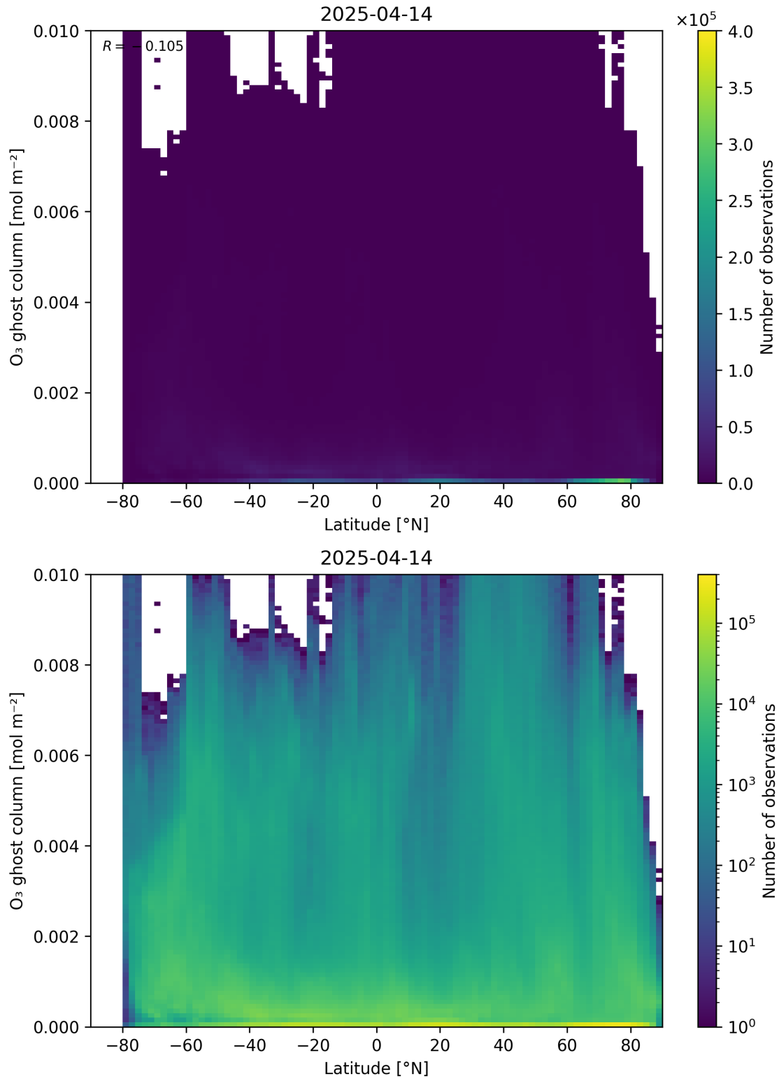
Figure 35: Scatter density plot of “Latitude” against “O 3 ghost column” for 2025-04-13 to 2025-04-15.
