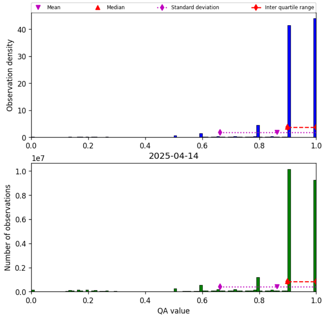
Figure 20: Histogram of “QA value” for 2025-04-13 to 2025-04-15
