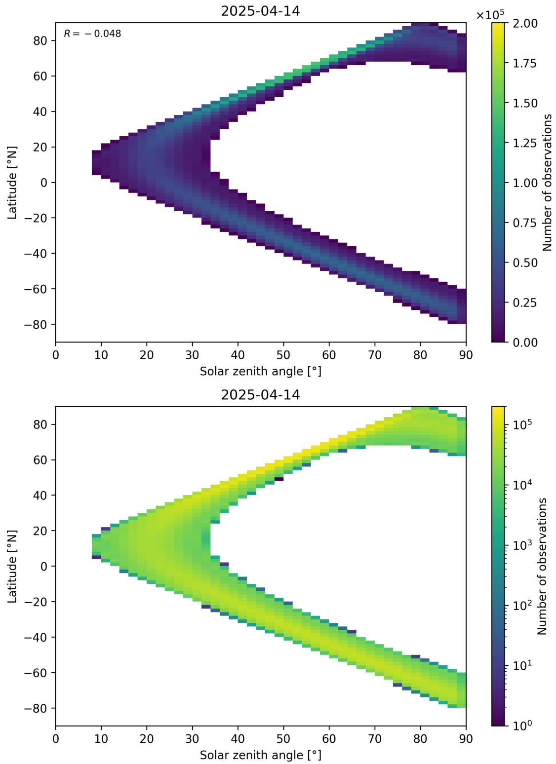
Figure 44: Scatter density plot of “Solar zenith angle” against “Latitude” for 2025-04-13 to 2025-04-15.
