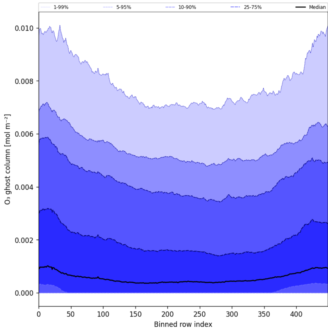
Figure 32: Along track statistics of “O 3 ghost column” for 2025-04-13 to 2025-04-15
