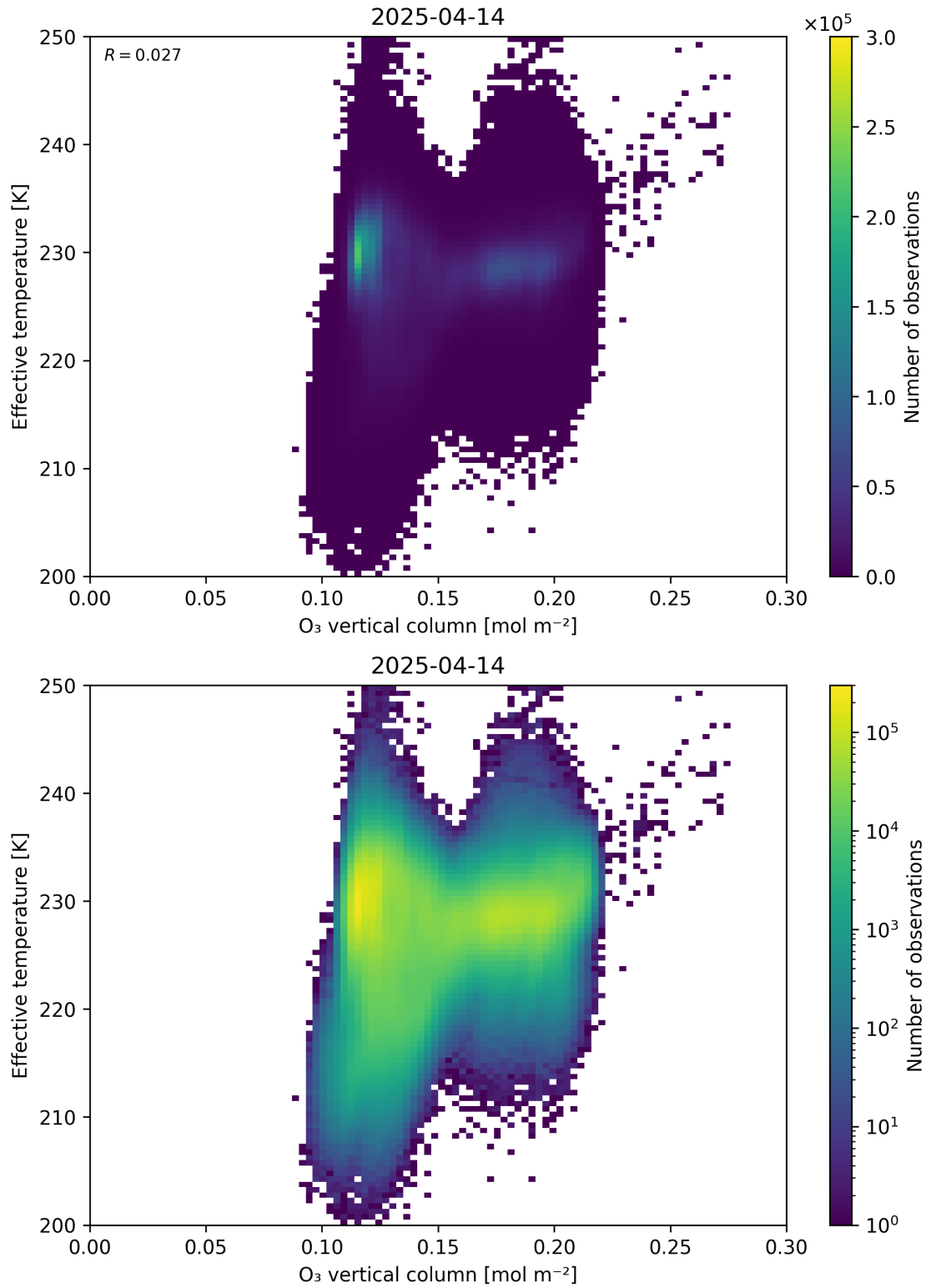
Figure 39: Scatter density plot of “O 3 vertical column” against “Effective temperature” for 2025-04-13 to 2025-04-15.
