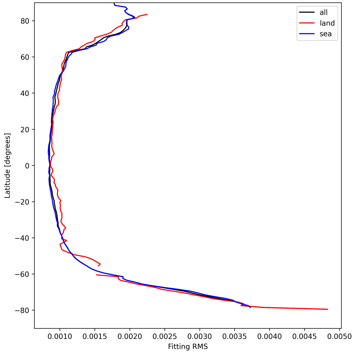
Figure 16: Zonal average of “Fitting RMS” for 2025-04-13 to 2025-04-15.
