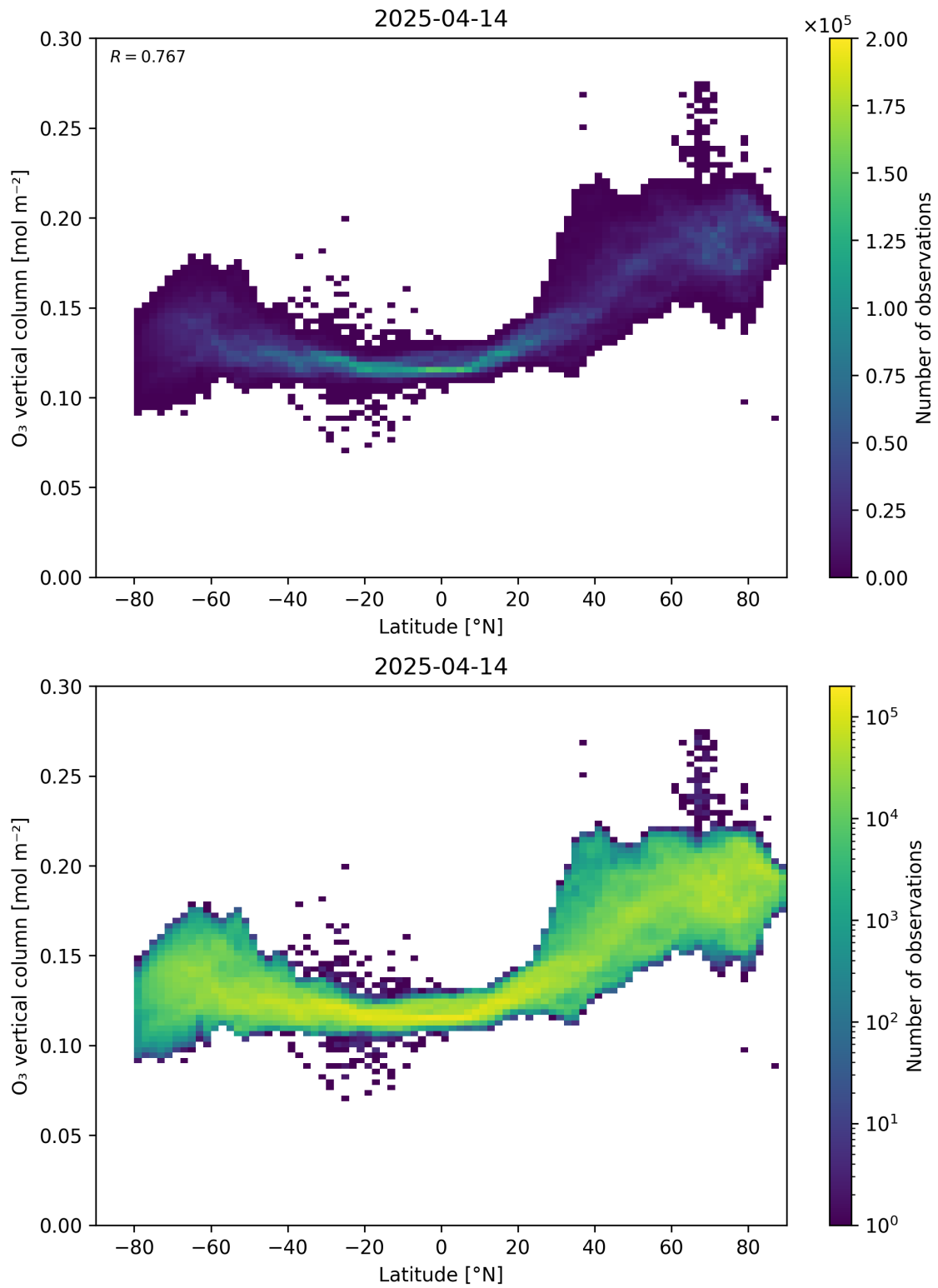
Figure 36: Scatter density plot of “Latitude” against “O 3 vertical column” for 2025-04-13 to 2025-04-15.
