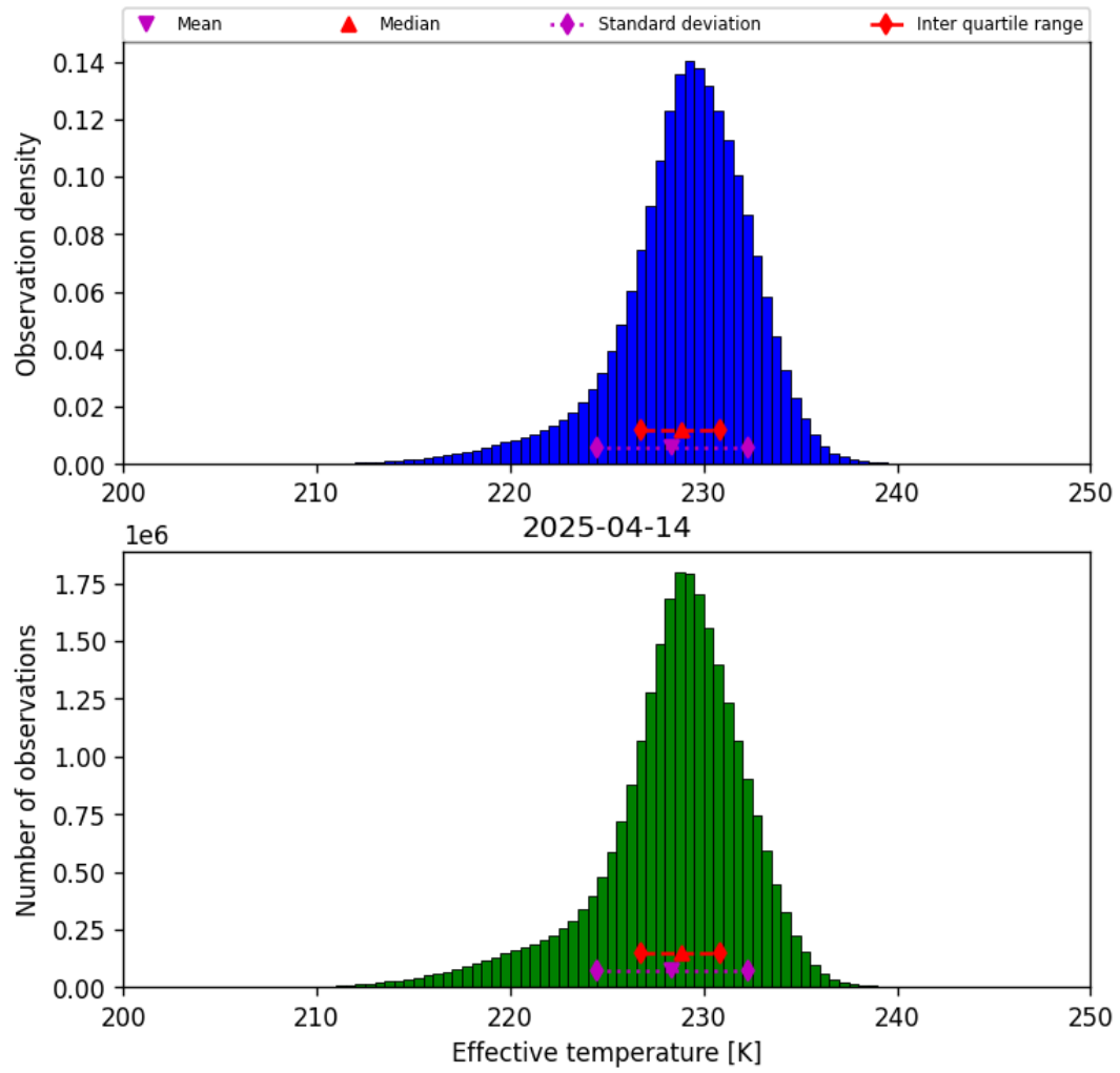
Figure 24: Histogram of “Effective temperature” for 2025-04-13 to 2025-04-15
