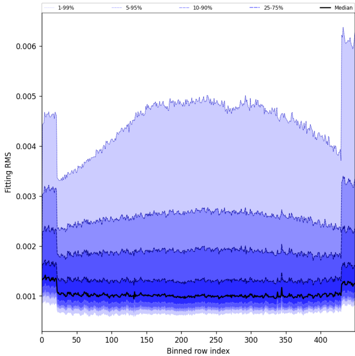
Figure 30: Along track statistics of “Fitting RMS” for 2025-04-13 to 2025-04-15
