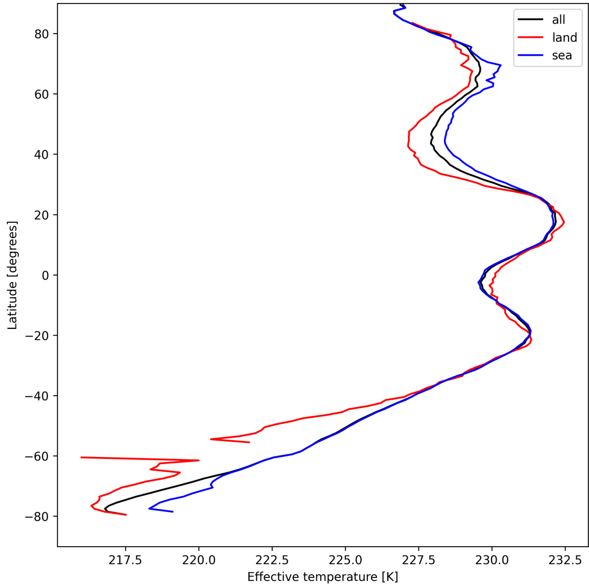
Figure 17: Zonal average of “Effective temperature” for 2025-04-13 to 2025-04-15.
