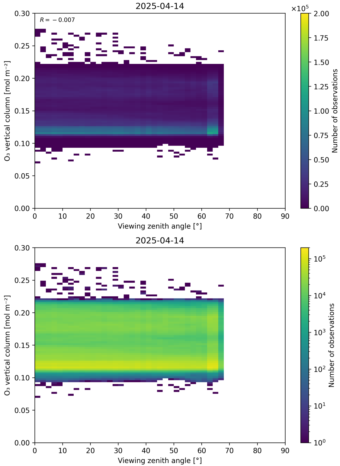
Figure 52: Scatter density plot of “Viewing zenith angle” against “O 3 vertical column” for 2025-04-13 to 2025-04-15.
