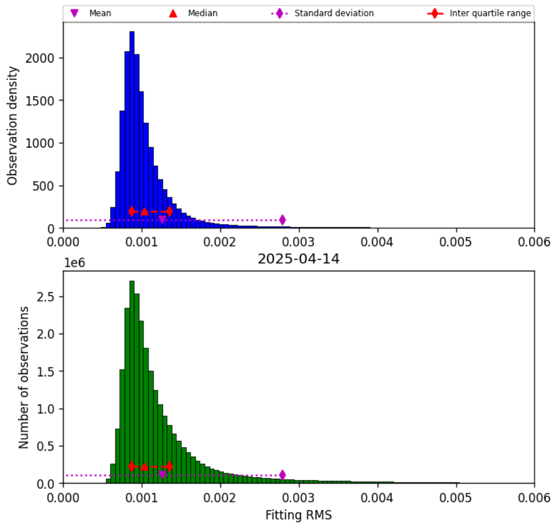
Figure 23: Histogram of “Fitting RMS” for 2025-04-13 to 2025-04-15
