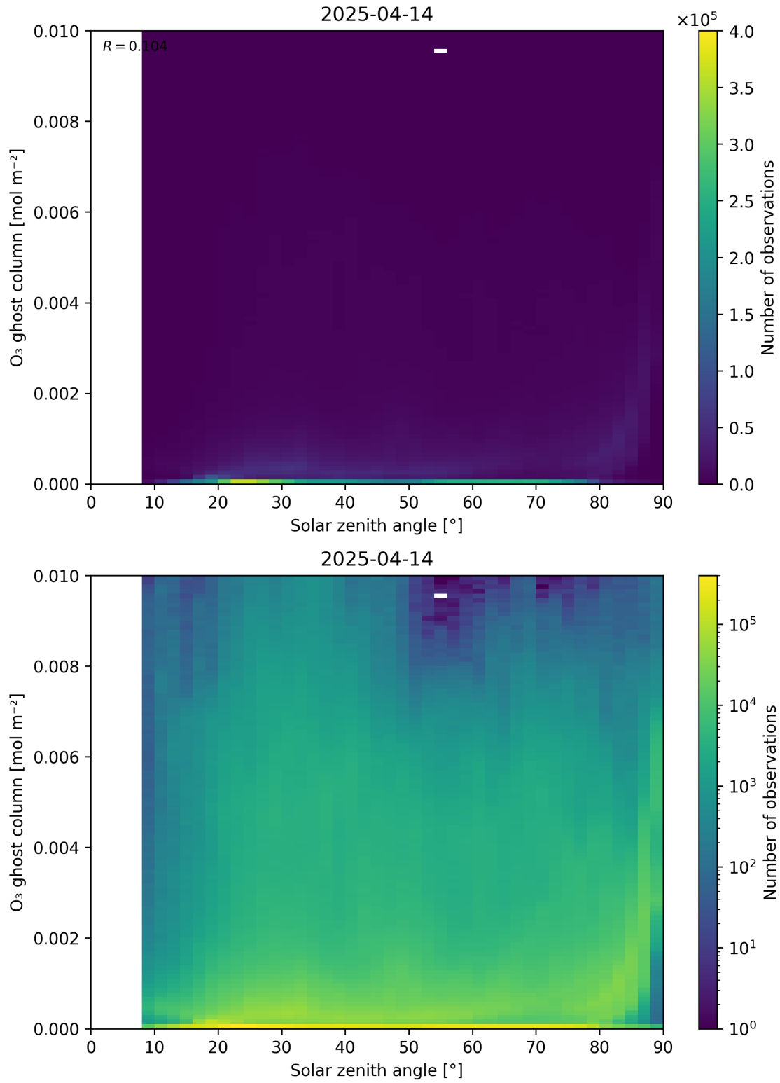
Figure 46: Scatter density plot of “Solar zenith angle” against “O 3 ghost column” for 2025-04-13 to 2025-04-15.
