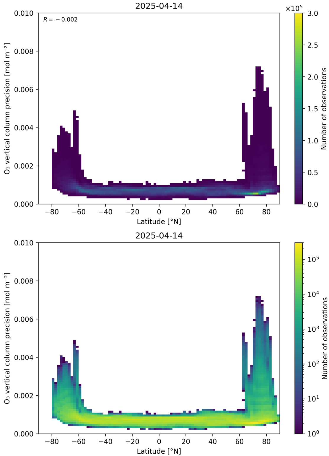
Figure 37: Scatter density plot of “Latitude” against “O 3 vertical column precision” for 2025-04-13 to 2025-04-15.
