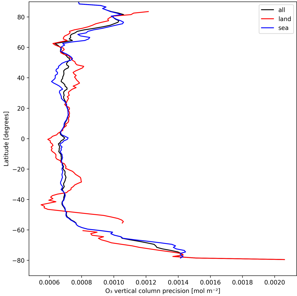
Figure 15: Zonal average of “O 3 vertical column precision” for 2025-04-13 to 2025-04-15.
