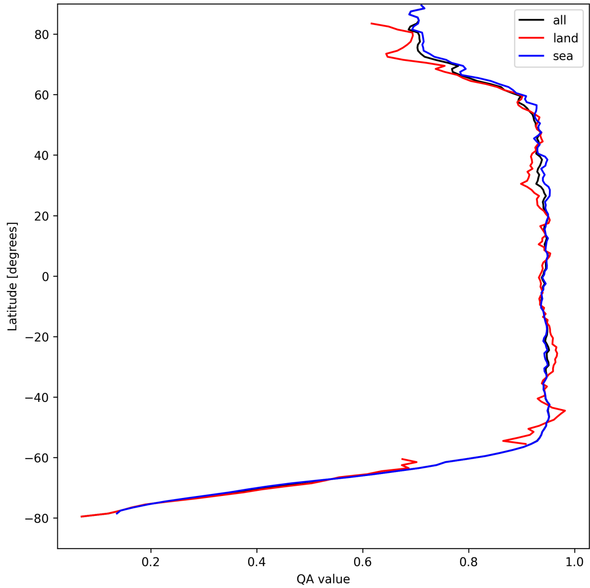
Figure 13: Zonal average of “QA value” for 2025-04-13 to 2025-04-15.
