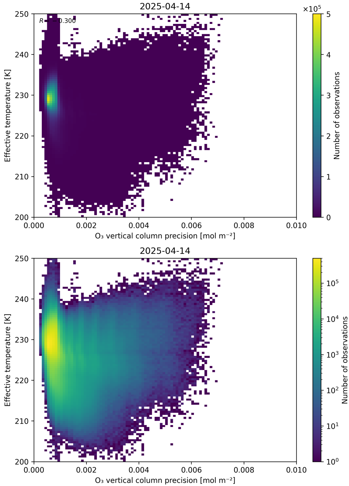
Figure 42: Scatter density plot of “ O_3 vertical column precision” against “Effective temperature” for 2025-04-13 to 2025-04-15.
