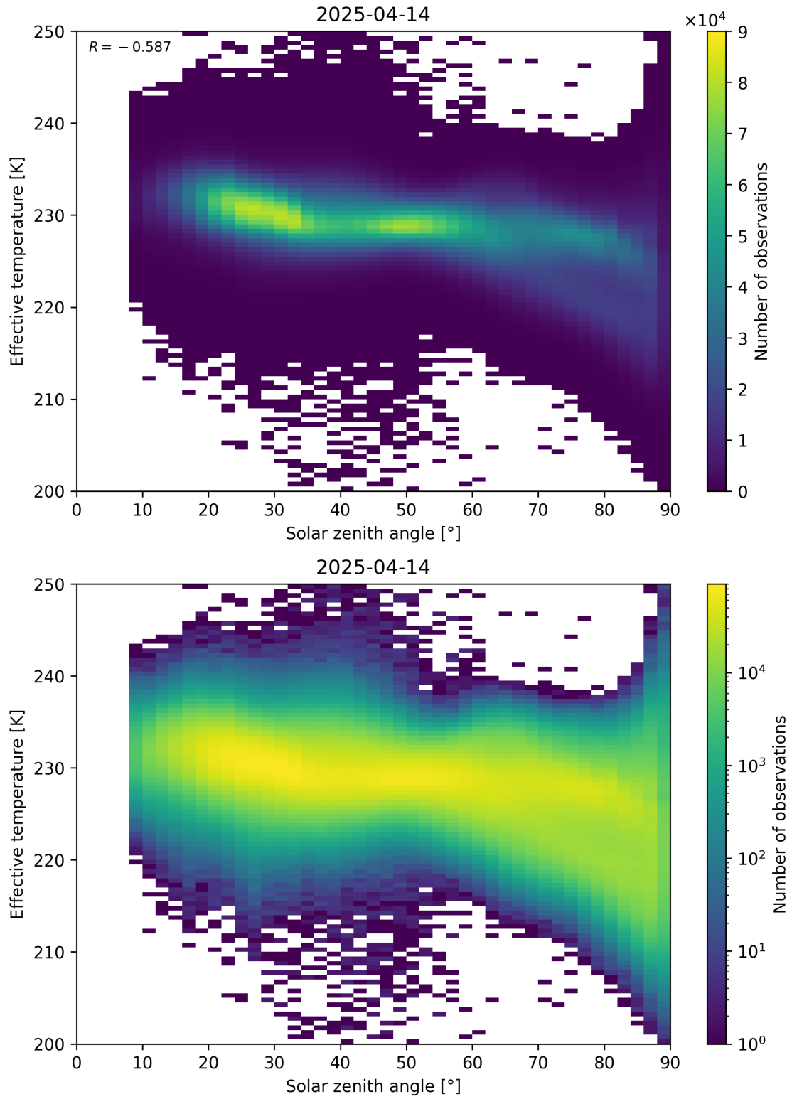
Figure 45: Scatter density plot of “Solar zenith angle” against “Effective temperature” for 2025-04-13 to 2025-04-15.
