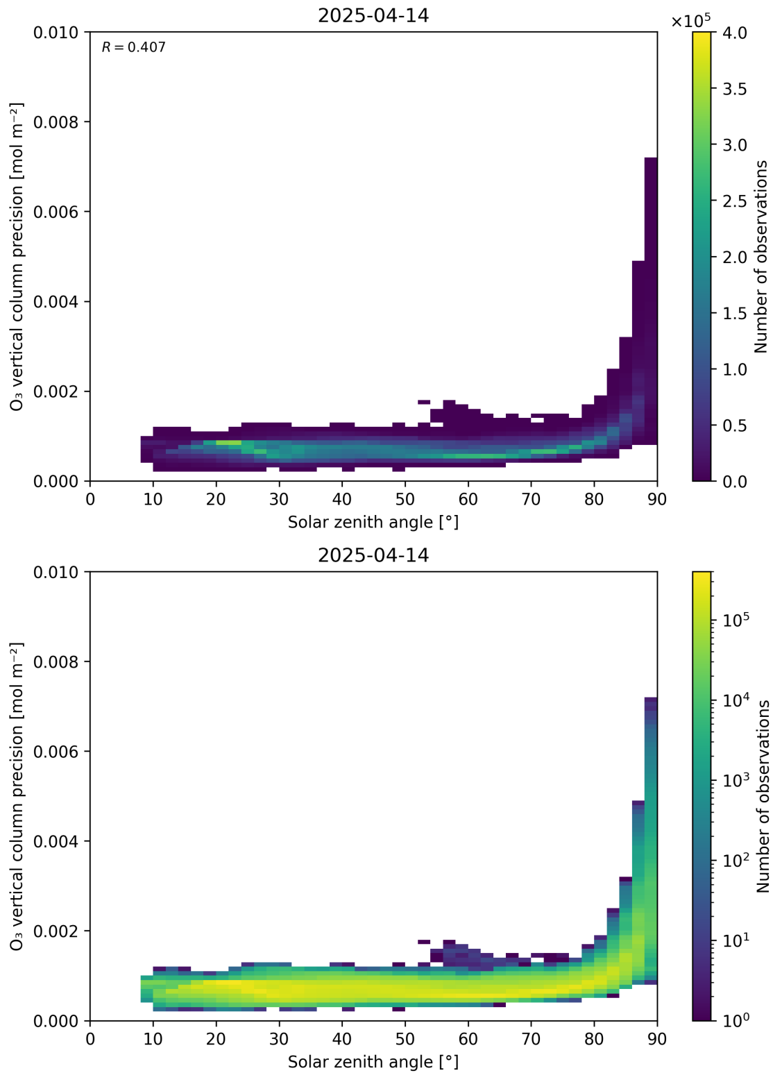
Figure 48: Scatter density plot of “Solar zenith angle” against “O 3 vertical column precision” for 2025-04-13 to 2025-04-15.
