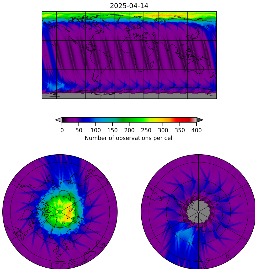
Figure 12: Map of the number of observations for 2025-04-13 to 2025-04-15
