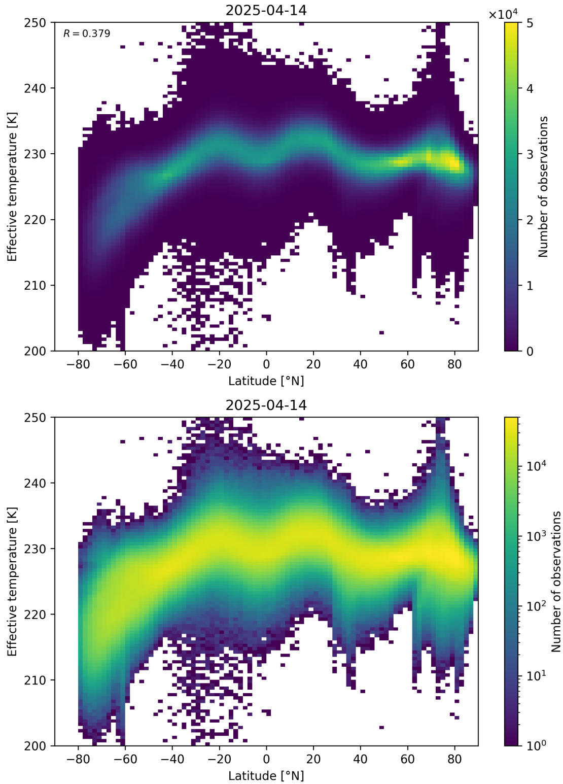
Figure 34: Scatter density plot of “Latitude” against “Effective temperature” for 2025-04-13 to 2025-04-15.
