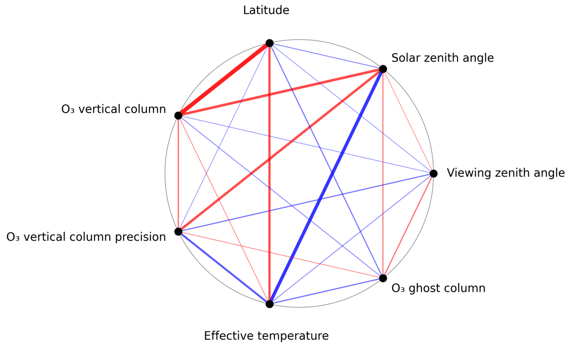
Figure 1: Map of correlation graph for 2025-04-13 to 2025-04-15.
