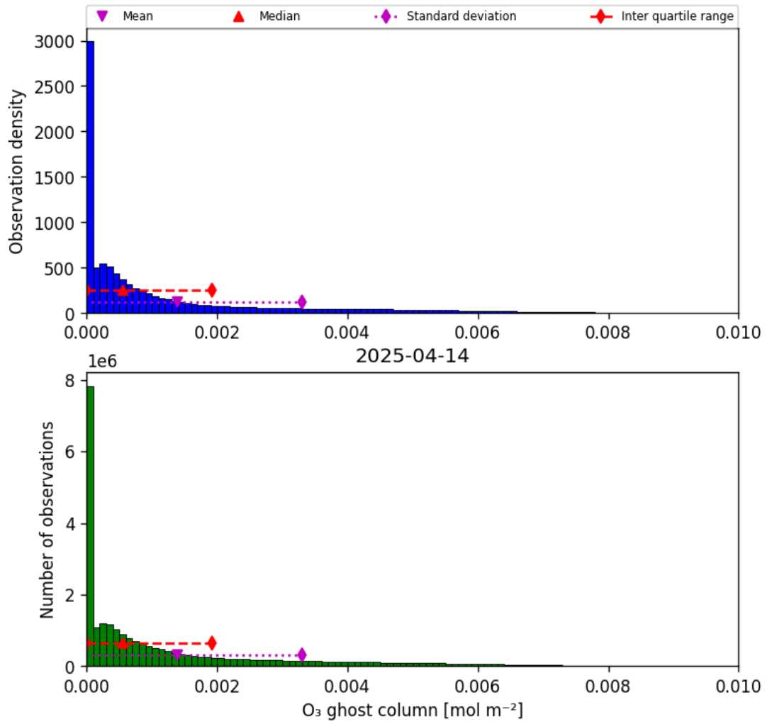
Figure 25: Histogram of “O 3 ghost column” for 2025-04-13 to 2025-04-15
