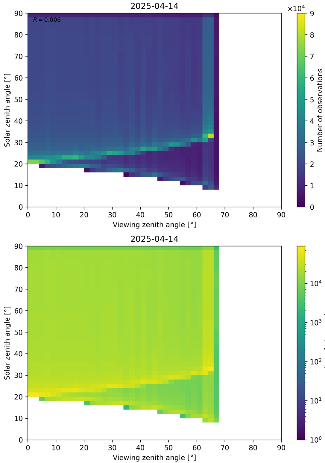
Figure 54: Scatter density plot of “Viewing zenith angle” against “Solar zenith angle” for 2025-04-13 to 2025-04-15.
