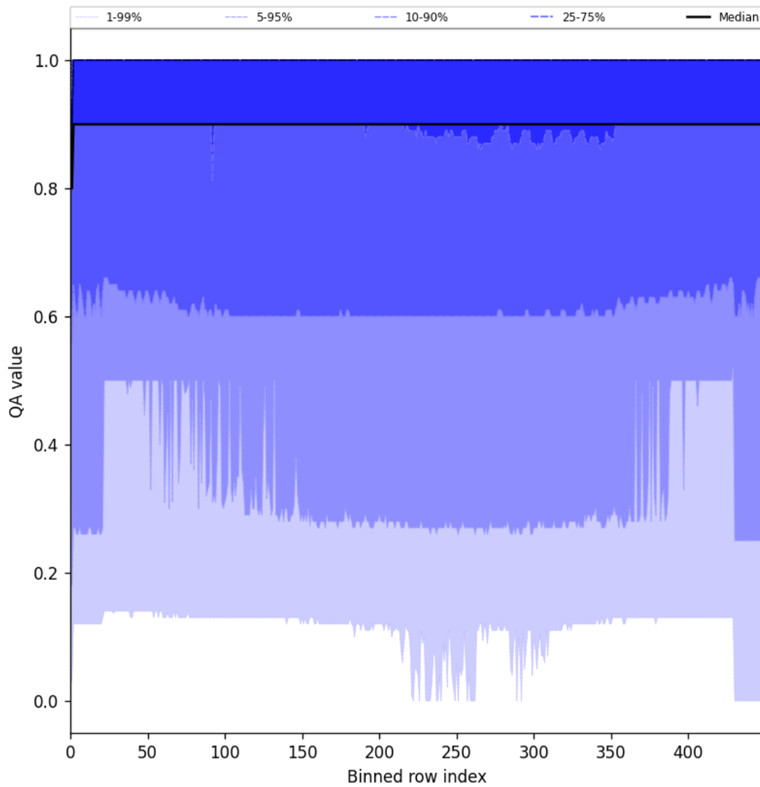
Figure 27: Along track statistics of “QA value” for 2025-04-14 to 2025-04-16
