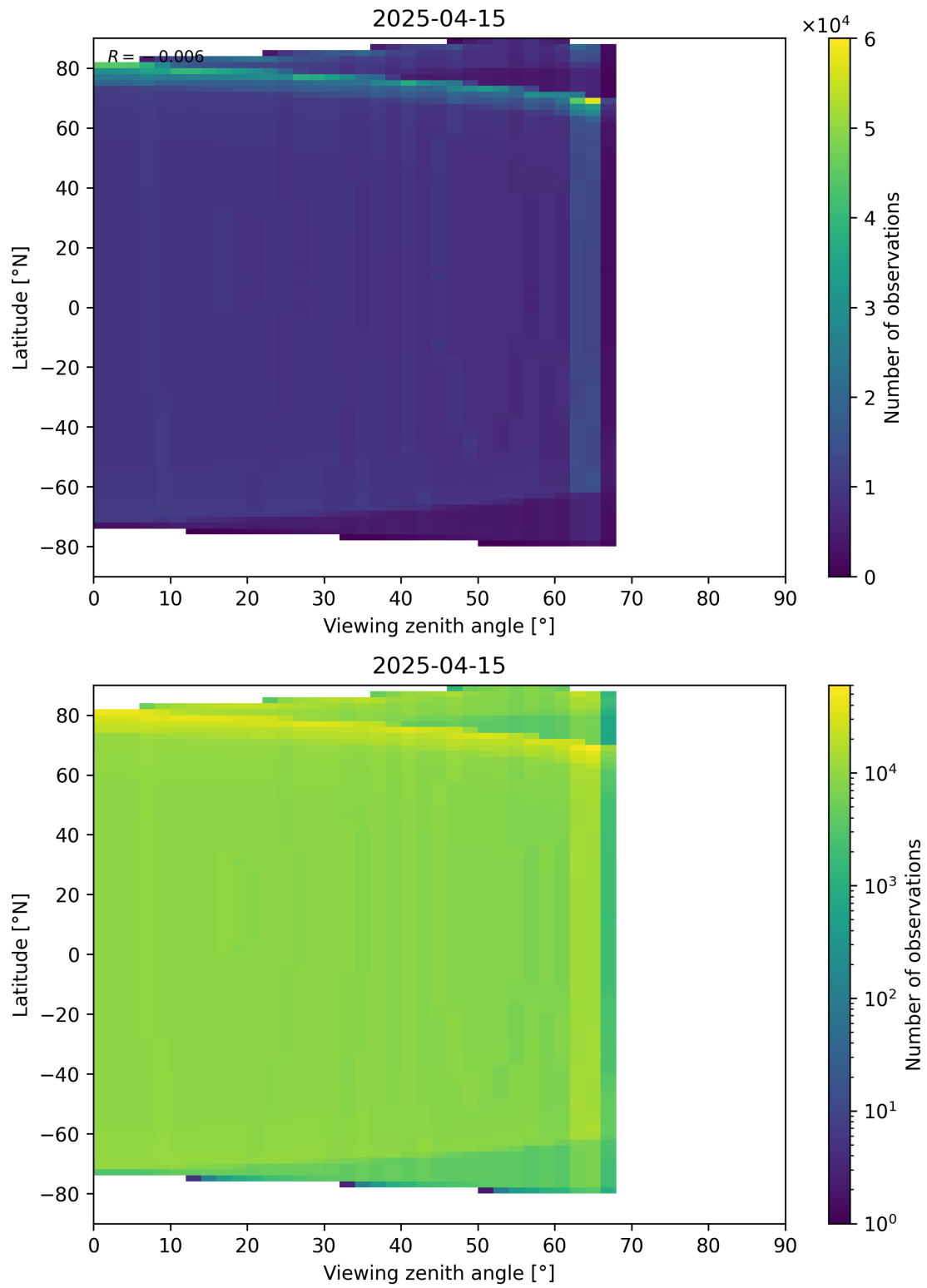
Figure 49: Scatter density plot of “Viewing zenith angle” against “Latitude” for 2025-04-14 to 2025-04-16.
