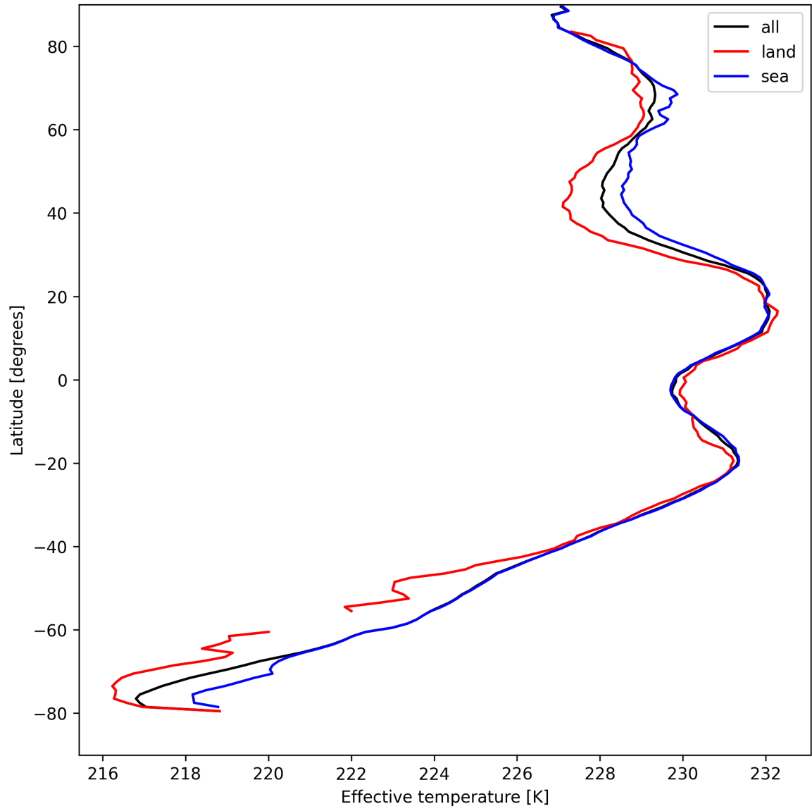
Figure 17: Zonal average of "Effective temperature" for 2025-04-14 to 2025-04-16.
