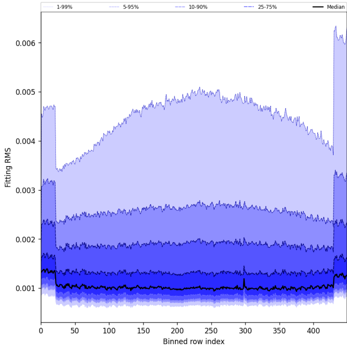
Figure 30: Along track statistics of “Fitting RMS” for 2025-04-14 to 2025-04-16
