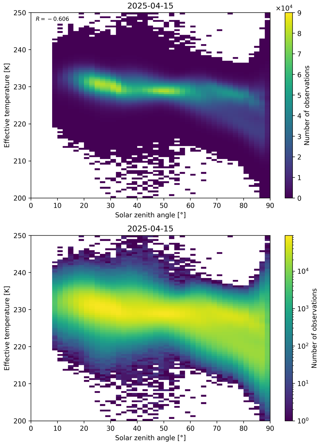
Figure 45: Scatter density plot of “Solar zenith angle” against “Effective temperature” for 2025-04-14 to 2025-04-16.
