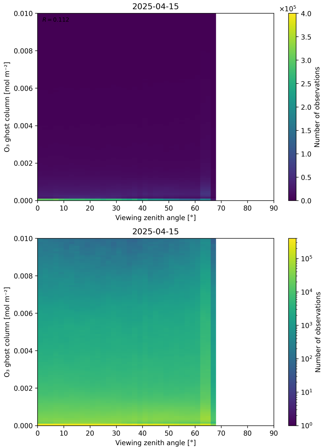
Figure 51: Scatter density plot of “Viewing zenith angle” against “O 3 ghost column” for 2025-04-14 to 2025-04-16.
