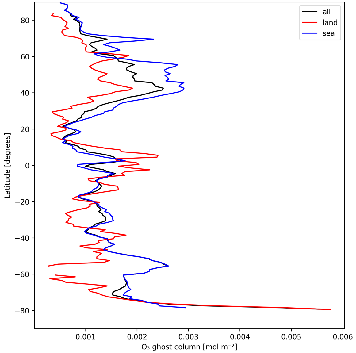
Figure 18: Zonal average of “O 3 ghost column” for 2025-04-14 to 2025-04-16.
