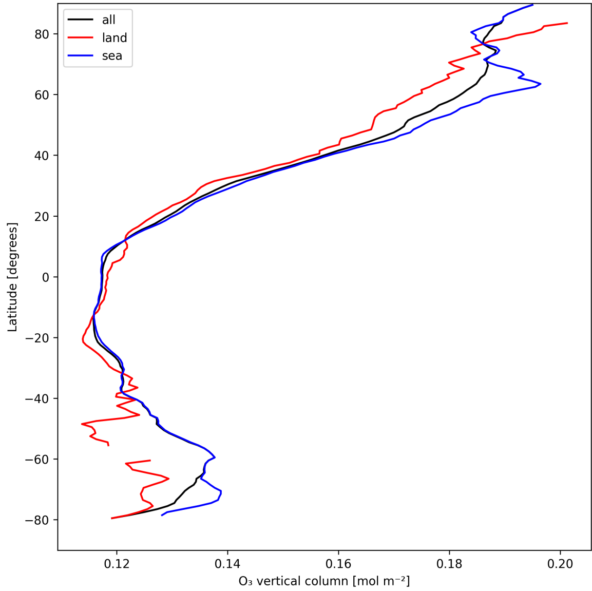
Figure 14: Zonal average of “O 3 vertical column” for 2025-04-14 to 2025-04-16.
