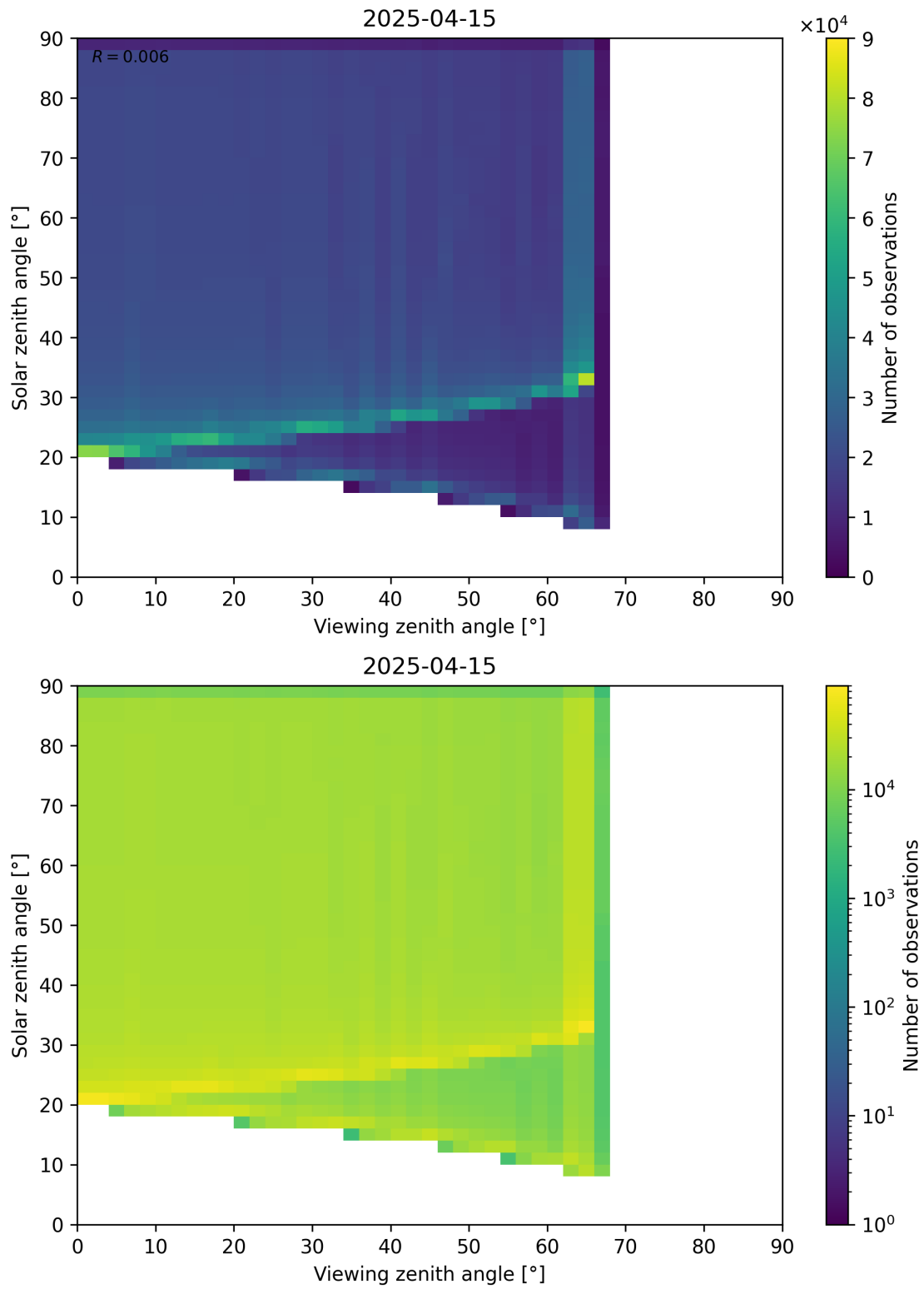
Figure 54: Scatter density plot of “Viewing zenith angle” against “Solar zenith angle” for 2025-04-14 to 2025-04-16.
