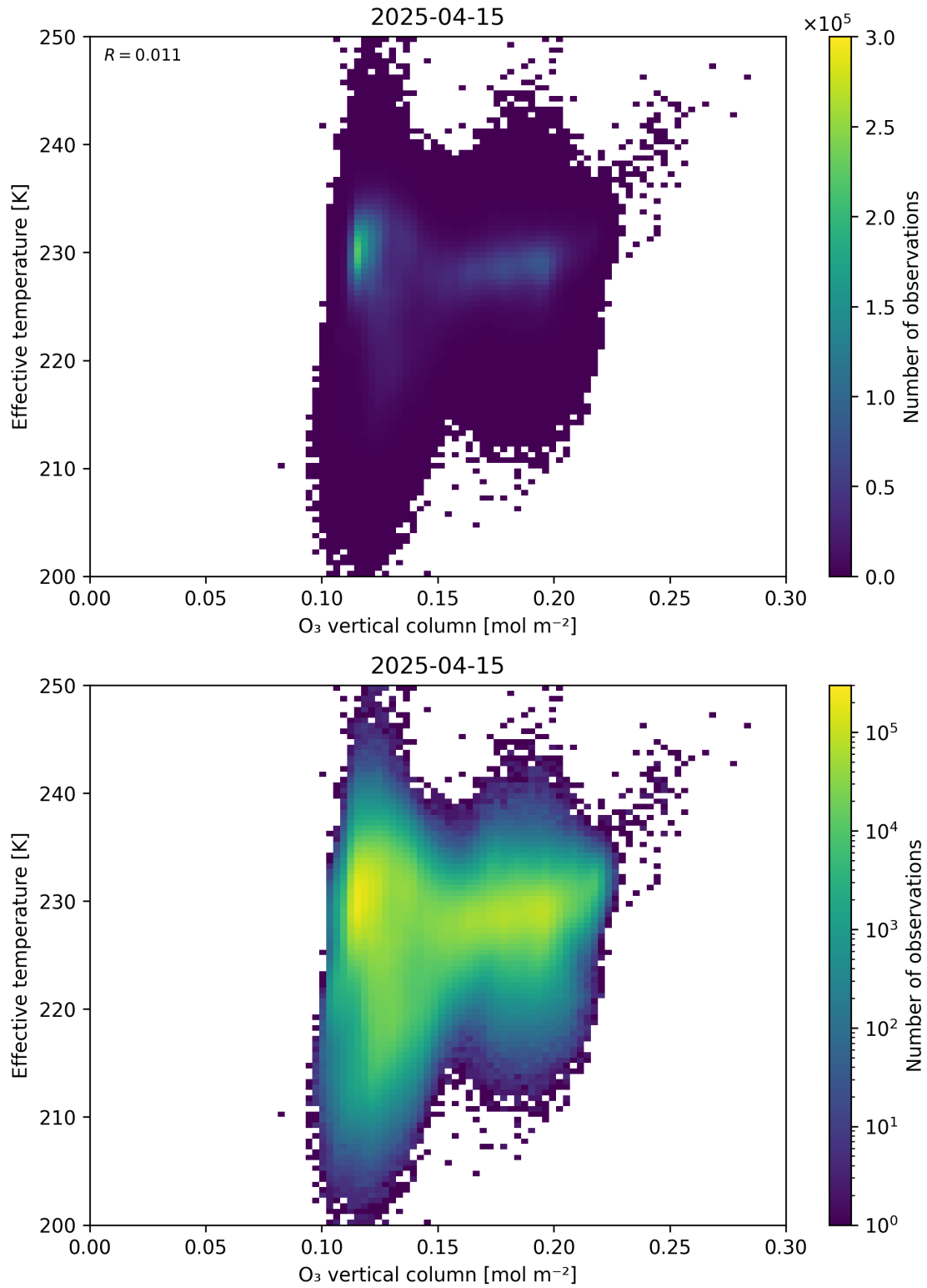
Figure 39: Scatter density plot of “O 3 vertical column” against “Effective temperature” for 2025-04-14 to 2025-04-16.
