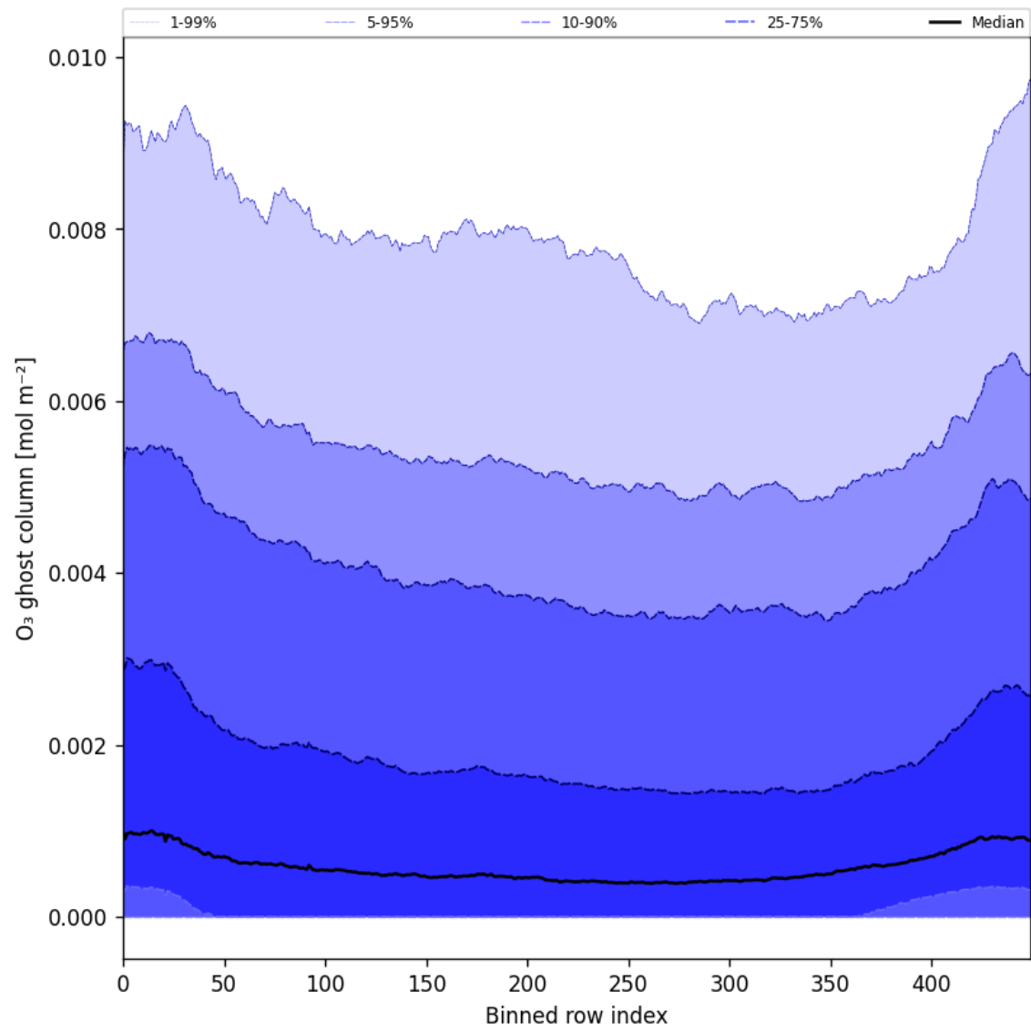
Figure 32: Along track statistics of “O 3 ghost column” for 2025-04-14 to 2025-04-16
