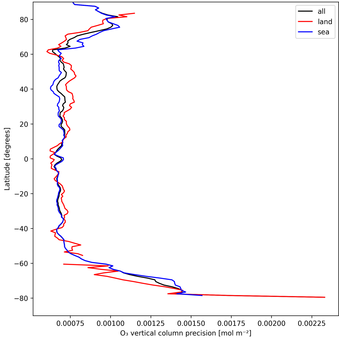
Figure 15: Zonal average of "O 3 vertical column precision" for 2025-04-14 to 2025-04-16.
