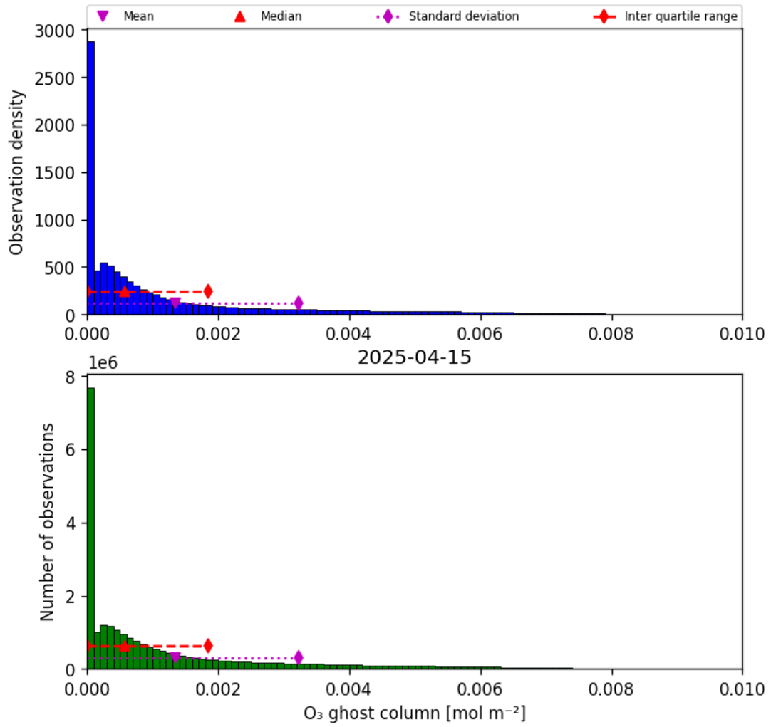
Figure 25: Histogram of “O 3 ghost column” for 2025-04-14 to 2025-04-16
