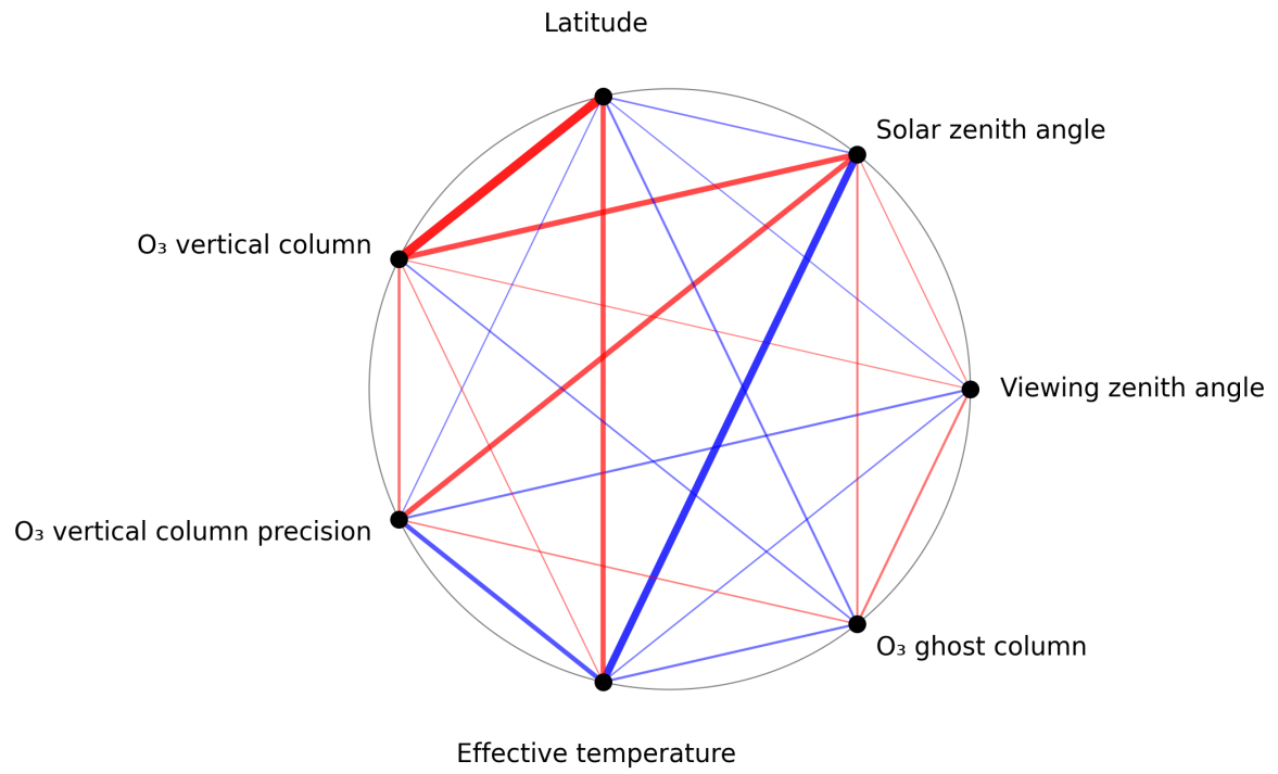
Figure 1: Map of correlation graph for 2025-04-14 to 2025-04-16.
