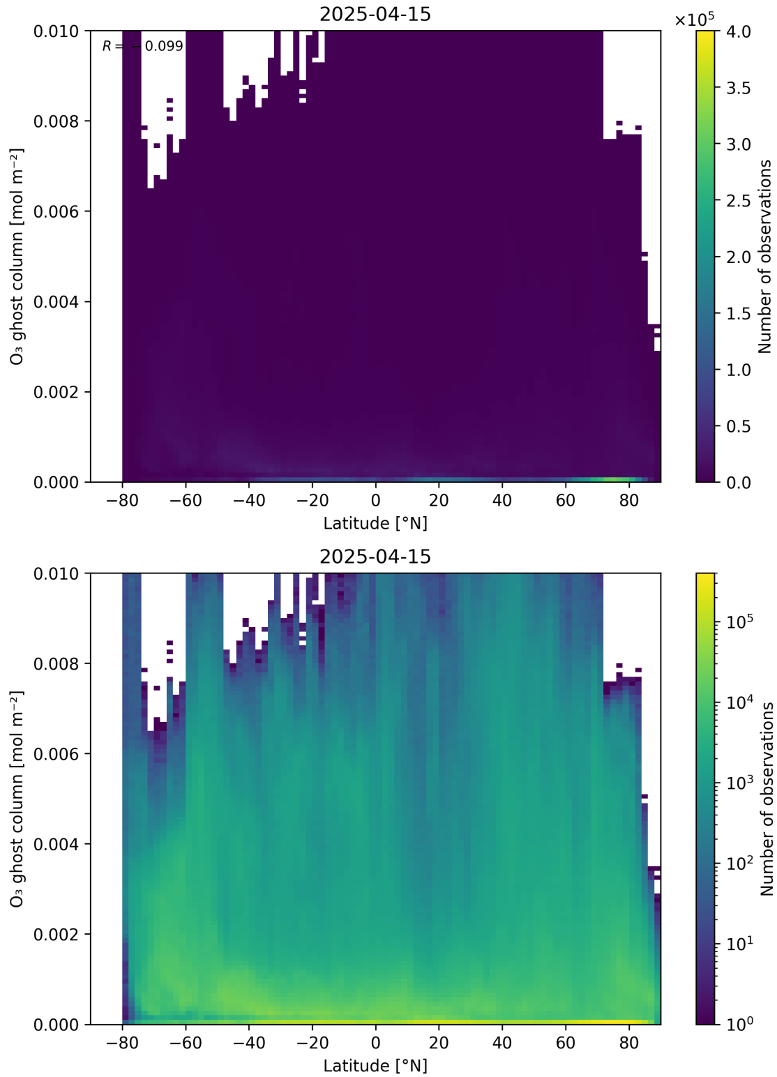
Figure 35: Scatter density plot of “Latitude” against “O 3 ghost column” for 2025-04-14 to 2025-04-16.
