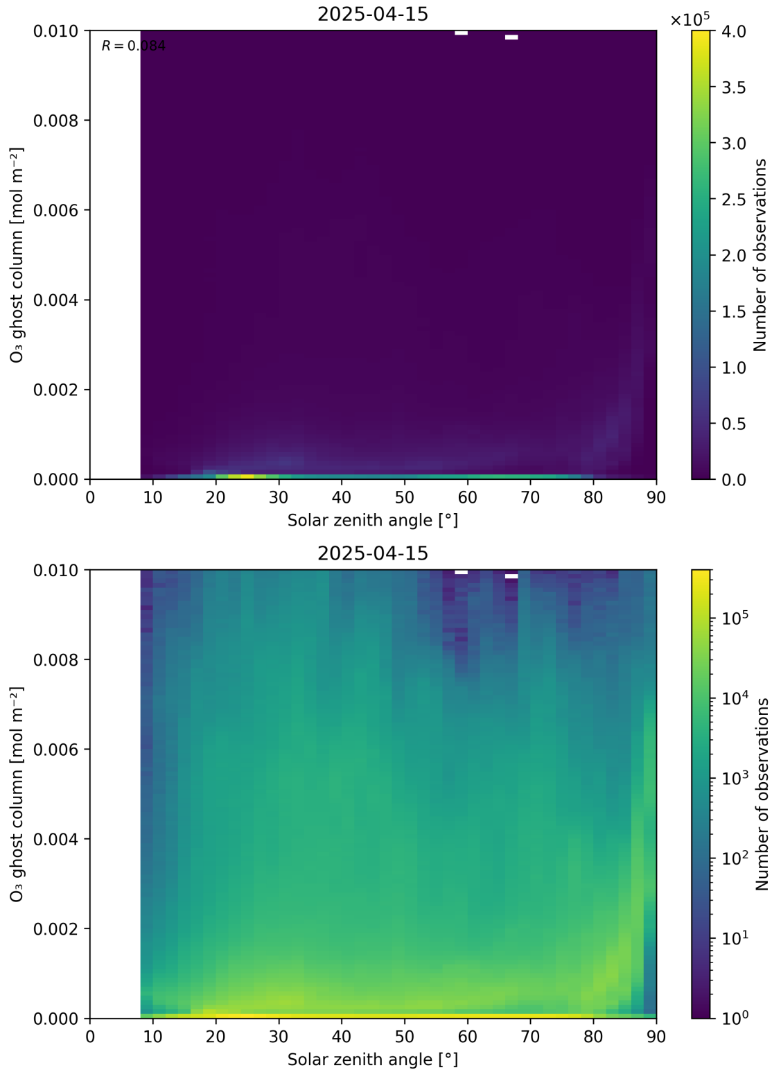
Figure 46: Scatter density plot of “Solar zenith angle” against “O 3 ghost column” for 2025-04-14 to 2025-04-16.
