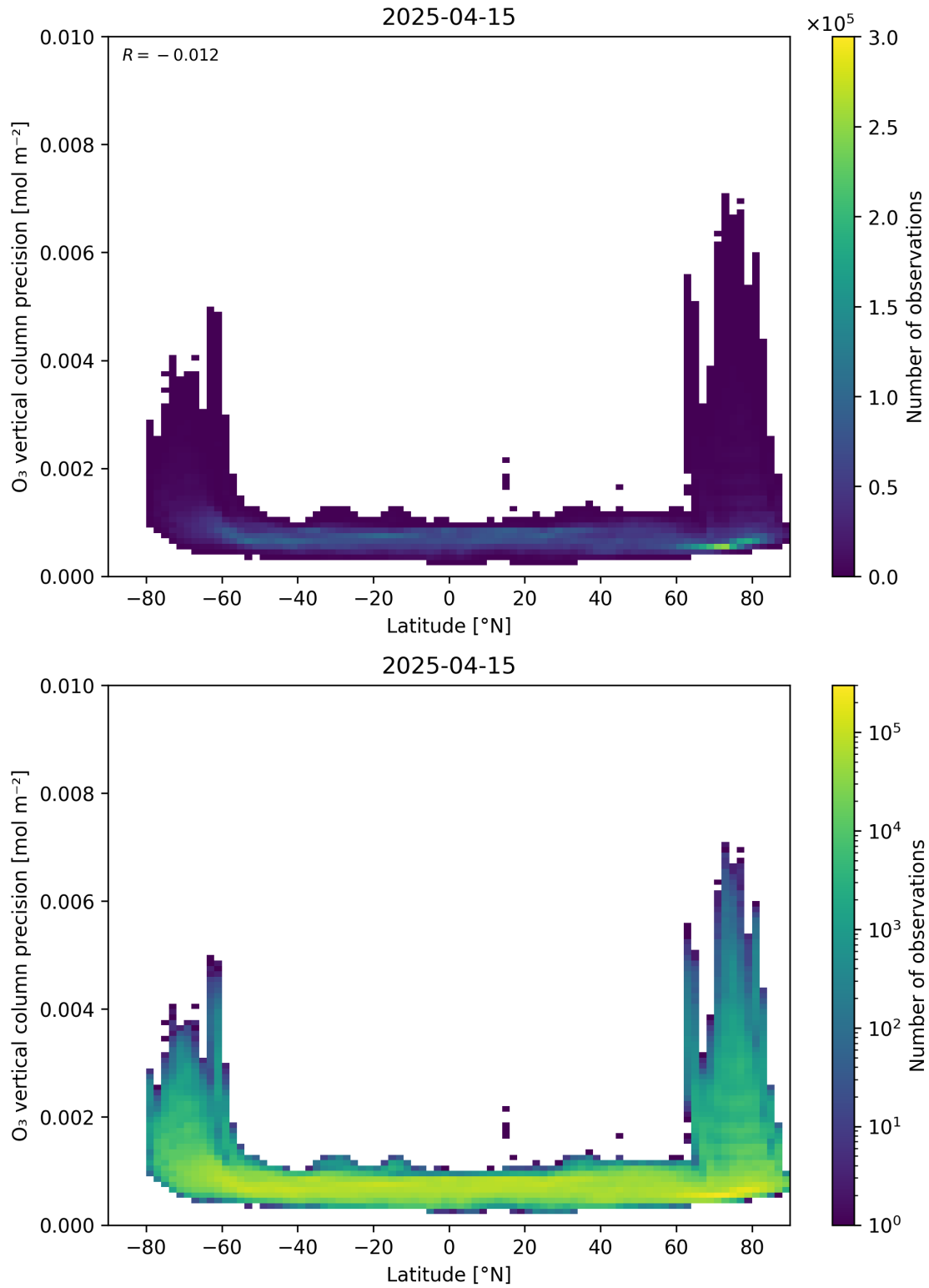
Figure 37: Scatter density plot of “Latitude” against “O 3 vertical column precision” for 2025-04-14 to 2025-04-16.
