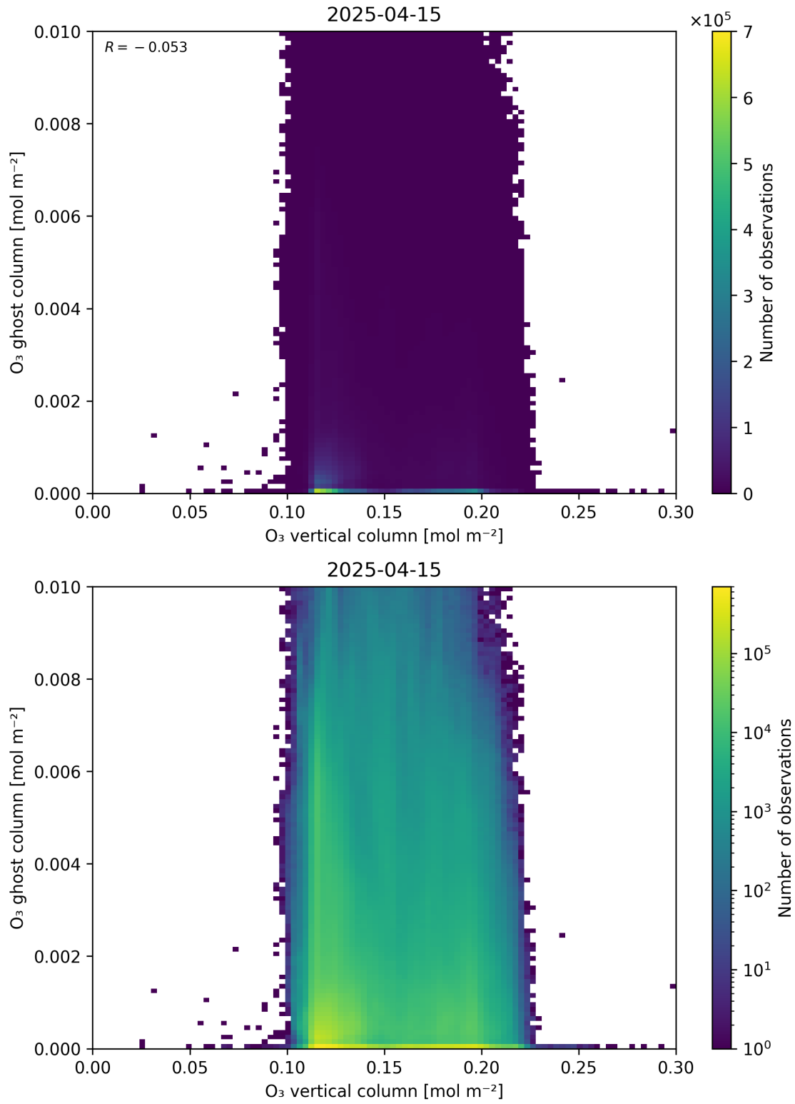
Figure 40: Scatter density plot of “O 3 vertical column” against “O 3 ghost column” for 2025-04-14 to 2025-04-16.
