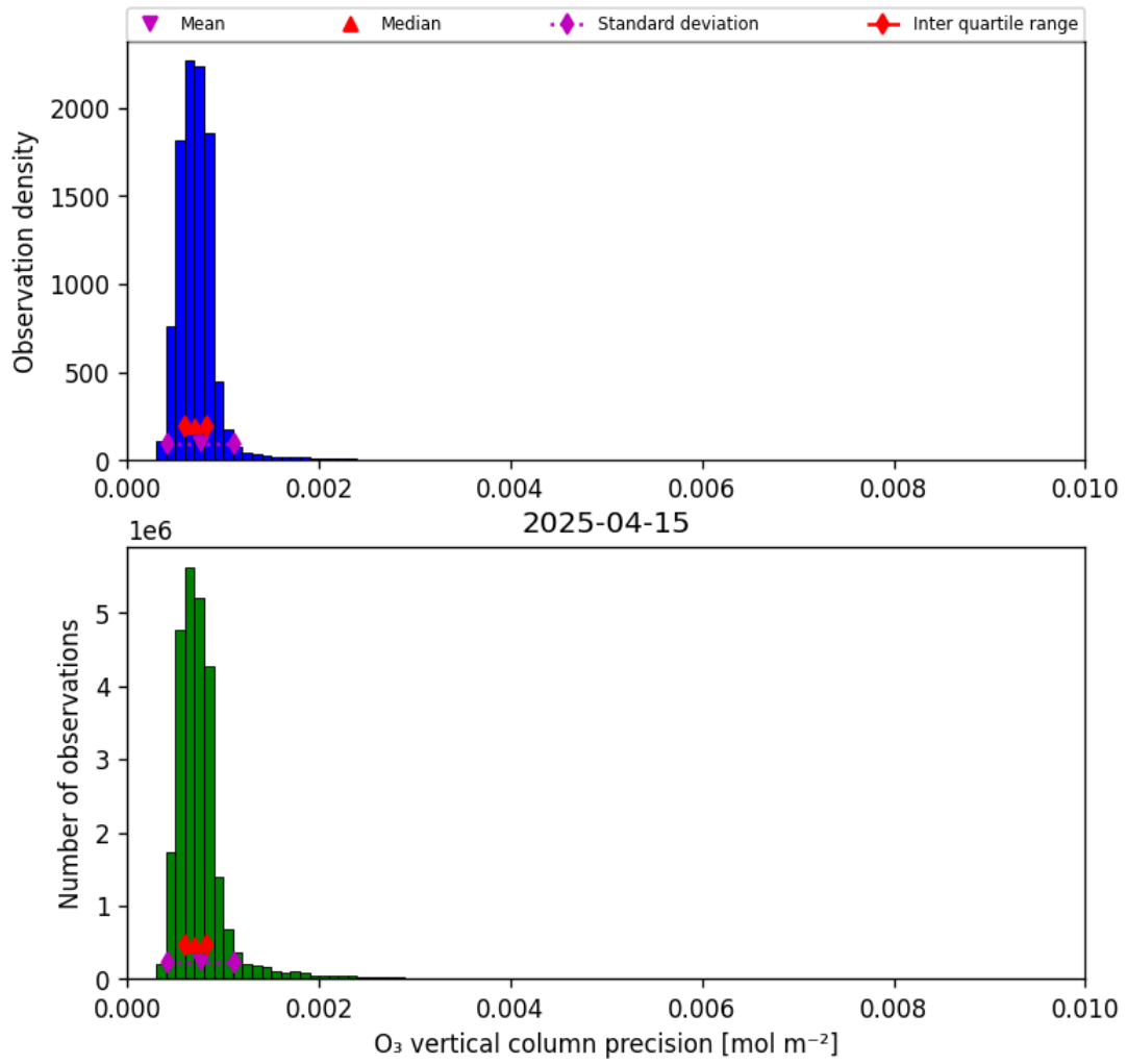
Figure 22: Histogram of “O 3 vertical column precision” for 2025-04-14 to 2025-04-16
