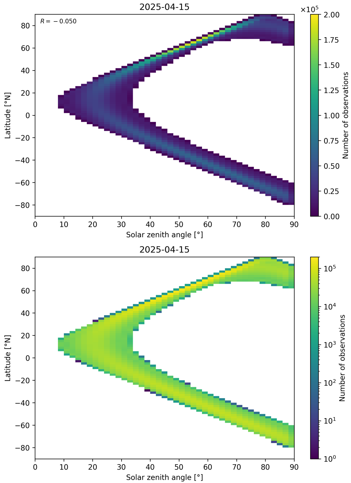
Figure 44: Scatter density plot of “Solar zenith angle” against “Latitude” for 2025-04-14 to 2025-04-16.
