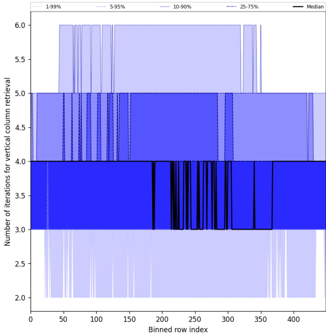
Figure 33: Along track statistics of “Number of iterations for vertical column retrieval” for 2025-04-14 to 2025-04-16
