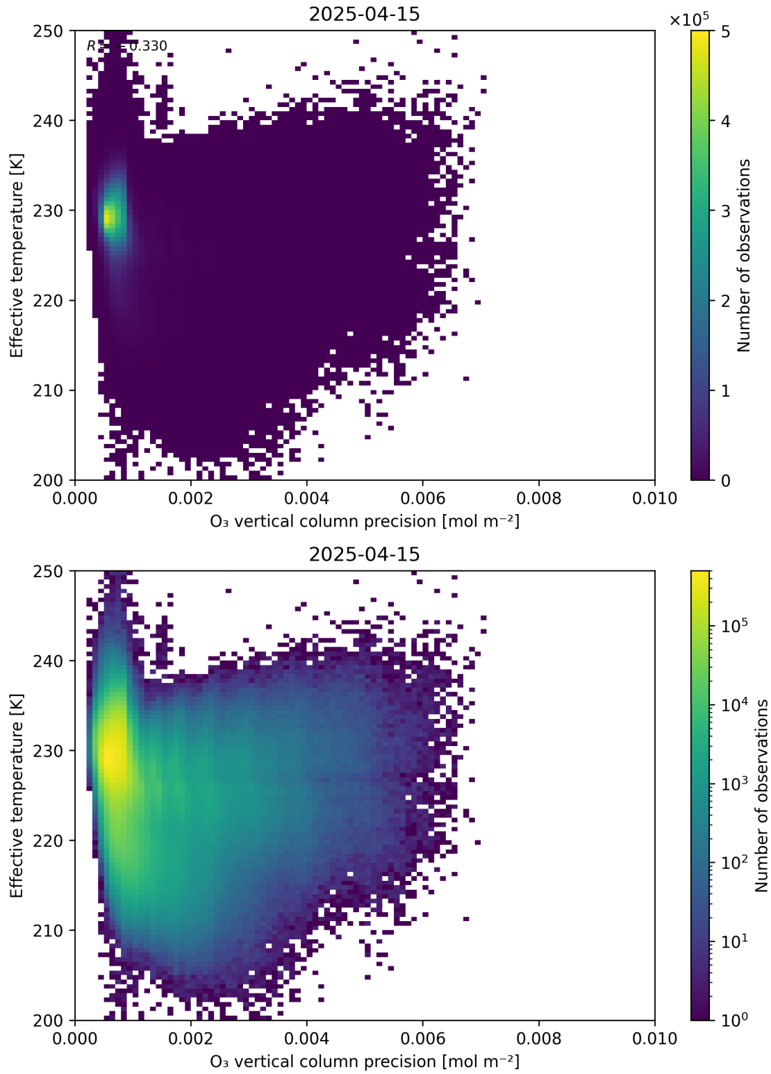
Figure 42: Scatter density plot of “O 3 vertical column precision” against “Effective temperature” for 2025-04-14 to 2025-04-16.
