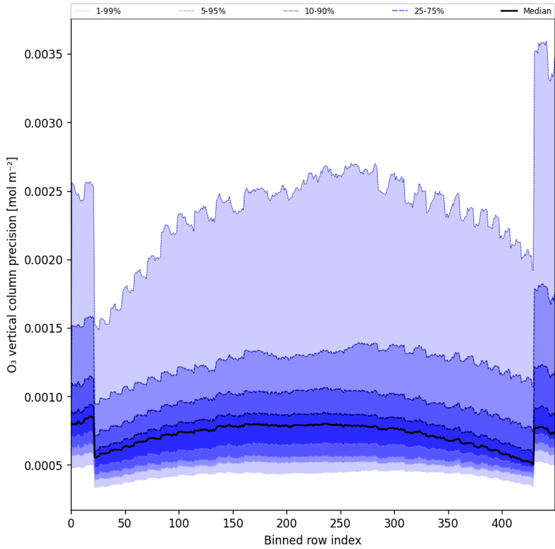
Figure 29: Along track statistics of “O 3 vertical column precision” for 2025-04-14 to 2025-04-16
