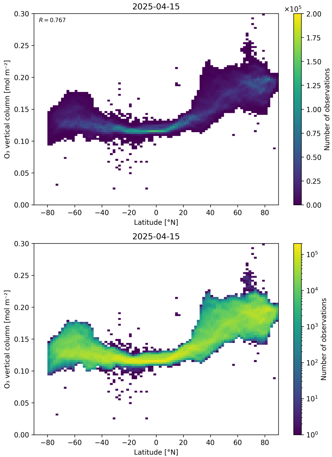
Figure 36: Scatter density plot of “Latitude” against “O 3 vertical column” for 2025-04-14 to 2025-04-16.
