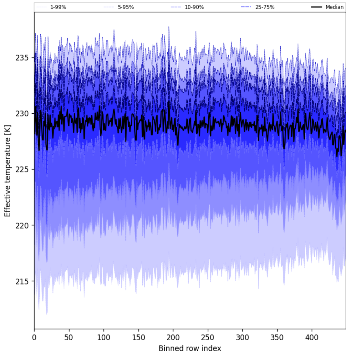
Figure 31: Along track statistics of “Effective temperature” for 2025-04-14 to 2025-04-16
