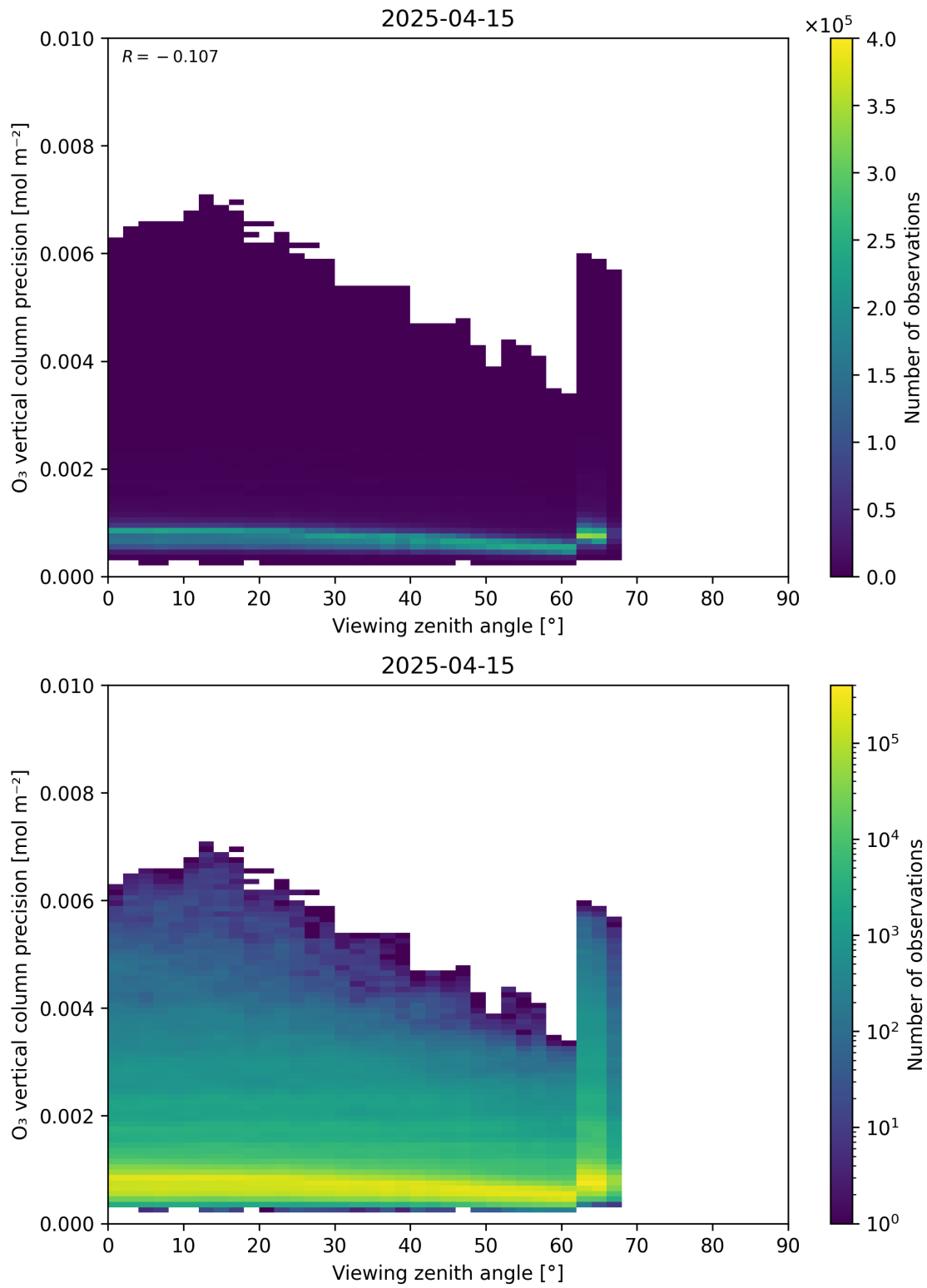
Figure 53: Scatter density plot of “Viewing zenith angle” against “O 3 vertical column precision” for 2025-04-14 to 2025-04-16.
