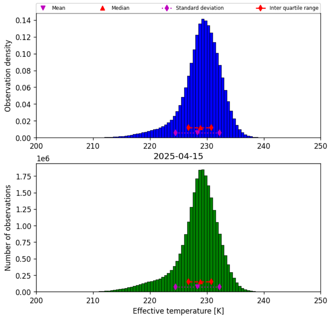
Figure 24: Histogram of “Effective temperature” for 2025-04-14 to 2025-04-16
