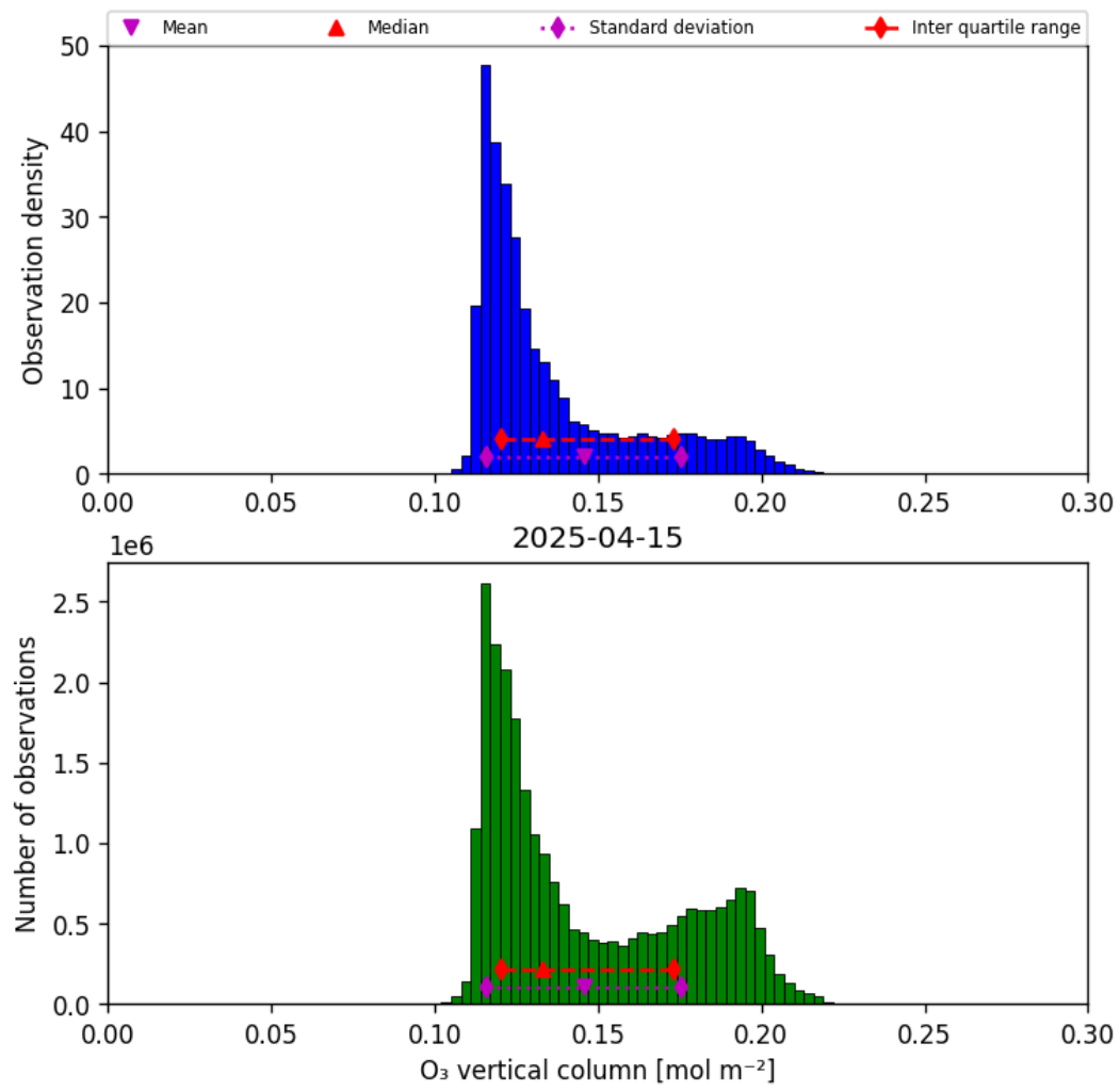
Figure 21: Histogram of “O 3 vertical column” for 2025-04-14 to 2025-04-16
