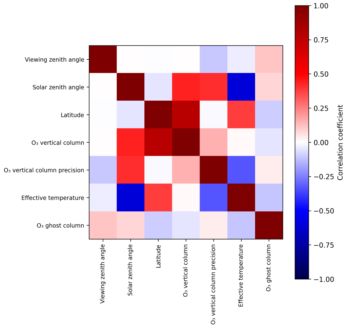
Figure 2: Map of correlation matrix for 2025-04-14 to 2025-04-16.
