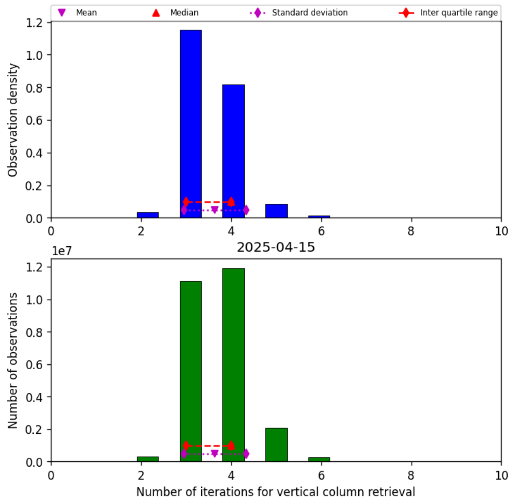
Figure 26: Histogram of “Number of iterations for vertical column retrieval” for 2025-04-14 to 2025-04-16
