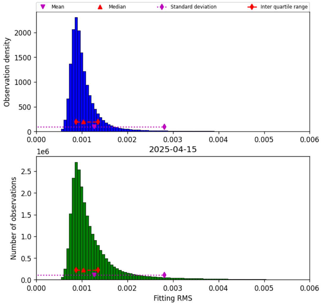
Figure 23: Histogram of “Fitting RMS” for 2025-04-14 to 2025-04-16
