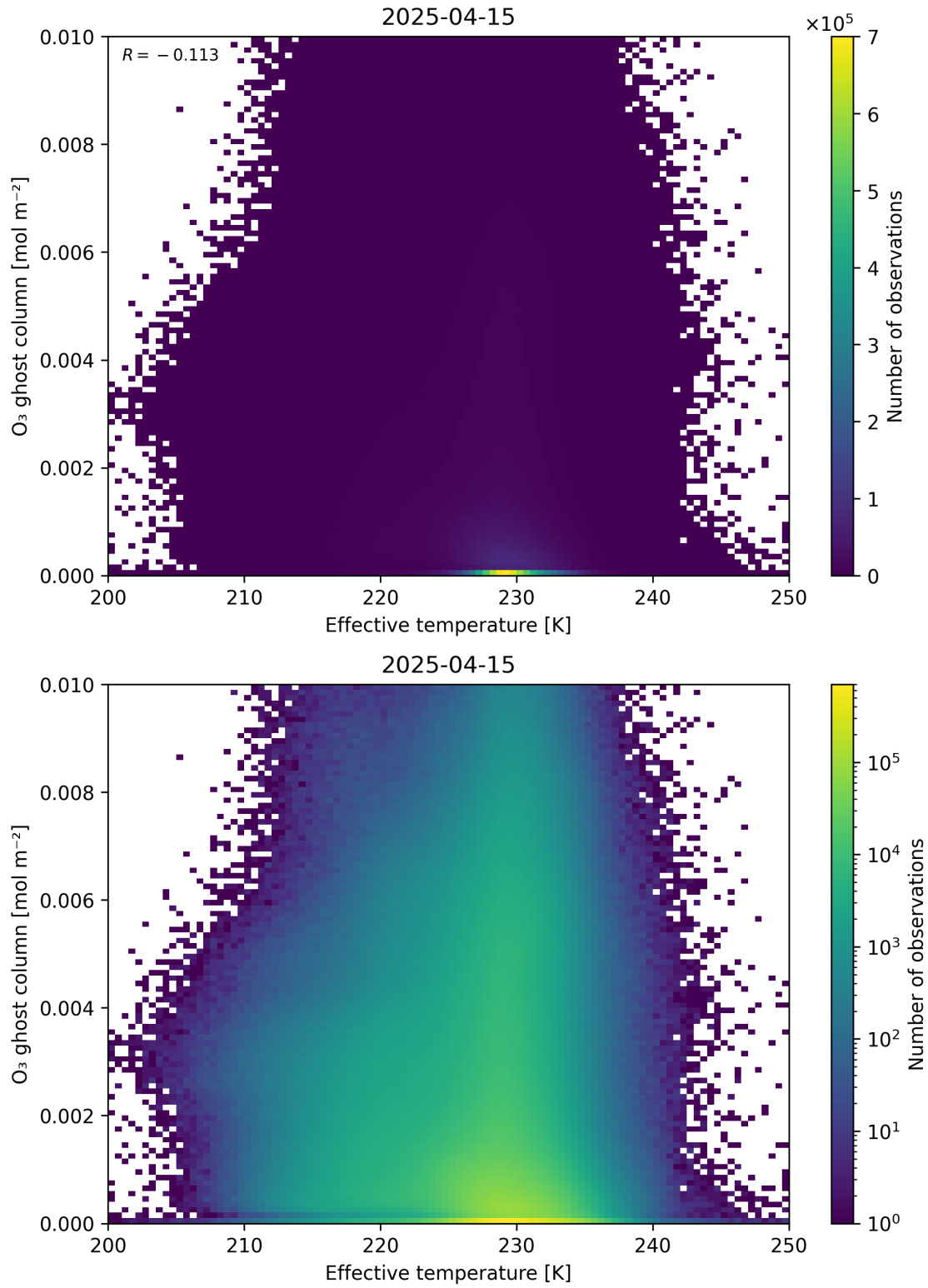
Figure 38: Scatter density plot of “Effective temperature” against “O 3 ghost column” for 2025-04-14 to 2025-04-16.
