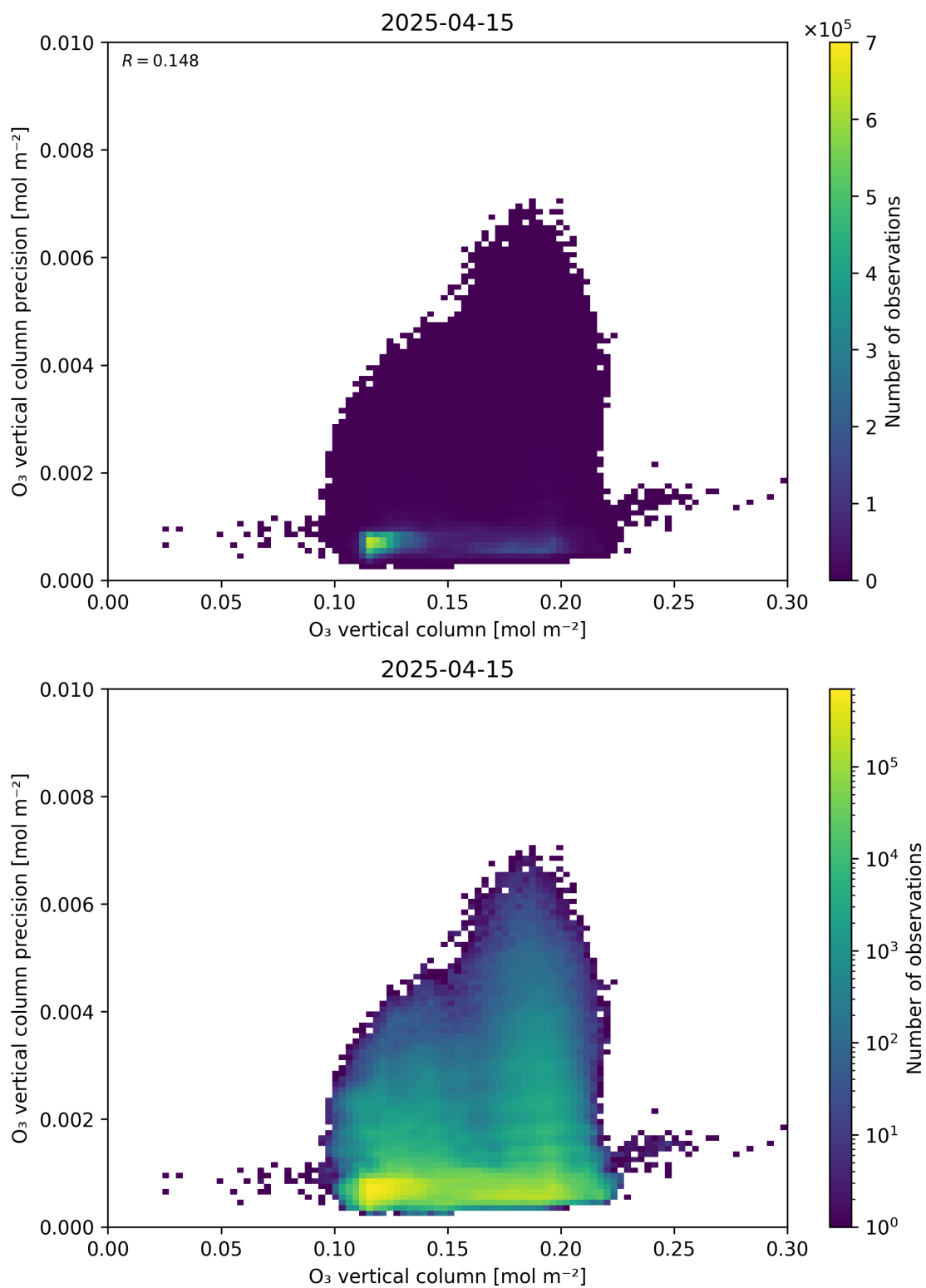
Figure 41: Scatter density plot of “O 3 vertical column” against “O 3 vertical column precision” for 2025-04-14 to 2025-04-16.
