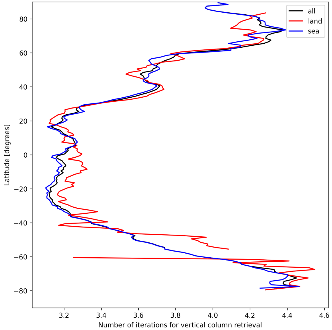
Figure 19: Zonal average of “Number of iterations for vertical column retrieval” for 2025-04-14 to 2025-04-16.
