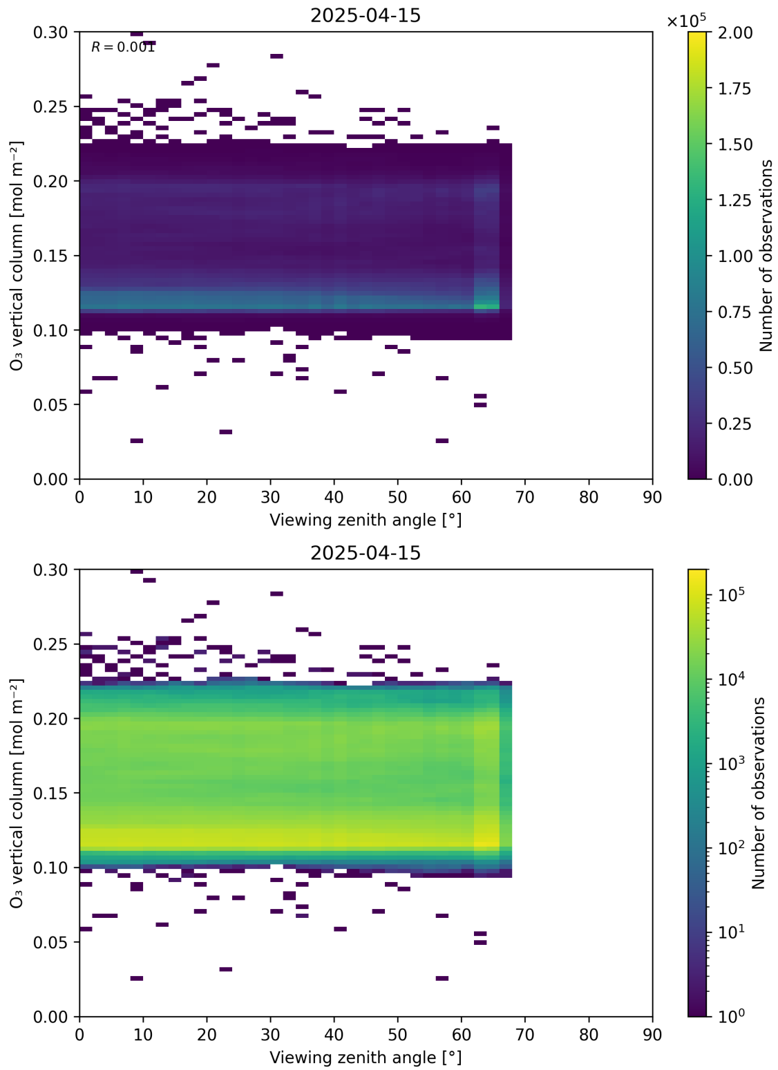
Figure 52: Scatter density plot of “Viewing zenith angle” against “O 3 vertical column” for 2025-04-14 to 2025-04-16.
