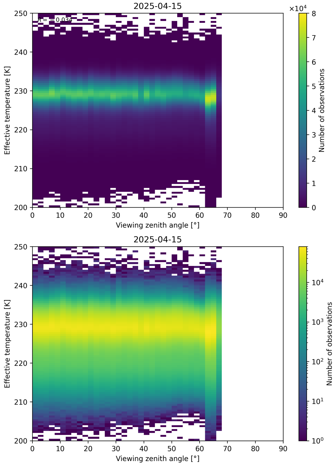
Figure 50: Scatter density plot of “Viewing zenith angle” against “Effective temperature” for 2025-04-14 to 2025-04-16.
