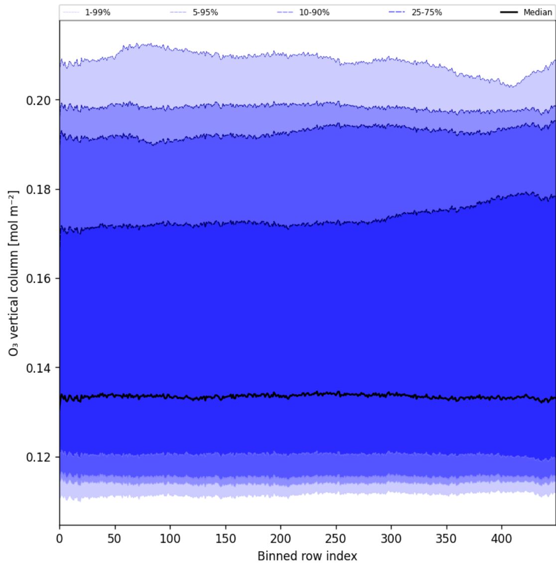
Figure 28: Along track statistics of “O 3 vertical column” for 2025-04-14 to 2025-04-16
