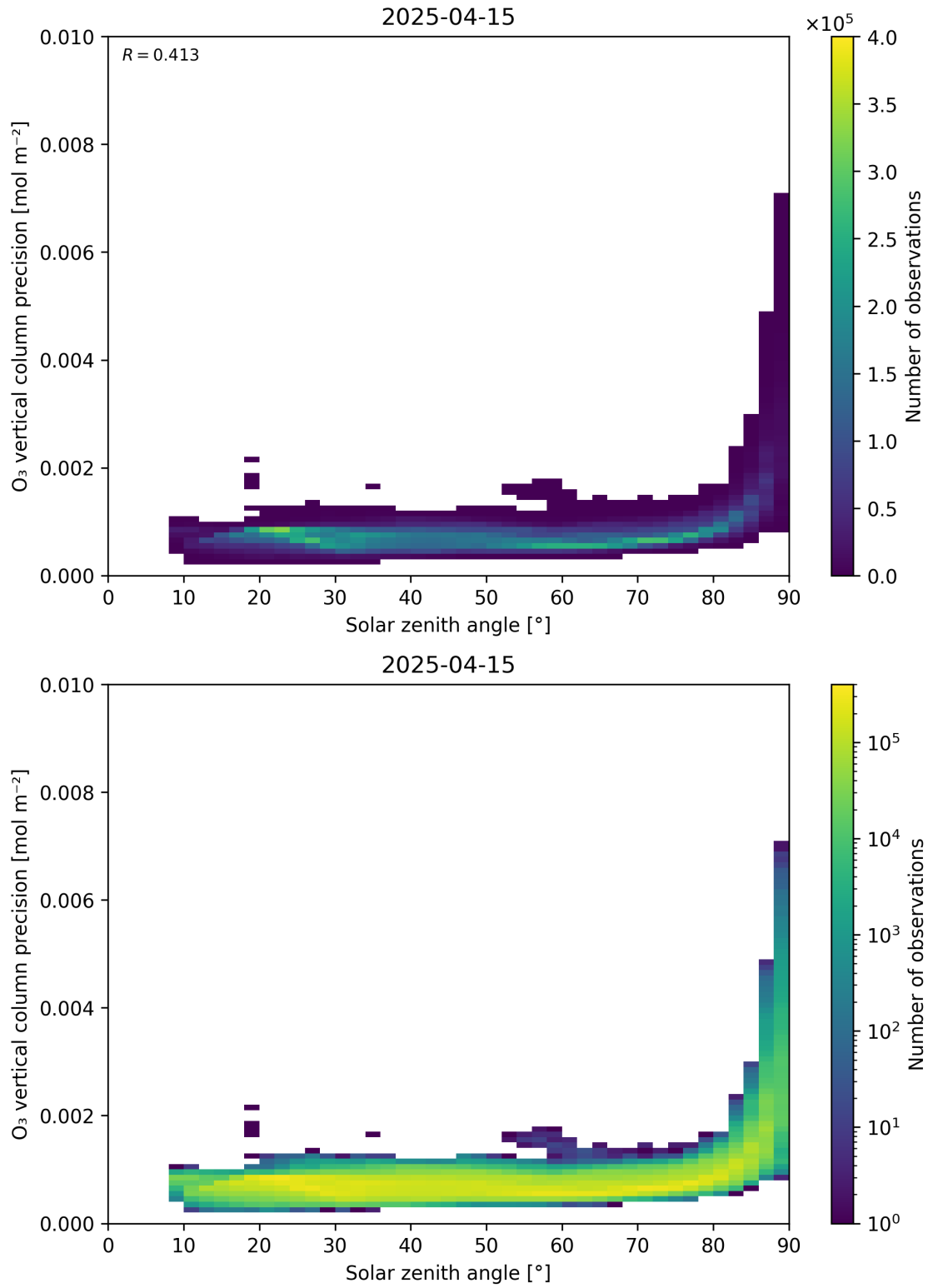
Figure 48: Scatter density plot of “Solar zenith angle” against “O 3 vertical column precision” for 2025-04-14 to 2025-04-16.
