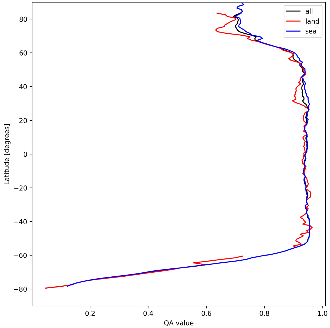
Figure 13: Zonal average of “QA value” for 2025-04-14 to 2025-04-16.
