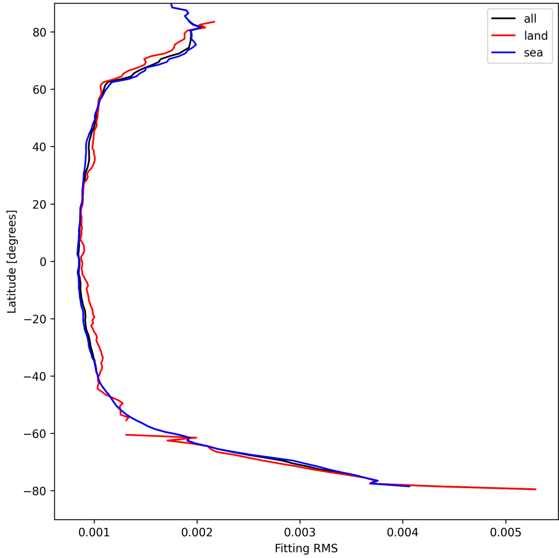
Figure 16: Zonal average of “Fitting RMS” for 2025-04-14 to 2025-04-16.
