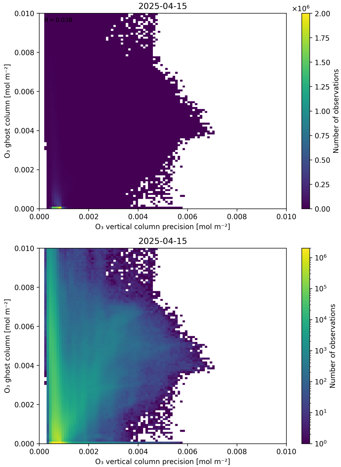
Figure 43: Scatter density plot of “ \text{O}_3 vertical column precision” against “ \text{O}_3 ghost column” for 2025-04-14 to 2025-04-16.
