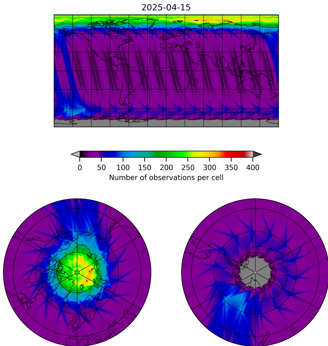
Figure 12: Map of the number of observations for 2025-04-14 to 2025-04-16
