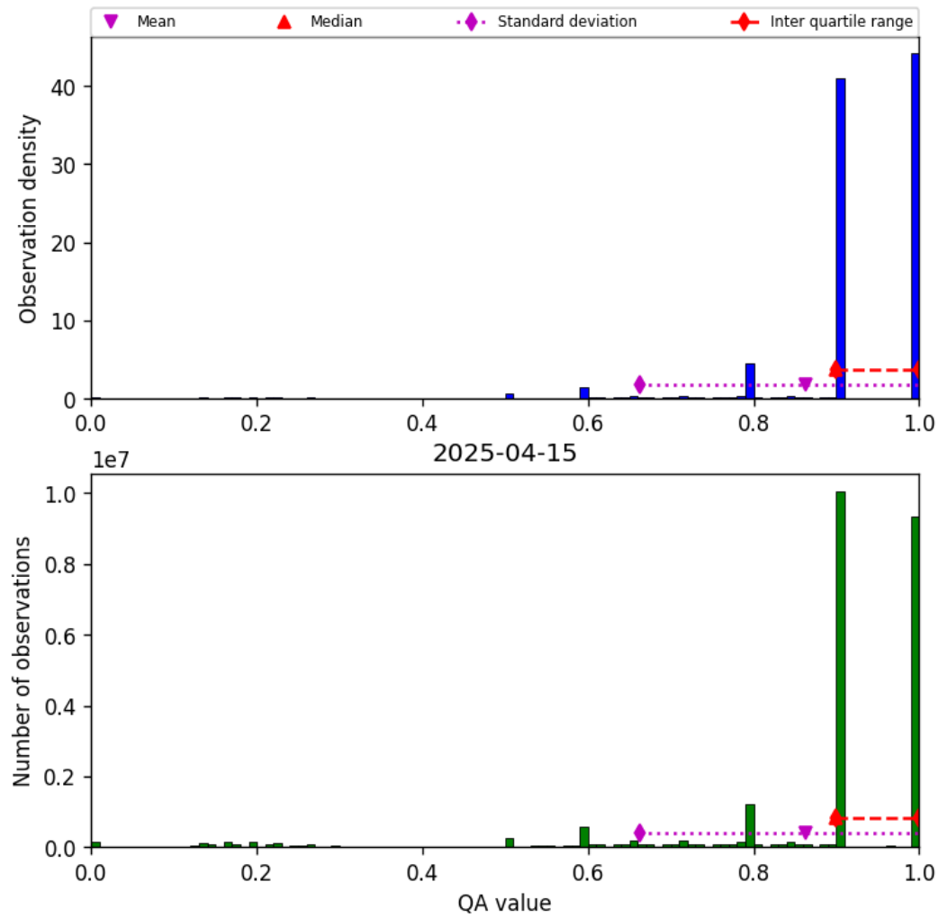
Figure 20: Histogram of “QA value” for 2025-04-14 to 2025-04-16
