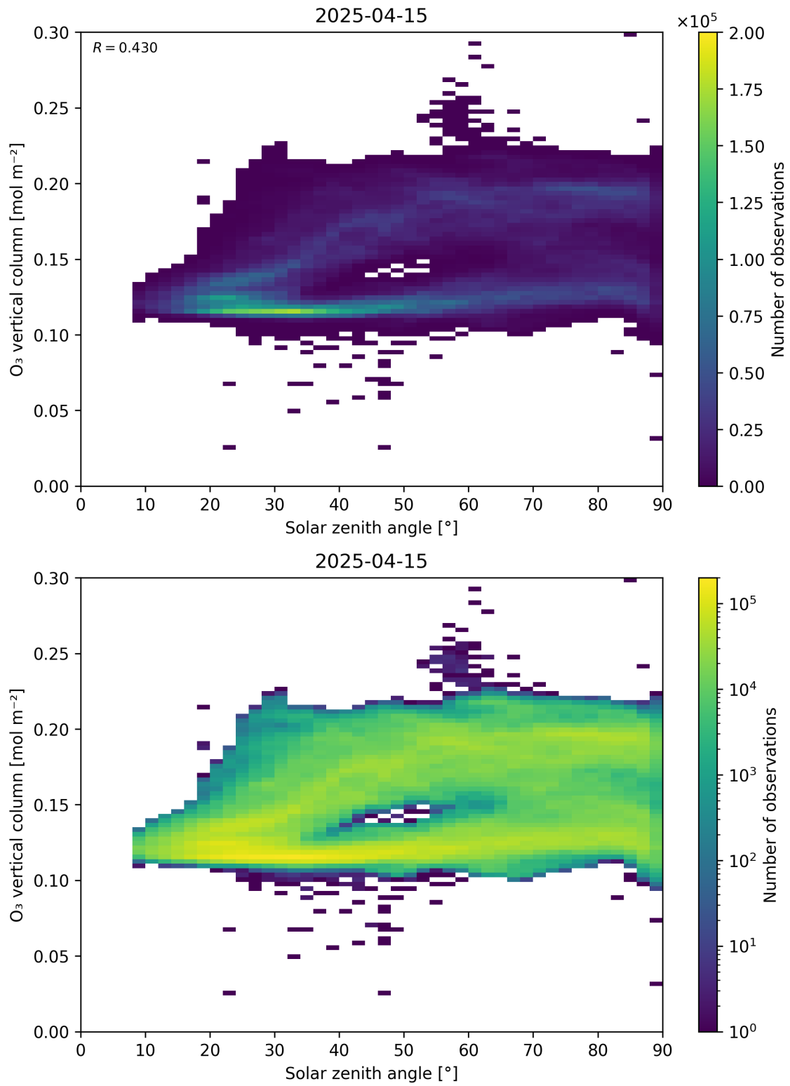
Figure 47: Scatter density plot of “Solar zenith angle” against “O 3 vertical column” for 2025-04-14 to 2025-04-16.
