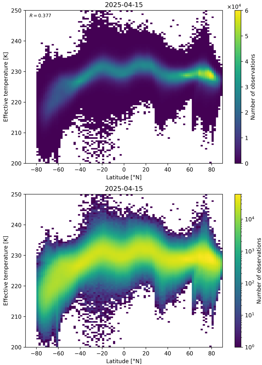
Figure 34: Scatter density plot of “Latitude” against “Effective temperature” for 2025-04-14 to 2025-04-16.
