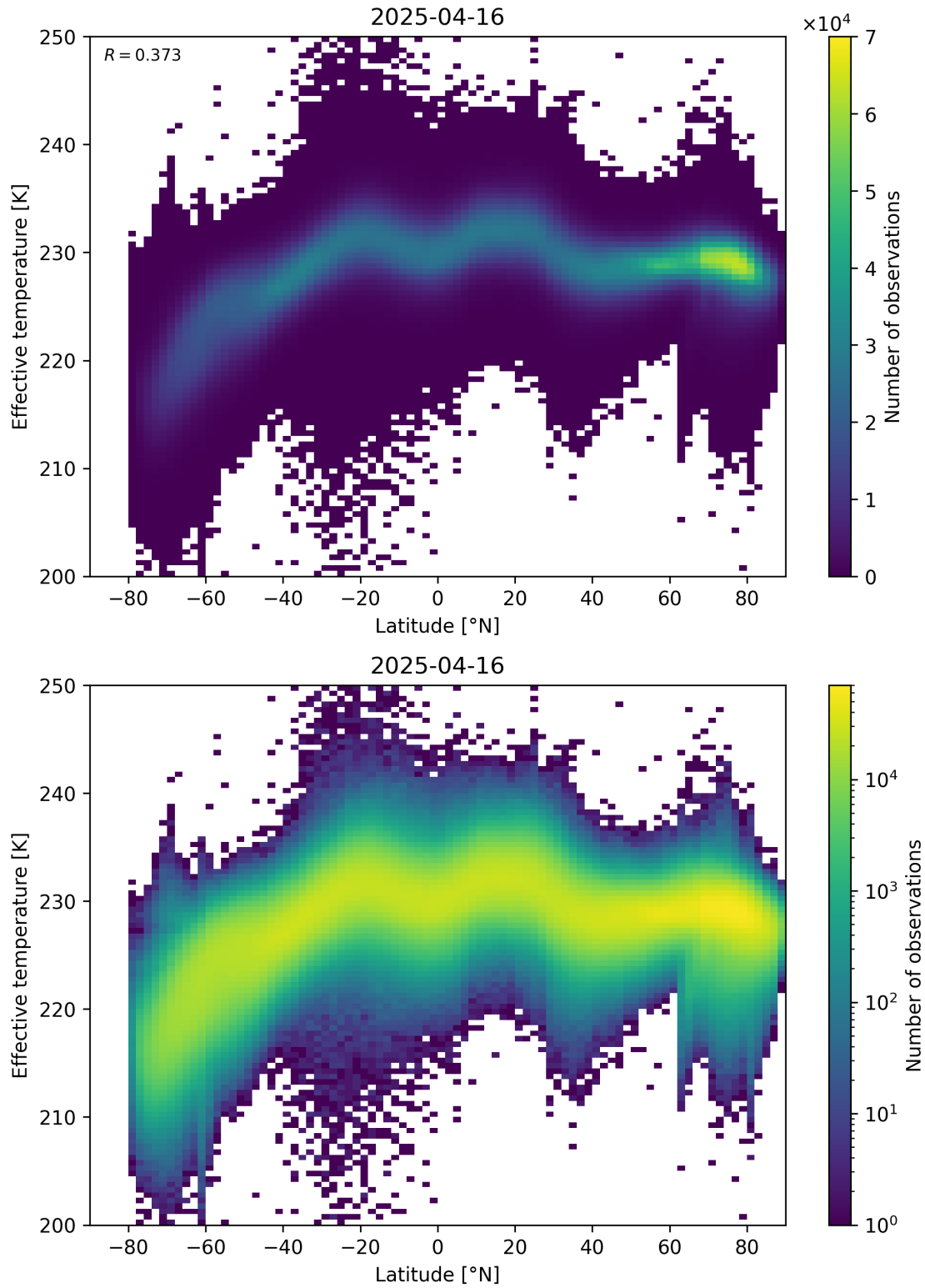
Figure 34: Scatter density plot of “Latitude” against “Effective temperature” for 2025-04-15 to 2025-04-17.
