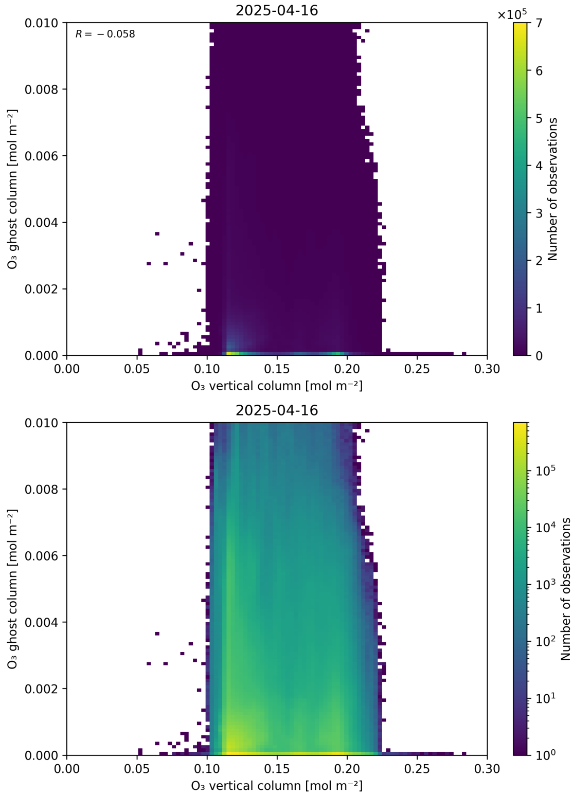
Figure 40: Scatter density plot of “O 3 vertical column” against “O 3 ghost column” for 2025-04-15 to 2025-04-17.
