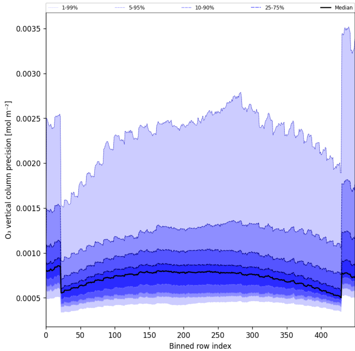
Figure 29: Along track statistics of “O 3 vertical column precision” for 2025-04-15 to 2025-04-17
