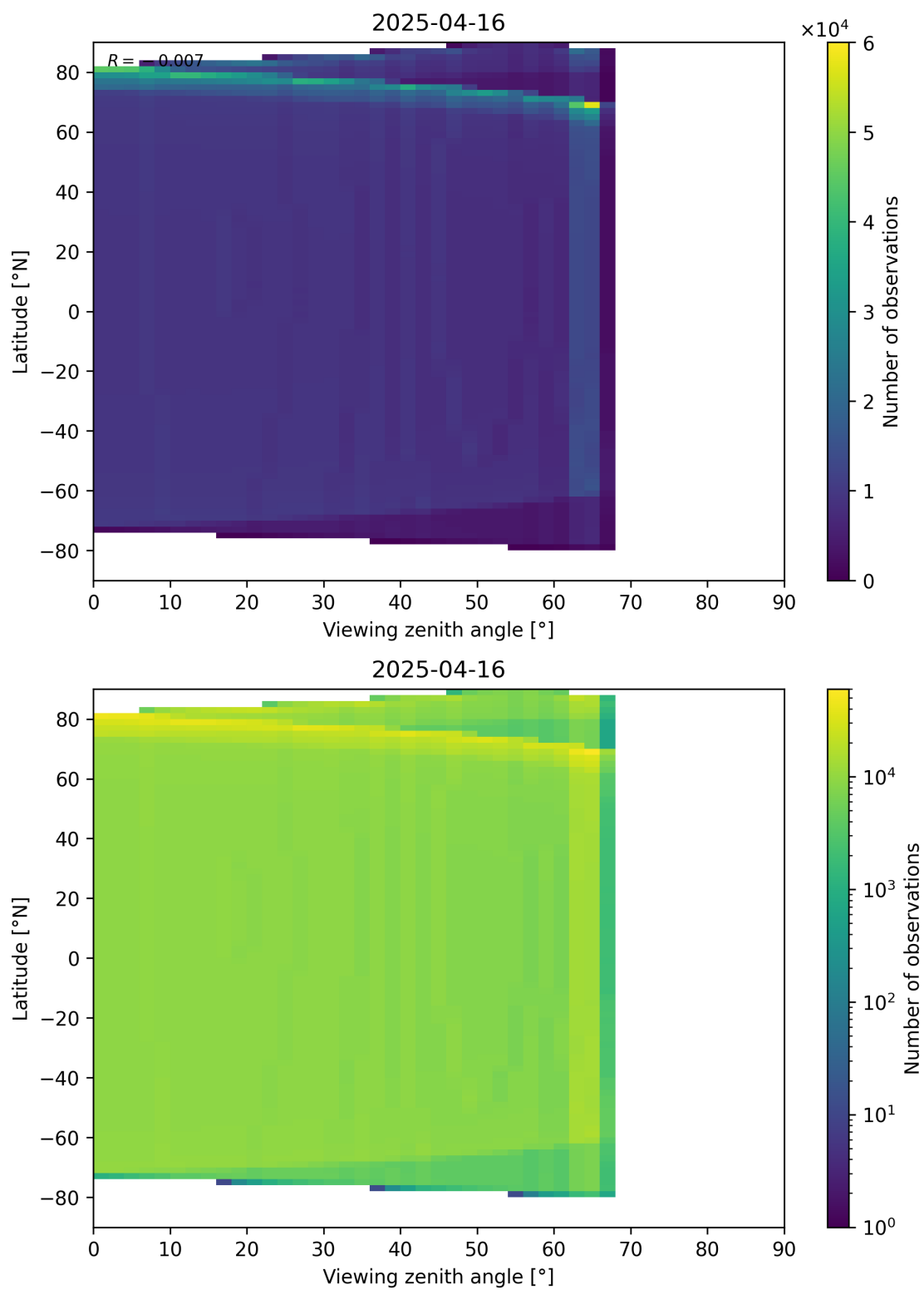
Figure 49: Scatter density plot of “Viewing zenith angle” against “Latitude” for 2025-04-15 to 2025-04-17.
