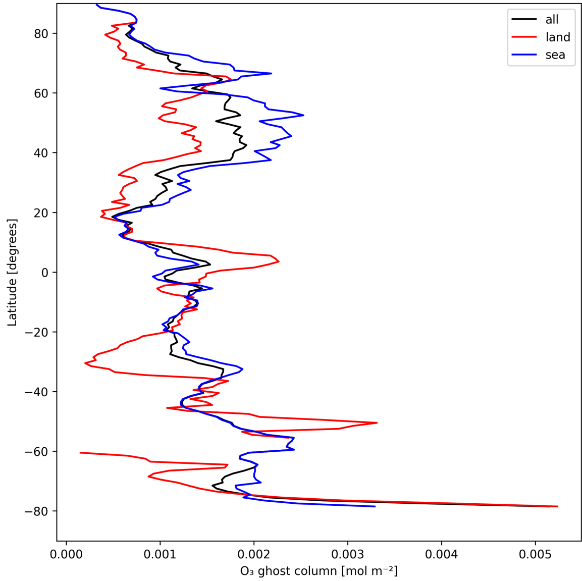
Figure 18: Zonal average of "O 3 ghost column" for 2025-04-15 to 2025-04-17.
