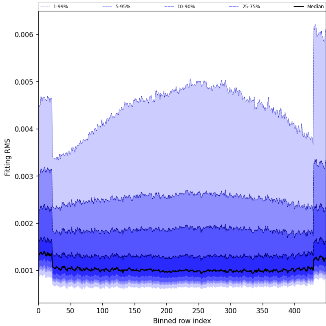
Figure 30: Along track statistics of “Fitting RMS” for 2025-04-15 to 2025-04-17
