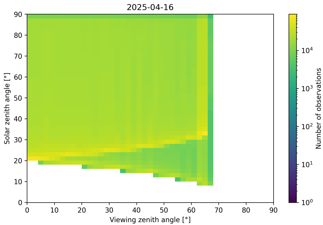
Figure 54: Scatter density plot of “Viewing zenith angle” against “Solar zenith angle” for 2025-04-15 to 2025-04-17.
