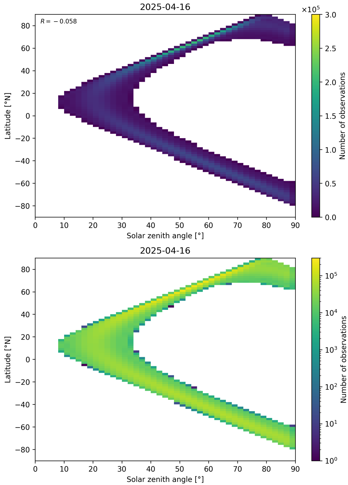
Figure 44: Scatter density plot of “Solar zenith angle” against “Latitude” for 2025-04-15 to 2025-04-17.
