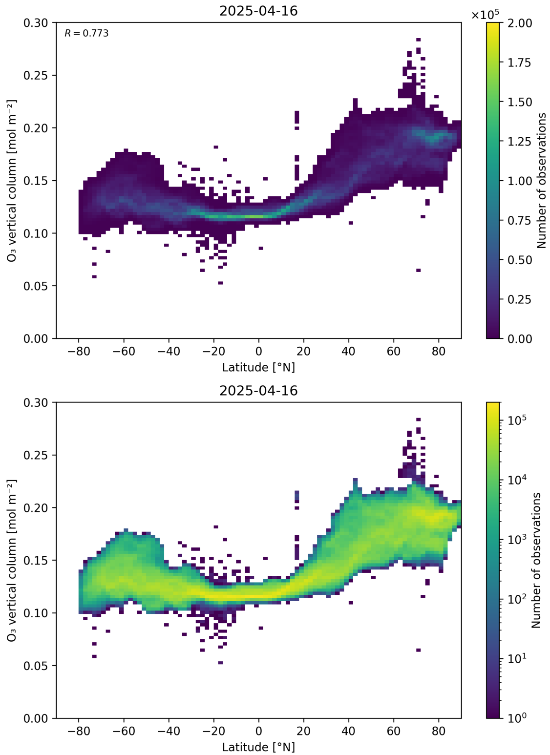
Figure 36: Scatter density plot of “Latitude” against “O 3 vertical column” for 2025-04-15 to 2025-04-17.
