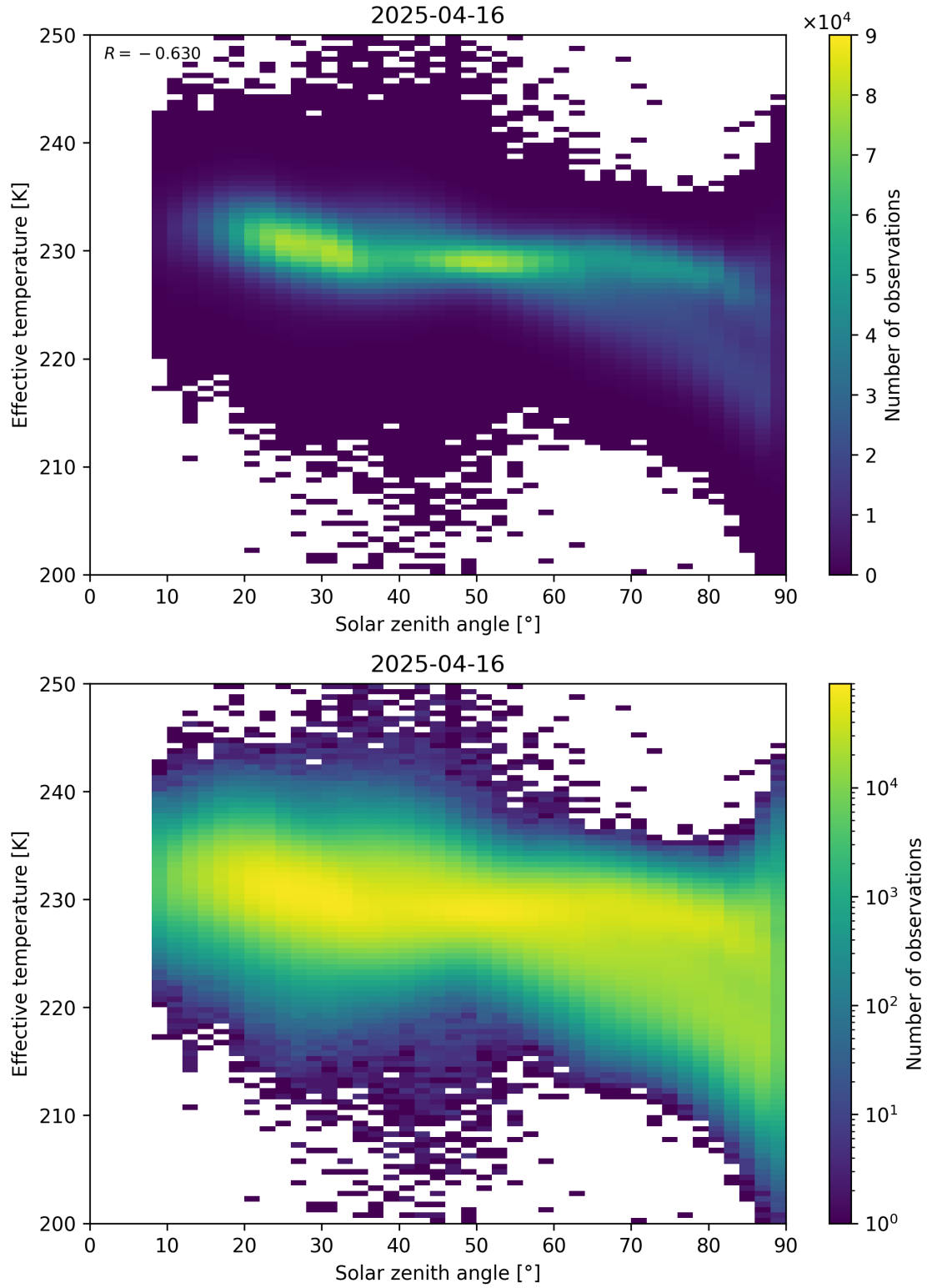
Figure 45: Scatter density plot of “Solar zenith angle” against “Effective temperature” for 2025-04-15 to 2025-04-17.
