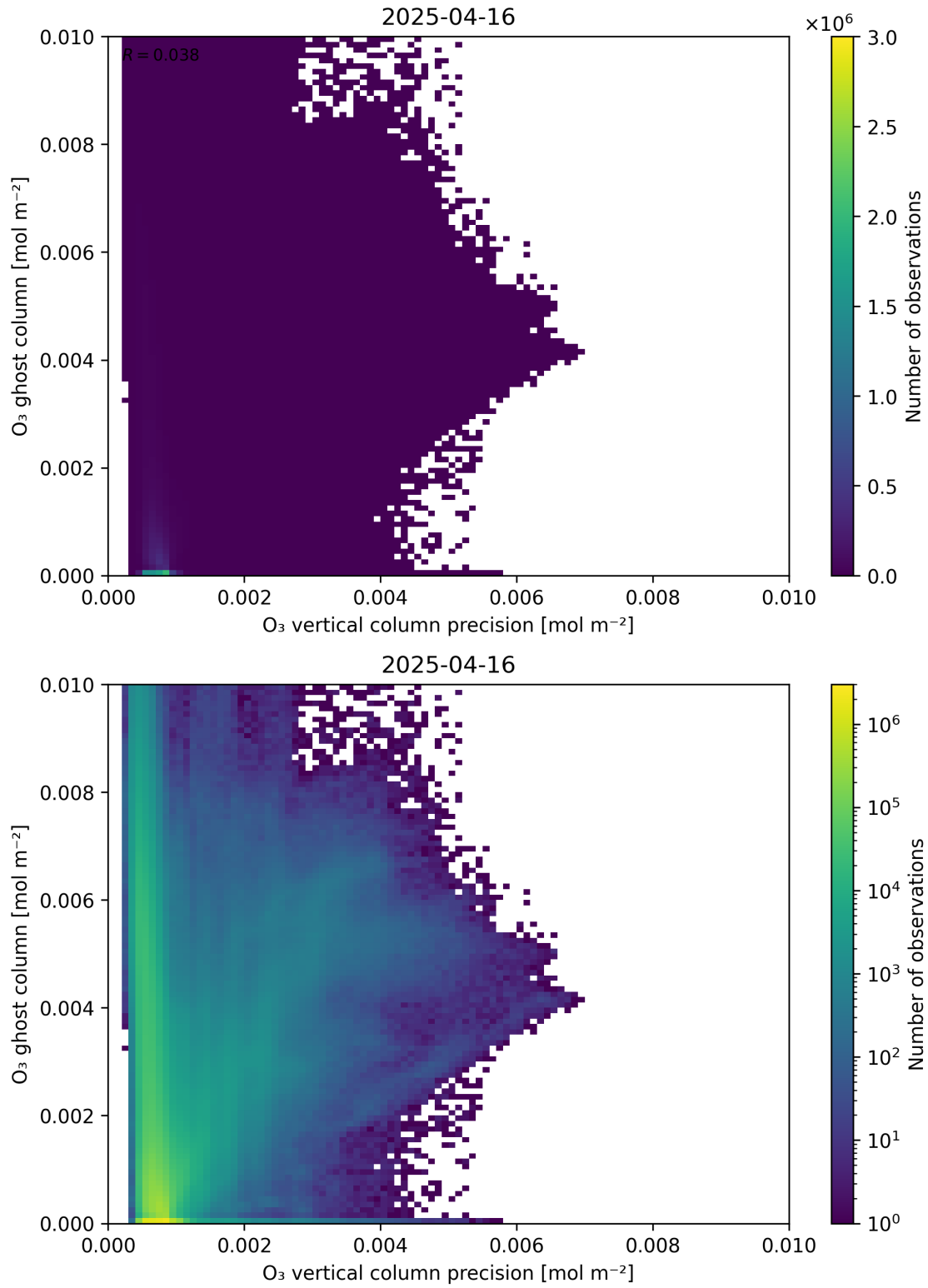
Figure 43: Scatter density plot of “ O_3 vertical column precision” against “ O_3 ghost column” for 2025-04-15 to 2025-04-17.
