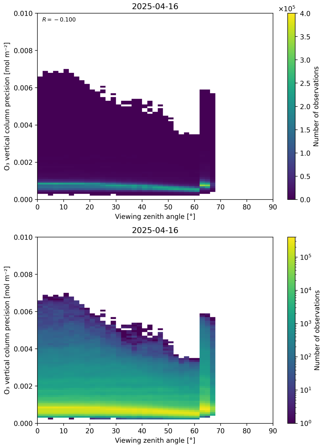
Figure 53: Scatter density plot of “Viewing zenith angle” against “O 3 vertical column precision” for 2025-04-15 to 2025-04-17.
