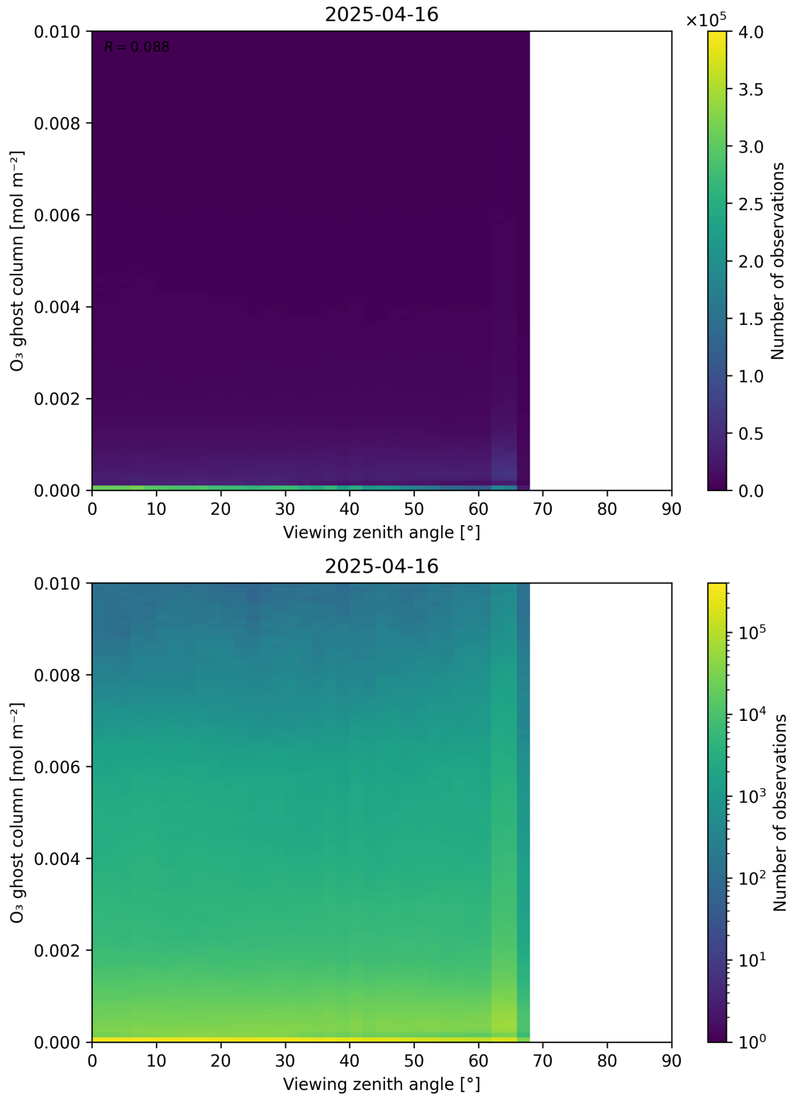
Figure 51: Scatter density plot of “Viewing zenith angle” against “O 3 ghost column” for 2025-04-15 to 2025-04-17.
