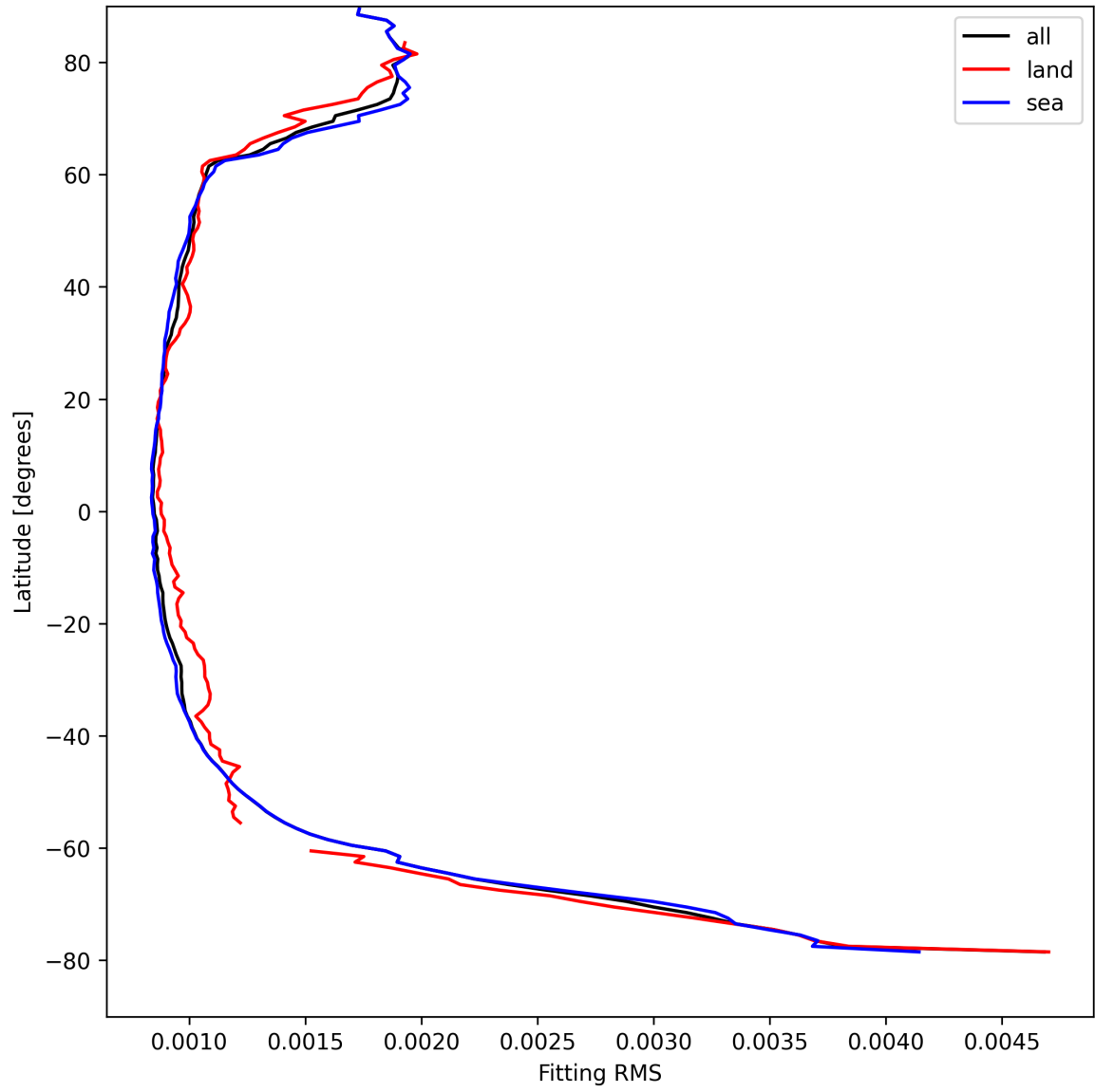
Figure 16: Zonal average of “Fitting RMS” for 2025-04-15 to 2025-04-17.
