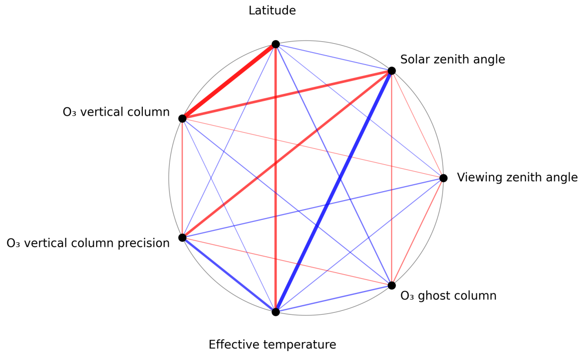
Figure 1: Map of correlation graph for 2025-04-15 to 2025-04-17.
