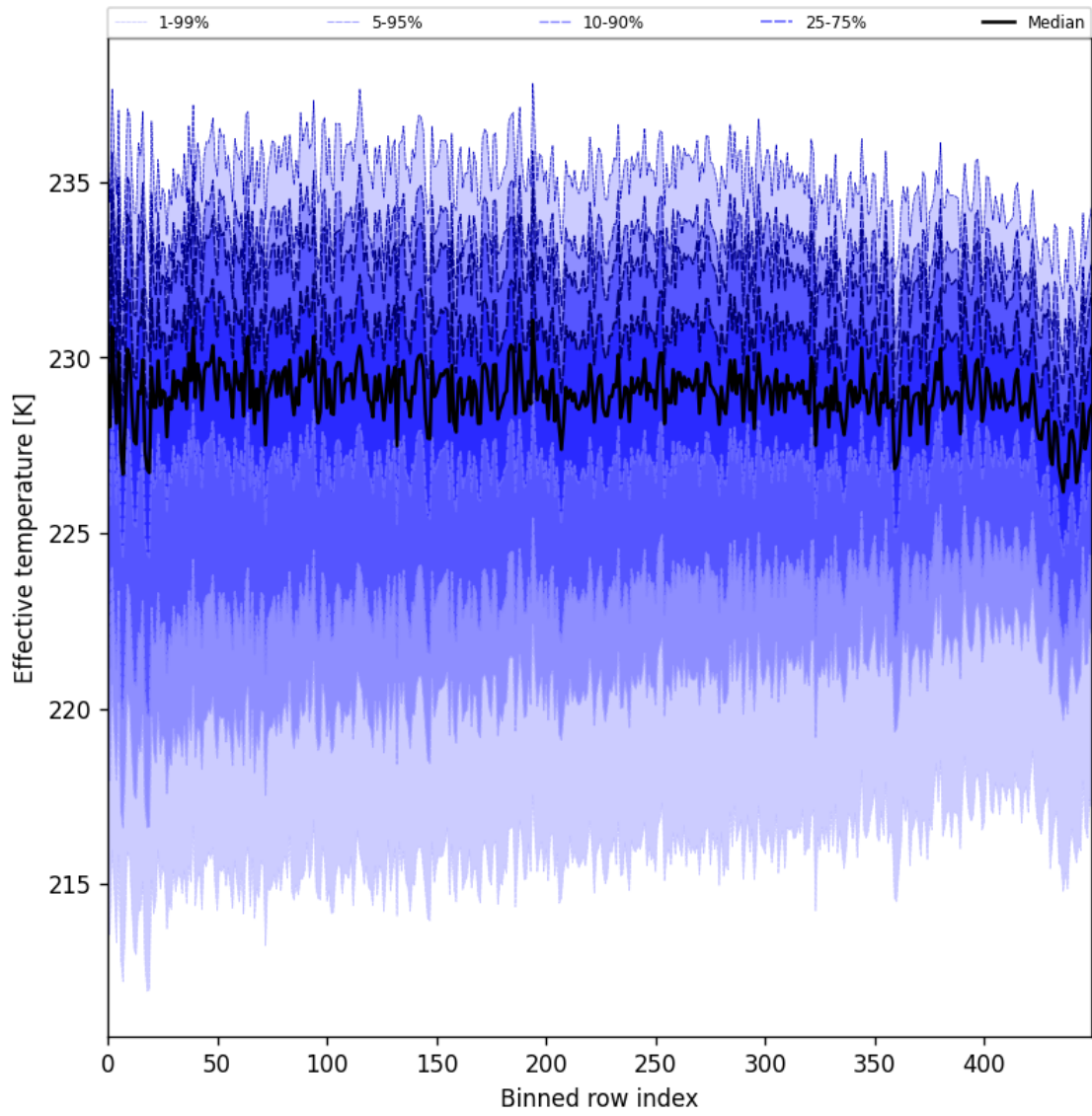
Figure 31: Along track statistics of “Effective temperature” for 2025-04-15 to 2025-04-17
