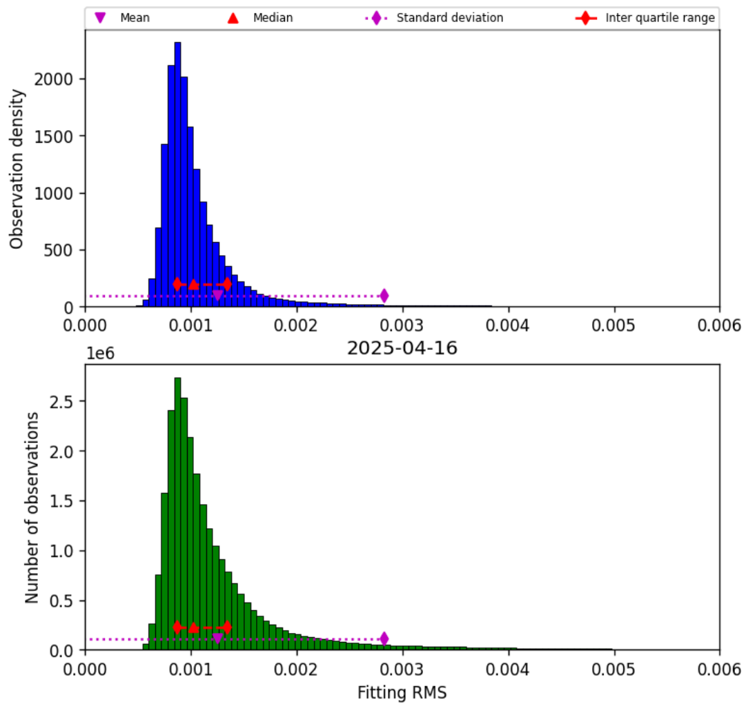
Figure 23: Histogram of “Fitting RMS” for 2025-04-15 to 2025-04-17
