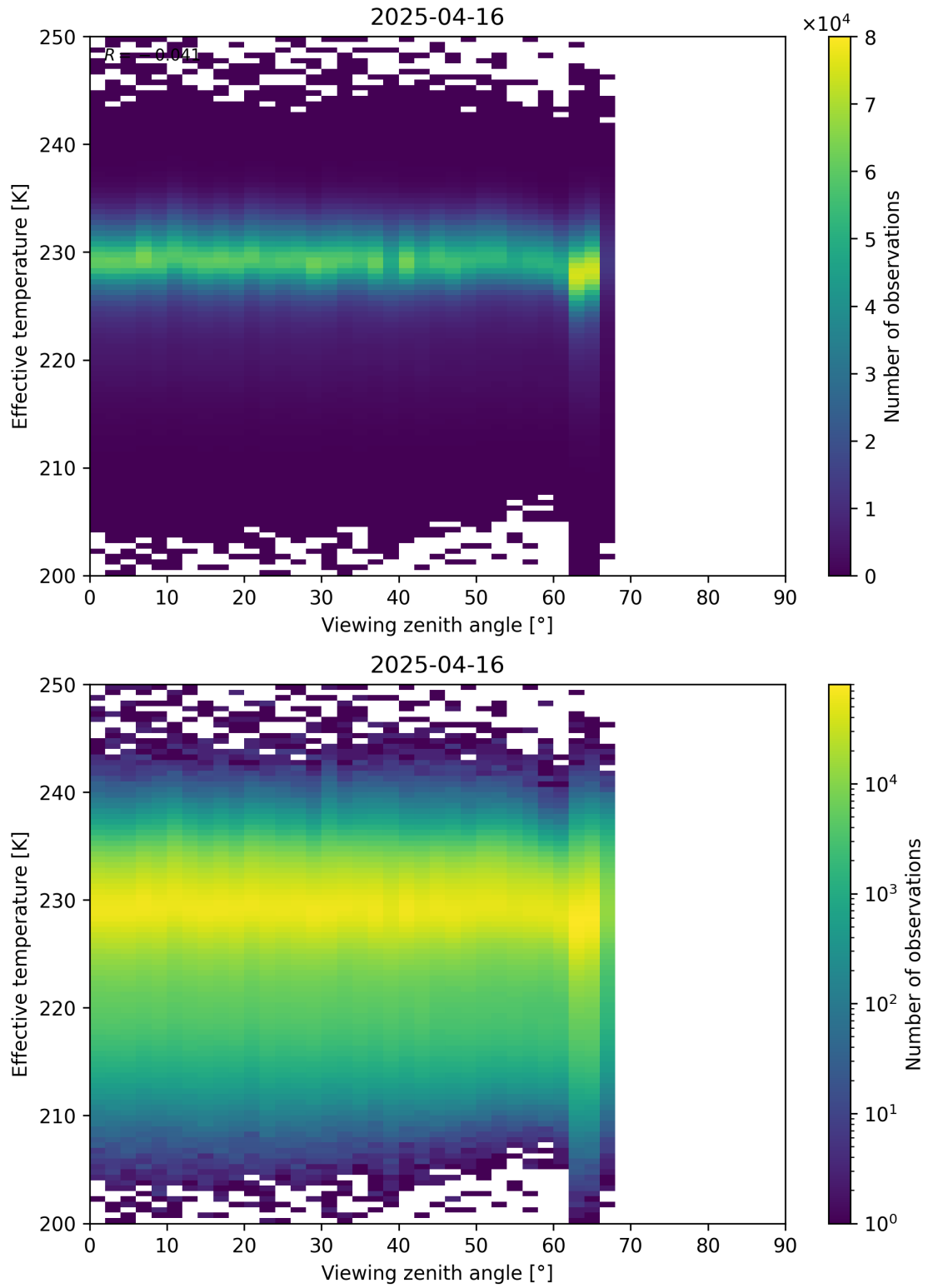
Figure 50: Scatter density plot of “Viewing zenith angle” against “Effective temperature” for 2025-04-15 to 2025-04-17.
