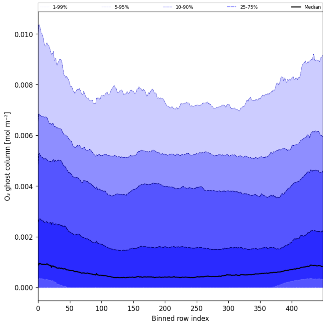
Figure 32: Along track statistics of “O 3 ghost column” for 2025-04-15 to 2025-04-17
