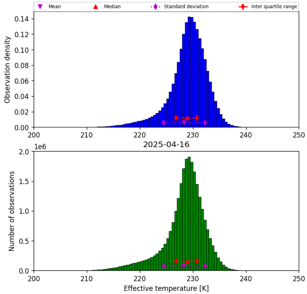
Figure 24: Histogram of “Effective temperature” for 2025-04-15 to 2025-04-17
