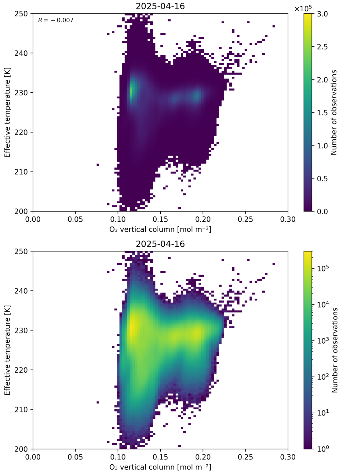
Figure 39: Scatter density plot of “O 3 vertical column” against “Effective temperature” for 2025-04-15 to 2025-04-17.
