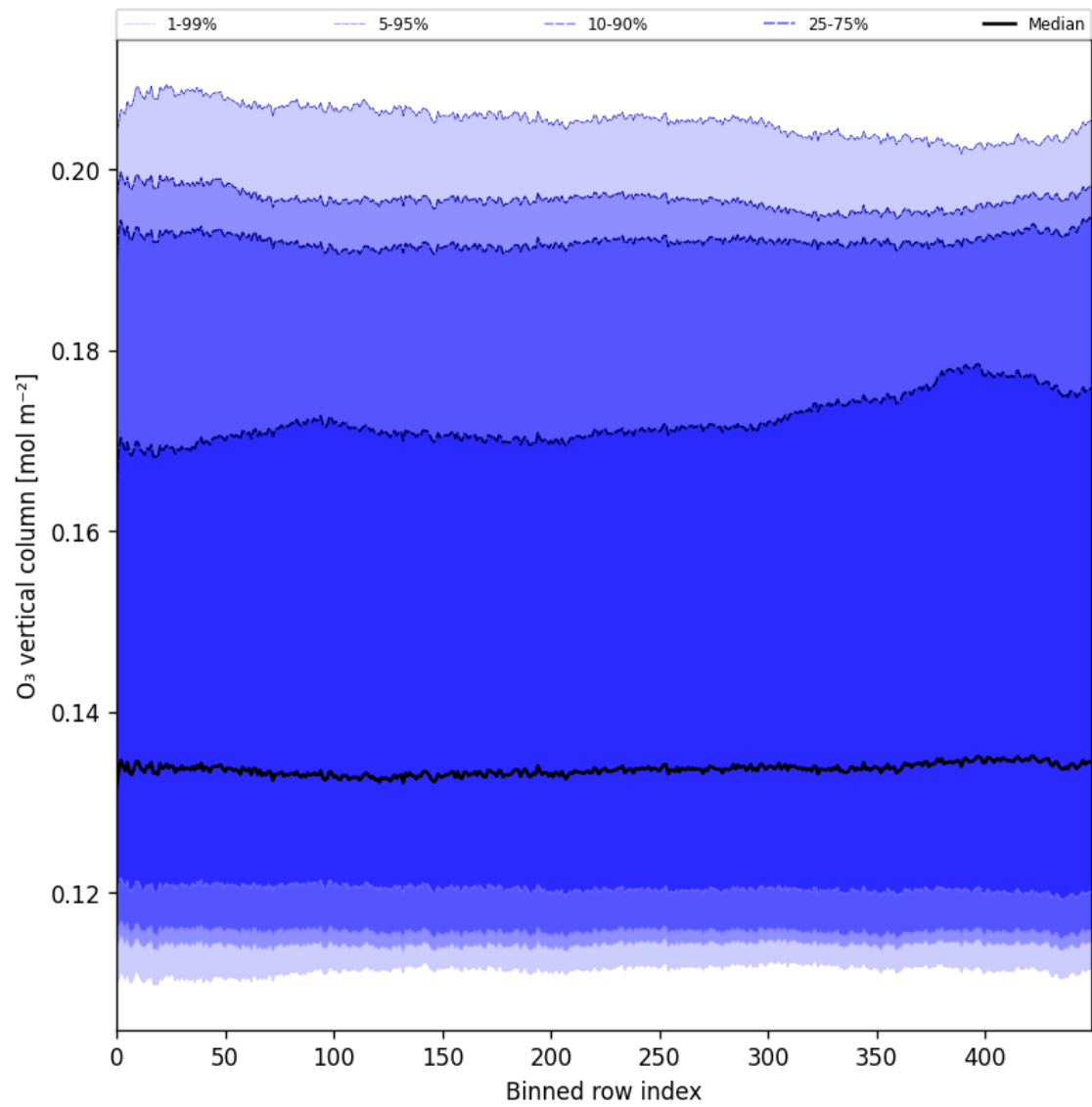
Figure 28: Along track statistics of “O 3 vertical column” for 2025-04-15 to 2025-04-17
