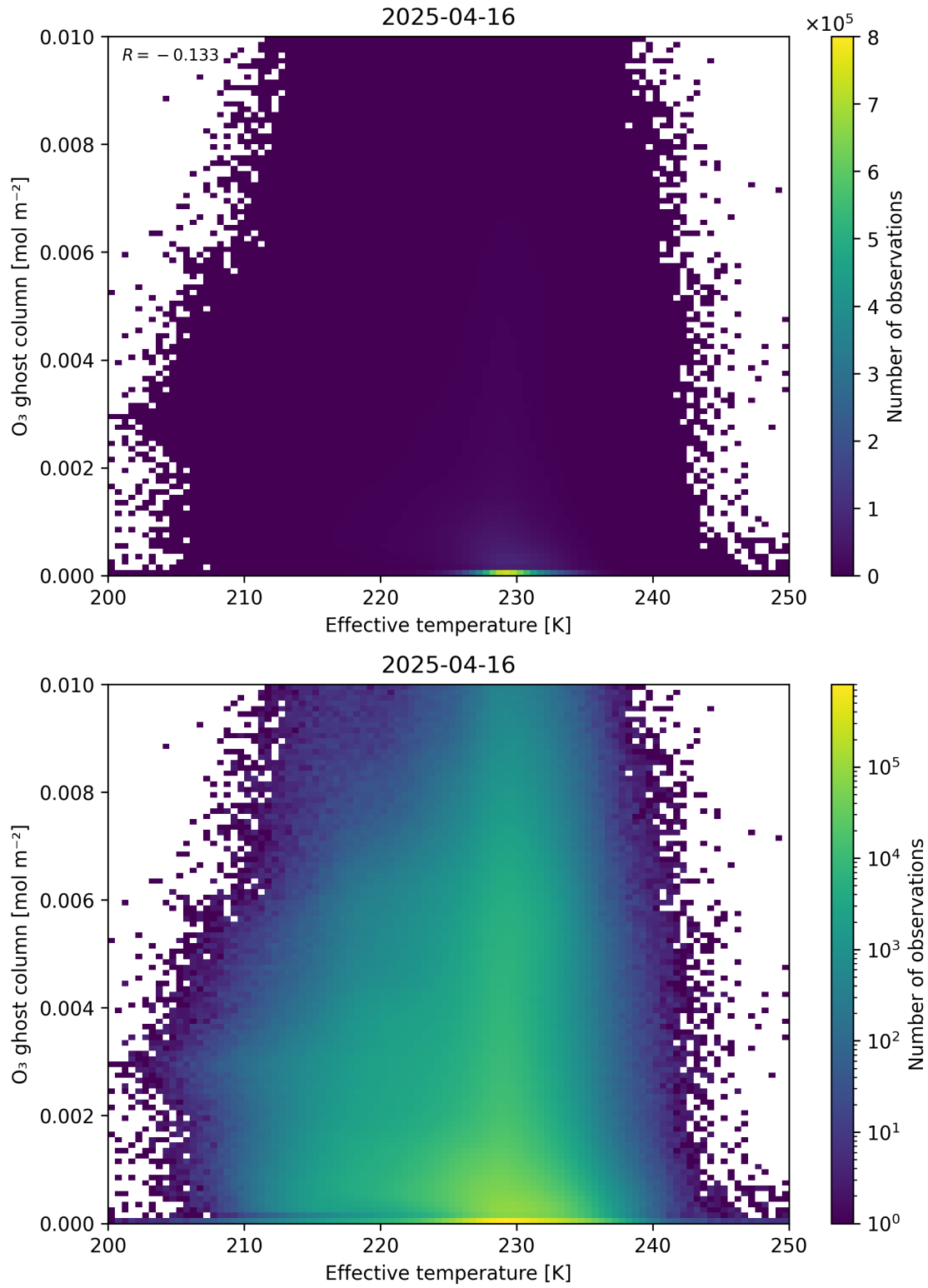
Figure 38: Scatter density plot of “Effective temperature” against “O 3 ghost column” for 2025-04-15 to 2025-04-17.
