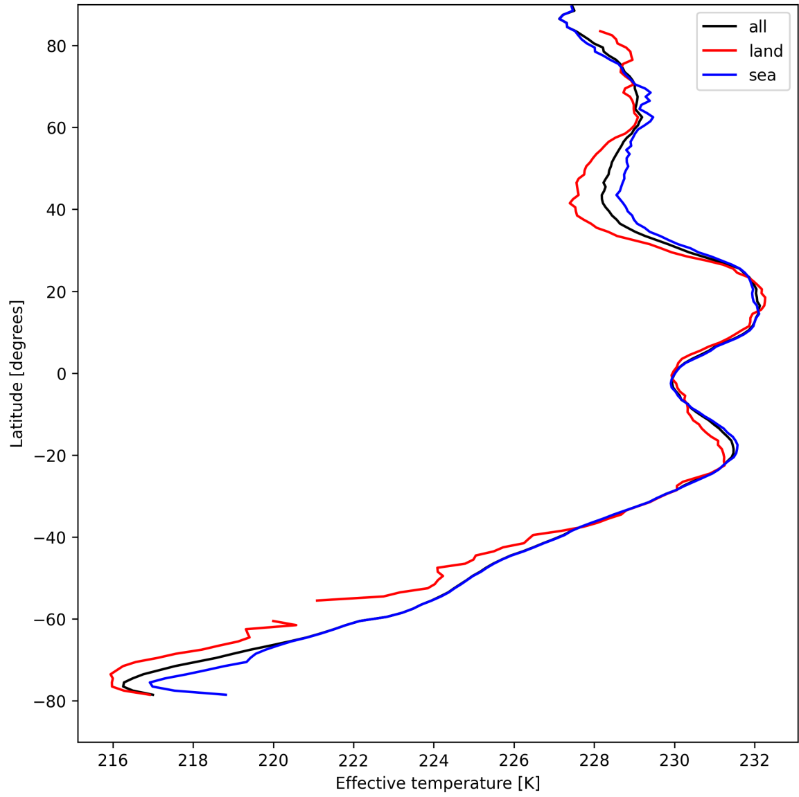
Figure 17: Zonal average of "Effective temperature" for 2025-04-15 to 2025-04-17.
