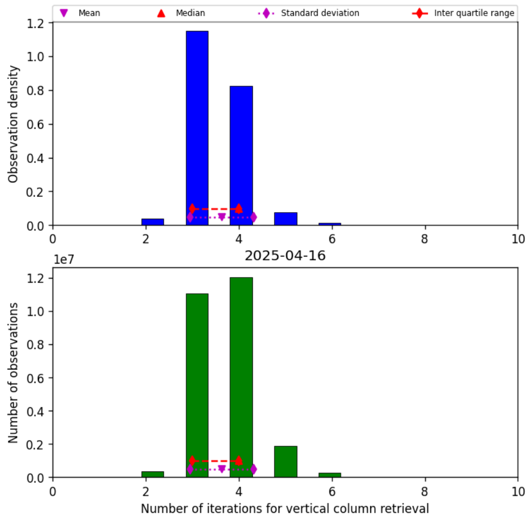
Figure 26: Histogram of “Number of iterations for vertical column retrieval” for 2025-04-15 to 2025-04-17
