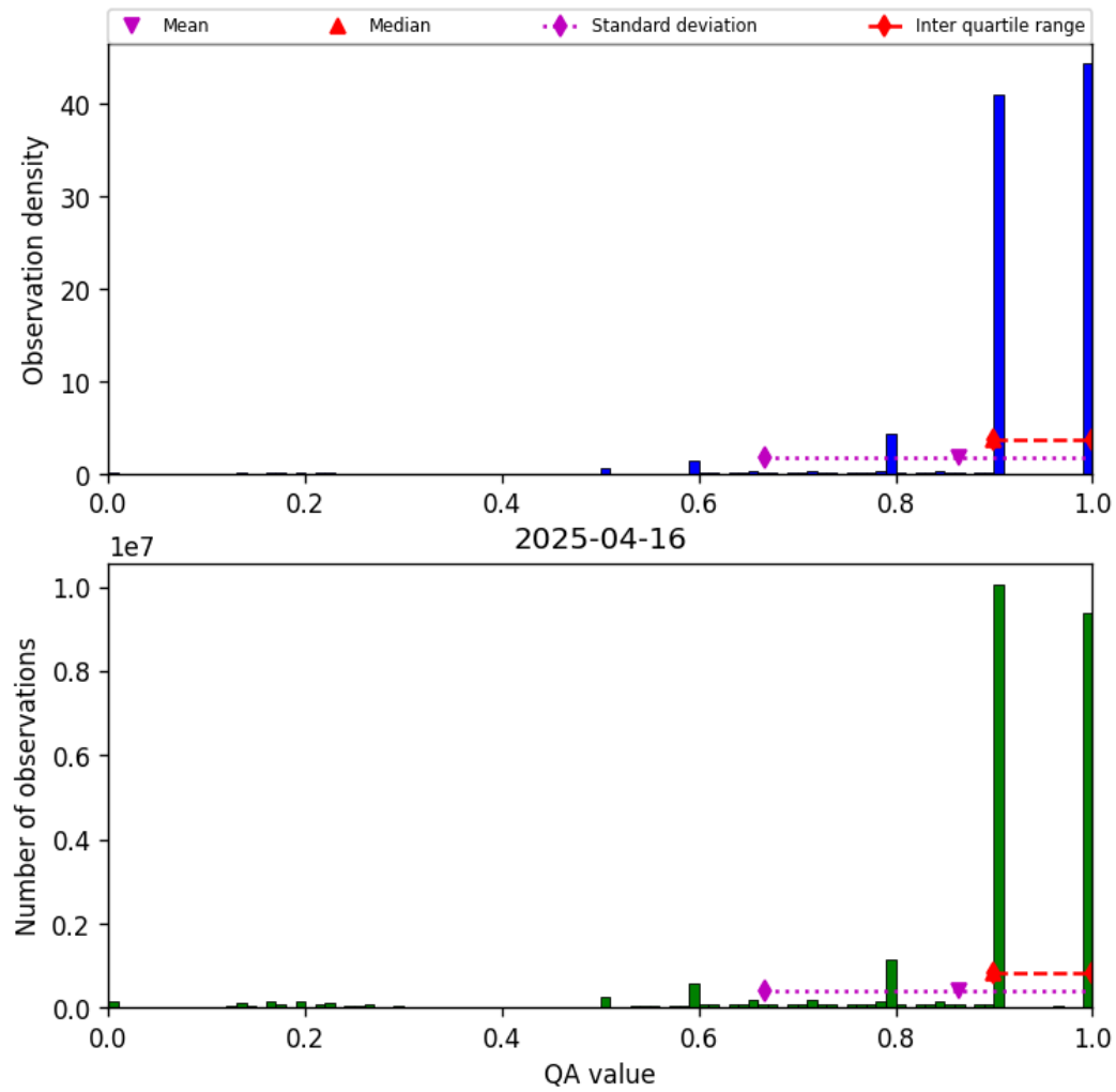
Figure 20: Histogram of “QA value” for 2025-04-15 to 2025-04-17
