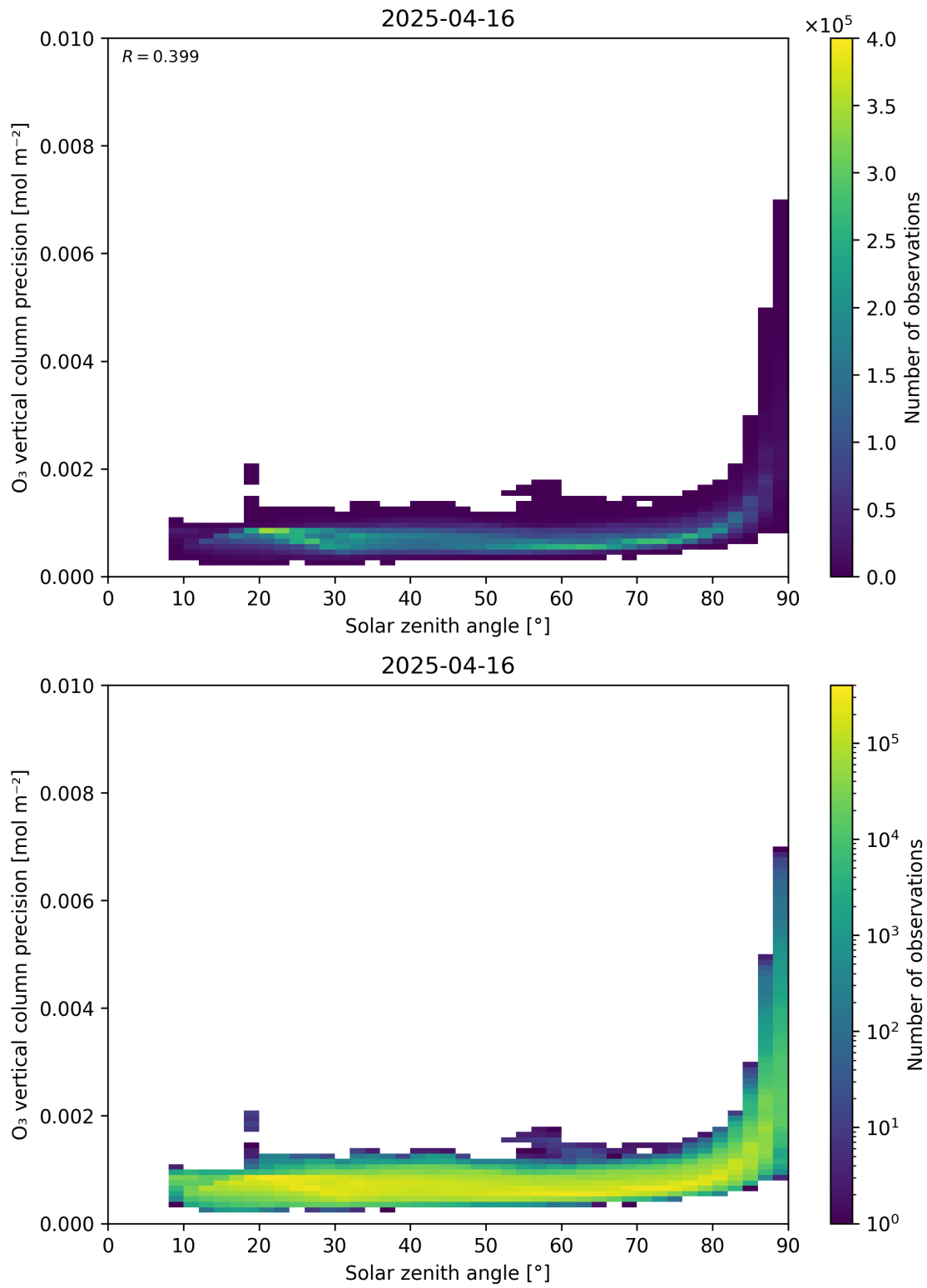
Figure 48: Scatter density plot of “Solar zenith angle” against “O 3 vertical column precision” for 2025-04-15 to 2025-04-17.
