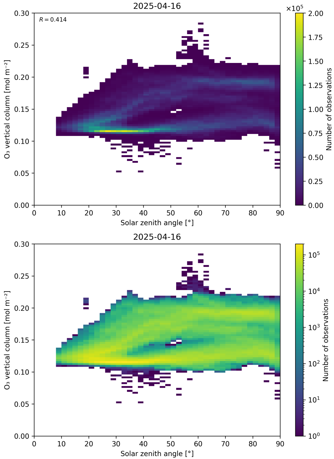
Figure 47: Scatter density plot of “Solar zenith angle” against “O 3 vertical column” for 2025-04-15 to 2025-04-17.
