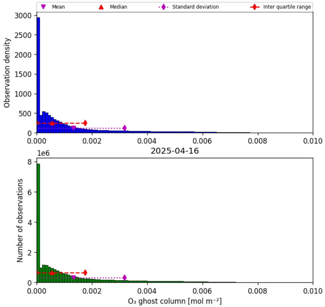
Figure 25: Histogram of “O 3 ghost column” for 2025-04-15 to 2025-04-17
