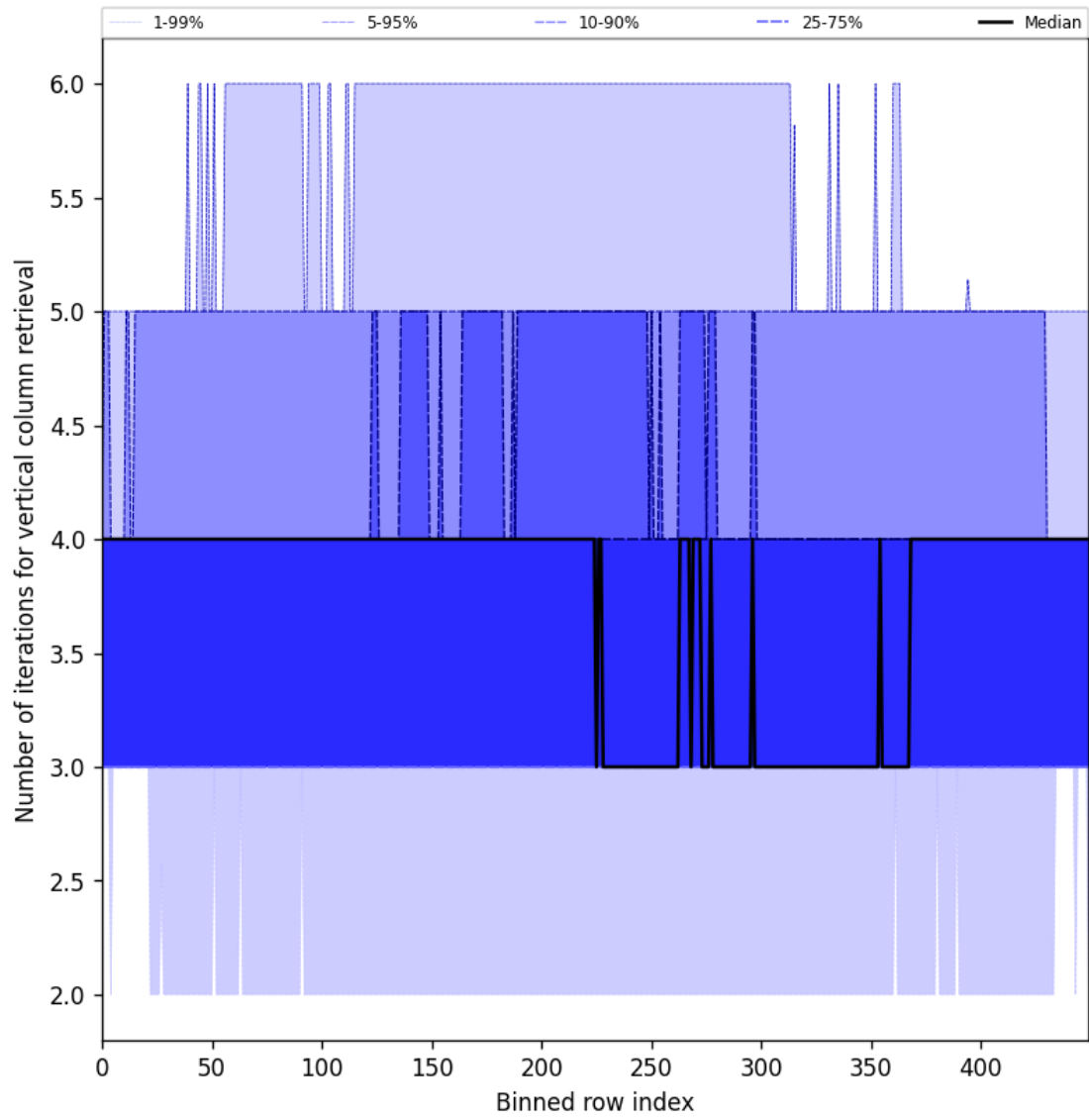
Figure 33: Along track statistics of “Number of iterations for vertical column retrieval” for 2025-04-15 to 2025-04-17
