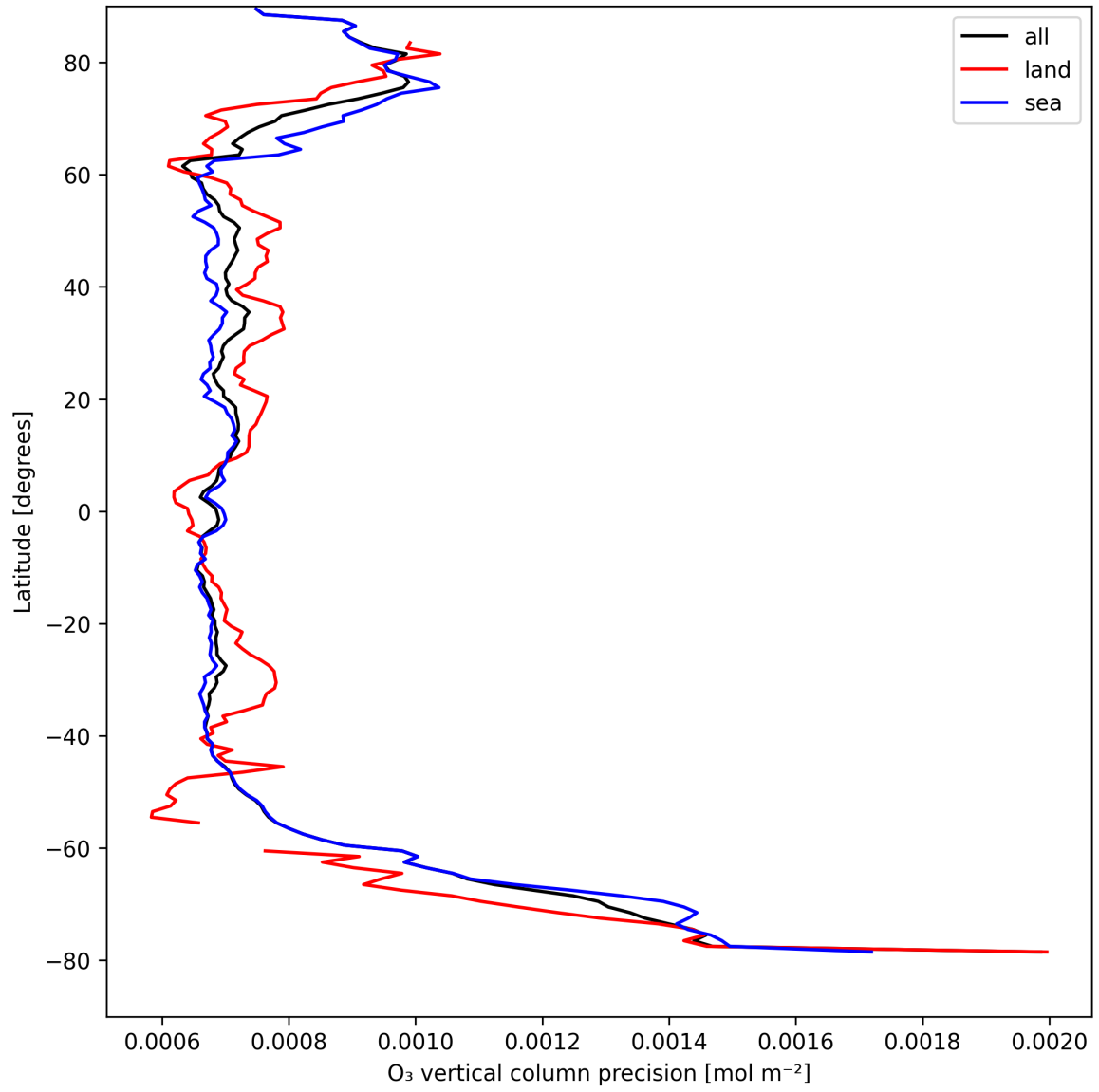
Figure 15: Zonal average of “O 3 vertical column precision” for 2025-04-15 to 2025-04-17.
