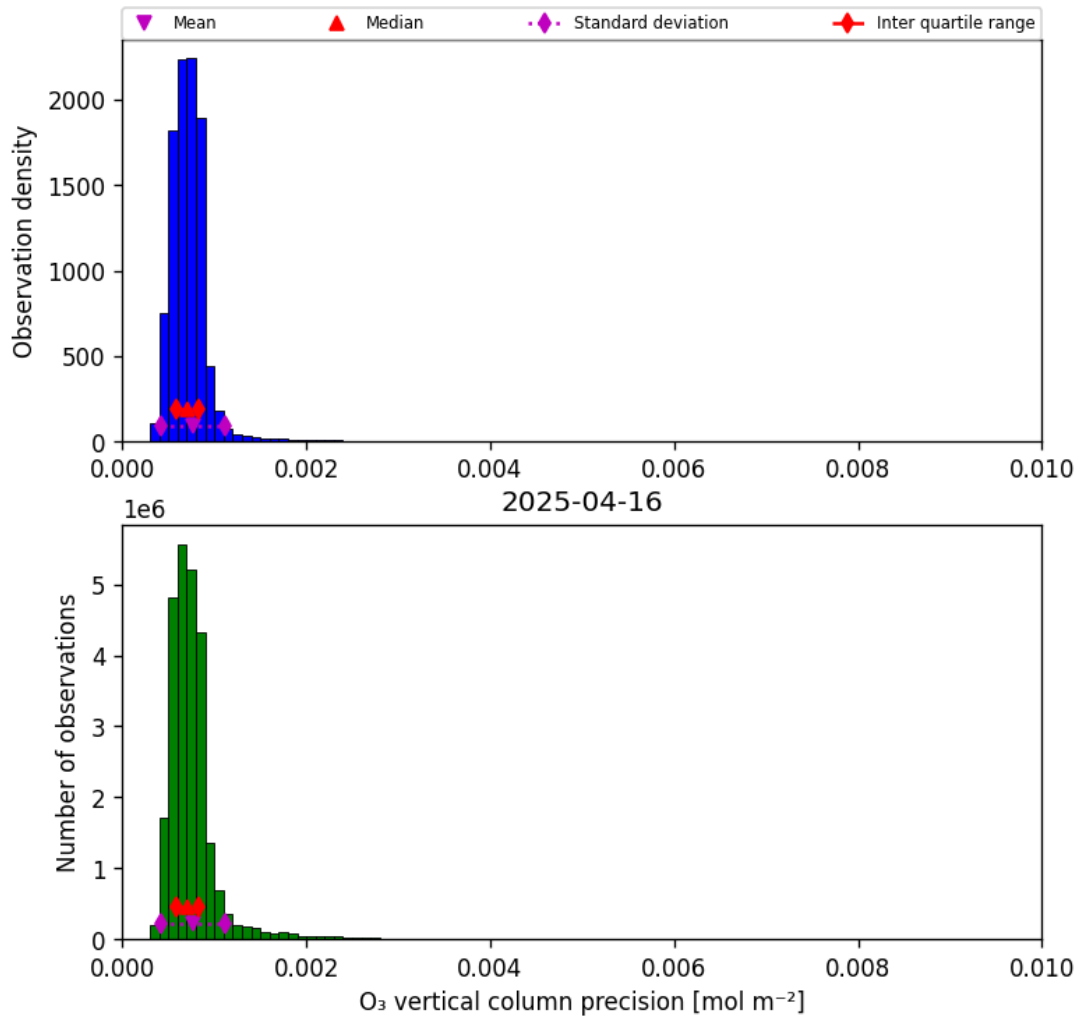
Figure 22: Histogram of “O 3 vertical column precision” for 2025-04-15 to 2025-04-17
