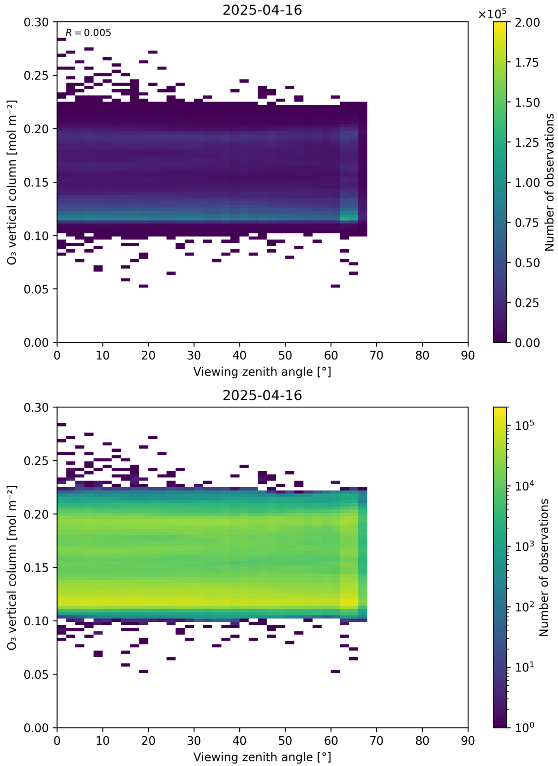
Figure 52: Scatter density plot of “Viewing zenith angle” against “O 3 vertical column” for 2025-04-15 to 2025-04-17.
