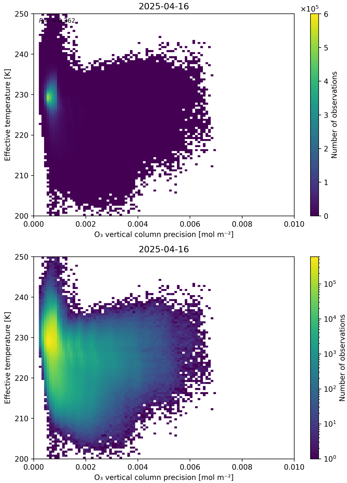
Figure 42: Scatter density plot of “O 3 vertical column precision” against “Effective temperature” for 2025-04-15 to 2025-04-17.
