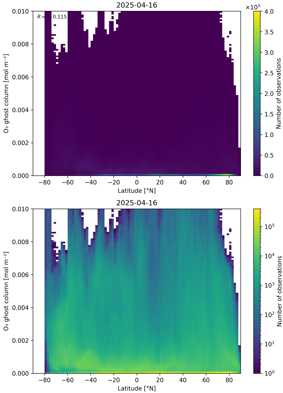
Figure 35: Scatter density plot of “Latitude” against “O 3 ghost column” for 2025-04-15 to 2025-04-17.
