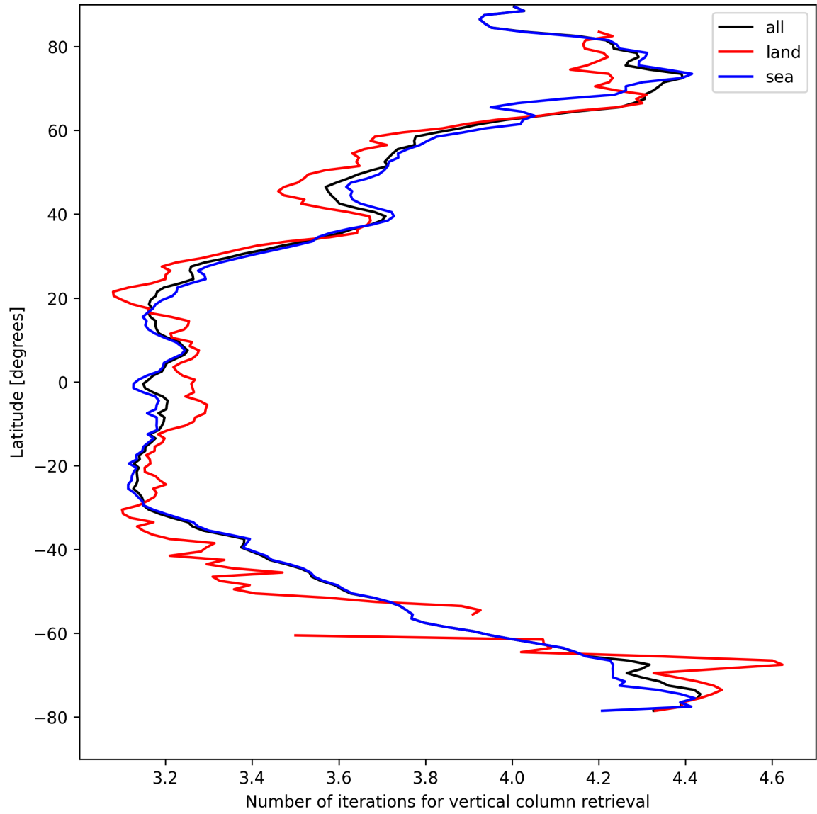
Figure 19: Zonal average of “Number of iterations for vertical column retrieval” for 2025-04-15 to 2025-04-17.
