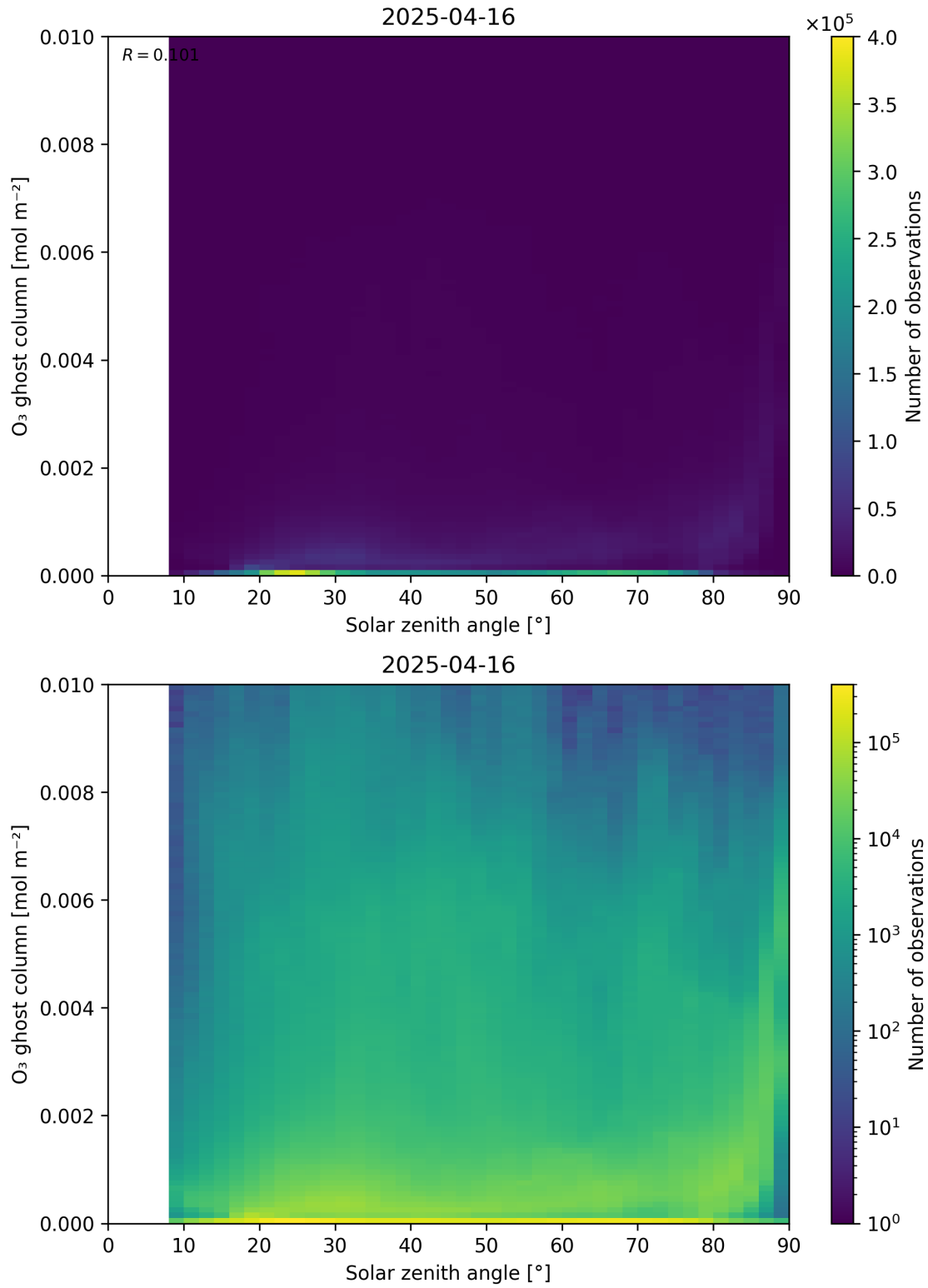
Figure 46: Scatter density plot of “Solar zenith angle” against “O 3 ghost column” for 2025-04-15 to 2025-04-17.
