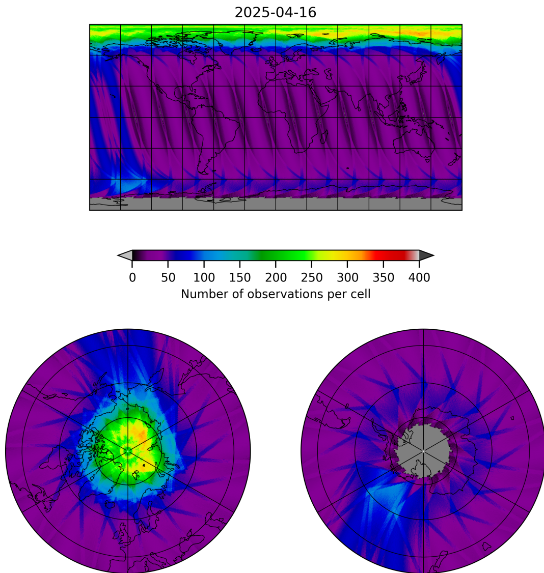
Figure 12: Map of the number of observations for 2025-04-15 to 2025-04-17
