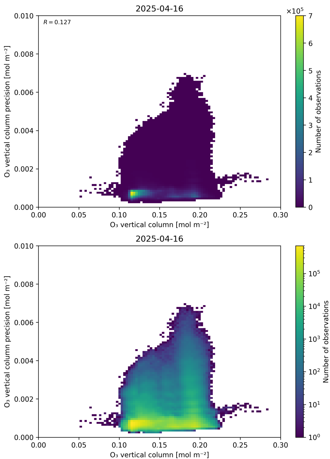
Figure 41: Scatter density plot of “O 3 vertical column” against “O 3 vertical column precision” for 2025-04-15 to 2025-04-17.
