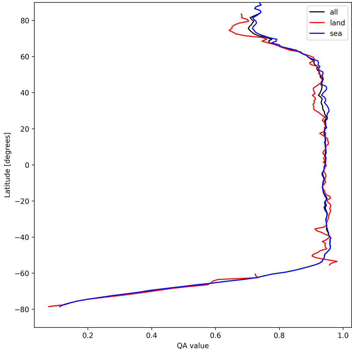
Figure 13: Zonal average of “QA value” for 2025-04-15 to 2025-04-17.
