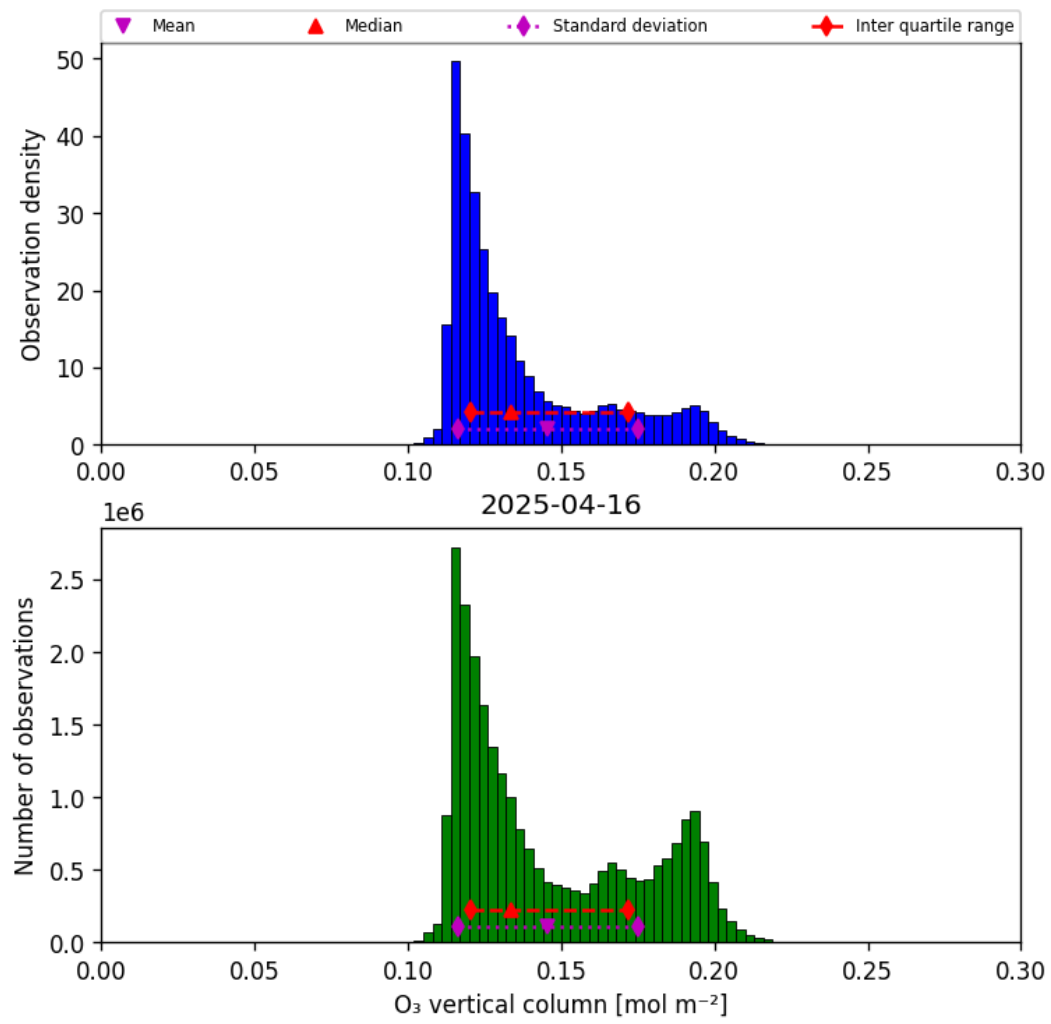
Figure 21: Histogram of “O 3 vertical column” for 2025-04-15 to 2025-04-17
