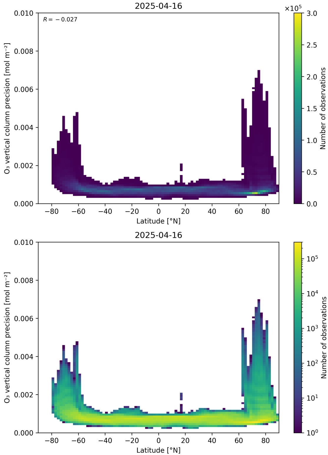
Figure 37: Scatter density plot of “Latitude” against “O 3 vertical column precision” for 2025-04-15 to 2025-04-17.
