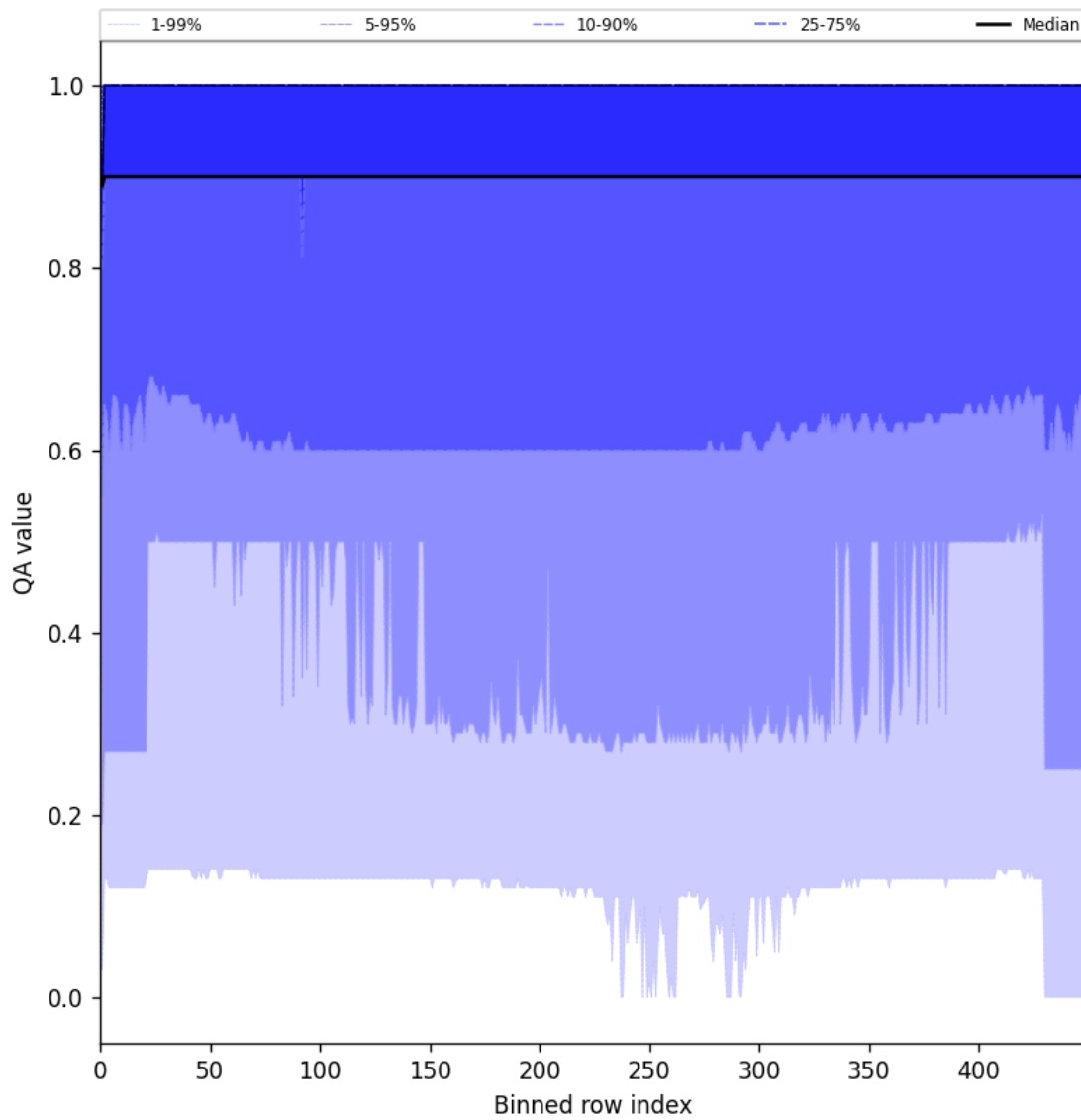
Figure 27: Along track statistics of “QA value” for 2025-04-15 to 2025-04-17
