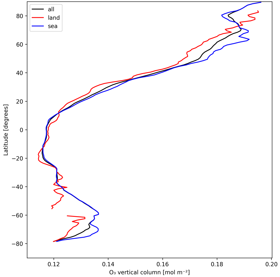
Figure 14: Zonal average of “O 3 vertical column” for 2025-04-15 to 2025-04-17.
