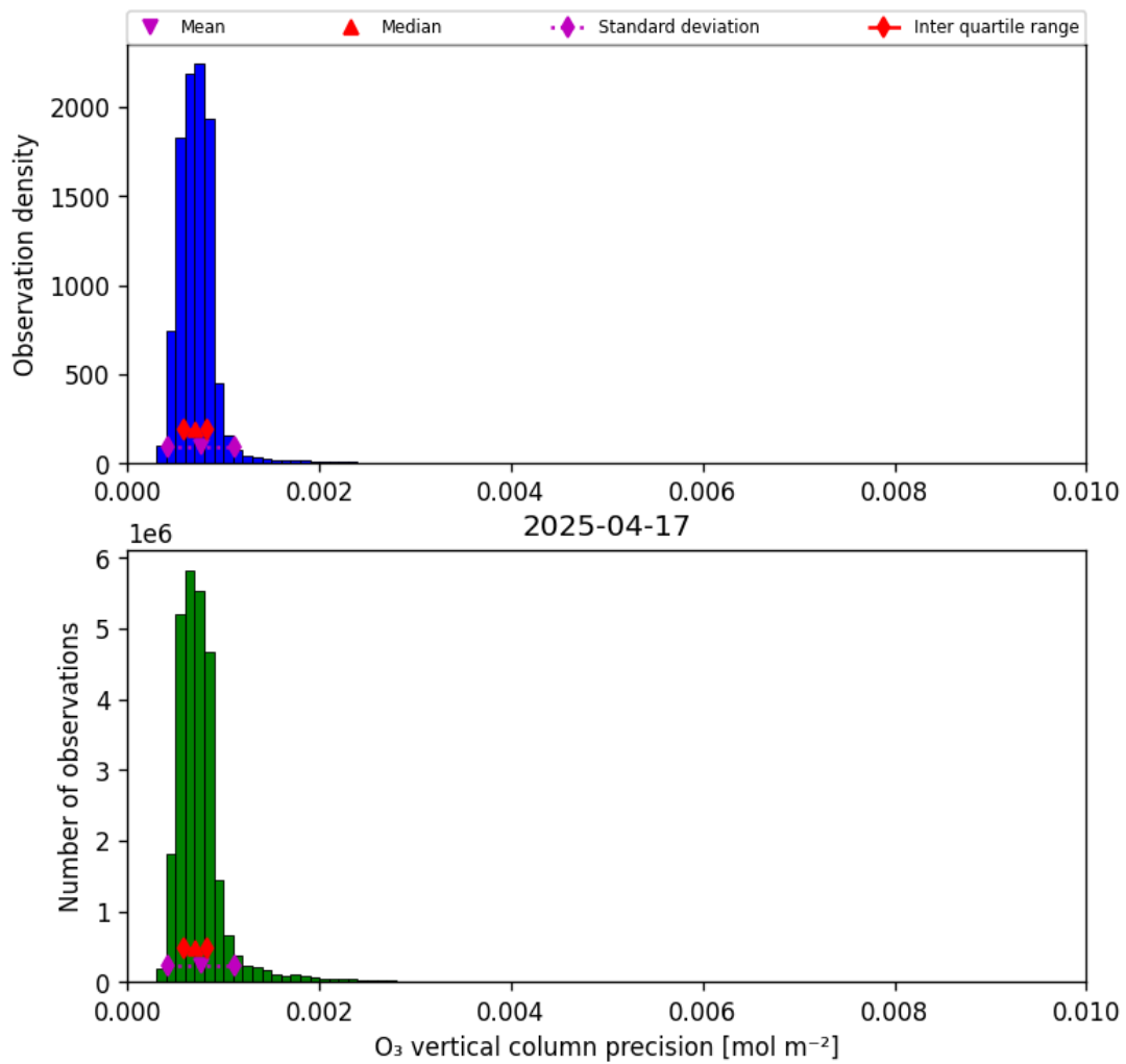
Figure 22: Histogram of “O 3 vertical column precision” for 2025-04-16 to 2025-04-18
