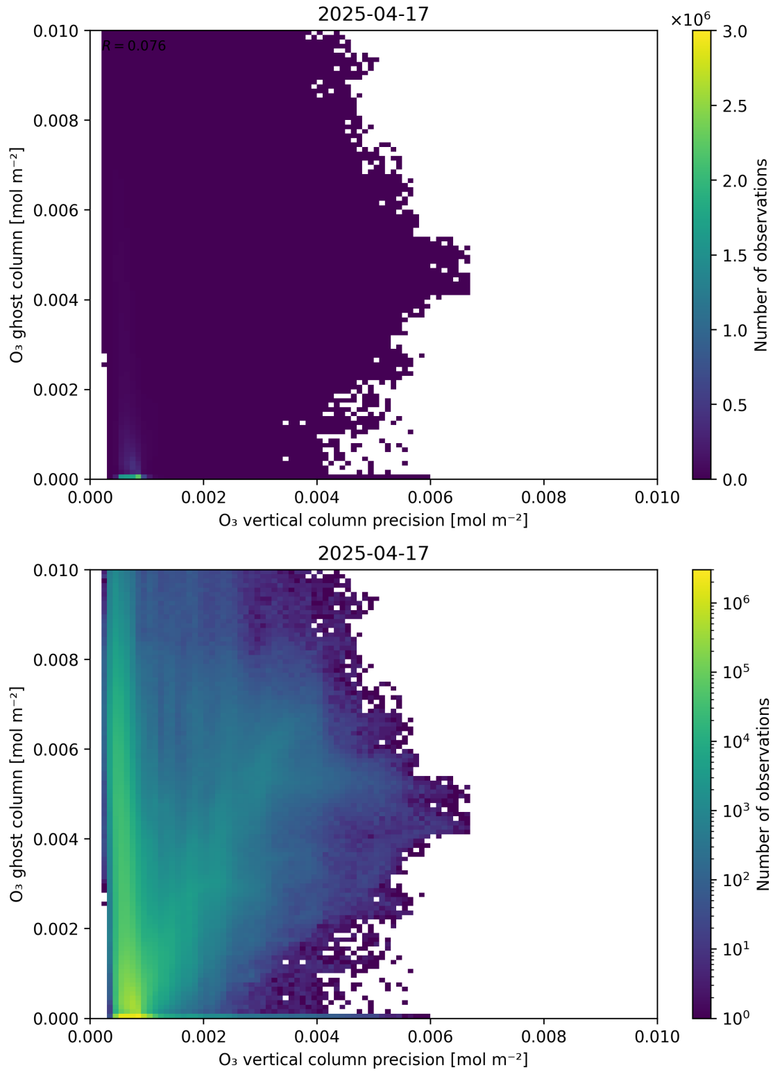
Figure 43: Scatter density plot of “ \text{O}_3 vertical column precision” against “ \text{O}_3 ghost column” for 2025-04-16 to 2025-04-18.
