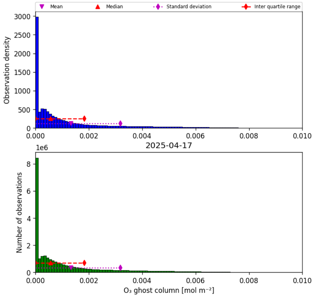
Figure 25: Histogram of “O 3 ghost column” for 2025-04-16 to 2025-04-18
