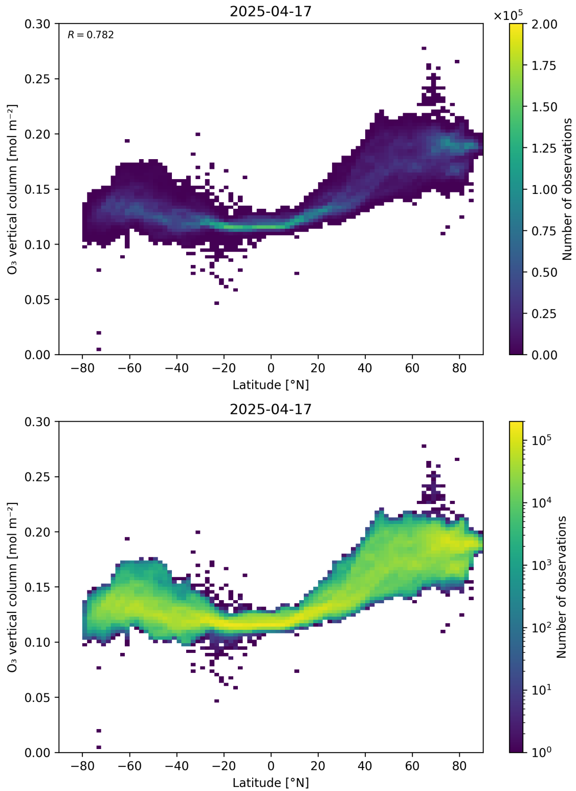
Figure 36: Scatter density plot of “Latitude” against “O 3 vertical column” for 2025-04-16 to 2025-04-18.
