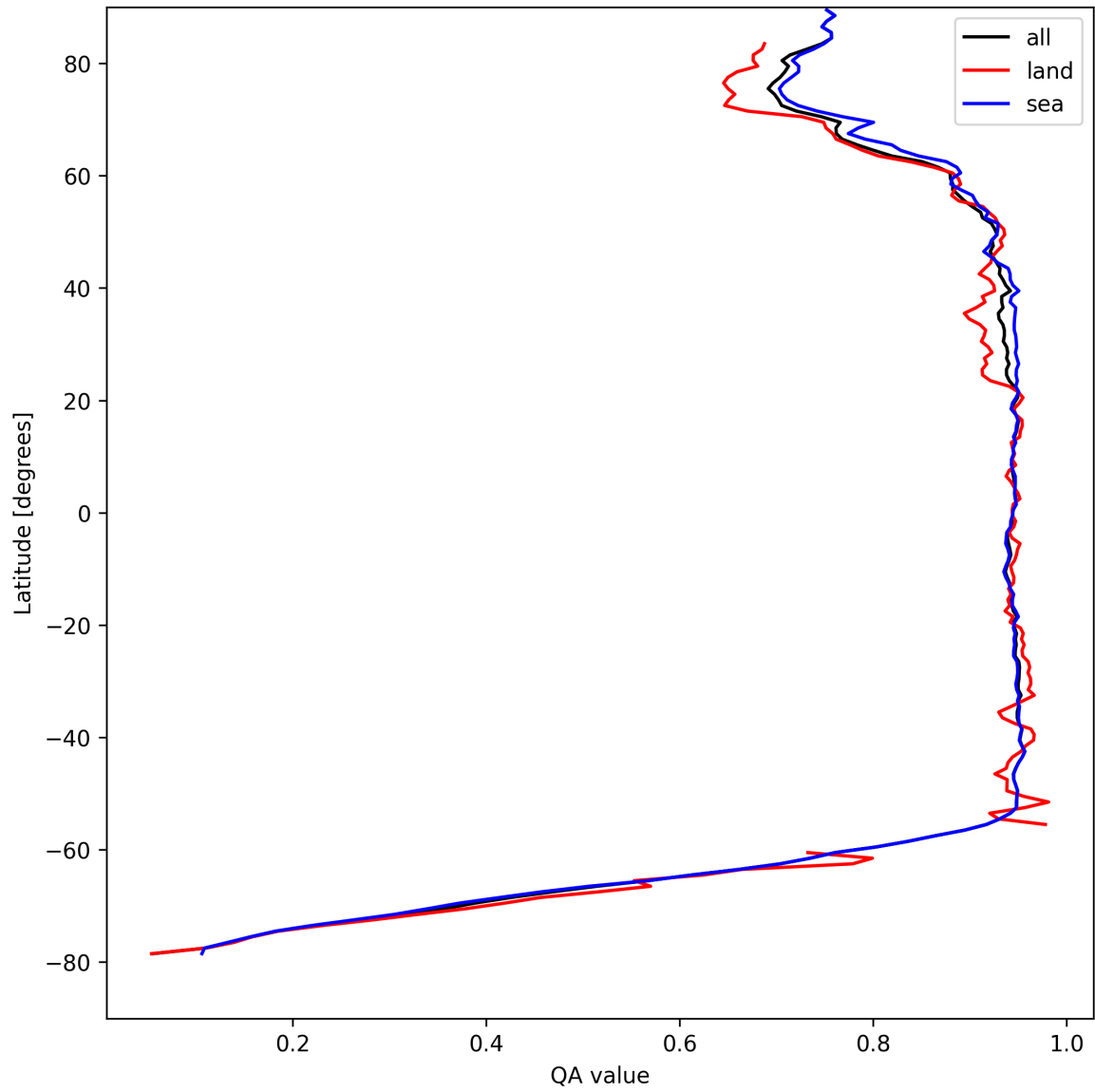
Figure 13: Zonal average of “QA value” for 2025-04-16 to 2025-04-18.
