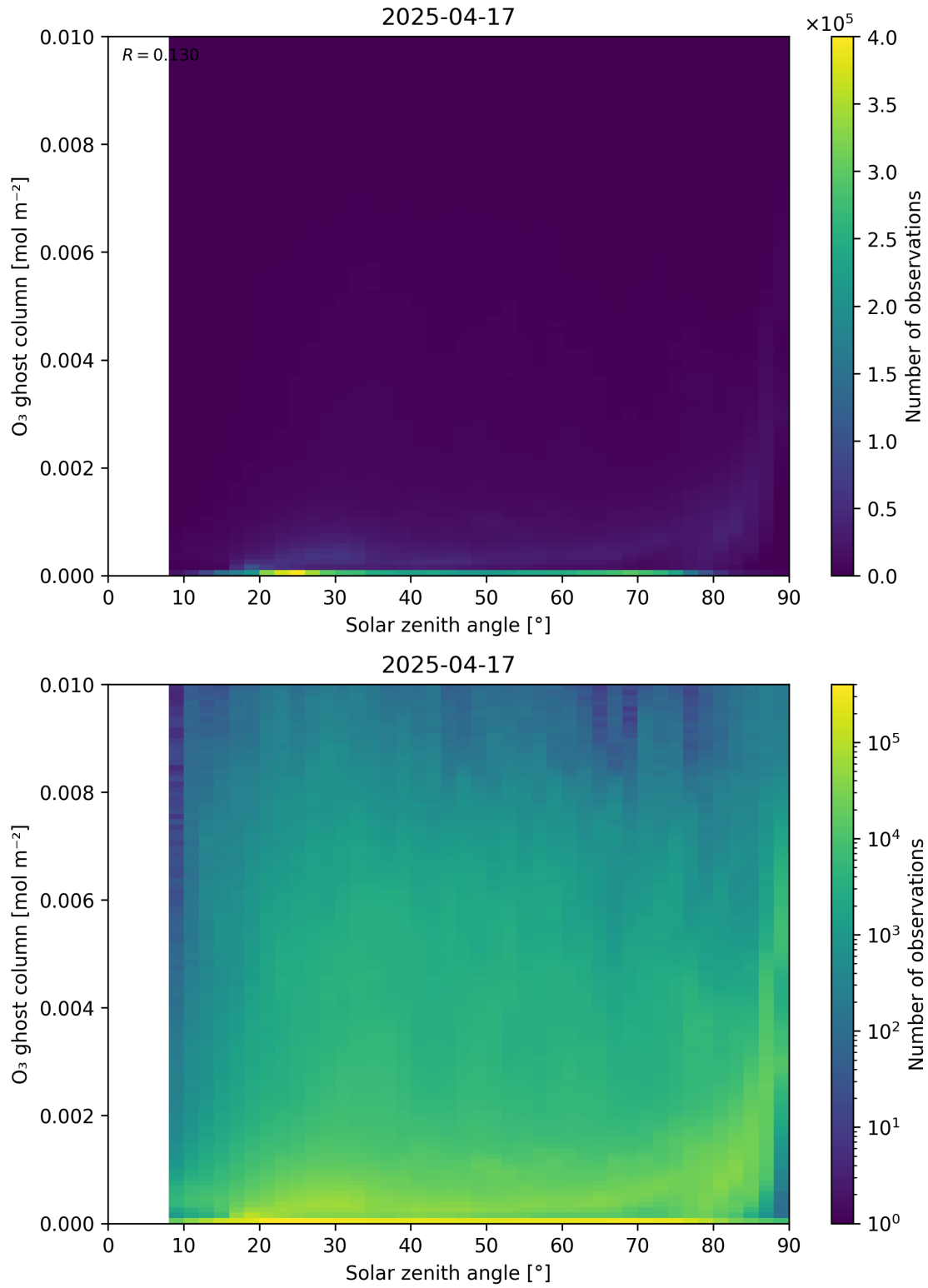
Figure 46: Scatter density plot of “Solar zenith angle” against “O 3 ghost column” for 2025-04-16 to 2025-04-18.
