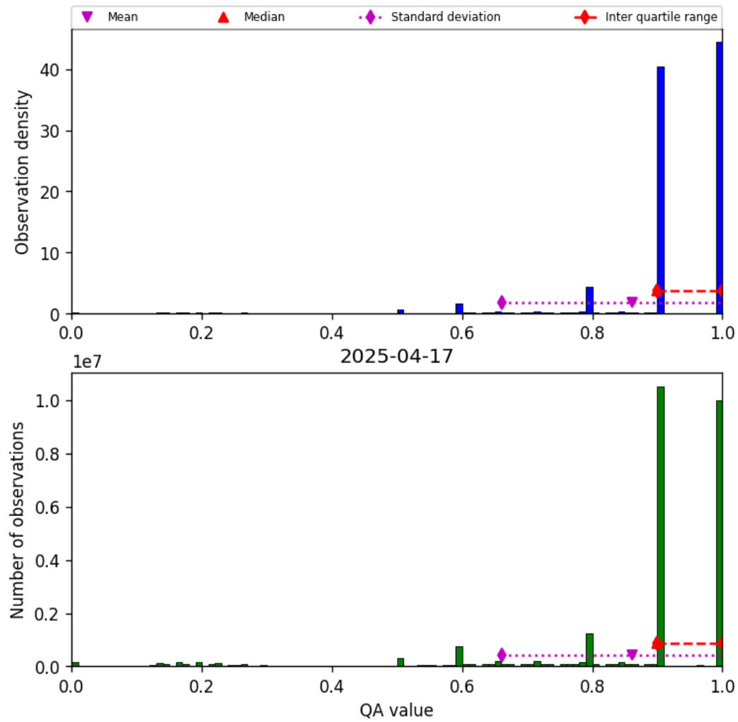
Figure 20: Histogram of “QA value” for 2025-04-16 to 2025-04-18
