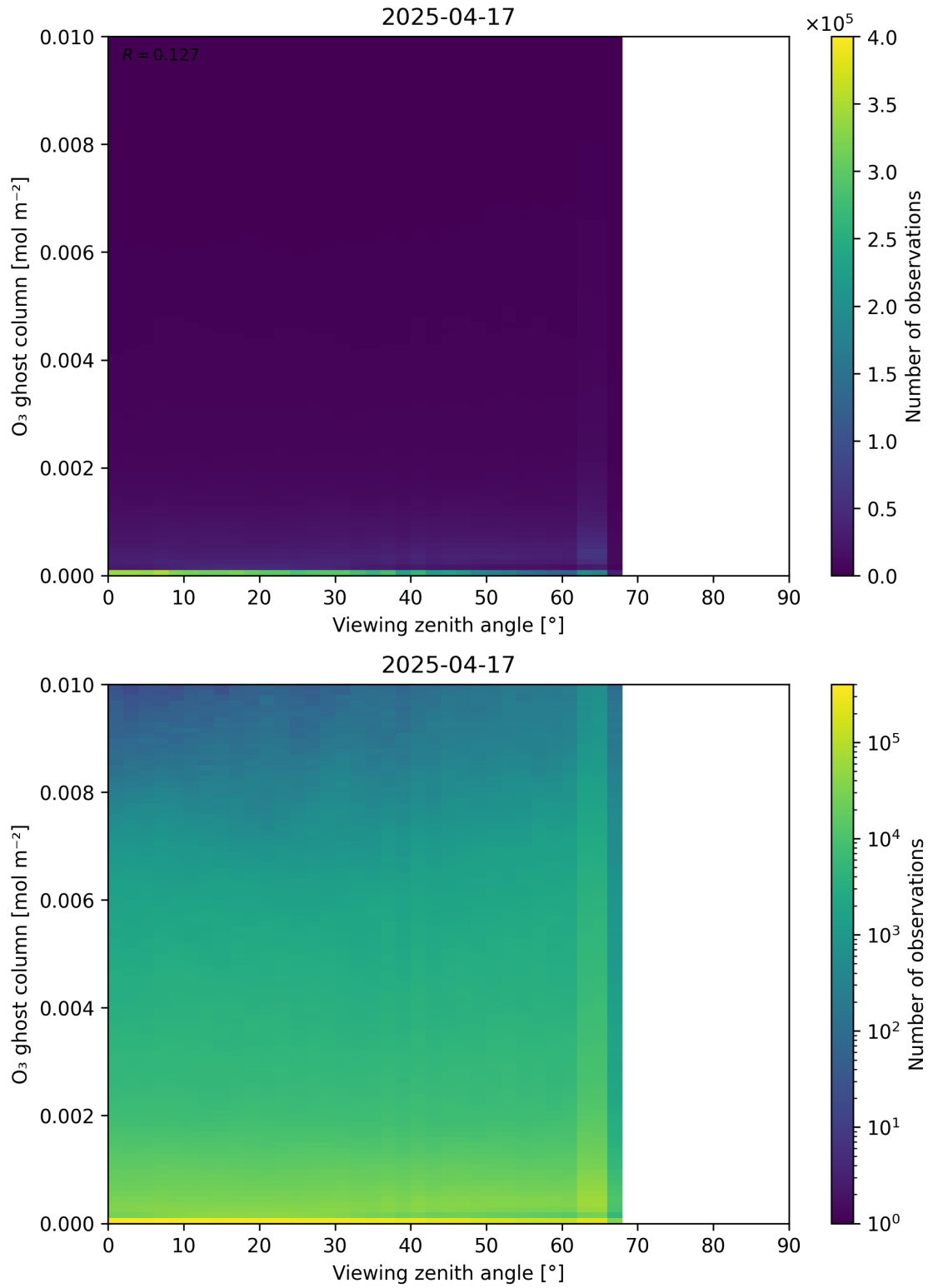
Figure 51: Scatter density plot of “Viewing zenith angle” against “O 3 ghost column” for 2025-04-16 to 2025-04-18.
