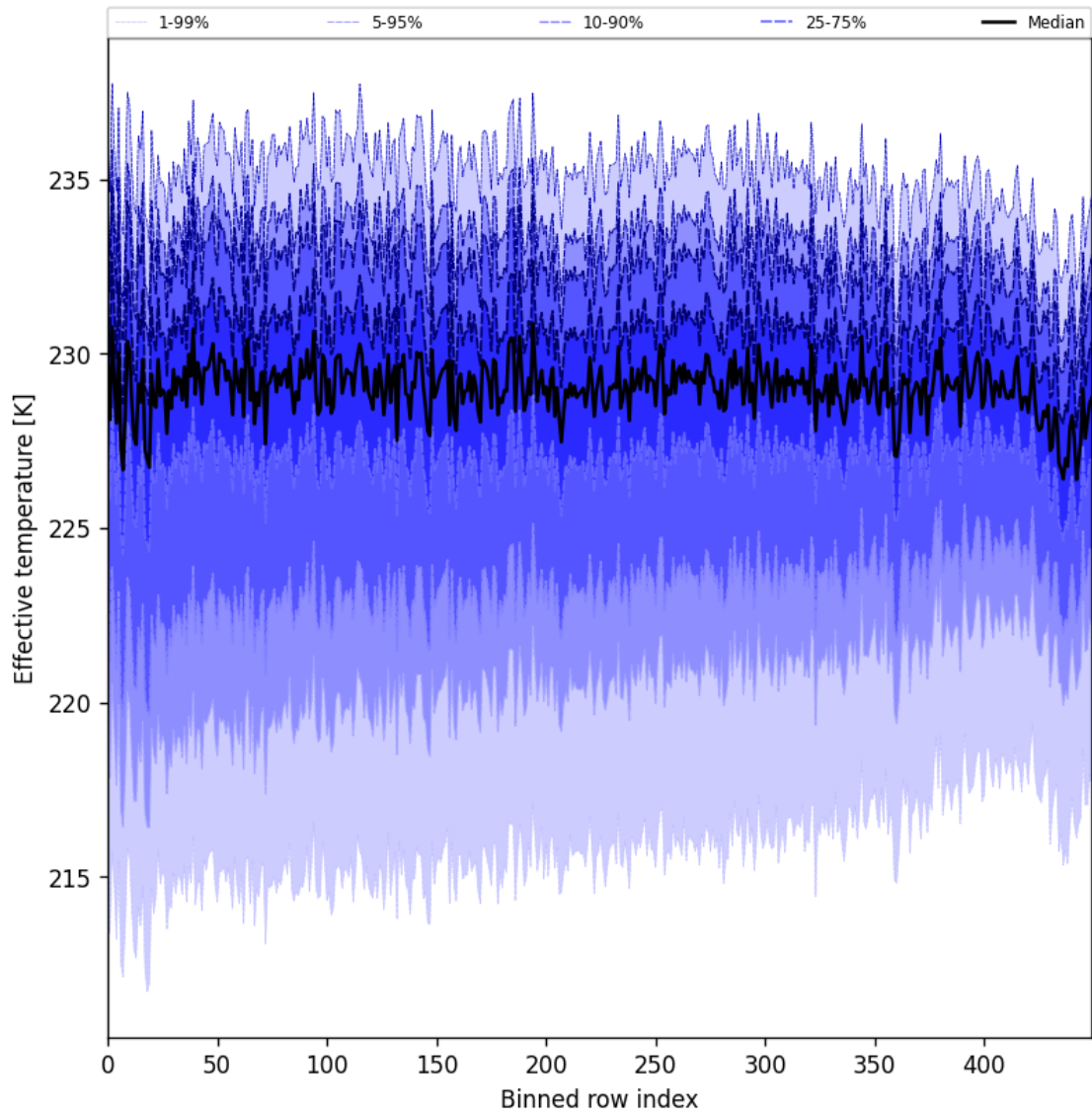
Figure 31: Along track statistics of “Effective temperature” for 2025-04-16 to 2025-04-18
