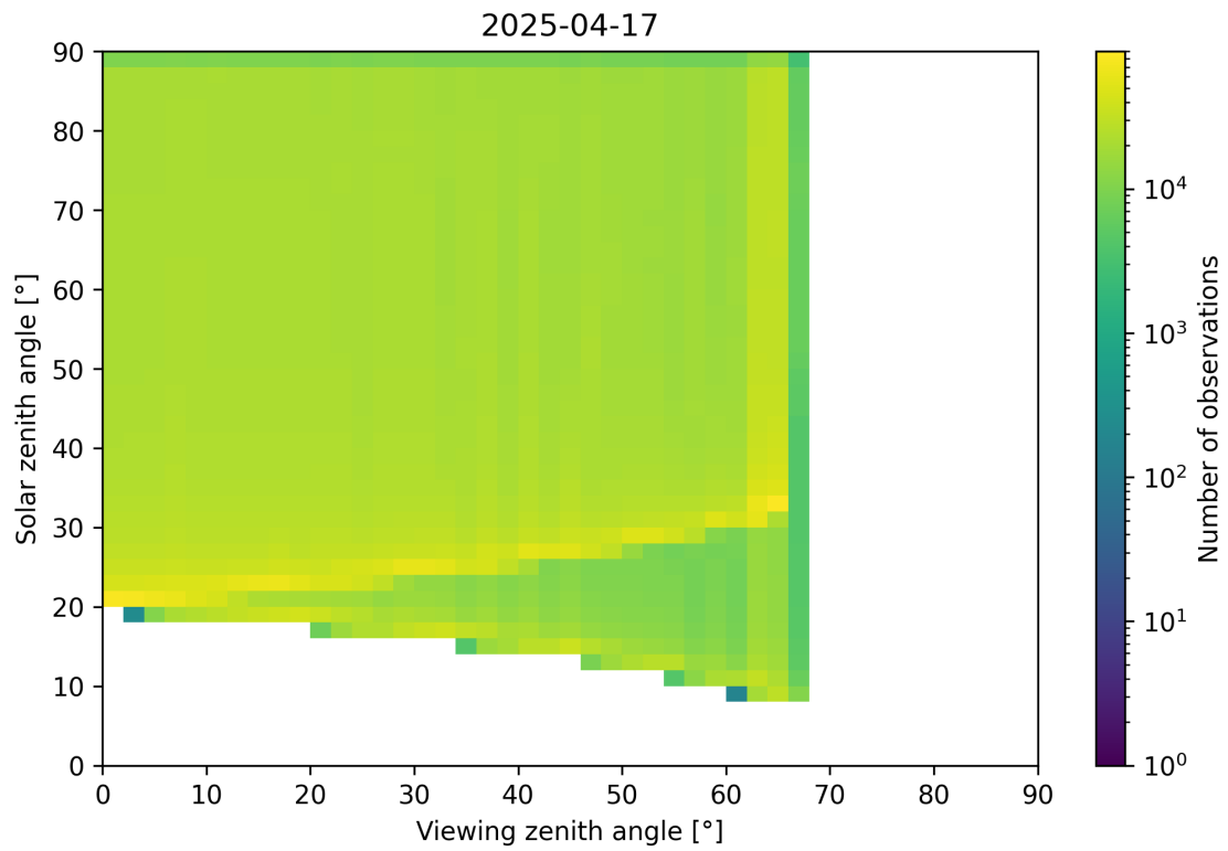
Figure 54: Scatter density plot of “Viewing zenith angle” against “Solar zenith angle” for 2025-04-16 to 2025-04-18.
