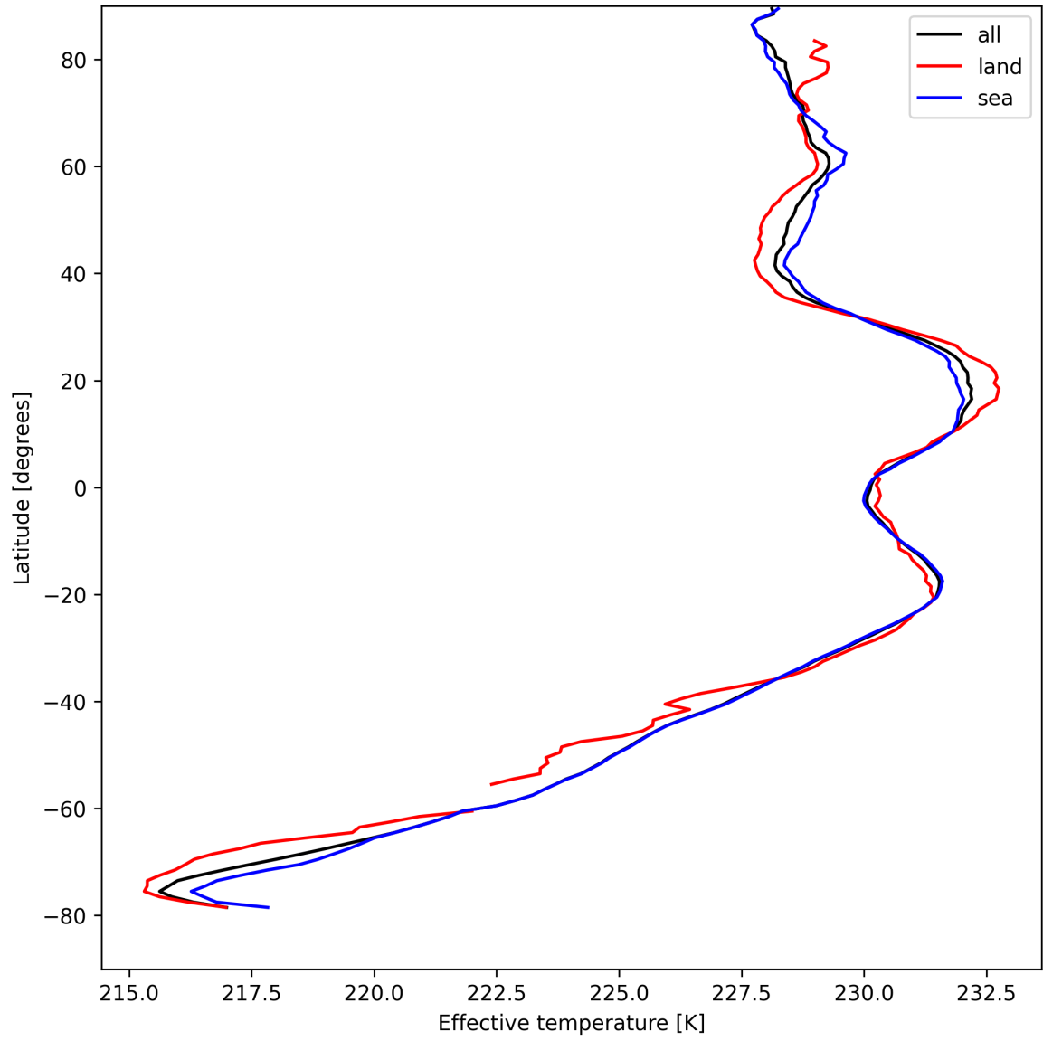
Figure 17: Zonal average of “Effective temperature” for 2025-04-16 to 2025-04-18.
