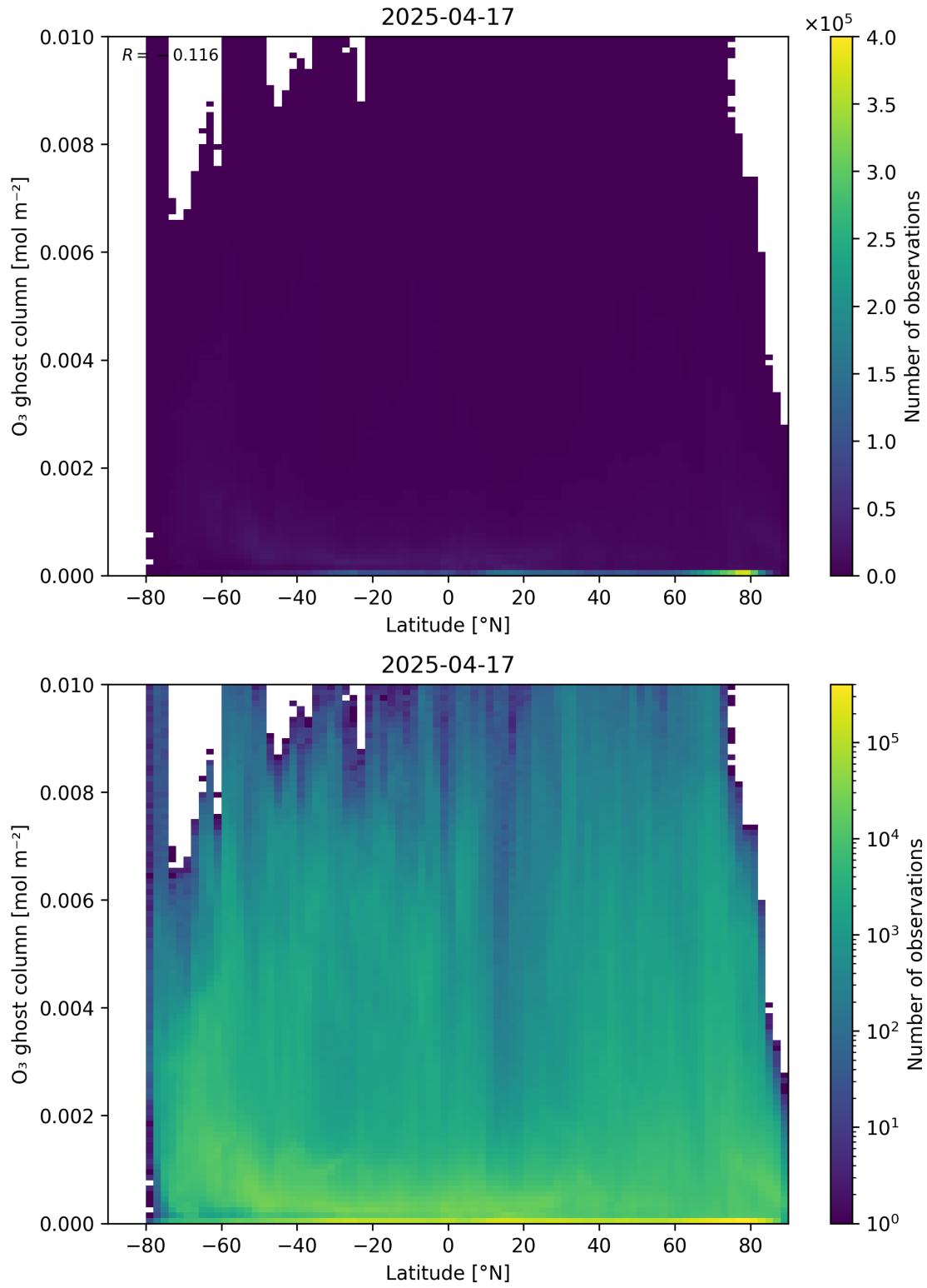
Figure 35: Scatter density plot of “Latitude” against “O 3 ghost column” for 2025-04-16 to 2025-04-18.
