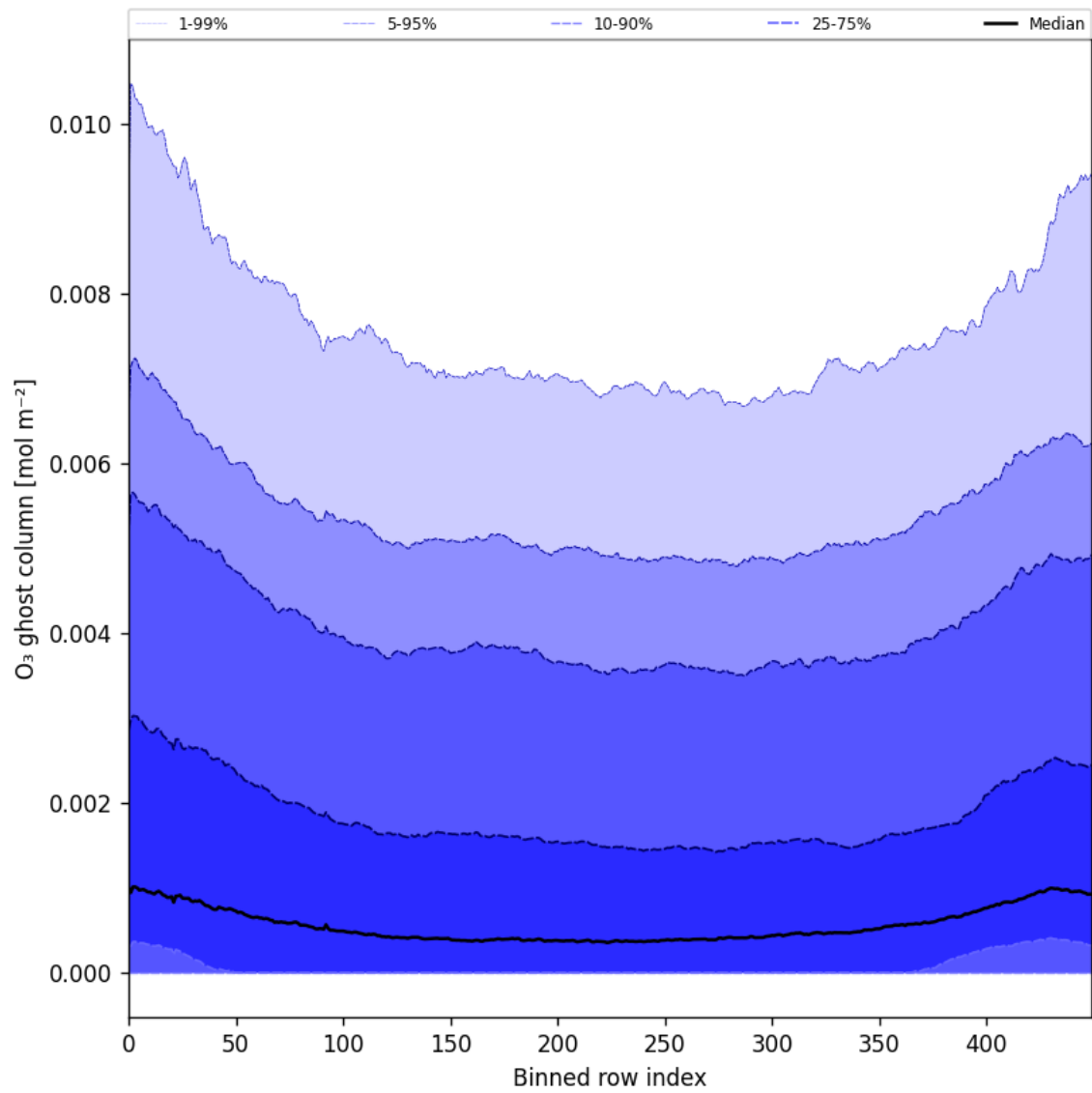
Figure 32: Along track statistics of “O 3 ghost column” for 2025-04-16 to 2025-04-18
