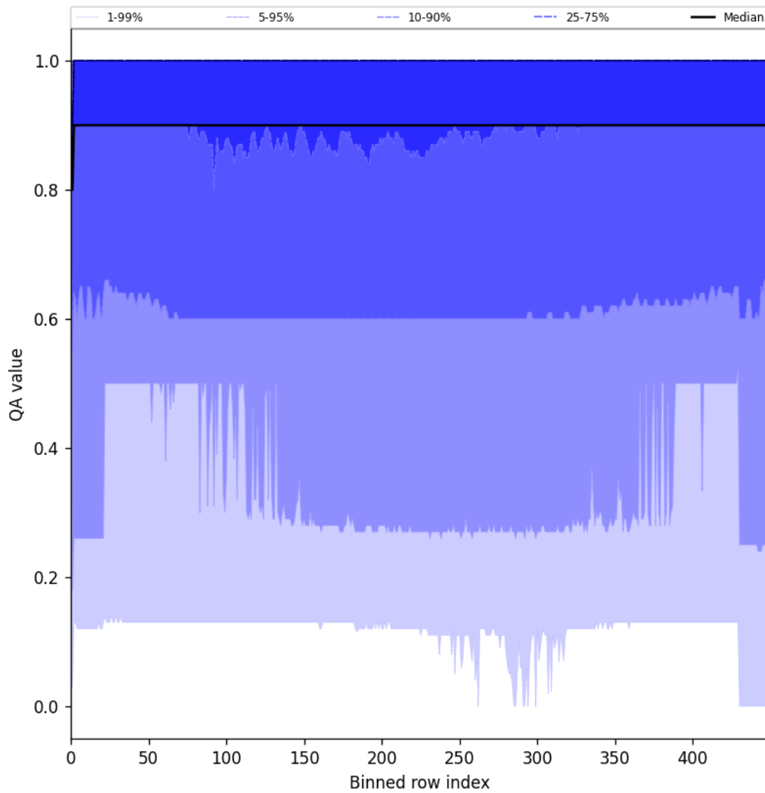
Figure 27: Along track statistics of “QA value” for 2025-04-16 to 2025-04-18
