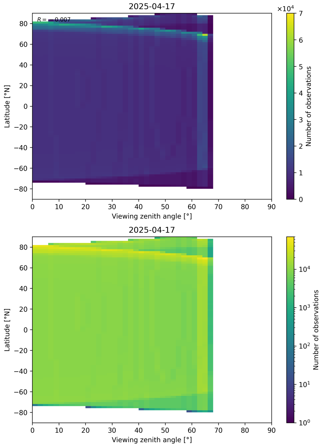
Figure 49: Scatter density plot of “Viewing zenith angle” against “Latitude” for 2025-04-16 to 2025-04-18.
