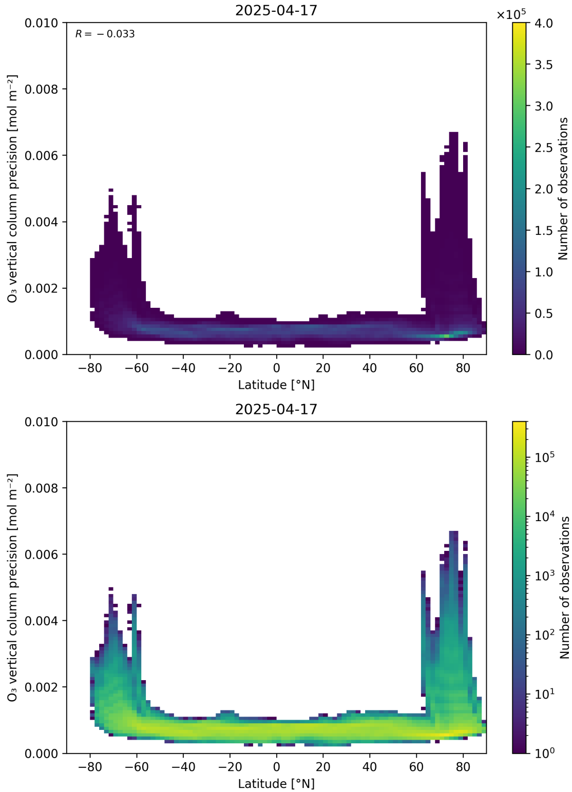
Figure 37: Scatter density plot of “Latitude” against “O 3 vertical column precision” for 2025-04-16 to 2025-04-18.
