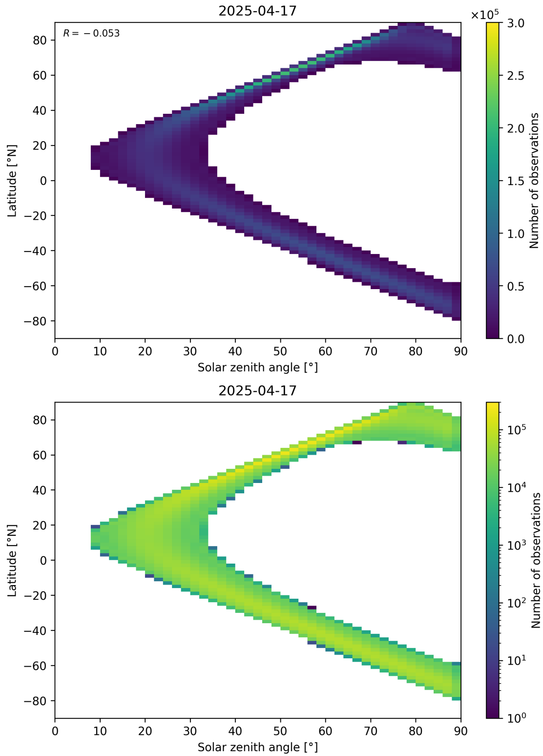
Figure 44: Scatter density plot of “Solar zenith angle” against “Latitude” for 2025-04-16 to 2025-04-18.
