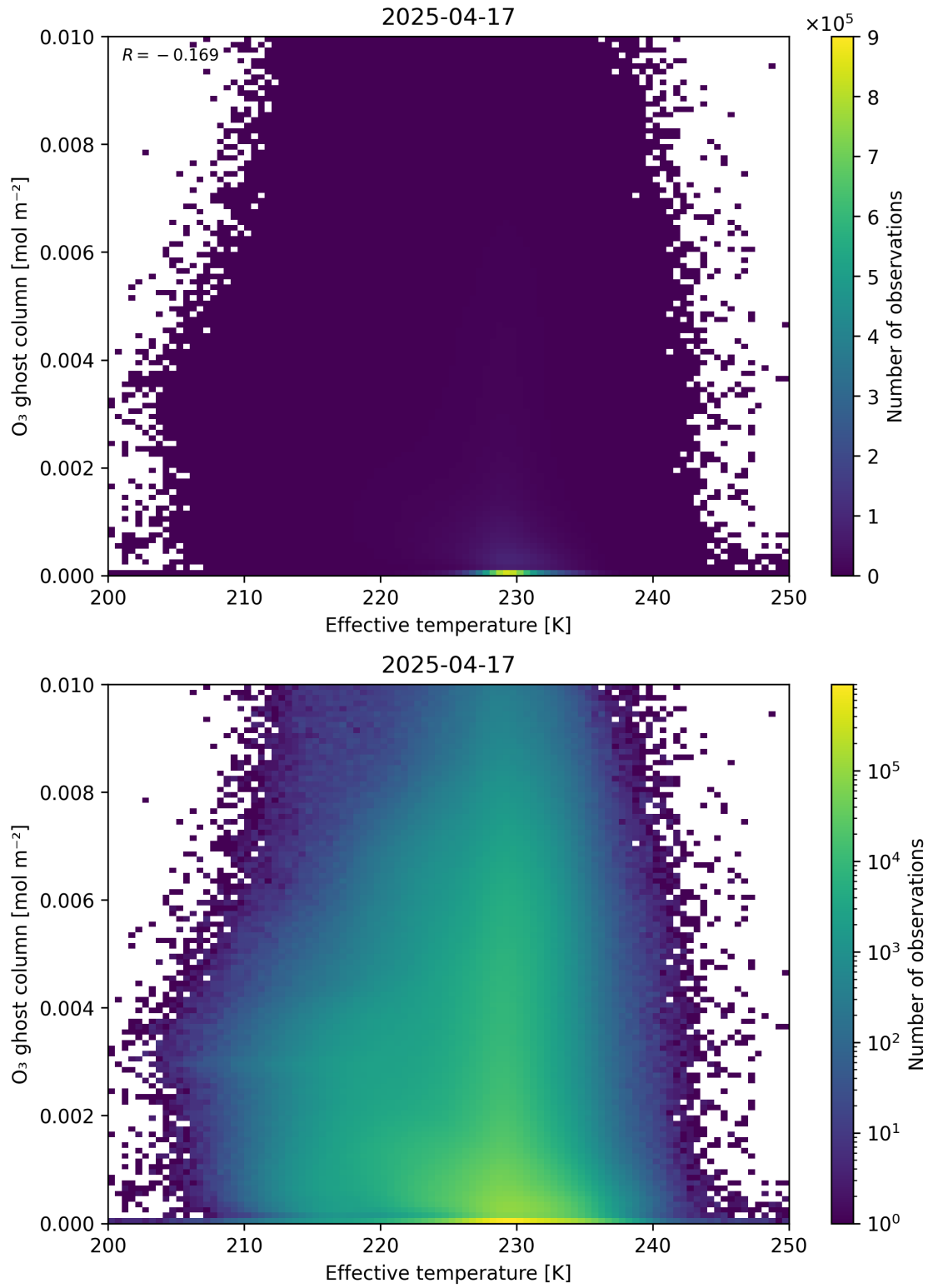
Figure 38: Scatter density plot of “Effective temperature” against “O 3 ghost column” for 2025-04-16 to 2025-04-18.
