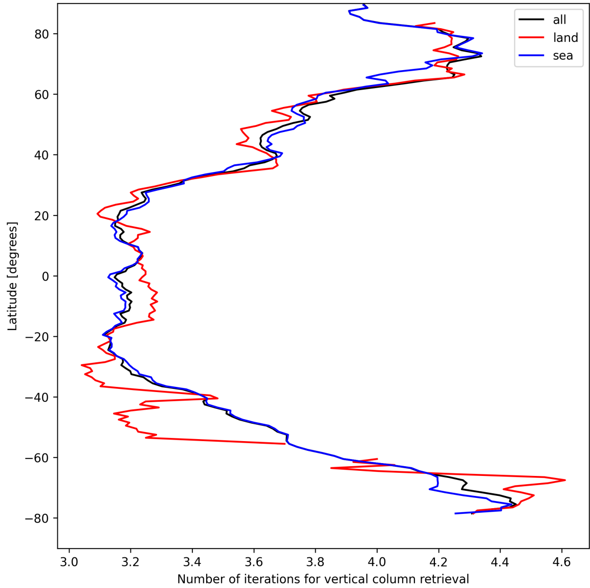
Figure 19: Zonal average of “Number of iterations for vertical column retrieval” for 2025-04-16 to 2025-04-18.
