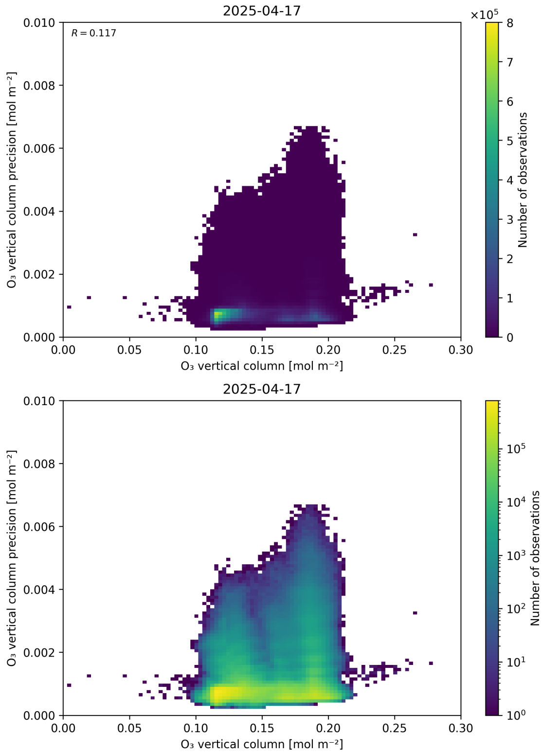
Figure 41: Scatter density plot of “O 3 vertical column” against “O 3 vertical column precision” for 2025-04-16 to 2025-04-18.
