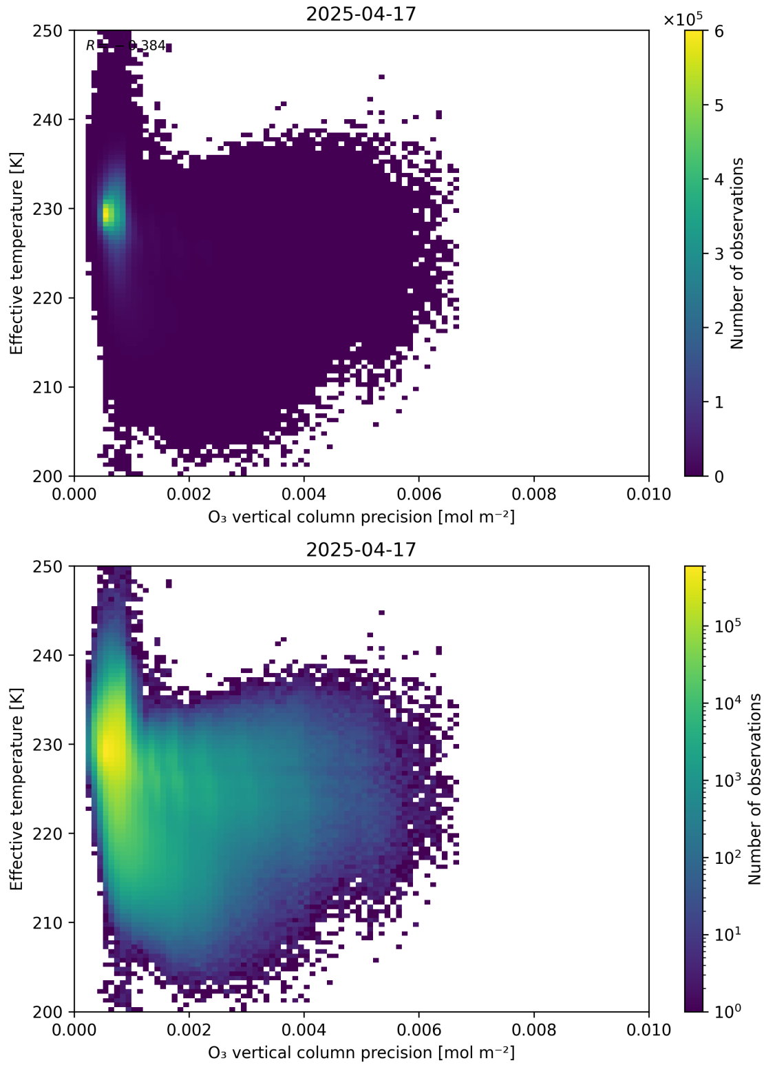
Figure 42: Scatter density plot of “O 3 vertical column precision” against “Effective temperature” for 2025-04-16 to 2025-04-18.
