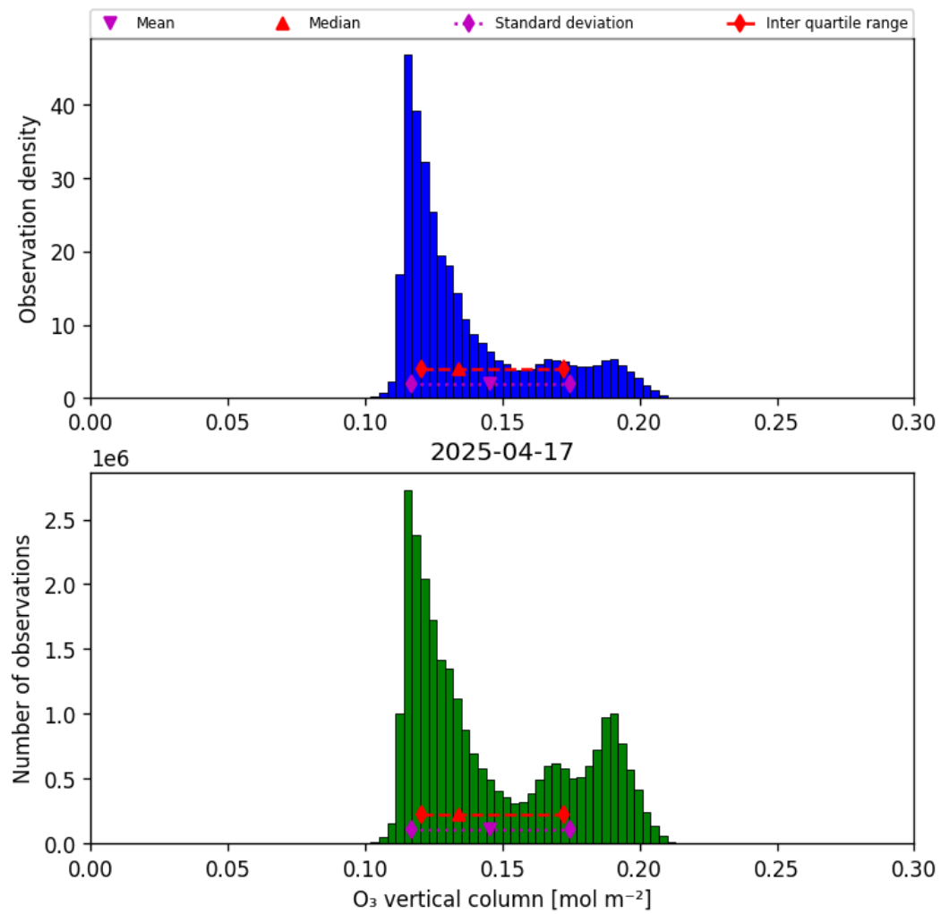
Figure 21: Histogram of “O 3 vertical column” for 2025-04-16 to 2025-04-18
