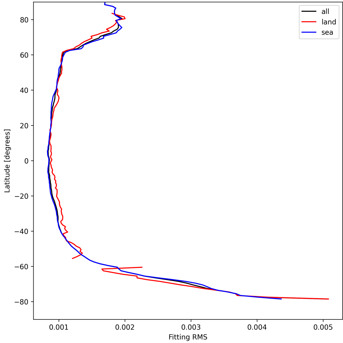
Figure 16: Zonal average of “Fitting RMS” for 2025-04-16 to 2025-04-18.
