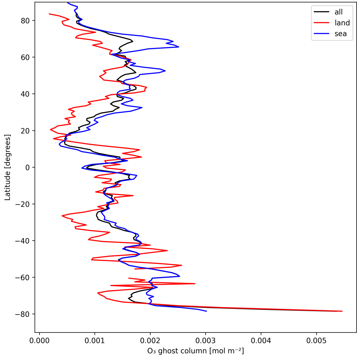
Figure 18: Zonal average of “O 3 ghost column” for 2025-04-16 to 2025-04-18.
