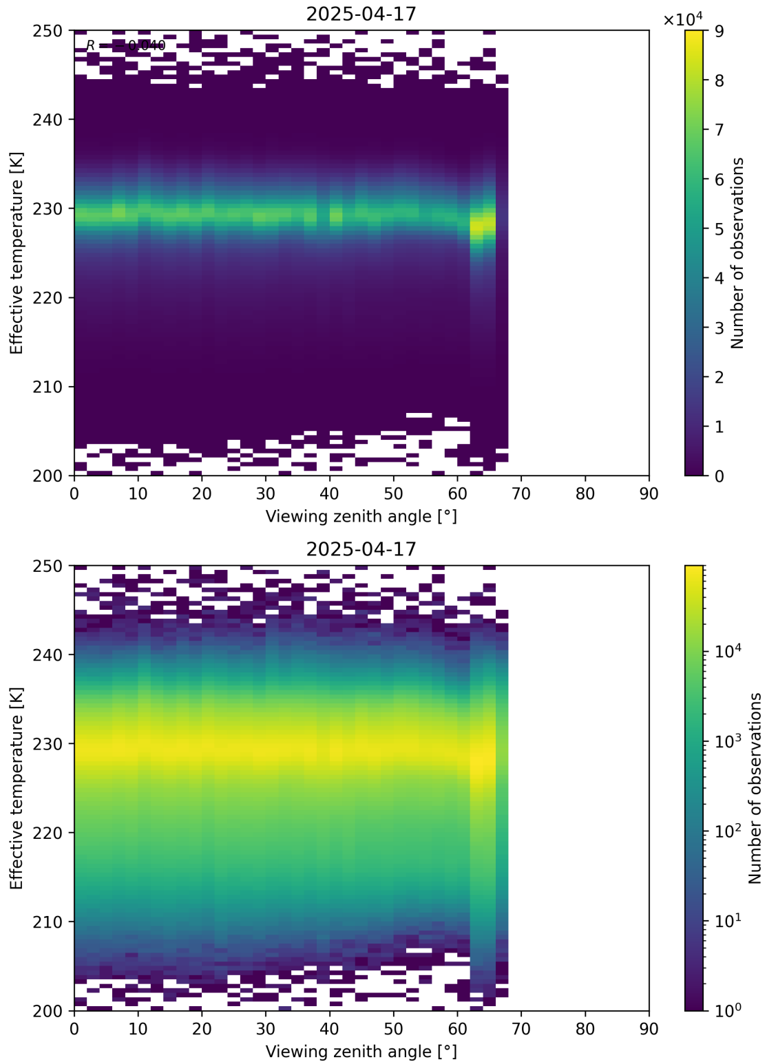
Figure 50: Scatter density plot of “Viewing zenith angle” against “Effective temperature” for 2025-04-16 to 2025-04-18.
