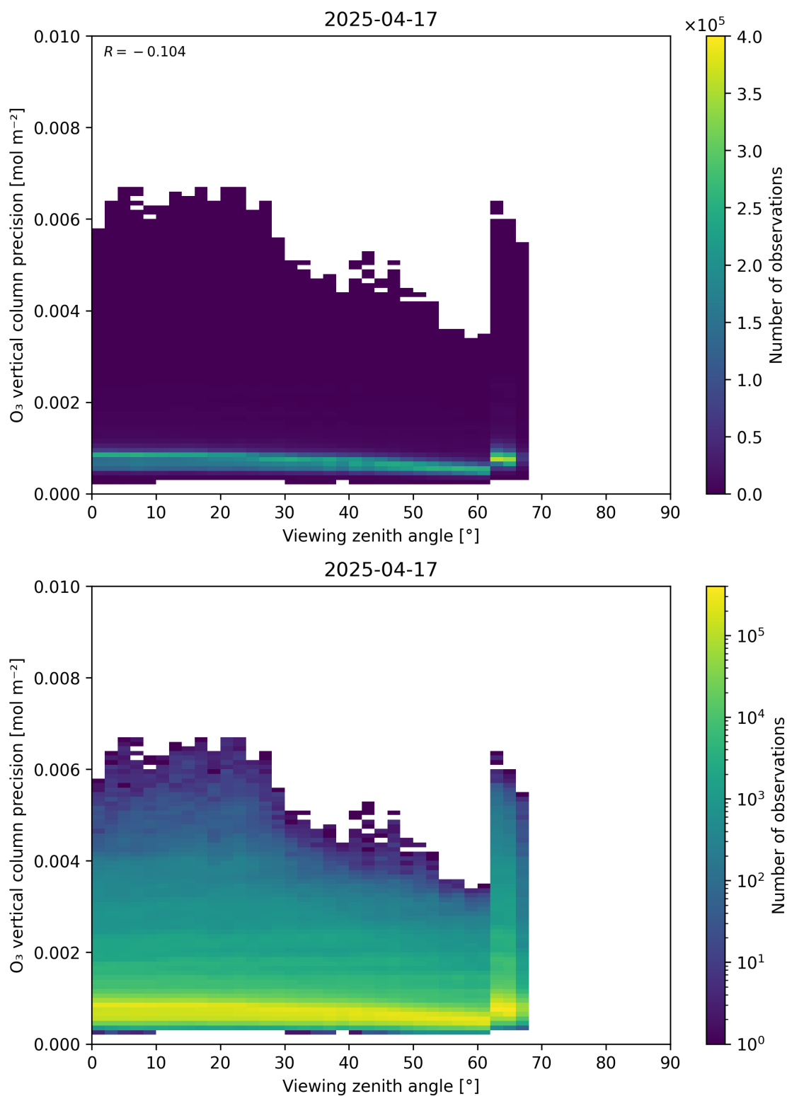
Figure 53: Scatter density plot of “Viewing zenith angle” against “O 3 vertical column precision” for 2025-04-16 to 2025-04-18.
