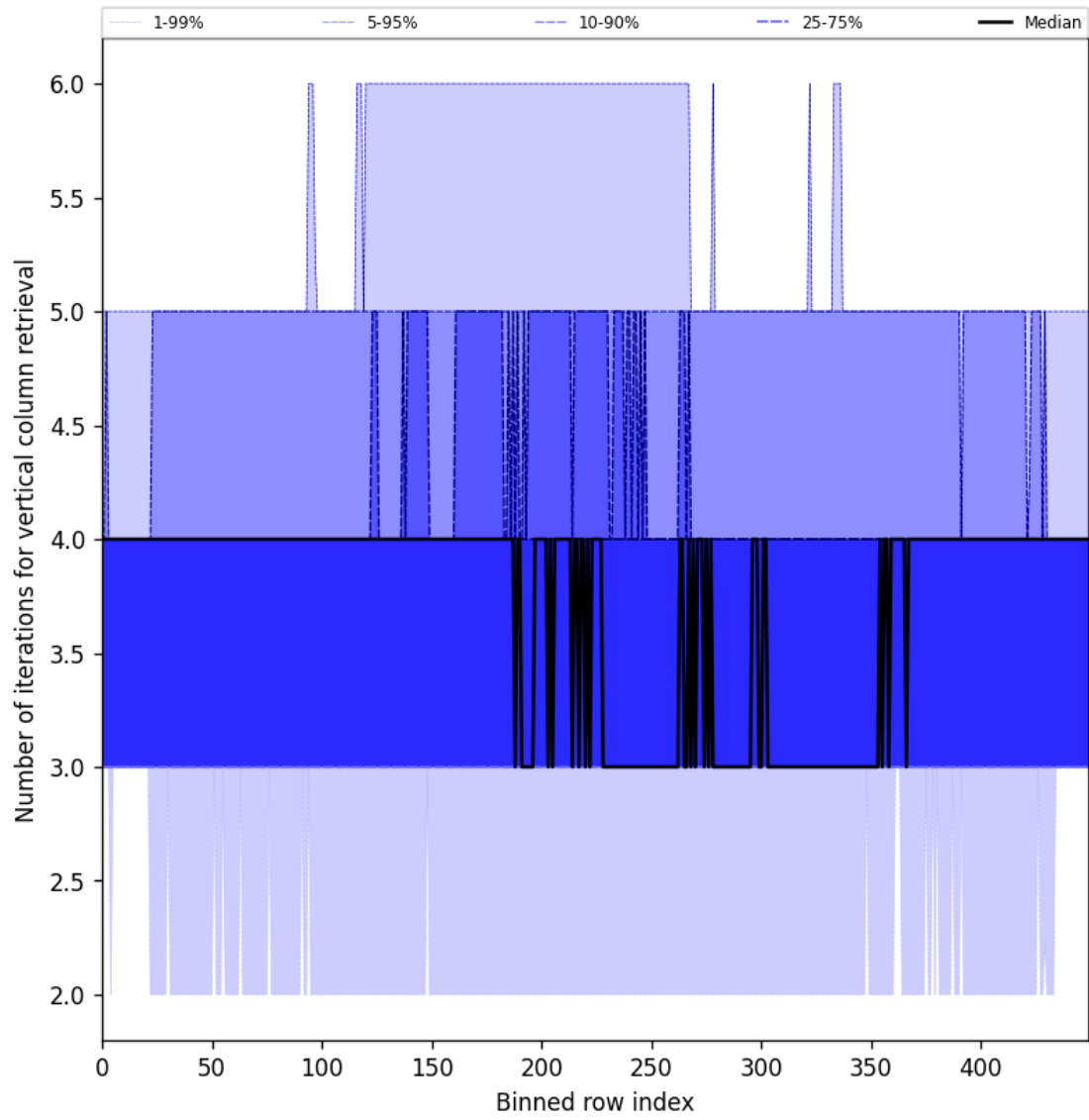
Figure 33: Along track statistics of “Number of iterations for vertical column retrieval” for 2025-04-16 to 2025-04-18
