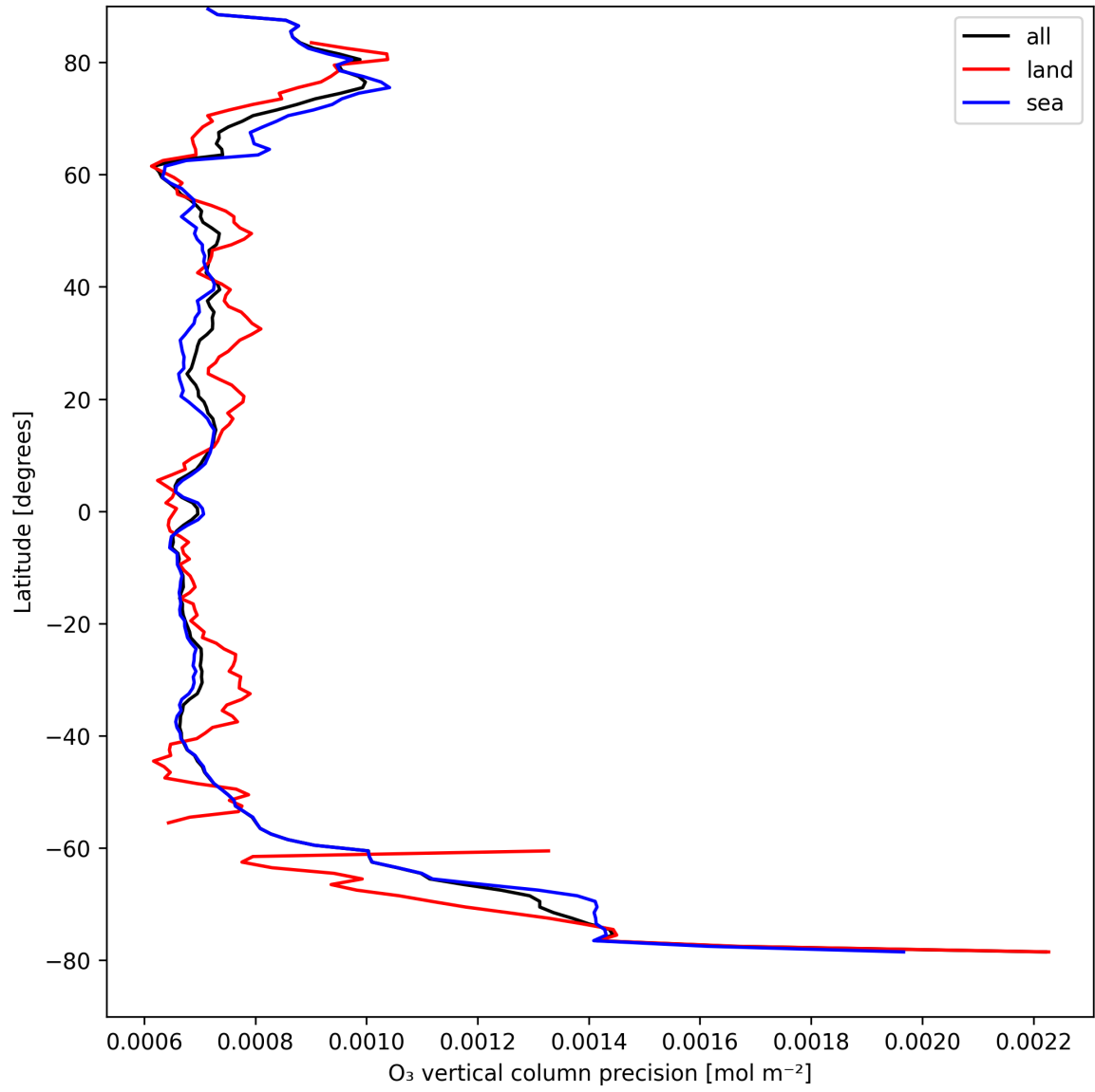
Figure 15: Zonal average of "O 3 vertical column precision" for 2025-04-16 to 2025-04-18.
