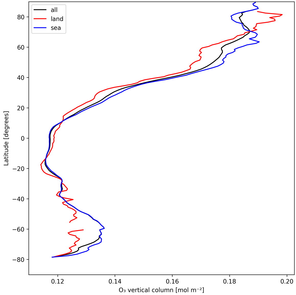
Figure 14: Zonal average of “O 3 vertical column” for 2025-04-16 to 2025-04-18.
