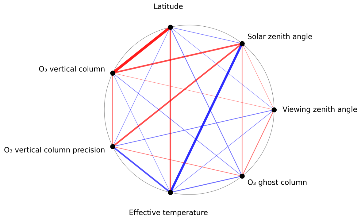
Figure 1: Map of correlation graph for 2025-04-16 to 2025-04-18.
