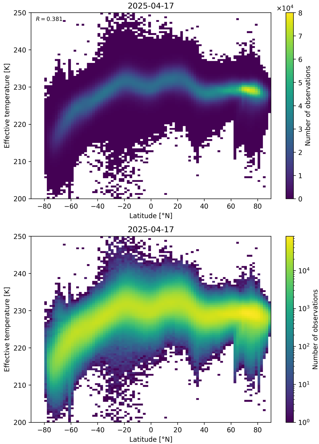
Figure 34: Scatter density plot of “Latitude” against “Effective temperature” for 2025-04-16 to 2025-04-18.
