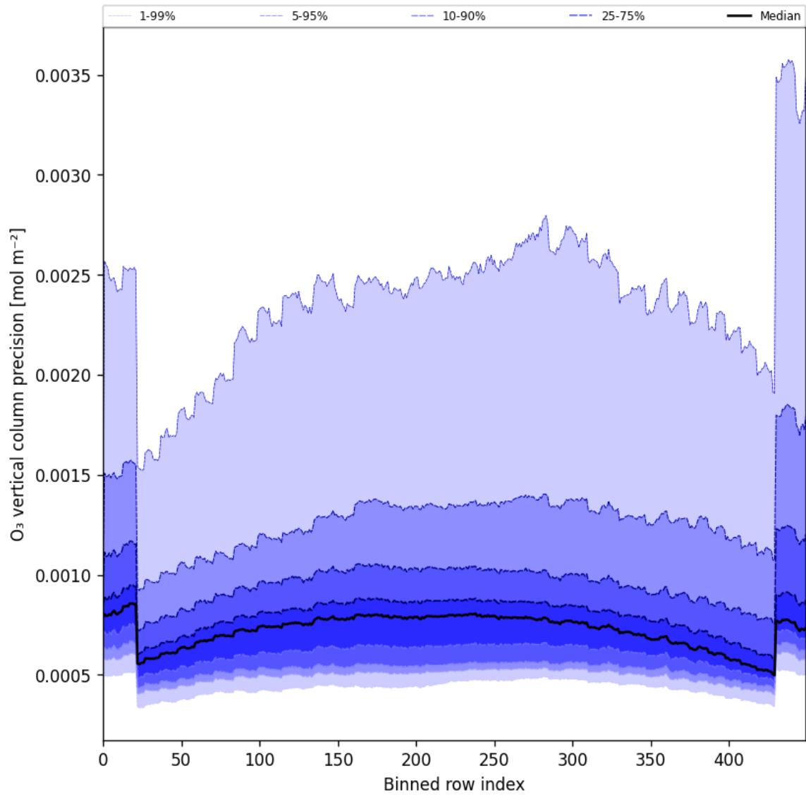
Figure 29: Along track statistics of “O 3 vertical column precision” for 2025-04-16 to 2025-04-18
