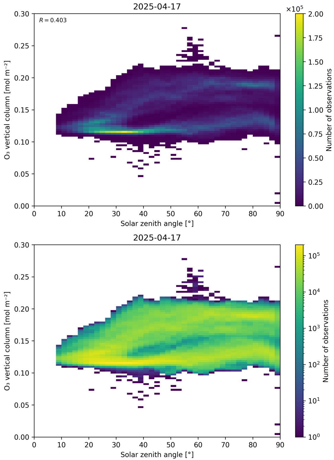
Figure 47: Scatter density plot of “Solar zenith angle” against “O 3 vertical column” for 2025-04-16 to 2025-04-18.
