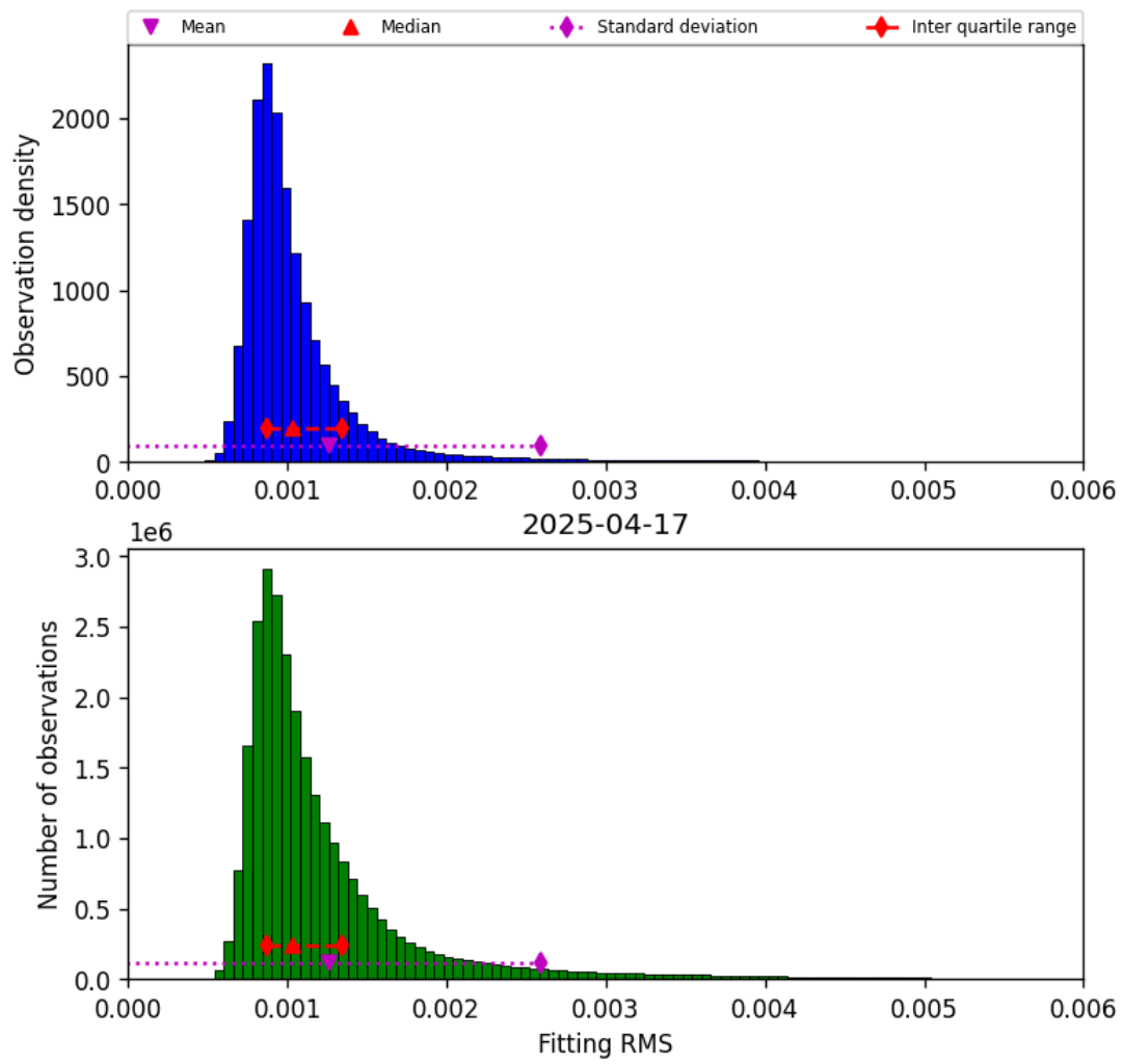
Figure 23: Histogram of “Fitting RMS” for 2025-04-16 to 2025-04-18
