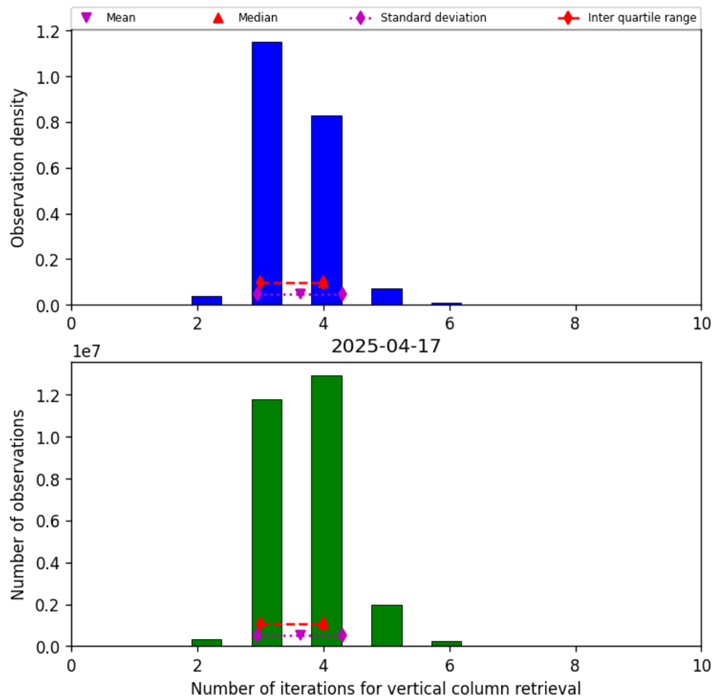
Figure 26: Histogram of “Number of iterations for vertical column retrieval” for 2025-04-16 to 2025-04-18
