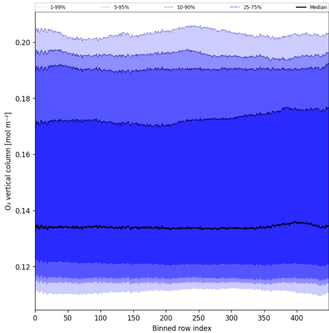
Figure 28: Along track statistics of “O 3 vertical column” for 2025-04-16 to 2025-04-18
