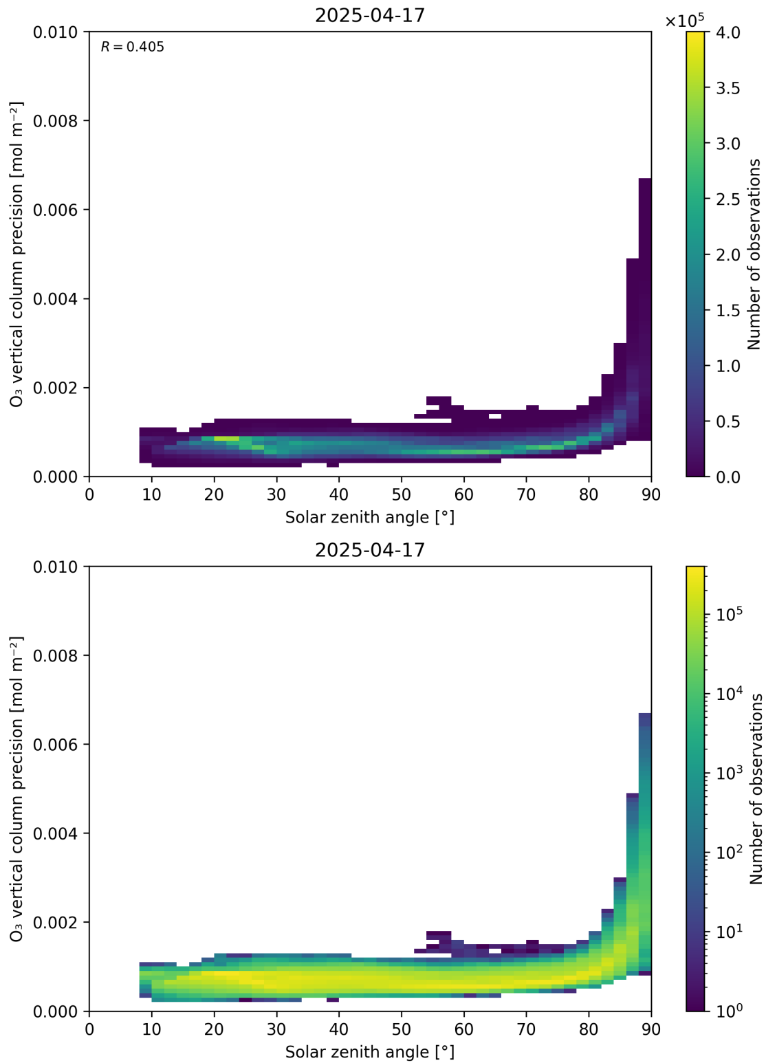
Figure 48: Scatter density plot of “Solar zenith angle” against “O 3 vertical column precision” for 2025-04-16 to 2025-04-18.
