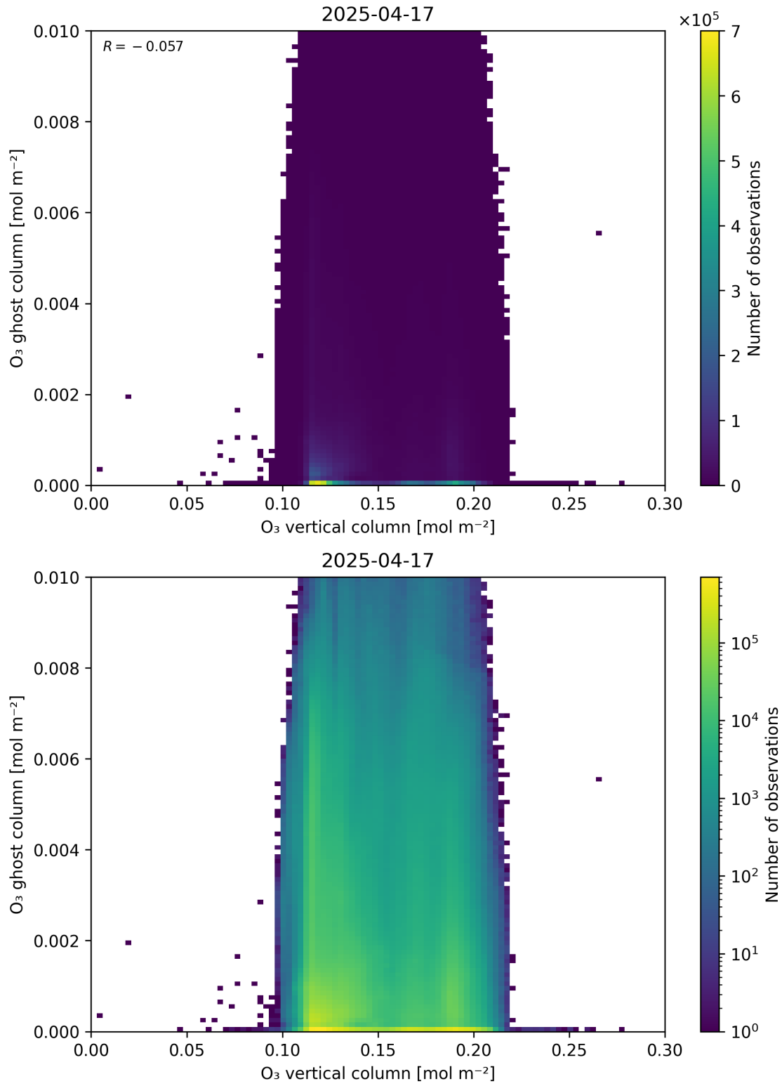
Figure 40: Scatter density plot of “O 3 vertical column” against “O 3 ghost column” for 2025-04-16 to 2025-04-18.
