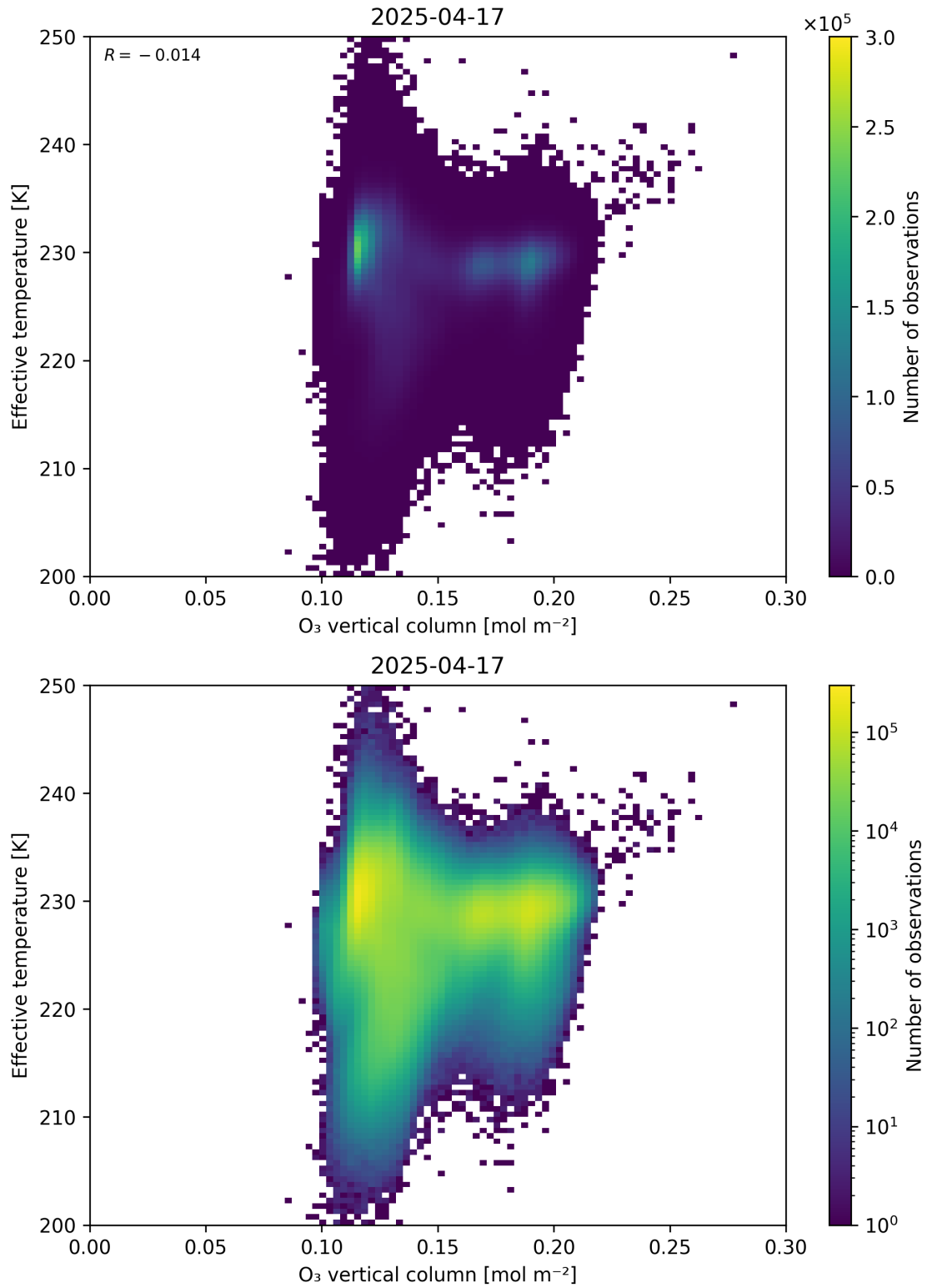
Figure 39: Scatter density plot of “O 3 vertical column” against “Effective temperature” for 2025-04-16 to 2025-04-18.
