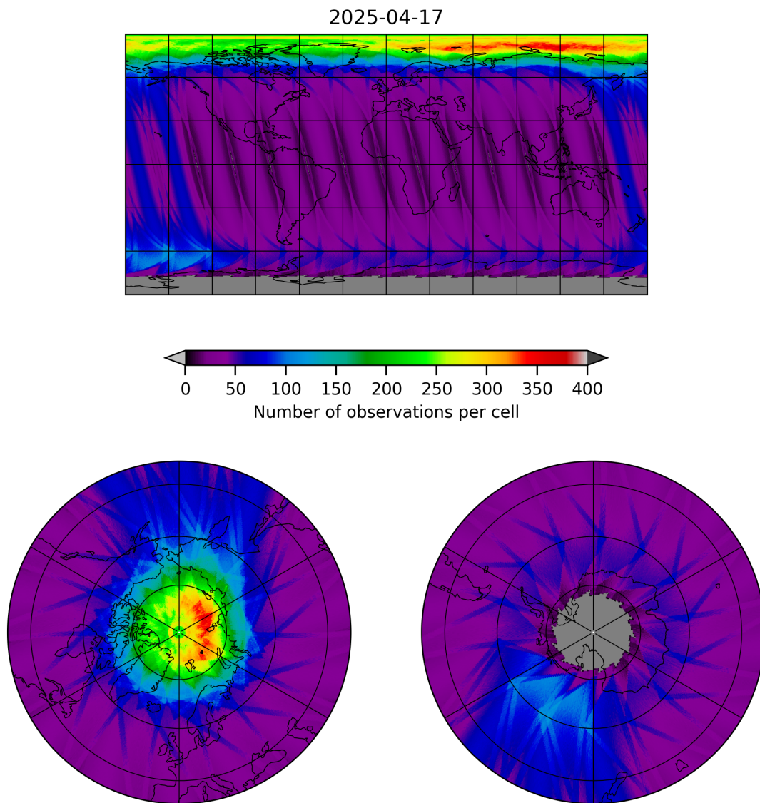
Figure 12: Map of the number of observations for 2025-04-16 to 2025-04-18
