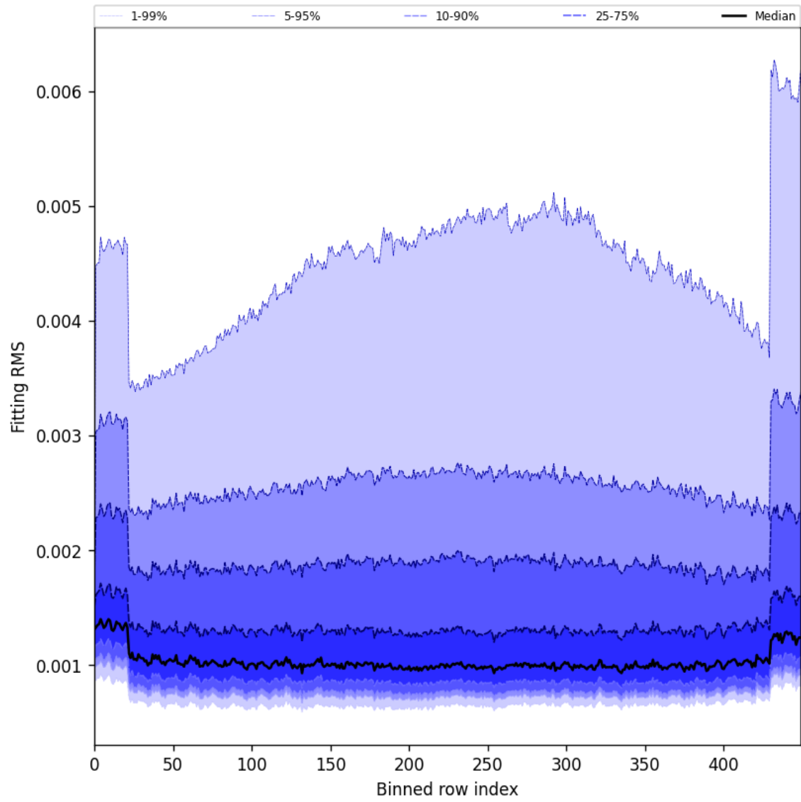
Figure 30: Along track statistics of “Fitting RMS” for 2025-04-16 to 2025-04-18
