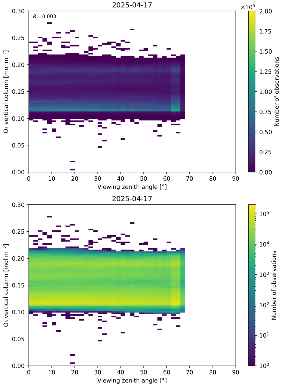
Figure 52: Scatter density plot of “Viewing zenith angle” against “O 3 vertical column” for 2025-04-16 to 2025-04-18.
