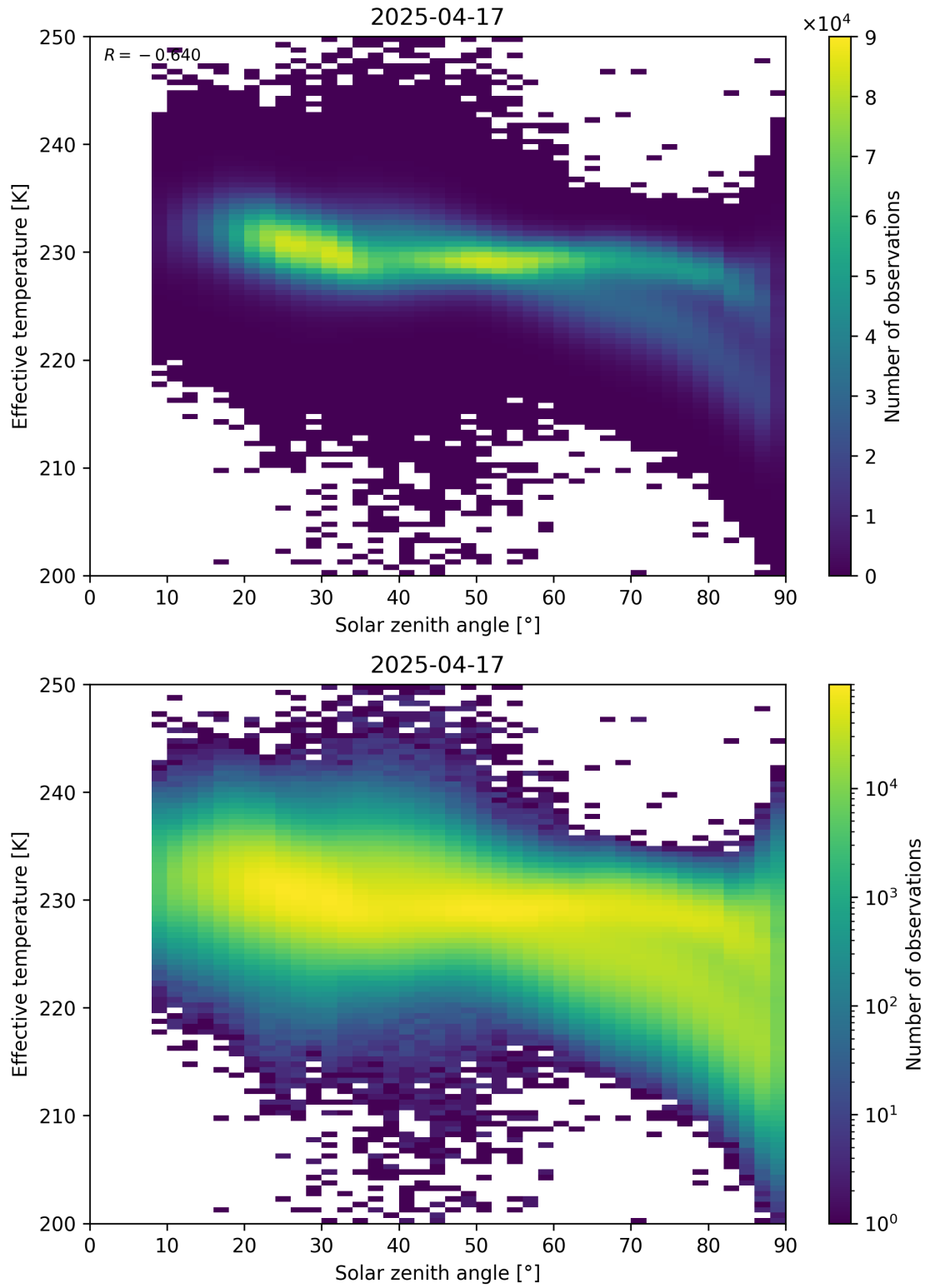
Figure 45: Scatter density plot of “Solar zenith angle” against “Effective temperature” for 2025-04-16 to 2025-04-18.
