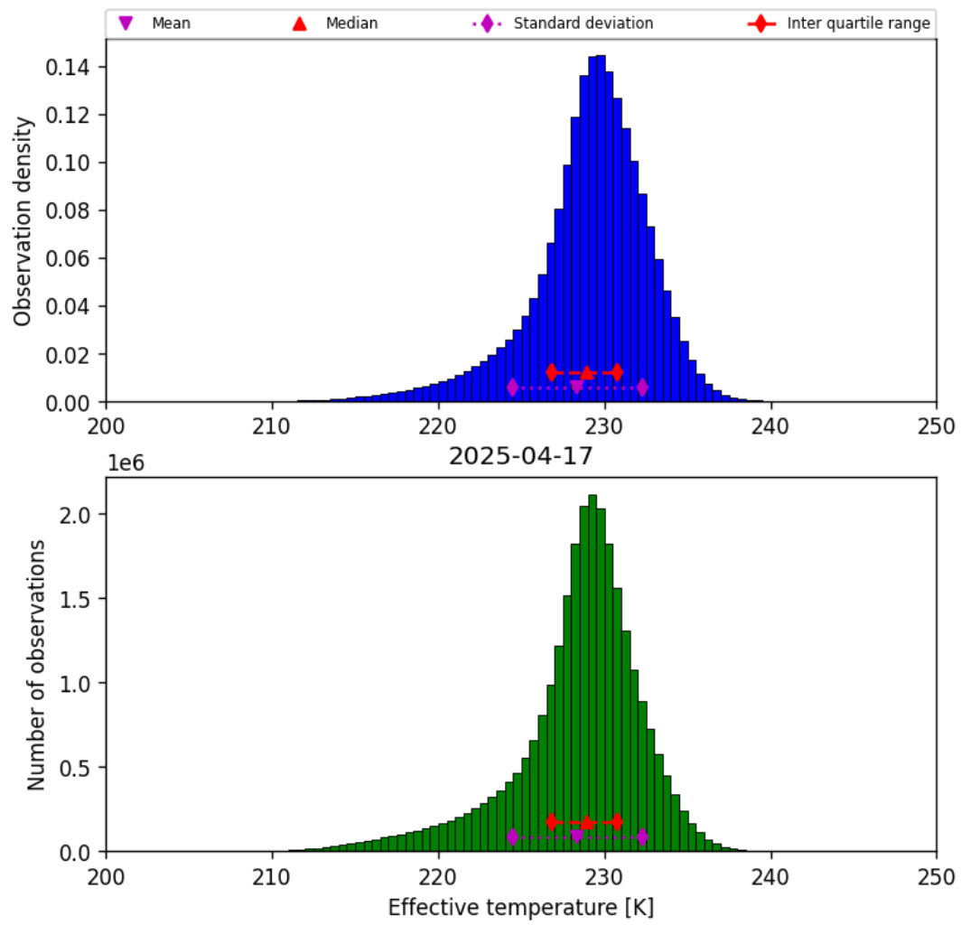
Figure 24: Histogram of “Effective temperature” for 2025-04-16 to 2025-04-18
