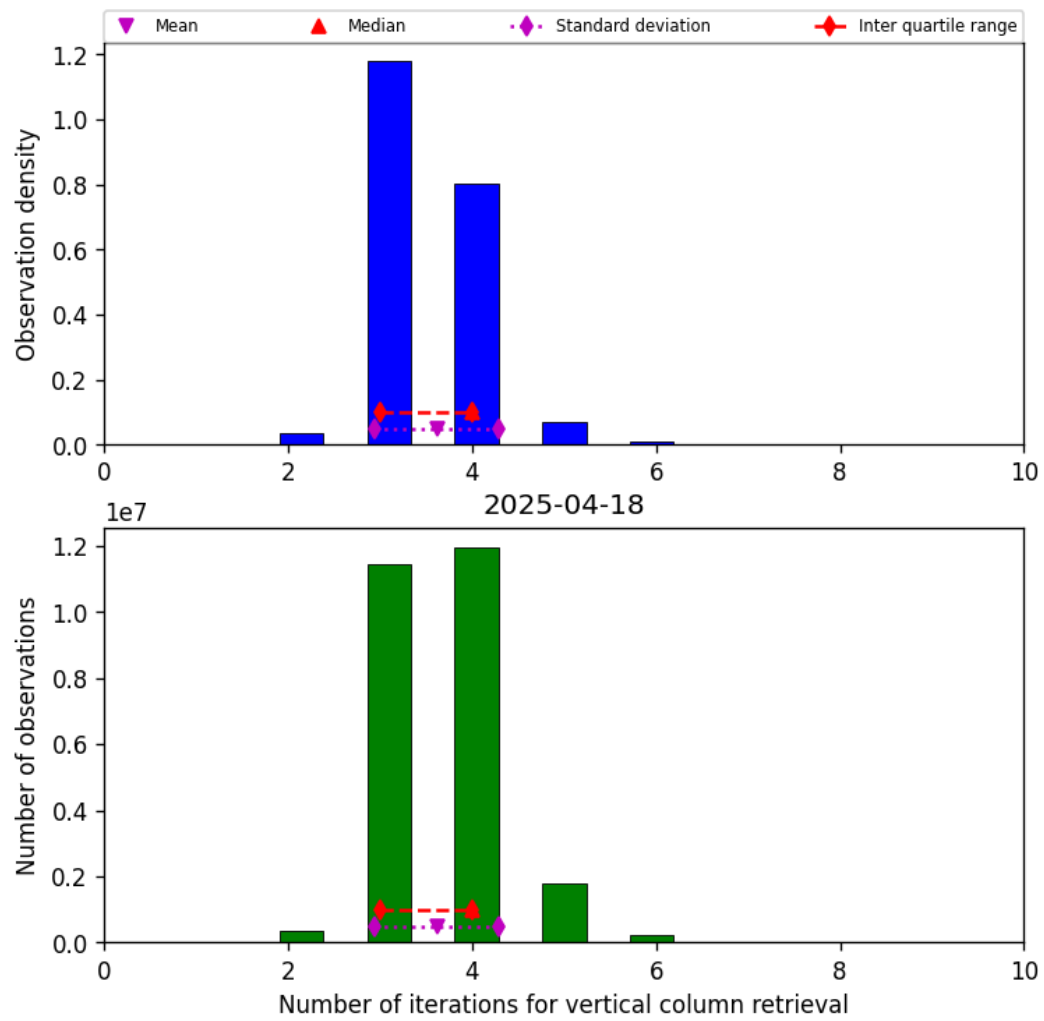
Figure 26: Histogram of “Number of iterations for vertical column retrieval” for 2025-04-18 to 2025-04-19
