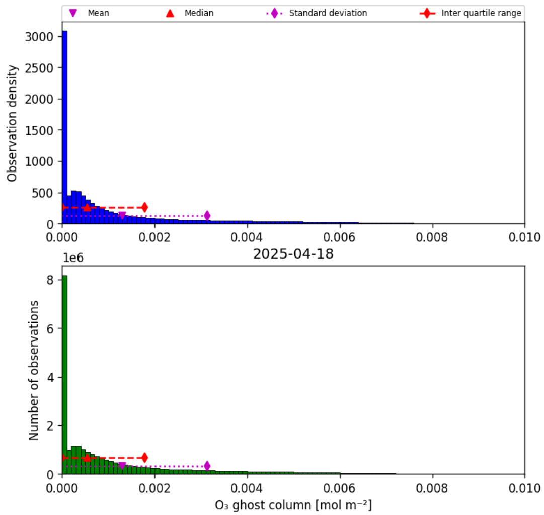
Figure 25: Histogram of “O 3 ghost column” for 2025-04-18 to 2025-04-19
