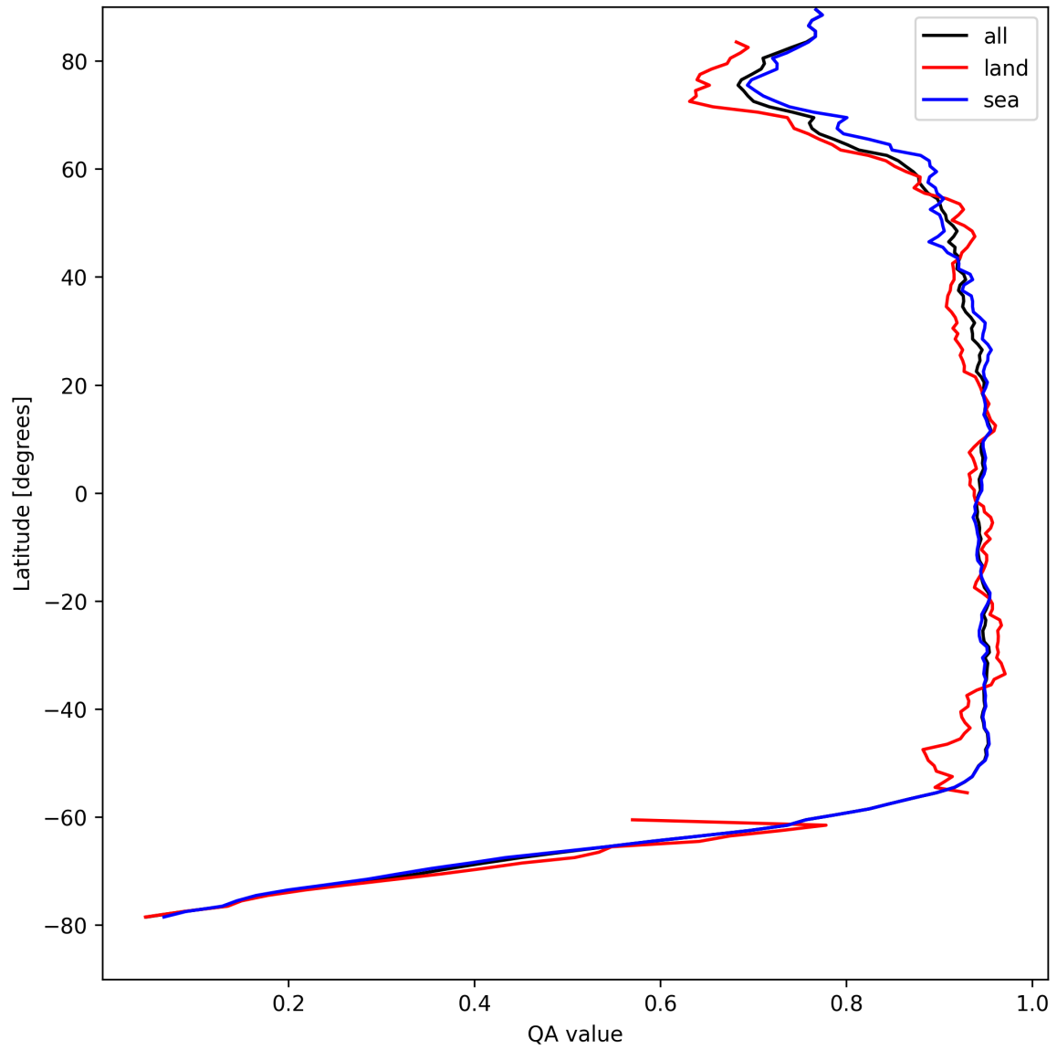
Figure 13: Zonal average of “QA value” for 2025-04-18 to 2025-04-19.
