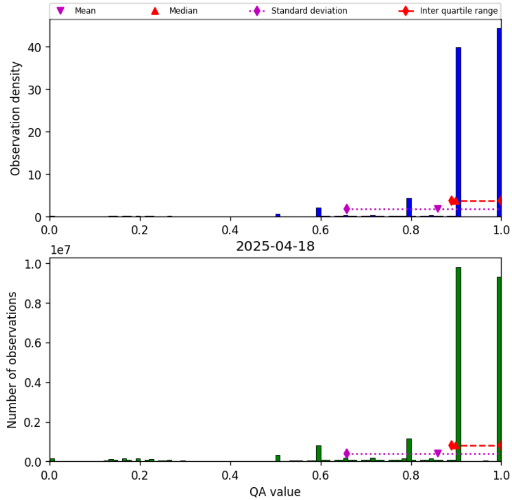
Figure 20: Histogram of “QA value” for 2025-04-18 to 2025-04-19
