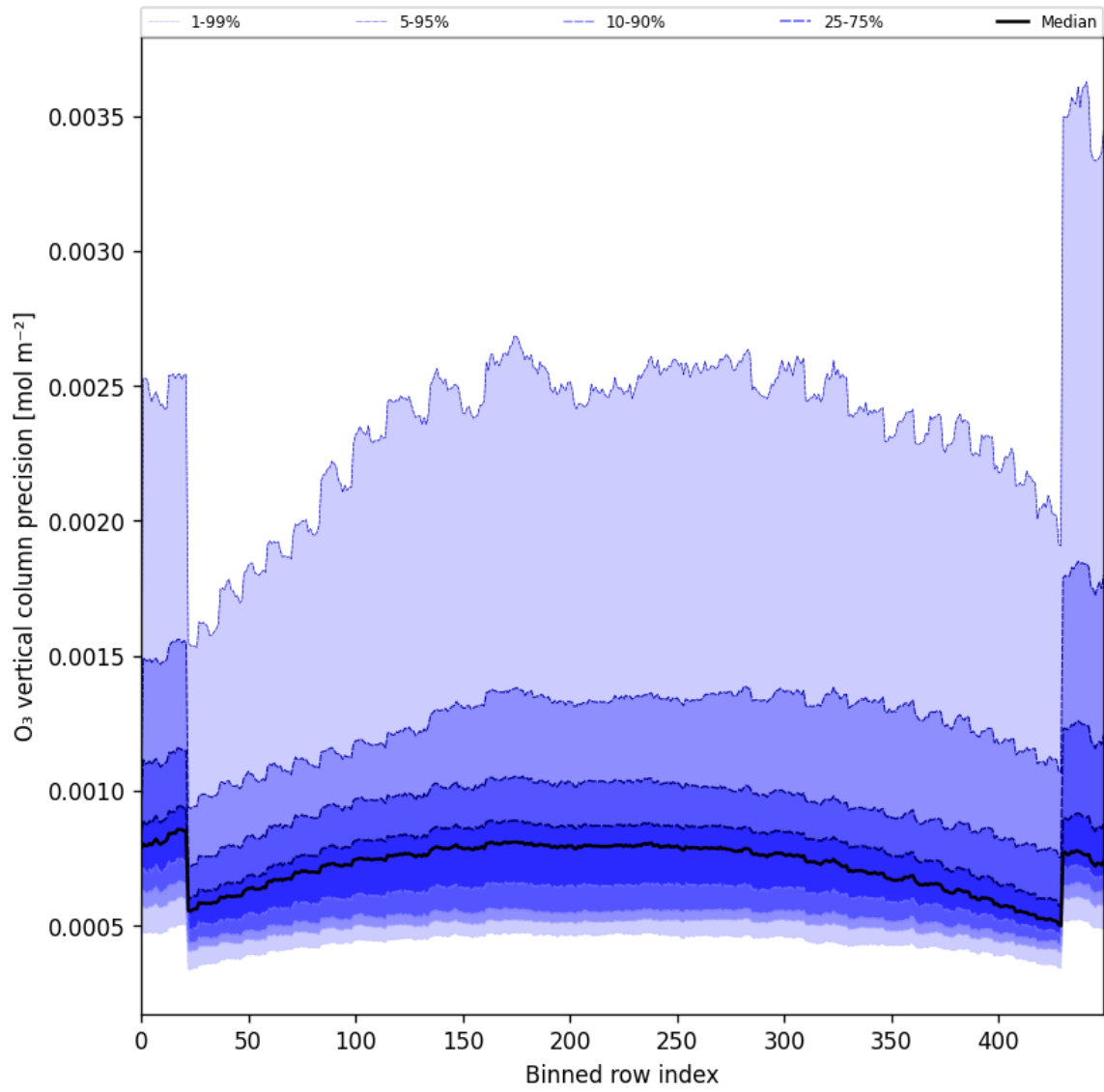
Figure 29: Along track statistics of “O 3 vertical column precision” for 2025-04-18 to 2025-04-19
