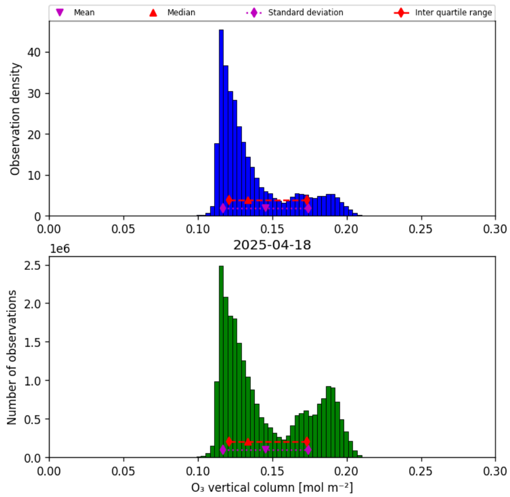
Figure 21: Histogram of “O 3 vertical column” for 2025-04-18 to 2025-04-19
