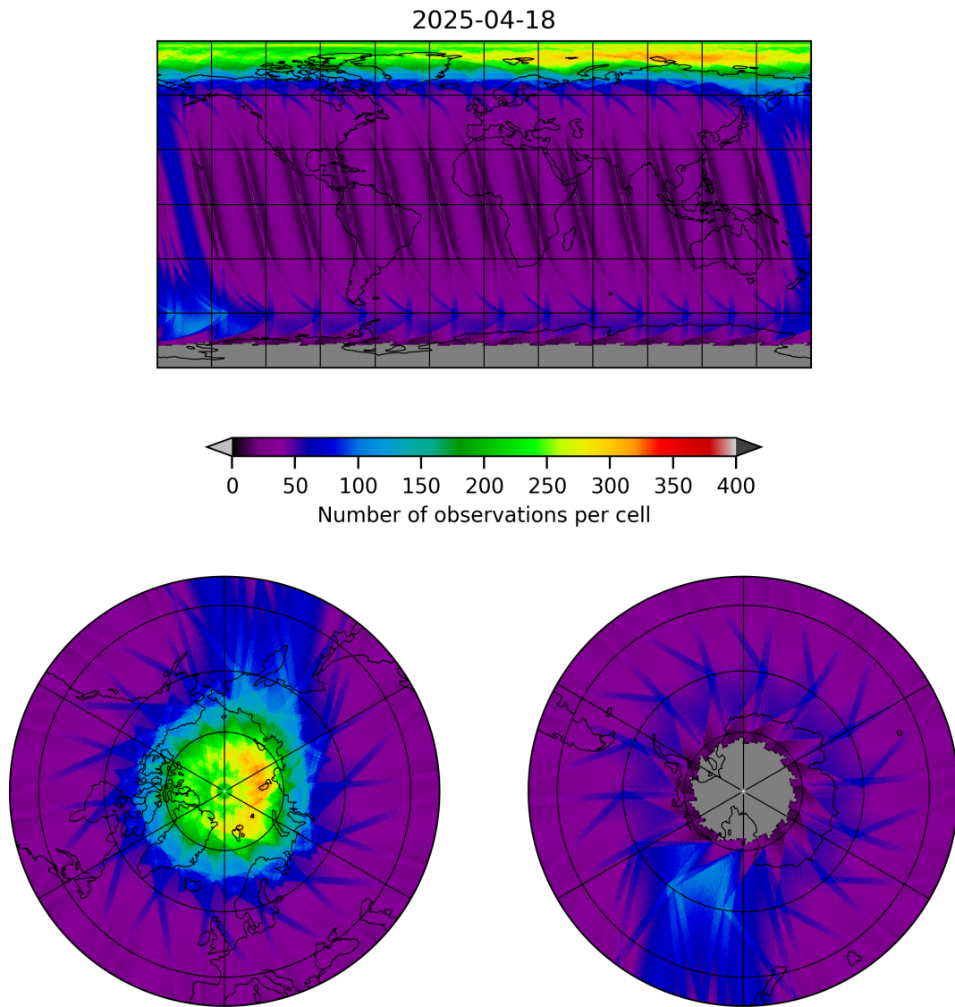
Figure 12: Map of the number of observations for 2025-04-18 to 2025-04-19
