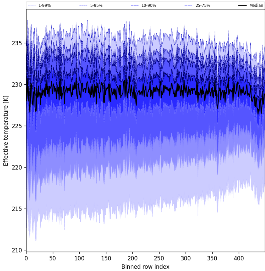
Figure 31: Along track statistics of “Effective temperature” for 2025-04-18 to 2025-04-19
