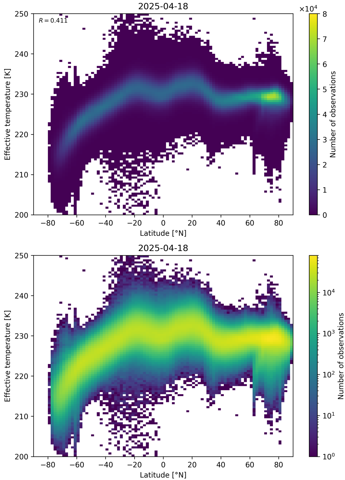
Figure 34: Scatter density plot of “Latitude” against “Effective temperature” for 2025-04-18 to 2025-04-19.
