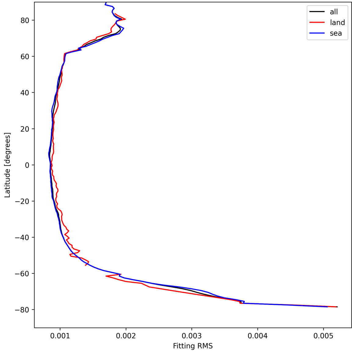
Figure 16: Zonal average of “Fitting RMS” for 2025-04-18 to 2025-04-19.
