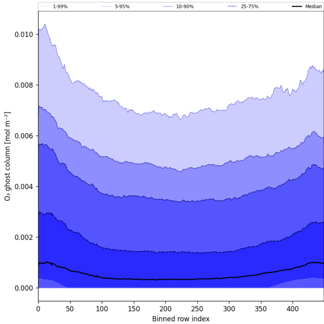
Figure 32: Along track statistics of “O 3 ghost column” for 2025-04-18 to 2025-04-19
