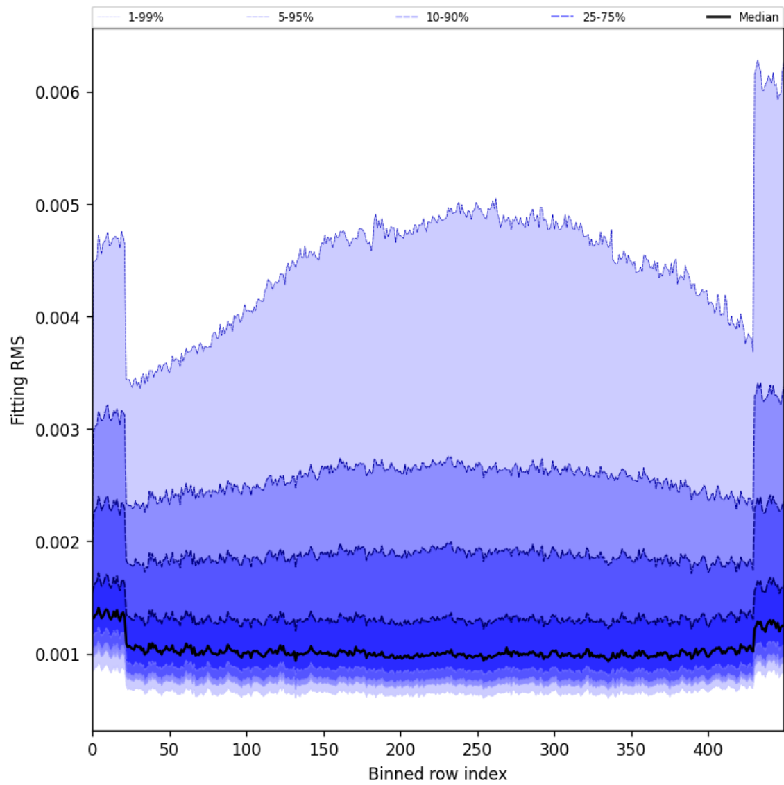
Figure 30: Along track statistics of “Fitting RMS” for 2025-04-18 to 2025-04-19
