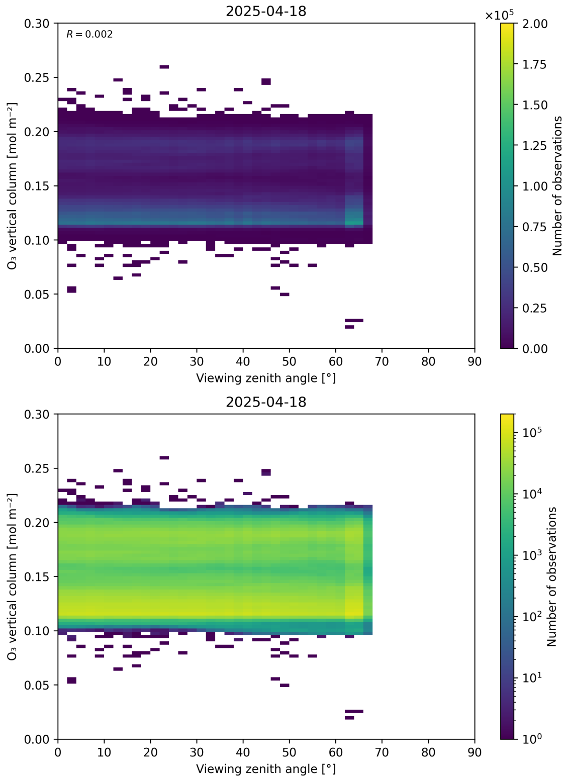
Figure 52: Scatter density plot of “Viewing zenith angle” against “O 3 vertical column” for 2025-04-18 to 2025-04-19.
