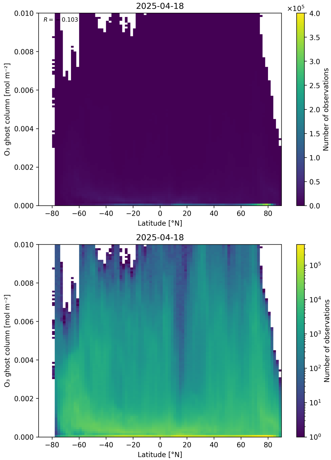
Figure 35: Scatter density plot of “Latitude” against “O 3 ghost column” for 2025-04-18 to 2025-04-19.
