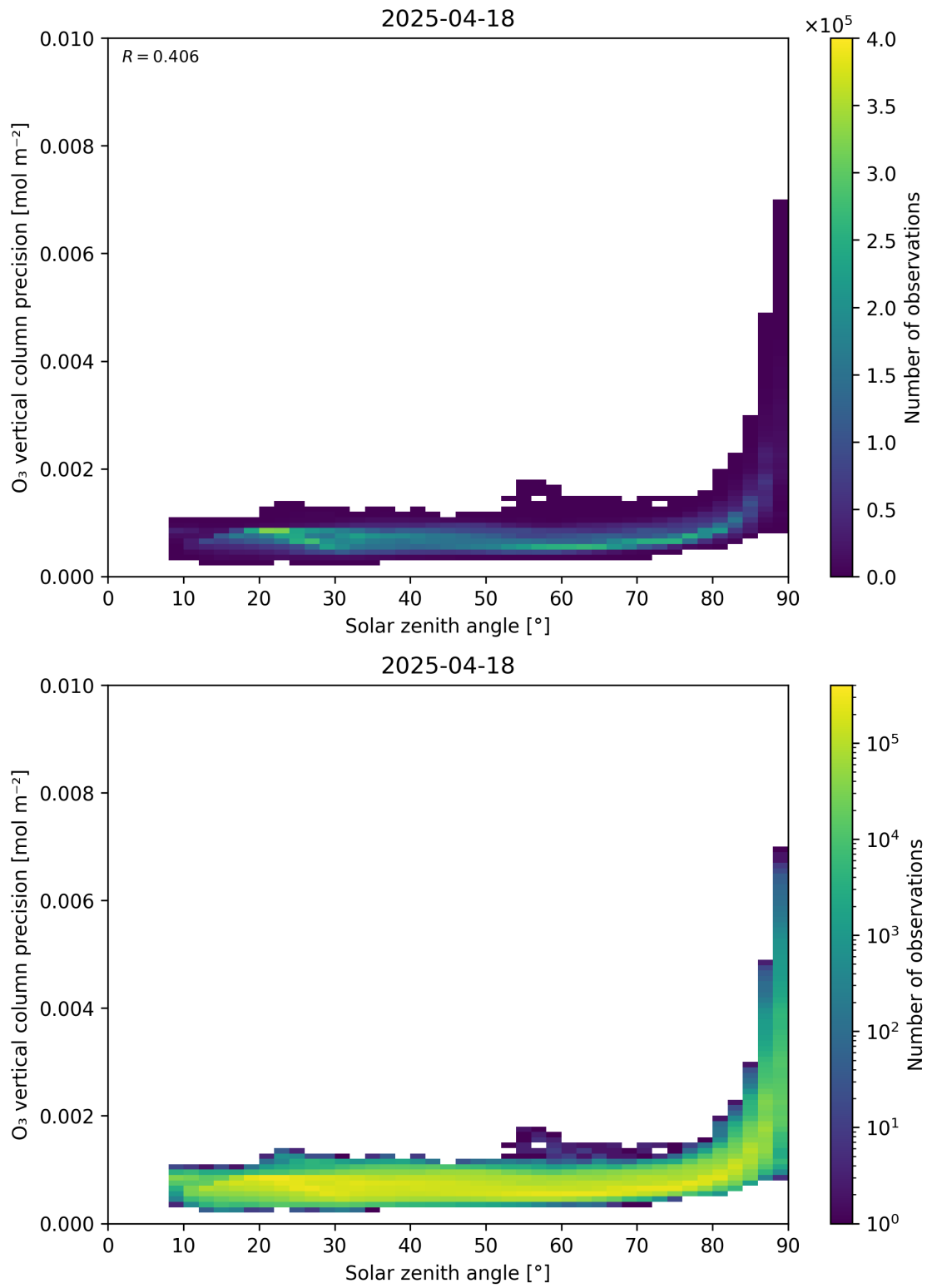
Figure 48: Scatter density plot of “Solar zenith angle” against “O 3 vertical column precision” for 2025-04-18 to 2025-04-19.
