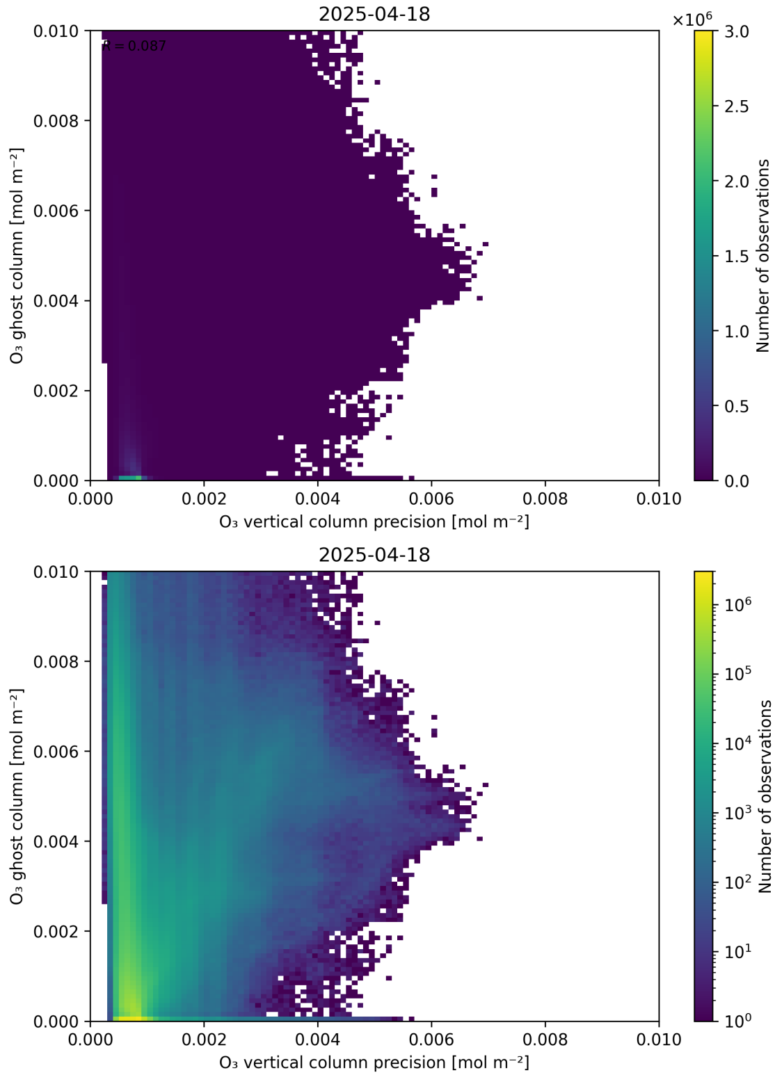
Figure 43: Scatter density plot of “O 3 vertical column precision” against “O 3 ghost column” for 2025-04-18 to 2025-04-19.
