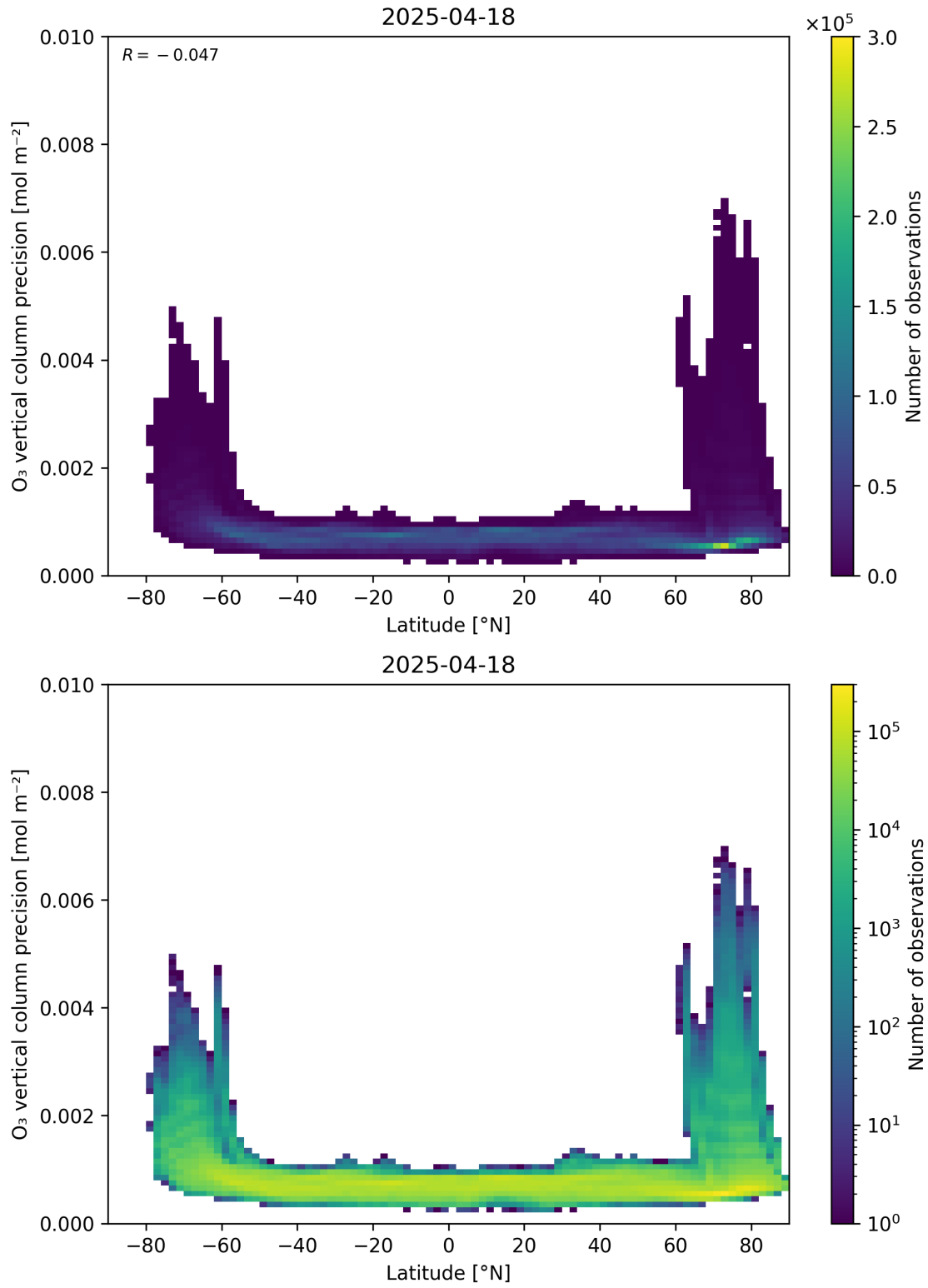
Figure 37: Scatter density plot of “Latitude” against “O 3 vertical column precision” for 2025-04-18 to 2025-04-19.
