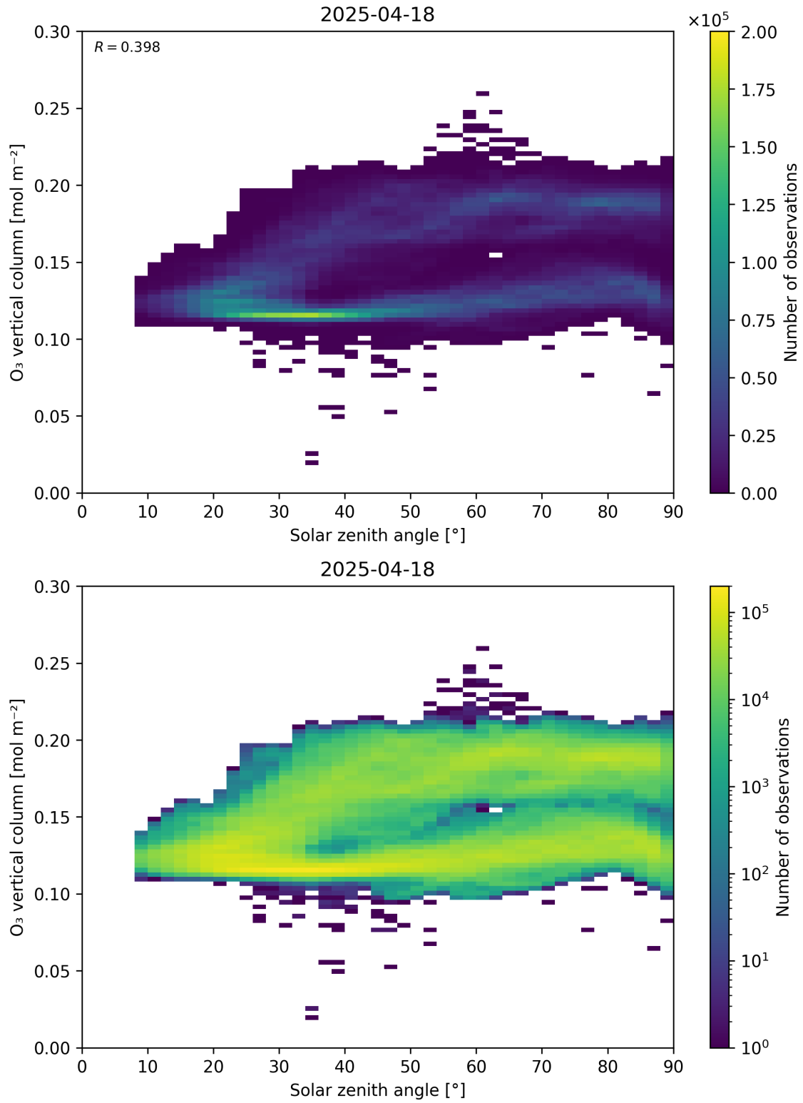
Figure 47: Scatter density plot of “Solar zenith angle” against “O 3 vertical column” for 2025-04-18 to 2025-04-19.
