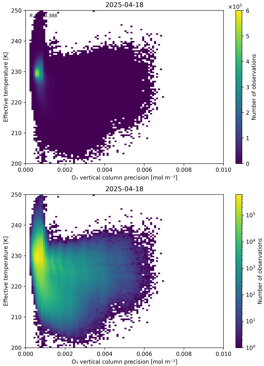
Figure 42: Scatter density plot of “O 3 vertical column precision” against “Effective temperature” for 2025-04-18 to 2025-04-19.
