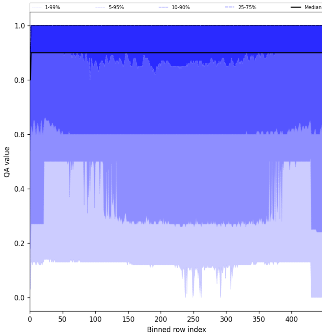
Figure 27: Along track statistics of “QA value” for 2025-04-18 to 2025-04-19
