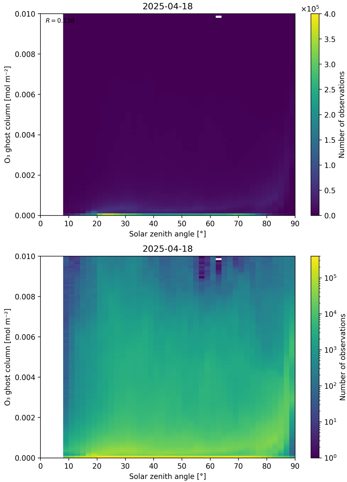
Figure 46: Scatter density plot of “Solar zenith angle” against “O 3 ghost column” for 2025-04-18 to 2025-04-19.
