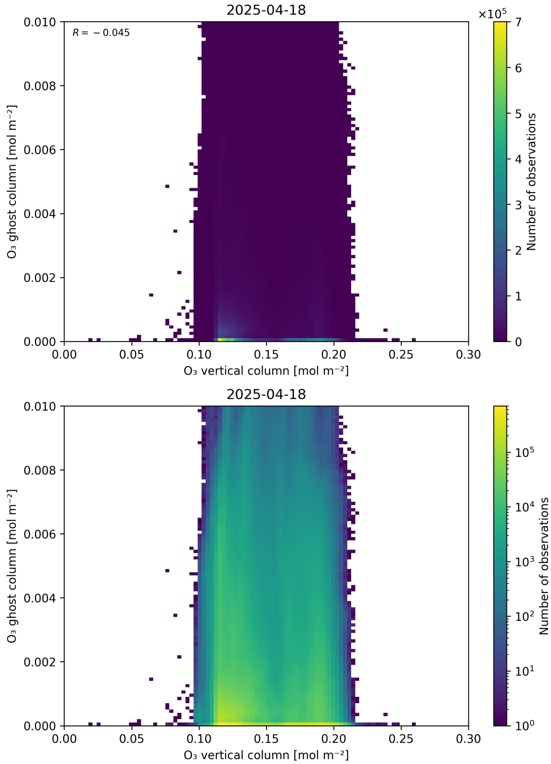
Figure 40: Scatter density plot of “O 3 vertical column” against “O 3 ghost column” for 2025-04-18 to 2025-04-19.
