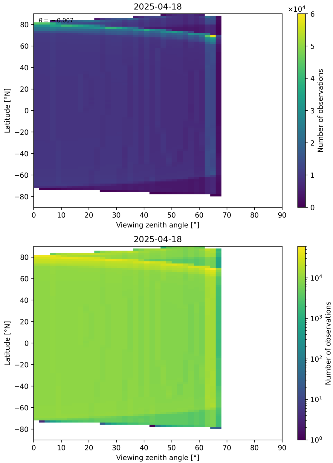
Figure 49: Scatter density plot of “Viewing zenith angle” against “Latitude” for 2025-04-18 to 2025-04-19.
