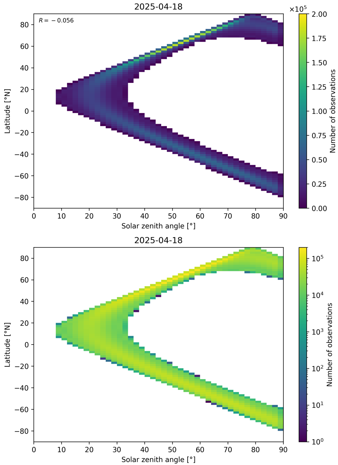
Figure 44: Scatter density plot of “Solar zenith angle” against “Latitude” for 2025-04-18 to 2025-04-19.
