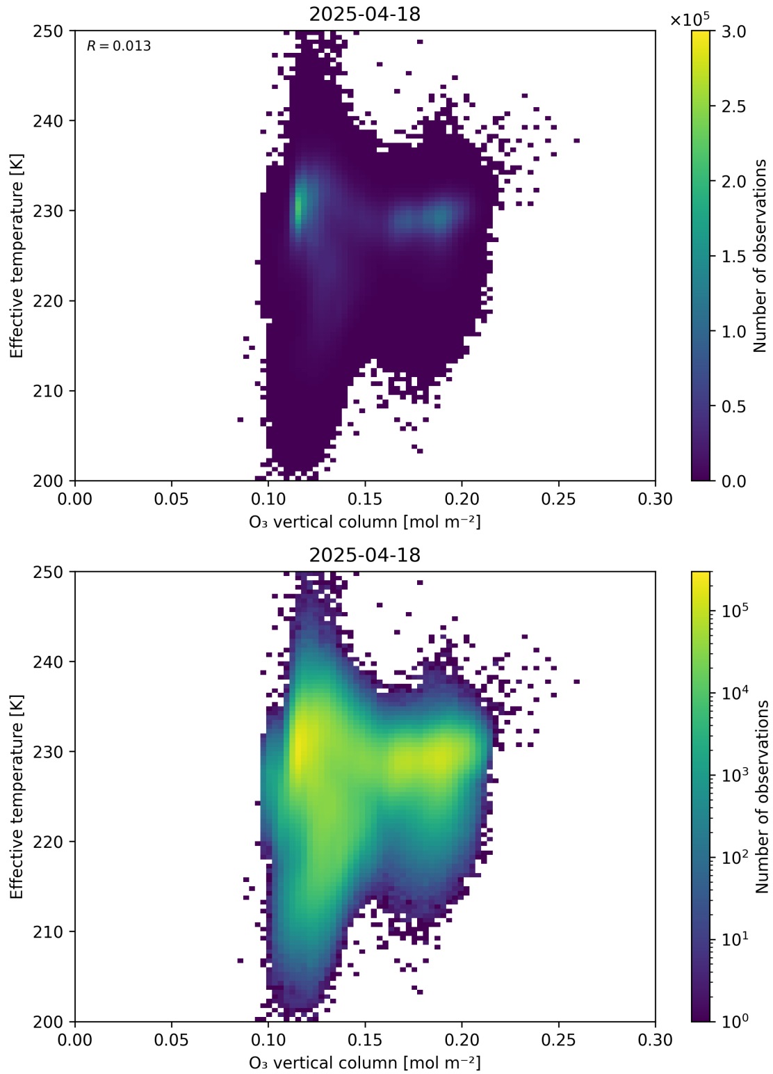
Figure 39: Scatter density plot of “O 3 vertical column” against “Effective temperature” for 2025-04-18 to 2025-04-19.
