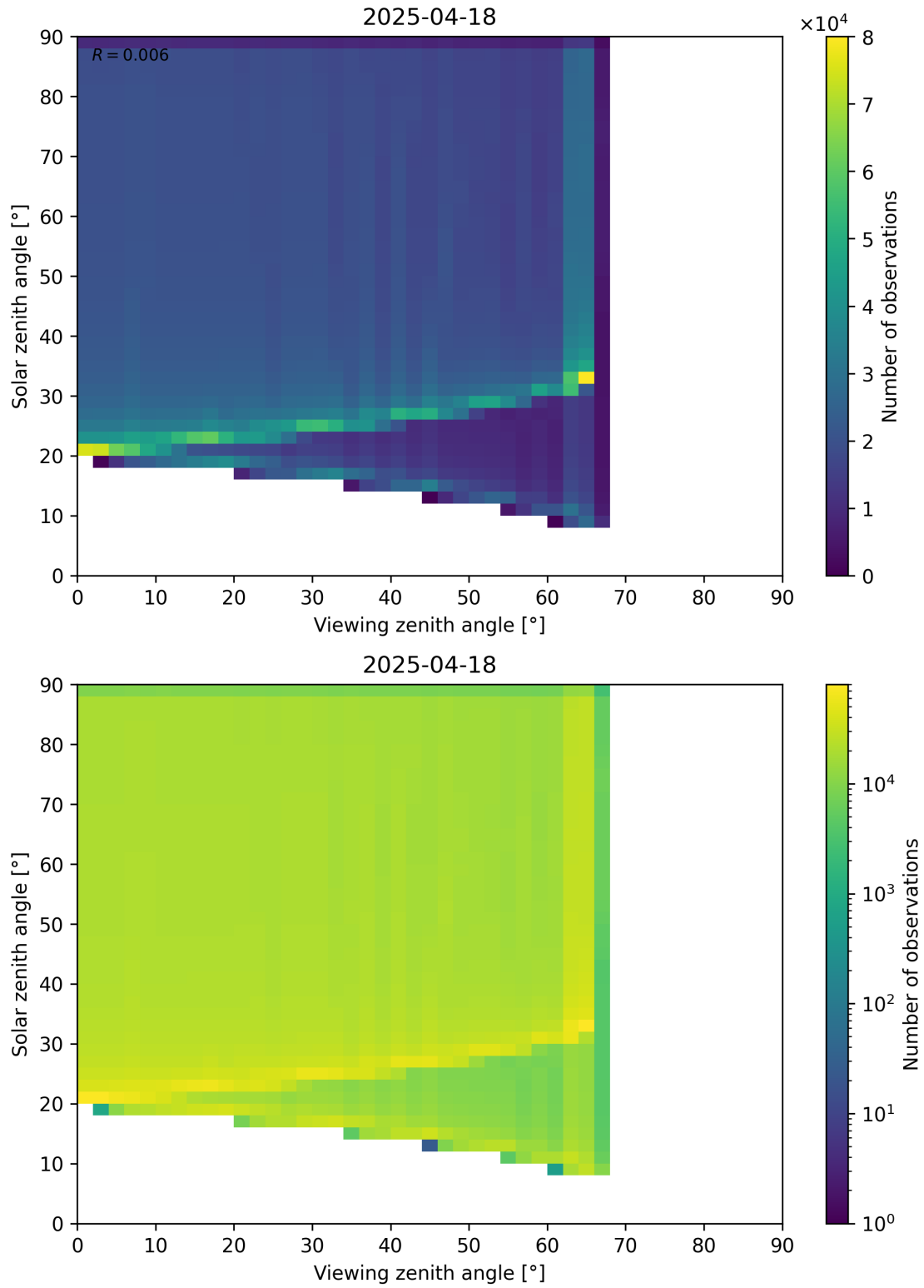
Figure 54: Scatter density plot of “Viewing zenith angle” against “Solar zenith angle” for 2025-04-18 to 2025-04-19.
