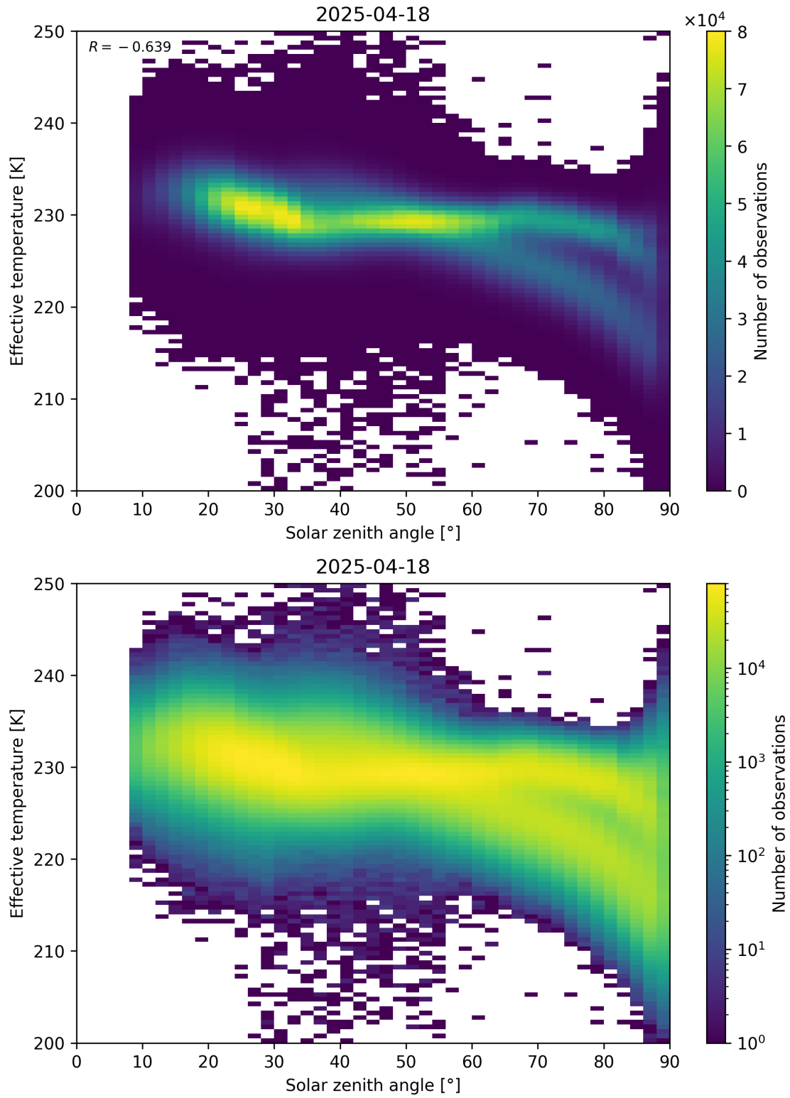
Figure 45: Scatter density plot of “Solar zenith angle” against “Effective temperature” for 2025-04-18 to 2025-04-19.
