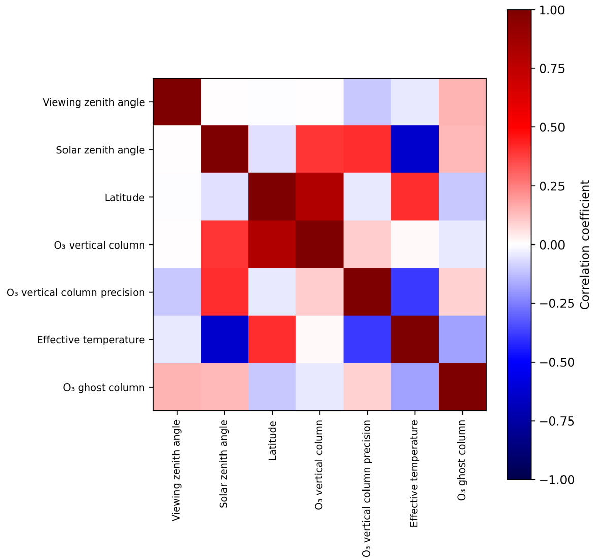
Figure 2: Map of correlation matrix for 2025-04-18 to 2025-04-19.
