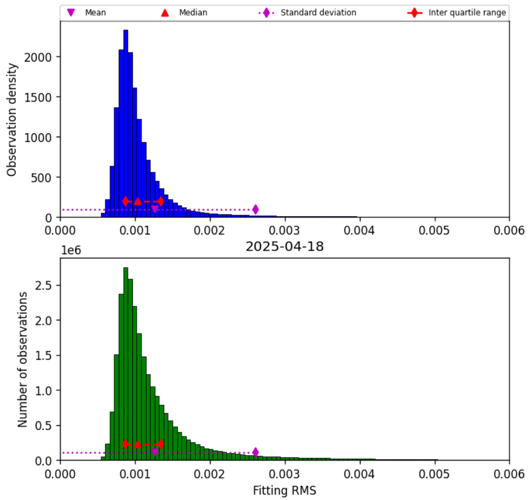
Figure 23: Histogram of “Fitting RMS” for 2025-04-18 to 2025-04-19
