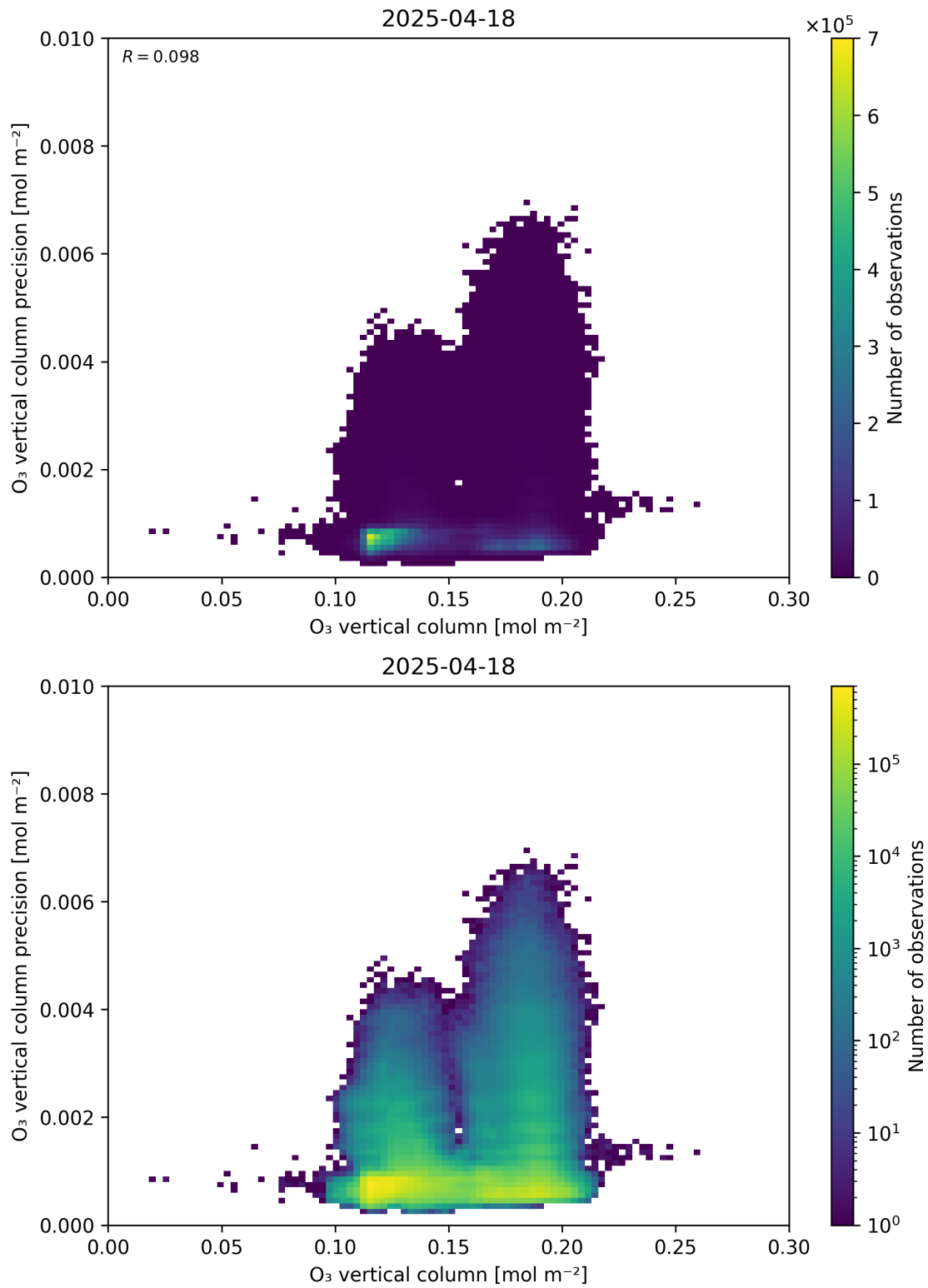
Figure 41: Scatter density plot of “O 3 vertical column” against “O 3 vertical column precision” for 2025-04-18 to 2025-04-19.
