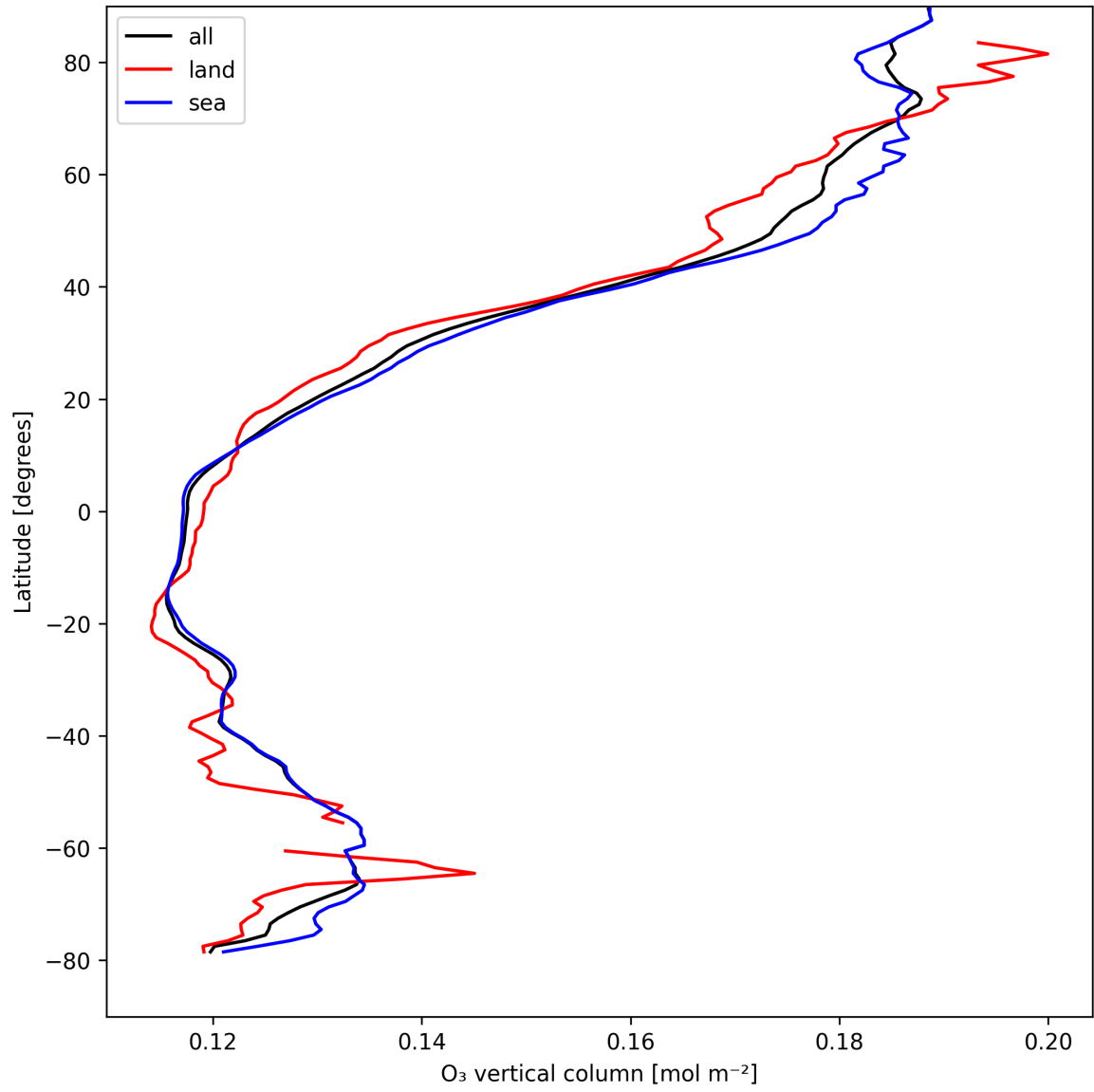
Figure 14: Zonal average of “O 3 vertical column” for 2025-04-18 to 2025-04-19.
