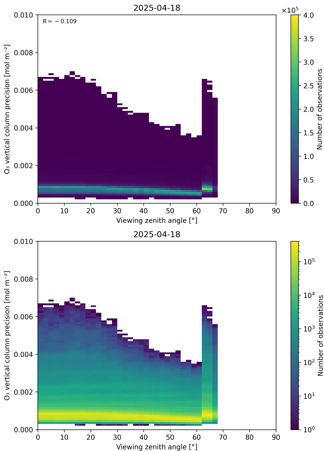
Figure 53: Scatter density plot of “Viewing zenith angle” against “O 3 vertical column precision” for 2025-04-18 to 2025-04-19.
