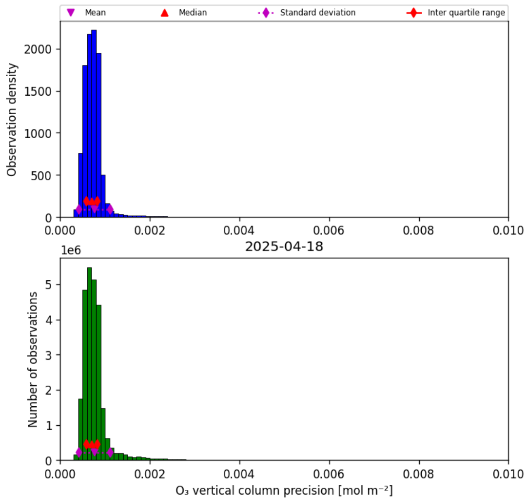
Figure 22: Histogram of “O 3 vertical column precision” for 2025-04-18 to 2025-04-19
