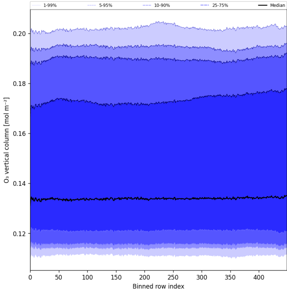
Figure 28: Along track statistics of “O 3 vertical column” for 2025-04-18 to 2025-04-19
