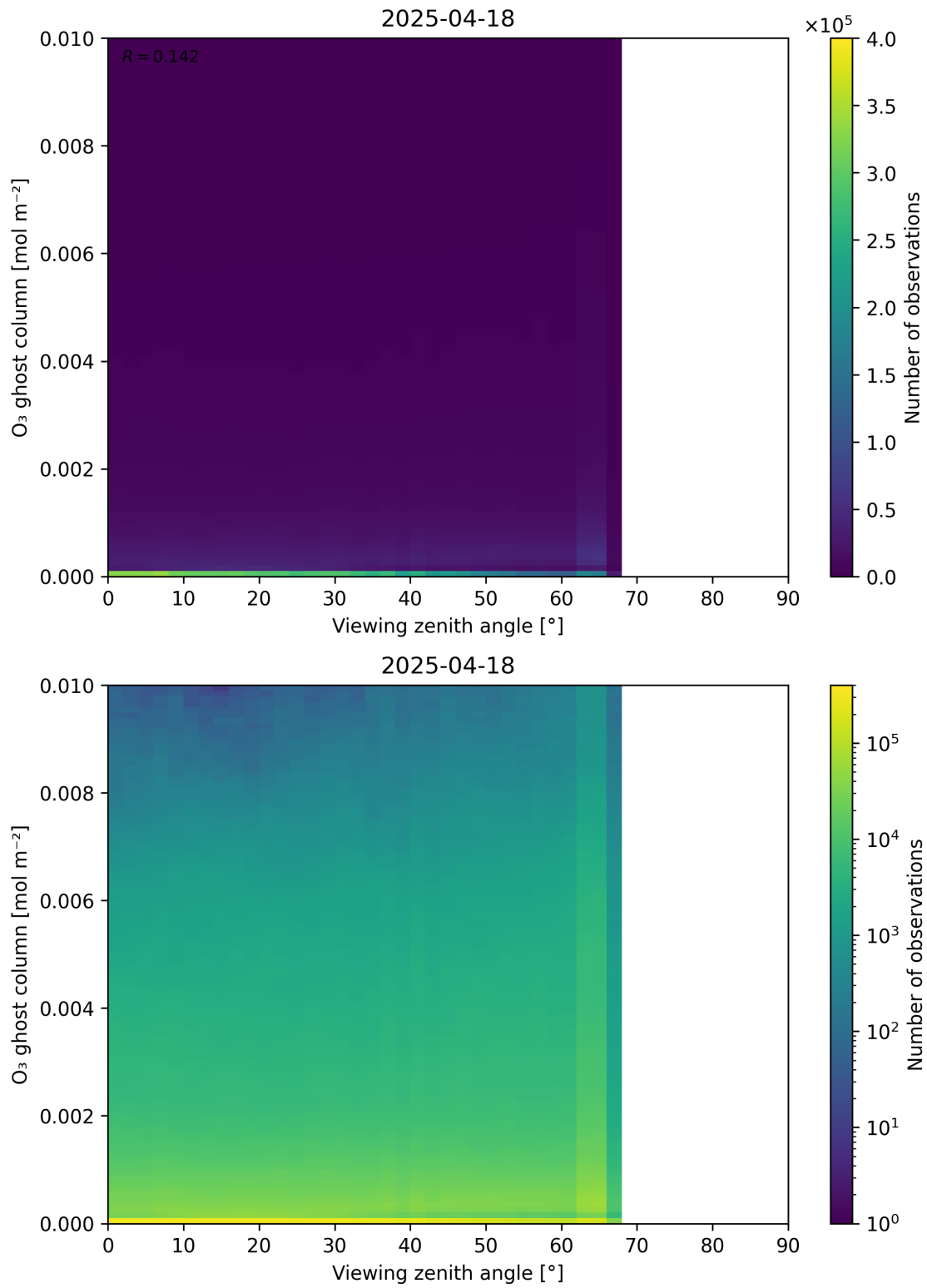
Figure 51: Scatter density plot of “Viewing zenith angle” against “O 3 ghost column” for 2025-04-18 to 2025-04-19.
