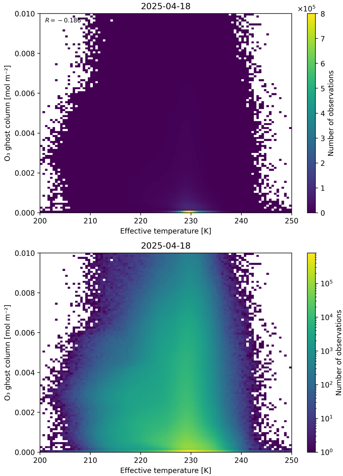
Figure 38: Scatter density plot of “Effective temperature” against “O 3 ghost column” for 2025-04-18 to 2025-04-19.
