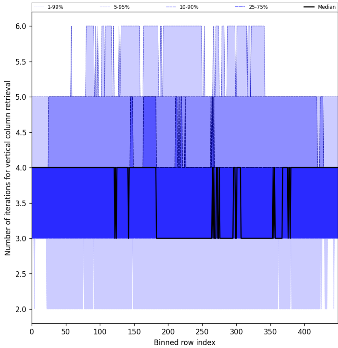
Figure 33: Along track statistics of “Number of iterations for vertical column retrieval” for 2025-04-18 to 2025-04-19
