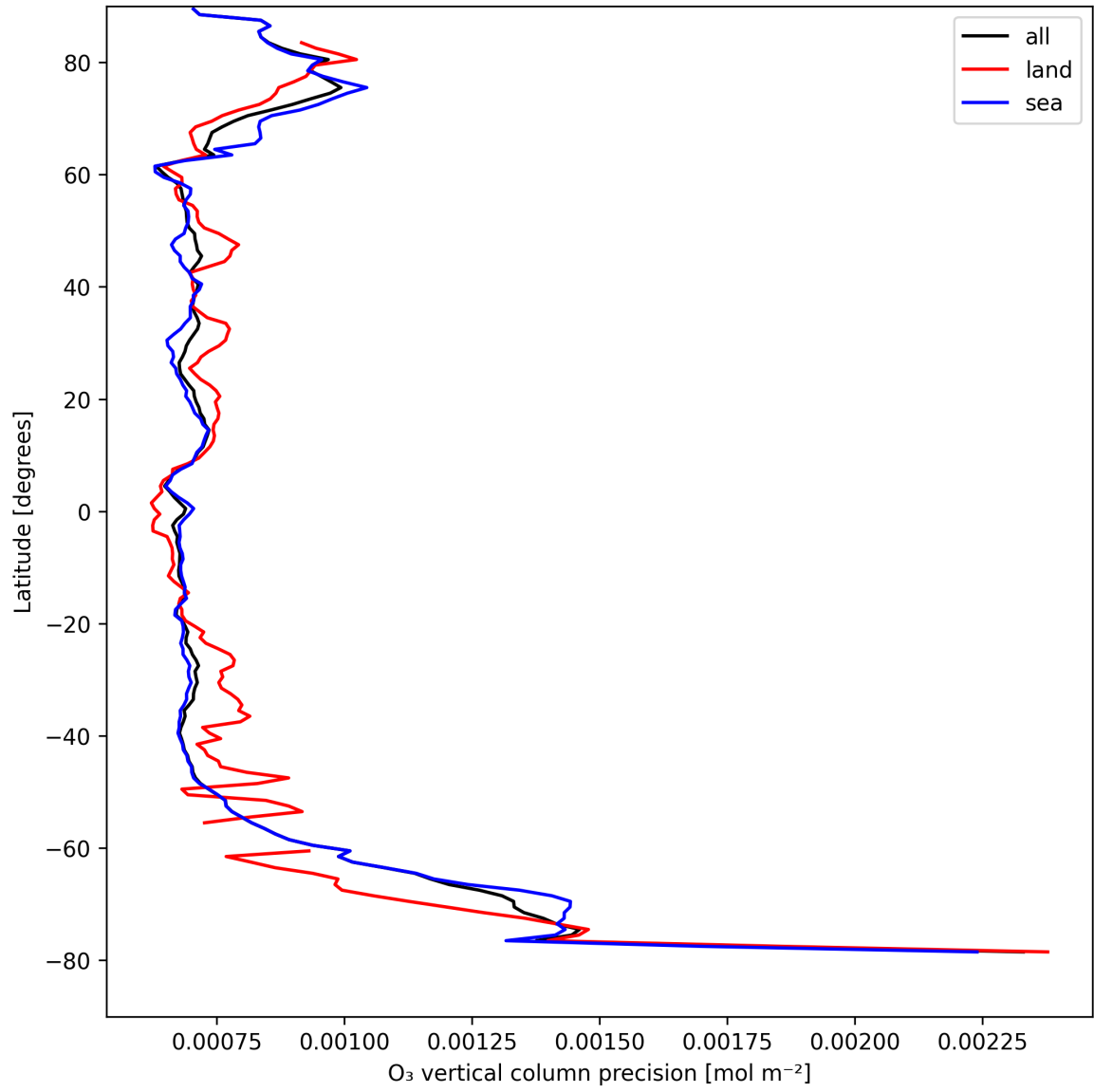
Figure 15: Zonal average of "O 3 vertical column precision" for 2025-04-18 to 2025-04-19.
