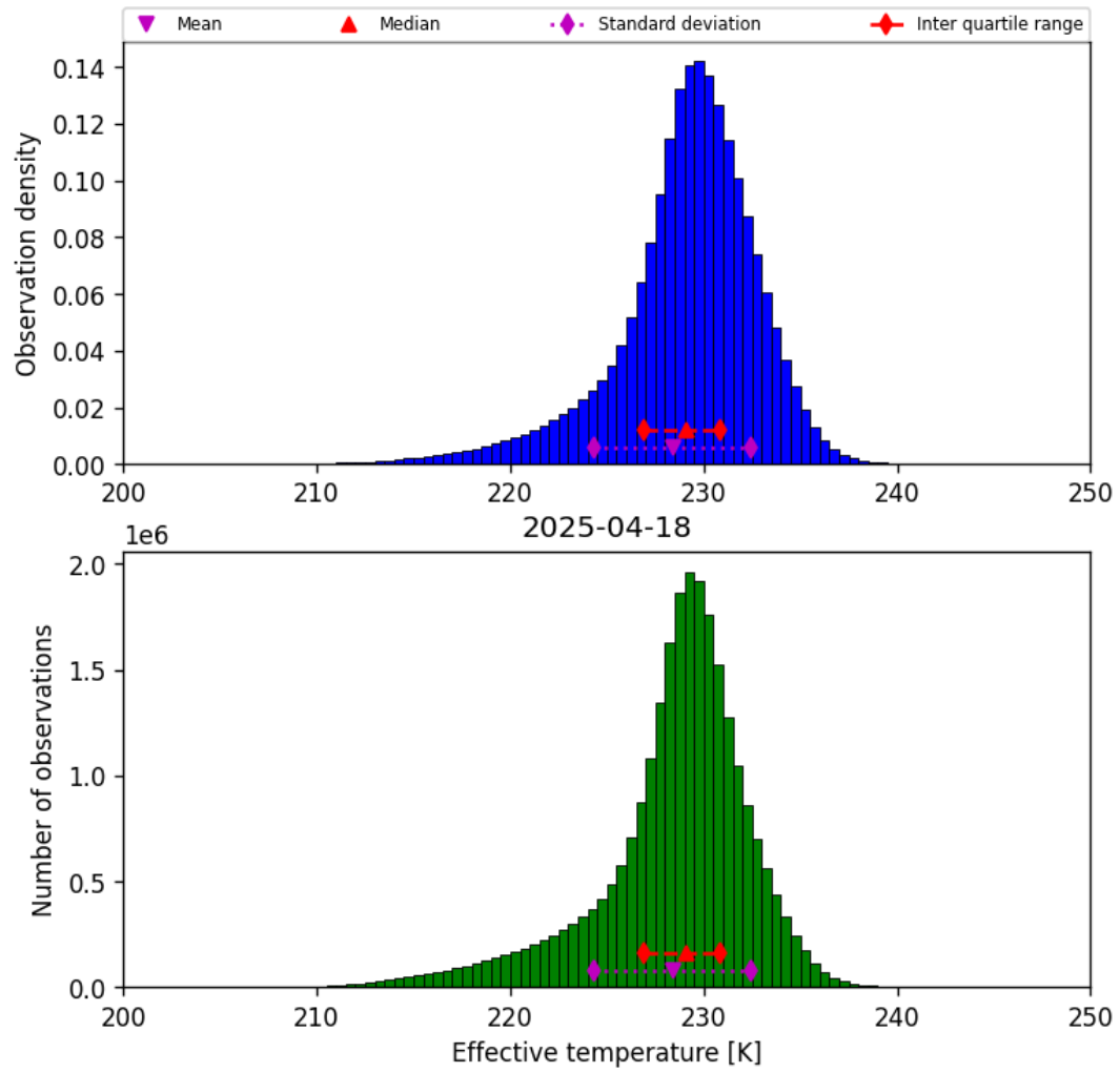
Figure 24: Histogram of “Effective temperature” for 2025-04-18 to 2025-04-19
