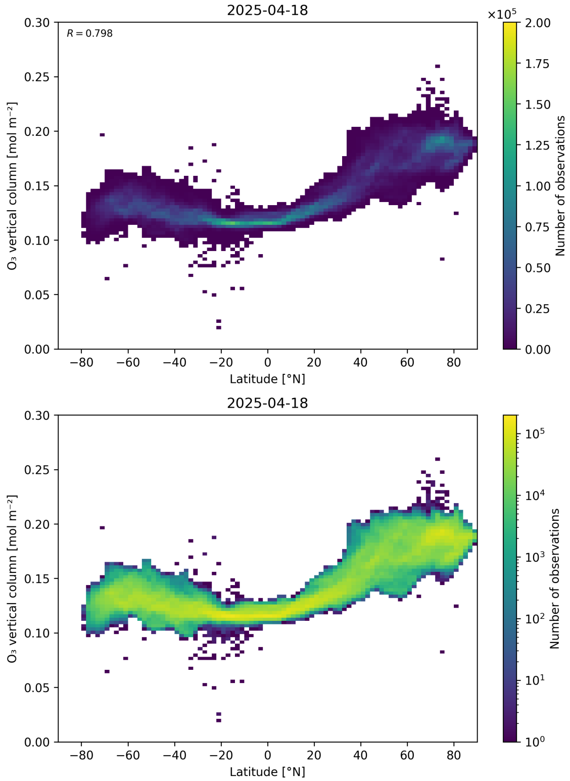
Figure 36: Scatter density plot of “Latitude” against “O 3 vertical column” for 2025-04-18 to 2025-04-19.
