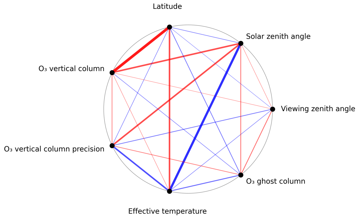
Figure 1: Map of correlation graph for 2025-04-18 to 2025-04-19.
