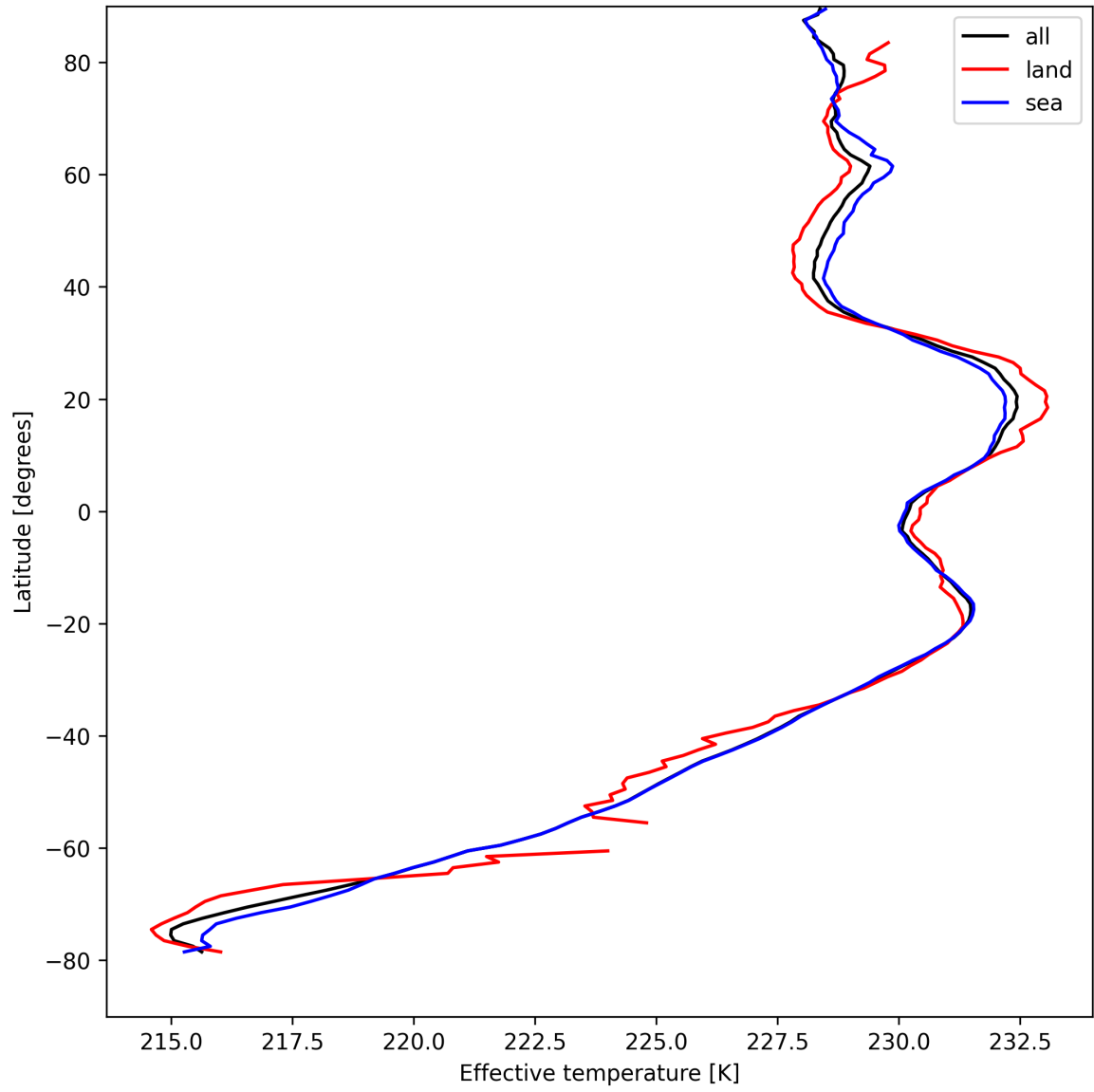
Figure 17: Zonal average of “Effective temperature” for 2025-04-18 to 2025-04-19.
