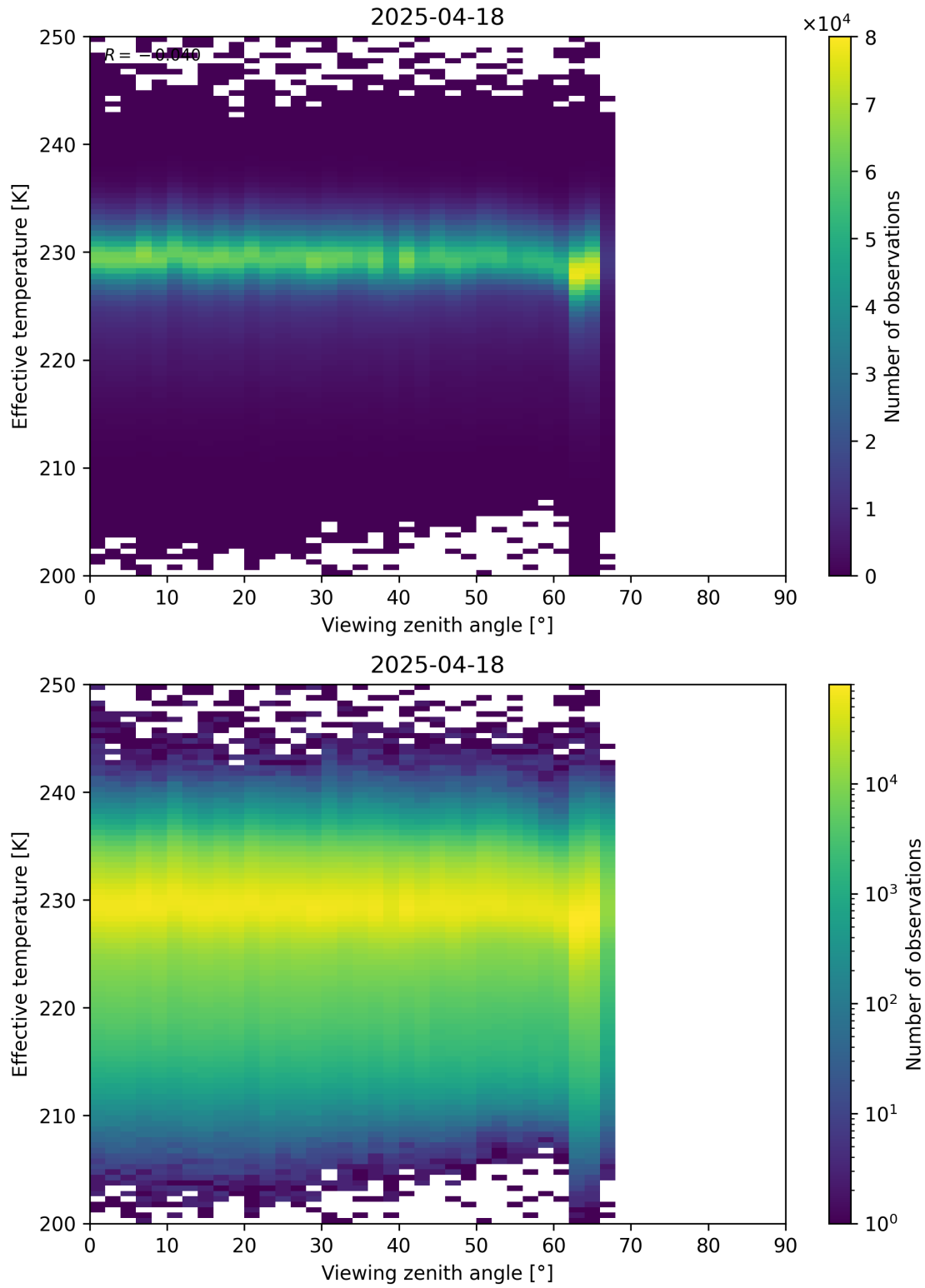
Figure 50: Scatter density plot of “Viewing zenith angle” against “Effective temperature” for 2025-04-18 to 2025-04-19.
