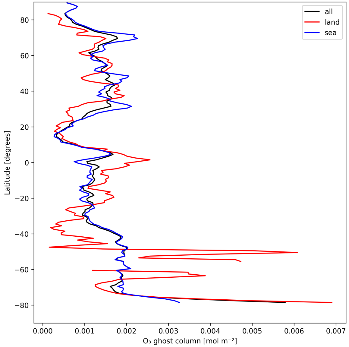
Figure 18: Zonal average of "O 3 ghost column" for 2025-04-18 to 2025-04-19.
