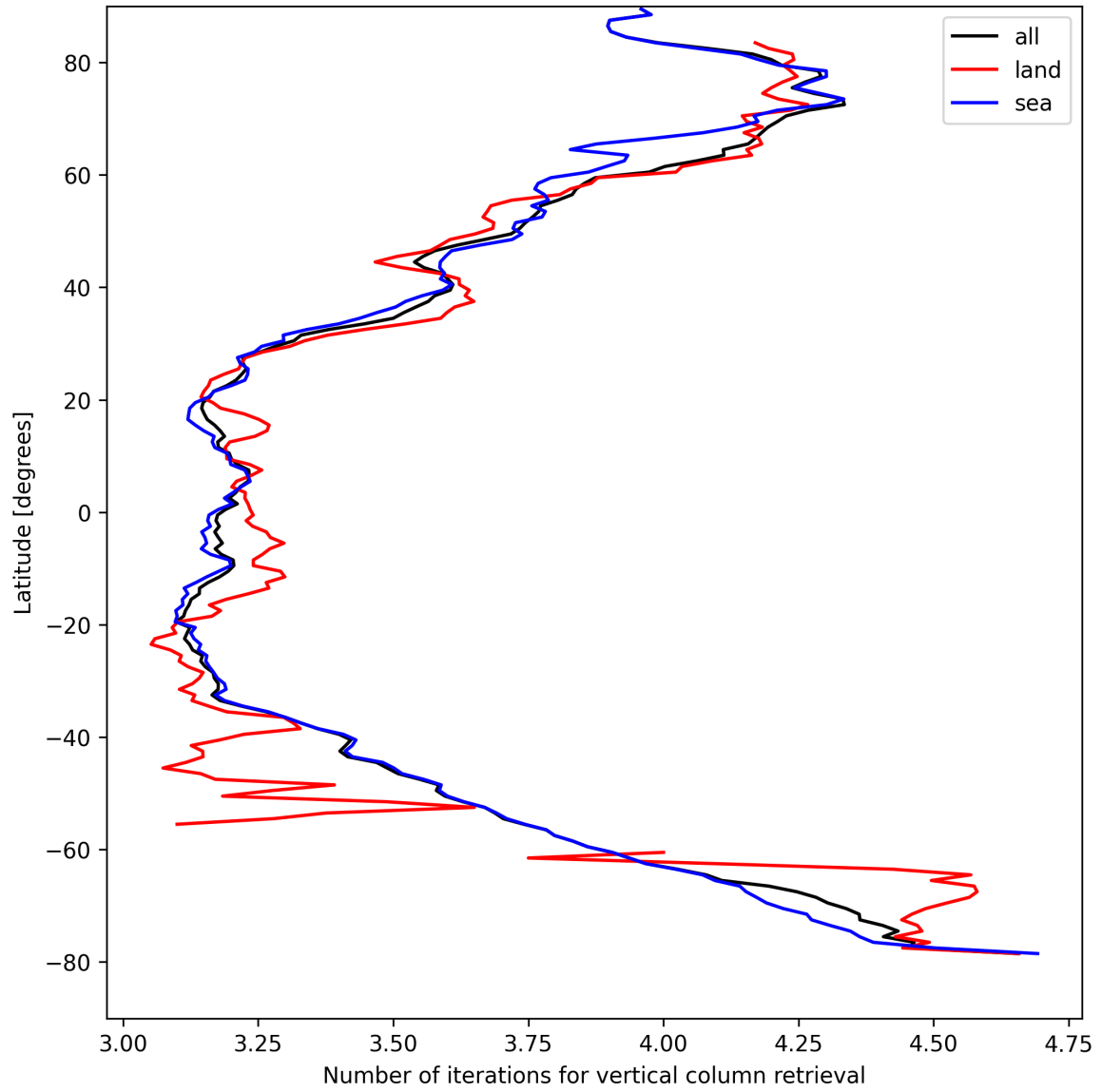
Figure 19: Zonal average of “Number of iterations for vertical column retrieval” for 2025-04-18 to 2025-04-19.
