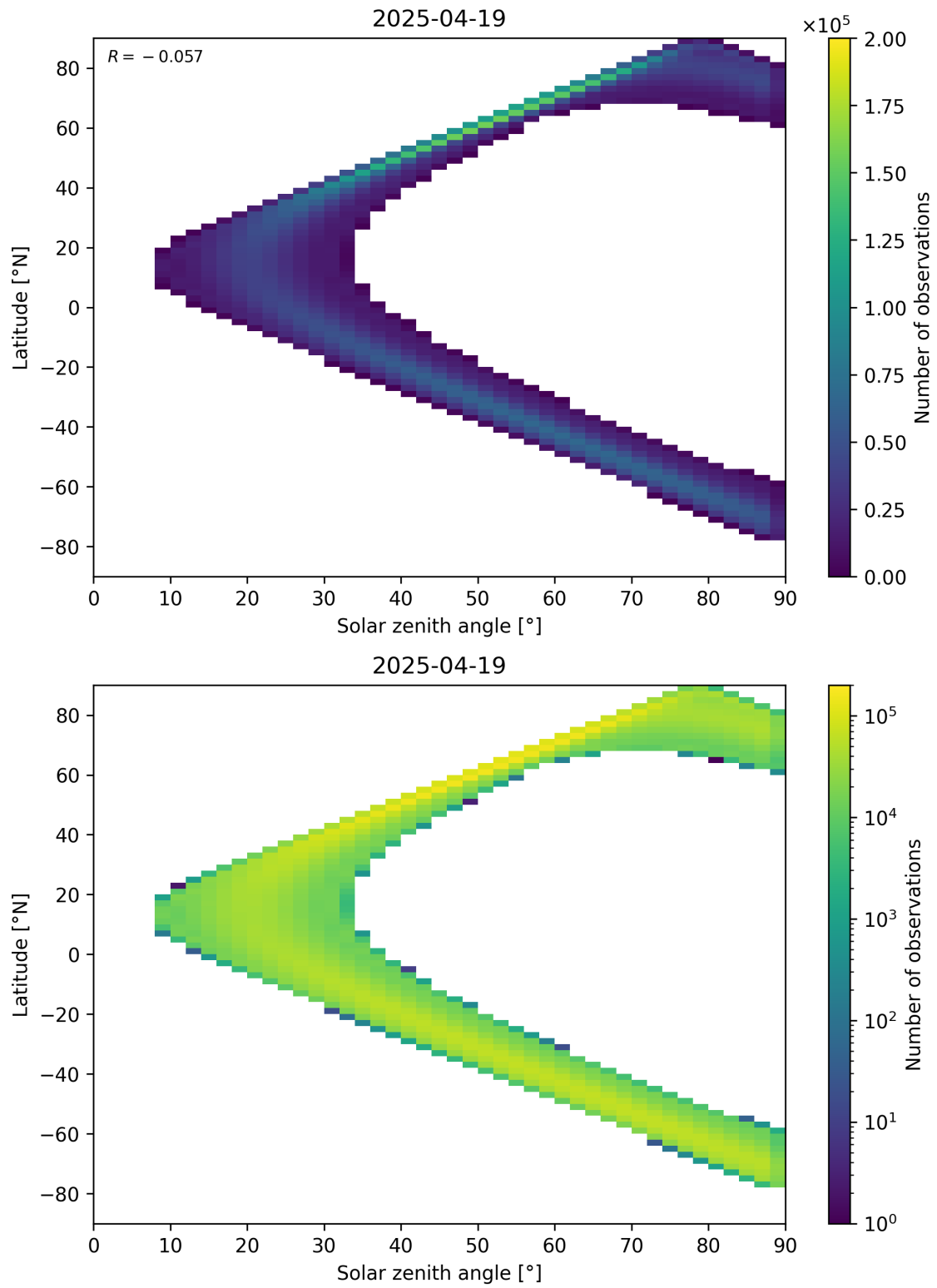
Figure 44: Scatter density plot of “Solar zenith angle” against “Latitude” for 2025-04-19 to 2025-04-20.
