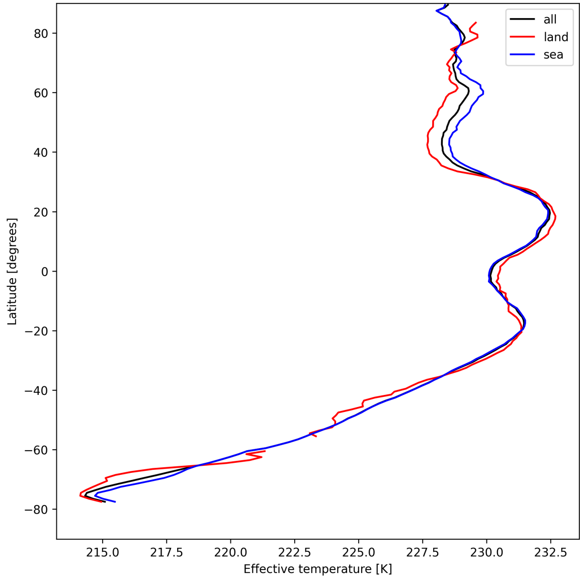
Figure 17: Zonal average of "Effective temperature" for 2025-04-19 to 2025-04-20.
