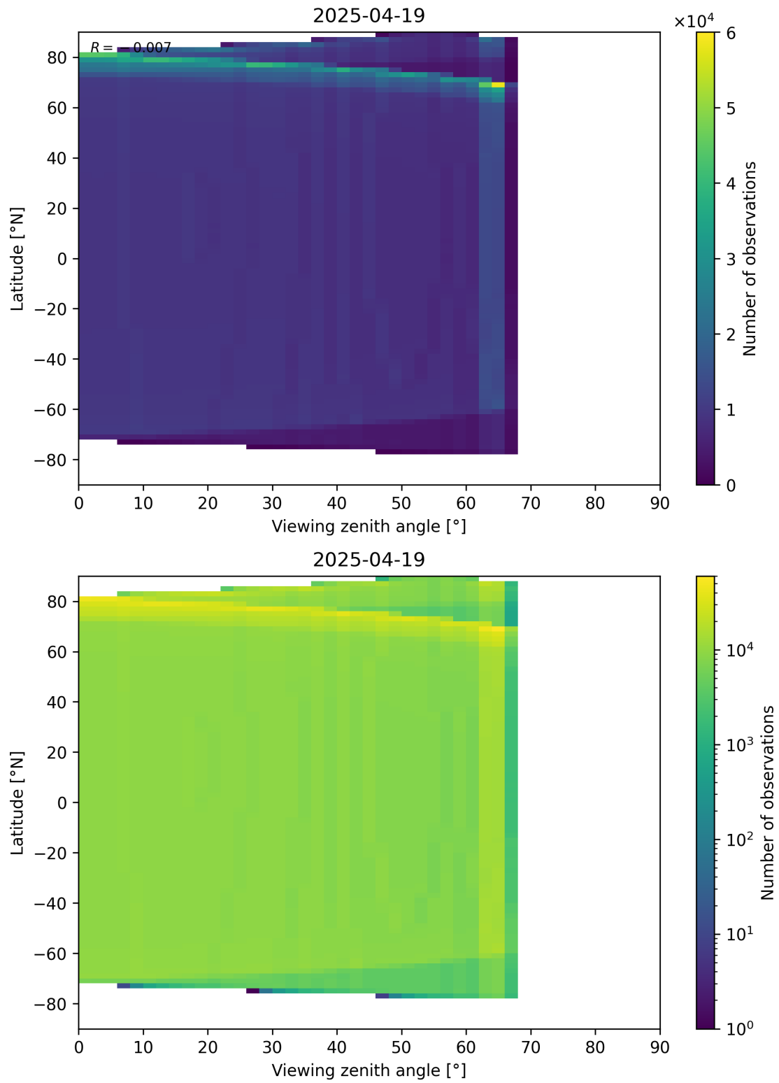
Figure 49: Scatter density plot of “Viewing zenith angle” against “Latitude” for 2025-04-19 to 2025-04-20.
