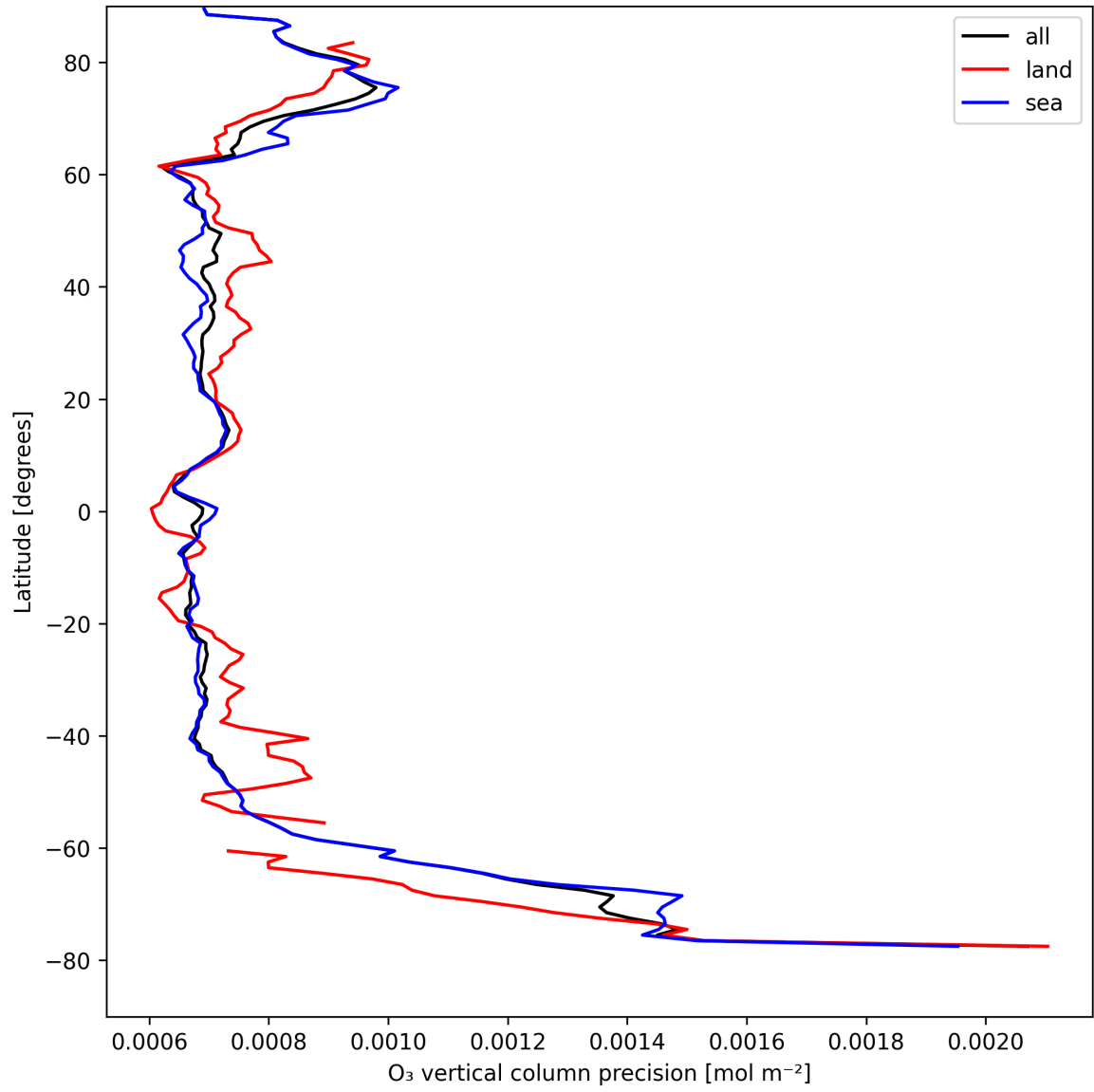
Figure 15: Zonal average of “O 3 vertical column precision” for 2025-04-19 to 2025-04-20.
