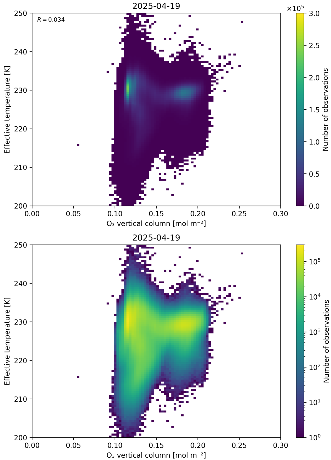
Figure 39: Scatter density plot of “O 3 vertical column” against “Effective temperature” for 2025-04-19 to 2025-04-20.
