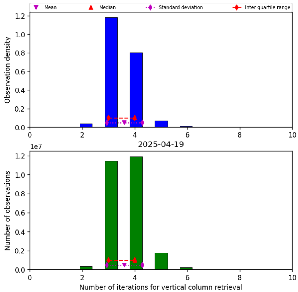
Figure 26: Histogram of “Number of iterations for vertical column retrieval” for 2025-04-19 to 2025-04-20
