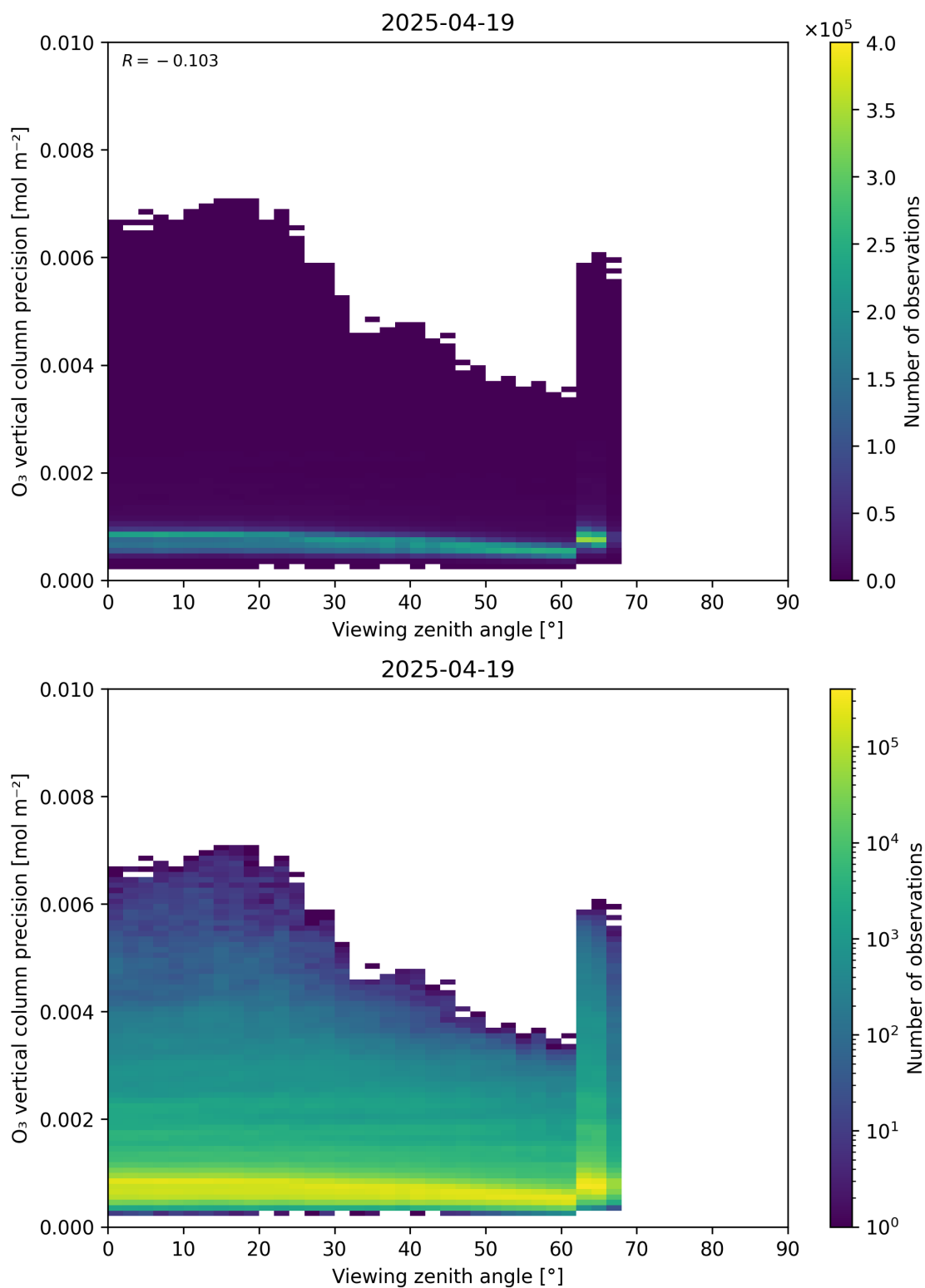
Figure 53: Scatter density plot of “Viewing zenith angle” against “O 3 vertical column precision” for 2025-04-19 to 2025-04-20.
