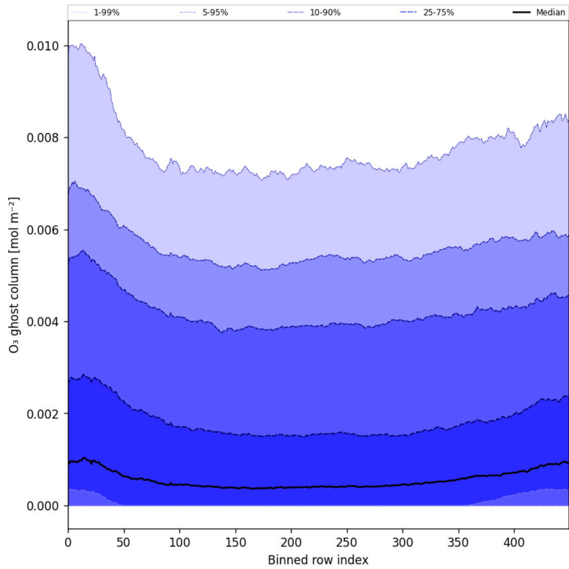
Figure 32: Along track statistics of “O 3 ghost column” for 2025-04-19 to 2025-04-20
