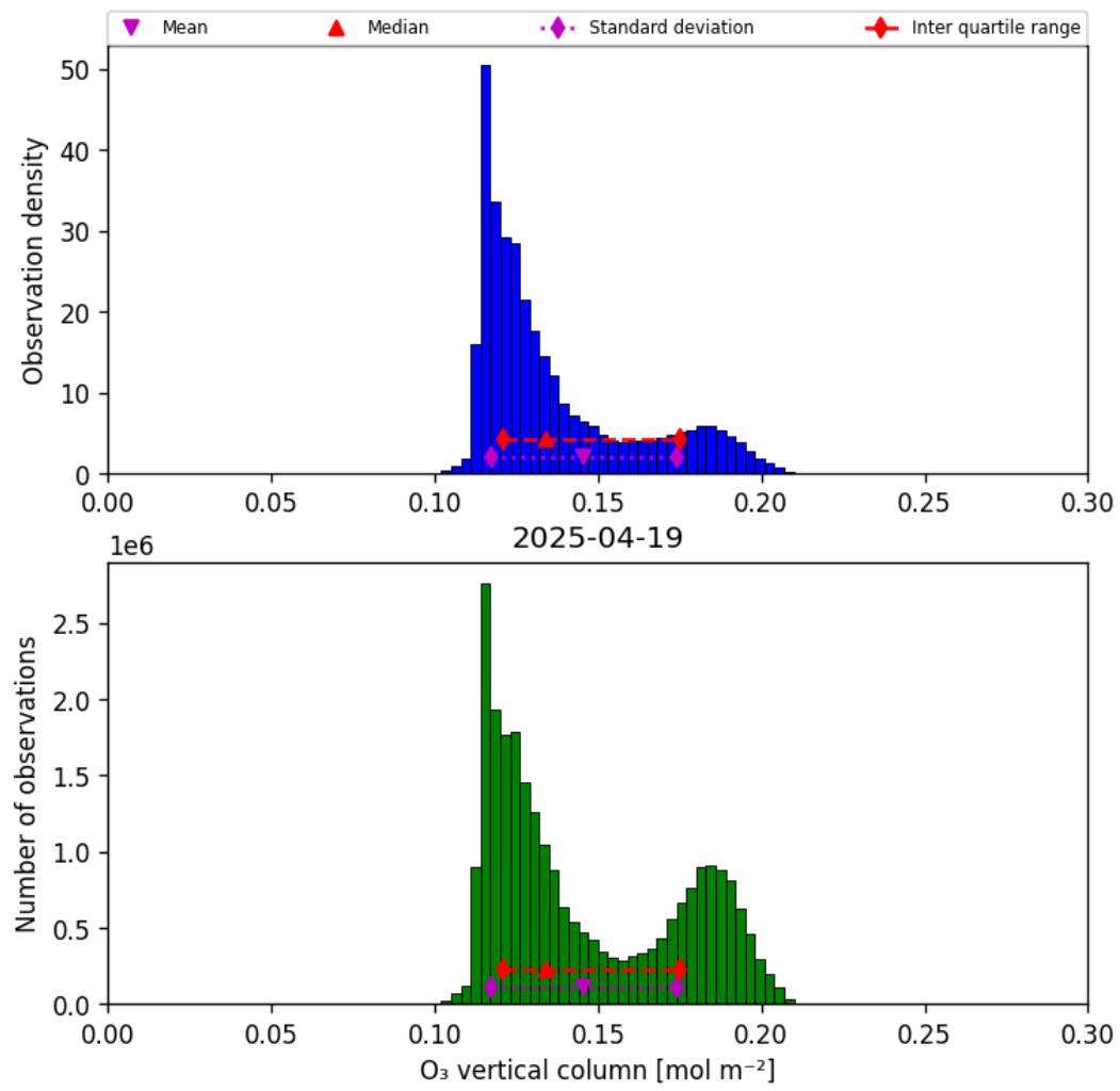
Figure 21: Histogram of “O 3 vertical column” for 2025-04-19 to 2025-04-20
