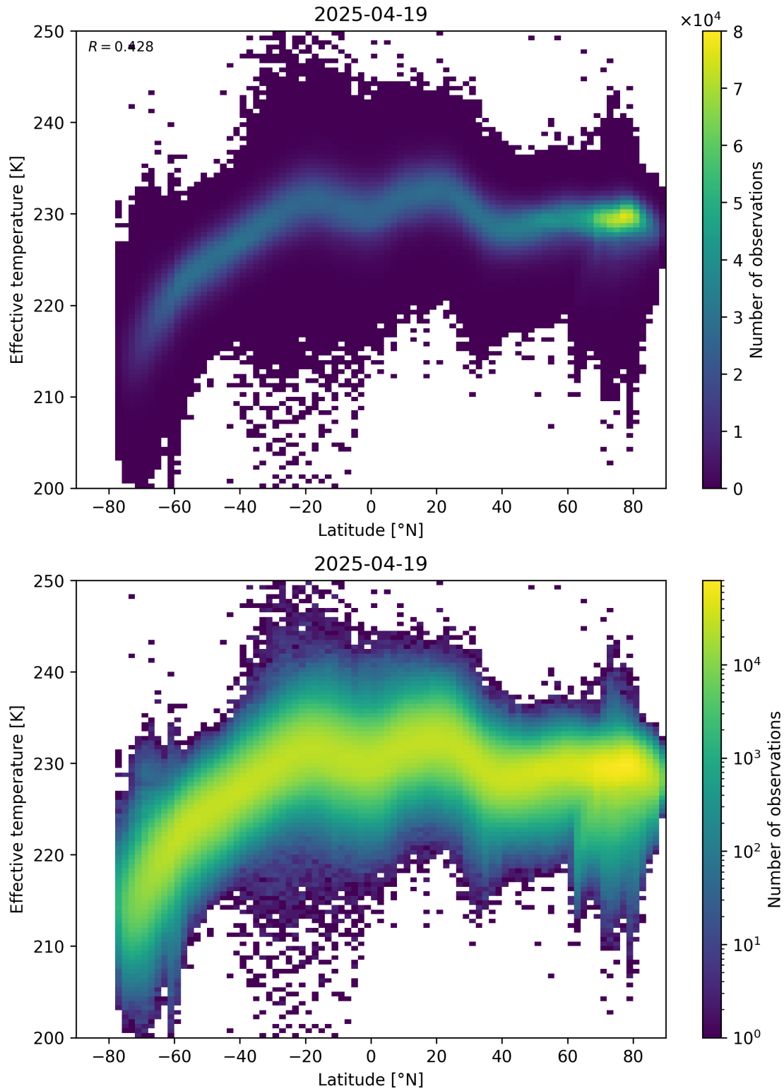
Figure 34: Scatter density plot of “Latitude” against “Effective temperature” for 2025-04-19 to 2025-04-20.
