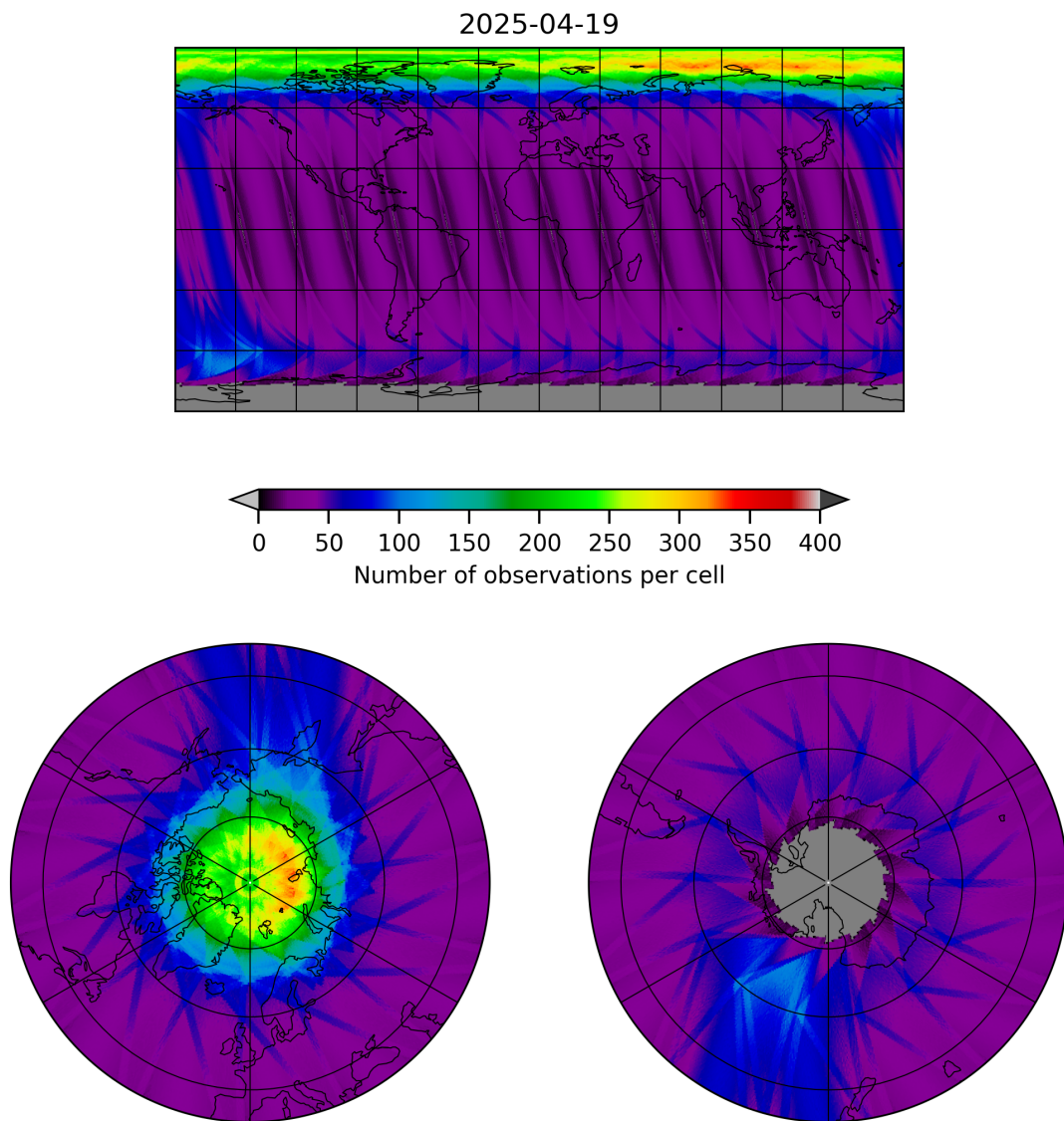
Figure 12: Map of the number of observations for 2025-04-19 to 2025-04-20
