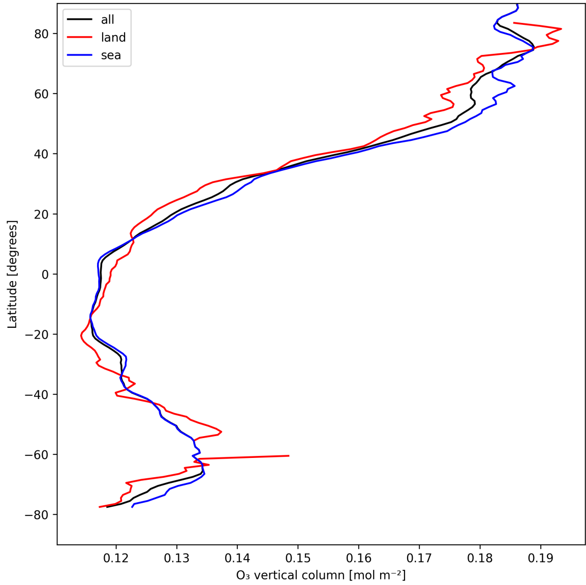
Figure 14: Zonal average of “O 3 vertical column” for 2025-04-19 to 2025-04-20.
