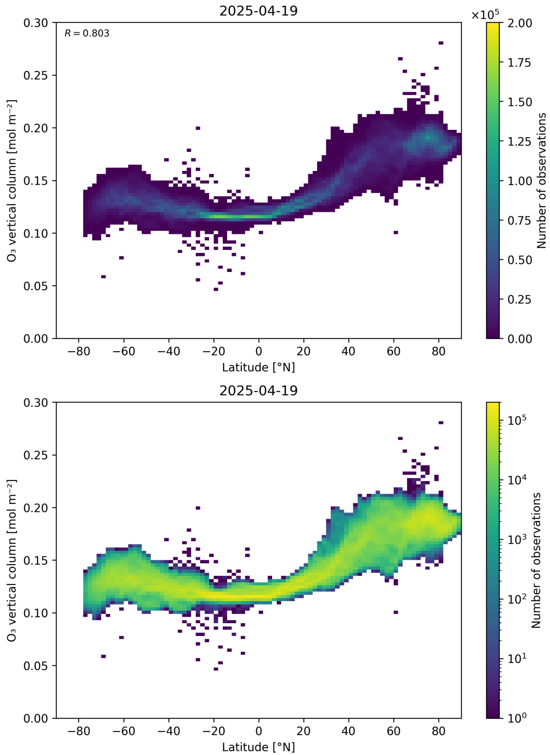
Figure 36: Scatter density plot of “Latitude” against “O 3 vertical column” for 2025-04-19 to 2025-04-20.
