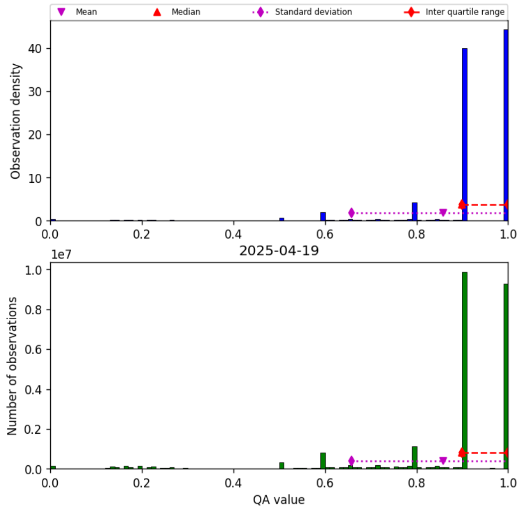
Figure 20: Histogram of “QA value” for 2025-04-19 to 2025-04-20
