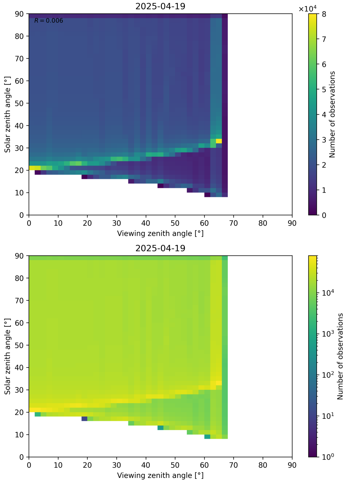
Figure 54: Scatter density plot of “Viewing zenith angle” against “Solar zenith angle” for 2025-04-19 to 2025-04-20.
