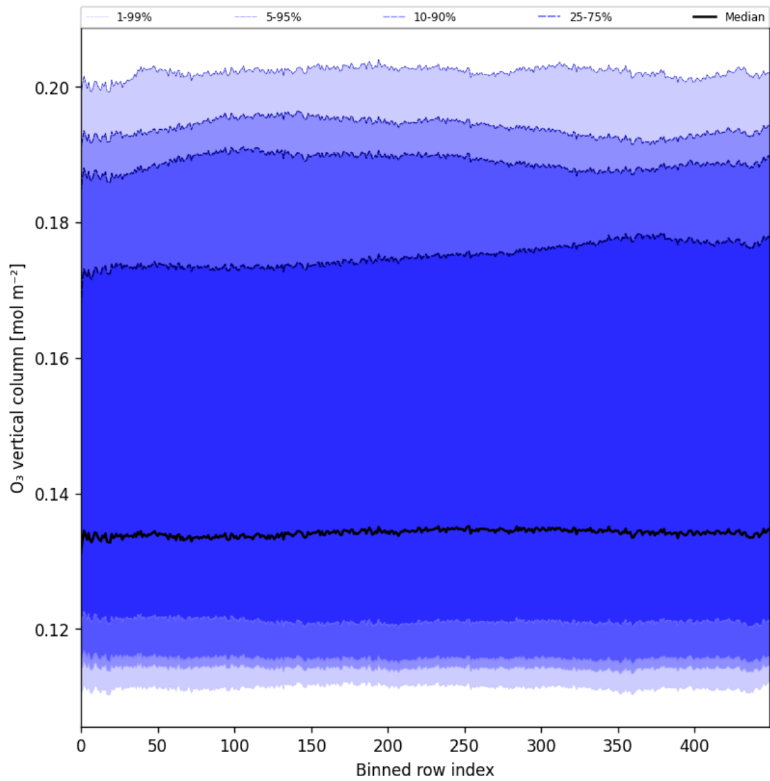
Figure 28: Along track statistics of “ \text{O}_3 vertical column” for 2025-04-19 to 2025-04-20
