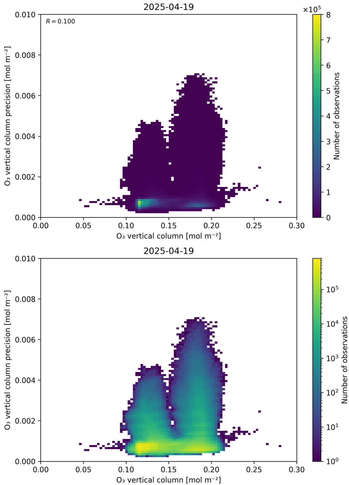
Figure 41: Scatter density plot of “O 3 vertical column” against “O 3 vertical column precision” for 2025-04-19 to 2025-04-20.
