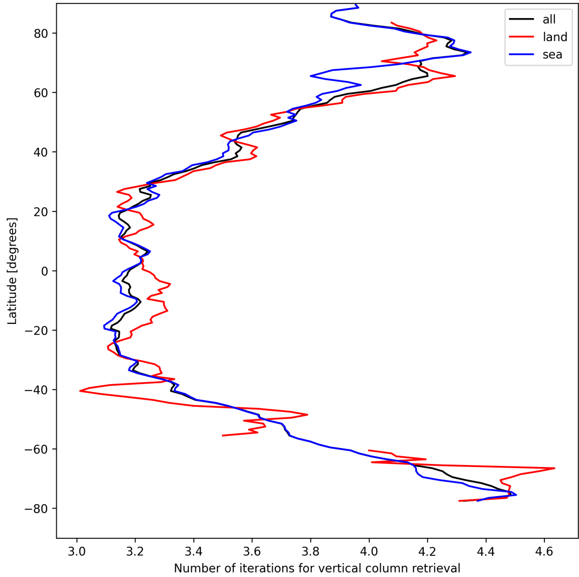
Figure 19: Zonal average of “Number of iterations for vertical column retrieval” for 2025-04-19 to 2025-04-20.
