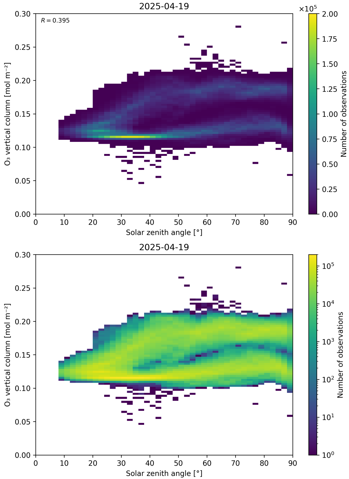
Figure 47: Scatter density plot of “Solar zenith angle” against “O 3 vertical column” for 2025-04-19 to 2025-04-20.
