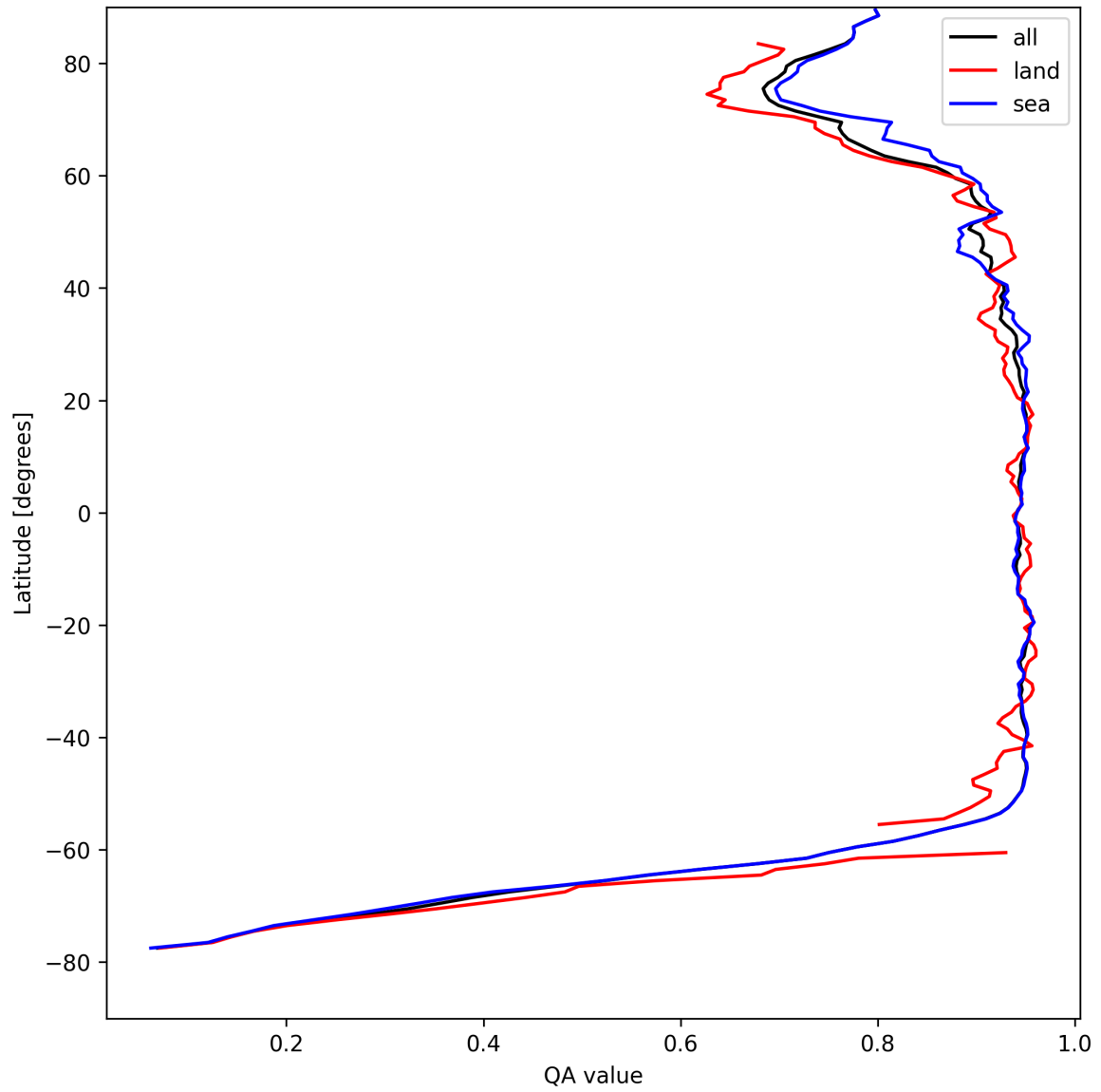
Figure 13: Zonal average of “QA value” for 2025-04-19 to 2025-04-20.
