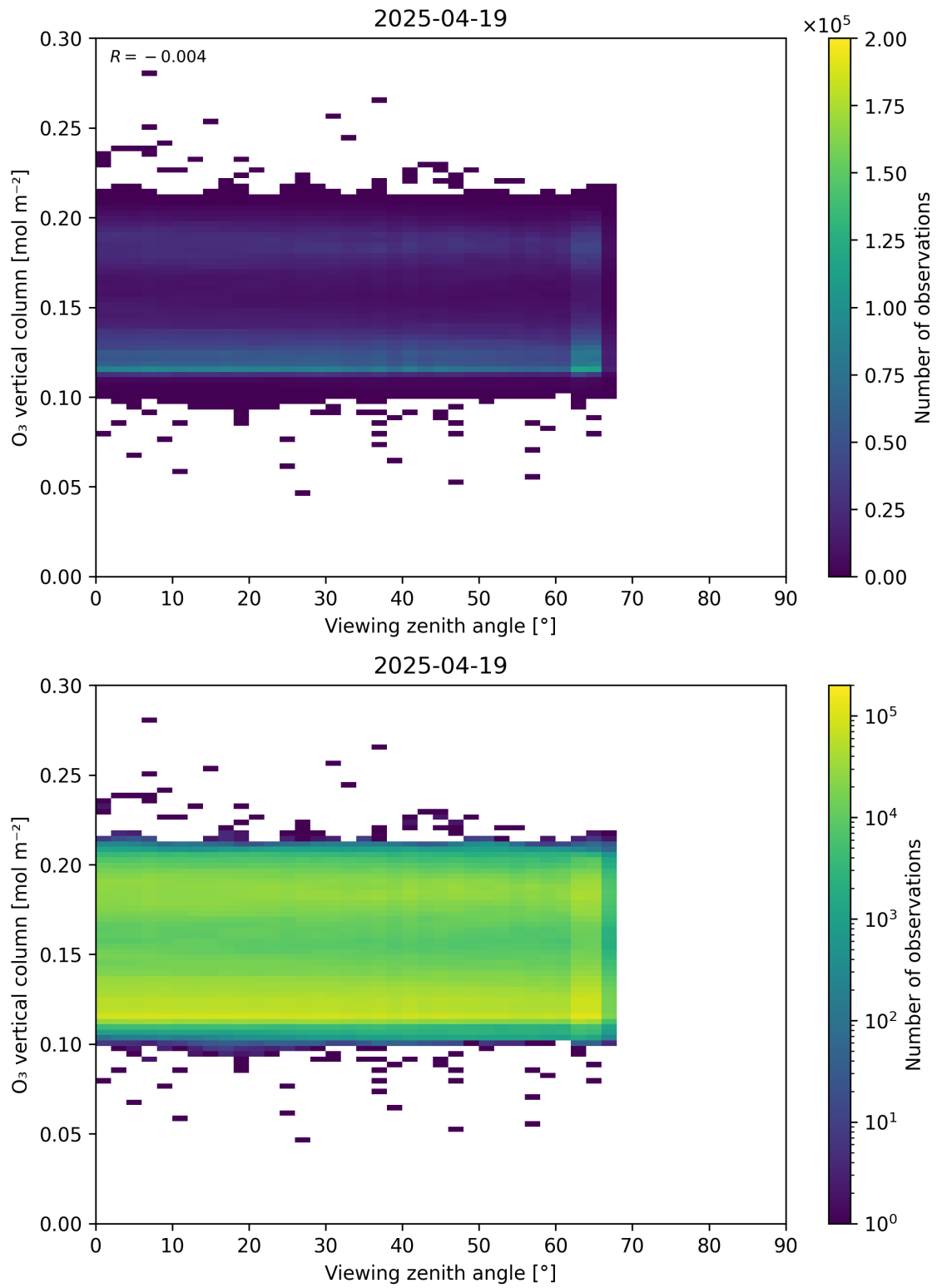
Figure 52: Scatter density plot of “Viewing zenith angle” against “O 3 vertical column” for 2025-04-19 to 2025-04-20.
