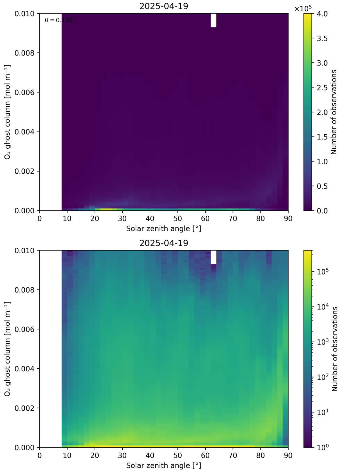
Figure 46: Scatter density plot of “Solar zenith angle” against “O 3 ghost column” for 2025-04-19 to 2025-04-20.
