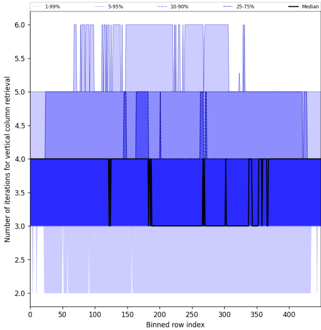
Figure 33: Along track statistics of “Number of iterations for vertical column retrieval” for 2025-04-19 to 2025-04-20
