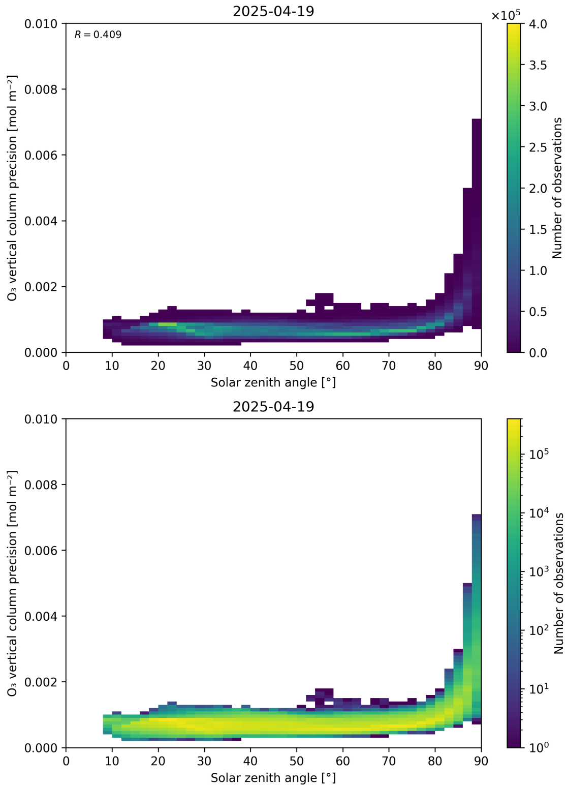
Figure 48: Scatter density plot of “Solar zenith angle” against “O 3 vertical column precision” for 2025-04-19 to 2025-04-20.
