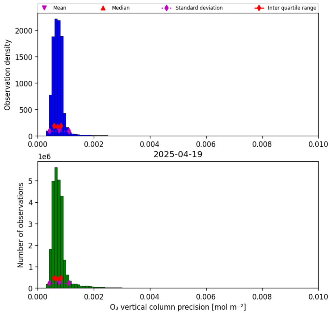
Figure 22: Histogram of “O 3 vertical column precision” for 2025-04-19 to 2025-04-20
