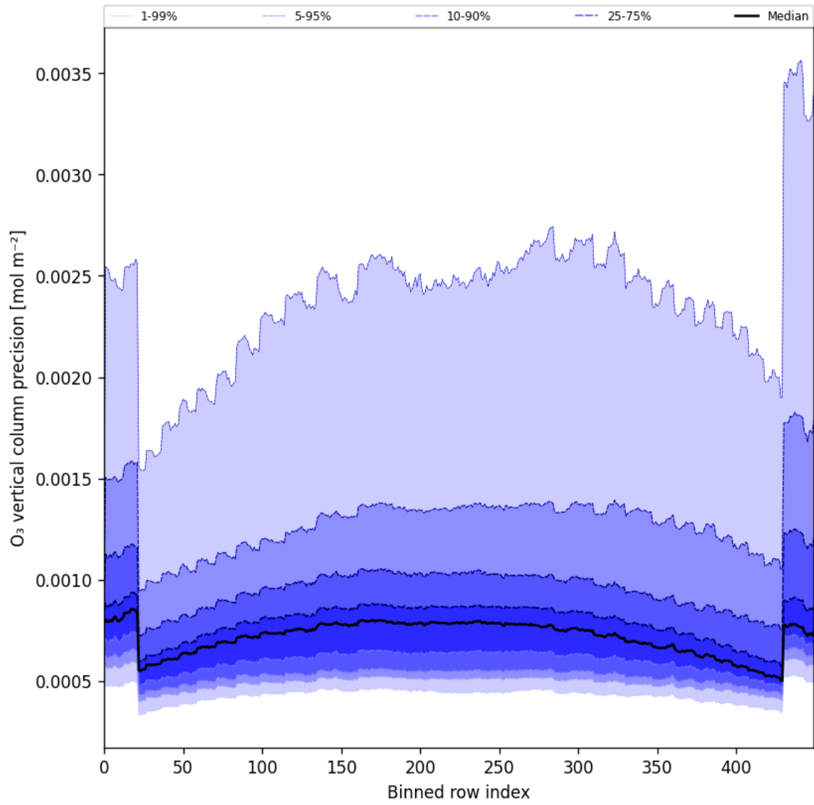
Figure 29: Along track statistics of “O 3 vertical column precision” for 2025-04-19 to 2025-04-20
