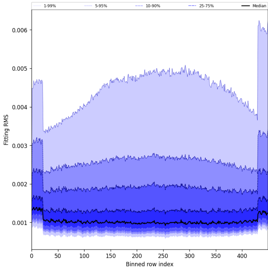
Figure 30: Along track statistics of “Fitting RMS” for 2025-04-19 to 2025-04-20
