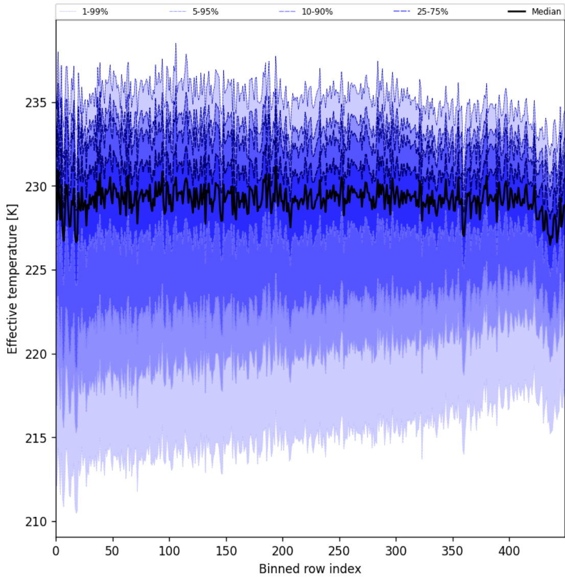
Figure 31: Along track statistics of “Effective temperature” for 2025-04-19 to 2025-04-20
