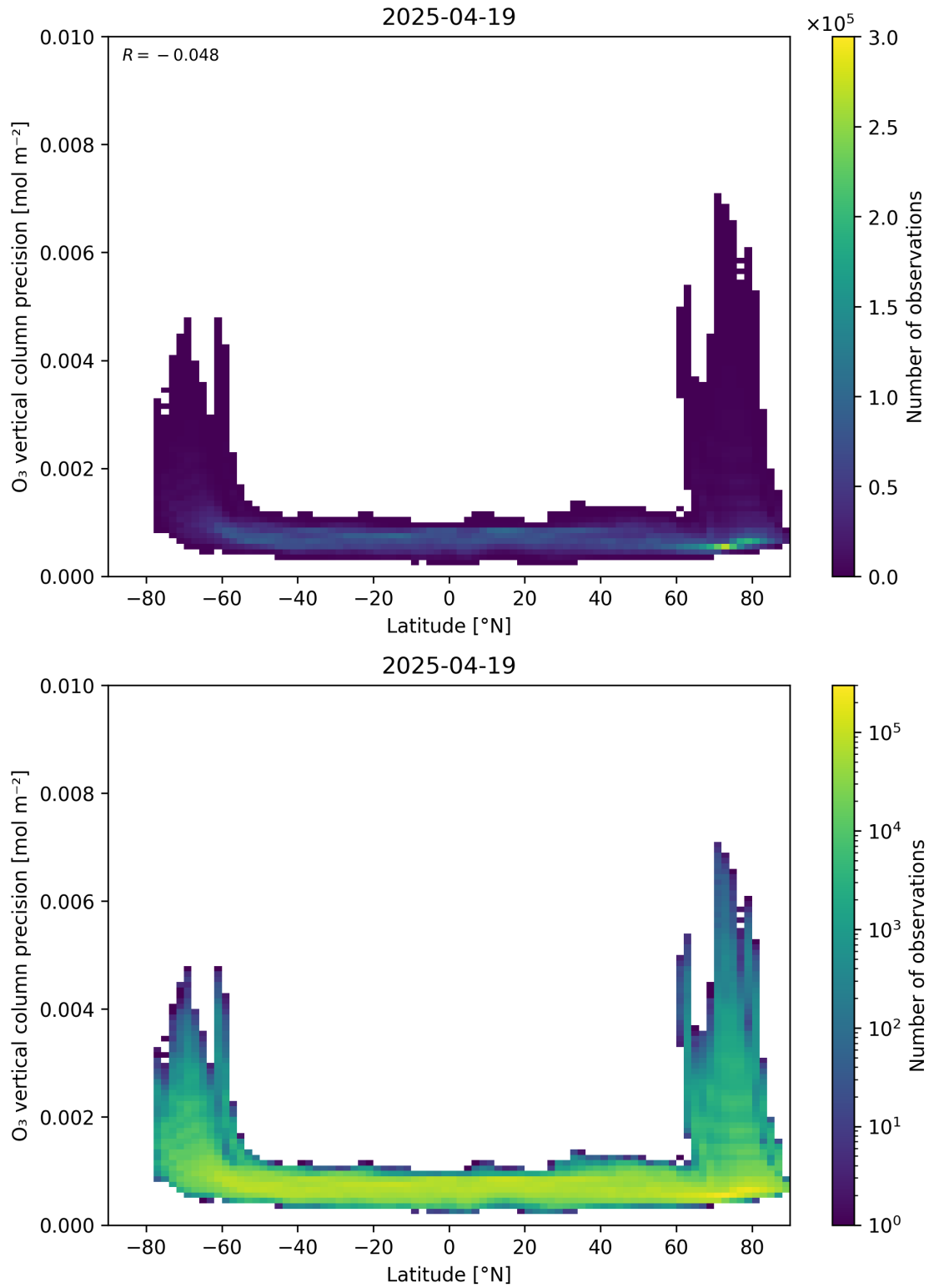
Figure 37: Scatter density plot of “Latitude” against “O 3 vertical column precision” for 2025-04-19 to 2025-04-20.
