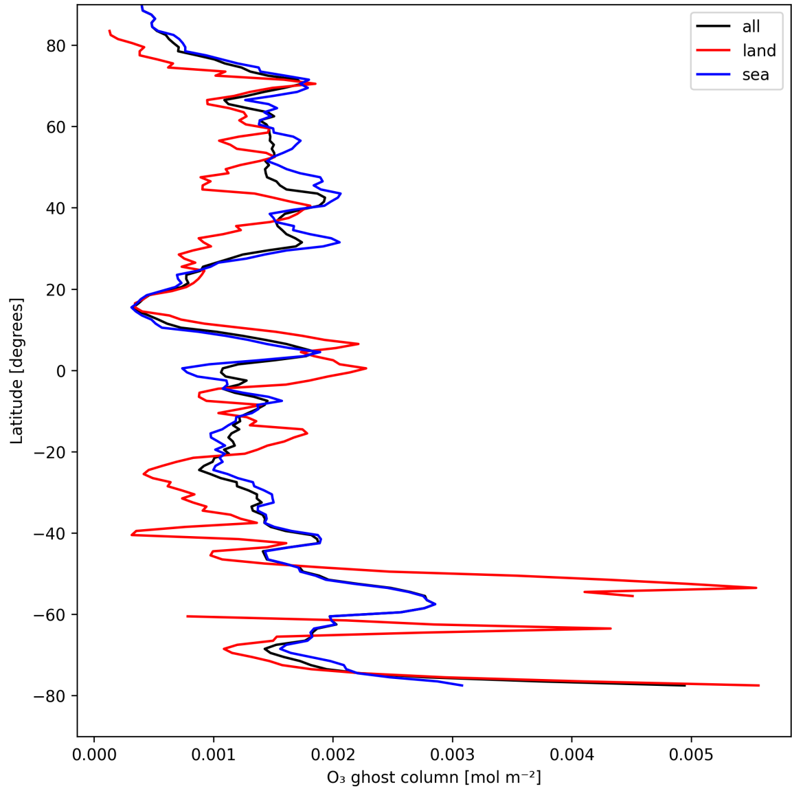
Figure 18: Zonal average of “O 3 ghost column” for 2025-04-19 to 2025-04-20.
