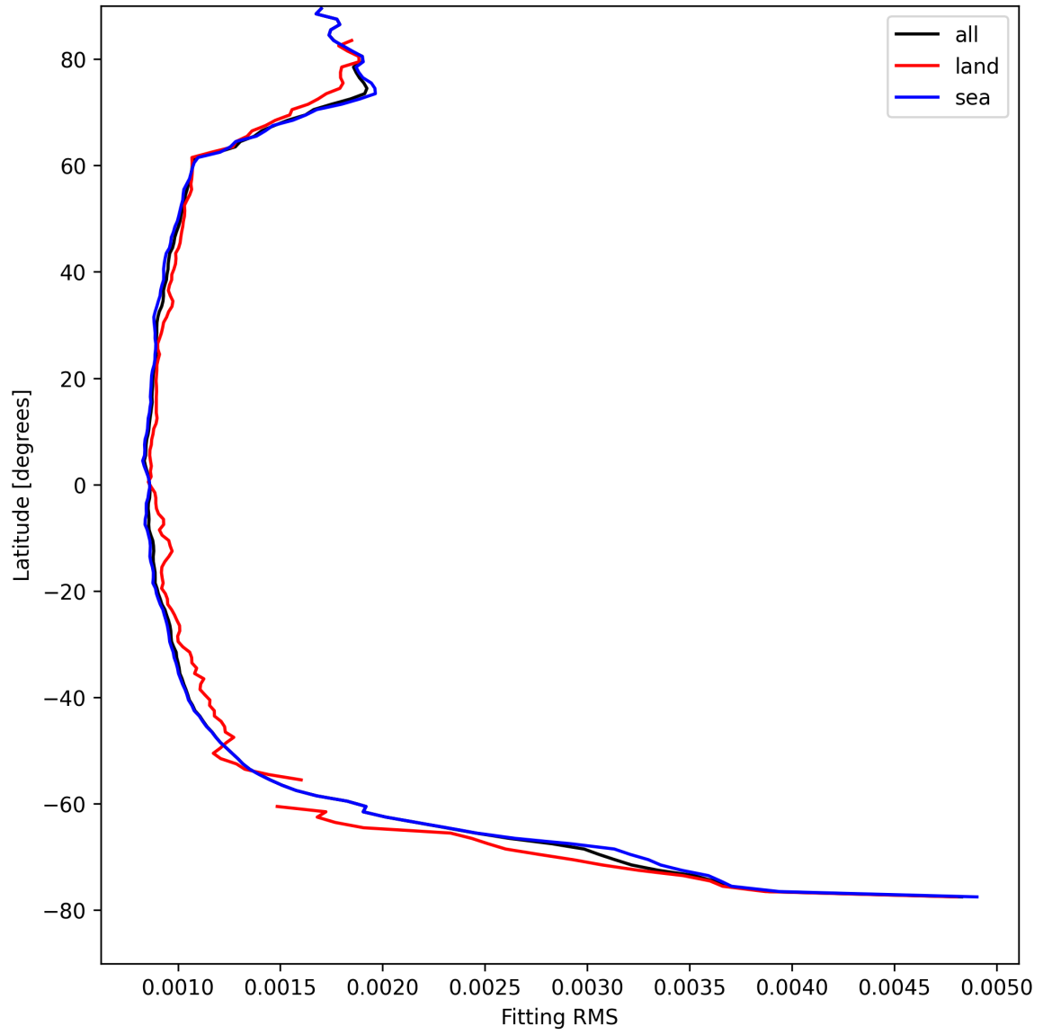
Figure 16: Zonal average of “Fitting RMS” for 2025-04-19 to 2025-04-20.
