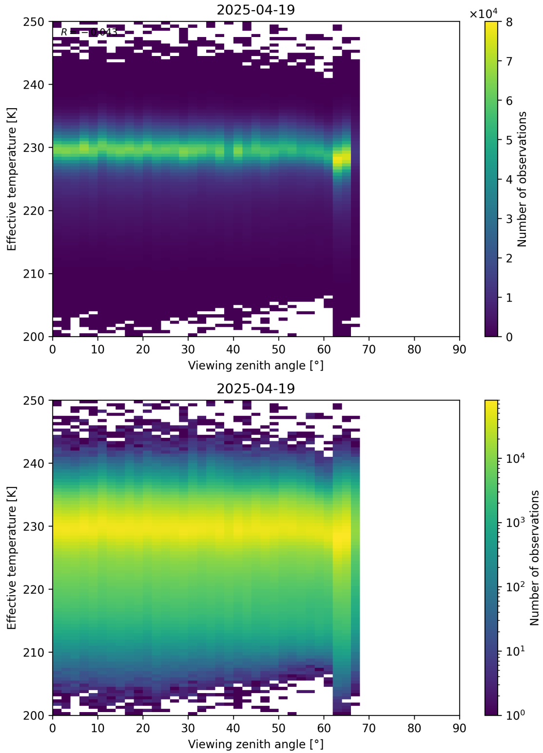
Figure 50: Scatter density plot of “Viewing zenith angle” against “Effective temperature” for 2025-04-19 to 2025-04-20.
