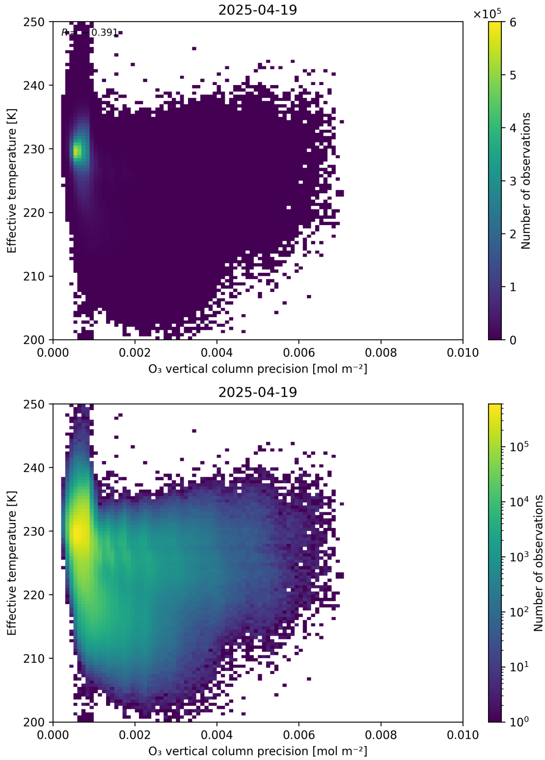
Figure 42: Scatter density plot of “O 3 vertical column precision” against “Effective temperature” for 2025-04-19 to 2025-04-20.
