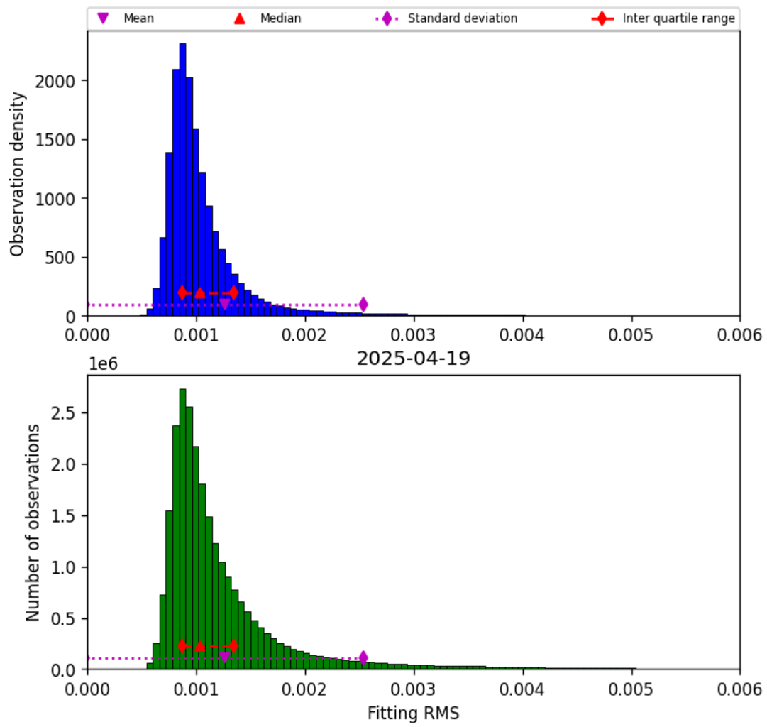
Figure 23: Histogram of “Fitting RMS” for 2025-04-19 to 2025-04-20
