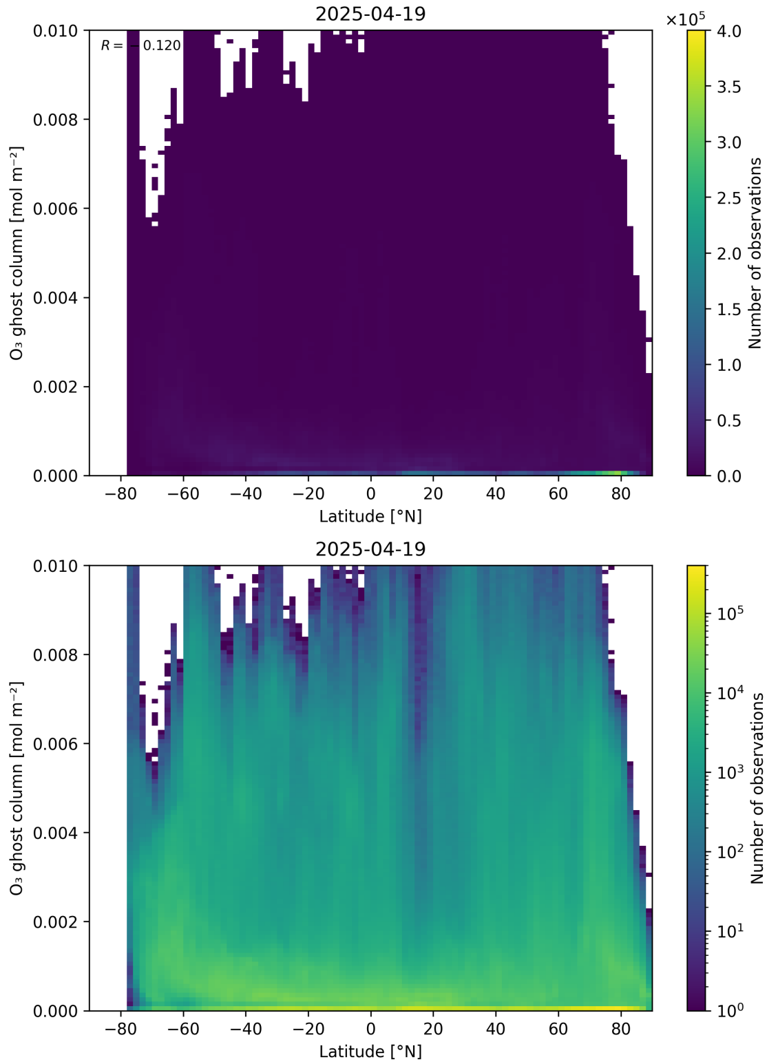
Figure 35: Scatter density plot of “Latitude” against “O 3 ghost column” for 2025-04-19 to 2025-04-20.
