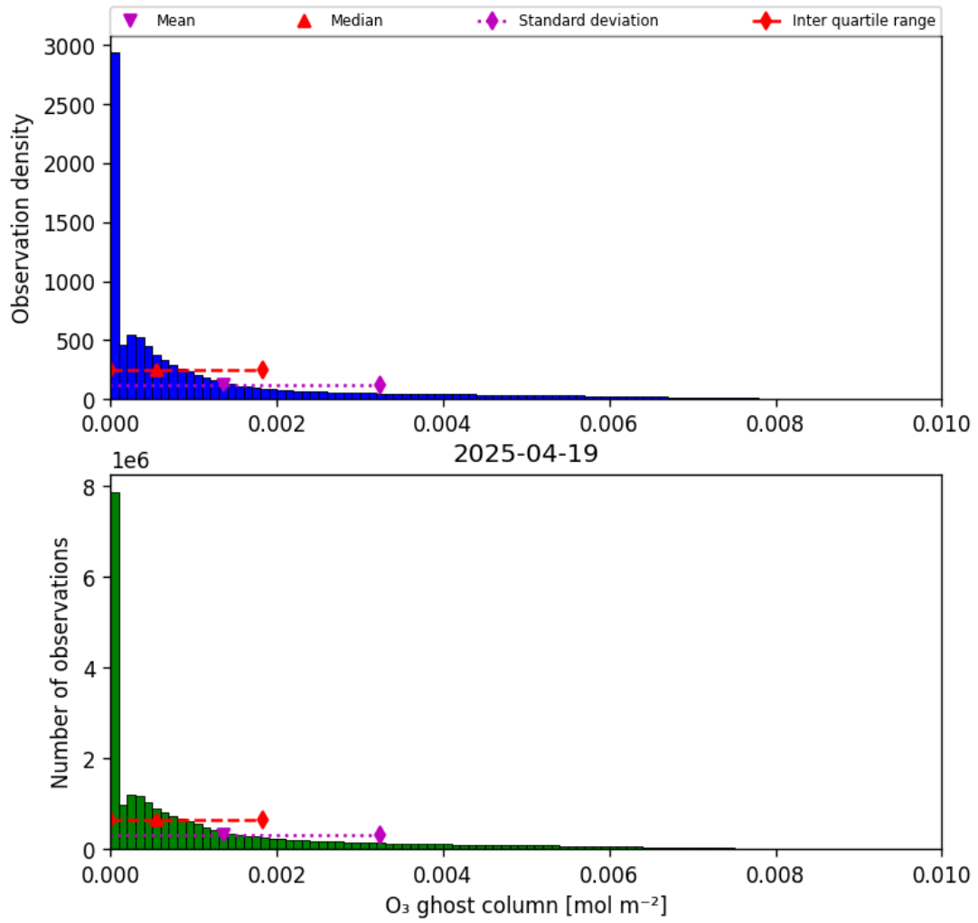
Figure 25: Histogram of “O 3 ghost column” for 2025-04-19 to 2025-04-20
