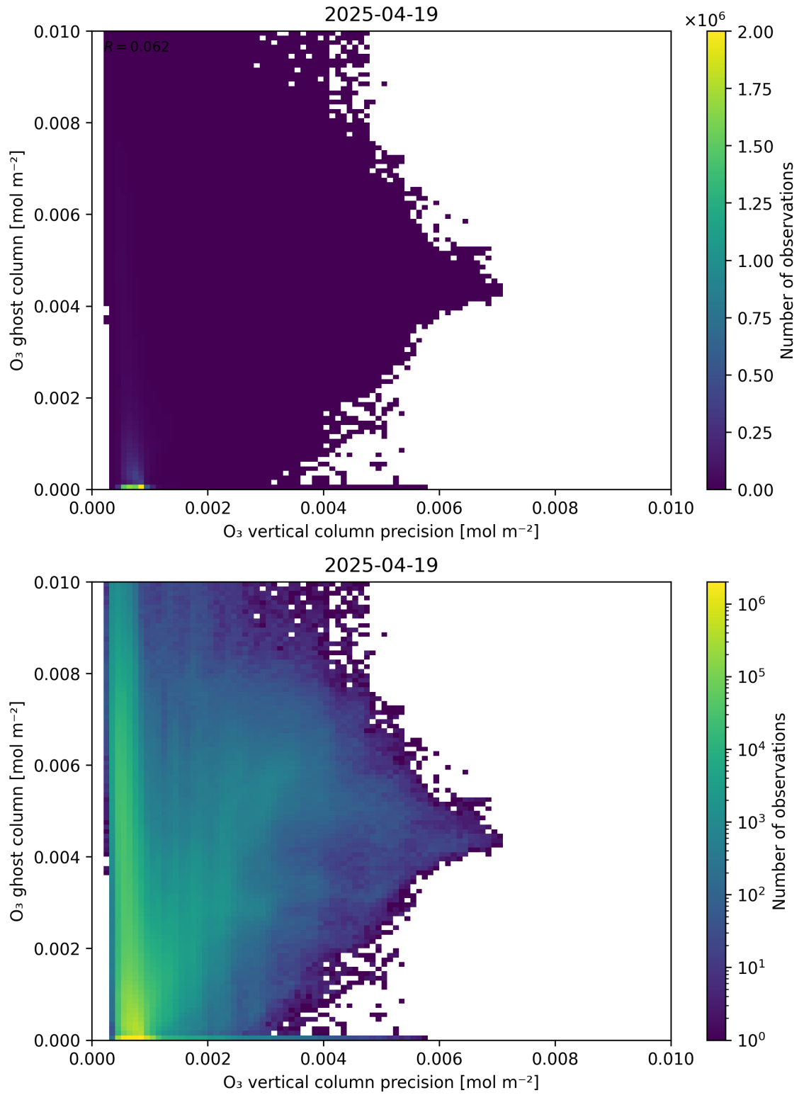
Figure 43: Scatter density plot of “O 3 vertical column precision” against “O 3 ghost column” for 2025-04-19 to 2025-04-20.
