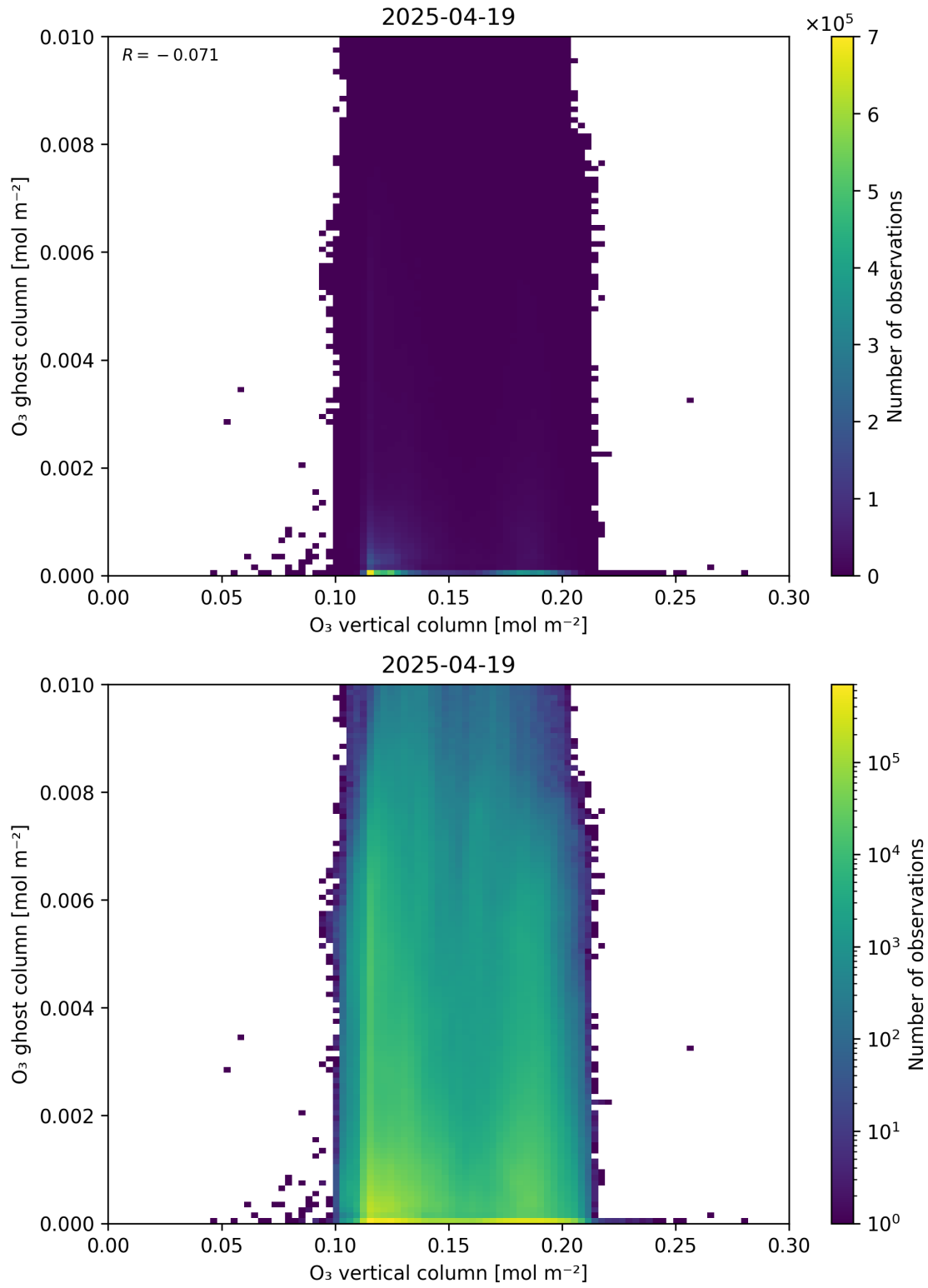
Figure 40: Scatter density plot of “O 3 vertical column” against “O 3 ghost column” for 2025-04-19 to 2025-04-20.
