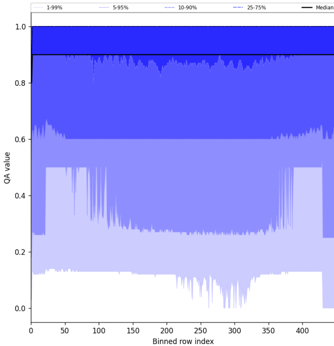
Figure 27: Along track statistics of “QA value” for 2025-04-19 to 2025-04-20
