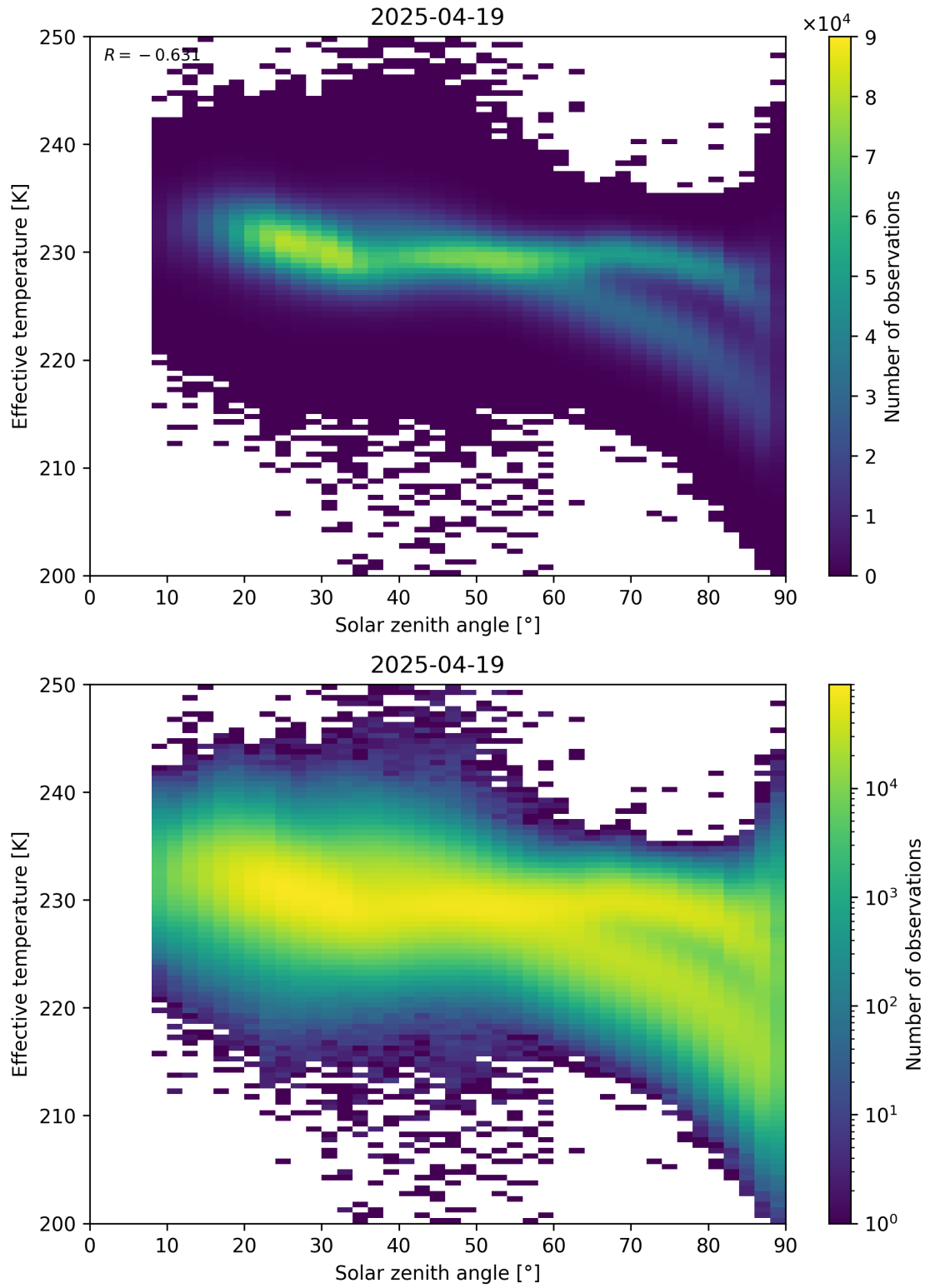
Figure 45: Scatter density plot of “Solar zenith angle” against “Effective temperature” for 2025-04-19 to 2025-04-20.
