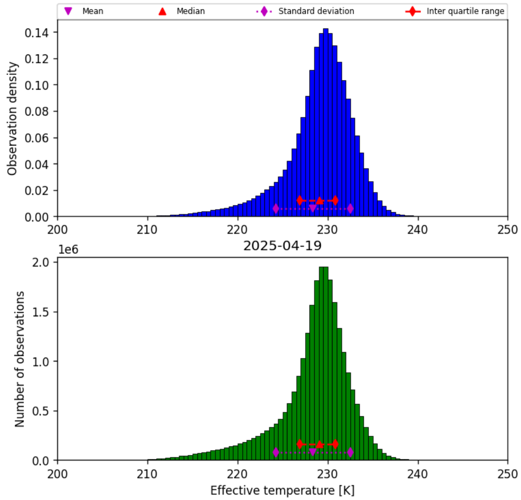
Figure 24: Histogram of “Effective temperature” for 2025-04-19 to 2025-04-20
