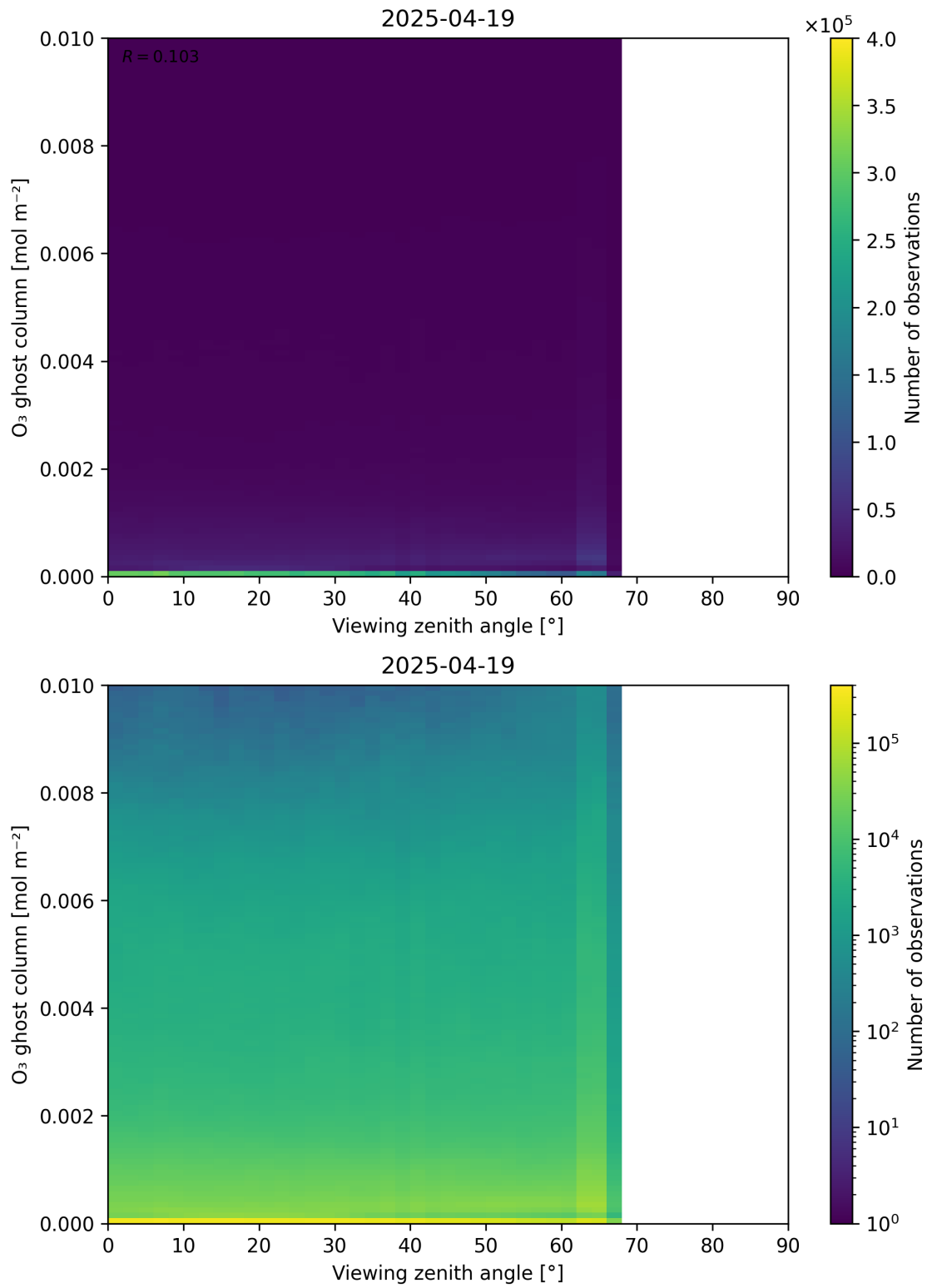
Figure 51: Scatter density plot of “Viewing zenith angle” against “O 3 ghost column” for 2025-04-19 to 2025-04-20.
