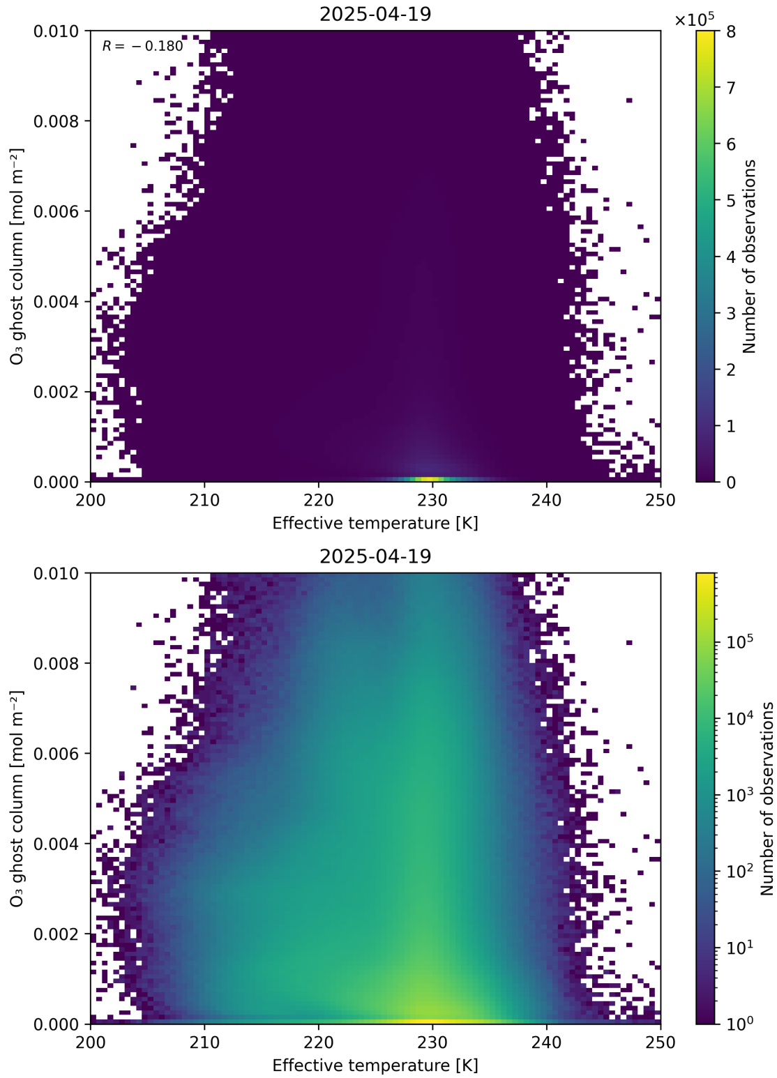
Figure 38: Scatter density plot of “Effective temperature” against “O 3 ghost column” for 2025-04-19 to 2025-04-20.
