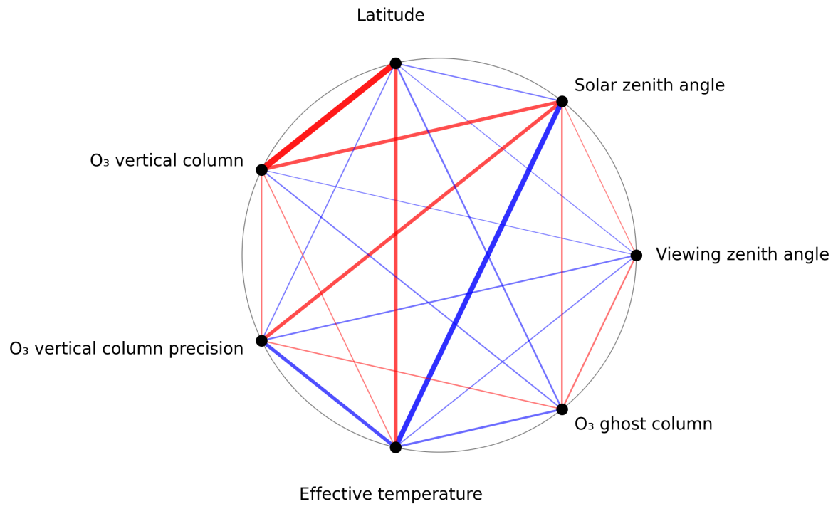
Figure 1: Map of correlation graph for 2025-04-19 to 2025-04-20.
