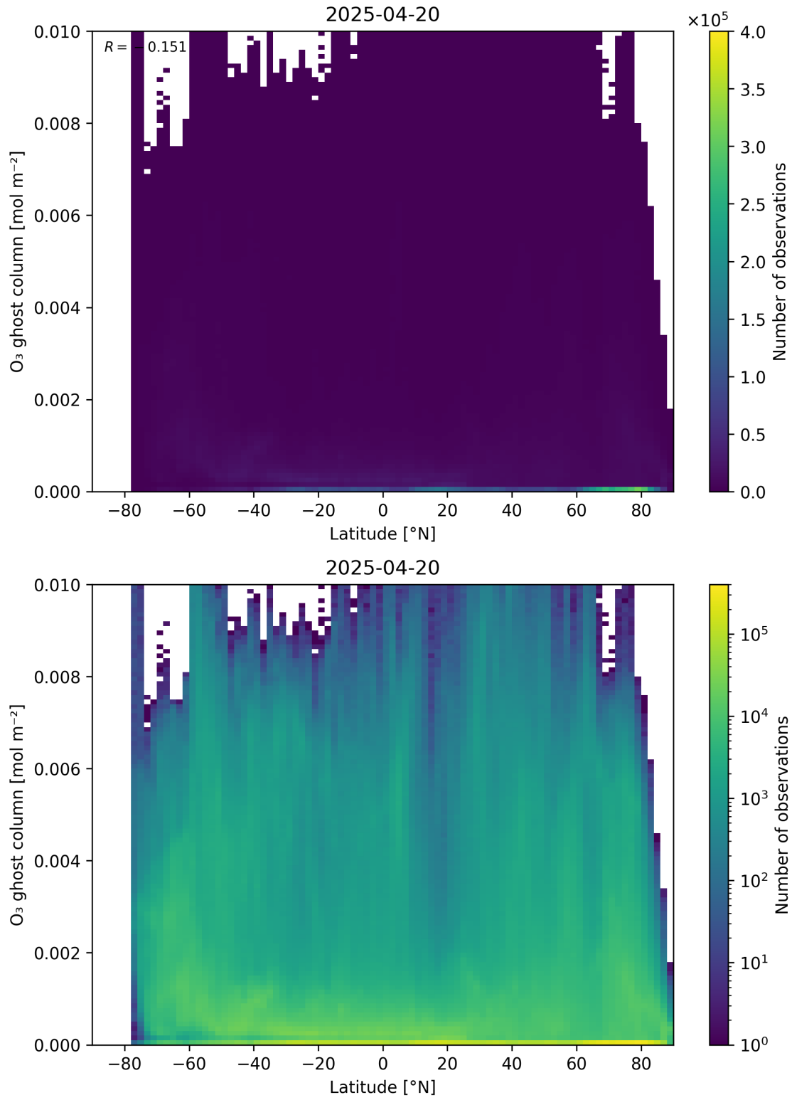
Figure 35: Scatter density plot of “Latitude” against “O 3 ghost column” for 2025-04-19 to 2025-04-21.
