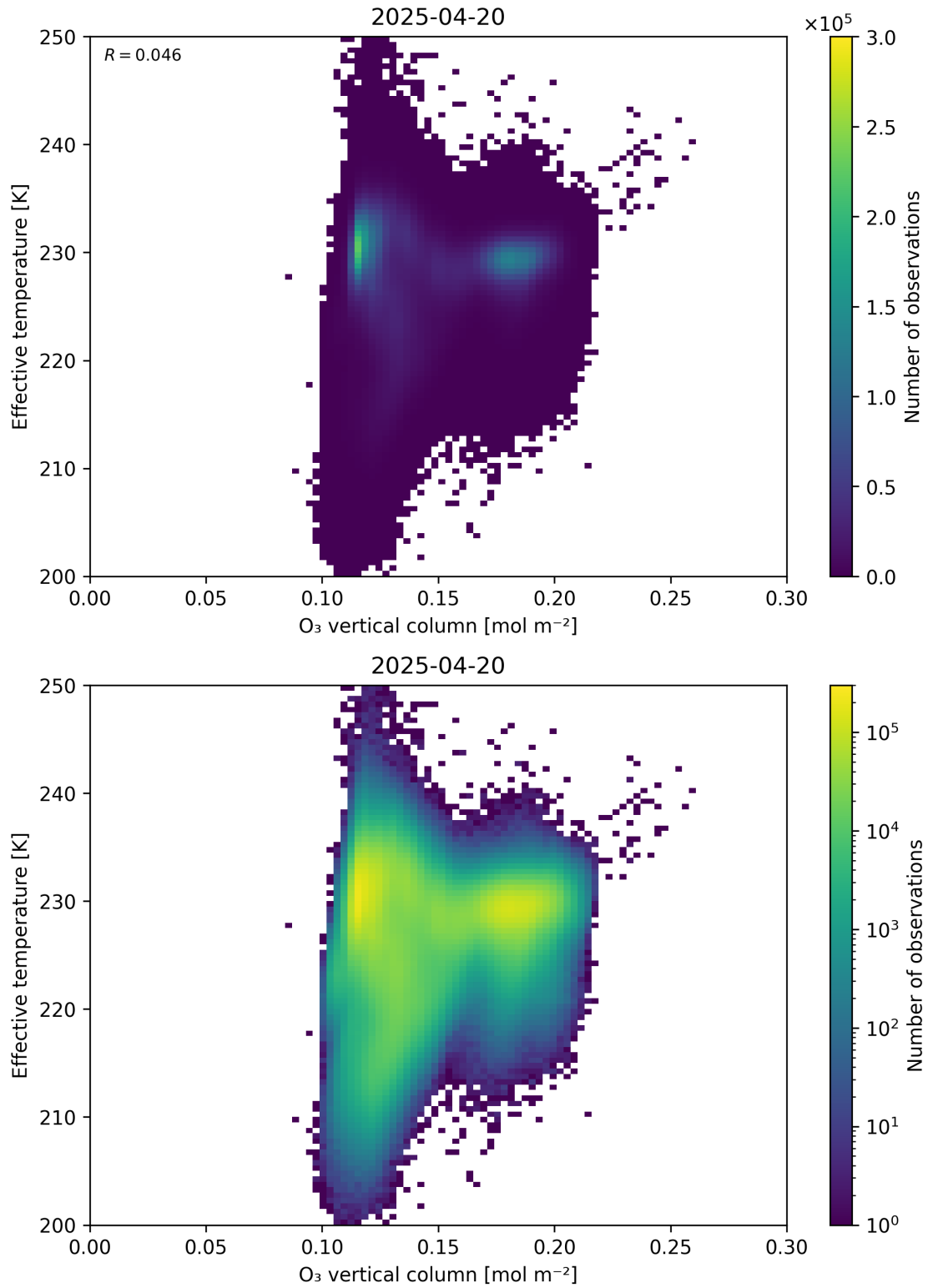
Figure 39: Scatter density plot of “O 3 vertical column” against “Effective temperature” for 2025-04-19 to 2025-04-21.
