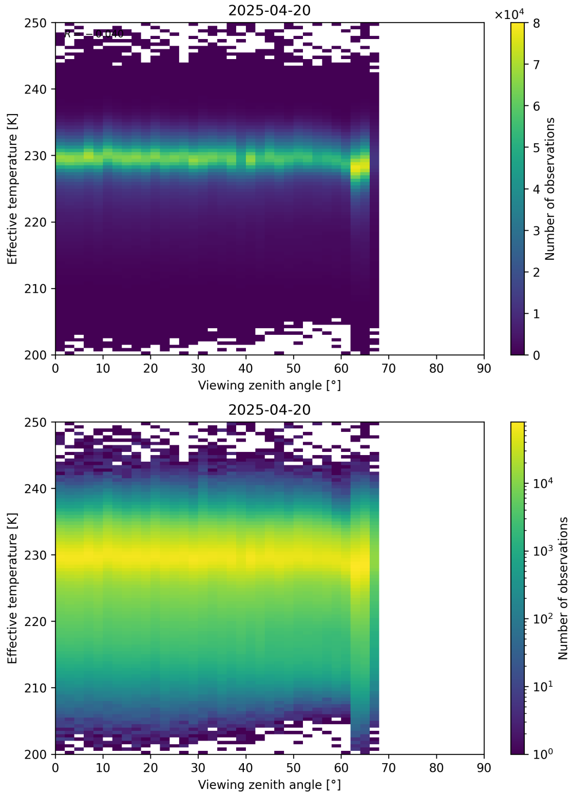
Figure 50: Scatter density plot of “Viewing zenith angle” against “Effective temperature” for 2025-04-19 to 2025-04-21.
