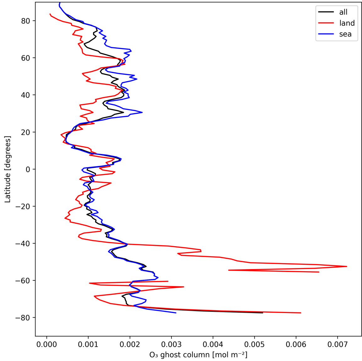
Figure 18: Zonal average of “O 3 ghost column” for 2025-04-19 to 2025-04-21.
