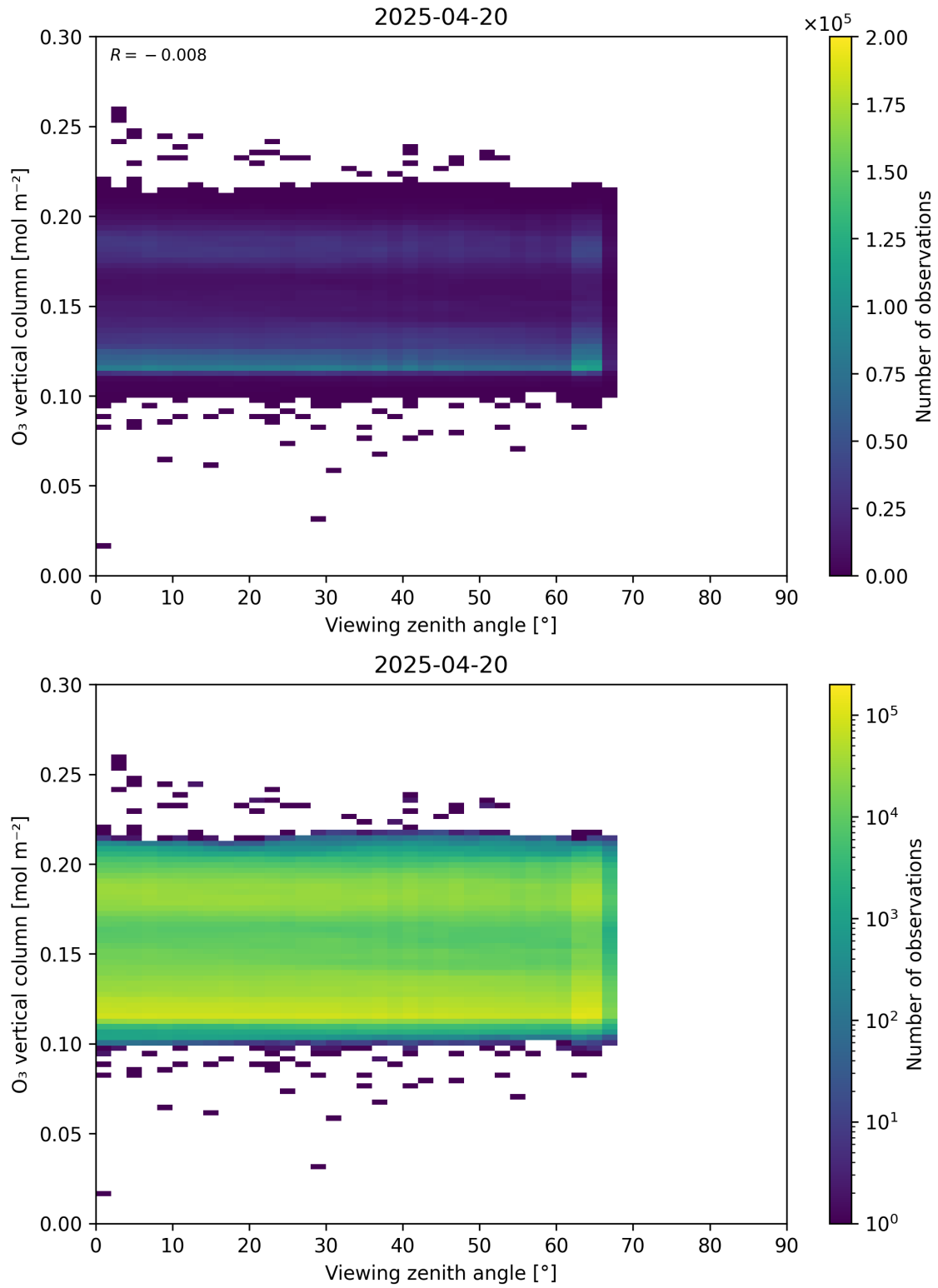
Figure 52: Scatter density plot of “Viewing zenith angle” against “O 3 vertical column” for 2025-04-19 to 2025-04-21.
