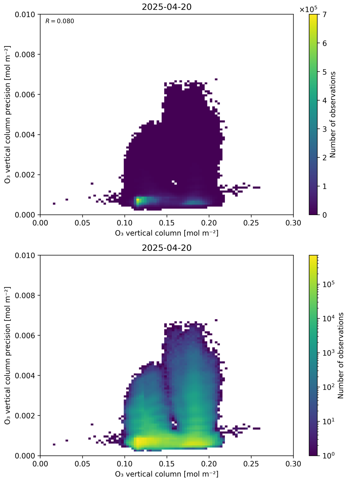
Figure 41: Scatter density plot of “O 3 vertical column” against “O 3 vertical column precision” for 2025-04-19 to 2025-04-21.
