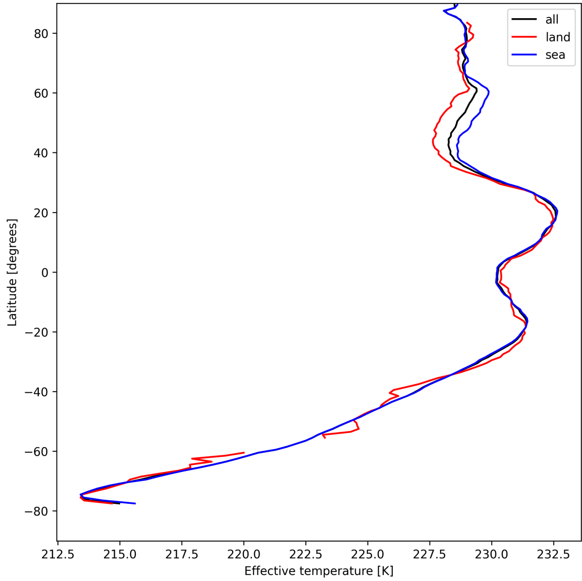
Figure 17: Zonal average of "Effective temperature" for 2025-04-19 to 2025-04-21.
