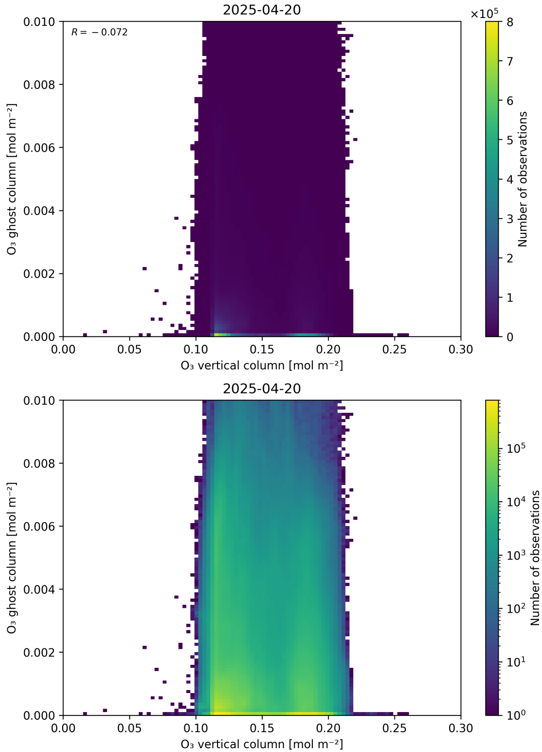
Figure 40: Scatter density plot of “O 3 vertical column” against “O 3 ghost column” for 2025-04-19 to 2025-04-21.
