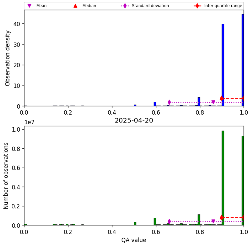
Figure 20: Histogram of “QA value” for 2025-04-19 to 2025-04-21
