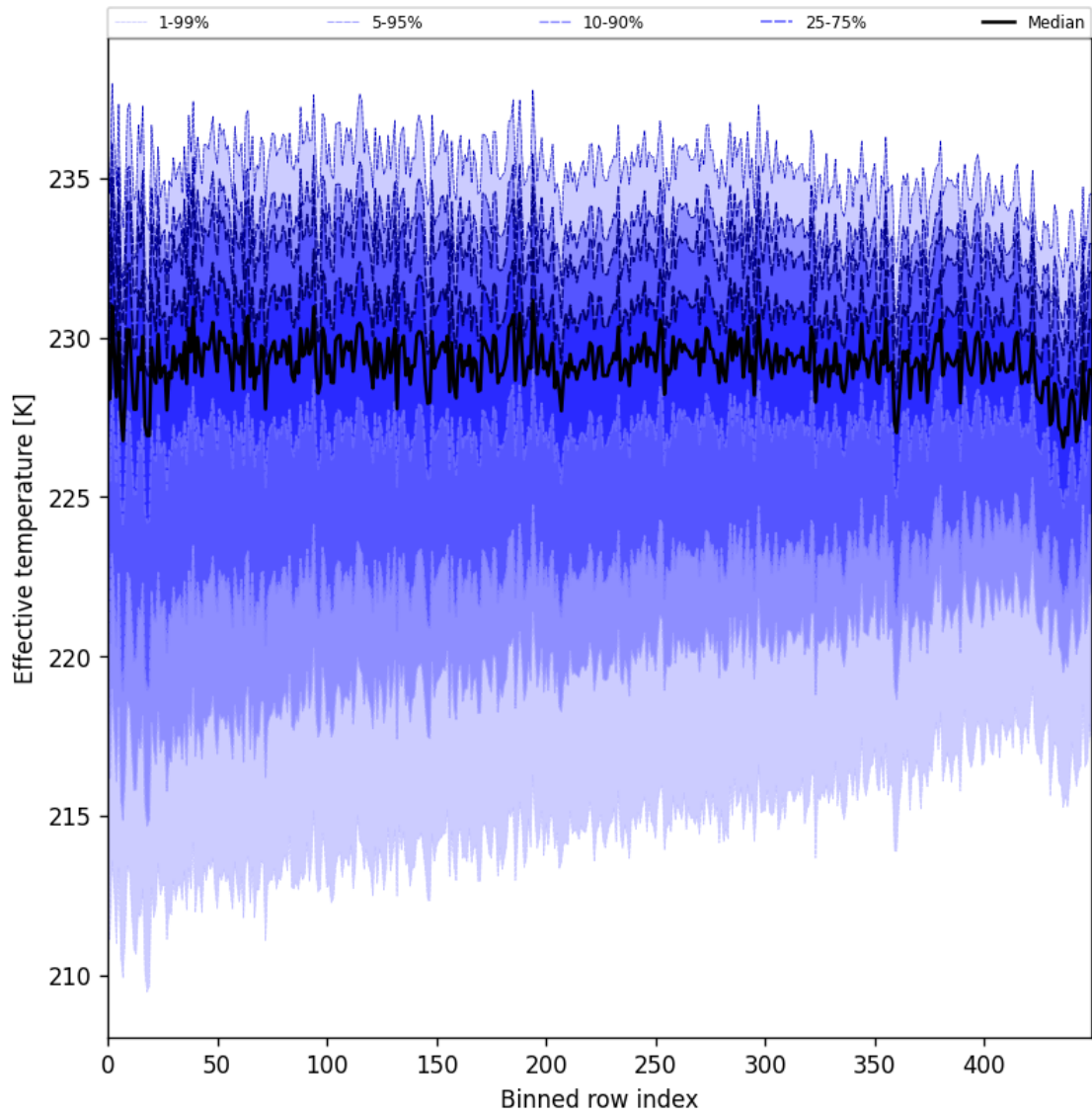
Figure 31: Along track statistics of “Effective temperature” for 2025-04-19 to 2025-04-21
