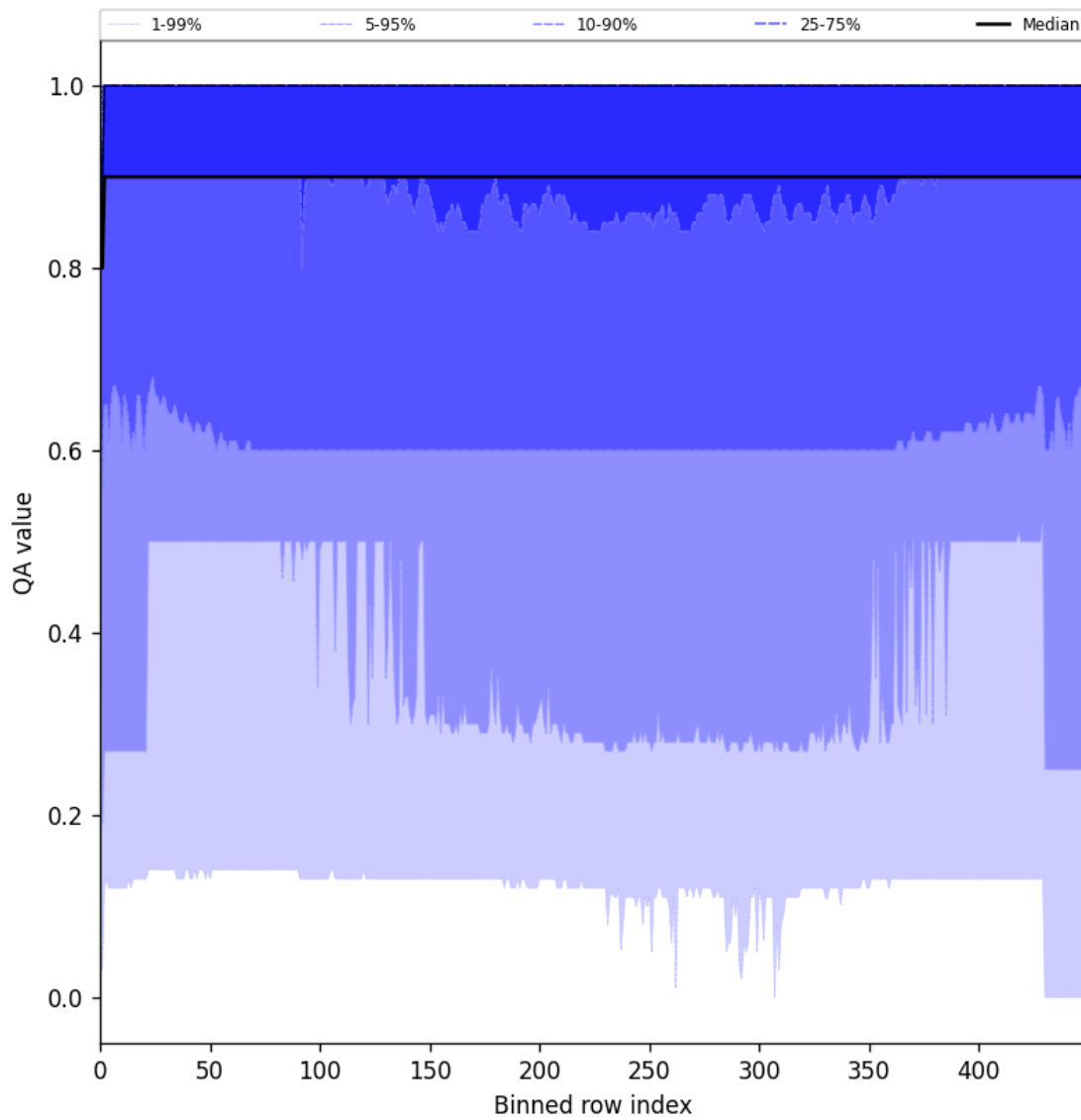
Figure 27: Along track statistics of “QA value” for 2025-04-19 to 2025-04-21
