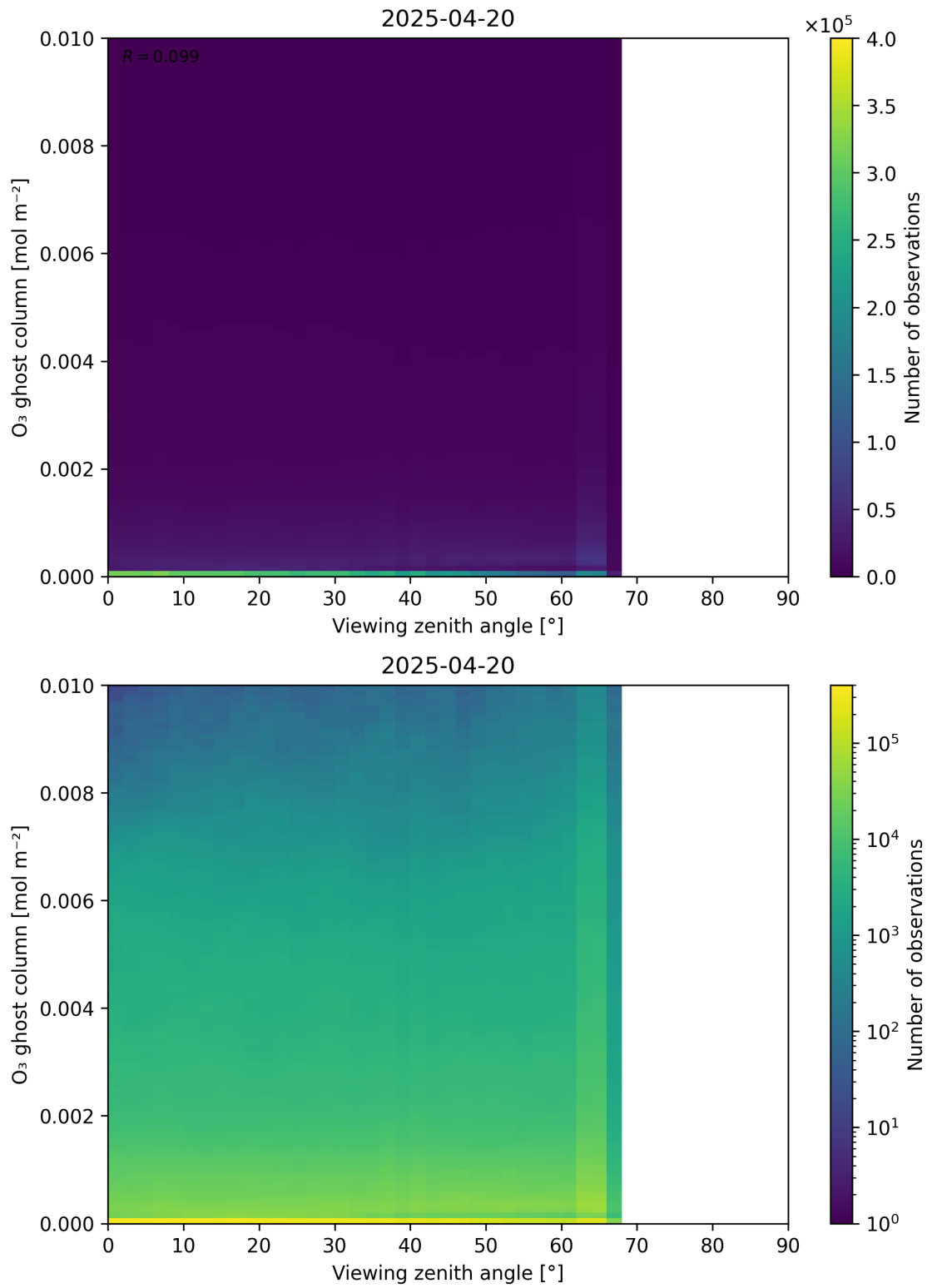
Figure 51: Scatter density plot of “Viewing zenith angle” against “O 3 ghost column” for 2025-04-19 to 2025-04-21.
