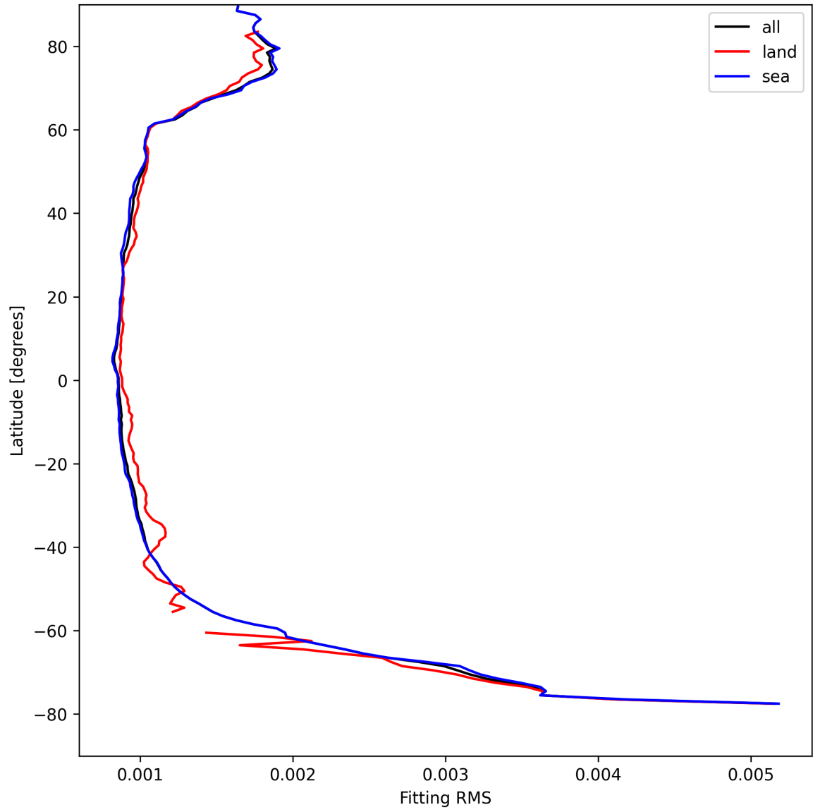
Figure 16: Zonal average of “Fitting RMS” for 2025-04-19 to 2025-04-21.
