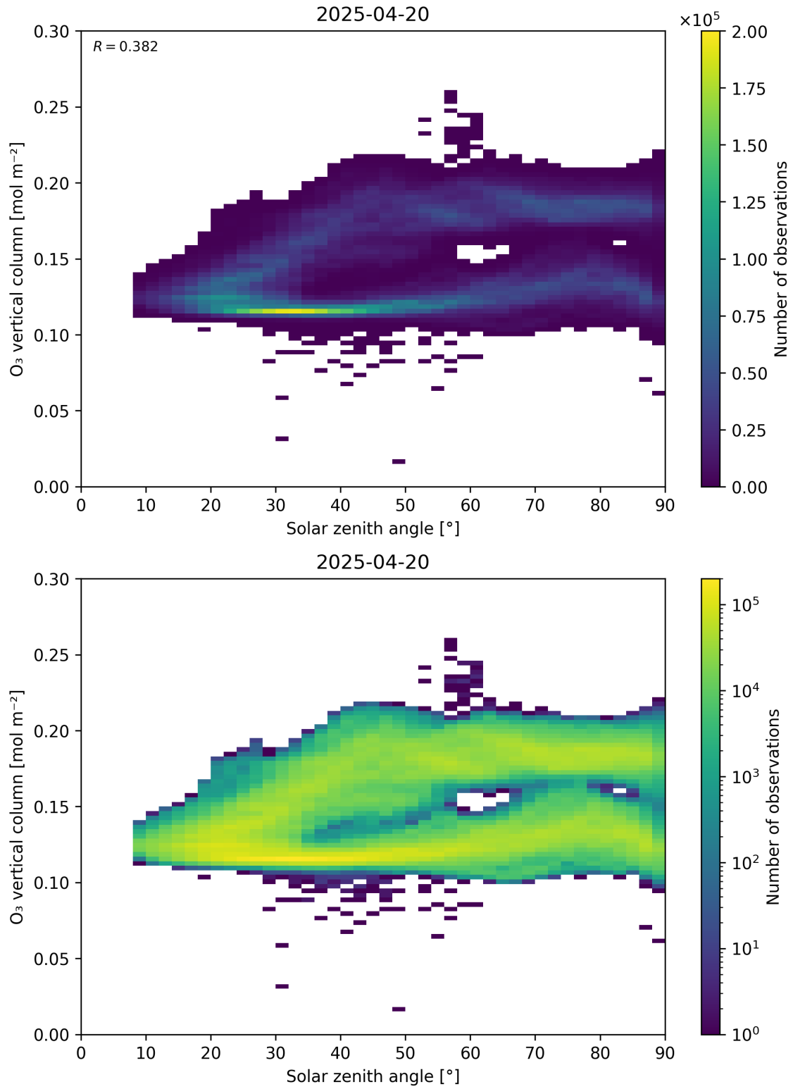
Figure 47: Scatter density plot of “Solar zenith angle” against “O 3 vertical column” for 2025-04-19 to 2025-04-21.
