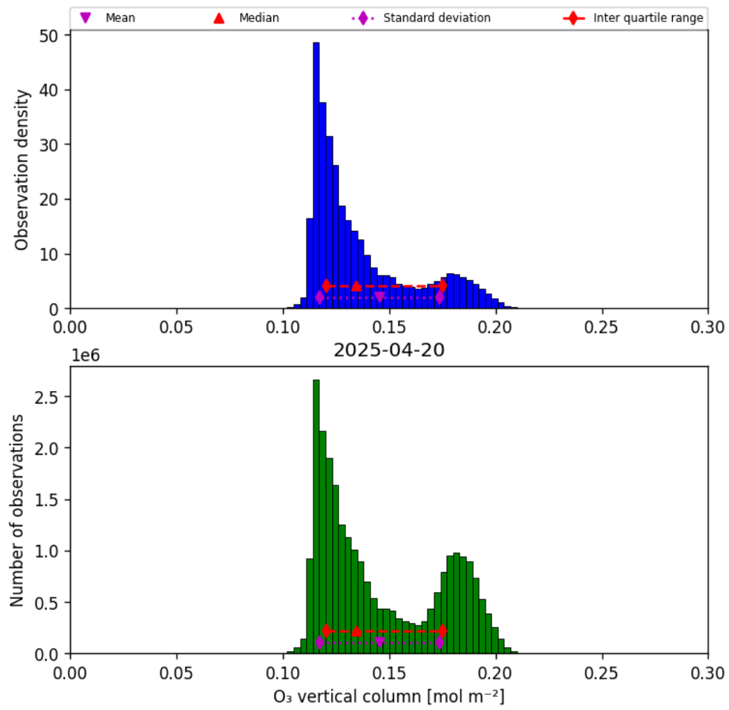
Figure 21: Histogram of “O 3 vertical column” for 2025-04-19 to 2025-04-21
