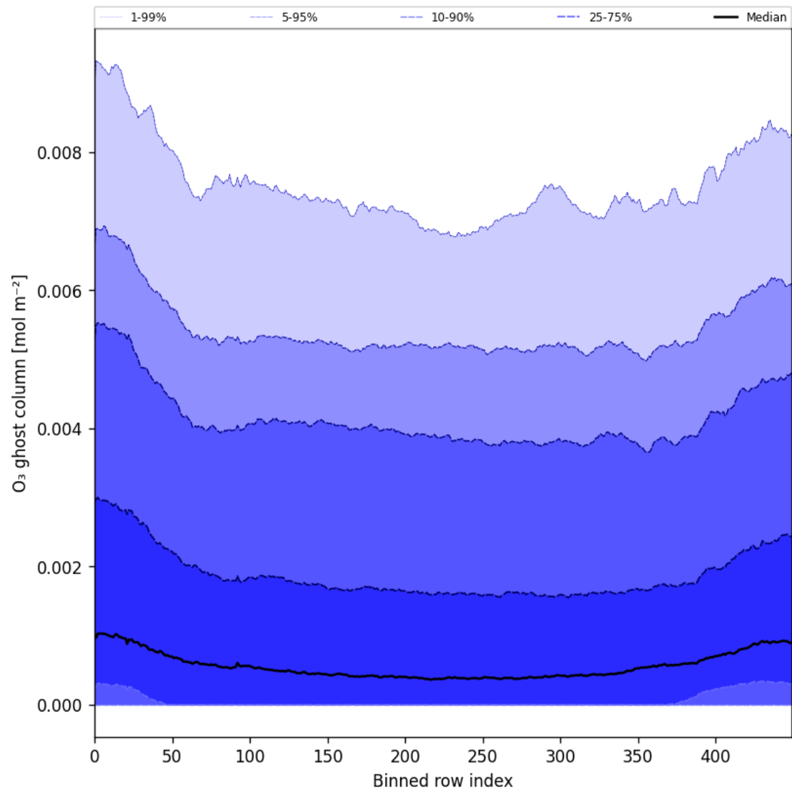
Figure 32: Along track statistics of “O 3 ghost column” for 2025-04-19 to 2025-04-21
