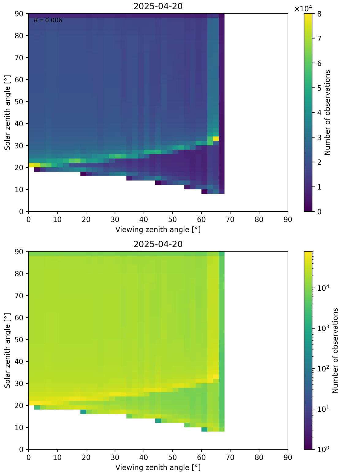
Figure 54: Scatter density plot of “Viewing zenith angle” against “Solar zenith angle” for 2025-04-19 to 2025-04-21.
