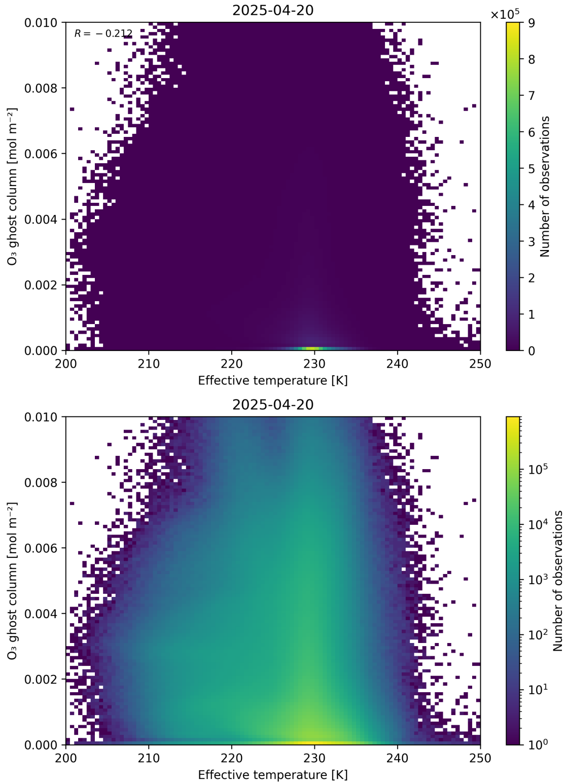
Figure 38: Scatter density plot of “Effective temperature” against “O 3 ghost column” for 2025-04-19 to 2025-04-21.
