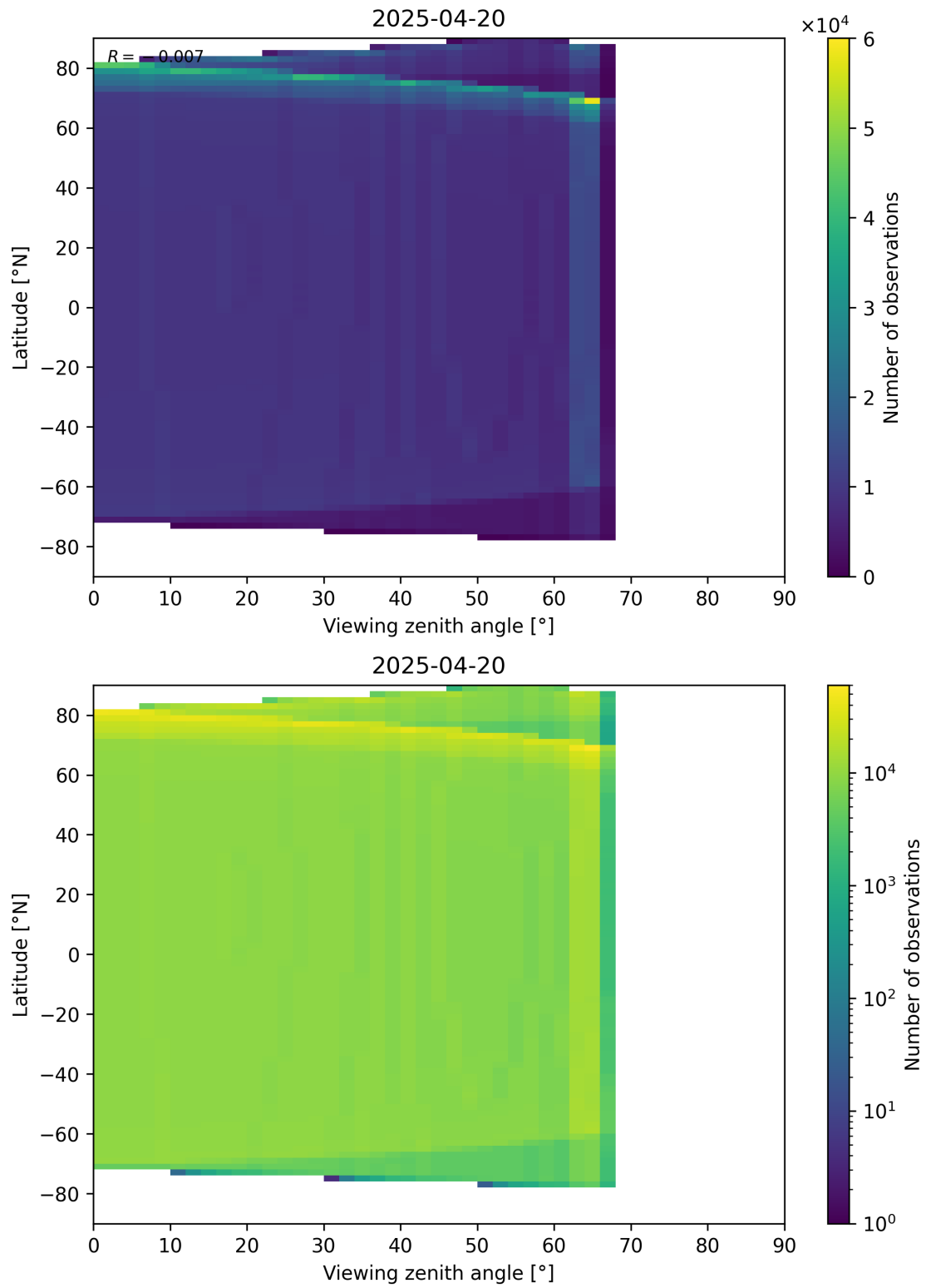
Figure 49: Scatter density plot of “Viewing zenith angle” against “Latitude” for 2025-04-19 to 2025-04-21.
