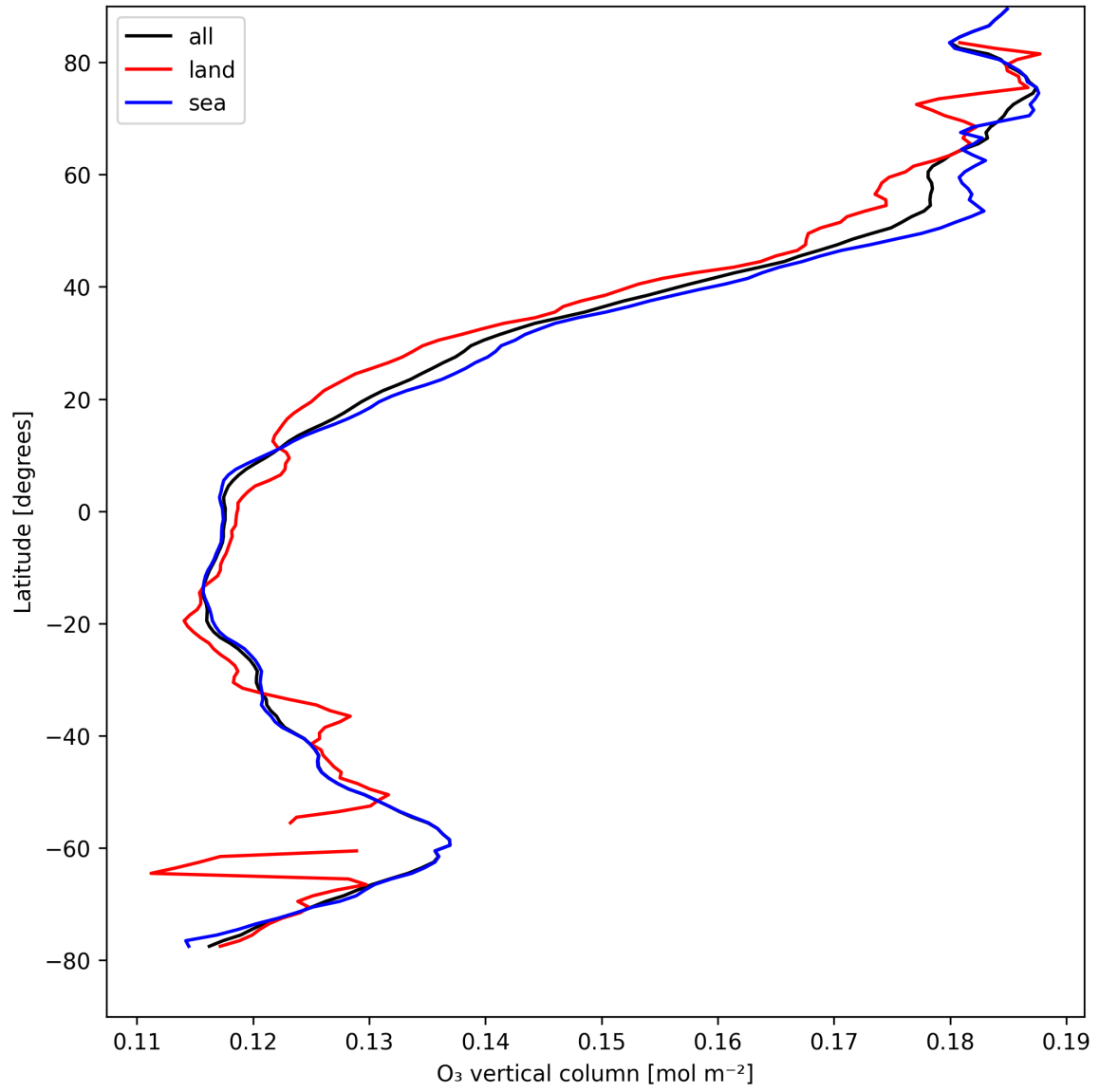
Figure 14: Zonal average of “O 3 vertical column” for 2025-04-19 to 2025-04-21.
