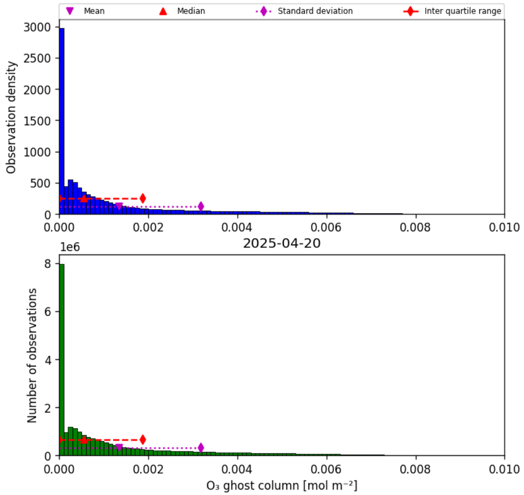
Figure 25: Histogram of “O 3 ghost column” for 2025-04-19 to 2025-04-21
