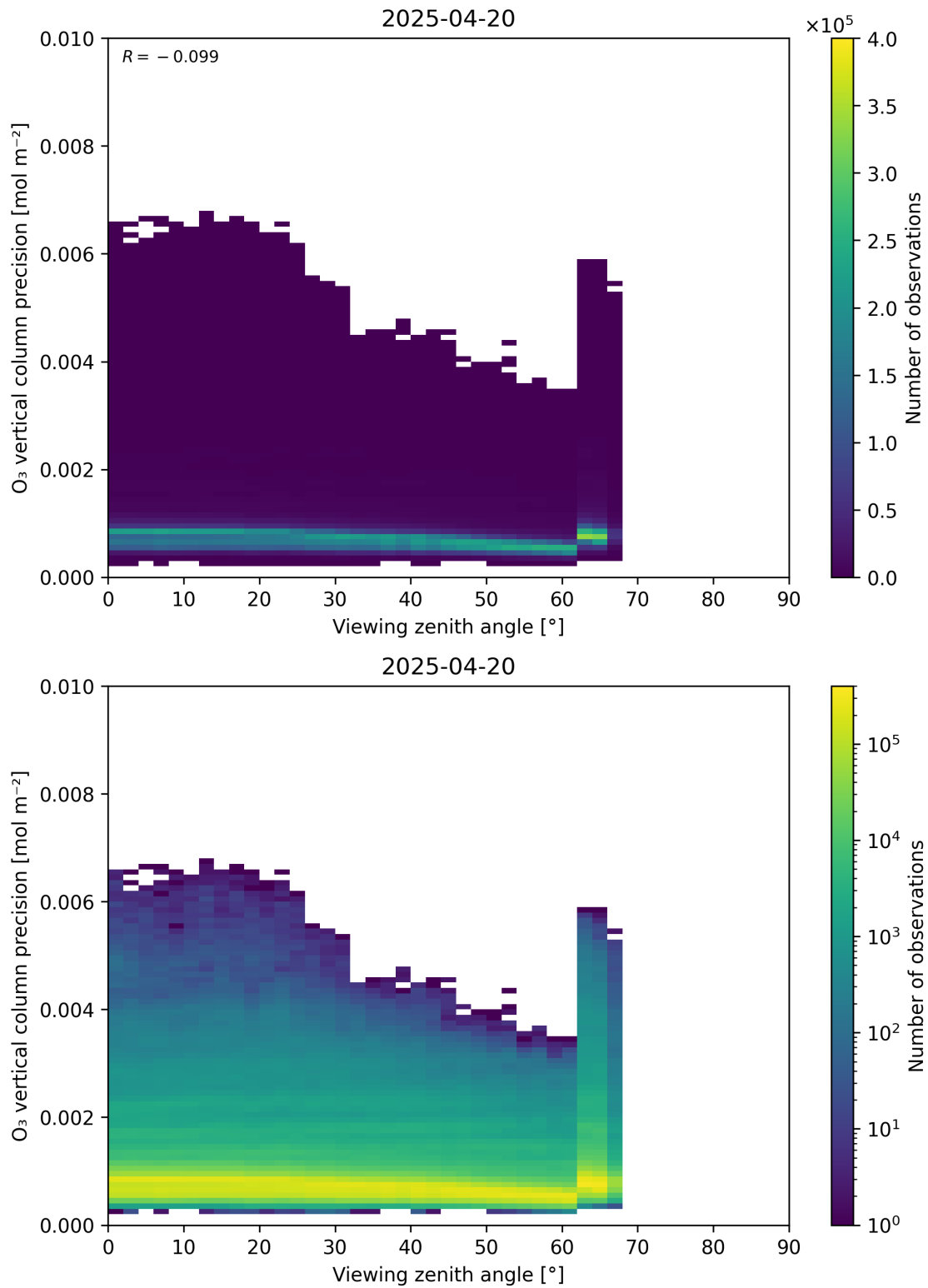
Figure 53: Scatter density plot of “Viewing zenith angle” against “O 3 vertical column precision” for 2025-04-19 to 2025-04-21.
