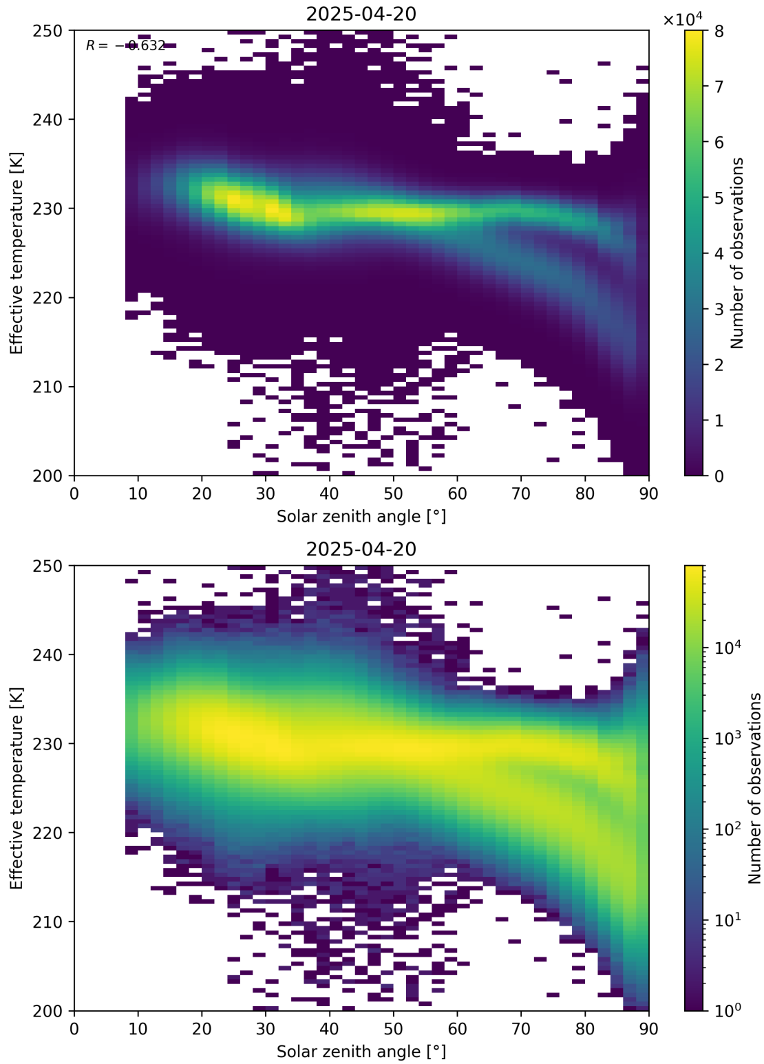
Figure 45: Scatter density plot of “Solar zenith angle” against “Effective temperature” for 2025-04-19 to 2025-04-21.
