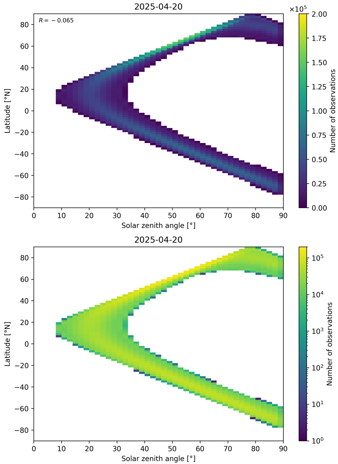
Figure 44: Scatter density plot of “Solar zenith angle” against “Latitude” for 2025-04-19 to 2025-04-21.
