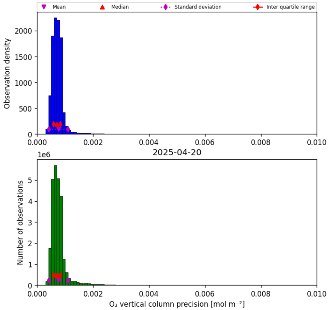
Figure 22: Histogram of “O 3 vertical column precision” for 2025-04-19 to 2025-04-21
