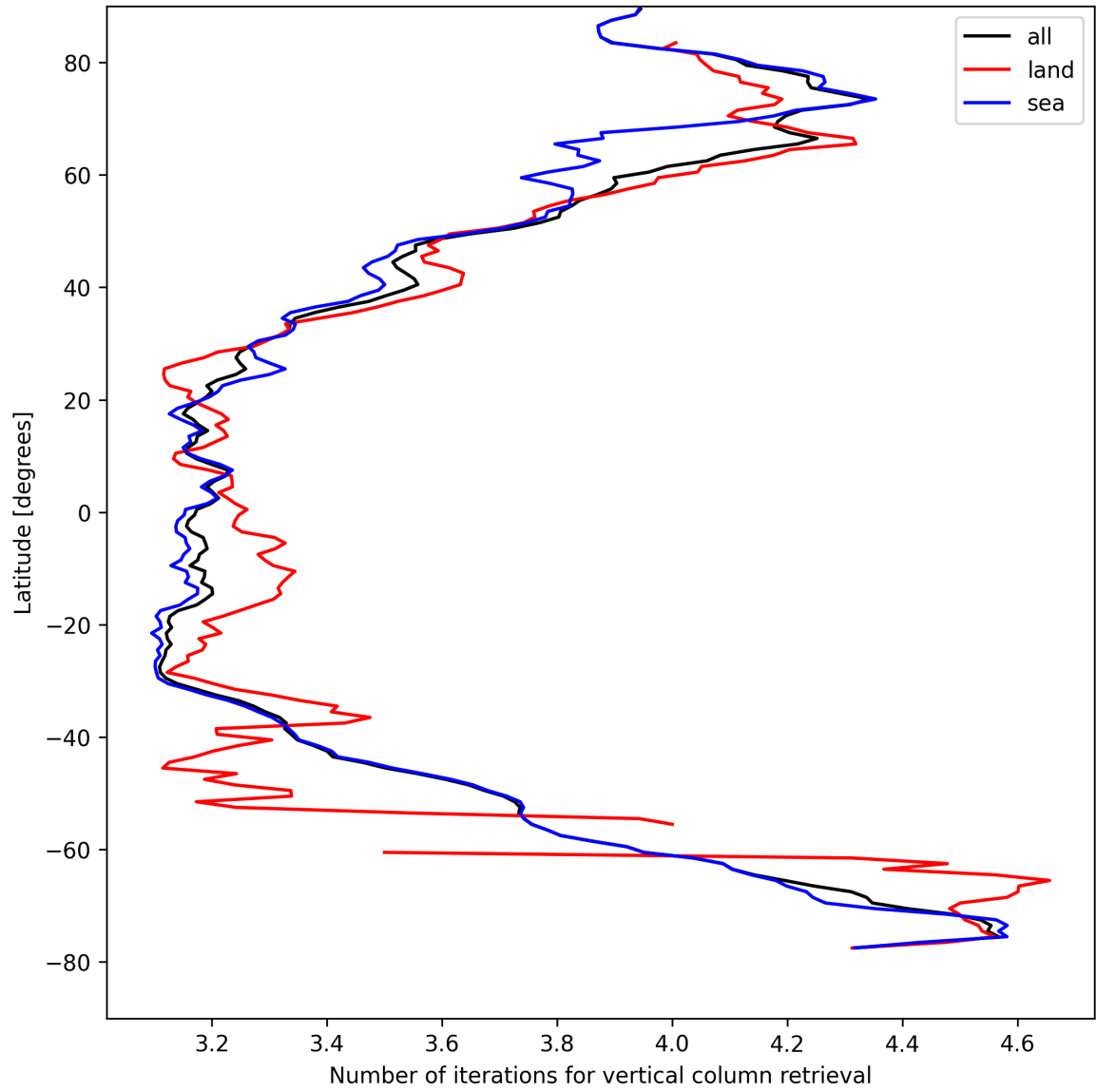
Figure 19: Zonal average of “Number of iterations for vertical column retrieval” for 2025-04-19 to 2025-04-21.
