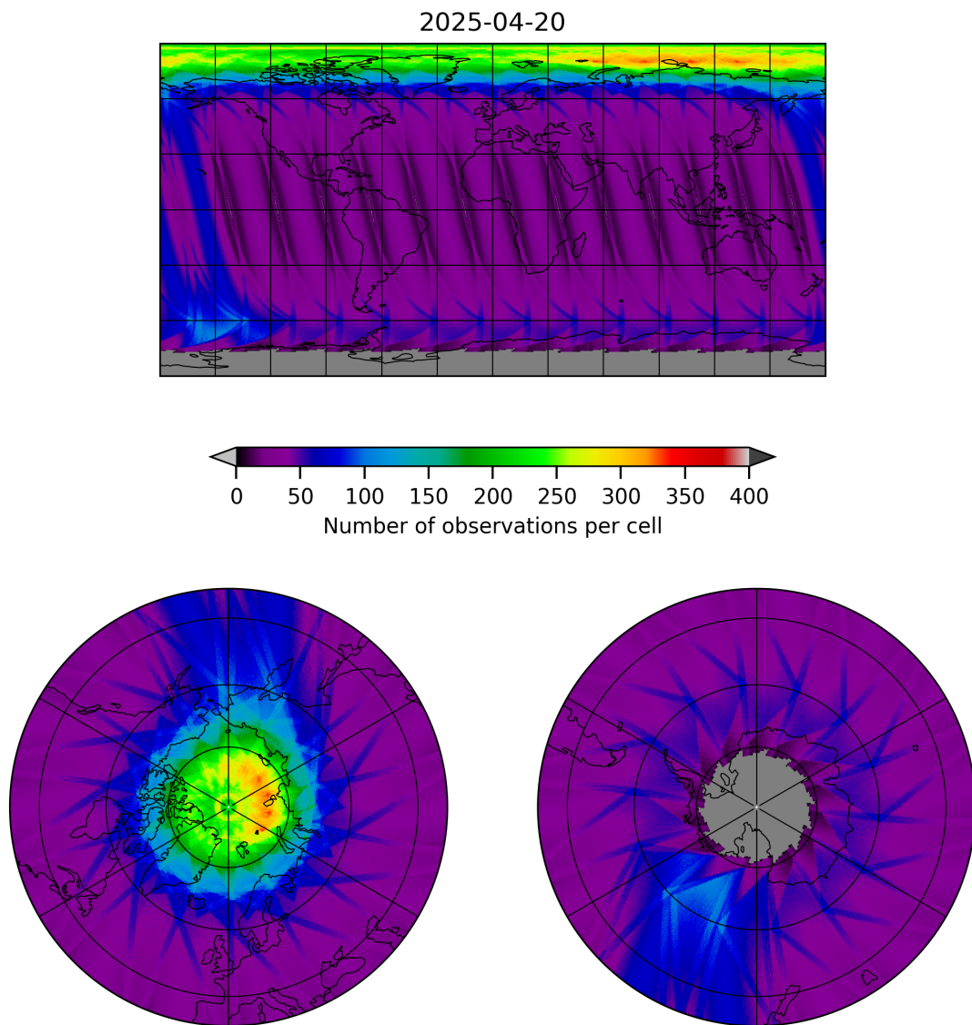
Figure 12: Map of the number of observations for 2025-04-19 to 2025-04-21
