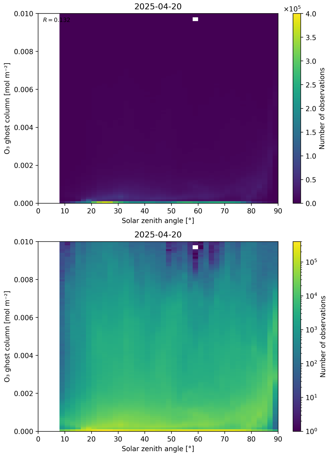
Figure 46: Scatter density plot of “Solar zenith angle” against “O 3 ghost column” for 2025-04-19 to 2025-04-21.
