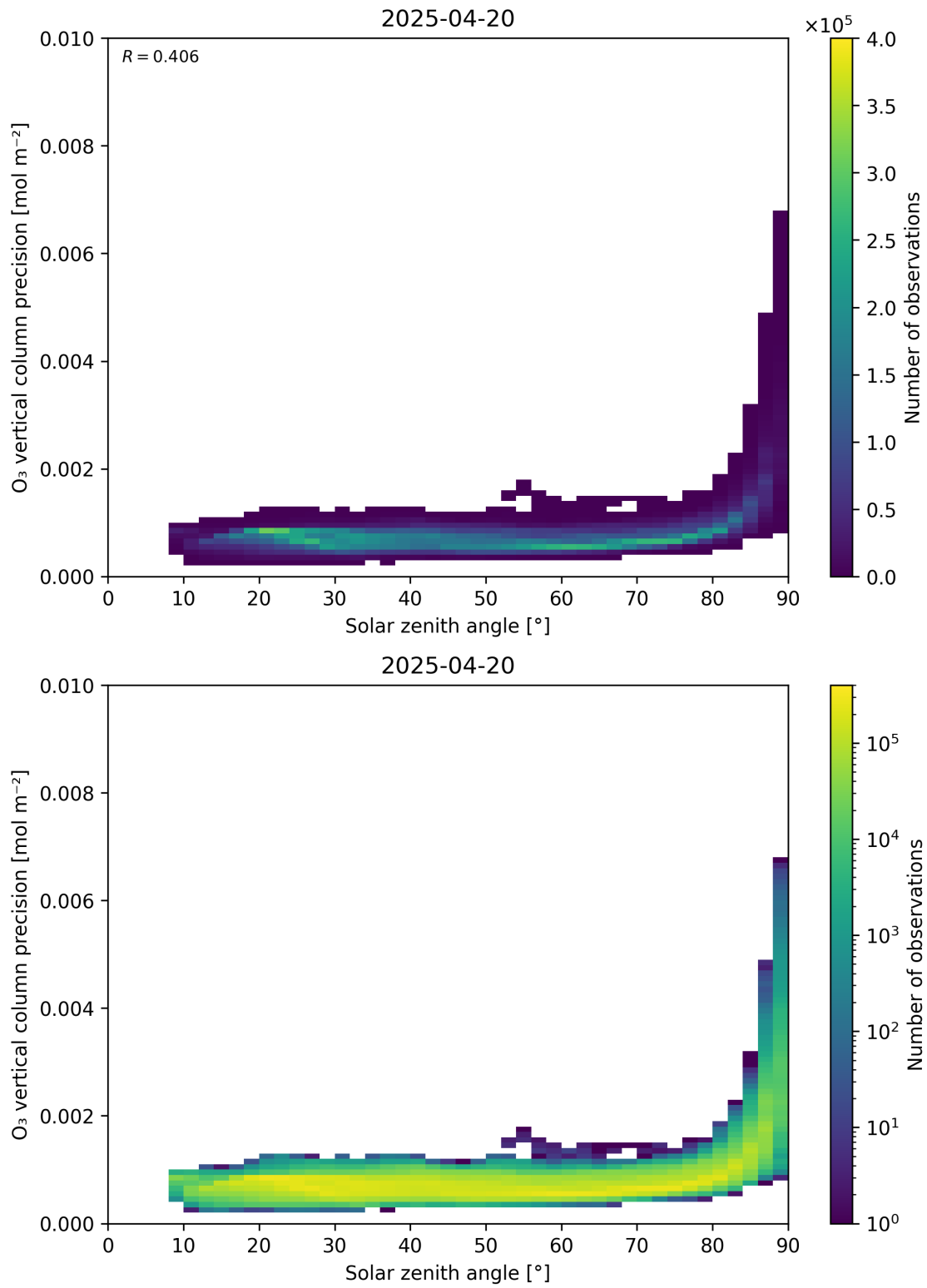
Figure 48: Scatter density plot of “Solar zenith angle” against “O 3 vertical column precision” for 2025-04-19 to 2025-04-21.
