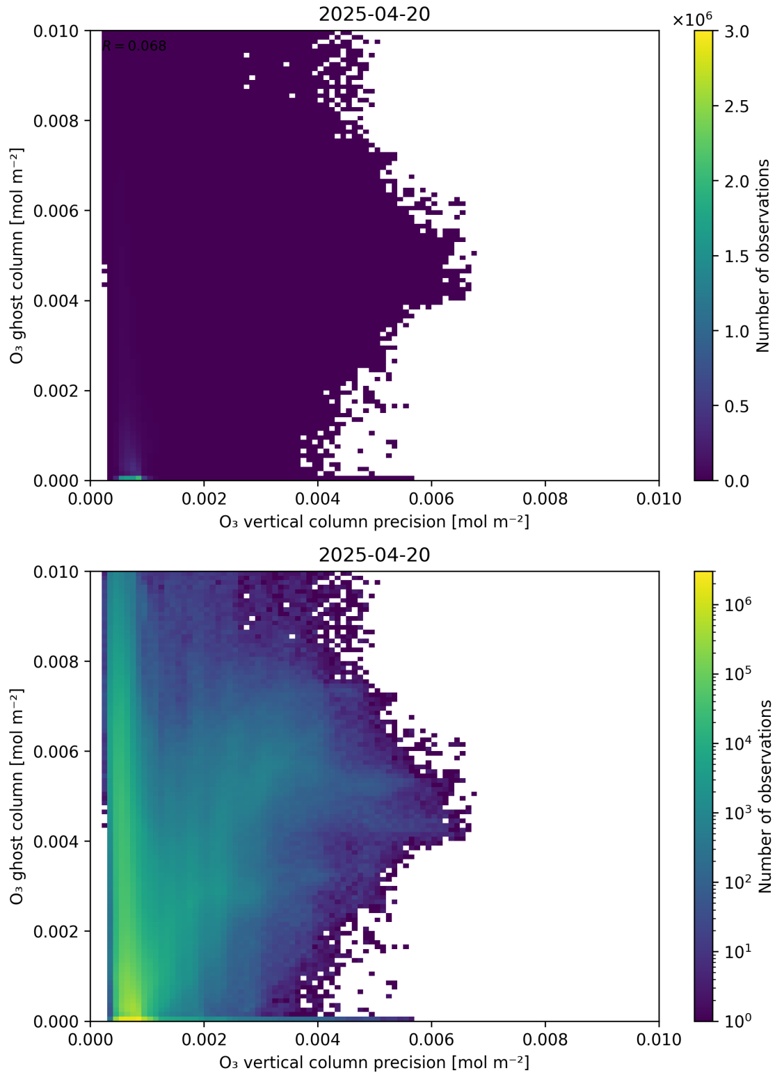
Figure 43: Scatter density plot of “ \text{O}_3 vertical column precision” against “ \text{O}_3 ghost column” for 2025-04-19 to 2025-04-21.
