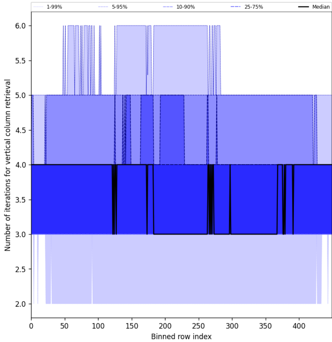
Figure 33: Along track statistics of “Number of iterations for vertical column retrieval” for 2025-04-19 to 2025-04-21
