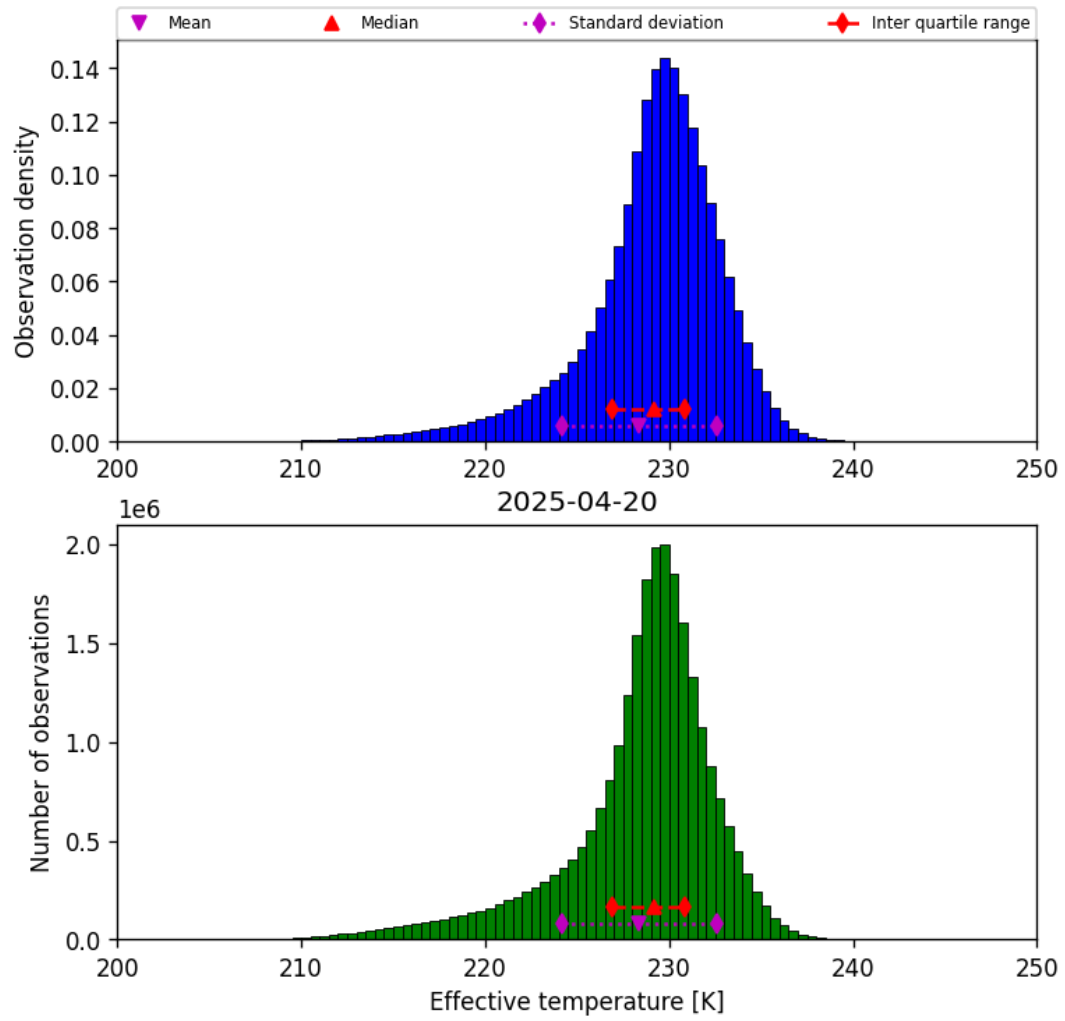
Figure 24: Histogram of “Effective temperature” for 2025-04-19 to 2025-04-21
