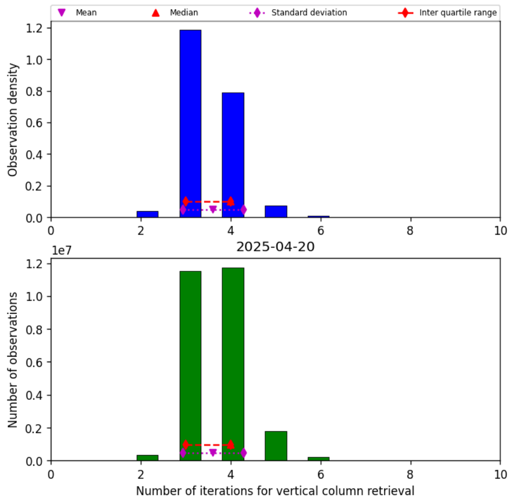
Figure 26: Histogram of “Number of iterations for vertical column retrieval” for 2025-04-19 to 2025-04-21
