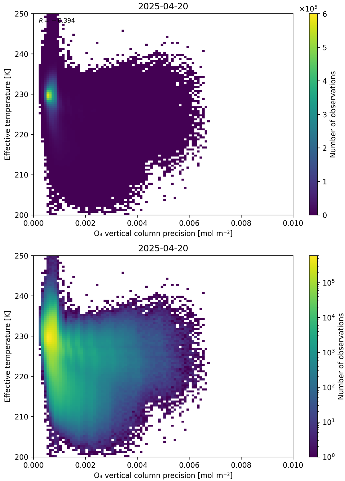
Figure 42: Scatter density plot of “O 3 vertical column precision” against “Effective temperature” for 2025-04-19 to 2025-04-21.
