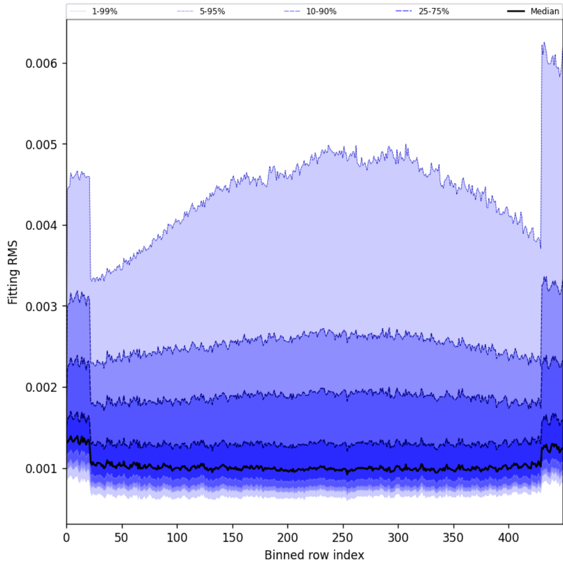
Figure 30: Along track statistics of “Fitting RMS” for 2025-04-19 to 2025-04-21
