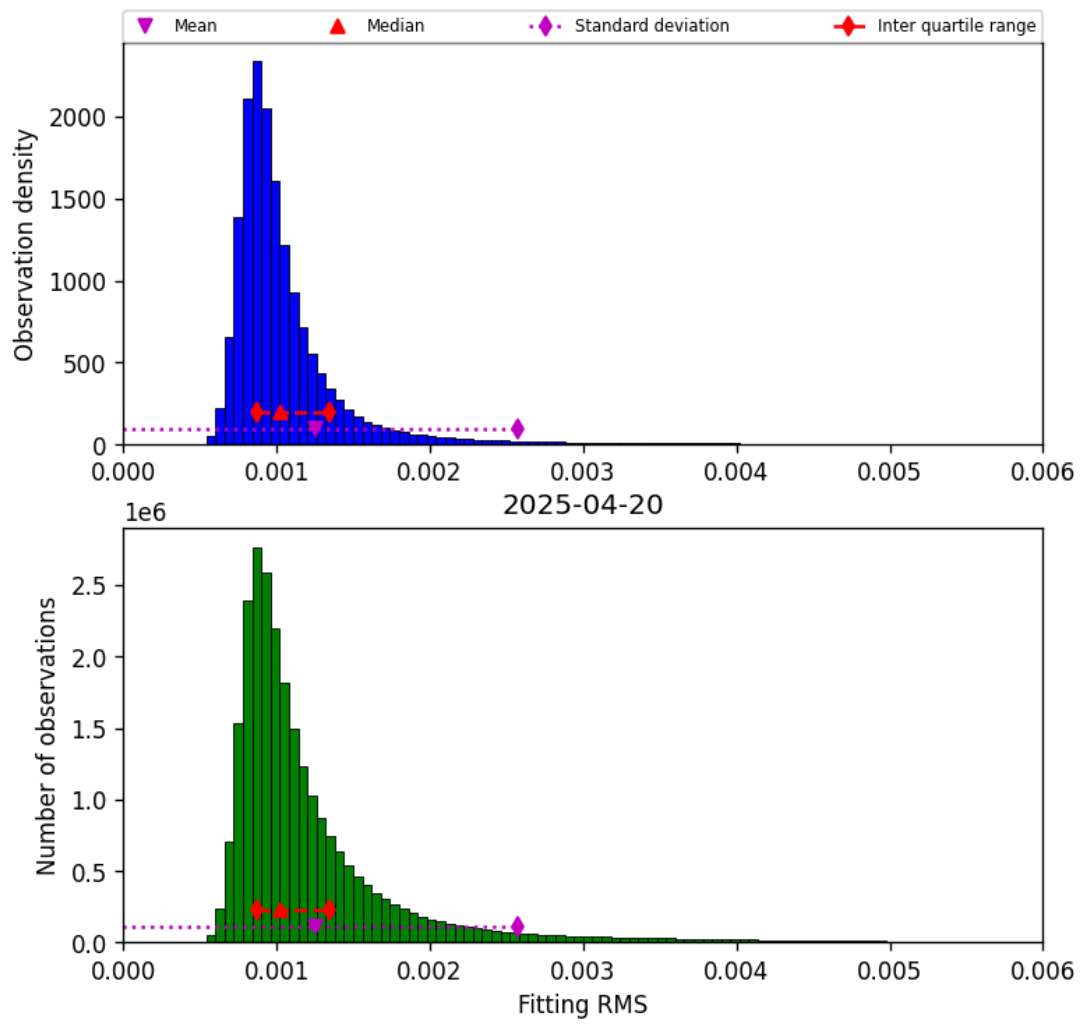
Figure 23: Histogram of “Fitting RMS” for 2025-04-19 to 2025-04-21
