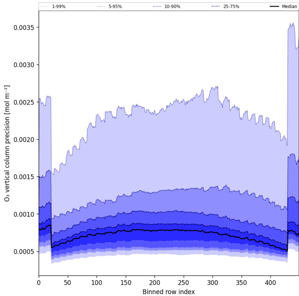
Figure 29: Along track statistics of “O 3 vertical column precision” for 2025-04-19 to 2025-04-21
