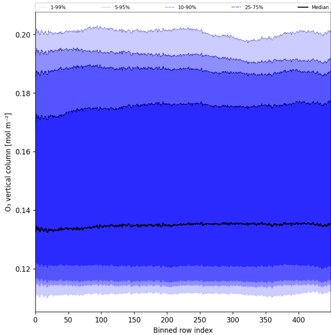
Figure 28: Along track statistics of “O 3 vertical column” for 2025-04-19 to 2025-04-21
