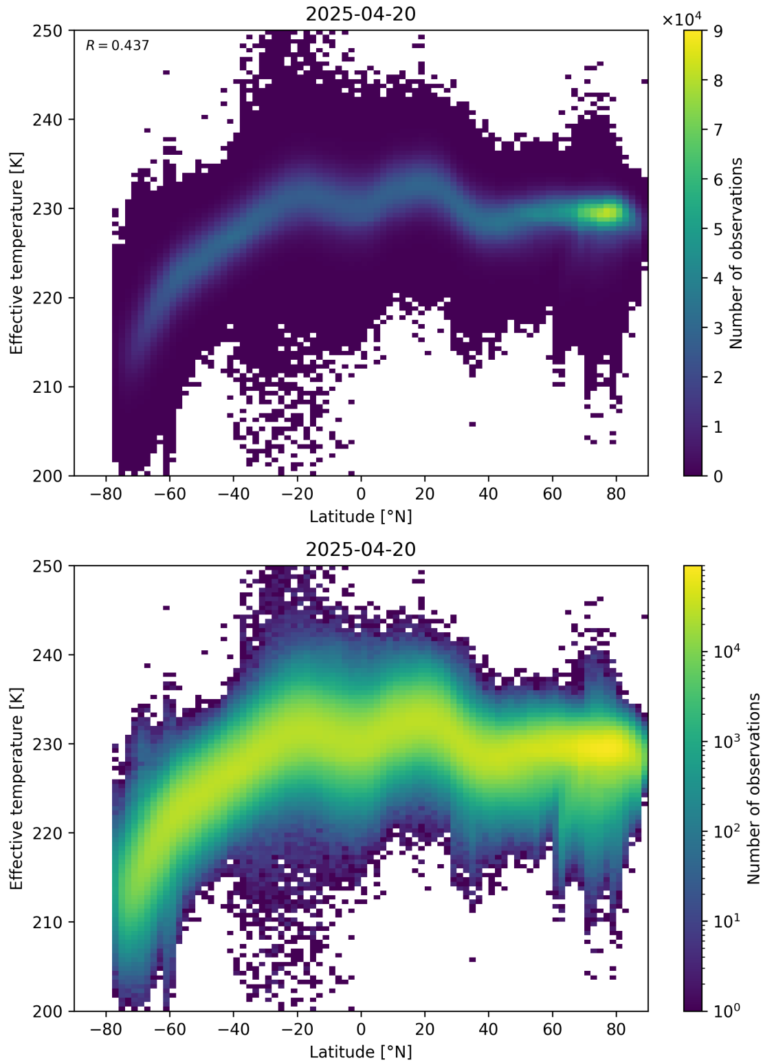
Figure 34: Scatter density plot of “Latitude” against “Effective temperature” for 2025-04-19 to 2025-04-21.
