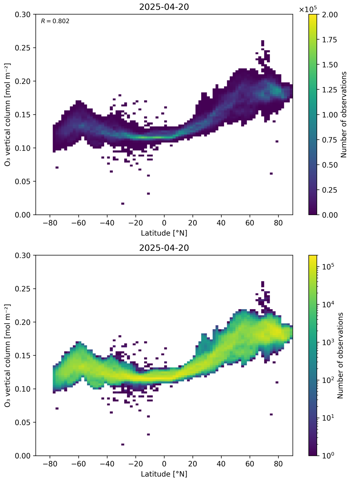
Figure 36: Scatter density plot of “Latitude” against “O 3 vertical column” for 2025-04-19 to 2025-04-21.
