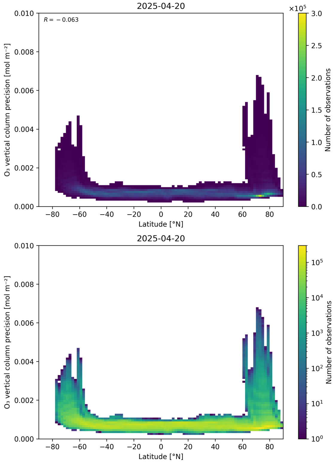
Figure 37: Scatter density plot of “Latitude” against “O 3 vertical column precision” for 2025-04-19 to 2025-04-21.
