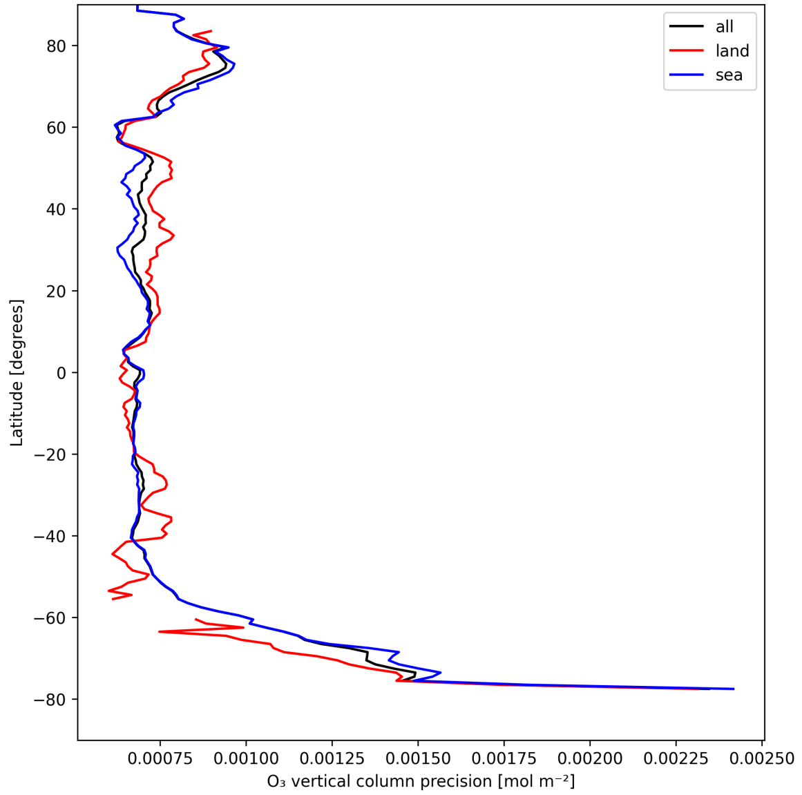
Figure 15: Zonal average of “O 3 vertical column precision” for 2025-04-19 to 2025-04-21.
