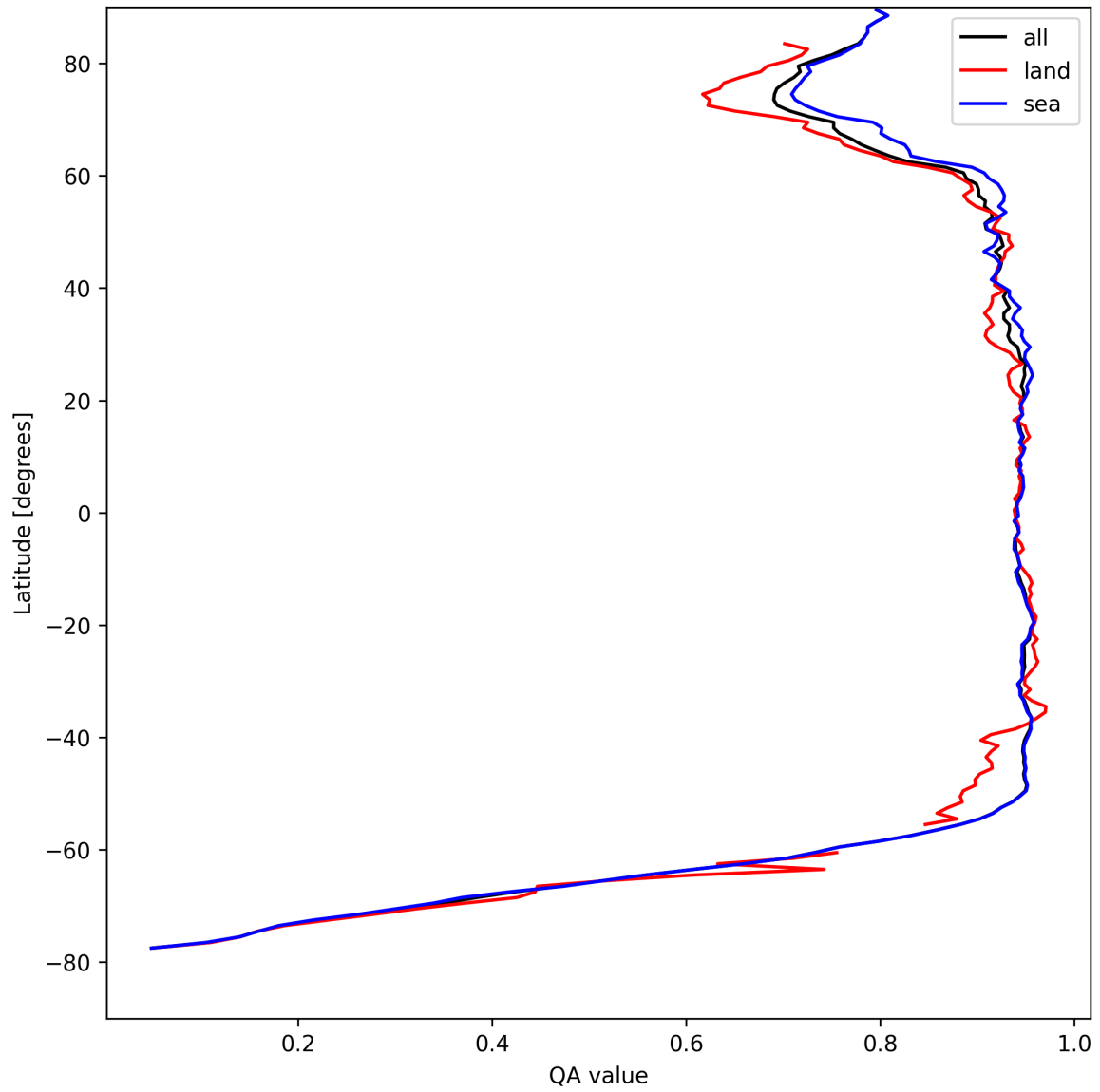
Figure 13: Zonal average of “QA value” for 2025-04-19 to 2025-04-21.
