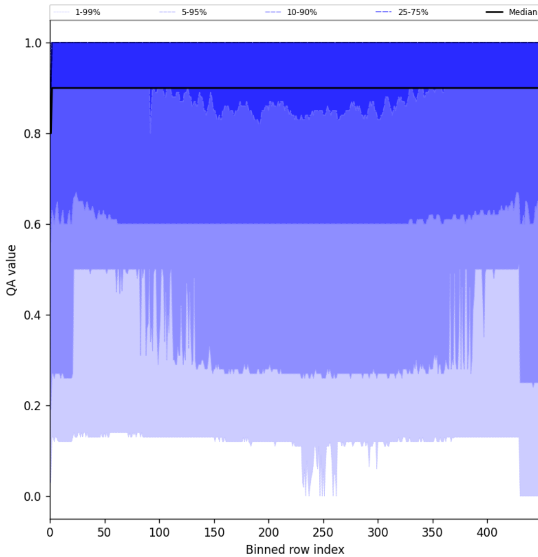
Figure 27: Along track statistics of “QA value” for 2025-04-20 to 2025-04-22
