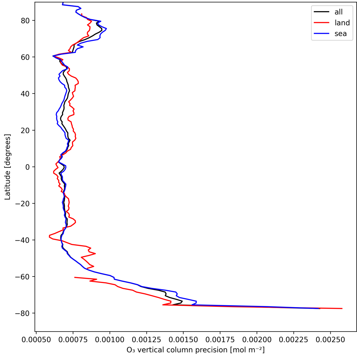
Figure 15: Zonal average of “O 3 vertical column precision” for 2025-04-20 to 2025-04-22.
