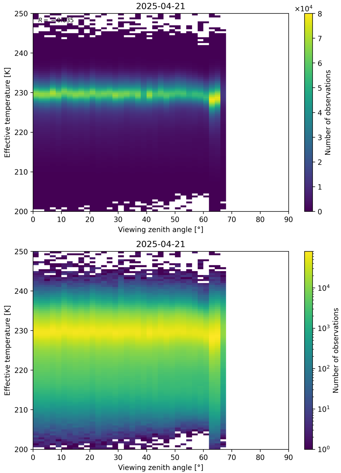
Figure 50: Scatter density plot of “Viewing zenith angle” against “Effective temperature” for 2025-04-20 to 2025-04-22.
