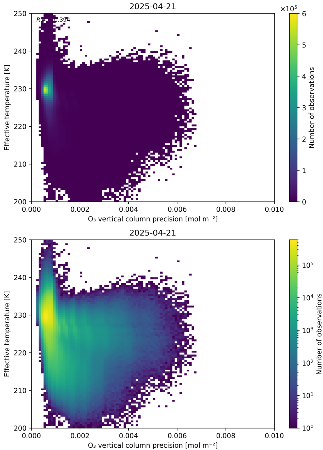
Figure 42: Scatter density plot of “O 3 vertical column precision” against “Effective temperature” for 2025-04-20 to 2025-04-22.
