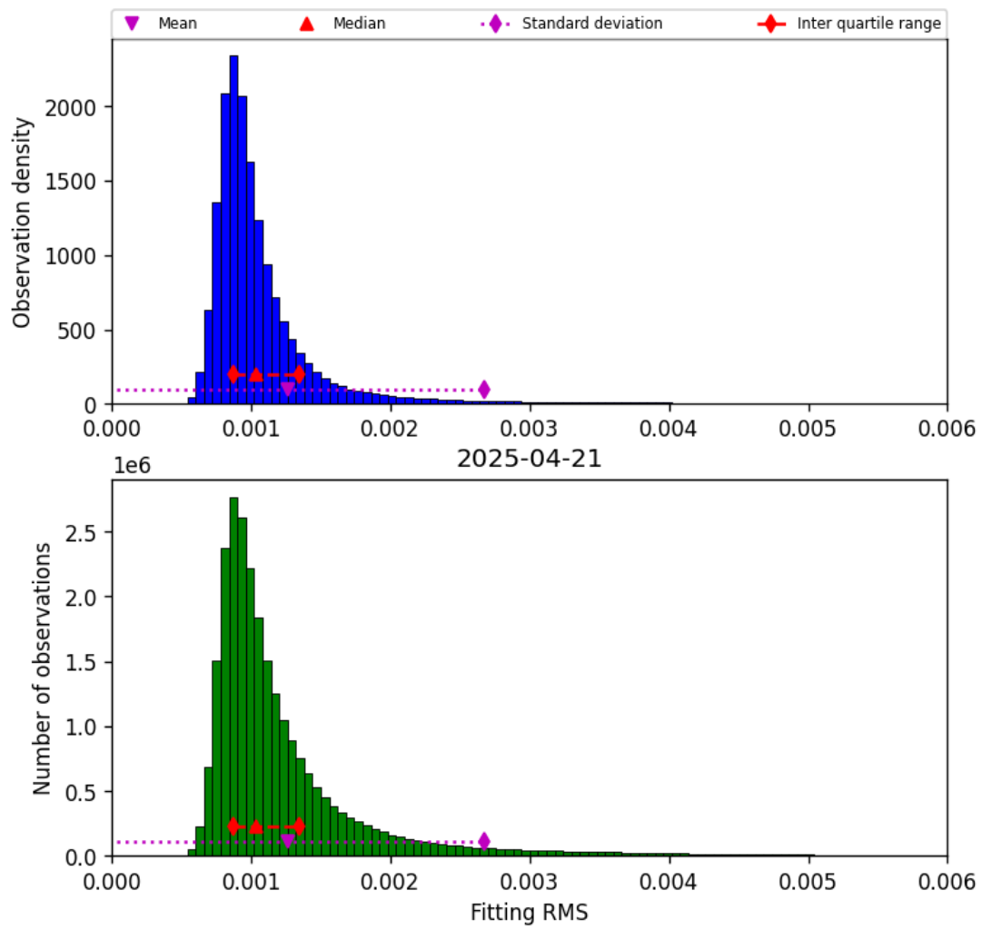
Figure 23: Histogram of “Fitting RMS” for 2025-04-20 to 2025-04-22
