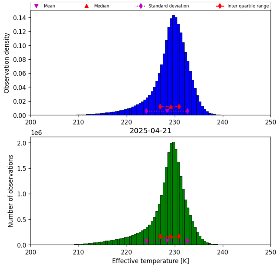
Figure 24: Histogram of “Effective temperature” for 2025-04-20 to 2025-04-22
