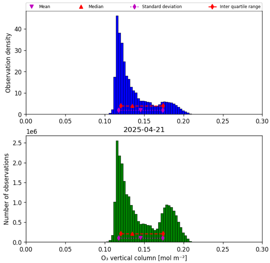
Figure 21: Histogram of “O 3 vertical column” for 2025-04-20 to 2025-04-22
