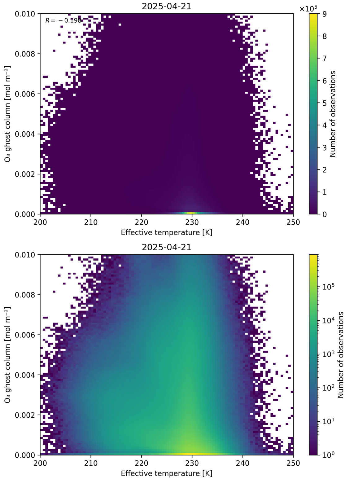
Figure 38: Scatter density plot of “Effective temperature” against “O 3 ghost column” for 2025-04-20 to 2025-04-22.
