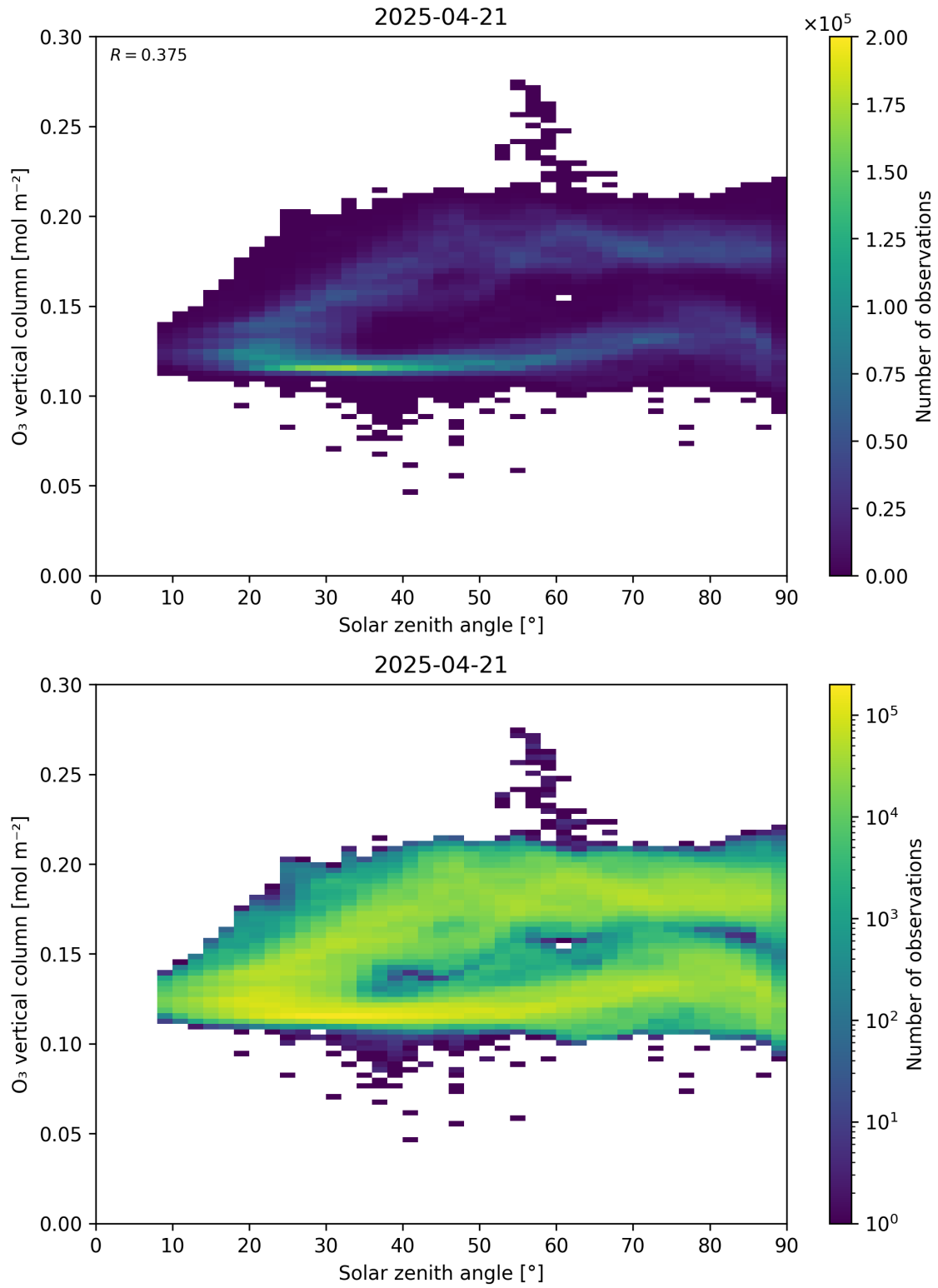
Figure 47: Scatter density plot of “Solar zenith angle” against “O 3 vertical column” for 2025-04-20 to 2025-04-22.
