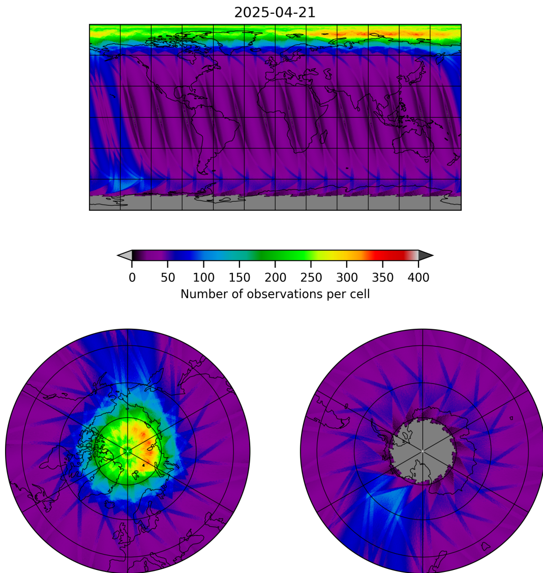
Figure 12: Map of the number of observations for 2025-04-20 to 2025-04-22
