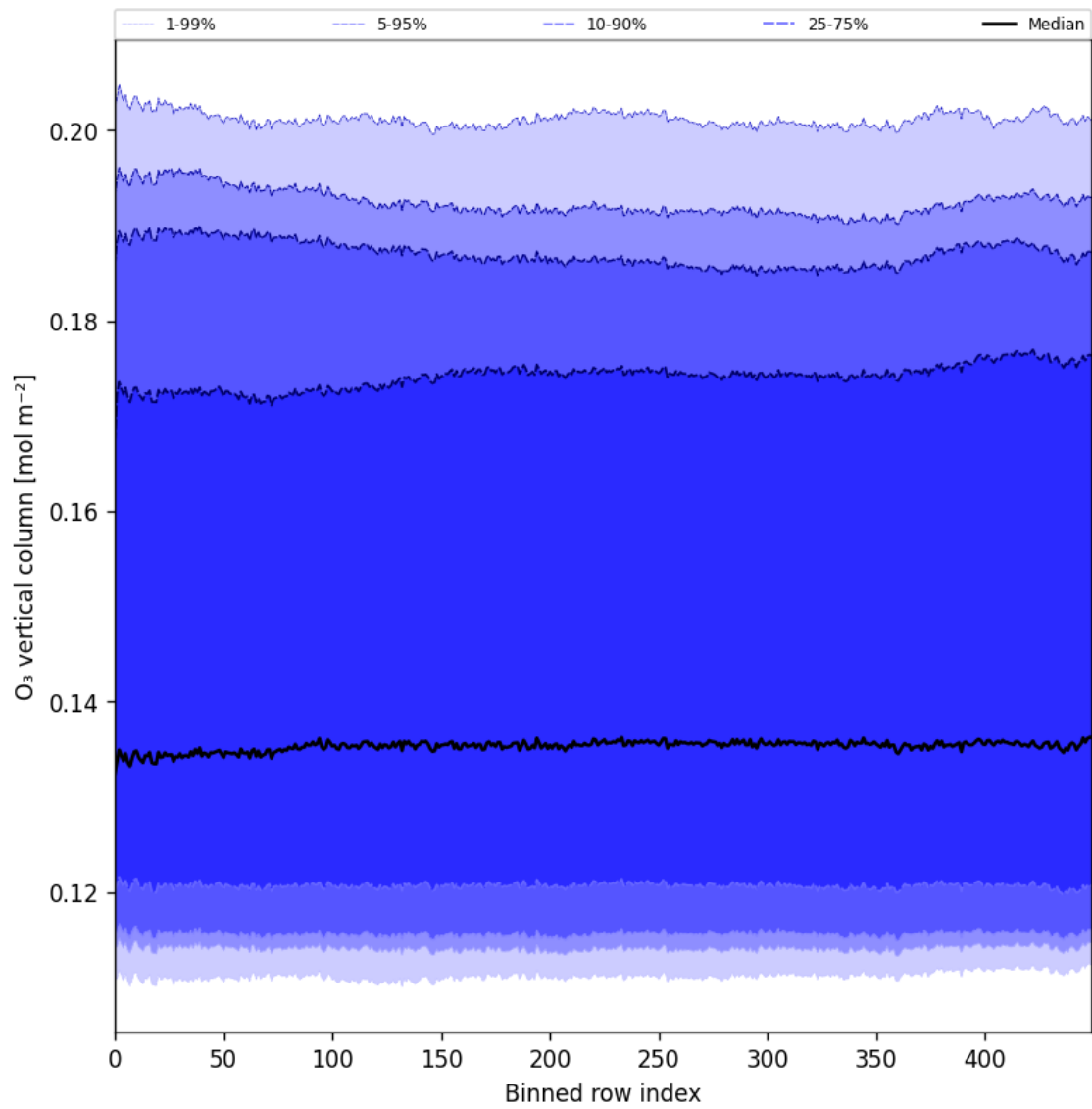
Figure 28: Along track statistics of “O 3 vertical column” for 2025-04-20 to 2025-04-22
