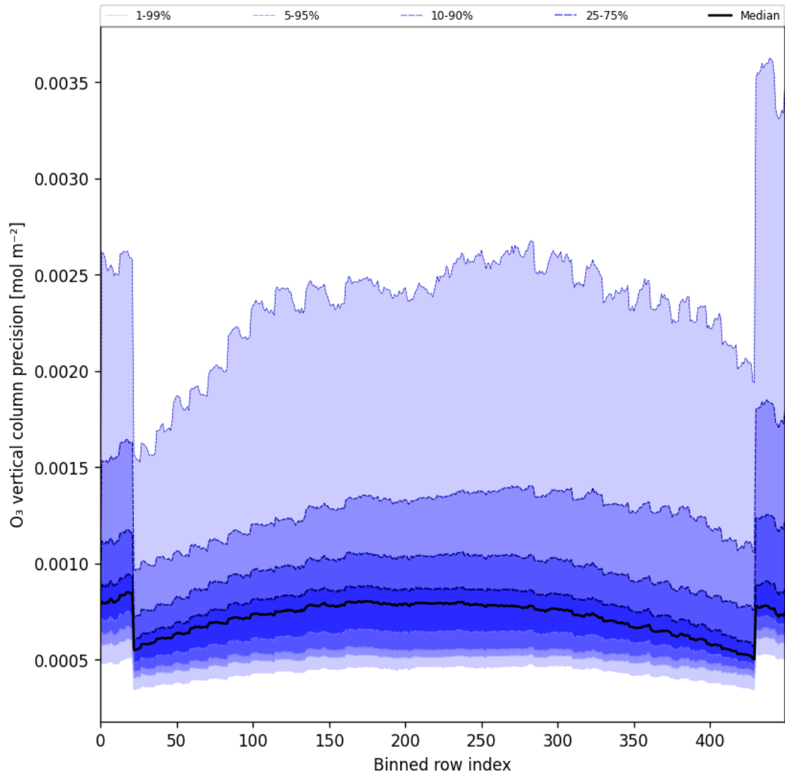
Figure 29: Along track statistics of “O 3 vertical column precision” for 2025-04-20 to 2025-04-22
