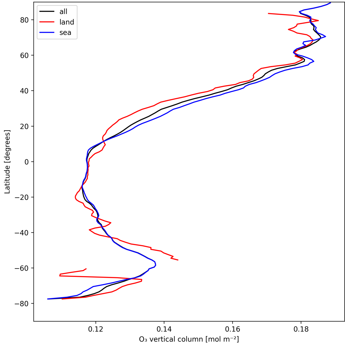
Figure 14: Zonal average of “O 3 vertical column” for 2025-04-20 to 2025-04-22.
