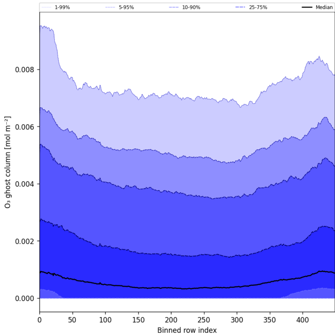
Figure 32: Along track statistics of “O 3 ghost column” for 2025-04-20 to 2025-04-22
