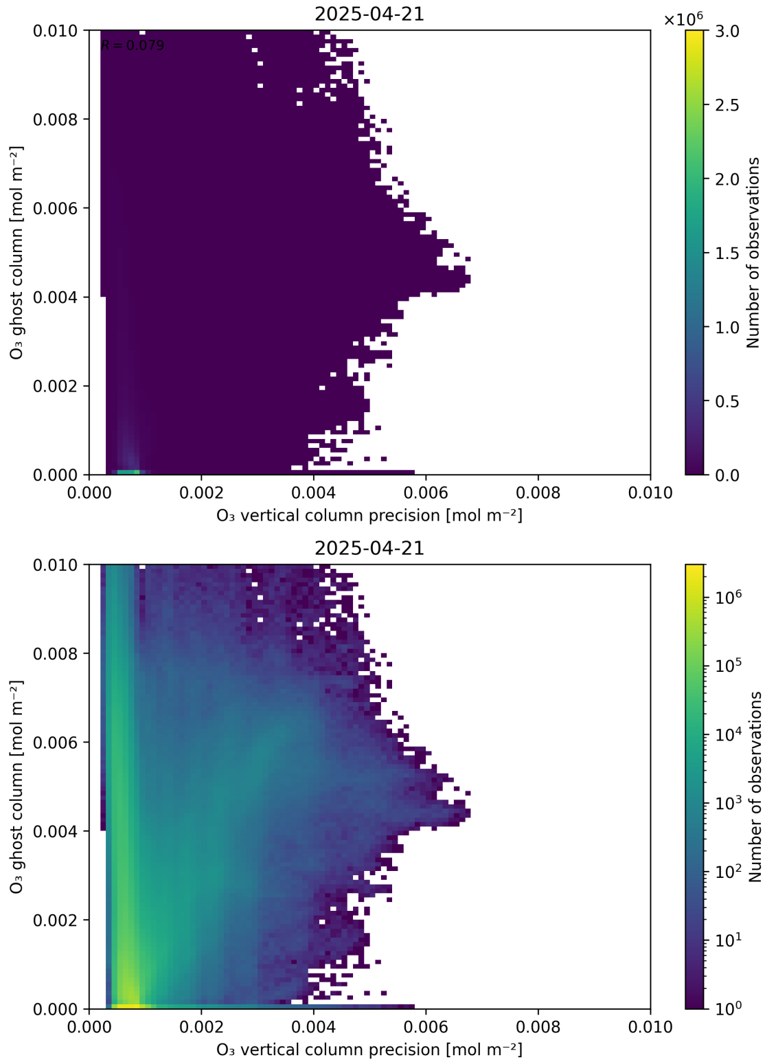
Figure 43: Scatter density plot of “O 3 vertical column precision” against “O 3 ghost column” for 2025-04-20 to 2025-04-22.
