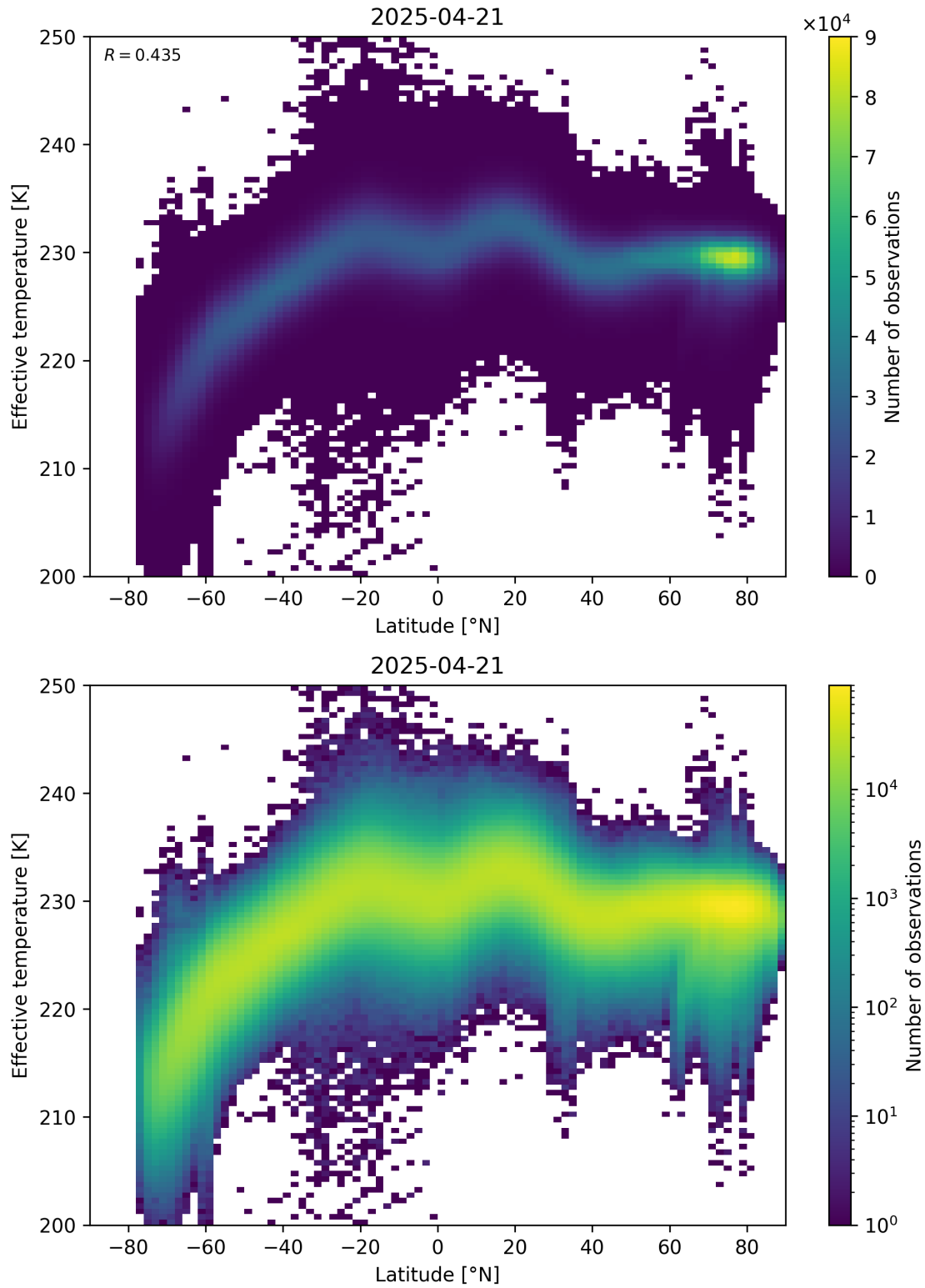
Figure 34: Scatter density plot of “Latitude” against “Effective temperature” for 2025-04-20 to 2025-04-22.
