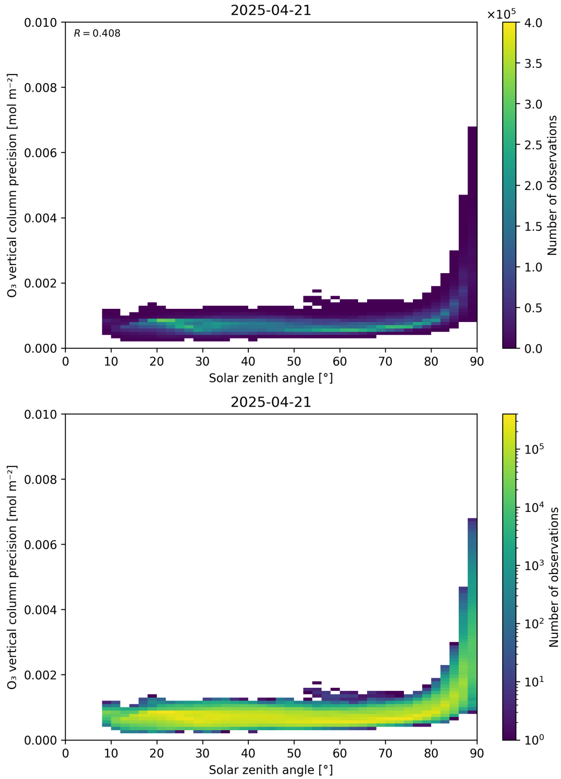
Figure 48: Scatter density plot of “Solar zenith angle” against “O 3 vertical column precision” for 2025-04-20 to 2025-04-22.
