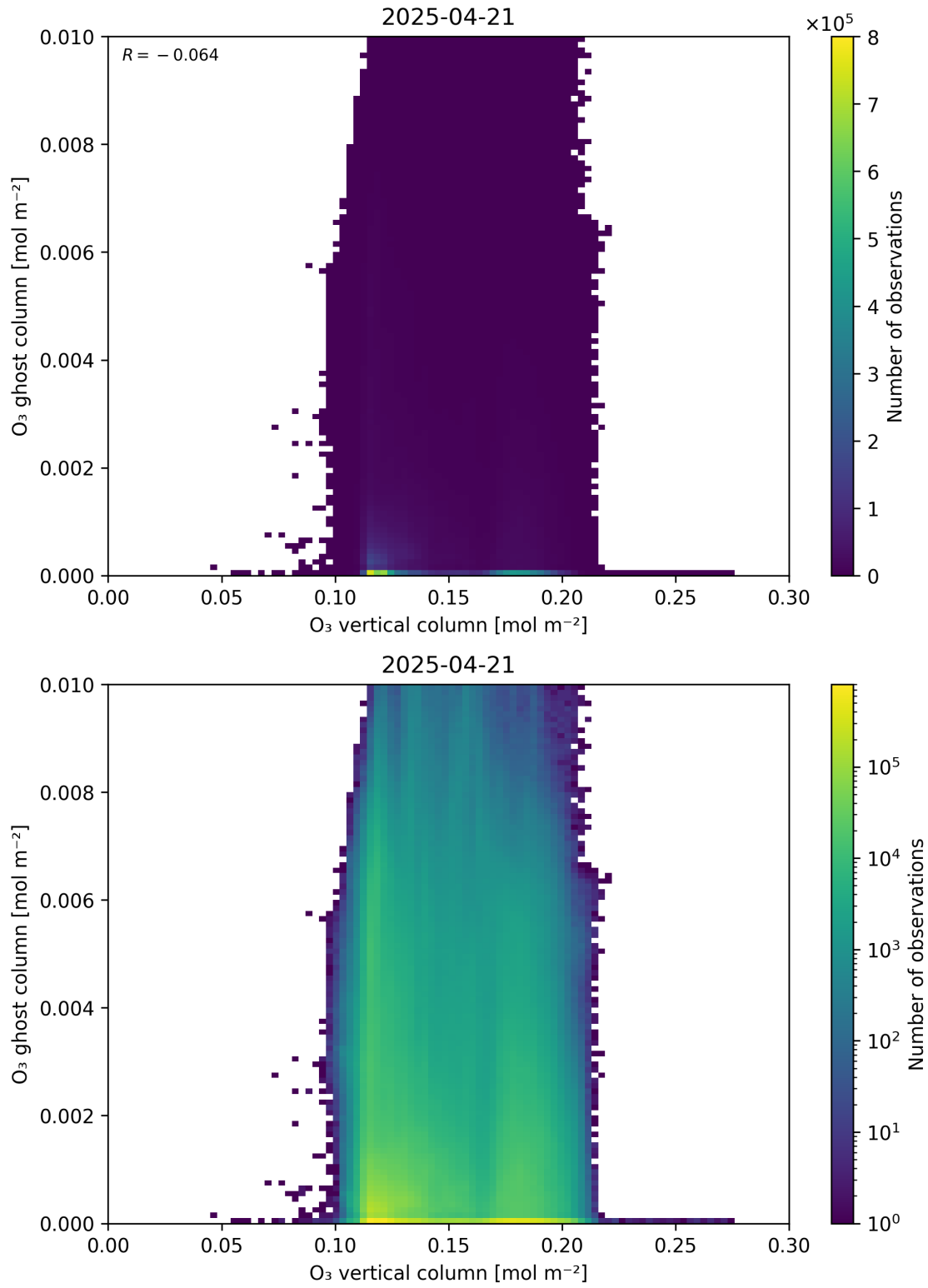
Figure 40: Scatter density plot of “O 3 vertical column” against “O 3 ghost column” for 2025-04-20 to 2025-04-22.
