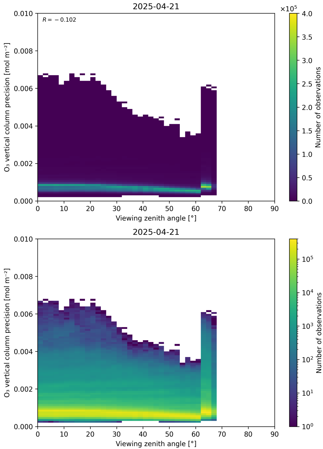
Figure 53: Scatter density plot of “Viewing zenith angle” against “O 3 vertical column precision” for 2025-04-20 to 2025-04-22.
