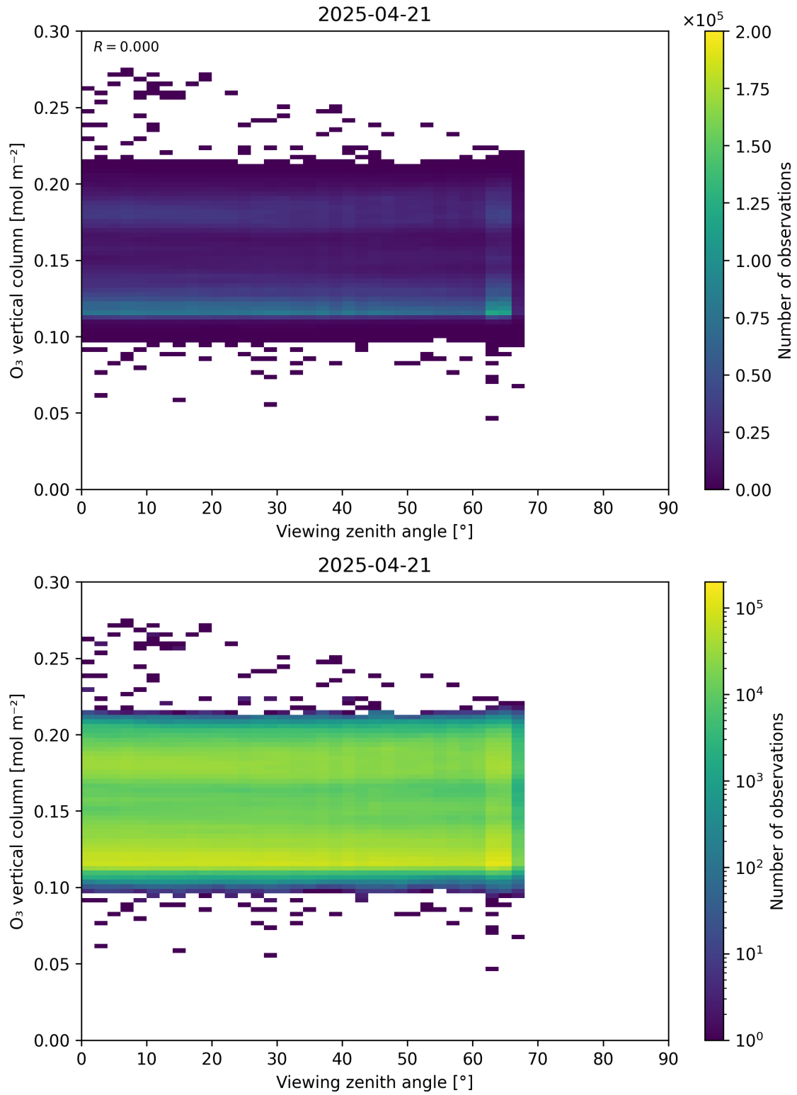
Figure 52: Scatter density plot of “Viewing zenith angle” against “O 3 vertical column” for 2025-04-20 to 2025-04-22.
