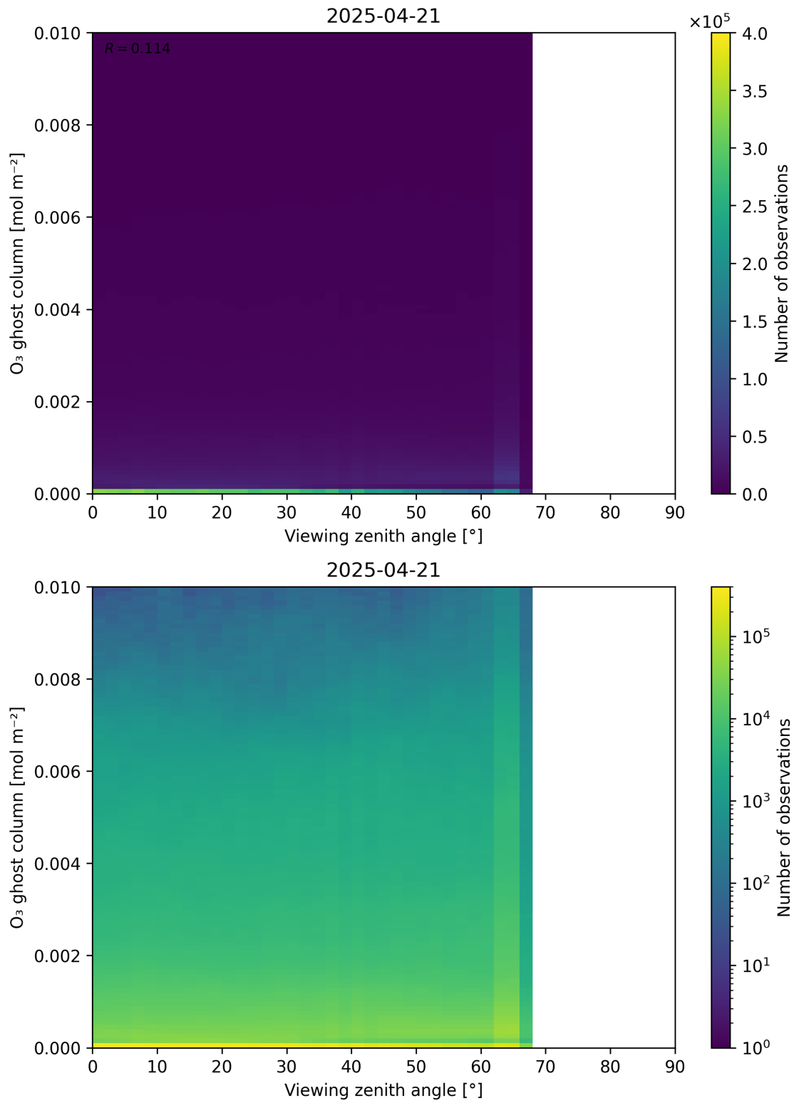
Figure 51: Scatter density plot of “Viewing zenith angle” against “O 3 ghost column” for 2025-04-20 to 2025-04-22.
