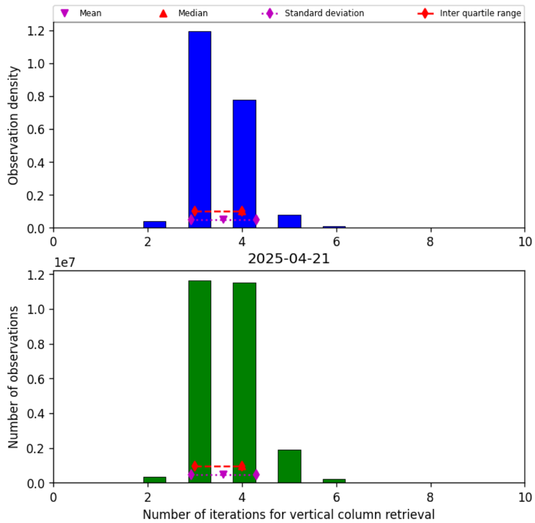
Figure 26: Histogram of “Number of iterations for vertical column retrieval” for 2025-04-20 to 2025-04-22
