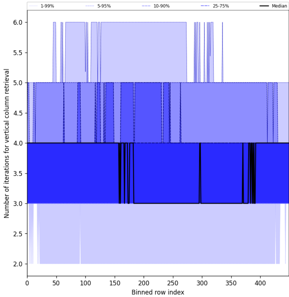
Figure 33: Along track statistics of “Number of iterations for vertical column retrieval” for 2025-04-20 to 2025-04-22
