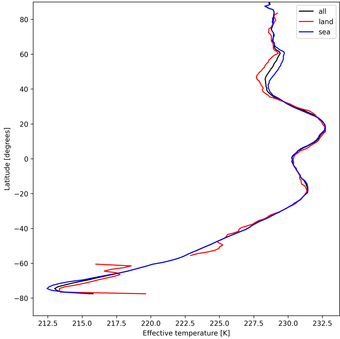
Figure 17: Zonal average of "Effective temperature" for 2025-04-20 to 2025-04-22.
