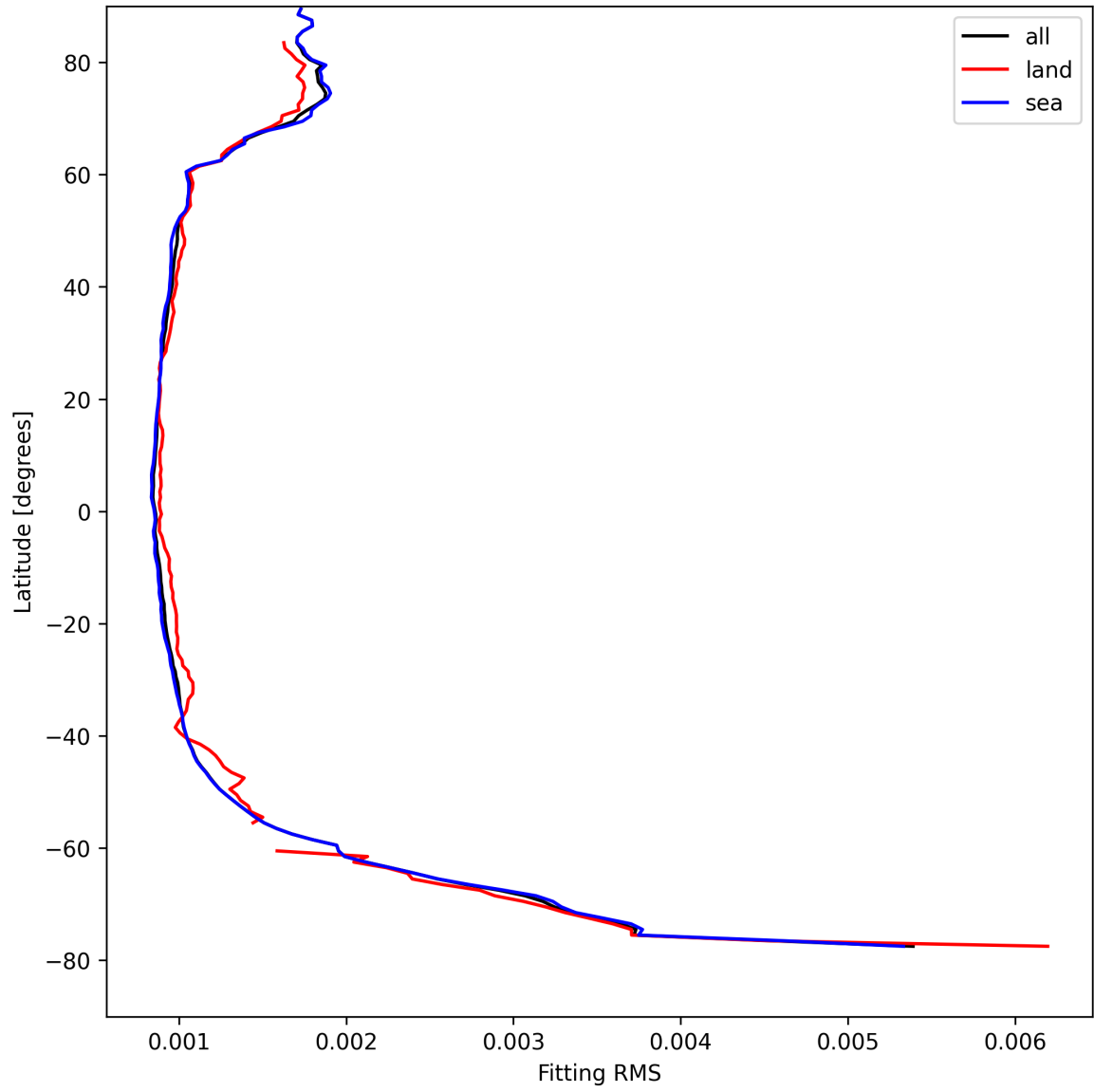
Figure 16: Zonal average of “Fitting RMS” for 2025-04-20 to 2025-04-22.
