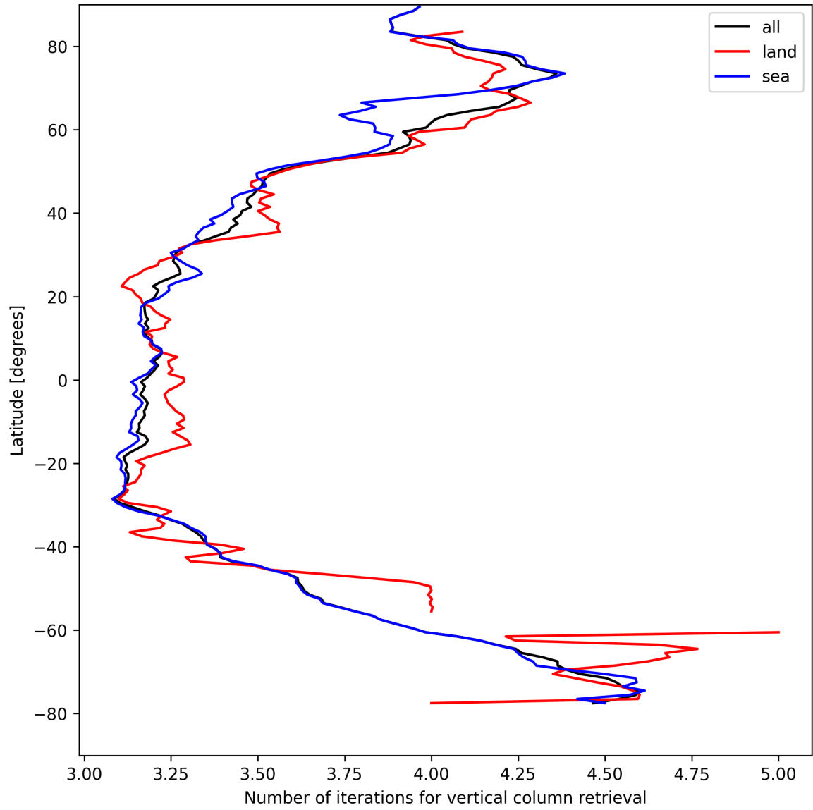
Figure 19: Zonal average of “Number of iterations for vertical column retrieval” for 2025-04-20 to 2025-04-22.
