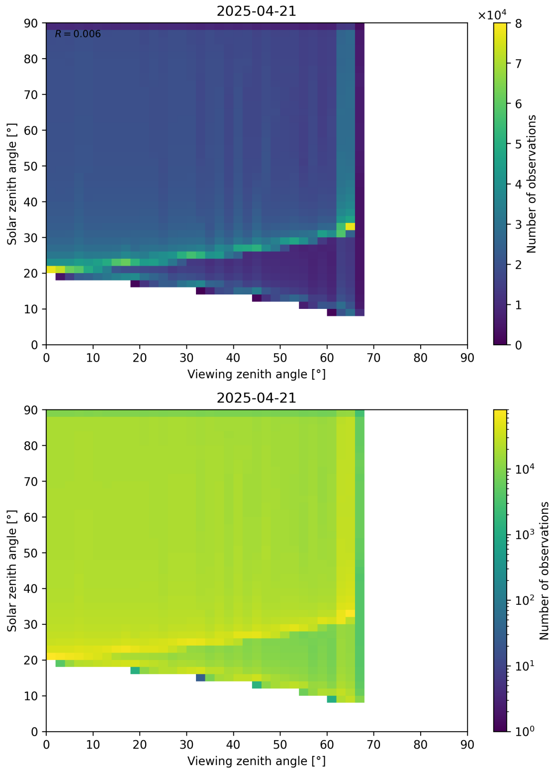
Figure 54: Scatter density plot of “Viewing zenith angle” against “Solar zenith angle” for 2025-04-20 to 2025-04-22.
