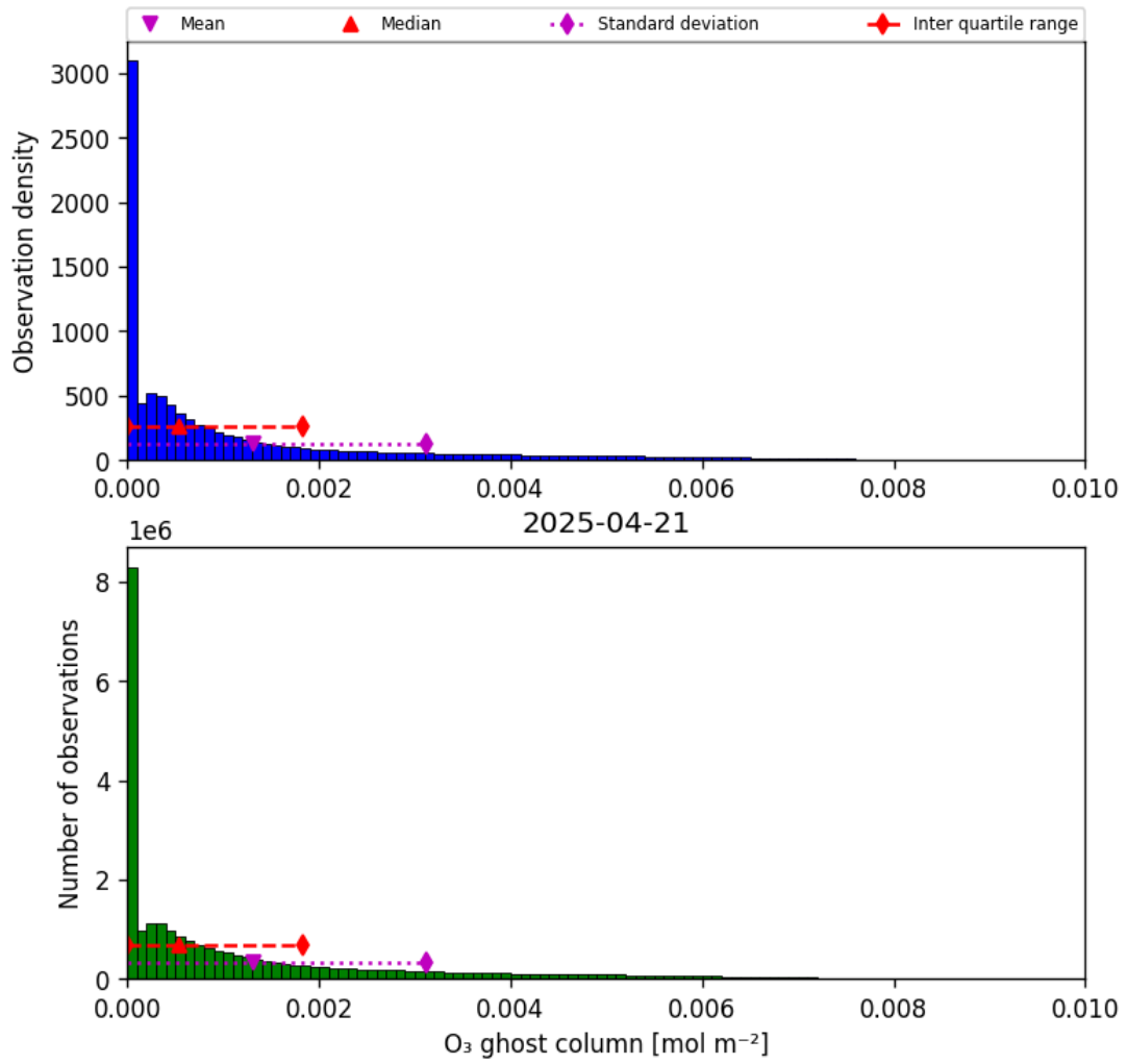
Figure 25: Histogram of "O 3 ghost column" for 2025-04-20 to 2025-04-22
