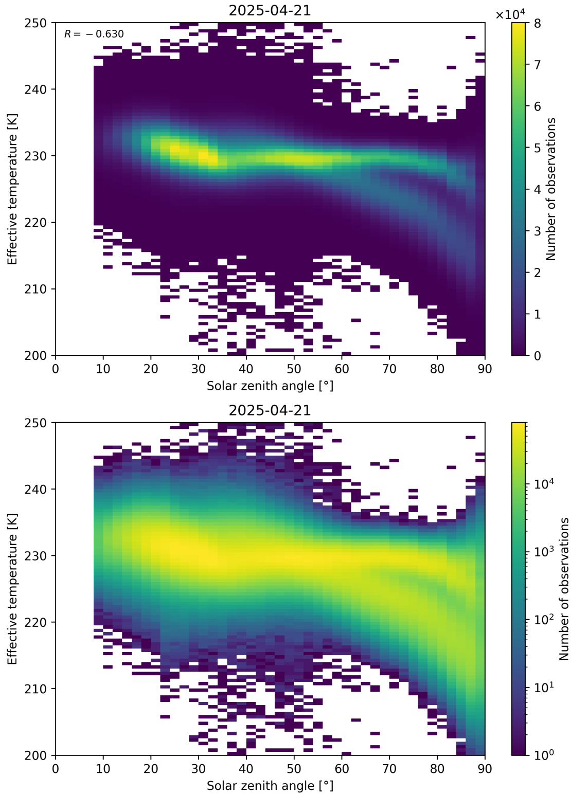
Figure 45: Scatter density plot of “Solar zenith angle” against “Effective temperature” for 2025-04-20 to 2025-04-22.
