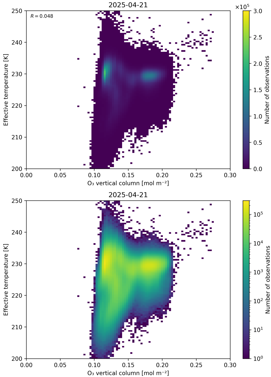
Figure 39: Scatter density plot of “O 3 vertical column” against “Effective temperature” for 2025-04-20 to 2025-04-22.
