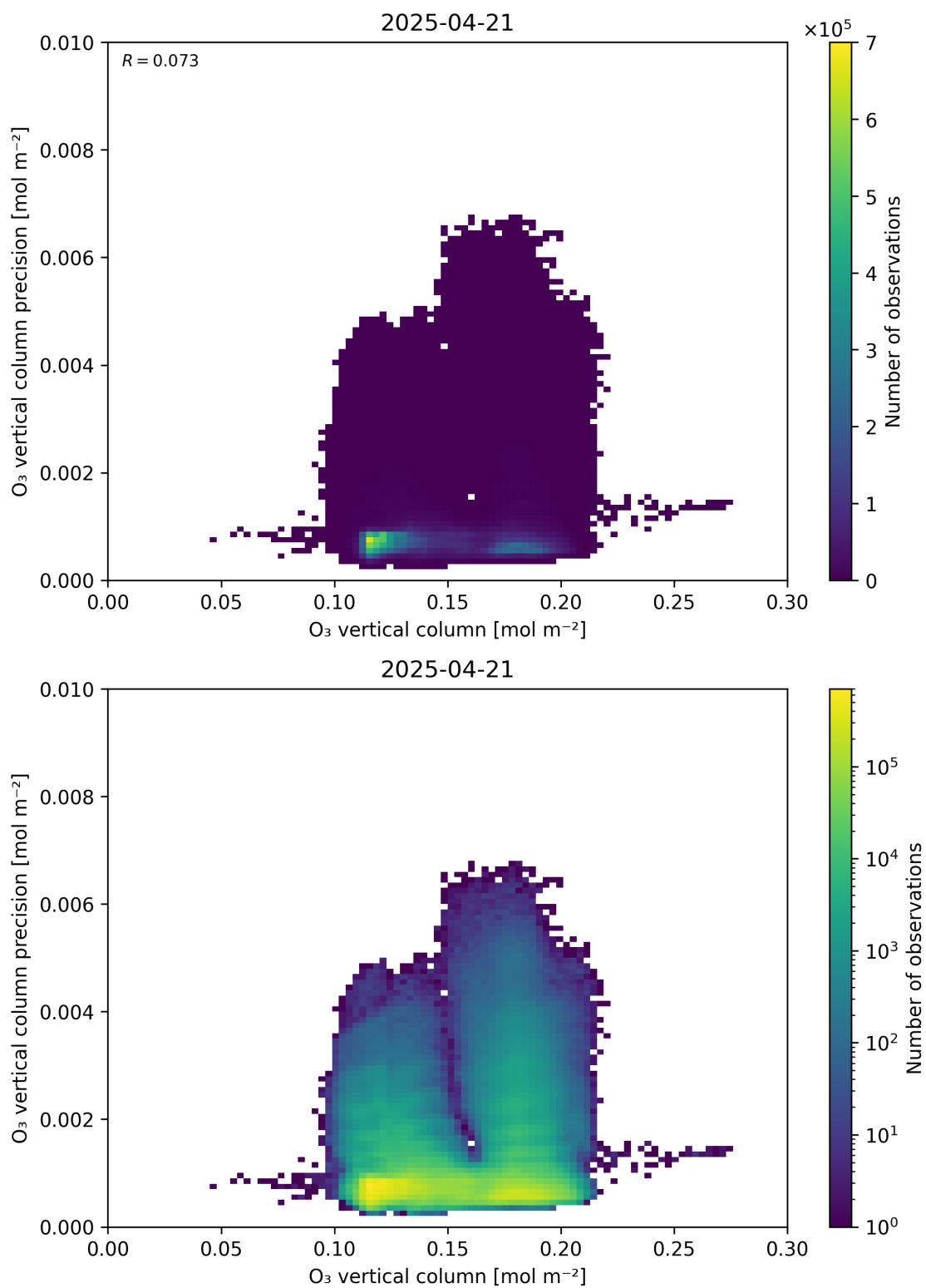
Figure 41: Scatter density plot of “O 3 vertical column” against “O 3 vertical column precision” for 2025-04-20 to 2025-04-22.
