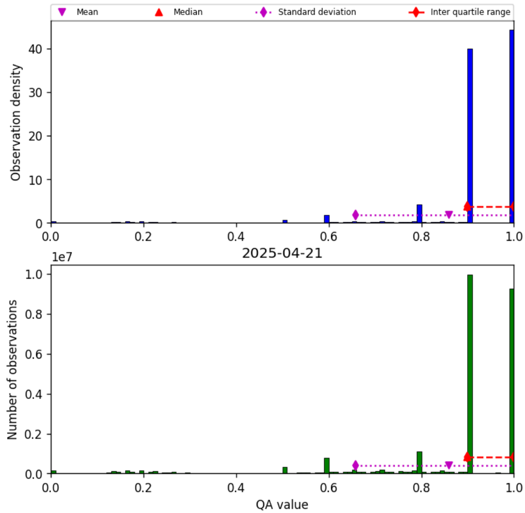
Figure 20: Histogram of “QA value” for 2025-04-20 to 2025-04-22
