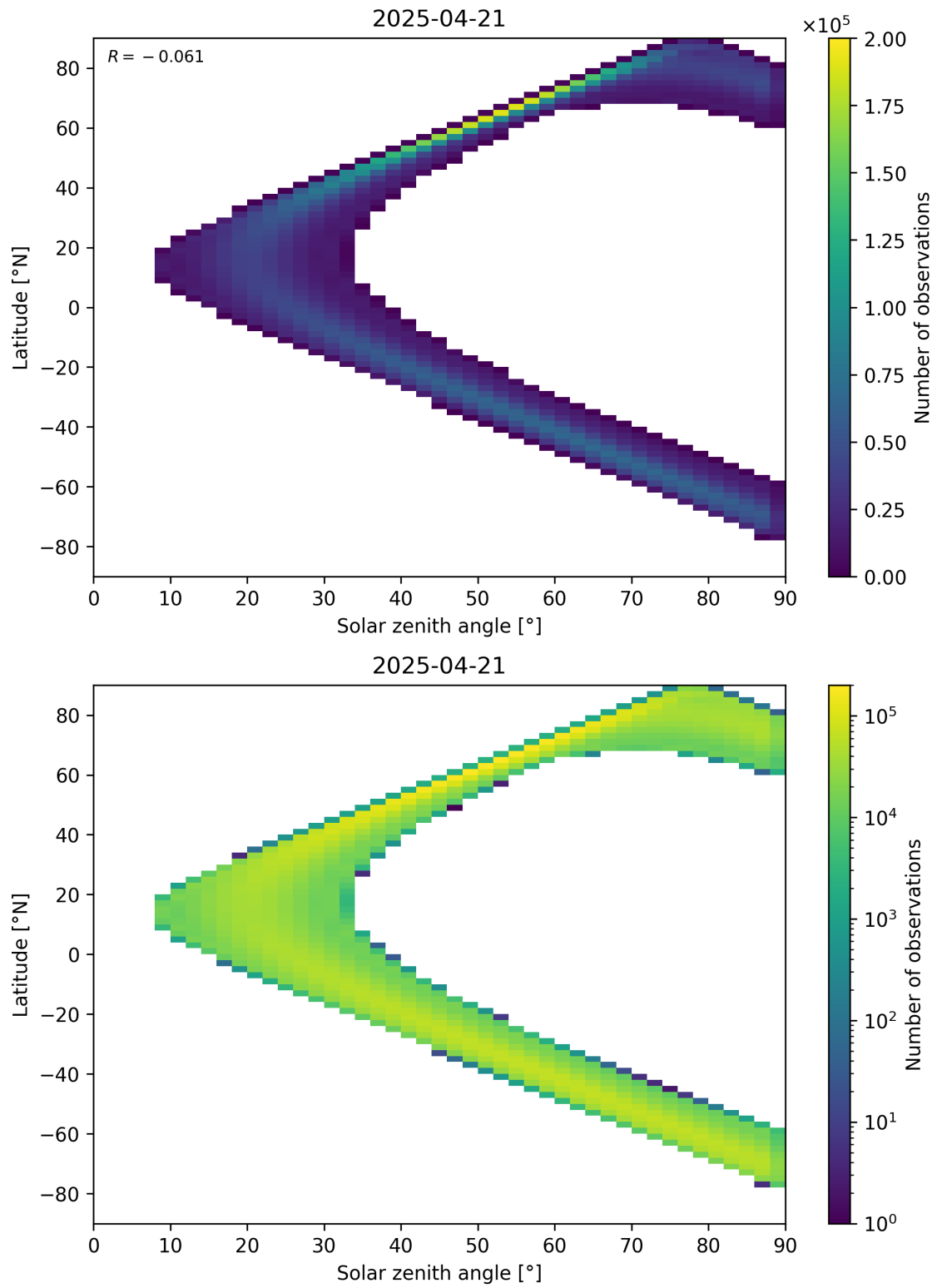
Figure 44: Scatter density plot of “Solar zenith angle” against “Latitude” for 2025-04-20 to 2025-04-22.
