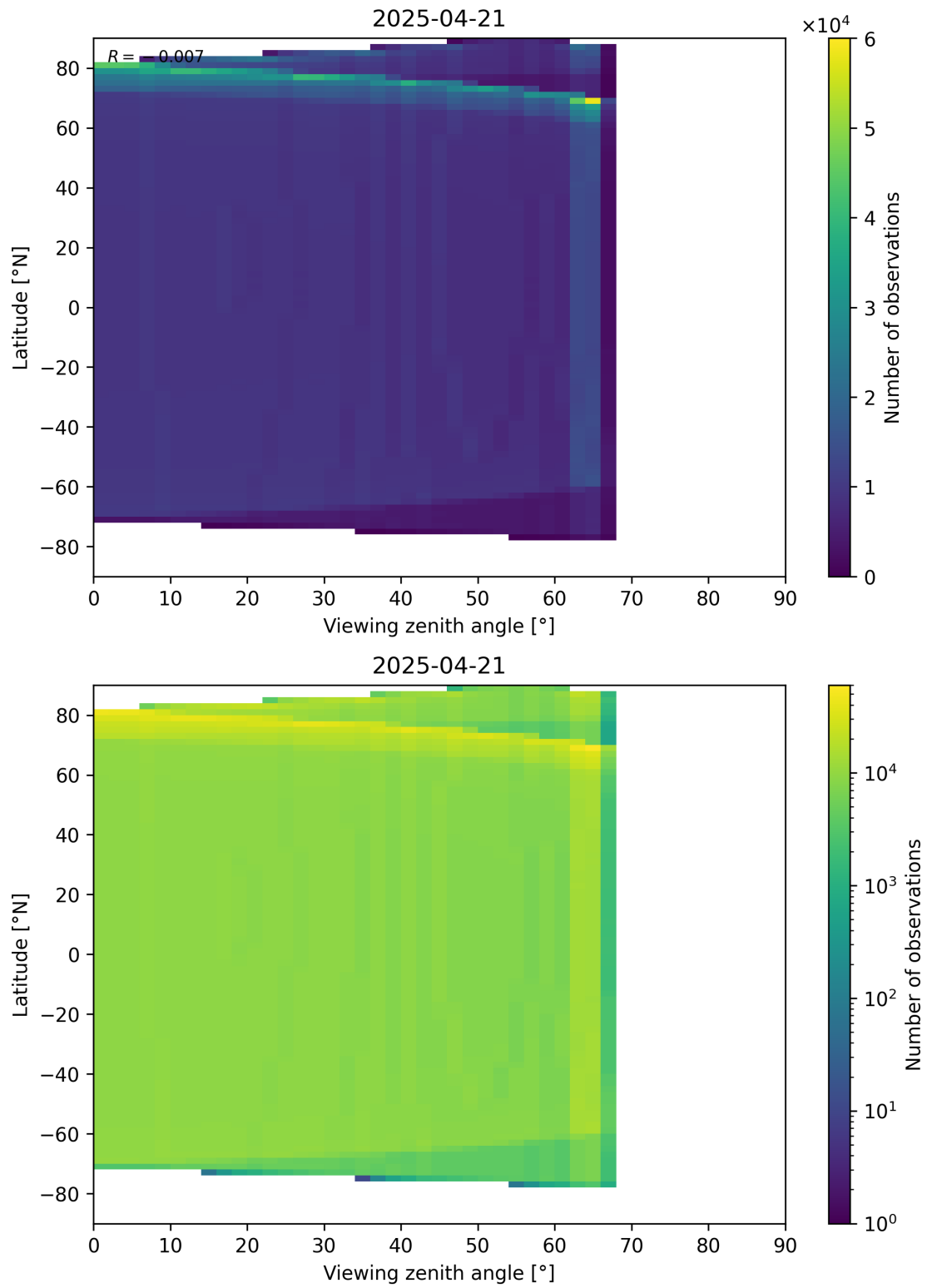
Figure 49: Scatter density plot of “Viewing zenith angle” against “Latitude” for 2025-04-20 to 2025-04-22.
