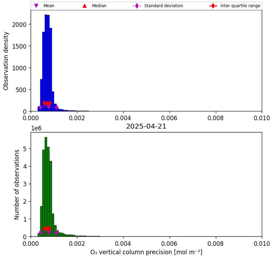
Figure 22: Histogram of “O 3 vertical column precision” for 2025-04-20 to 2025-04-22
