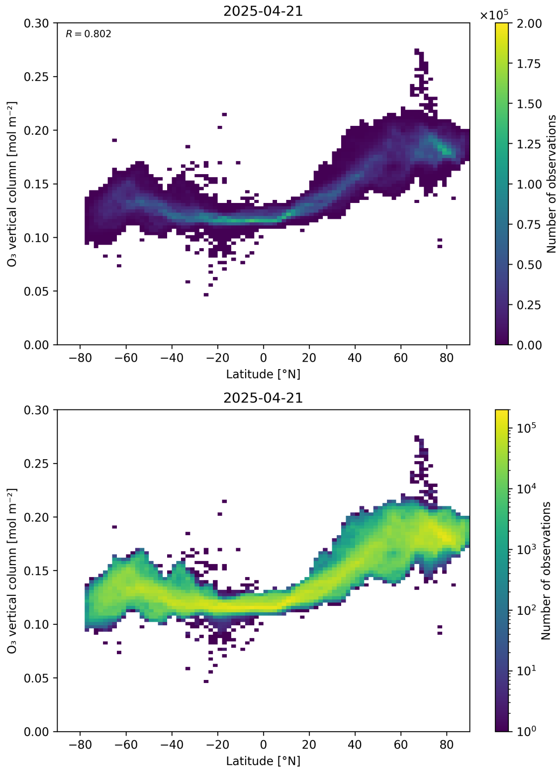
Figure 36: Scatter density plot of “Latitude” against “O 3 vertical column” for 2025-04-20 to 2025-04-22.
