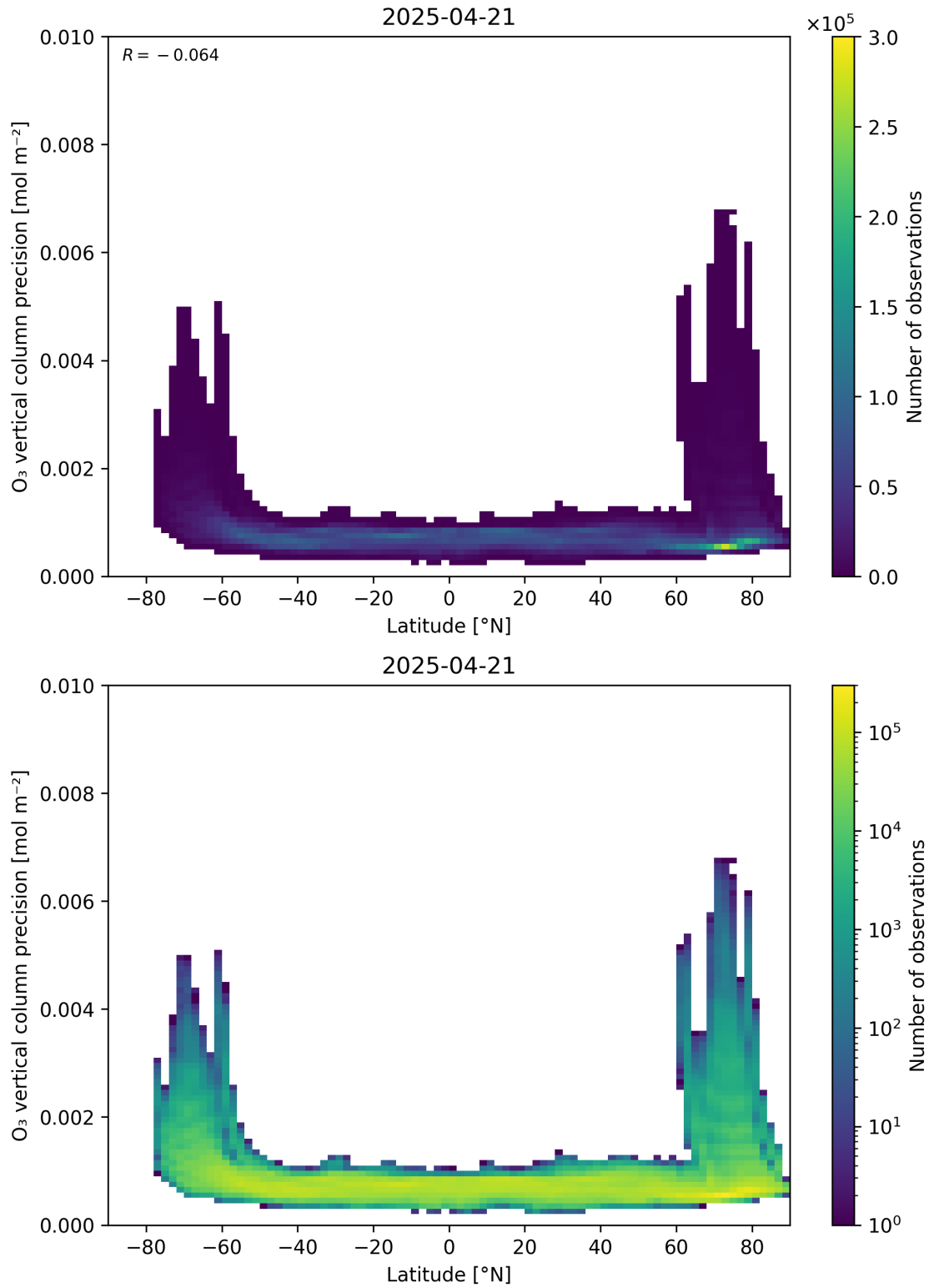
Figure 37: Scatter density plot of “Latitude” against “O 3 vertical column precision” for 2025-04-20 to 2025-04-22.
