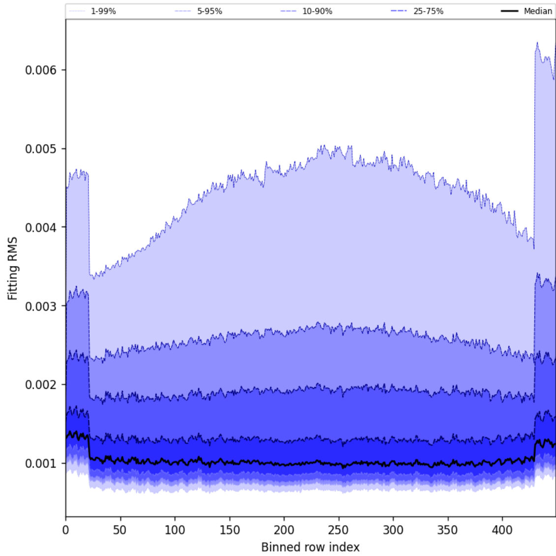
Figure 30: Along track statistics of “Fitting RMS” for 2025-04-20 to 2025-04-22
