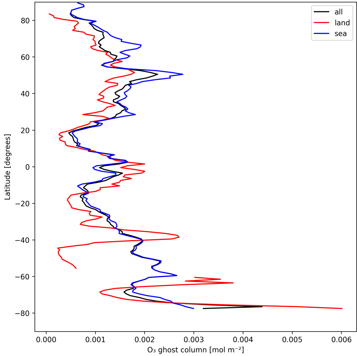
Figure 18: Zonal average of “O 3 ghost column” for 2025-04-20 to 2025-04-22.
