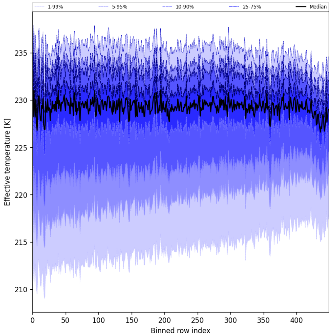
Figure 31: Along track statistics of “Effective temperature” for 2025-04-20 to 2025-04-22
