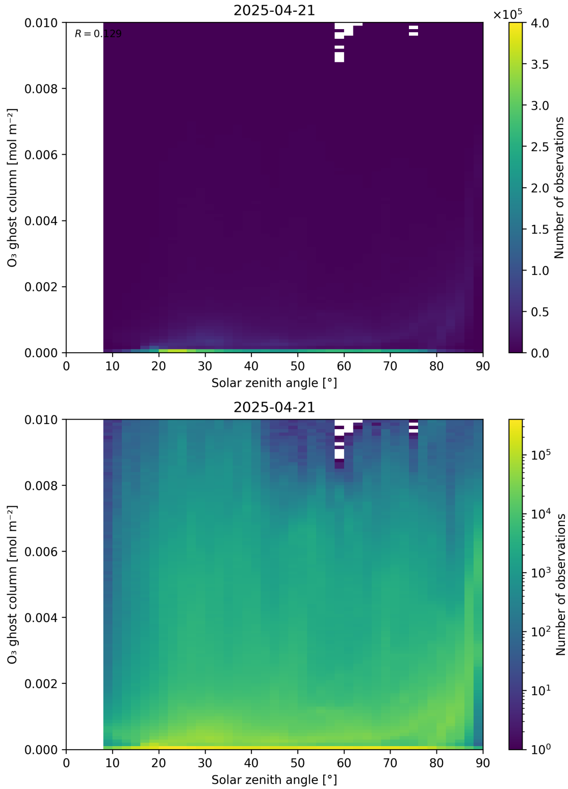
Figure 46: Scatter density plot of “Solar zenith angle” against “O 3 ghost column” for 2025-04-20 to 2025-04-22.
