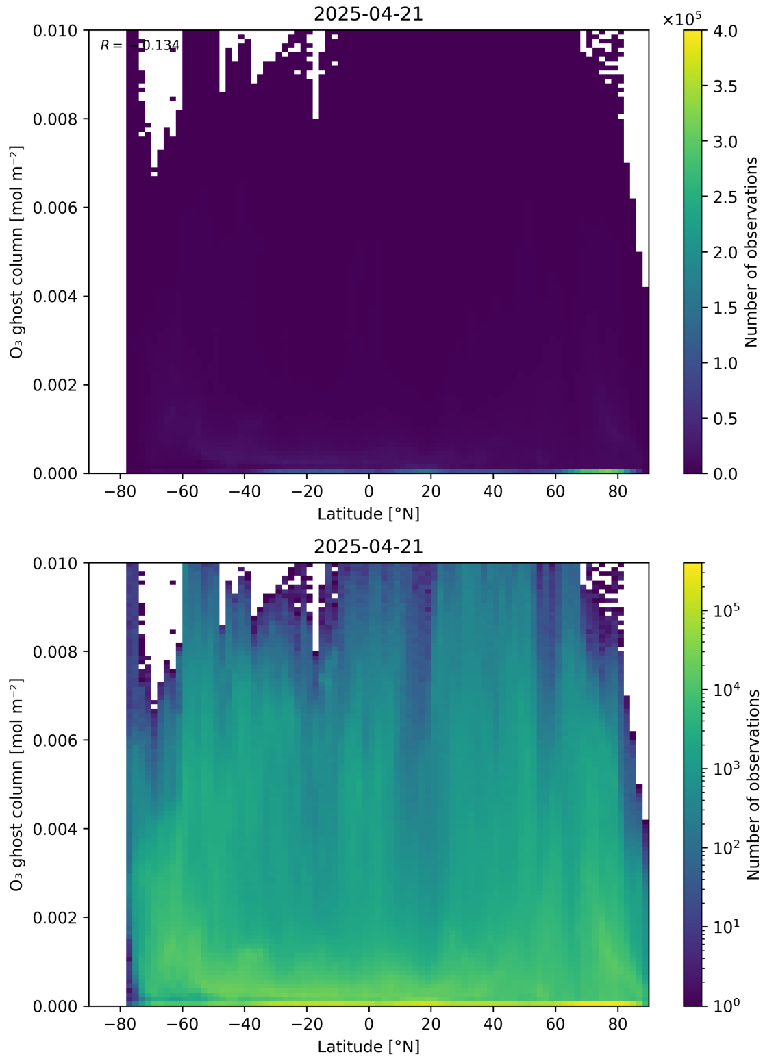
Figure 35: Scatter density plot of “Latitude” against “O 3 ghost column” for 2025-04-20 to 2025-04-22.
