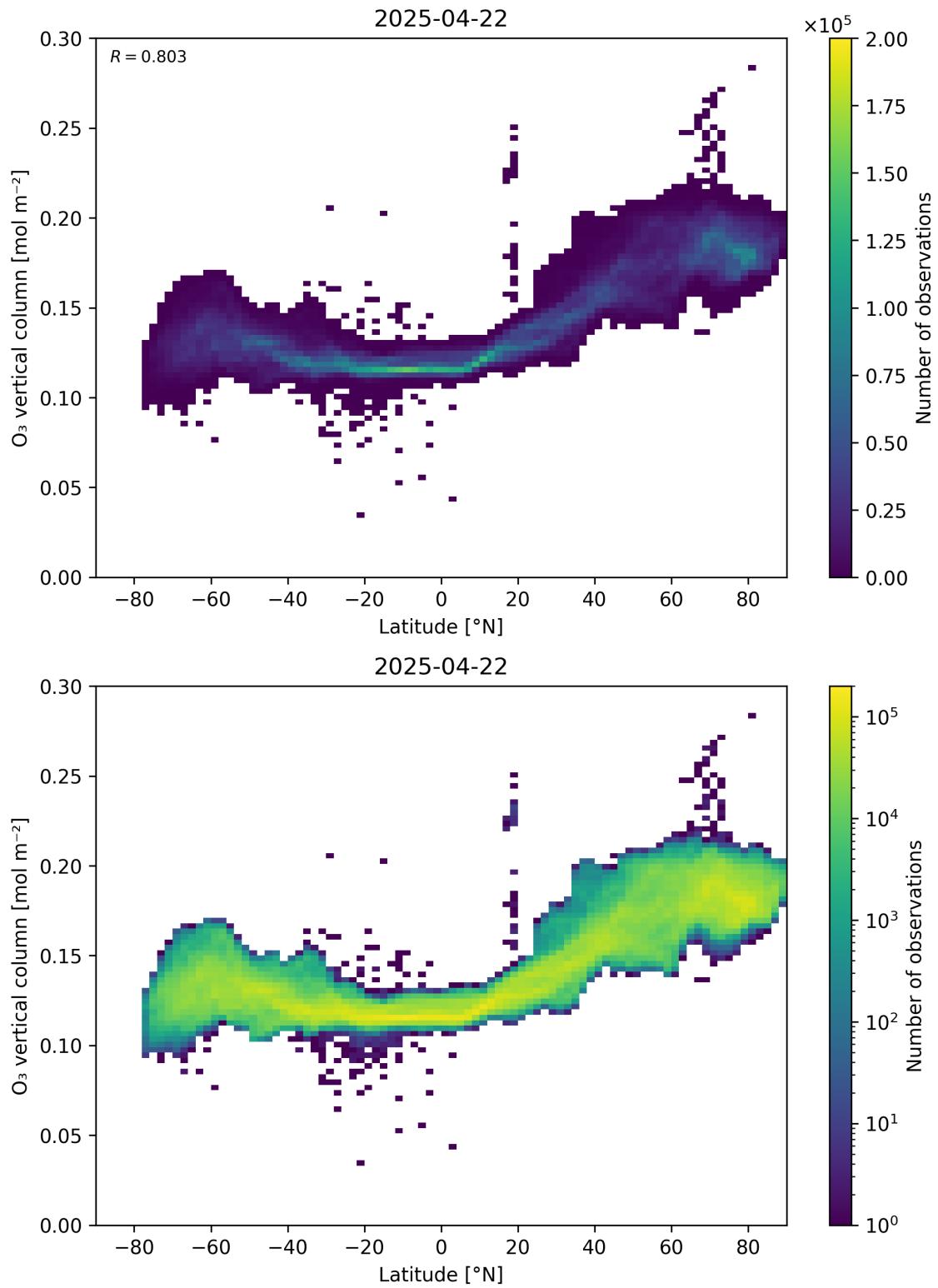
Figure 36: Scatter density plot of “Latitude” against “O 3 vertical column” for 2025-04-21 to 2025-04-23.
