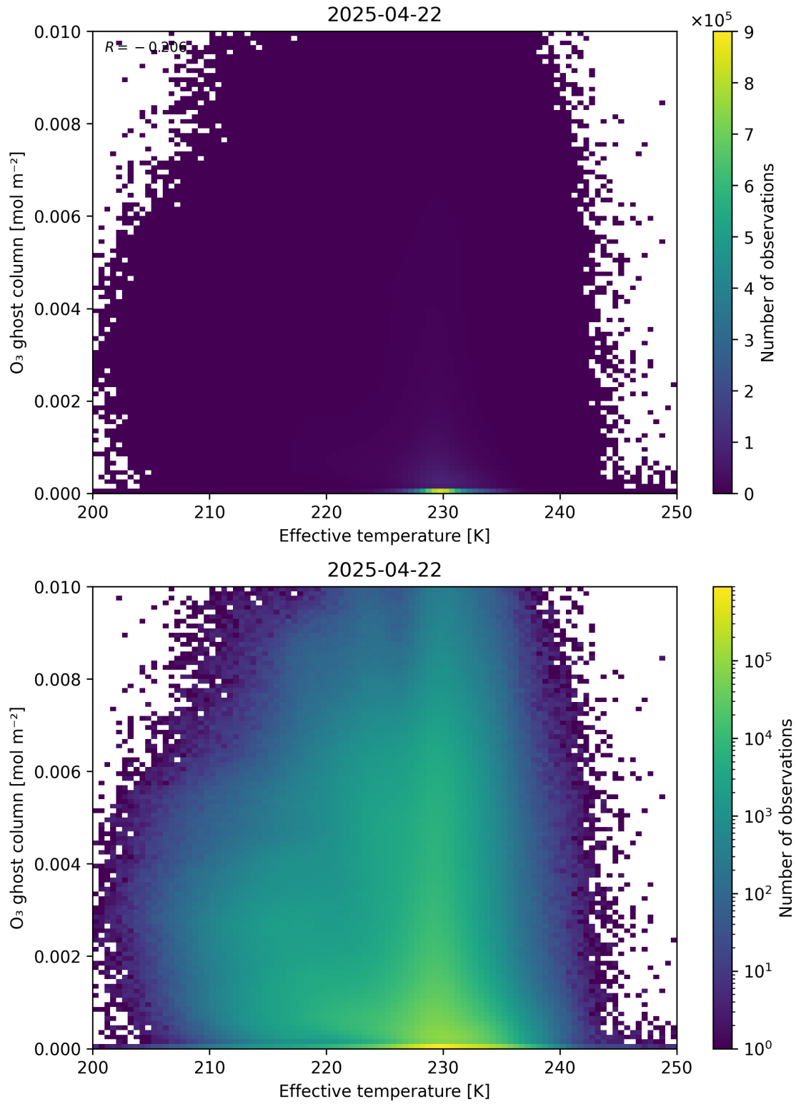
Figure 38: Scatter density plot of “Effective temperature” against “O 3 ghost column” for 2025-04-21 to 2025-04-23.
