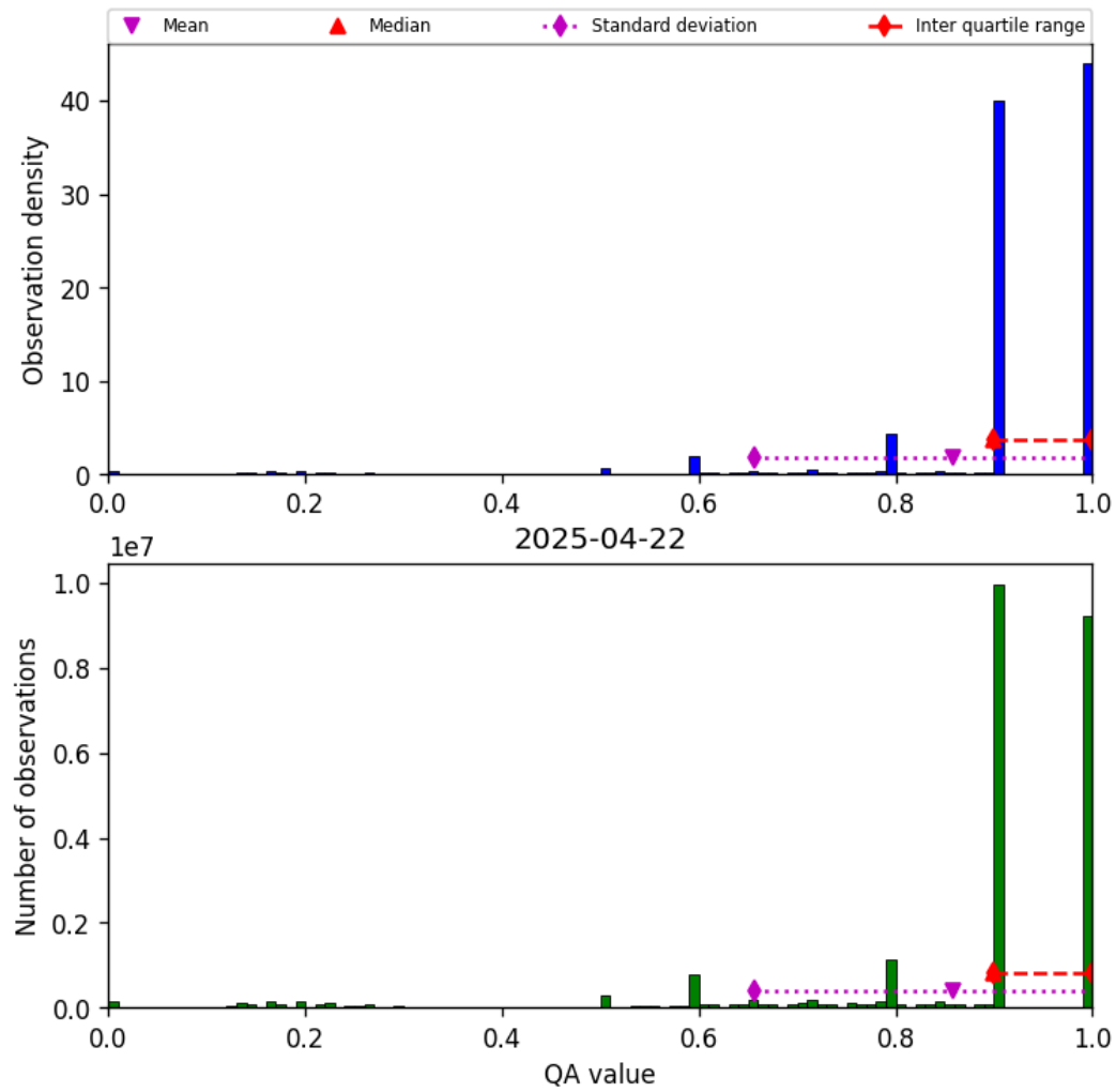
Figure 20: Histogram of “QA value” for 2025-04-21 to 2025-04-23
