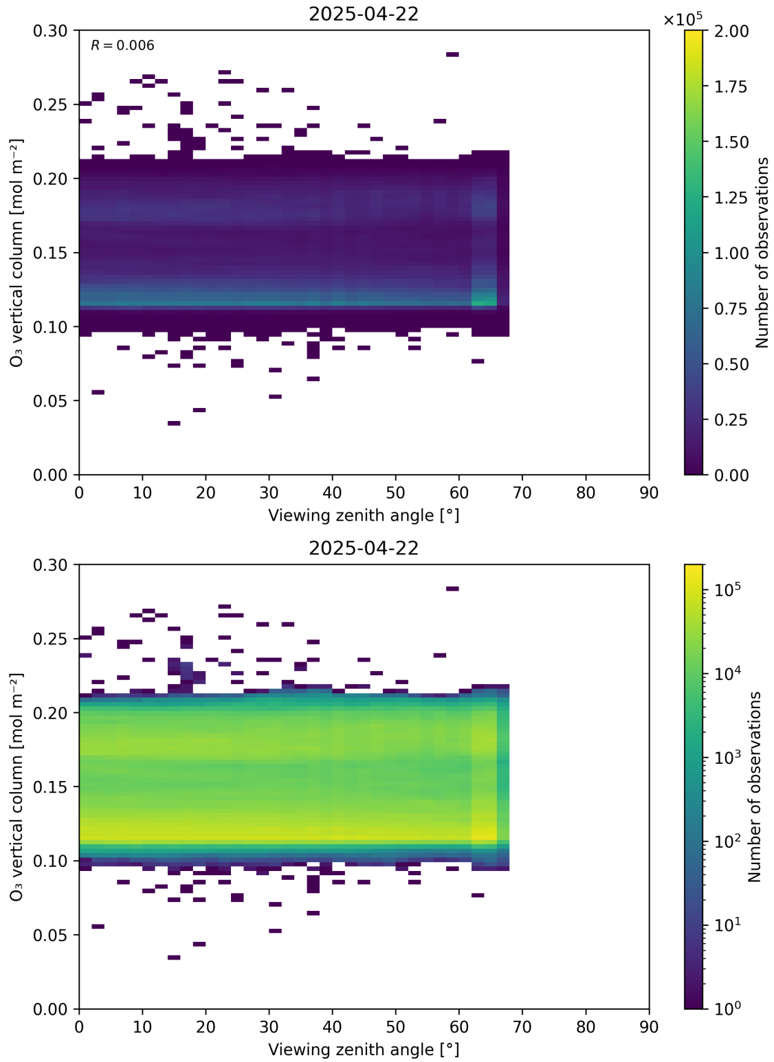
Figure 52: Scatter density plot of “Viewing zenith angle” against “O 3 vertical column” for 2025-04-21 to 2025-04-23.
