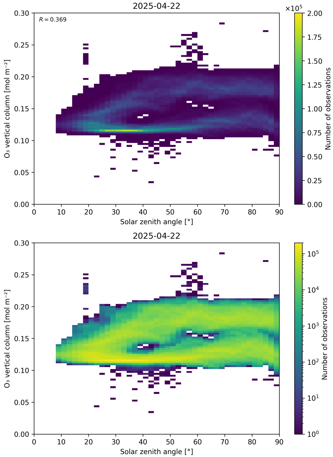
Figure 47: Scatter density plot of “Solar zenith angle” against “O 3 vertical column” for 2025-04-21 to 2025-04-23.
