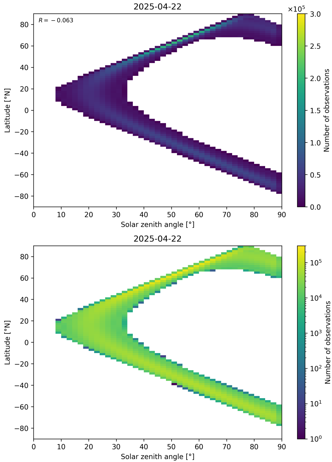
Figure 44: Scatter density plot of “Solar zenith angle” against “Latitude” for 2025-04-21 to 2025-04-23.
