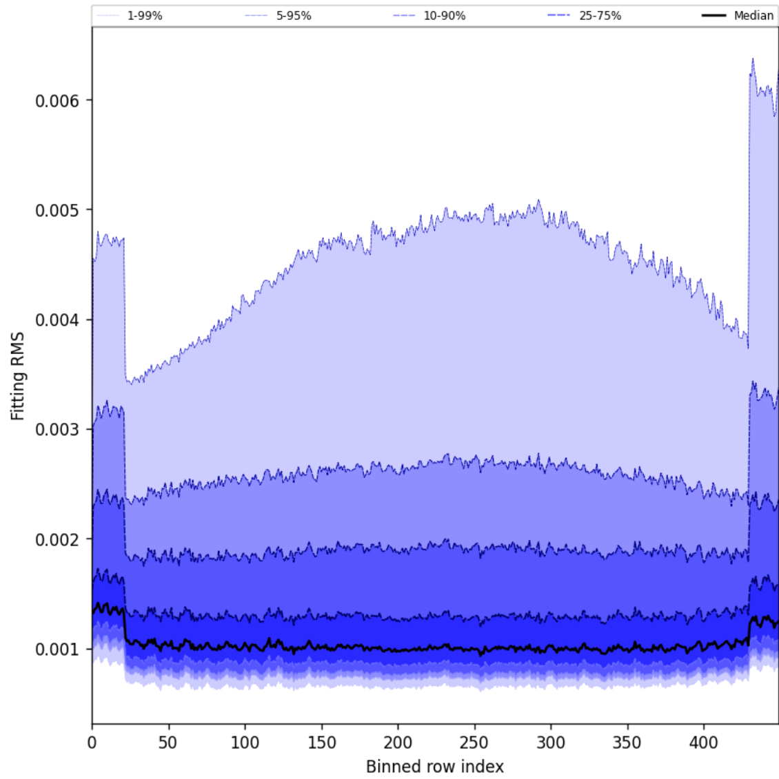
Figure 30: Along track statistics of “Fitting RMS” for 2025-04-21 to 2025-04-23
