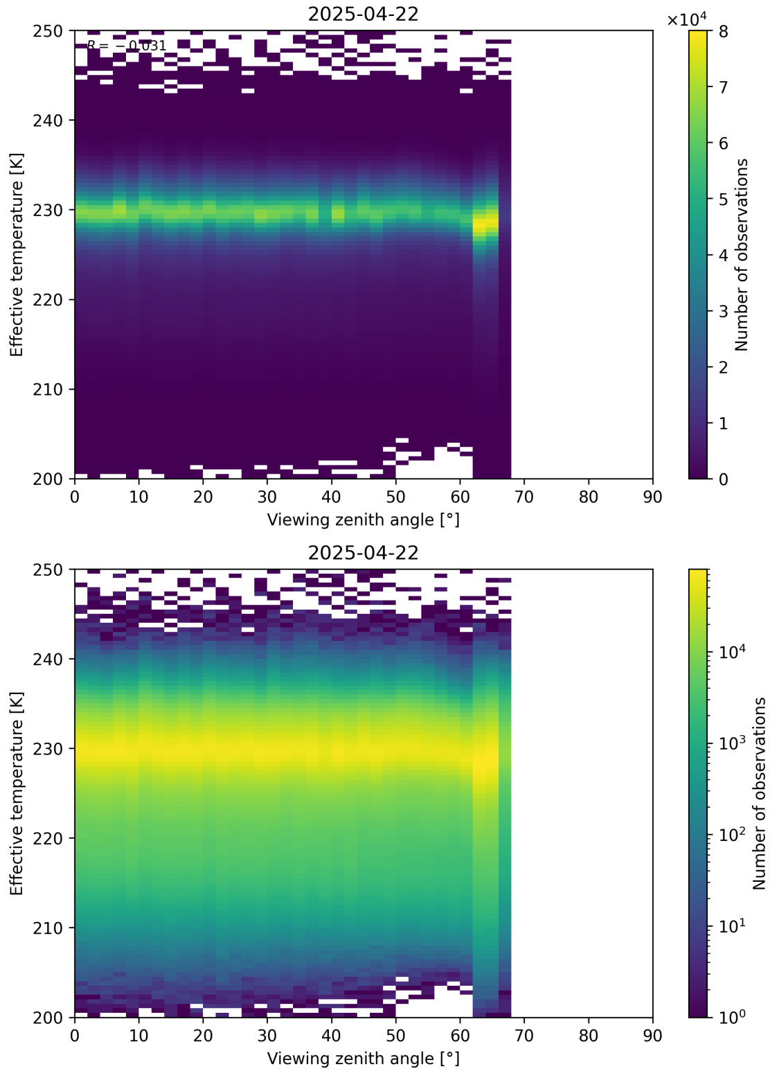
Figure 50: Scatter density plot of “Viewing zenith angle” against “Effective temperature” for 2025-04-21 to 2025-04-23.
