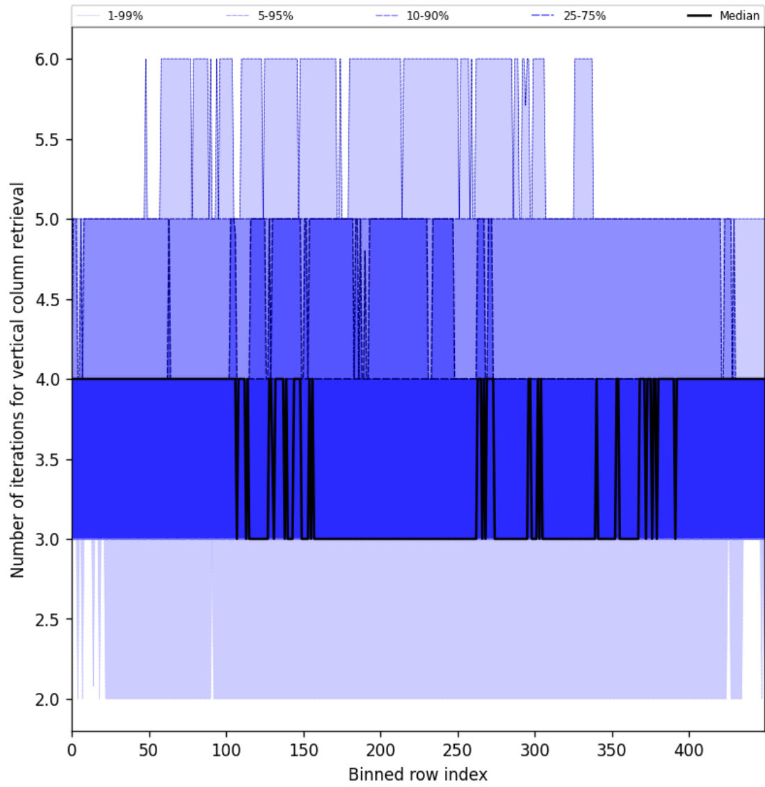
Figure 33: Along track statistics of “Number of iterations for vertical column retrieval” for 2025-04-21 to 2025-04-23
