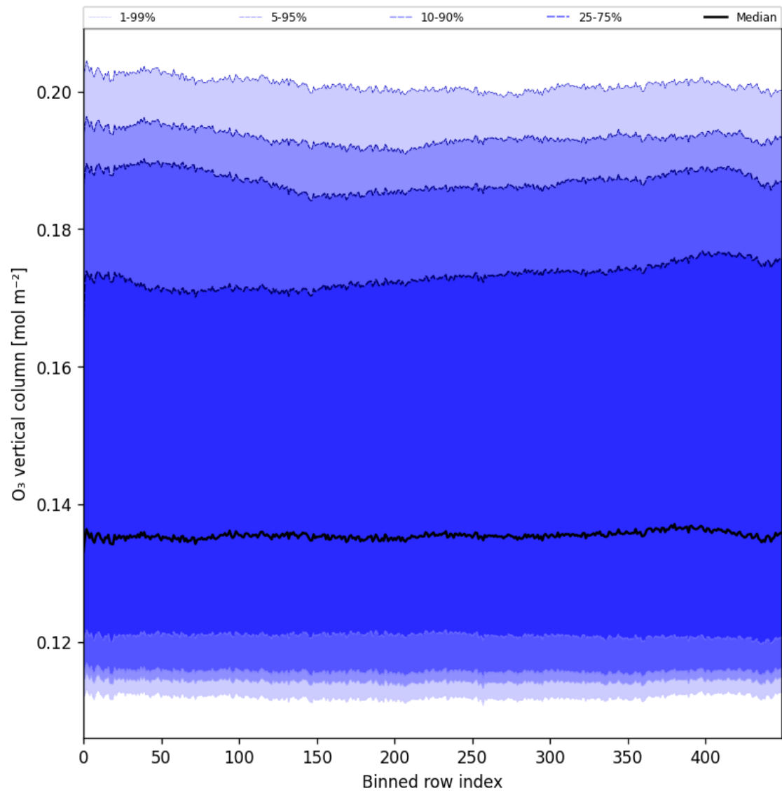
Figure 28: Along track statistics of “O 3 vertical column” for 2025-04-21 to 2025-04-23
