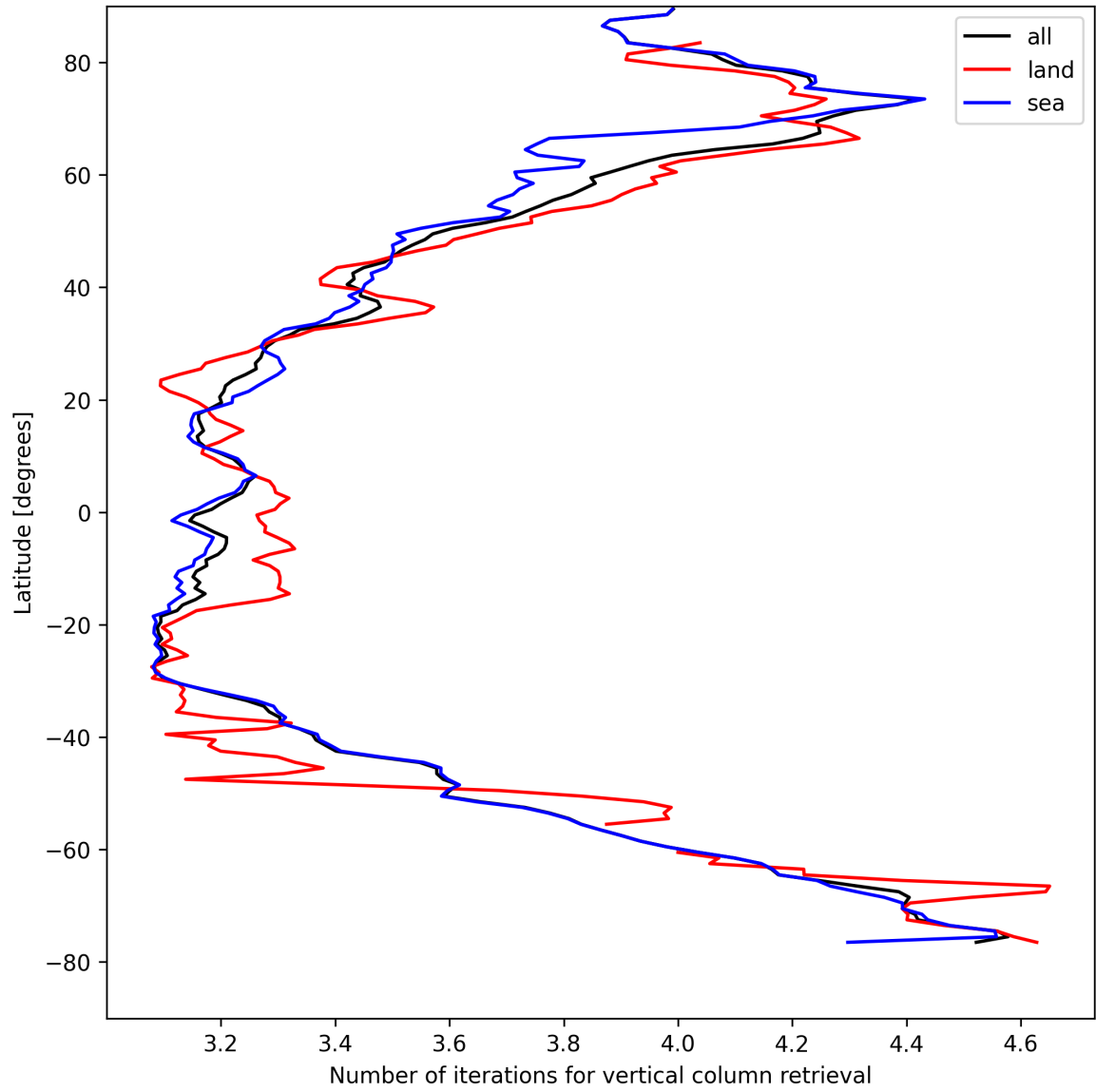
Figure 19: Zonal average of “Number of iterations for vertical column retrieval” for 2025-04-21 to 2025-04-23.
