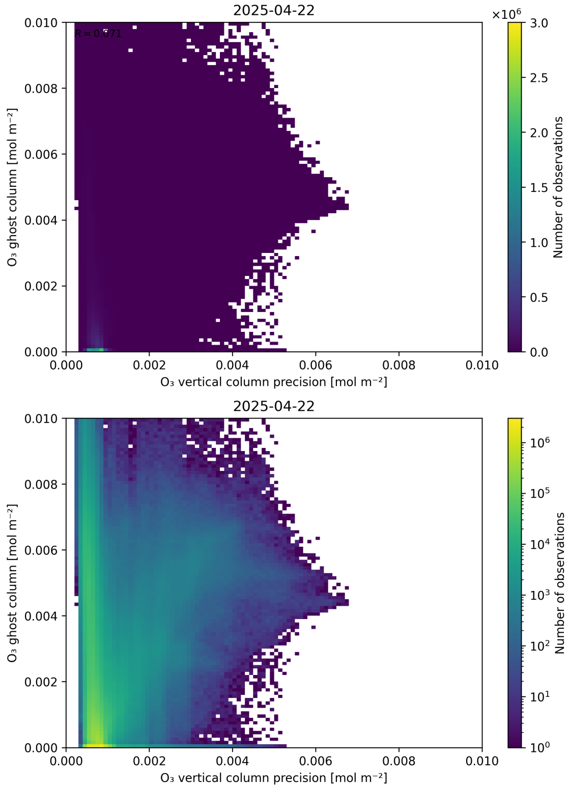
Figure 43: Scatter density plot of “ \text{O}_3 vertical column precision” against “ \text{O}_3 ghost column” for 2025-04-21 to 2025-04-23.
