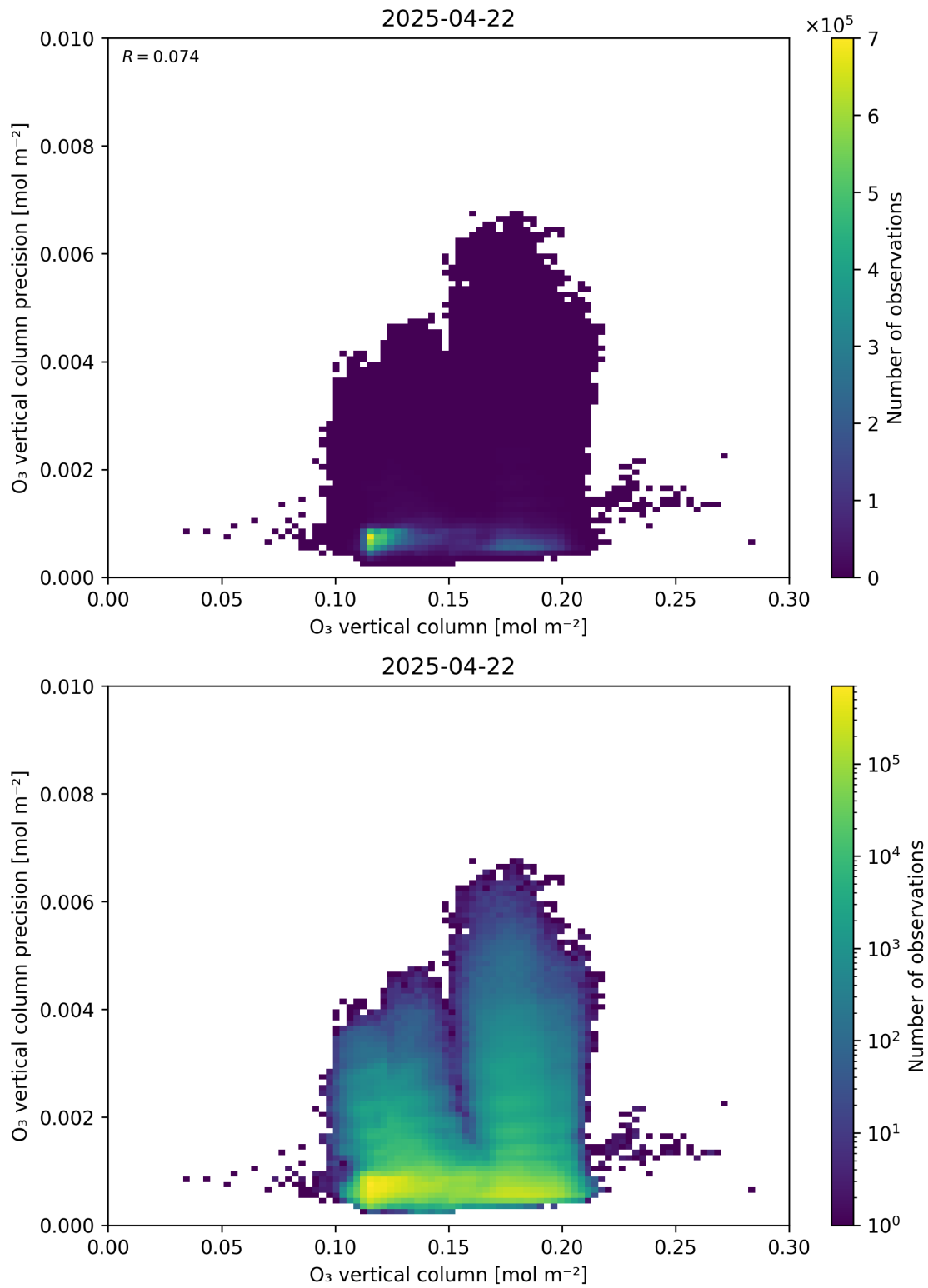
Figure 41: Scatter density plot of “O 3 vertical column” against “O 3 vertical column precision” for 2025-04-21 to 2025-04-23.
