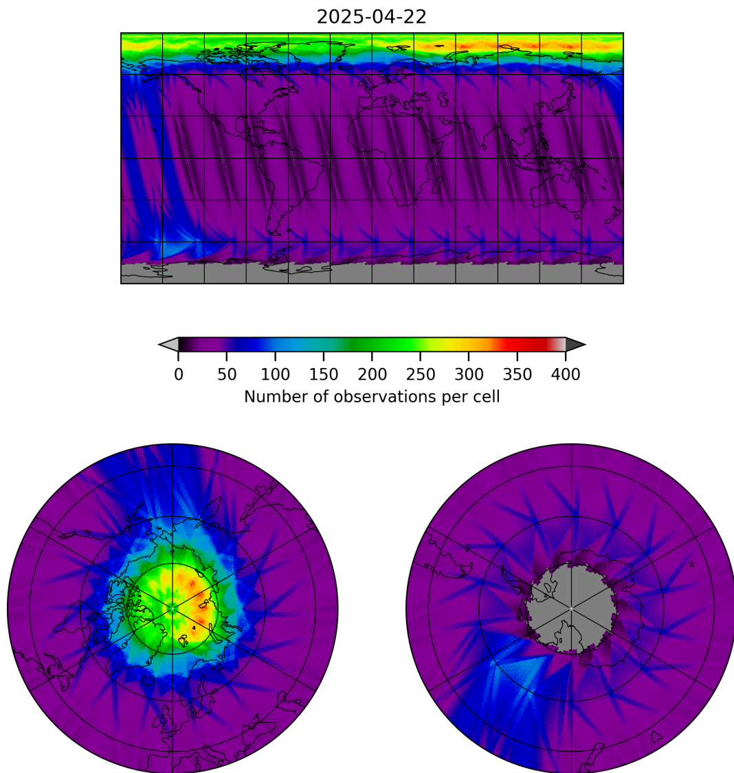
Figure 12: Map of the number of observations for 2025-04-21 to 2025-04-23
