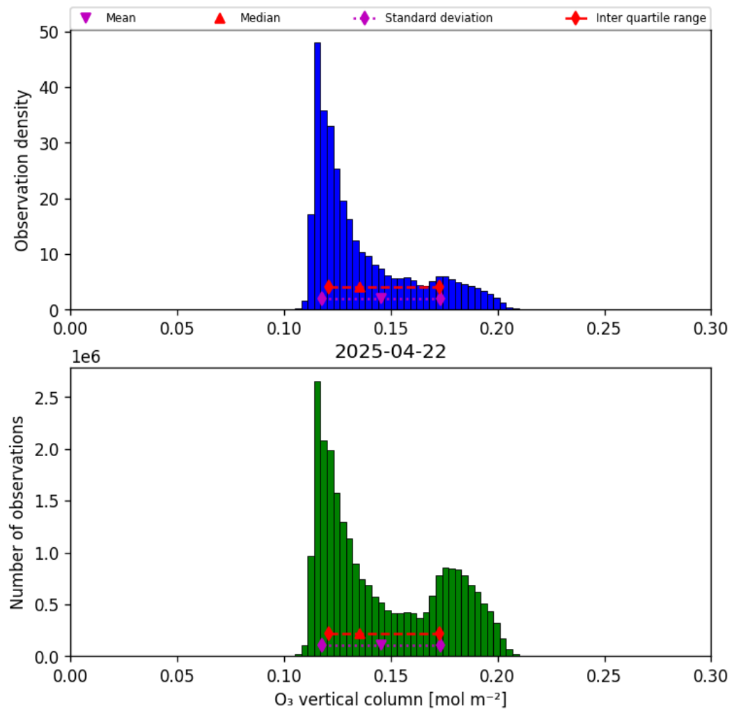
Figure 21: Histogram of “O 3 vertical column” for 2025-04-21 to 2025-04-23
