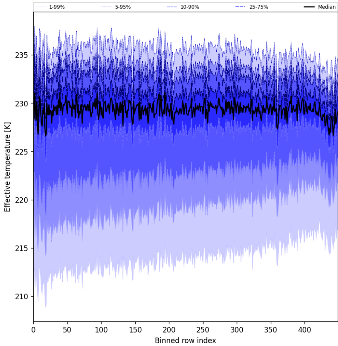
Figure 31: Along track statistics of “Effective temperature” for 2025-04-21 to 2025-04-23
