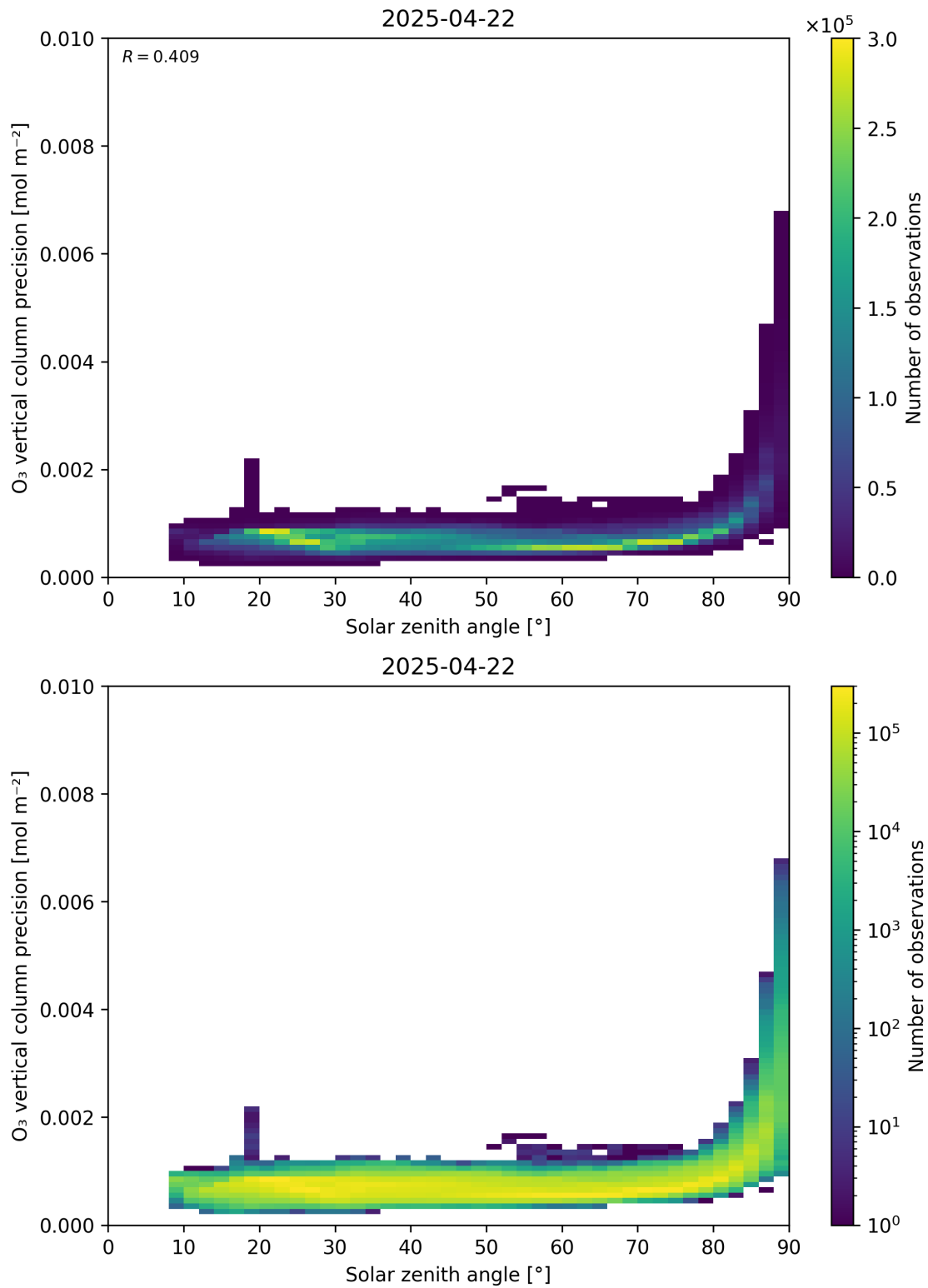
Figure 48: Scatter density plot of “Solar zenith angle” against “O 3 vertical column precision” for 2025-04-21 to 2025-04-23.
