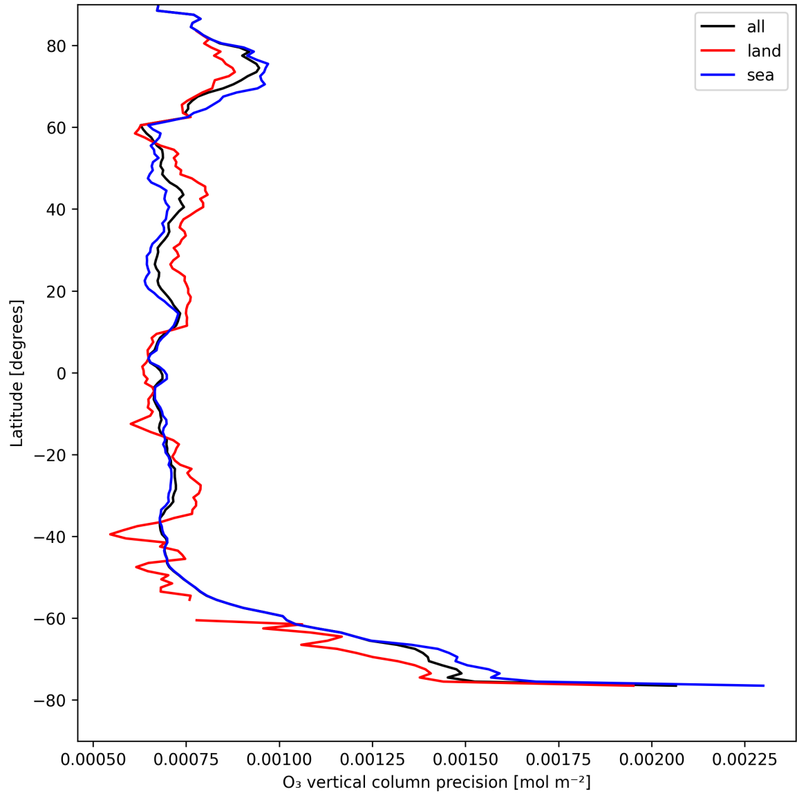
Figure 15: Zonal average of "O 3 vertical column precision" for 2025-04-21 to 2025-04-23.
