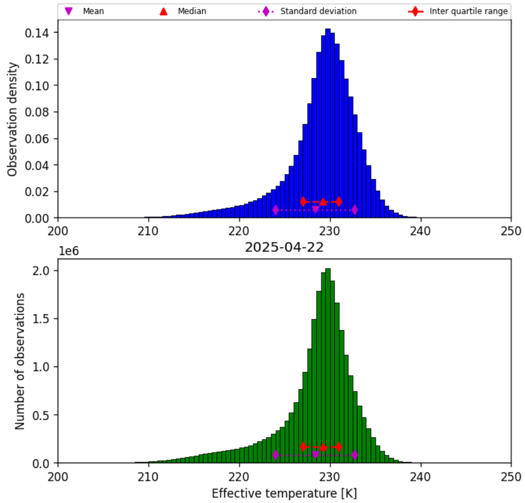
Figure 24: Histogram of “Effective temperature” for 2025-04-21 to 2025-04-23
