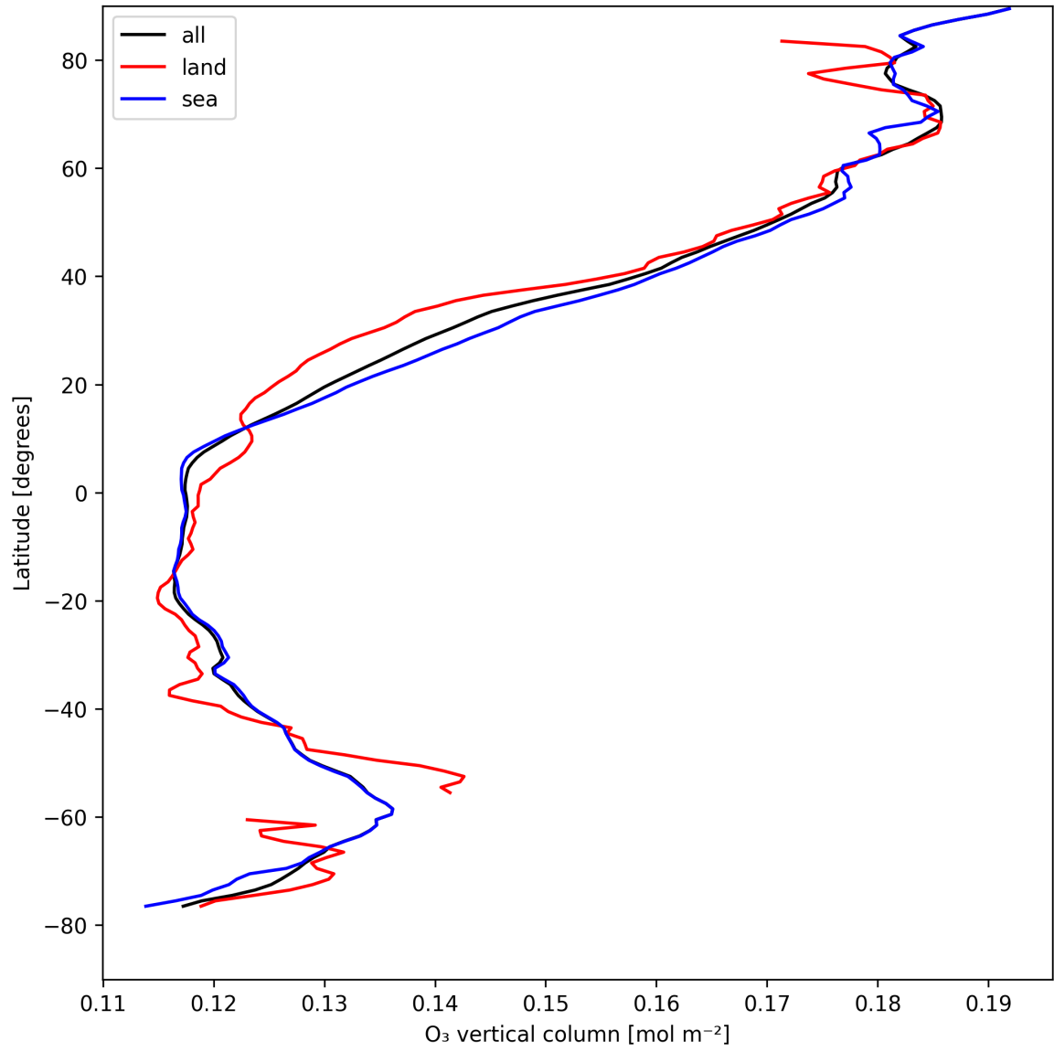
Figure 14: Zonal average of “O 3 vertical column” for 2025-04-21 to 2025-04-23.
