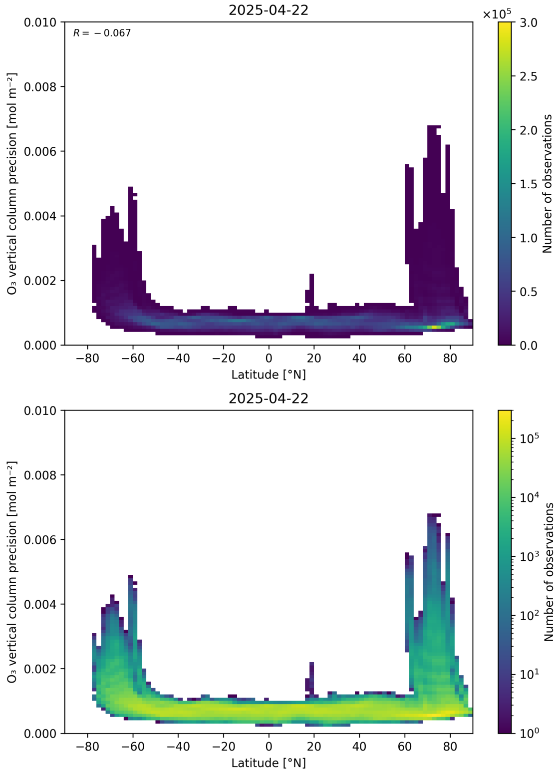
Figure 37: Scatter density plot of “Latitude” against “O 3 vertical column precision” for 2025-04-21 to 2025-04-23.
