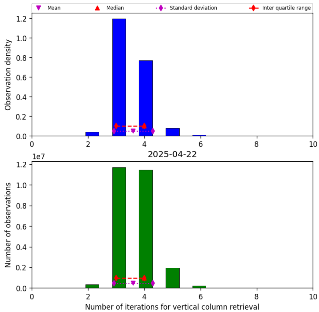
Figure 26: Histogram of “Number of iterations for vertical column retrieval” for 2025-04-21 to 2025-04-23
