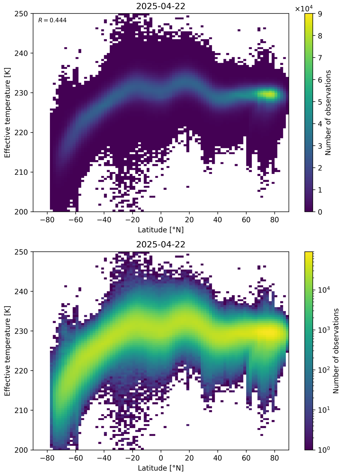
Figure 34: Scatter density plot of “Latitude” against “Effective temperature” for 2025-04-21 to 2025-04-23.
