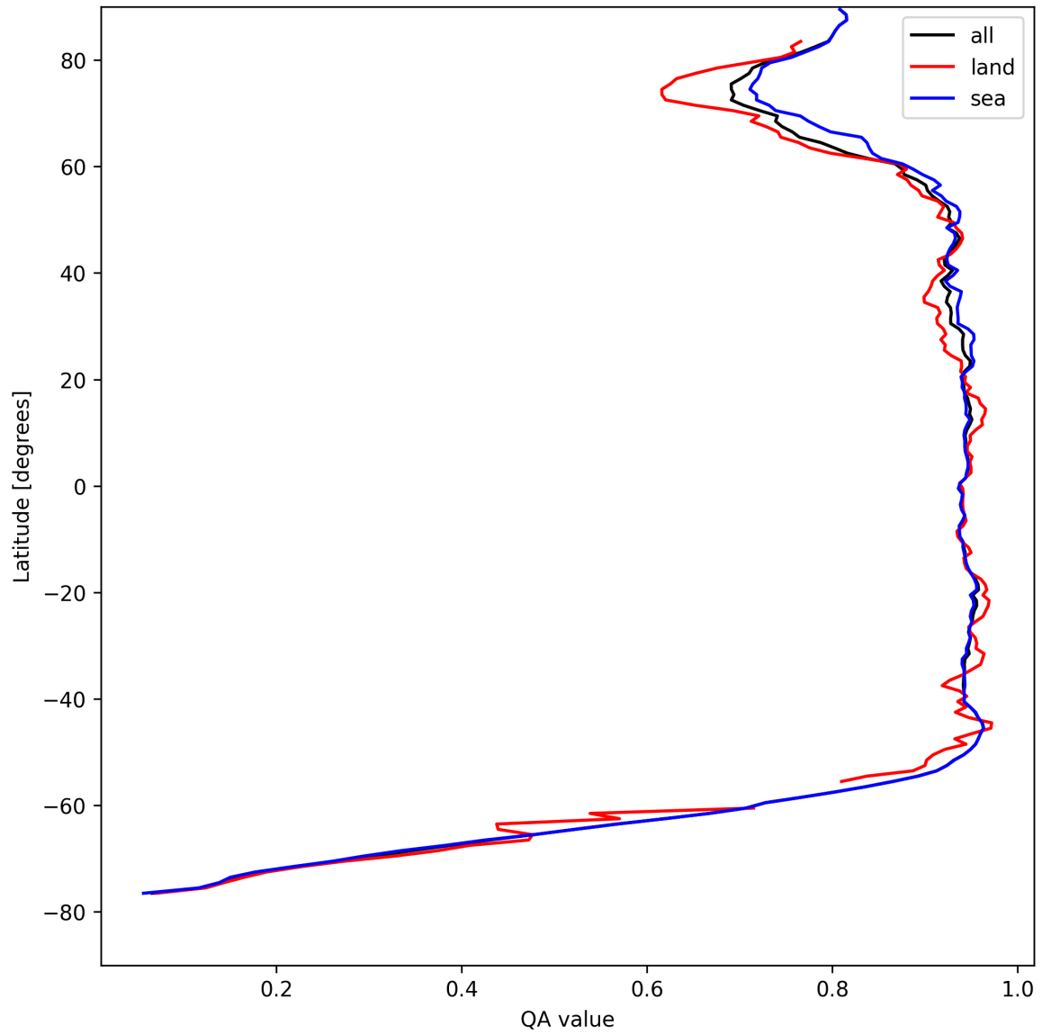
Figure 13: Zonal average of “QA value” for 2025-04-21 to 2025-04-23.
