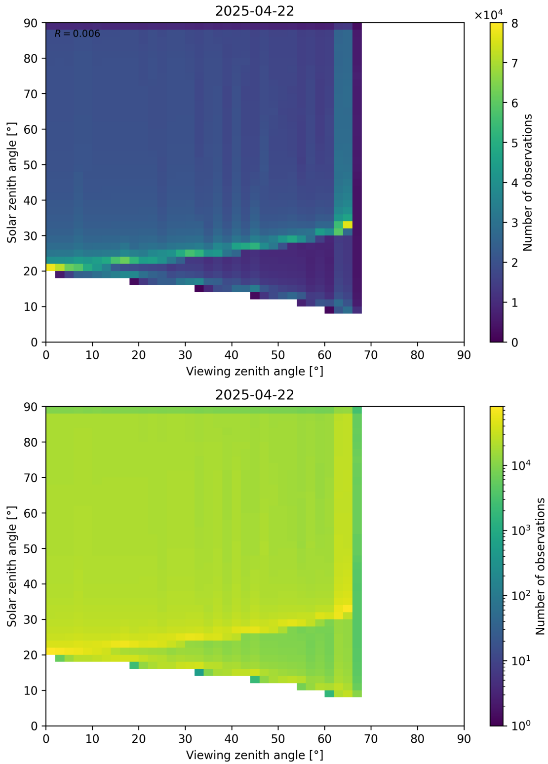
Figure 54: Scatter density plot of “Viewing zenith angle” against “Solar zenith angle” for 2025-04-21 to 2025-04-23.
