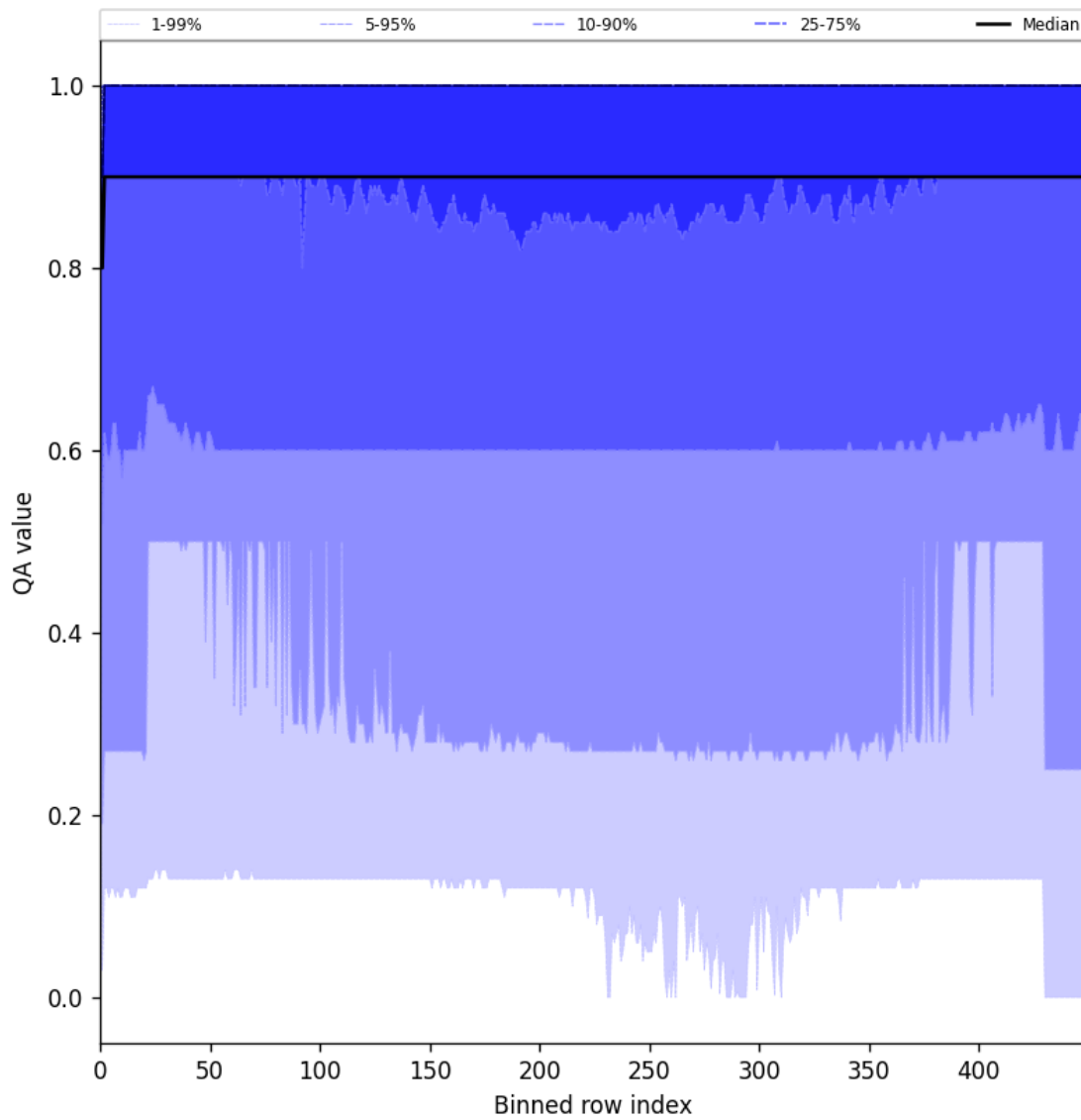
Figure 27: Along track statistics of “QA value” for 2025-04-21 to 2025-04-23
