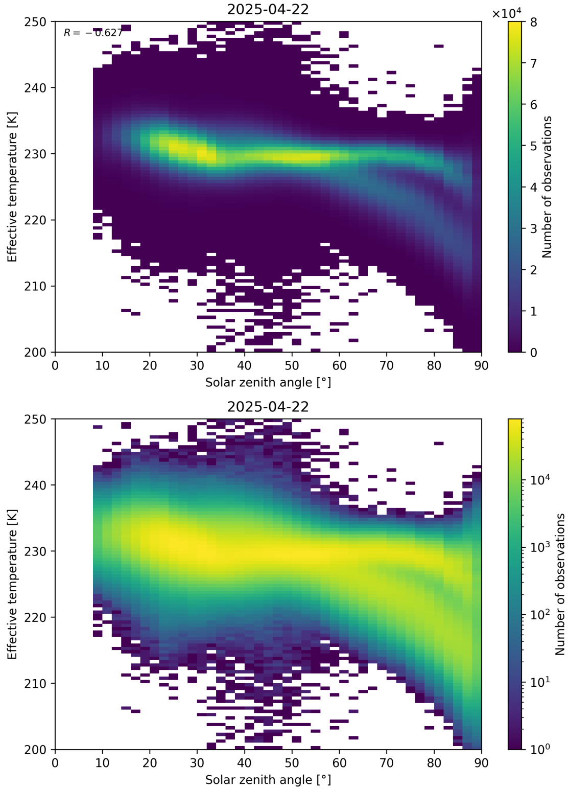
Figure 45: Scatter density plot of “Solar zenith angle” against “Effective temperature” for 2025-04-21 to 2025-04-23.
