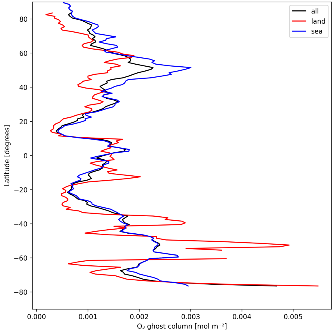
Figure 18: Zonal average of “O 3 ghost column” for 2025-04-21 to 2025-04-23.
