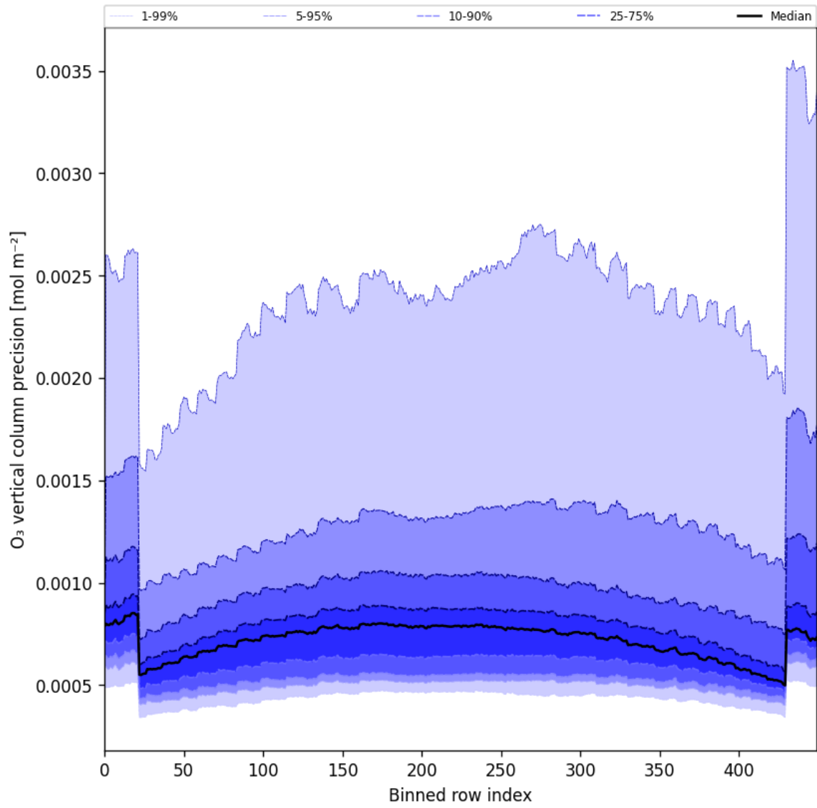
Figure 29: Along track statistics of “O 3 vertical column precision” for 2025-04-21 to 2025-04-23
