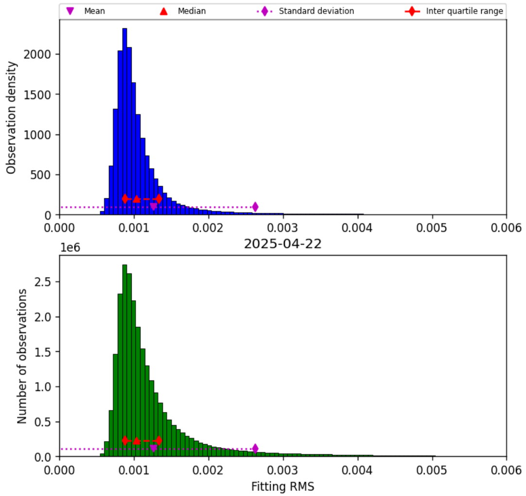
Figure 23: Histogram of “Fitting RMS” for 2025-04-21 to 2025-04-23
