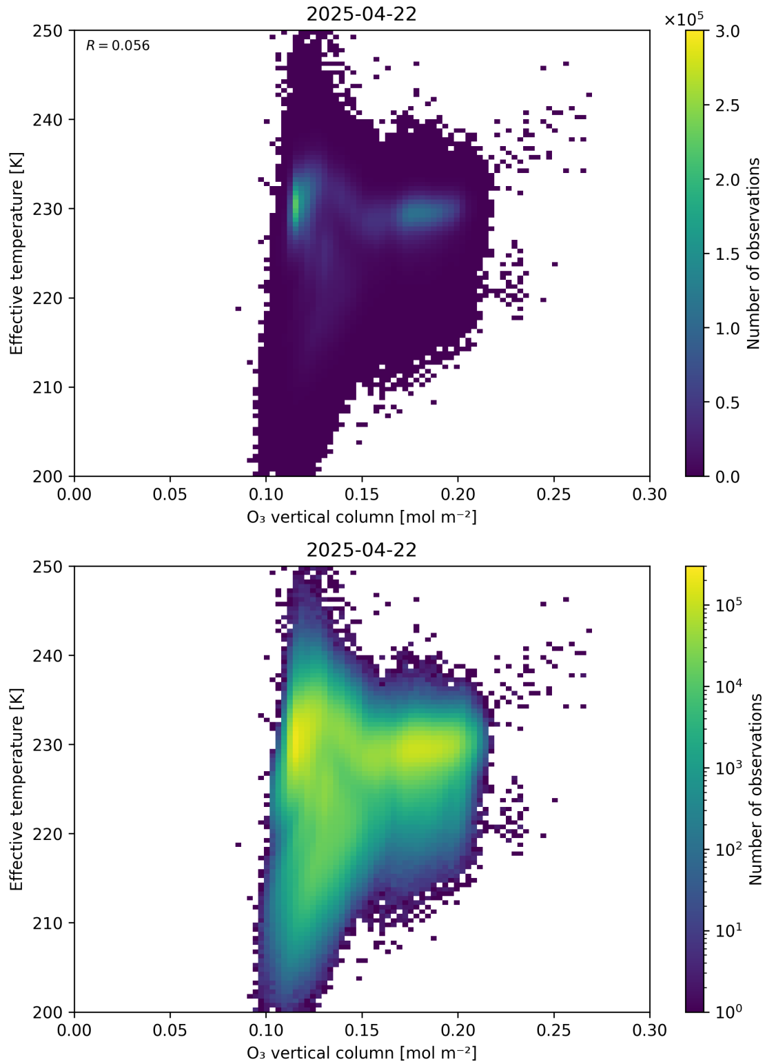
Figure 39: Scatter density plot of “O 3 vertical column” against “Effective temperature” for 2025-04-21 to 2025-04-23.
