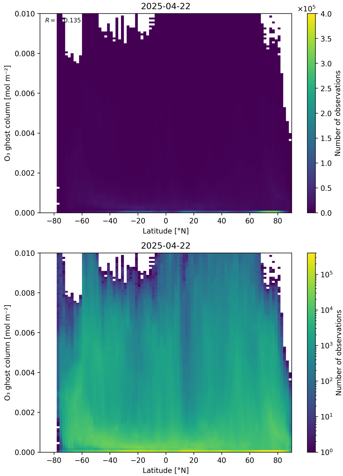
Figure 35: Scatter density plot of “Latitude” against “O 3 ghost column” for 2025-04-21 to 2025-04-23.
