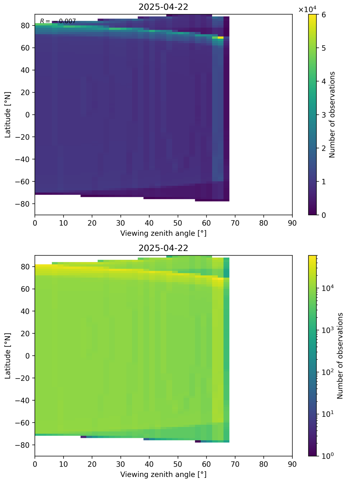
Figure 49: Scatter density plot of “Viewing zenith angle” against “Latitude” for 2025-04-21 to 2025-04-23.
