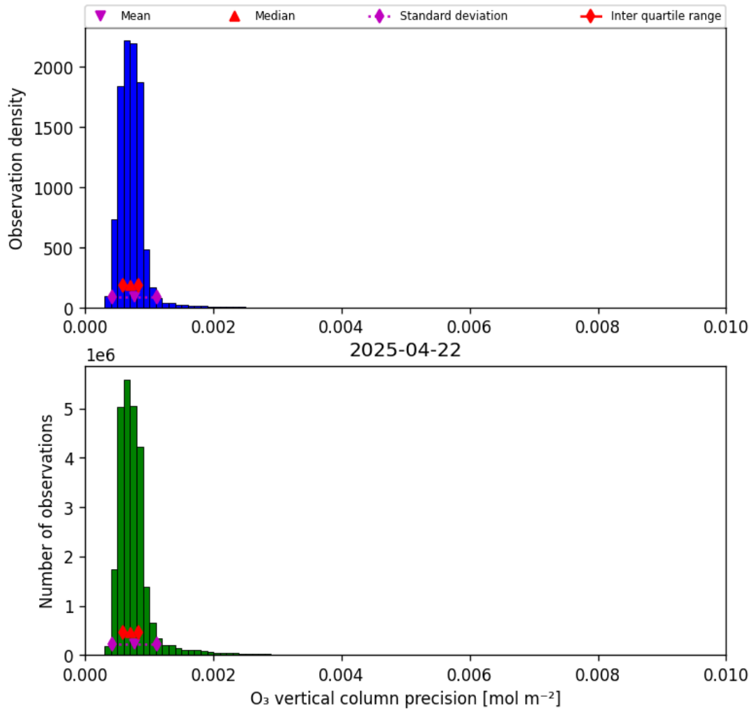
Figure 22: Histogram of “O 3 vertical column precision” for 2025-04-21 to 2025-04-23
