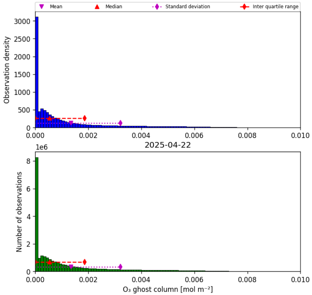
Figure 25: Histogram of “O 3 ghost column” for 2025-04-21 to 2025-04-23
