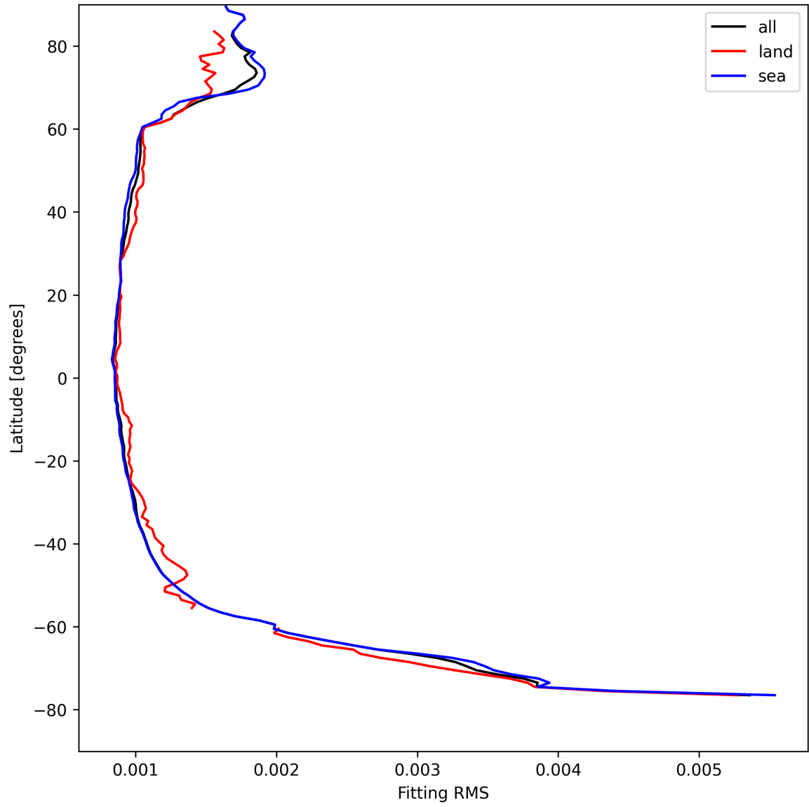
Figure 16: Zonal average of “Fitting RMS” for 2025-04-22 to 2025-04-24.
