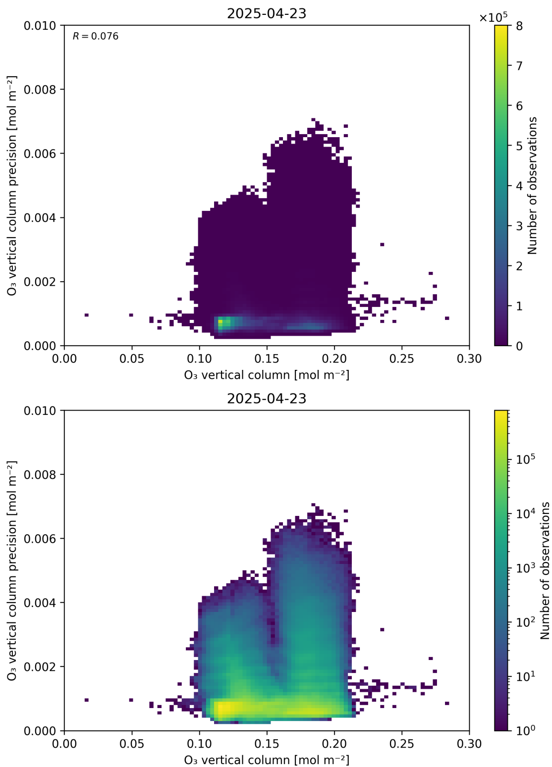
Figure 41: Scatter density plot of “O 3 vertical column” against “O 3 vertical column precision” for 2025-04-22 to 2025-04-24.
