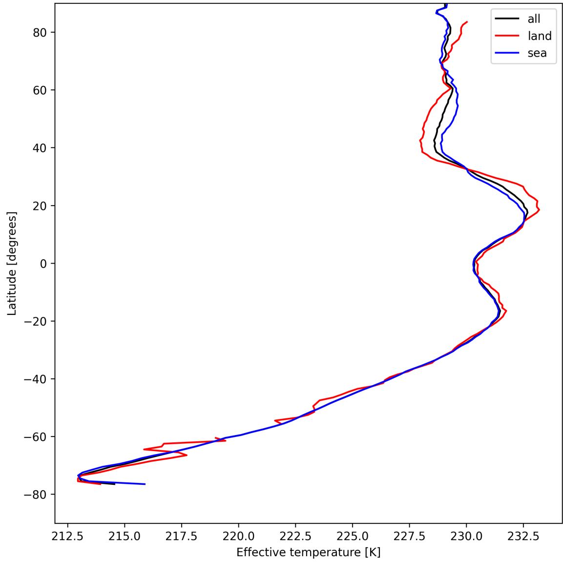
Figure 17: Zonal average of "Effective temperature" for 2025-04-22 to 2025-04-24.
