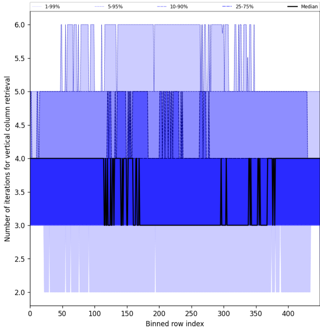
Figure 33: Along track statistics of “Number of iterations for vertical column retrieval” for 2025-04-22 to 2025-04-24
