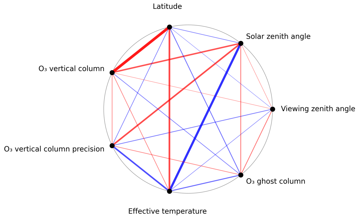
Figure 1: Map of correlation graph for 2025-04-22 to 2025-04-24.
