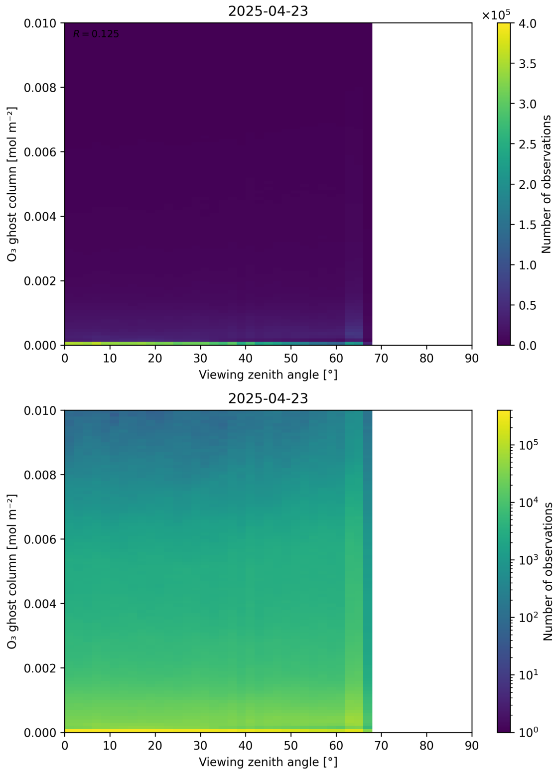
Figure 51: Scatter density plot of “Viewing zenith angle” against “O 3 ghost column” for 2025-04-22 to 2025-04-24.
