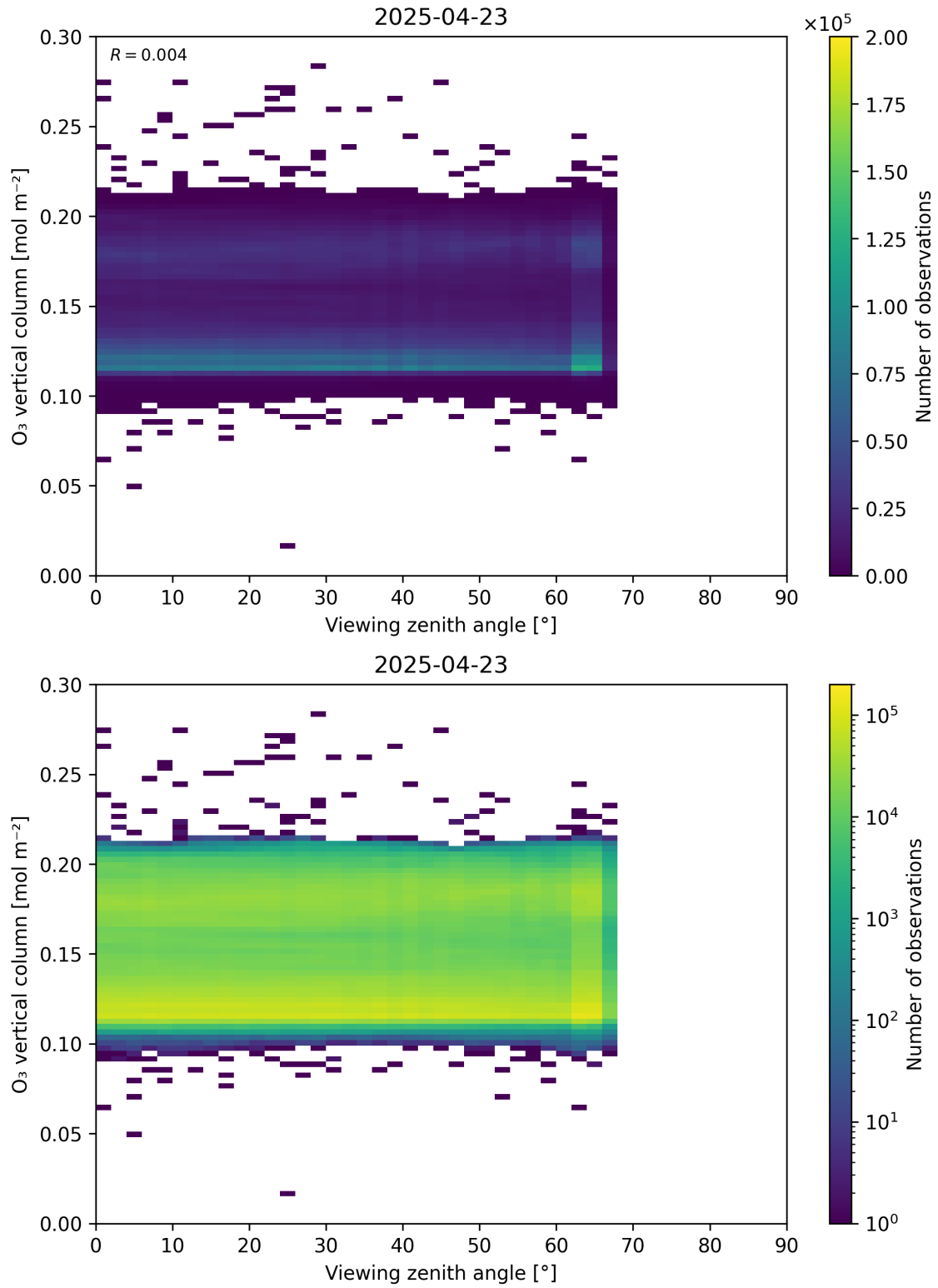
Figure 52: Scatter density plot of “Viewing zenith angle” against “O 3 vertical column” for 2025-04-22 to 2025-04-24.
