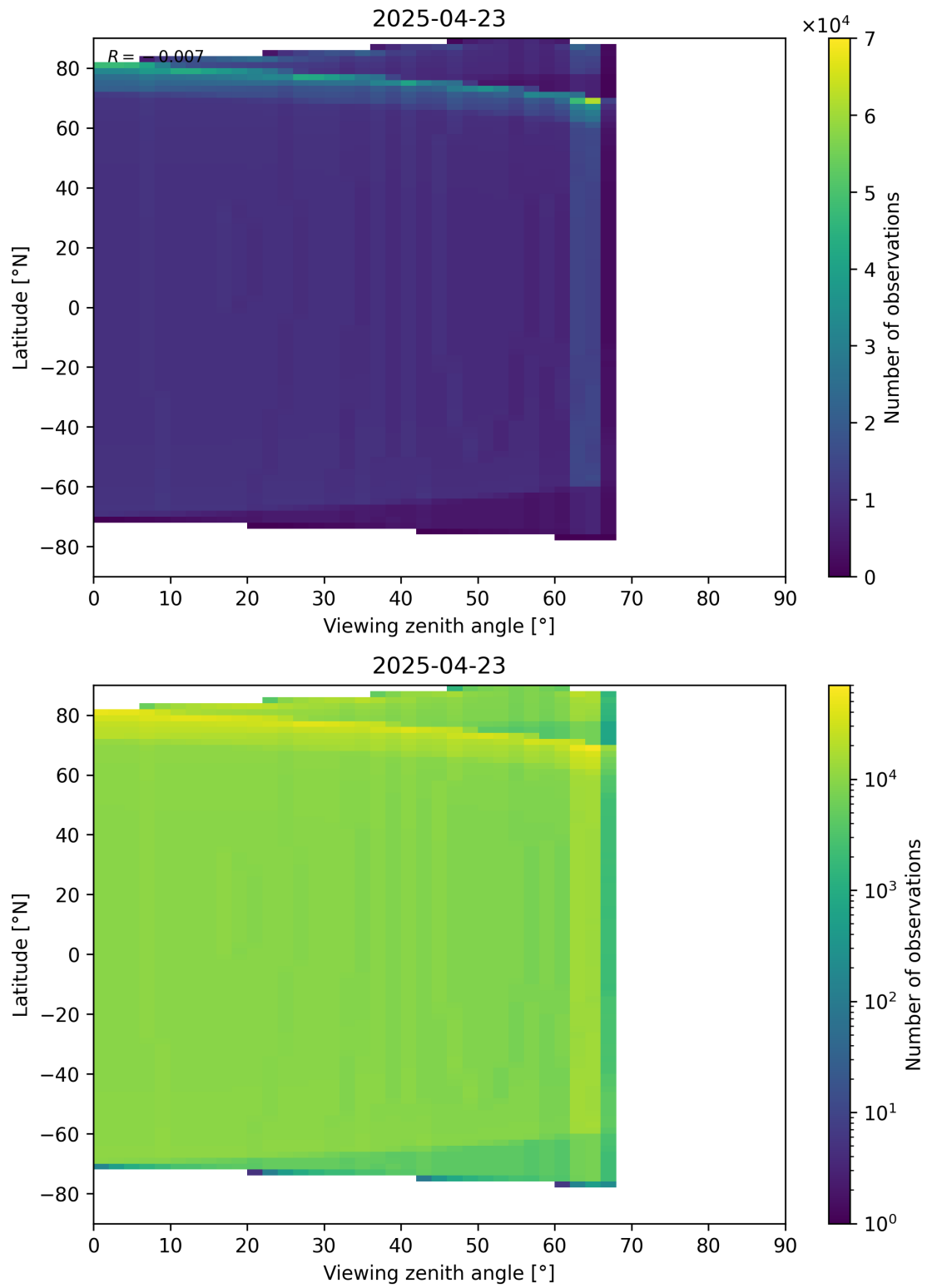
Figure 49: Scatter density plot of “Viewing zenith angle” against “Latitude” for 2025-04-22 to 2025-04-24.
