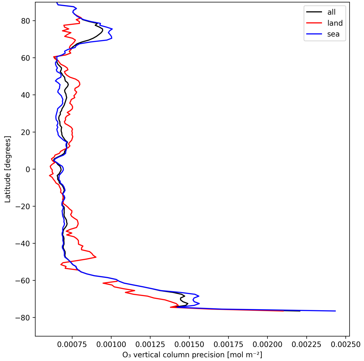
Figure 15: Zonal average of “O 3 vertical column precision” for 2025-04-22 to 2025-04-24.
