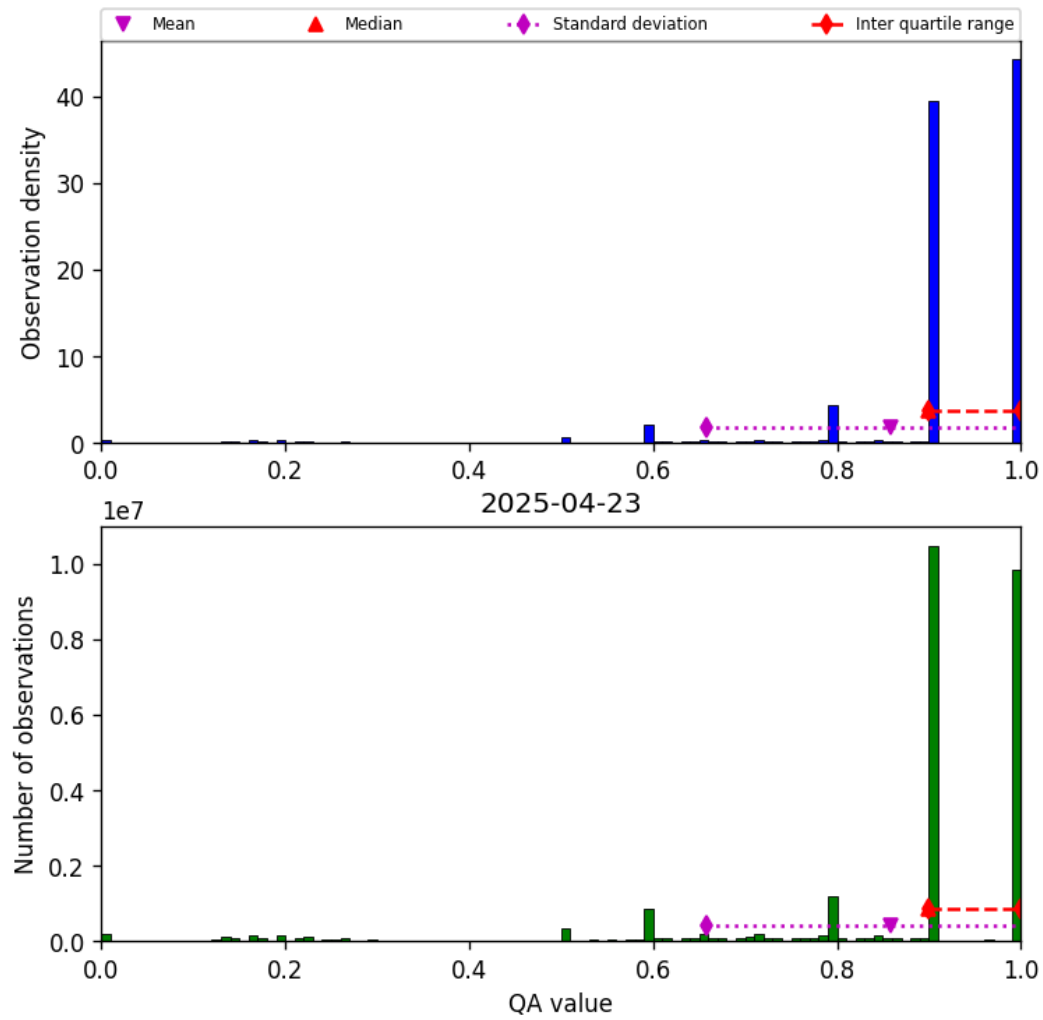
Figure 20: Histogram of “QA value” for 2025-04-22 to 2025-04-24
