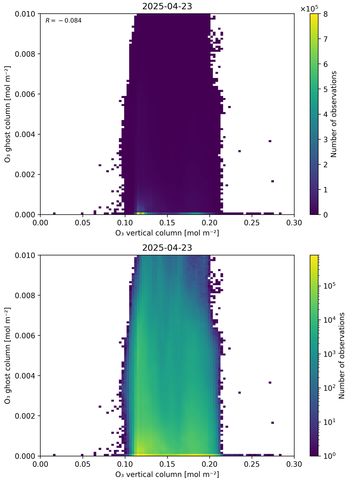
Figure 40: Scatter density plot of “O 3 vertical column” against “O 3 ghost column” for 2025-04-22 to 2025-04-24.
