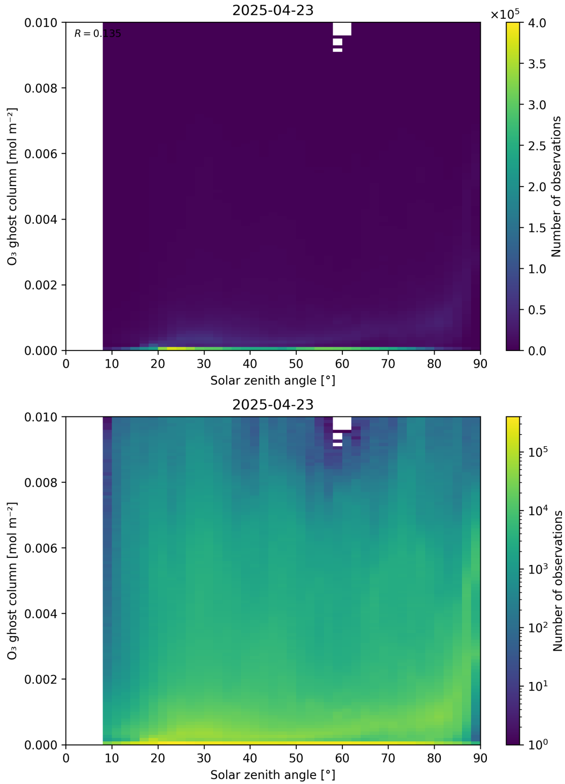
Figure 46: Scatter density plot of “Solar zenith angle” against “O 3 ghost column” for 2025-04-22 to 2025-04-24.
