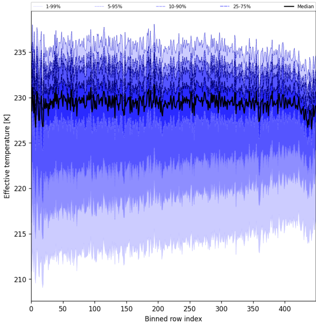
Figure 31: Along track statistics of “Effective temperature” for 2025-04-22 to 2025-04-24
