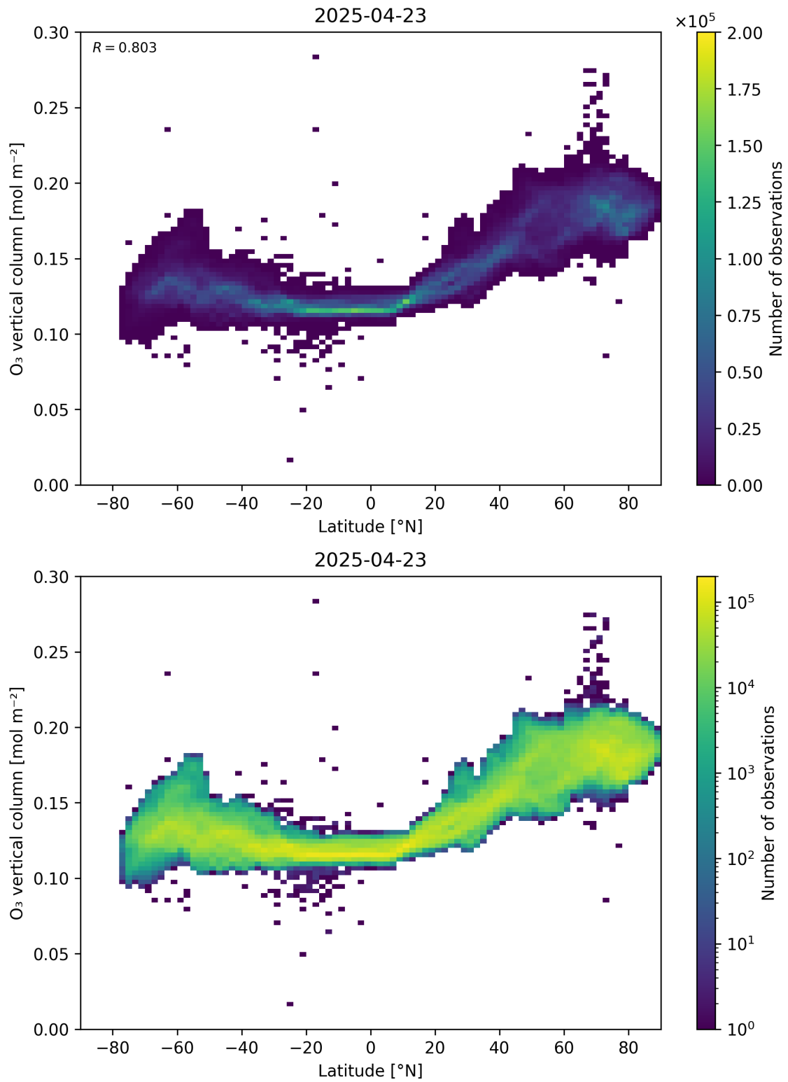
Figure 36: Scatter density plot of “Latitude” against “O 3 vertical column” for 2025-04-22 to 2025-04-24.
