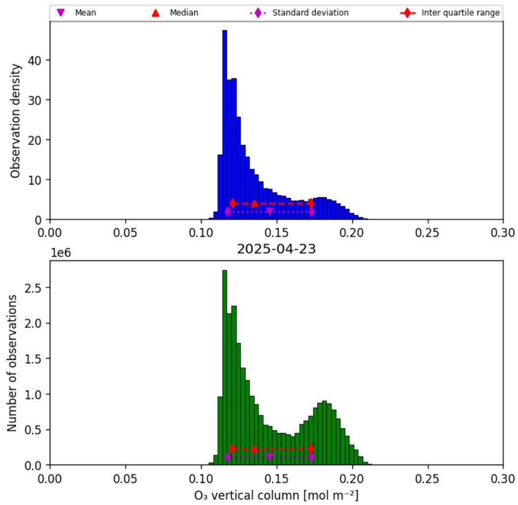
Figure 21: Histogram of “O 3 vertical column” for 2025-04-22 to 2025-04-24
