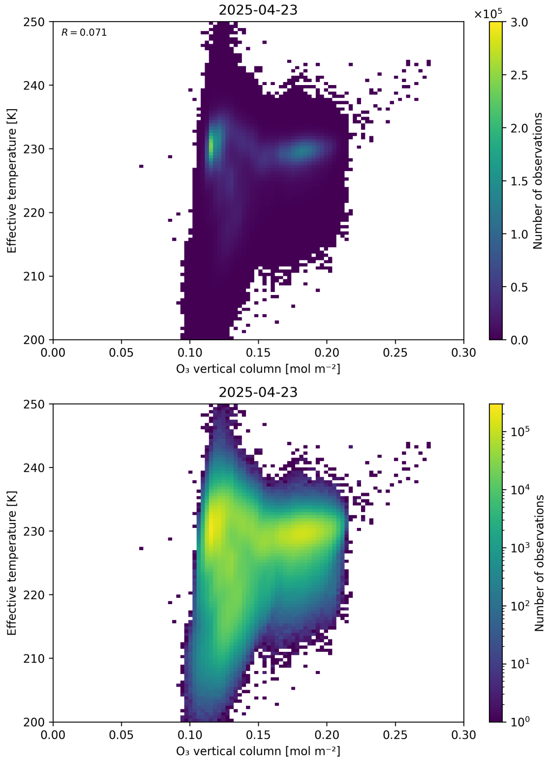
Figure 39: Scatter density plot of “O 3 vertical column” against “Effective temperature” for 2025-04-22 to 2025-04-24.
