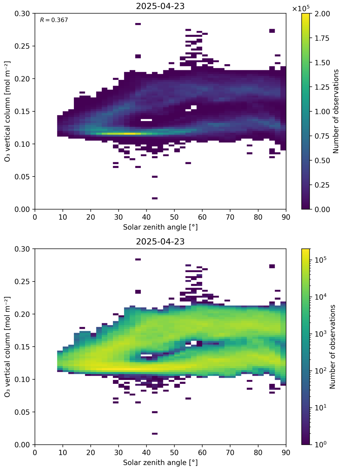
Figure 47: Scatter density plot of “Solar zenith angle” against “O 3 vertical column” for 2025-04-22 to 2025-04-24.
