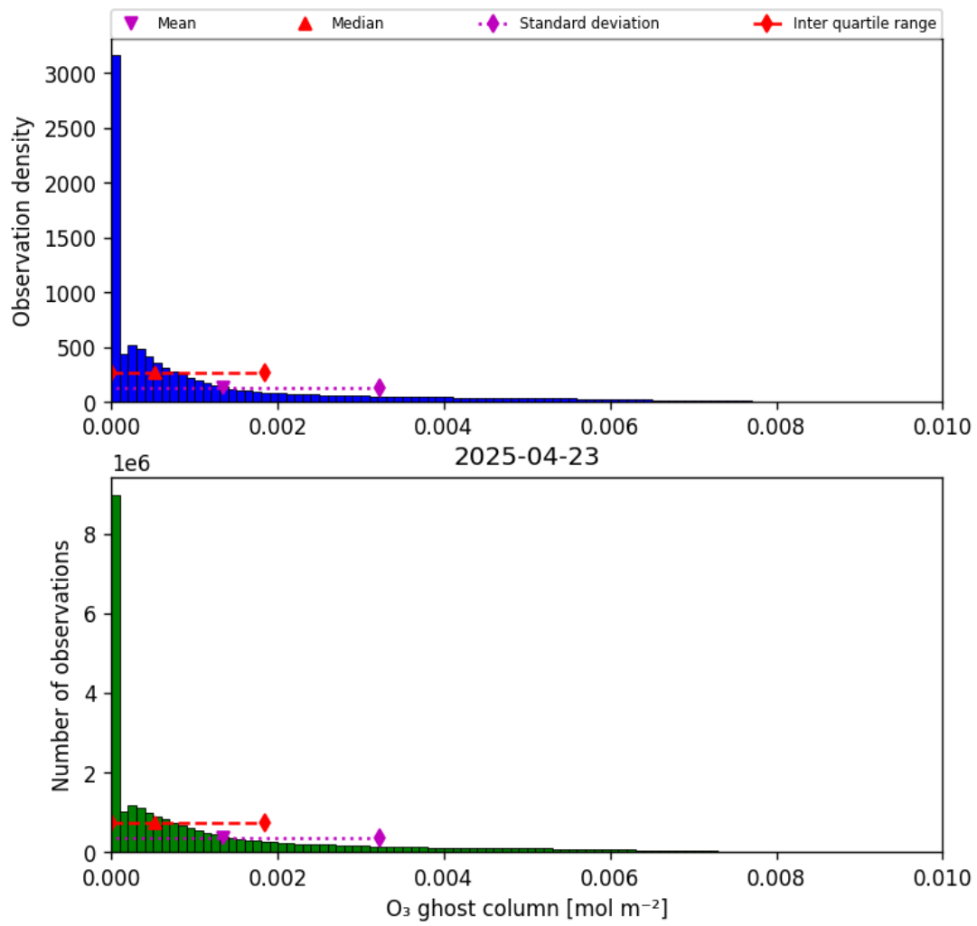
Figure 25: Histogram of “O 3 ghost column” for 2025-04-22 to 2025-04-24
