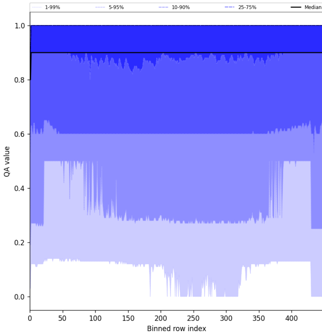
Figure 27: Along track statistics of “QA value” for 2025-04-22 to 2025-04-24
