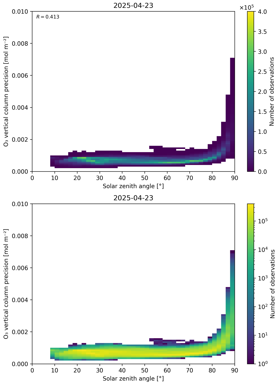
Figure 48: Scatter density plot of “Solar zenith angle” against “O 3 vertical column precision” for 2025-04-22 to 2025-04-24.
