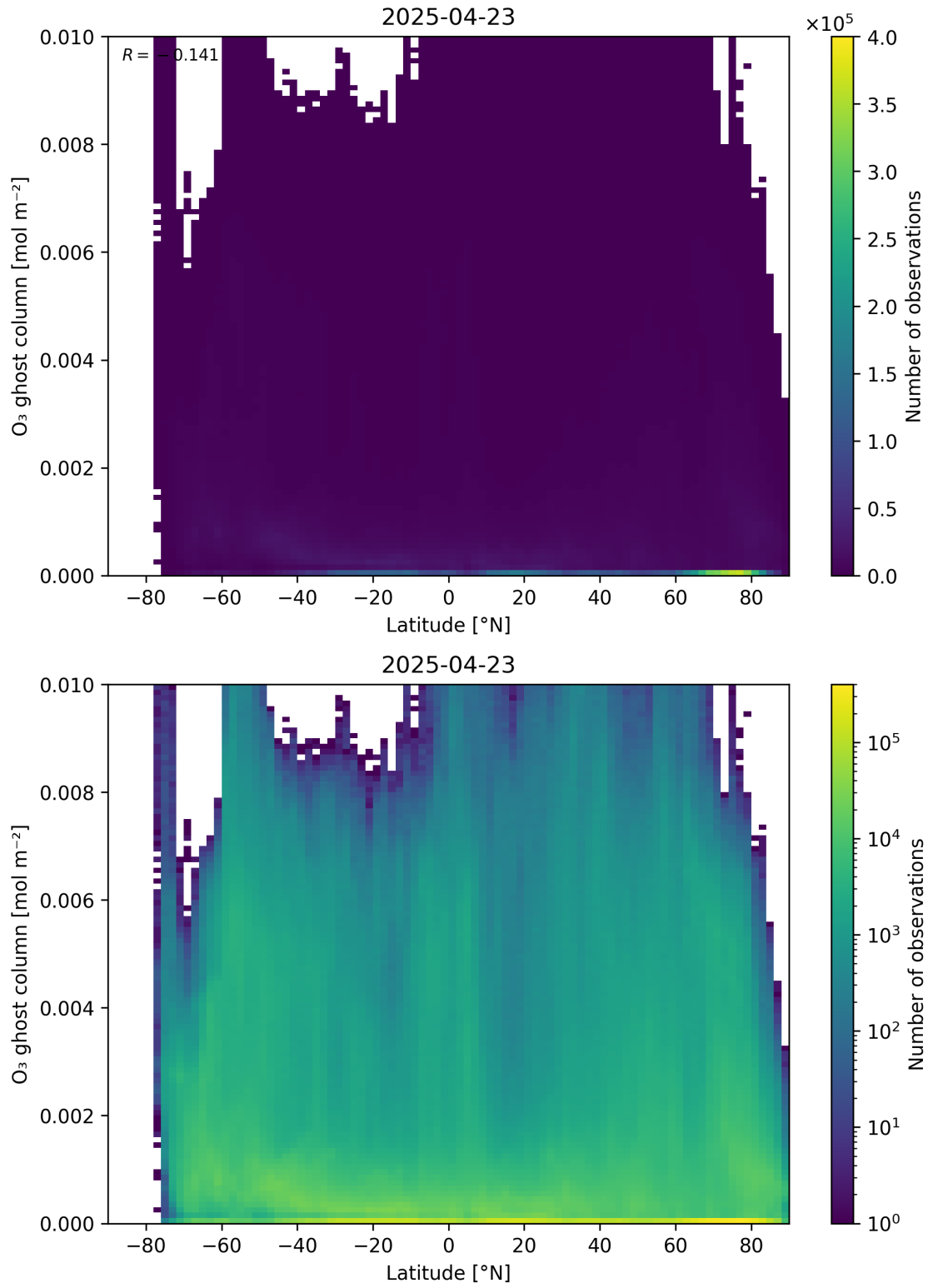
Figure 35: Scatter density plot of “Latitude” against “O 3 ghost column” for 2025-04-22 to 2025-04-24.
