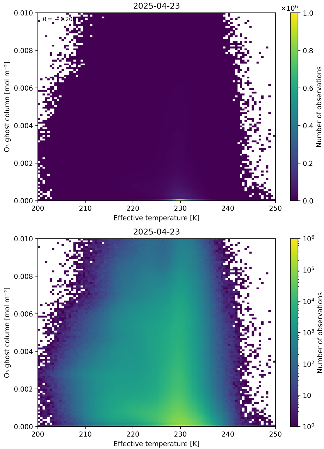
Figure 38: Scatter density plot of “Effective temperature” against “O 3 ghost column” for 2025-04-22 to 2025-04-24.
