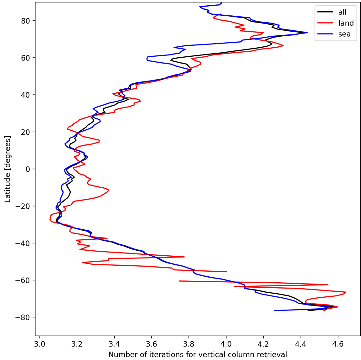
Figure 19: Zonal average of “Number of iterations for vertical column retrieval” for 2025-04-22 to 2025-04-24.
