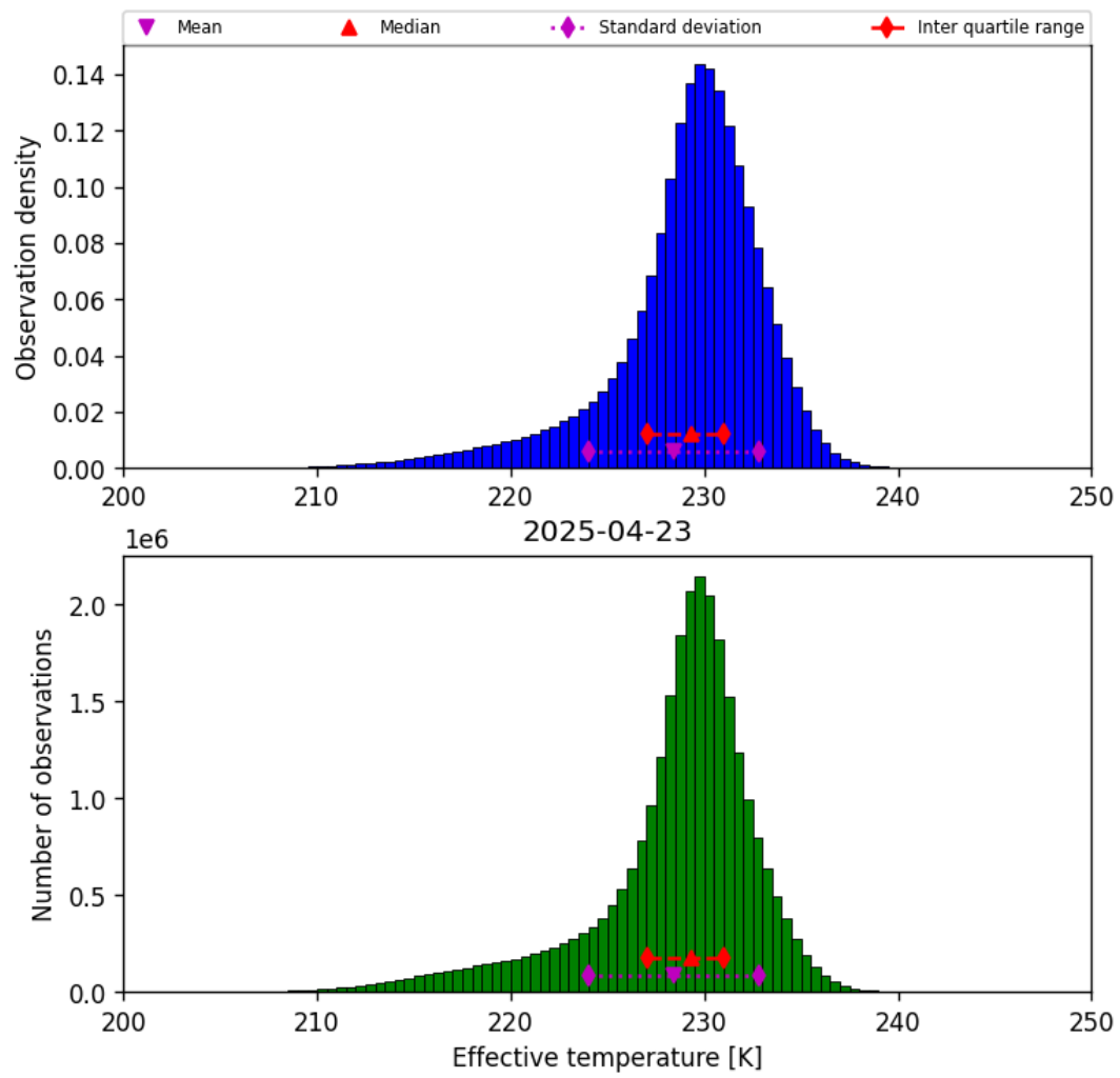
Figure 24: Histogram of “Effective temperature” for 2025-04-22 to 2025-04-24
