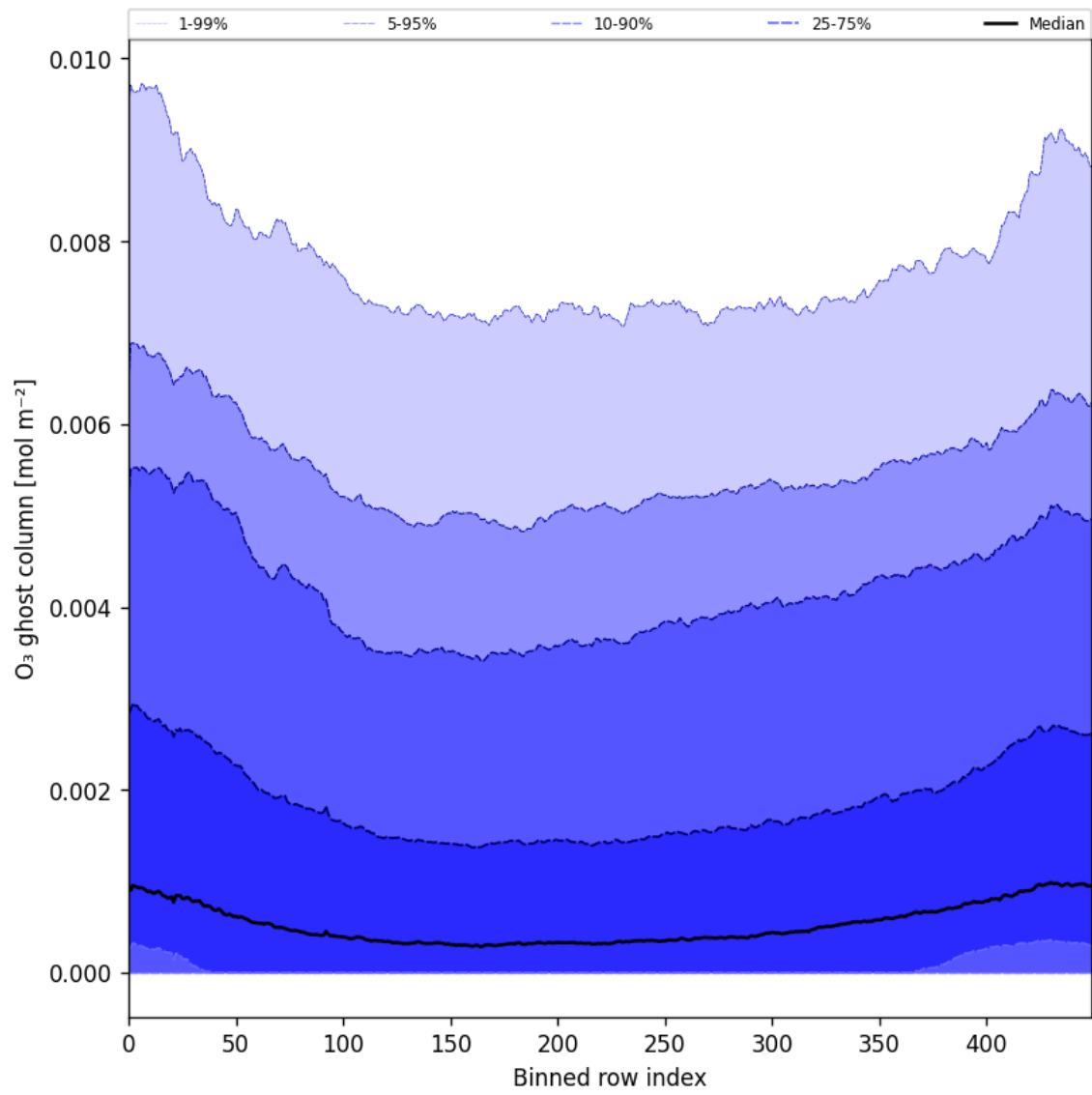
Figure 32: Along track statistics of “O 3 ghost column” for 2025-04-22 to 2025-04-24
