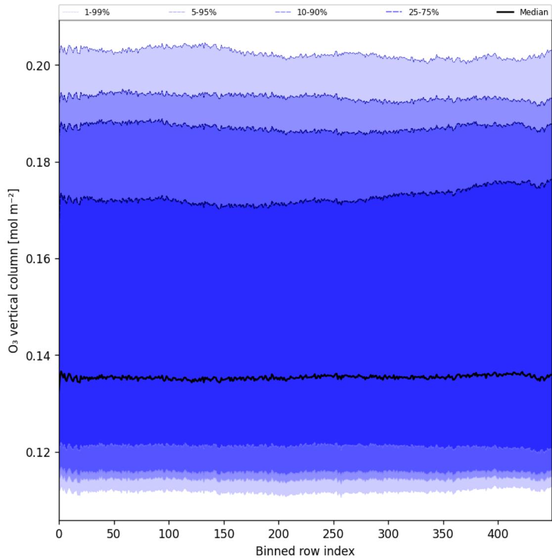
Figure 28: Along track statistics of “O 3 vertical column” for 2025-04-22 to 2025-04-24
