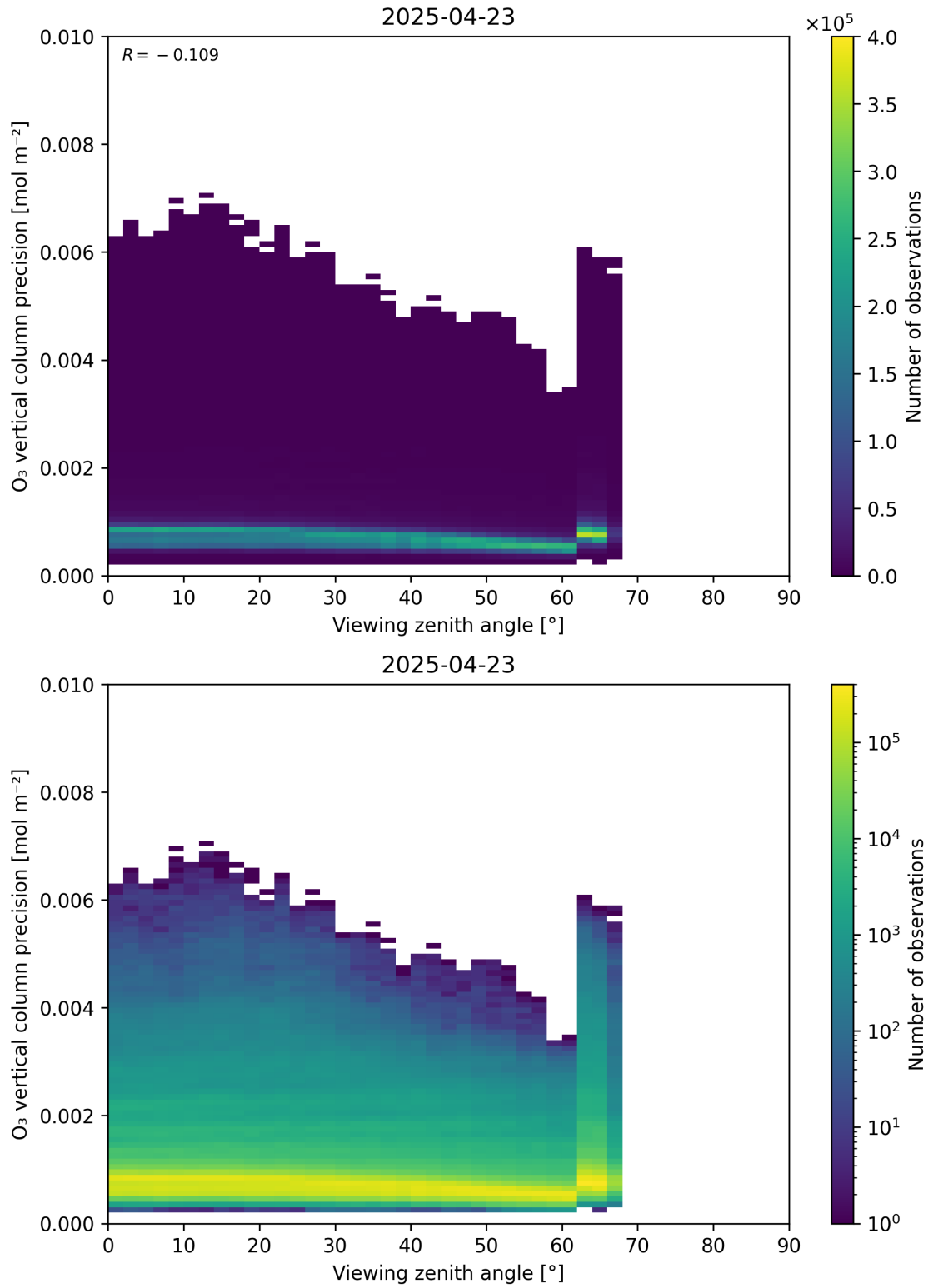
Figure 53: Scatter density plot of “Viewing zenith angle” against “O 3 vertical column precision” for 2025-04-22 to 2025-04-24.
