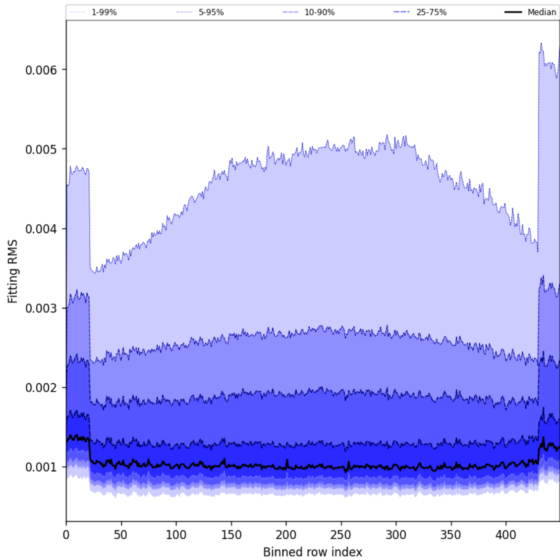
Figure 30: Along track statistics of “Fitting RMS” for 2025-04-22 to 2025-04-24
