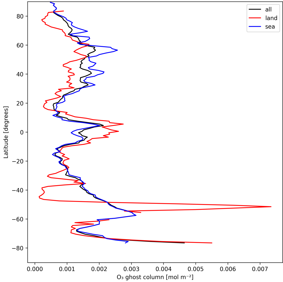
Figure 18: Zonal average of “O 3 ghost column” for 2025-04-22 to 2025-04-24.
