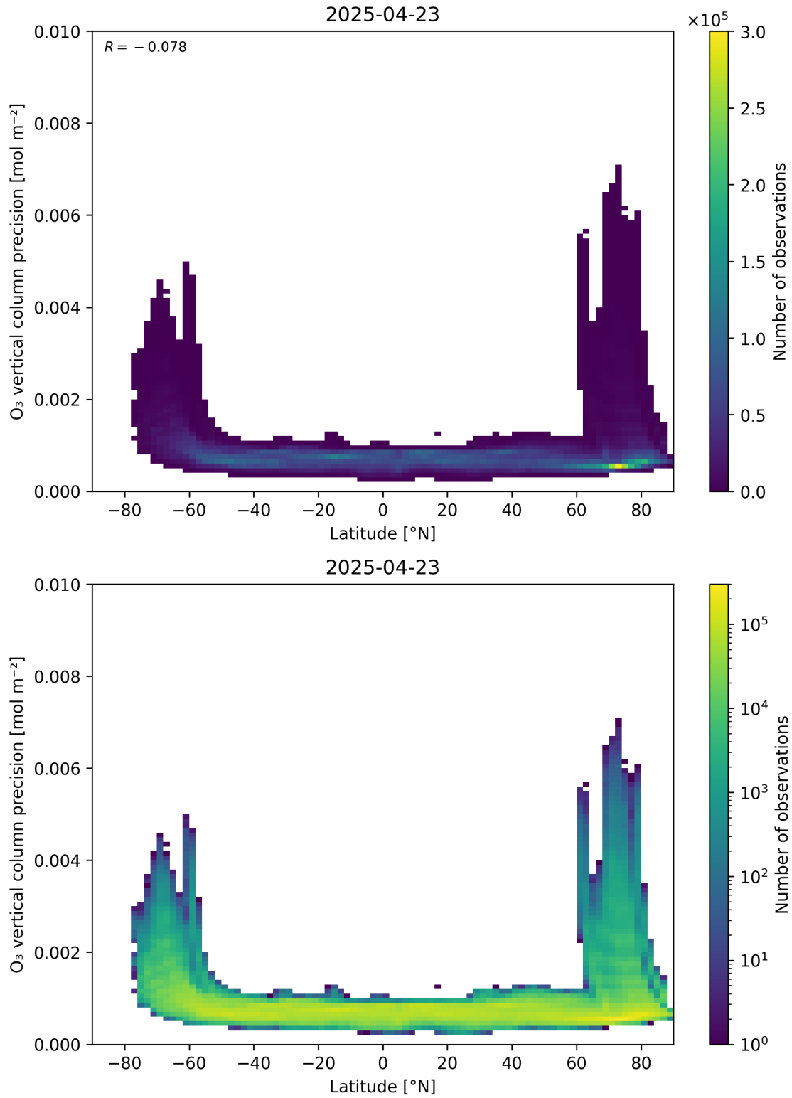
Figure 37: Scatter density plot of “Latitude” against “O 3 vertical column precision” for 2025-04-22 to 2025-04-24.
