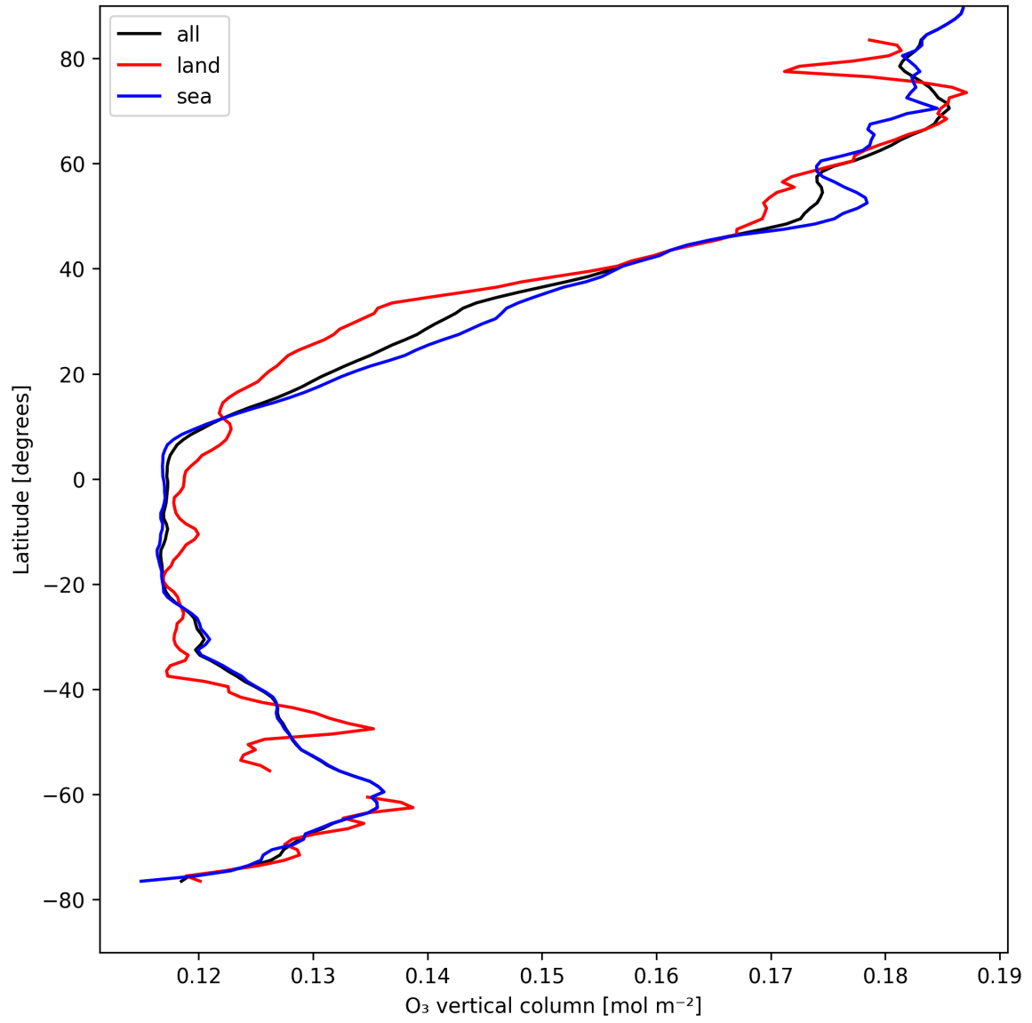
Figure 14: Zonal average of “O 3 vertical column” for 2025-04-22 to 2025-04-24.
