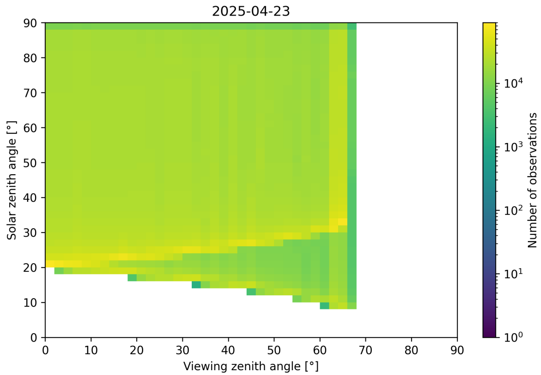
Figure 54: Scatter density plot of “Viewing zenith angle” against “Solar zenith angle” for 2025-04-22 to 2025-04-24.
