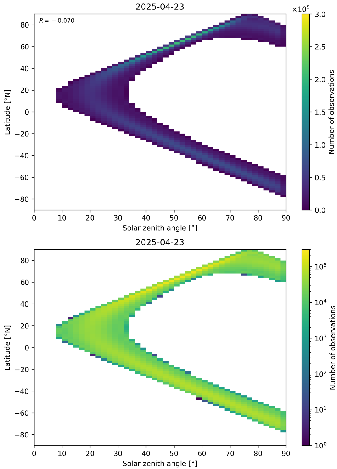
Figure 44: Scatter density plot of “Solar zenith angle” against “Latitude” for 2025-04-22 to 2025-04-24.
