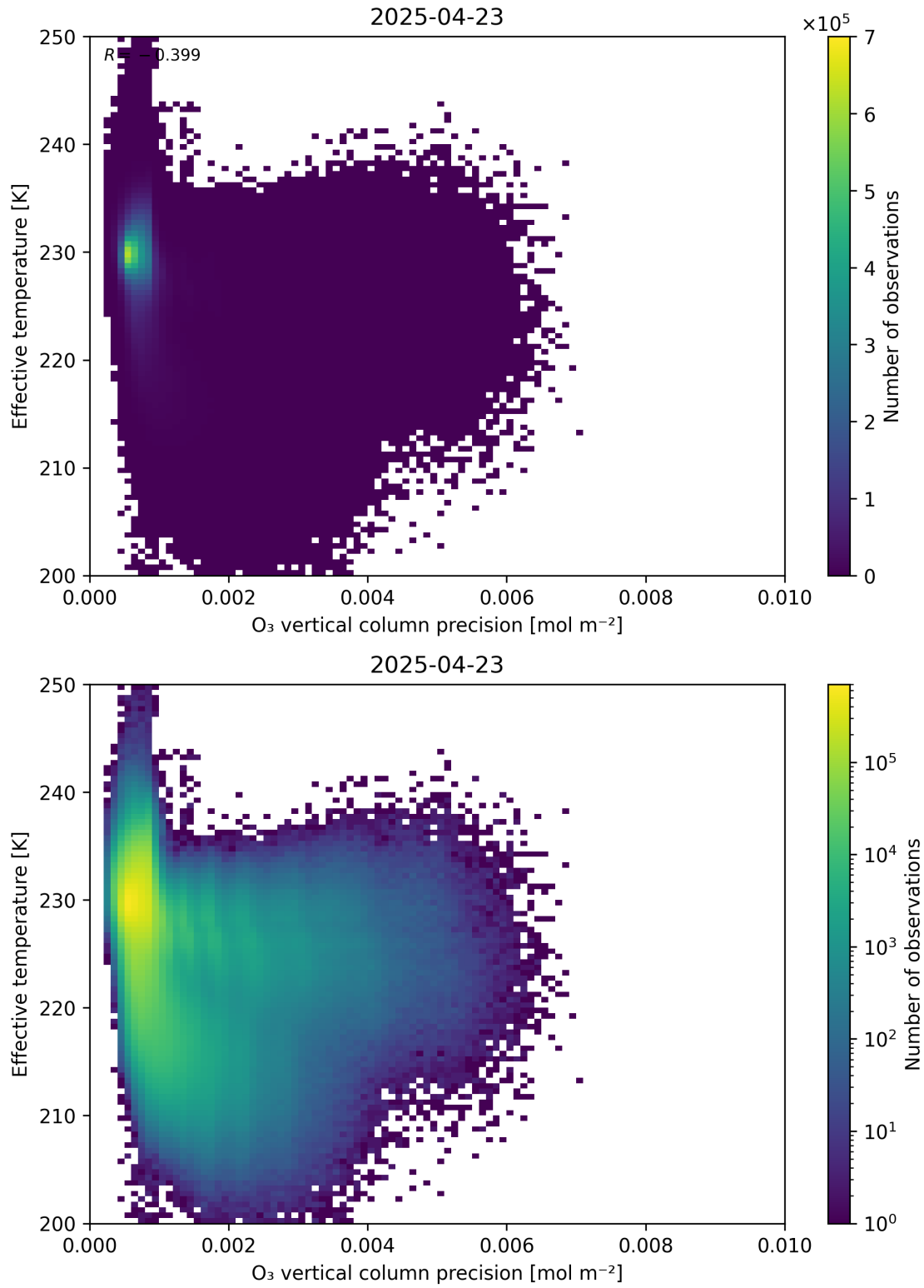
Figure 42: Scatter density plot of “O 3 vertical column precision” against “Effective temperature” for 2025-04-22 to 2025-04-24.
