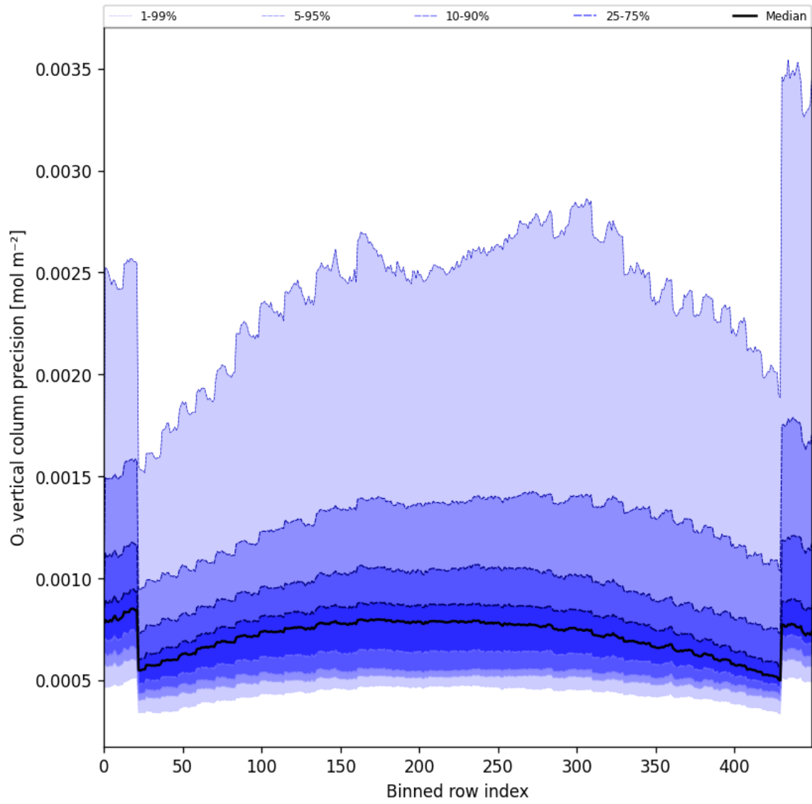
Figure 29: Along track statistics of “O 3 vertical column precision” for 2025-04-22 to 2025-04-24
