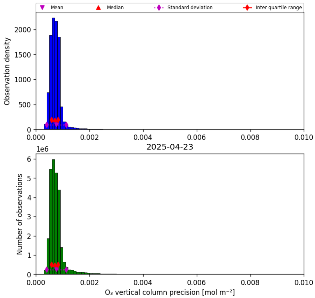
Figure 22: Histogram of “O 3 vertical column precision” for 2025-04-22 to 2025-04-24
