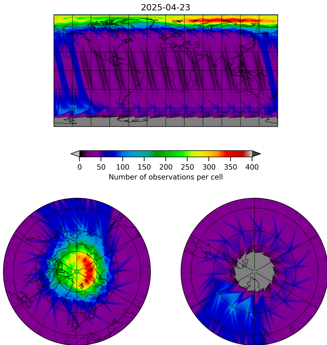
Figure 12: Map of the number of observations for 2025-04-22 to 2025-04-24
