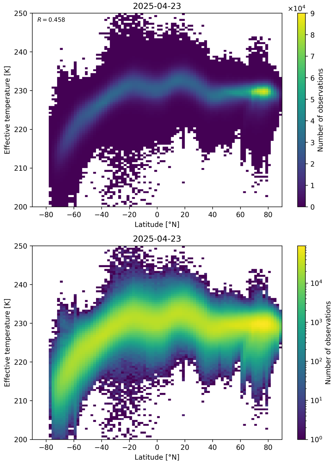
Figure 34: Scatter density plot of “Latitude” against “Effective temperature” for 2025-04-22 to 2025-04-24.
