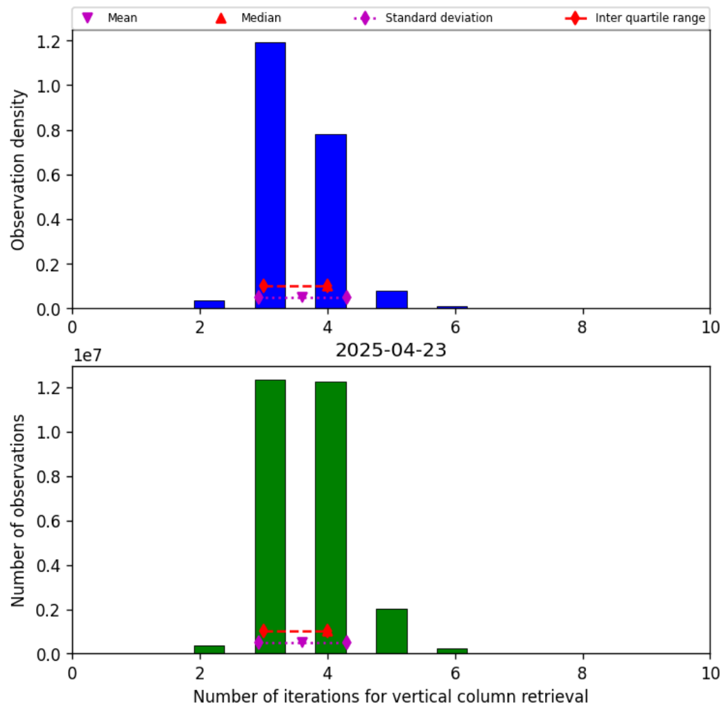
Figure 26: Histogram of “Number of iterations for vertical column retrieval” for 2025-04-22 to 2025-04-24
