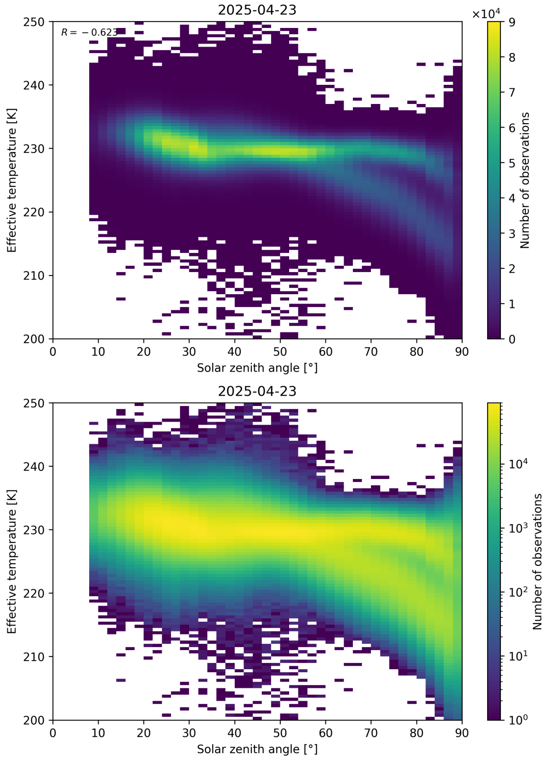
Figure 45: Scatter density plot of “Solar zenith angle” against “Effective temperature” for 2025-04-22 to 2025-04-24.
