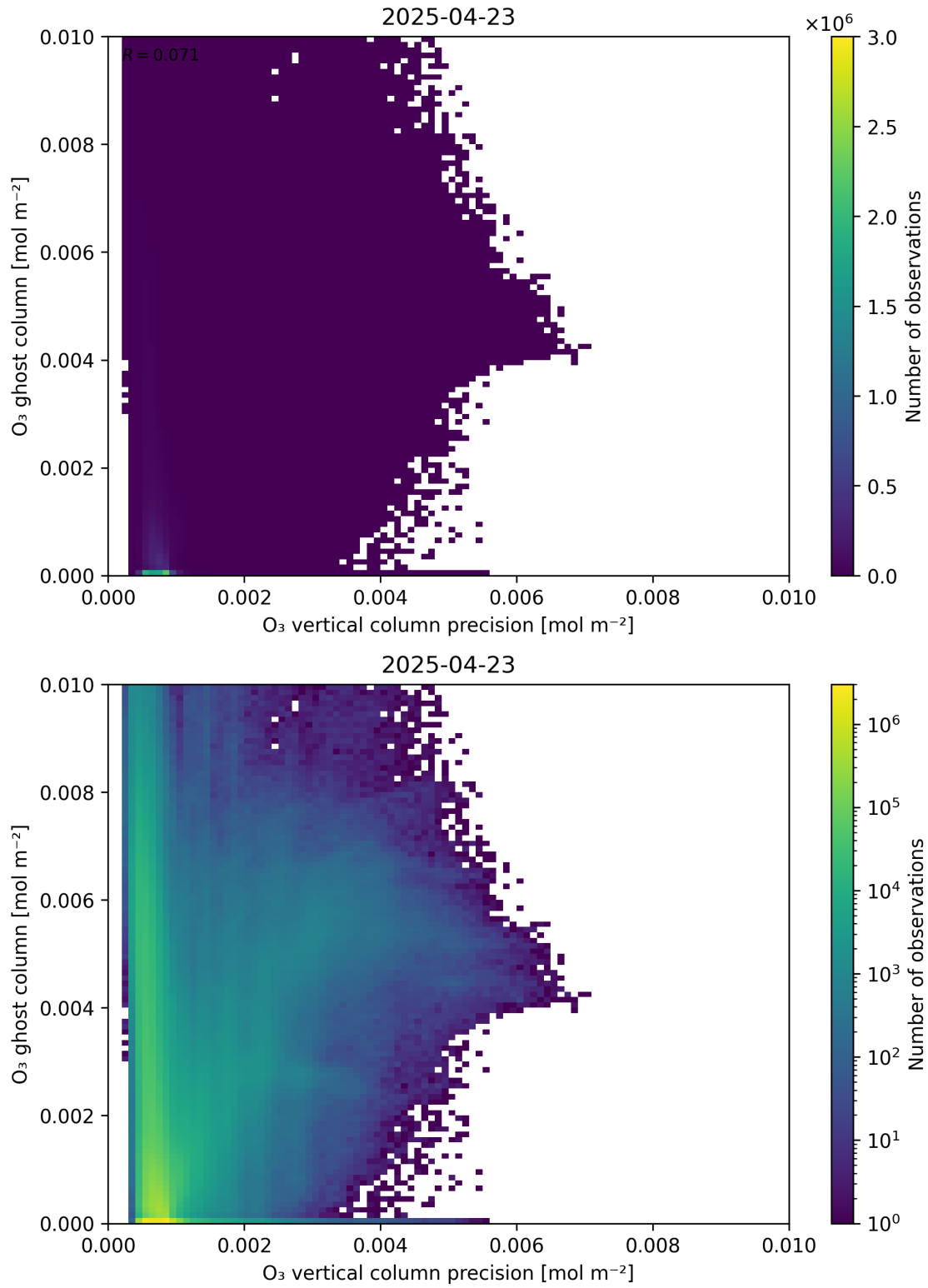
Figure 43: Scatter density plot of “ \text{O}_3 vertical column precision” against “ \text{O}_3 ghost column” for 2025-04-22 to 2025-04-24.
