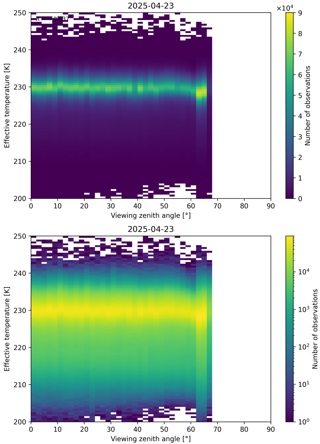
Figure 50: Scatter density plot of “Viewing zenith angle” against “Effective temperature” for 2025-04-22 to 2025-04-24.
