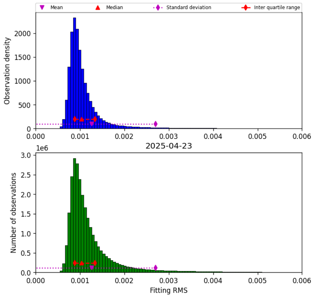
Figure 23: Histogram of “Fitting RMS” for 2025-04-22 to 2025-04-24
