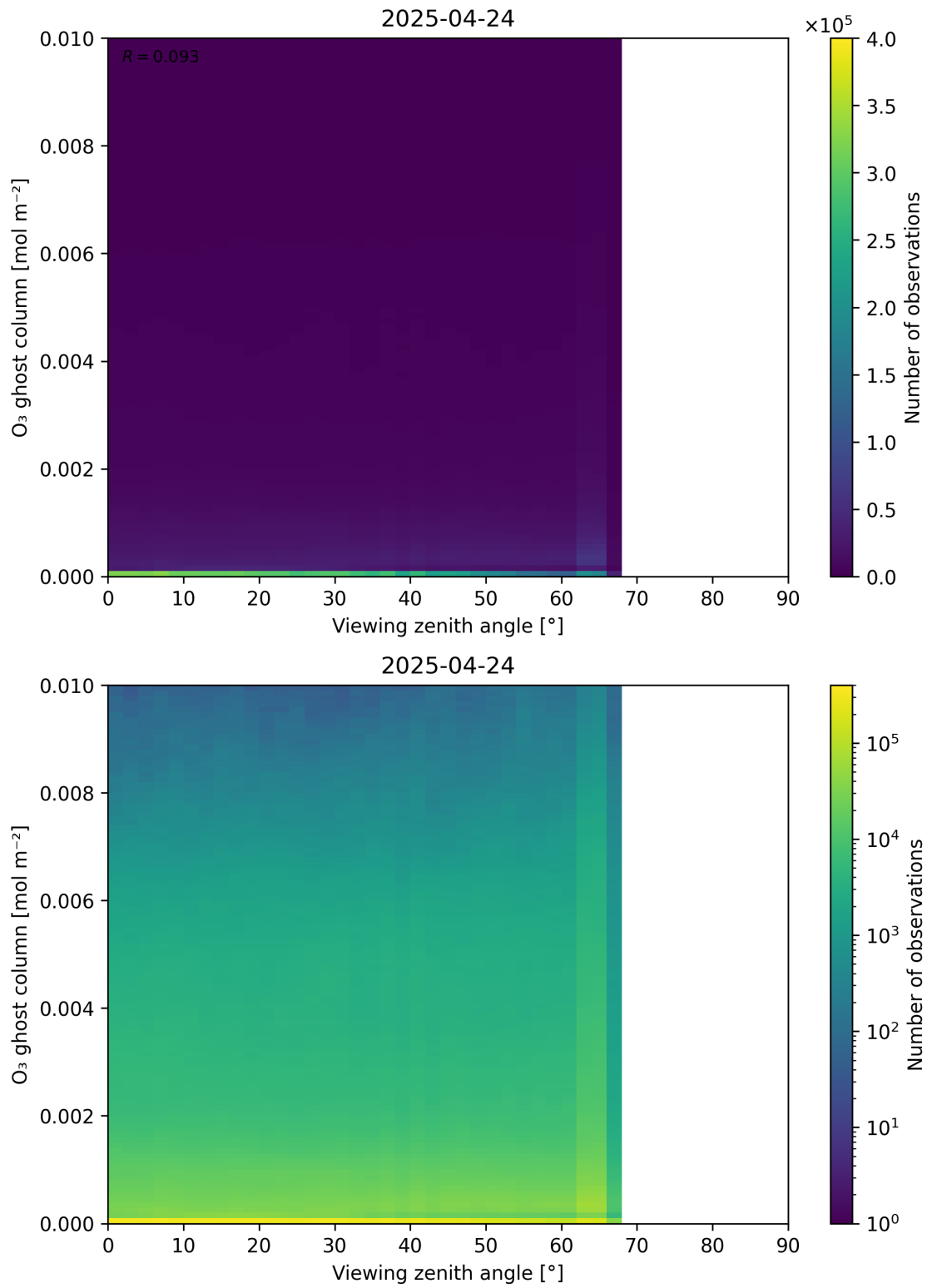
Figure 51: Scatter density plot of “Viewing zenith angle” against “O 3 ghost column” for 2025-04-24 to 2025-04-25.
