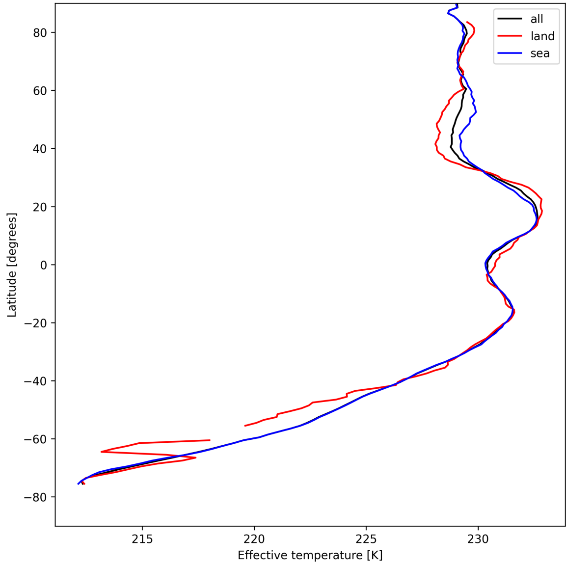
Figure 17: Zonal average of "Effective temperature" for 2025-04-24 to 2025-04-25.
