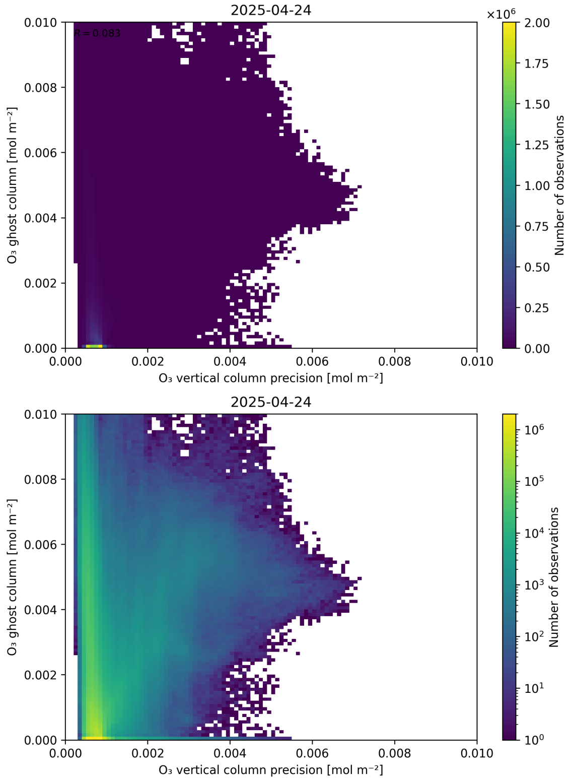
Figure 43: Scatter density plot of “ O_3 vertical column precision” against “ O_3 ghost column” for 2025-04-24 to 2025-04-25.
