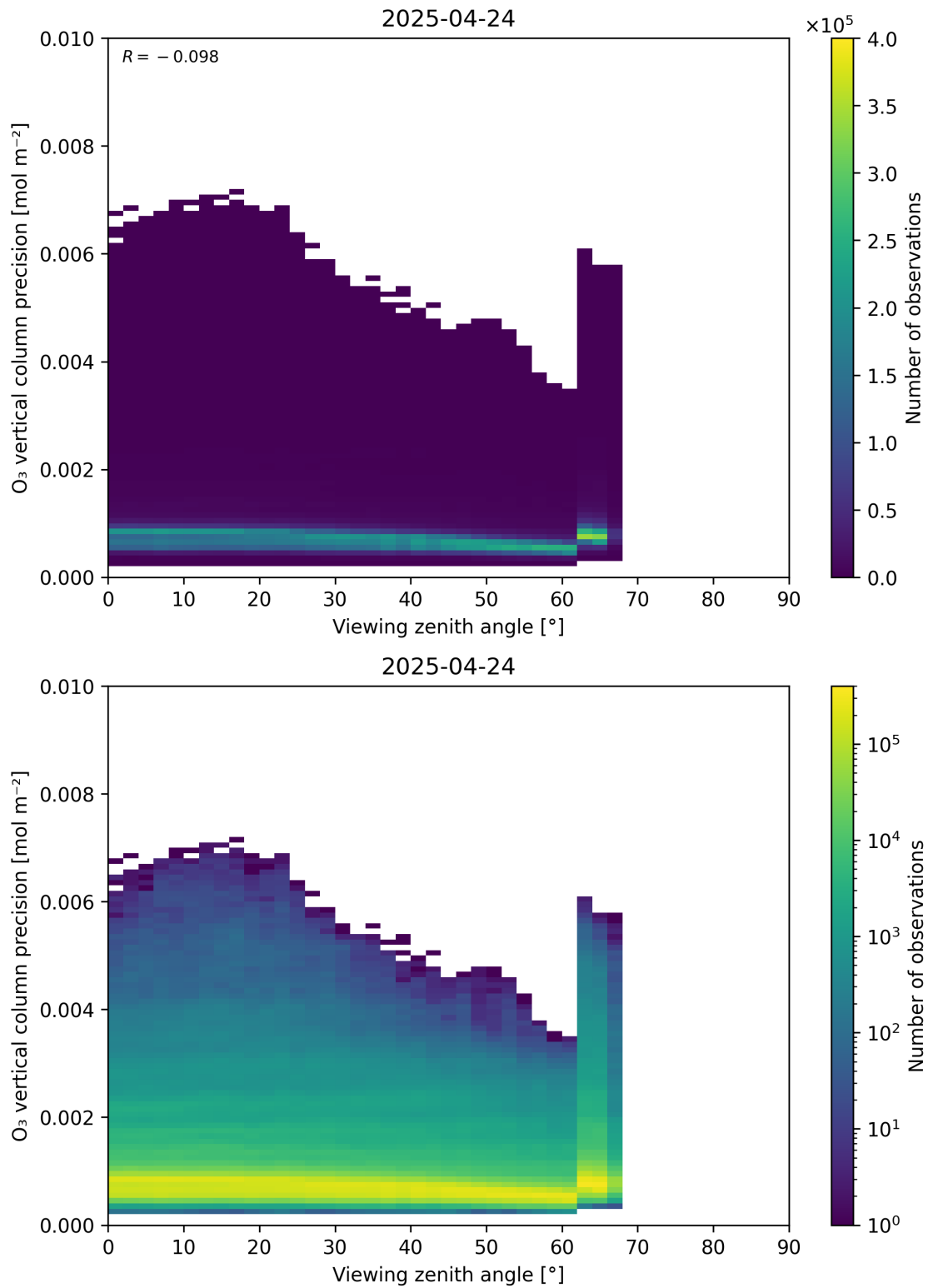
Figure 53: Scatter density plot of “Viewing zenith angle” against “O 3 vertical column precision” for 2025-04-24 to 2025-04-25.
