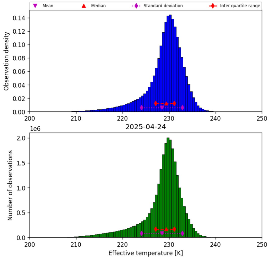
Figure 24: Histogram of “Effective temperature” for 2025-04-24 to 2025-04-25
