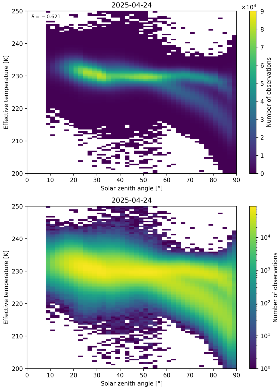
Figure 45: Scatter density plot of “Solar zenith angle” against “Effective temperature” for 2025-04-24 to 2025-04-25.
