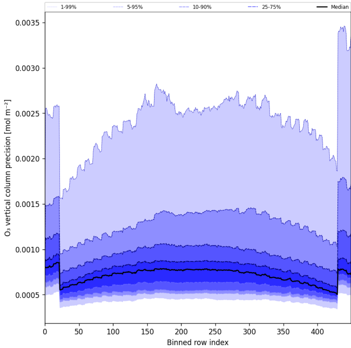
Figure 29: Along track statistics of “O 3 vertical column precision” for 2025-04-24 to 2025-04-25
