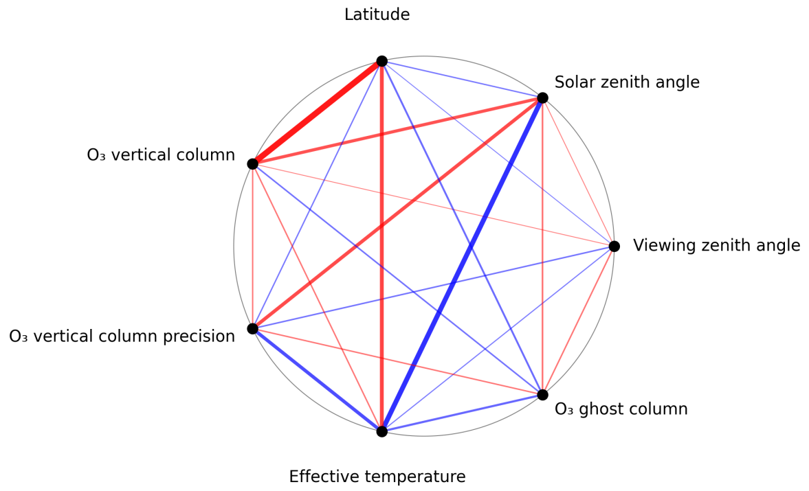
Figure 1: Map of correlation graph for 2025-04-24 to 2025-04-25.
