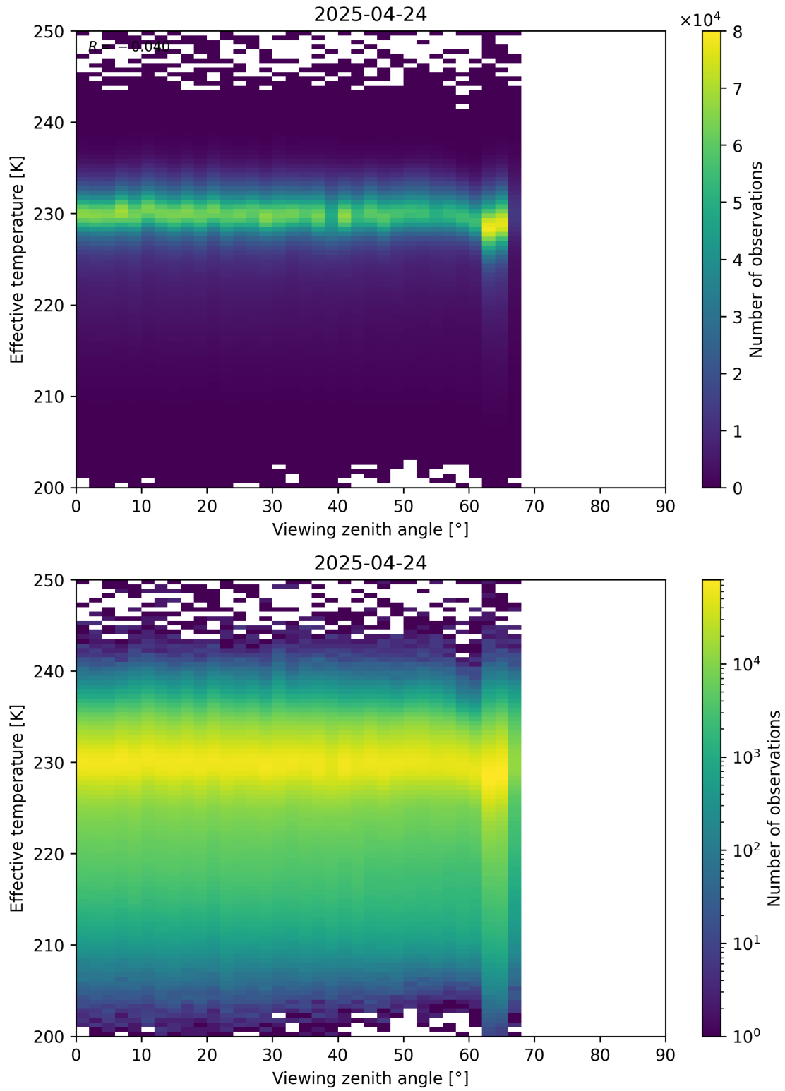
Figure 50: Scatter density plot of “Viewing zenith angle” against “Effective temperature” for 2025-04-24 to 2025-04-25.
