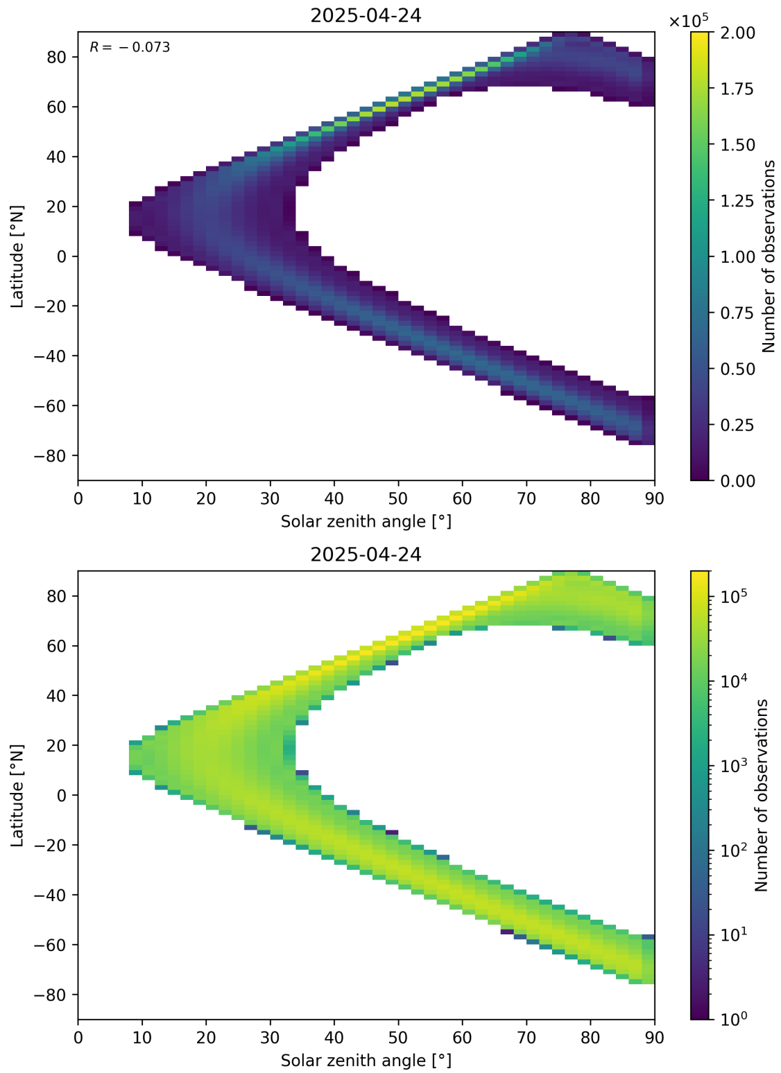
Figure 44: Scatter density plot of “Solar zenith angle” against “Latitude” for 2025-04-24 to 2025-04-25.
