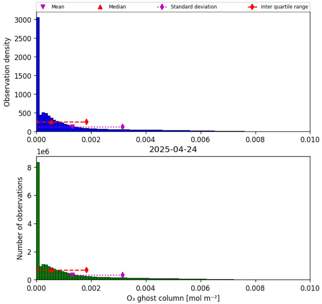
Figure 25: Histogram of “O 3 ghost column” for 2025-04-24 to 2025-04-25
