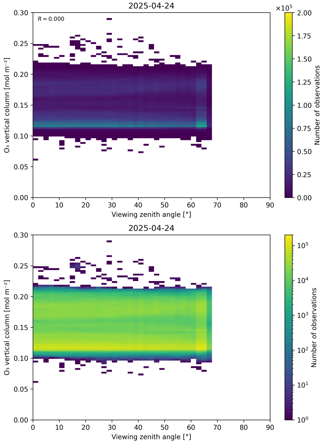
Figure 52: Scatter density plot of “Viewing zenith angle” against “O 3 vertical column” for 2025-04-24 to 2025-04-25.
