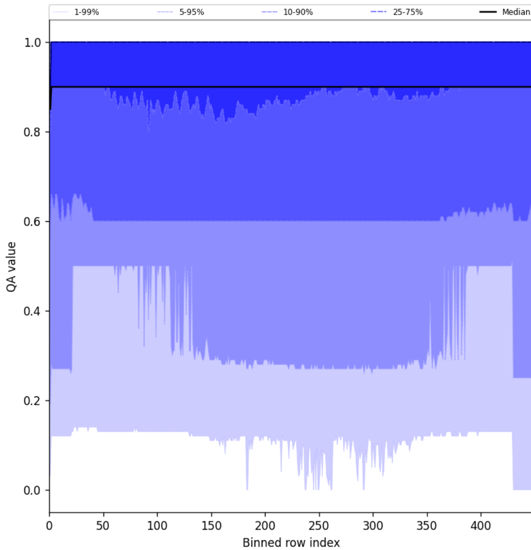
Figure 27: Along track statistics of “QA value” for 2025-04-24 to 2025-04-25
