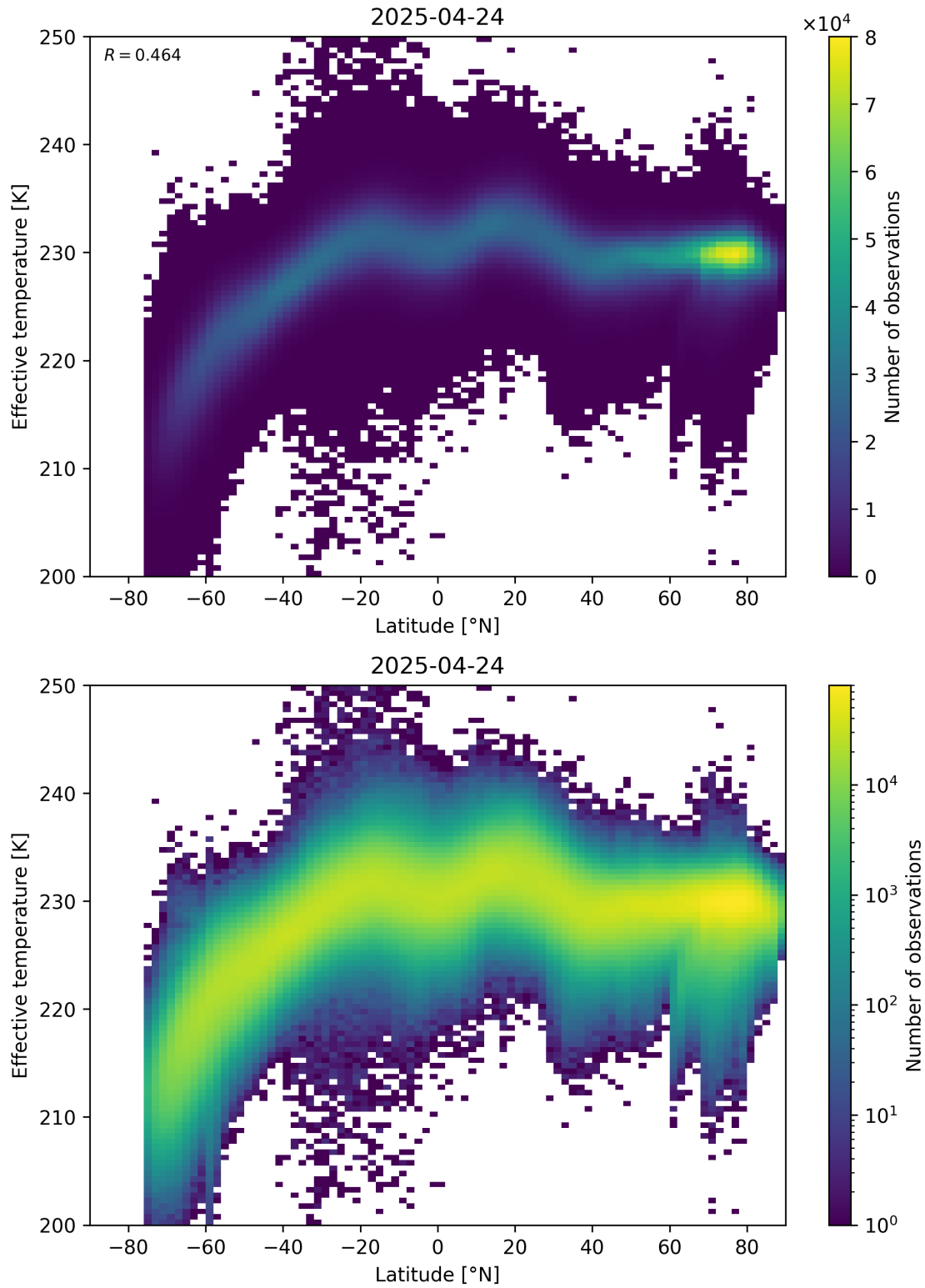
Figure 34: Scatter density plot of “Latitude” against “Effective temperature” for 2025-04-24 to 2025-04-25.
