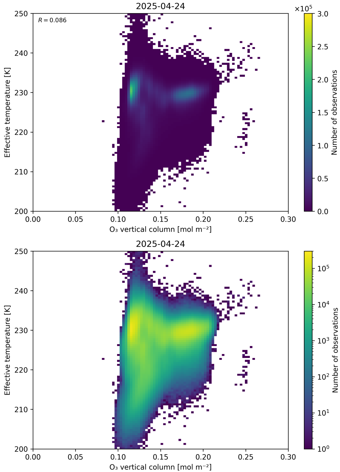
Figure 39: Scatter density plot of “O 3 vertical column” against “Effective temperature” for 2025-04-24 to 2025-04-25.
