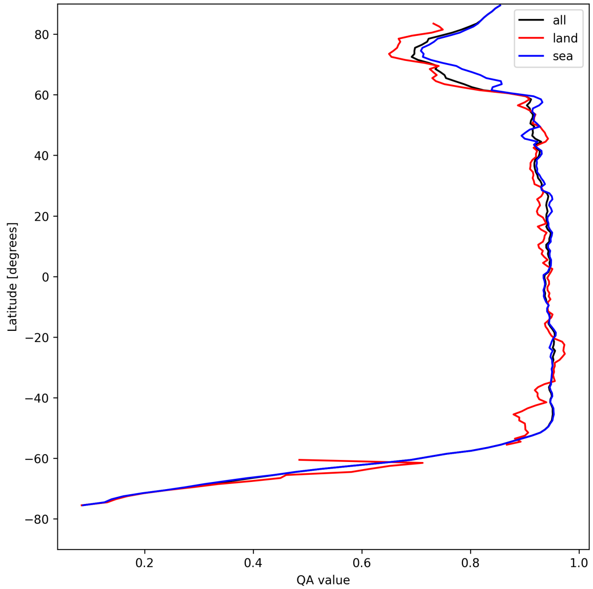
Figure 13: Zonal average of “QA value” for 2025-04-24 to 2025-04-25.
