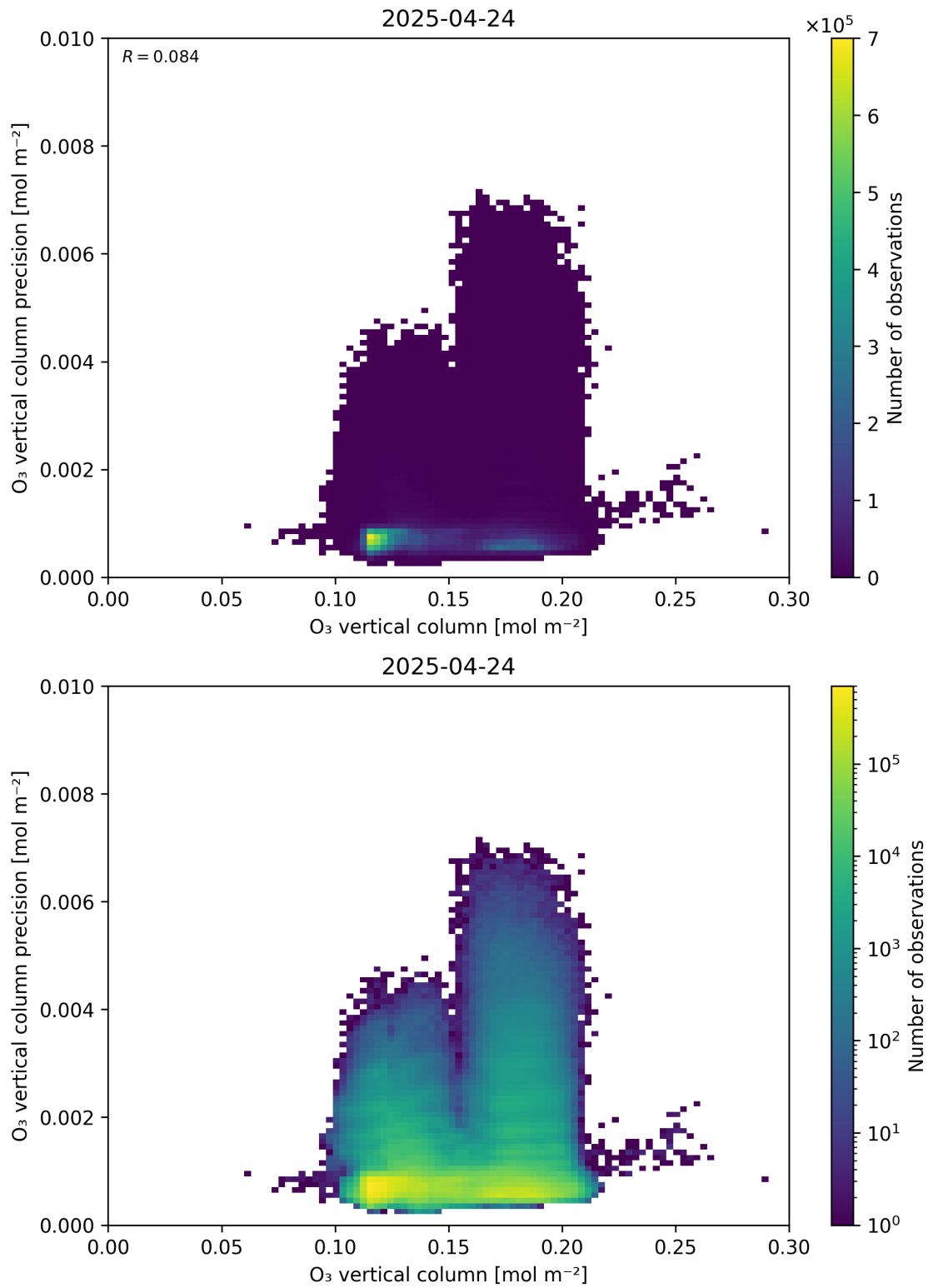
Figure 41: Scatter density plot of “O 3 vertical column” against “O 3 vertical column precision” for 2025-04-24 to 2025-04-25.
