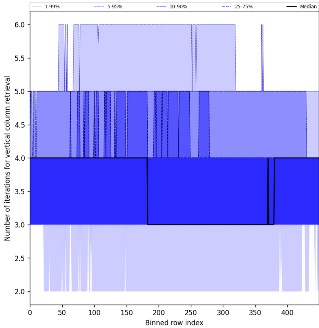
Figure 33: Along track statistics of “Number of iterations for vertical column retrieval” for 2025-04-24 to 2025-04-25
