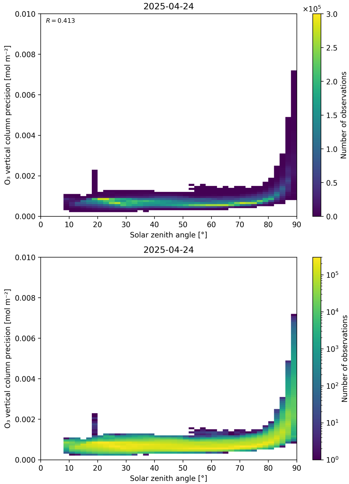
Figure 48: Scatter density plot of “Solar zenith angle” against “O 3 vertical column precision” for 2025-04-24 to 2025-04-25.
