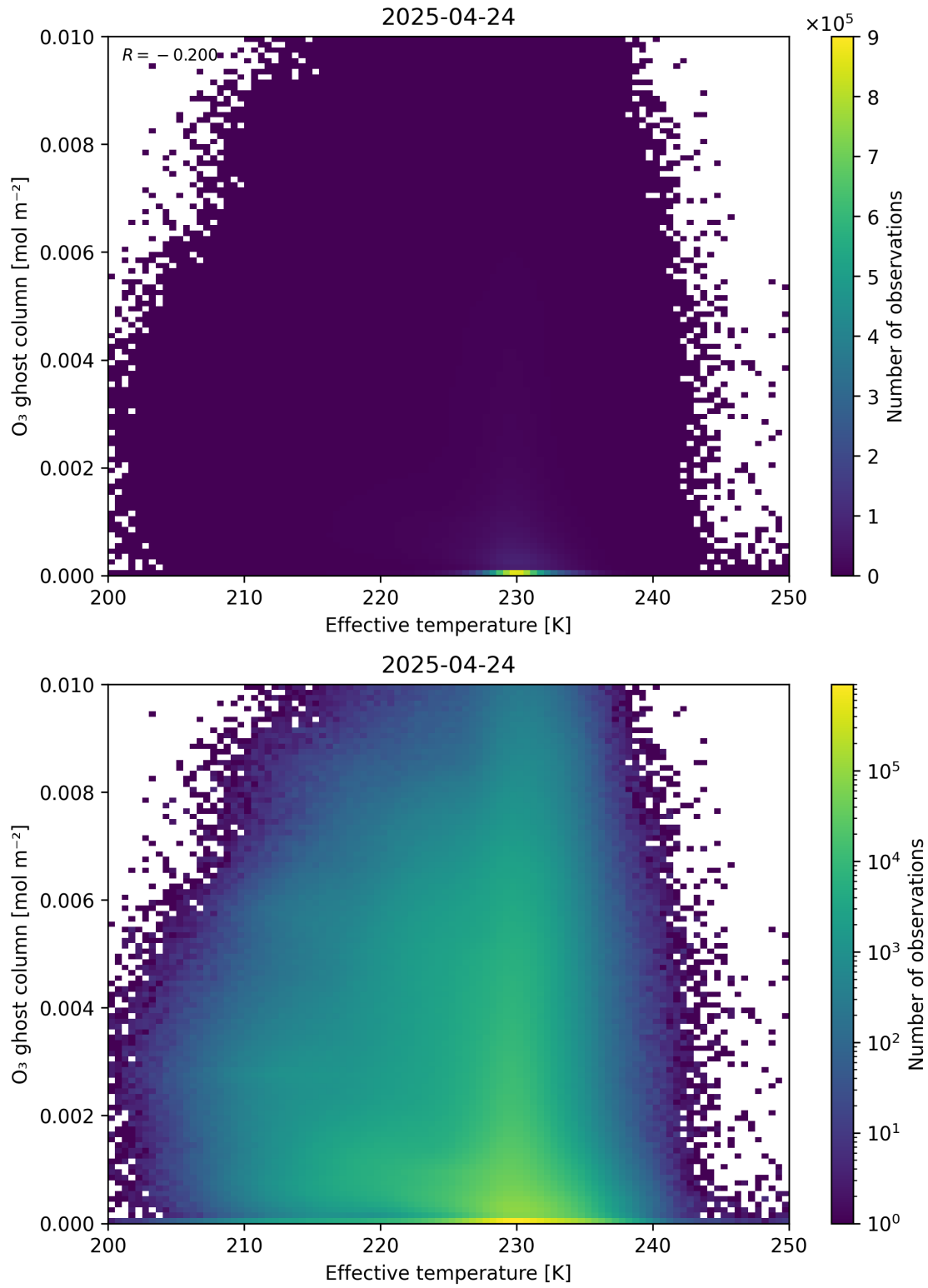
Figure 38: Scatter density plot of “Effective temperature” against “O 3 ghost column” for 2025-04-24 to 2025-04-25.
