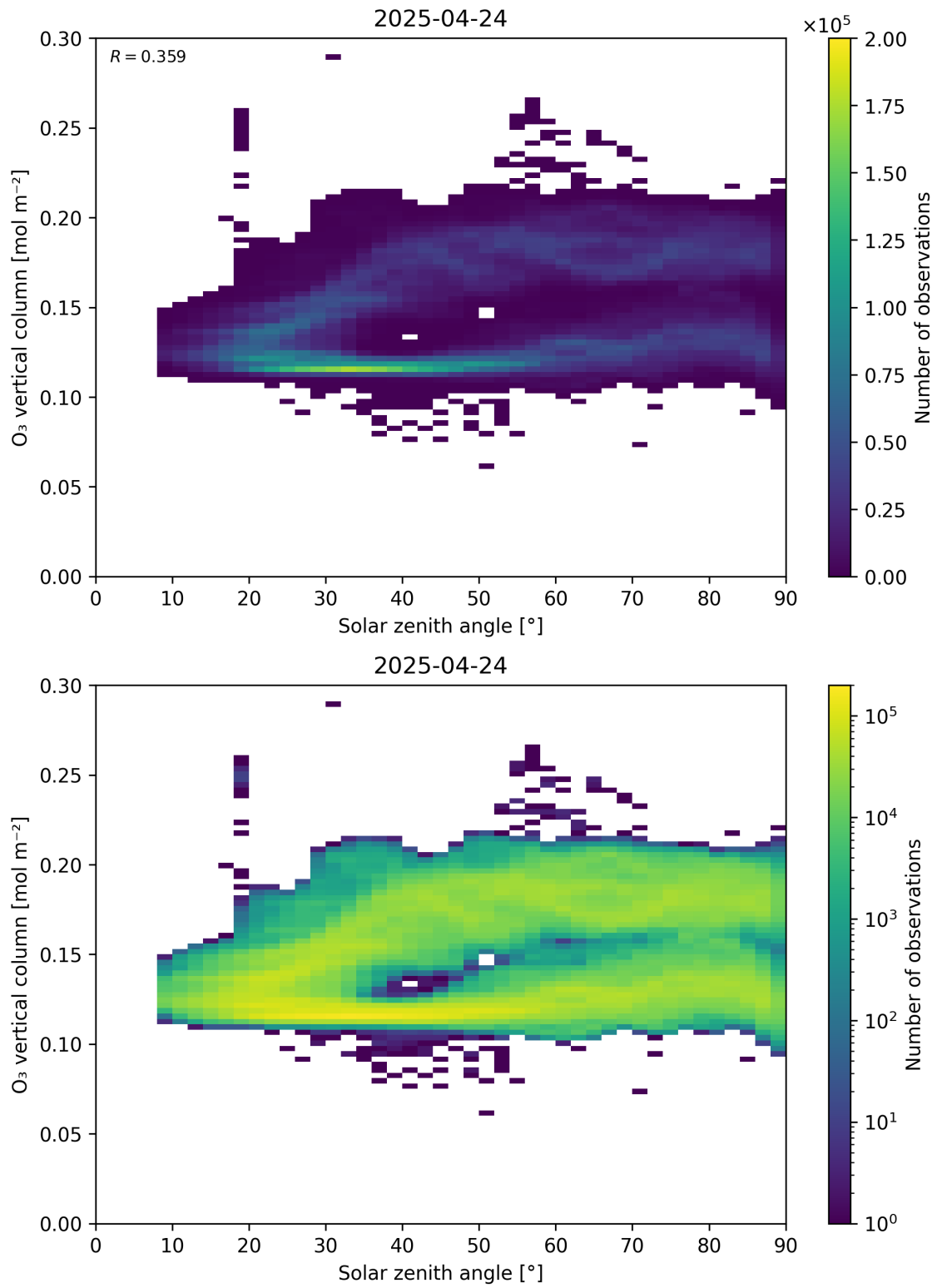
Figure 47: Scatter density plot of “Solar zenith angle” against “O 3 vertical column” for 2025-04-24 to 2025-04-25.
