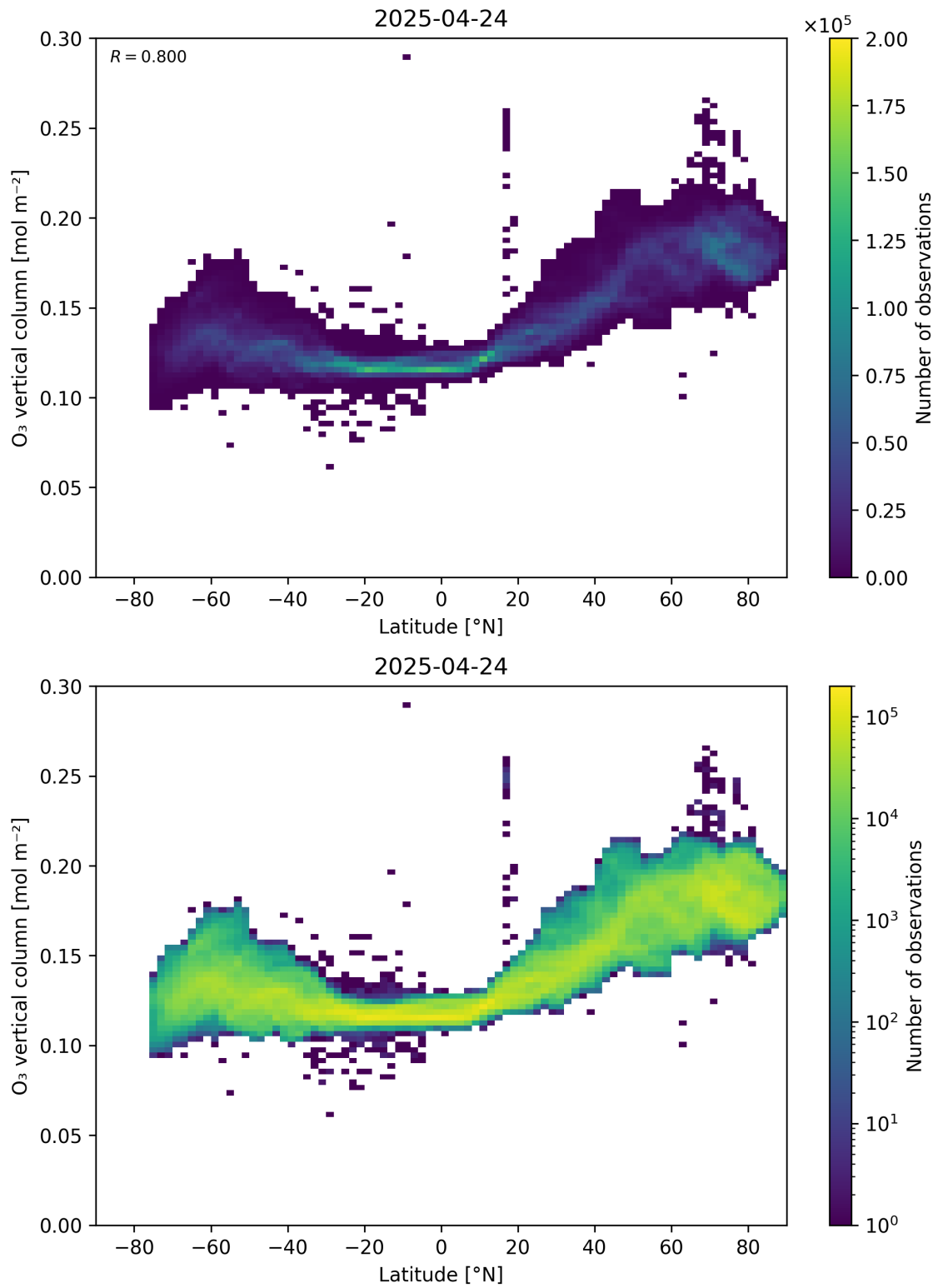
Figure 36: Scatter density plot of “Latitude” against “O 3 vertical column” for 2025-04-24 to 2025-04-25.
