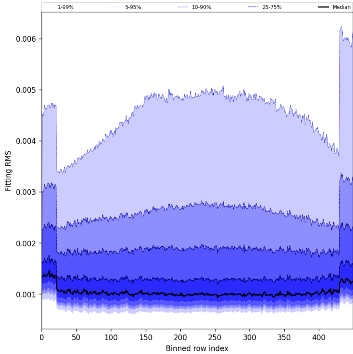
Figure 30: Along track statistics of “Fitting RMS” for 2025-04-24 to 2025-04-25
