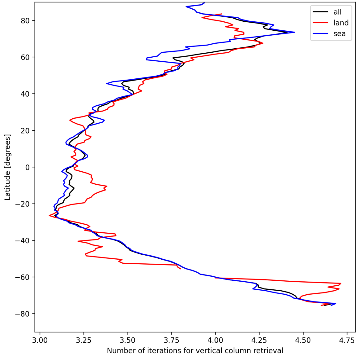
Figure 19: Zonal average of “Number of iterations for vertical column retrieval” for 2025-04-24 to 2025-04-25.
