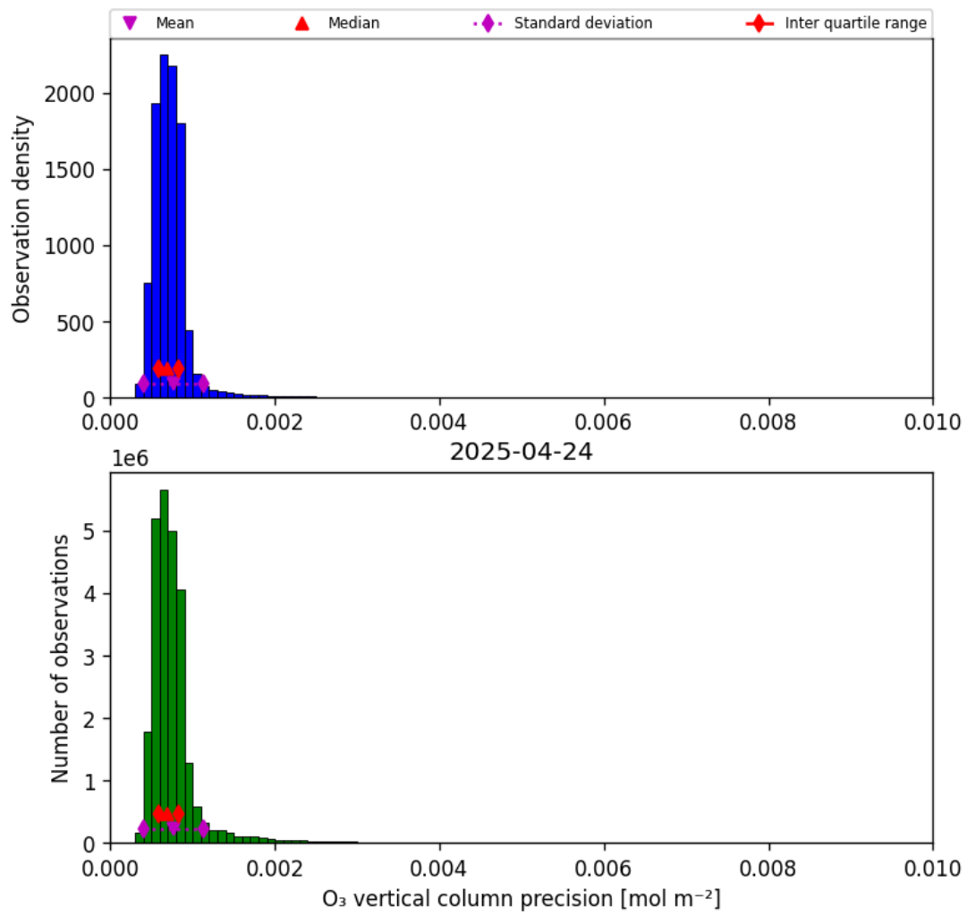
Figure 22: Histogram of “O 3 vertical column precision” for 2025-04-24 to 2025-04-25
