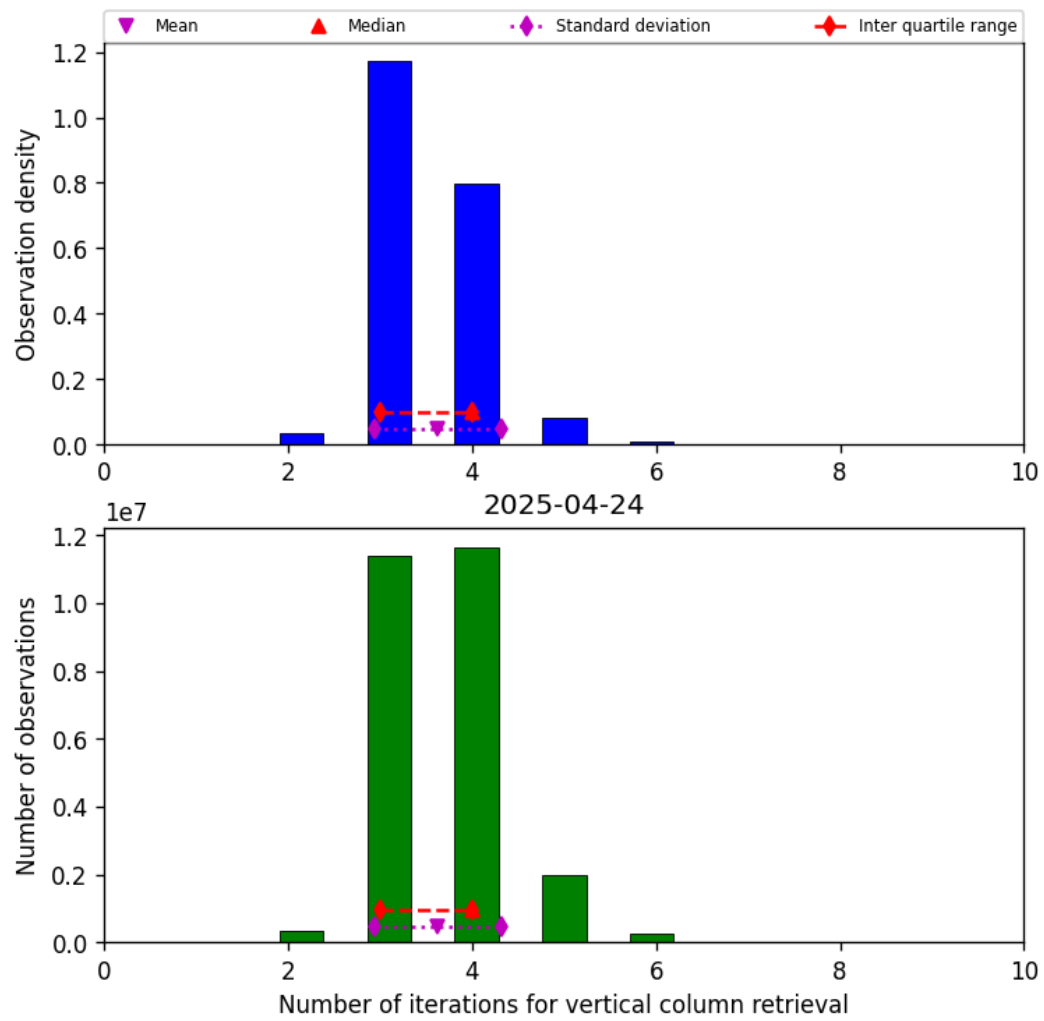
Figure 26: Histogram of “Number of iterations for vertical column retrieval” for 2025-04-24 to 2025-04-25
