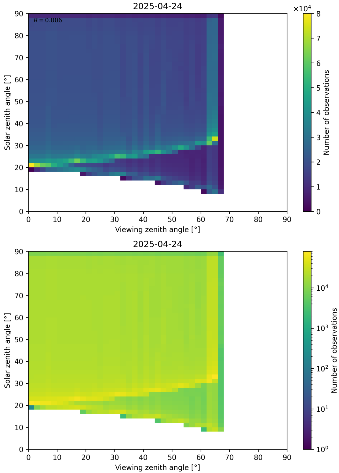
Figure 54: Scatter density plot of “Viewing zenith angle” against “Solar zenith angle” for 2025-04-24 to 2025-04-25.
