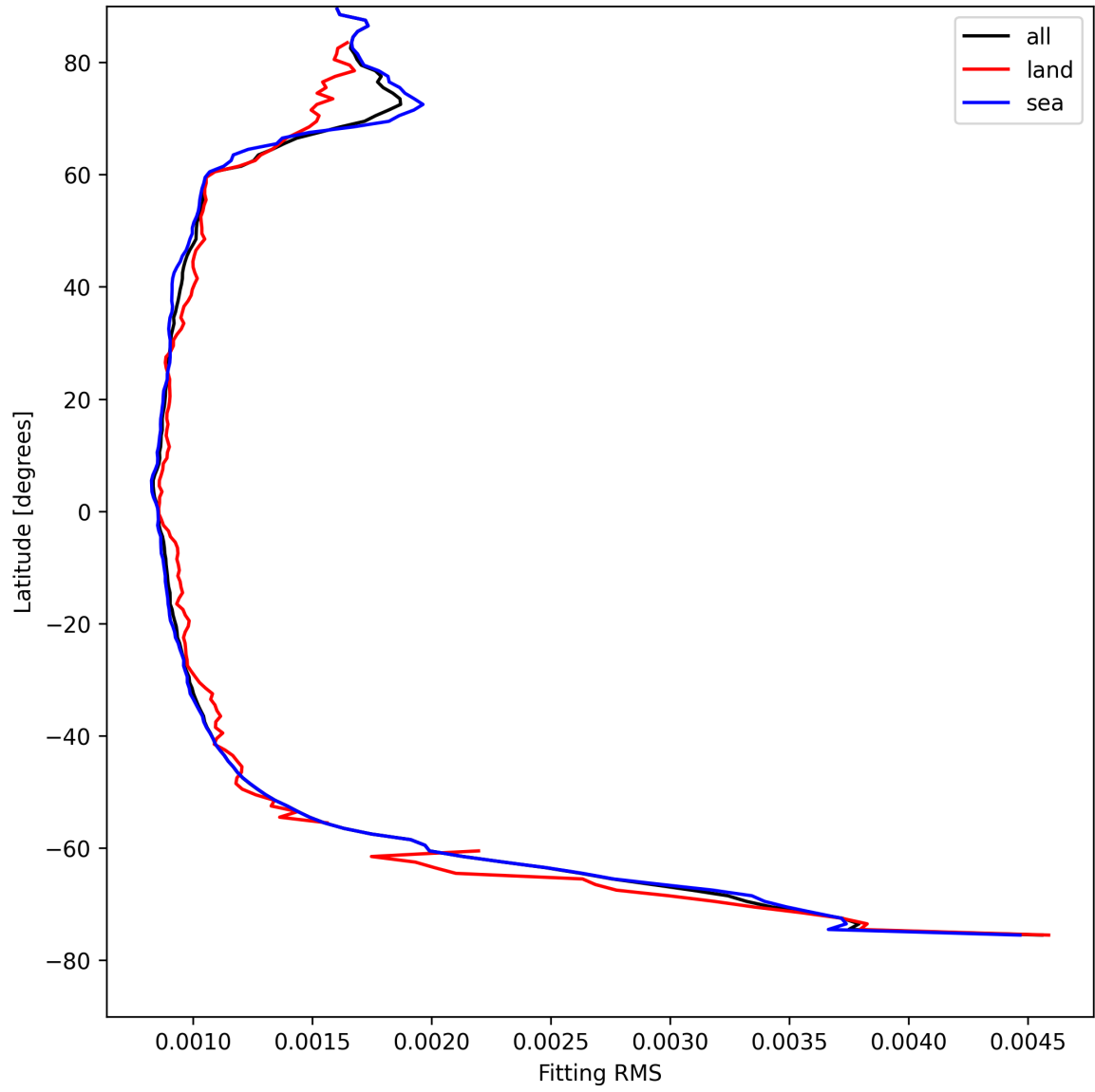
Figure 16: Zonal average of “Fitting RMS” for 2025-04-24 to 2025-04-25.
