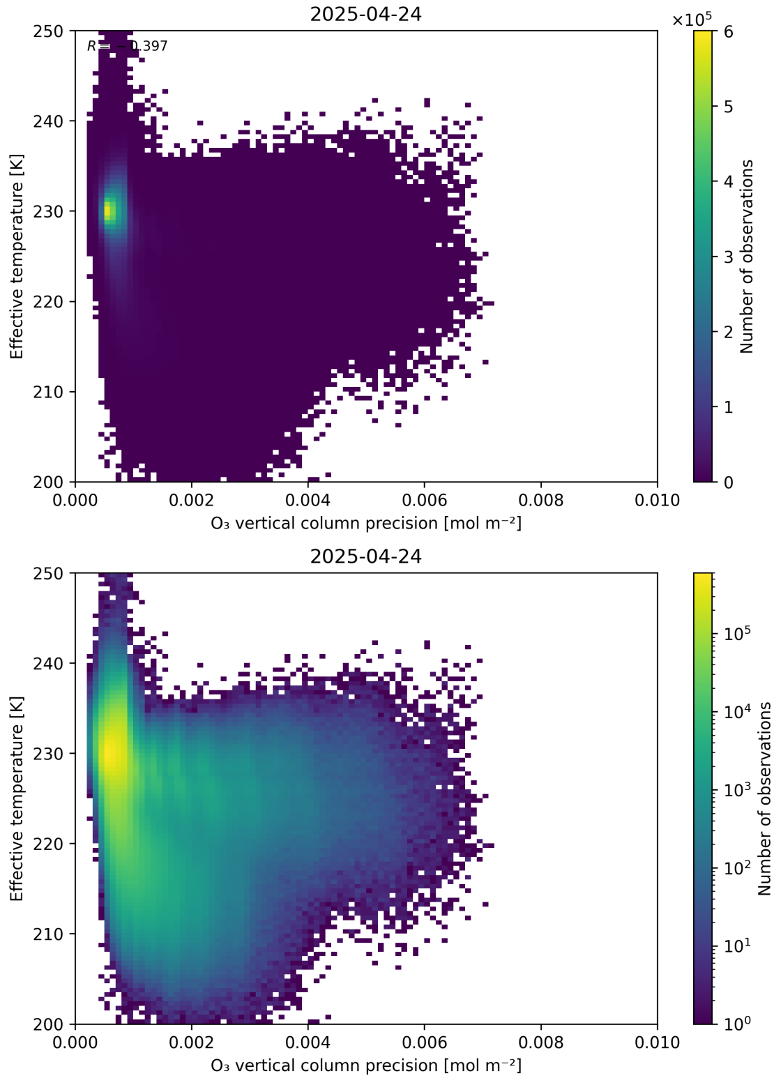
Figure 42: Scatter density plot of “O 3 vertical column precision” against “Effective temperature” for 2025-04-24 to 2025-04-25.
