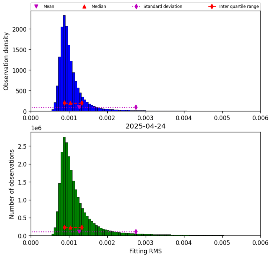
Figure 23: Histogram of “Fitting RMS” for 2025-04-24 to 2025-04-25
