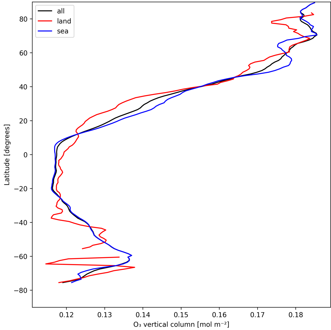
Figure 14: Zonal average of “O 3 vertical column” for 2025-04-24 to 2025-04-25.
