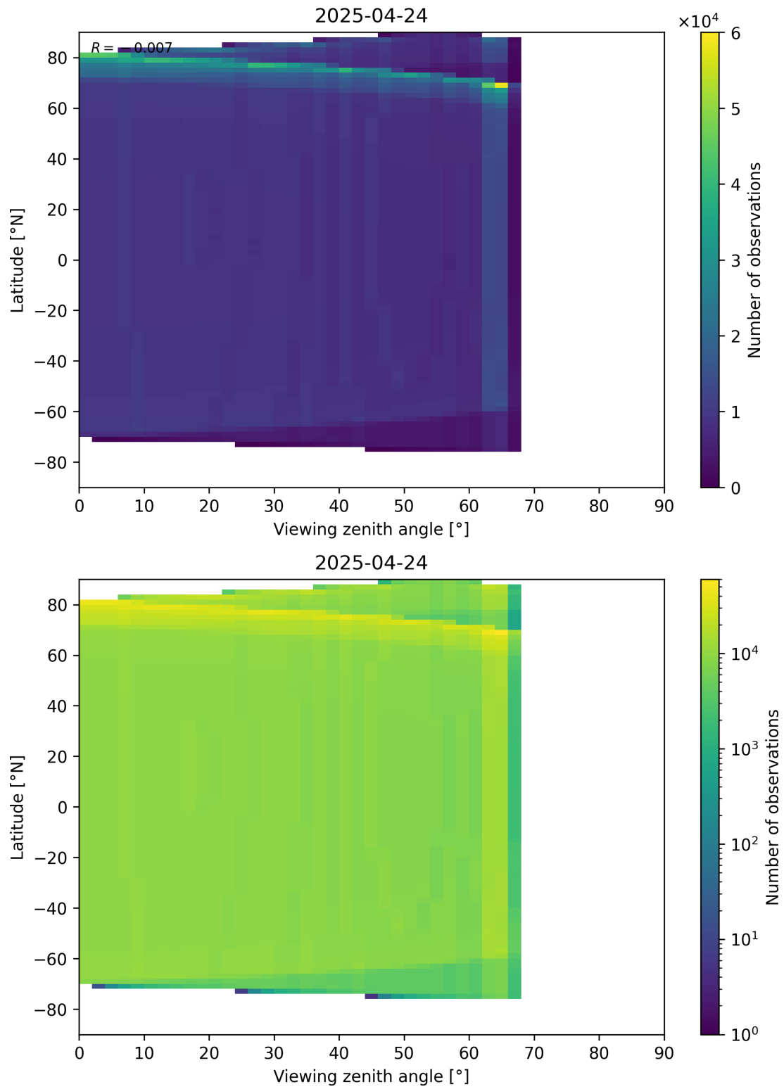
Figure 49: Scatter density plot of “Viewing zenith angle” against “Latitude” for 2025-04-24 to 2025-04-25.
