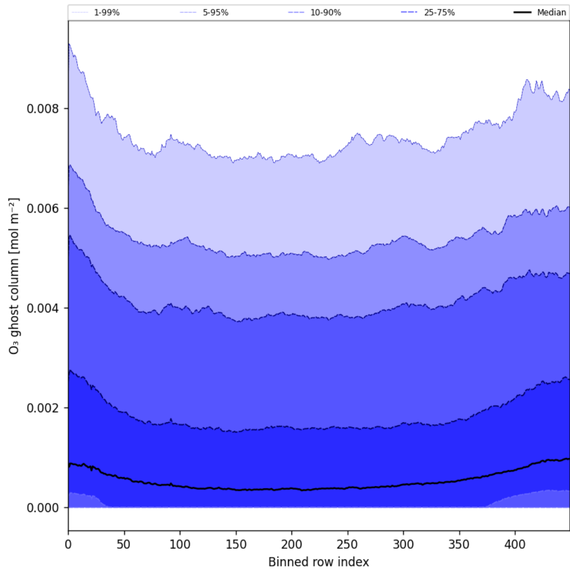
Figure 32: Along track statistics of “O 3 ghost column” for 2025-04-24 to 2025-04-25
