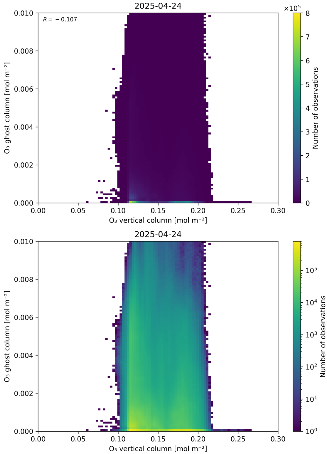
Figure 40: Scatter density plot of “O 3 vertical column” against “O 3 ghost column” for 2025-04-24 to 2025-04-25.
