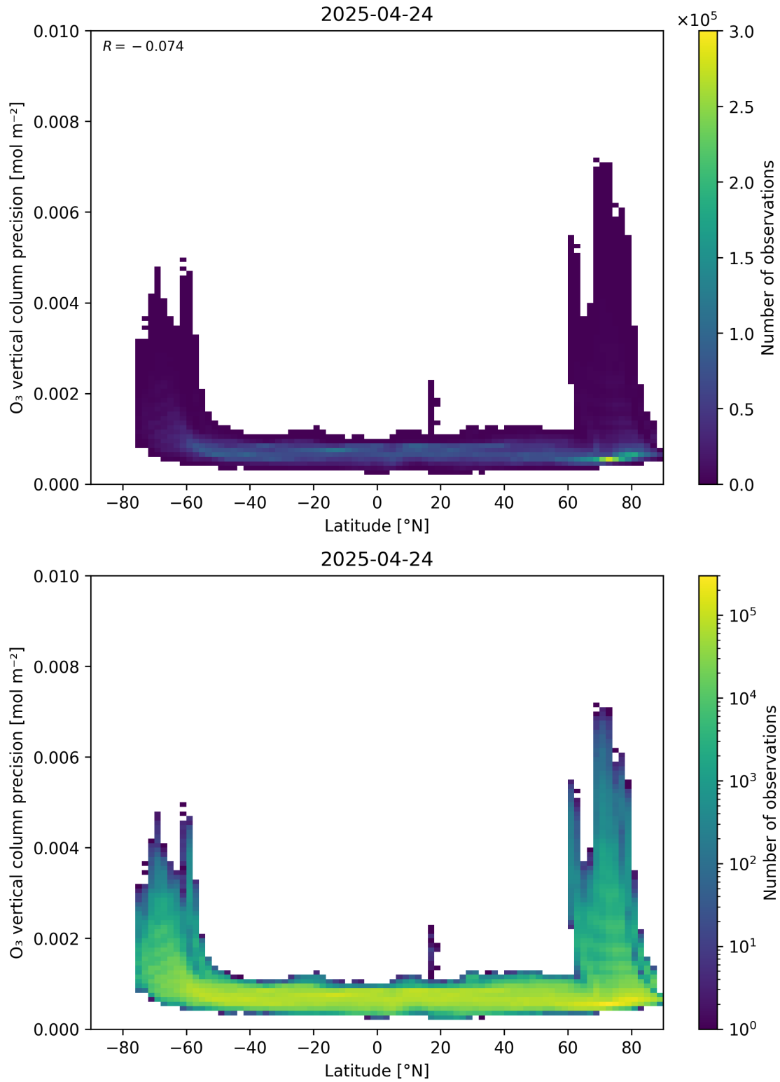
Figure 37: Scatter density plot of “Latitude” against “O 3 vertical column precision” for 2025-04-24 to 2025-04-25.
