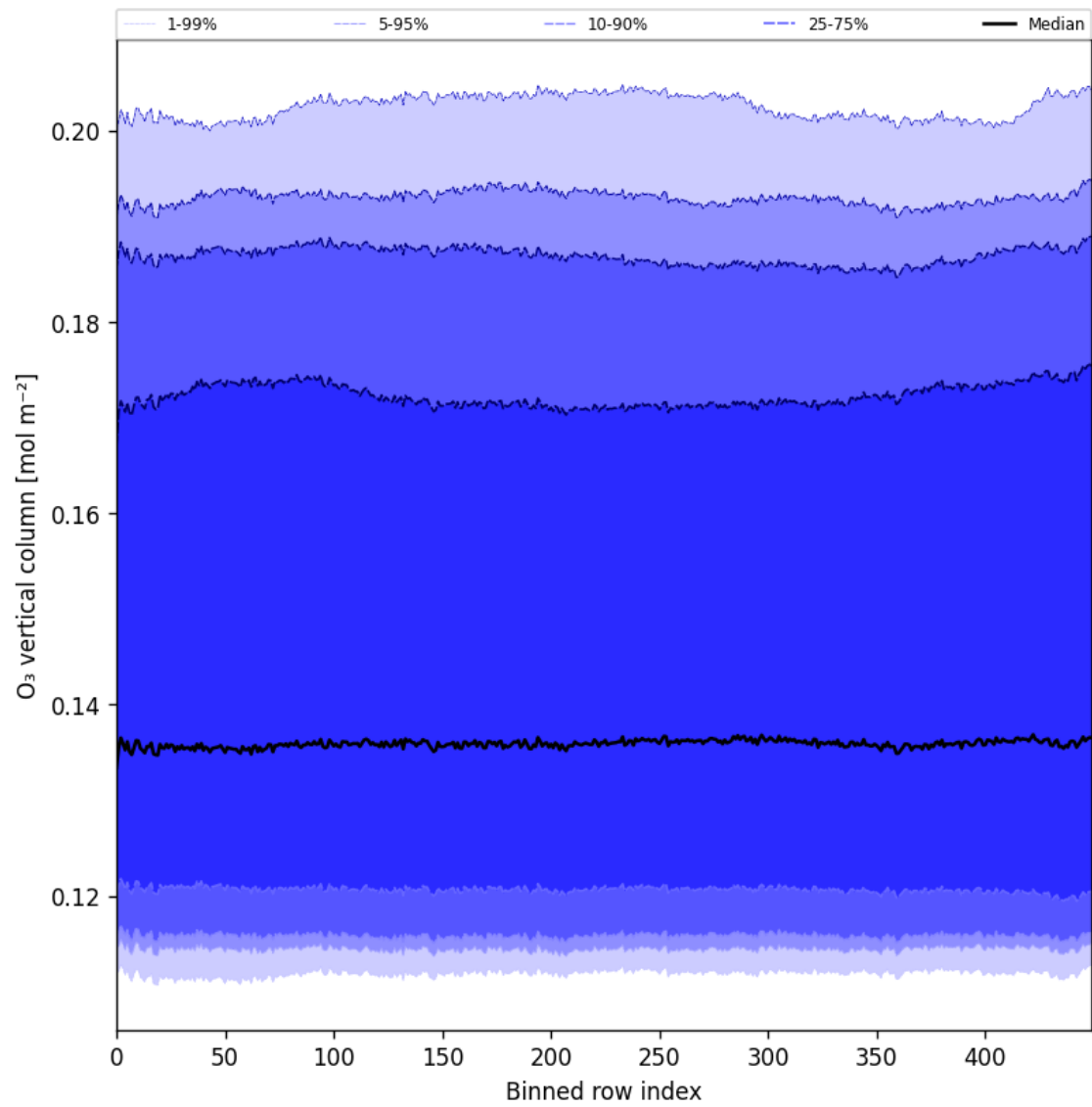
Figure 28: Along track statistics of “ \text{O}_3 vertical column” for 2025-04-24 to 2025-04-25
