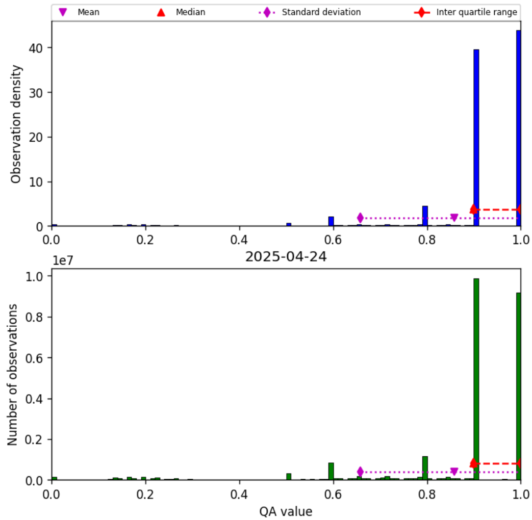
Figure 20: Histogram of “QA value” for 2025-04-24 to 2025-04-25
