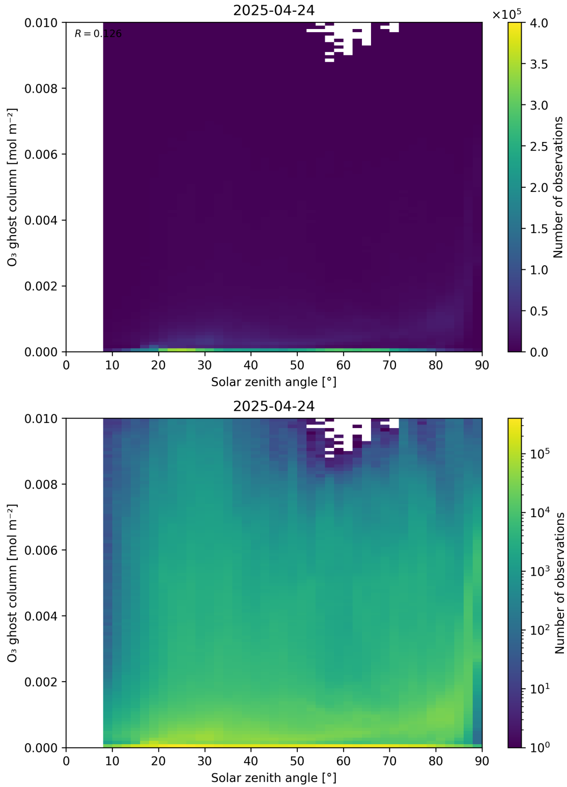
Figure 46: Scatter density plot of “Solar zenith angle” against “O 3 ghost column” for 2025-04-24 to 2025-04-25.
