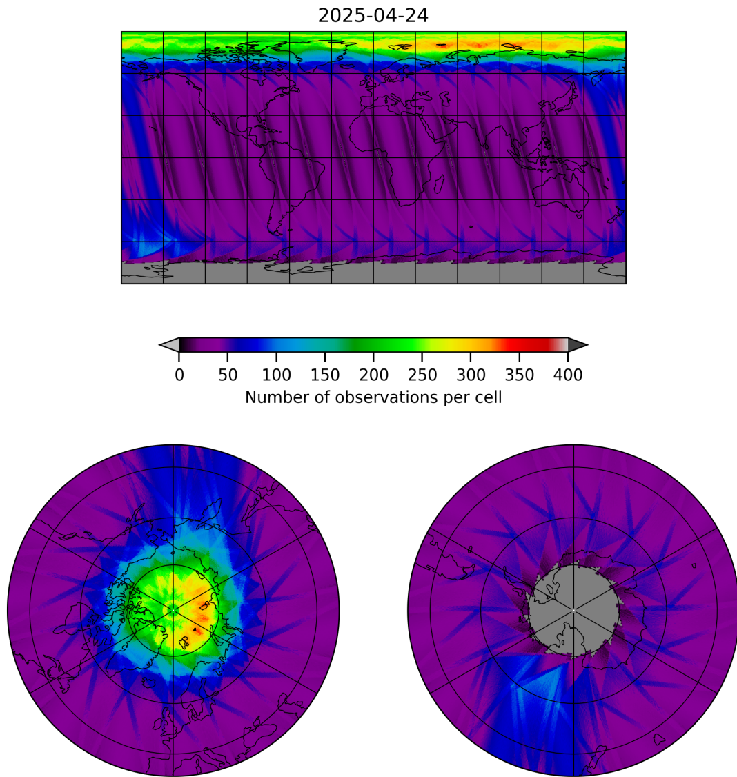
Figure 12: Map of the number of observations for 2025-04-24 to 2025-04-25
