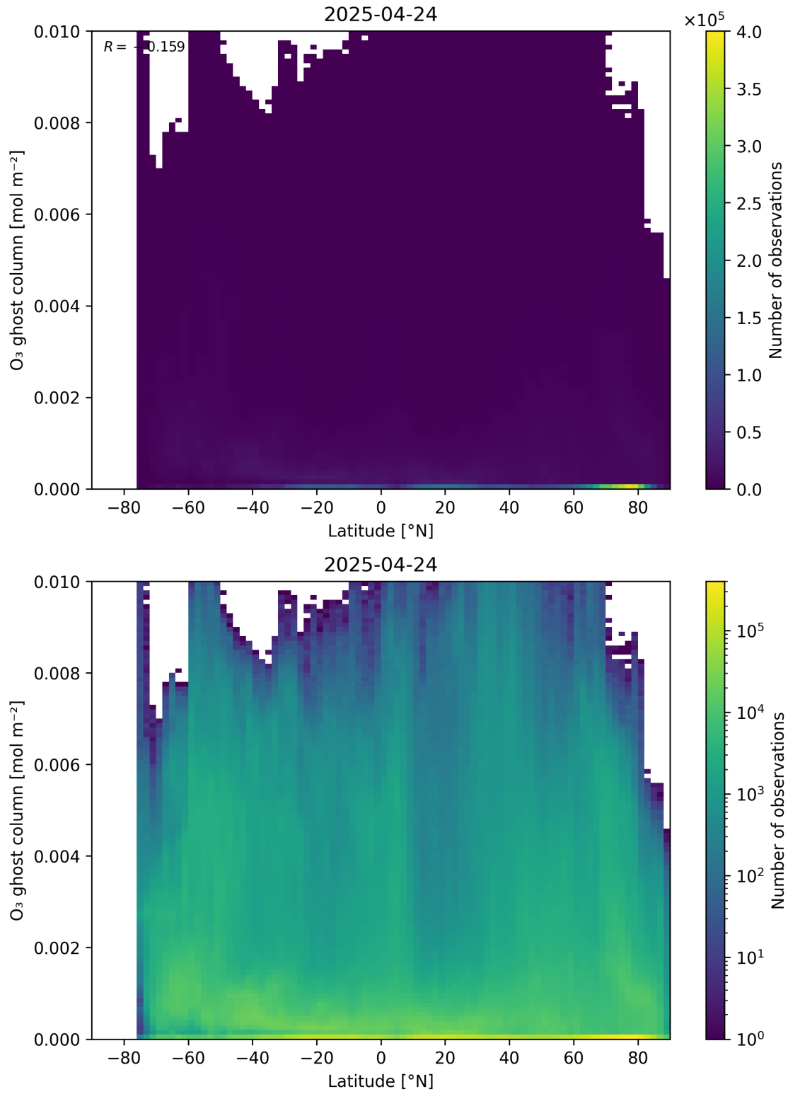
Figure 35: Scatter density plot of “Latitude” against “O 3 ghost column” for 2025-04-24 to 2025-04-25.
