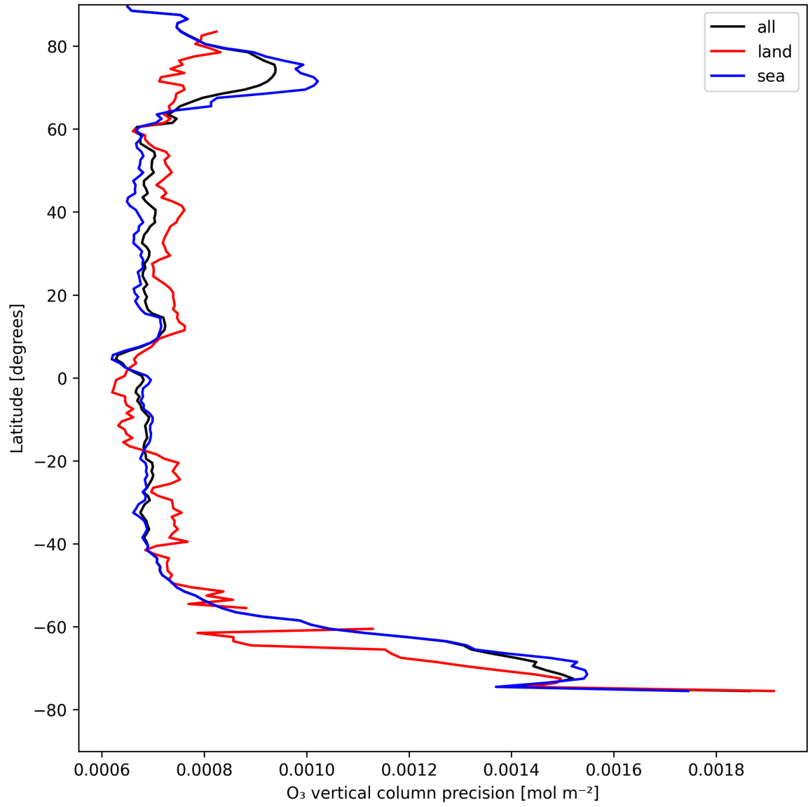
Figure 15: Zonal average of “O 3 vertical column precision” for 2025-04-24 to 2025-04-25.
