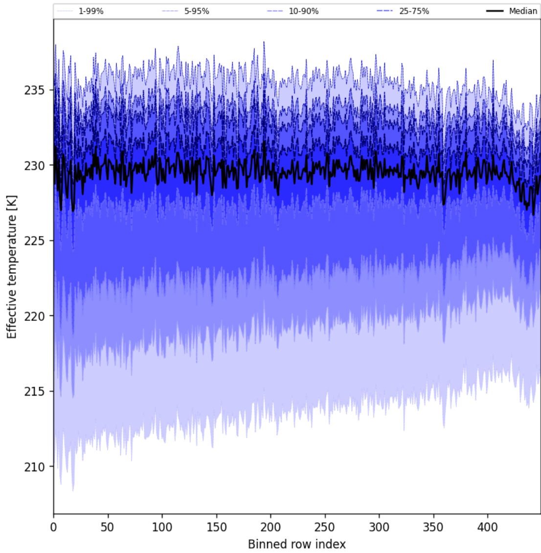
Figure 31: Along track statistics of “Effective temperature” for 2025-04-24 to 2025-04-25
