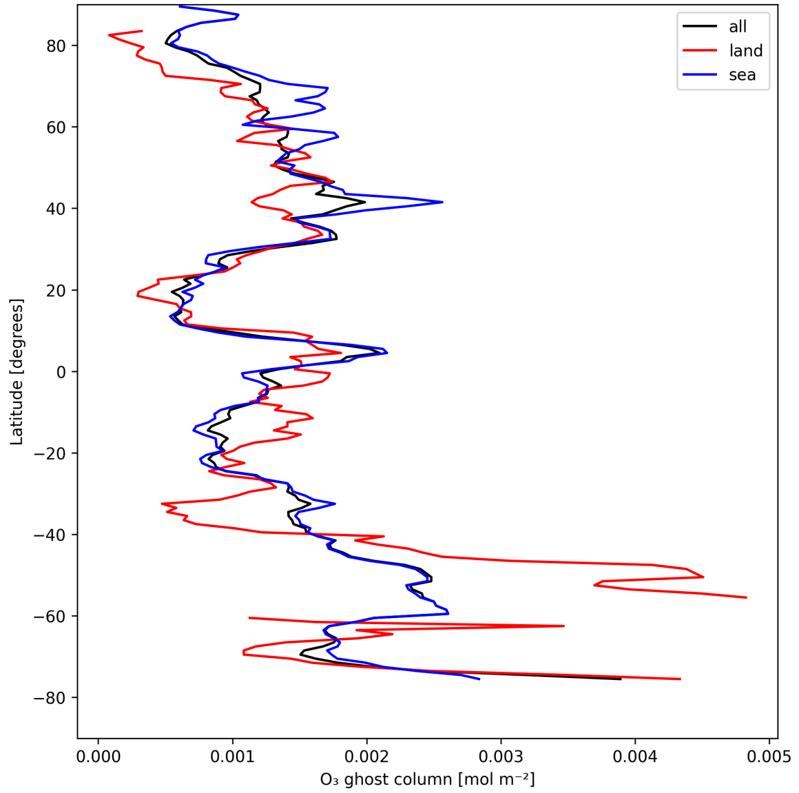
Figure 18: Zonal average of "O 3 ghost column" for 2025-04-24 to 2025-04-25.
