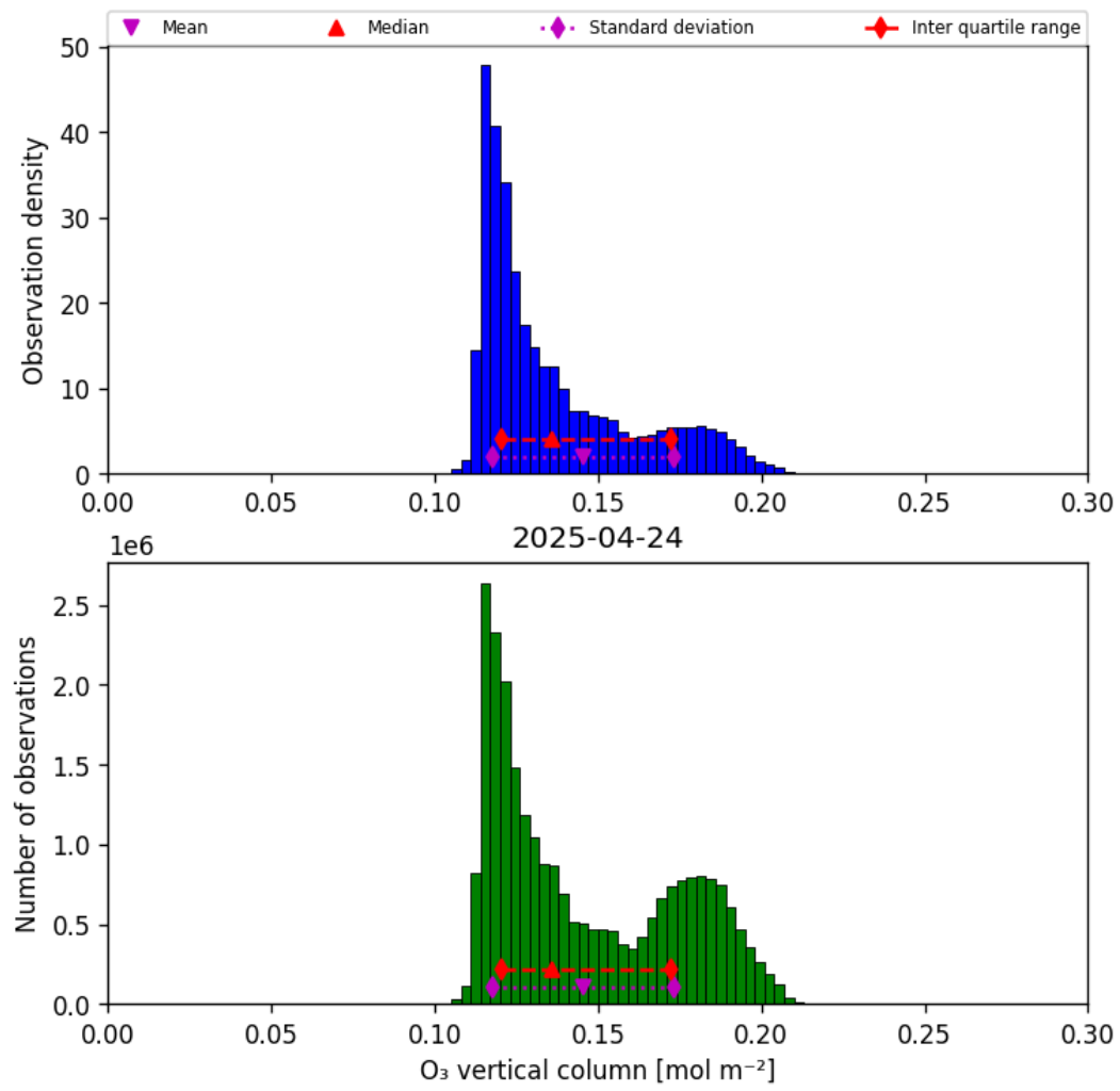
Figure 21: Histogram of “O 3 vertical column” for 2025-04-24 to 2025-04-25
