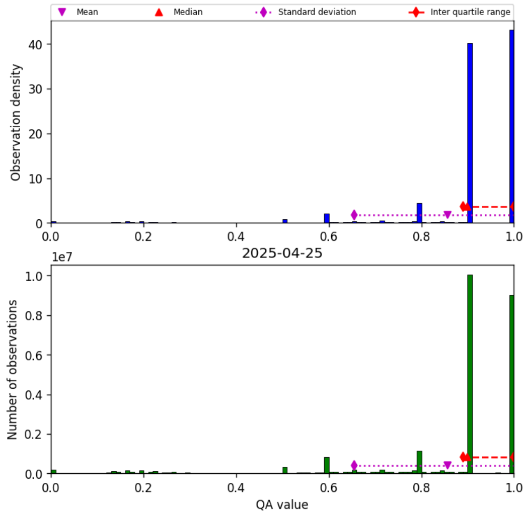
Figure 20: Histogram of “QA value” for 2025-04-24 to 2025-04-26
