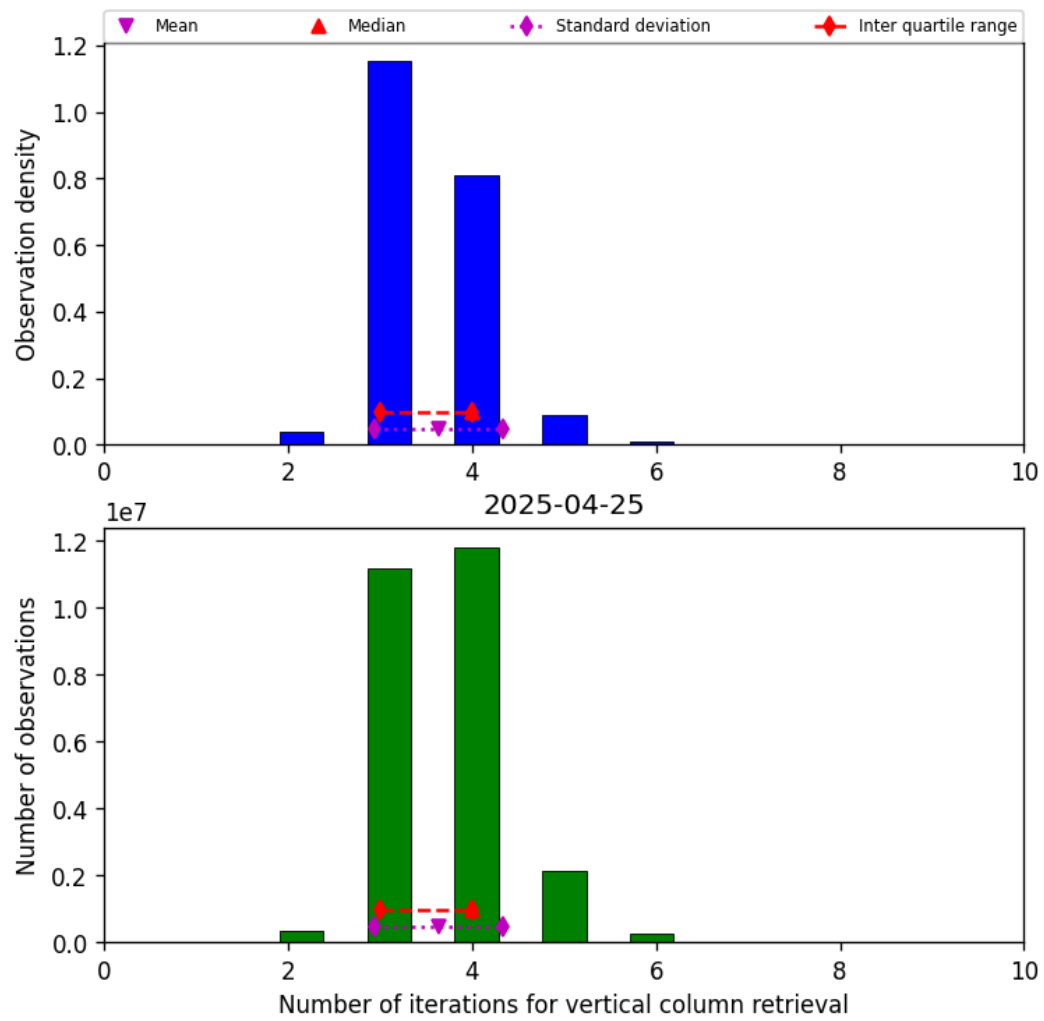
Figure 26: Histogram of “Number of iterations for vertical column retrieval” for 2025-04-24 to 2025-04-26
