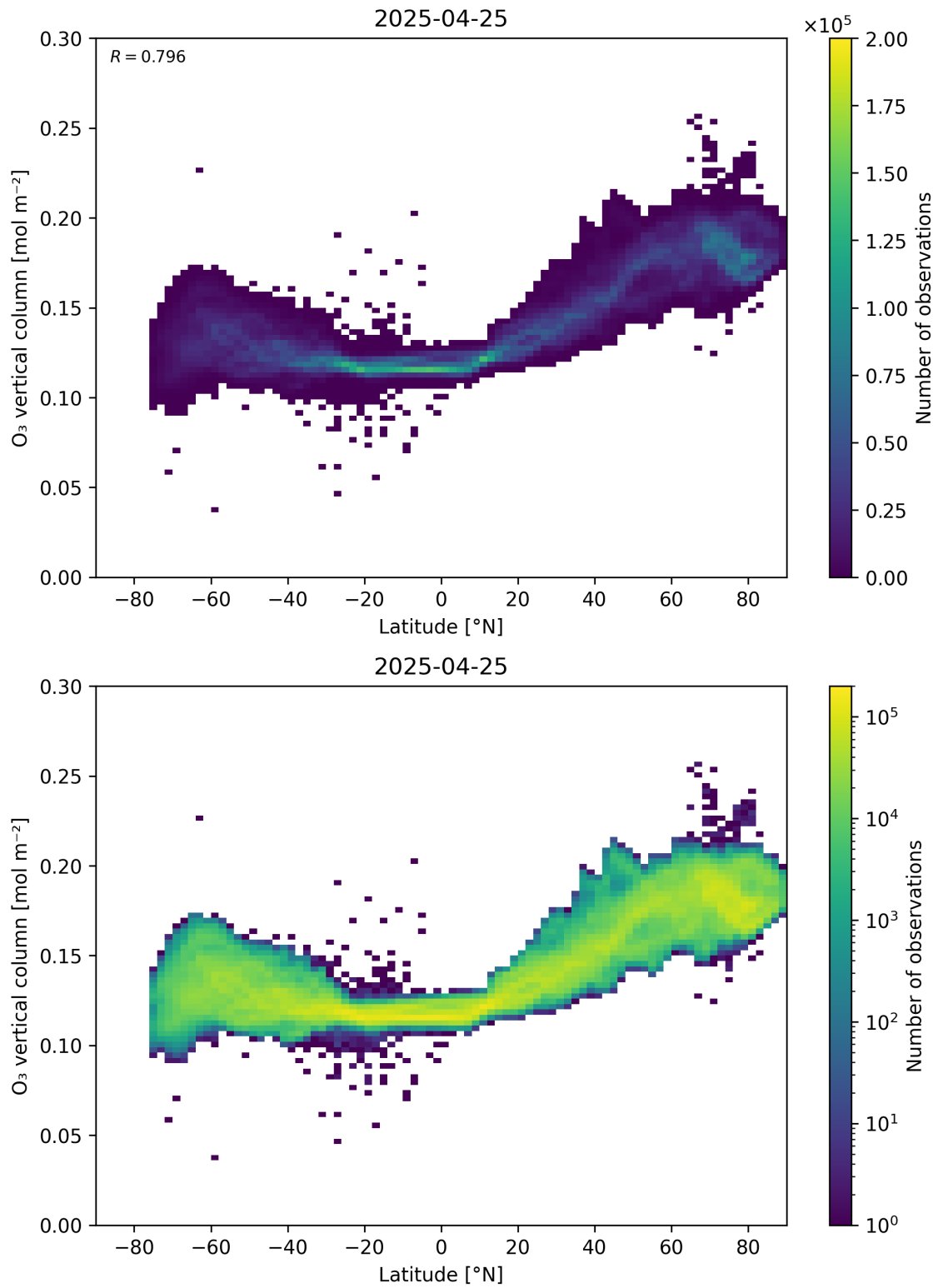
Figure 36: Scatter density plot of “Latitude” against “O 3 vertical column” for 2025-04-24 to 2025-04-26.
