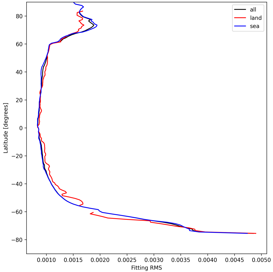
Figure 16: Zonal average of “Fitting RMS” for 2025-04-24 to 2025-04-26.
