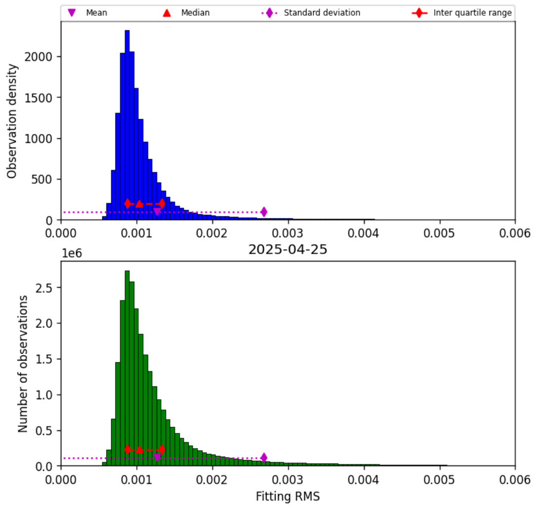
Figure 23: Histogram of “Fitting RMS” for 2025-04-24 to 2025-04-26
