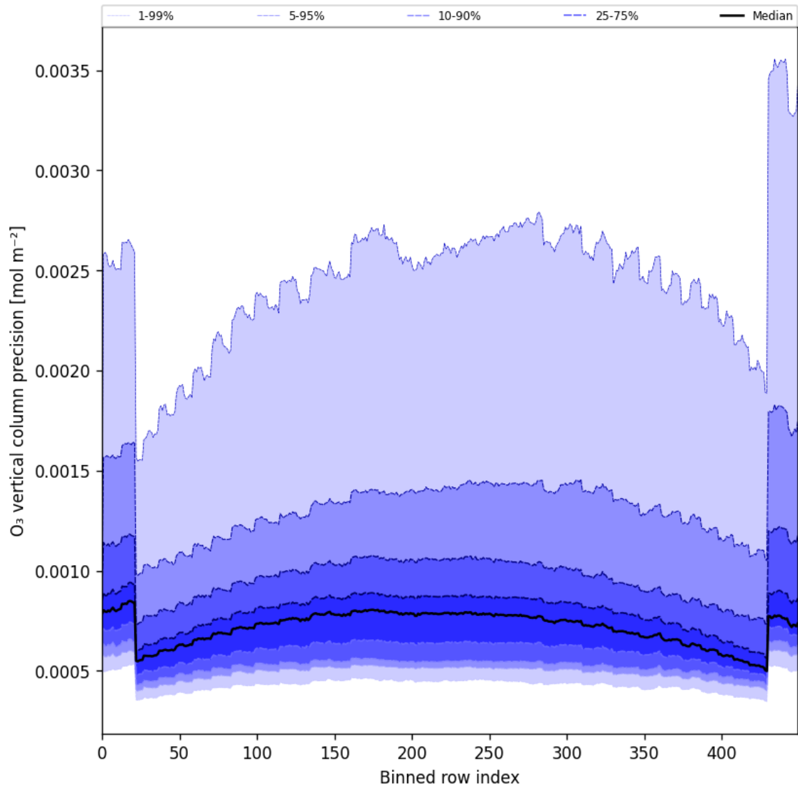
Figure 29: Along track statistics of “O 3 vertical column precision” for 2025-04-24 to 2025-04-26
