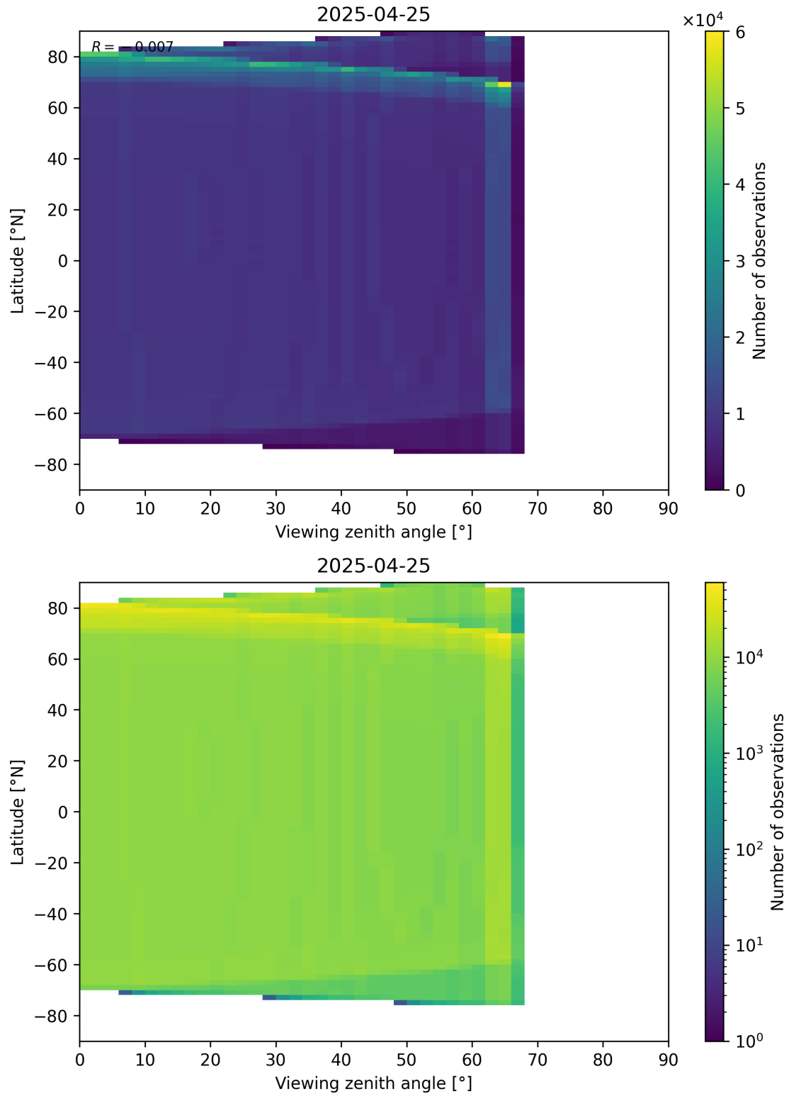
Figure 49: Scatter density plot of “Viewing zenith angle” against “Latitude” for 2025-04-24 to 2025-04-26.
