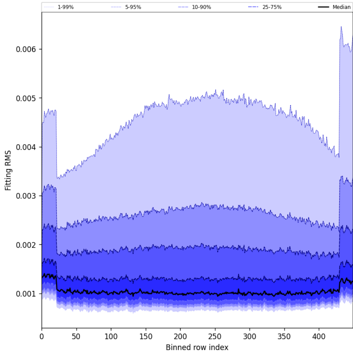
Figure 30: Along track statistics of “Fitting RMS” for 2025-04-24 to 2025-04-26
