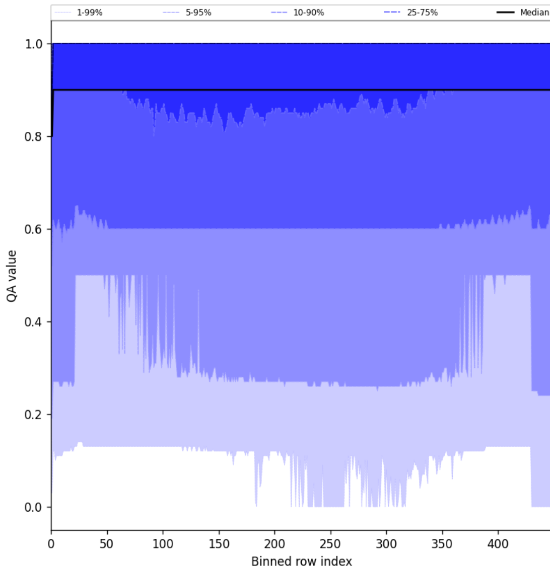
Figure 27: Along track statistics of “QA value” for 2025-04-24 to 2025-04-26
