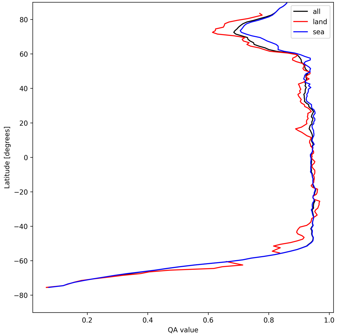
Figure 13: Zonal average of “QA value” for 2025-04-24 to 2025-04-26.
