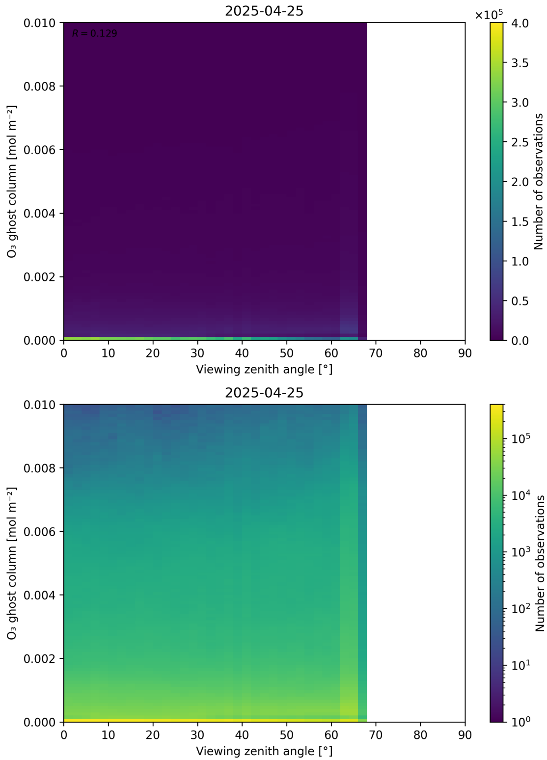
Figure 51: Scatter density plot of “Viewing zenith angle” against “O 3 ghost column” for 2025-04-24 to 2025-04-26.
