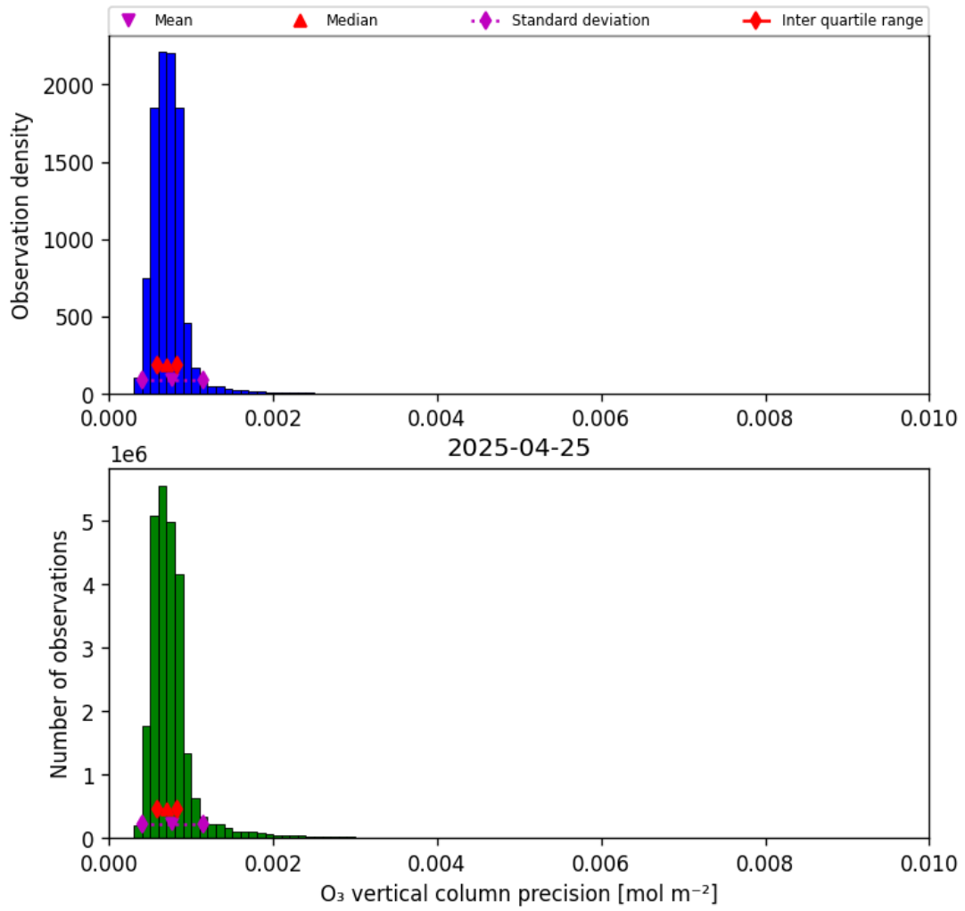
Figure 22: Histogram of “O 3 vertical column precision” for 2025-04-24 to 2025-04-26
