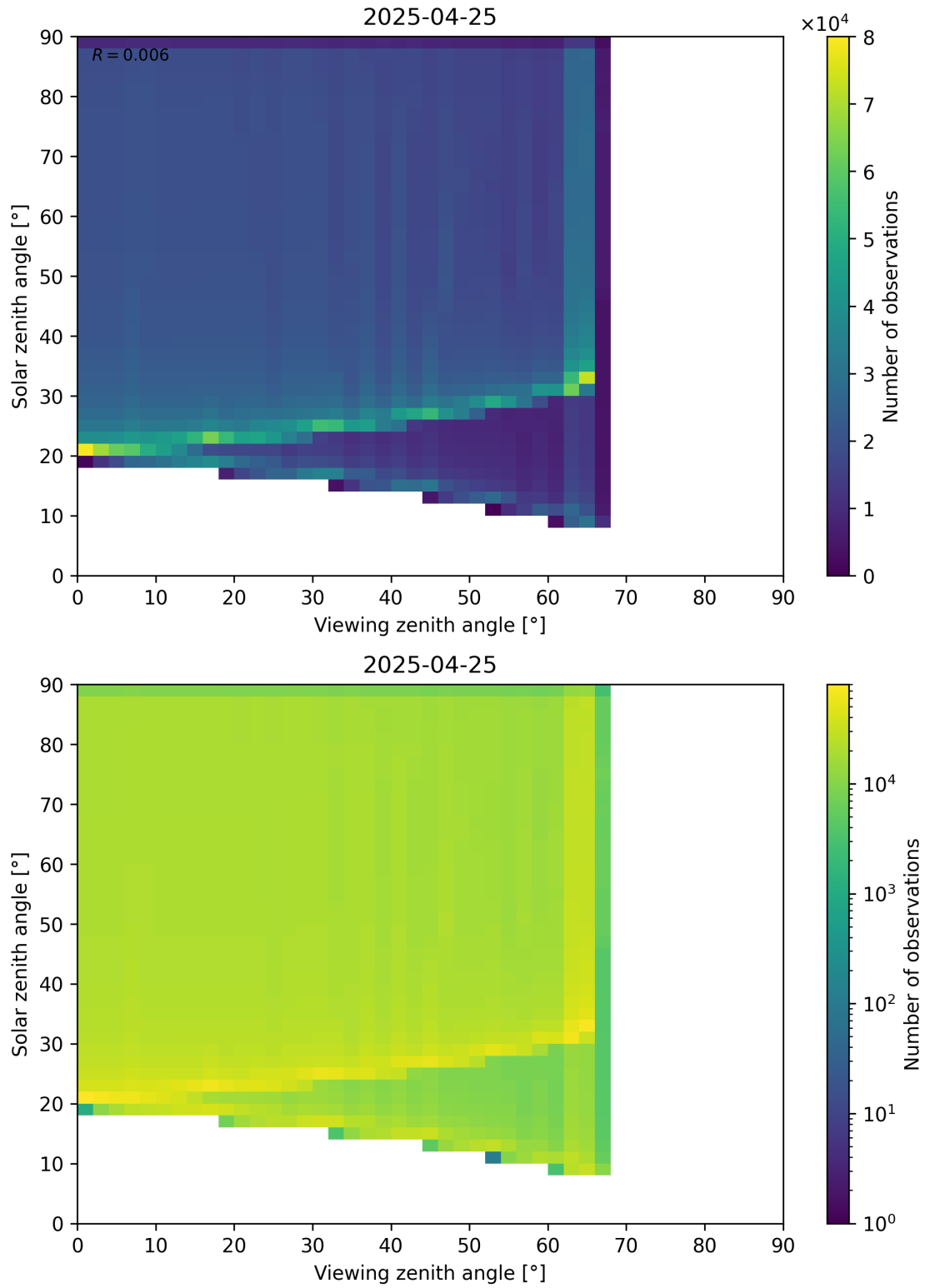
Figure 54: Scatter density plot of “Viewing zenith angle” against “Solar zenith angle” for 2025-04-24 to 2025-04-26.
