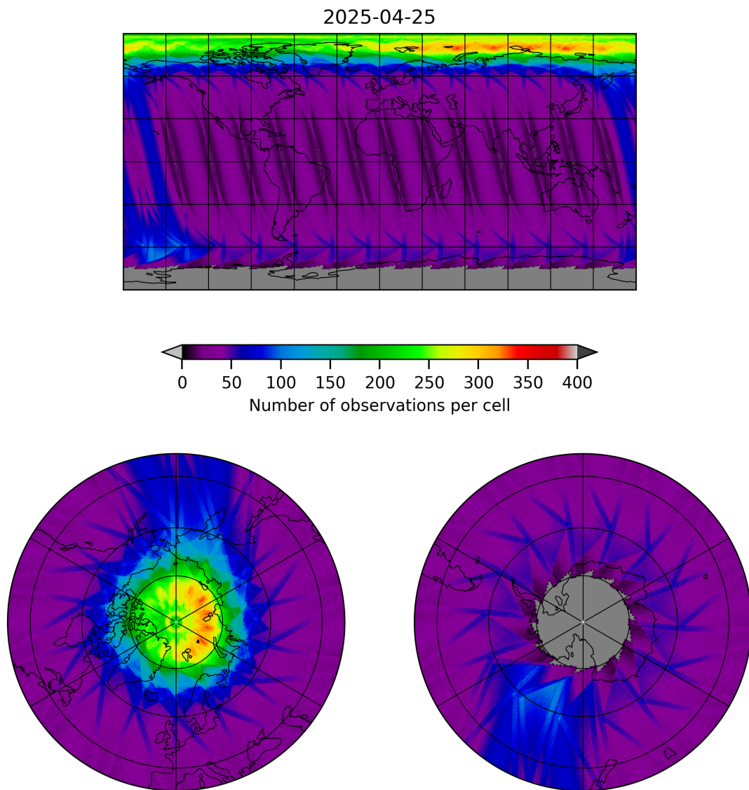
Figure 12: Map of the number of observations for 2025-04-24 to 2025-04-26
