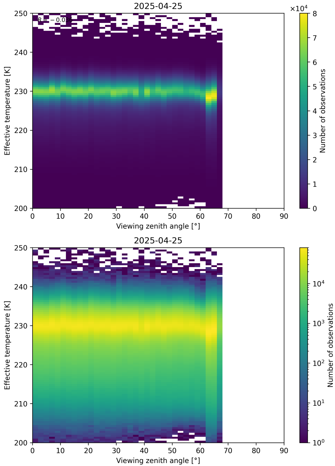
Figure 50: Scatter density plot of “Viewing zenith angle” against “Effective temperature” for 2025-04-24 to 2025-04-26.
