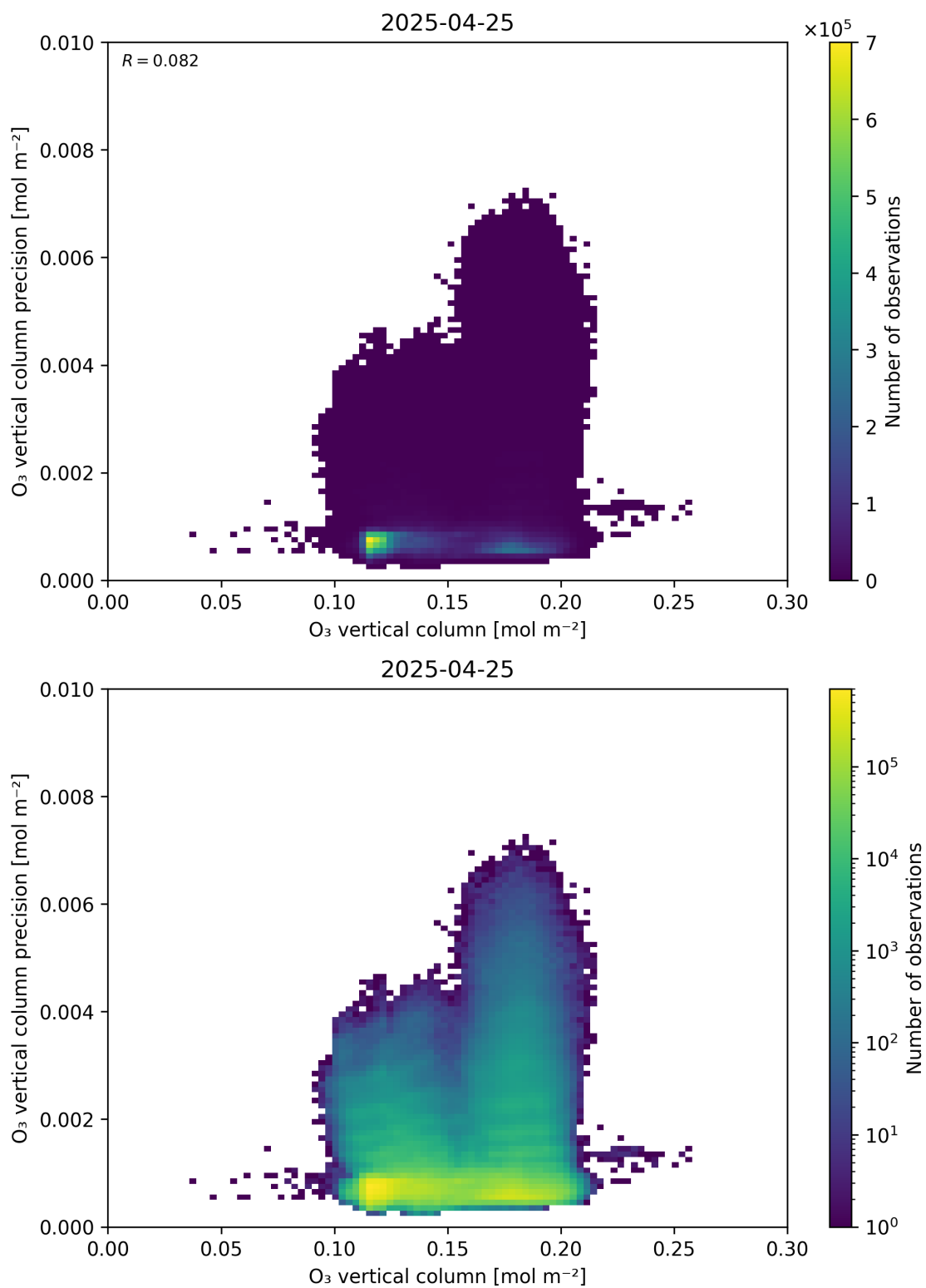
Figure 41: Scatter density plot of “O 3 vertical column” against “O 3 vertical column precision” for 2025-04-24 to 2025-04-26.
