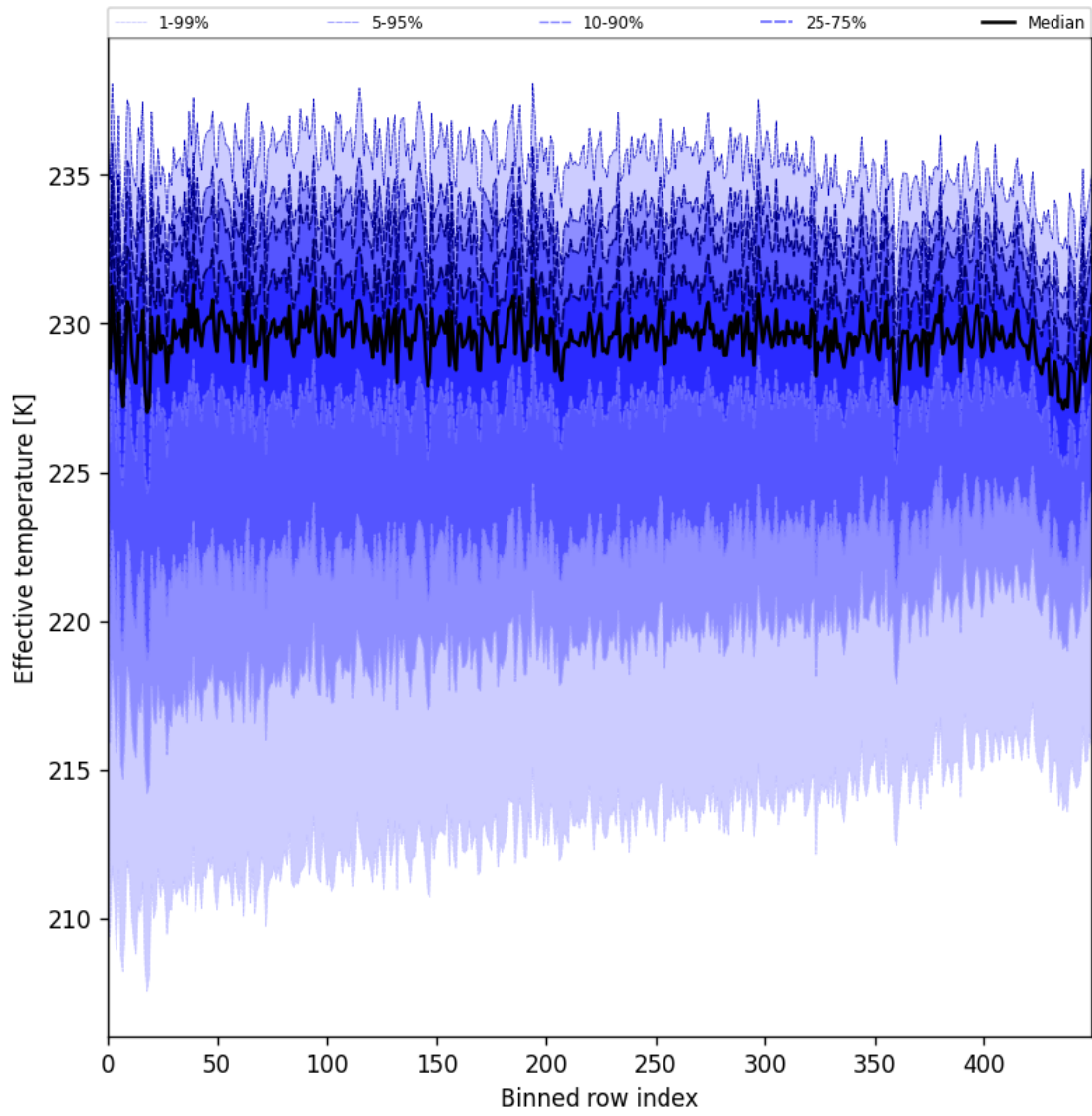
Figure 31: Along track statistics of “Effective temperature” for 2025-04-24 to 2025-04-26
