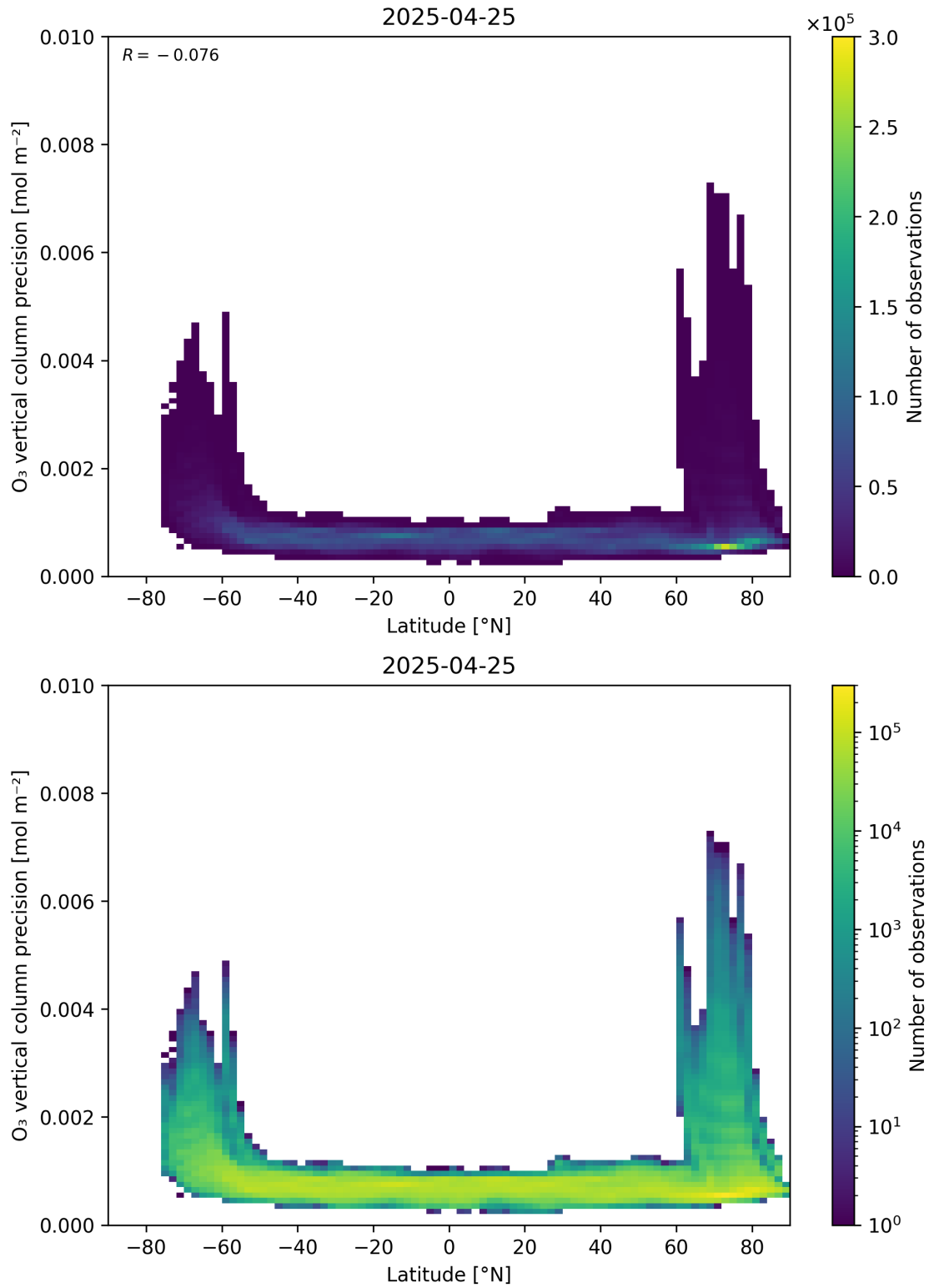
Figure 37: Scatter density plot of “Latitude” against “O 3 vertical column precision” for 2025-04-24 to 2025-04-26.
