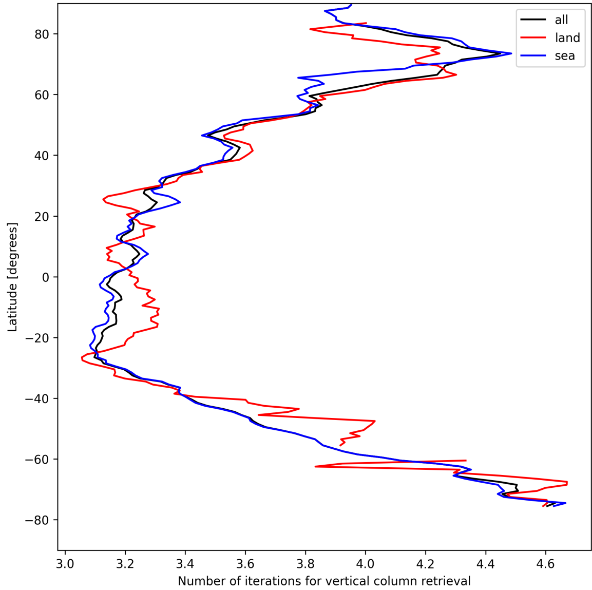
Figure 19: Zonal average of “Number of iterations for vertical column retrieval” for 2025-04-24 to 2025-04-26.
