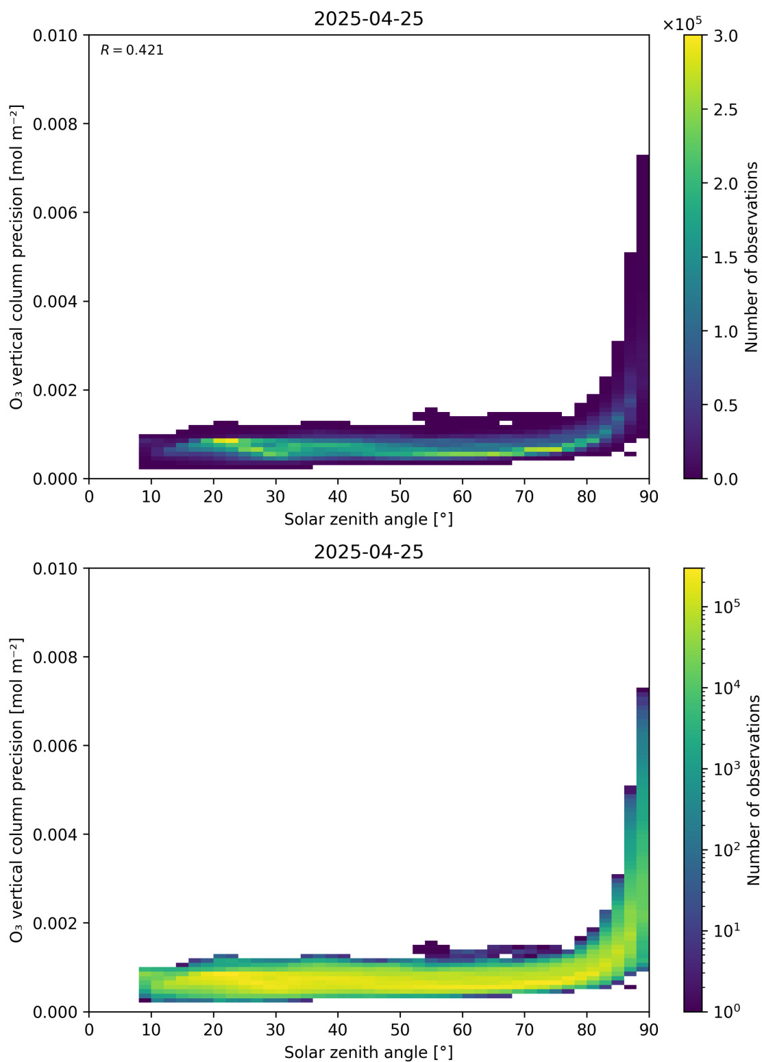
Figure 48: Scatter density plot of “Solar zenith angle” against “O 3 vertical column precision” for 2025-04-24 to 2025-04-26.
