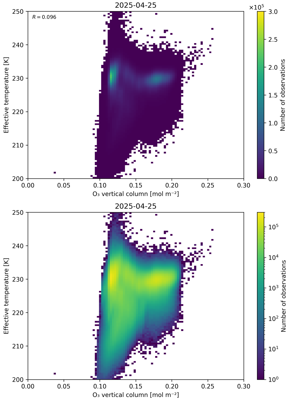
Figure 39: Scatter density plot of “O 3 vertical column” against “Effective temperature” for 2025-04-24 to 2025-04-26.
