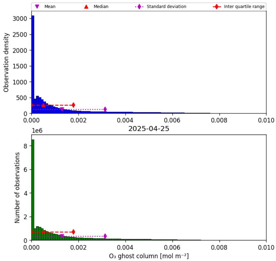
Figure 25: Histogram of “O 3 ghost column” for 2025-04-24 to 2025-04-26
