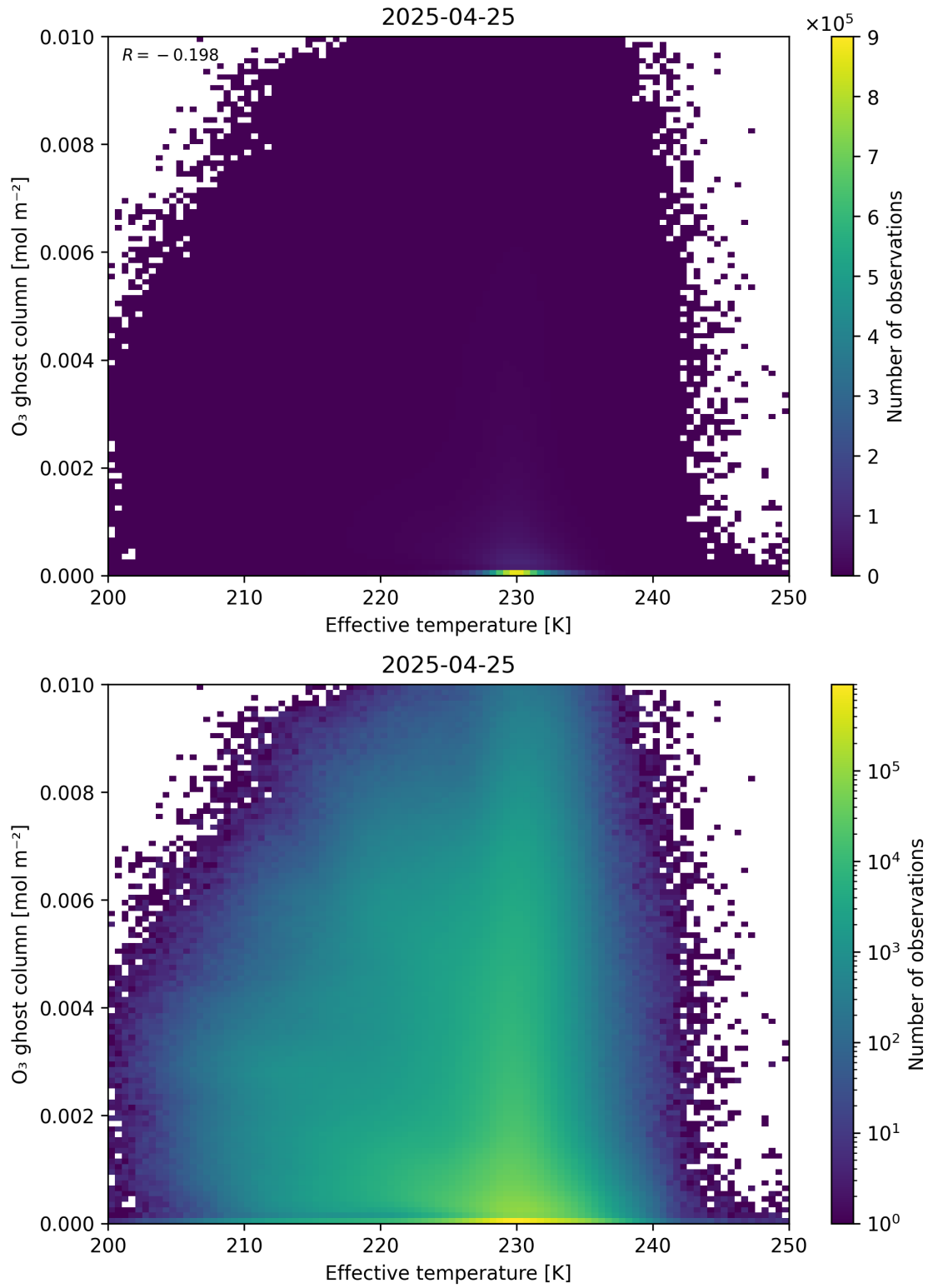
Figure 38: Scatter density plot of “Effective temperature” against “O 3 ghost column” for 2025-04-24 to 2025-04-26.
