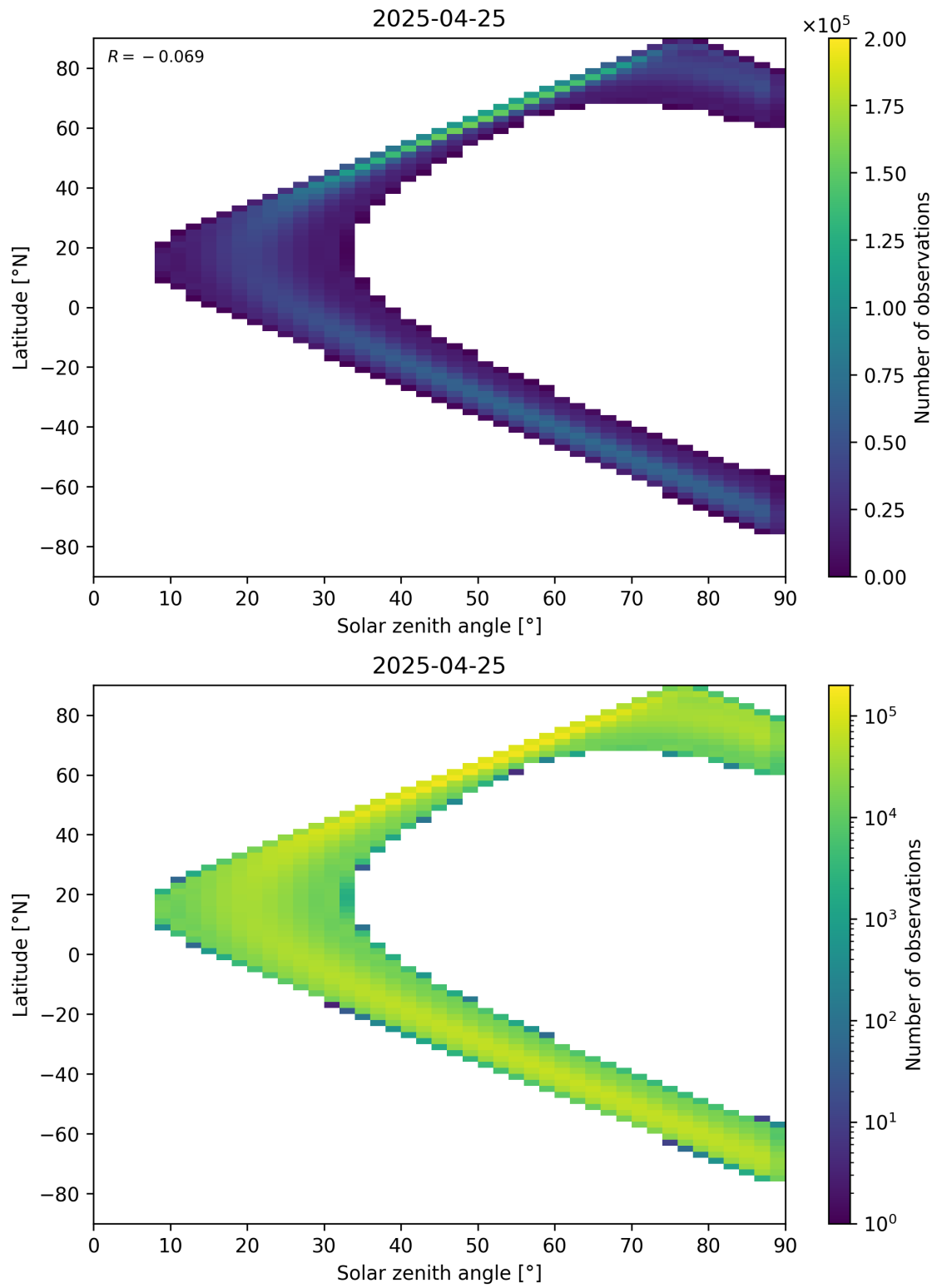
Figure 44: Scatter density plot of “Solar zenith angle” against “Latitude” for 2025-04-24 to 2025-04-26.
