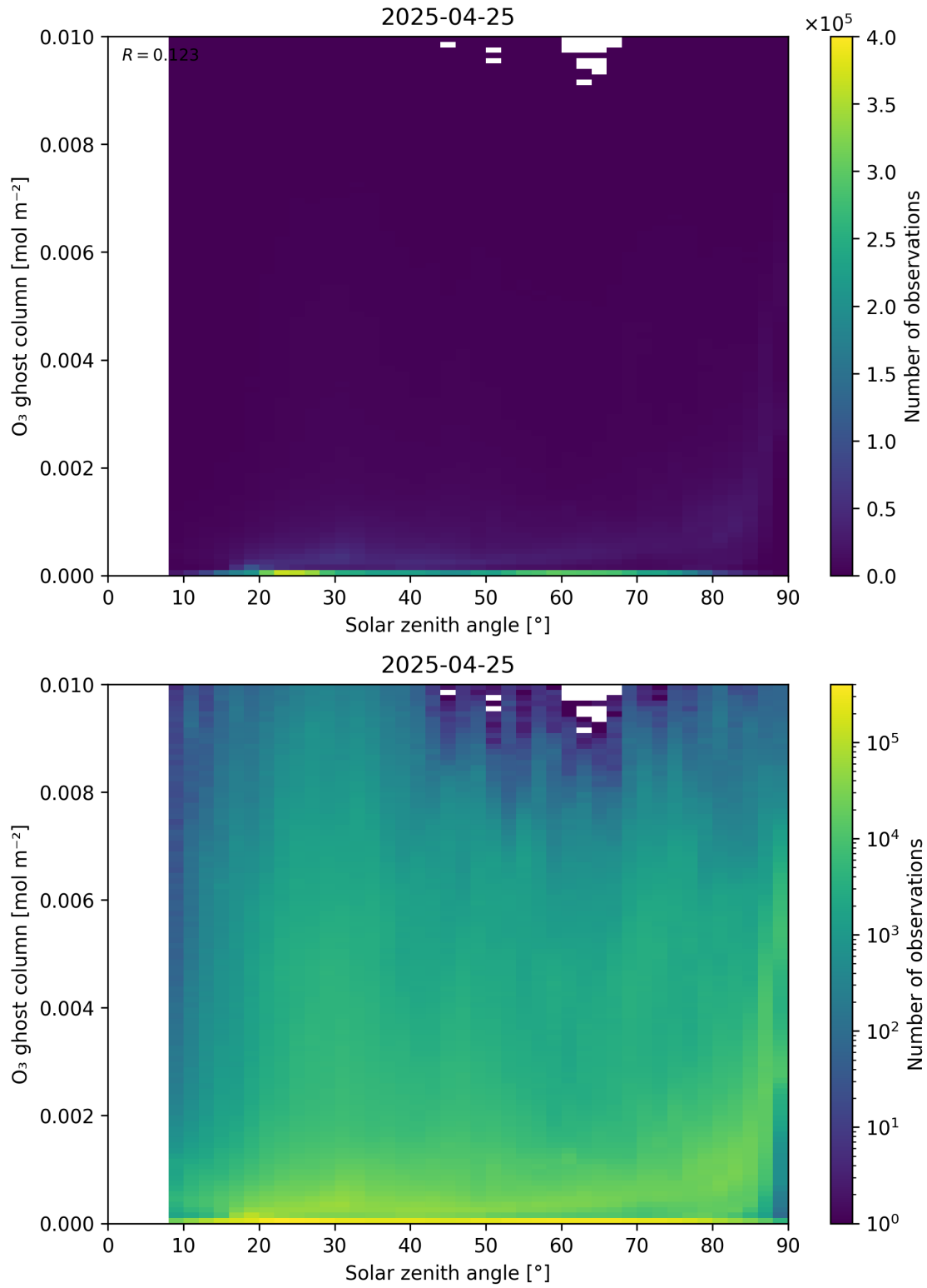
Figure 46: Scatter density plot of “Solar zenith angle” against “O 3 ghost column” for 2025-04-24 to 2025-04-26.
