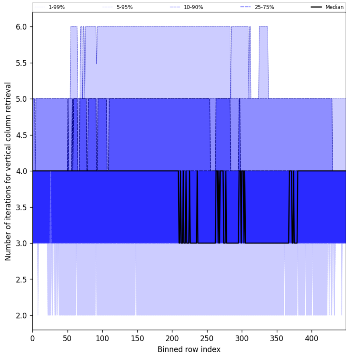
Figure 33: Along track statistics of “Number of iterations for vertical column retrieval” for 2025-04-24 to 2025-04-26
