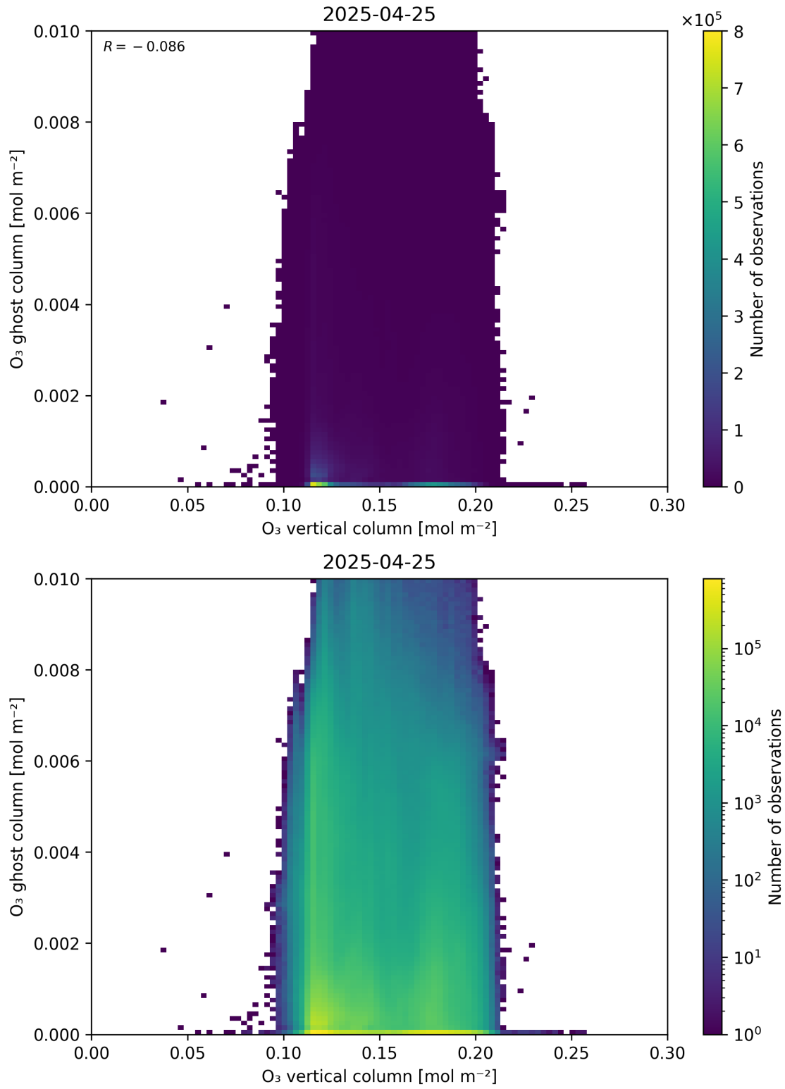
Figure 40: Scatter density plot of “O 3 vertical column” against “O 3 ghost column” for 2025-04-24 to 2025-04-26.
