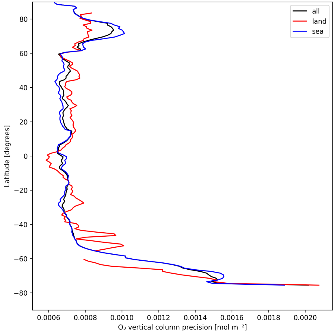
Figure 15: Zonal average of “O 3 vertical column precision” for 2025-04-24 to 2025-04-26.
