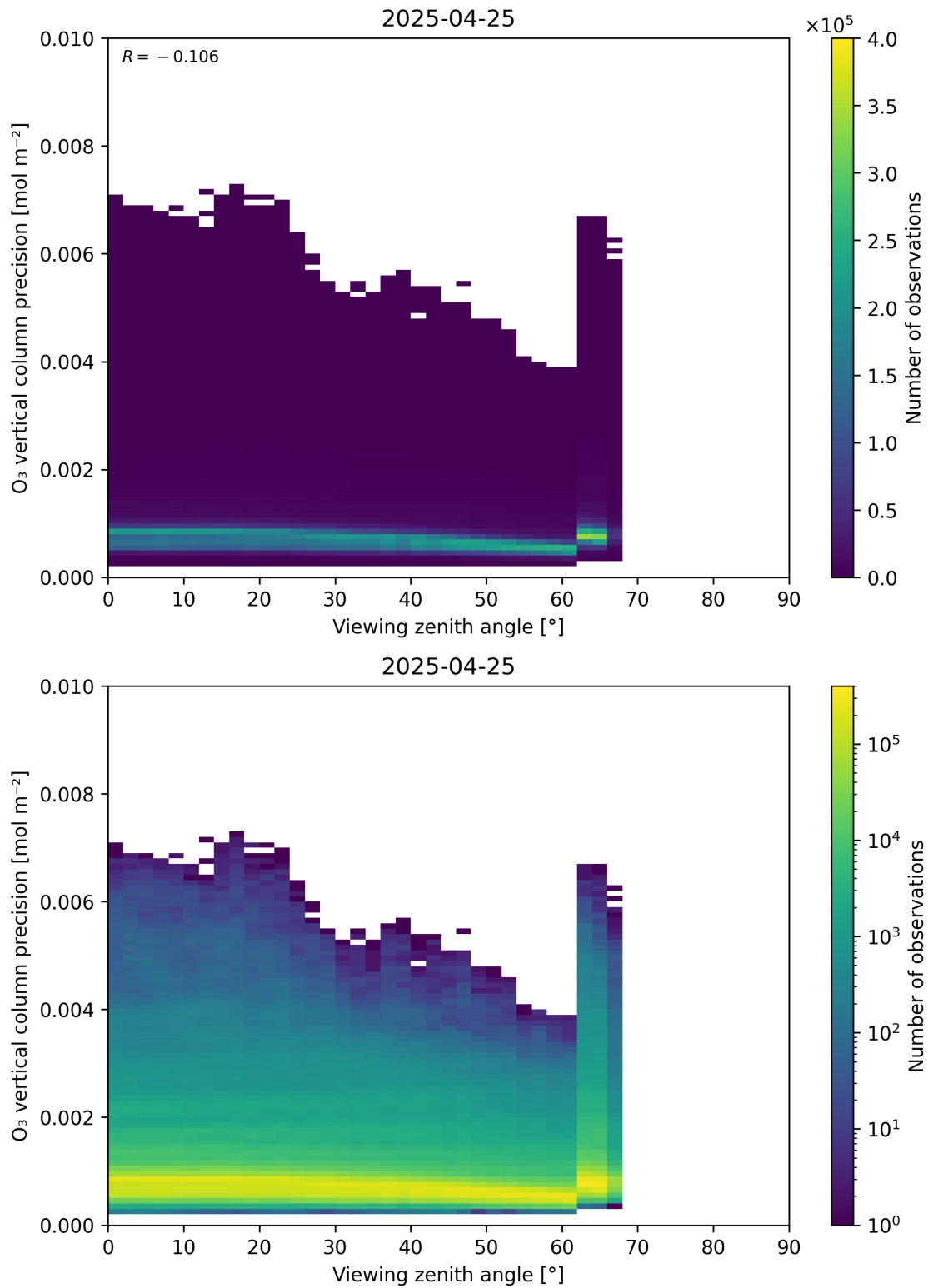
Figure 53: Scatter density plot of “Viewing zenith angle” against “O 3 vertical column precision” for 2025-04-24 to 2025-04-26.
