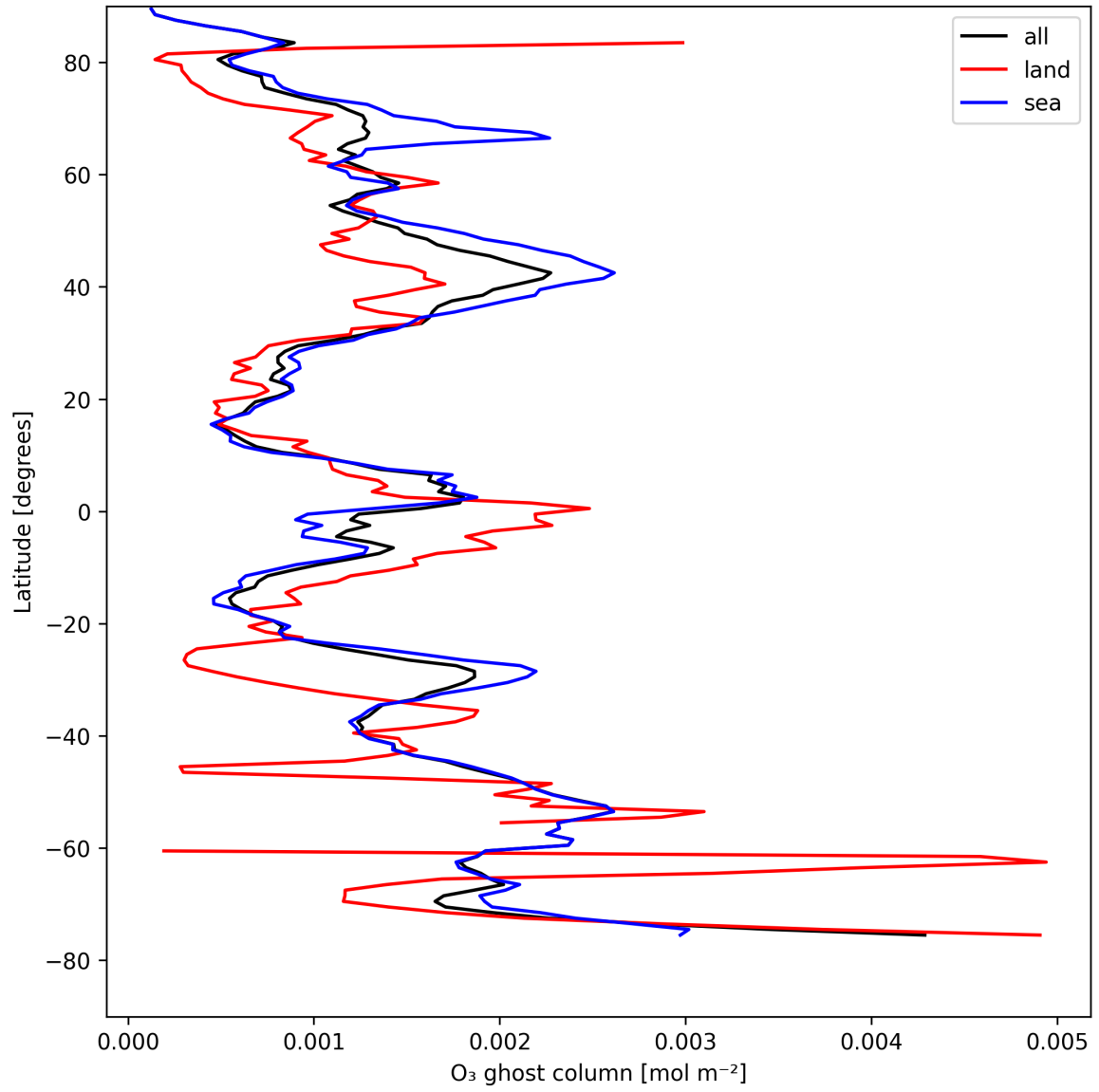
Figure 18: Zonal average of “O 3 ghost column” for 2025-04-24 to 2025-04-26.
