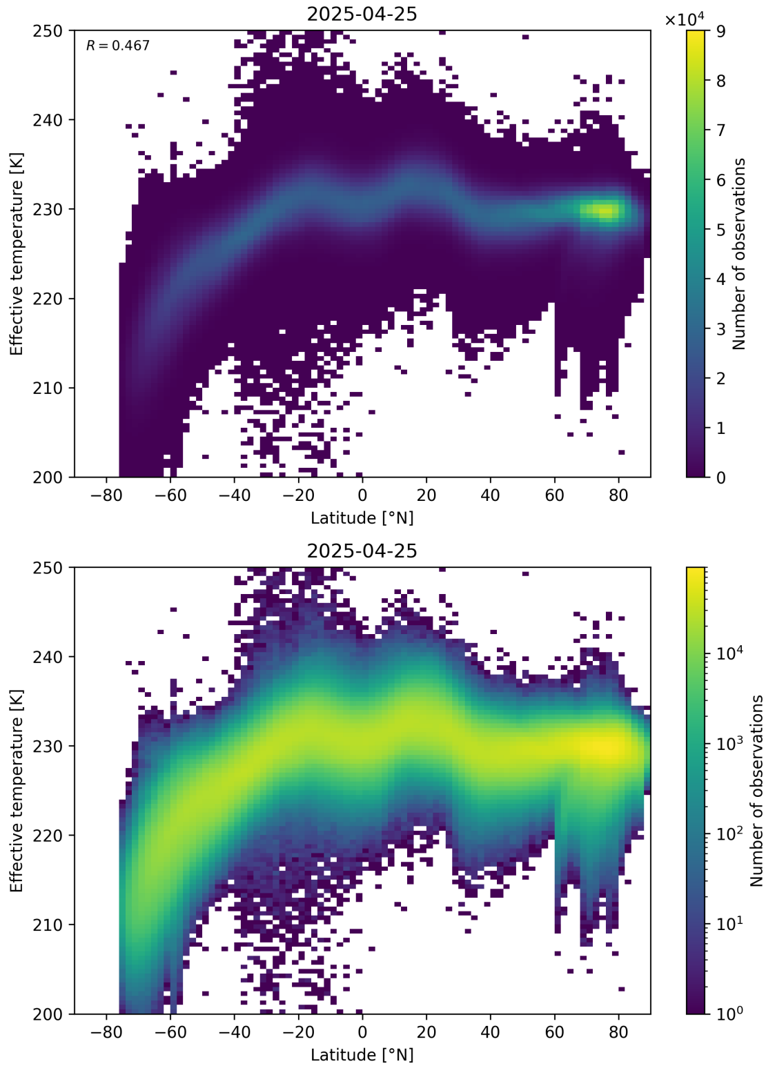
Figure 34: Scatter density plot of “Latitude” against “Effective temperature” for 2025-04-24 to 2025-04-26.
