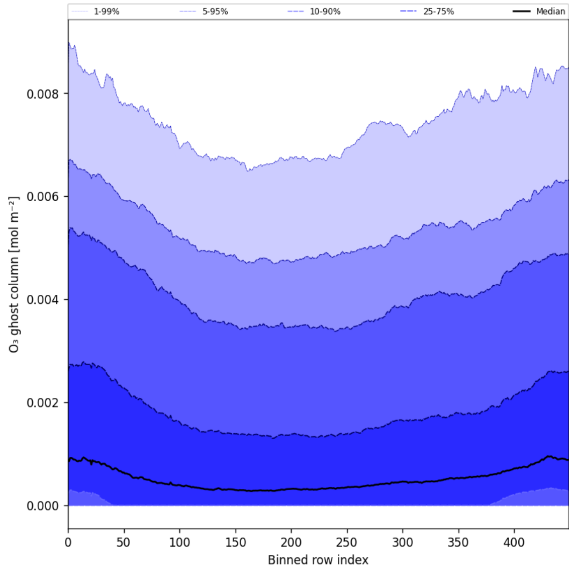
Figure 32: Along track statistics of “O 3 ghost column” for 2025-04-24 to 2025-04-26
