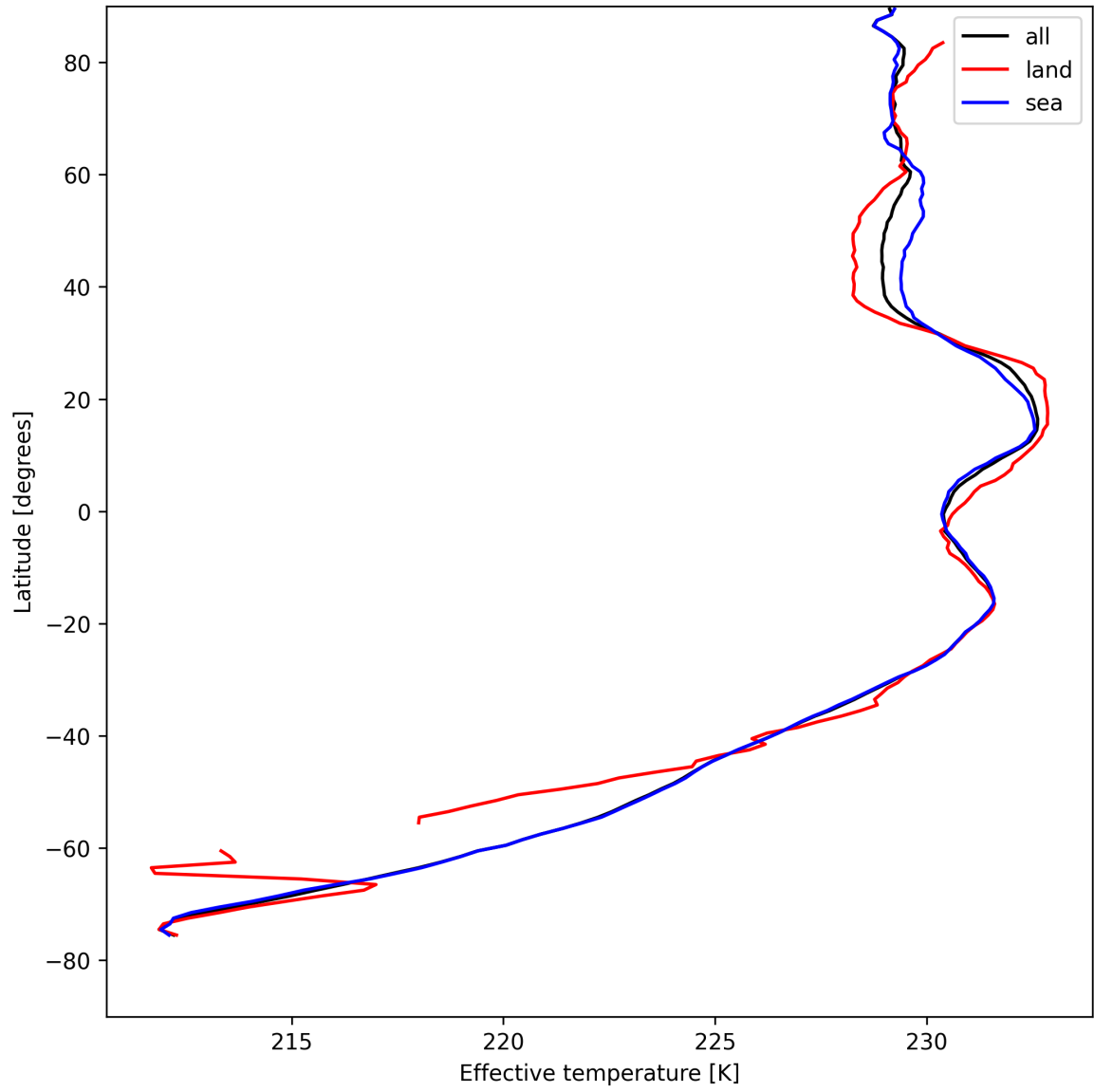
Figure 17: Zonal average of "Effective temperature" for 2025-04-24 to 2025-04-26.
