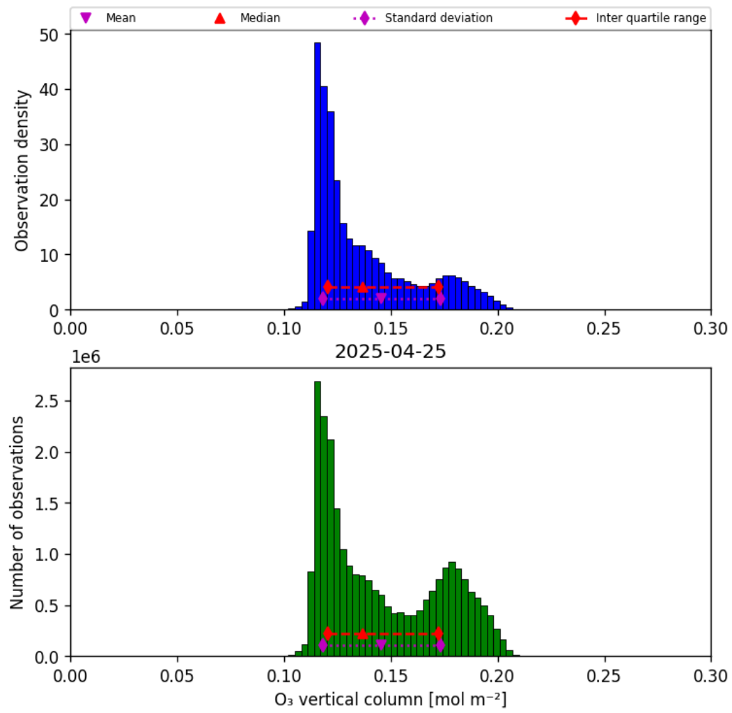
Figure 21: Histogram of “O 3 vertical column” for 2025-04-24 to 2025-04-26
