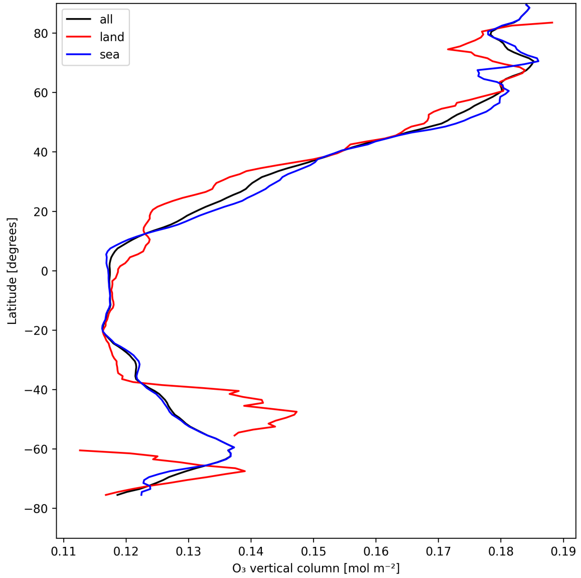
Figure 14: Zonal average of “O 3 vertical column” for 2025-04-24 to 2025-04-26.
