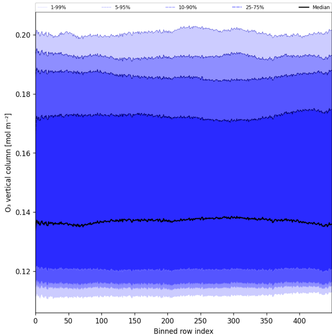
Figure 28: Along track statistics of “O 3 vertical column” for 2025-04-24 to 2025-04-26
