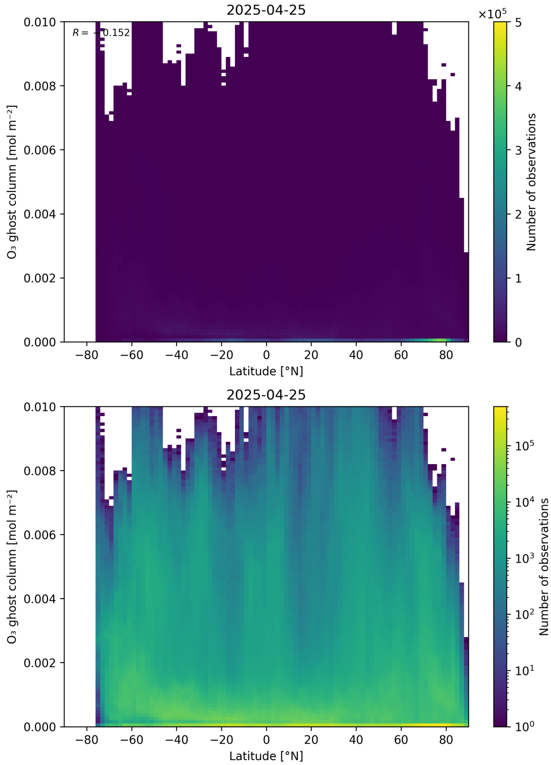
Figure 35: Scatter density plot of “Latitude” against “O 3 ghost column” for 2025-04-24 to 2025-04-26.
