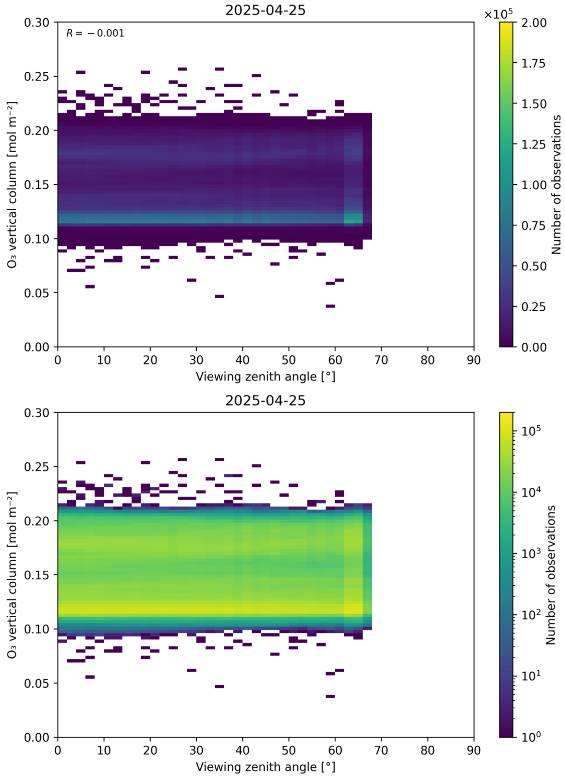
Figure 52: Scatter density plot of “Viewing zenith angle” against “O 3 vertical column” for 2025-04-24 to 2025-04-26.
