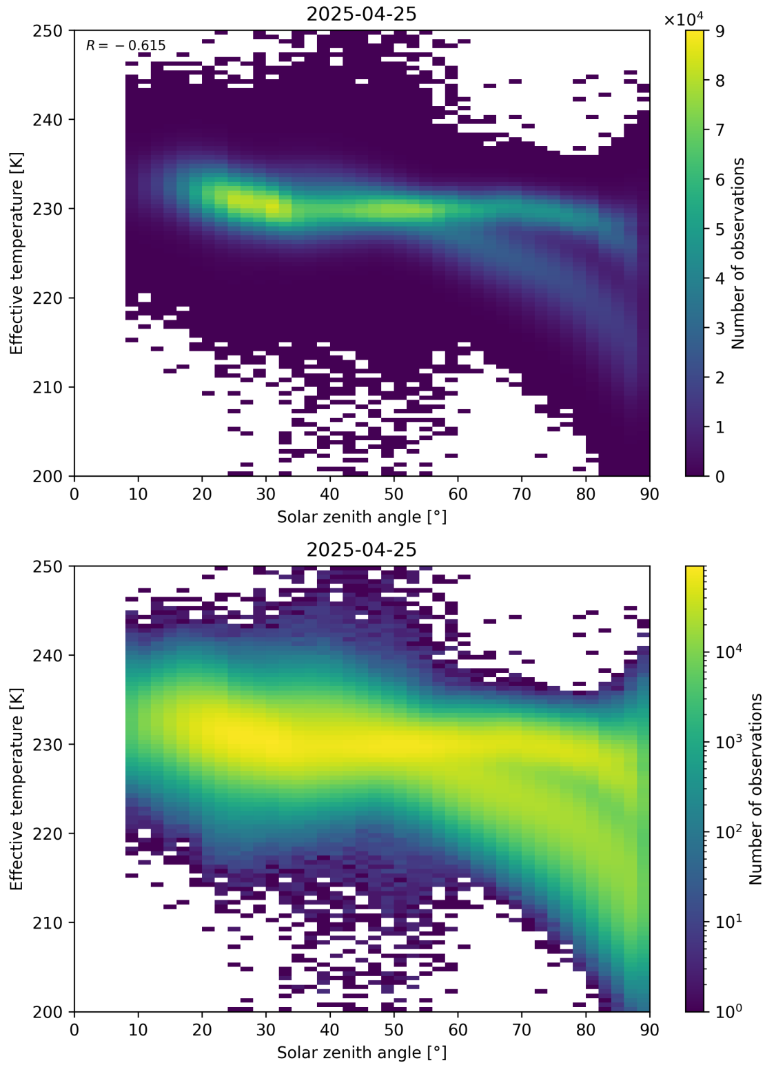
Figure 45: Scatter density plot of “Solar zenith angle” against “Effective temperature” for 2025-04-24 to 2025-04-26.
