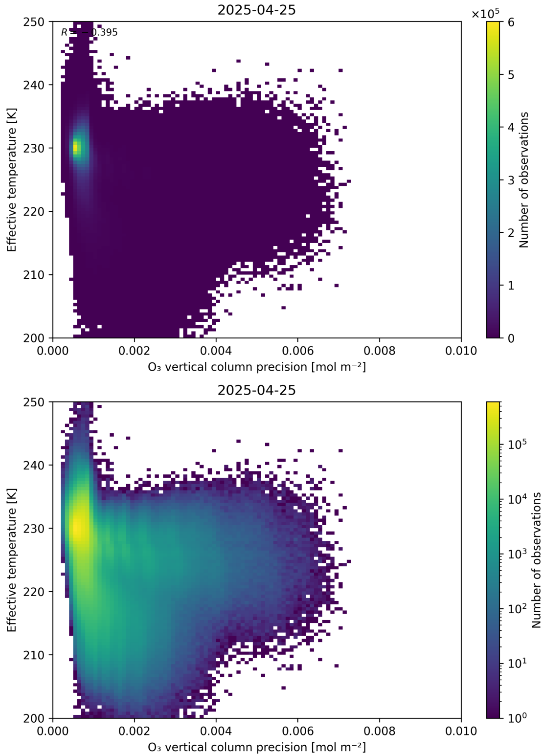
Figure 42: Scatter density plot of “O 3 vertical column precision” against “Effective temperature” for 2025-04-24 to 2025-04-26.
