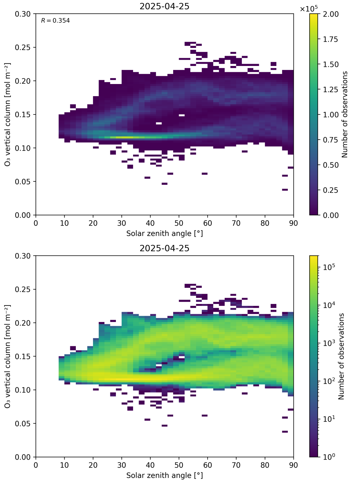
Figure 47: Scatter density plot of “Solar zenith angle” against “O 3 vertical column” for 2025-04-24 to 2025-04-26.
