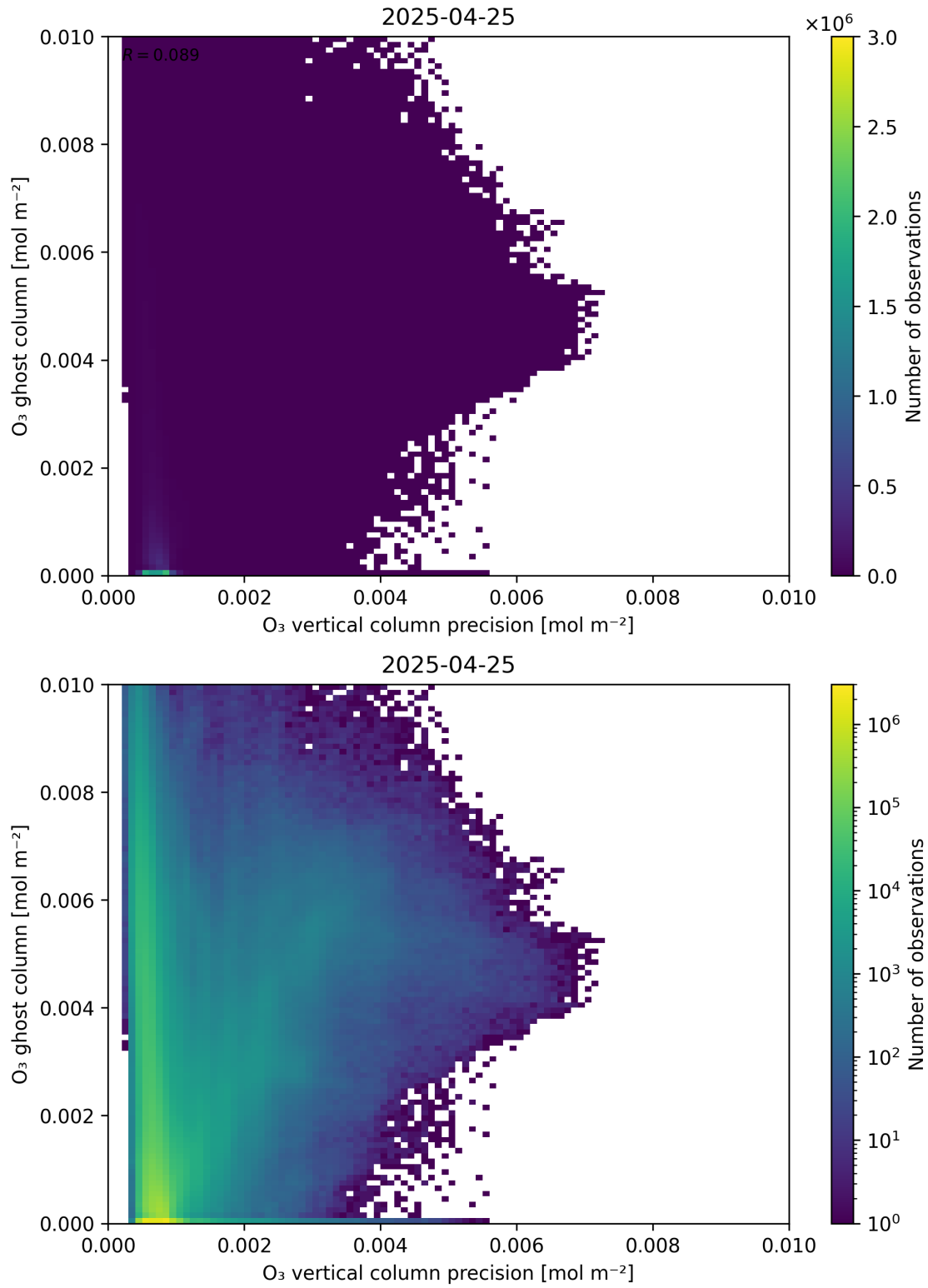
Figure 43: Scatter density plot of “ \text{O}_3 vertical column precision” against “ \text{O}_3 ghost column” for 2025-04-24 to 2025-04-26.
