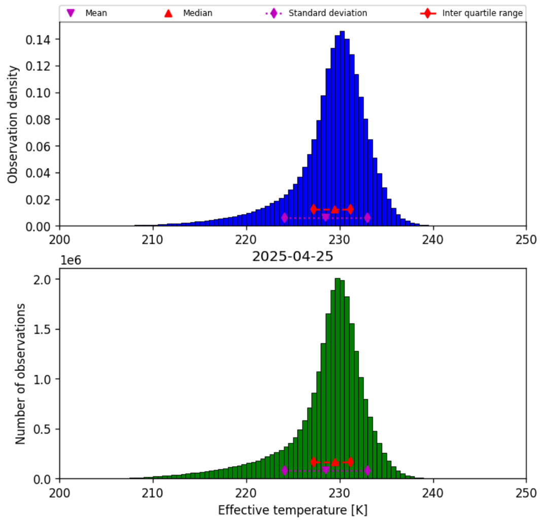
Figure 24: Histogram of “Effective temperature” for 2025-04-24 to 2025-04-26
