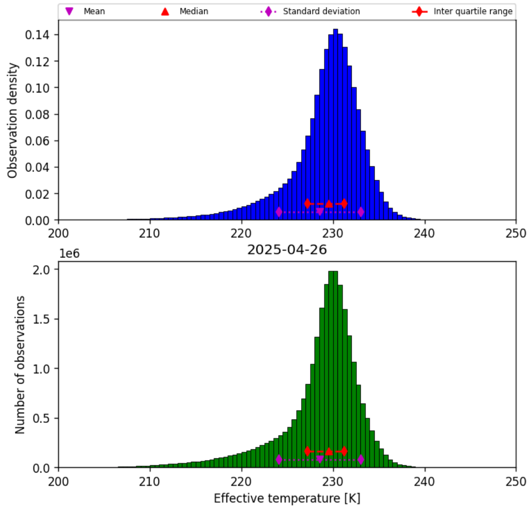
Figure 24: Histogram of “Effective temperature” for 2025-04-25 to 2025-04-27
