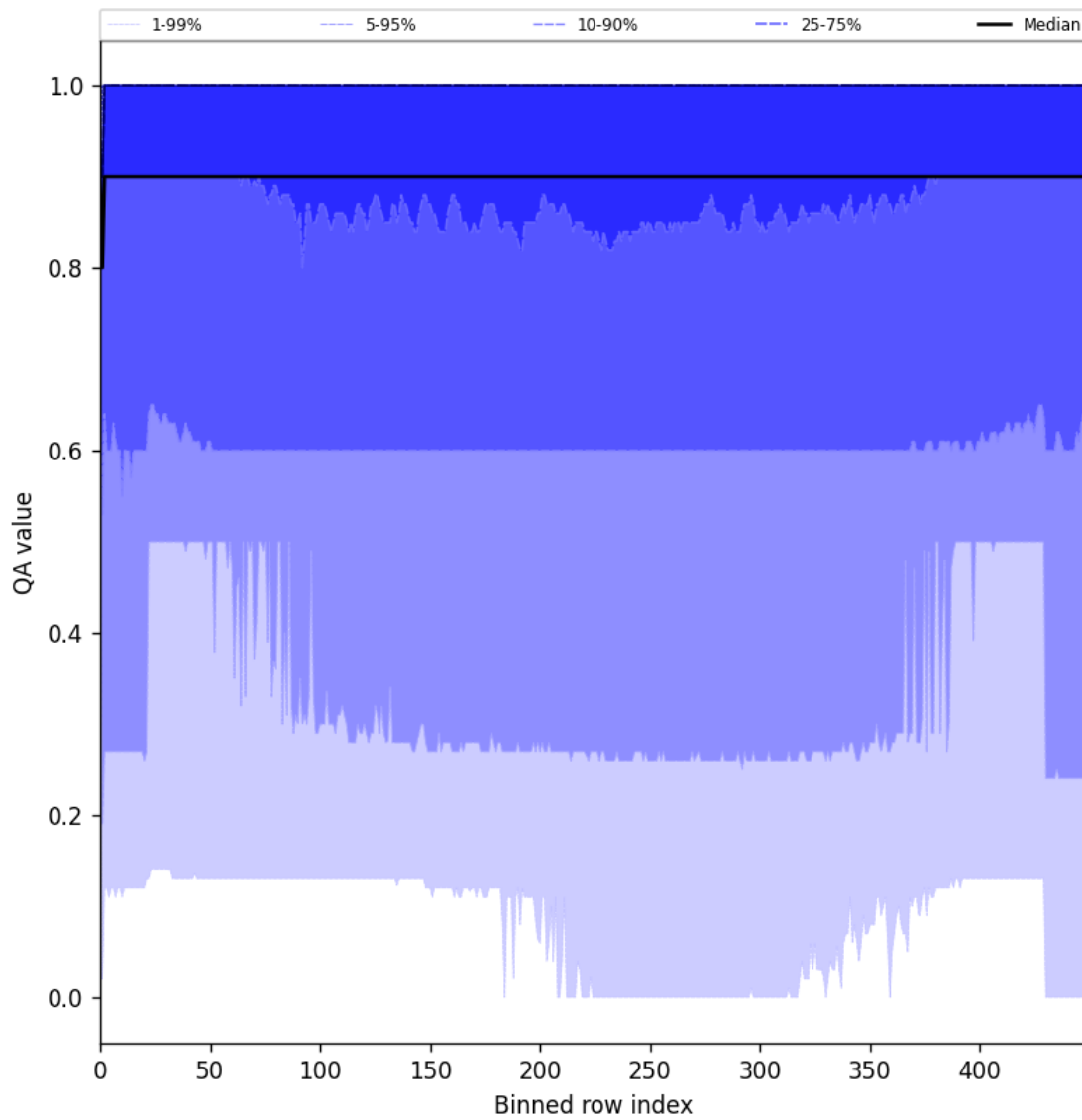
Figure 27: Along track statistics of “QA value” for 2025-04-25 to 2025-04-27
