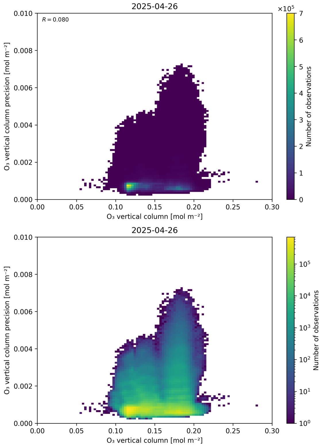
Figure 41: Scatter density plot of “O 3 vertical column” against “O 3 vertical column precision” for 2025-04-25 to 2025-04-27.
