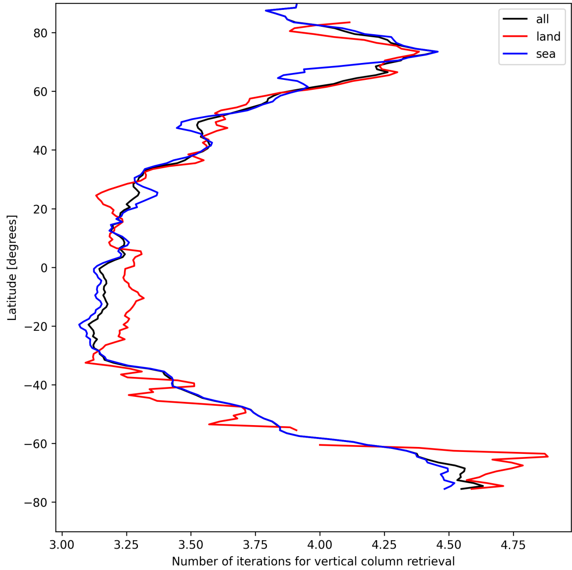
Figure 19: Zonal average of “Number of iterations for vertical column retrieval” for 2025-04-25 to 2025-04-27.
