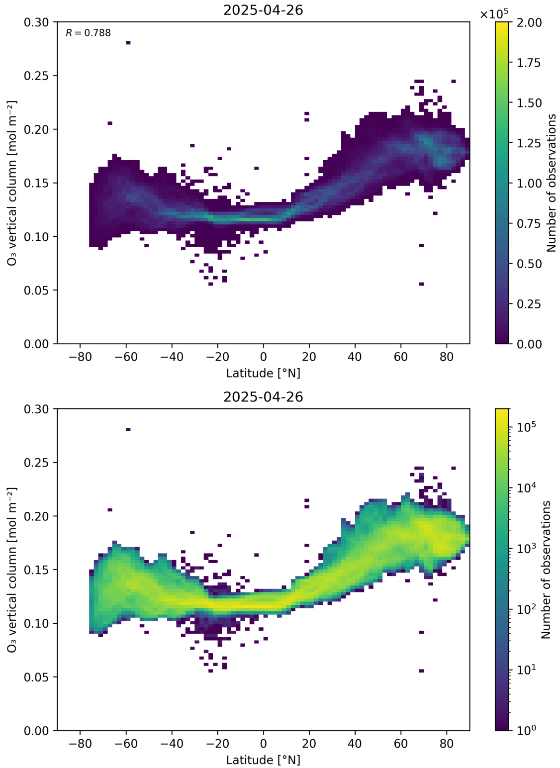
Figure 36: Scatter density plot of “Latitude” against “O 3 vertical column” for 2025-04-25 to 2025-04-27.
