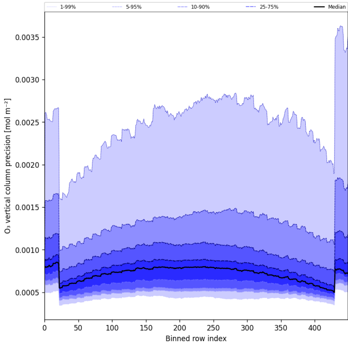
Figure 29: Along track statistics of “O 3 vertical column precision” for 2025-04-25 to 2025-04-27
