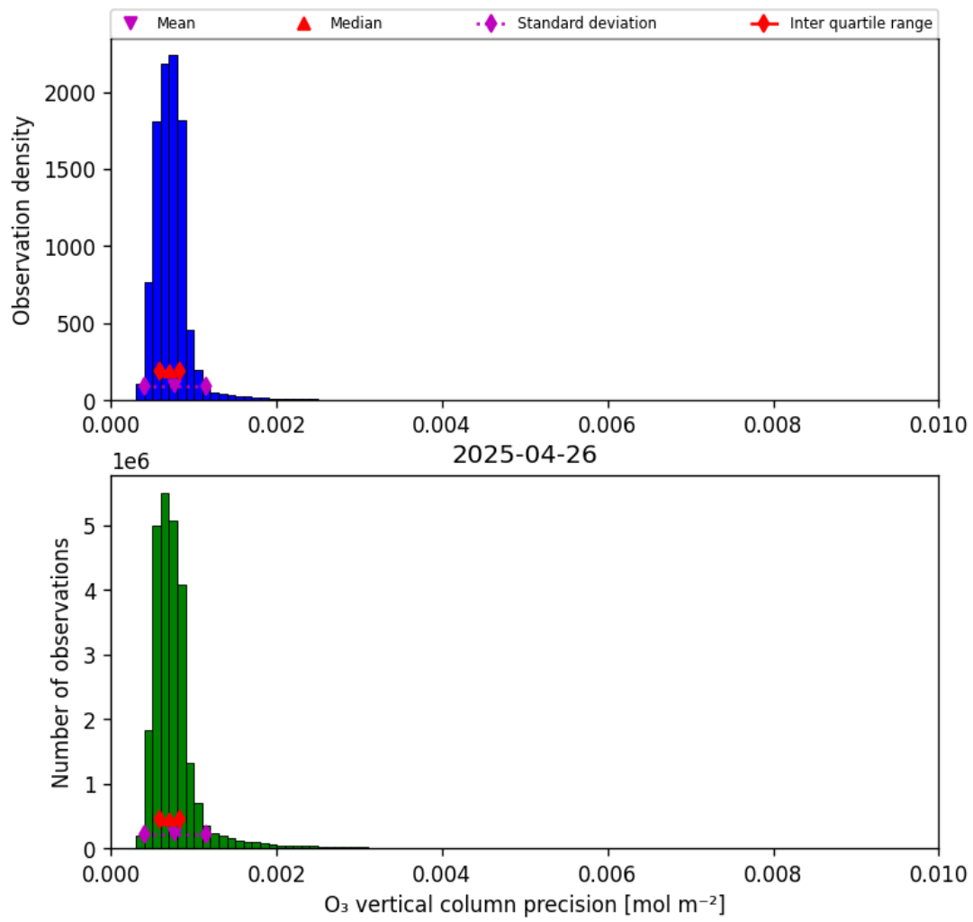
Figure 22: Histogram of “O 3 vertical column precision” for 2025-04-25 to 2025-04-27
