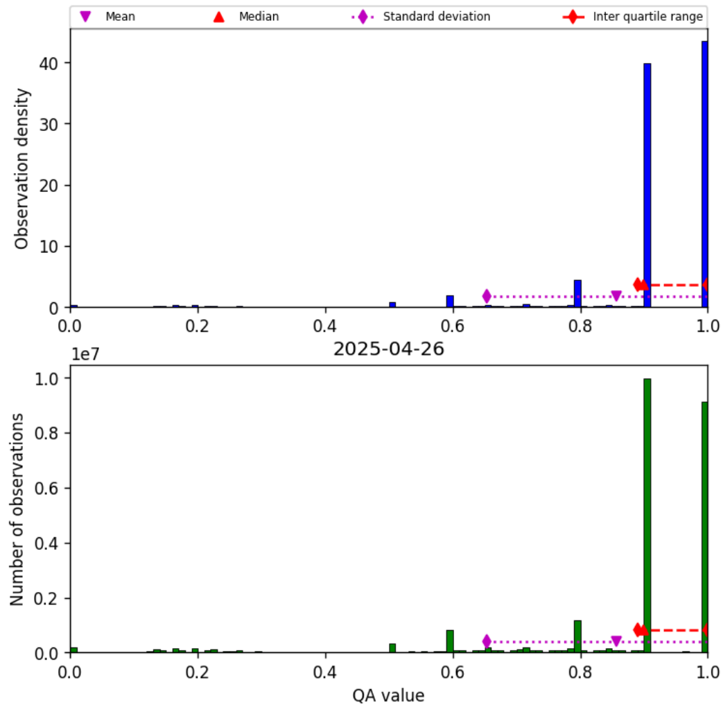
Figure 20: Histogram of “QA value” for 2025-04-25 to 2025-04-27
