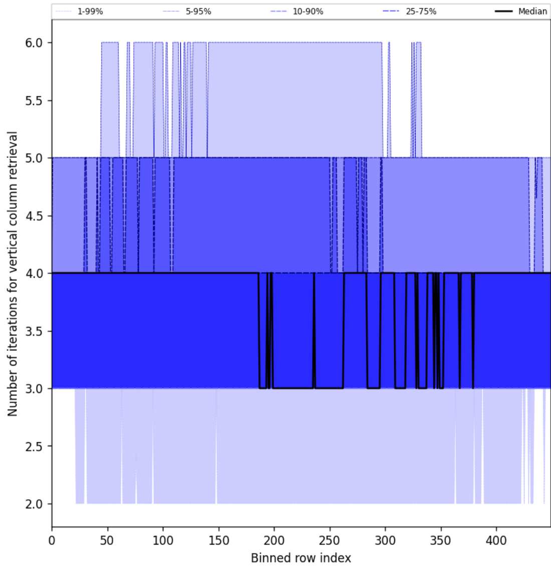
Figure 33: Along track statistics of “Number of iterations for vertical column retrieval” for 2025-04-25 to 2025-04-27
