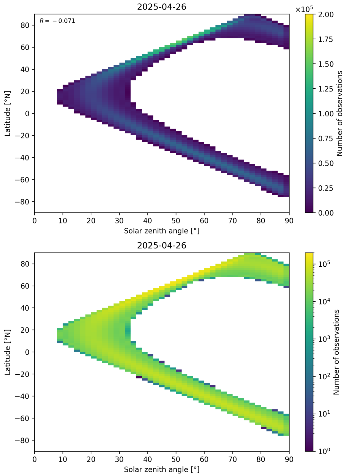
Figure 44: Scatter density plot of “Solar zenith angle” against “Latitude” for 2025-04-25 to 2025-04-27.
