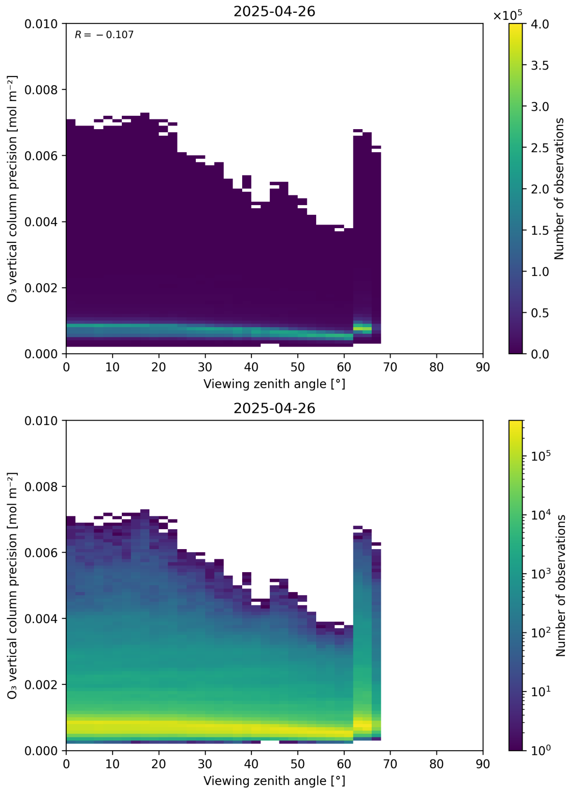
Figure 53: Scatter density plot of “Viewing zenith angle” against “O 3 vertical column precision” for 2025-04-25 to 2025-04-27.
