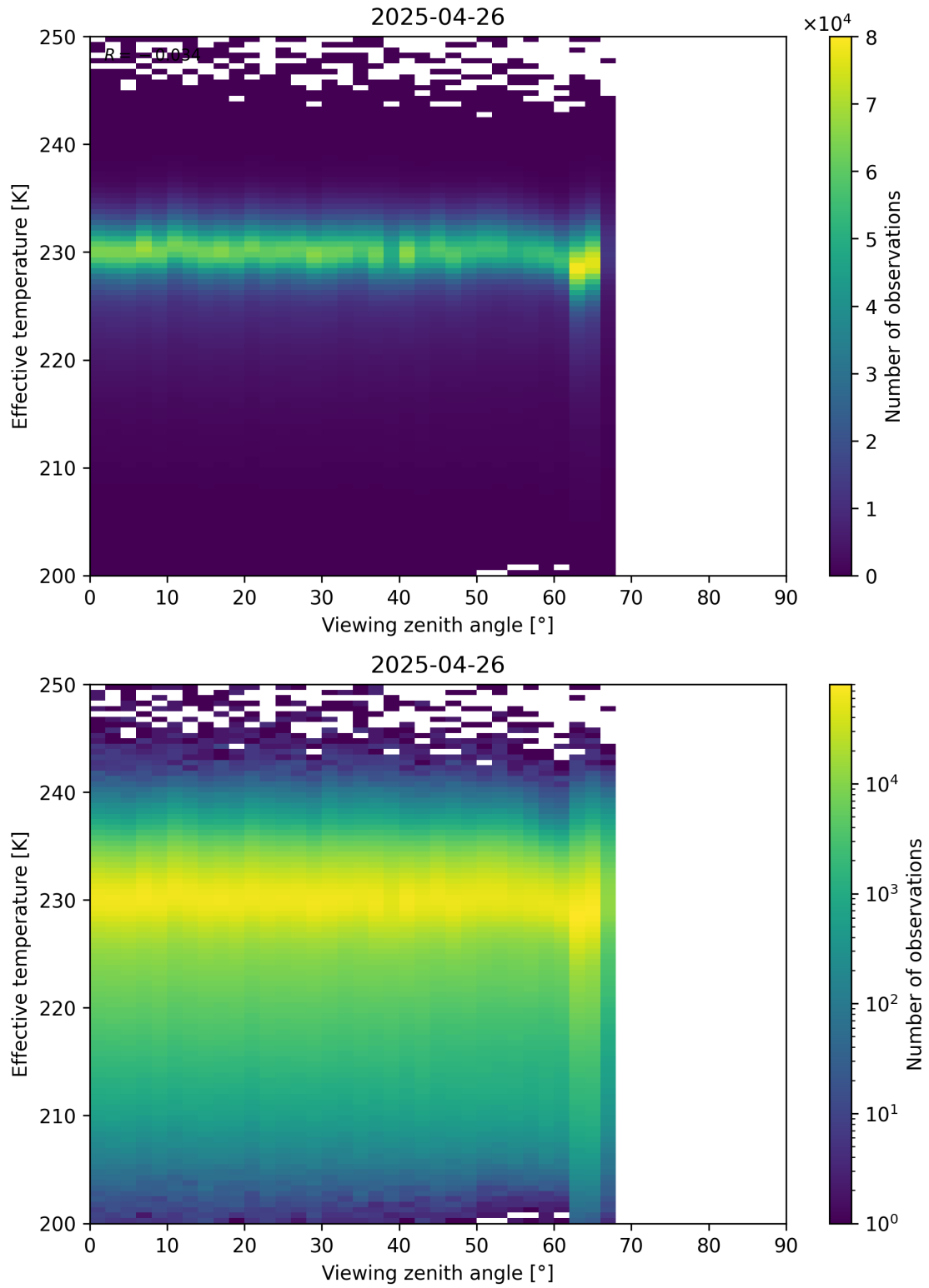
Figure 50: Scatter density plot of “Viewing zenith angle” against “Effective temperature” for 2025-04-25 to 2025-04-27.
