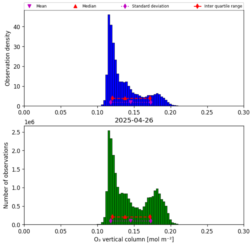
Figure 21: Histogram of “O 3 vertical column” for 2025-04-25 to 2025-04-27
