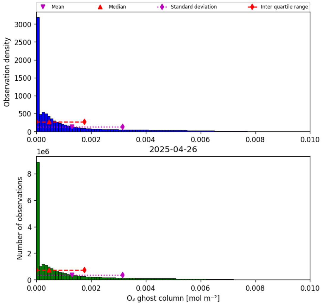
Figure 25: Histogram of “O 3 ghost column” for 2025-04-25 to 2025-04-27
