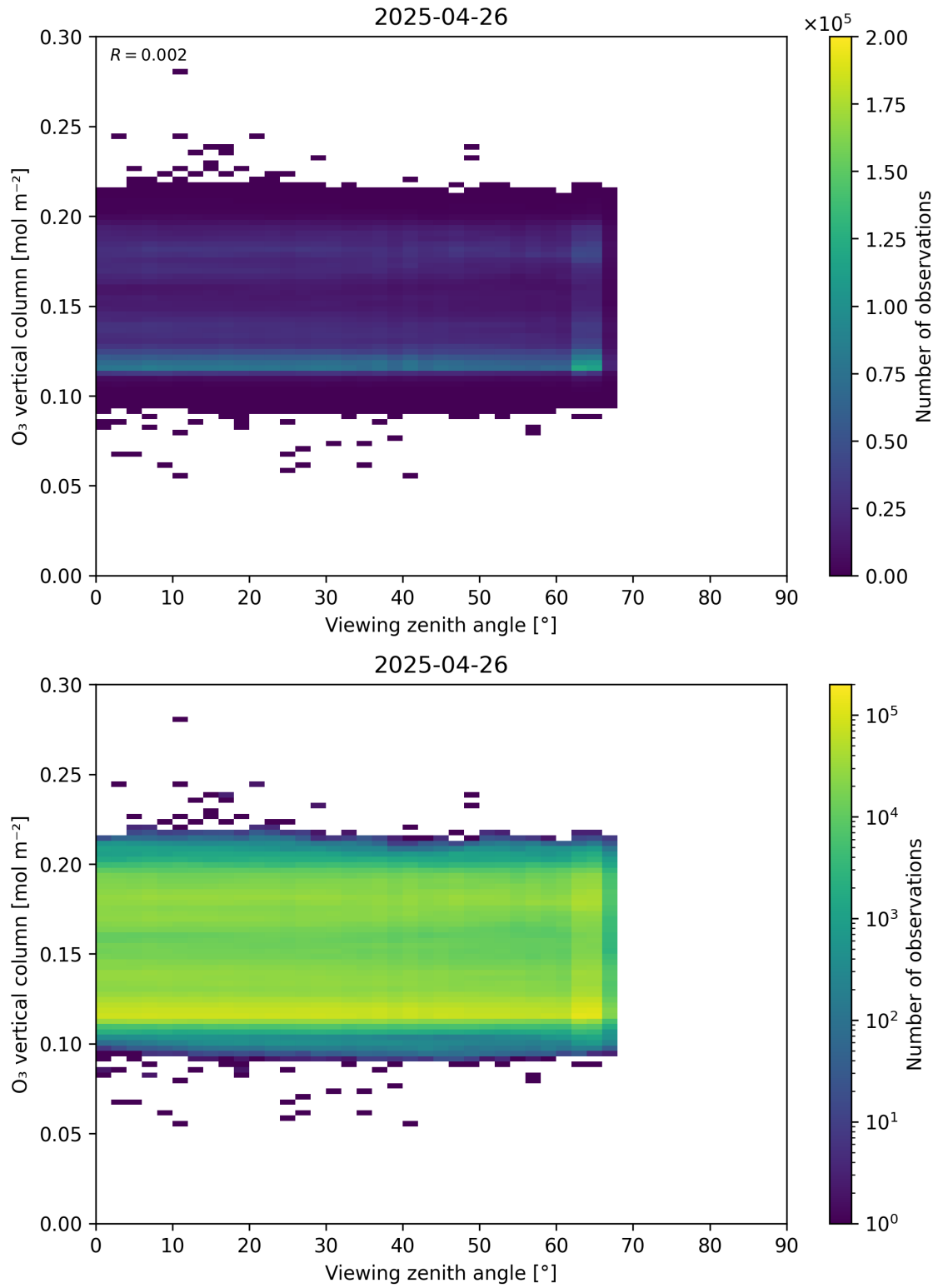
Figure 52: Scatter density plot of “Viewing zenith angle” against “O 3 vertical column” for 2025-04-25 to 2025-04-27.
