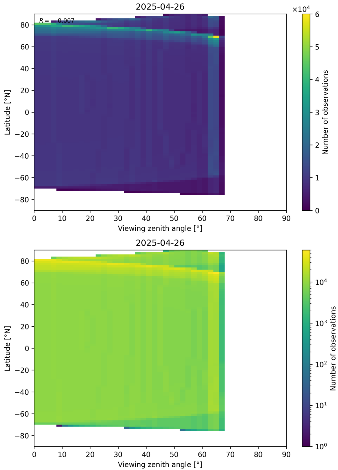
Figure 49: Scatter density plot of “Viewing zenith angle” against “Latitude” for 2025-04-25 to 2025-04-27.
