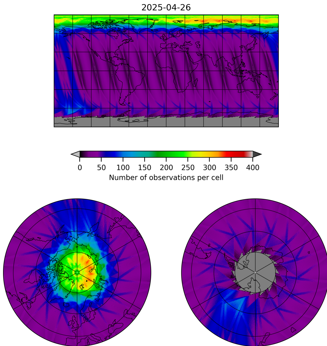
Figure 12: Map of the number of observations for 2025-04-25 to 2025-04-27
