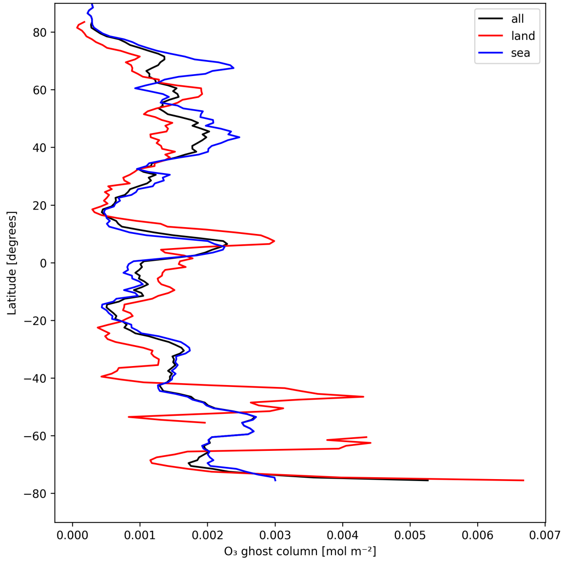
Figure 18: Zonal average of “O 3 ghost column” for 2025-04-25 to 2025-04-27.
