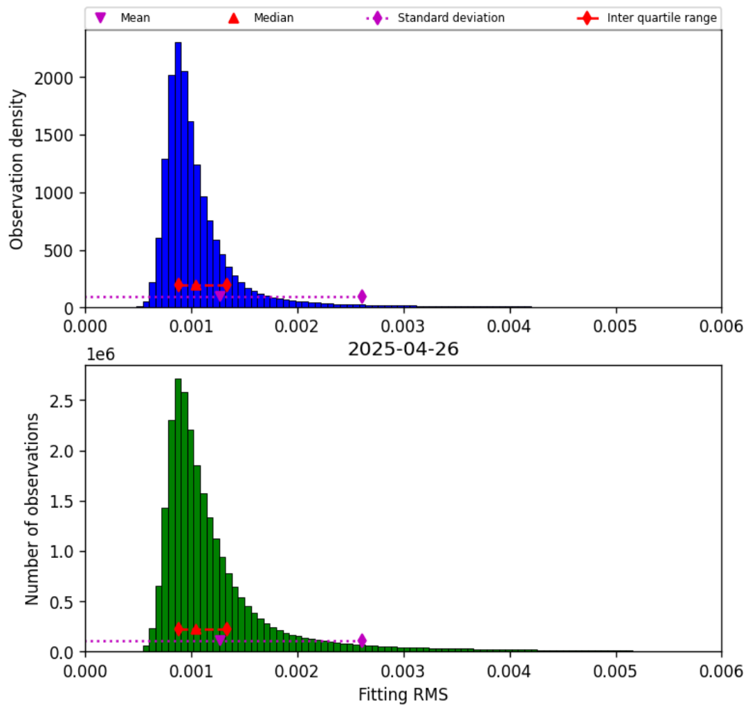
Figure 23: Histogram of “Fitting RMS” for 2025-04-25 to 2025-04-27
