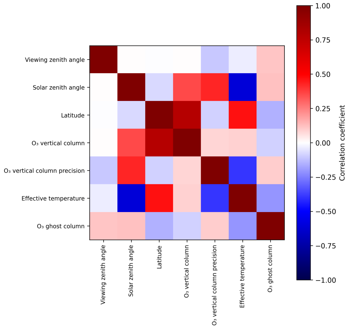
Figure 2: Map of correlation matrix for 2025-04-25 to 2025-04-27.
