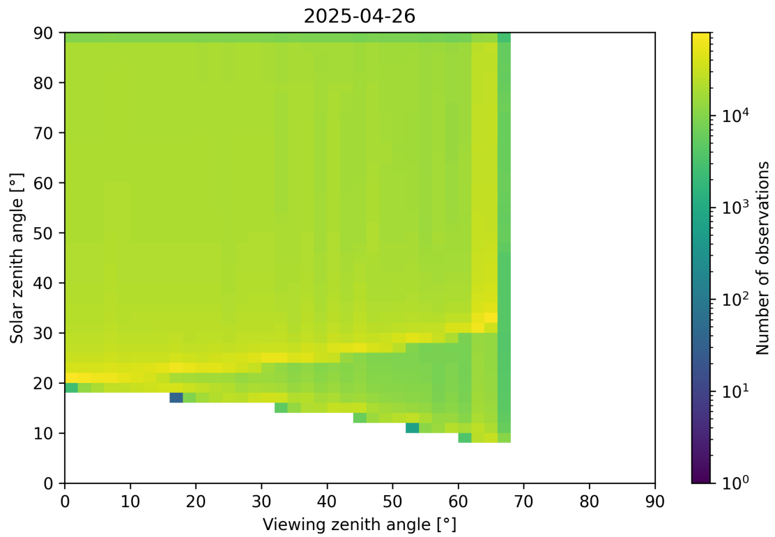
Figure 54: Scatter density plot of “Viewing zenith angle” against “Solar zenith angle” for 2025-04-25 to 2025-04-27.
