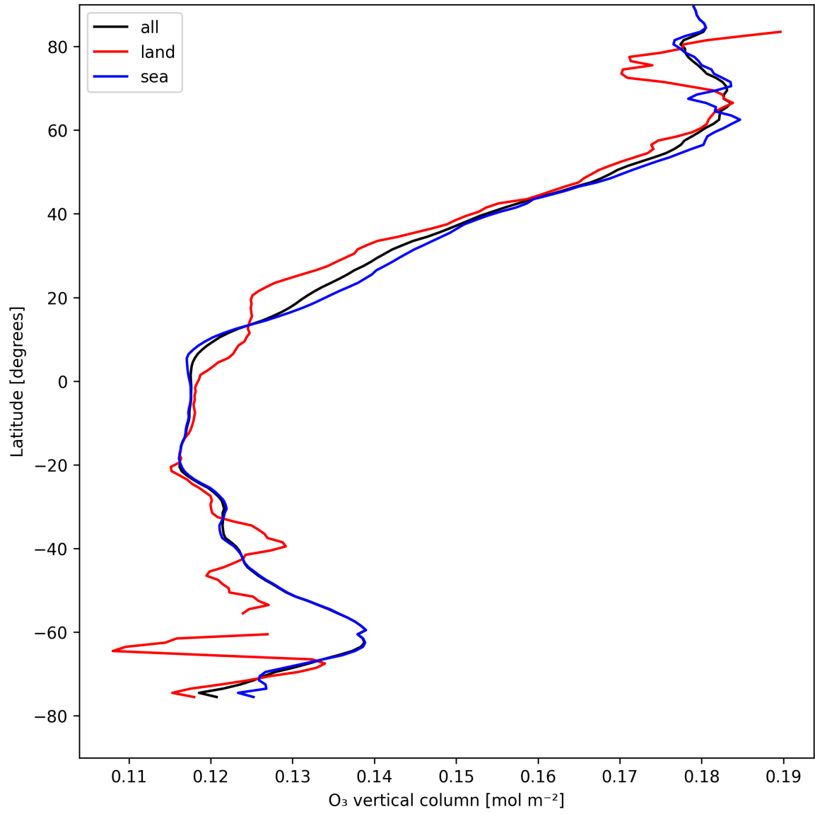
Figure 14: Zonal average of “O 3 vertical column” for 2025-04-25 to 2025-04-27.
