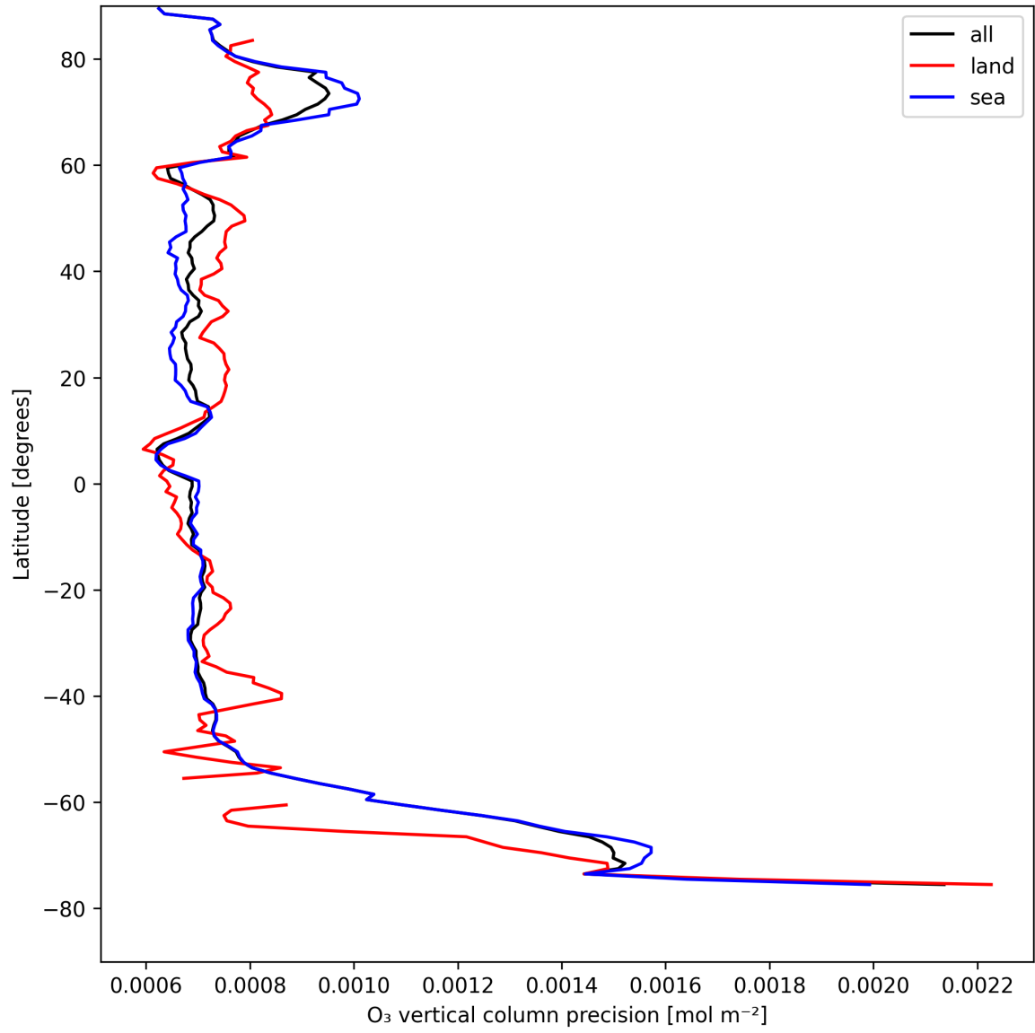
Figure 15: Zonal average of "O 3 vertical column precision" for 2025-04-25 to 2025-04-27.
