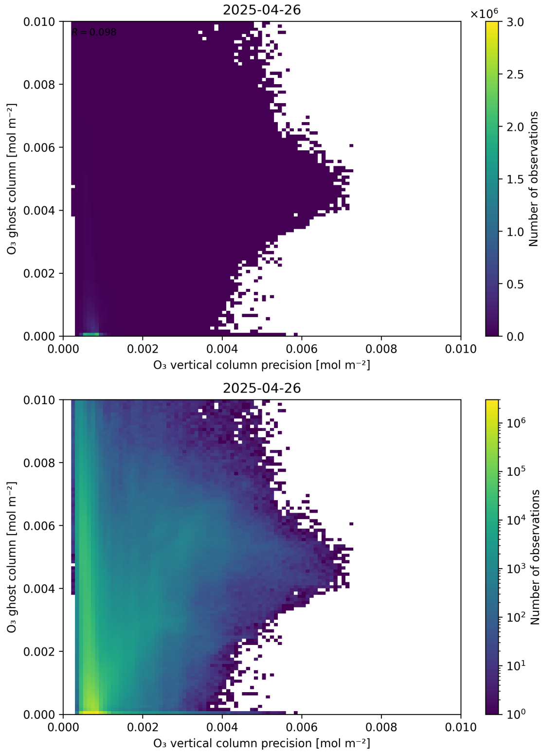
Figure 43: Scatter density plot of “ \text{O}_3 vertical column precision” against “ \text{O}_3 ghost column” for 2025-04-25 to 2025-04-27.
