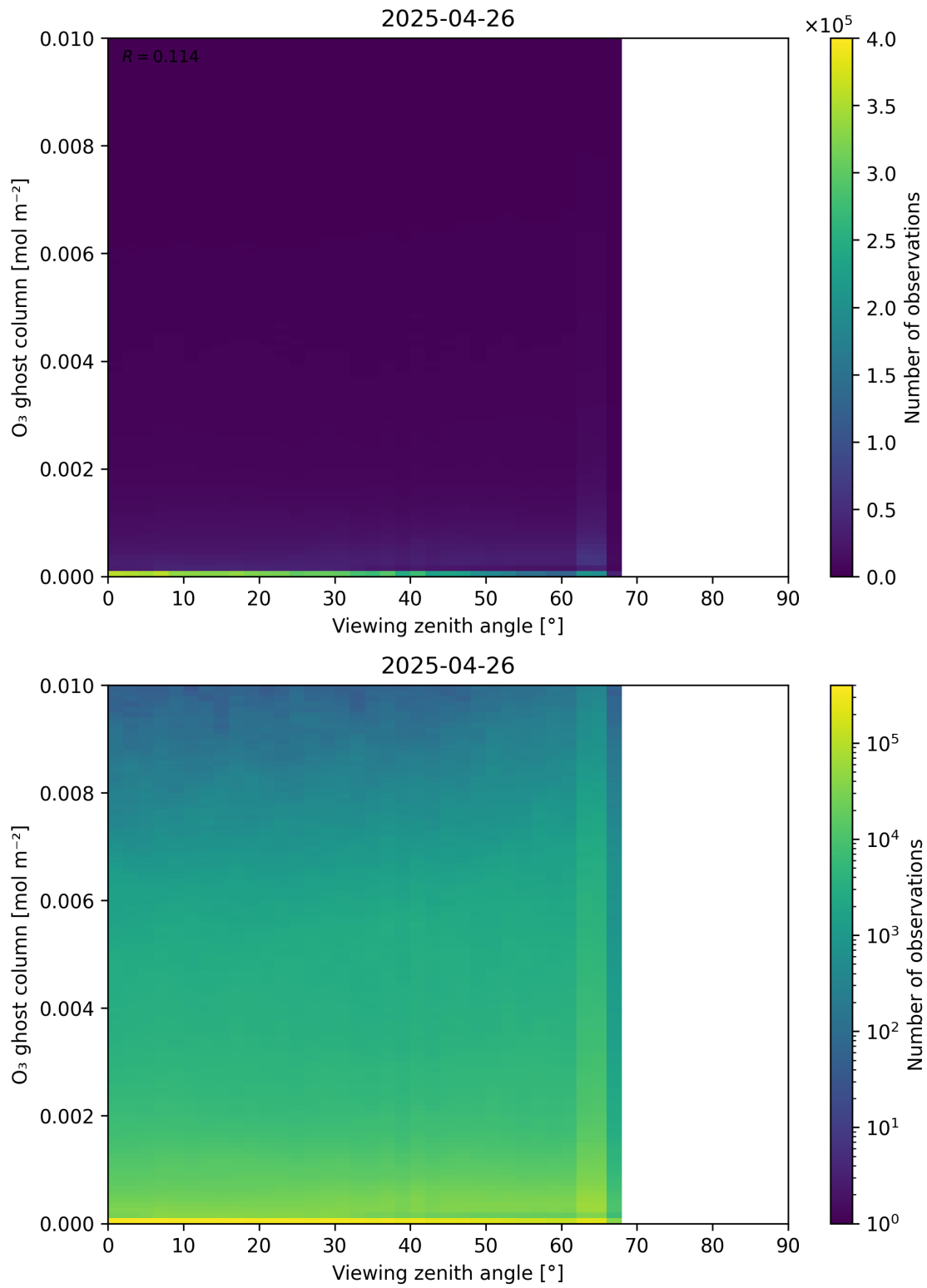
Figure 51: Scatter density plot of “Viewing zenith angle” against “O 3 ghost column” for 2025-04-25 to 2025-04-27.
