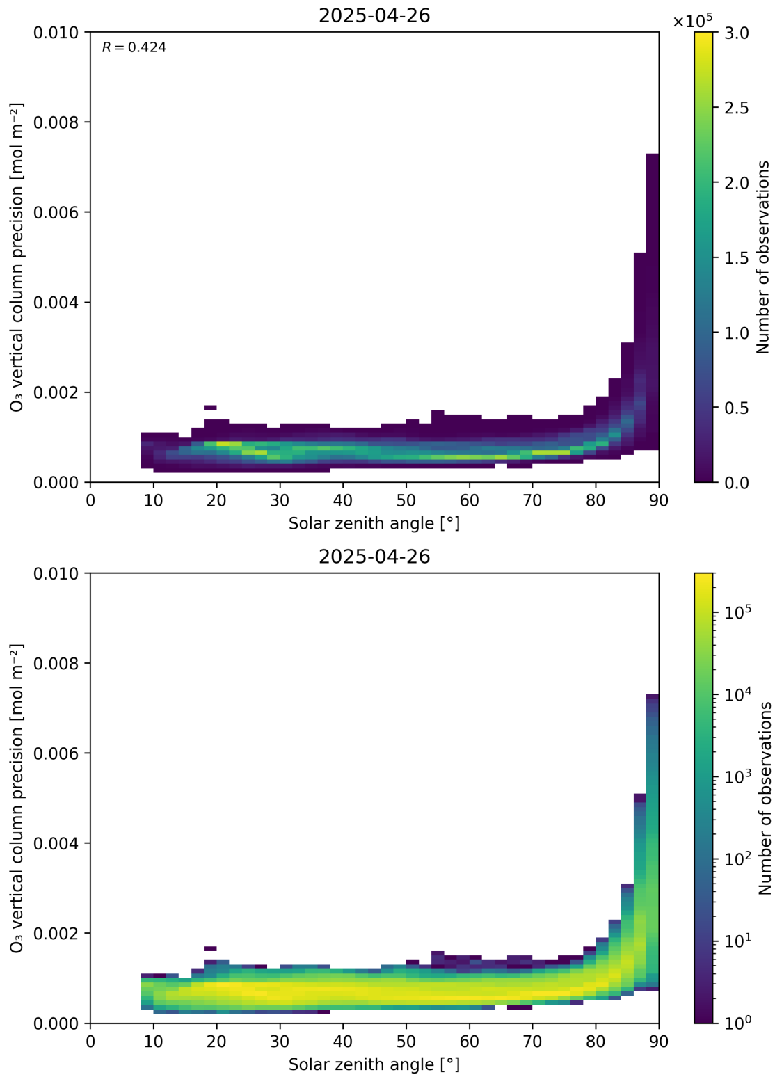
Figure 48: Scatter density plot of “Solar zenith angle” against “O 3 vertical column precision” for 2025-04-25 to 2025-04-27.
