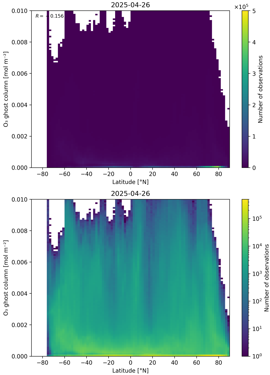
Figure 35: Scatter density plot of “Latitude” against “O 3 ghost column” for 2025-04-25 to 2025-04-27.
