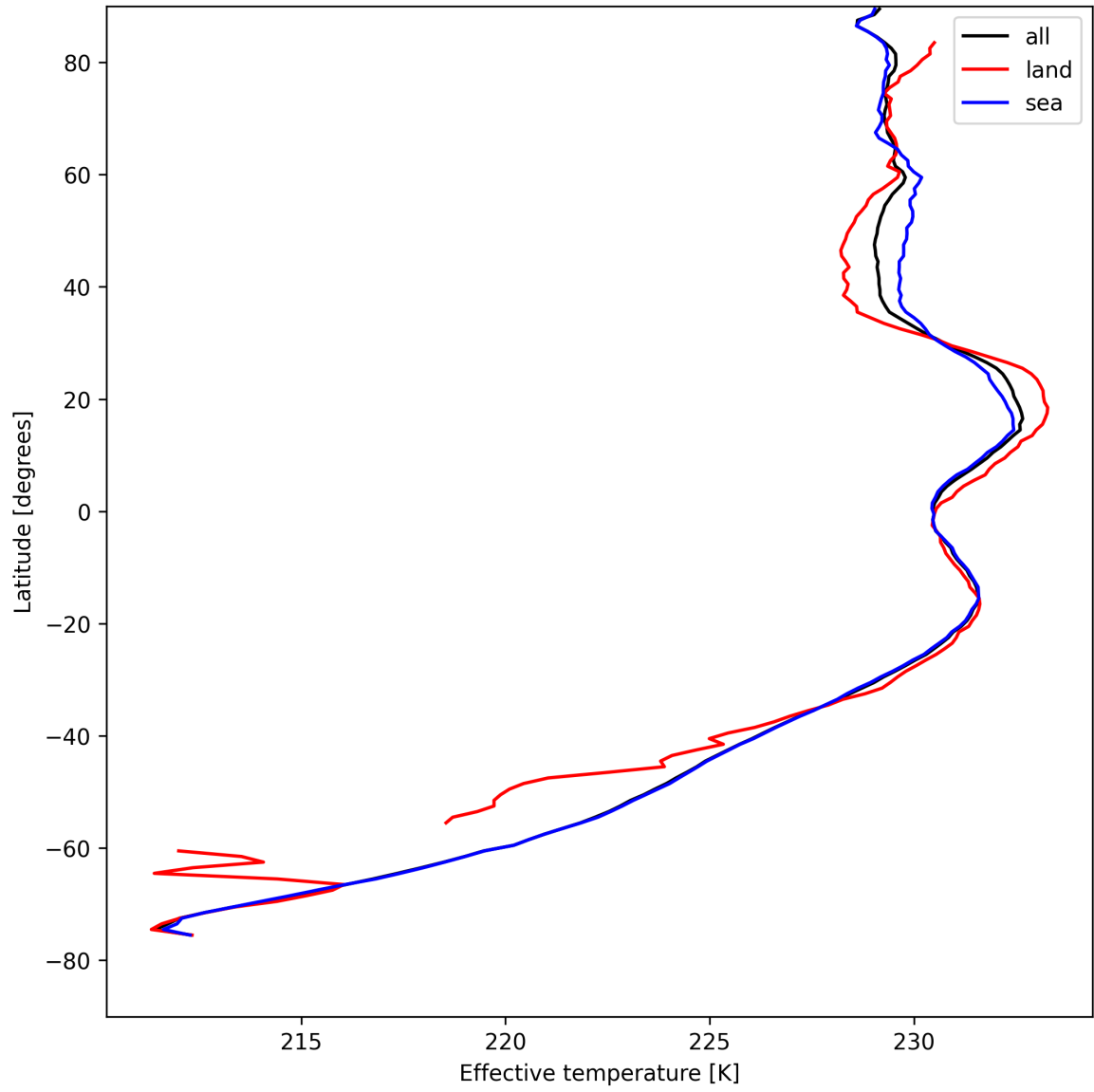
Figure 17: Zonal average of "Effective temperature" for 2025-04-25 to 2025-04-27.
