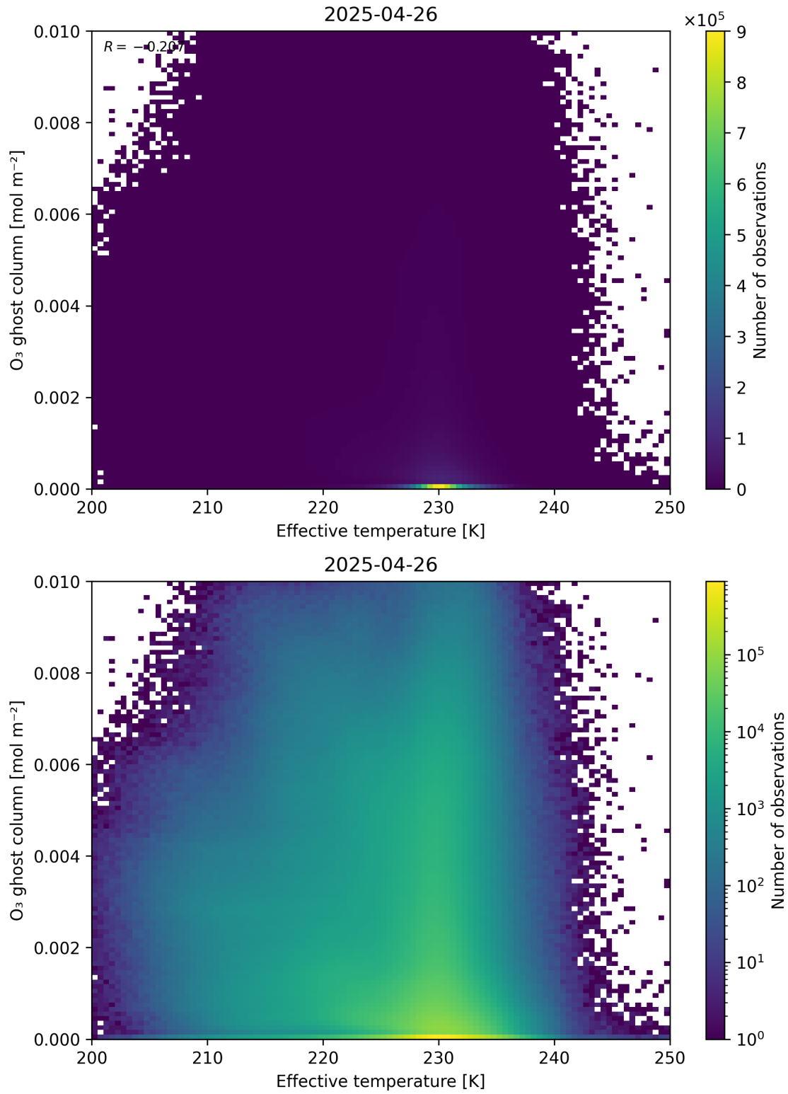
Figure 38: Scatter density plot of “Effective temperature” against “O 3 ghost column” for 2025-04-25 to 2025-04-27.
