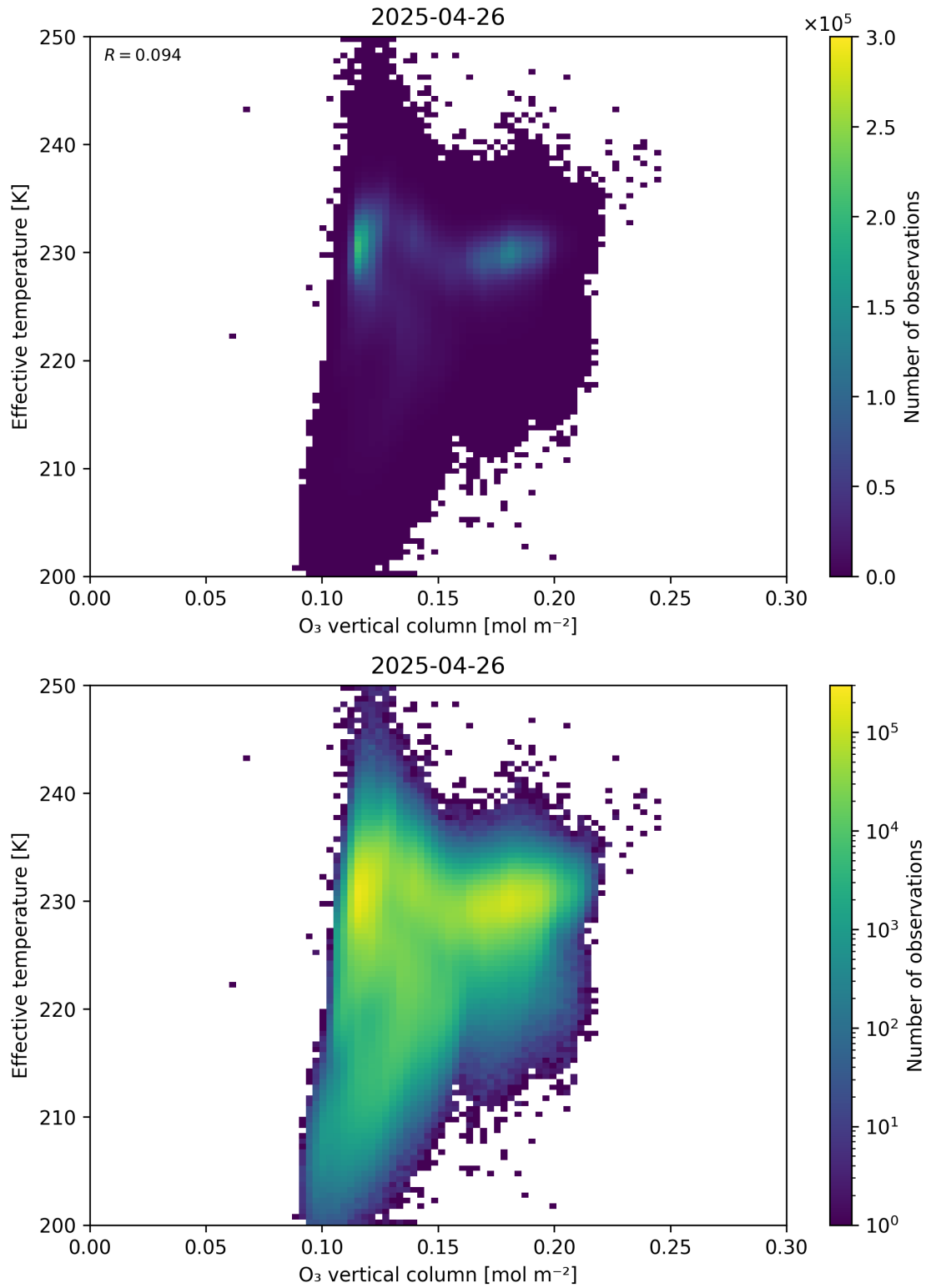
Figure 39: Scatter density plot of “O 3 vertical column” against “Effective temperature” for 2025-04-25 to 2025-04-27.
