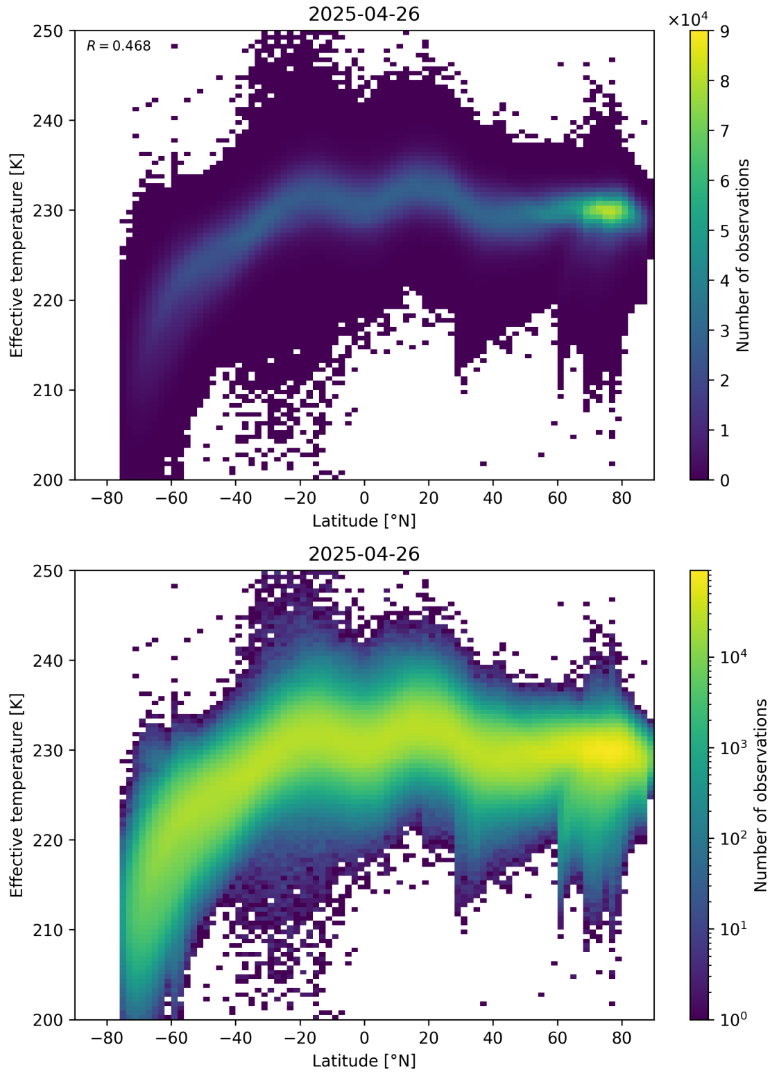
Figure 34: Scatter density plot of “Latitude” against “Effective temperature” for 2025-04-25 to 2025-04-27.
