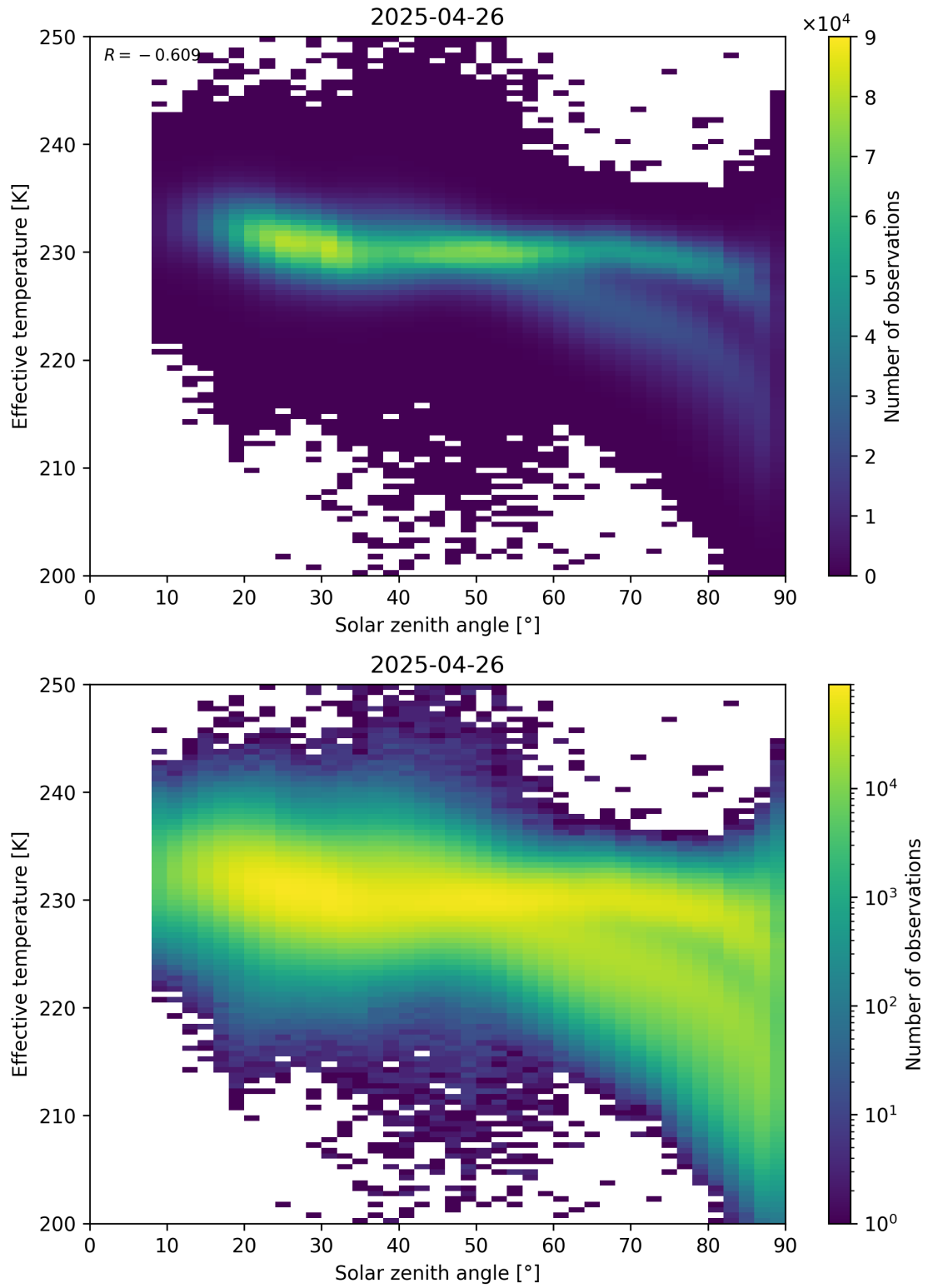
Figure 45: Scatter density plot of “Solar zenith angle” against “Effective temperature” for 2025-04-25 to 2025-04-27.
