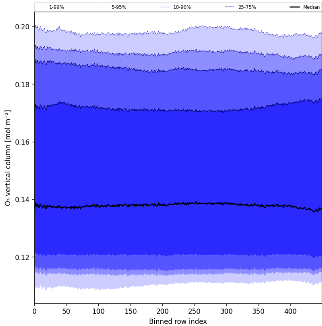
Figure 28: Along track statistics of “ O_3 vertical column” for 2025-04-25 to 2025-04-27
