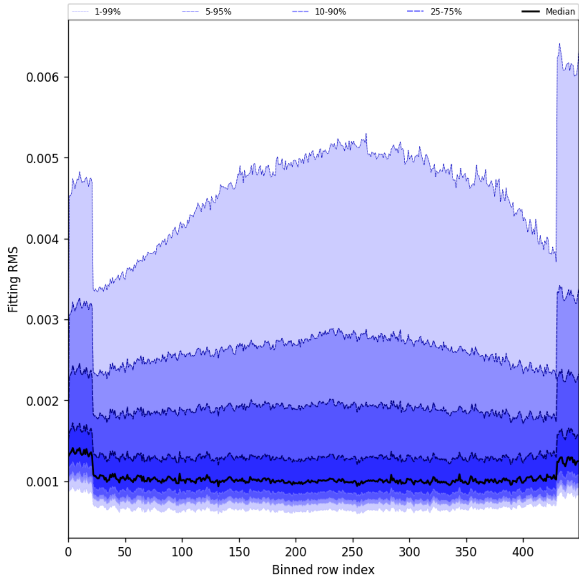
Figure 30: Along track statistics of “Fitting RMS” for 2025-04-25 to 2025-04-27
