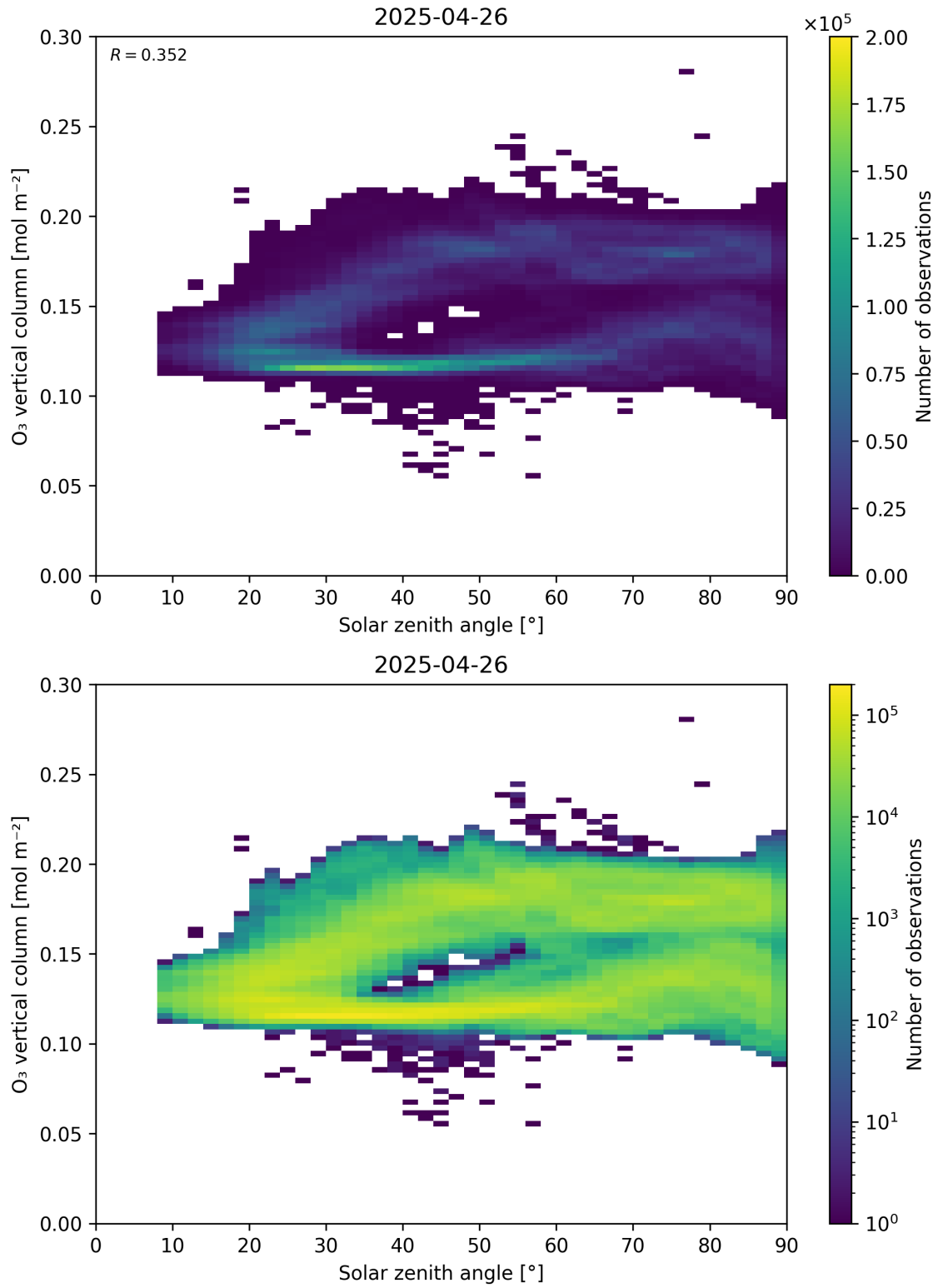
Figure 47: Scatter density plot of “Solar zenith angle” against “O 3 vertical column” for 2025-04-25 to 2025-04-27.
