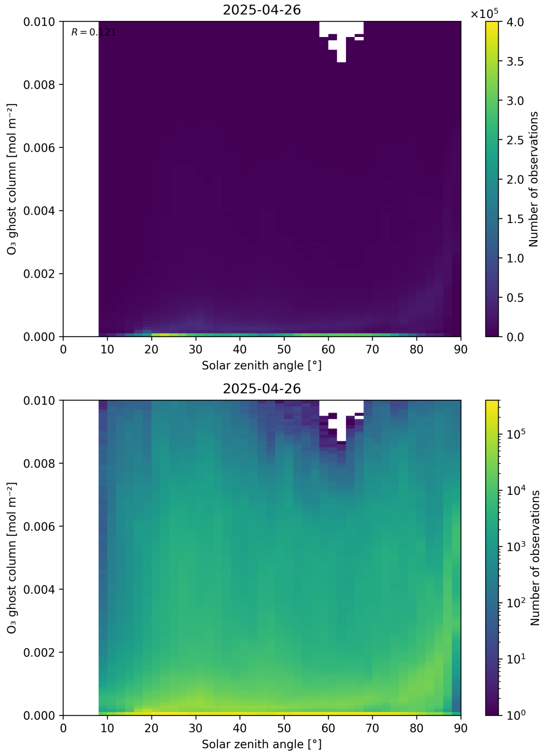
Figure 46: Scatter density plot of “Solar zenith angle” against “O 3 ghost column” for 2025-04-25 to 2025-04-27.
