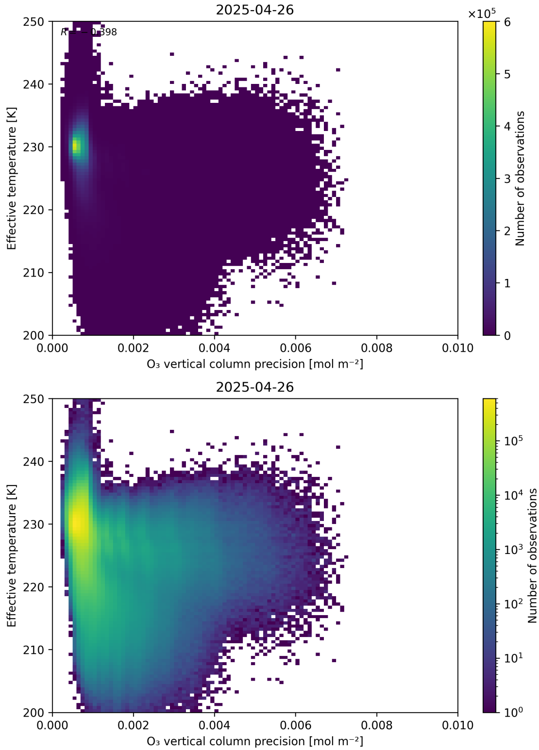
Figure 42: Scatter density plot of “O 3 vertical column precision” against “Effective temperature” for 2025-04-25 to 2025-04-27.
