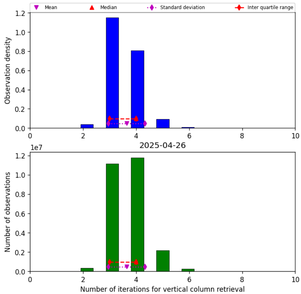
Figure 26: Histogram of “Number of iterations for vertical column retrieval” for 2025-04-25 to 2025-04-27
