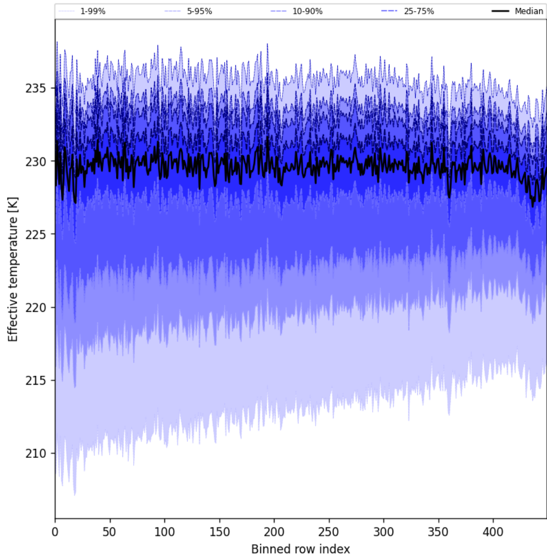
Figure 31: Along track statistics of “Effective temperature” for 2025-04-25 to 2025-04-27
