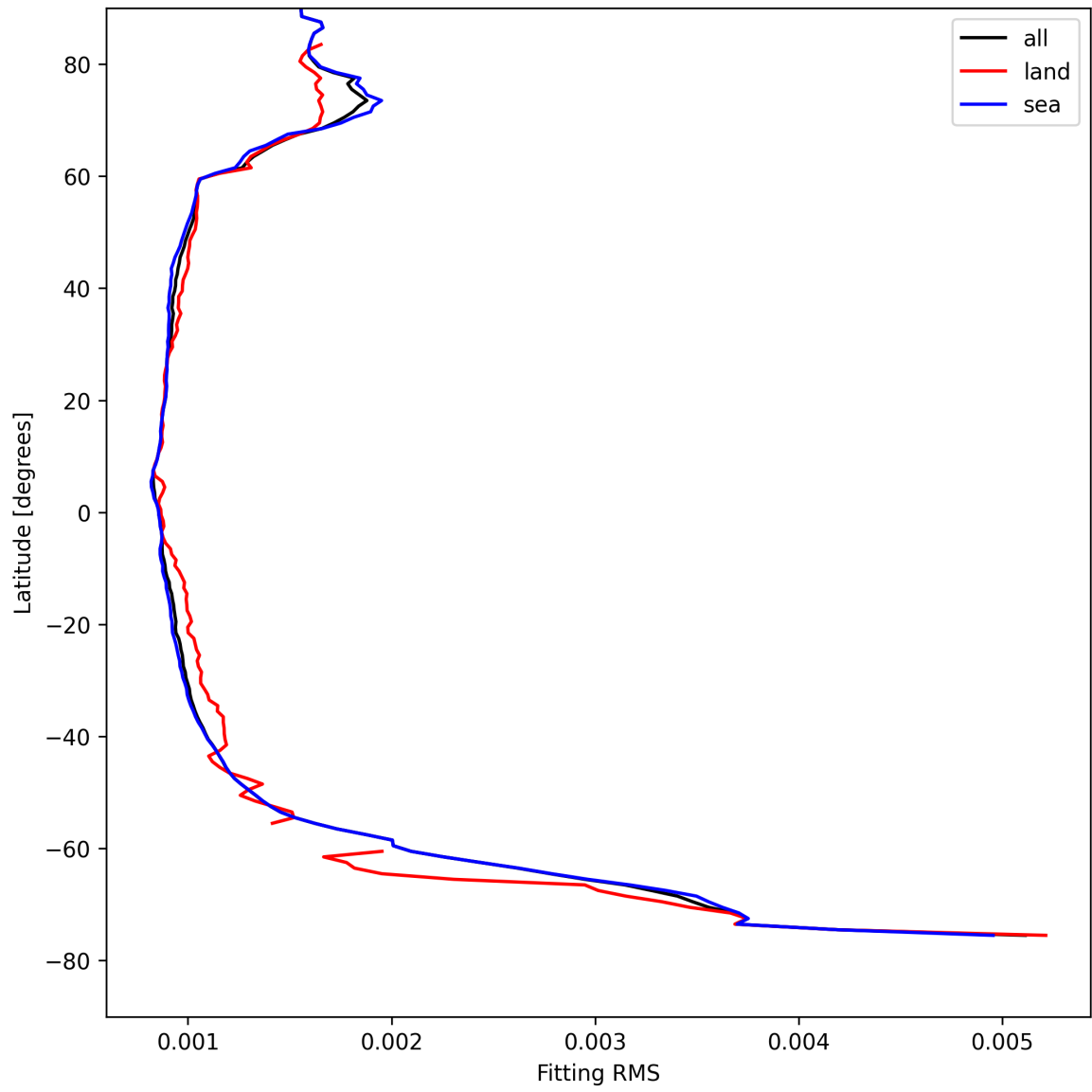
Figure 16: Zonal average of “Fitting RMS” for 2025-04-25 to 2025-04-27.
