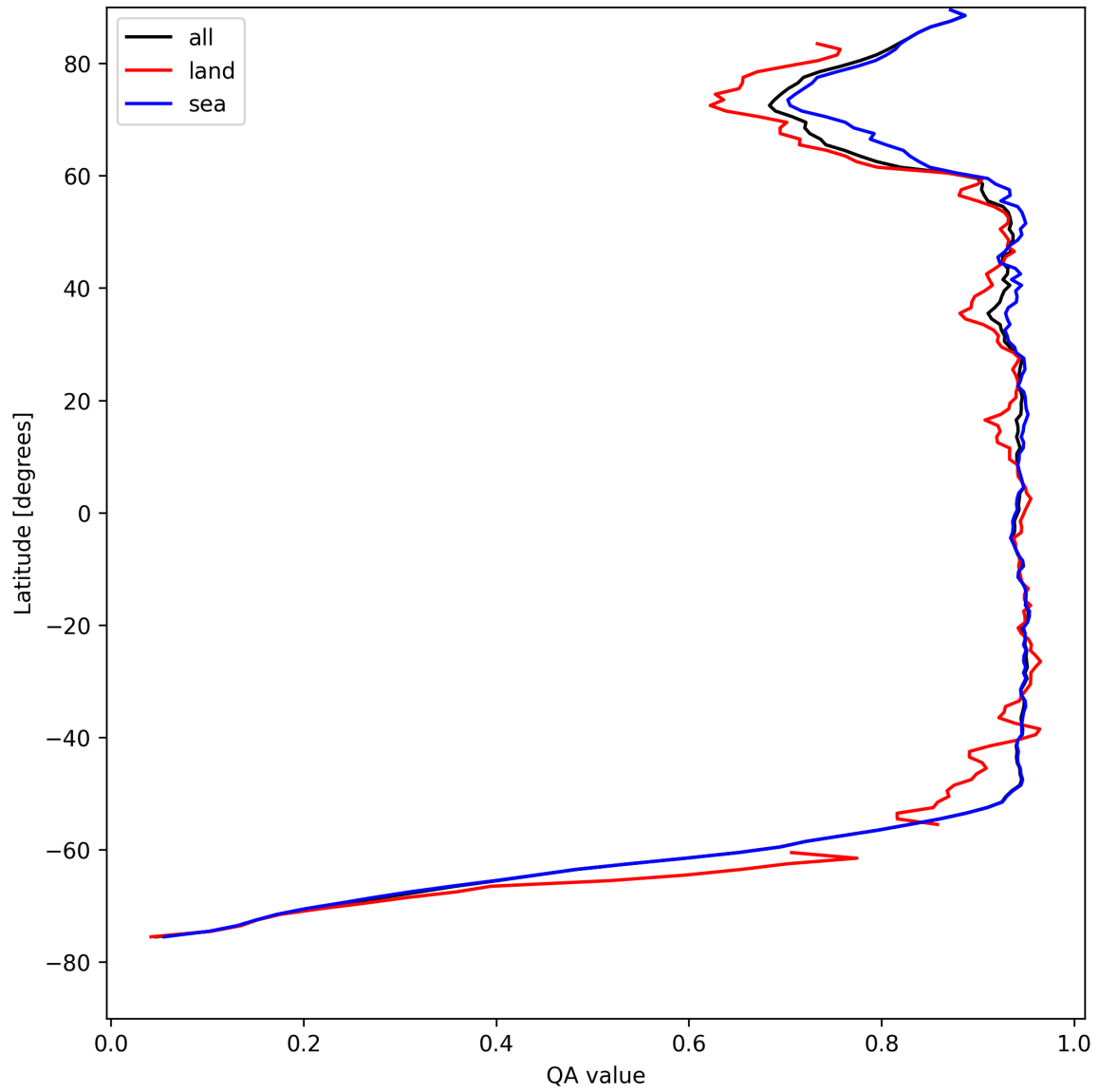
Figure 13: Zonal average of “QA value” for 2025-04-25 to 2025-04-27.
