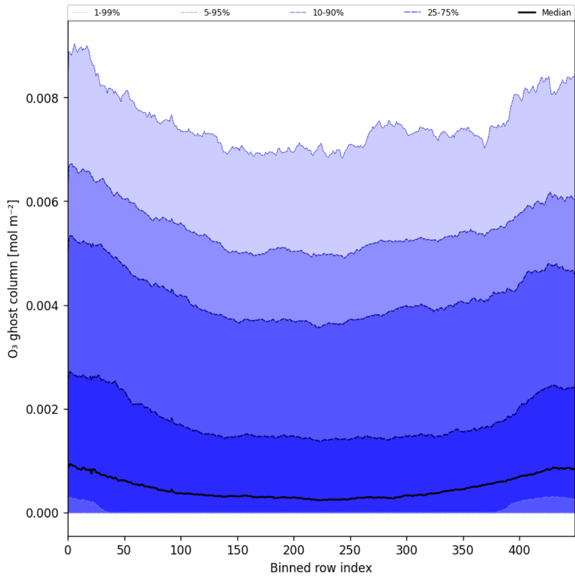
Figure 32: Along track statistics of “O 3 ghost column” for 2025-04-25 to 2025-04-27
