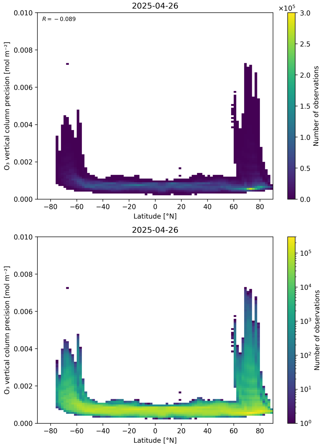
Figure 37: Scatter density plot of “Latitude” against “O 3 vertical column precision” for 2025-04-25 to 2025-04-27.
