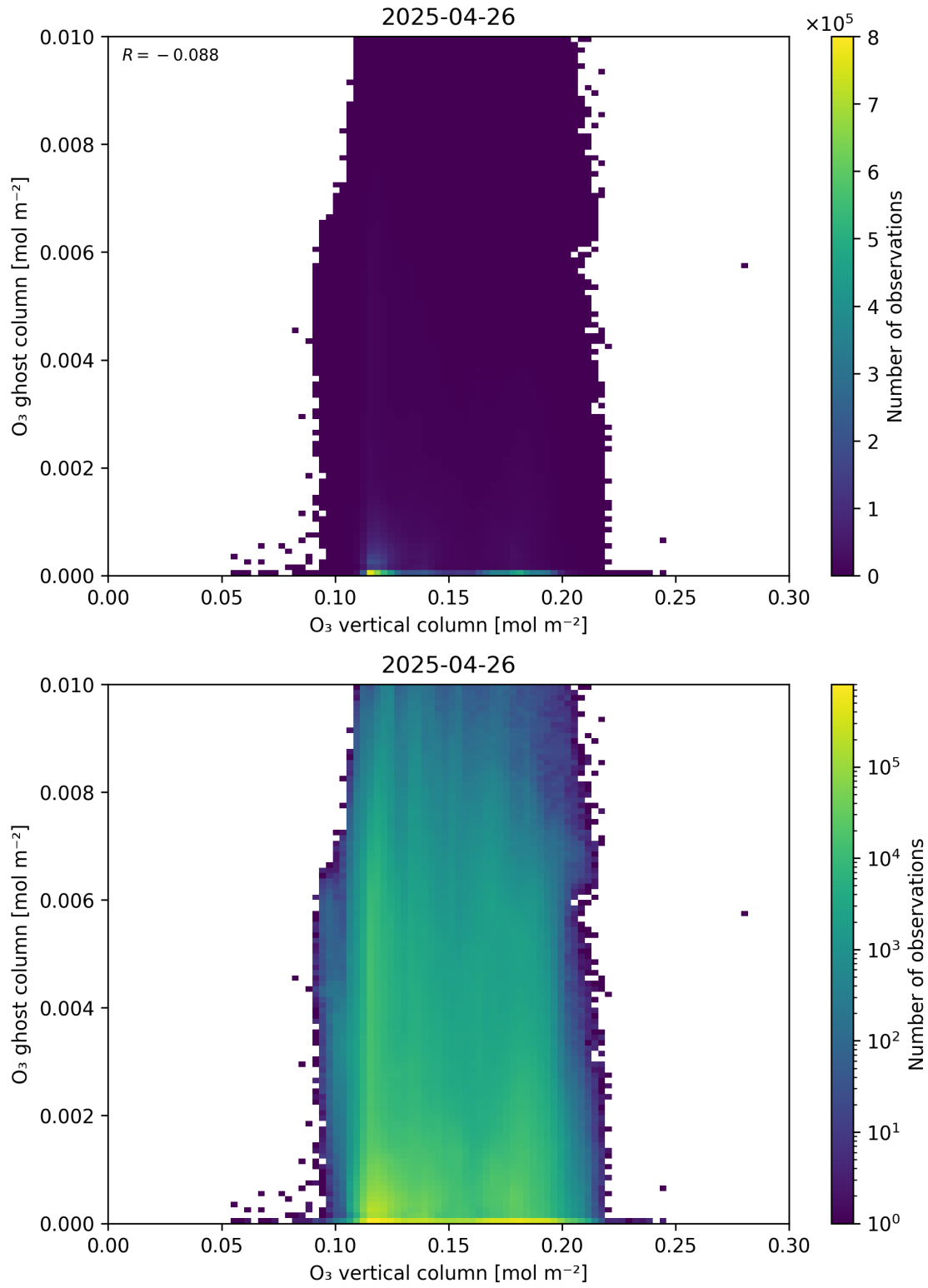
Figure 40: Scatter density plot of “O 3 vertical column” against “O 3 ghost column” for 2025-04-25 to 2025-04-27.
