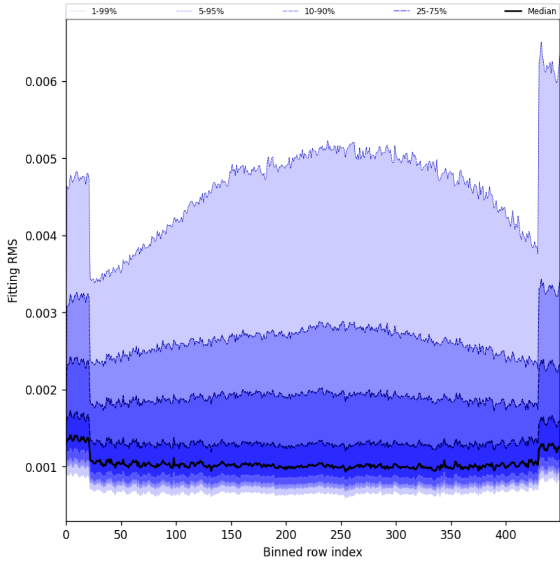
Figure 30: Along track statistics of “Fitting RMS” for 2025-04-26 to 2025-04-28
