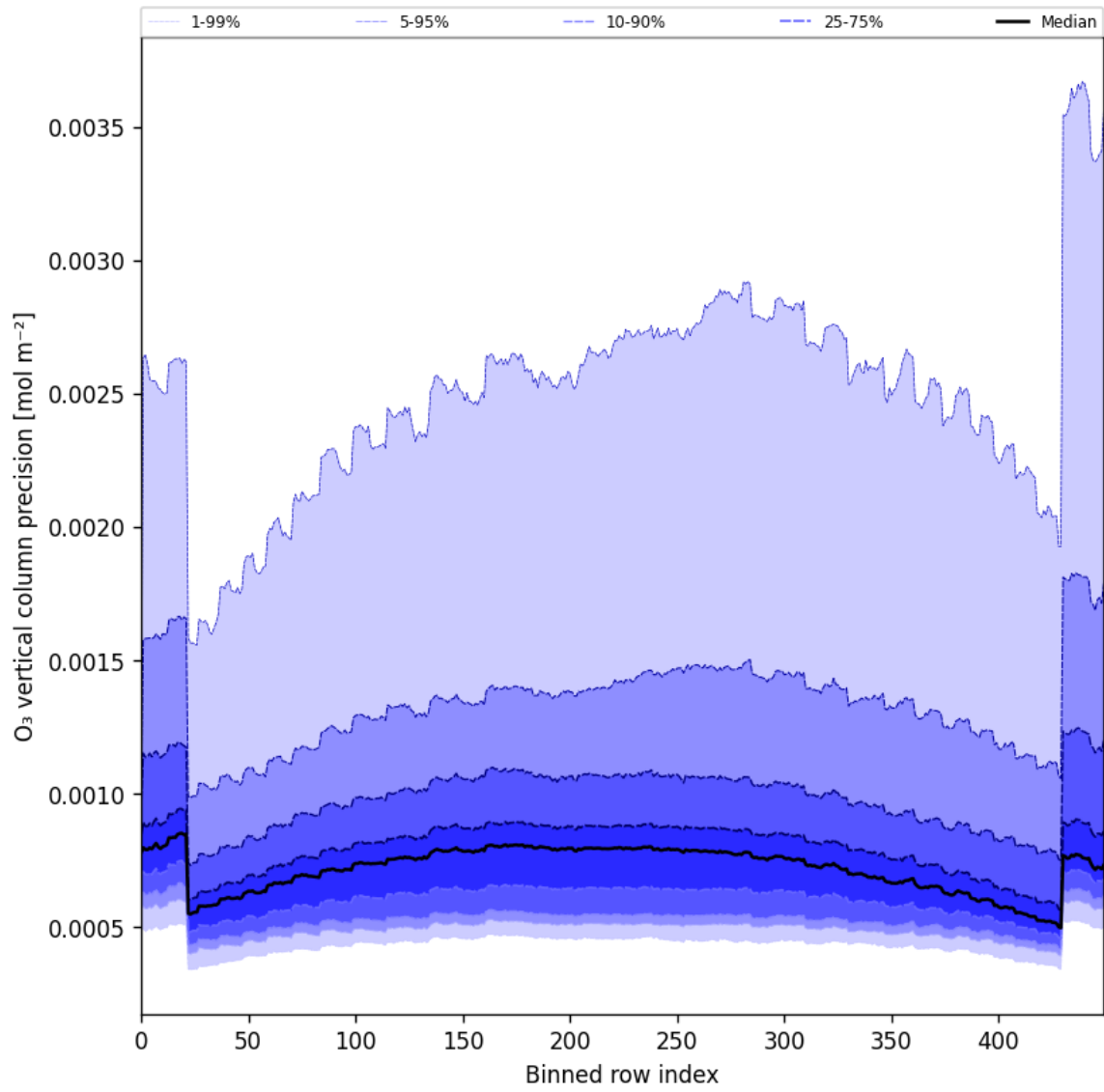
Figure 29: Along track statistics of “O 3 vertical column precision” for 2025-04-26 to 2025-04-28
