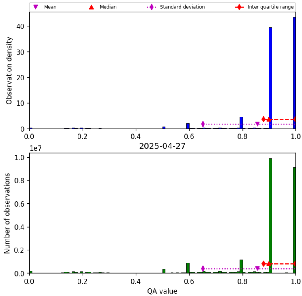
Figure 20: Histogram of “QA value” for 2025-04-26 to 2025-04-28
