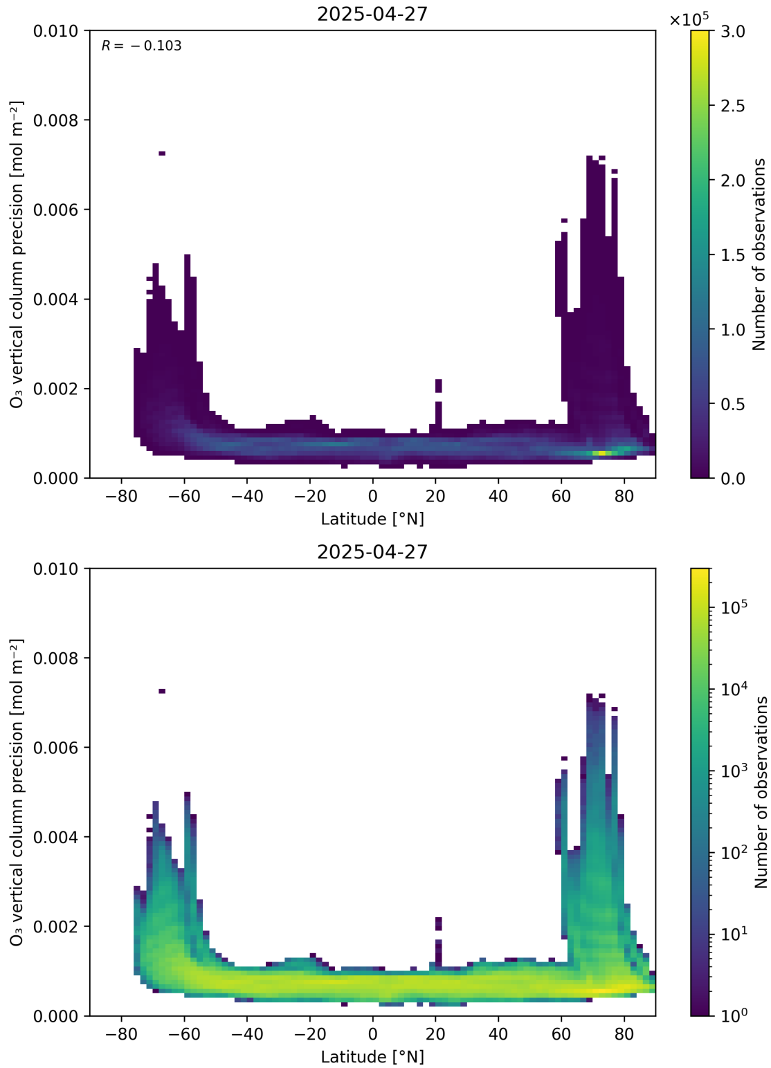
Figure 37: Scatter density plot of “Latitude” against “O 3 vertical column precision” for 2025-04-26 to 2025-04-28.
