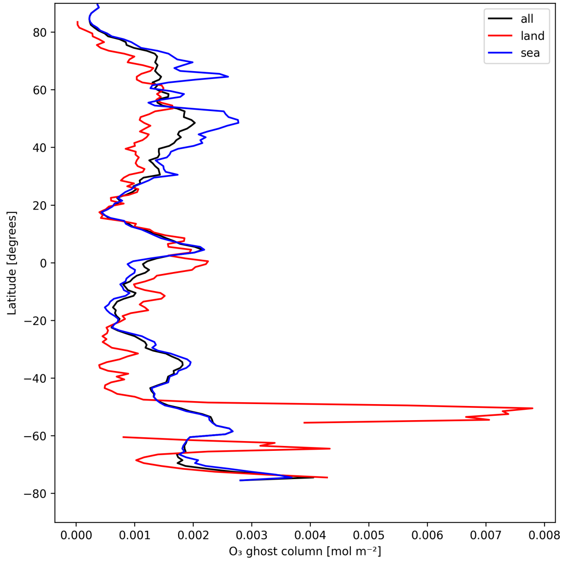
Figure 18: Zonal average of “O 3 ghost column” for 2025-04-26 to 2025-04-28.
