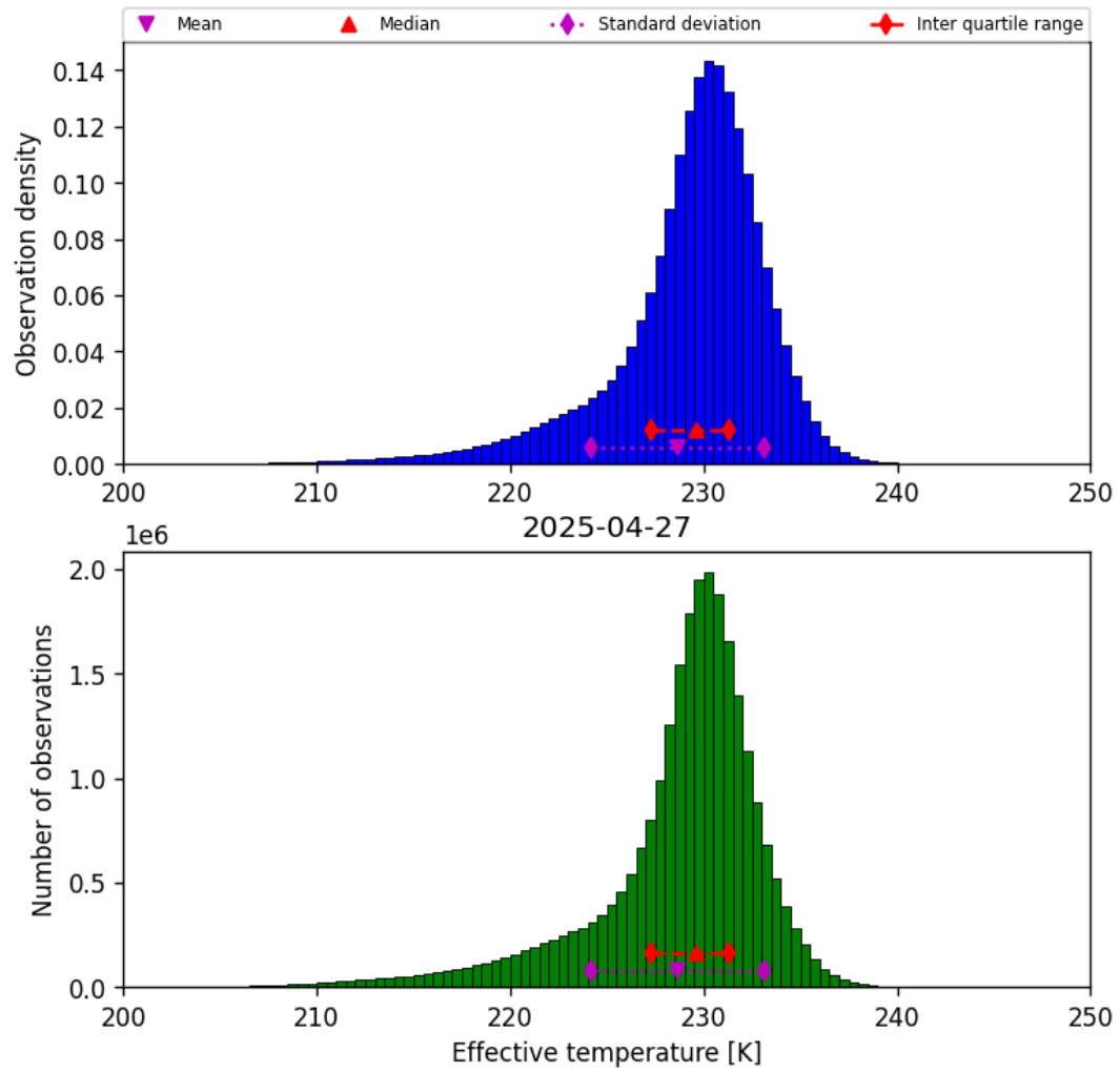
Figure 24: Histogram of “Effective temperature” for 2025-04-26 to 2025-04-28
