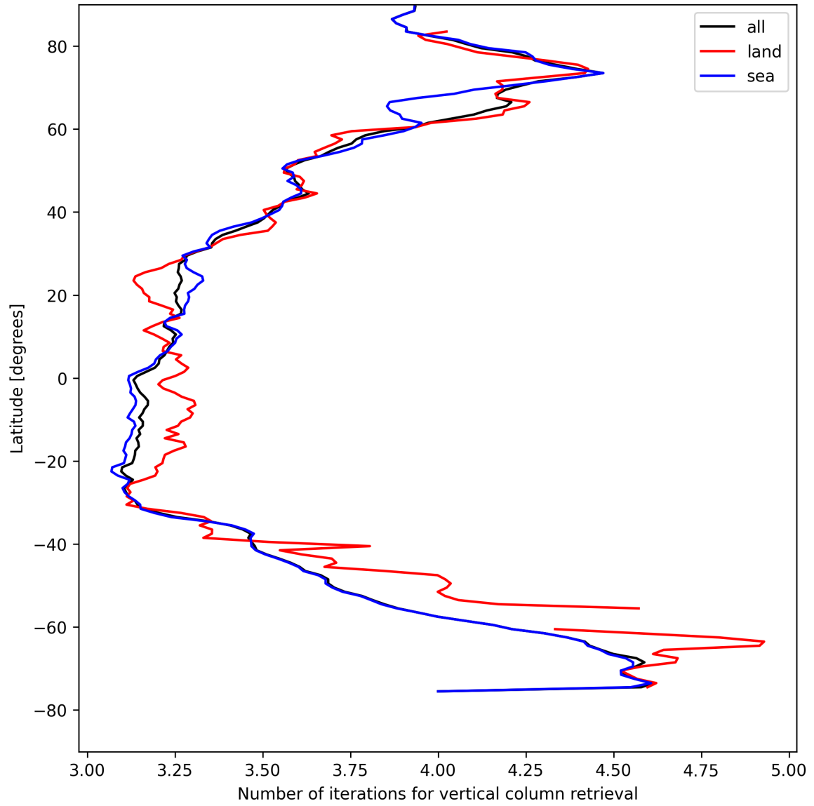
Figure 19: Zonal average of “Number of iterations for vertical column retrieval” for 2025-04-26 to 2025-04-28.
