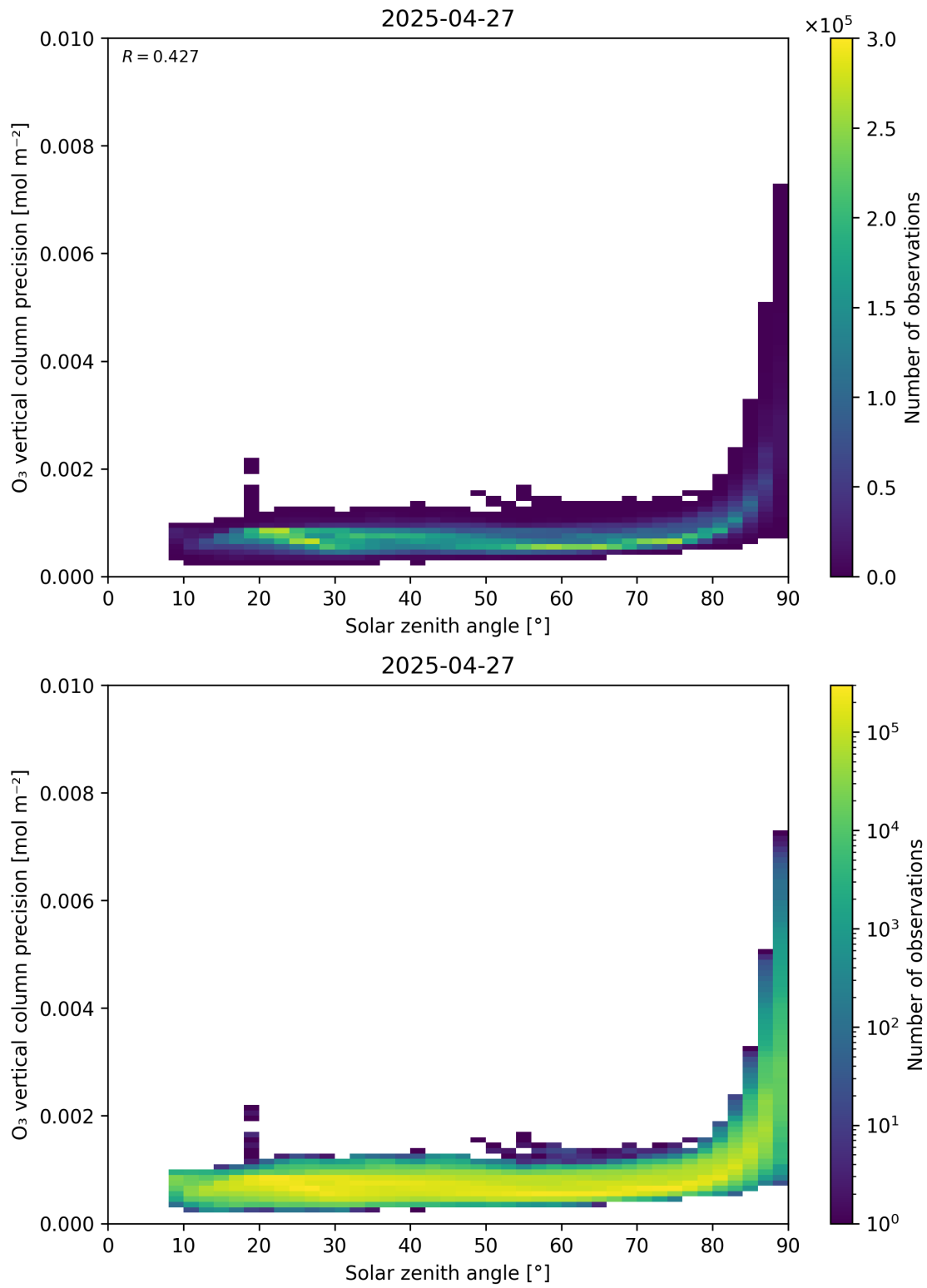
Figure 48: Scatter density plot of “Solar zenith angle” against “O 3 vertical column precision” for 2025-04-26 to 2025-04-28.
