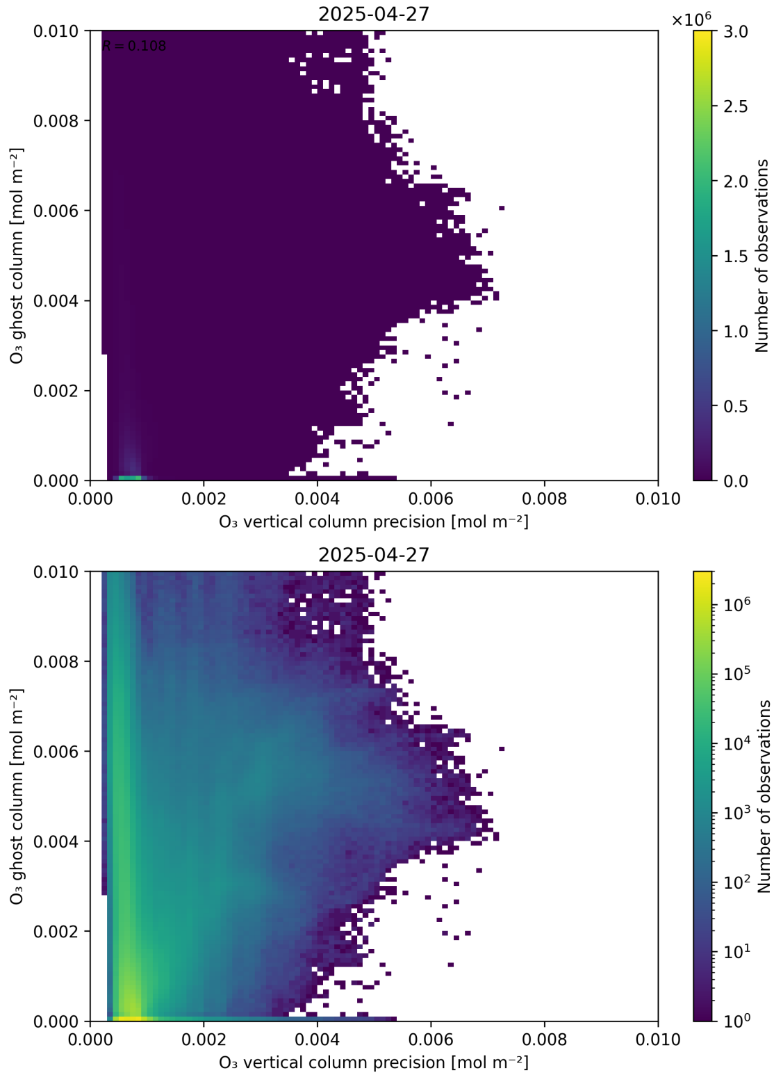
Figure 43: Scatter density plot of “O 3 vertical column precision” against “O 3 ghost column” for 2025-04-26 to 2025-04-28.
