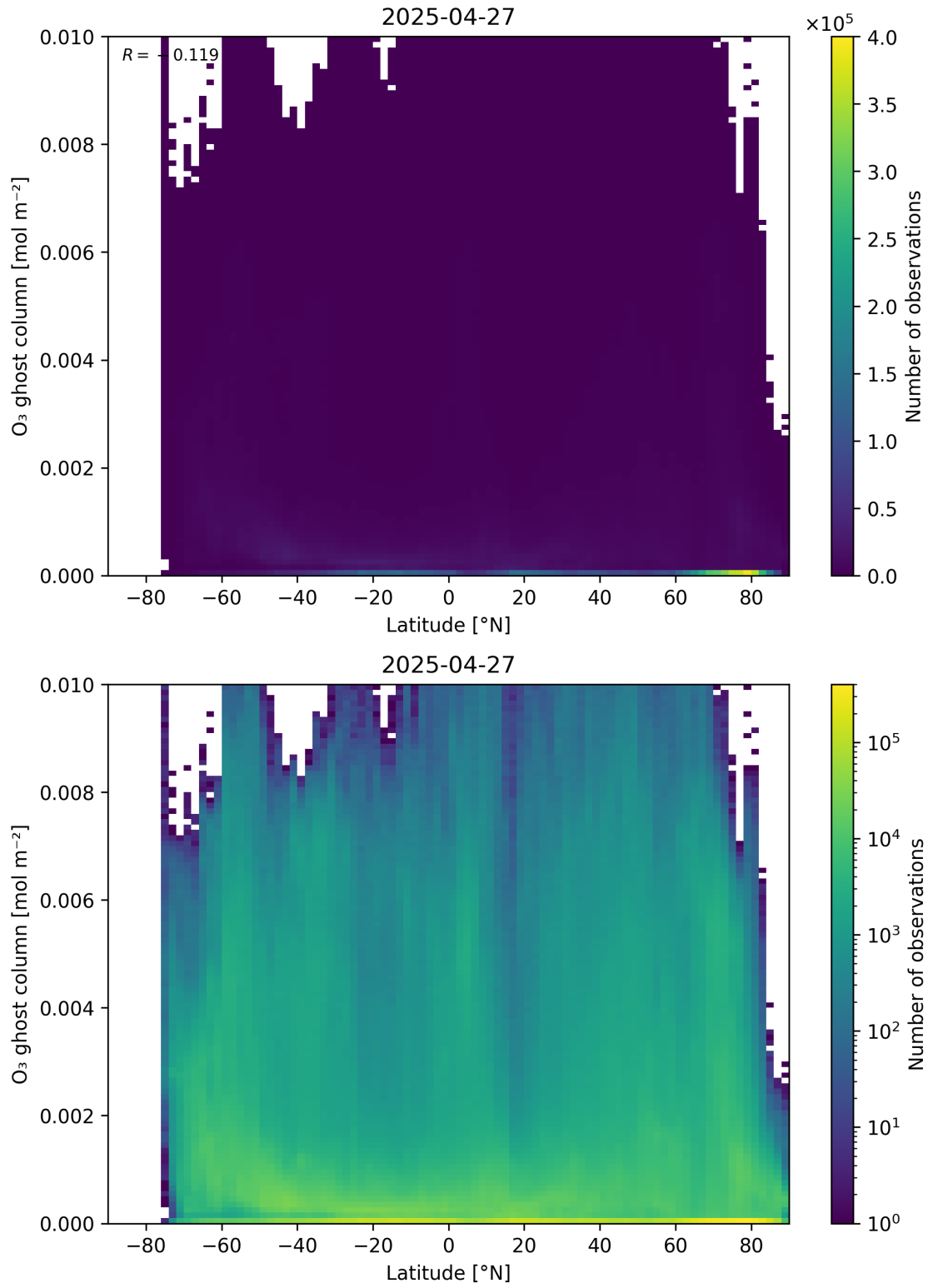
Figure 35: Scatter density plot of “Latitude” against “O 3 ghost column” for 2025-04-26 to 2025-04-28.
