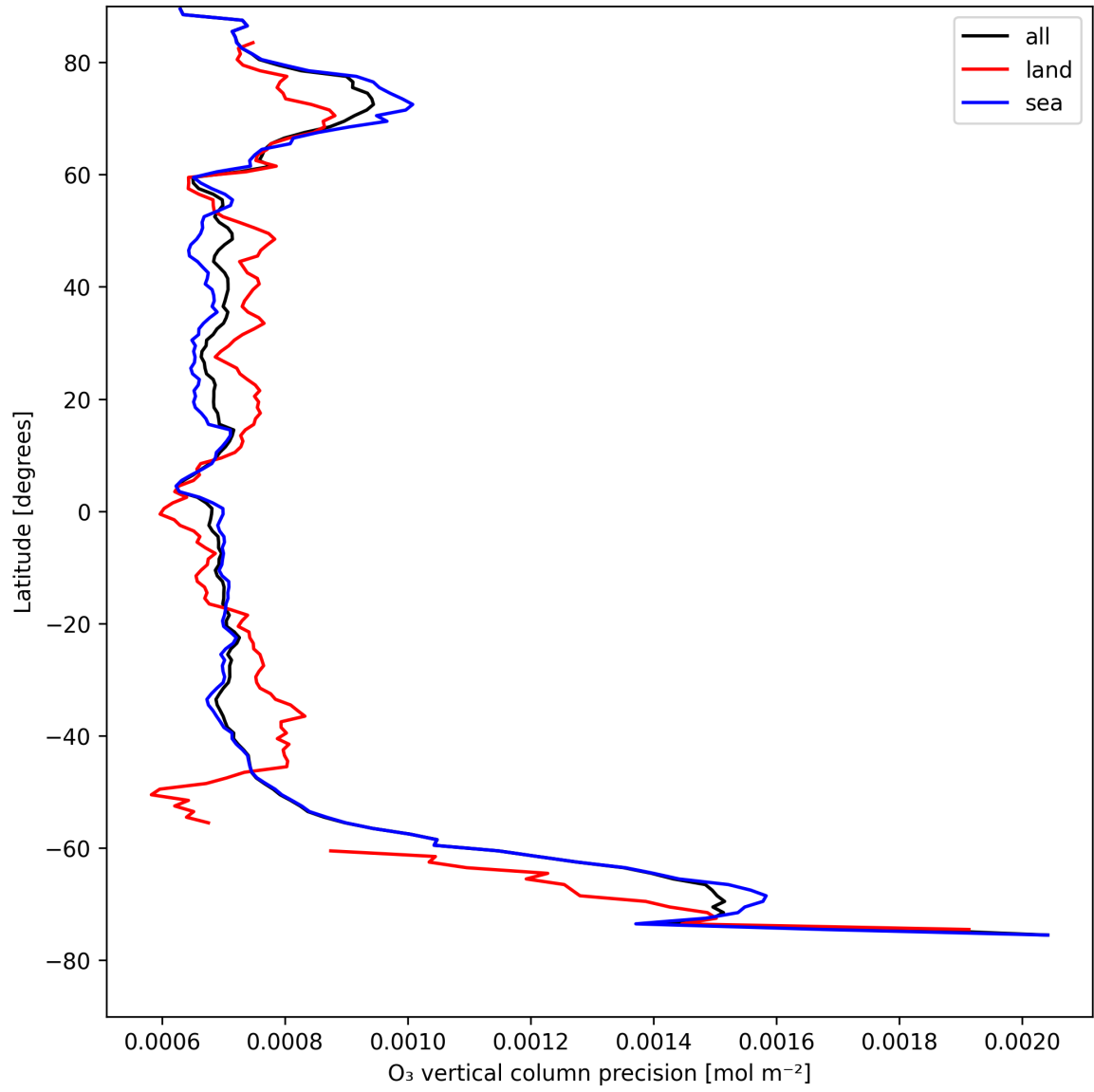
Figure 15: Zonal average of "O 3 vertical column precision" for 2025-04-26 to 2025-04-28.
