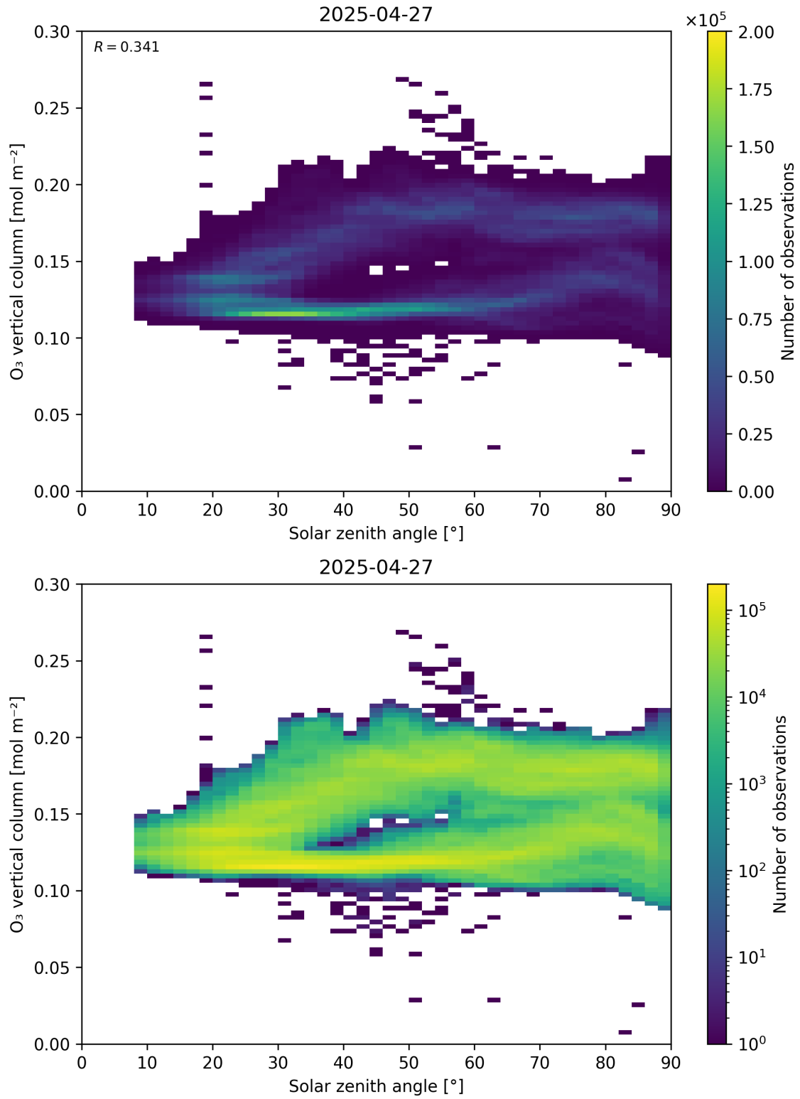
Figure 47: Scatter density plot of “Solar zenith angle” against “O 3 vertical column” for 2025-04-26 to 2025-04-28.
