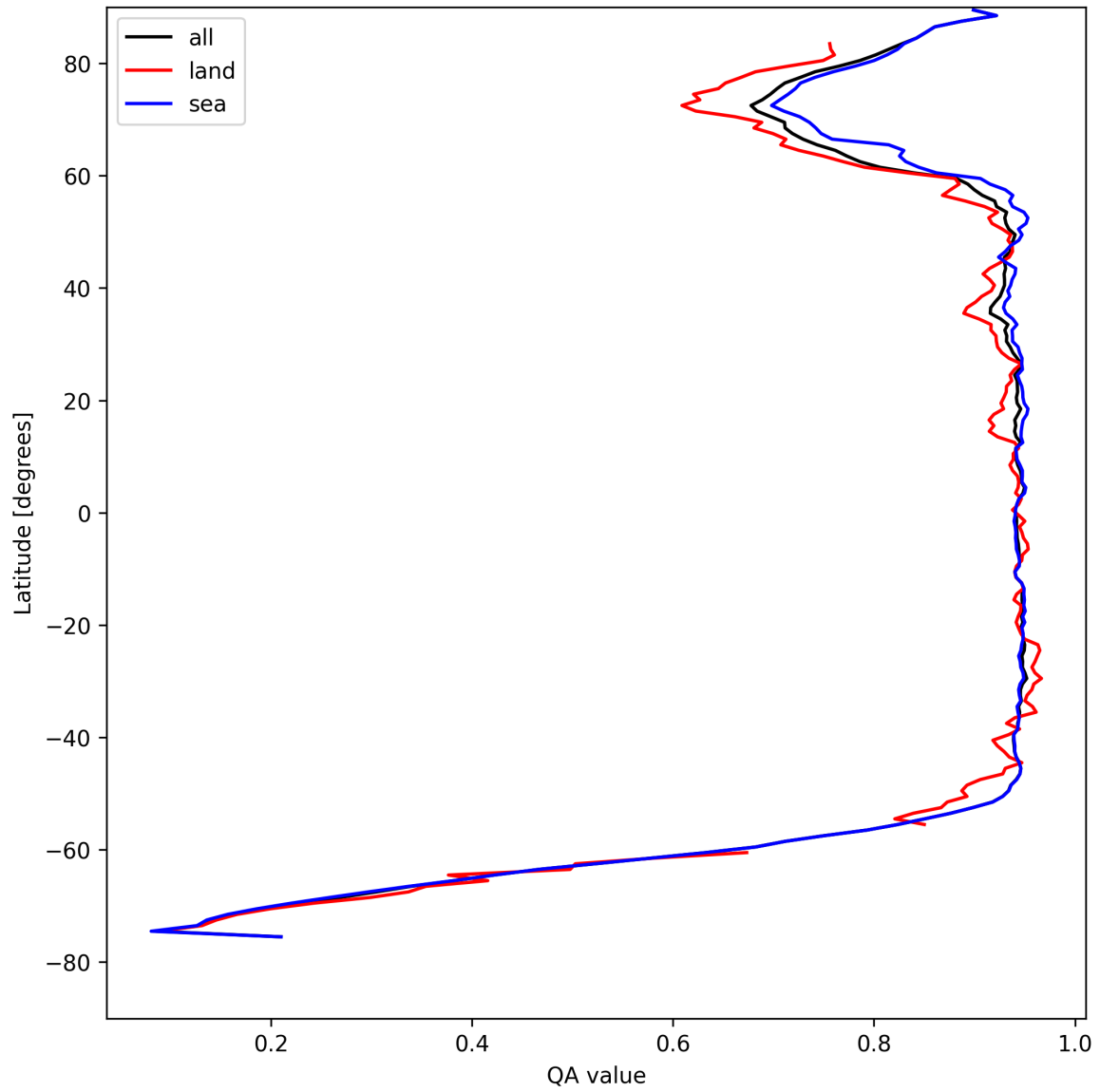
Figure 13: Zonal average of “QA value” for 2025-04-26 to 2025-04-28.
