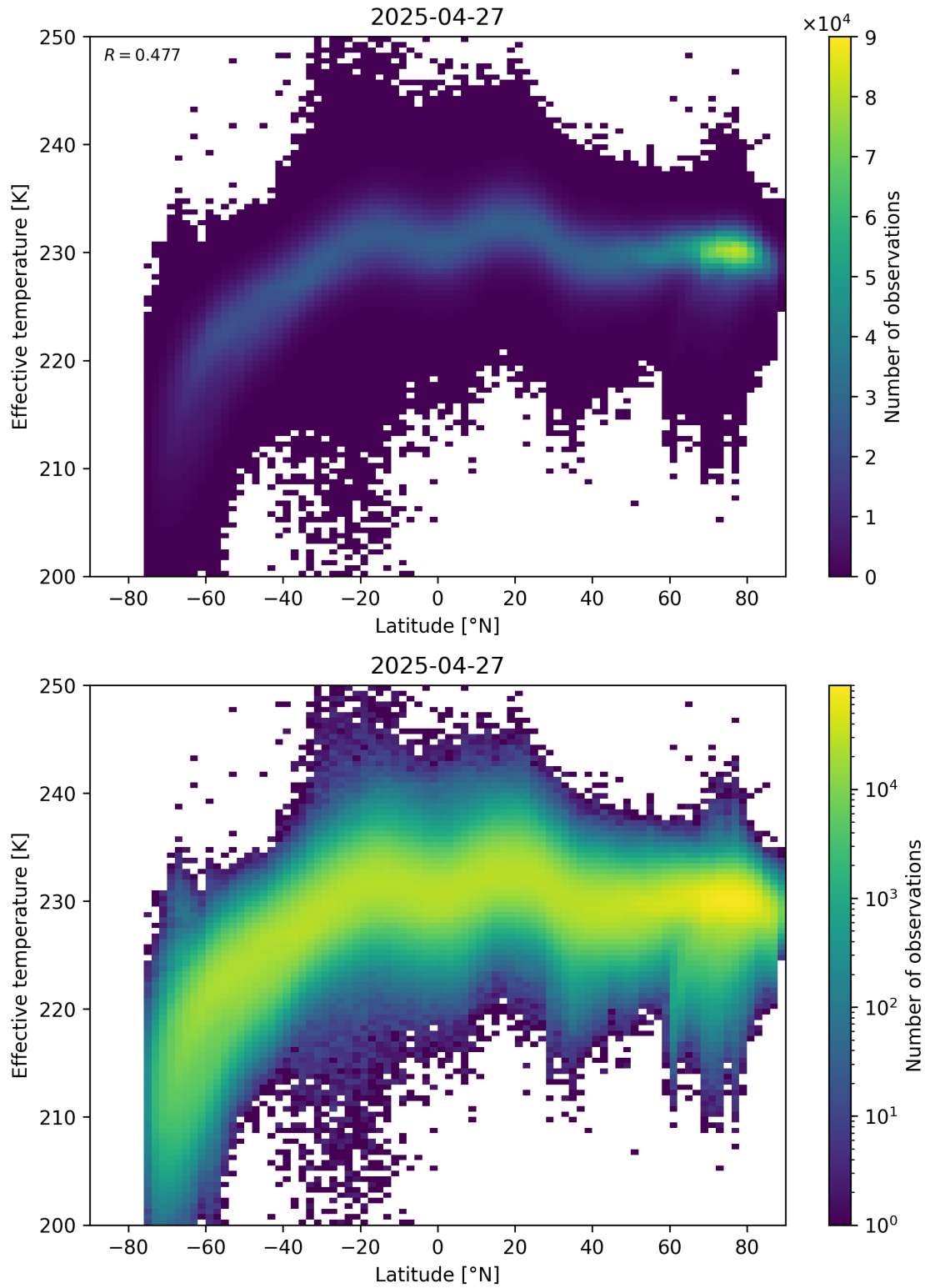
Figure 34: Scatter density plot of “Latitude” against “Effective temperature” for 2025-04-26 to 2025-04-28.
