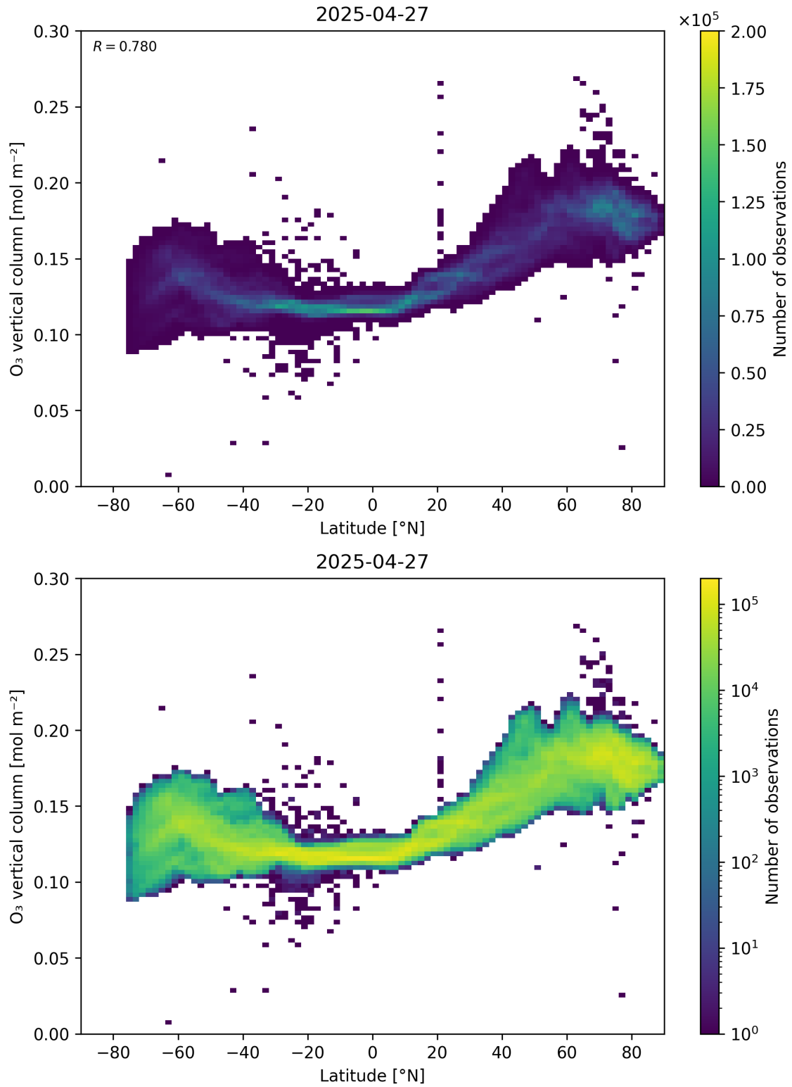
Figure 36: Scatter density plot of “Latitude” against “O 3 vertical column” for 2025-04-26 to 2025-04-28.
