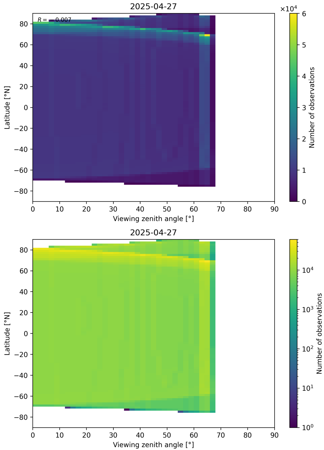
Figure 49: Scatter density plot of “Viewing zenith angle” against “Latitude” for 2025-04-26 to 2025-04-28.
