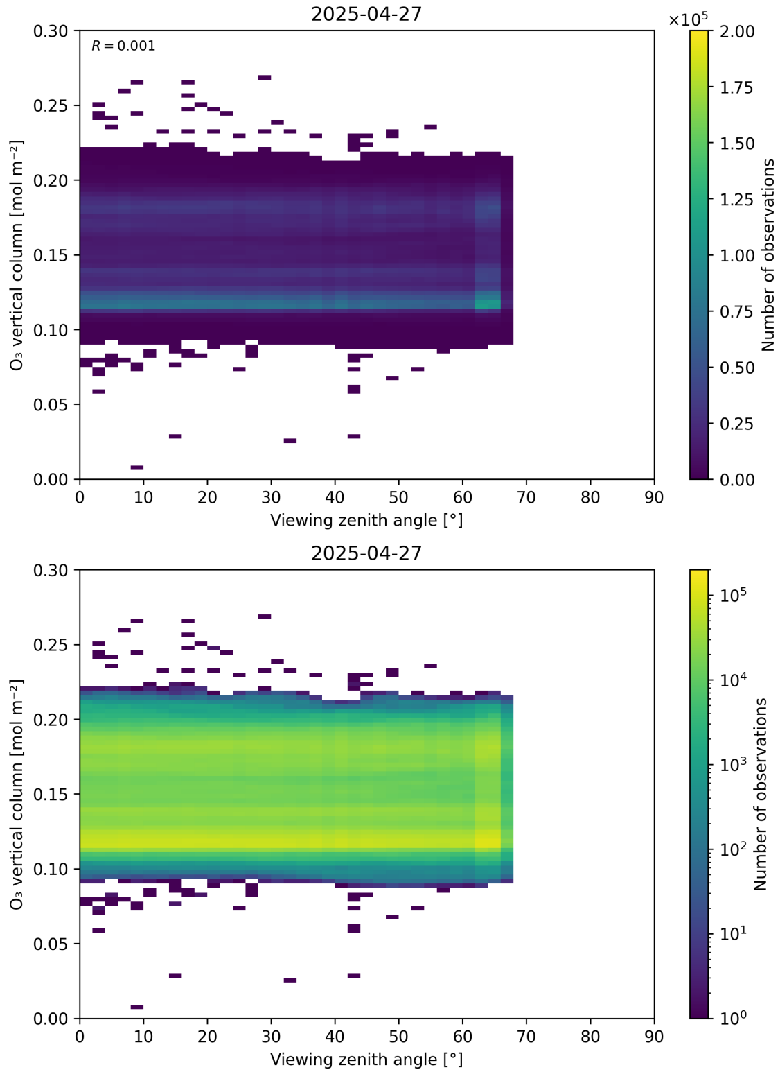
Figure 52: Scatter density plot of “Viewing zenith angle” against “O 3 vertical column” for 2025-04-26 to 2025-04-28.
