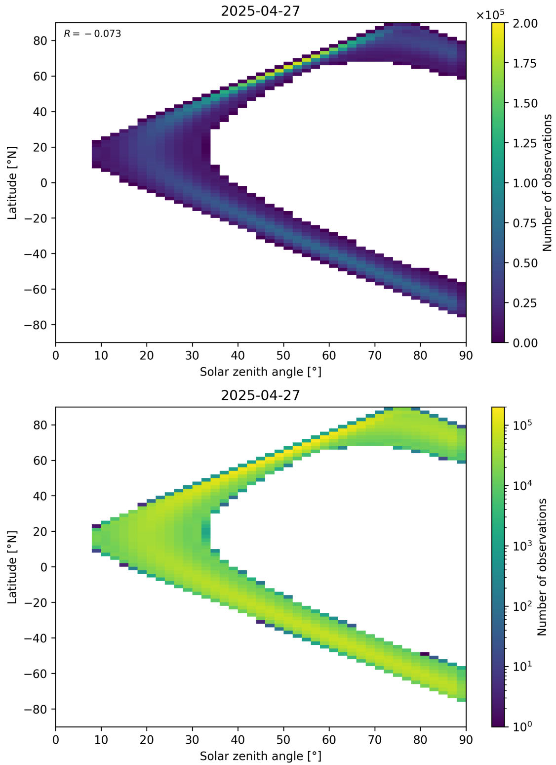
Figure 44: Scatter density plot of “Solar zenith angle” against “Latitude” for 2025-04-26 to 2025-04-28.
