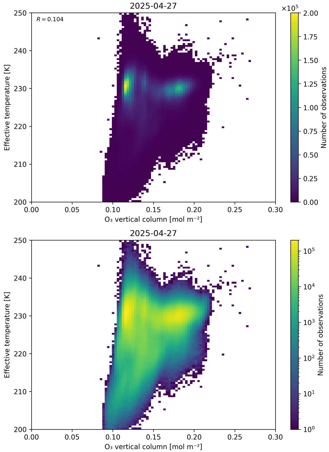
Figure 39: Scatter density plot of “O 3 vertical column” against “Effective temperature” for 2025-04-26 to 2025-04-28.
