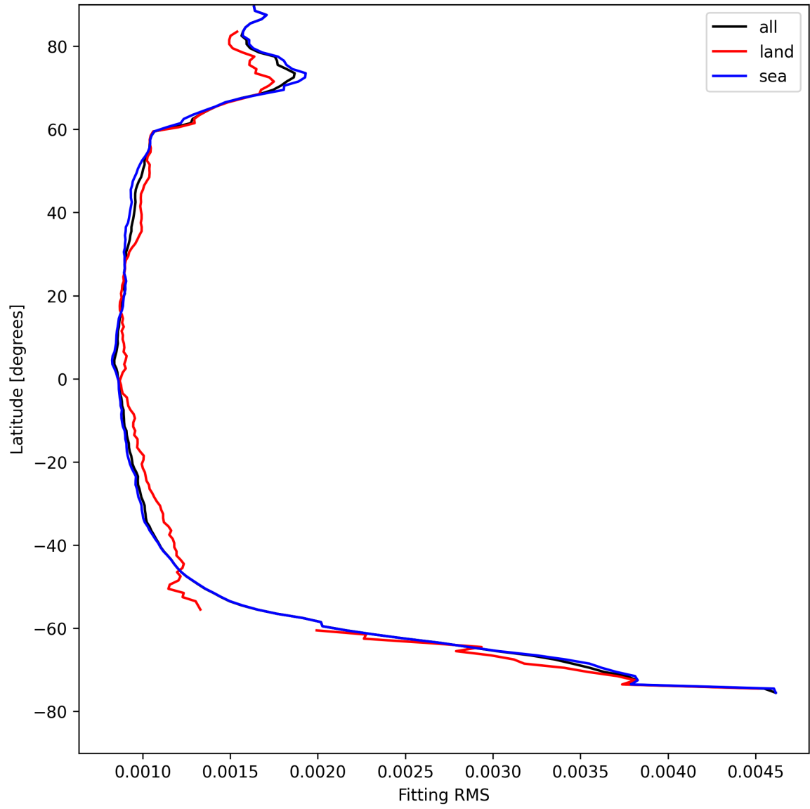
Figure 16: Zonal average of “Fitting RMS” for 2025-04-26 to 2025-04-28.
