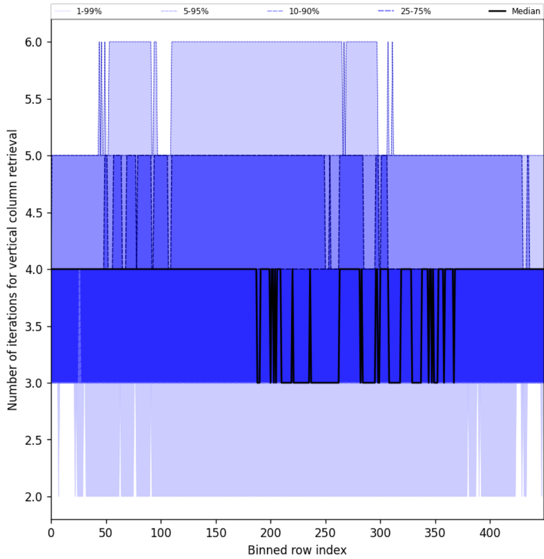
Figure 33: Along track statistics of “Number of iterations for vertical column retrieval” for 2025-04-26 to 2025-04-28
