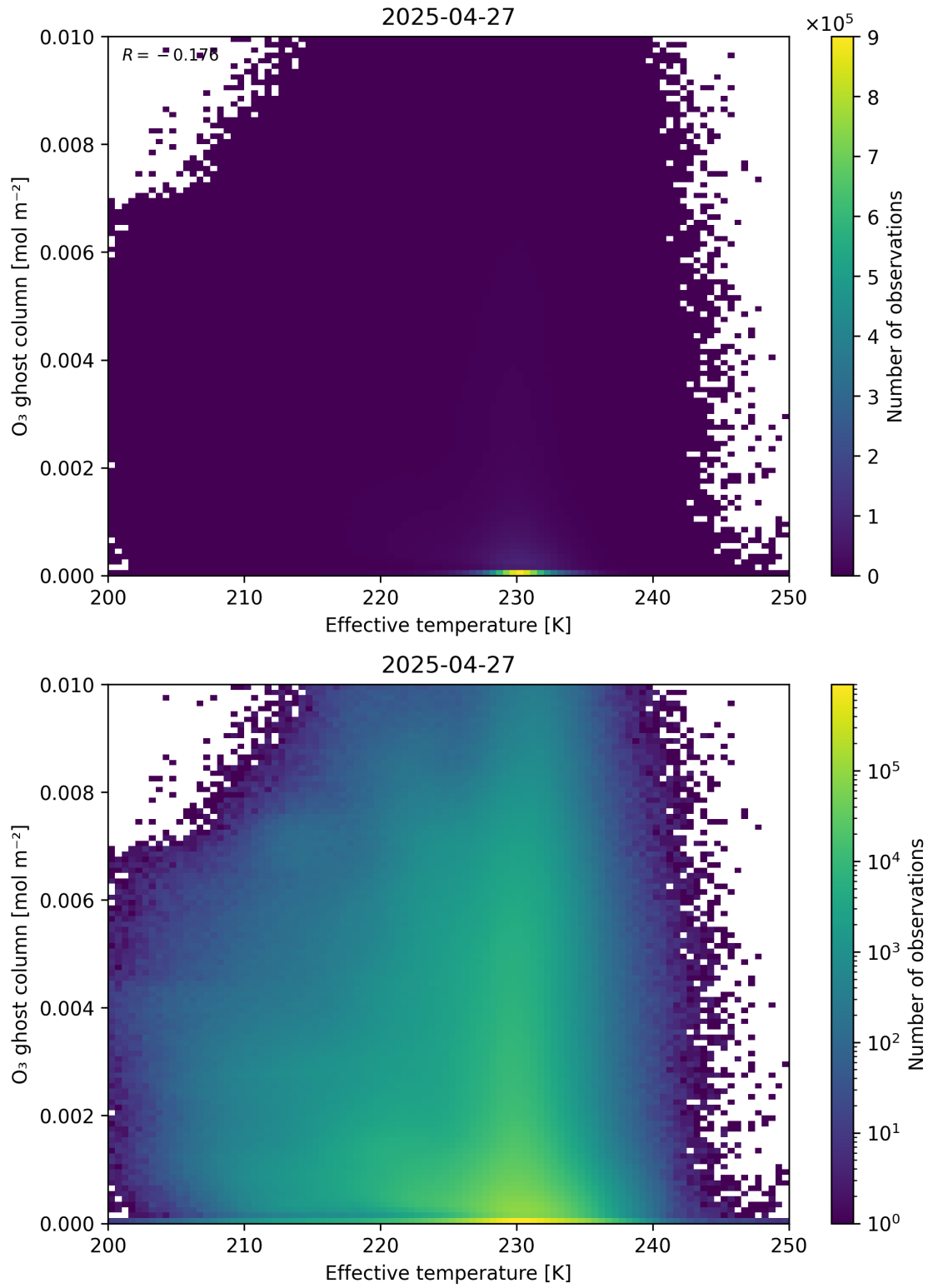
Figure 38: Scatter density plot of “Effective temperature” against “O 3 ghost column” for 2025-04-26 to 2025-04-28.
