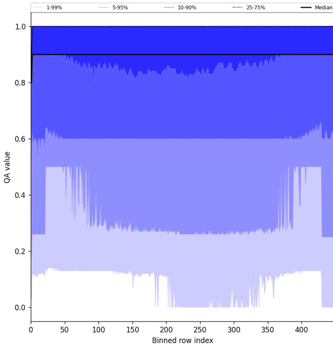
Figure 27: Along track statistics of “QA value” for 2025-04-26 to 2025-04-28
