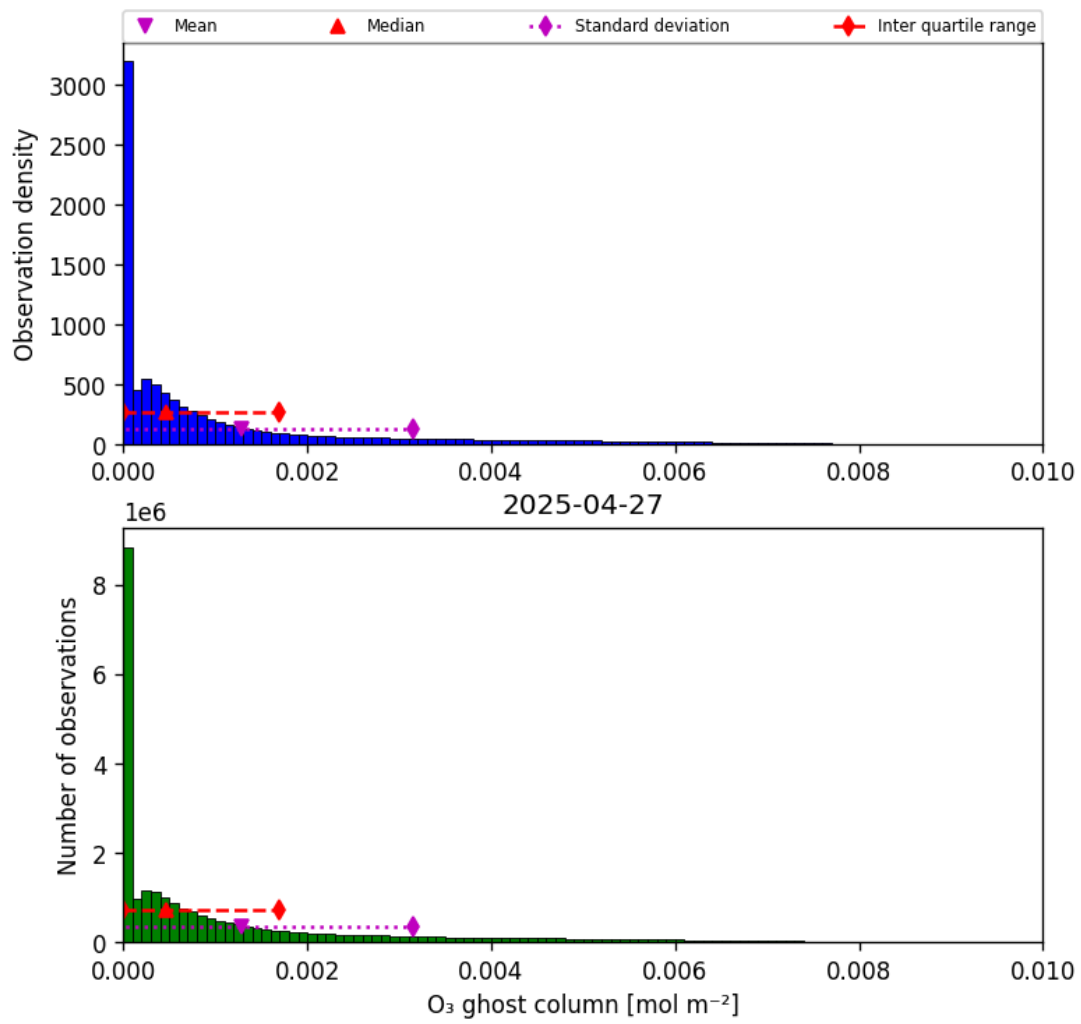
Figure 25: Histogram of “O 3 ghost column” for 2025-04-26 to 2025-04-28
