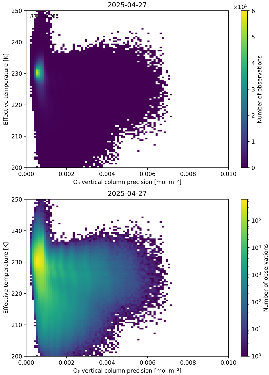
Figure 42: Scatter density plot of “O 3 vertical column precision” against “Effective temperature” for 2025-04-26 to 2025-04-28.
