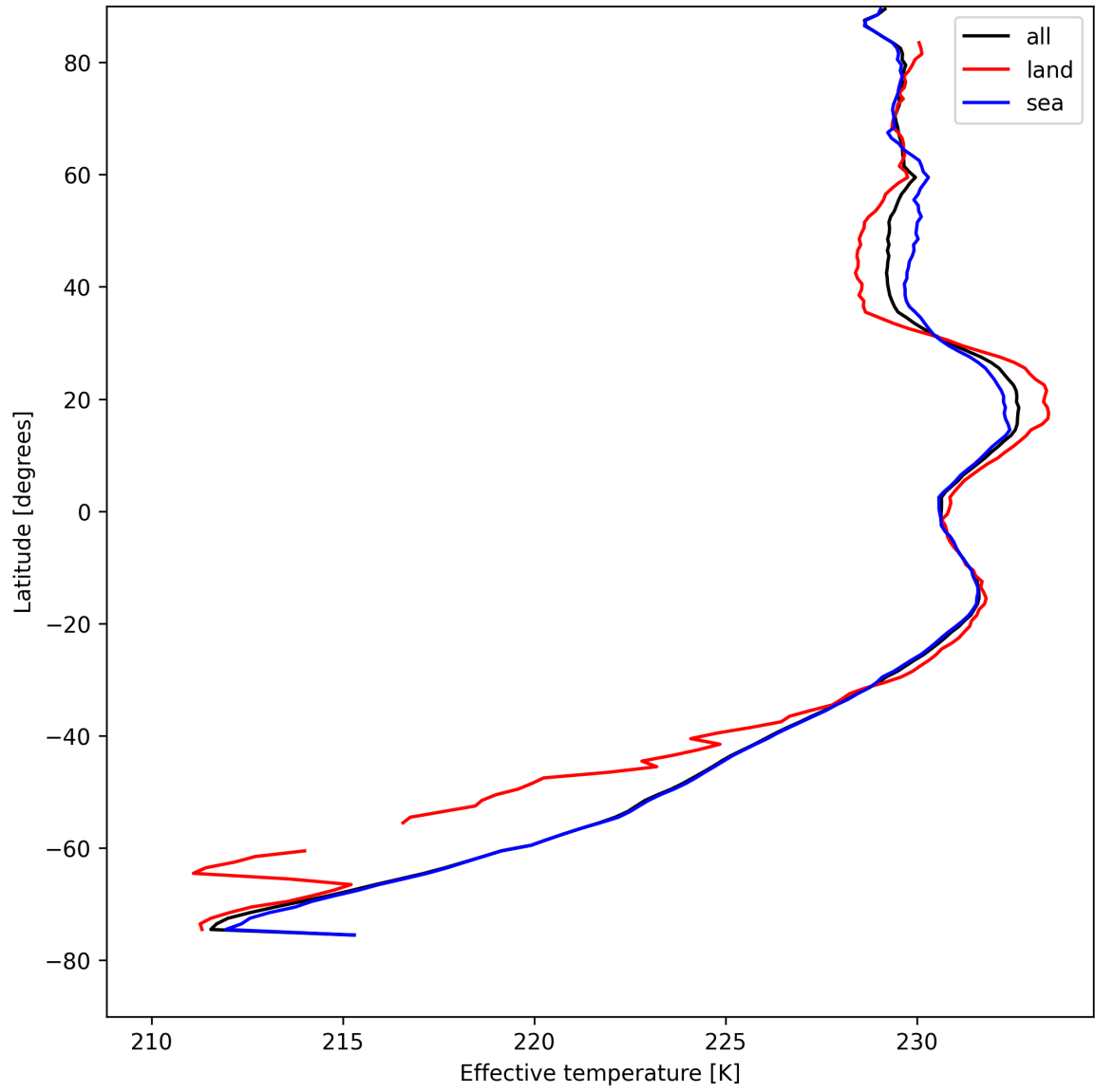
Figure 17: Zonal average of "Effective temperature" for 2025-04-26 to 2025-04-28.
