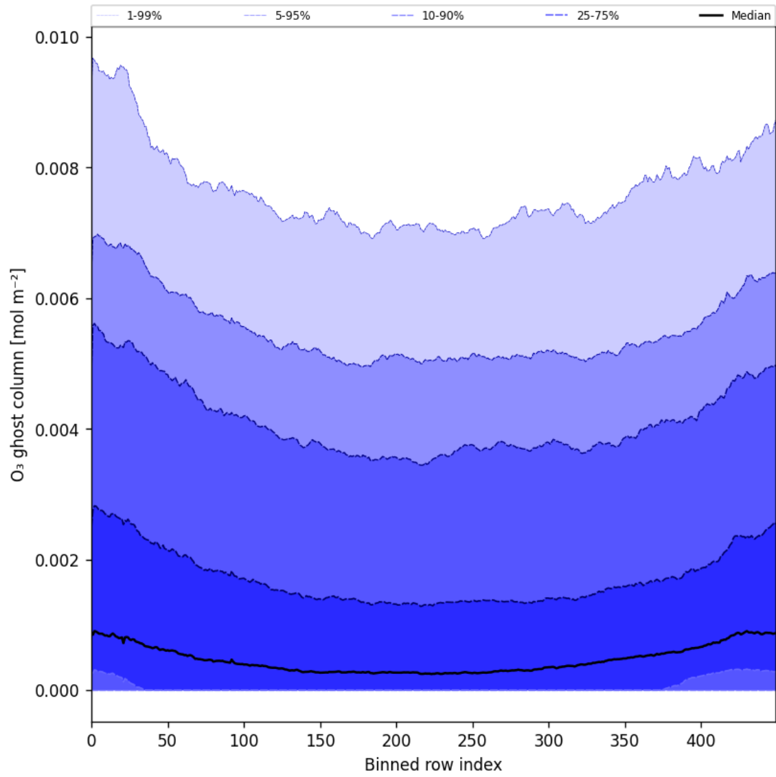
Figure 32: Along track statistics of "O 3 ghost column" for 2025-04-26 to 2025-04-28
