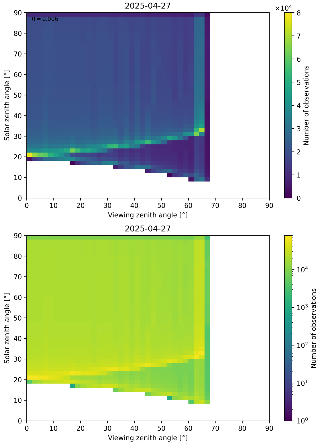
Figure 54: Scatter density plot of “Viewing zenith angle” against “Solar zenith angle” for 2025-04-26 to 2025-04-28.
