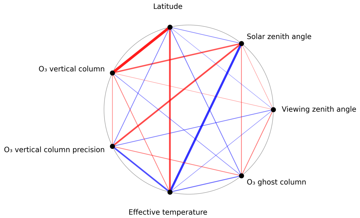
Figure 1: Map of correlation graph for 2025-04-26 to 2025-04-28.
