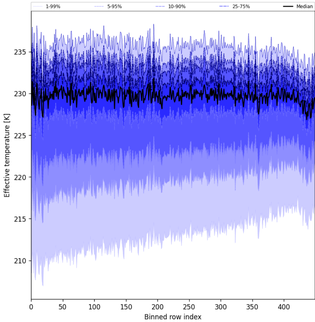
Figure 31: Along track statistics of “Effective temperature” for 2025-04-26 to 2025-04-28
