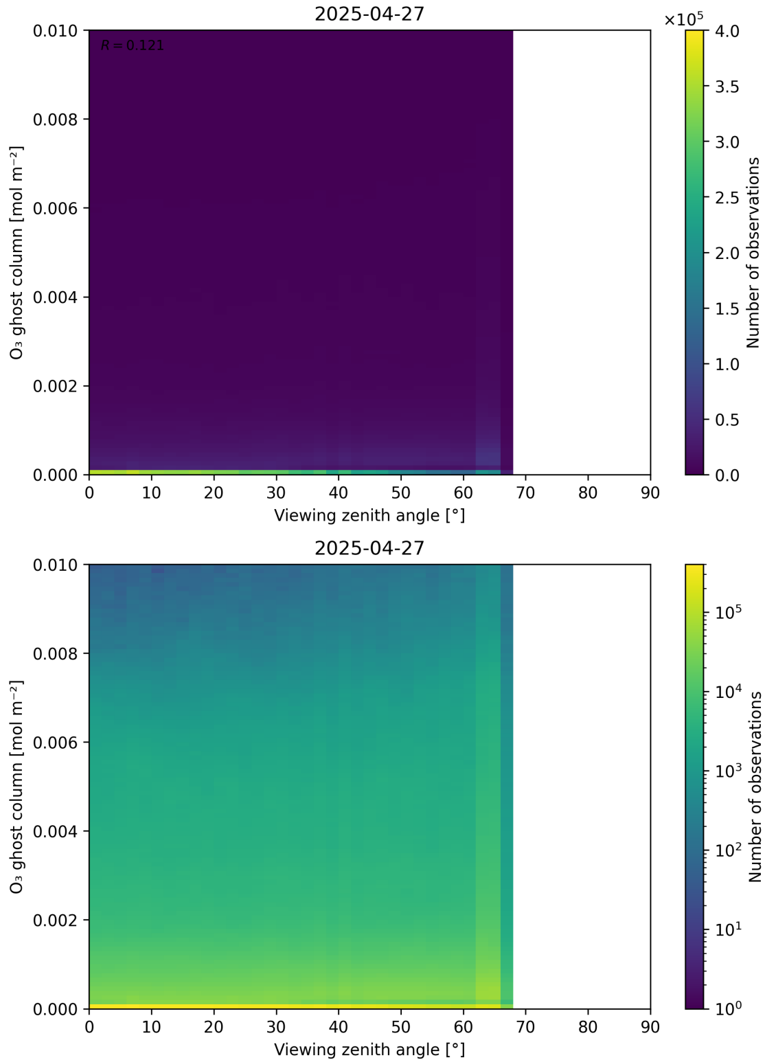
Figure 51: Scatter density plot of “Viewing zenith angle” against “O 3 ghost column” for 2025-04-26 to 2025-04-28.
