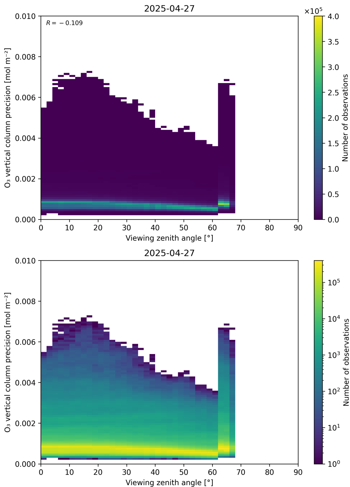
Figure 53: Scatter density plot of “Viewing zenith angle” against “O 3 vertical column precision” for 2025-04-26 to 2025-04-28.
