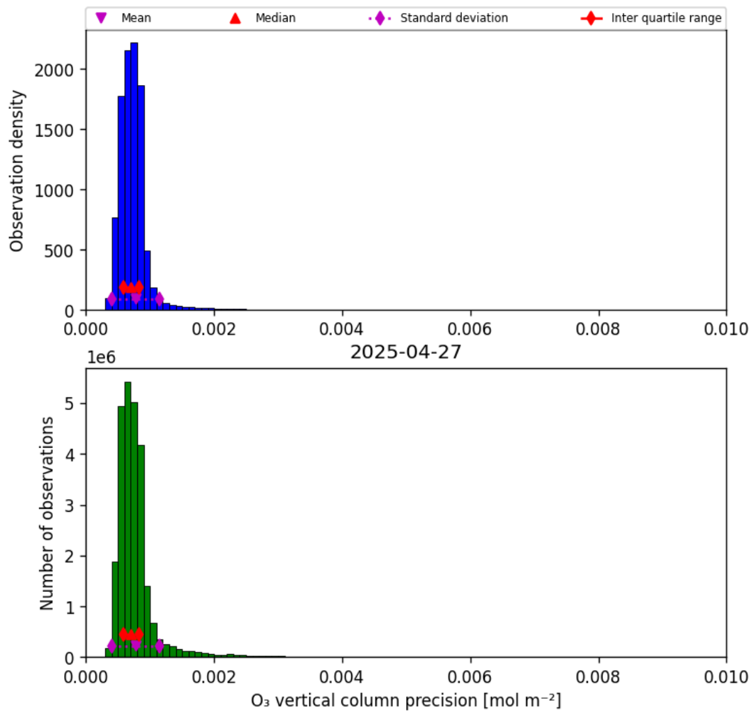
Figure 22: Histogram of “O 3 vertical column precision” for 2025-04-26 to 2025-04-28
