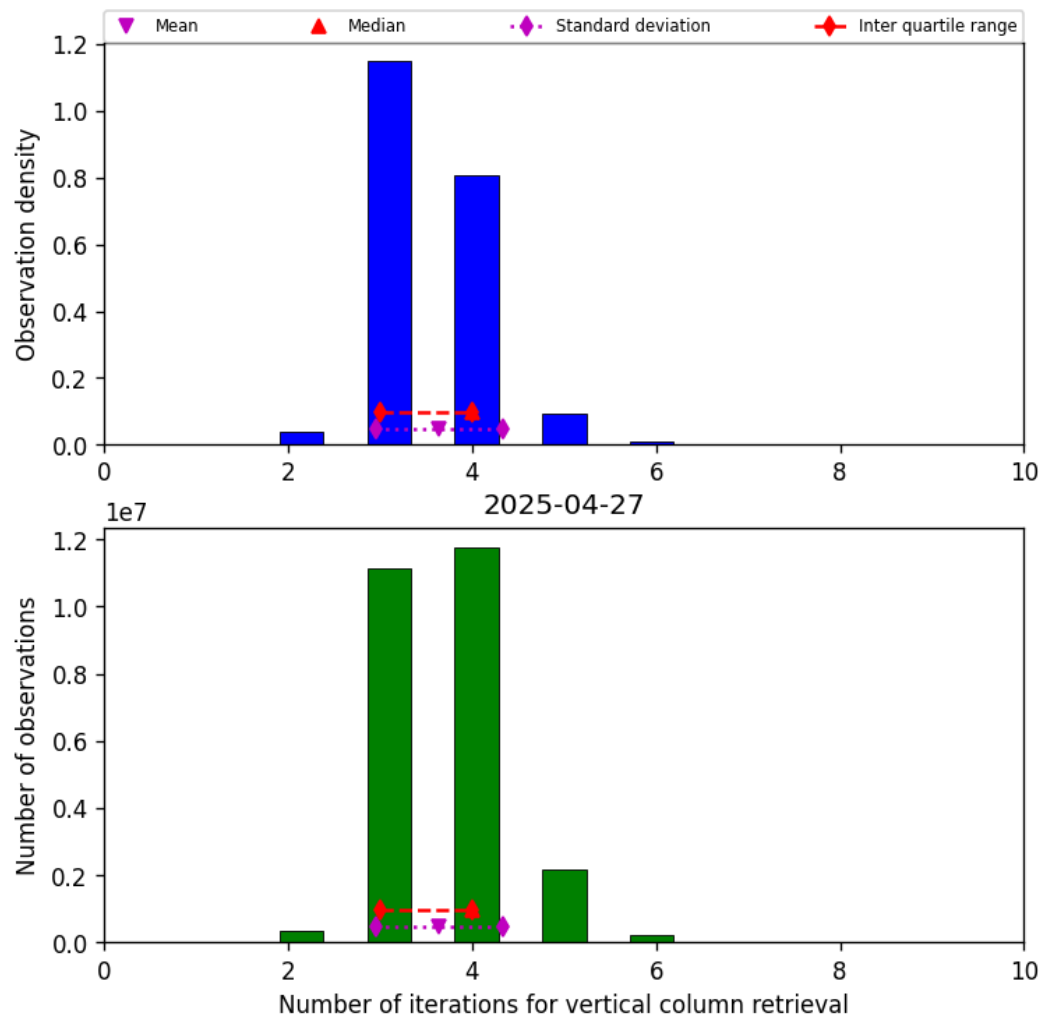
Figure 26: Histogram of “Number of iterations for vertical column retrieval” for 2025-04-26 to 2025-04-28
