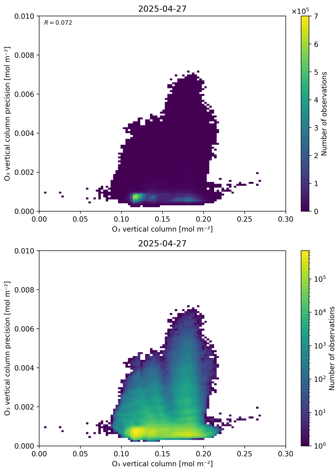
Figure 41: Scatter density plot of “O 3 vertical column” against “O 3 vertical column precision” for 2025-04-26 to 2025-04-28.
