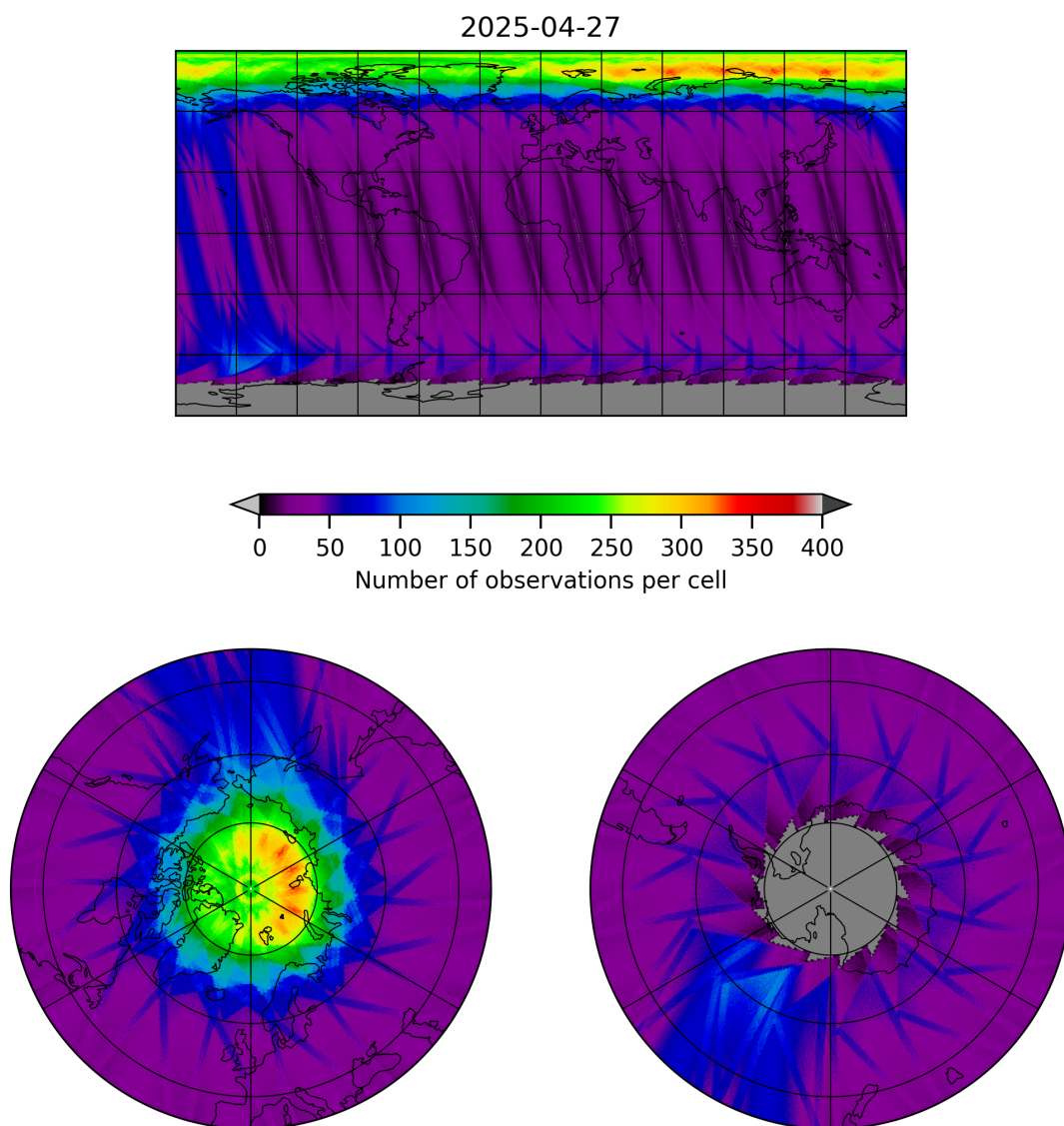
Figure 12: Map of the number of observations for 2025-04-26 to 2025-04-28
