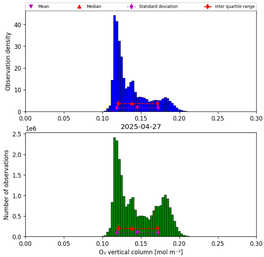
Figure 21: Histogram of “O 3 vertical column” for 2025-04-26 to 2025-04-28
