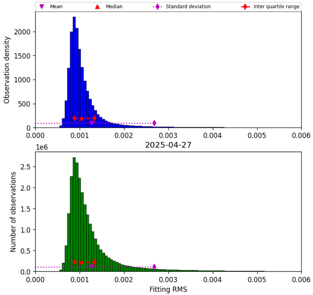
Figure 23: Histogram of “Fitting RMS” for 2025-04-26 to 2025-04-28
