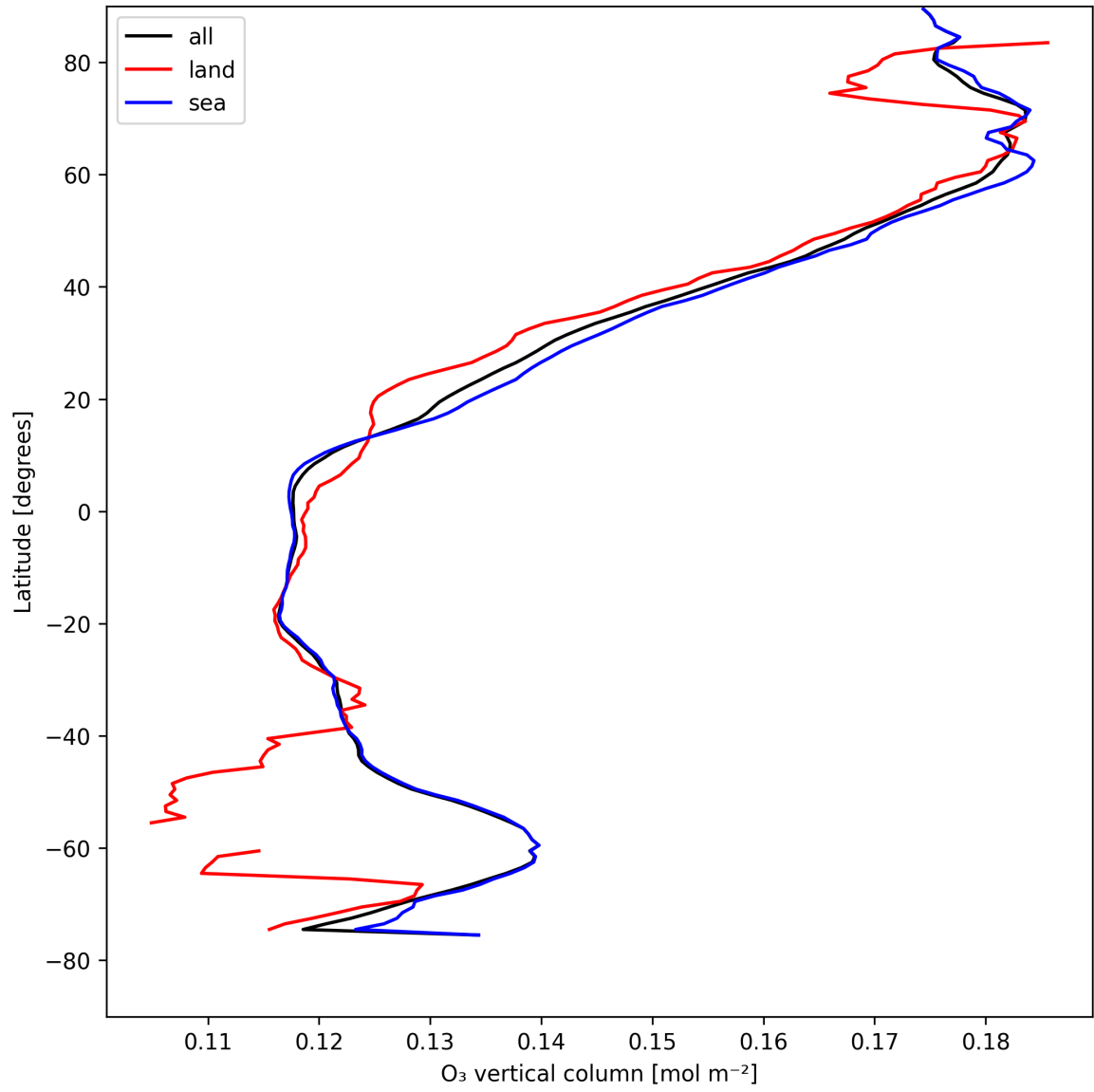
Figure 14: Zonal average of “O 3 vertical column” for 2025-04-26 to 2025-04-28.
