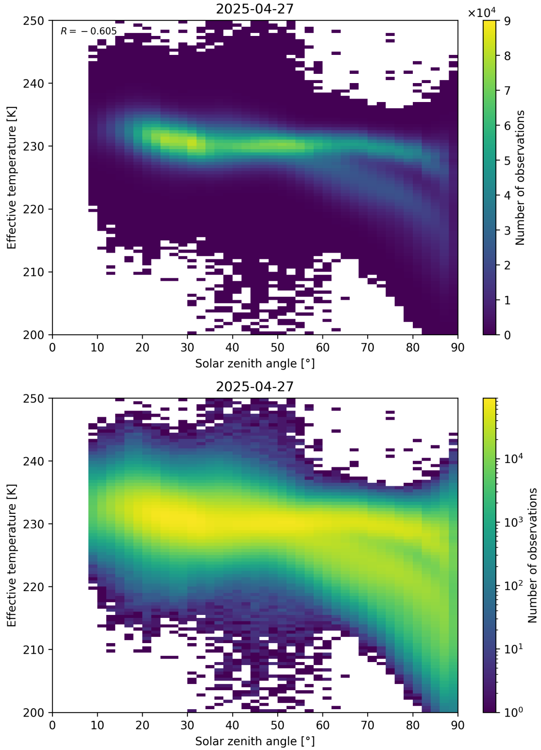
Figure 45: Scatter density plot of “Solar zenith angle” against “Effective temperature” for 2025-04-26 to 2025-04-28.
