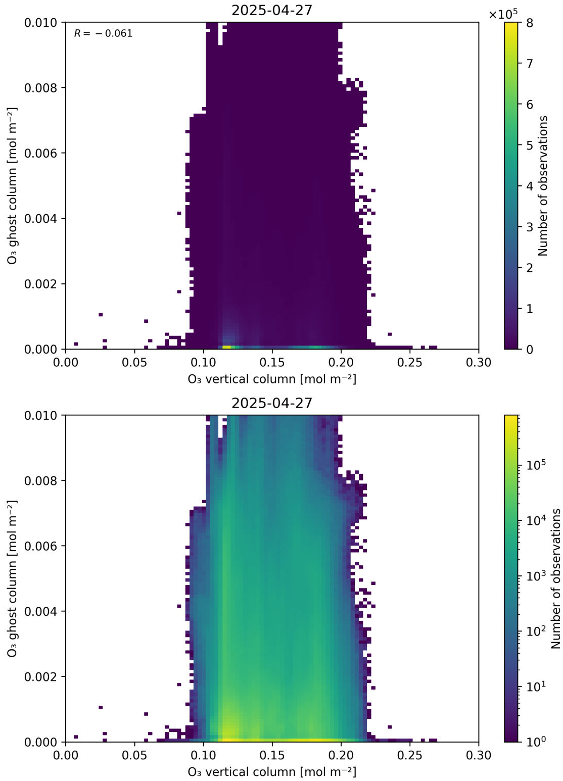
Figure 40: Scatter density plot of “O 3 vertical column” against “O 3 ghost column” for 2025-04-26 to 2025-04-28.
