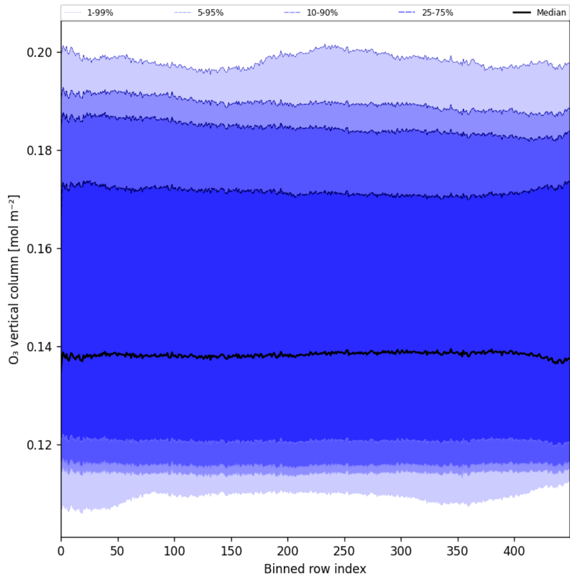
Figure 28: Along track statistics of “O 3 vertical column” for 2025-04-26 to 2025-04-28
