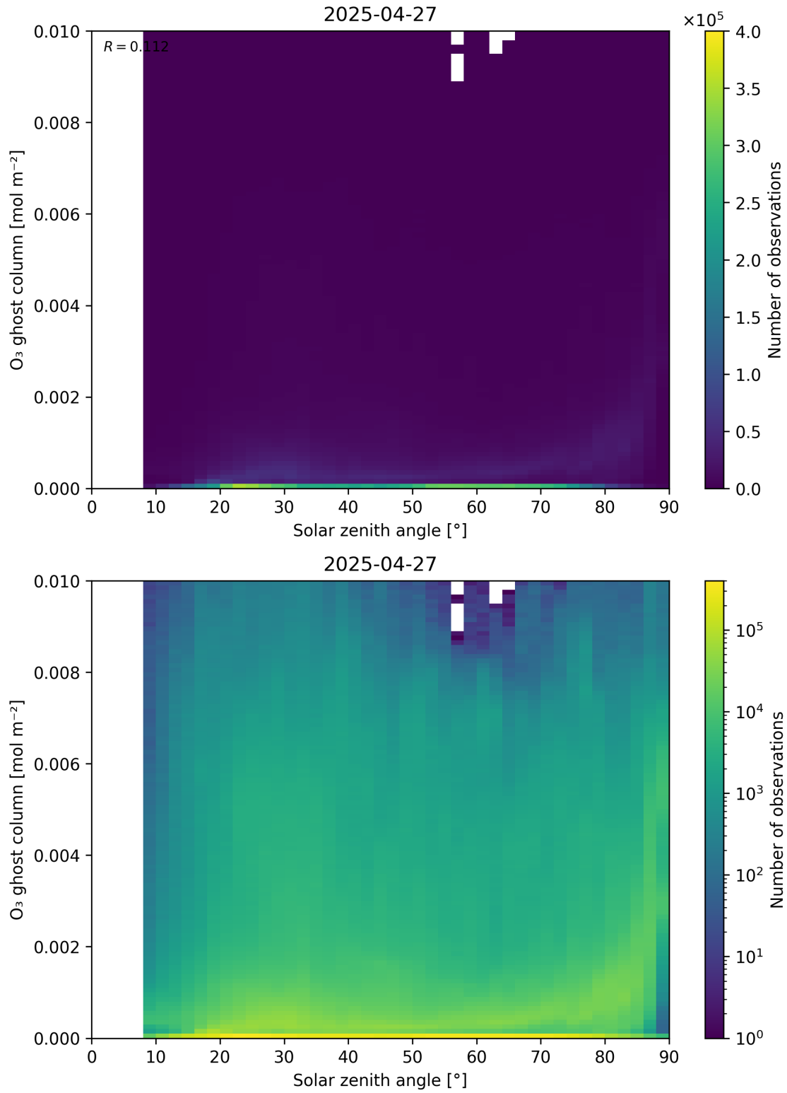
Figure 46: Scatter density plot of “Solar zenith angle” against “O 3 ghost column” for 2025-04-26 to 2025-04-28.
