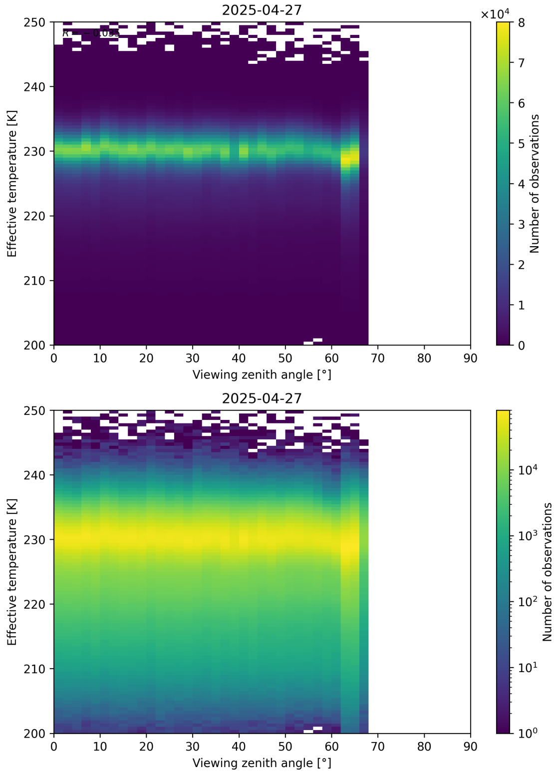
Figure 50: Scatter density plot of “Viewing zenith angle” against “Effective temperature” for 2025-04-26 to 2025-04-28.
