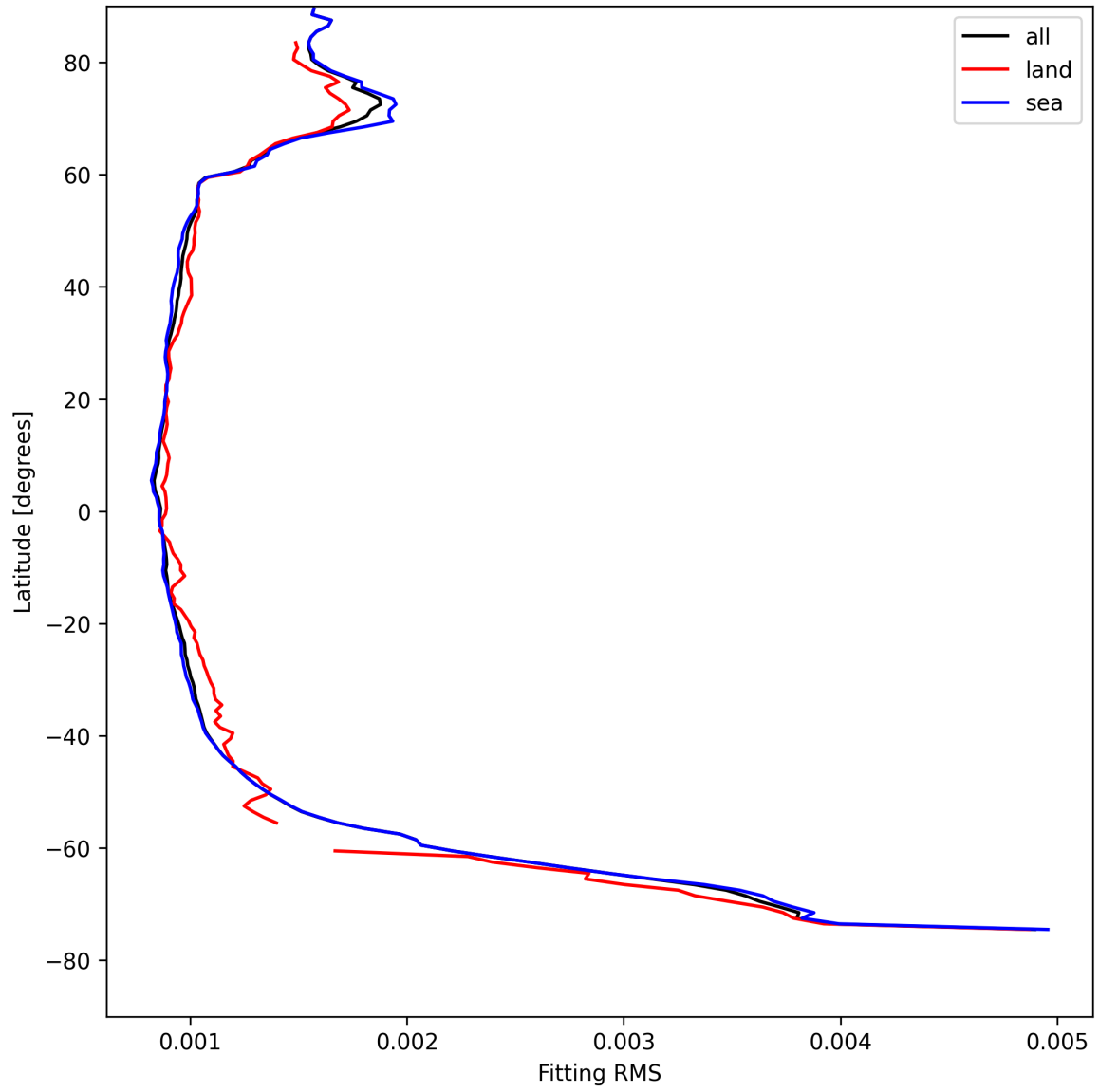
Figure 16: Zonal average of “Fitting RMS” for 2025-04-27 to 2025-04-29.
