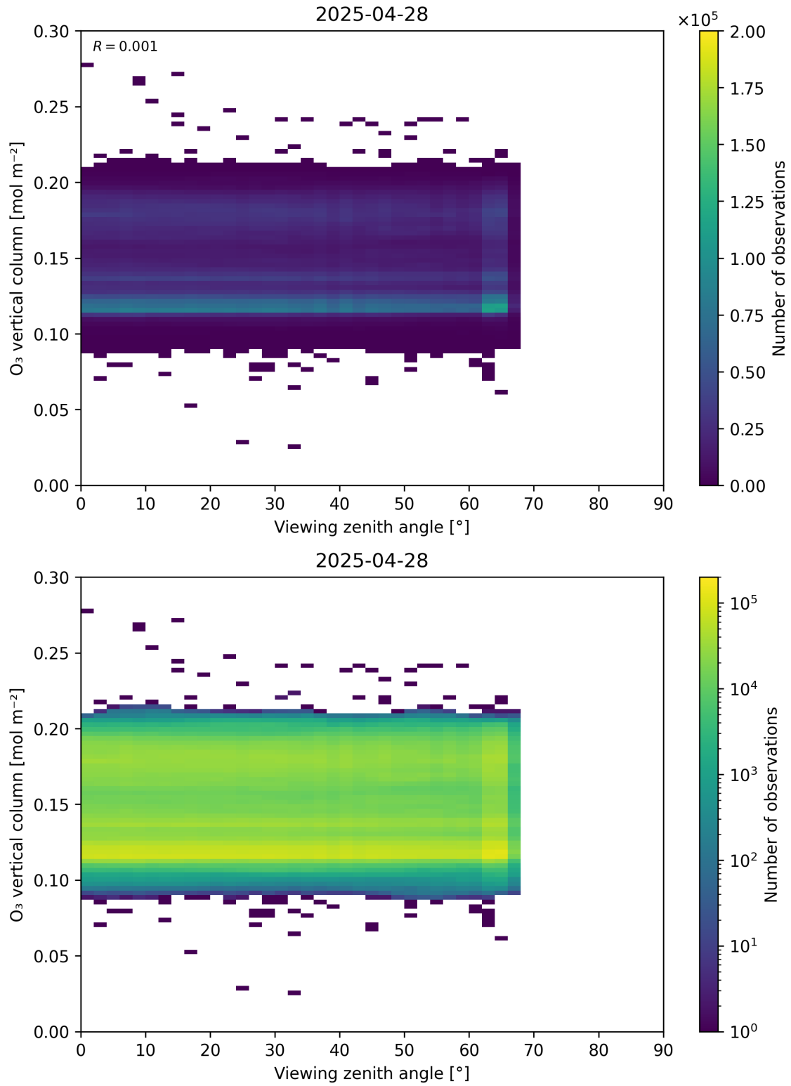
Figure 52: Scatter density plot of “Viewing zenith angle” against “O 3 vertical column” for 2025-04-27 to 2025-04-29.
