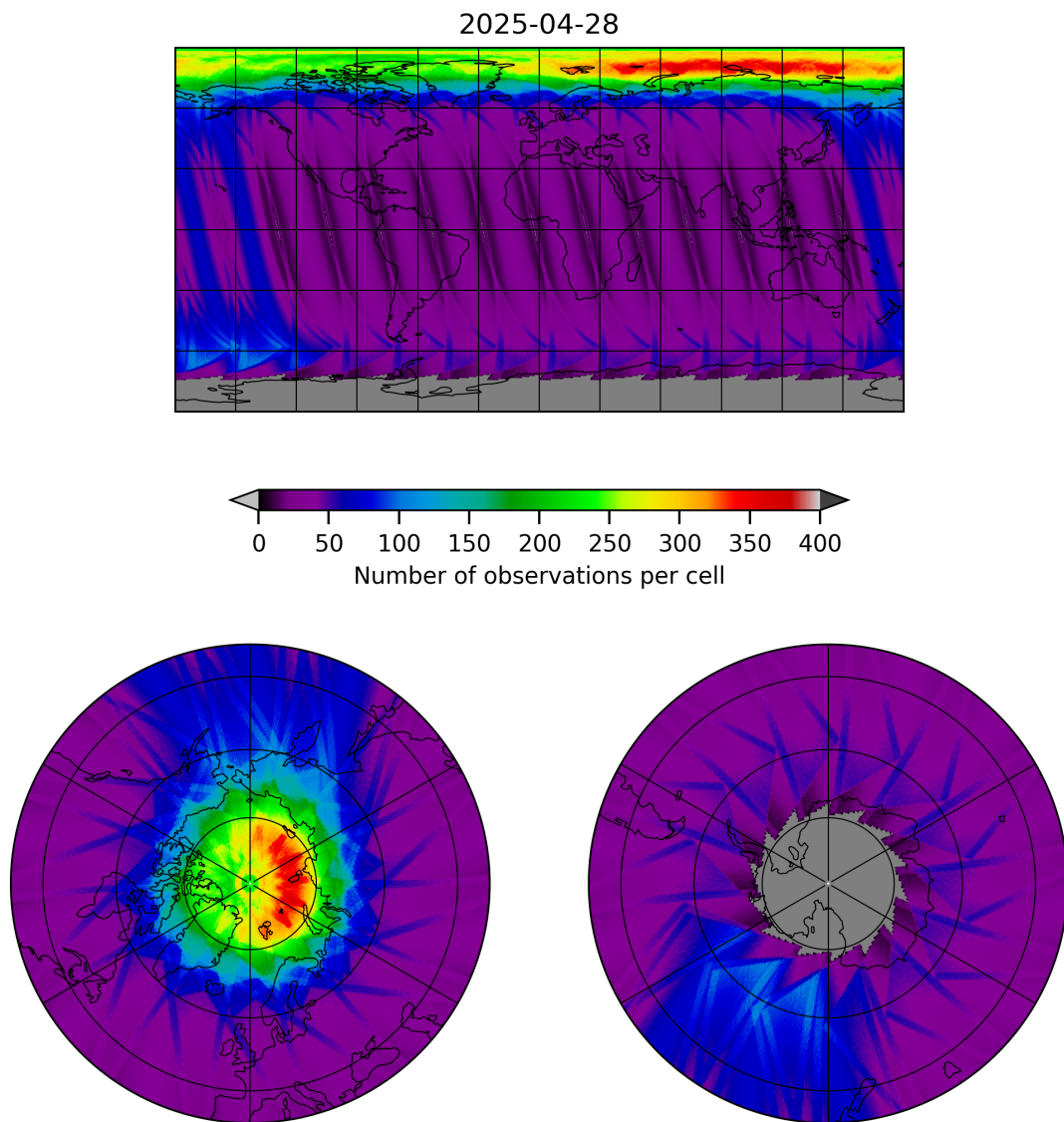
Figure 12: Map of the number of observations for 2025-04-27 to 2025-04-29
