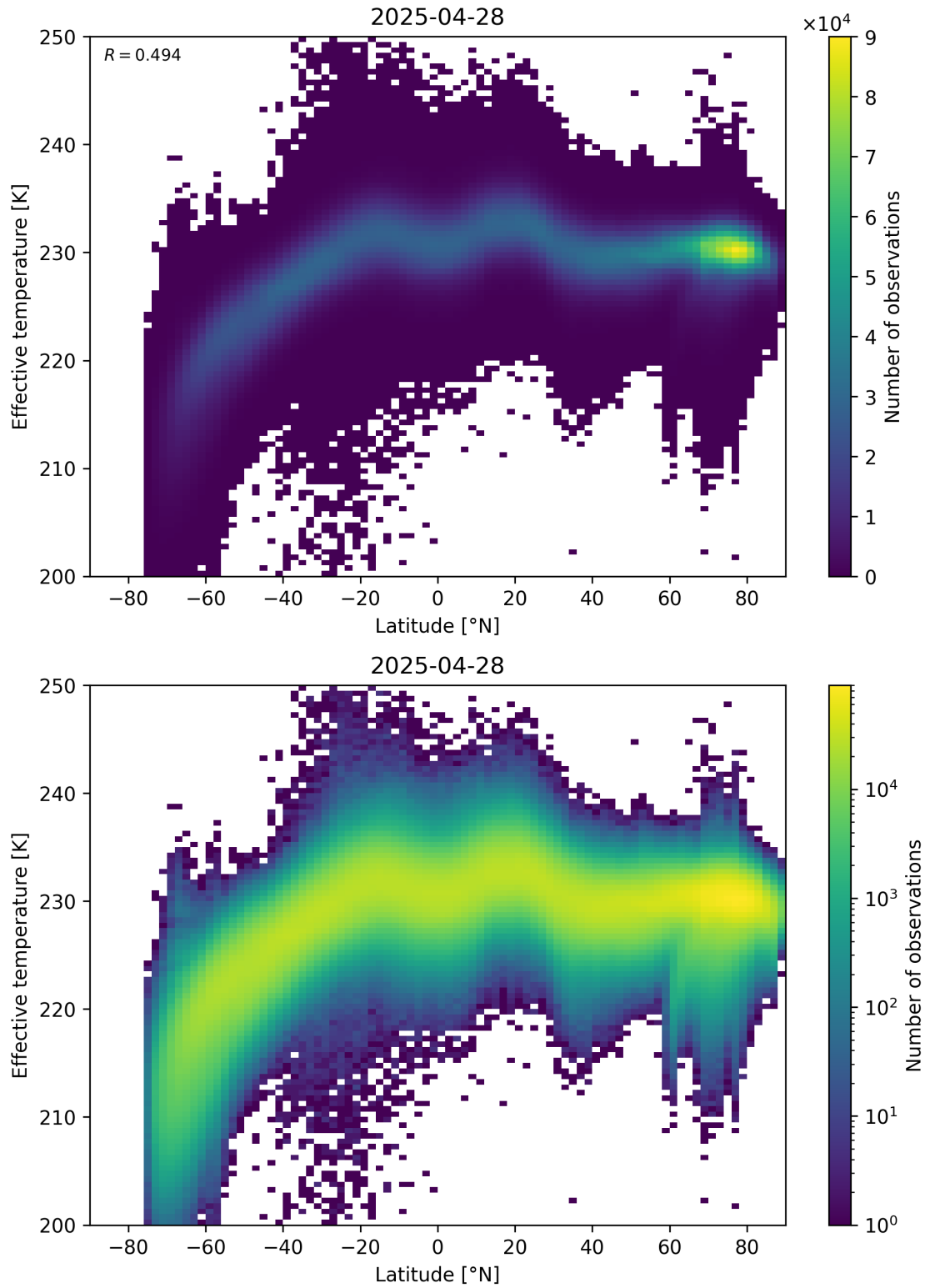
Figure 34: Scatter density plot of “Latitude” against “Effective temperature” for 2025-04-27 to 2025-04-29.
