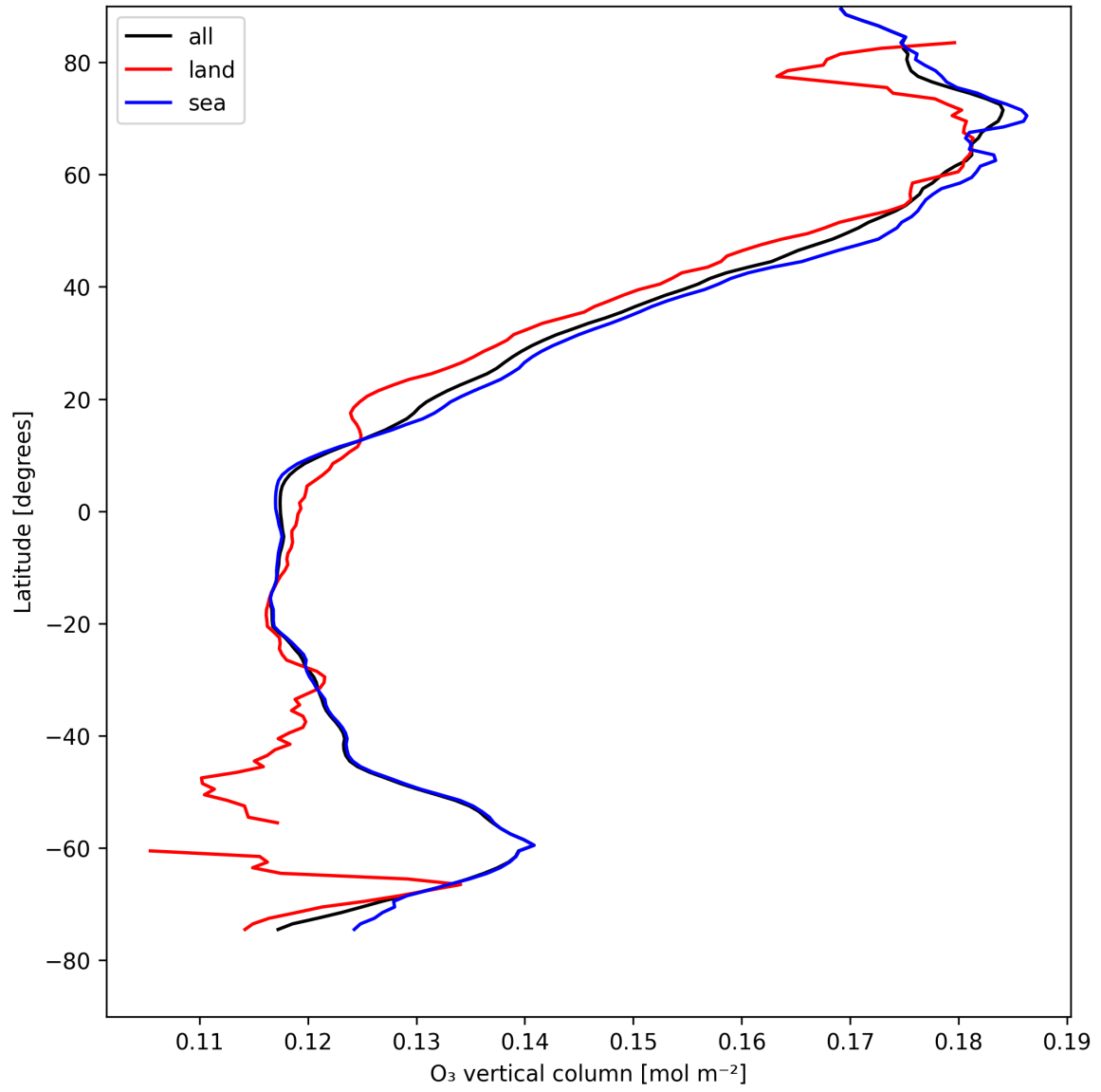
Figure 14: Zonal average of “O 3 vertical column” for 2025-04-27 to 2025-04-29.
