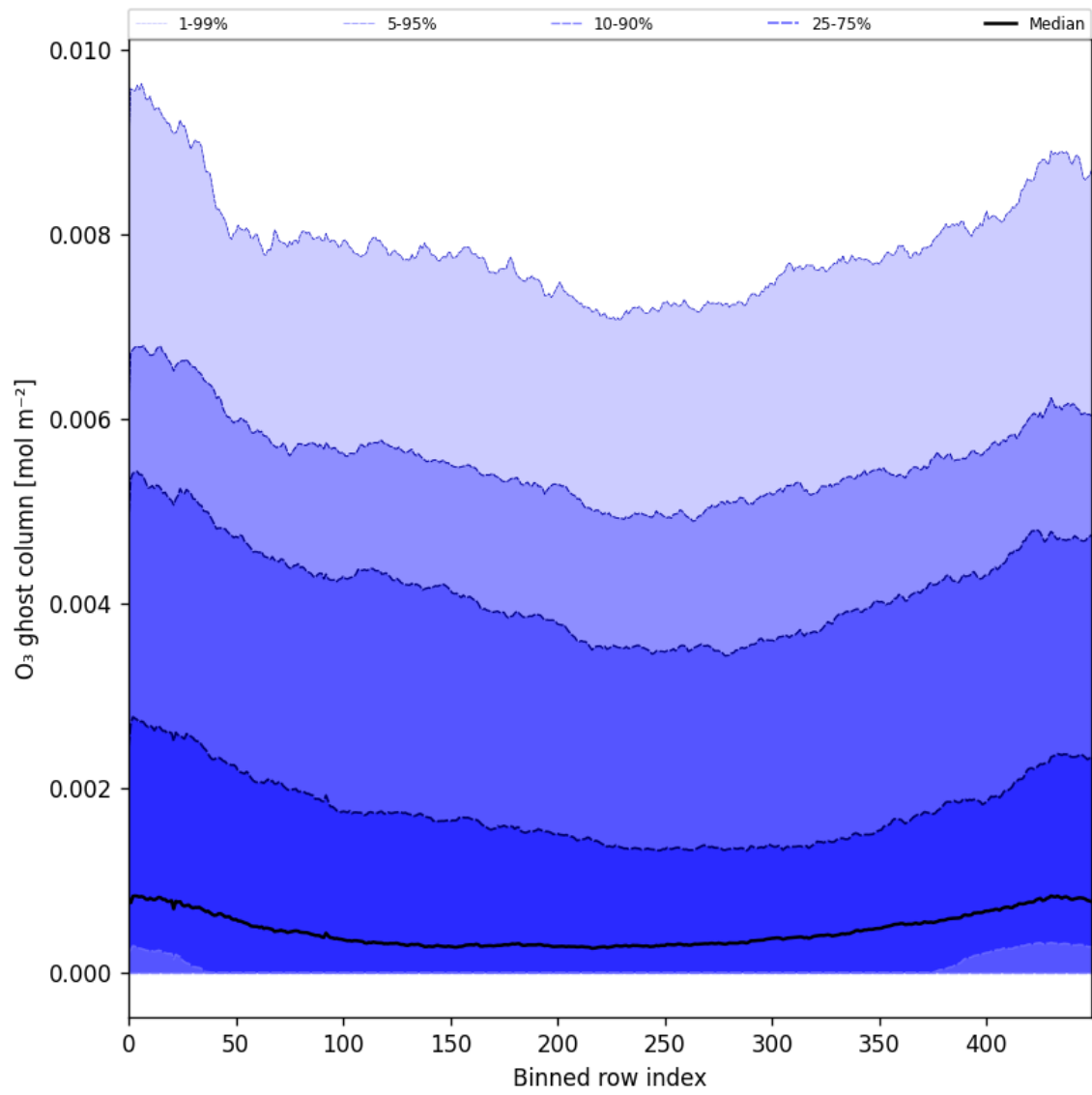
Figure 32: Along track statistics of “O 3 ghost column” for 2025-04-27 to 2025-04-29
