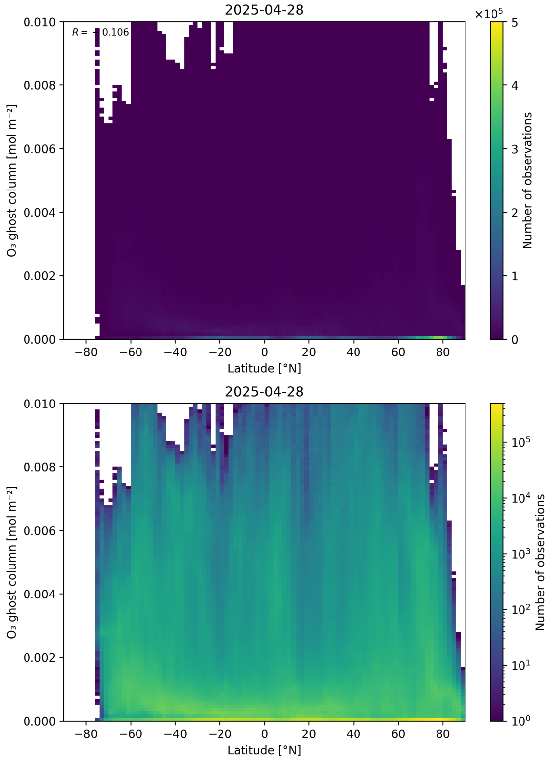
Figure 35: Scatter density plot of “Latitude” against “O 3 ghost column” for 2025-04-27 to 2025-04-29.
