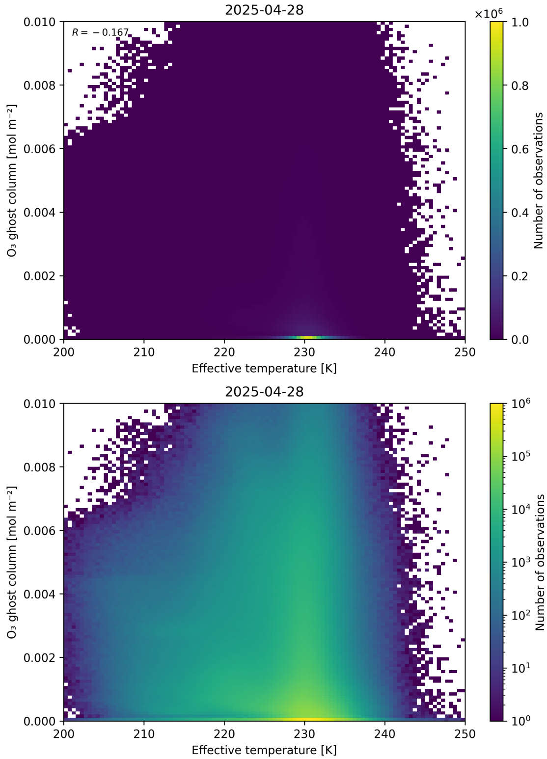
Figure 38: Scatter density plot of “Effective temperature” against “O 3 ghost column” for 2025-04-27 to 2025-04-29.
