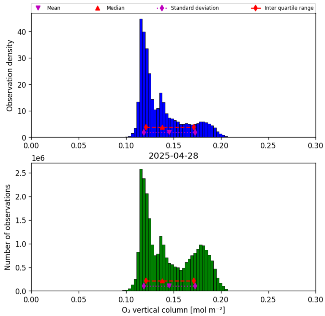
Figure 21: Histogram of “O 3 vertical column” for 2025-04-27 to 2025-04-29
