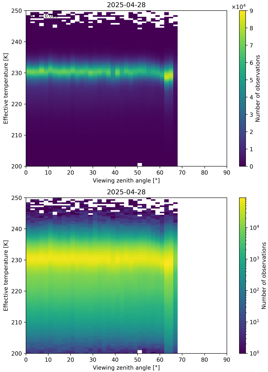
Figure 50: Scatter density plot of “Viewing zenith angle” against “Effective temperature” for 2025-04-27 to 2025-04-29.
