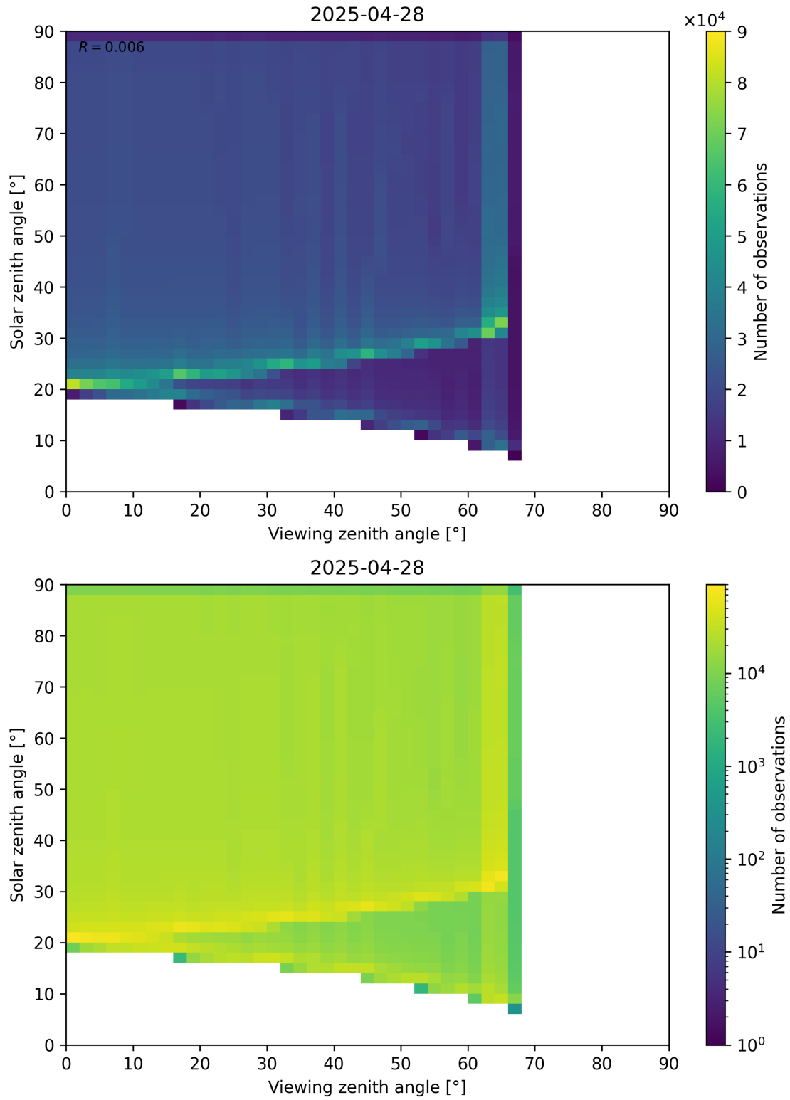
Figure 54: Scatter density plot of “Viewing zenith angle” against “Solar zenith angle” for 2025-04-27 to 2025-04-29.
