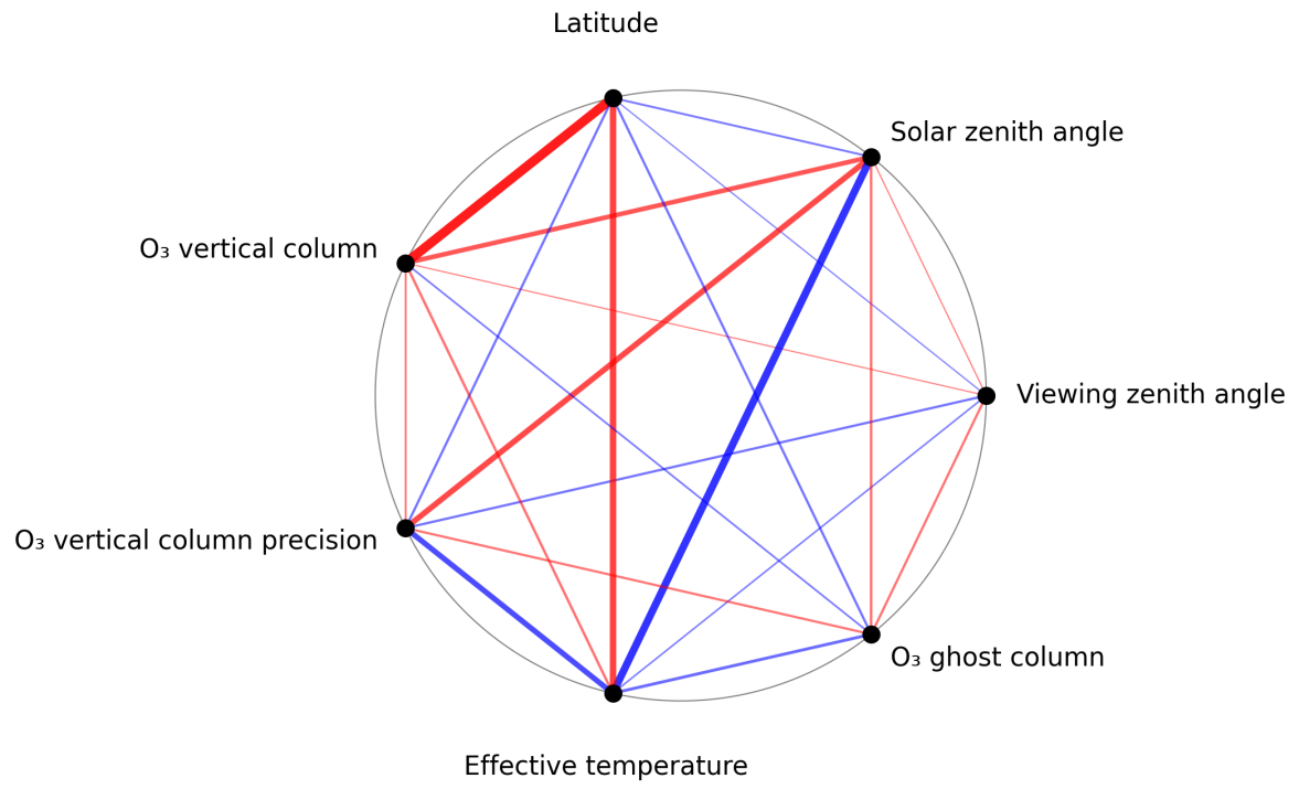
Figure 1: Map of correlation graph for 2025-04-27 to 2025-04-29.
