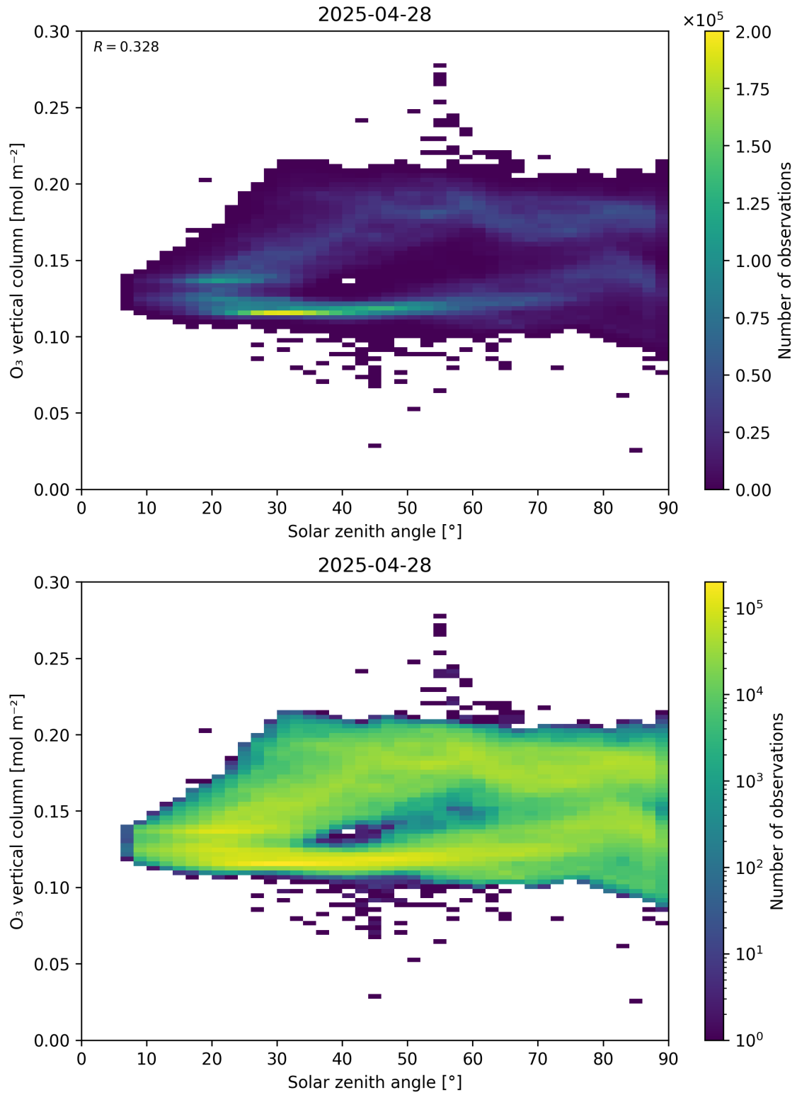
Figure 47: Scatter density plot of “Solar zenith angle” against “O 3 vertical column” for 2025-04-27 to 2025-04-29.
