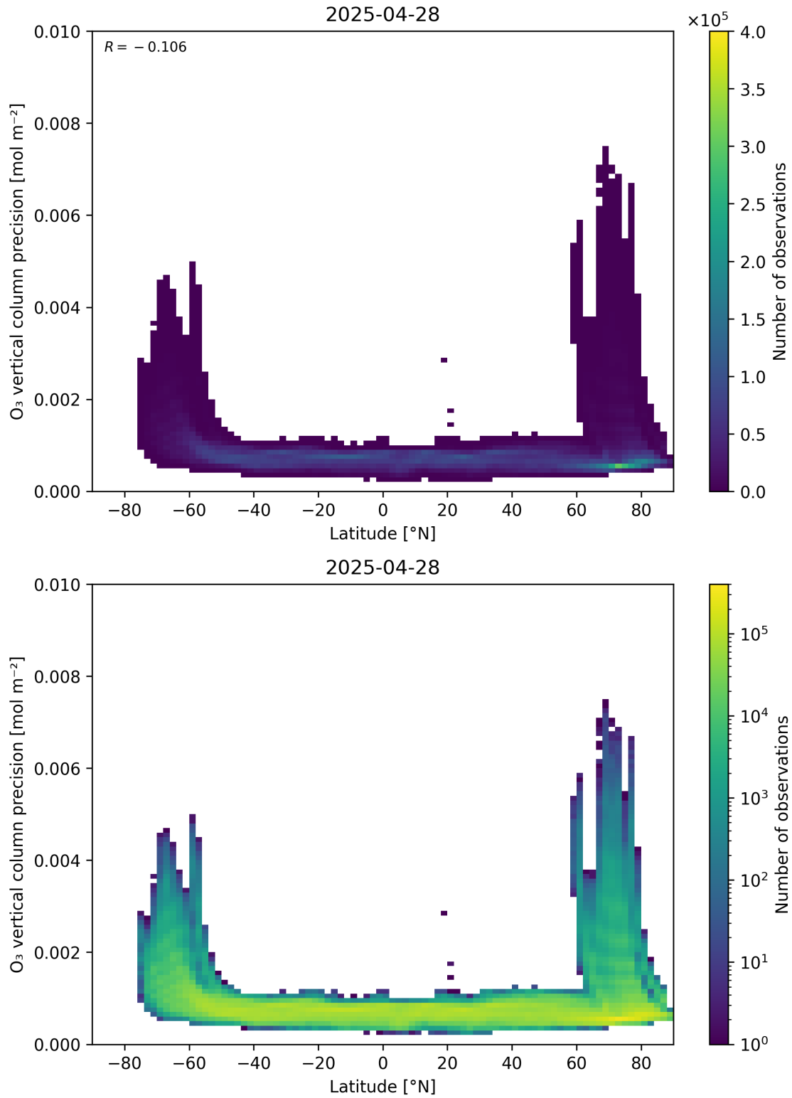
Figure 37: Scatter density plot of “Latitude” against “O 3 vertical column precision” for 2025-04-27 to 2025-04-29.
