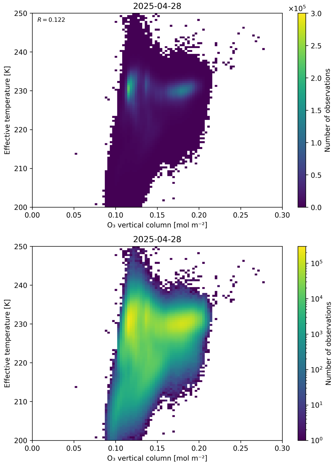
Figure 39: Scatter density plot of “O 3 vertical column” against “Effective temperature” for 2025-04-27 to 2025-04-29.
