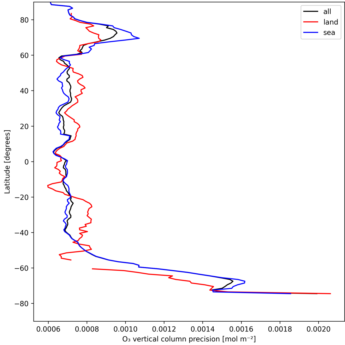
Figure 15: Zonal average of "O 3 vertical column precision" for 2025-04-27 to 2025-04-29.
