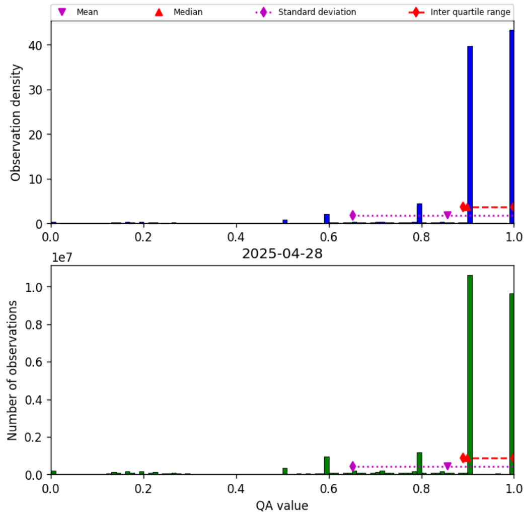
Figure 20: Histogram of “QA value” for 2025-04-27 to 2025-04-29
