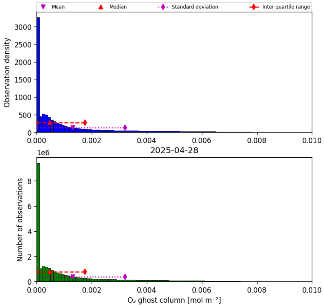
Figure 25: Histogram of “O 3 ghost column” for 2025-04-27 to 2025-04-29
