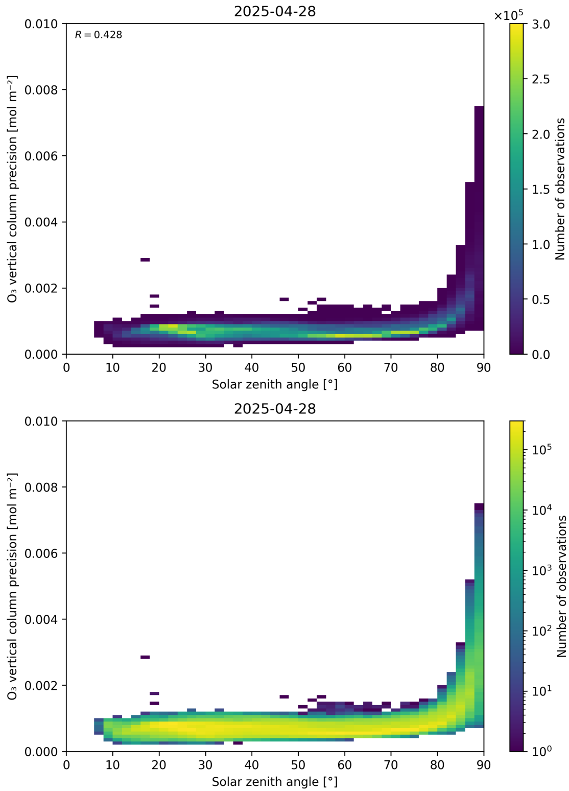
Figure 48: Scatter density plot of “Solar zenith angle” against “O 3 vertical column precision” for 2025-04-27 to 2025-04-29.
