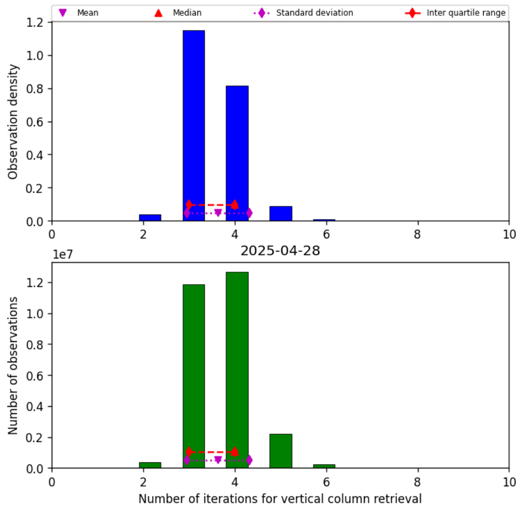
Figure 26: Histogram of “Number of iterations for vertical column retrieval” for 2025-04-27 to 2025-04-29
