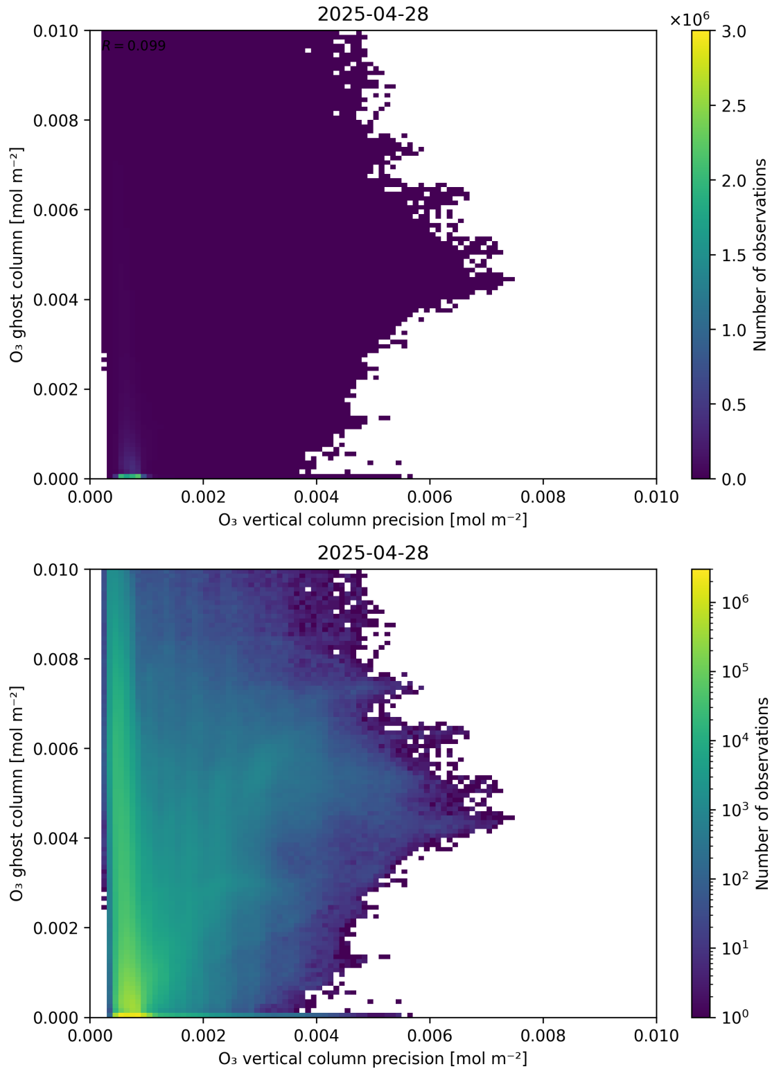
Figure 43: Scatter density plot of “O 3 vertical column precision” against “O 3 ghost column” for 2025-04-27 to 2025-04-29.
