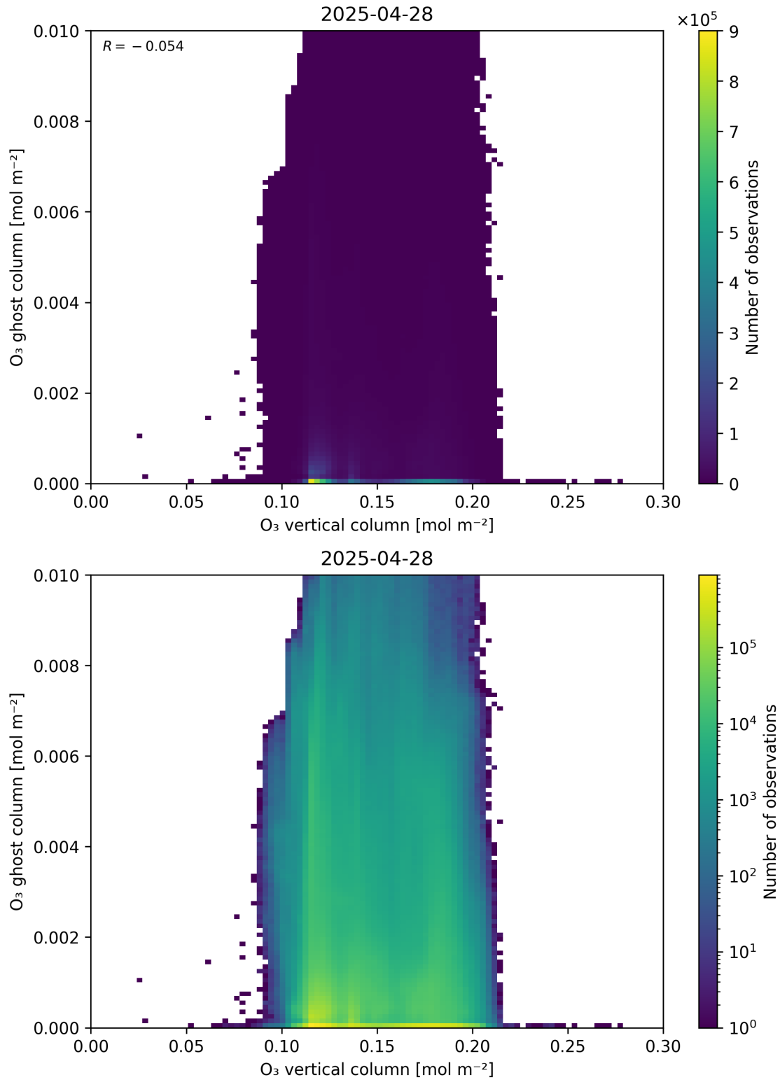
Figure 40: Scatter density plot of “O 3 vertical column” against “O 3 ghost column” for 2025-04-27 to 2025-04-29.
