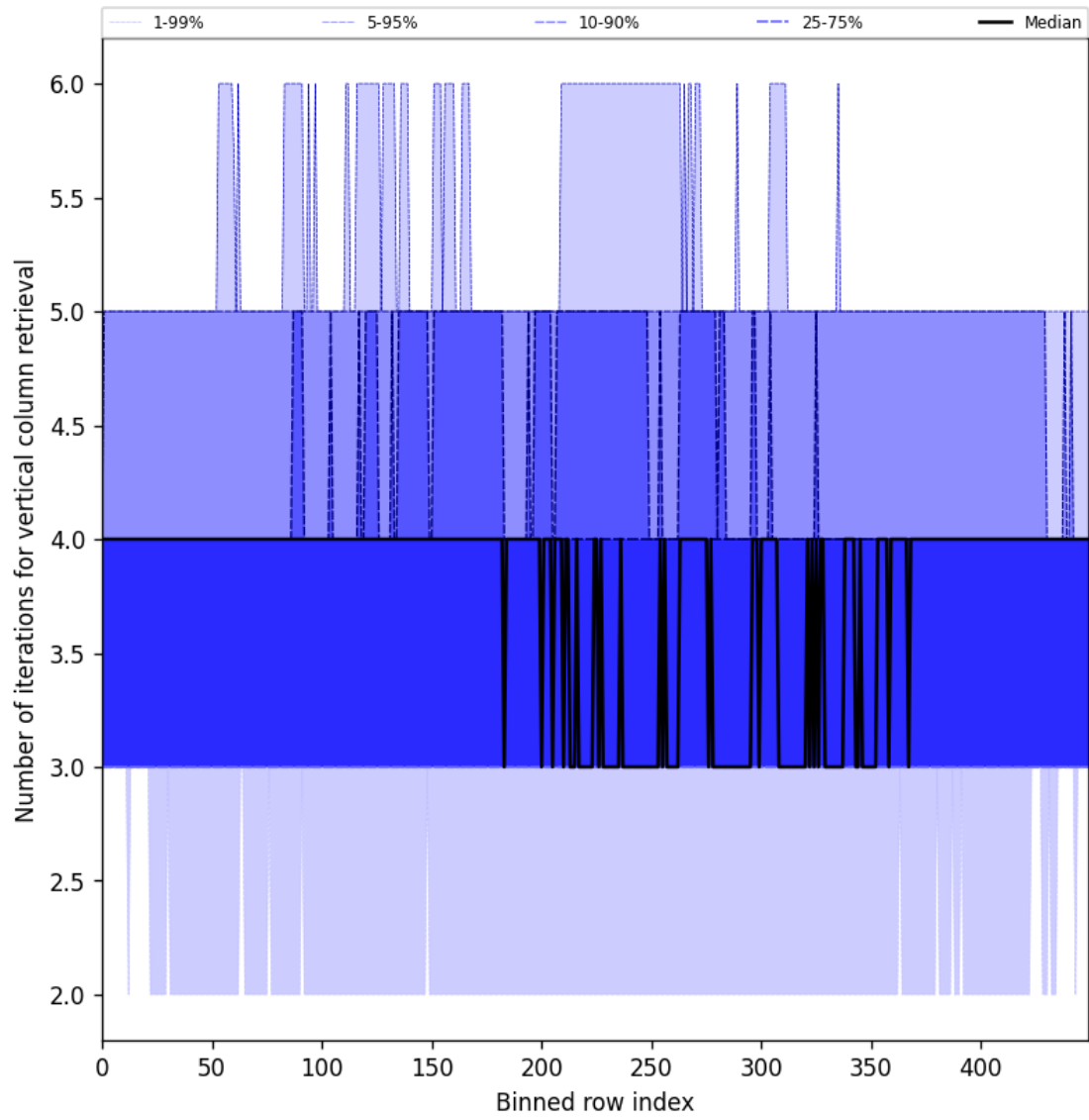
Figure 33: Along track statistics of “Number of iterations for vertical column retrieval” for 2025-04-27 to 2025-04-29
