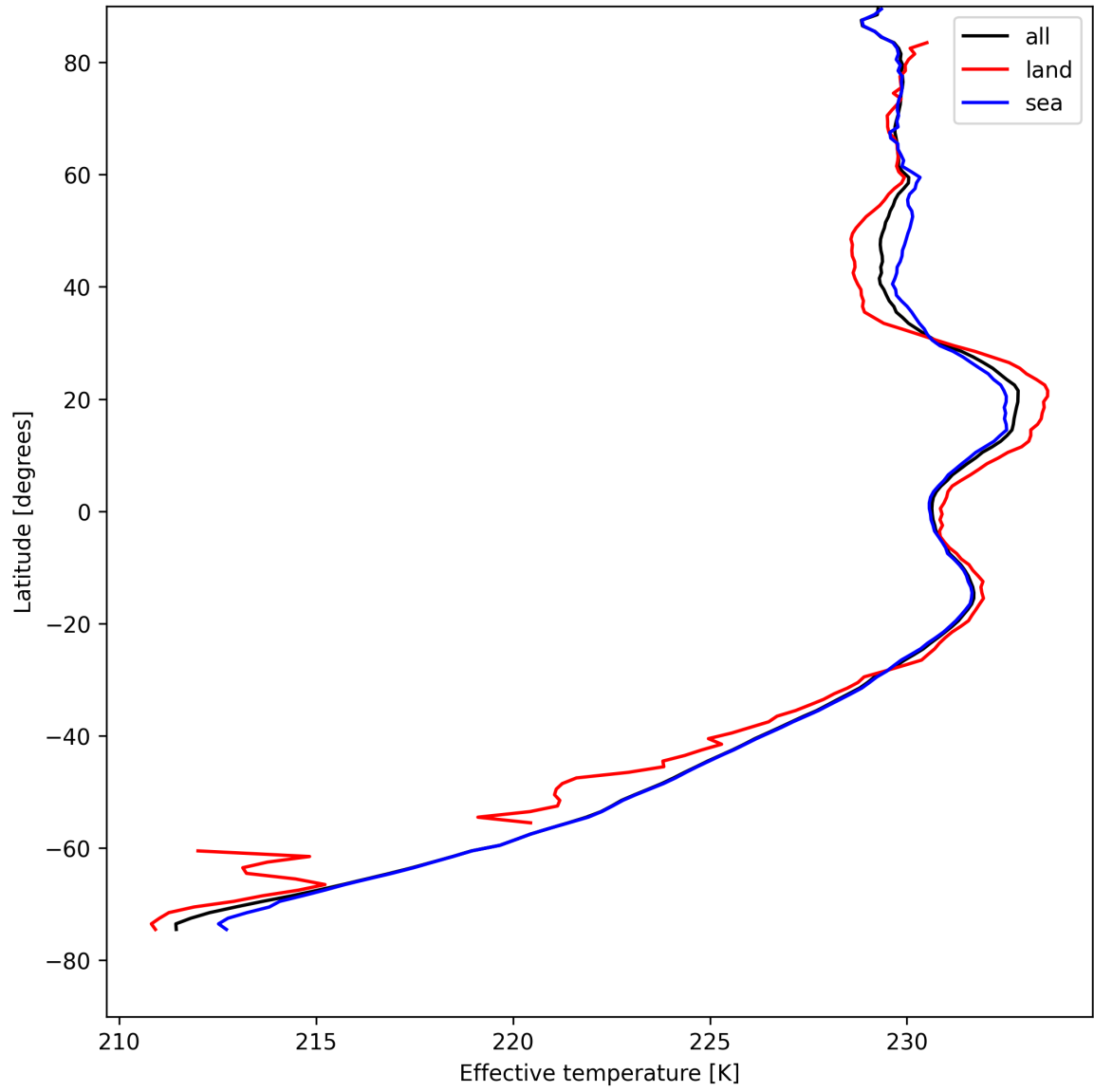
Figure 17: Zonal average of "Effective temperature" for 2025-04-27 to 2025-04-29.
