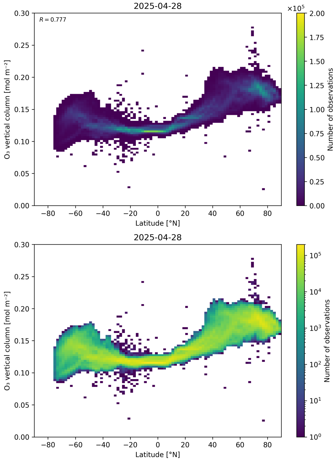
Figure 36: Scatter density plot of “Latitude” against “O 3 vertical column” for 2025-04-27 to 2025-04-29.
