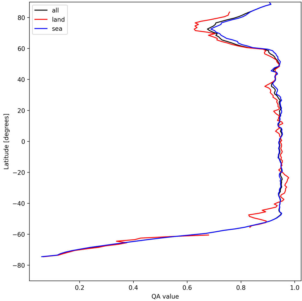
Figure 13: Zonal average of “QA value” for 2025-04-27 to 2025-04-29.
