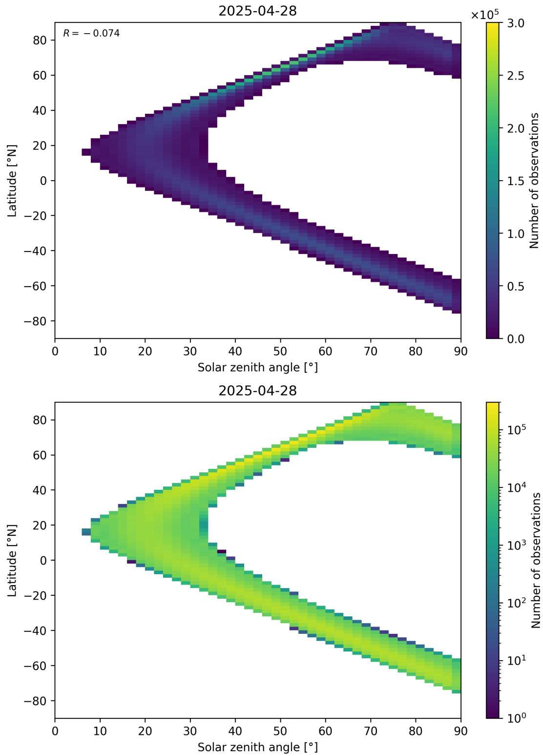
Figure 44: Scatter density plot of “Solar zenith angle” against “Latitude” for 2025-04-27 to 2025-04-29.
