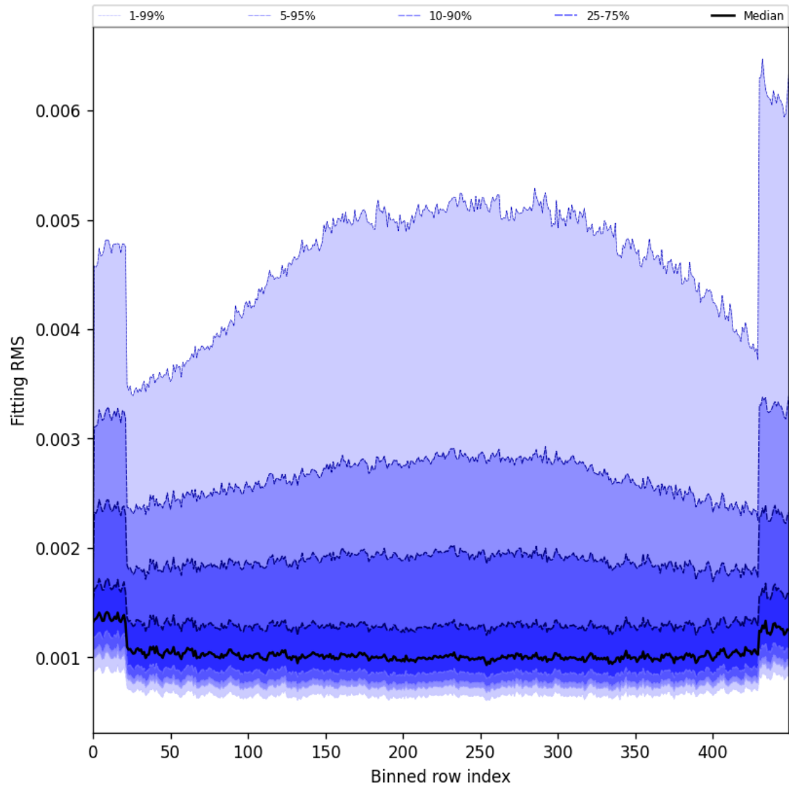
Figure 30: Along track statistics of “Fitting RMS” for 2025-04-27 to 2025-04-29
