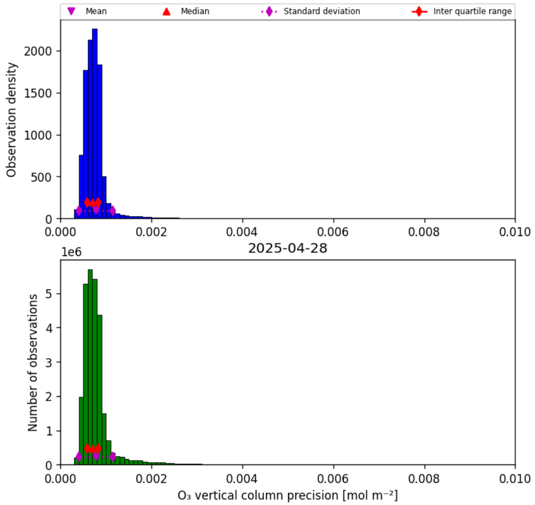
Figure 22: Histogram of “O 3 vertical column precision” for 2025-04-27 to 2025-04-29
