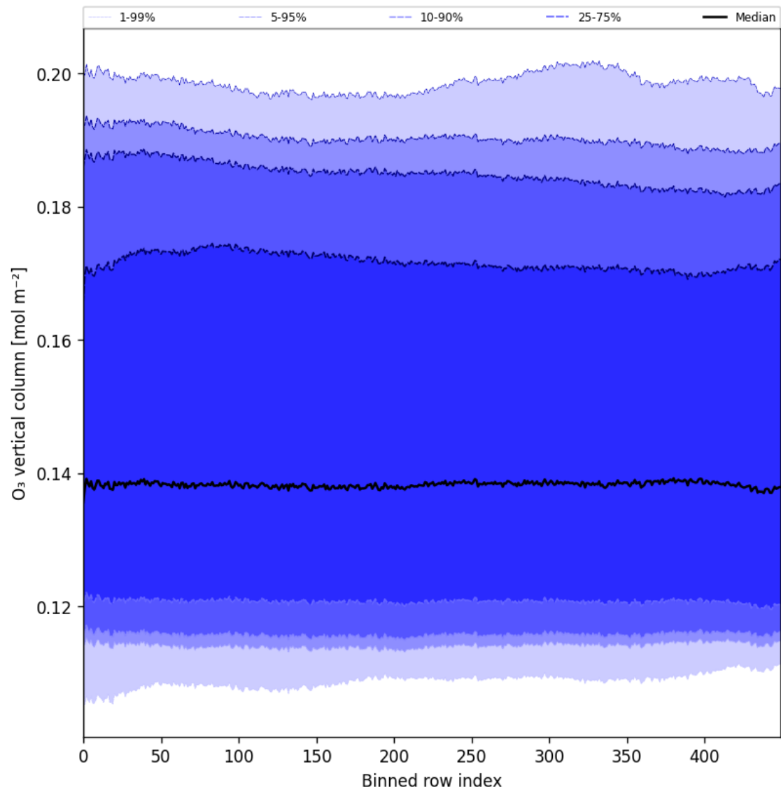
Figure 28: Along track statistics of “O 3 vertical column” for 2025-04-27 to 2025-04-29
