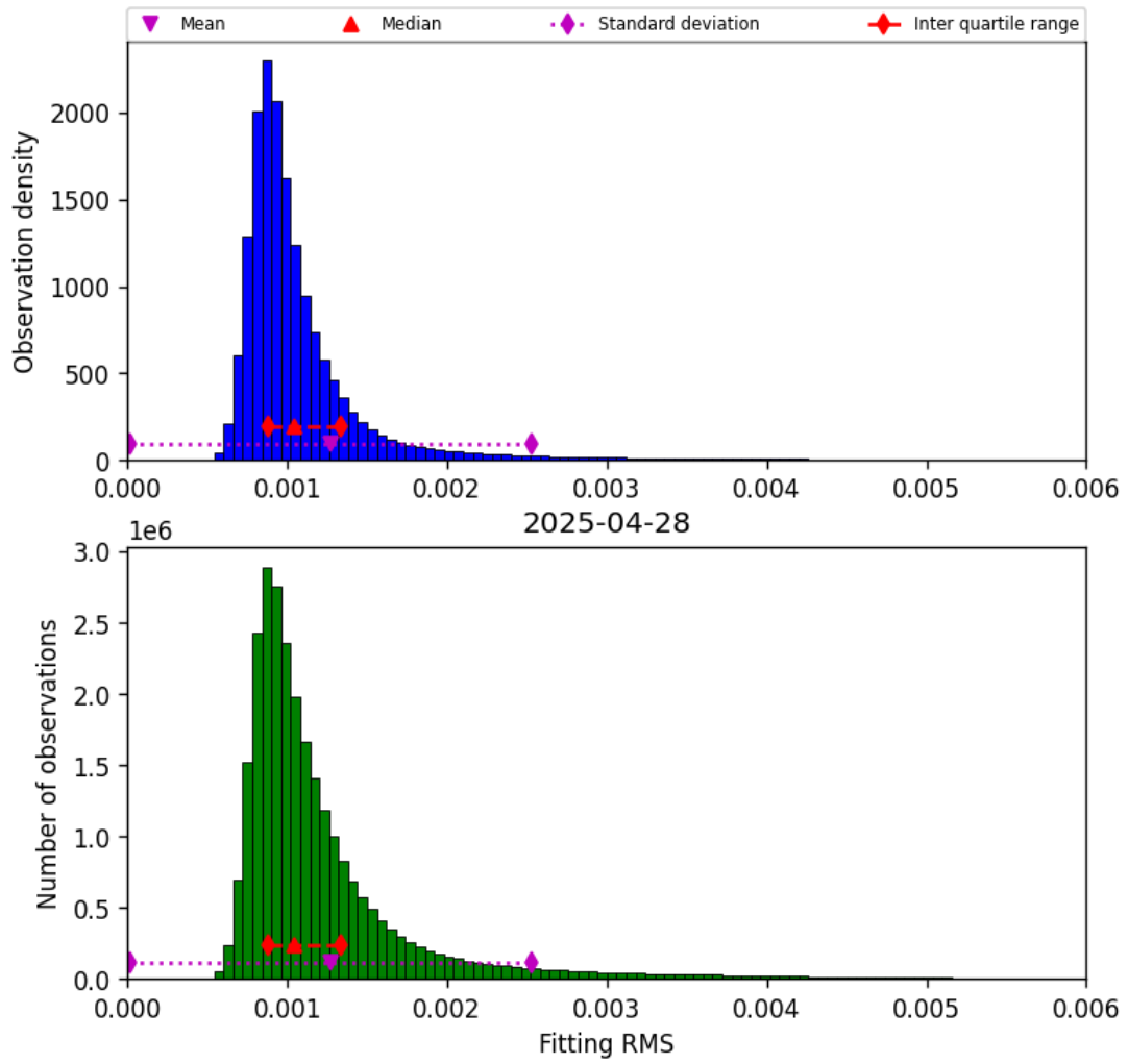
Figure 23: Histogram of “Fitting RMS” for 2025-04-27 to 2025-04-29
