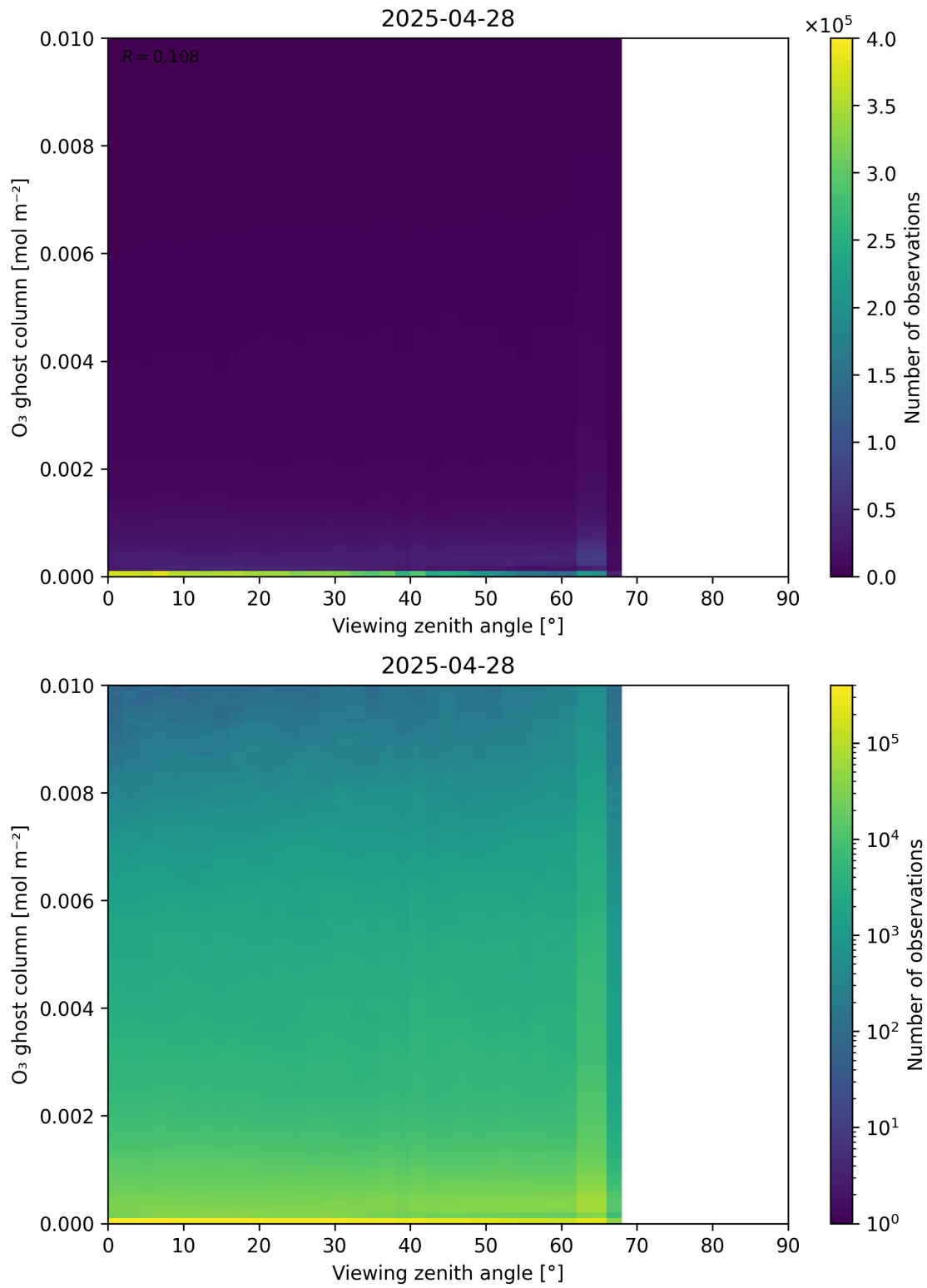
Figure 51: Scatter density plot of “Viewing zenith angle” against “O 3 ghost column” for 2025-04-27 to 2025-04-29.
