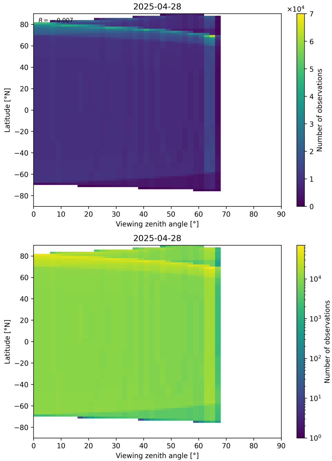
Figure 49: Scatter density plot of “Viewing zenith angle” against “Latitude” for 2025-04-27 to 2025-04-29.
