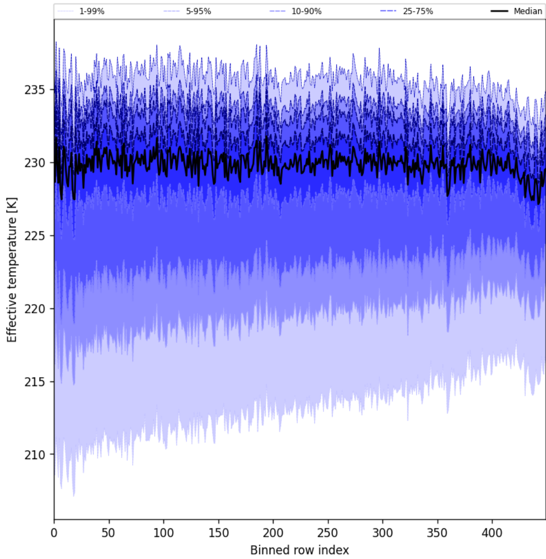
Figure 31: Along track statistics of “Effective temperature” for 2025-04-27 to 2025-04-29
