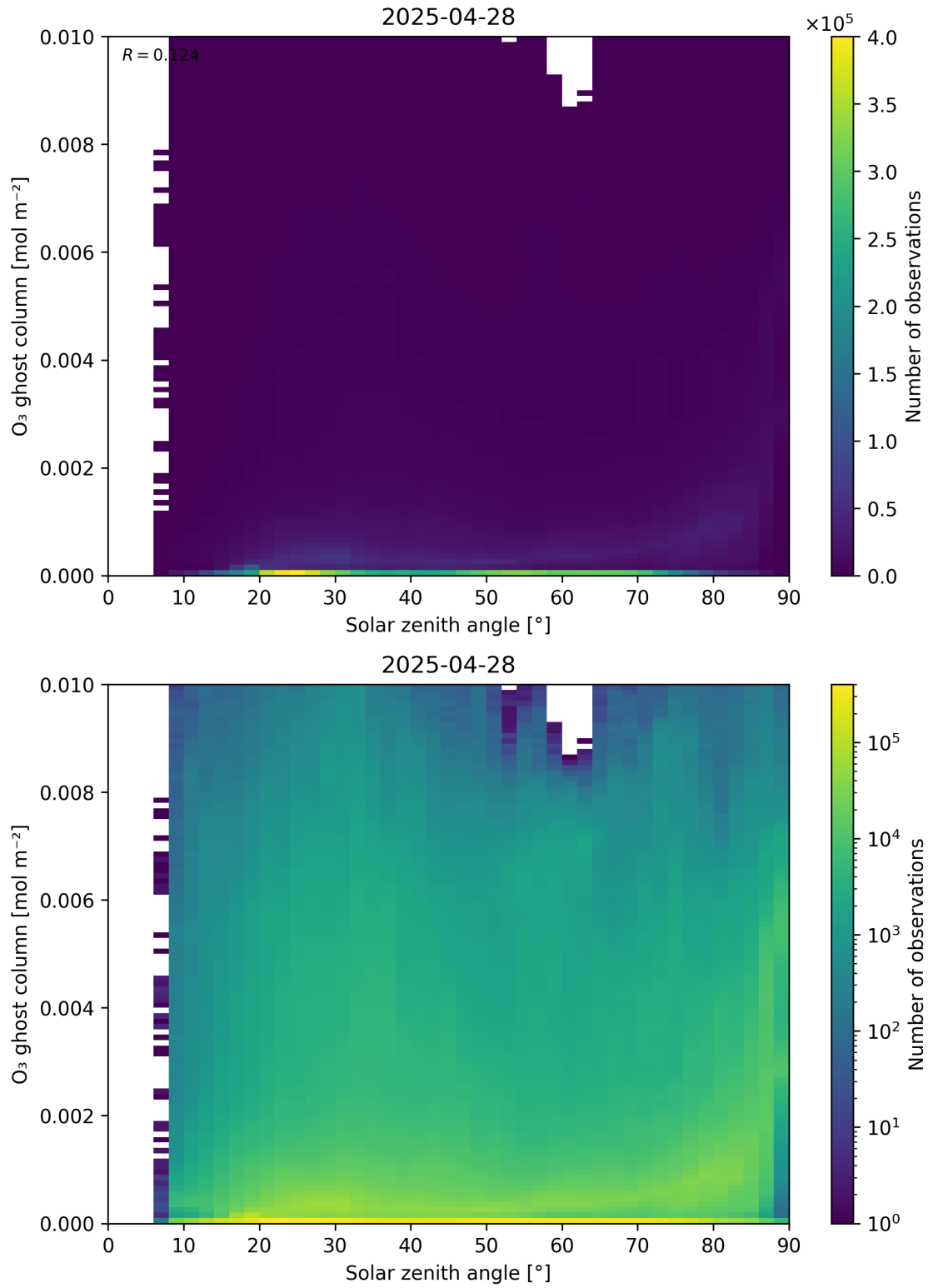
Figure 46: Scatter density plot of “Solar zenith angle” against “O 3 ghost column” for 2025-04-27 to 2025-04-29.
