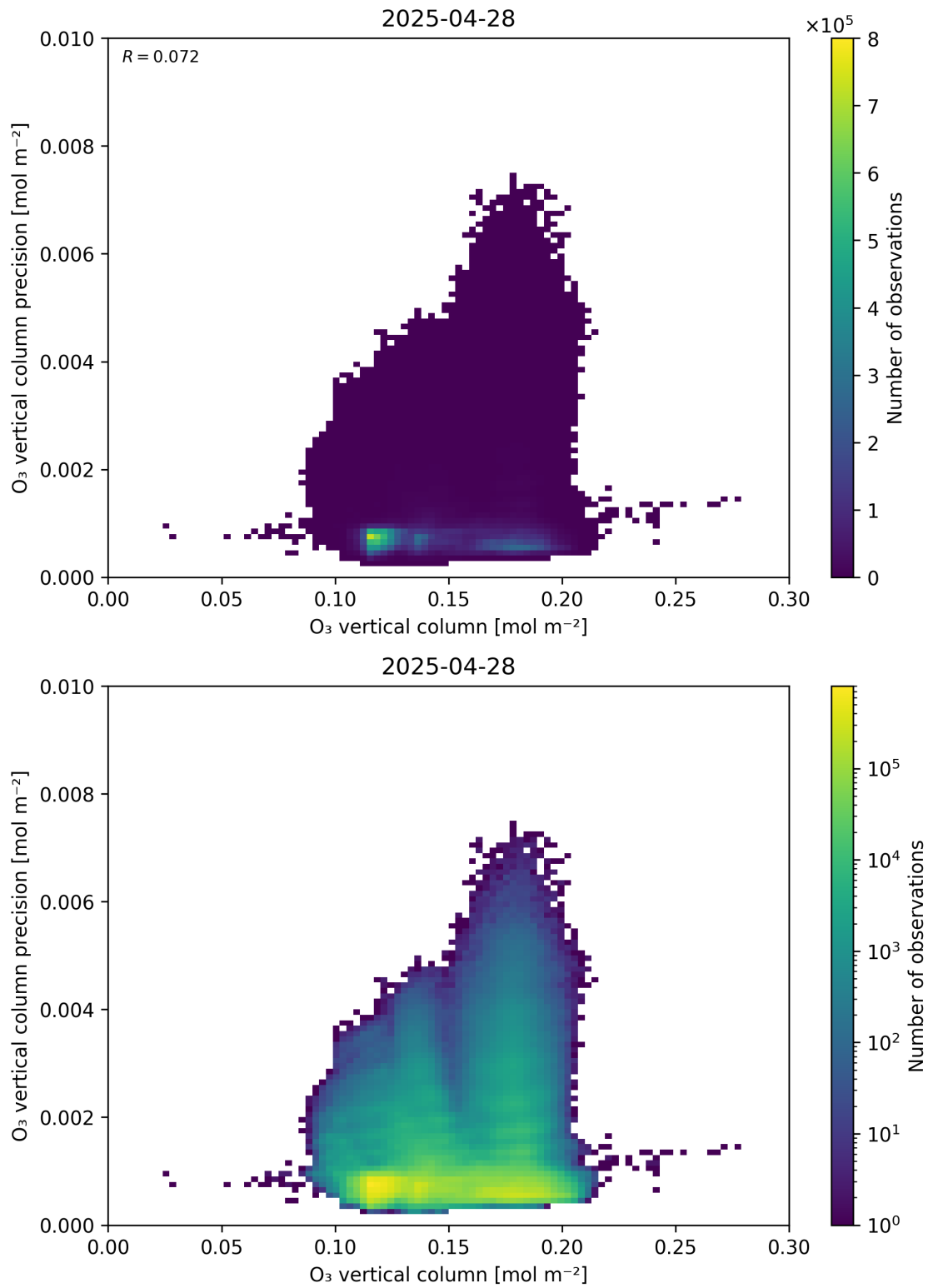
Figure 41: Scatter density plot of “O 3 vertical column” against “O 3 vertical column precision” for 2025-04-27 to 2025-04-29.
