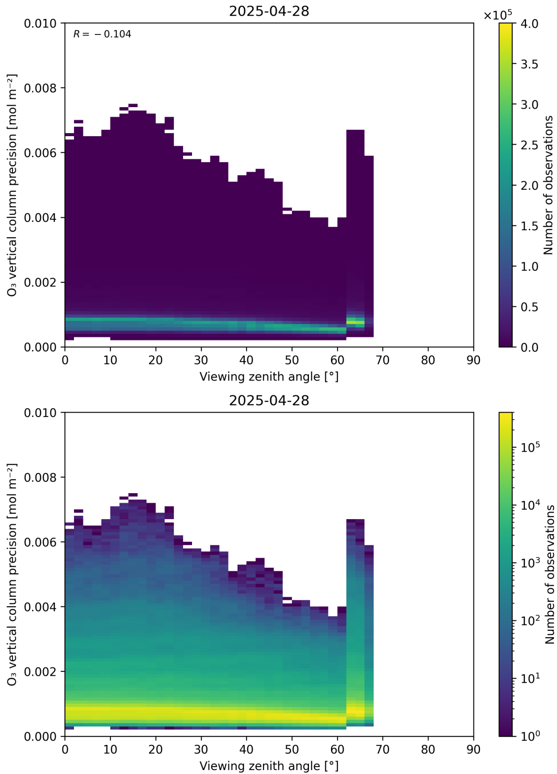
Figure 53: Scatter density plot of “Viewing zenith angle” against “O 3 vertical column precision” for 2025-04-27 to 2025-04-29.
