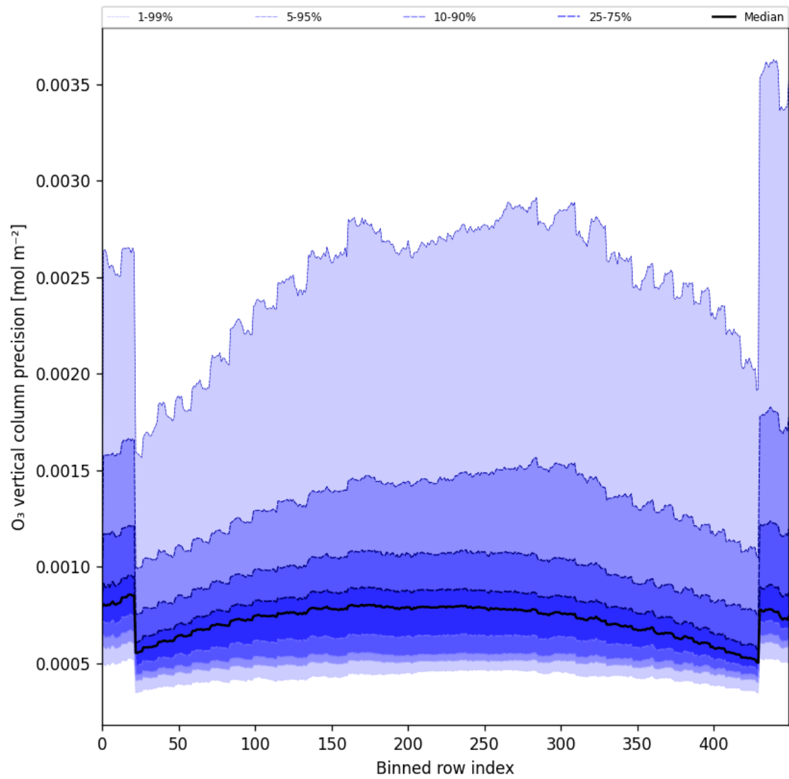
Figure 29: Along track statistics of “O 3 vertical column precision” for 2025-04-27 to 2025-04-29
