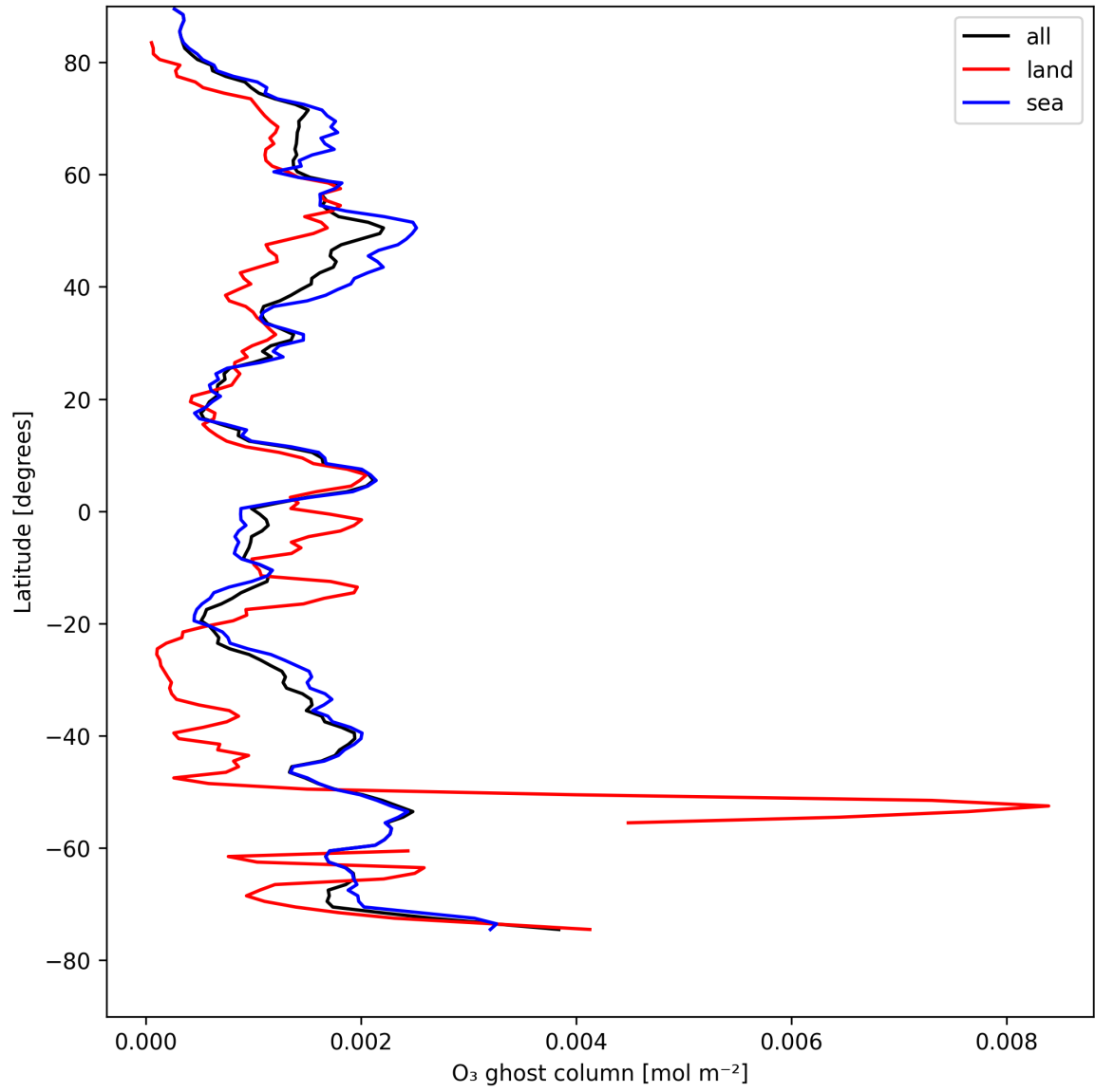
Figure 18: Zonal average of “O 3 ghost column” for 2025-04-27 to 2025-04-29.
