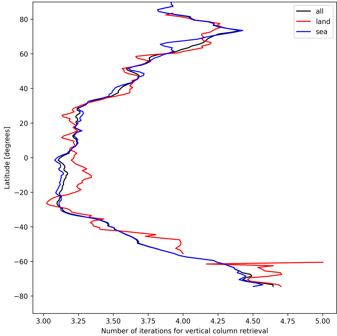
Figure 19: Zonal average of “Number of iterations for vertical column retrieval” for 2025-04-27 to 2025-04-29.
