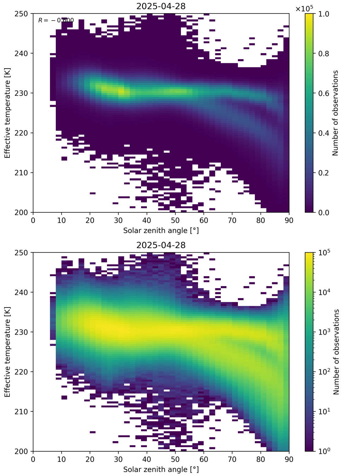
Figure 45: Scatter density plot of “Solar zenith angle” against “Effective temperature” for 2025-04-27 to 2025-04-29.
