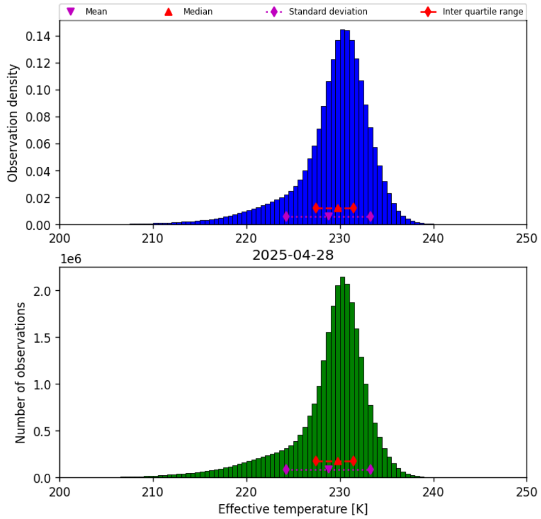
Figure 24: Histogram of “Effective temperature” for 2025-04-27 to 2025-04-29
