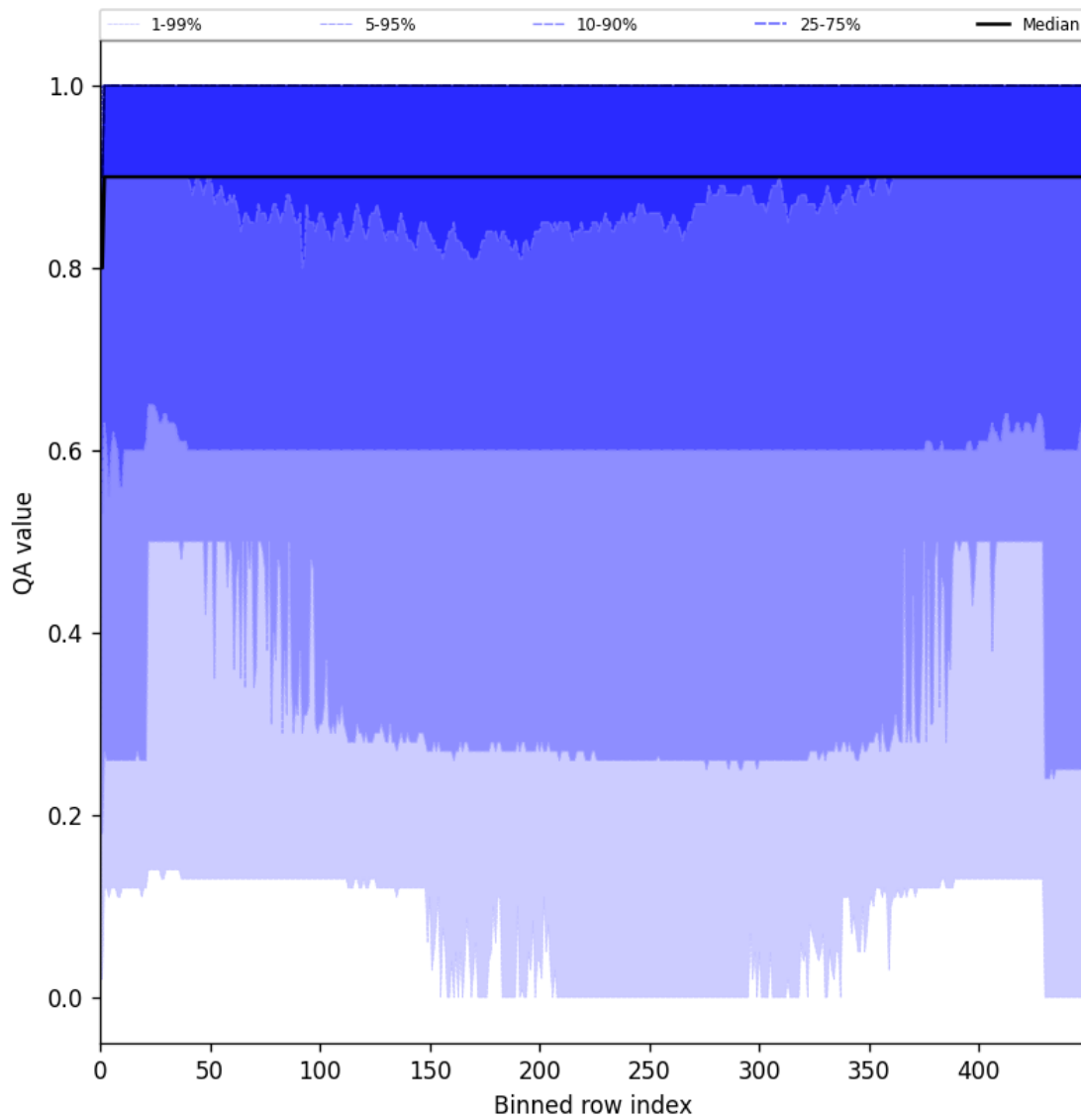
Figure 27: Along track statistics of “QA value” for 2025-04-27 to 2025-04-29
