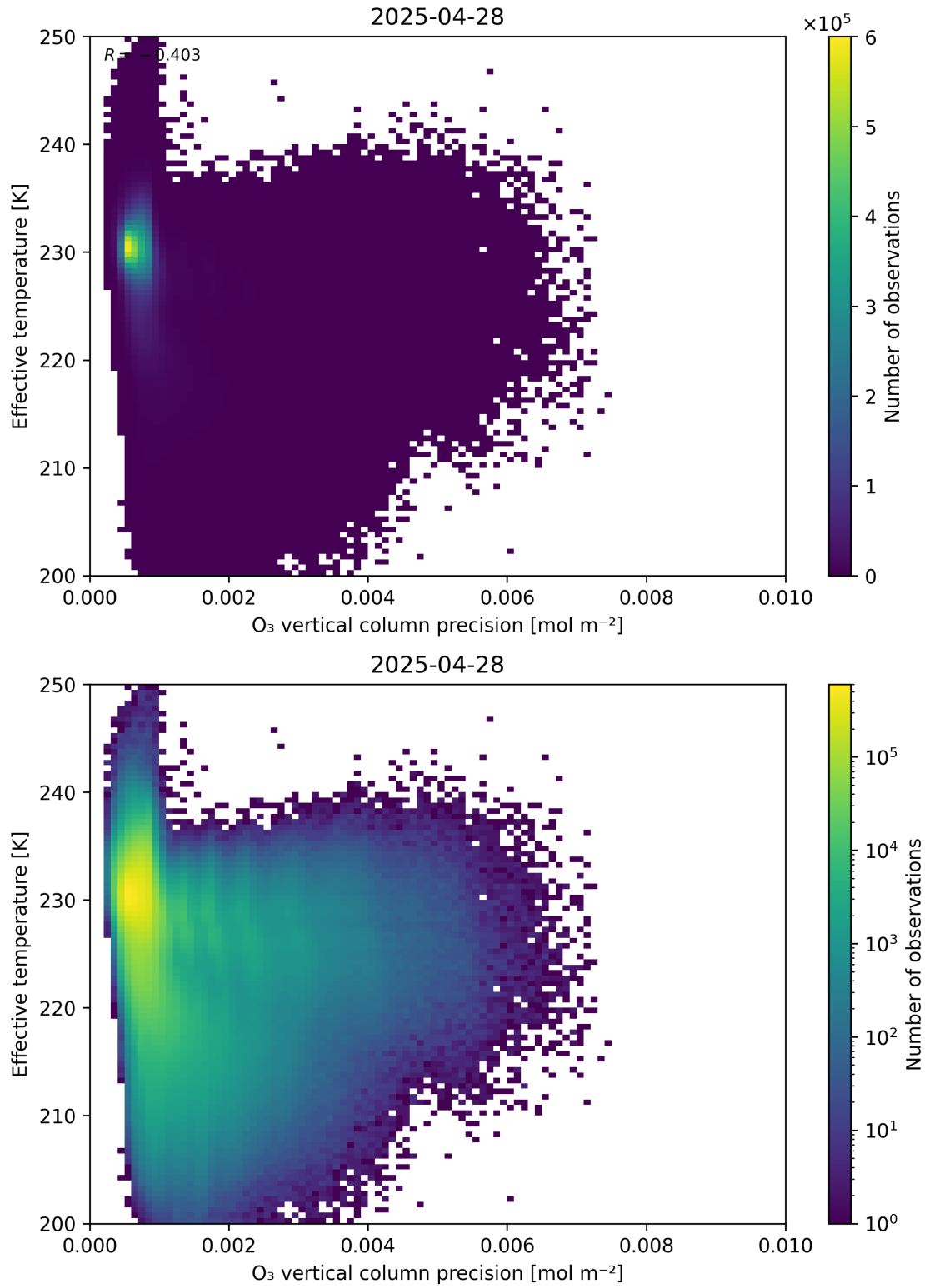
Figure 42: Scatter density plot of “O 3 vertical column precision” against “Effective temperature” for 2025-04-27 to 2025-04-29.
