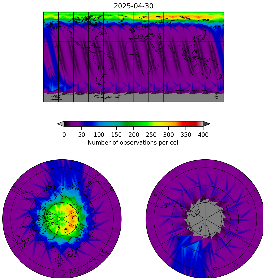
Figure 12: Map of the number of observations for 2025-04-29 to 2025-05-01
