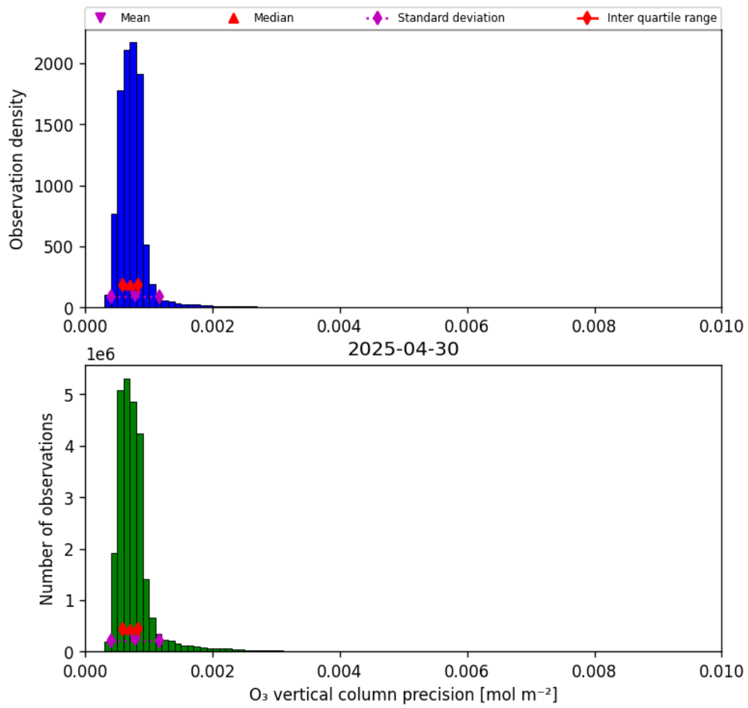
Figure 22: Histogram of “O 3 vertical column precision” for 2025-04-29 to 2025-05-01
