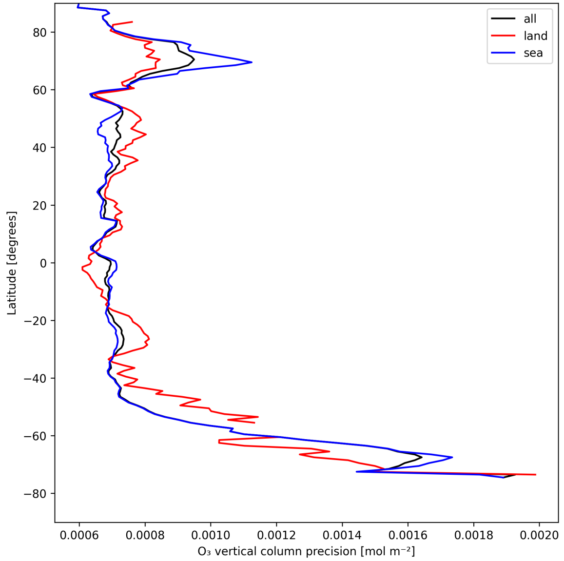
Figure 15: Zonal average of “O 3 vertical column precision” for 2025-04-29 to 2025-05-01.
