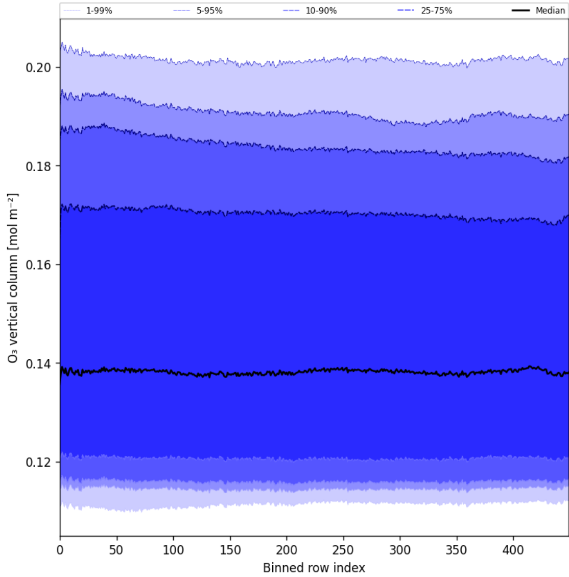
Figure 28: Along track statistics of “O 3 vertical column” for 2025-04-29 to 2025-05-01
