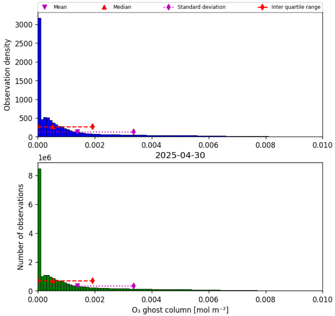
Figure 25: Histogram of “O 3 ghost column” for 2025-04-29 to 2025-05-01
