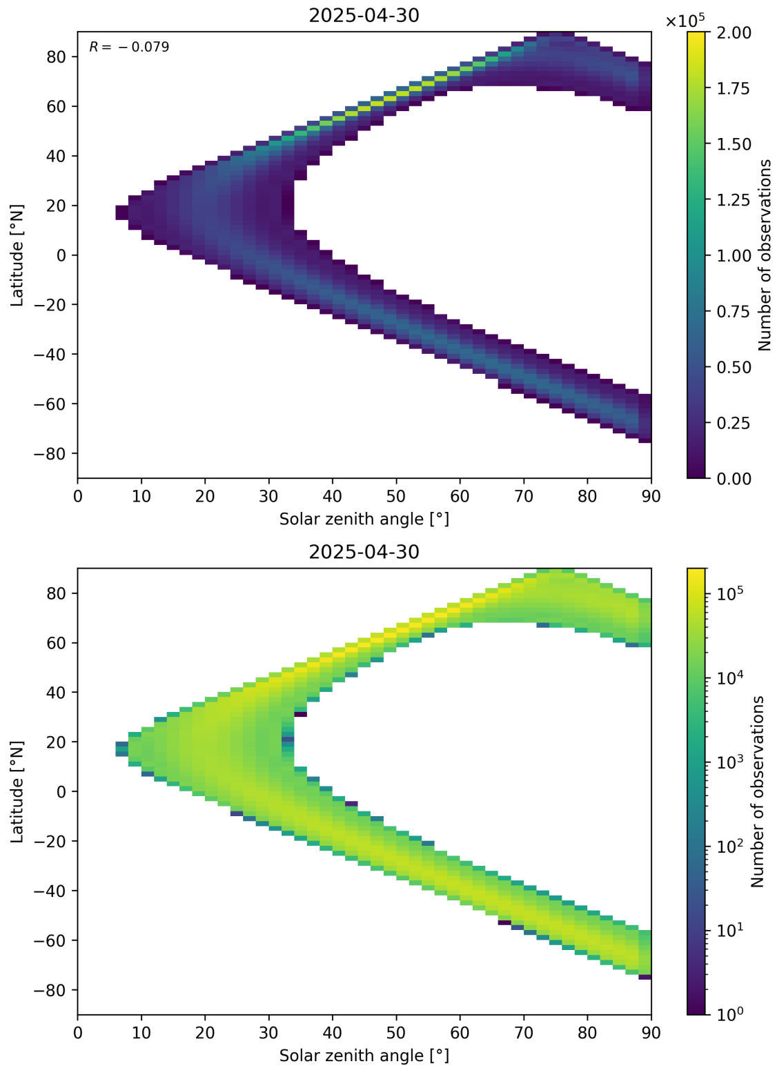
Figure 44: Scatter density plot of “Solar zenith angle” against “Latitude” for 2025-04-29 to 2025-05-01.
