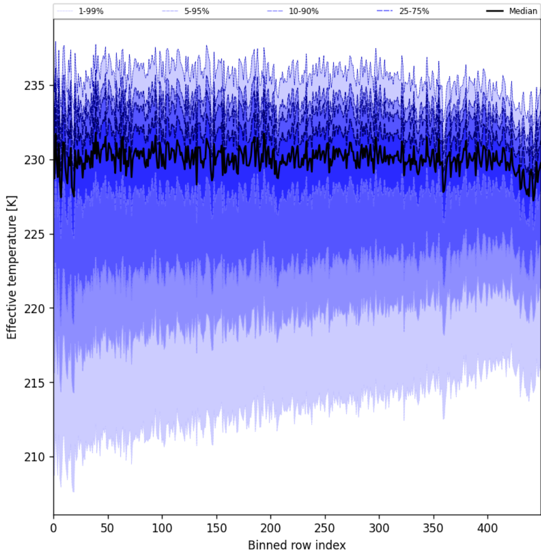
Figure 31: Along track statistics of “Effective temperature” for 2025-04-29 to 2025-05-01
