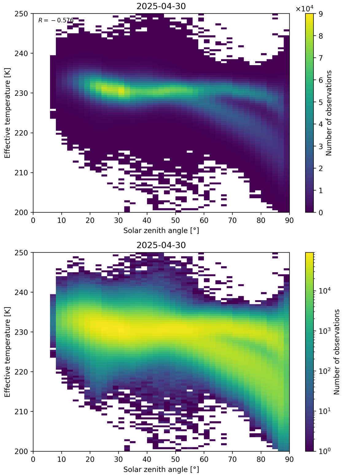
Figure 45: Scatter density plot of “Solar zenith angle” against “Effective temperature” for 2025-04-29 to 2025-05-01.
