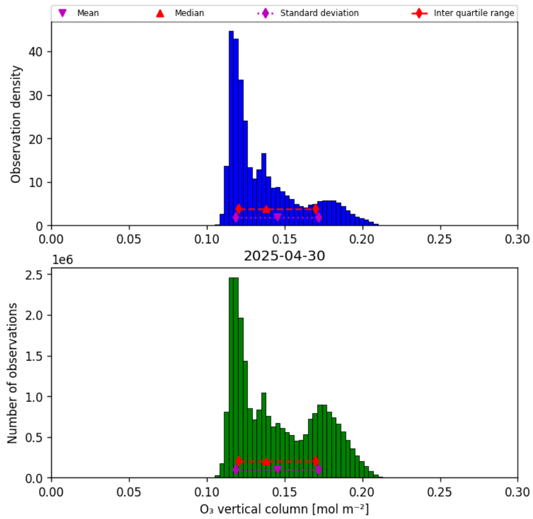
Figure 21: Histogram of “O 3 vertical column” for 2025-04-29 to 2025-05-01
