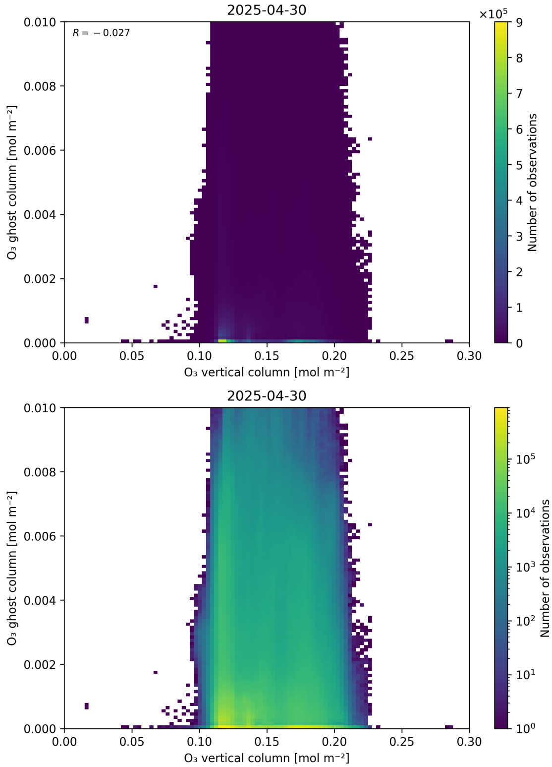
Figure 40: Scatter density plot of “ O_3 vertical column” against “ O_3 ghost column” for 2025-04-29 to 2025-05-01.
