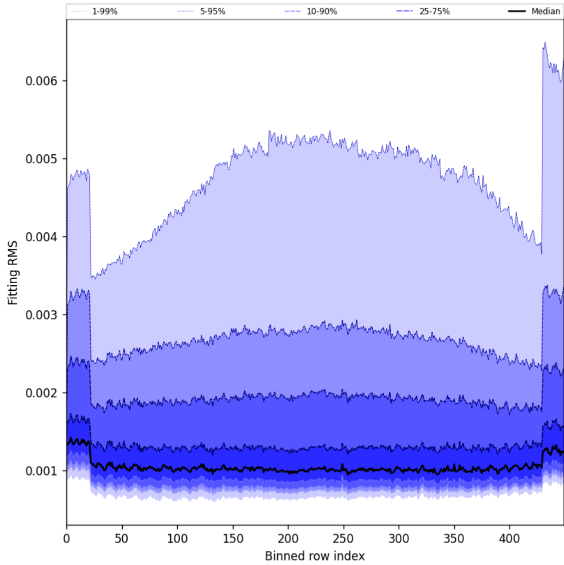
Figure 30: Along track statistics of “Fitting RMS” for 2025-04-29 to 2025-05-01
