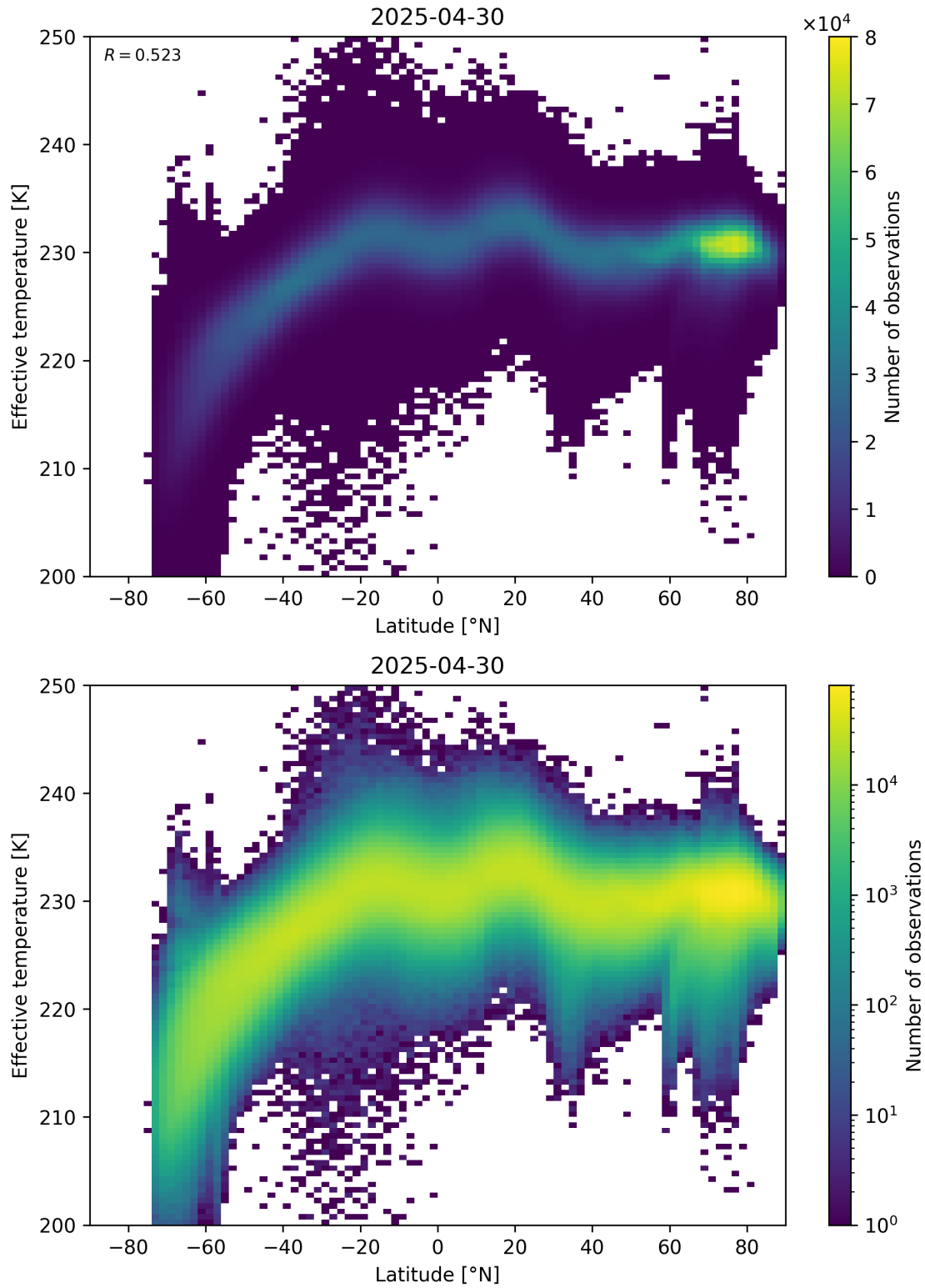
Figure 34: Scatter density plot of “Latitude” against “Effective temperature” for 2025-04-29 to 2025-05-01.
