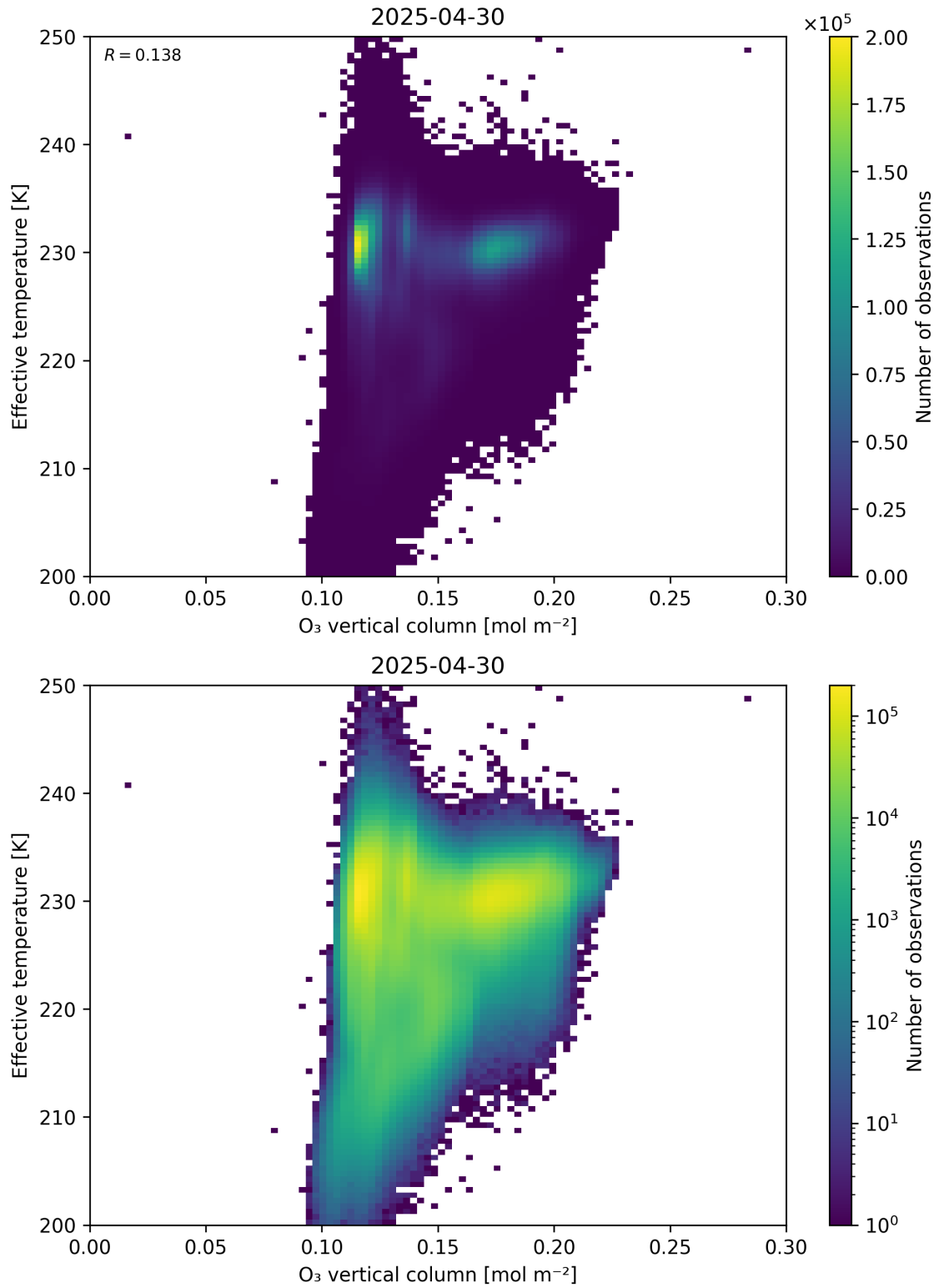
Figure 39: Scatter density plot of “O 3 vertical column” against “Effective temperature” for 2025-04-29 to 2025-05-01.
