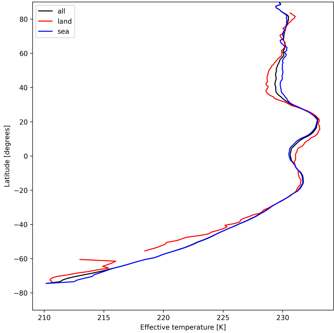
Figure 17: Zonal average of "Effective temperature" for 2025-04-29 to 2025-05-01.
