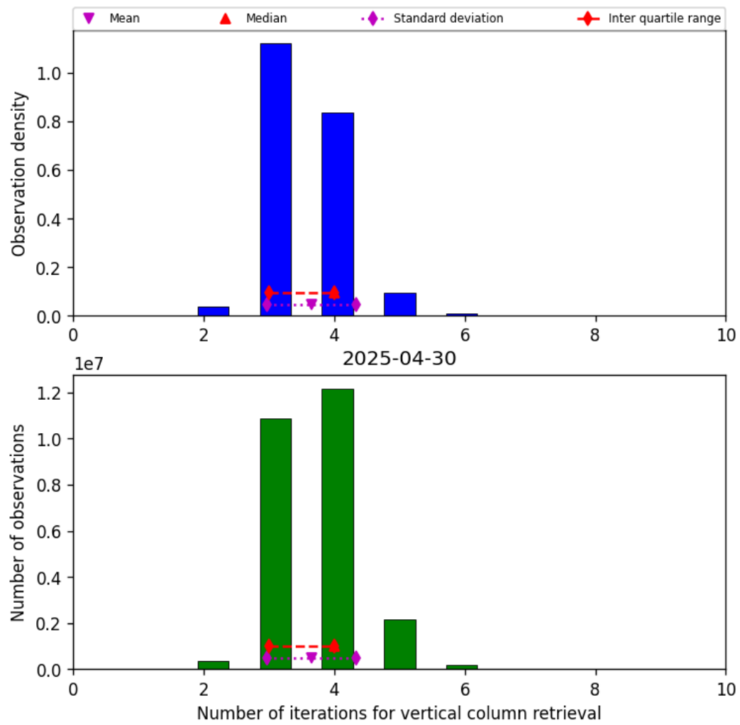
Figure 26: Histogram of “Number of iterations for vertical column retrieval” for 2025-04-29 to 2025-05-01
