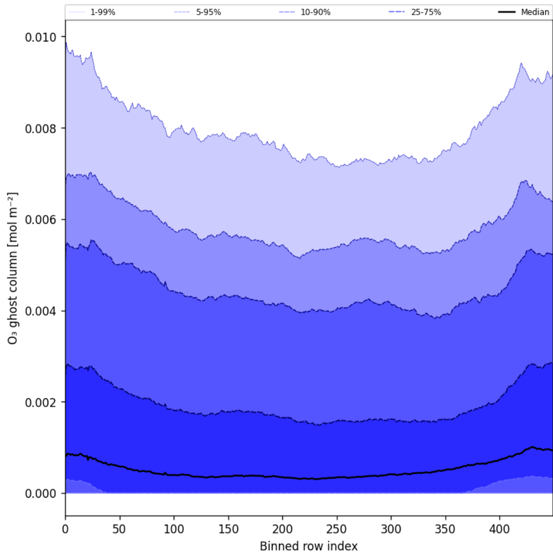
Figure 32: Along track statistics of “O 3 ghost column” for 2025-04-29 to 2025-05-01
