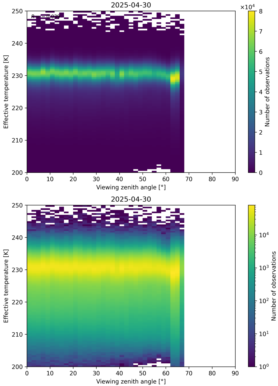
Figure 50: Scatter density plot of “Viewing zenith angle” against “Effective temperature” for 2025-04-29 to 2025-05-01.
