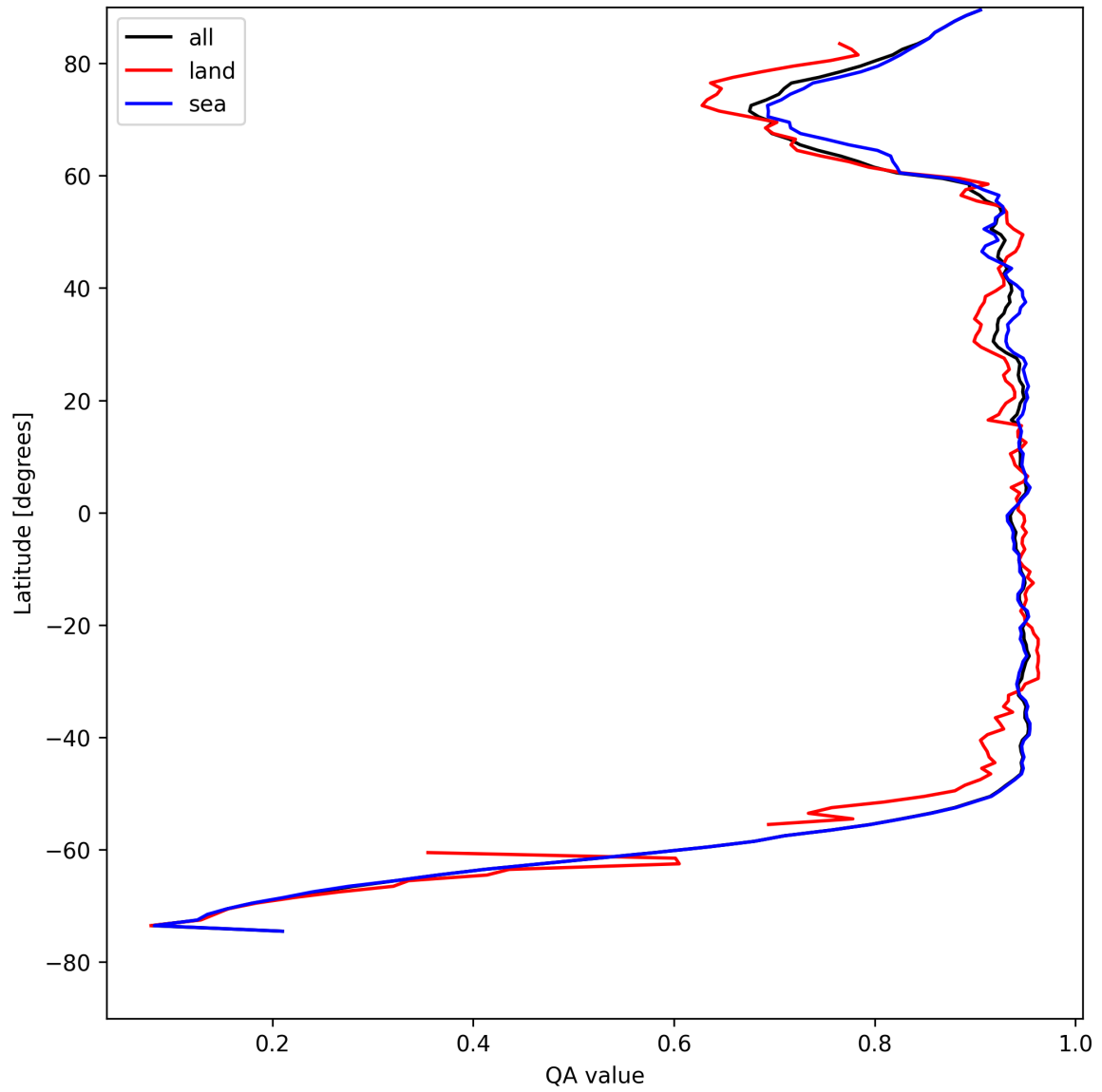
Figure 13: Zonal average of “QA value” for 2025-04-29 to 2025-05-01.
