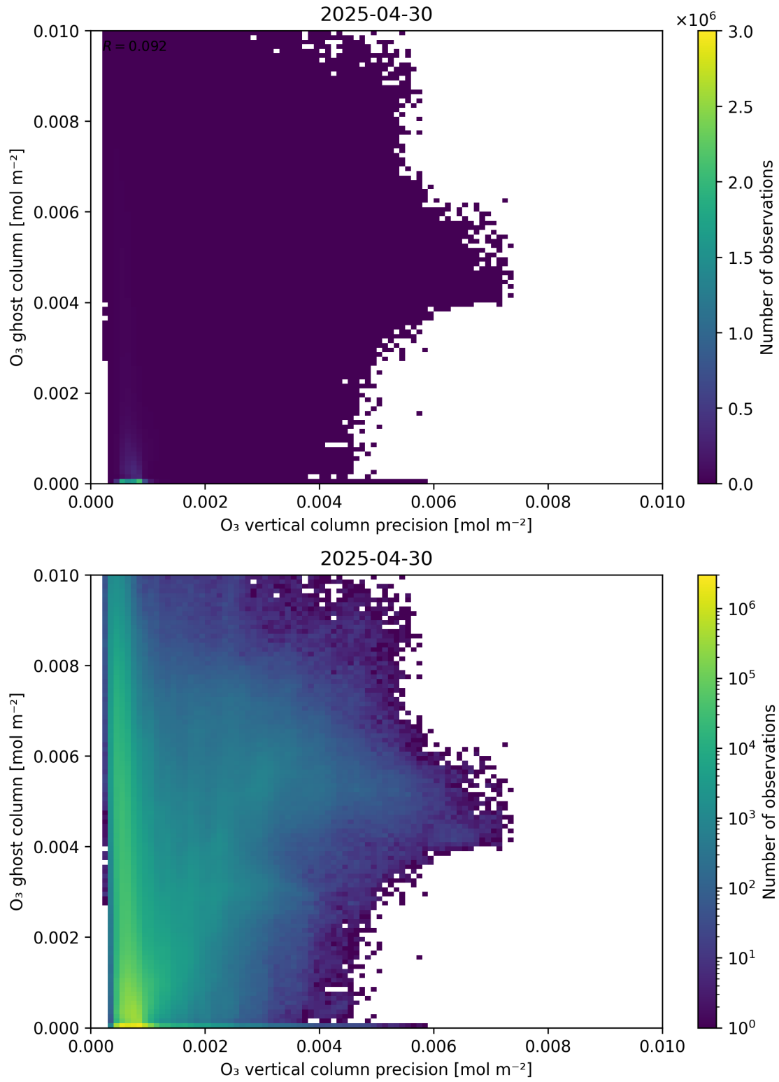
Figure 43: Scatter density plot of “ O_3 vertical column precision” against “ O_3 ghost column” for 2025-04-29 to 2025-05-01.
