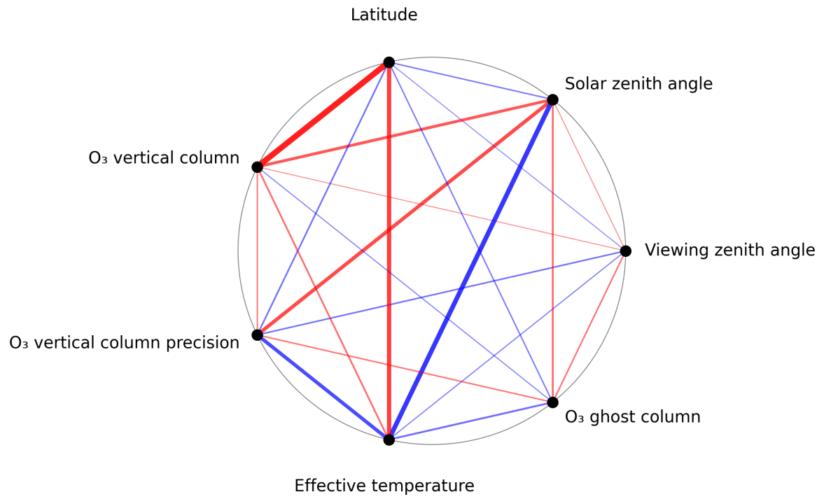
Figure 1: Map of correlation graph for 2025-04-29 to 2025-05-01.
