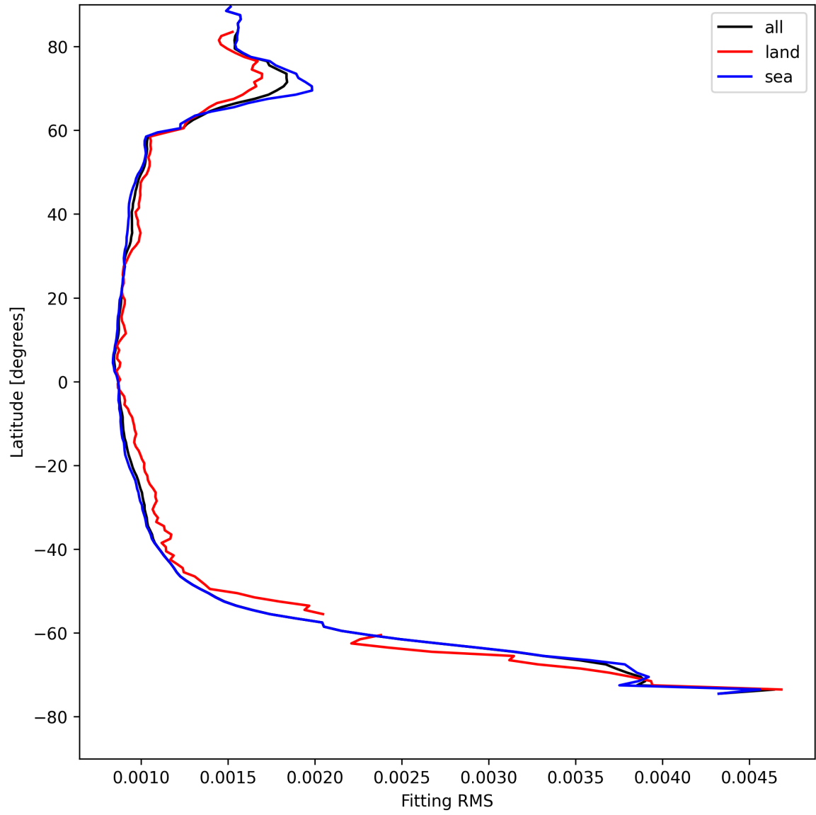
Figure 16: Zonal average of “Fitting RMS” for 2025-04-29 to 2025-05-01.
