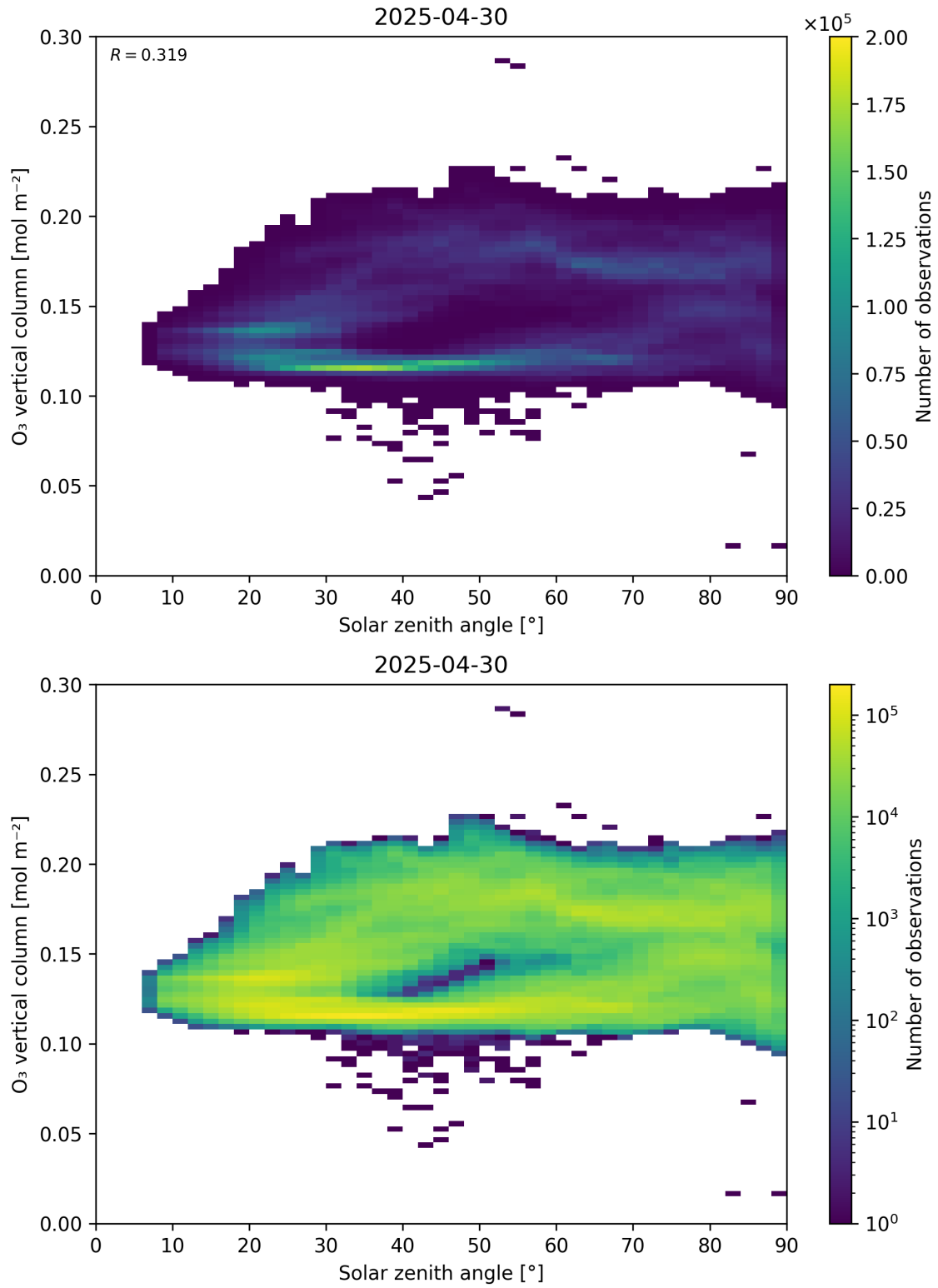
Figure 47: Scatter density plot of “Solar zenith angle” against “O 3 vertical column” for 2025-04-29 to 2025-05-01.
