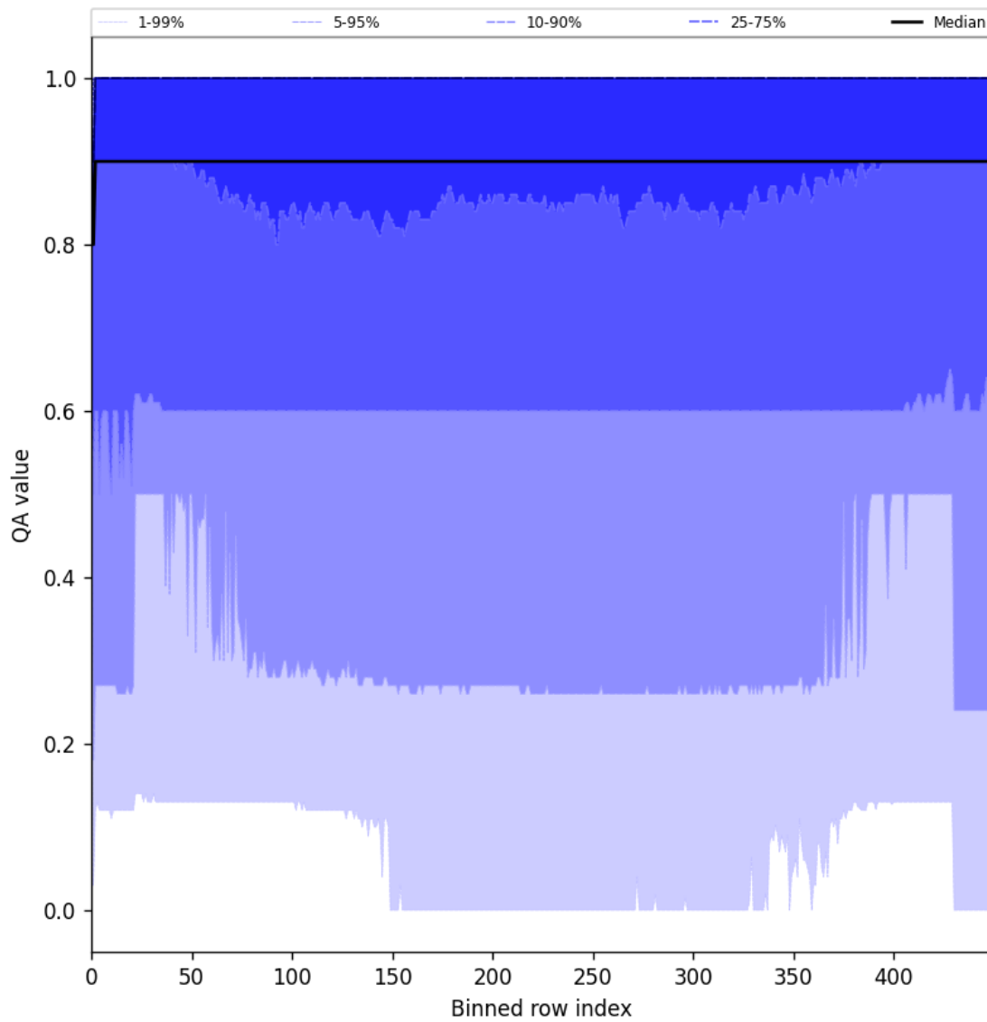
Figure 27: Along track statistics of “QA value” for 2025-04-29 to 2025-05-01
