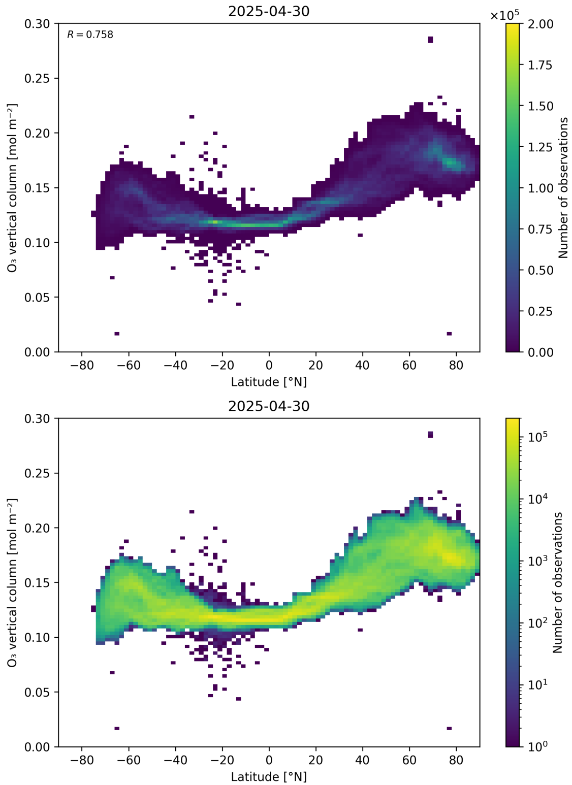
Figure 36: Scatter density plot of “Latitude” against “O 3 vertical column” for 2025-04-29 to 2025-05-01.
