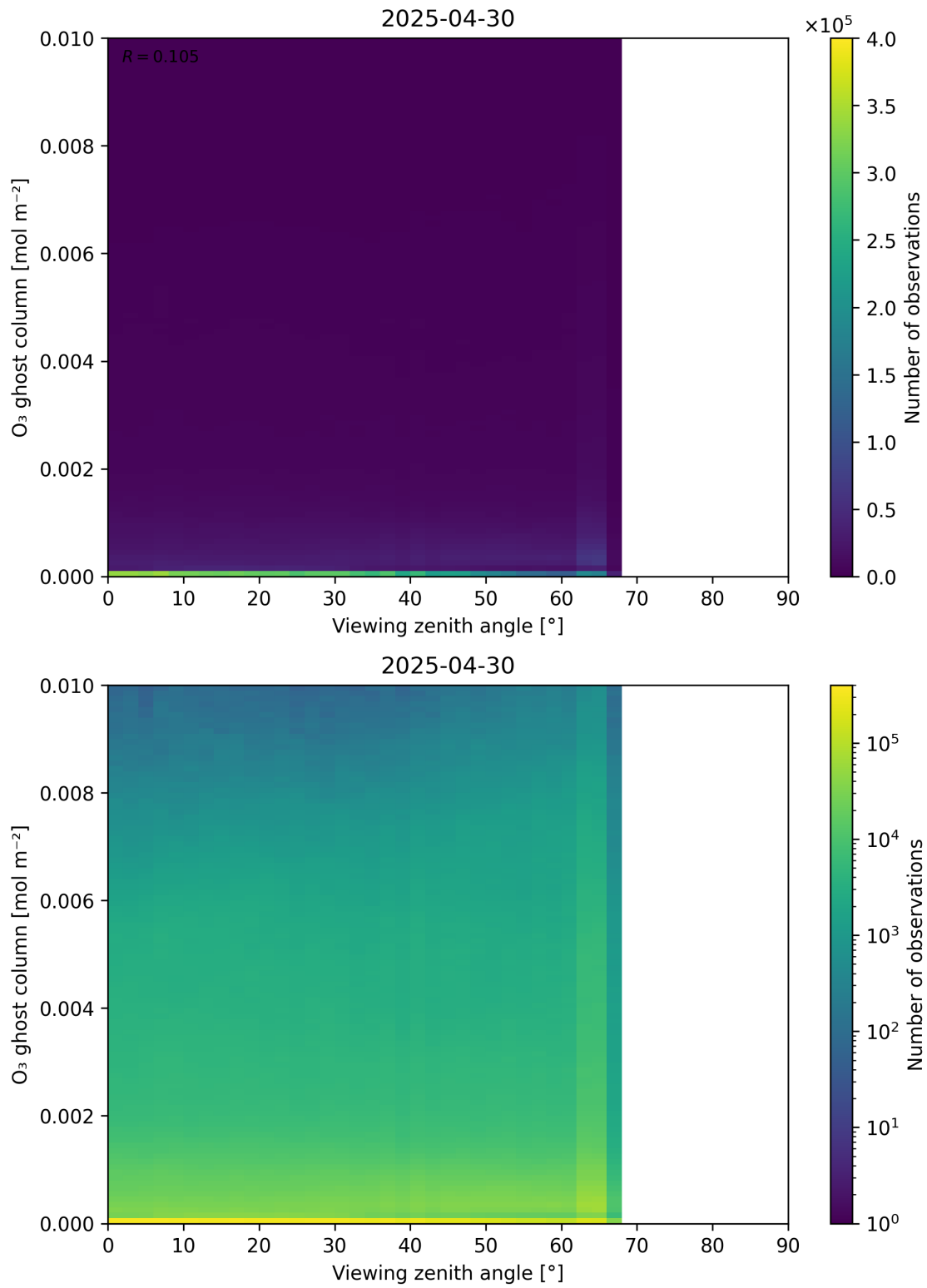
Figure 51: Scatter density plot of “Viewing zenith angle” against “O 3 ghost column” for 2025-04-29 to 2025-05-01.
