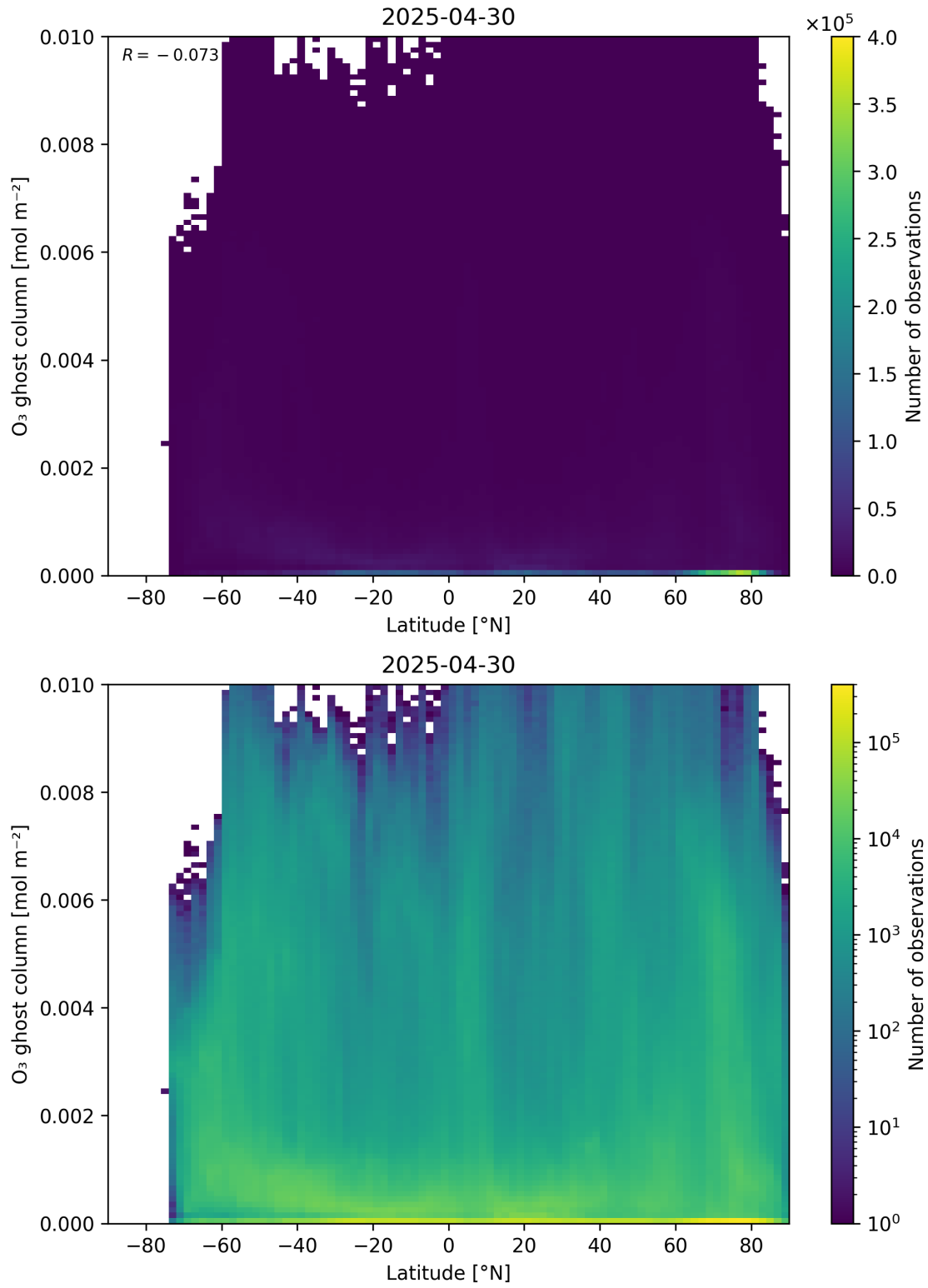
Figure 35: Scatter density plot of “Latitude” against “O 3 ghost column” for 2025-04-29 to 2025-05-01.
