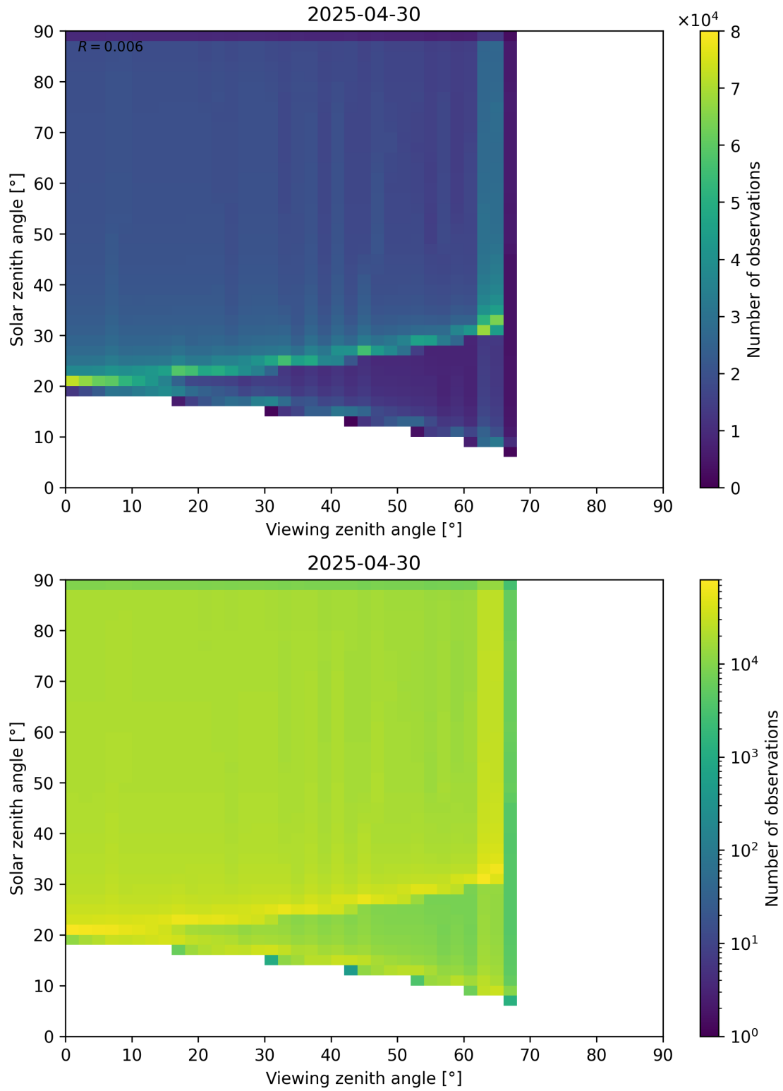
Figure 54: Scatter density plot of “Viewing zenith angle” against “Solar zenith angle” for 2025-04-29 to 2025-05-01.
