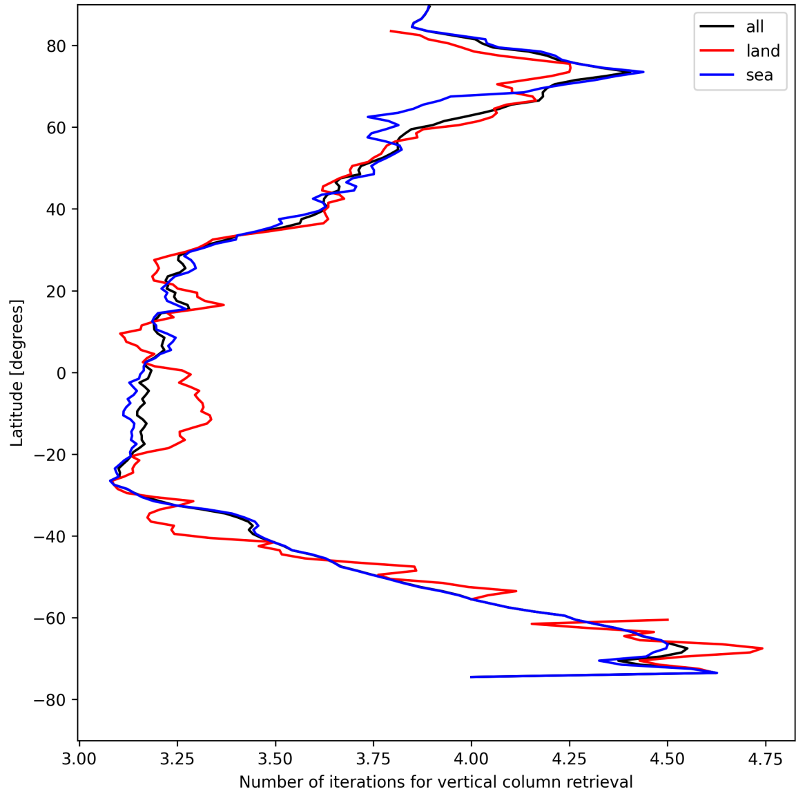
Figure 19: Zonal average of “Number of iterations for vertical column retrieval” for 2025-04-29 to 2025-05-01.
