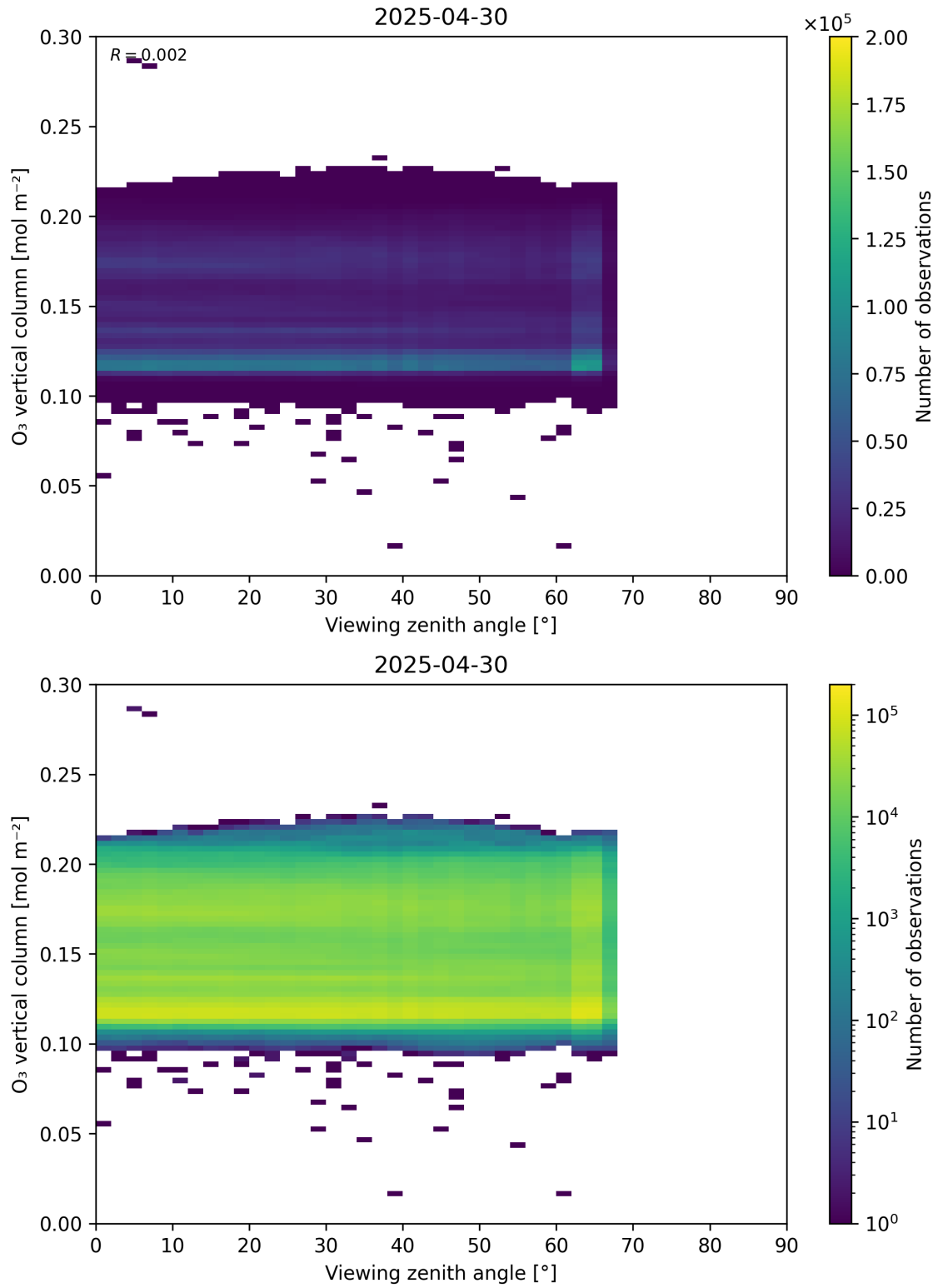
Figure 52: Scatter density plot of “Viewing zenith angle” against “O 3 vertical column” for 2025-04-29 to 2025-05-01.
