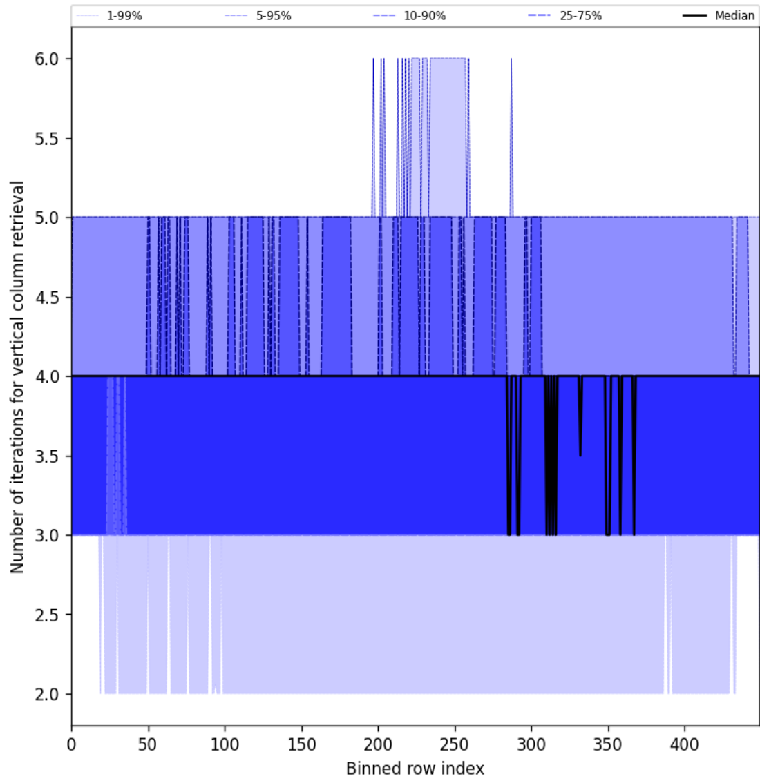
Figure 33: Along track statistics of “Number of iterations for vertical column retrieval” for 2025-04-29 to 2025-05-01
