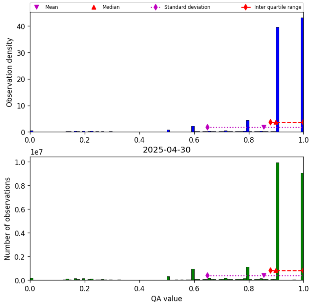
Figure 20: Histogram of “QA value” for 2025-04-29 to 2025-05-01
