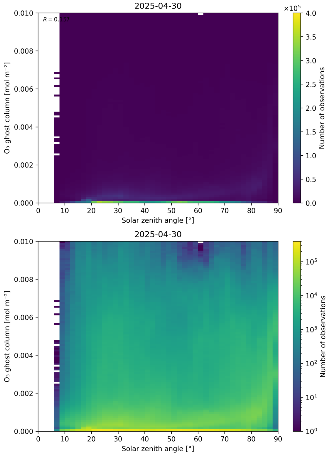
Figure 46: Scatter density plot of “Solar zenith angle” against “O 3 ghost column” for 2025-04-29 to 2025-05-01.
