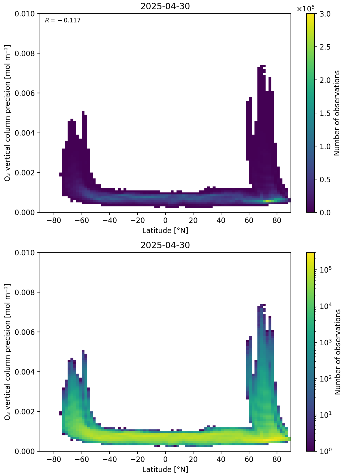
Figure 37: Scatter density plot of “Latitude” against “O 3 vertical column precision” for 2025-04-29 to 2025-05-01.
