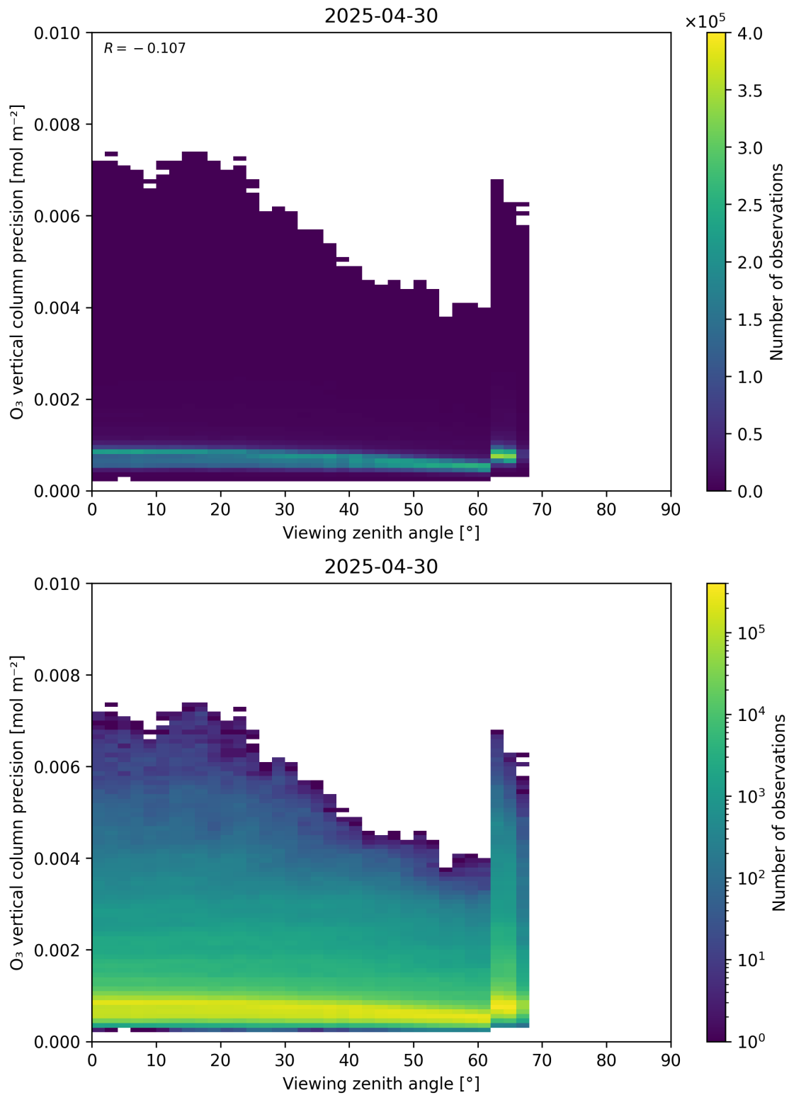
Figure 53: Scatter density plot of “Viewing zenith angle” against “O 3 vertical column precision” for 2025-04-29 to 2025-05-01.
