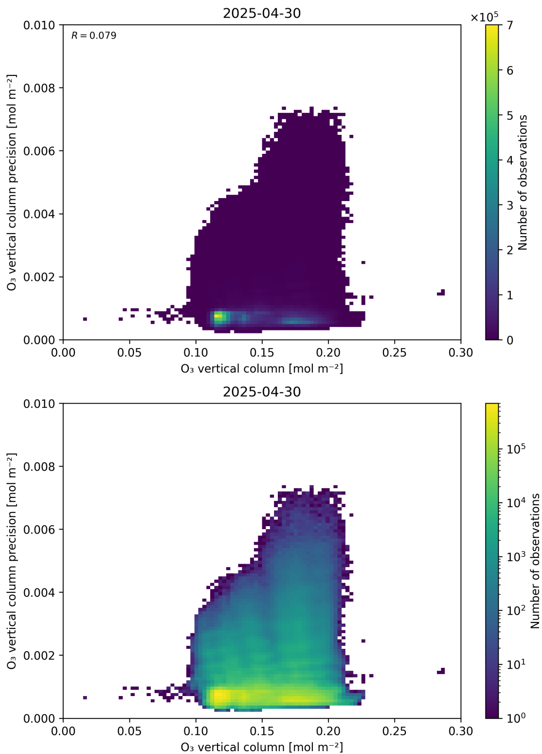
Figure 41: Scatter density plot of “O 3 vertical column” against “O 3 vertical column precision” for 2025-04-29 to 2025-05-01.
