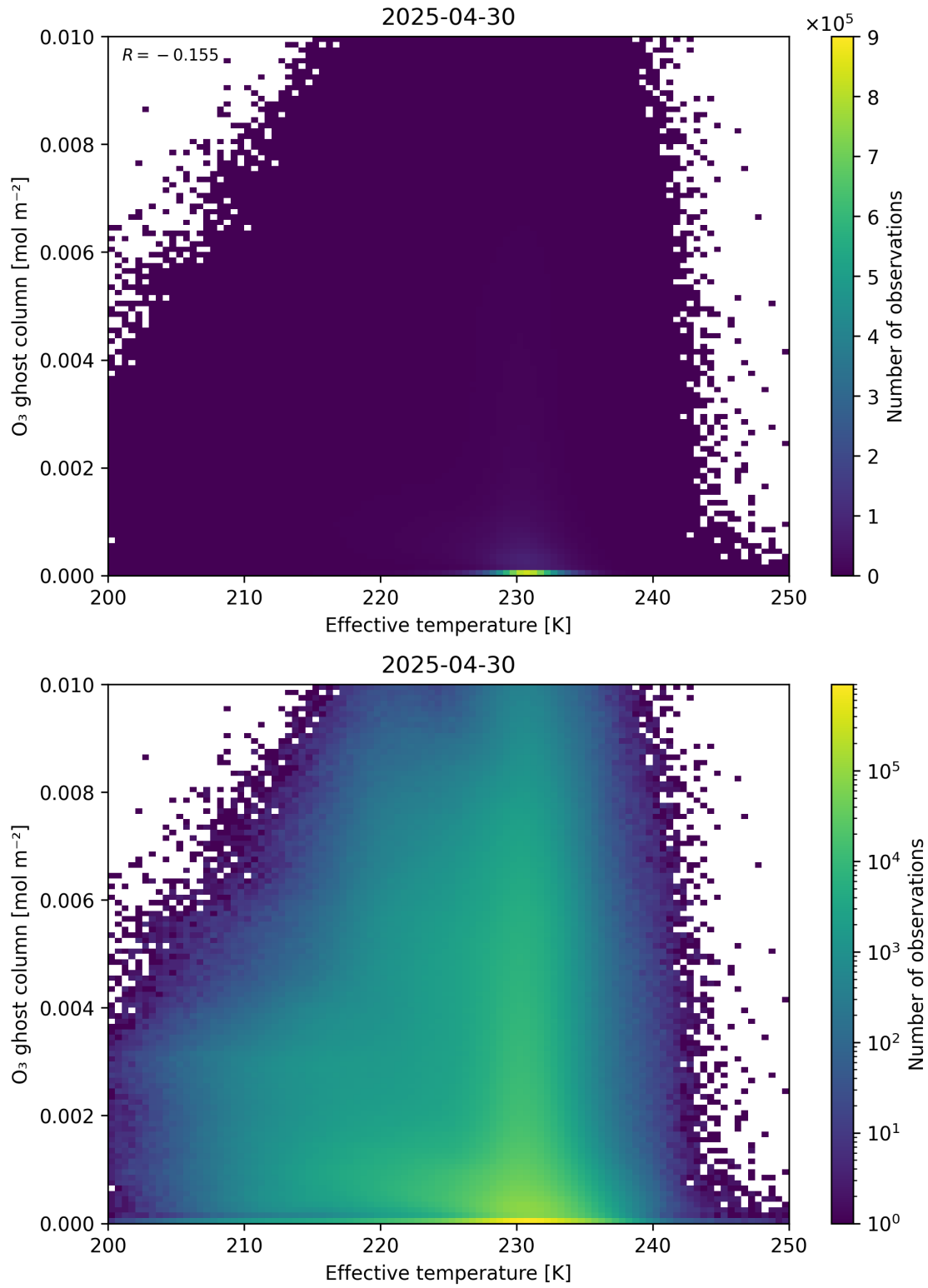
Figure 38: Scatter density plot of “Effective temperature” against “O 3 ghost column” for 2025-04-29 to 2025-05-01.
