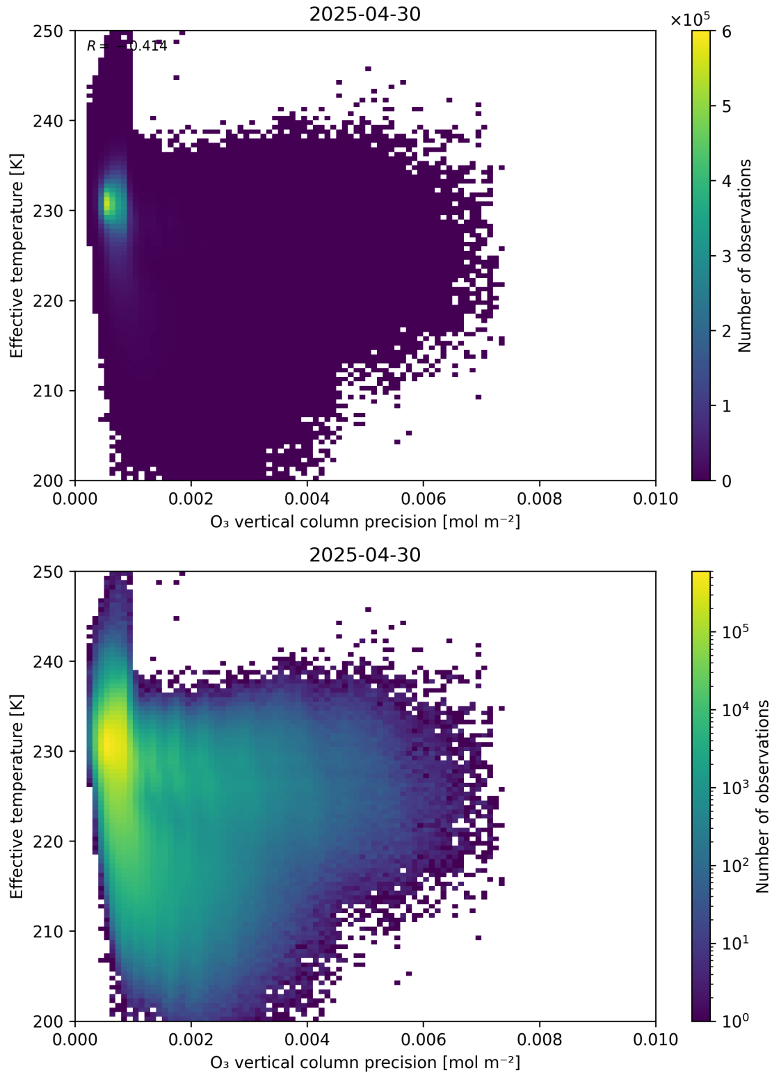
Figure 42: Scatter density plot of “O 3 vertical column precision” against “Effective temperature” for 2025-04-29 to 2025-05-01.
