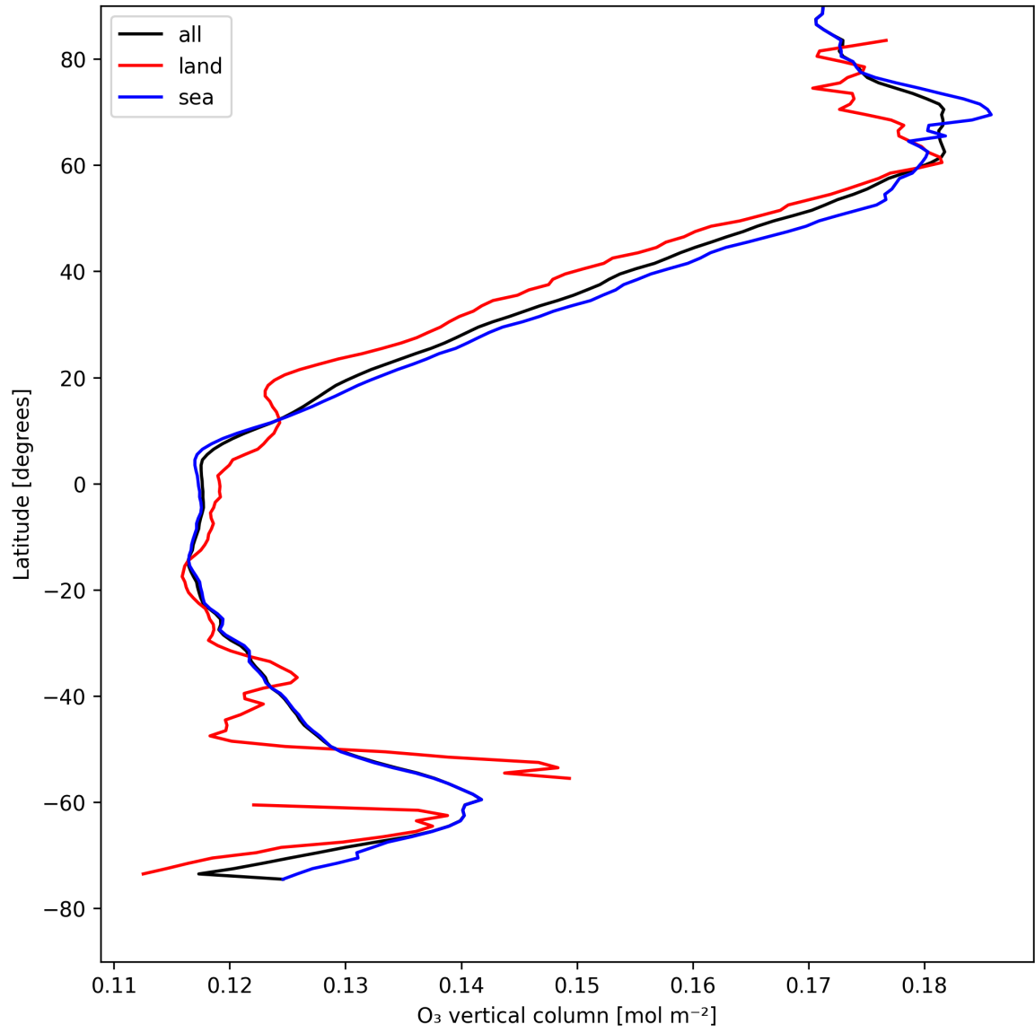
Figure 14: Zonal average of “O 3 vertical column” for 2025-04-29 to 2025-05-01.
