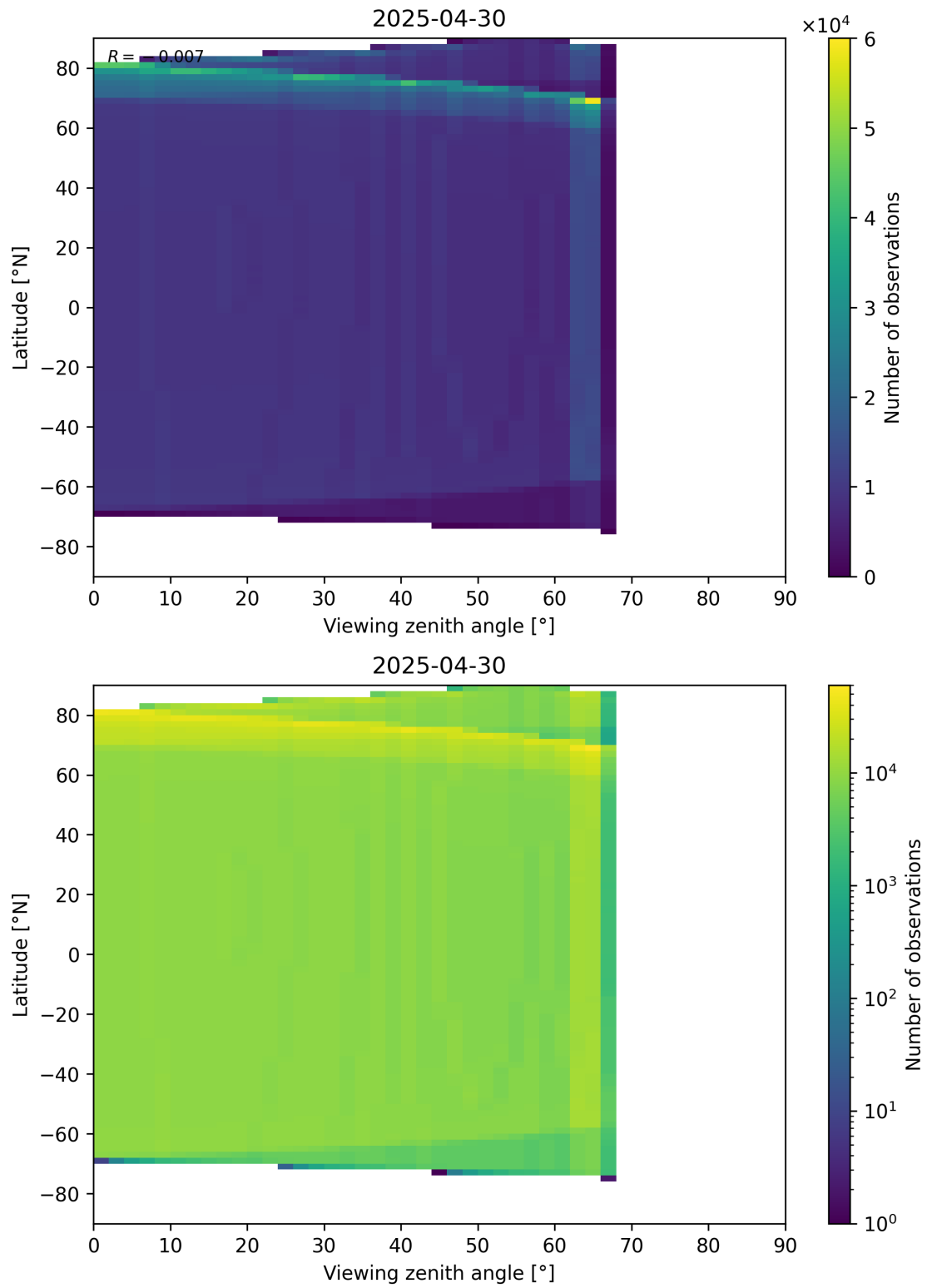
Figure 49: Scatter density plot of “Viewing zenith angle” against “Latitude” for 2025-04-29 to 2025-05-01.
