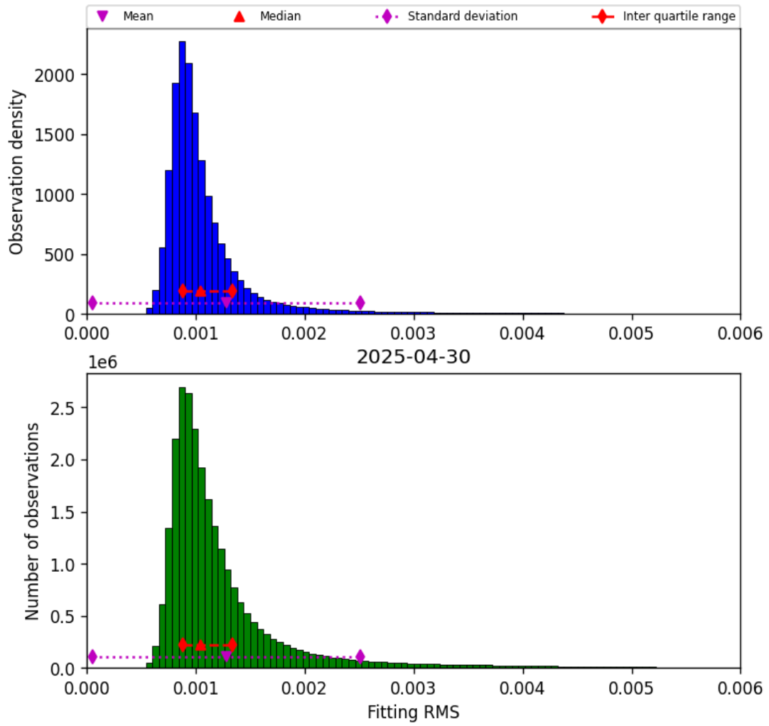
Figure 23: Histogram of “Fitting RMS” for 2025-04-29 to 2025-05-01
