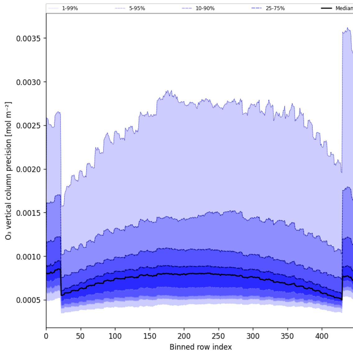
Figure 29: Along track statistics of “O 3 vertical column precision” for 2025-04-29 to 2025-05-01
