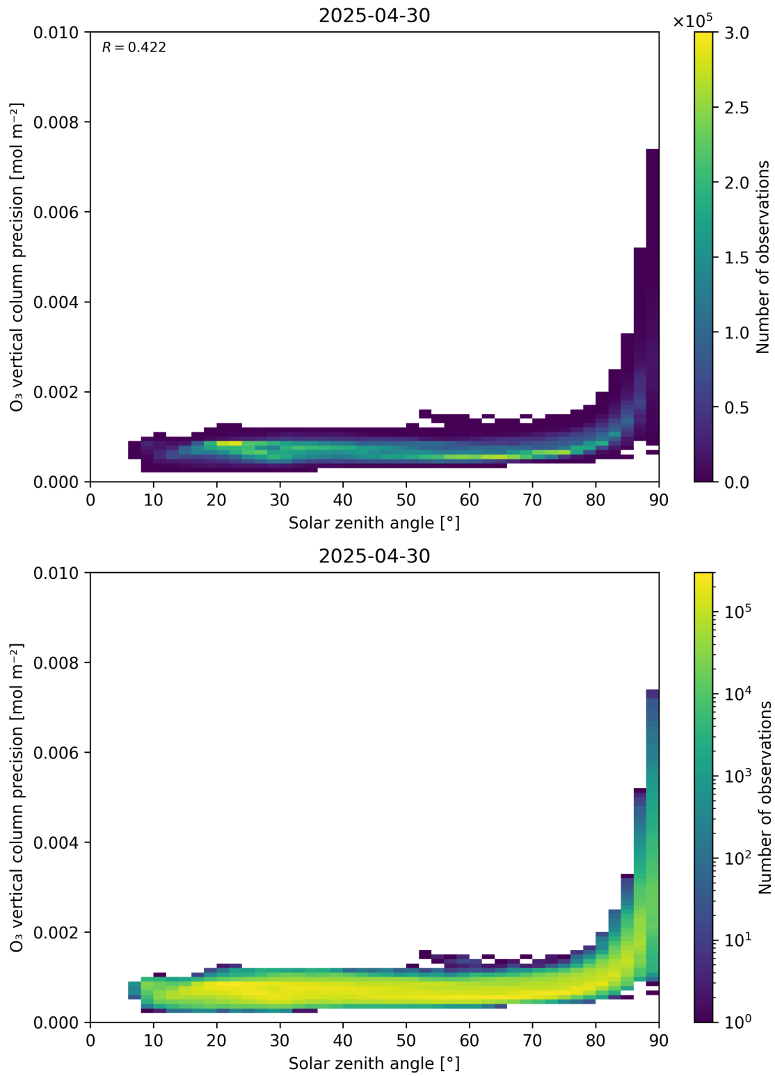
Figure 48: Scatter density plot of “Solar zenith angle” against “O 3 vertical column precision” for 2025-04-29 to 2025-05-01.
