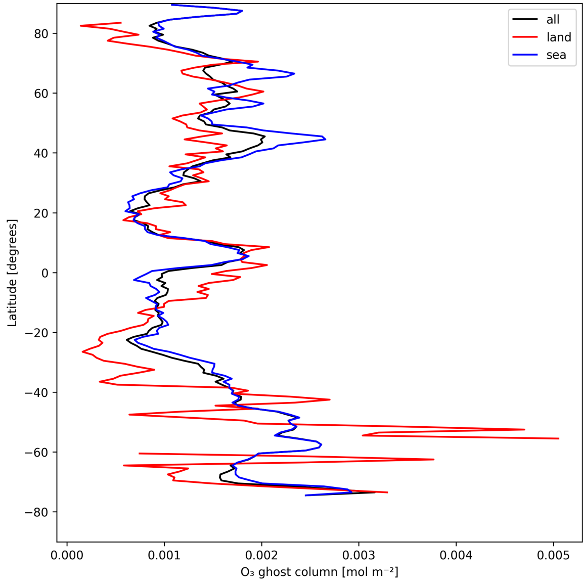
Figure 18: Zonal average of "O 3 ghost column" for 2025-04-29 to 2025-05-01.
