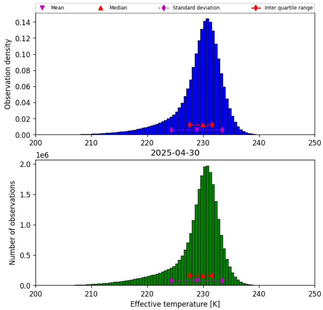
Figure 24: Histogram of “Effective temperature” for 2025-04-29 to 2025-05-01
