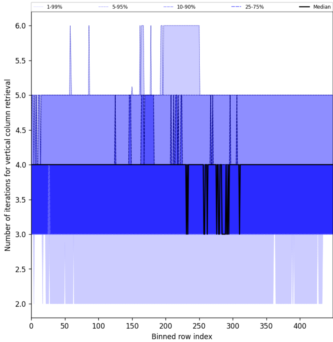
Figure 33: Along track statistics of “Number of iterations for vertical column retrieval” for 2025-05-01 to 2025-05-03
