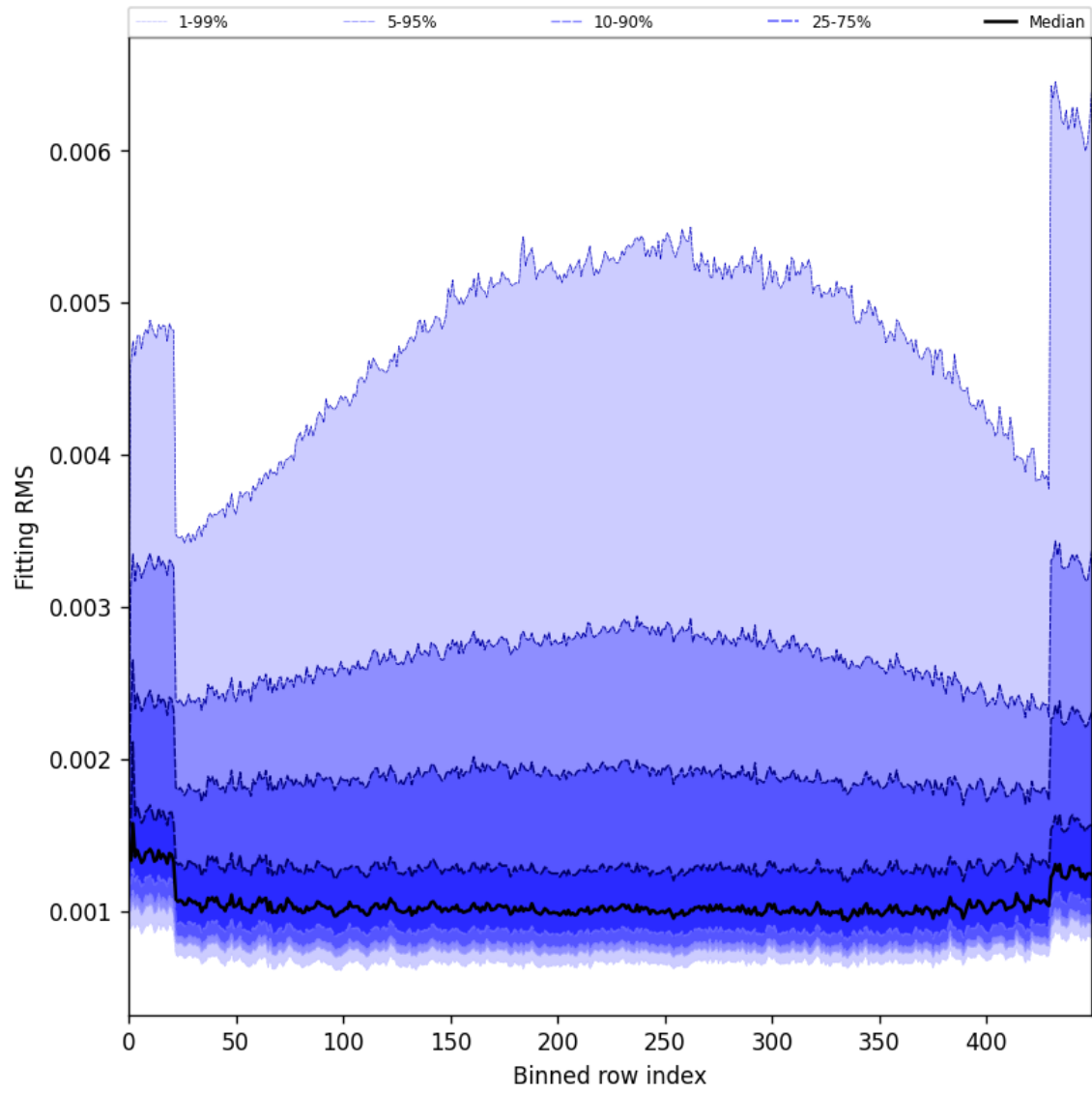
Figure 30: Along track statistics of “Fitting RMS” for 2025-05-01 to 2025-05-03
