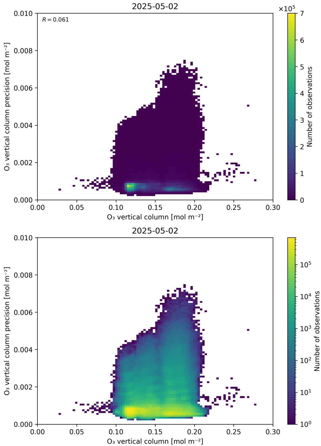
Figure 41: Scatter density plot of “O 3 vertical column” against “O 3 vertical column precision” for 2025-05-01 to 2025-05-03.
