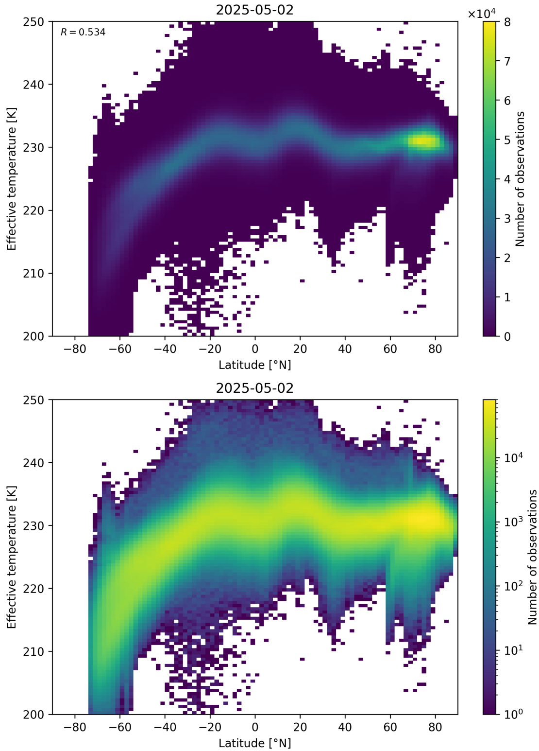
Figure 34: Scatter density plot of “Latitude” against “Effective temperature” for 2025-05-01 to 2025-05-03.
