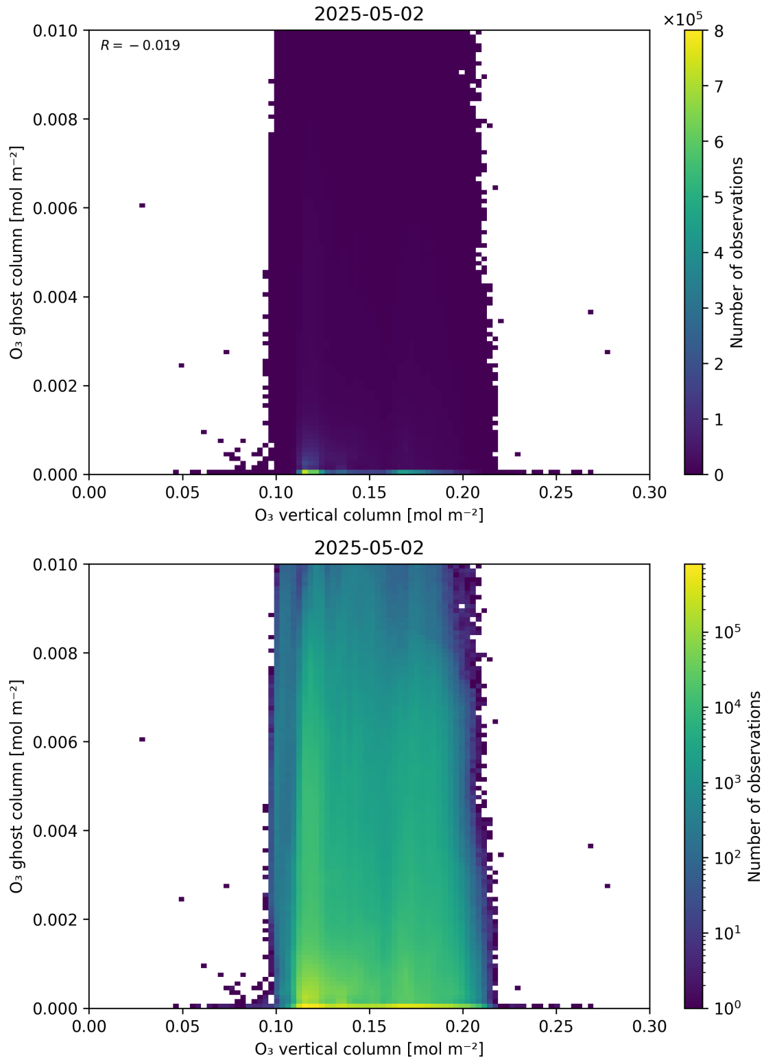
Figure 40: Scatter density plot of “O 3 vertical column” against “O 3 ghost column” for 2025-05-01 to 2025-05-03.
