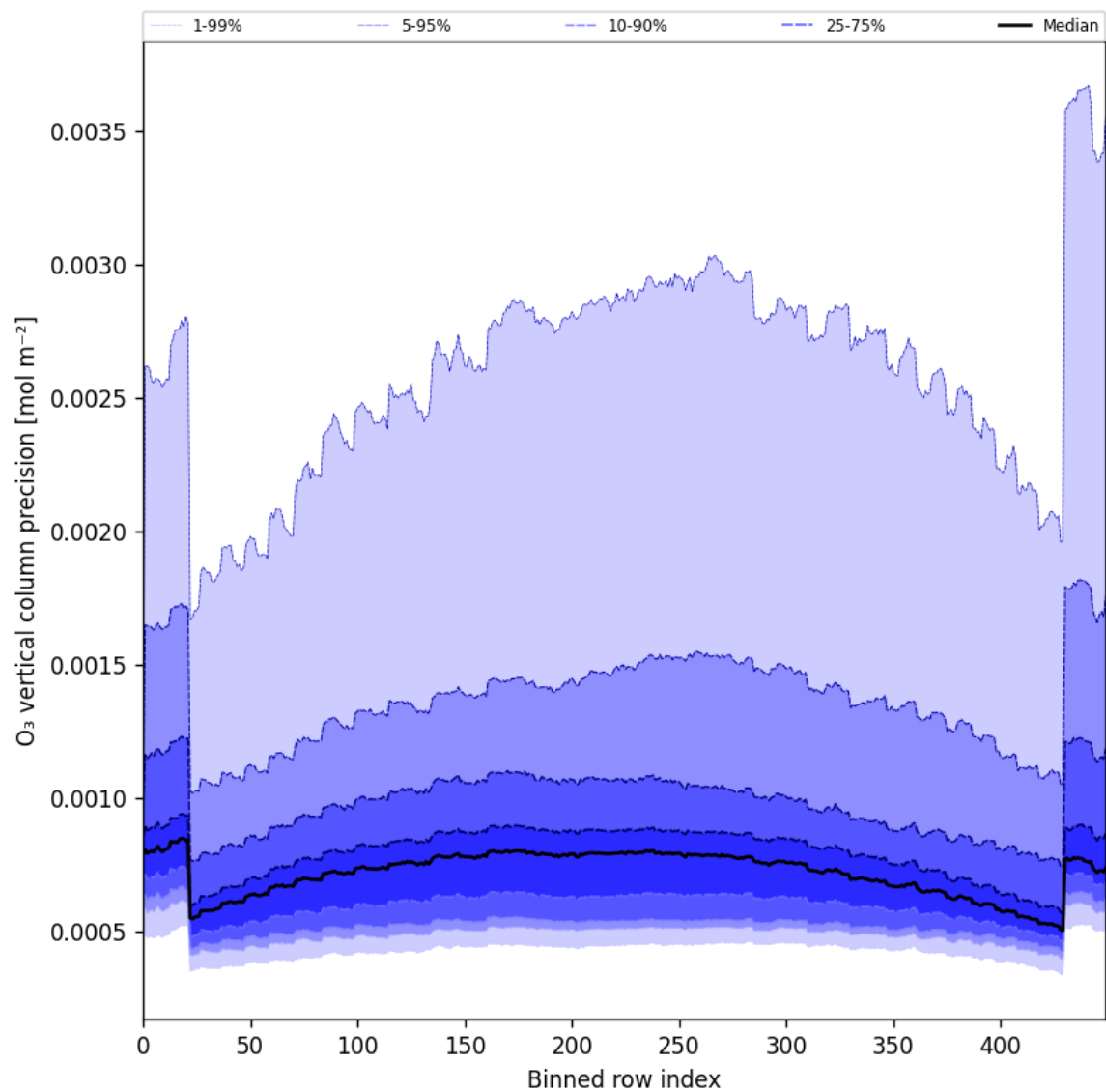
Figure 29: Along track statistics of “O 3 vertical column precision” for 2025-05-01 to 2025-05-03
