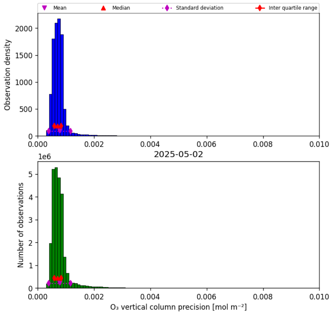
Figure 22: Histogram of “O 3 vertical column precision” for 2025-05-01 to 2025-05-03
