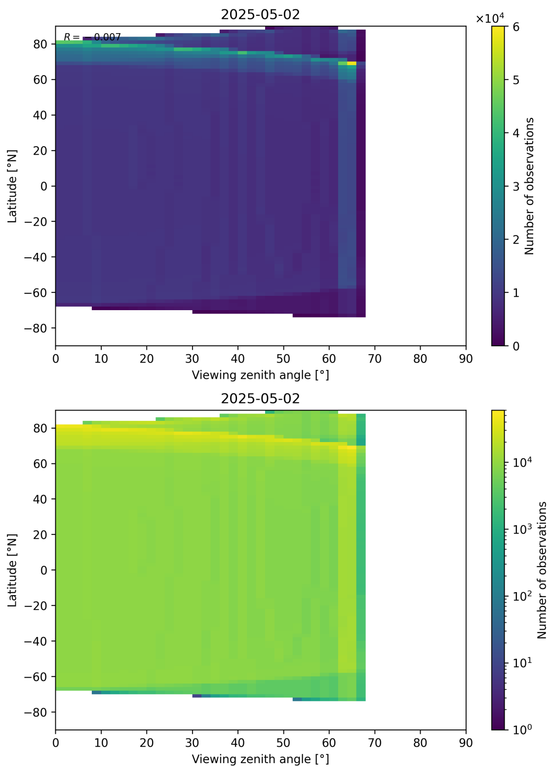
Figure 49: Scatter density plot of “Viewing zenith angle” against “Latitude” for 2025-05-01 to 2025-05-03.
