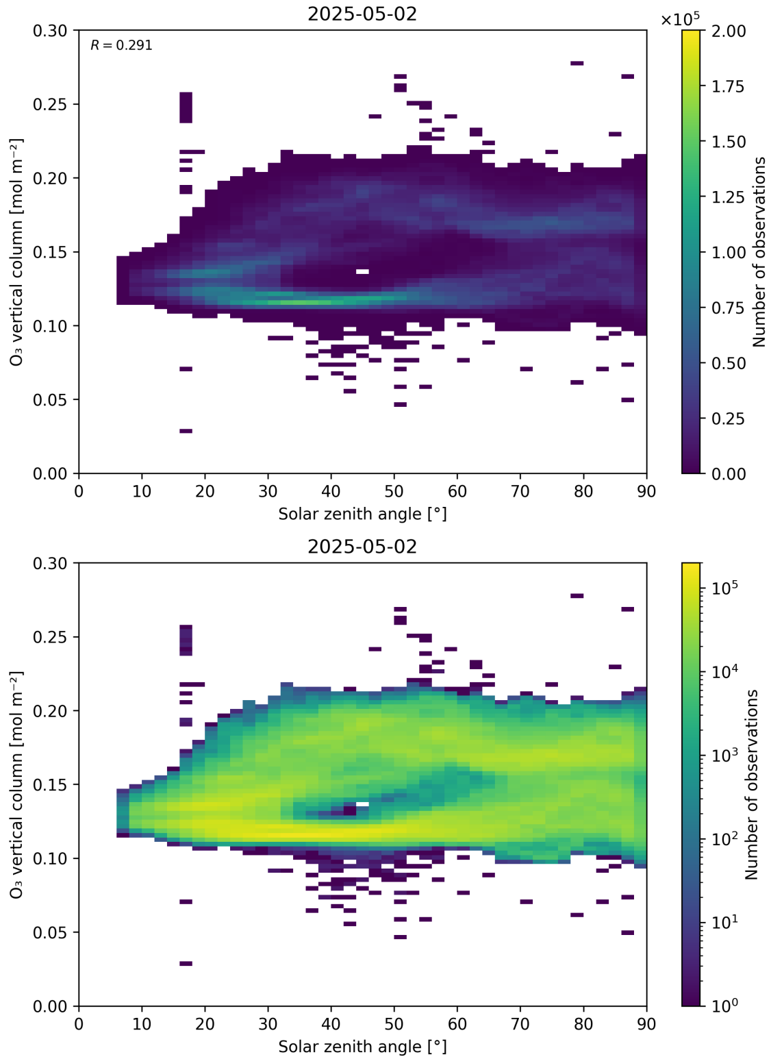
Figure 47: Scatter density plot of “Solar zenith angle” against “O 3 vertical column” for 2025-05-01 to 2025-05-03.
