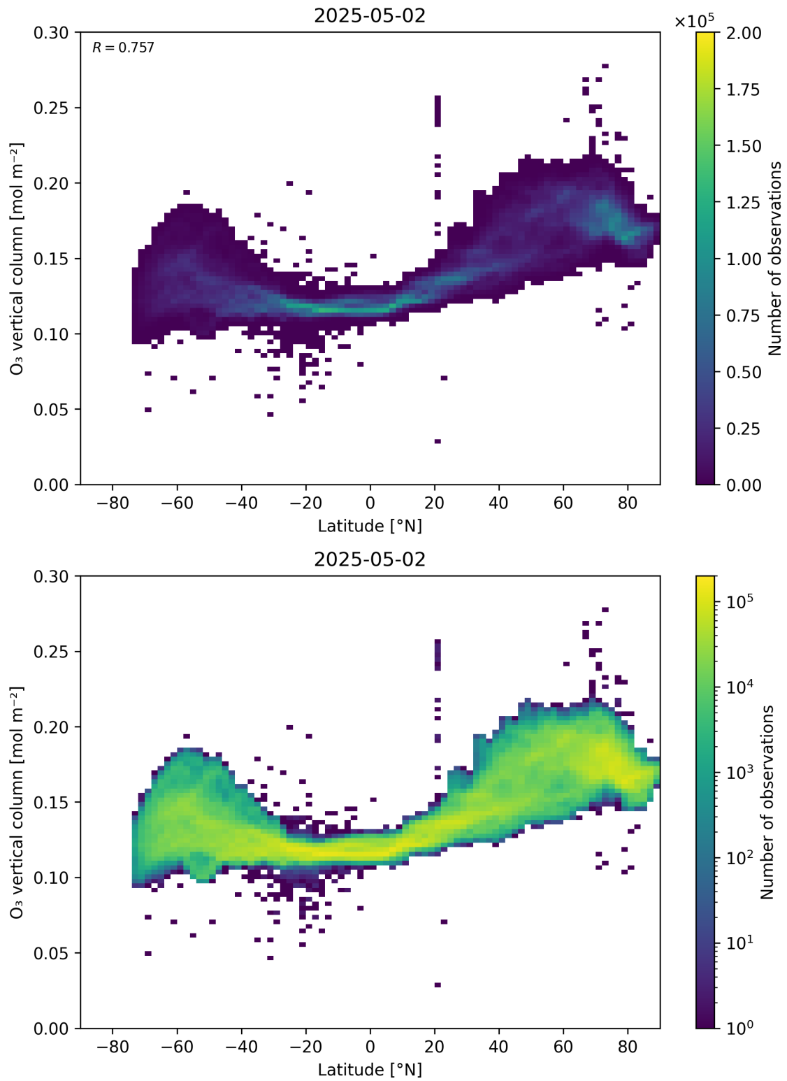
Figure 36: Scatter density plot of “Latitude” against “O 3 vertical column” for 2025-05-01 to 2025-05-03.
