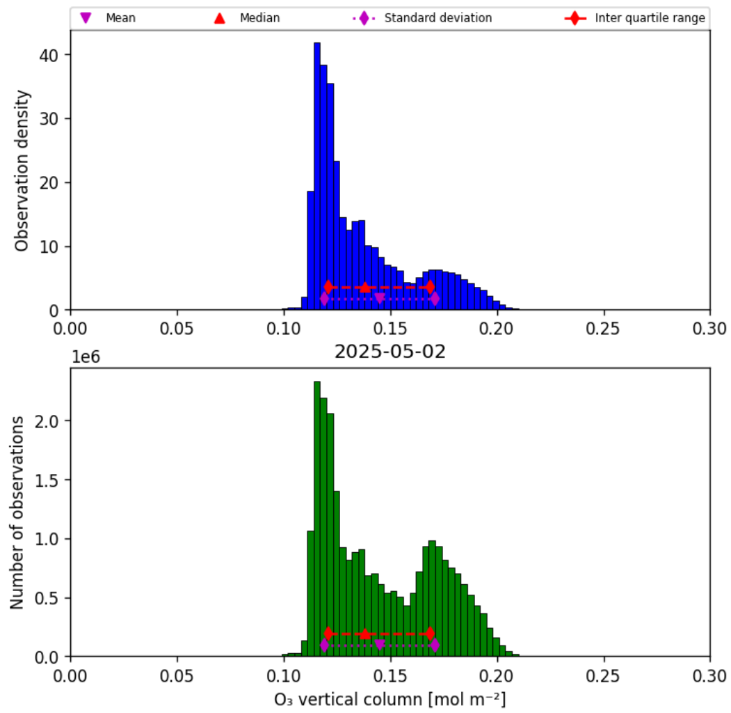
Figure 21: Histogram of “O 3 vertical column” for 2025-05-01 to 2025-05-03
