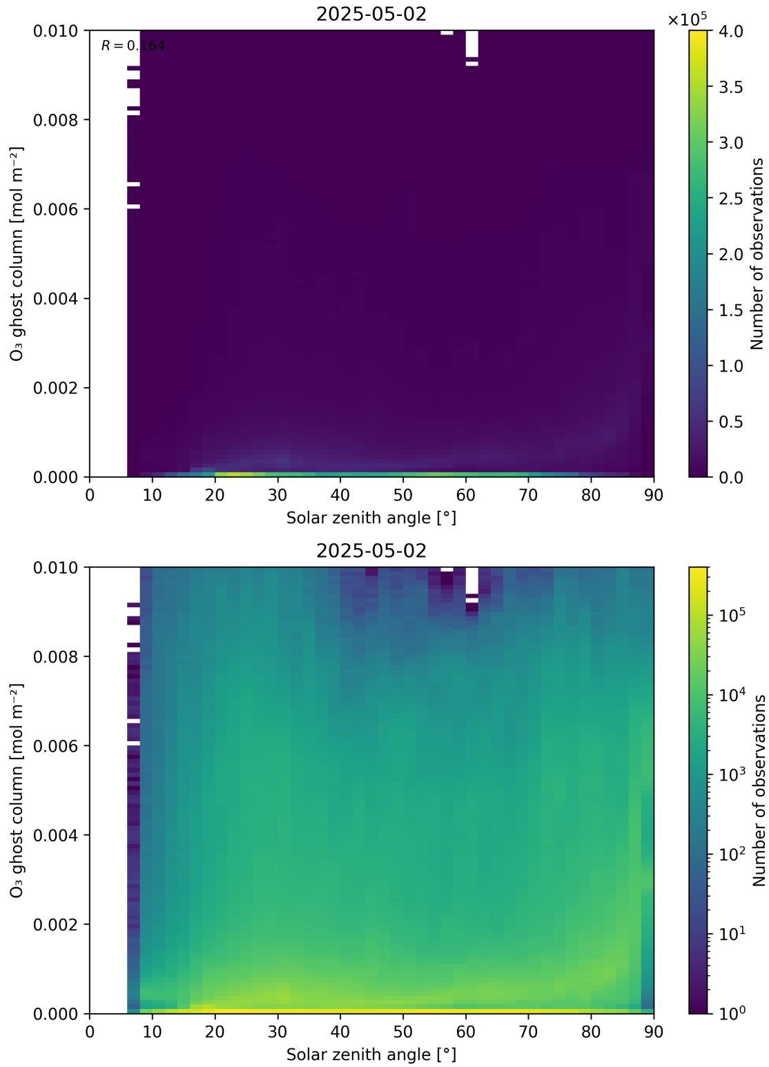
Figure 46: Scatter density plot of “Solar zenith angle” against “O 3 ghost column” for 2025-05-01 to 2025-05-03.
