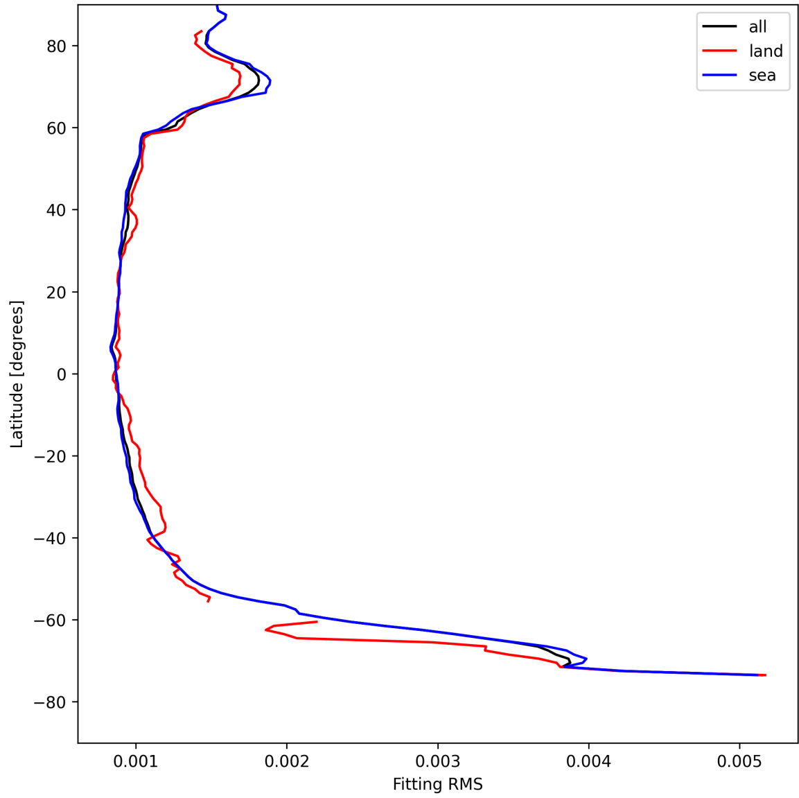
Figure 16: Zonal average of “Fitting RMS” for 2025-05-01 to 2025-05-03.
