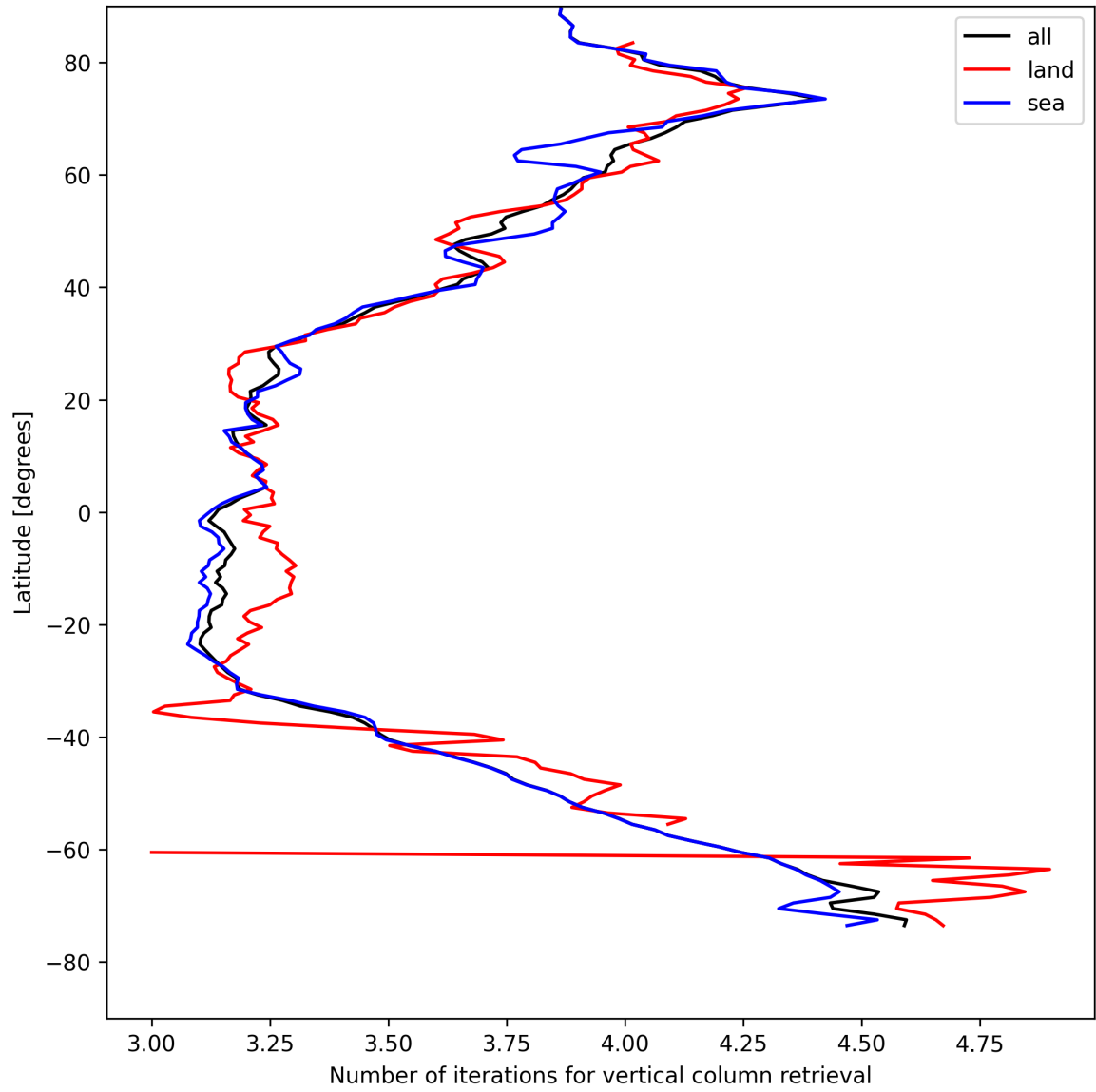
Figure 19: Zonal average of “Number of iterations for vertical column retrieval” for 2025-05-01 to 2025-05-03.
