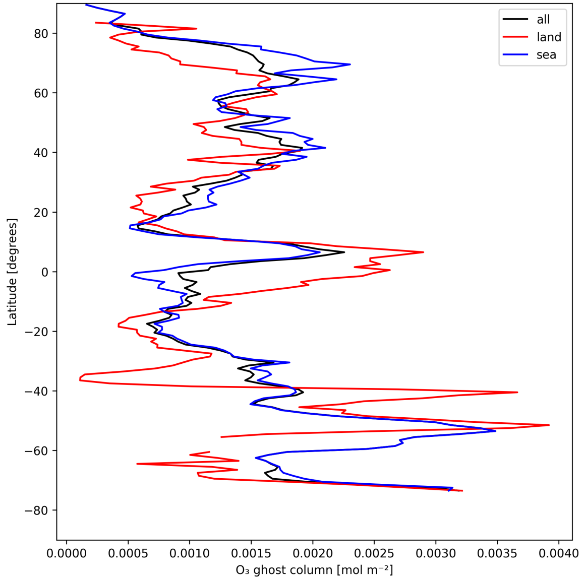
Figure 18: Zonal average of "O 3 ghost column" for 2025-05-01 to 2025-05-03.
