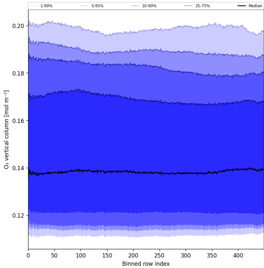
Figure 28: Along track statistics of “O 3 vertical column” for 2025-05-01 to 2025-05-03
