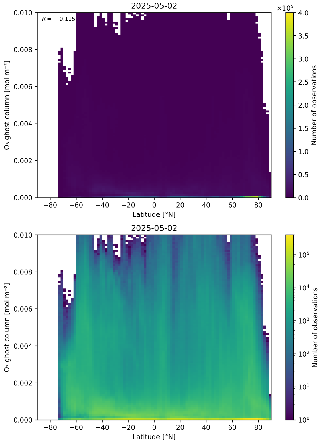
Figure 35: Scatter density plot of “Latitude” against “O 3 ghost column” for 2025-05-01 to 2025-05-03.
