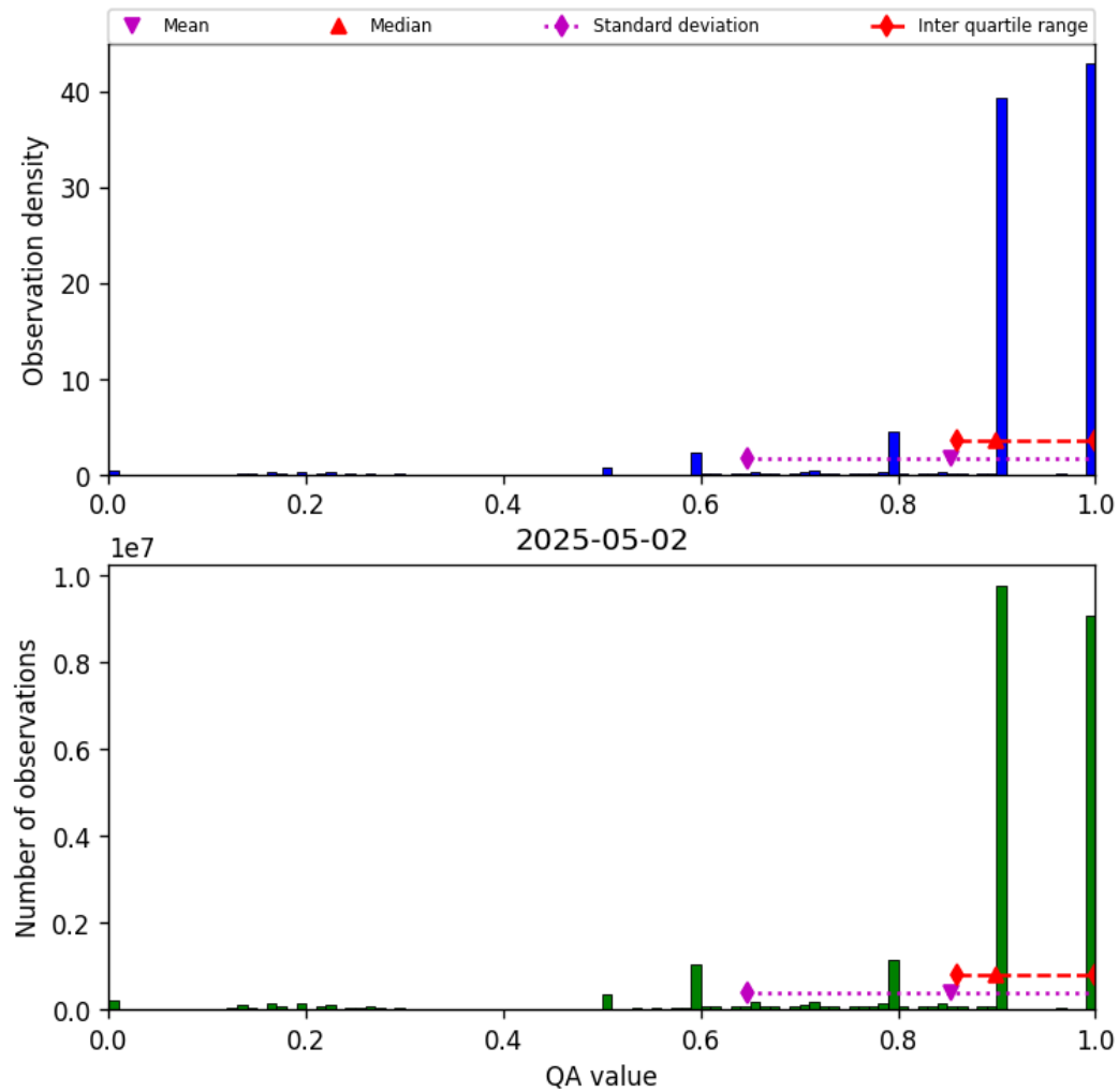
Figure 20: Histogram of “QA value” for 2025-05-01 to 2025-05-03
