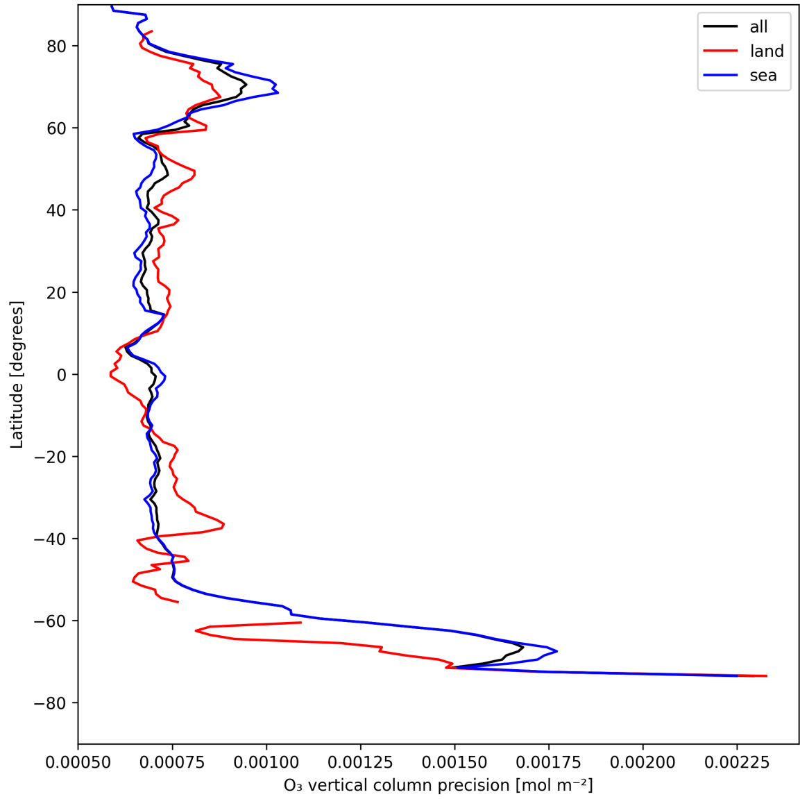
Figure 15: Zonal average of “O 3 vertical column precision” for 2025-05-01 to 2025-05-03.
