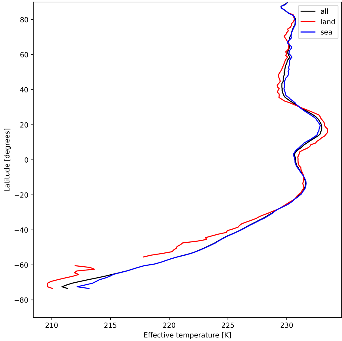
Figure 17: Zonal average of "Effective temperature" for 2025-05-01 to 2025-05-03.
