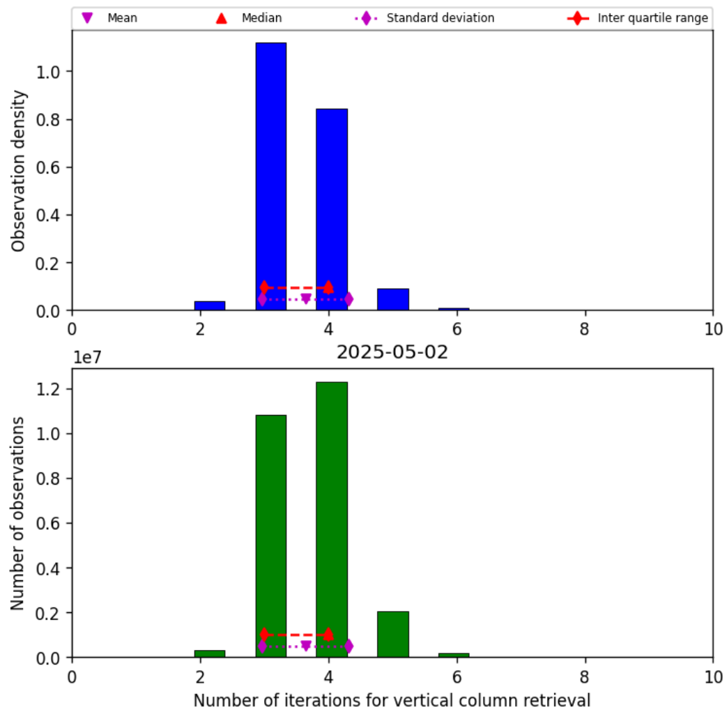
Figure 26: Histogram of “Number of iterations for vertical column retrieval” for 2025-05-01 to 2025-05-03
