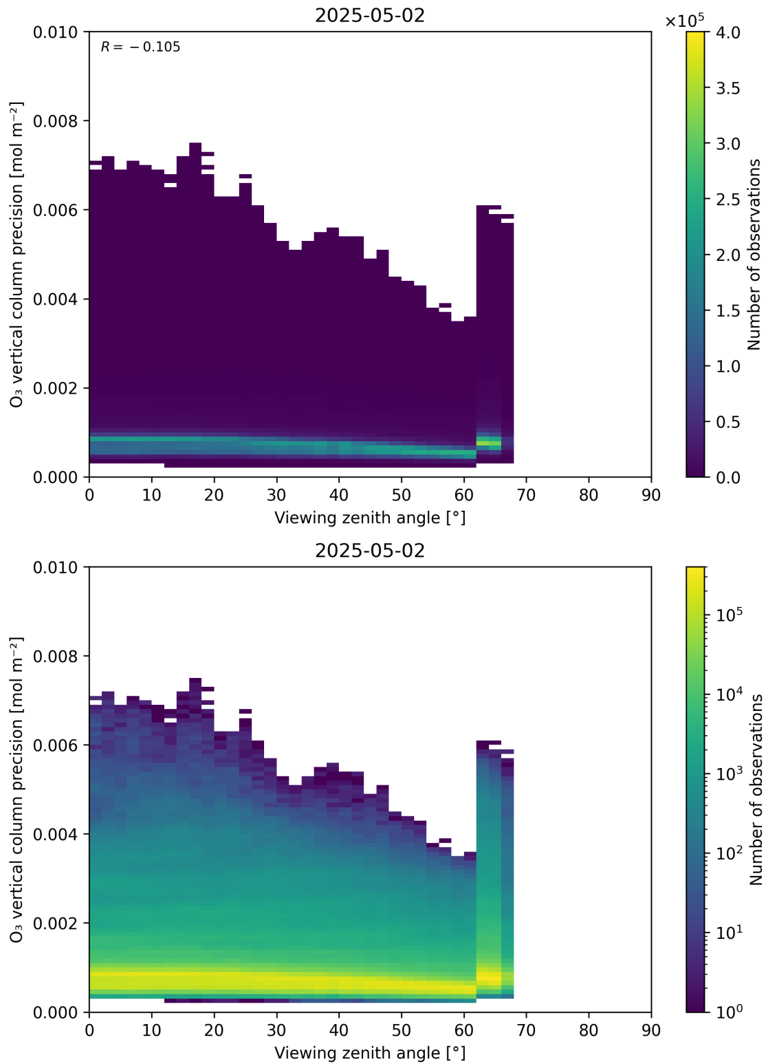
Figure 53: Scatter density plot of “Viewing zenith angle” against “O 3 vertical column precision” for 2025-05-01 to 2025-05-03.
