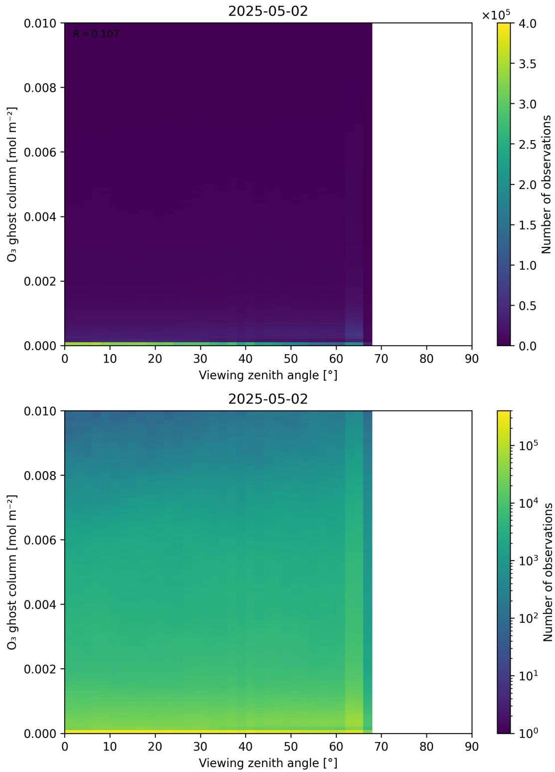
Figure 51: Scatter density plot of “Viewing zenith angle” against “O 3 ghost column” for 2025-05-01 to 2025-05-03.
