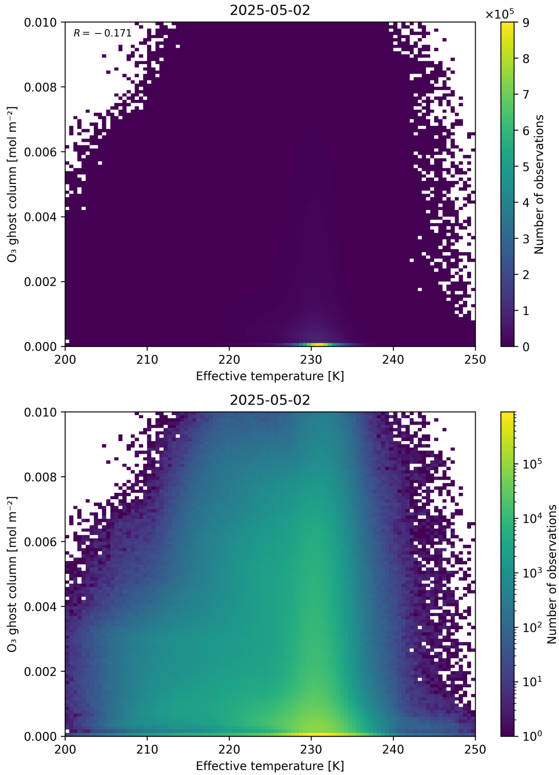
Figure 38: Scatter density plot of “Effective temperature” against “O 3 ghost column” for 2025-05-01 to 2025-05-03.
