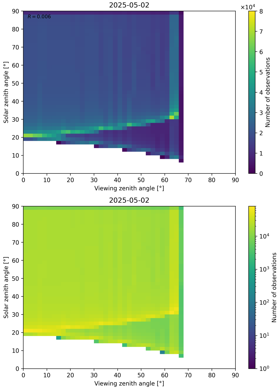
Figure 54: Scatter density plot of “Viewing zenith angle” against “Solar zenith angle” for 2025-05-01 to 2025-05-03.
