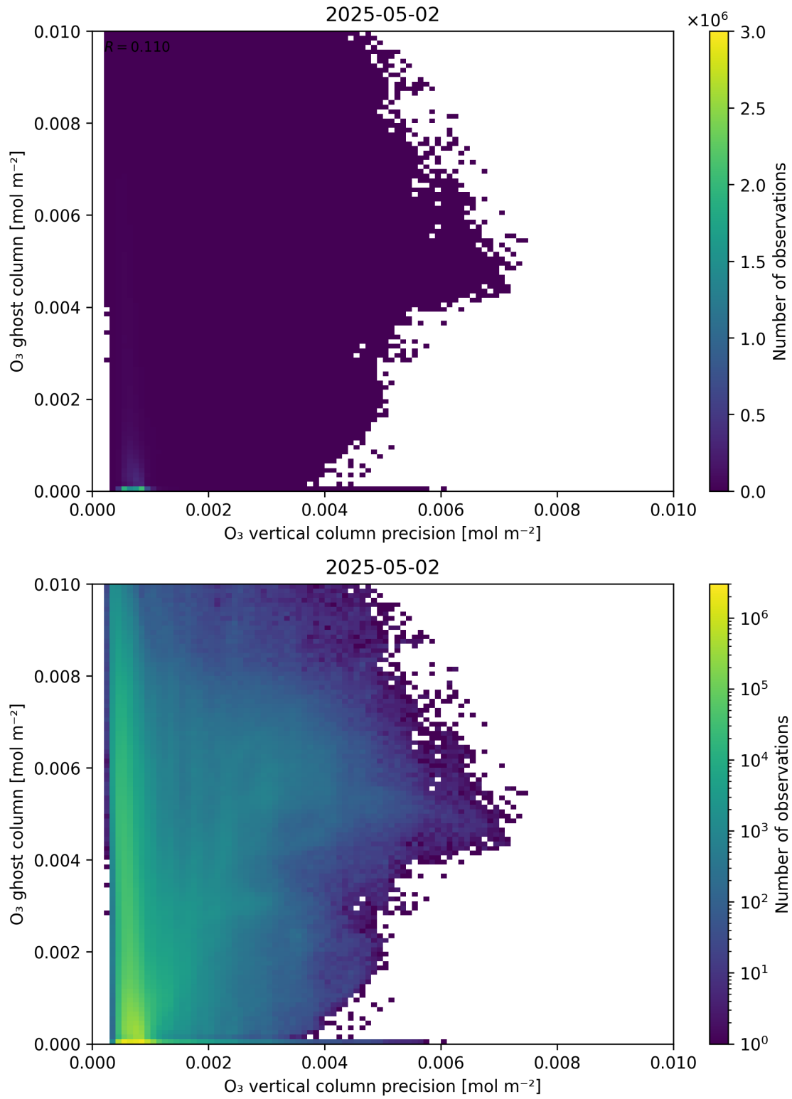
Figure 43: Scatter density plot of “O 3 vertical column precision” against “O 3 ghost column” for 2025-05-01 to 2025-05-03.
