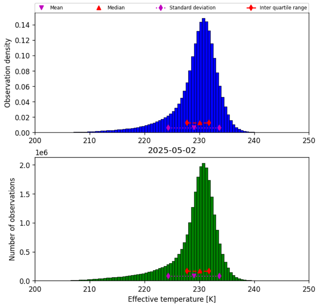
Figure 24: Histogram of “Effective temperature” for 2025-05-01 to 2025-05-03
