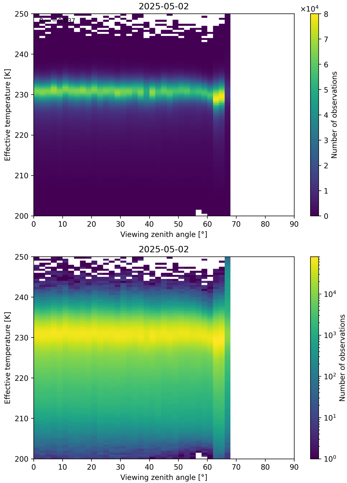
Figure 50: Scatter density plot of “Viewing zenith angle” against “Effective temperature” for 2025-05-01 to 2025-05-03.
