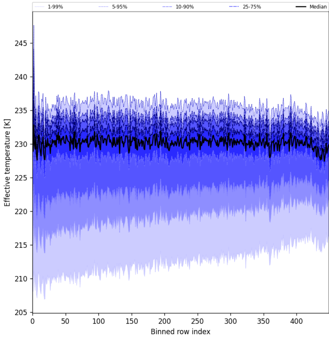
Figure 31: Along track statistics of “Effective temperature” for 2025-05-01 to 2025-05-03
