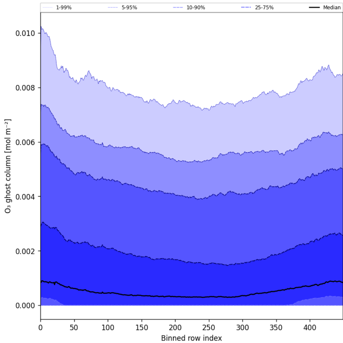
Figure 32: Along track statistics of “O 3 ghost column” for 2025-05-01 to 2025-05-03
