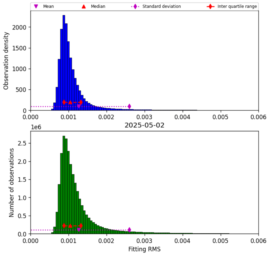
Figure 23: Histogram of “Fitting RMS” for 2025-05-01 to 2025-05-03
