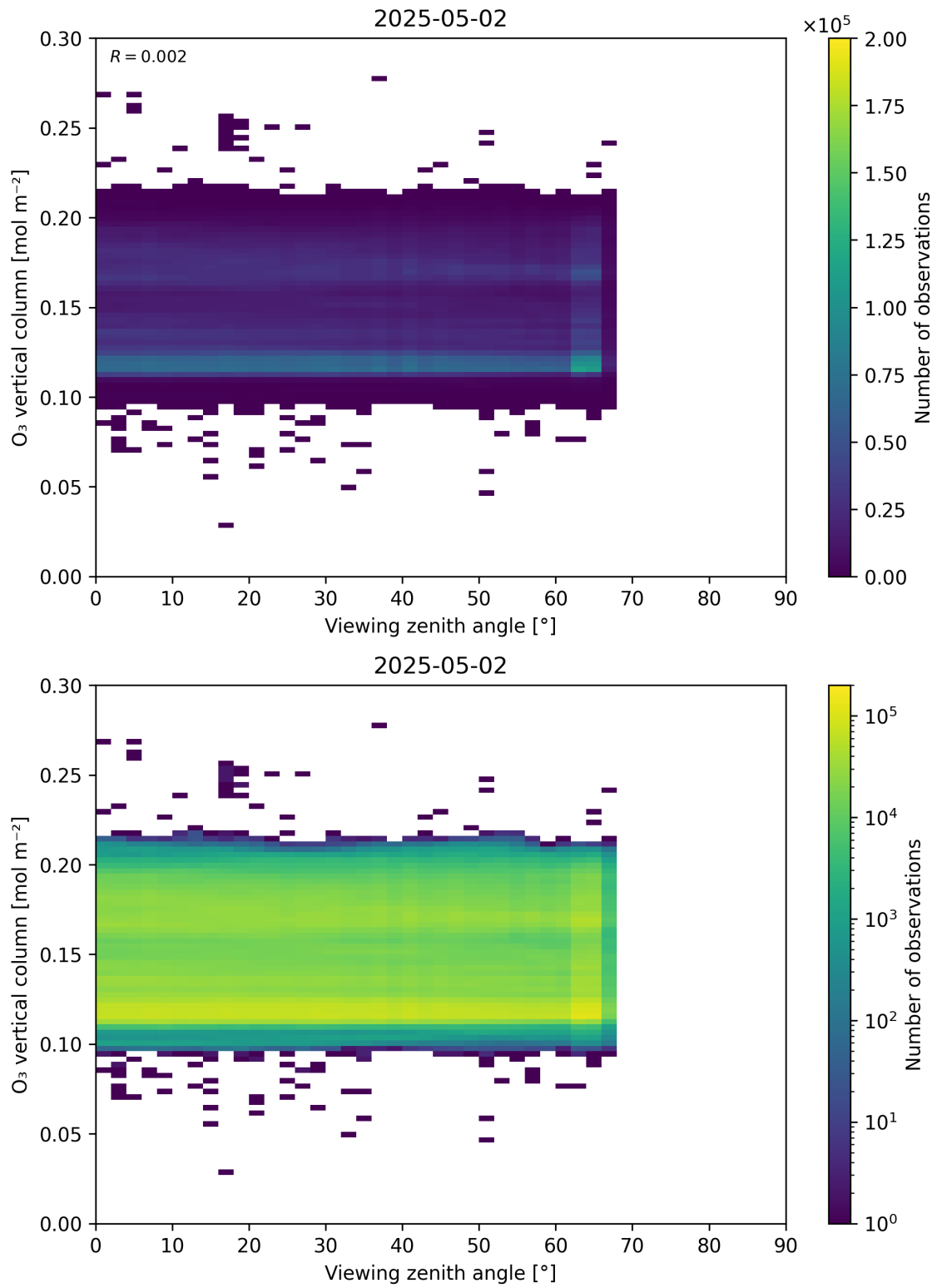
Figure 52: Scatter density plot of “Viewing zenith angle” against “O 3 vertical column” for 2025-05-01 to 2025-05-03.
