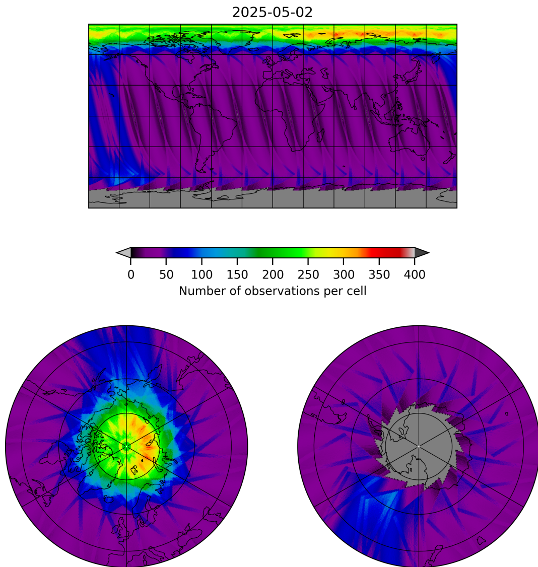
Figure 12: Map of the number of observations for 2025-05-01 to 2025-05-03
