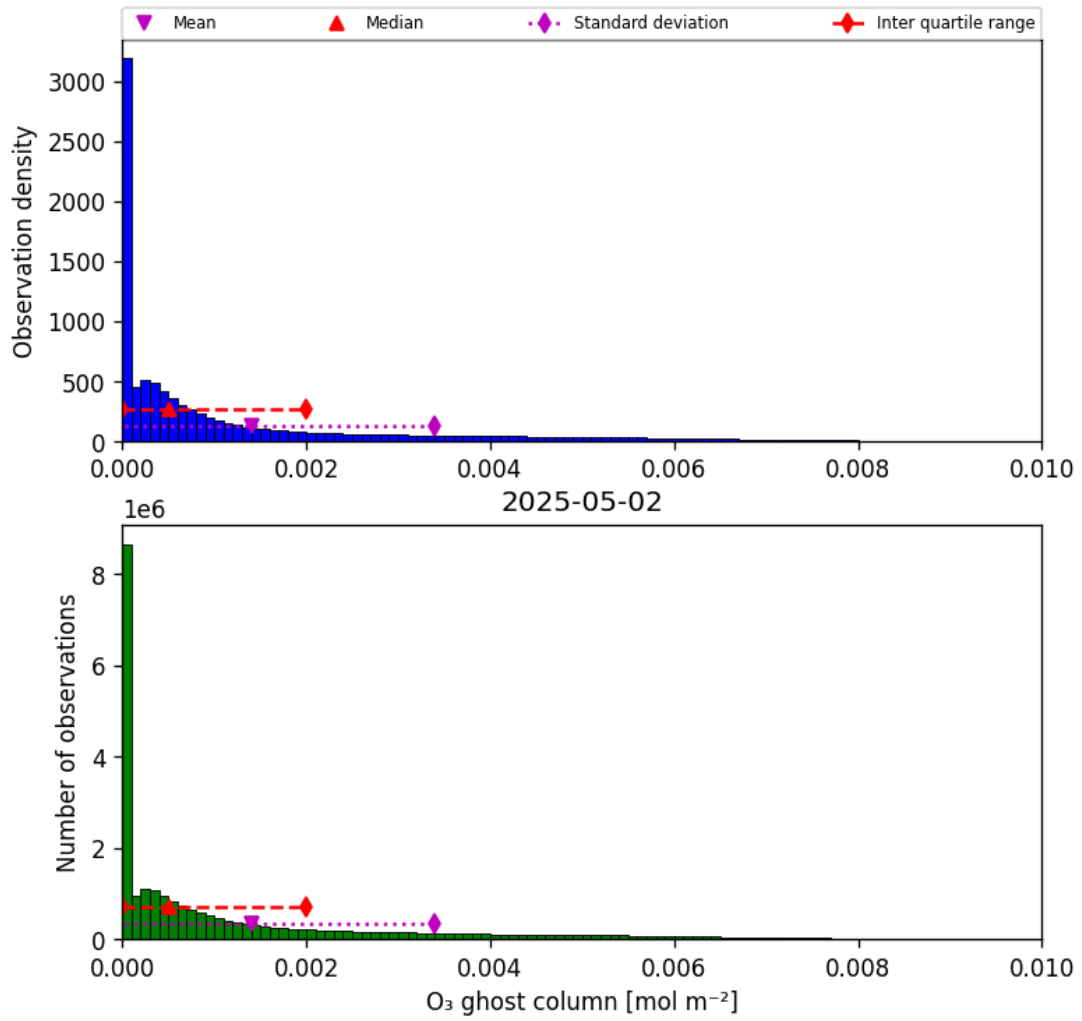
Figure 25: Histogram of “O 3 ghost column” for 2025-05-01 to 2025-05-03
