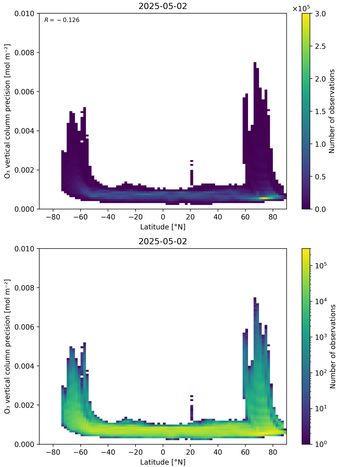
Figure 37: Scatter density plot of “Latitude” against “O 3 vertical column precision” for 2025-05-01 to 2025-05-03.
