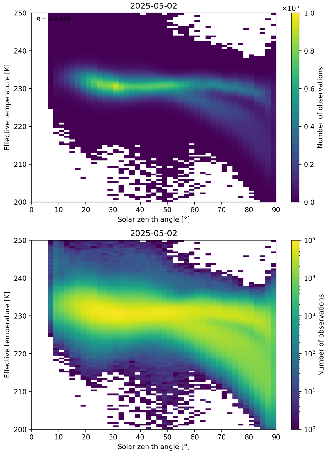
Figure 45: Scatter density plot of “Solar zenith angle” against “Effective temperature” for 2025-05-01 to 2025-05-03.
