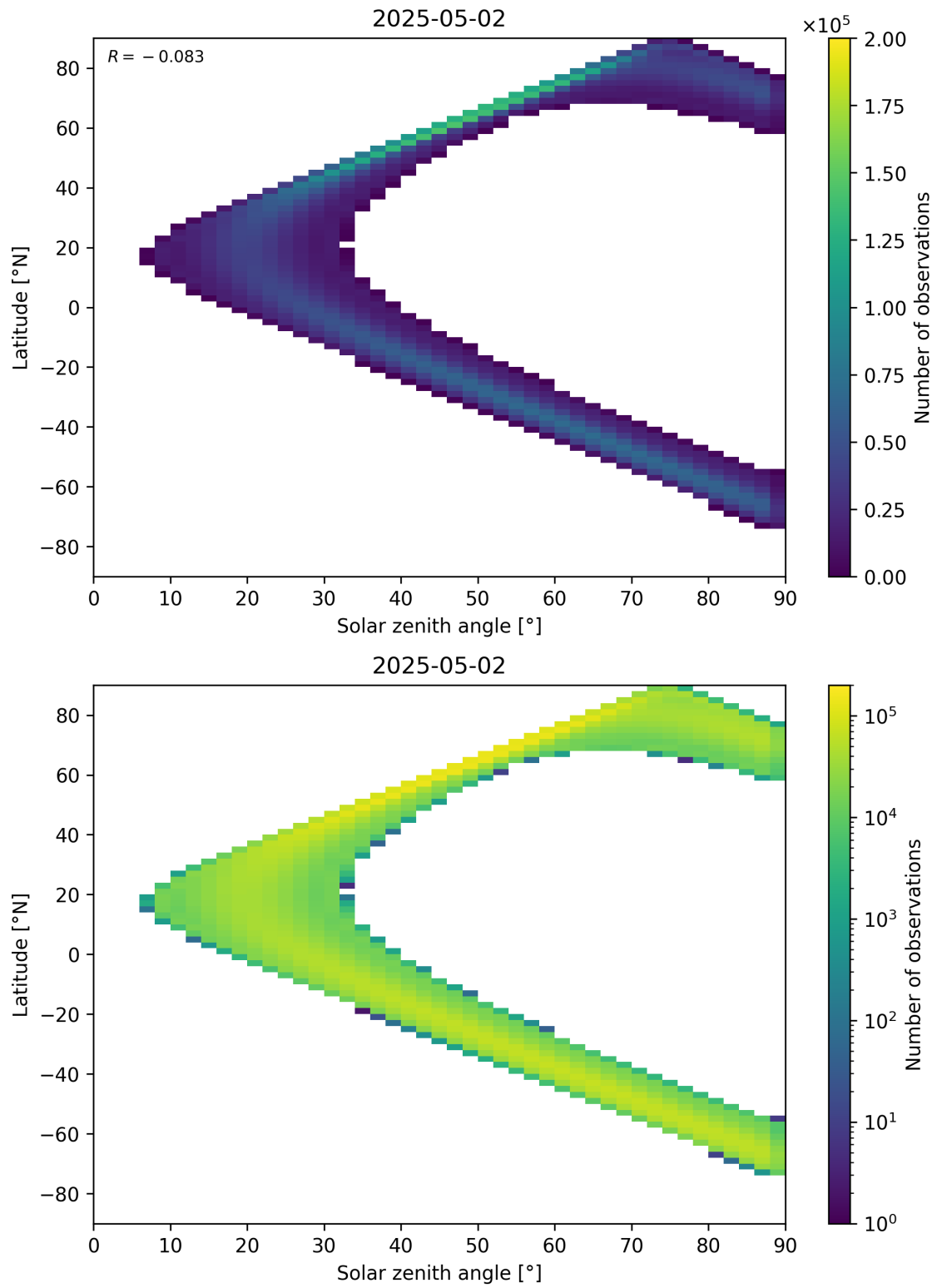
Figure 44: Scatter density plot of “Solar zenith angle” against “Latitude” for 2025-05-01 to 2025-05-03.
