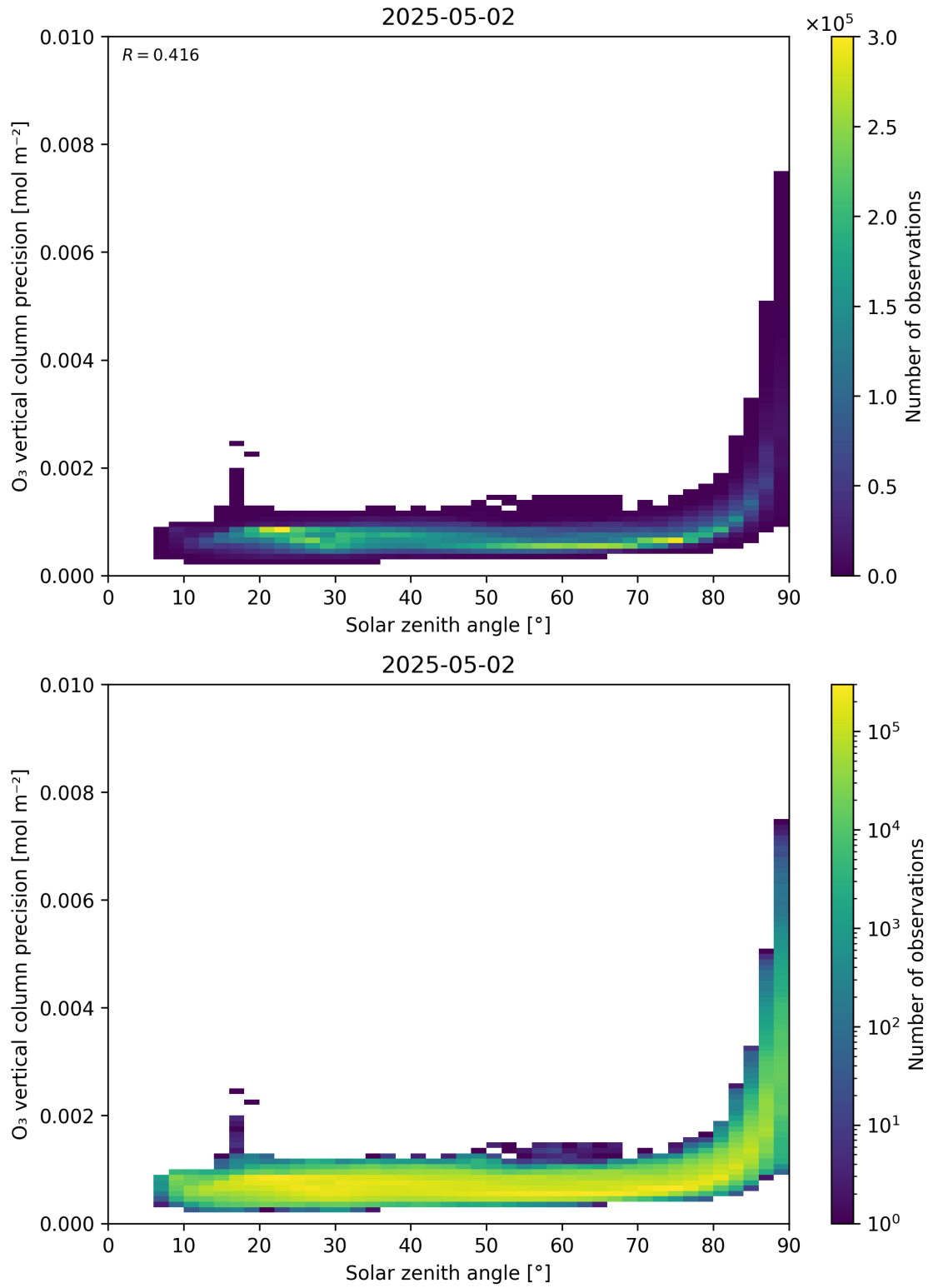
Figure 48: Scatter density plot of “Solar zenith angle” against “O 3 vertical column precision” for 2025-05-01 to 2025-05-03.
