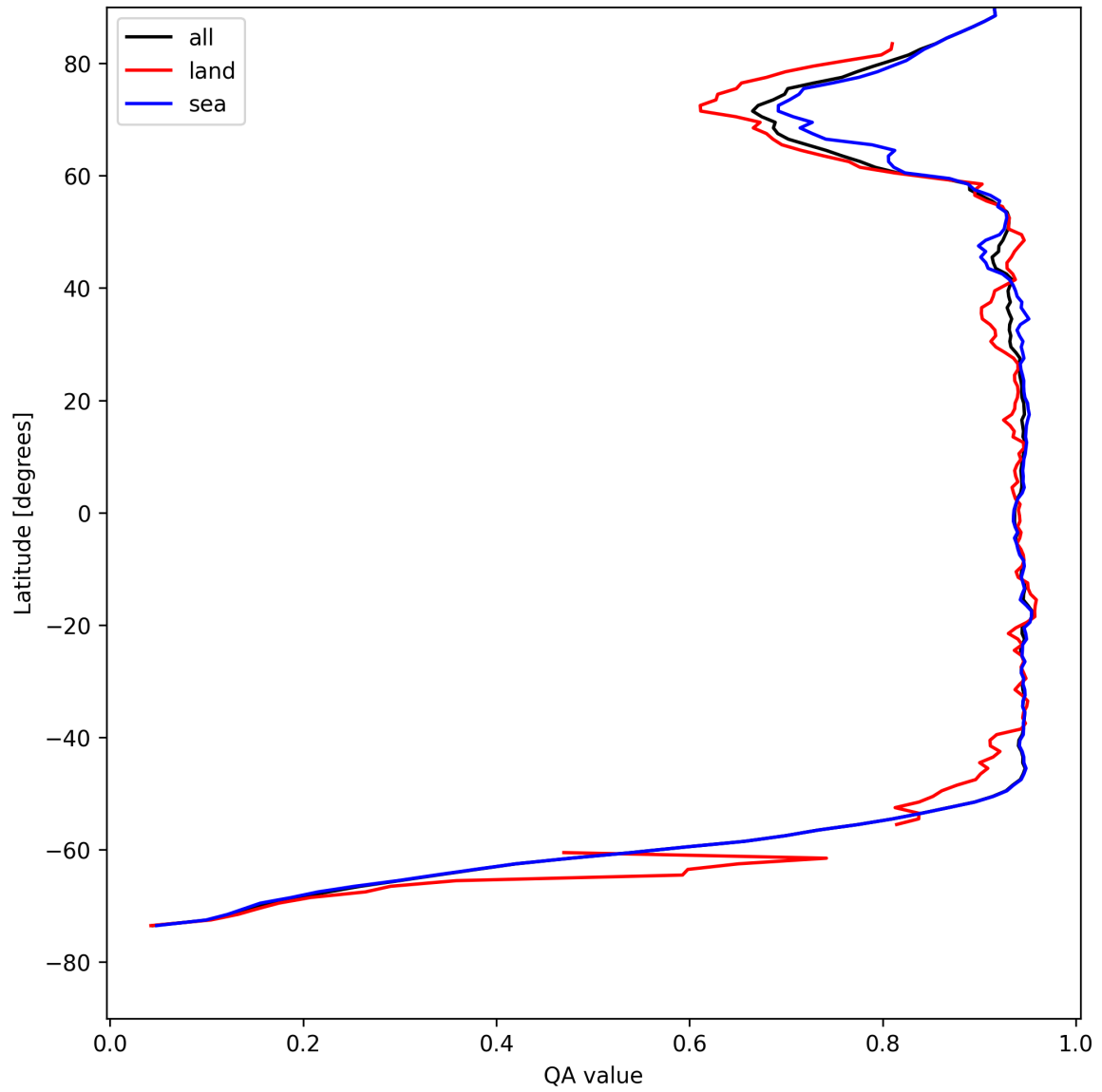
Figure 13: Zonal average of “QA value” for 2025-05-01 to 2025-05-03.
