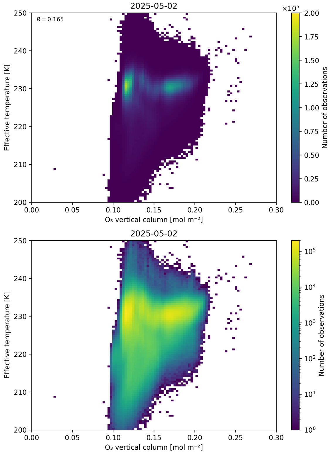
Figure 39: Scatter density plot of “O 3 vertical column” against “Effective temperature” for 2025-05-01 to 2025-05-03.
