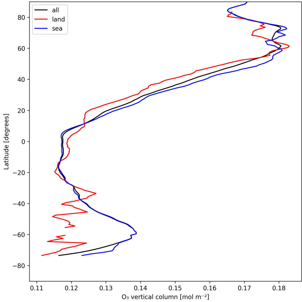
Figure 14: Zonal average of “O 3 vertical column” for 2025-05-01 to 2025-05-03.
