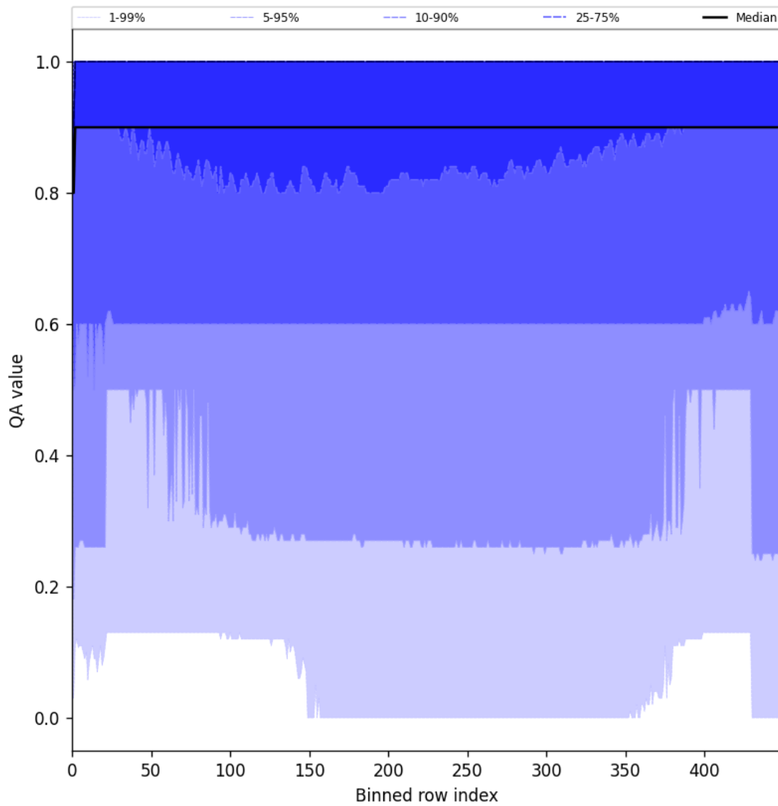
Figure 27: Along track statistics of “QA value” for 2025-05-01 to 2025-05-03
