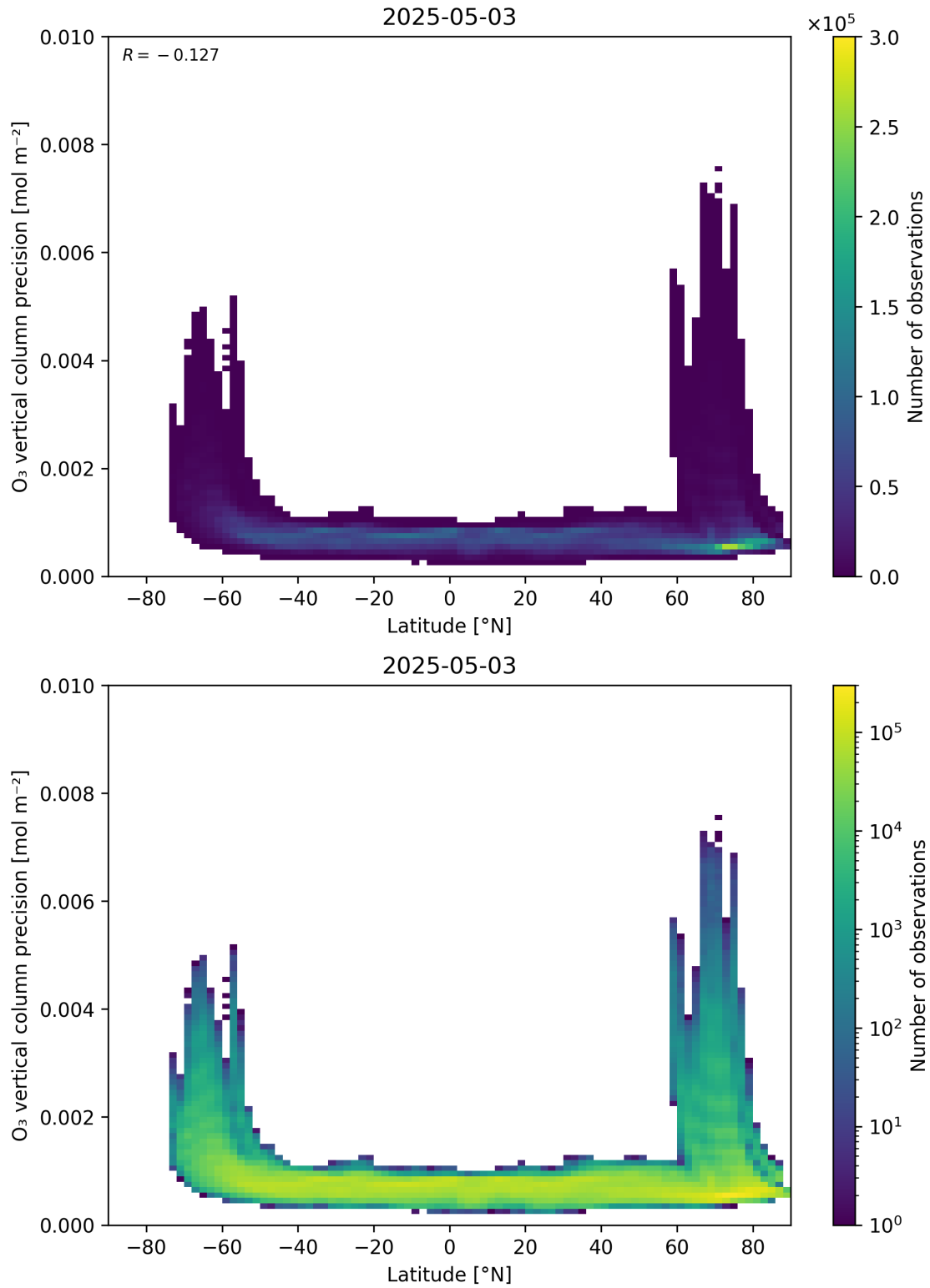
Figure 37: Scatter density plot of “Latitude” against “O 3 vertical column precision” for 2025-05-02 to 2025-05-04.
