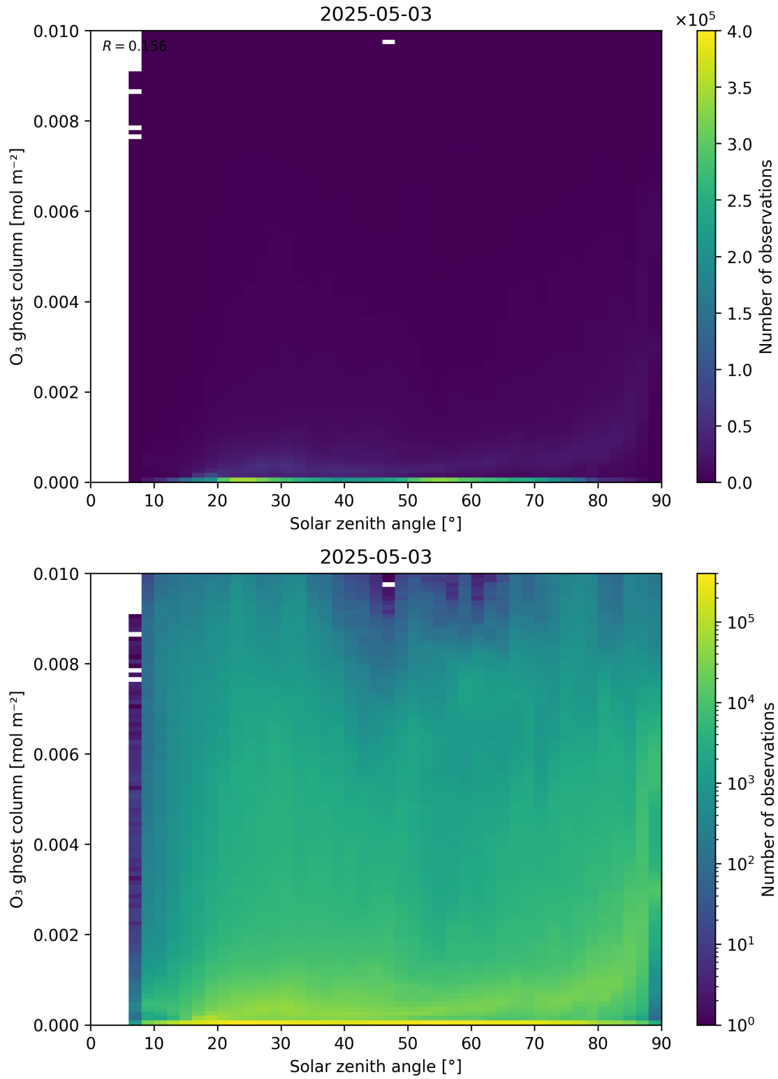
Figure 46: Scatter density plot of “Solar zenith angle” against “O 3 ghost column” for 2025-05-02 to 2025-05-04.
