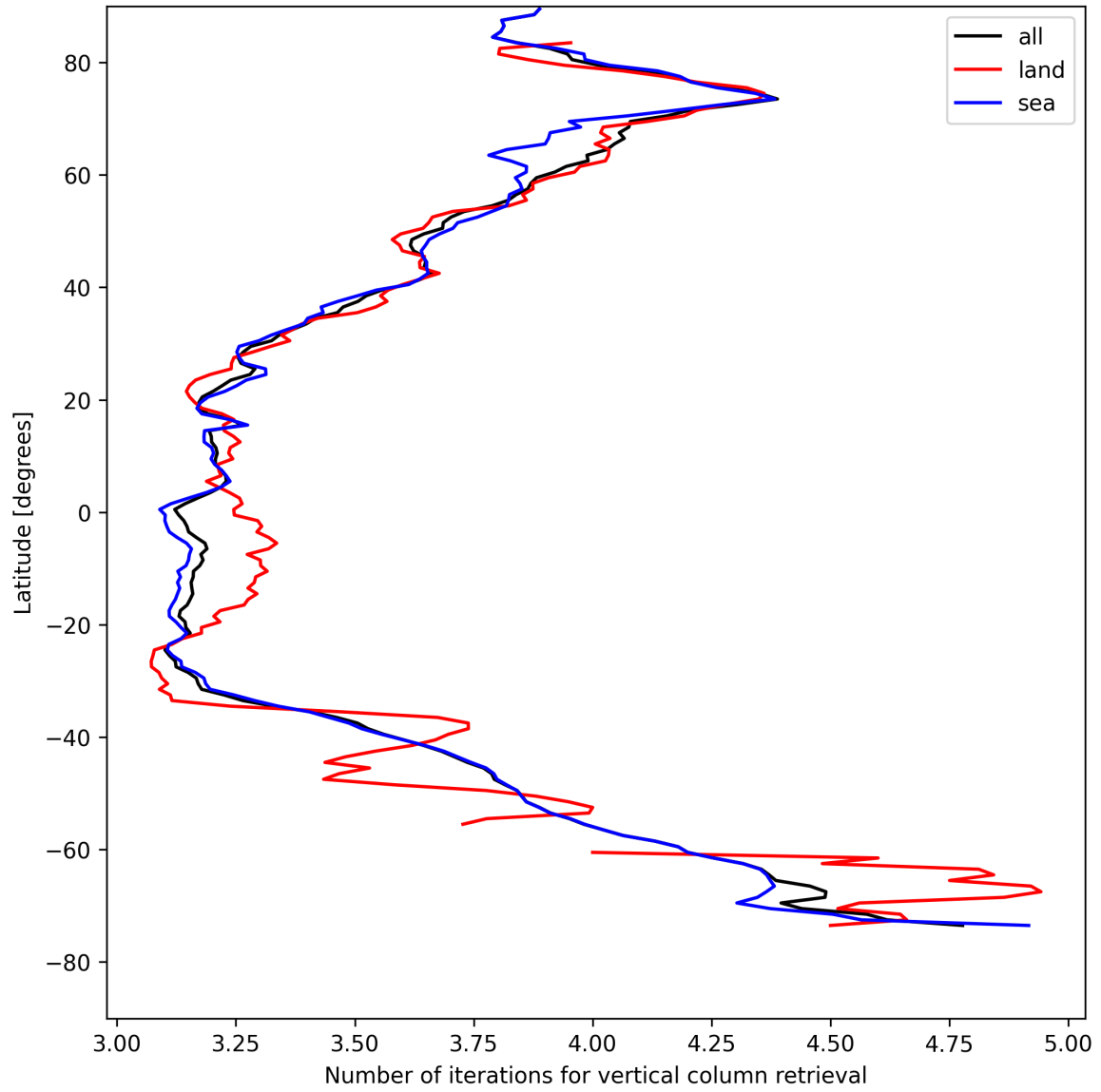
Figure 19: Zonal average of “Number of iterations for vertical column retrieval” for 2025-05-02 to 2025-05-04.
