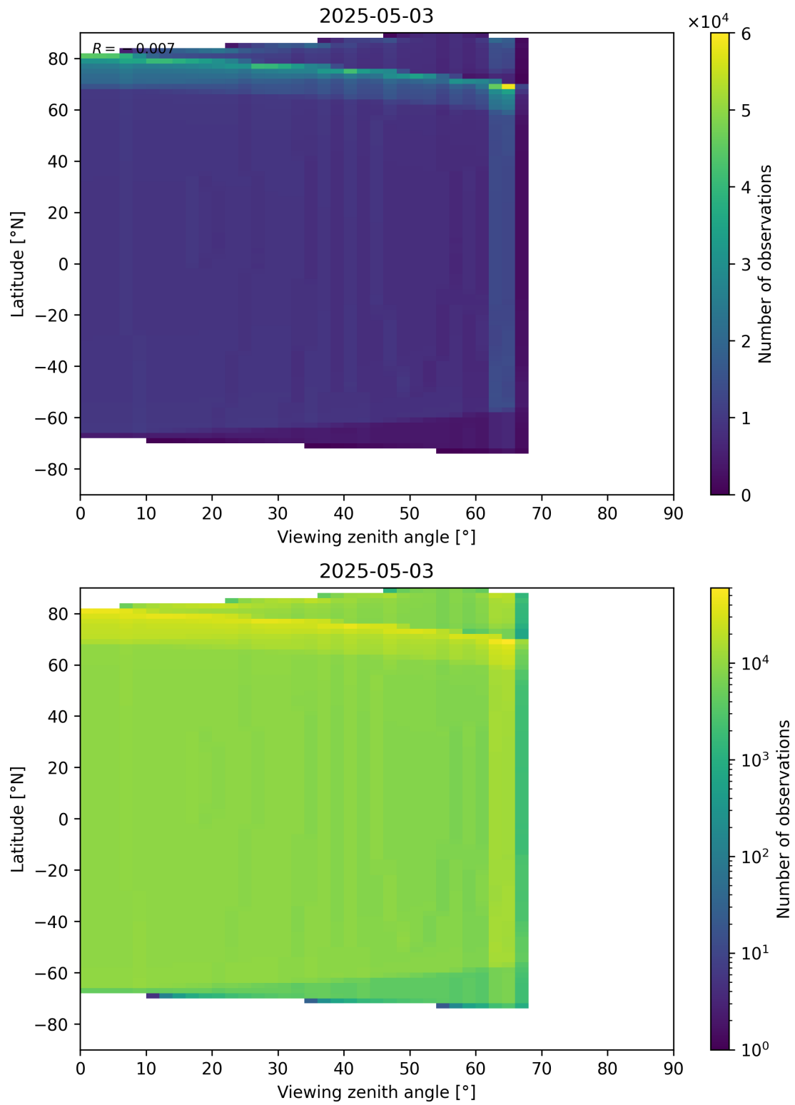
Figure 49: Scatter density plot of “Viewing zenith angle” against “Latitude” for 2025-05-02 to 2025-05-04.
