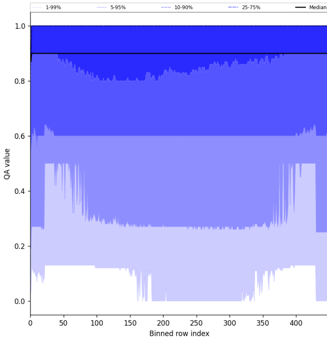
Figure 27: Along track statistics of “QA value” for 2025-05-02 to 2025-05-04
