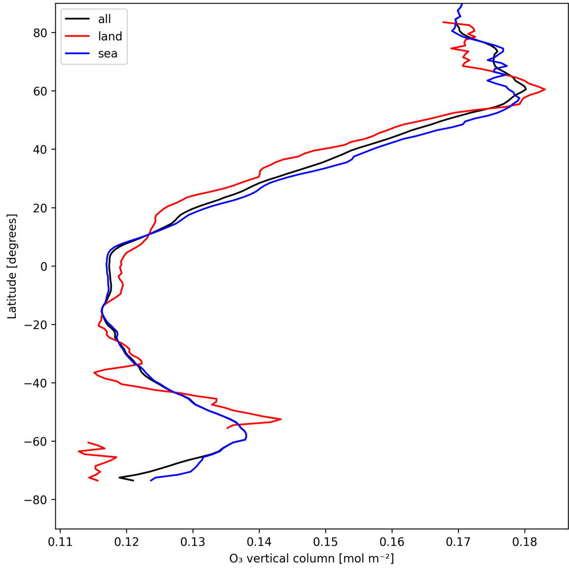
Figure 14: Zonal average of “O 3 vertical column” for 2025-05-02 to 2025-05-04.
