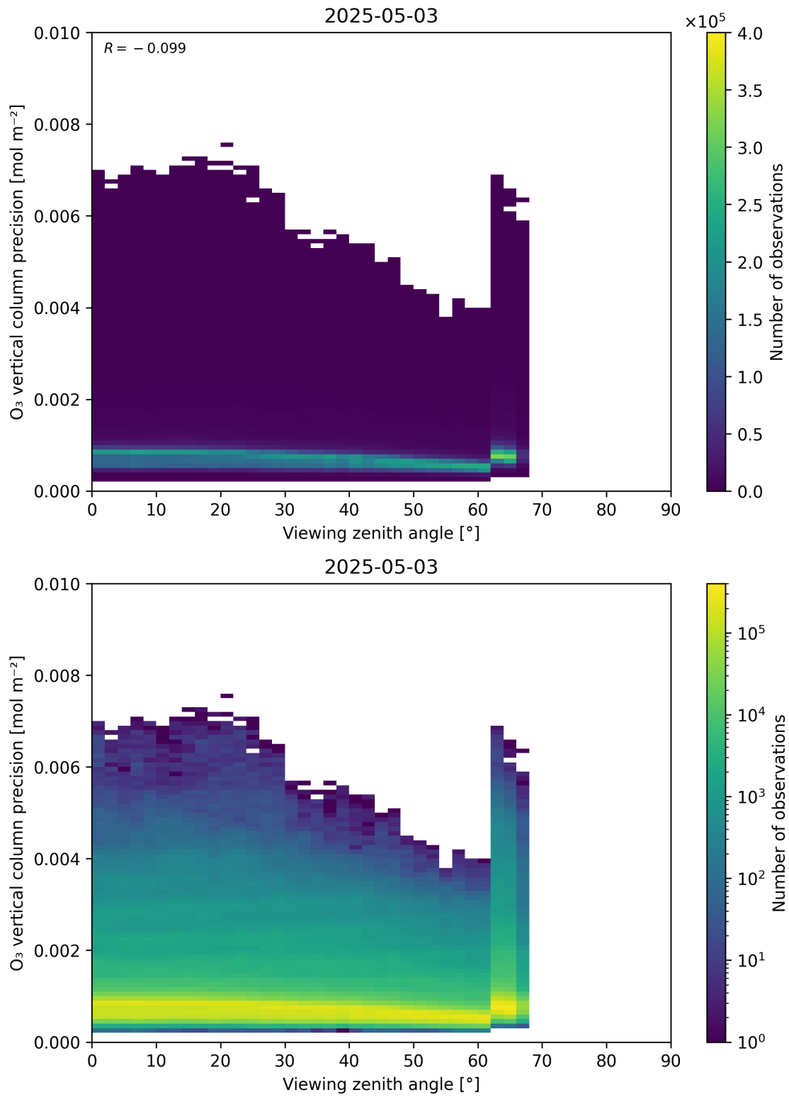
Figure 53: Scatter density plot of “Viewing zenith angle” against “O 3 vertical column precision” for 2025-05-02 to 2025-05-04.
