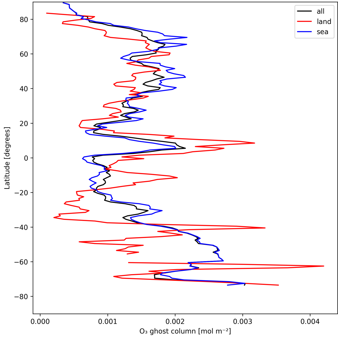
Figure 18: Zonal average of “O 3 ghost column” for 2025-05-02 to 2025-05-04.
