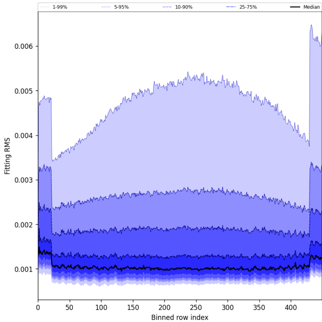
Figure 30: Along track statistics of “Fitting RMS” for 2025-05-02 to 2025-05-04
