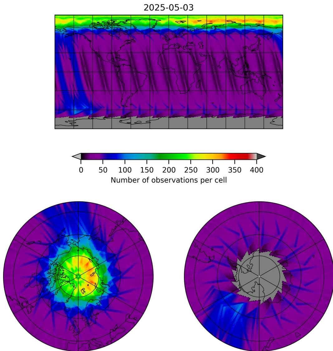
Figure 12: Map of the number of observations for 2025-05-02 to 2025-05-04
