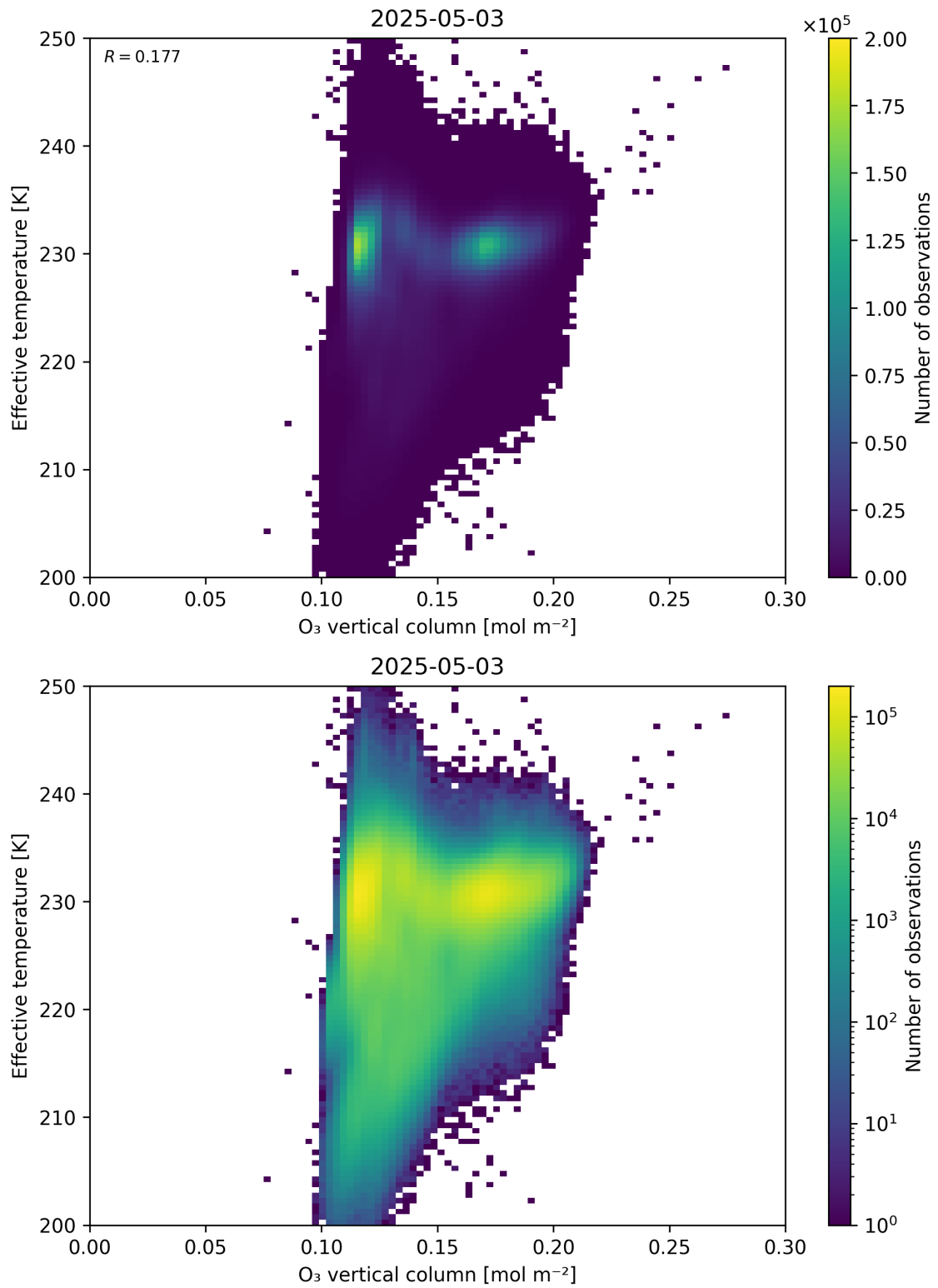
Figure 39: Scatter density plot of “O 3 vertical column” against “Effective temperature” for 2025-05-02 to 2025-05-04.
