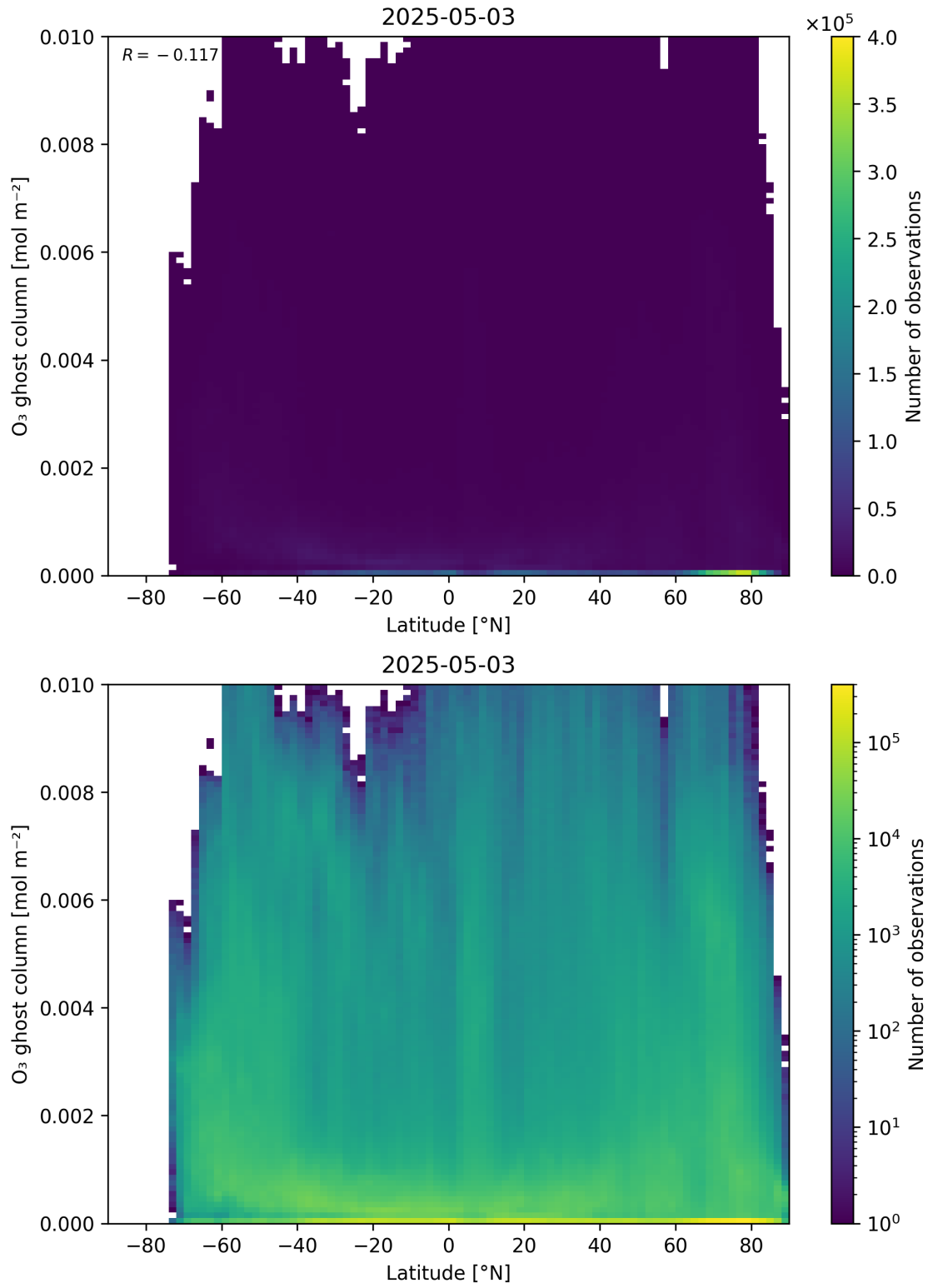
Figure 35: Scatter density plot of “Latitude” against “O 3 ghost column” for 2025-05-02 to 2025-05-04.
