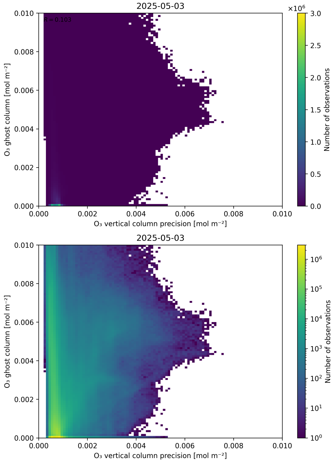
Figure 43: Scatter density plot of “ \text{O}_3 vertical column precision” against “ \text{O}_3 ghost column” for 2025-05-02 to 2025-05-04.
