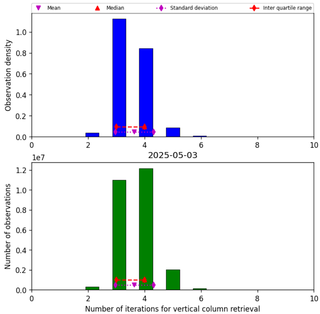
Figure 26: Histogram of “Number of iterations for vertical column retrieval” for 2025-05-02 to 2025-05-04
