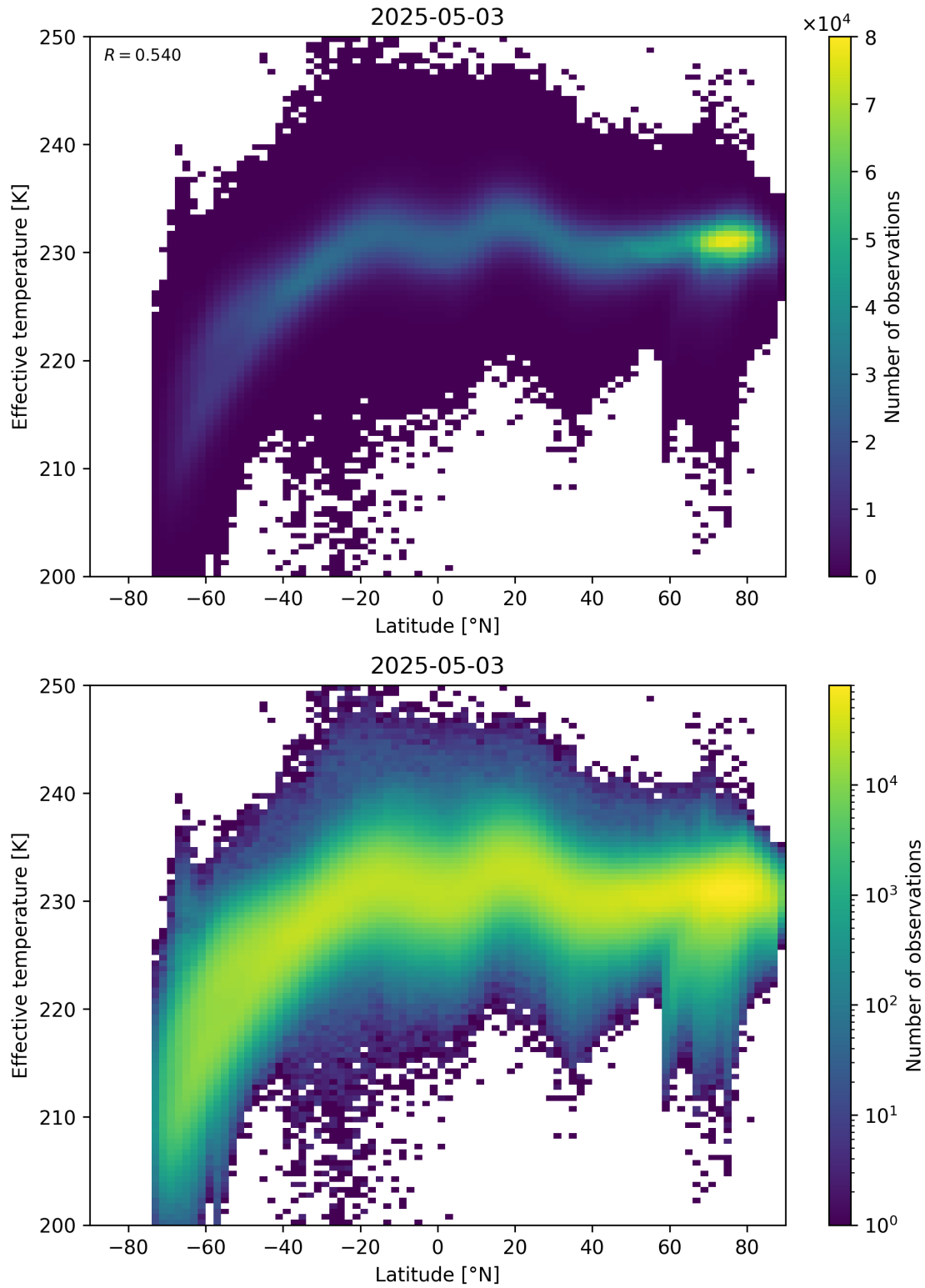
Figure 34: Scatter density plot of “Latitude” against “Effective temperature” for 2025-05-02 to 2025-05-04.
