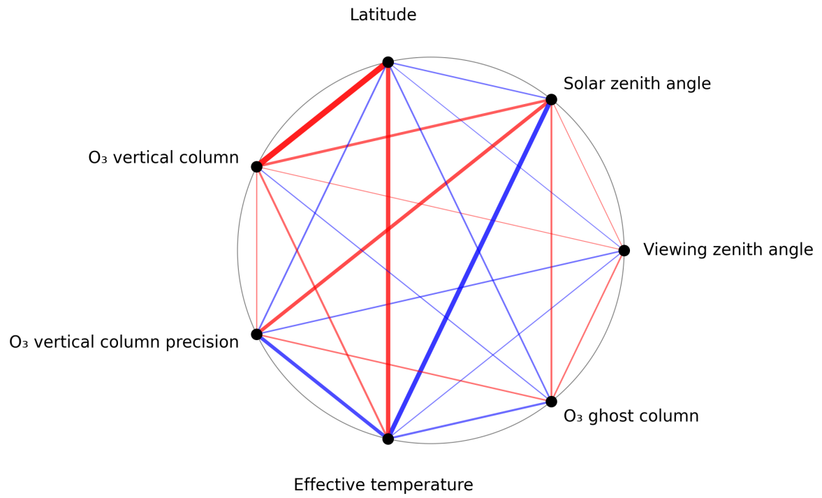
Figure 1: Map of correlation graph for 2025-05-02 to 2025-05-04.
