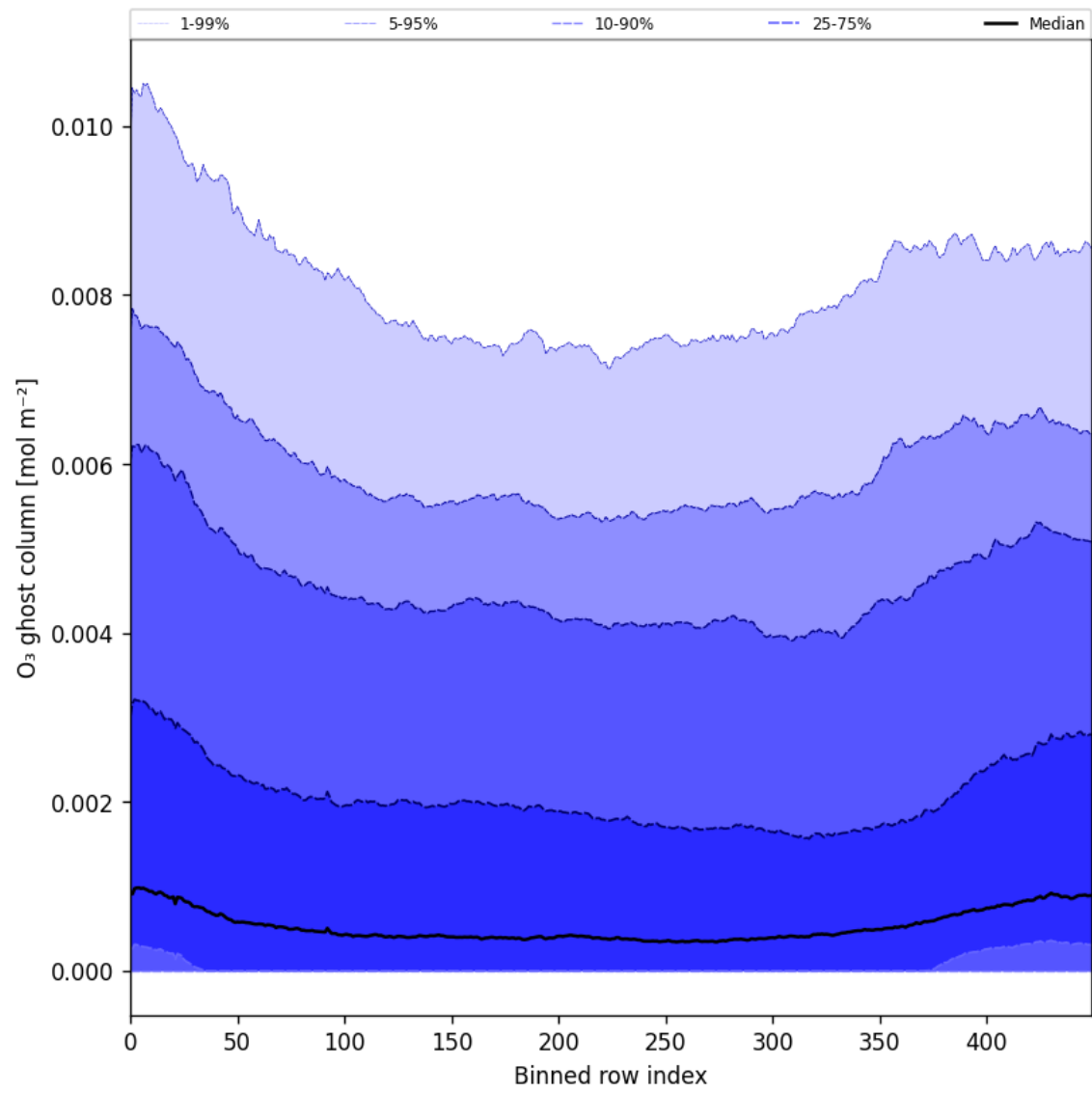
Figure 32: Along track statistics of “O 3 ghost column” for 2025-05-02 to 2025-05-04
