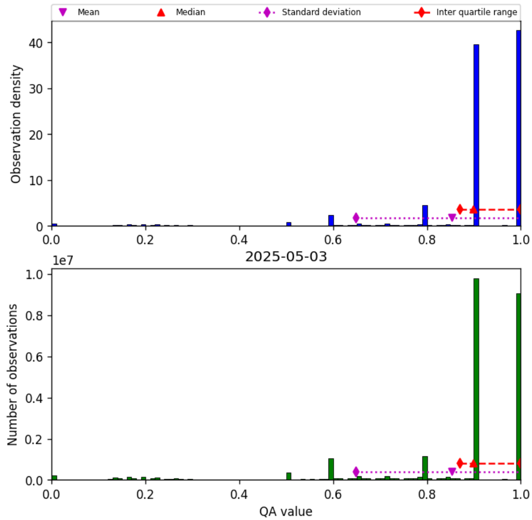
Figure 20: Histogram of “QA value” for 2025-05-02 to 2025-05-04
