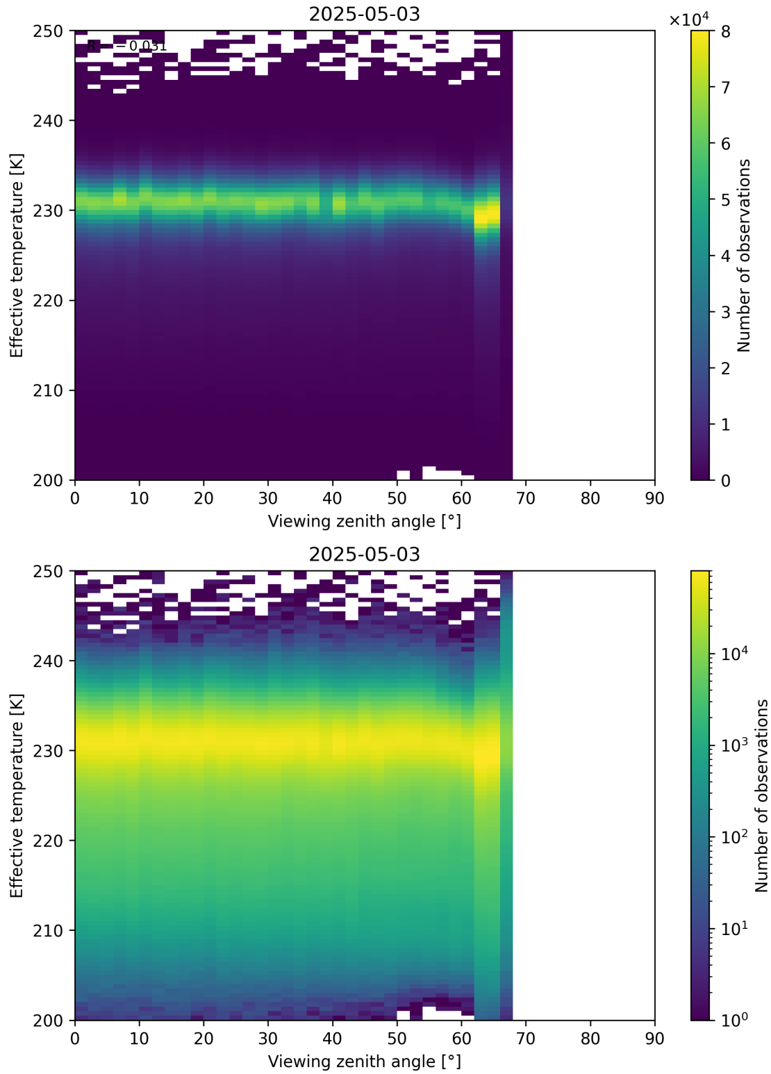
Figure 50: Scatter density plot of “Viewing zenith angle” against “Effective temperature” for 2025-05-02 to 2025-05-04.
