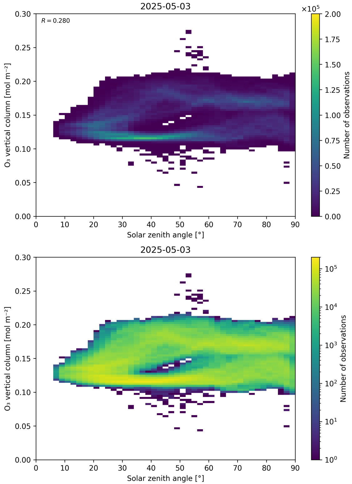
Figure 47: Scatter density plot of “Solar zenith angle” against “O 3 vertical column” for 2025-05-02 to 2025-05-04.
