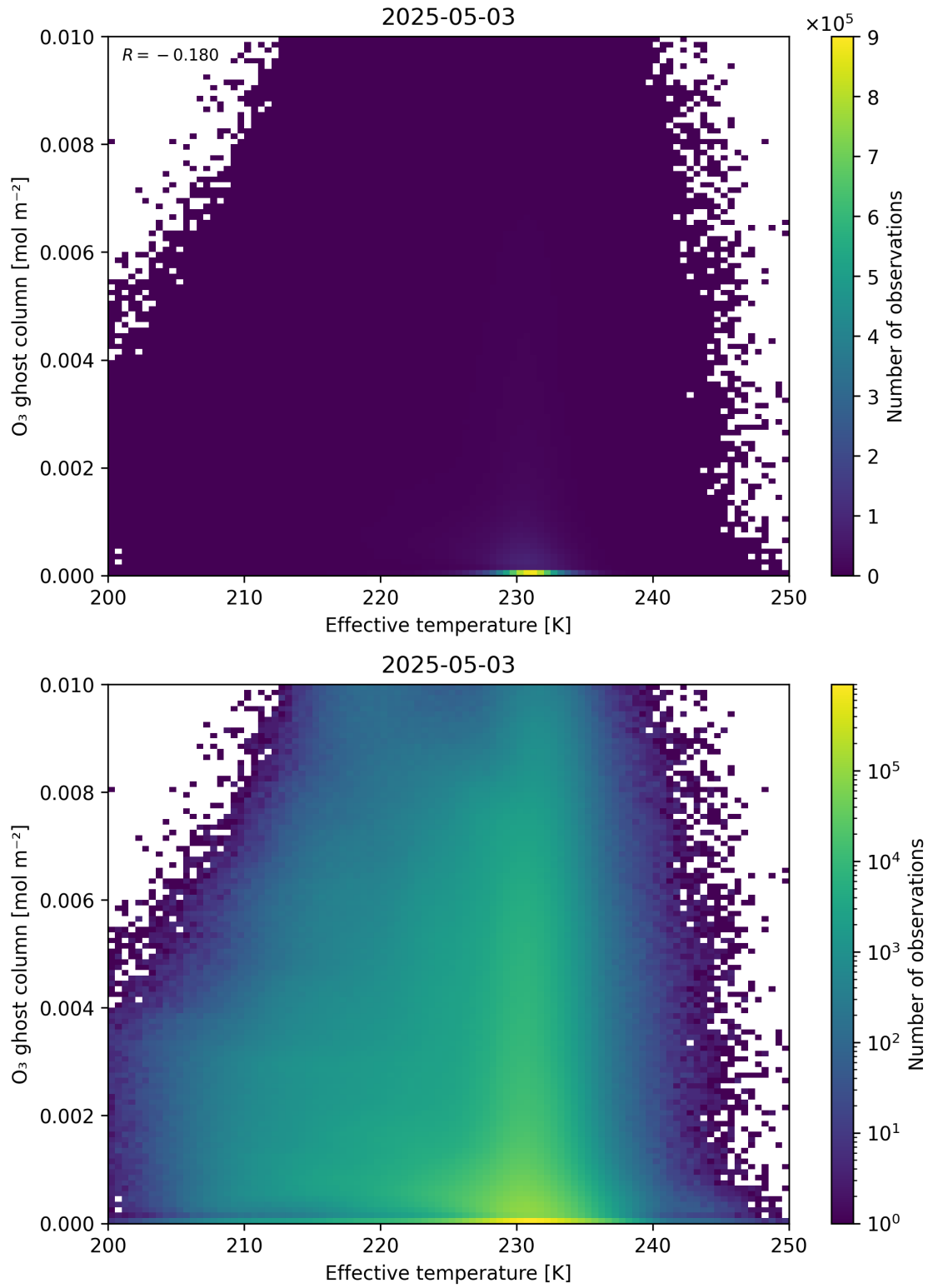
Figure 38: Scatter density plot of “Effective temperature” against “O 3 ghost column” for 2025-05-02 to 2025-05-04.
