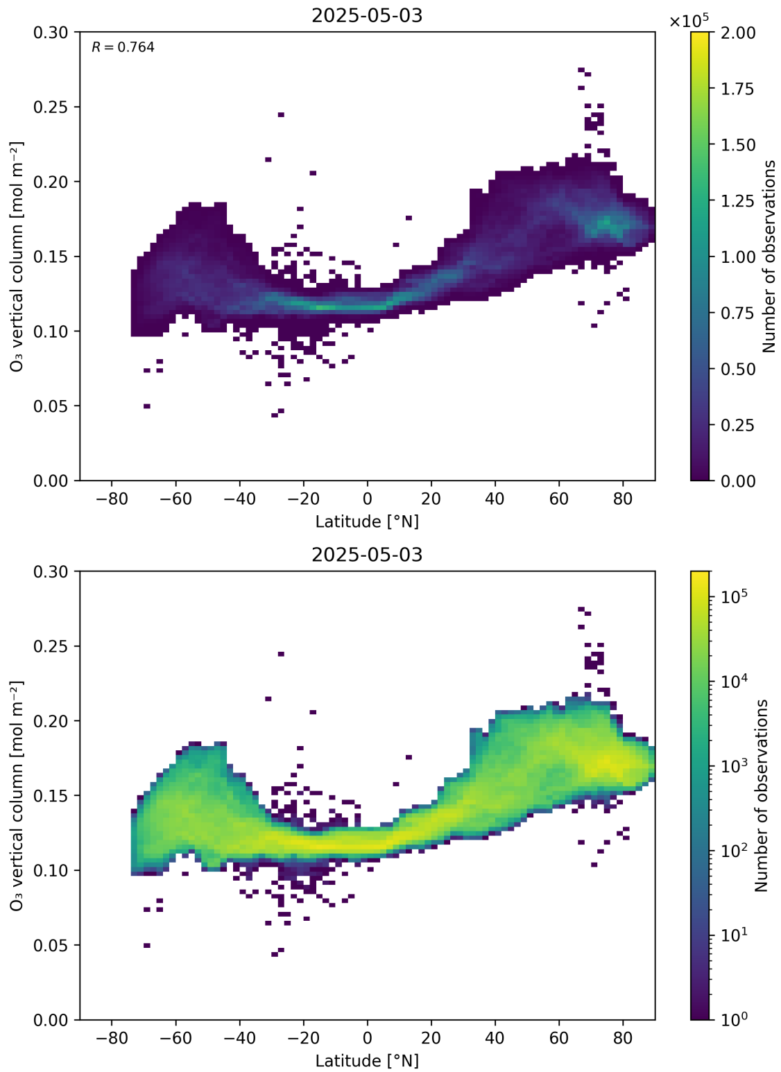
Figure 36: Scatter density plot of “Latitude” against “O 3 vertical column” for 2025-05-02 to 2025-05-04.
