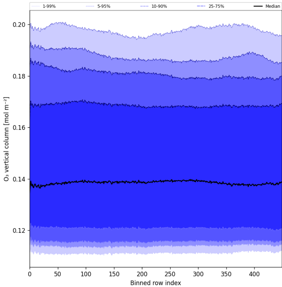
Figure 28: Along track statistics of “O 3 vertical column” for 2025-05-02 to 2025-05-04
