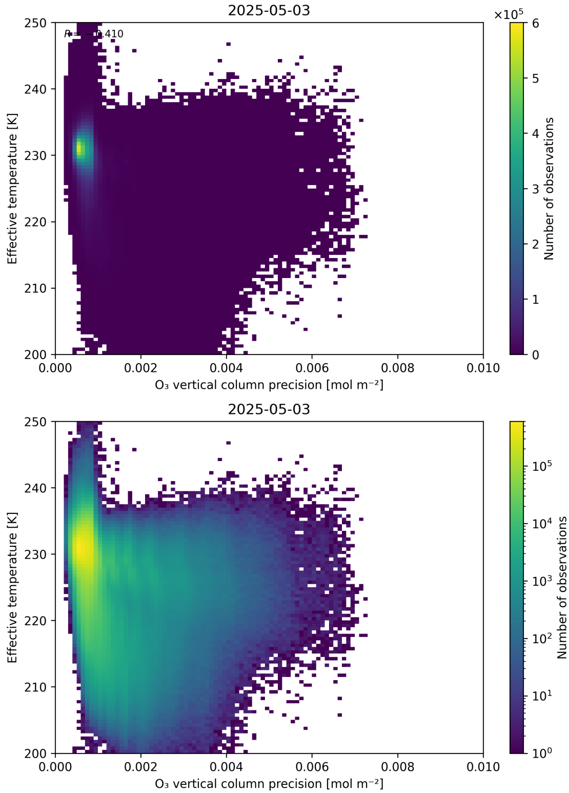
Figure 42: Scatter density plot of “O 3 vertical column precision” against “Effective temperature” for 2025-05-02 to 2025-05-04.
