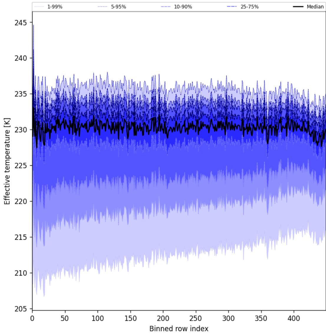
Figure 31: Along track statistics of “Effective temperature” for 2025-05-02 to 2025-05-04
