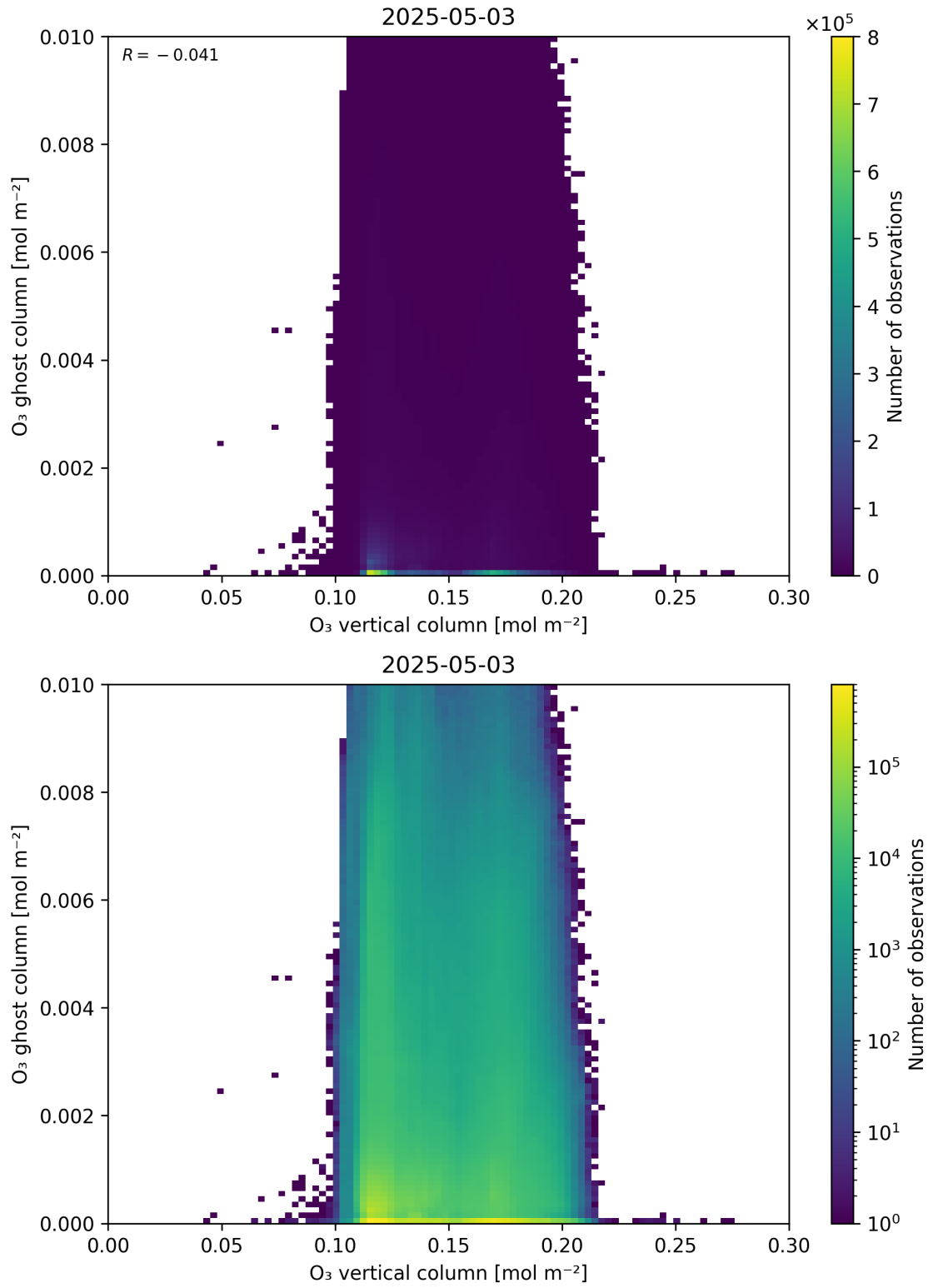
Figure 40: Scatter density plot of “O 3 vertical column” against “O 3 ghost column” for 2025-05-02 to 2025-05-04.
