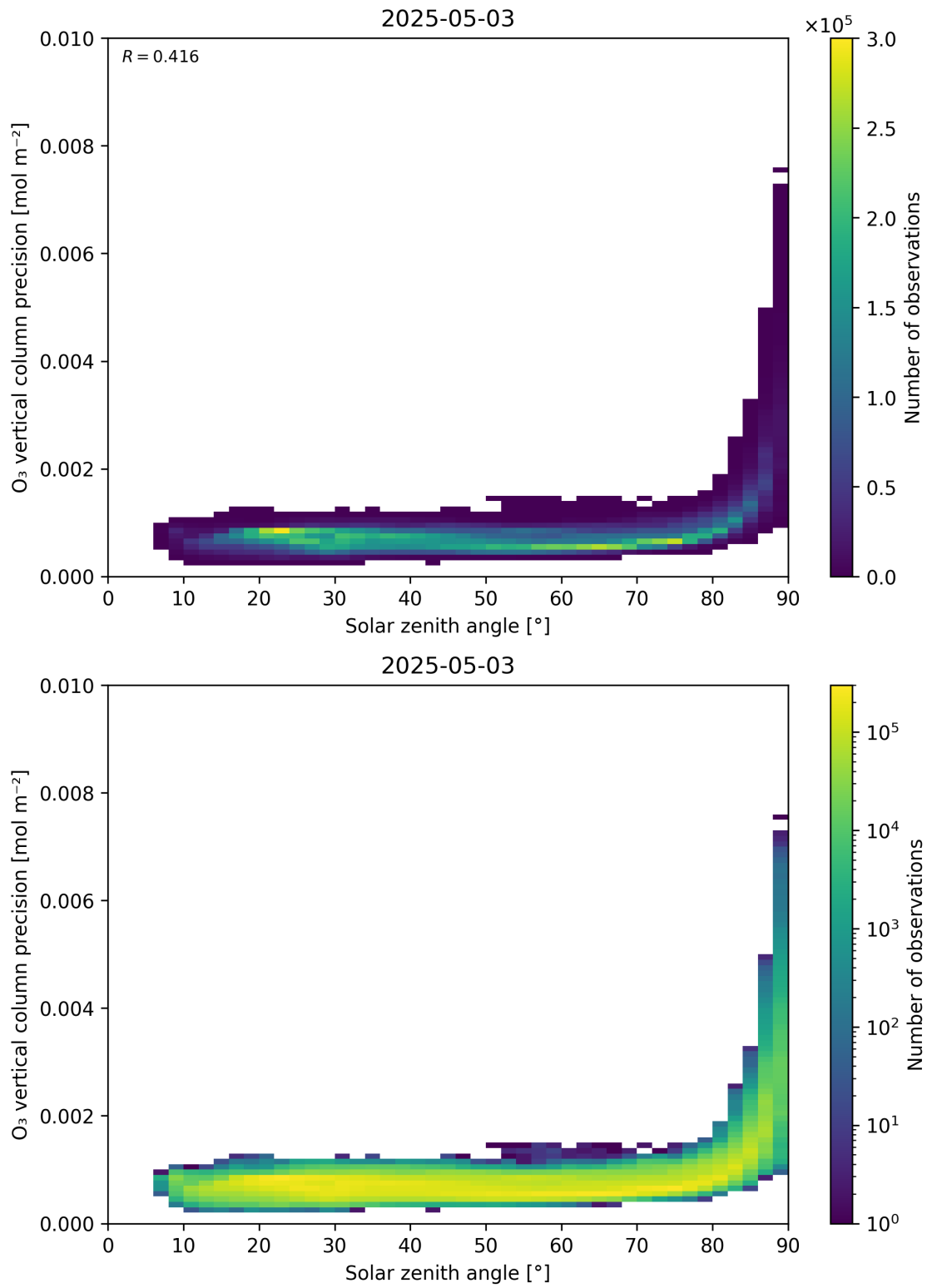
Figure 48: Scatter density plot of “Solar zenith angle” against “O 3 vertical column precision” for 2025-05-02 to 2025-05-04.
