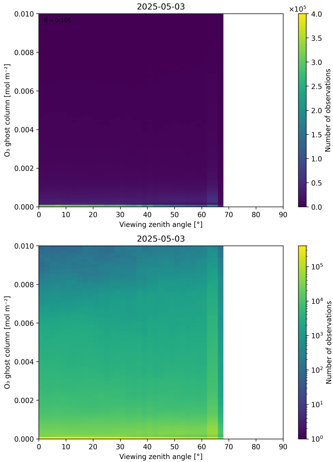
Figure 51: Scatter density plot of “Viewing zenith angle” against “O 3 ghost column” for 2025-05-02 to 2025-05-04.
