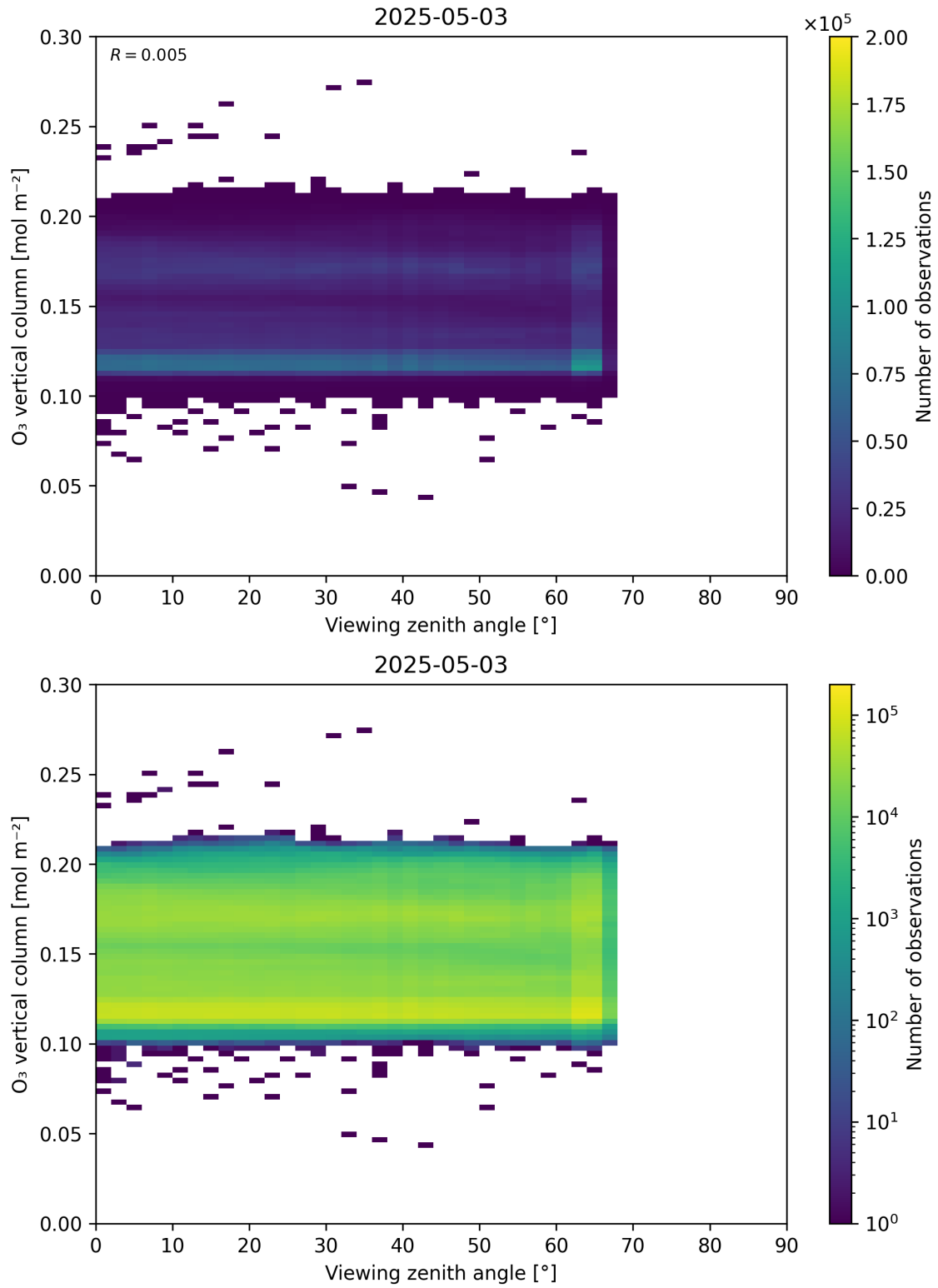
Figure 52: Scatter density plot of “Viewing zenith angle” against “O 3 vertical column” for 2025-05-02 to 2025-05-04.
