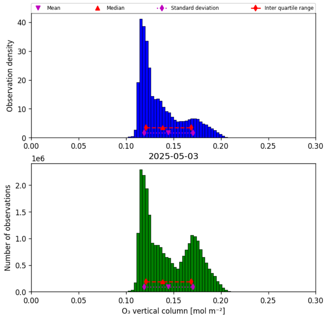
Figure 21: Histogram of “O 3 vertical column” for 2025-05-02 to 2025-05-04
