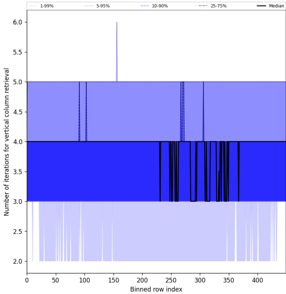
Figure 33: Along track statistics of “Number of iterations for vertical column retrieval” for 2025-05-02 to 2025-05-04
