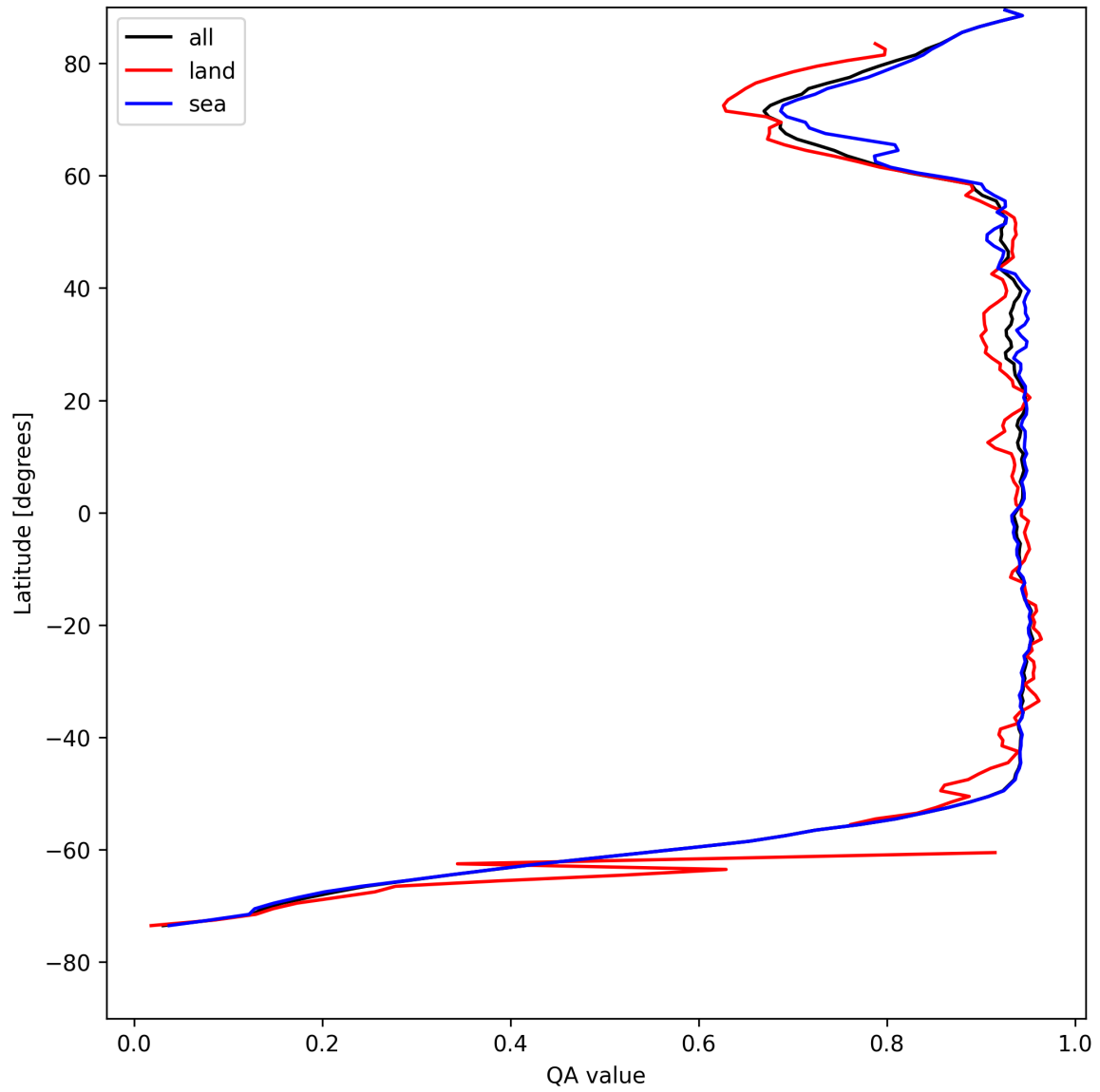
Figure 13: Zonal average of “QA value” for 2025-05-02 to 2025-05-04.
