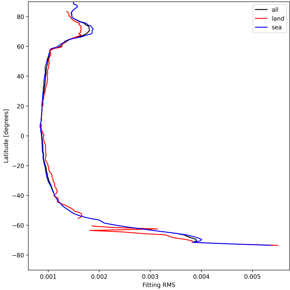
Figure 16: Zonal average of “Fitting RMS” for 2025-05-02 to 2025-05-04.
