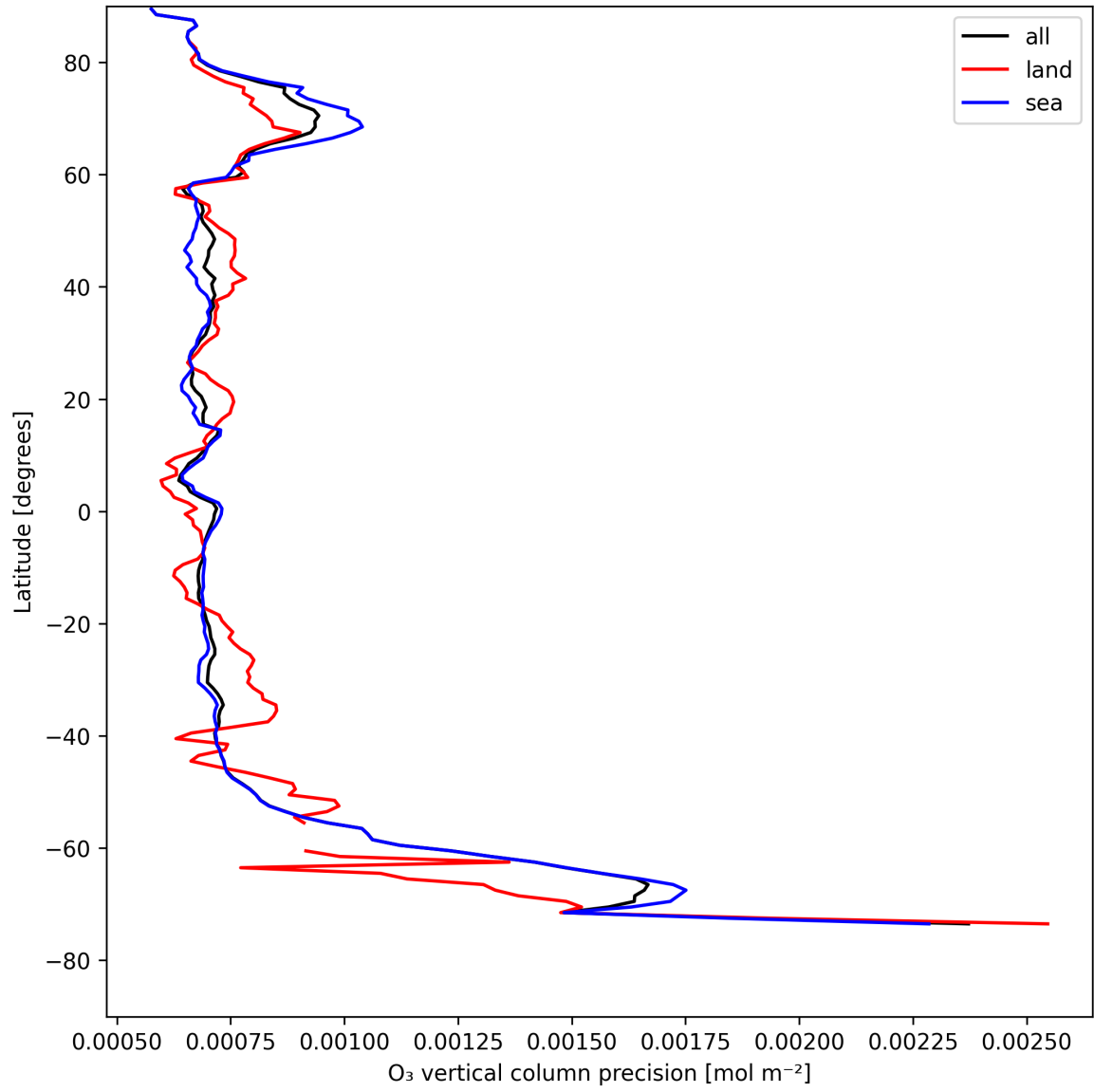
Figure 15: Zonal average of “O 3 vertical column precision” for 2025-05-02 to 2025-05-04.
