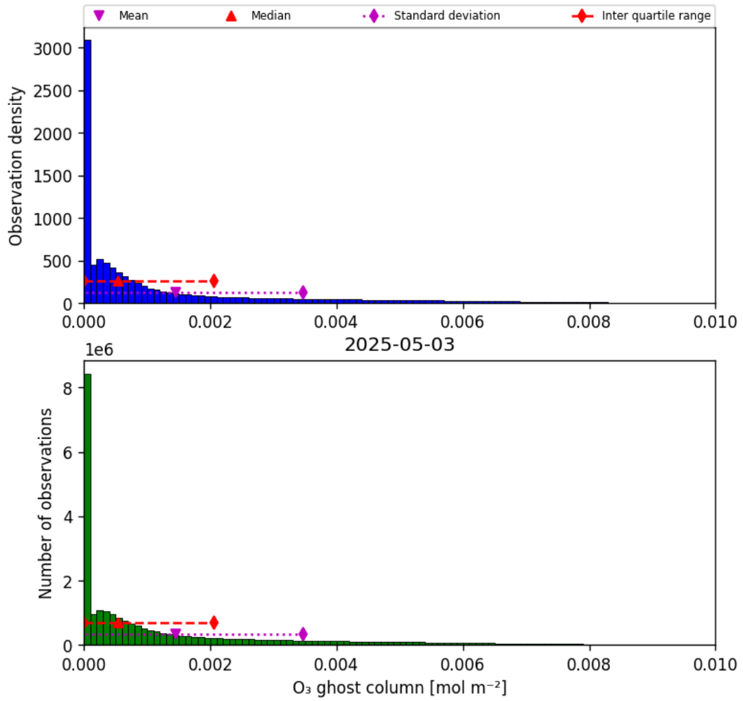
Figure 25: Histogram of “O 3 ghost column” for 2025-05-02 to 2025-05-04
