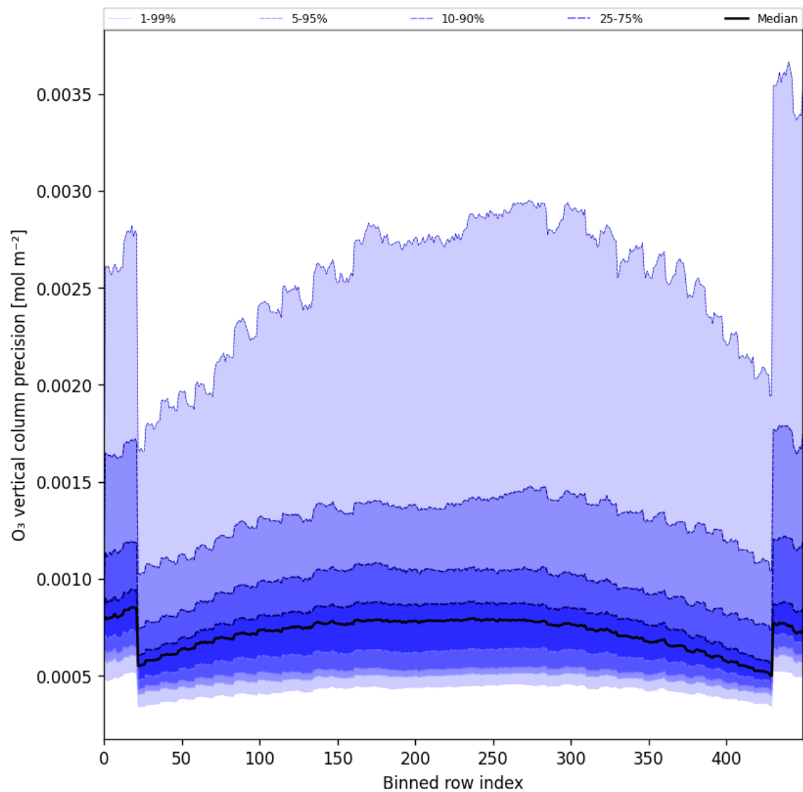
Figure 29: Along track statistics of “O 3 vertical column precision” for 2025-05-02 to 2025-05-04
