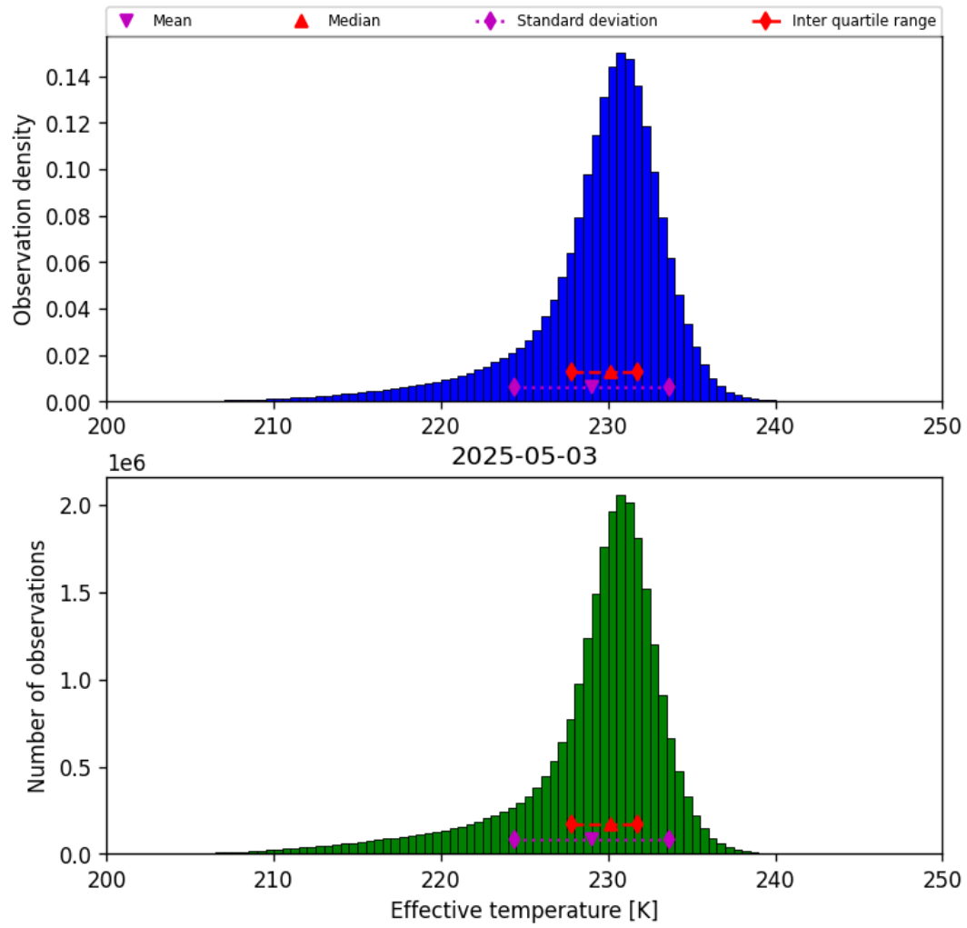
Figure 24: Histogram of “Effective temperature” for 2025-05-02 to 2025-05-04
