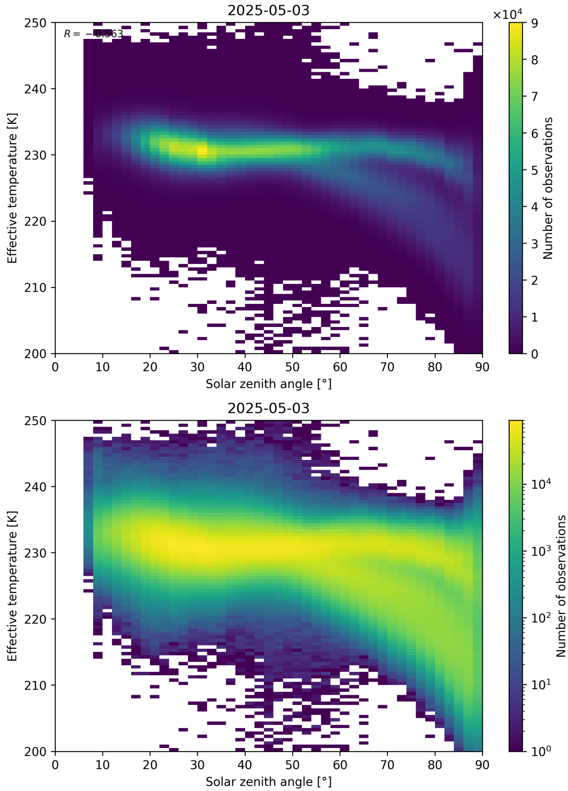
Figure 45: Scatter density plot of “Solar zenith angle” against “Effective temperature” for 2025-05-02 to 2025-05-04.
