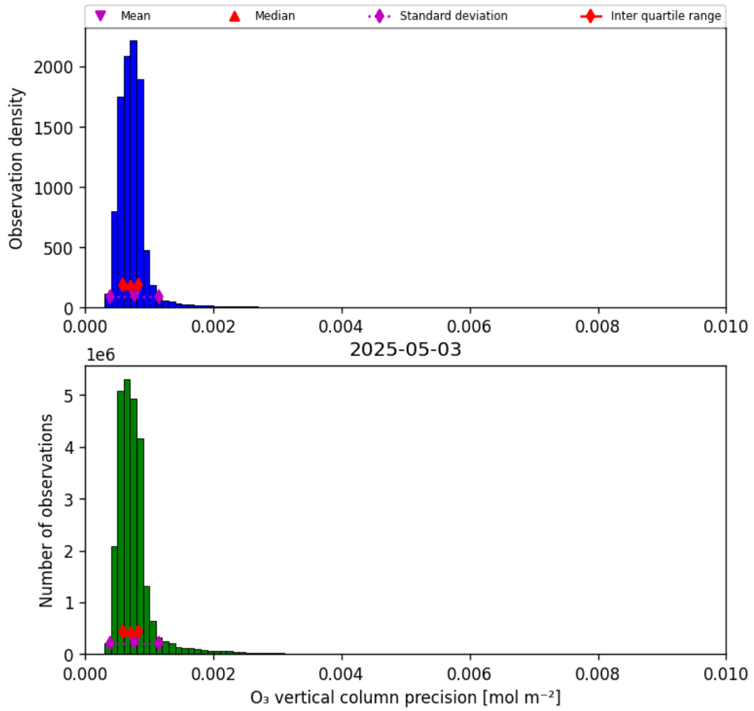
Figure 22: Histogram of “O 3 vertical column precision” for 2025-05-02 to 2025-05-04
