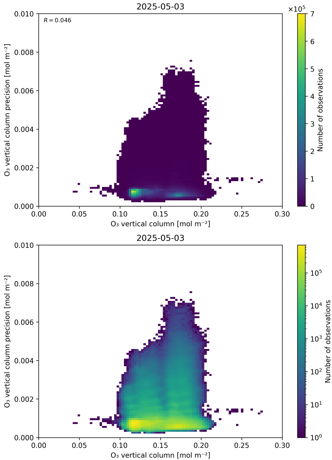
Figure 41: Scatter density plot of “O 3 vertical column” against “O 3 vertical column precision” for 2025-05-02 to 2025-05-04.
