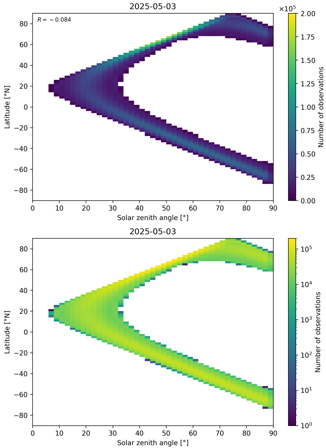
Figure 44: Scatter density plot of “Solar zenith angle” against “Latitude” for 2025-05-02 to 2025-05-04.
