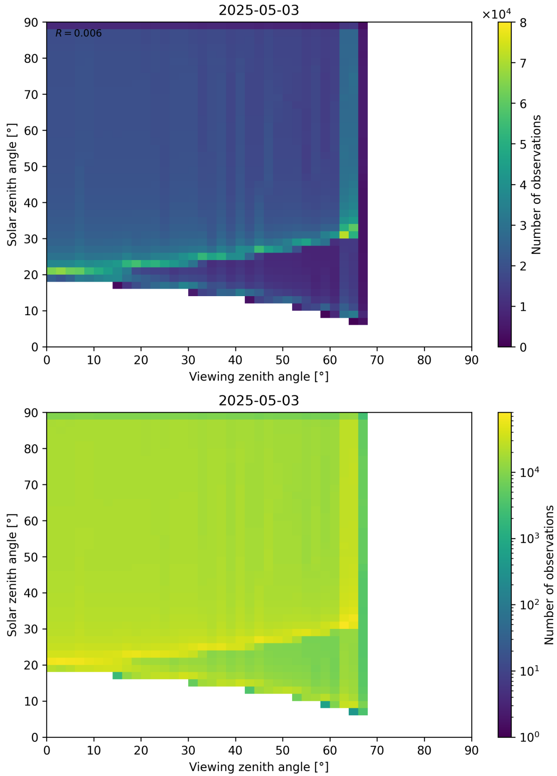
Figure 54: Scatter density plot of “Viewing zenith angle” against “Solar zenith angle” for 2025-05-02 to 2025-05-04.
