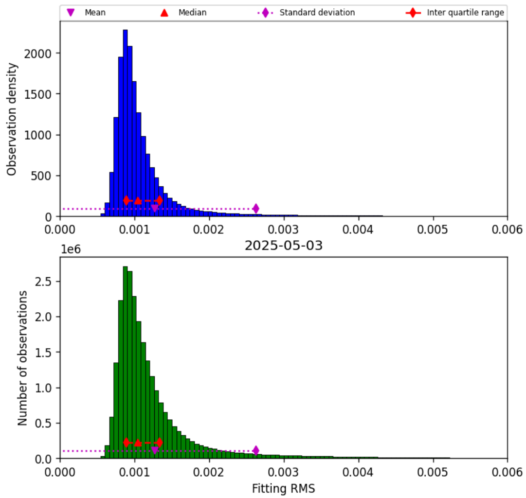
Figure 23: Histogram of “Fitting RMS” for 2025-05-02 to 2025-05-04
