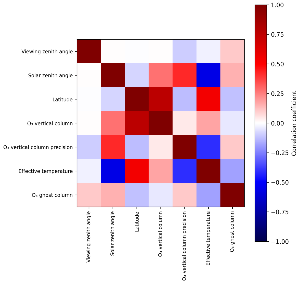
Figure 2: Map of correlation matrix for 2025-05-02 to 2025-05-04.
