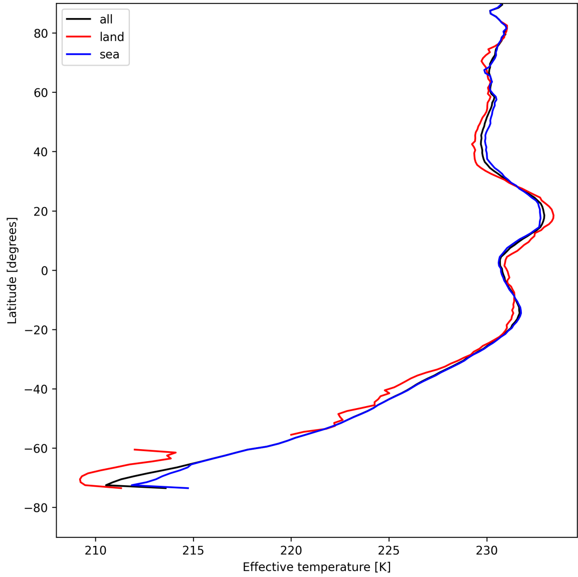
Figure 17: Zonal average of "Effective temperature" for 2025-05-02 to 2025-05-04.
