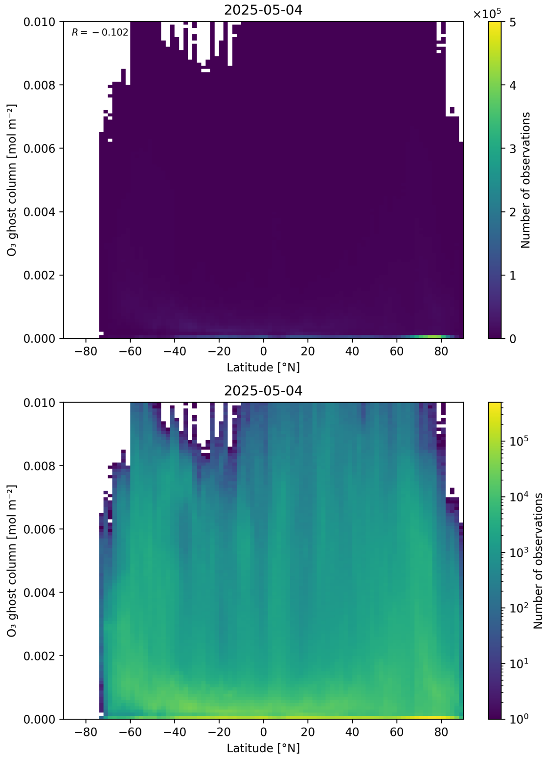
Figure 35: Scatter density plot of “Latitude” against “O 3 ghost column” for 2025-05-03 to 2025-05-05.
