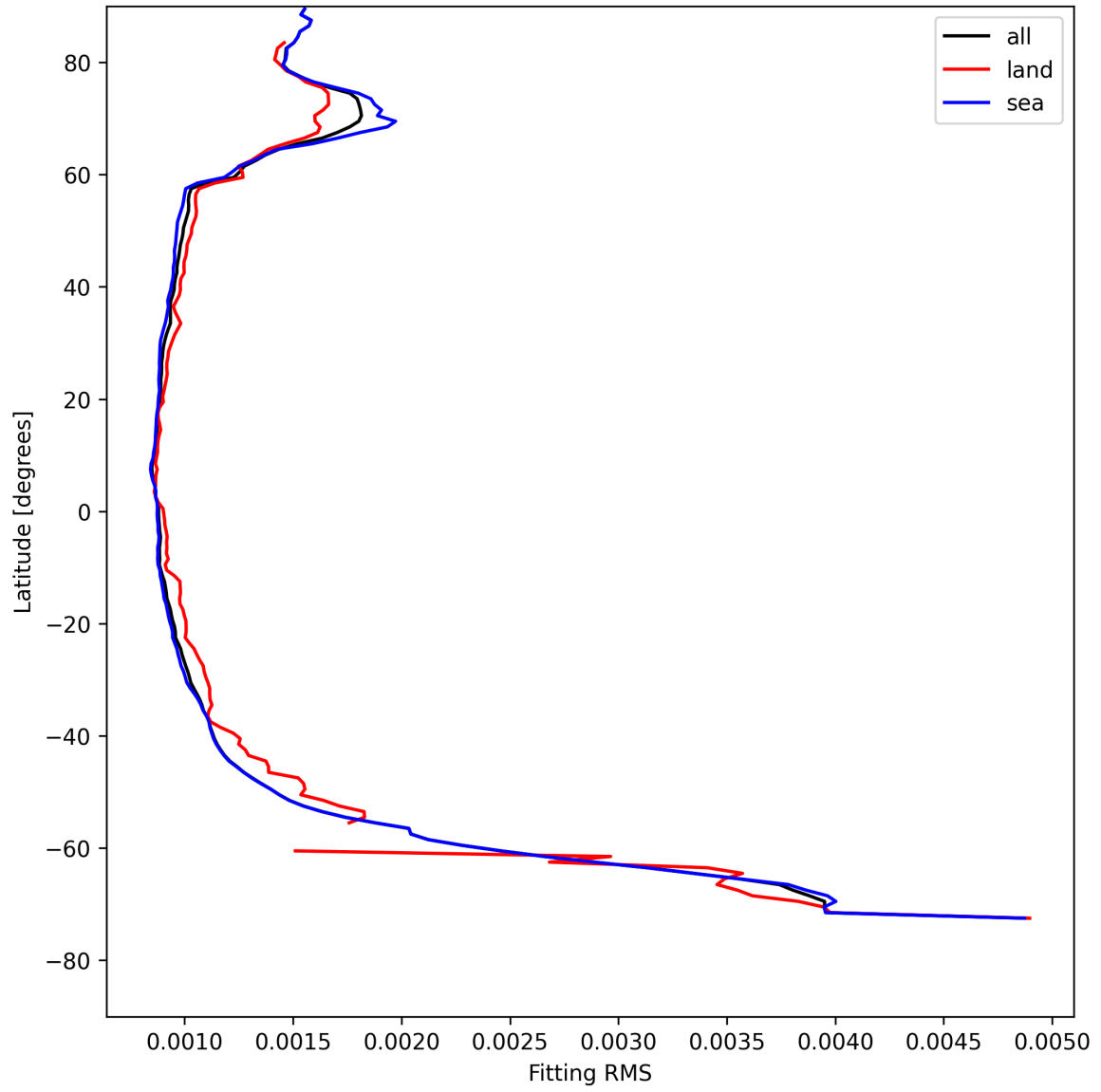
Figure 16: Zonal average of “Fitting RMS” for 2025-05-03 to 2025-05-05.
