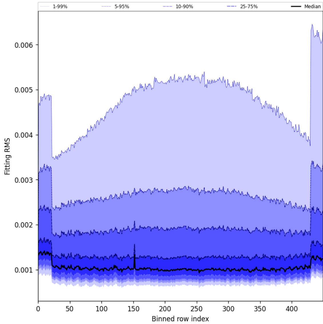
Figure 30: Along track statistics of “Fitting RMS” for 2025-05-03 to 2025-05-05
