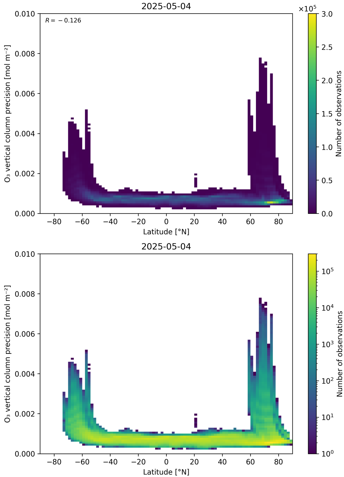
Figure 37: Scatter density plot of “Latitude” against “O 3 vertical column precision” for 2025-05-03 to 2025-05-05.
