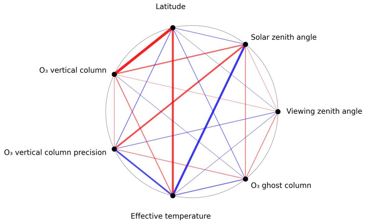
Figure 1: Map of correlation graph for 2025-05-03 to 2025-05-05.
