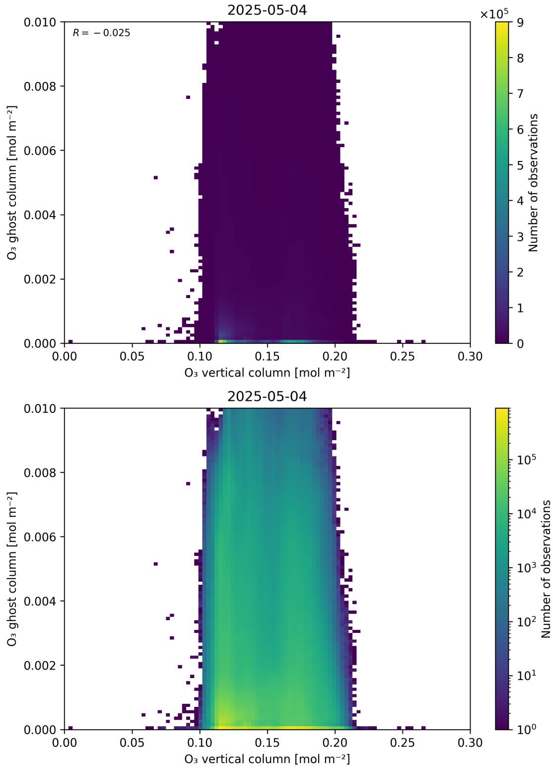
Figure 40: Scatter density plot of “O 3 vertical column” against “O 3 ghost column” for 2025-05-03 to 2025-05-05.
