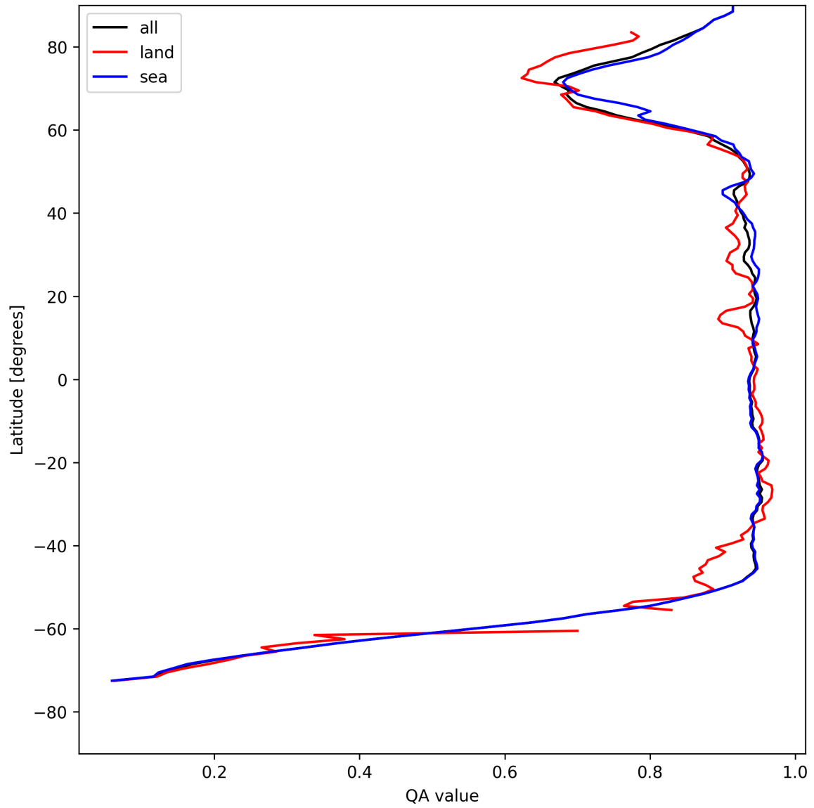
Figure 13: Zonal average of “QA value” for 2025-05-03 to 2025-05-05.
