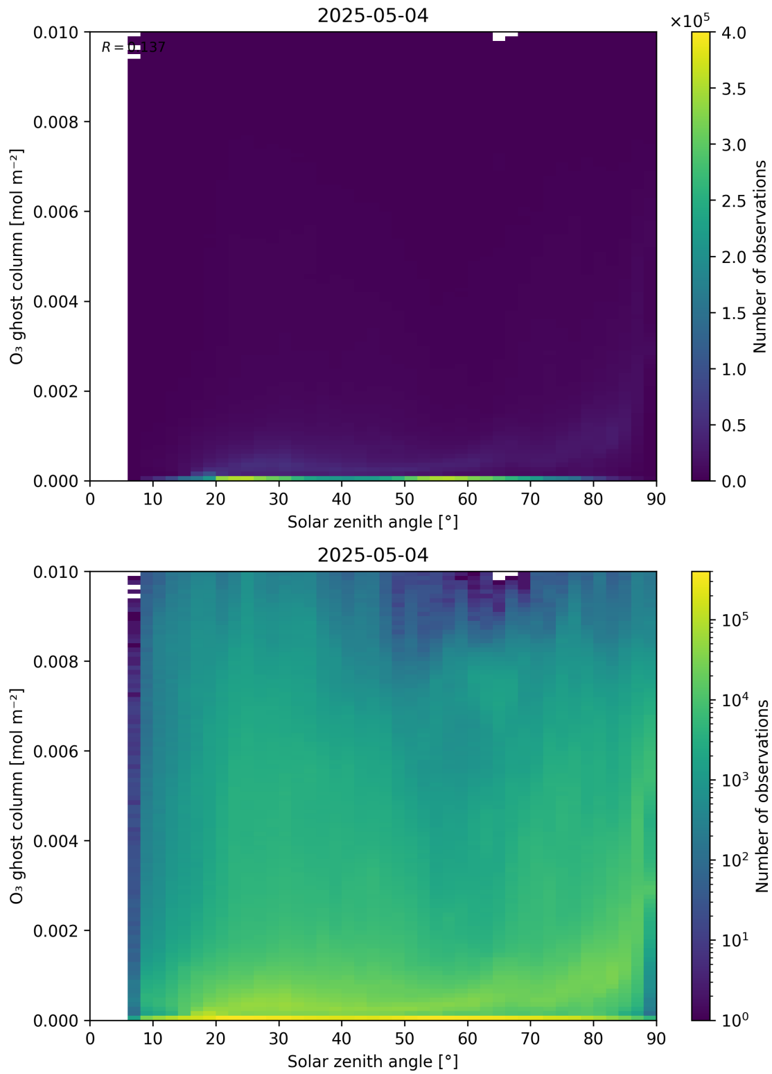
Figure 46: Scatter density plot of “Solar zenith angle” against “O 3 ghost column” for 2025-05-03 to 2025-05-05.
