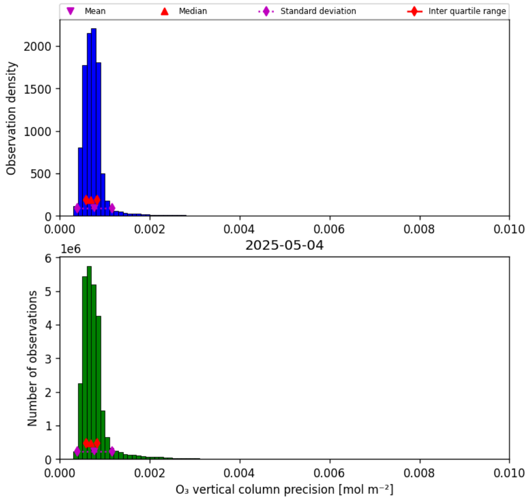
Figure 22: Histogram of “O 3 vertical column precision” for 2025-05-03 to 2025-05-05
