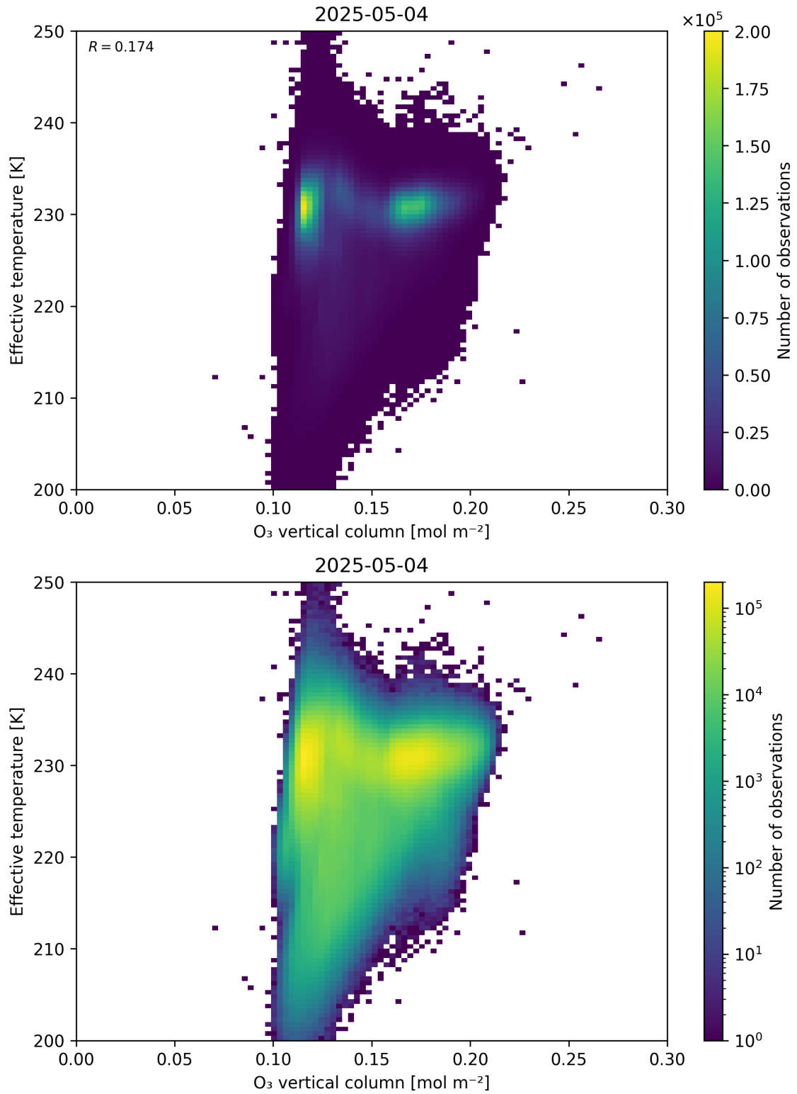
Figure 39: Scatter density plot of “O 3 vertical column” against “Effective temperature” for 2025-05-03 to 2025-05-05.
