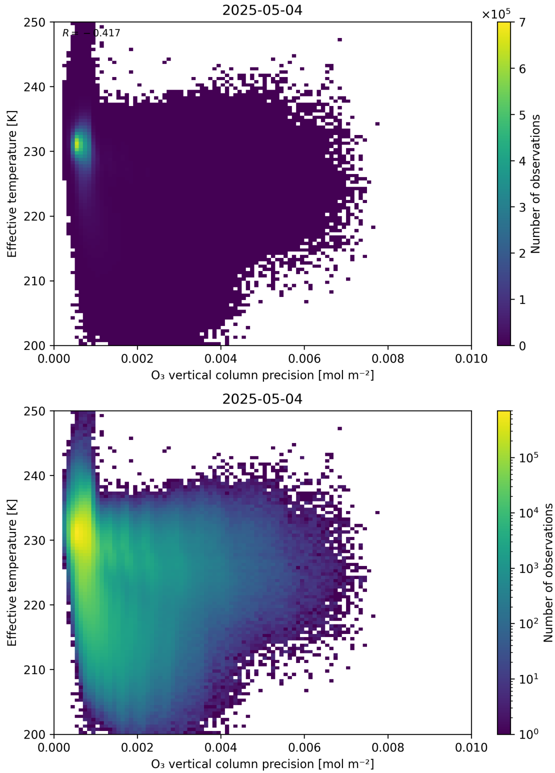
Figure 42: Scatter density plot of “O 3 vertical column precision” against “Effective temperature” for 2025-05-03 to 2025-05-05.
