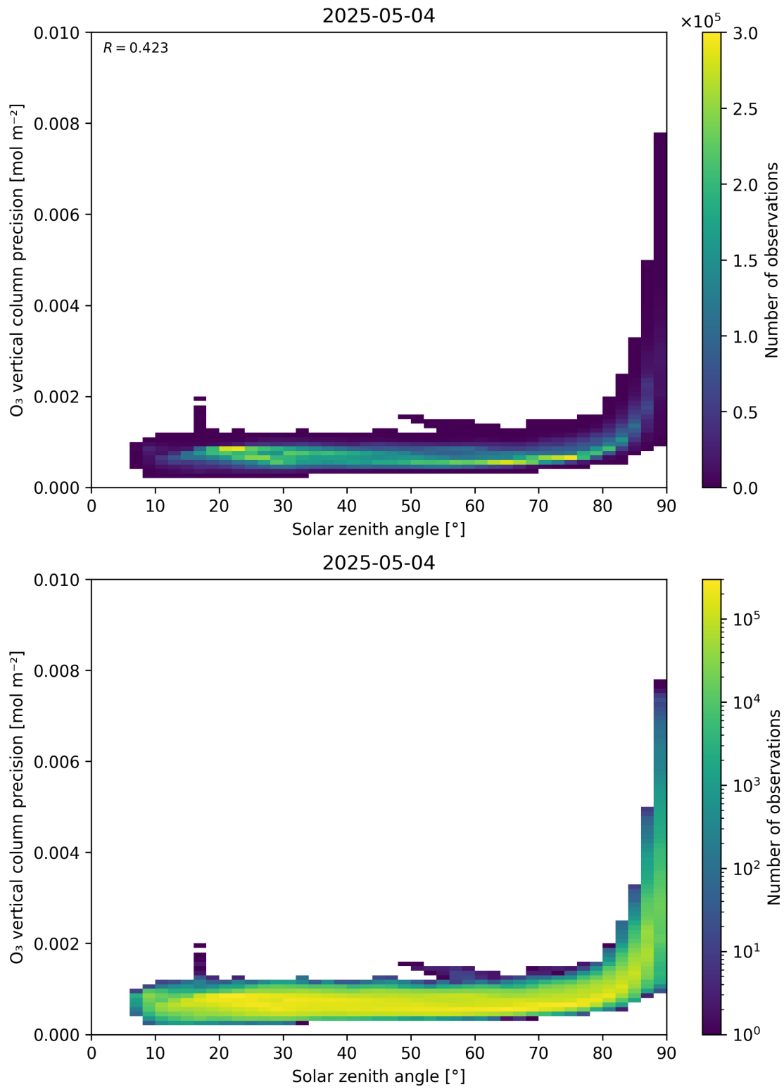
Figure 48: Scatter density plot of “Solar zenith angle” against “O 3 vertical column precision” for 2025-05-03 to 2025-05-05.
