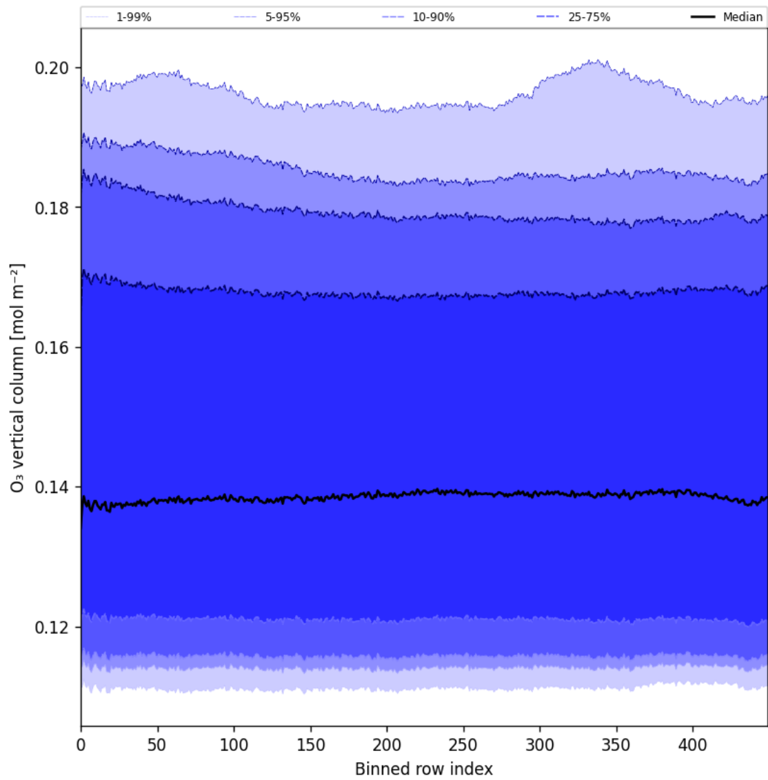
Figure 28: Along track statistics of “ \text{O}_3 vertical column” for 2025-05-03 to 2025-05-05
