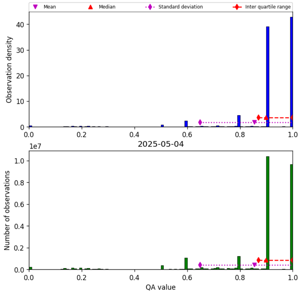
Figure 20: Histogram of “QA value” for 2025-05-03 to 2025-05-05
