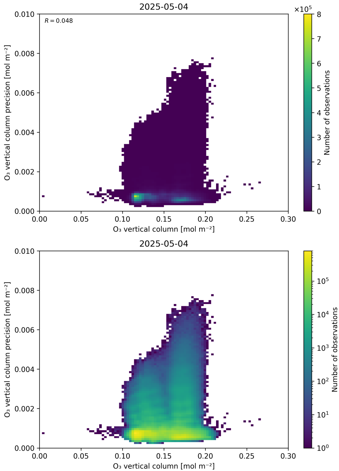
Figure 41: Scatter density plot of “O 3 vertical column” against “O 3 vertical column precision” for 2025-05-03 to 2025-05-05.
