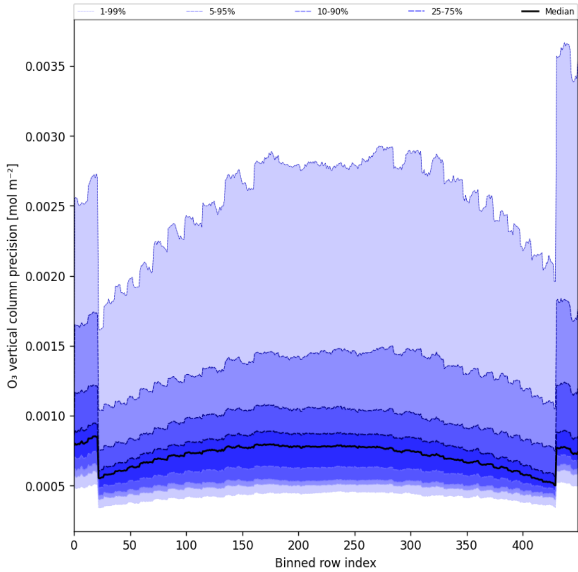
Figure 29: Along track statistics of “O 3 vertical column precision” for 2025-05-03 to 2025-05-05
