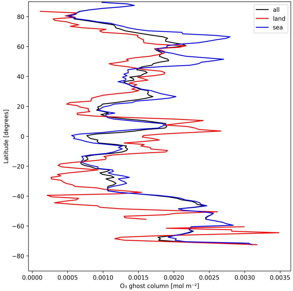
Figure 18: Zonal average of "O 3 ghost column" for 2025-05-03 to 2025-05-05.
