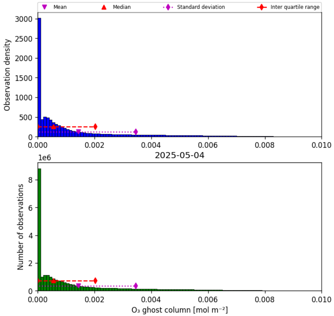
Figure 25: Histogram of “O 3 ghost column” for 2025-05-03 to 2025-05-05
