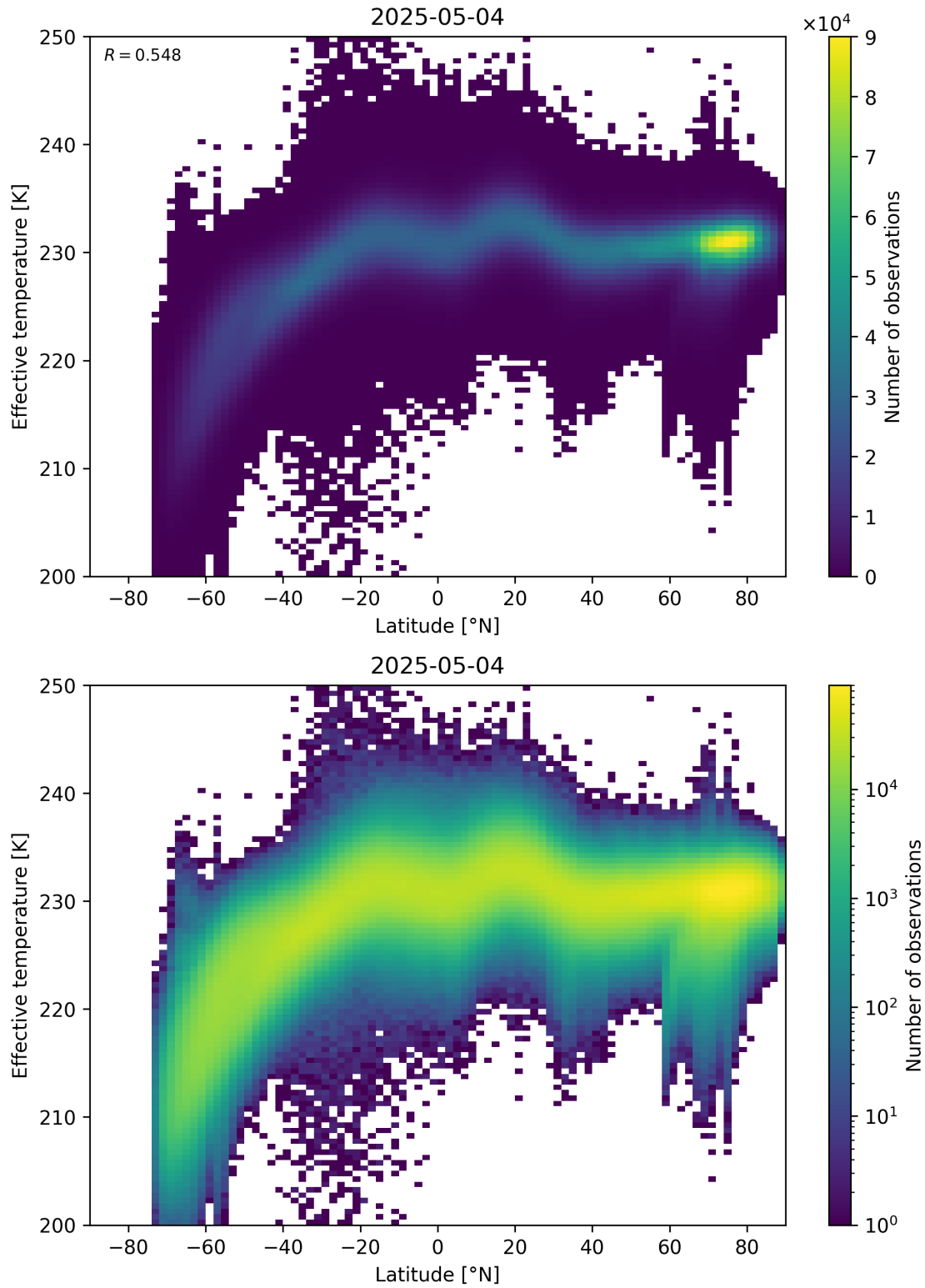
Figure 34: Scatter density plot of “Latitude” against “Effective temperature” for 2025-05-03 to 2025-05-05.
