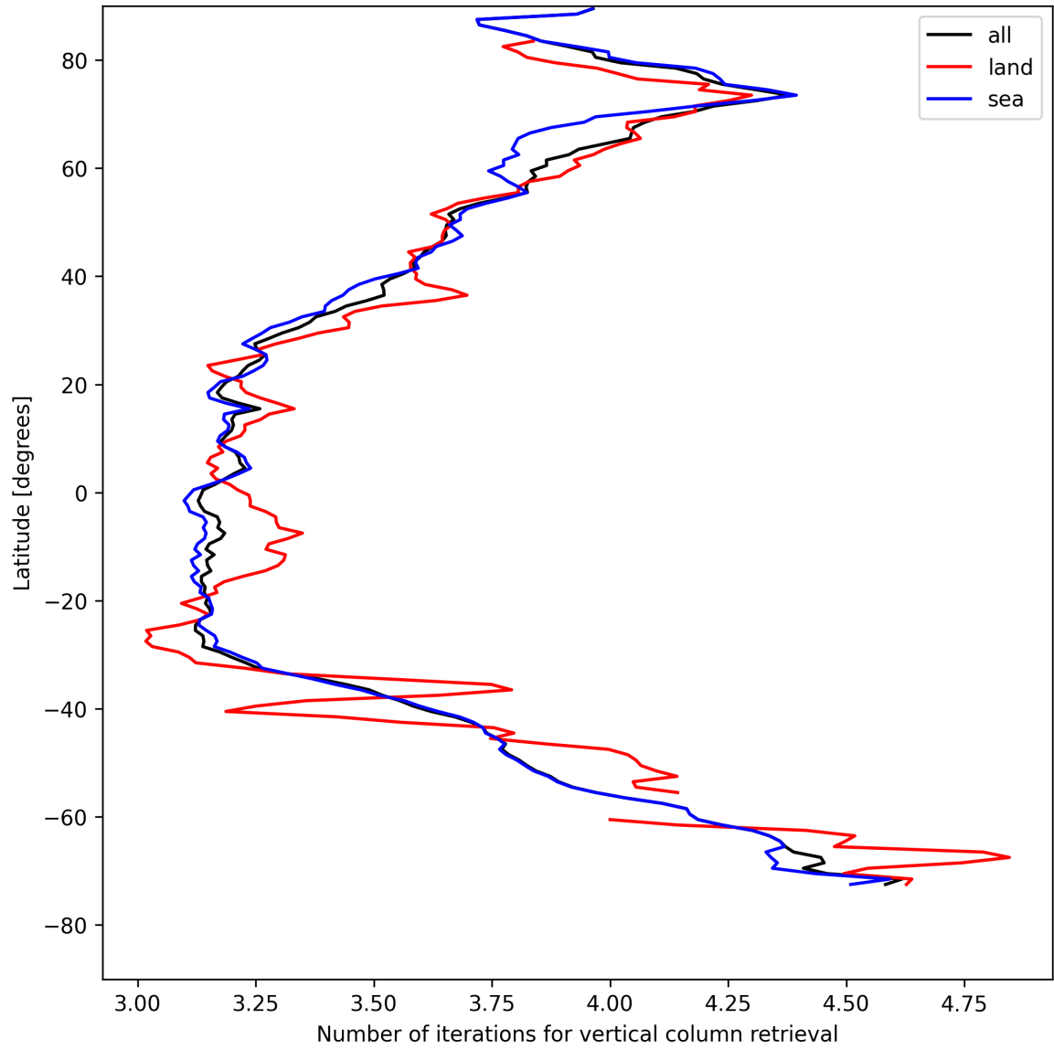
Figure 19: Zonal average of “Number of iterations for vertical column retrieval” for 2025-05-03 to 2025-05-05.
