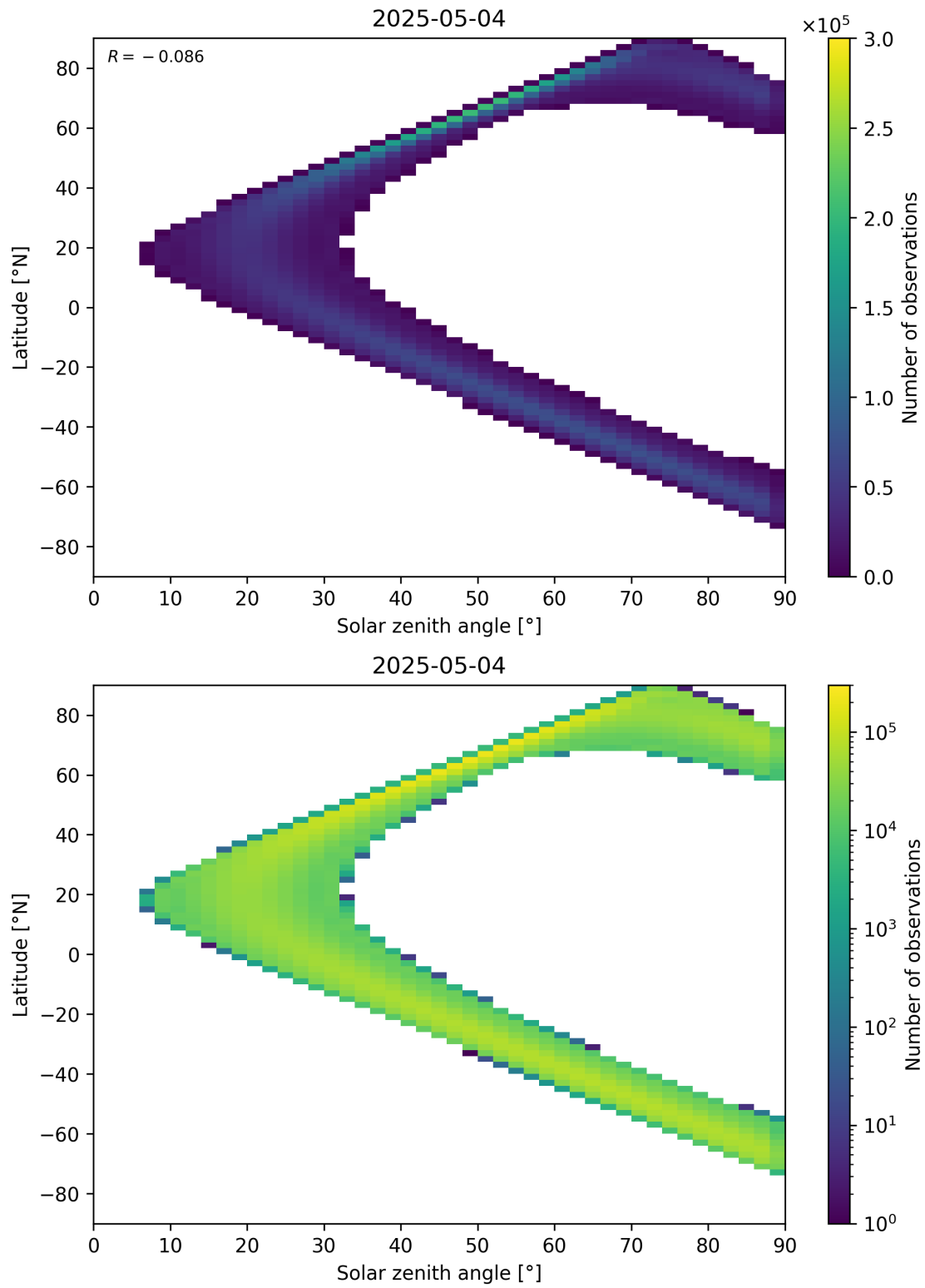
Figure 44: Scatter density plot of “Solar zenith angle” against “Latitude” for 2025-05-03 to 2025-05-05.
