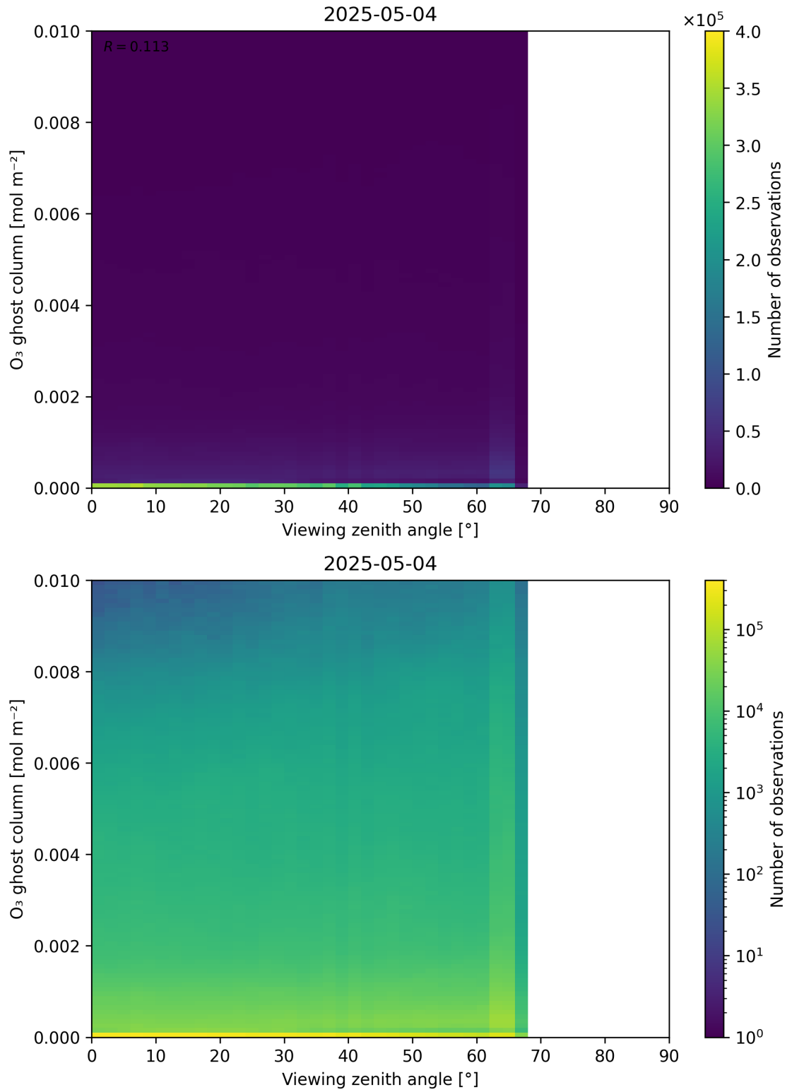
Figure 51: Scatter density plot of “Viewing zenith angle” against “O 3 ghost column” for 2025-05-03 to 2025-05-05.
