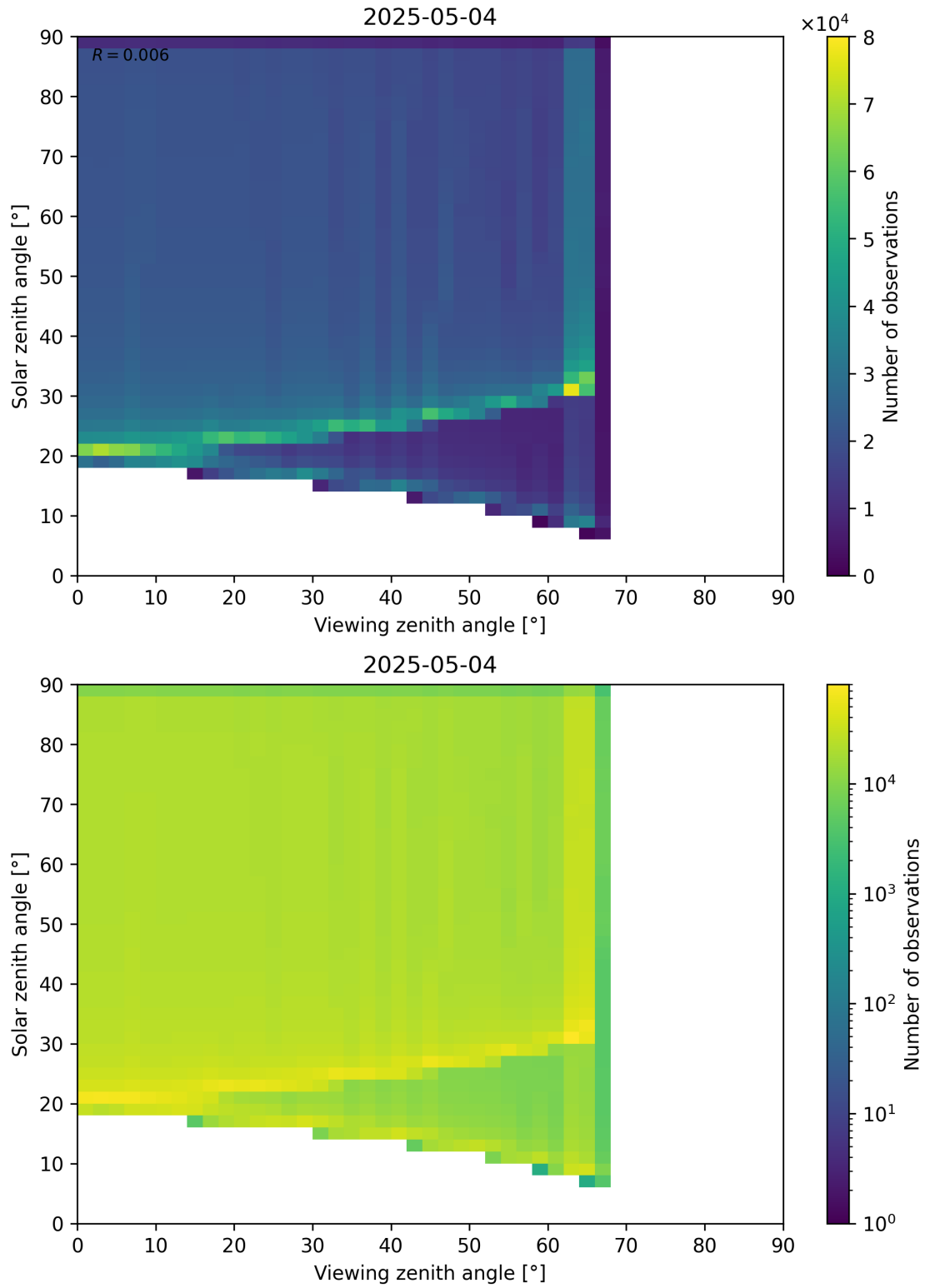
Figure 54: Scatter density plot of “Viewing zenith angle” against “Solar zenith angle” for 2025-05-03 to 2025-05-05.
