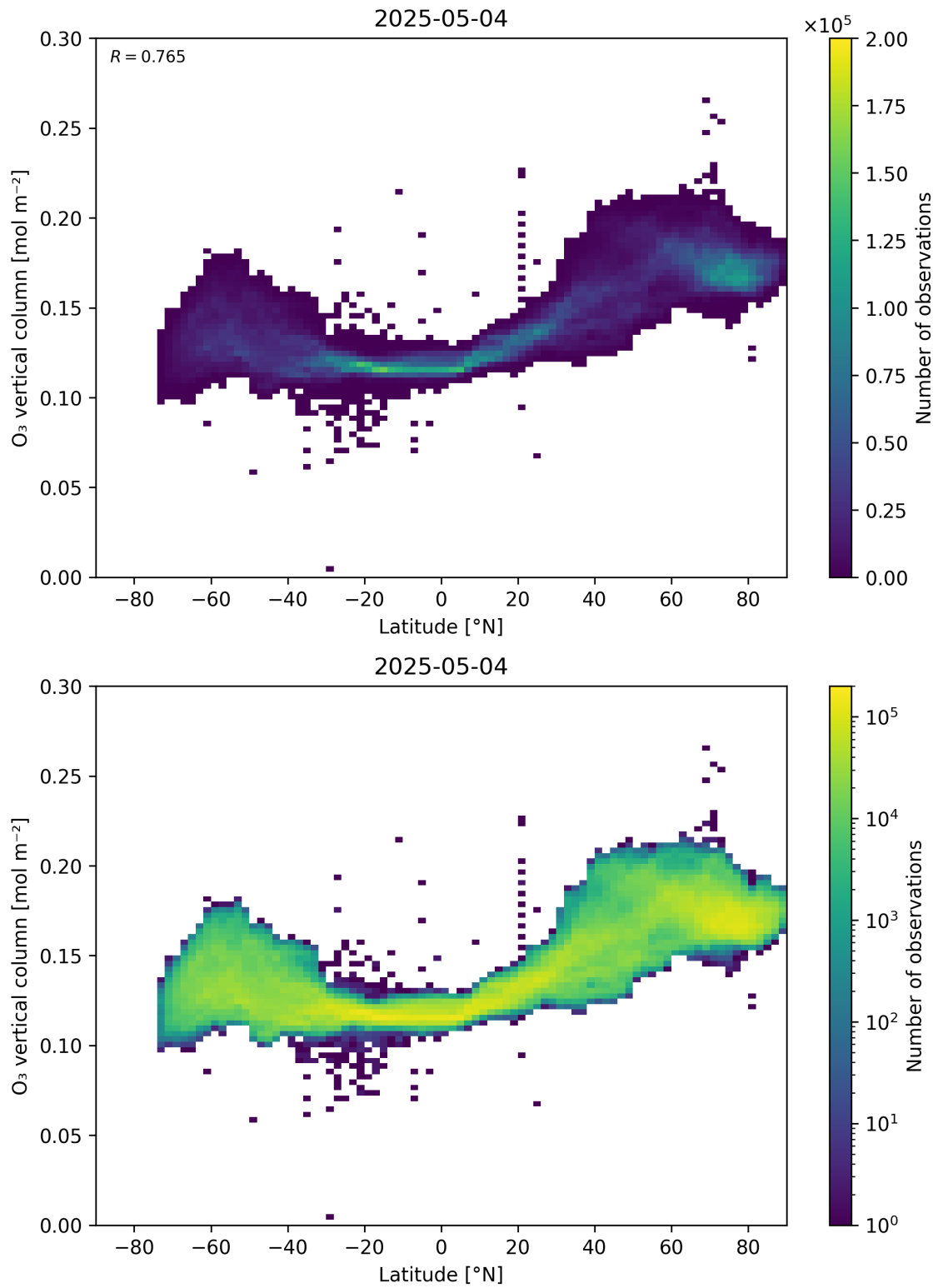
Figure 36: Scatter density plot of “Latitude” against “O 3 vertical column” for 2025-05-03 to 2025-05-05.
