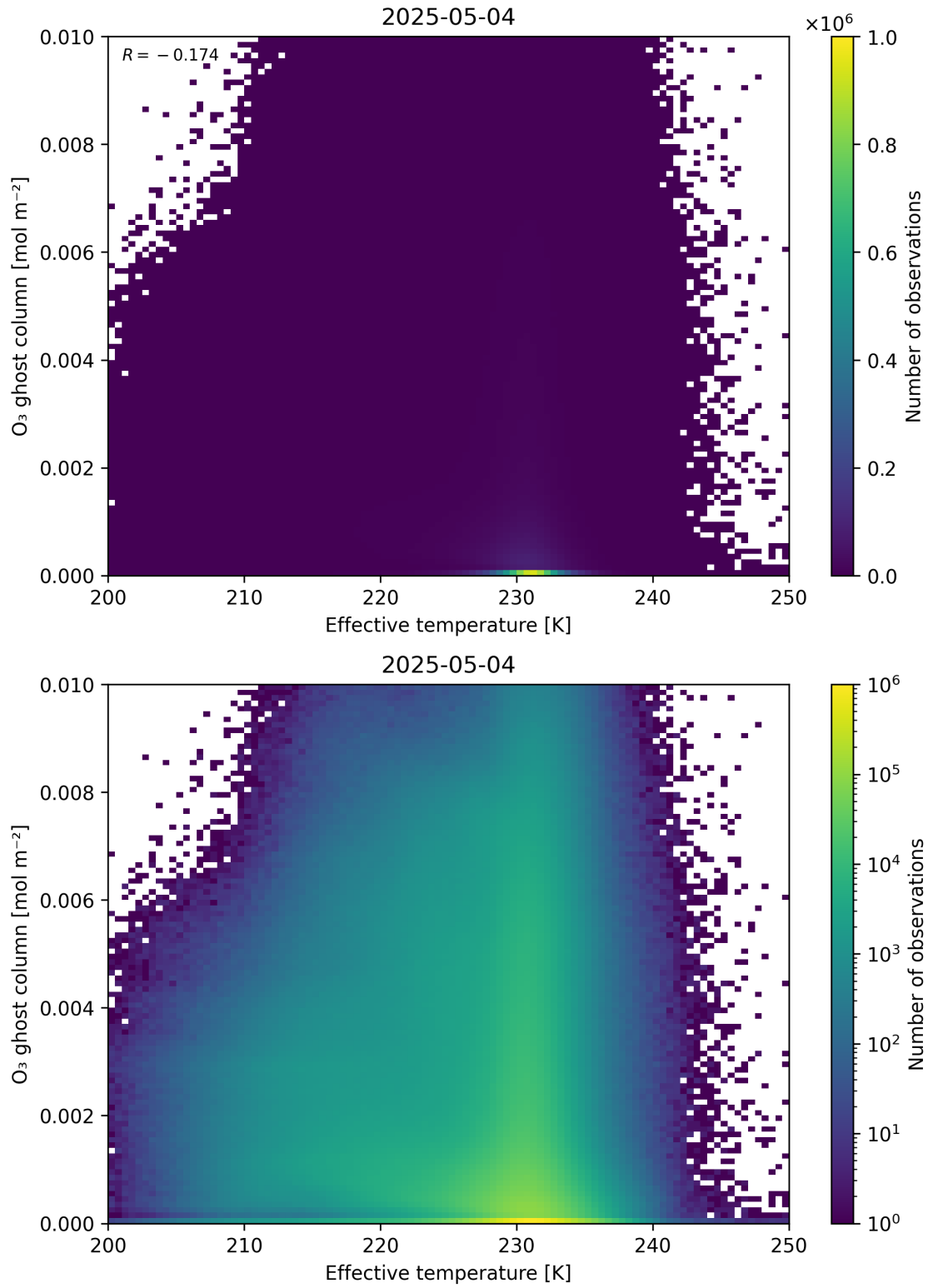
Figure 38: Scatter density plot of “Effective temperature” against “O 3 ghost column” for 2025-05-03 to 2025-05-05.
