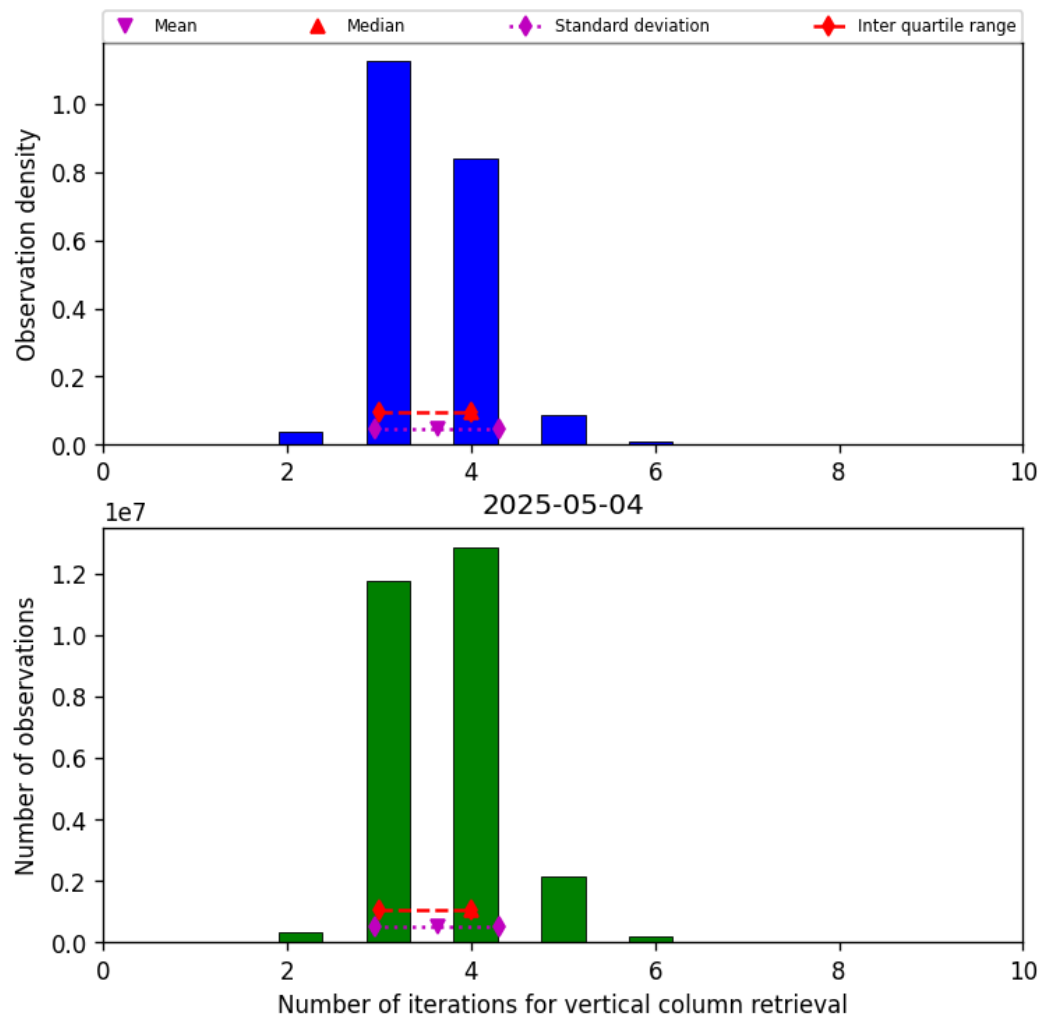
Figure 26: Histogram of “Number of iterations for vertical column retrieval” for 2025-05-03 to 2025-05-05
