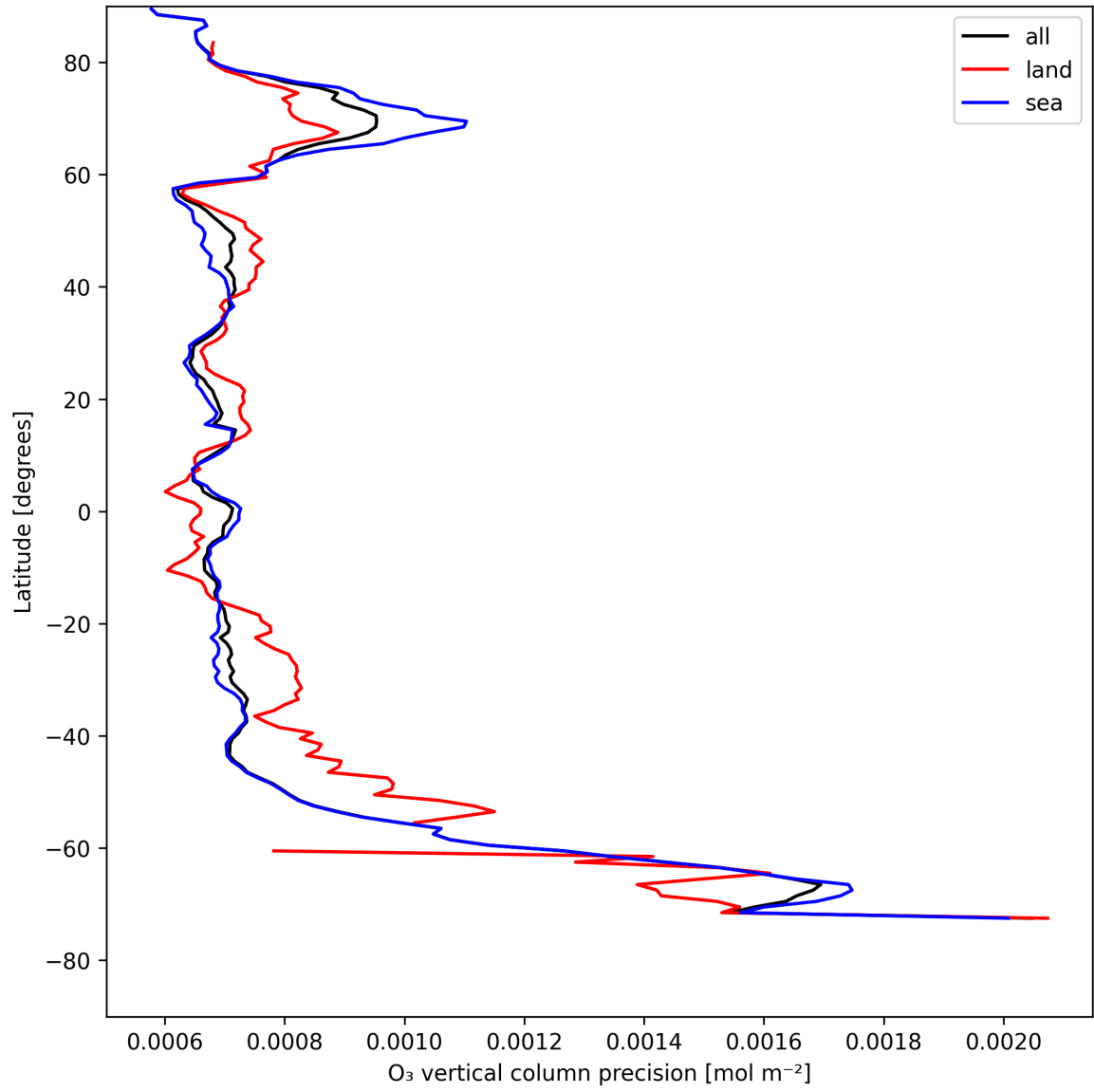
Figure 15: Zonal average of “O 3 vertical column precision” for 2025-05-03 to 2025-05-05.
