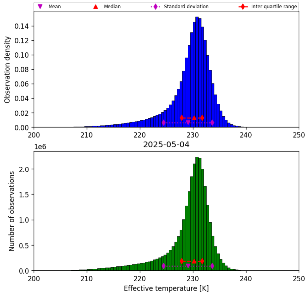
Figure 24: Histogram of “Effective temperature” for 2025-05-03 to 2025-05-05
