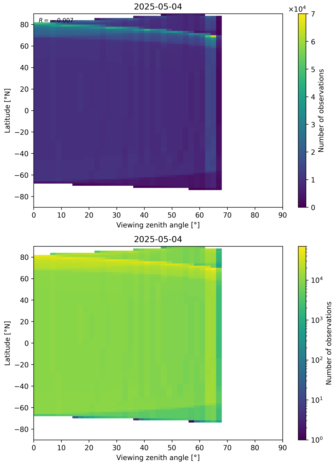
Figure 49: Scatter density plot of “Viewing zenith angle” against “Latitude” for 2025-05-03 to 2025-05-05.
