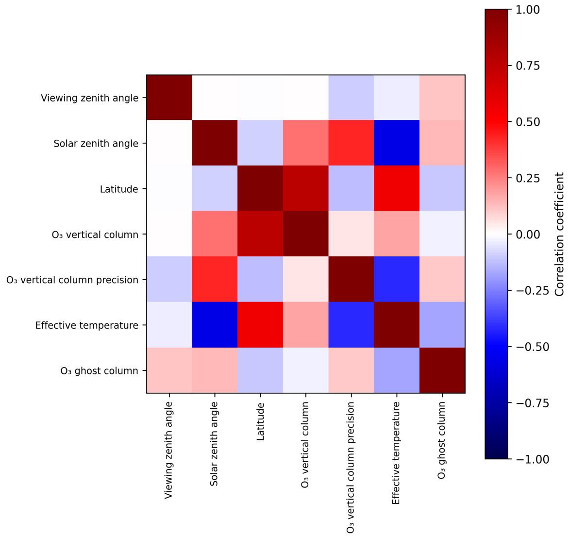
Figure 2: Map of correlation matrix for 2025-05-03 to 2025-05-05.
