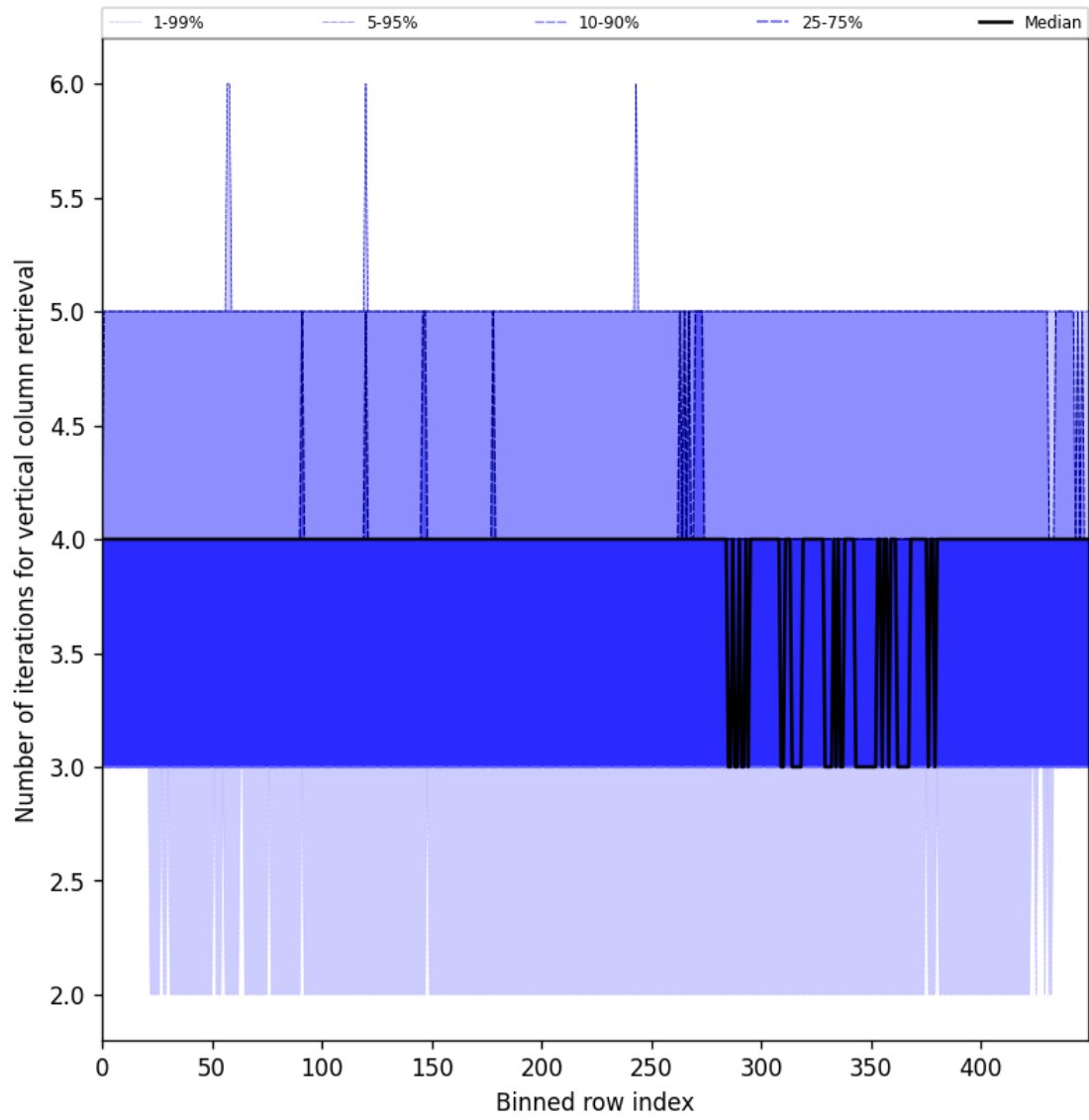
Figure 33: Along track statistics of “Number of iterations for vertical column retrieval” for 2025-05-03 to 2025-05-05
