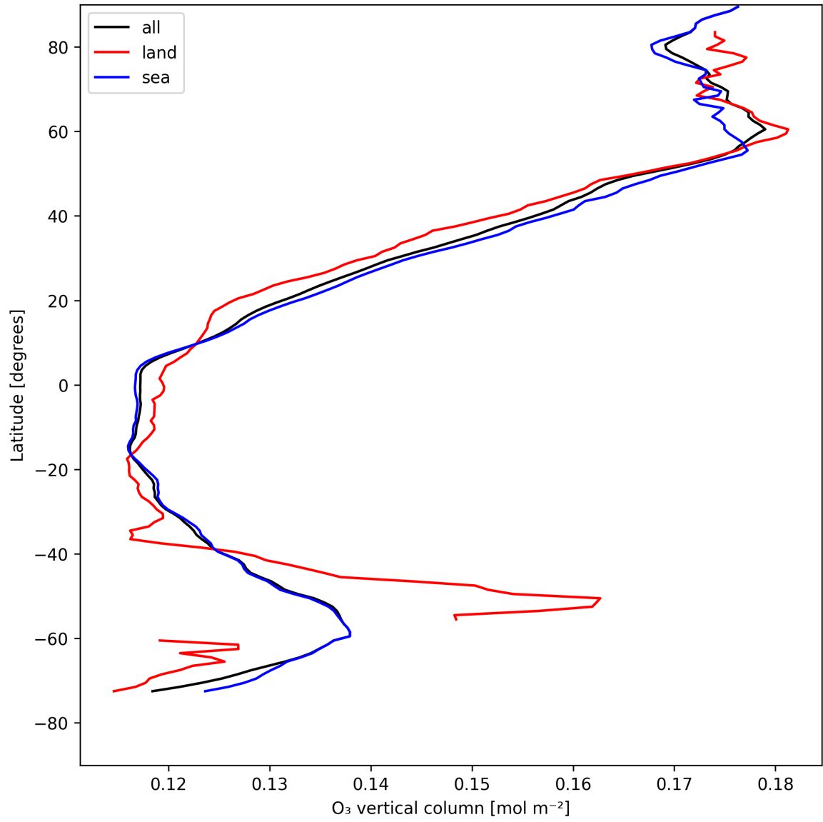
Figure 14: Zonal average of “O 3 vertical column” for 2025-05-03 to 2025-05-05.
