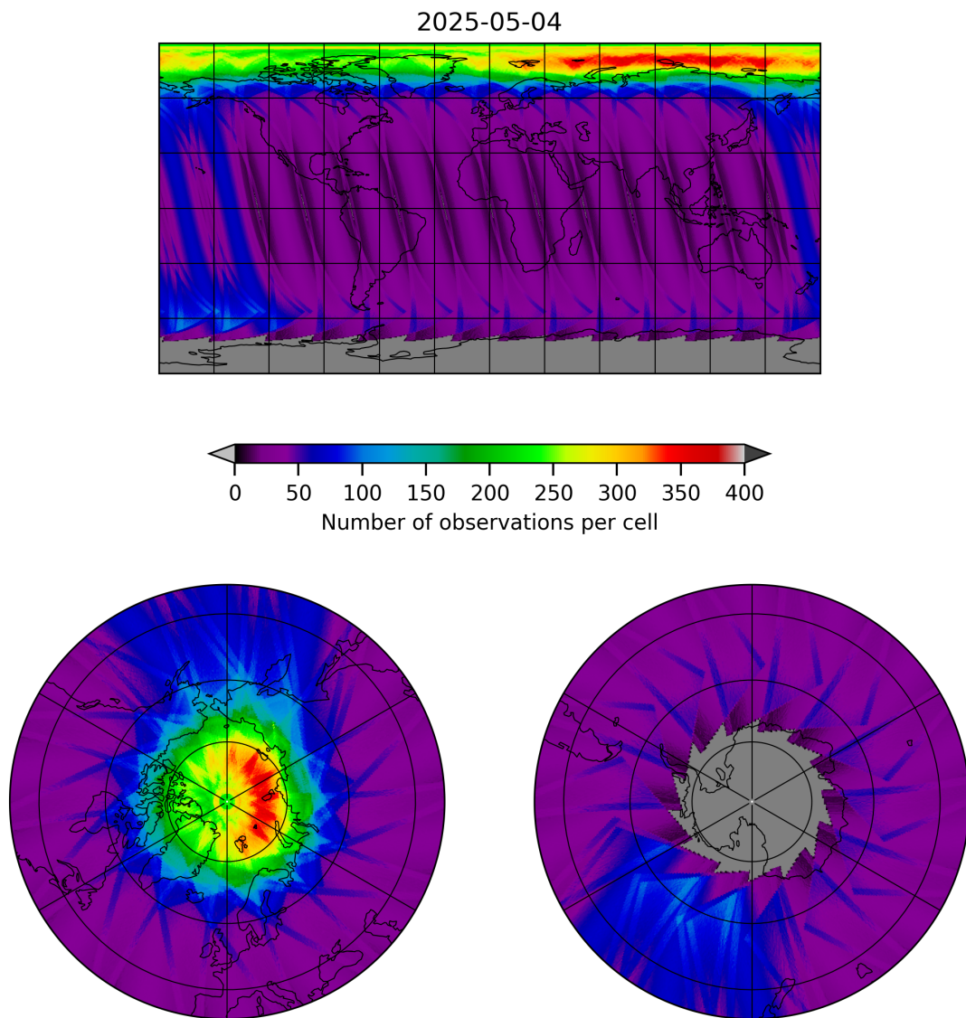
Figure 12: Map of the number of observations for 2025-05-03 to 2025-05-05
