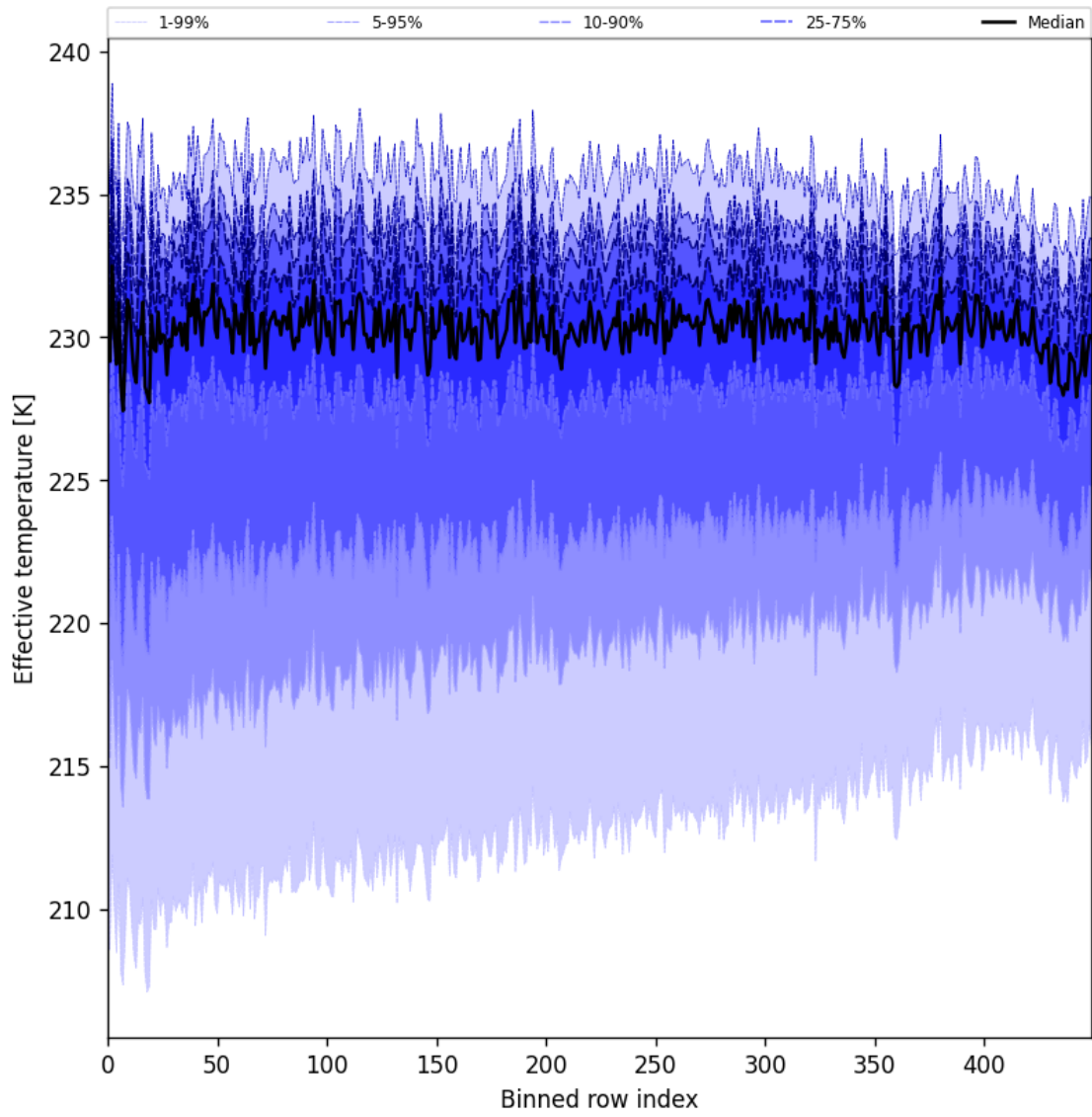
Figure 31: Along track statistics of “Effective temperature” for 2025-05-03 to 2025-05-05
