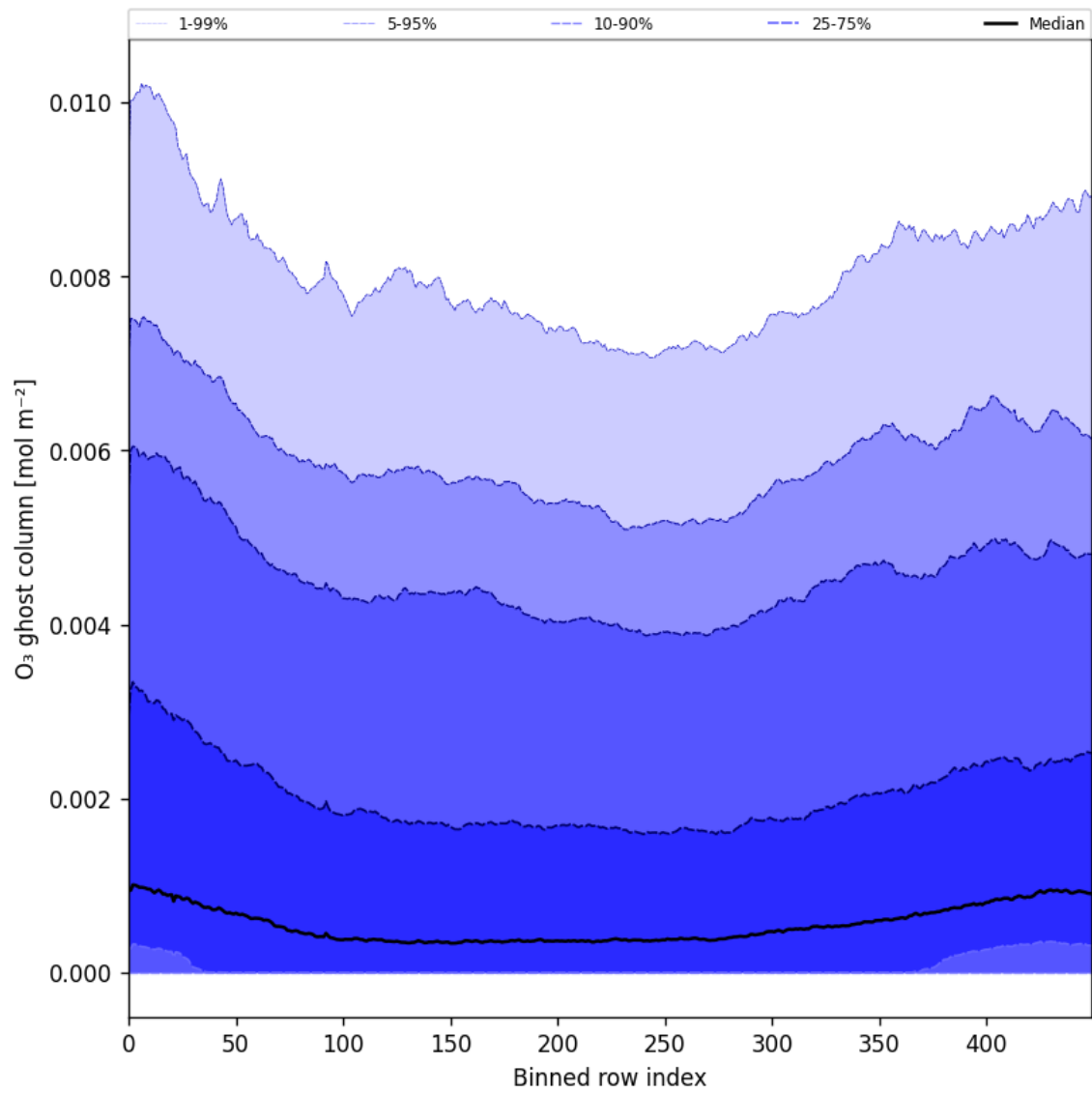
Figure 32: Along track statistics of “O 3 ghost column” for 2025-05-03 to 2025-05-05
