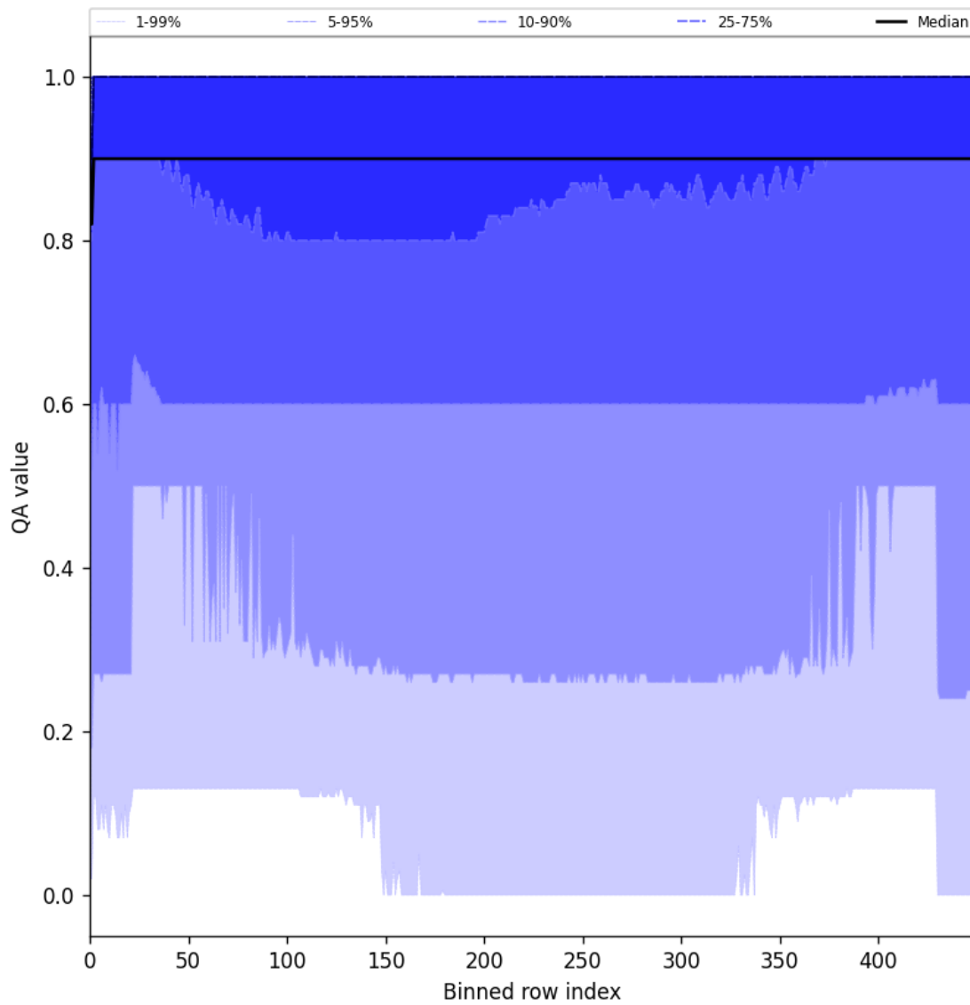
Figure 27: Along track statistics of “QA value” for 2025-05-03 to 2025-05-05
