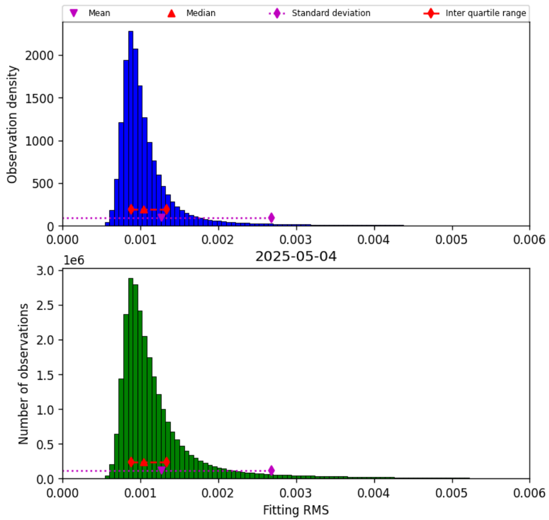
Figure 23: Histogram of “Fitting RMS” for 2025-05-03 to 2025-05-05
