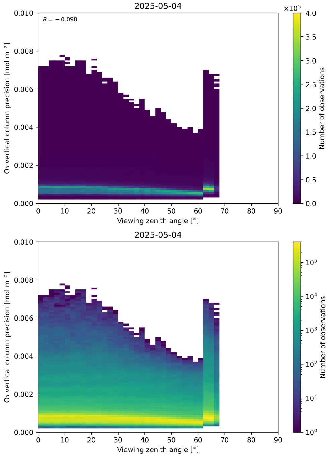
Figure 53: Scatter density plot of “Viewing zenith angle” against “O 3 vertical column precision” for 2025-05-03 to 2025-05-05.
