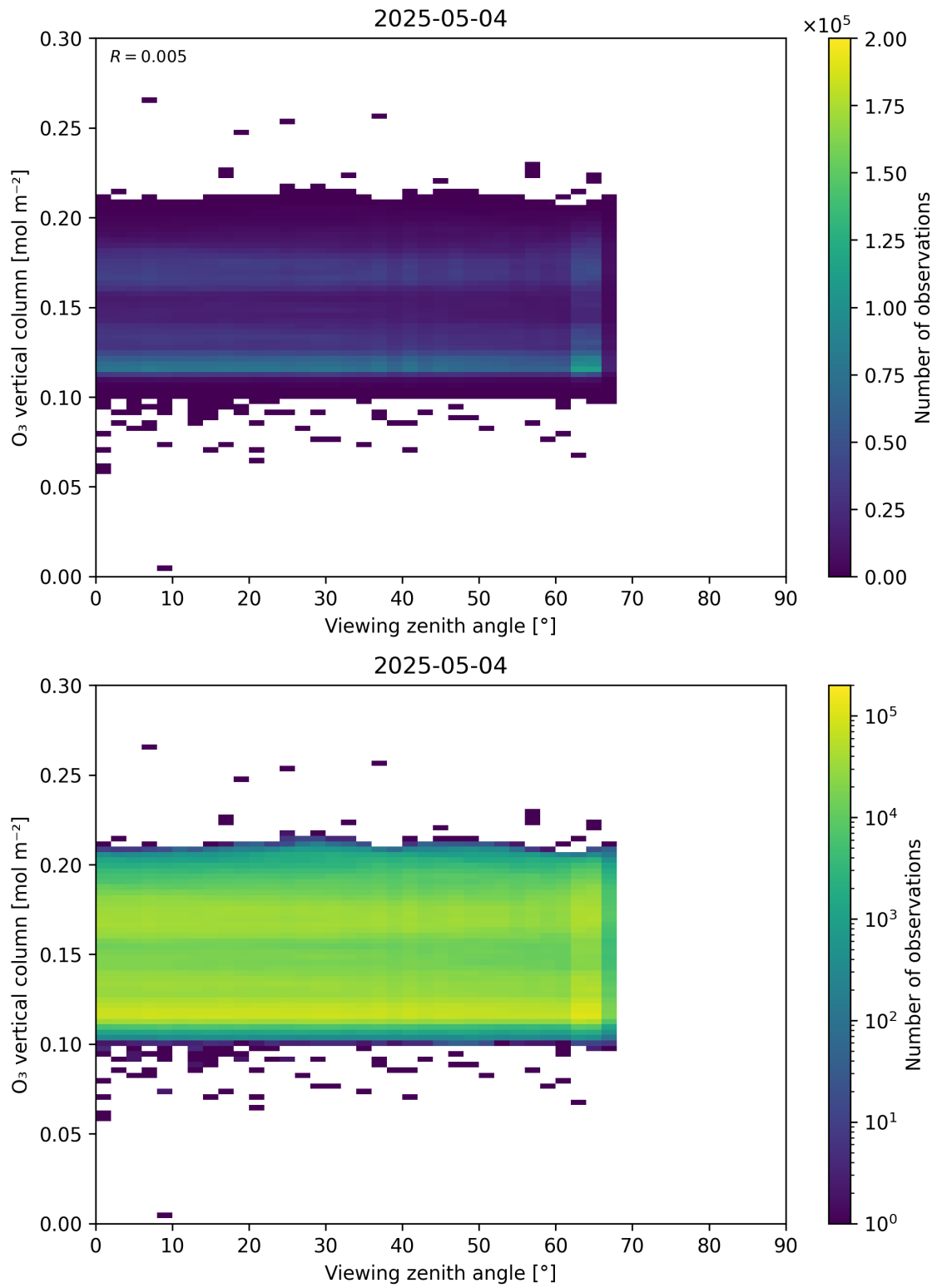
Figure 52: Scatter density plot of “Viewing zenith angle” against “O 3 vertical column” for 2025-05-03 to 2025-05-05.
