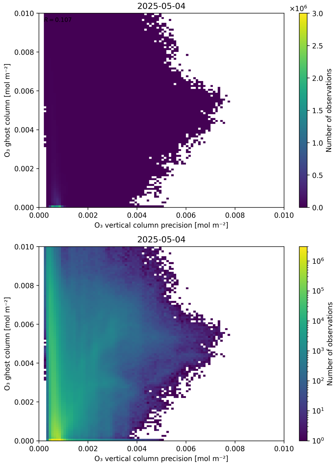
Figure 43: Scatter density plot of “ \text{O}_3 vertical column precision” against “ \text{O}_3 ghost column” for 2025-05-03 to 2025-05-05.
