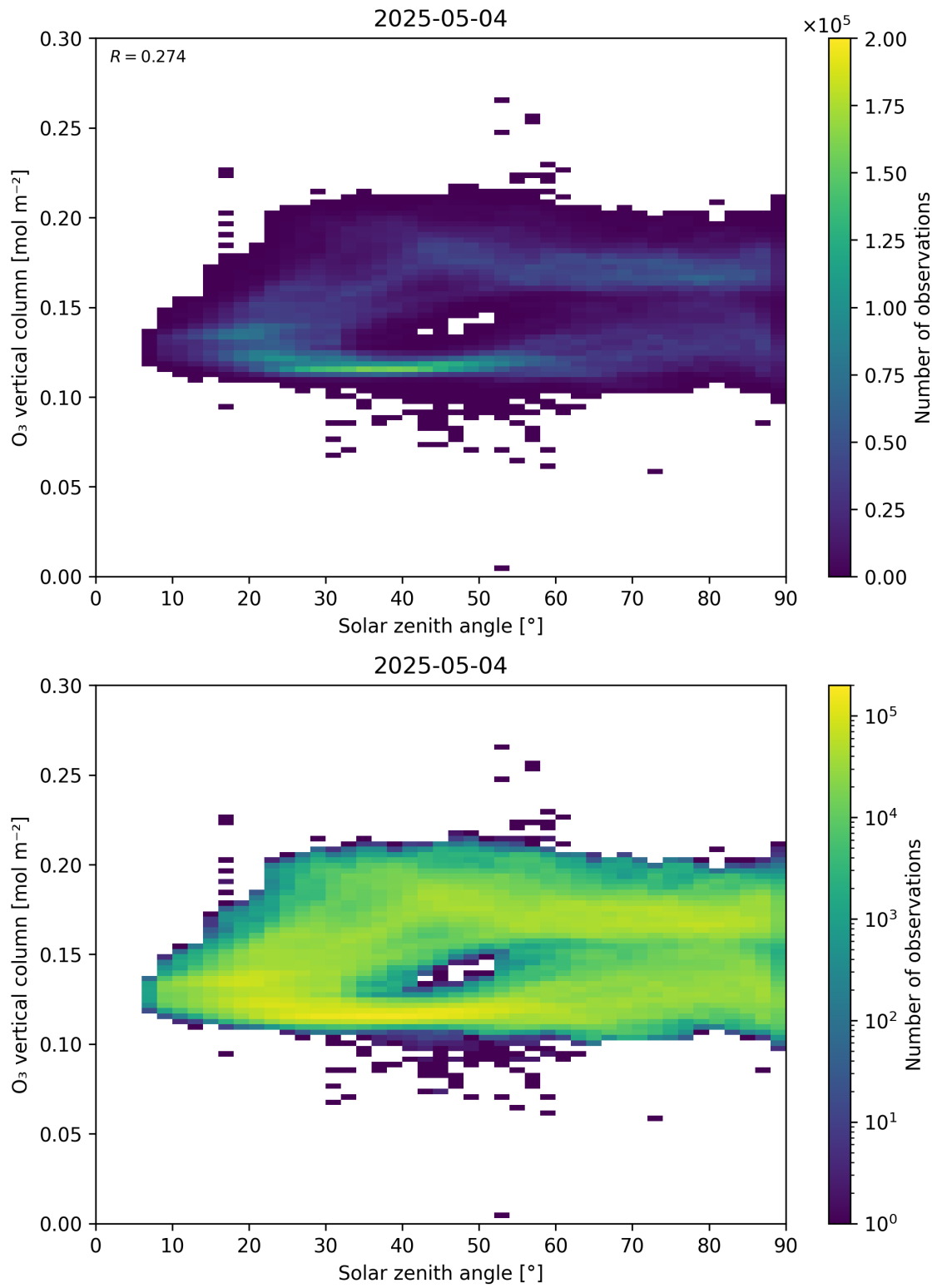
Figure 47: Scatter density plot of “Solar zenith angle” against “O 3 vertical column” for 2025-05-03 to 2025-05-05.
