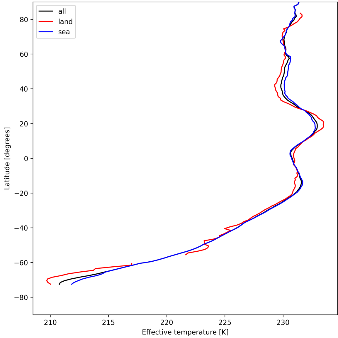
Figure 17: Zonal average of "Effective temperature" for 2025-05-03 to 2025-05-05.
