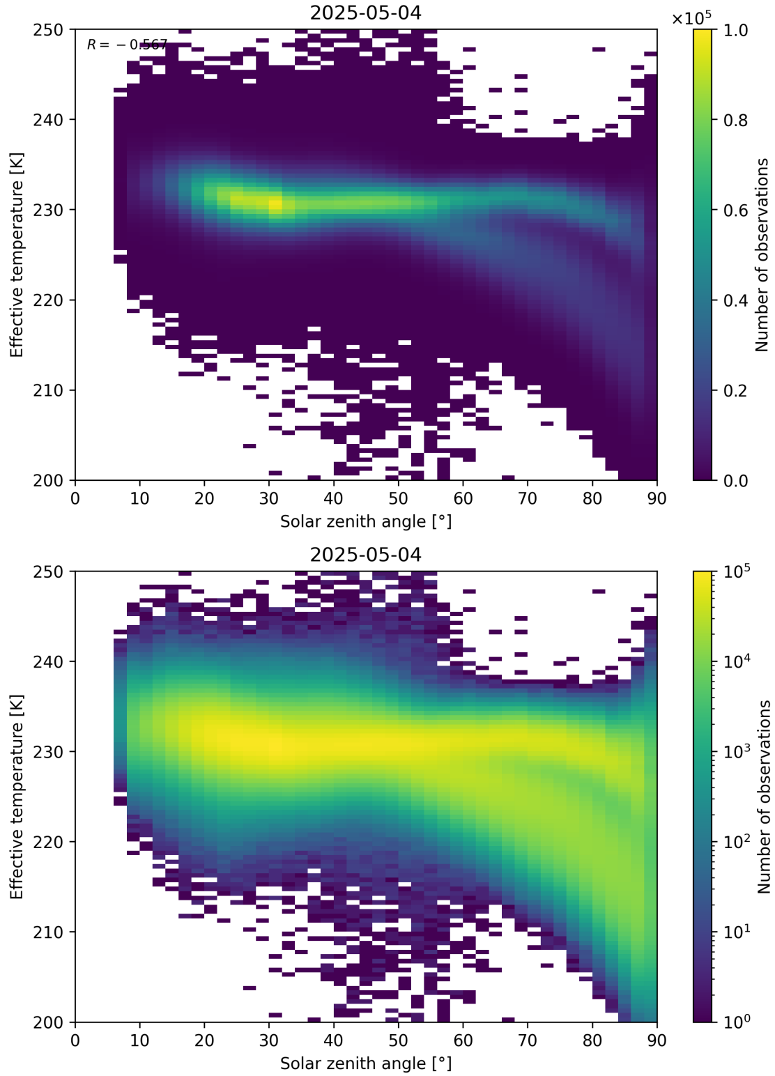
Figure 45: Scatter density plot of “Solar zenith angle” against “Effective temperature” for 2025-05-03 to 2025-05-05.
