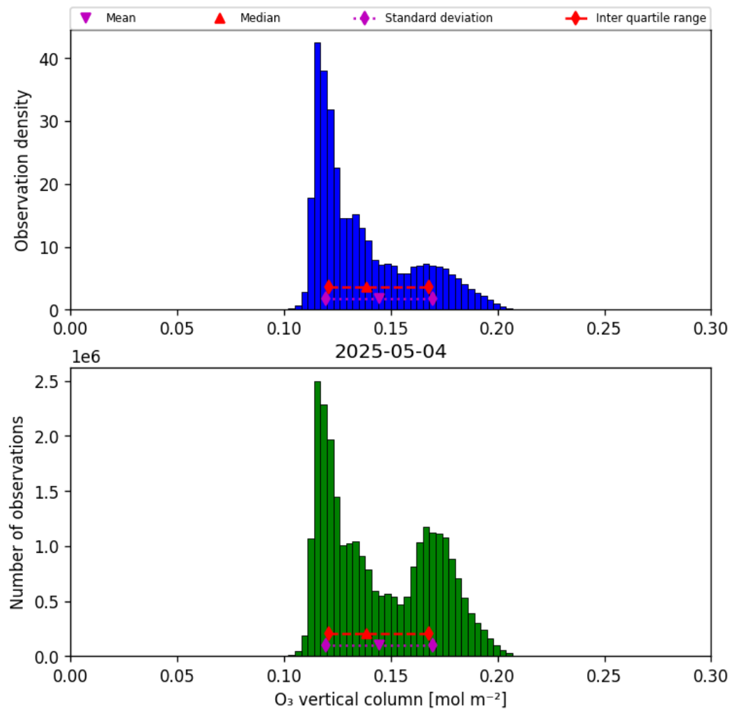
Figure 21: Histogram of “O 3 vertical column” for 2025-05-03 to 2025-05-05
