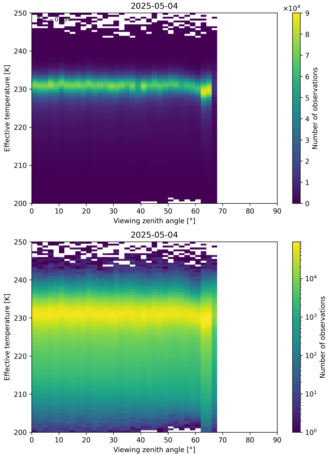
Figure 50: Scatter density plot of “Viewing zenith angle” against “Effective temperature” for 2025-05-03 to 2025-05-05.
