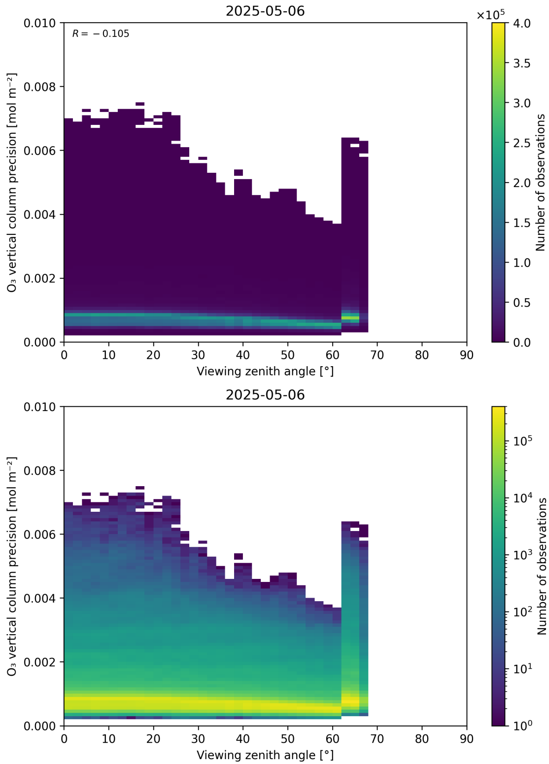
Figure 53: Scatter density plot of “Viewing zenith angle” against “O 3 vertical column precision” for 2025-05-05 to 2025-05-07.
