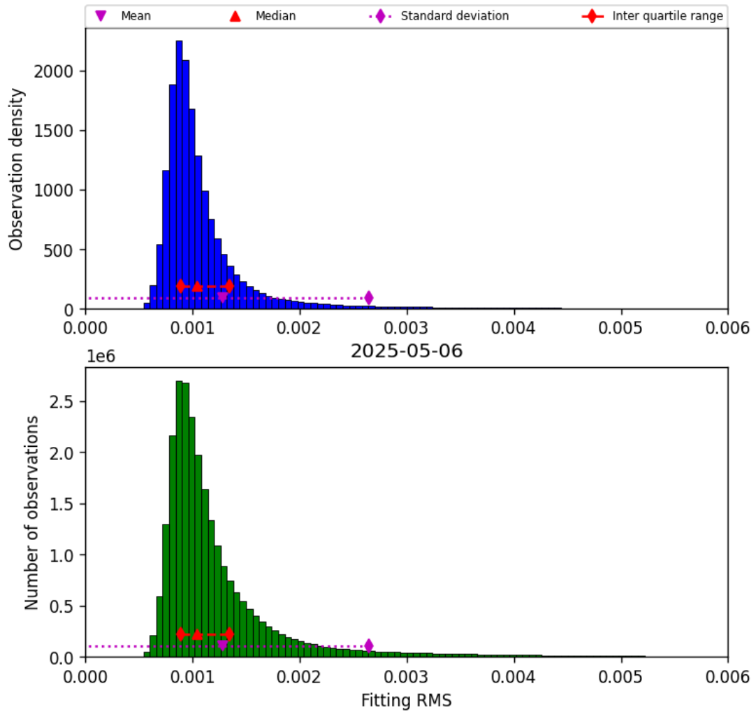
Figure 23: Histogram of “Fitting RMS” for 2025-05-05 to 2025-05-07
