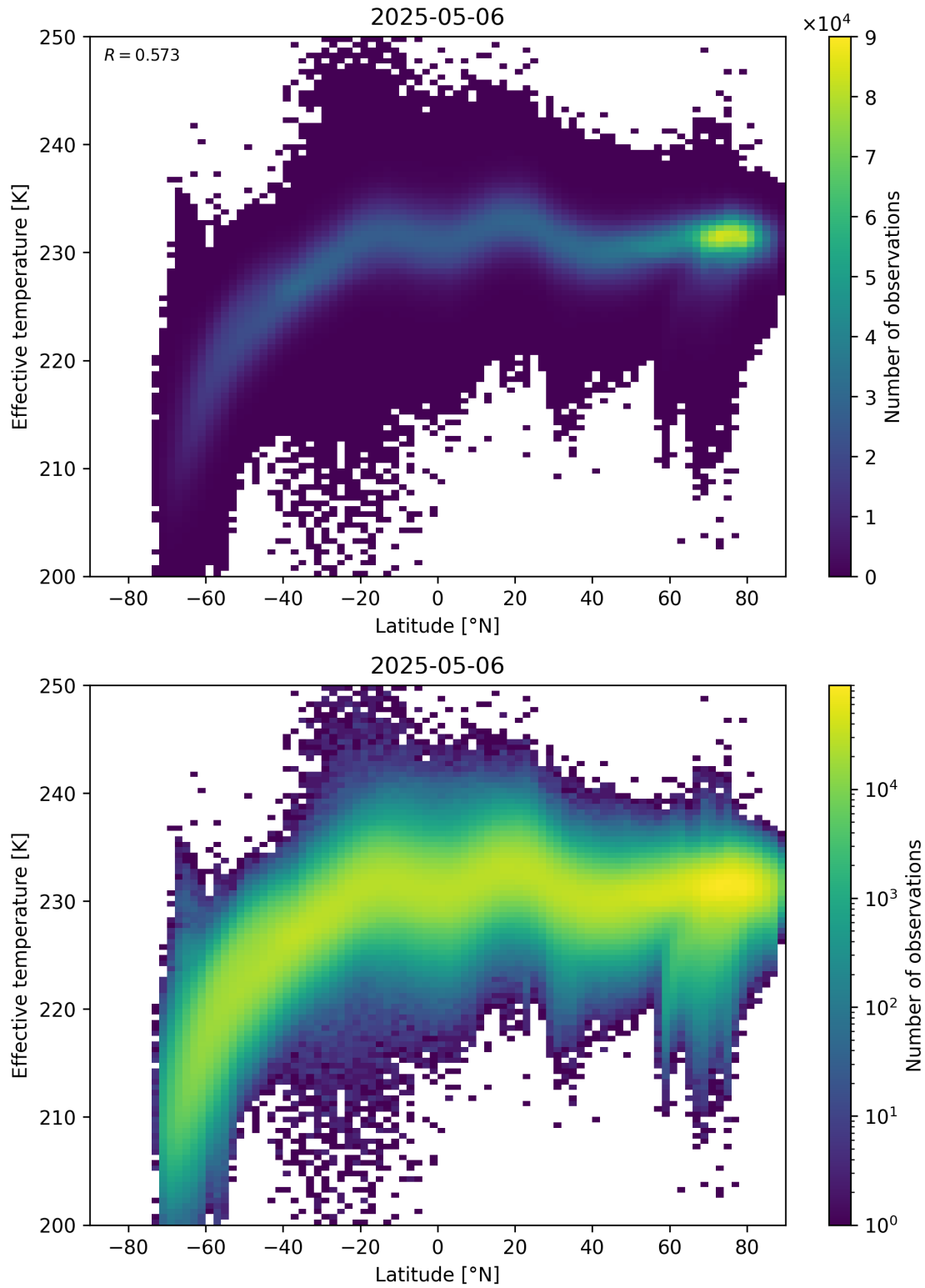
Figure 34: Scatter density plot of “Latitude” against “Effective temperature” for 2025-05-05 to 2025-05-07.
