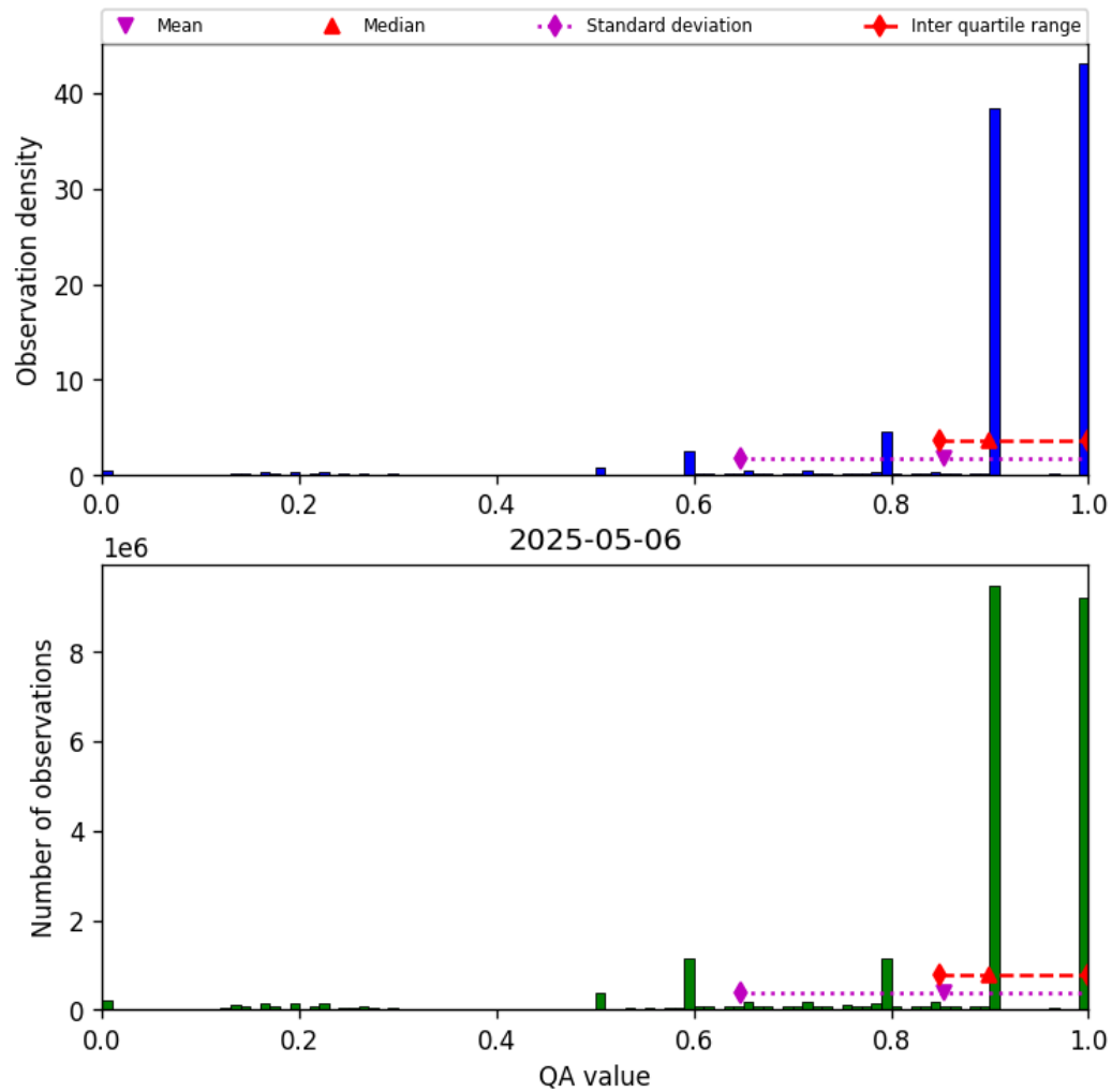
Figure 20: Histogram of “QA value” for 2025-05-05 to 2025-05-07
