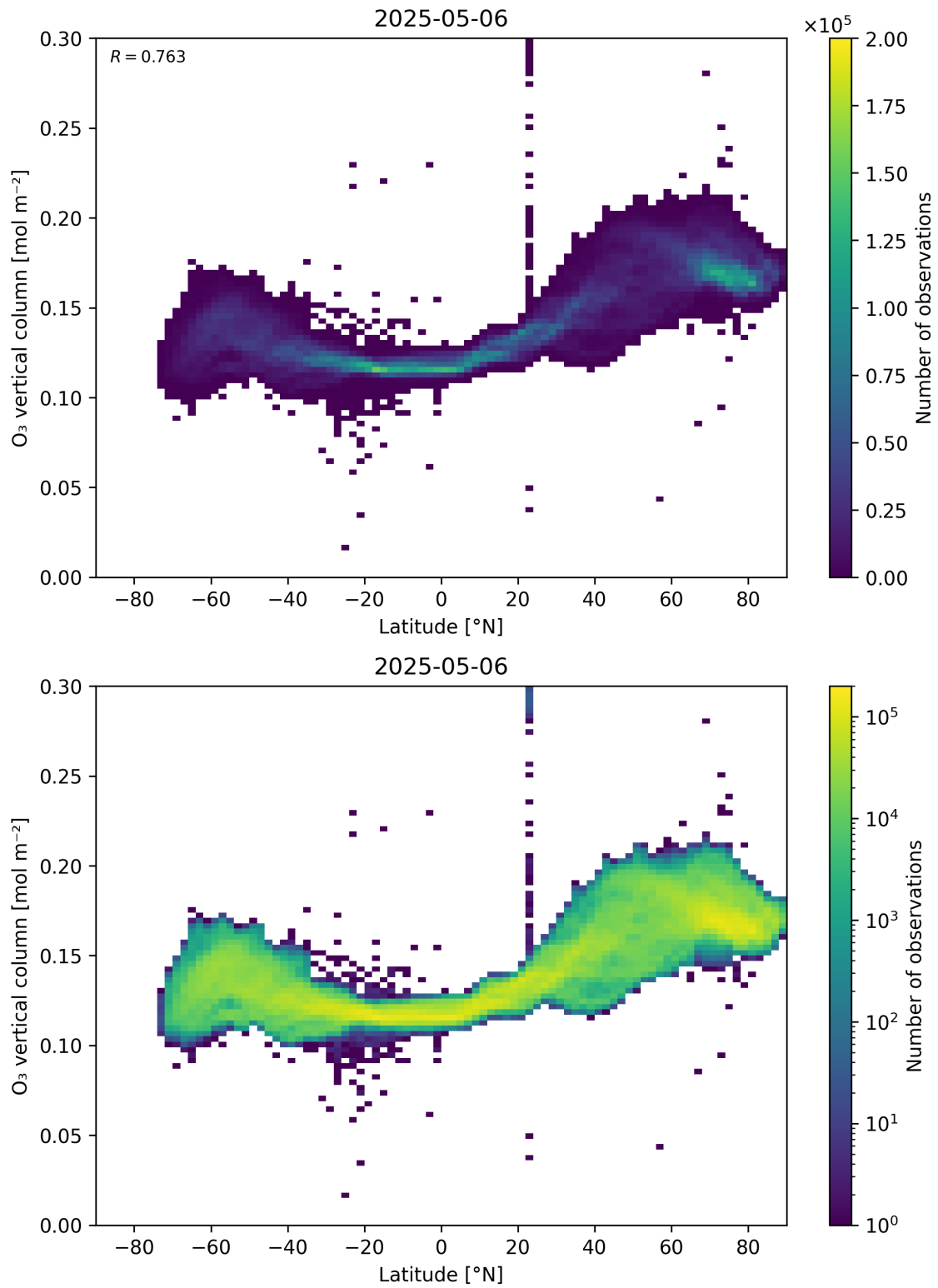
Figure 36: Scatter density plot of “Latitude” against “O 3 vertical column” for 2025-05-05 to 2025-05-07.
