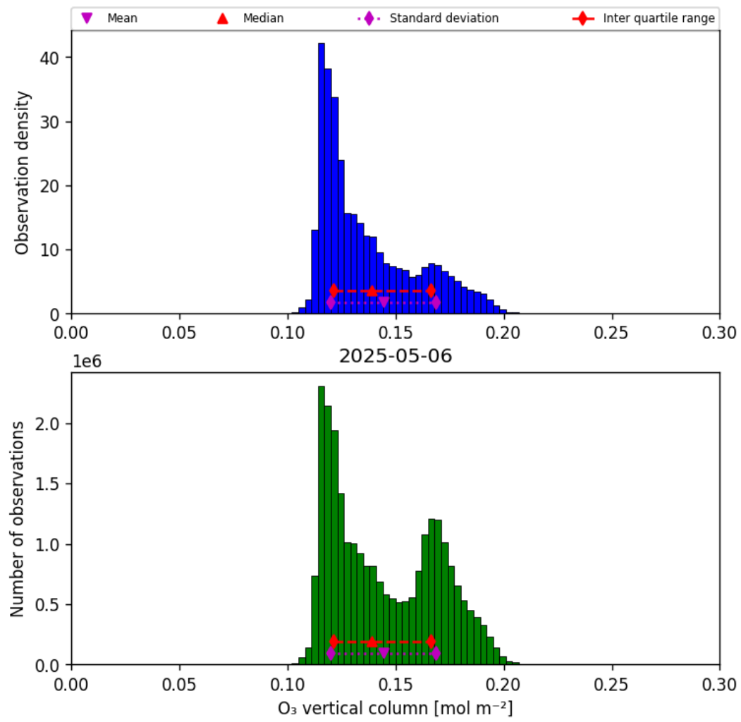
Figure 21: Histogram of “O 3 vertical column” for 2025-05-05 to 2025-05-07
