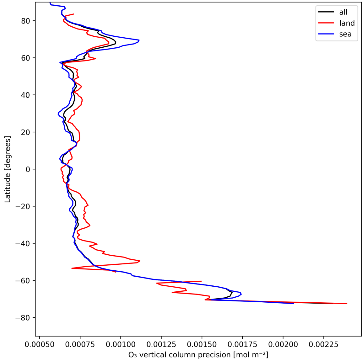
Figure 15: Zonal average of “O 3 vertical column precision” for 2025-05-05 to 2025-05-07.
