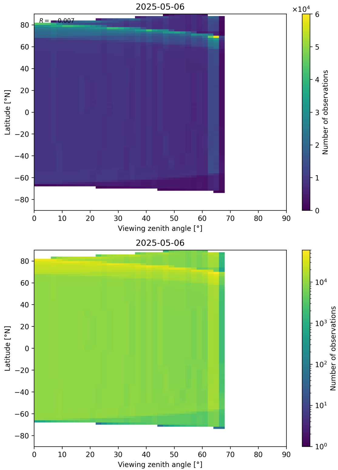
Figure 49: Scatter density plot of “Viewing zenith angle” against “Latitude” for 2025-05-05 to 2025-05-07.
