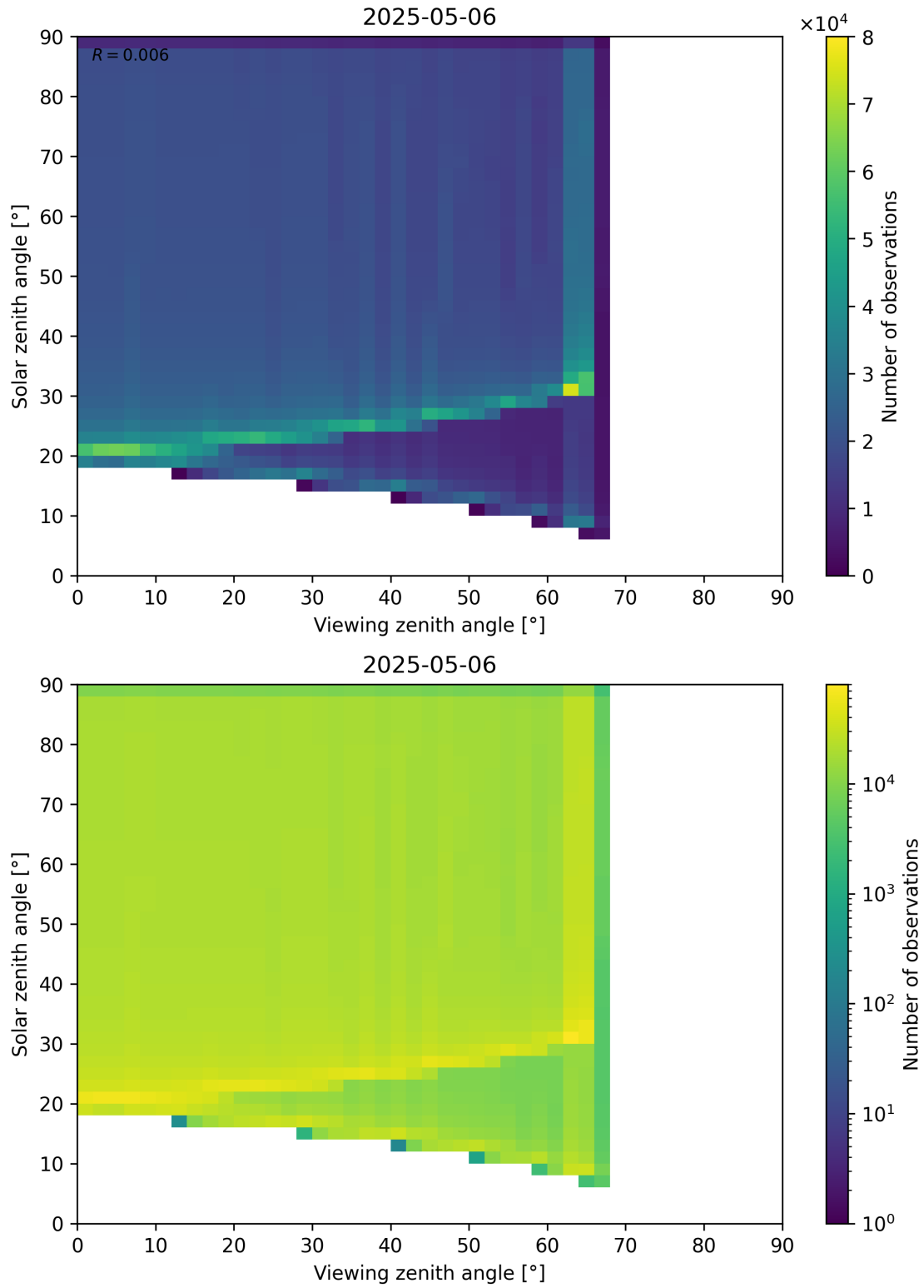
Figure 54: Scatter density plot of “Viewing zenith angle” against “Solar zenith angle” for 2025-05-05 to 2025-05-07.
