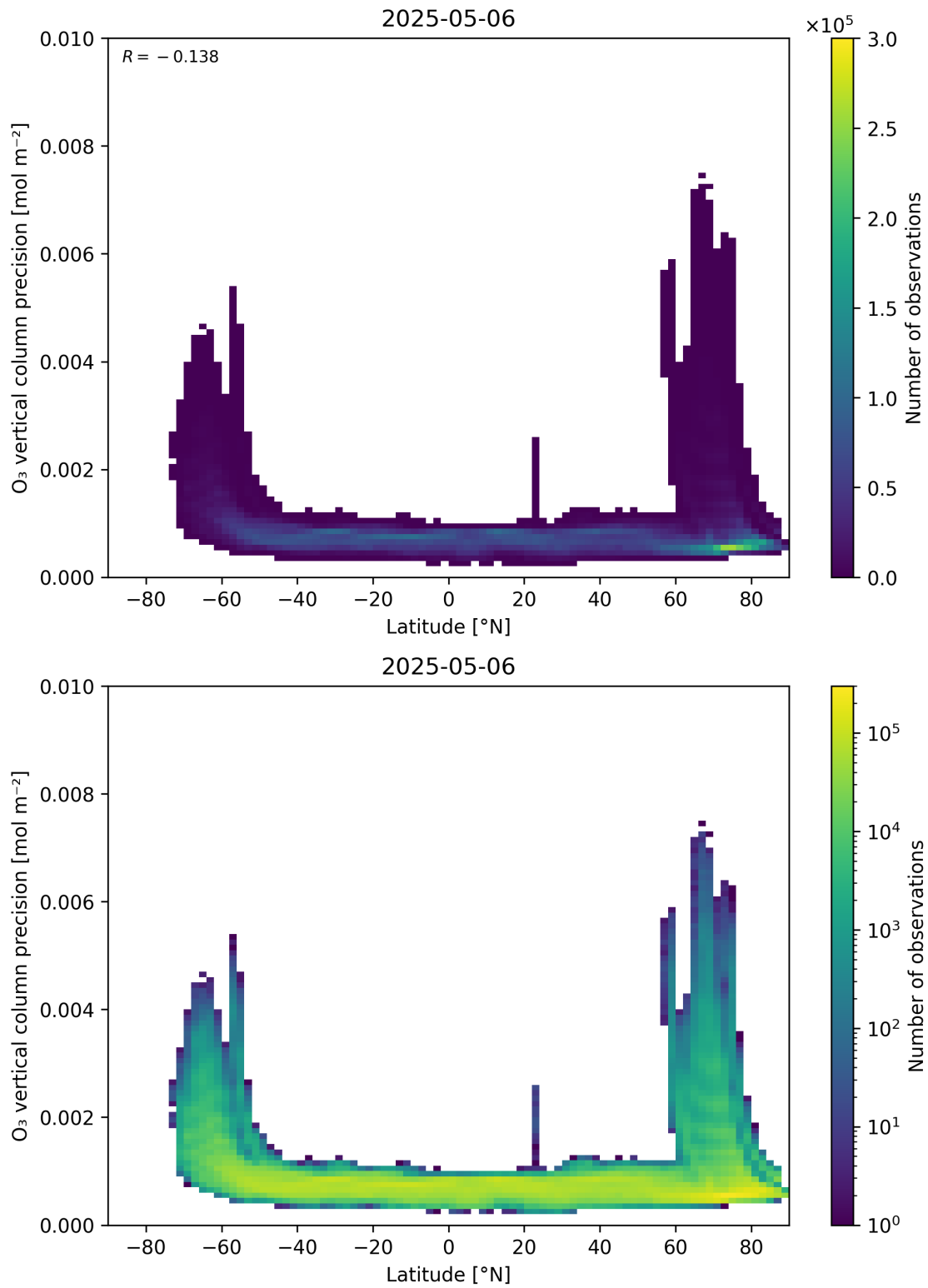
Figure 37: Scatter density plot of “Latitude” against “O 3 vertical column precision” for 2025-05-05 to 2025-05-07.
