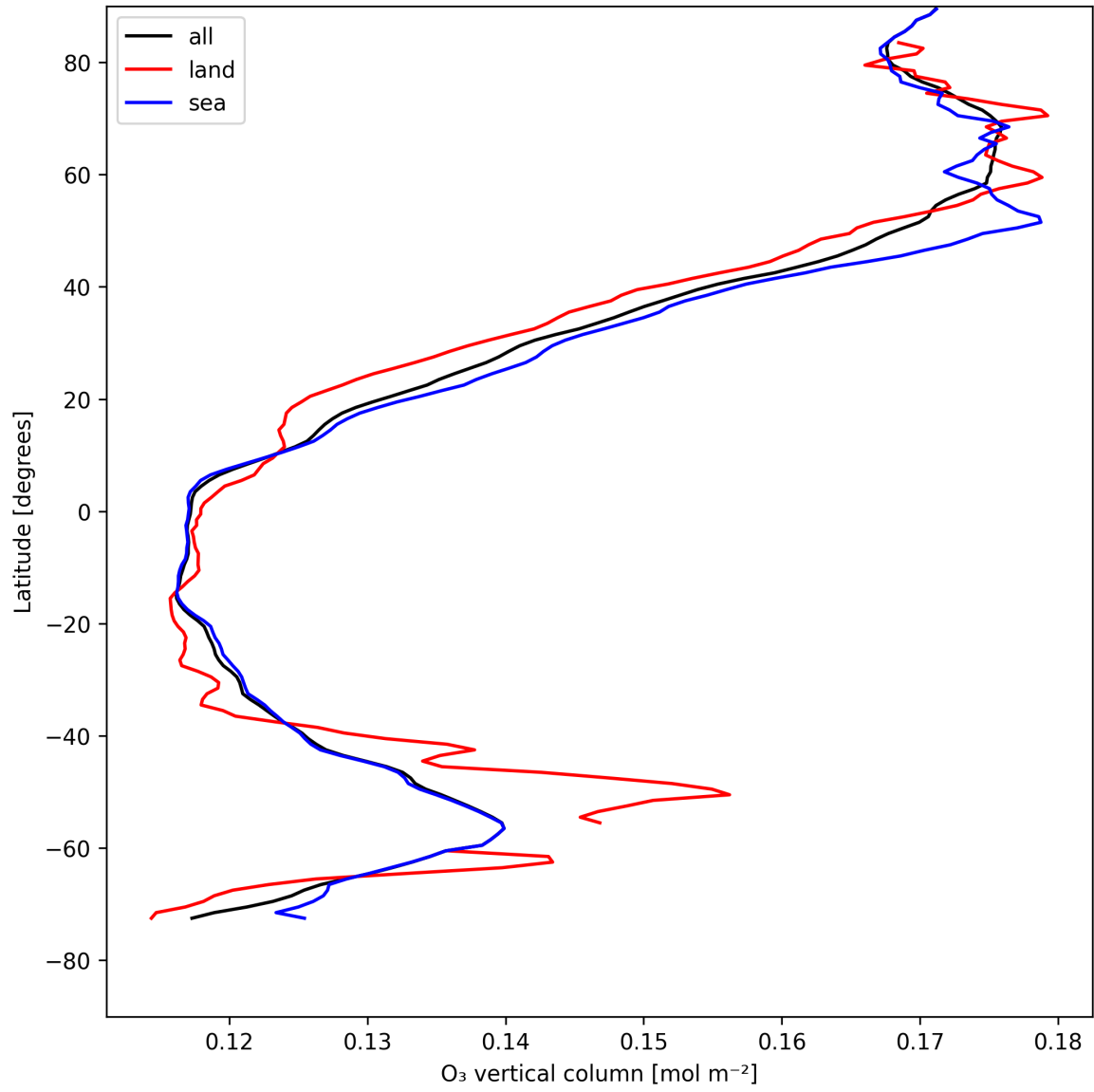
Figure 14: Zonal average of “O 3 vertical column” for 2025-05-05 to 2025-05-07.
