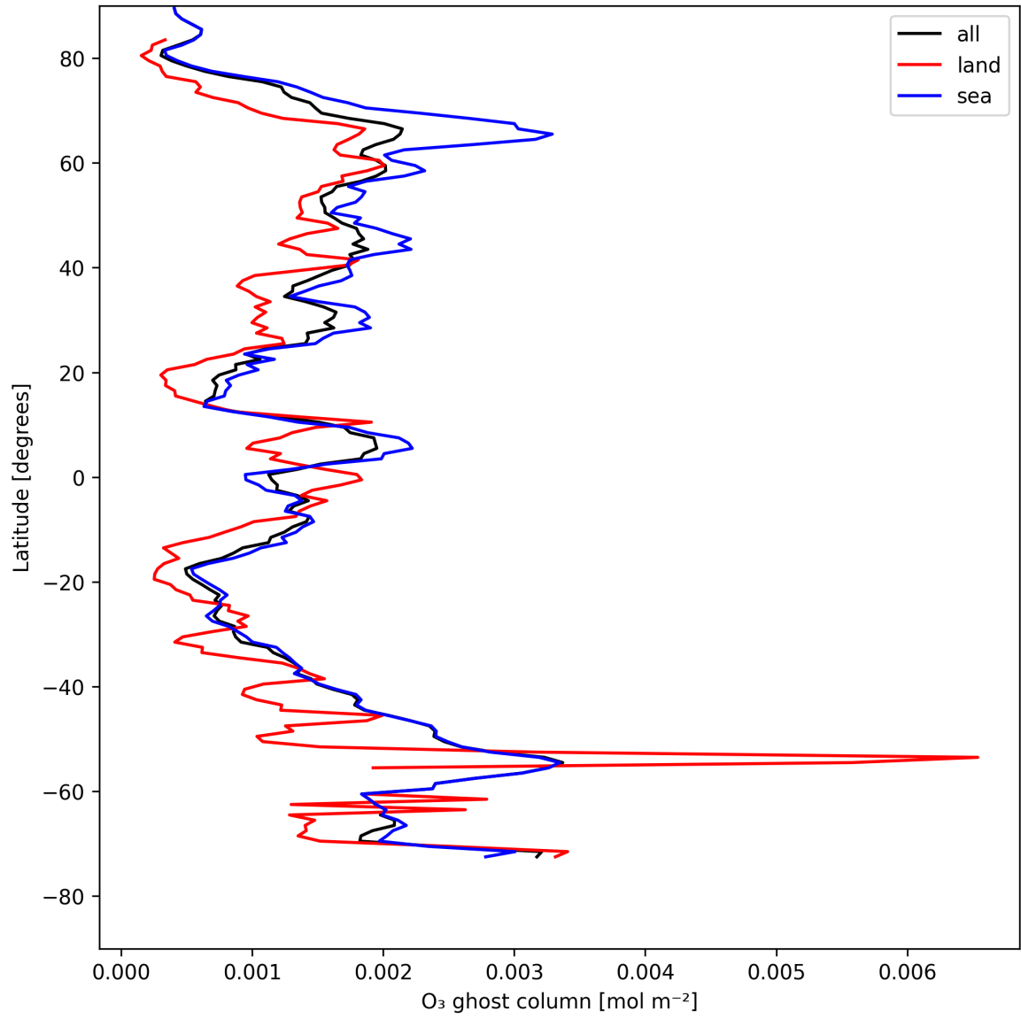
Figure 18: Zonal average of "O 3 ghost column" for 2025-05-05 to 2025-05-07.
