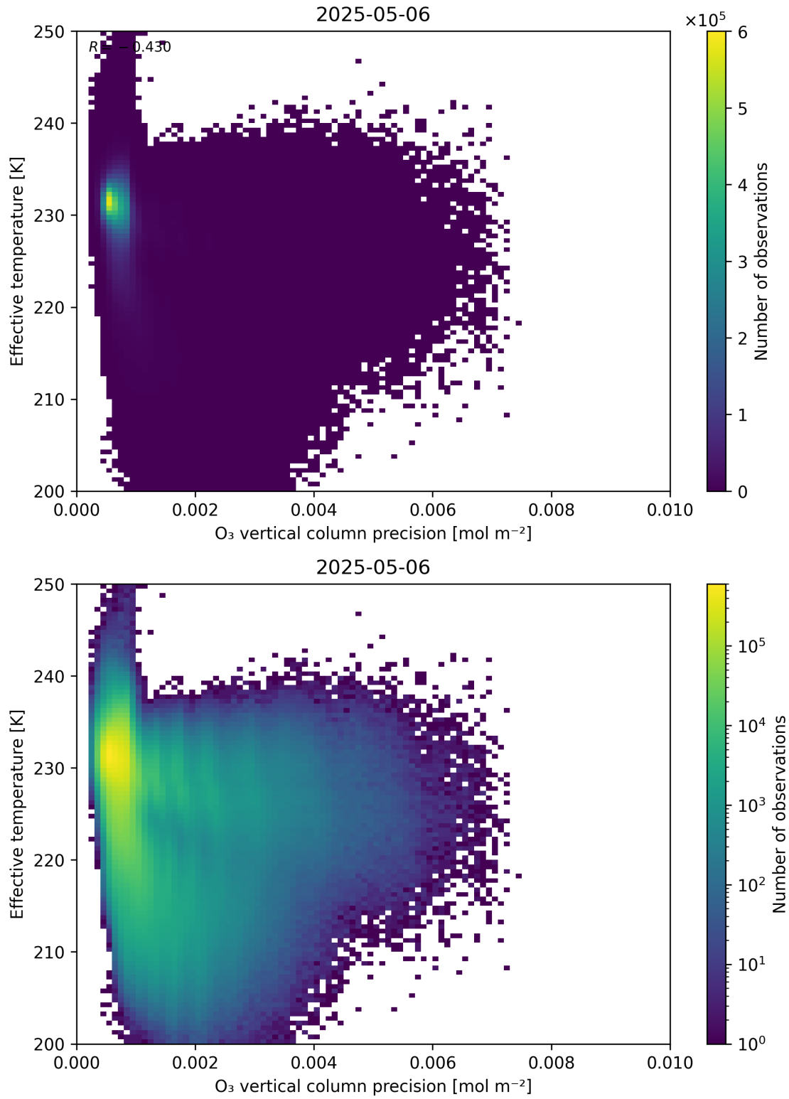
Figure 42: Scatter density plot of “O 3 vertical column precision” against “Effective temperature” for 2025-05-05 to 2025-05-07.
