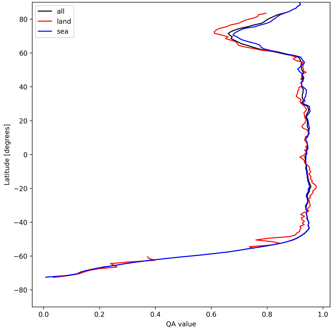
Figure 13: Zonal average of “QA value” for 2025-05-05 to 2025-05-07.
