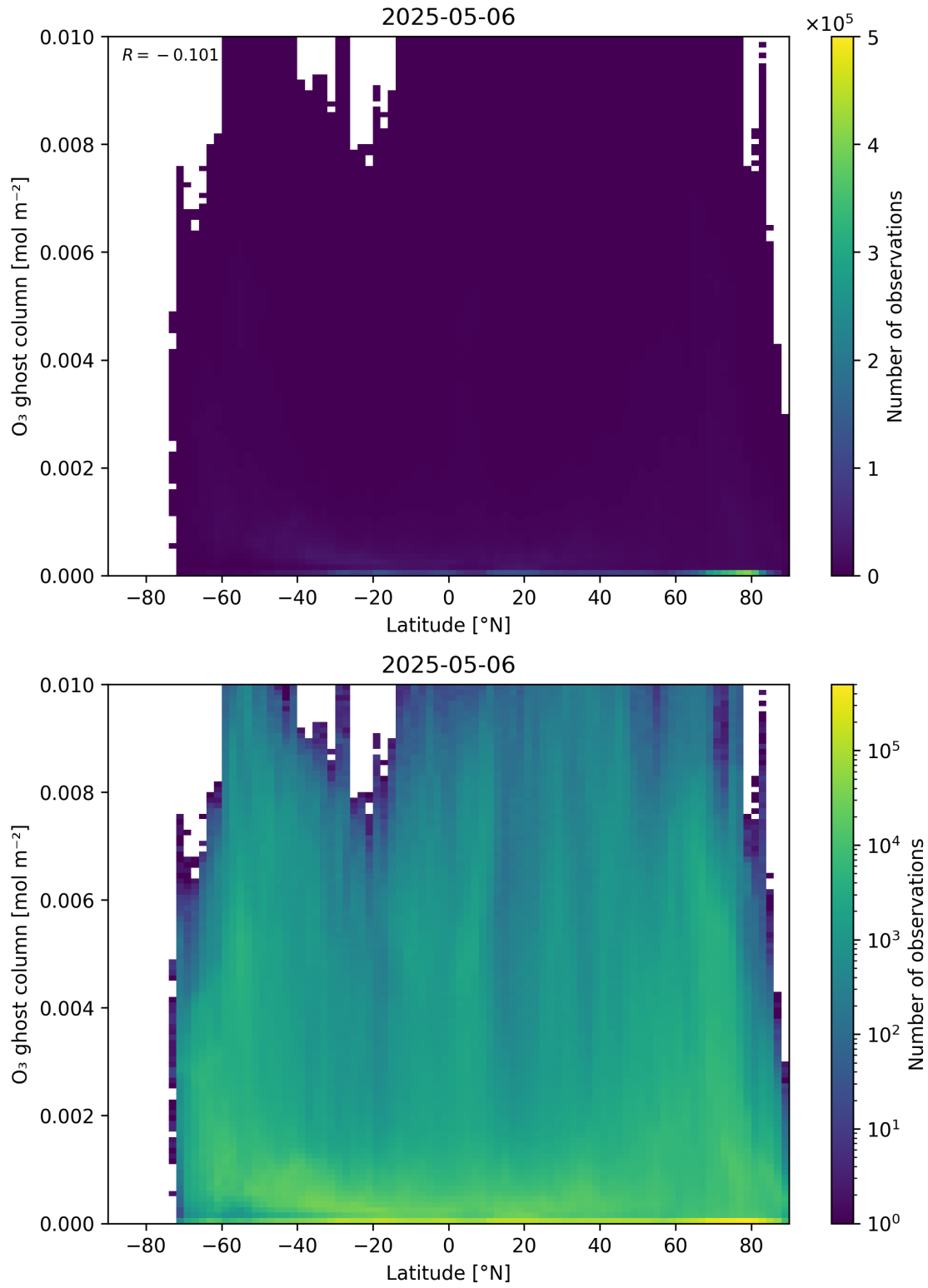
Figure 35: Scatter density plot of “Latitude” against “O 3 ghost column” for 2025-05-05 to 2025-05-07.
