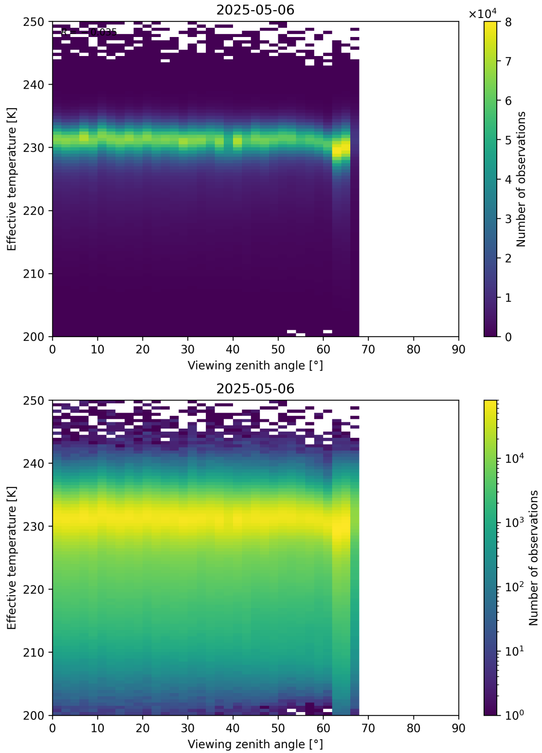
Figure 50: Scatter density plot of “Viewing zenith angle” against “Effective temperature” for 2025-05-05 to 2025-05-07.
