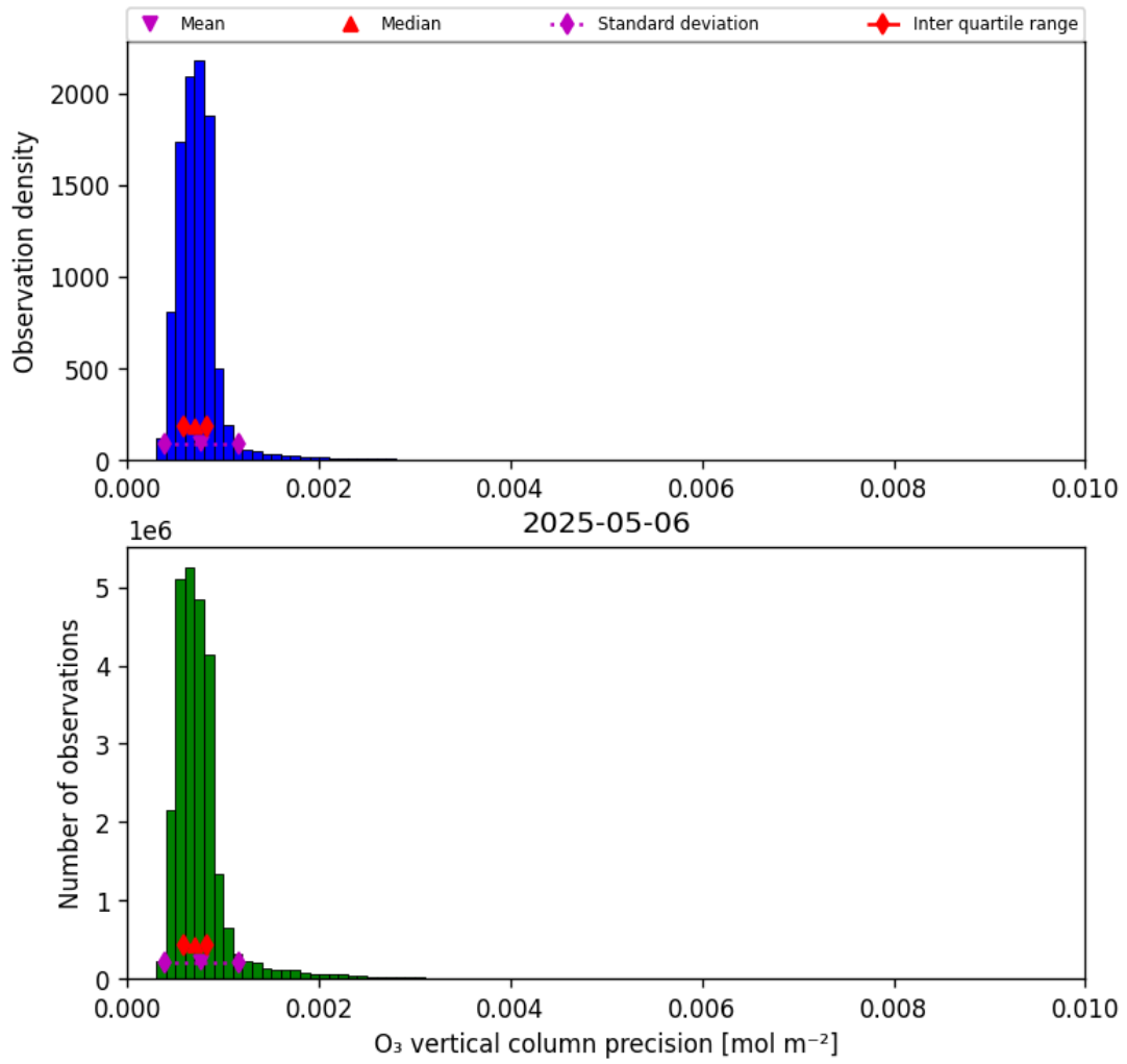
Figure 22: Histogram of “O 3 vertical column precision” for 2025-05-05 to 2025-05-07
