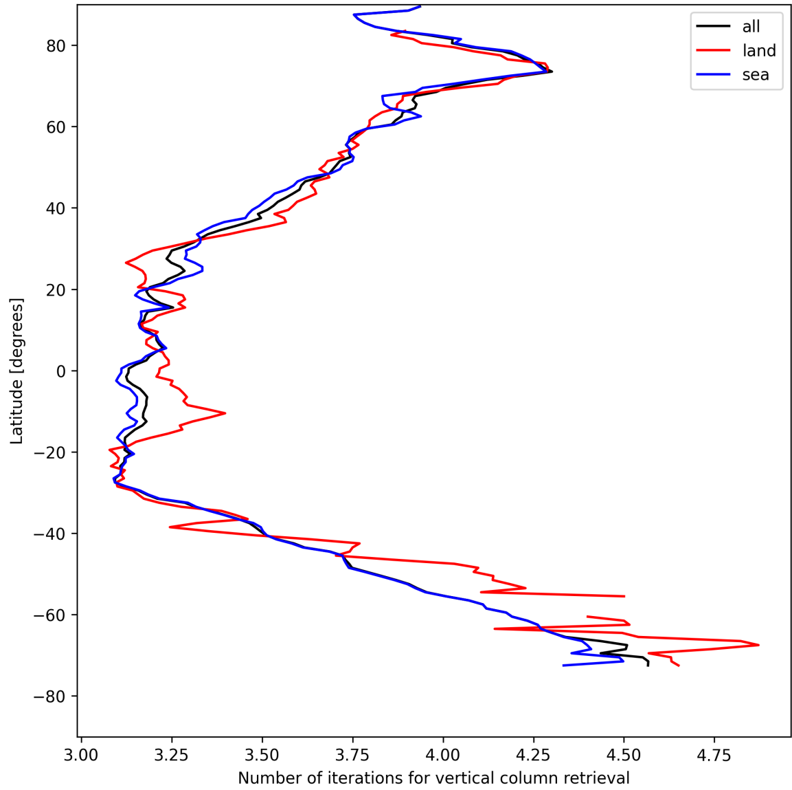
Figure 19: Zonal average of “Number of iterations for vertical column retrieval” for 2025-05-05 to 2025-05-07.
