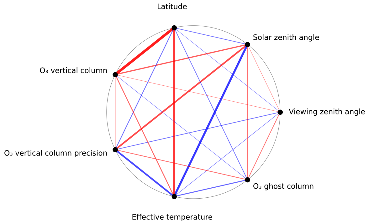
Figure 1: Map of correlation graph for 2025-05-05 to 2025-05-07.
