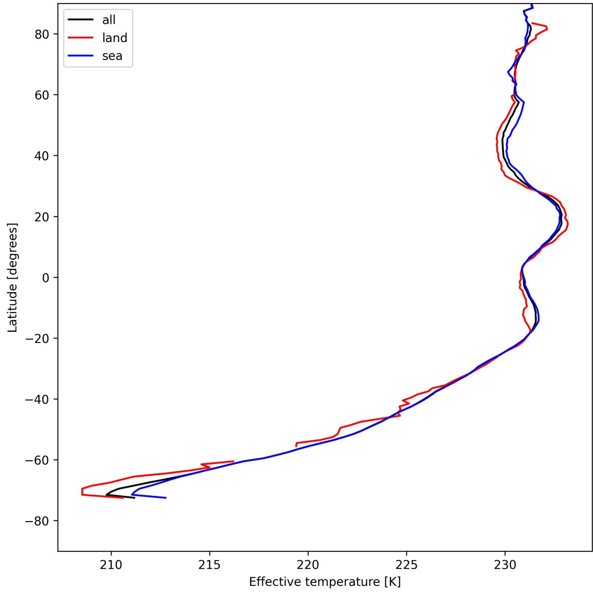
Figure 17: Zonal average of "Effective temperature" for 2025-05-05 to 2025-05-07.
