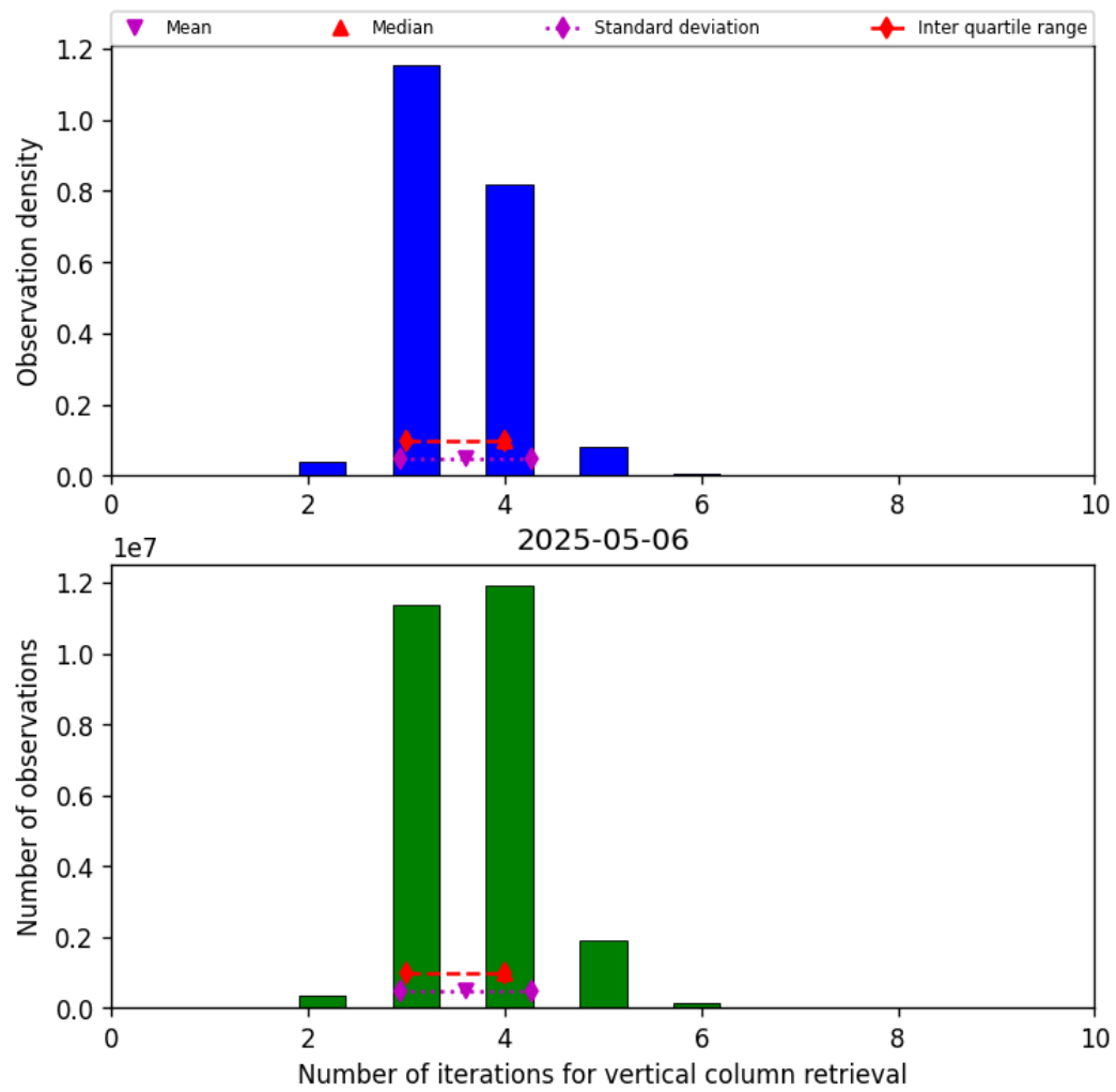
Figure 26: Histogram of “Number of iterations for vertical column retrieval” for 2025-05-05 to 2025-05-07
