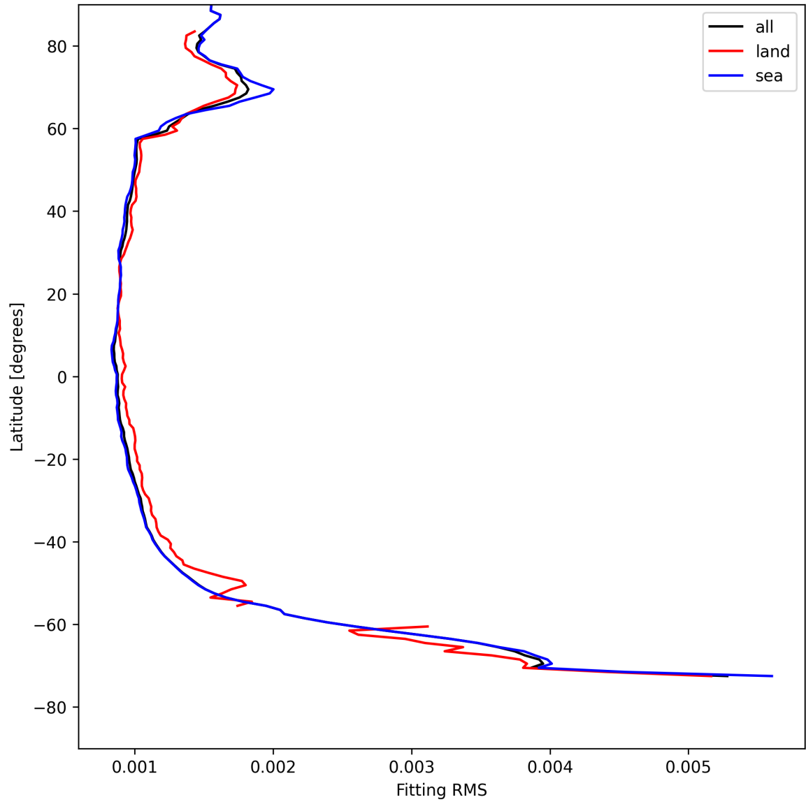
Figure 16: Zonal average of “Fitting RMS” for 2025-05-05 to 2025-05-07.
