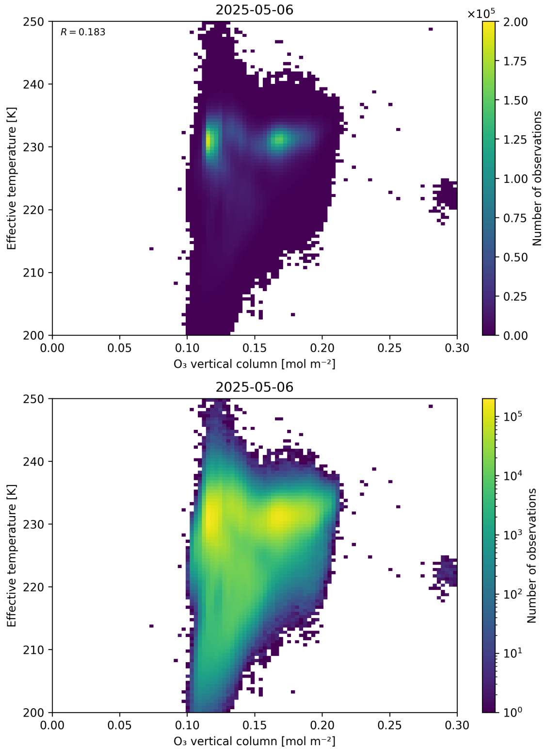
Figure 39: Scatter density plot of “O 3 vertical column” against “Effective temperature” for 2025-05-05 to 2025-05-07.
