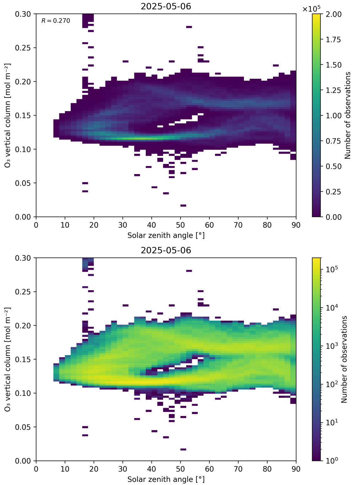
Figure 47: Scatter density plot of “Solar zenith angle” against “O 3 vertical column” for 2025-05-05 to 2025-05-07.
