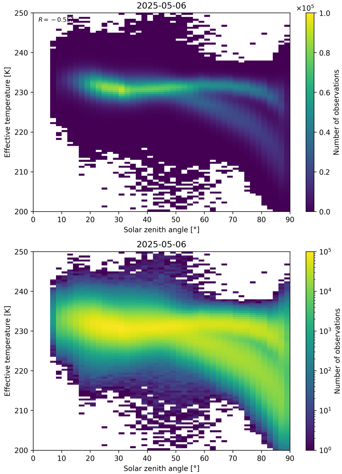
Figure 45: Scatter density plot of “Solar zenith angle” against “Effective temperature” for 2025-05-05 to 2025-05-07.
