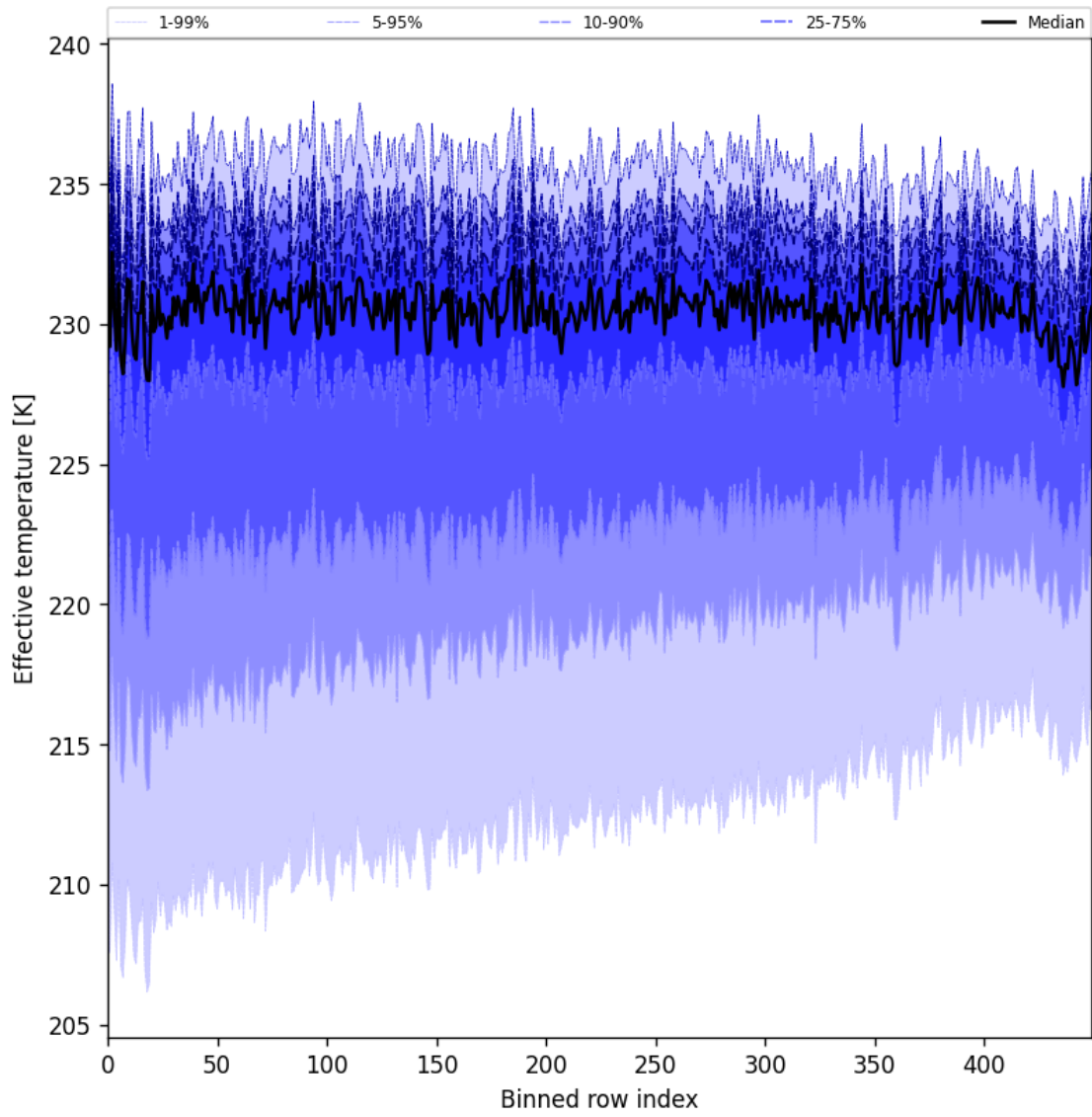
Figure 31: Along track statistics of “Effective temperature” for 2025-05-05 to 2025-05-07
