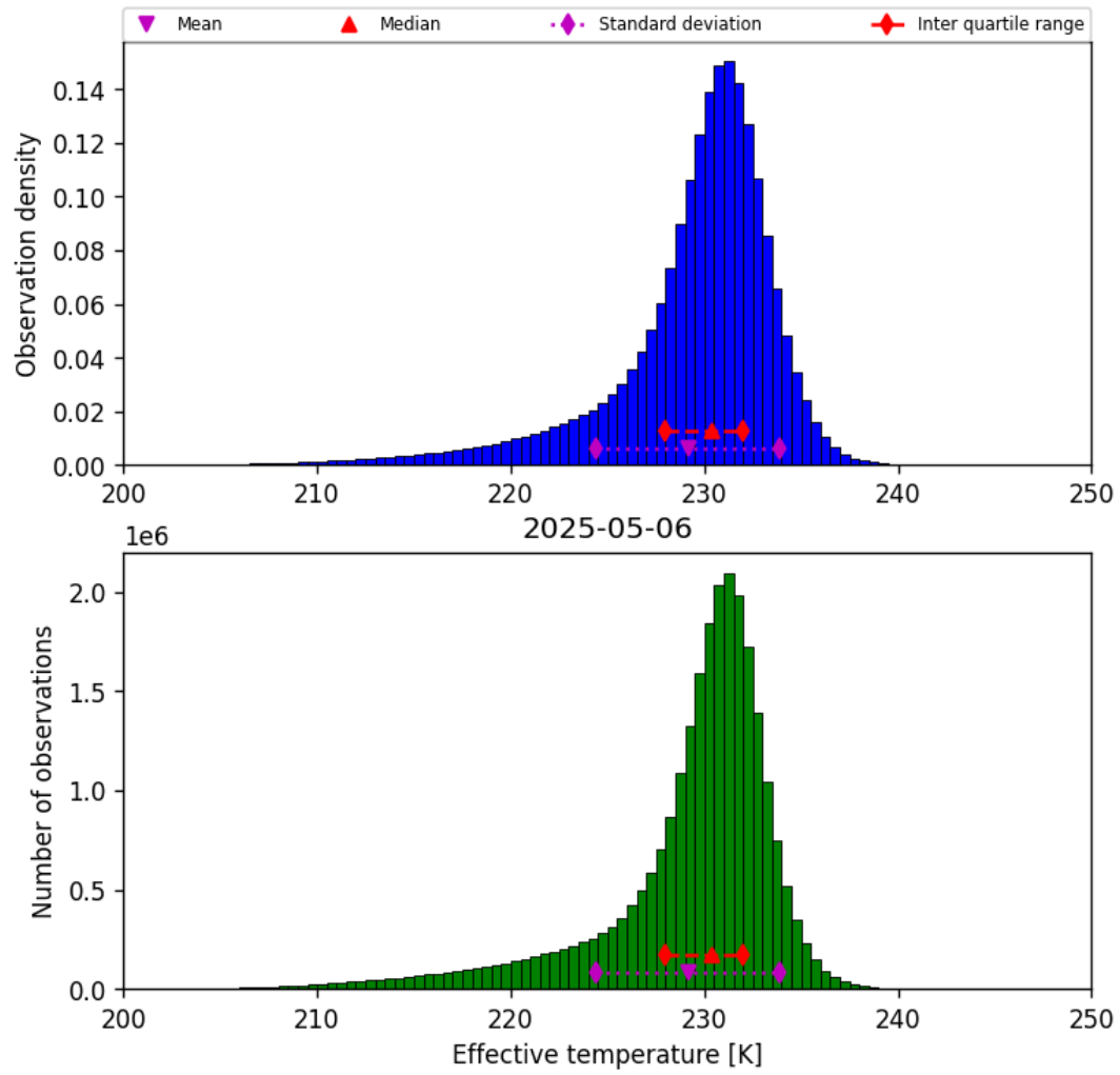
Figure 24: Histogram of “Effective temperature” for 2025-05-05 to 2025-05-07
