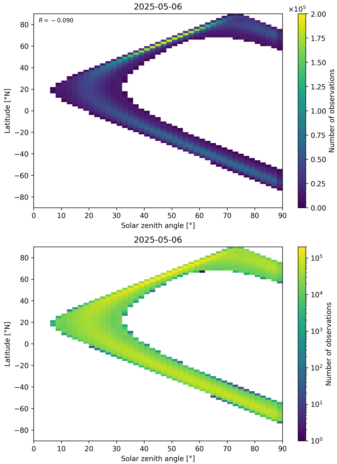
Figure 44: Scatter density plot of “Solar zenith angle” against “Latitude” for 2025-05-05 to 2025-05-07.
