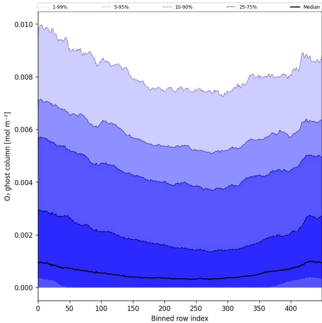
Figure 32: Along track statistics of “O 3 ghost column” for 2025-05-05 to 2025-05-07
