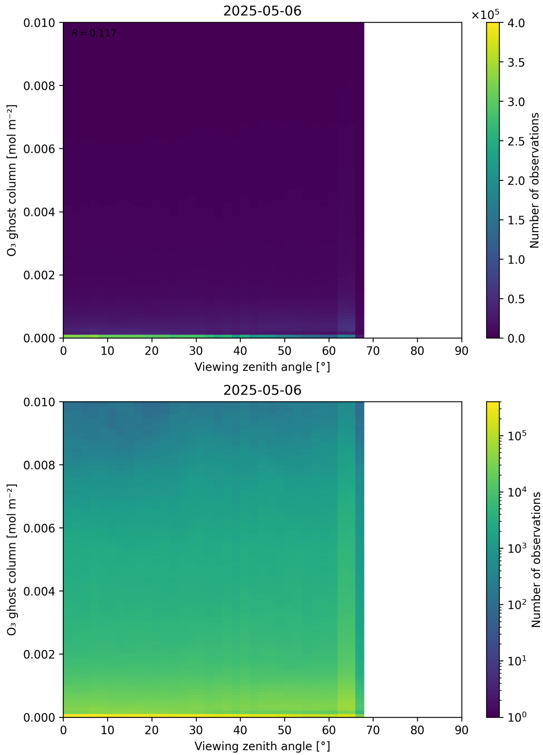
Figure 51: Scatter density plot of “Viewing zenith angle” against “O 3 ghost column” for 2025-05-05 to 2025-05-07.
