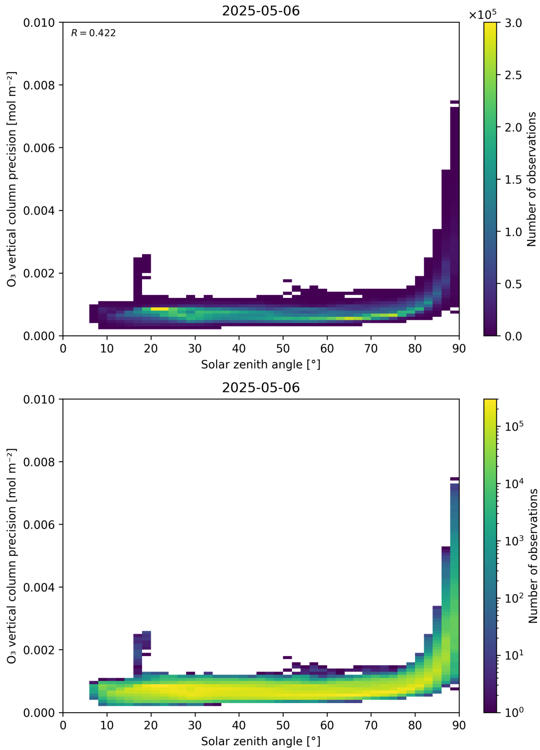
Figure 48: Scatter density plot of “Solar zenith angle” against “O 3 vertical column precision” for 2025-05-05 to 2025-05-07.
