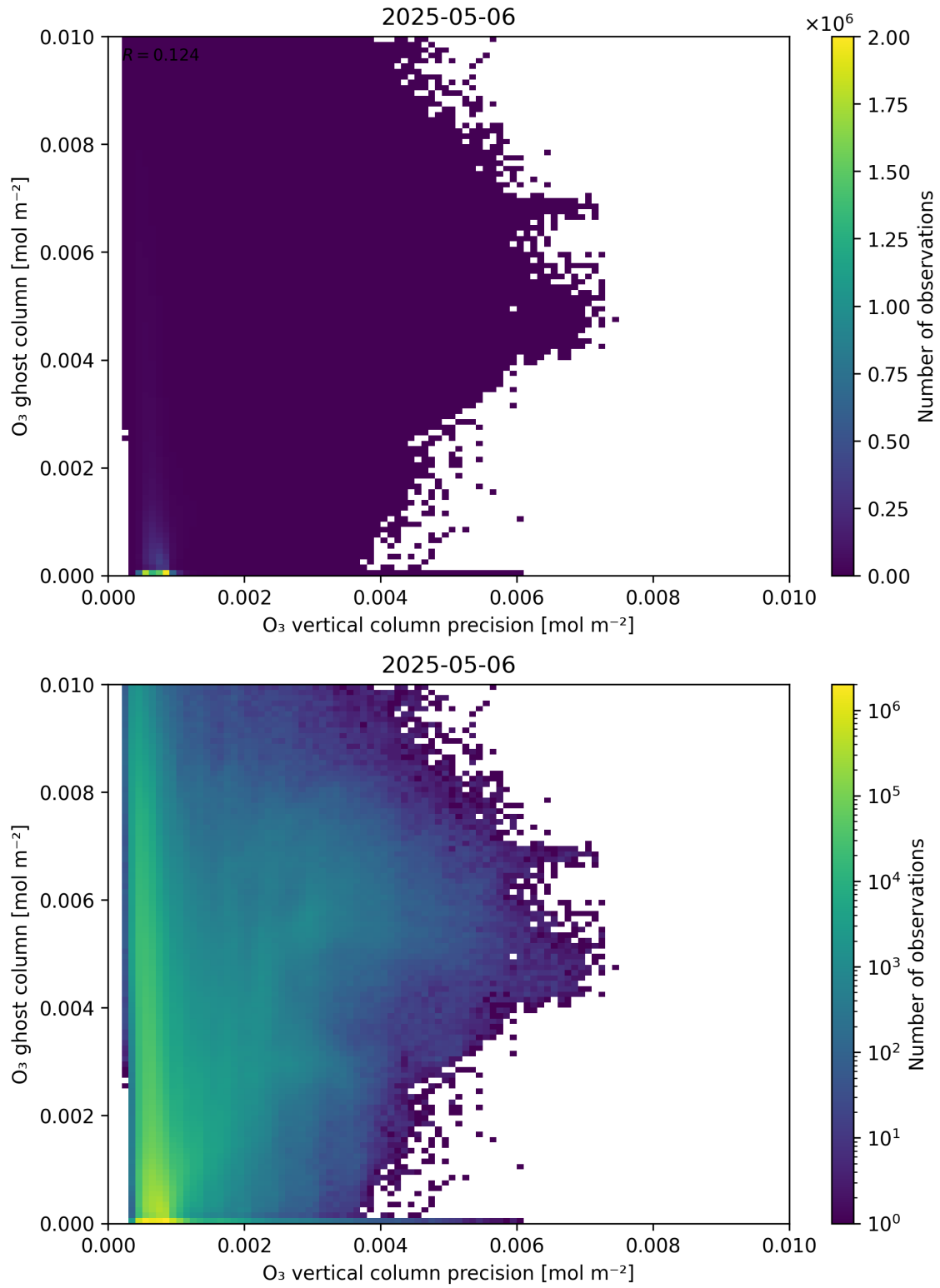
Figure 43: Scatter density plot of “O 3 vertical column precision” against “O 3 ghost column” for 2025-05-05 to 2025-05-07.
