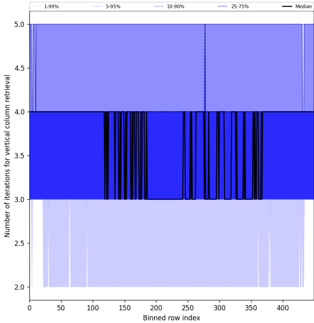
Figure 33: Along track statistics of “Number of iterations for vertical column retrieval” for 2025-05-05 to 2025-05-07
