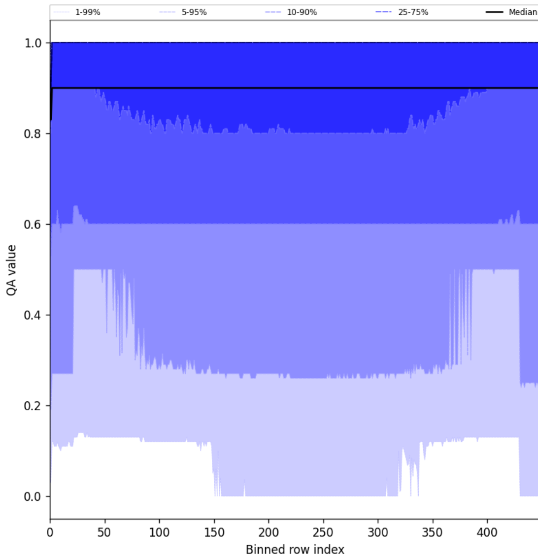
Figure 27: Along track statistics of “QA value” for 2025-05-05 to 2025-05-07
