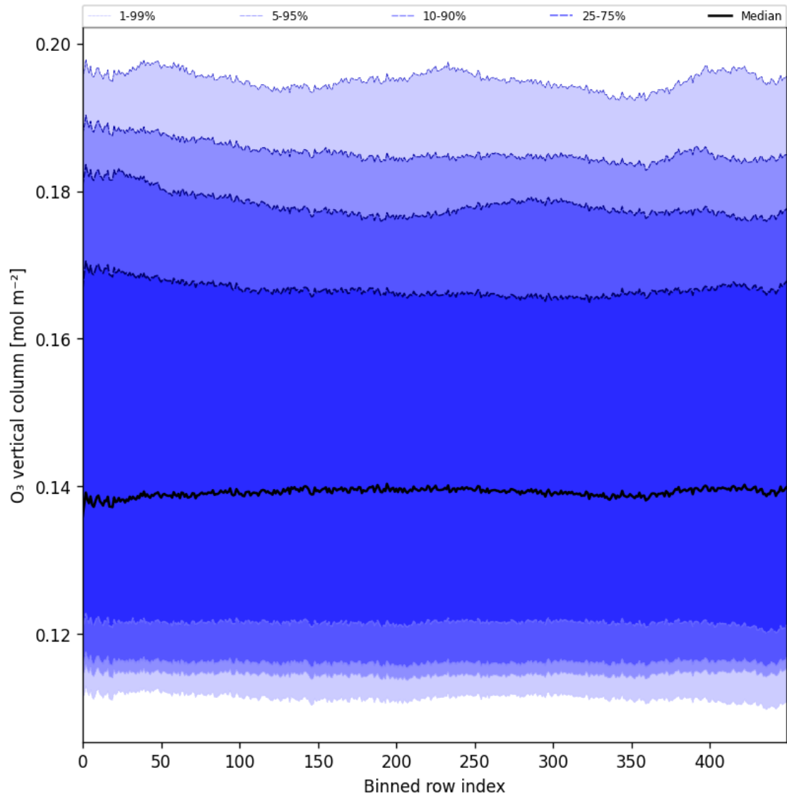
Figure 28: Along track statistics of “O 3 vertical column” for 2025-05-05 to 2025-05-07
