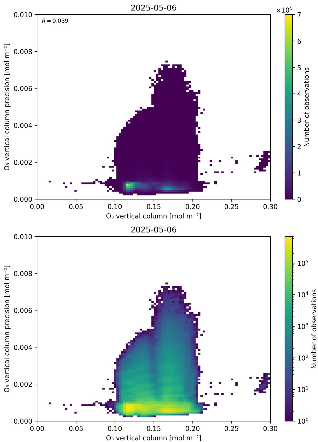
Figure 41: Scatter density plot of “O 3 vertical column” against “O 3 vertical column precision” for 2025-05-05 to 2025-05-07.
