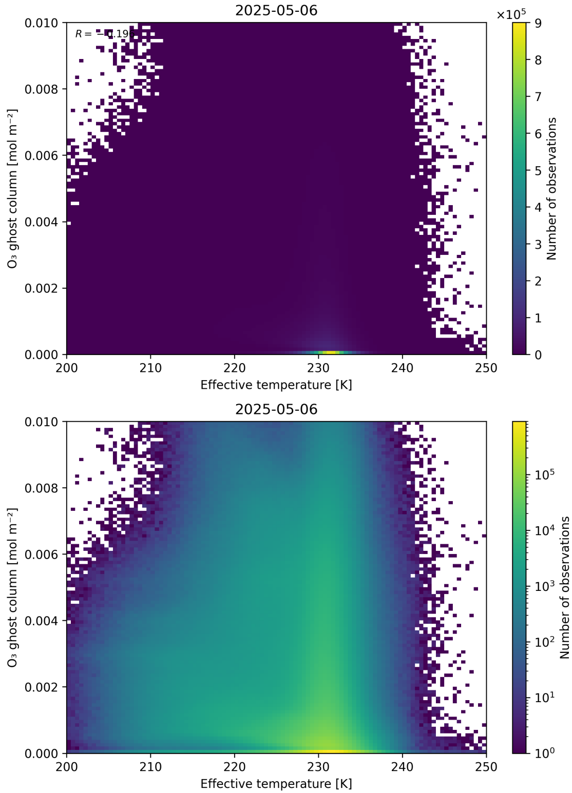
Figure 38: Scatter density plot of “Effective temperature” against “O 3 ghost column” for 2025-05-05 to 2025-05-07.
