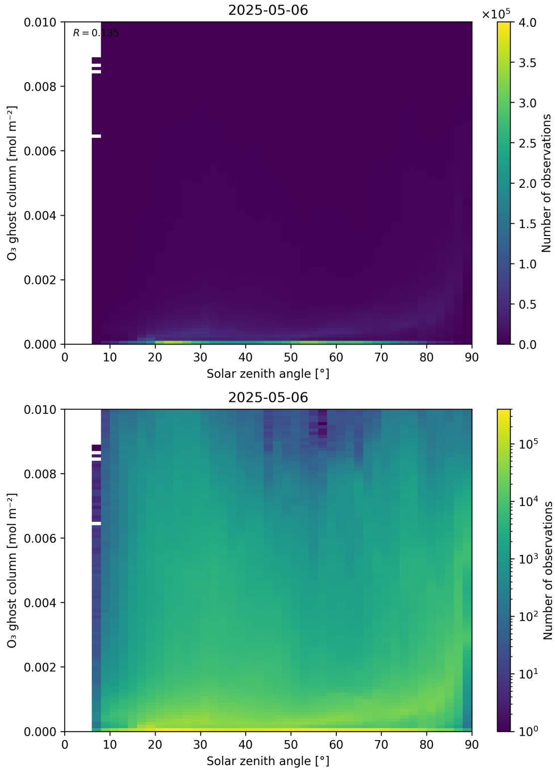
Figure 46: Scatter density plot of “Solar zenith angle” against “O 3 ghost column” for 2025-05-05 to 2025-05-07.
