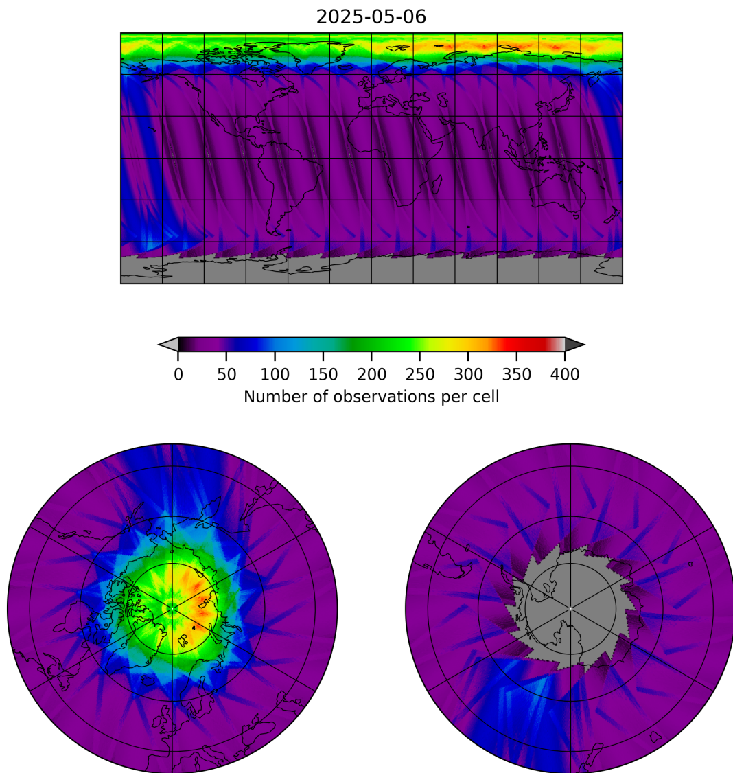
Figure 12: Map of the number of observations for 2025-05-05 to 2025-05-07
