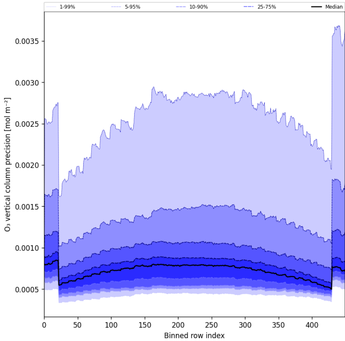
Figure 29: Along track statistics of “O 3 vertical column precision” for 2025-05-05 to 2025-05-07
