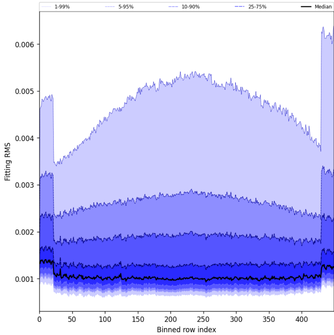
Figure 30: Along track statistics of “Fitting RMS” for 2025-05-05 to 2025-05-07
