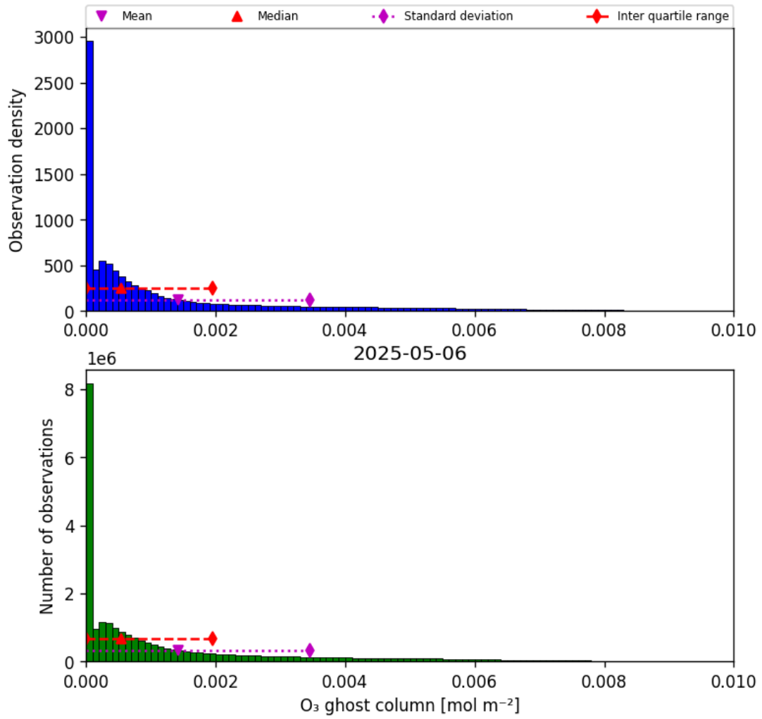
Figure 25: Histogram of “O 3 ghost column” for 2025-05-05 to 2025-05-07
