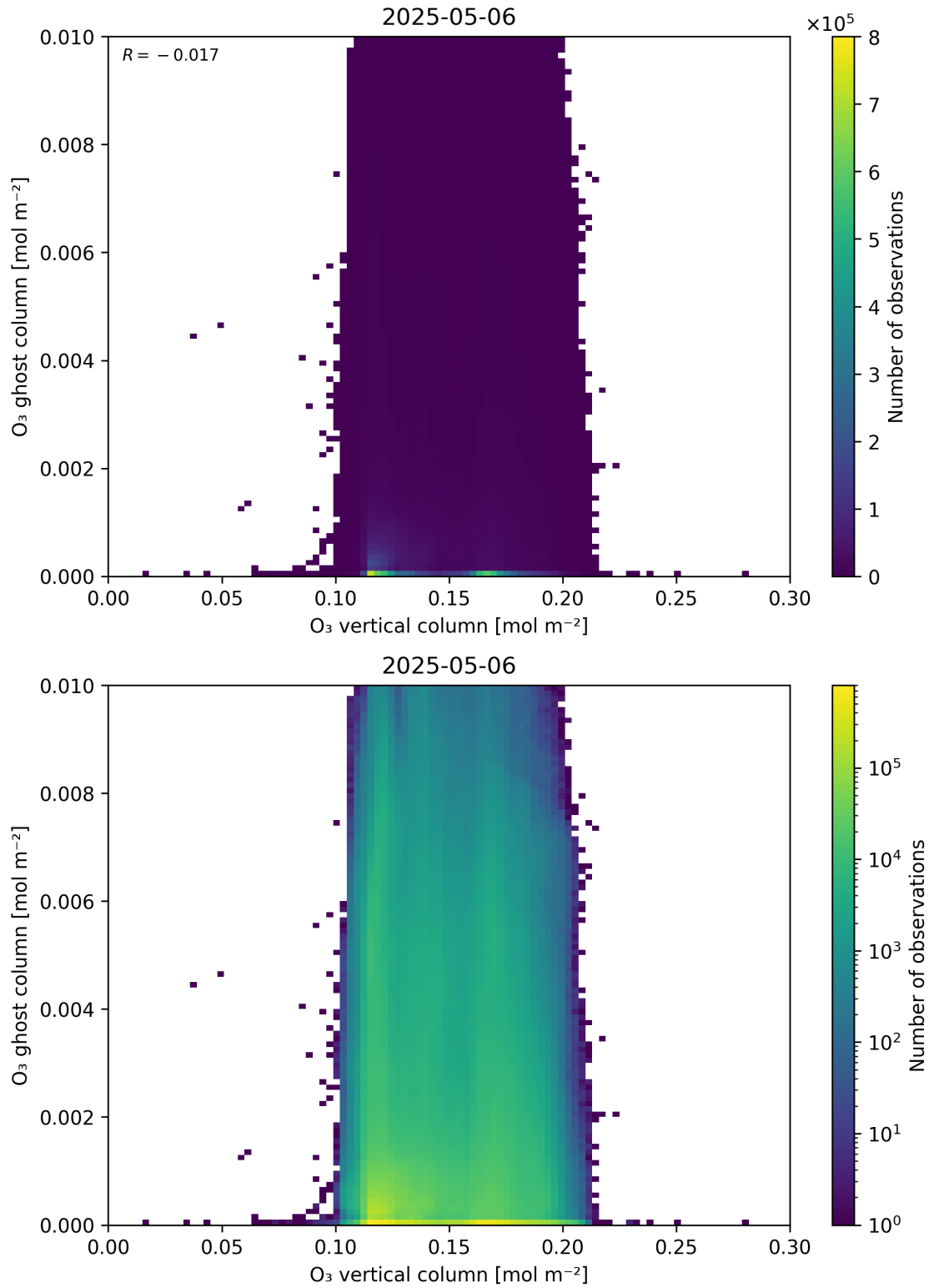
Figure 40: Scatter density plot of “O 3 vertical column” against “O 3 ghost column” for 2025-05-05 to 2025-05-07.
