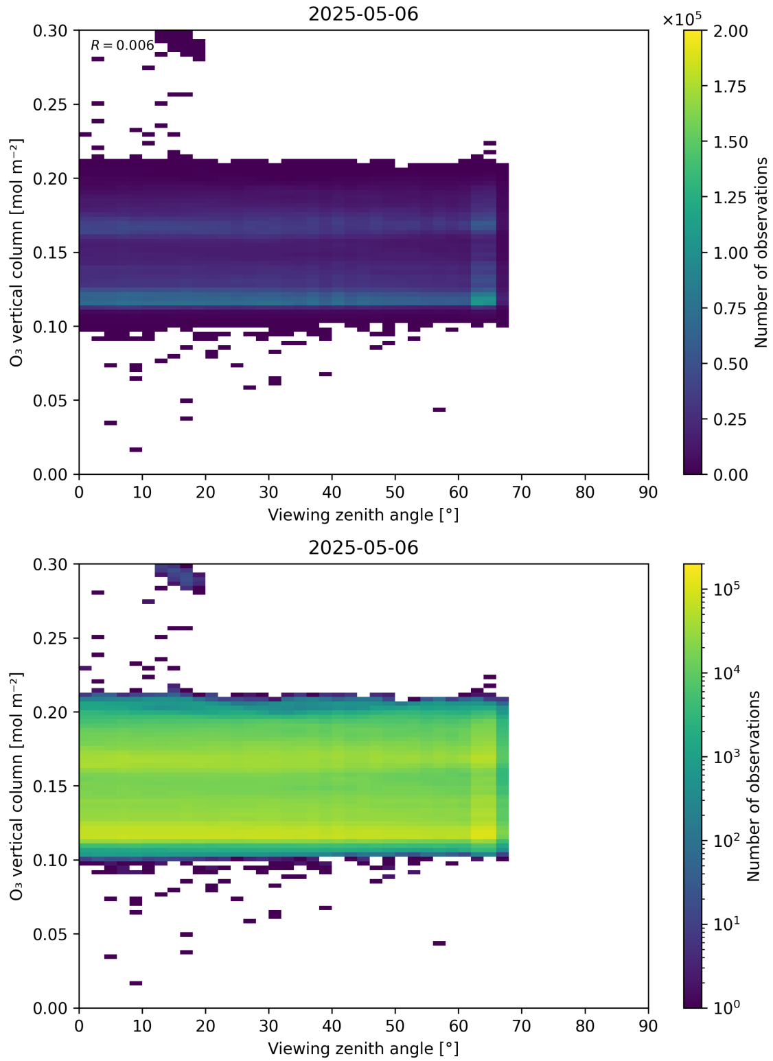
Figure 52: Scatter density plot of “Viewing zenith angle” against “O 3 vertical column” for 2025-05-05 to 2025-05-07.
