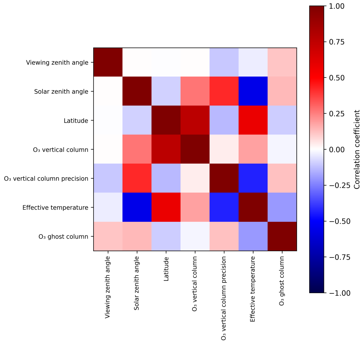
Figure 2: Map of correlation matrix for 2025-05-05 to 2025-05-07.
