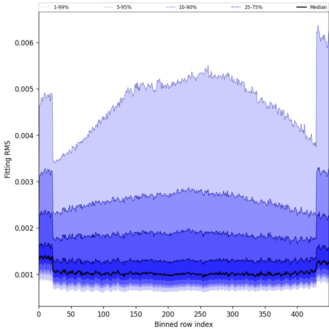
Figure 30: Along track statistics of “Fitting RMS” for 2025-05-06 to 2025-05-08
