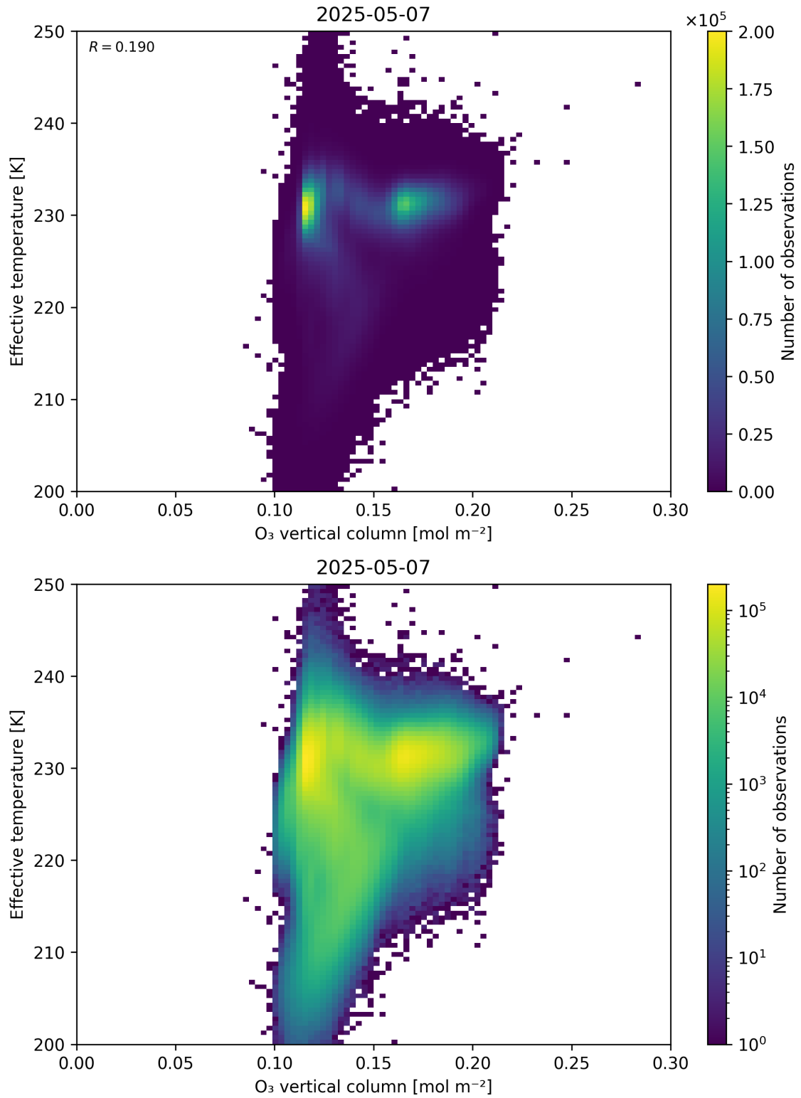
Figure 39: Scatter density plot of “O 3 vertical column” against “Effective temperature” for 2025-05-06 to 2025-05-08.
