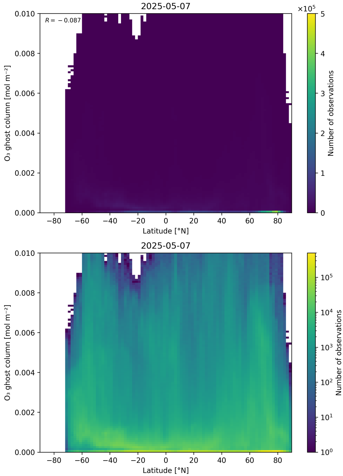
Figure 35: Scatter density plot of “Latitude” against “O 3 ghost column” for 2025-05-06 to 2025-05-08.
