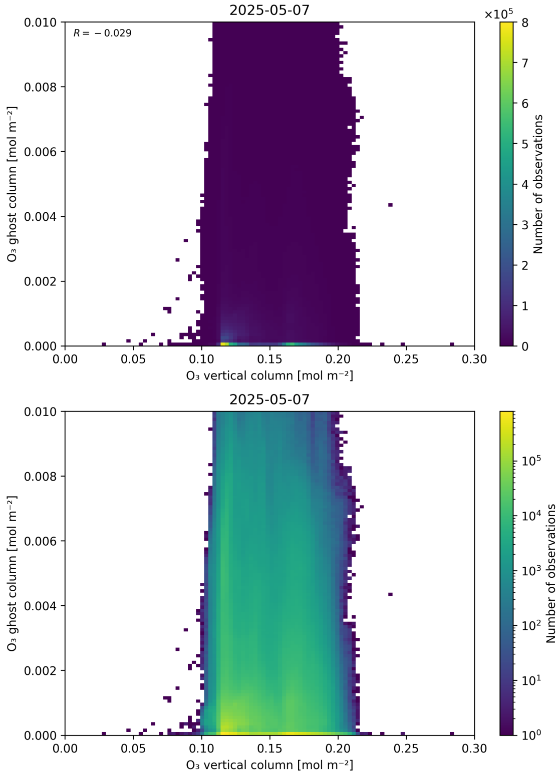
Figure 40: Scatter density plot of “O 3 vertical column” against “O 3 ghost column” for 2025-05-06 to 2025-05-08.
