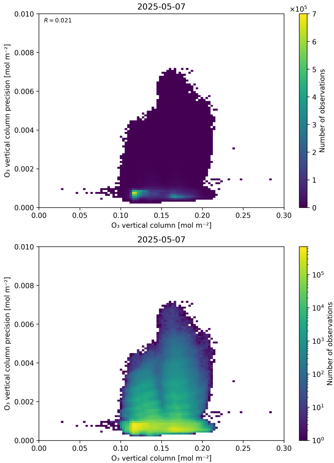
Figure 41: Scatter density plot of “O 3 vertical column” against “O 3 vertical column precision” for 2025-05-06 to 2025-05-08.
