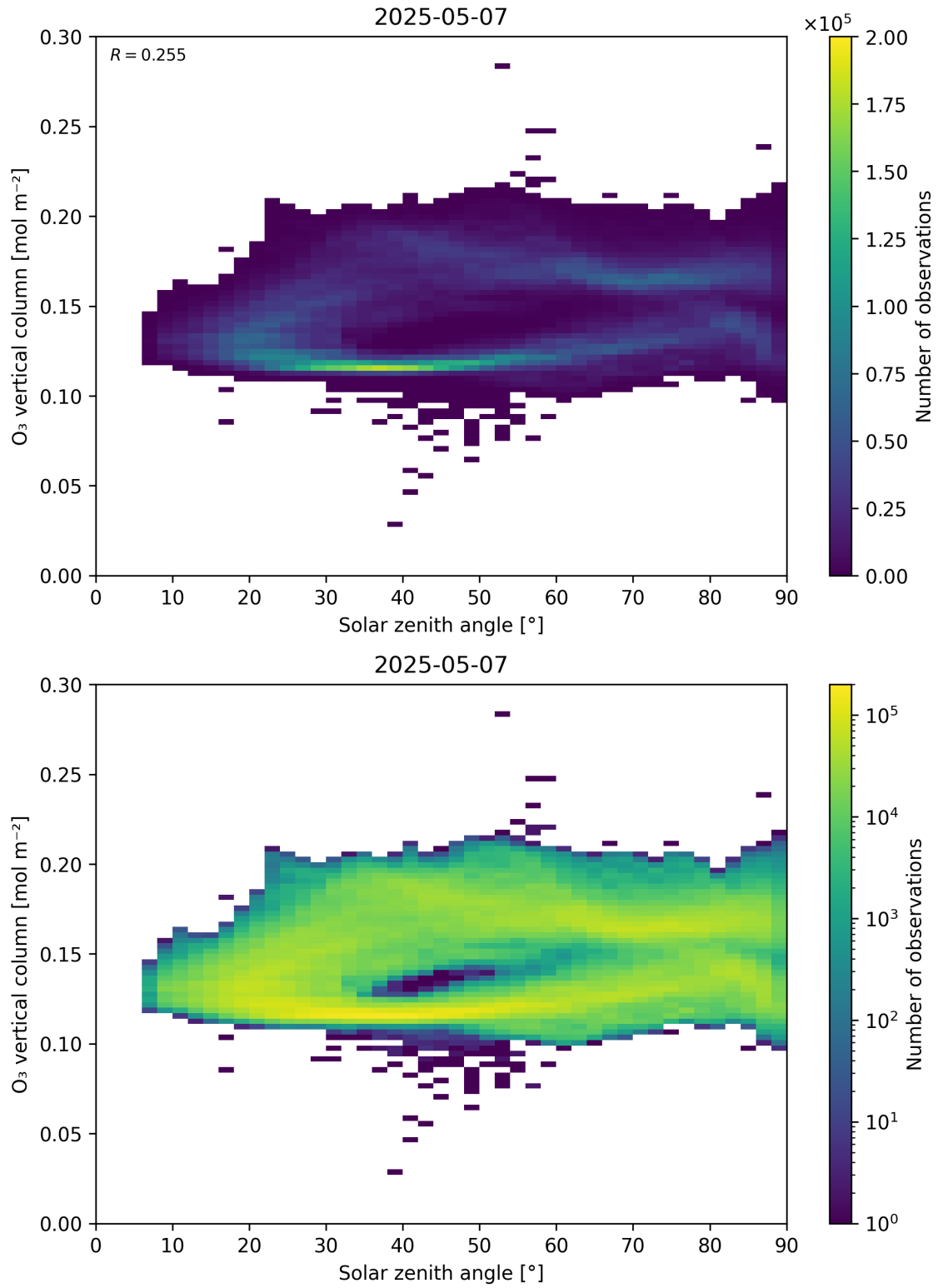
Figure 47: Scatter density plot of “Solar zenith angle” against “O 3 vertical column” for 2025-05-06 to 2025-05-08.
