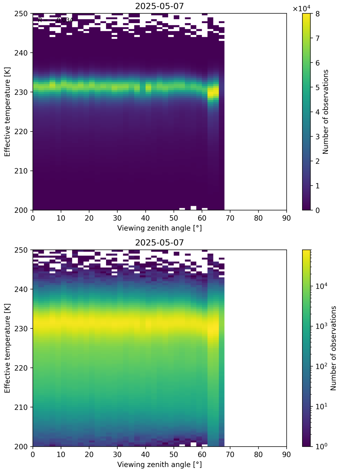
Figure 50: Scatter density plot of “Viewing zenith angle” against “Effective temperature” for 2025-05-06 to 2025-05-08.
