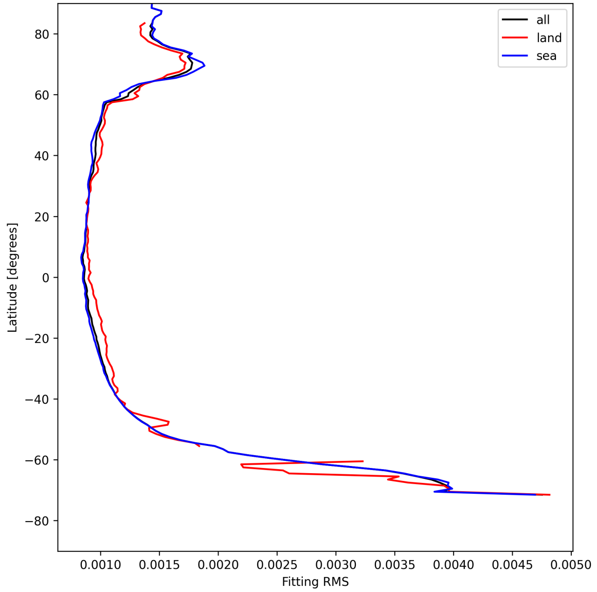
Figure 16: Zonal average of “Fitting RMS” for 2025-05-06 to 2025-05-08.
