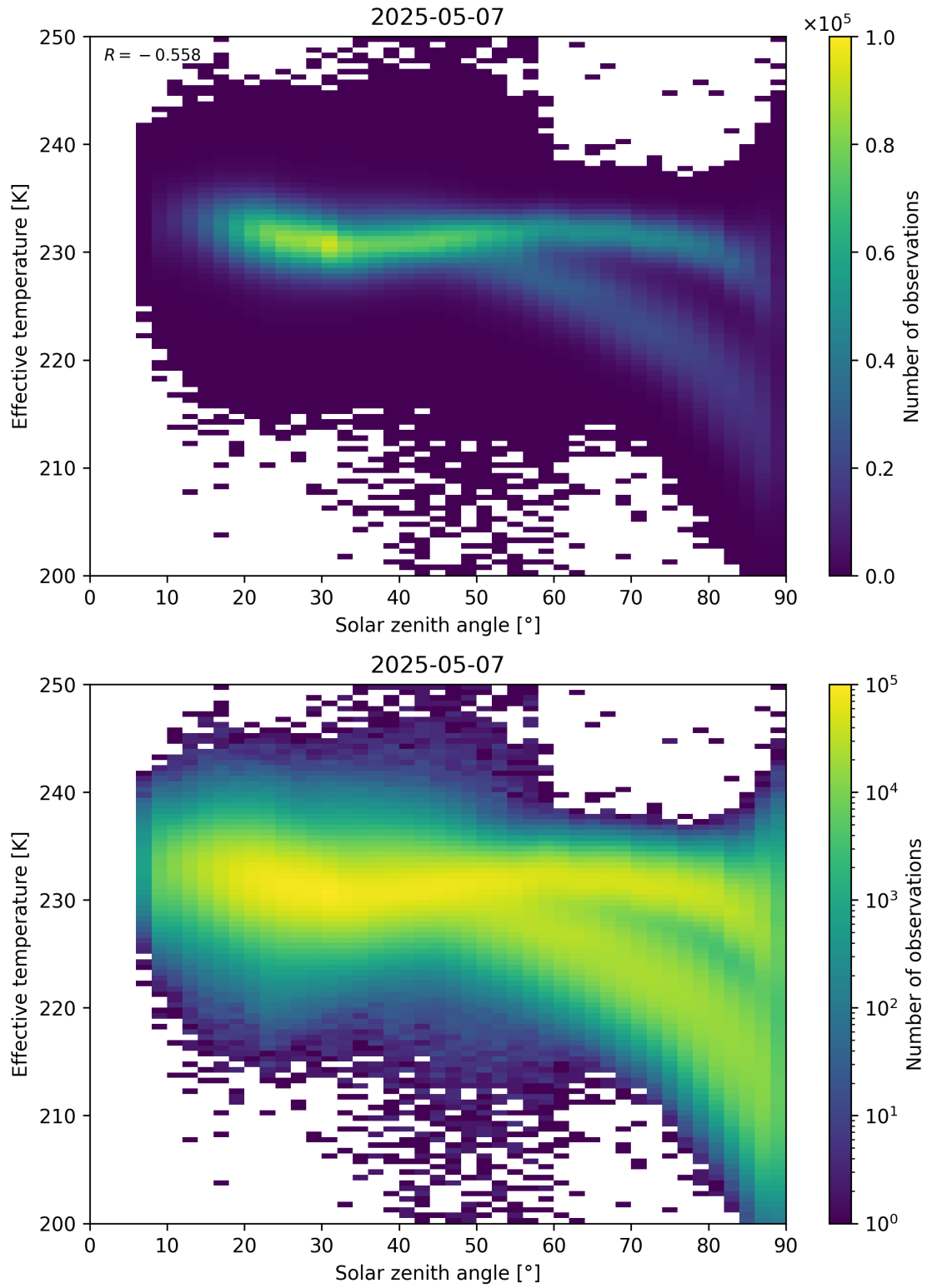
Figure 45: Scatter density plot of “Solar zenith angle” against “Effective temperature” for 2025-05-06 to 2025-05-08.
