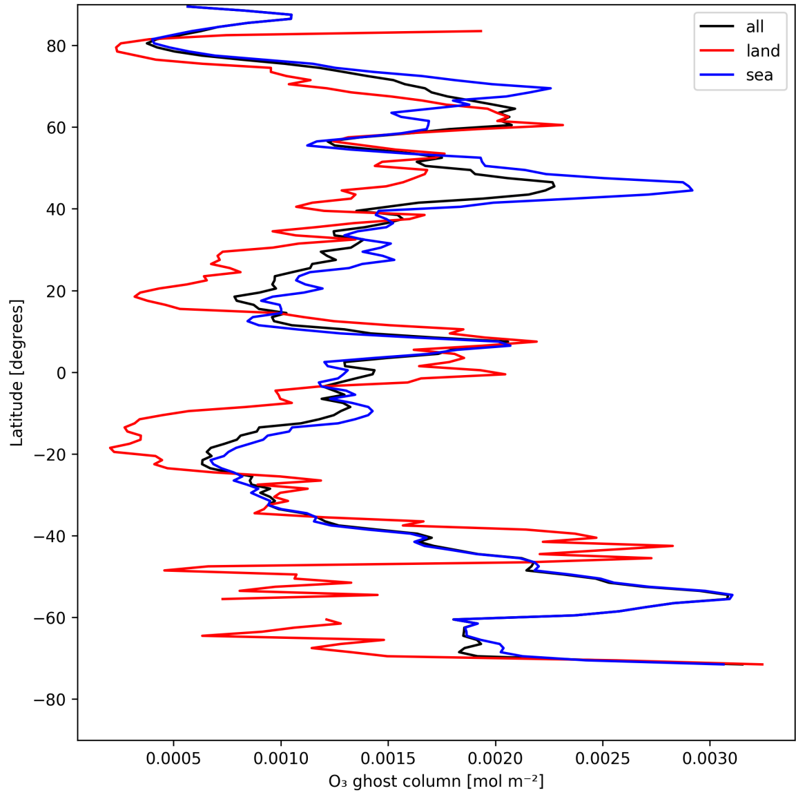
Figure 18: Zonal average of "O 3 ghost column" for 2025-05-06 to 2025-05-08.
