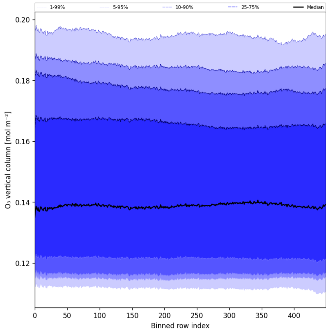
Figure 28: Along track statistics of “ \text{O}_3 vertical column” for 2025-05-06 to 2025-05-08
