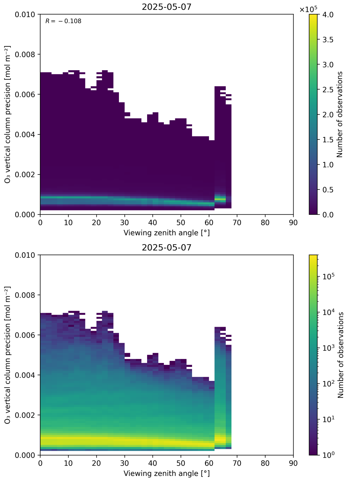
Figure 53: Scatter density plot of “Viewing zenith angle” against “O 3 vertical column precision” for 2025-05-06 to 2025-05-08.
