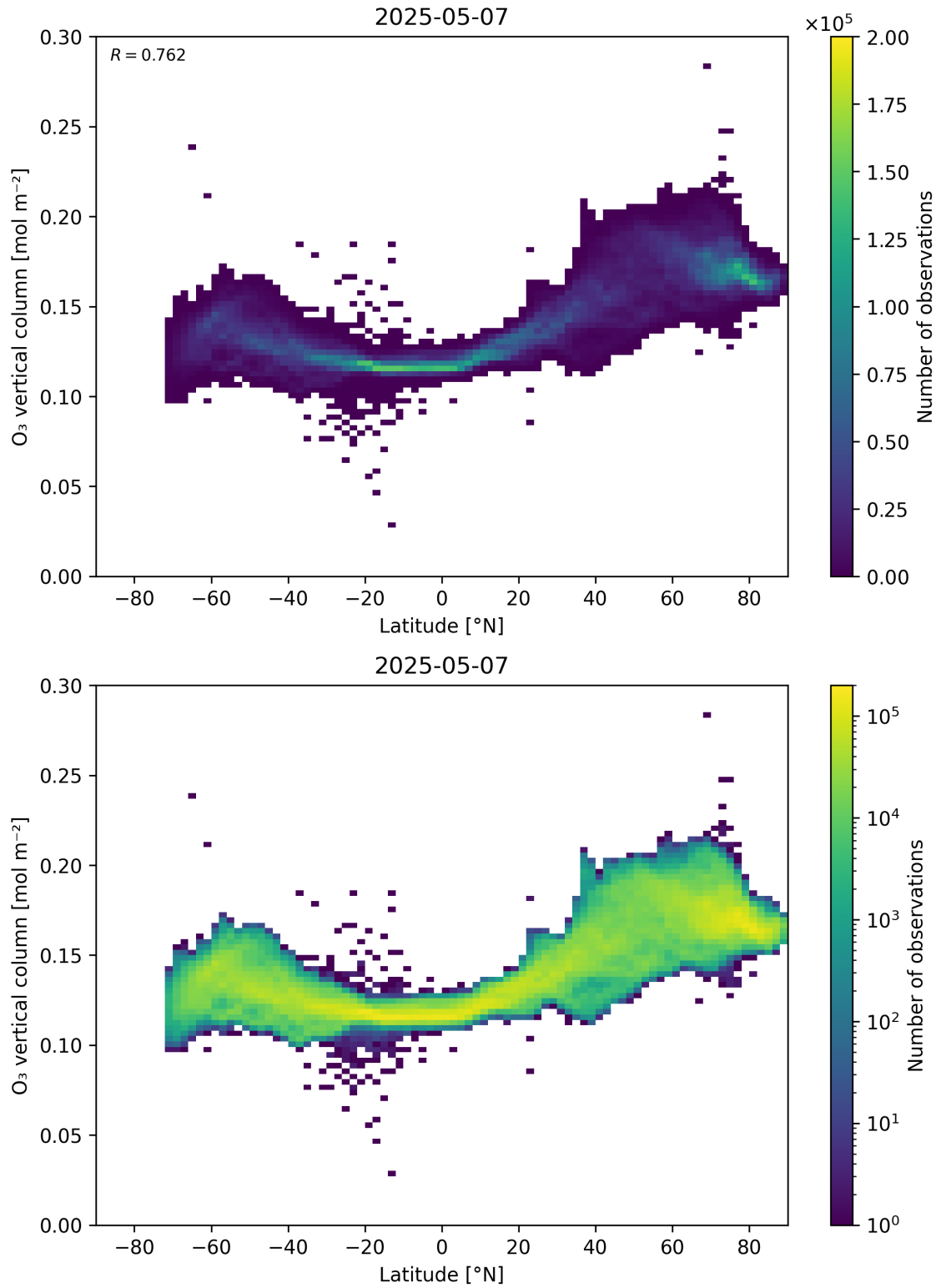
Figure 36: Scatter density plot of “Latitude” against “O 3 vertical column” for 2025-05-06 to 2025-05-08.
