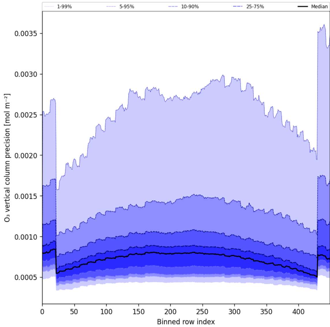
Figure 29: Along track statistics of “O 3 vertical column precision” for 2025-05-06 to 2025-05-08
