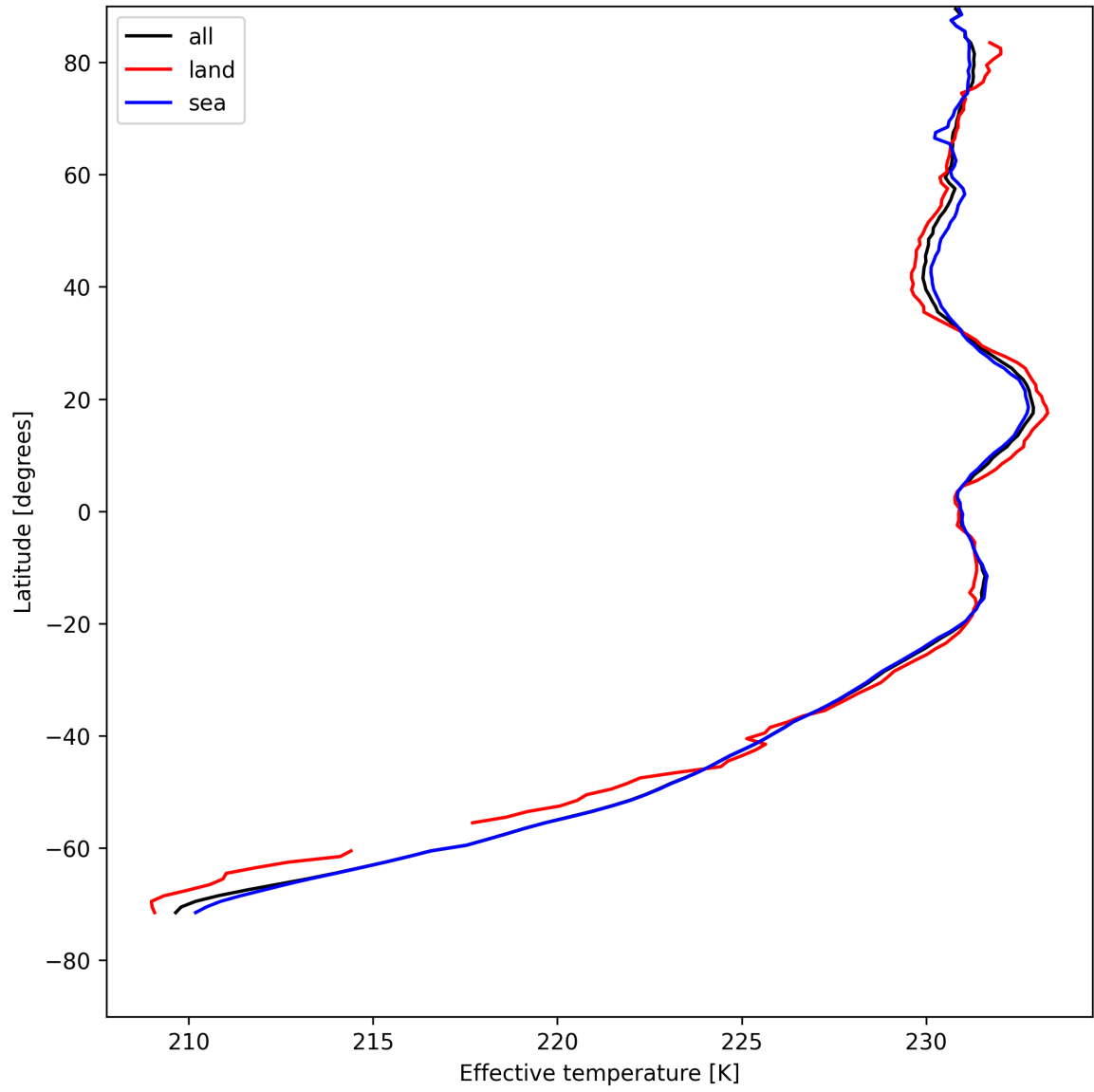
Figure 17: Zonal average of “Effective temperature” for 2025-05-06 to 2025-05-08.
