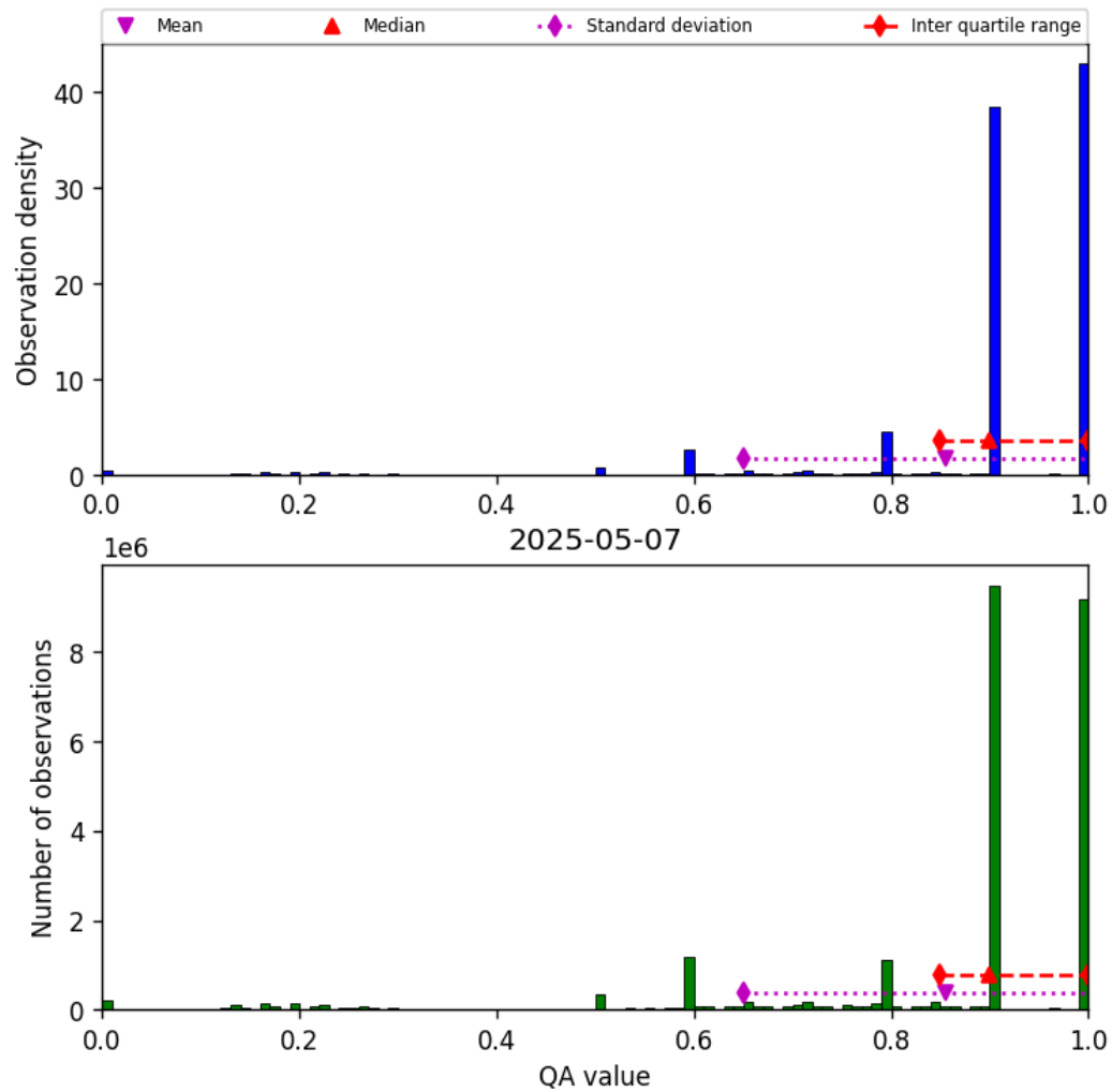
Figure 20: Histogram of “QA value” for 2025-05-06 to 2025-05-08
