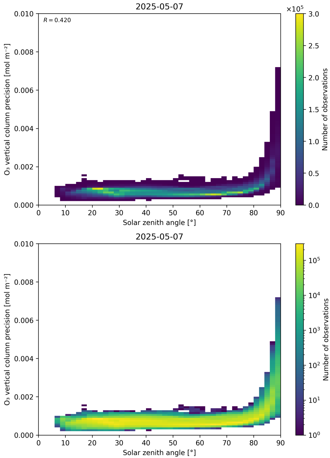
Figure 48: Scatter density plot of “Solar zenith angle” against “O 3 vertical column precision” for 2025-05-06 to 2025-05-08.
