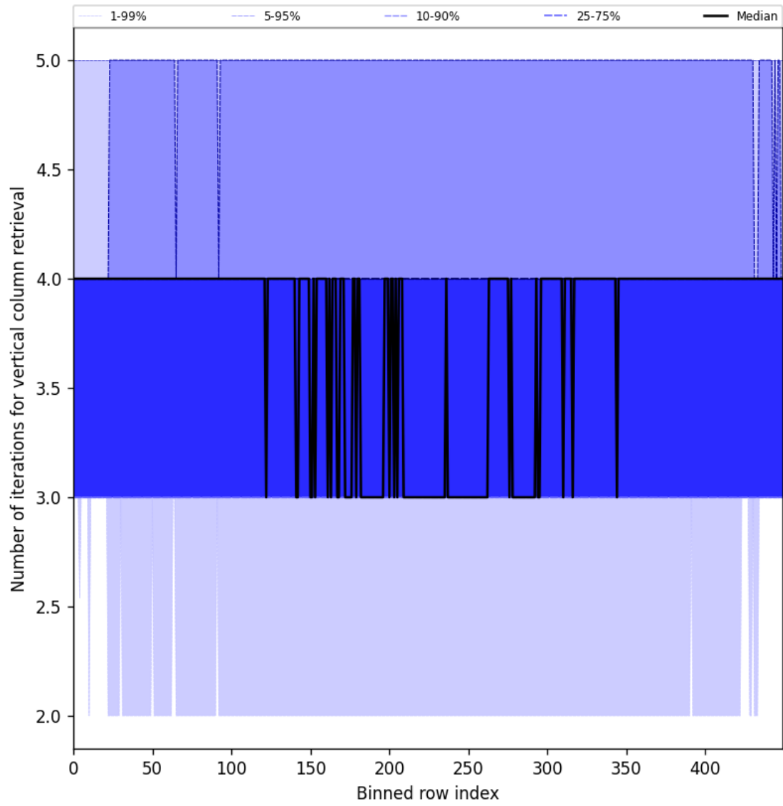
Figure 33: Along track statistics of “Number of iterations for vertical column retrieval” for 2025-05-06 to 2025-05-08
