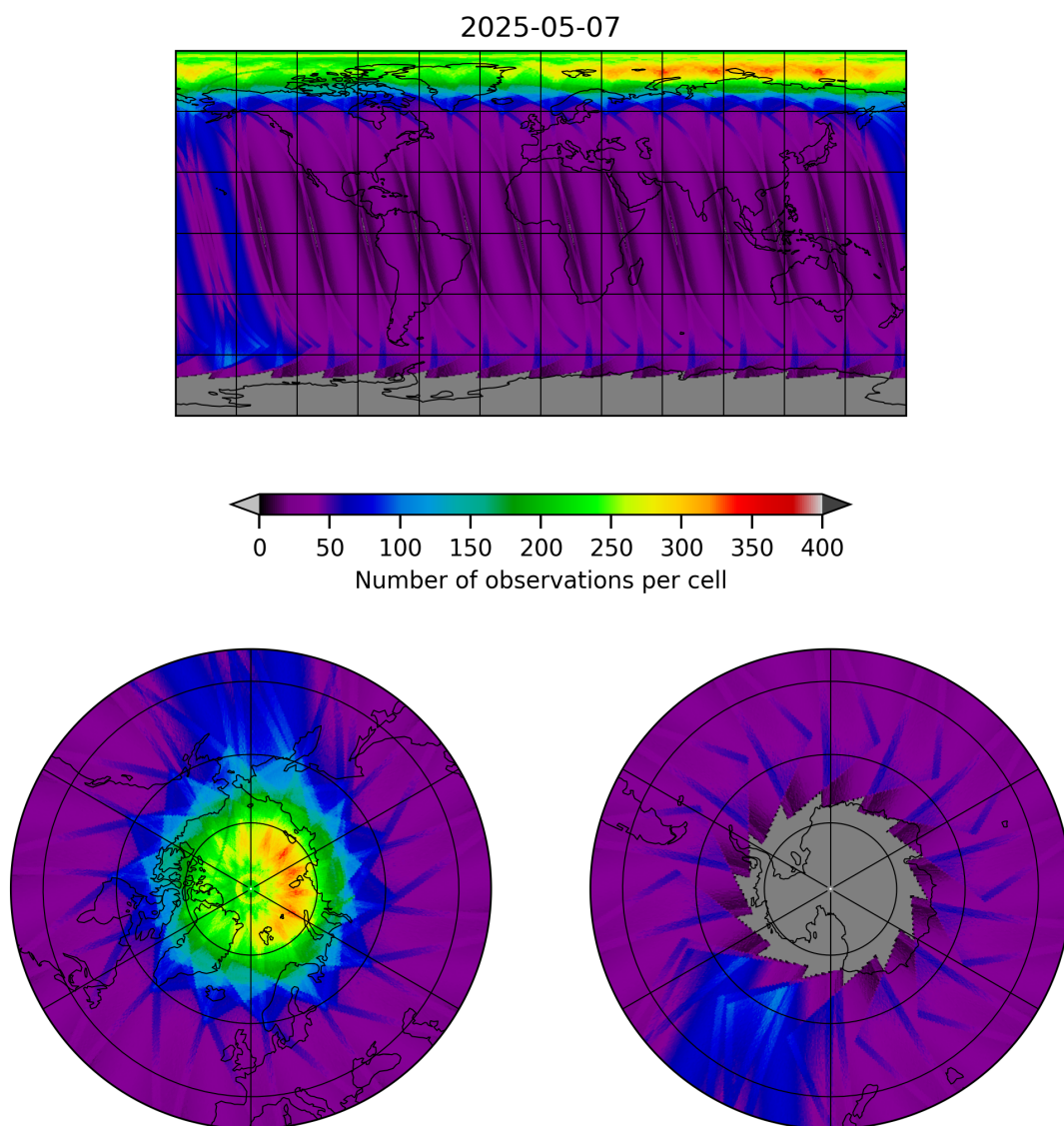
Figure 12: Map of the number of observations for 2025-05-06 to 2025-05-08
