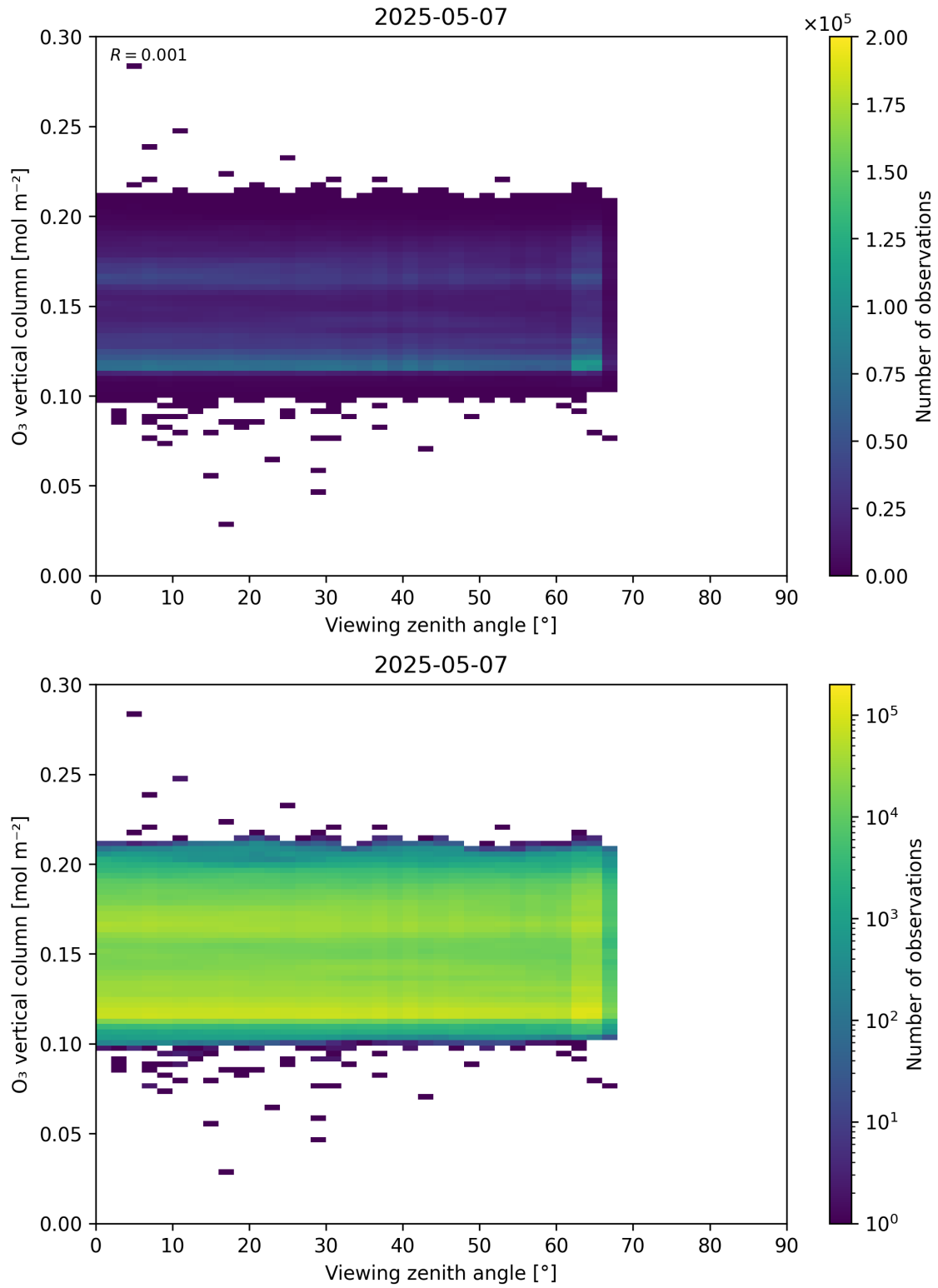
Figure 52: Scatter density plot of “Viewing zenith angle” against “O 3 vertical column” for 2025-05-06 to 2025-05-08.
