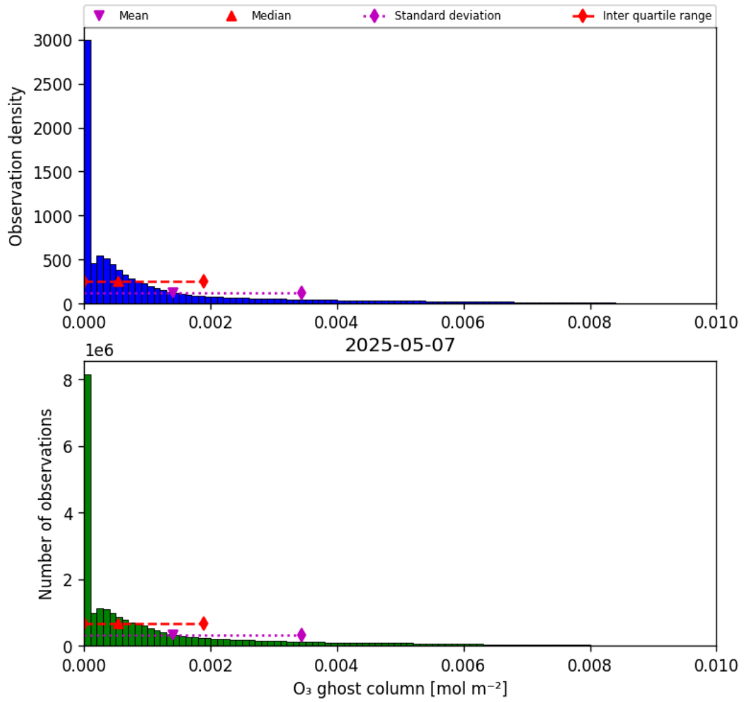
Figure 25: Histogram of “O 3 ghost column” for 2025-05-06 to 2025-05-08
