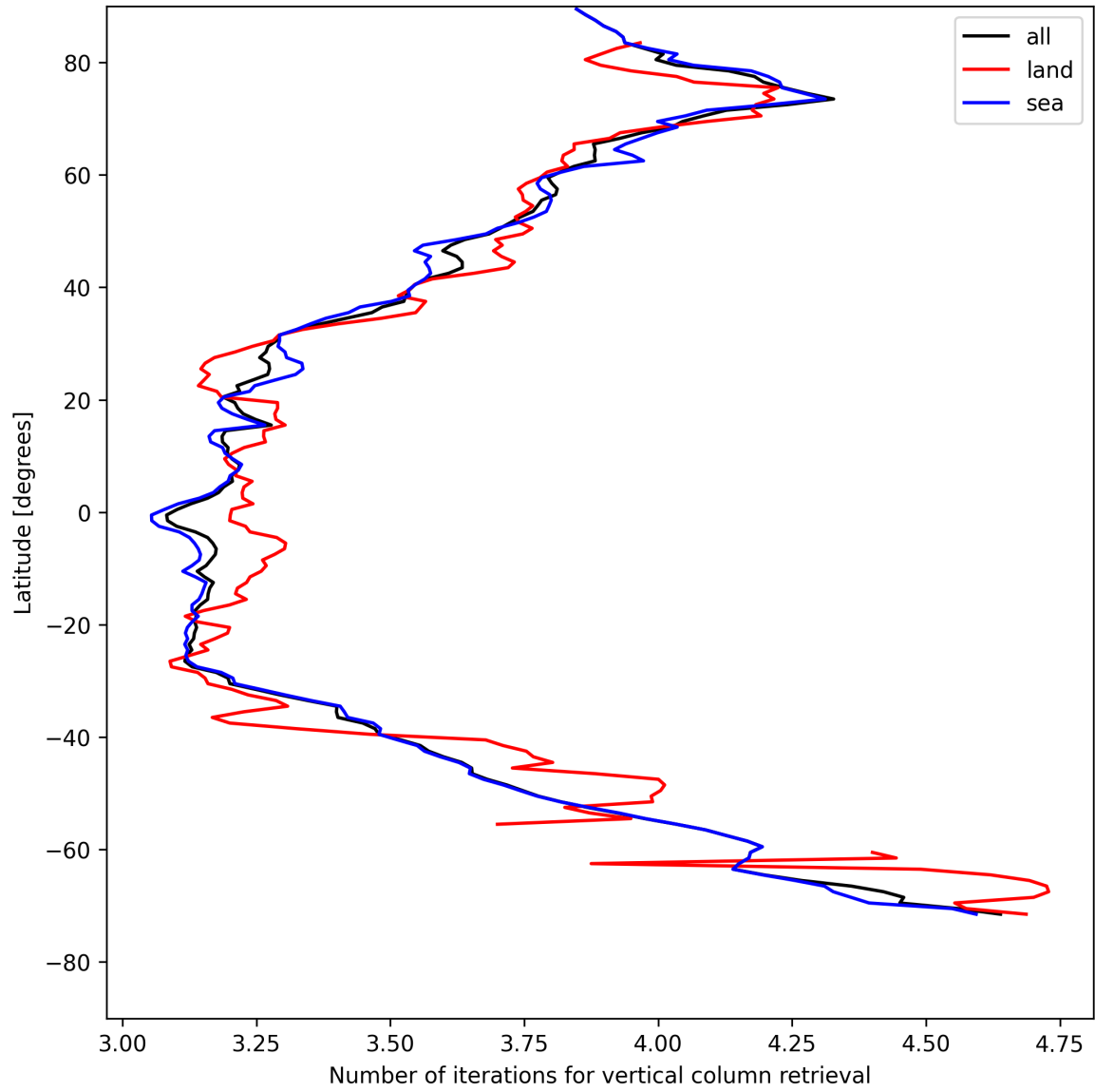
Figure 19: Zonal average of “Number of iterations for vertical column retrieval” for 2025-05-06 to 2025-05-08.
