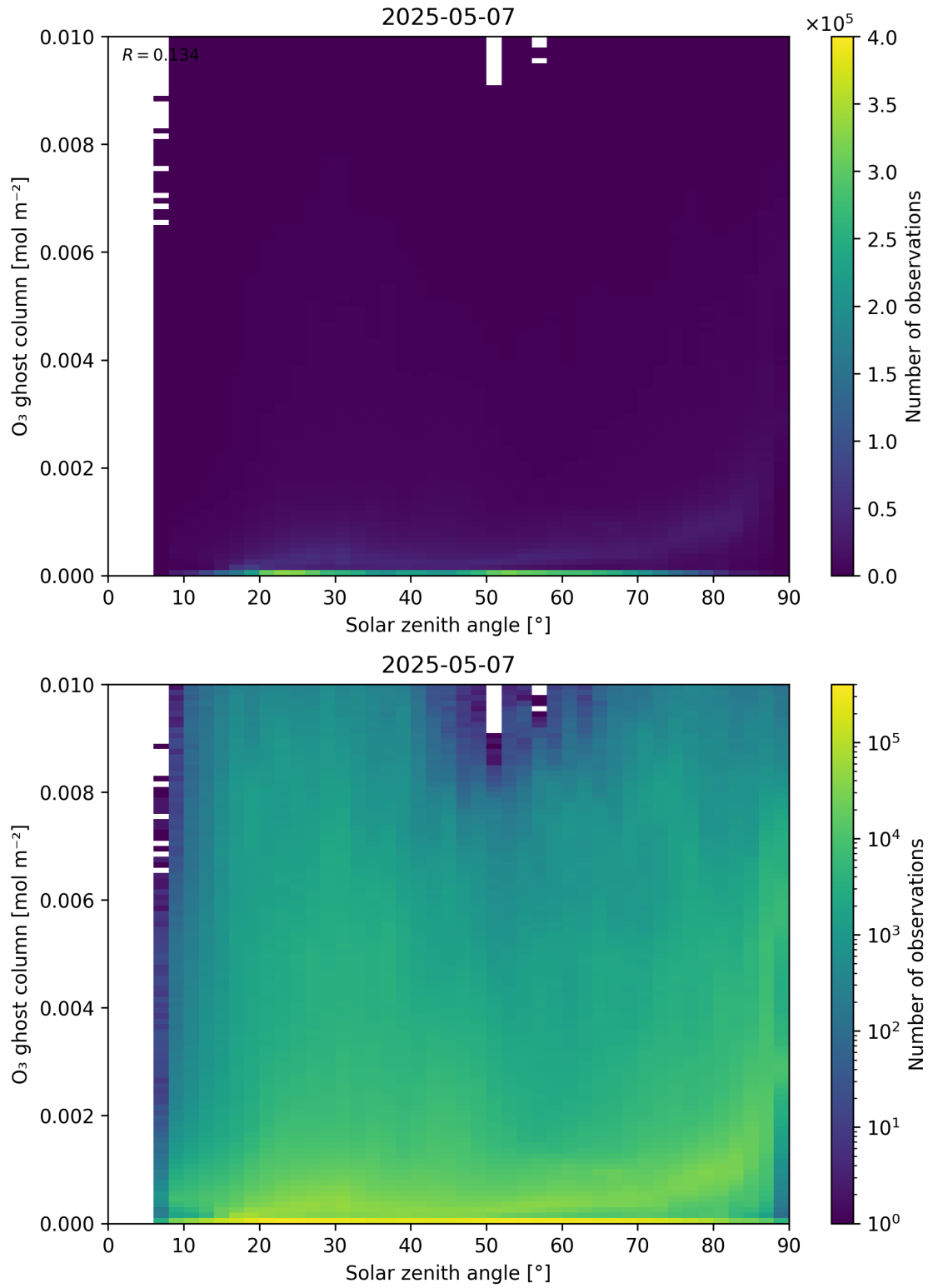
Figure 46: Scatter density plot of “Solar zenith angle” against “O 3 ghost column” for 2025-05-06 to 2025-05-08.
