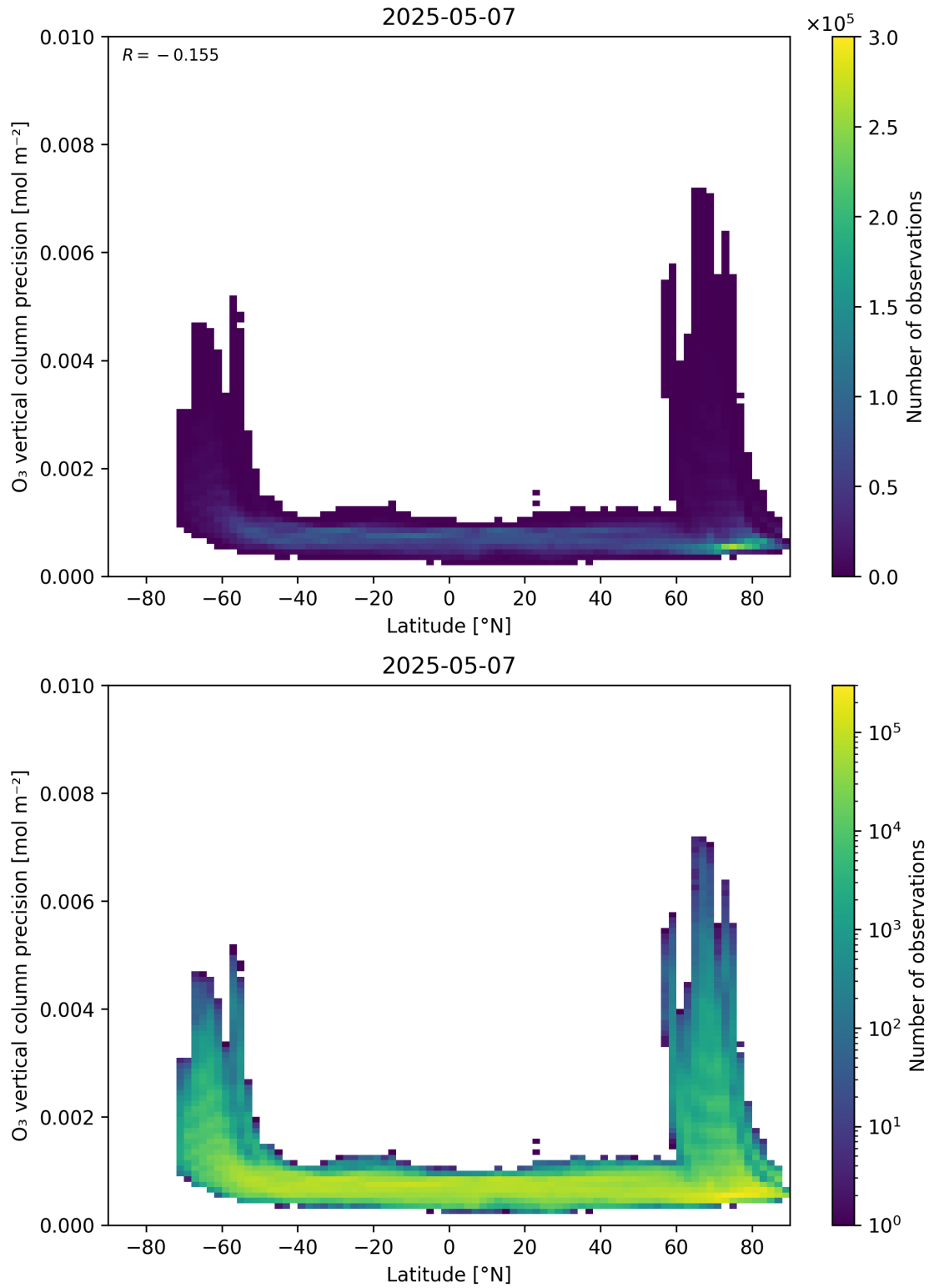
Figure 37: Scatter density plot of “Latitude” against “O 3 vertical column precision” for 2025-05-06 to 2025-05-08.
