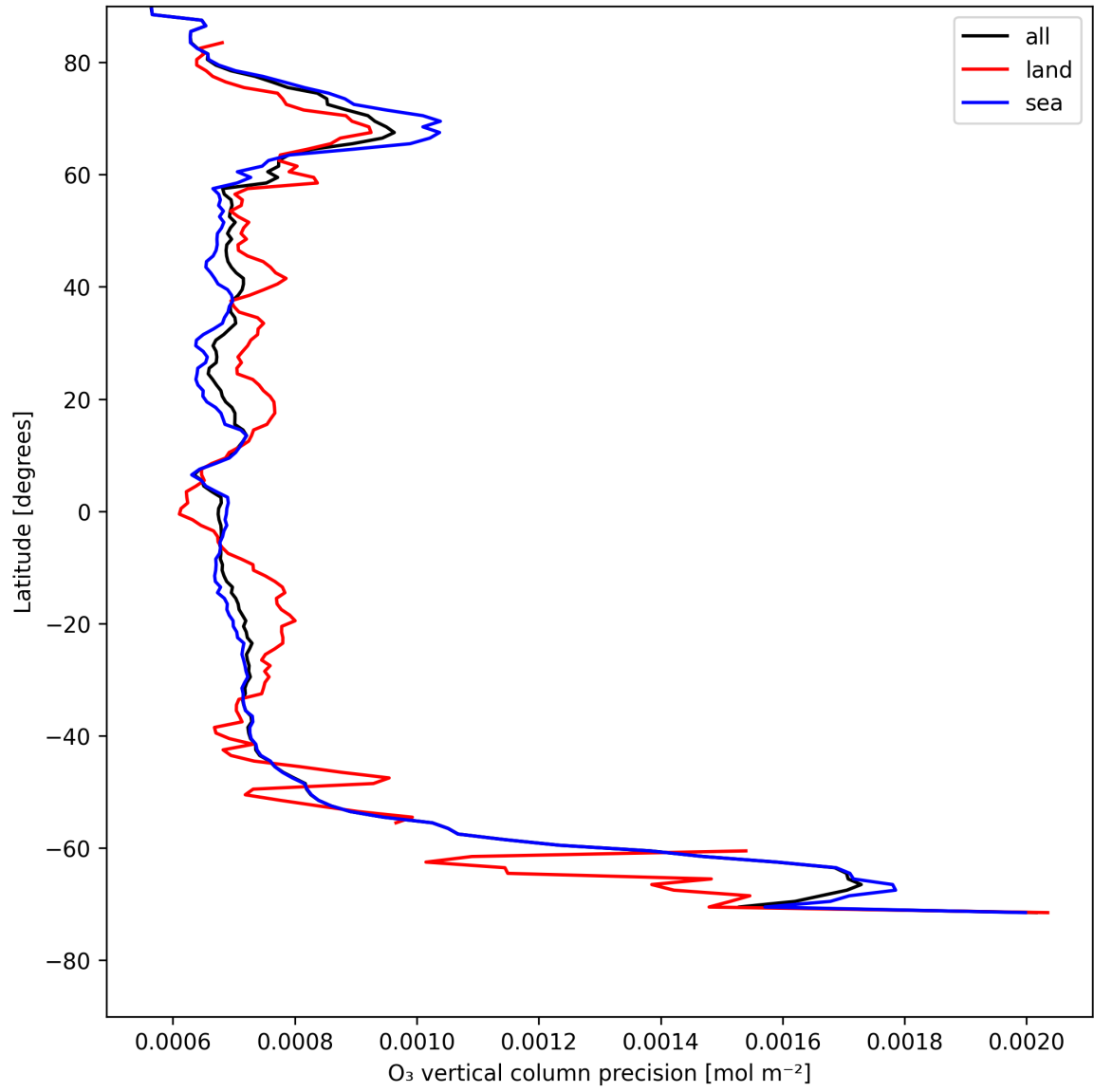
Figure 15: Zonal average of “O 3 vertical column precision” for 2025-05-06 to 2025-05-08.
