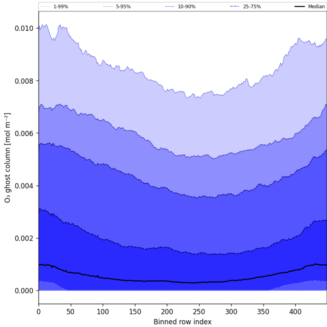
Figure 32: Along track statistics of “O 3 ghost column” for 2025-05-06 to 2025-05-08
