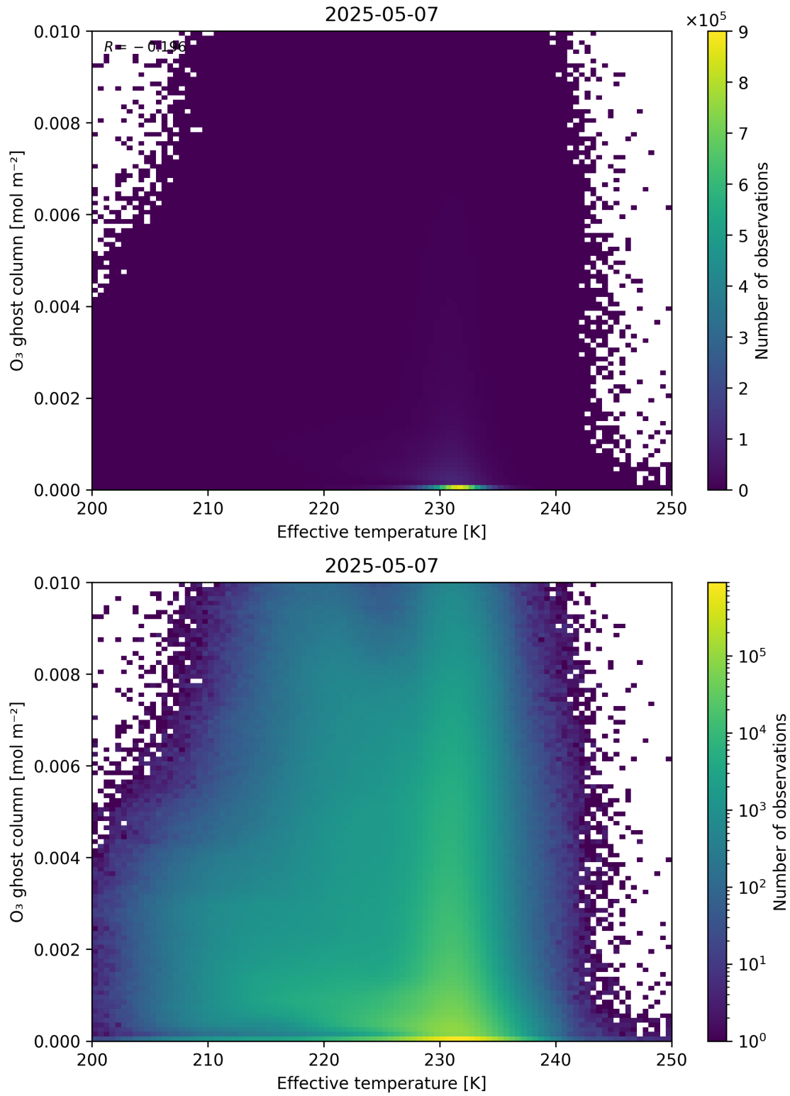
Figure 38: Scatter density plot of “Effective temperature” against “O 3 ghost column” for 2025-05-06 to 2025-05-08.
