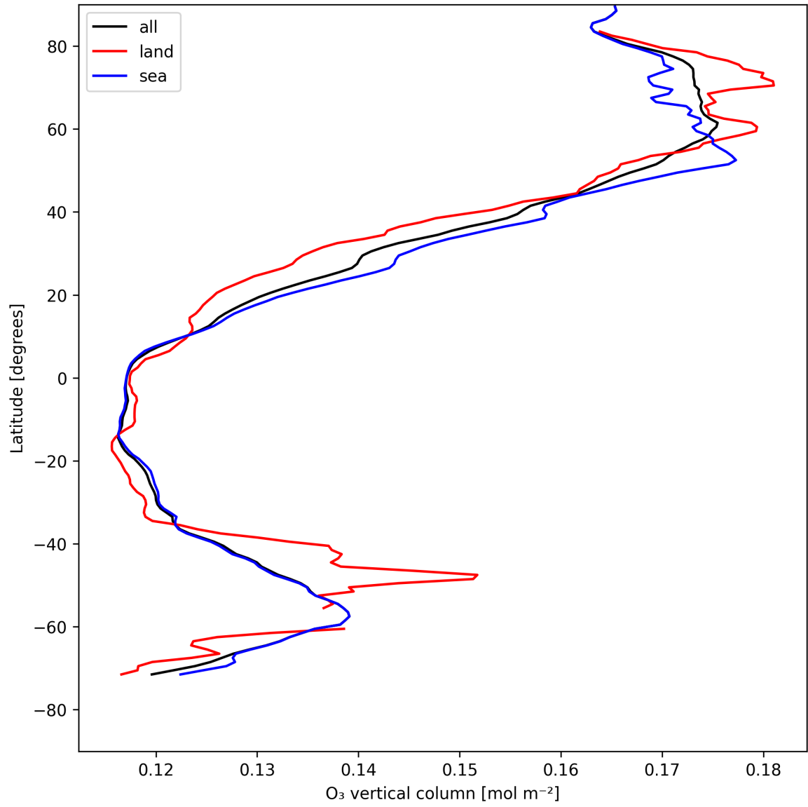
Figure 14: Zonal average of “O 3 vertical column” for 2025-05-06 to 2025-05-08.
