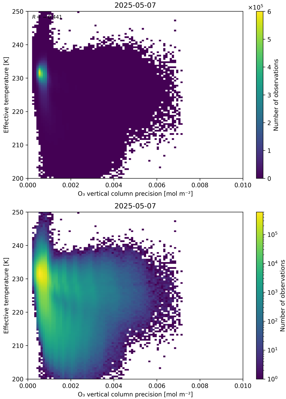
Figure 42: Scatter density plot of “O 3 vertical column precision” against “Effective temperature” for 2025-05-06 to 2025-05-08.
