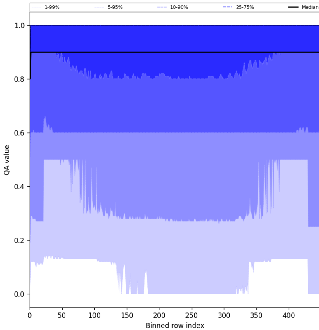
Figure 27: Along track statistics of “QA value” for 2025-05-06 to 2025-05-08
