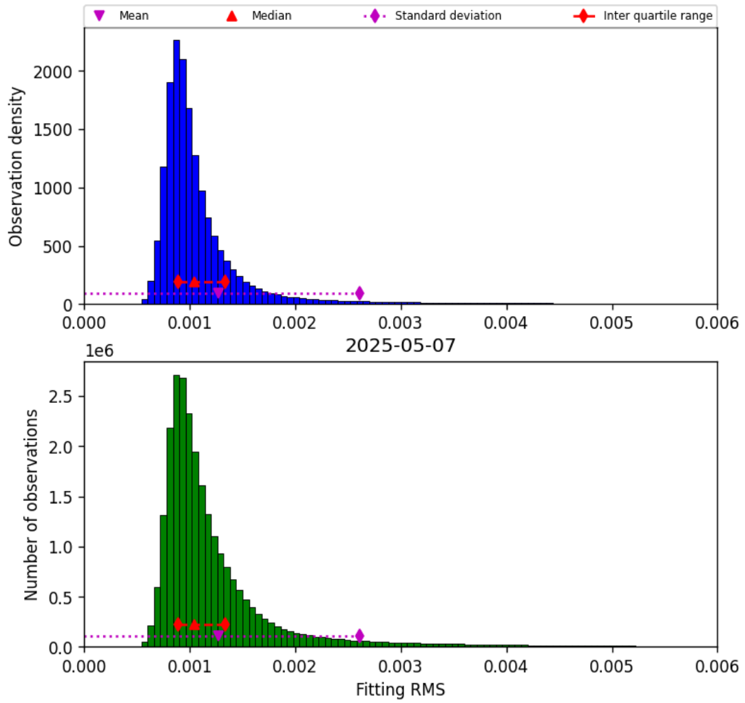
Figure 23: Histogram of “Fitting RMS” for 2025-05-06 to 2025-05-08
