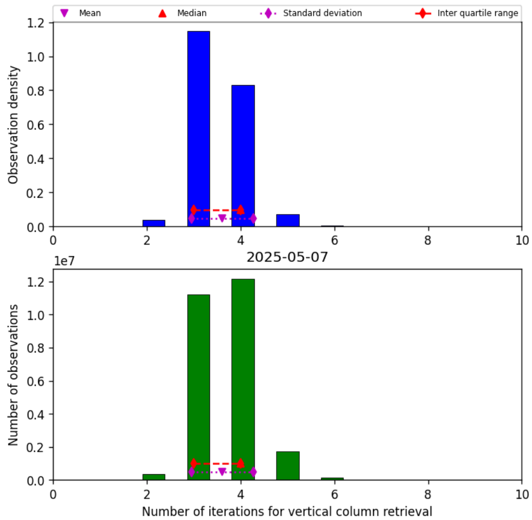
Figure 26: Histogram of “Number of iterations for vertical column retrieval” for 2025-05-06 to 2025-05-08
