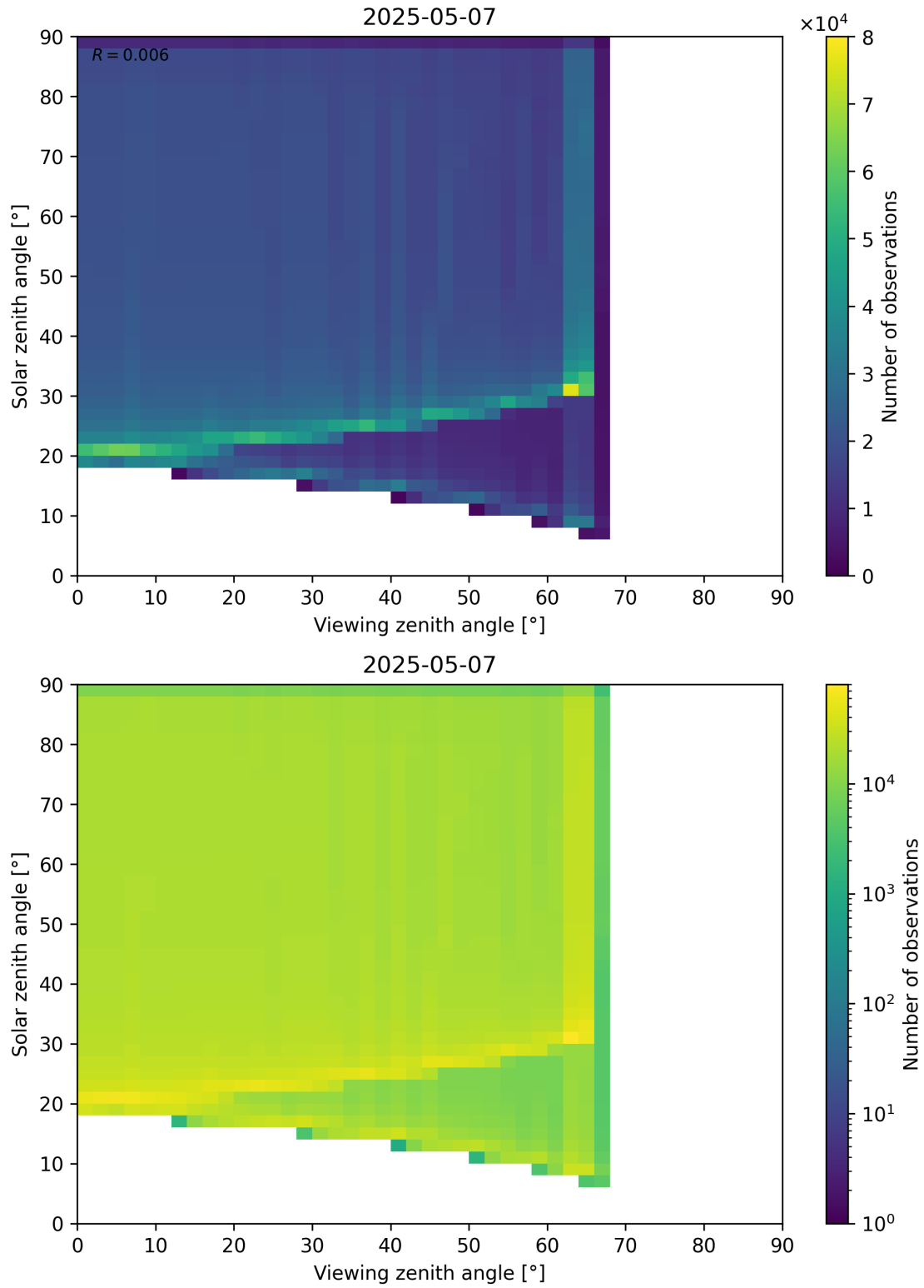
Figure 54: Scatter density plot of “Viewing zenith angle” against “Solar zenith angle” for 2025-05-06 to 2025-05-08.
