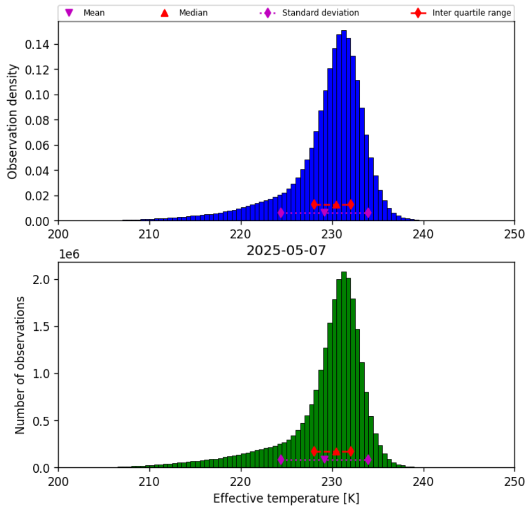
Figure 24: Histogram of “Effective temperature” for 2025-05-06 to 2025-05-08
