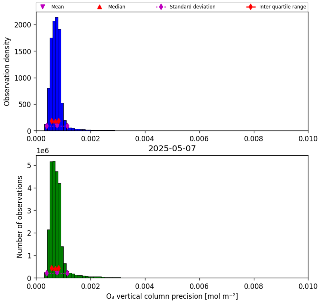
Figure 22: Histogram of “O 3 vertical column precision” for 2025-05-06 to 2025-05-08
