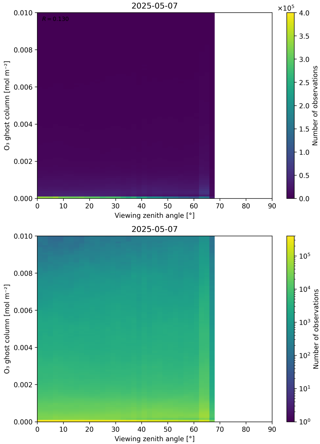
Figure 51: Scatter density plot of “Viewing zenith angle” against “O 3 ghost column” for 2025-05-06 to 2025-05-08.
