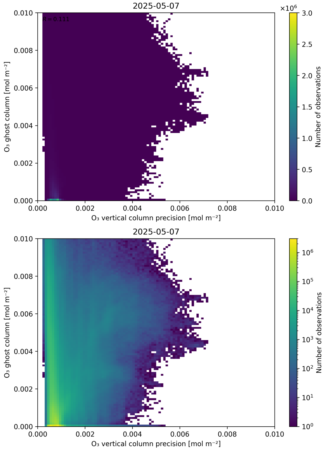
Figure 43: Scatter density plot of “O 3 vertical column precision” against “O 3 ghost column” for 2025-05-06 to 2025-05-08.
