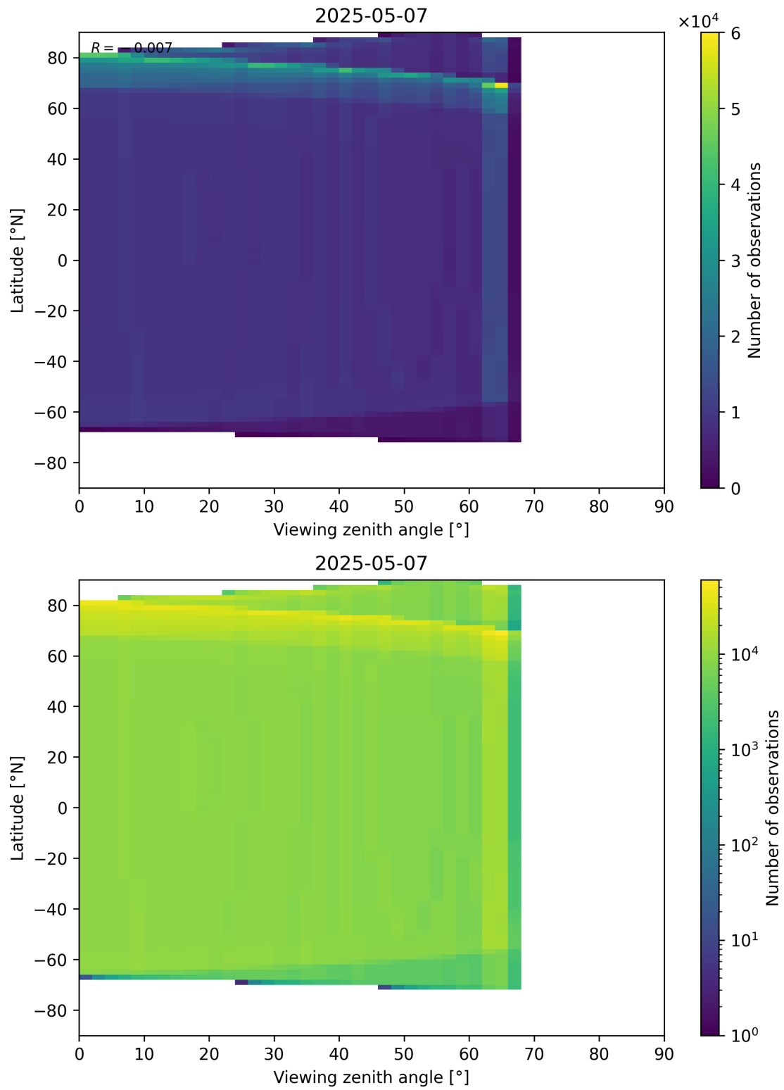
Figure 49: Scatter density plot of “Viewing zenith angle” against “Latitude” for 2025-05-06 to 2025-05-08.
