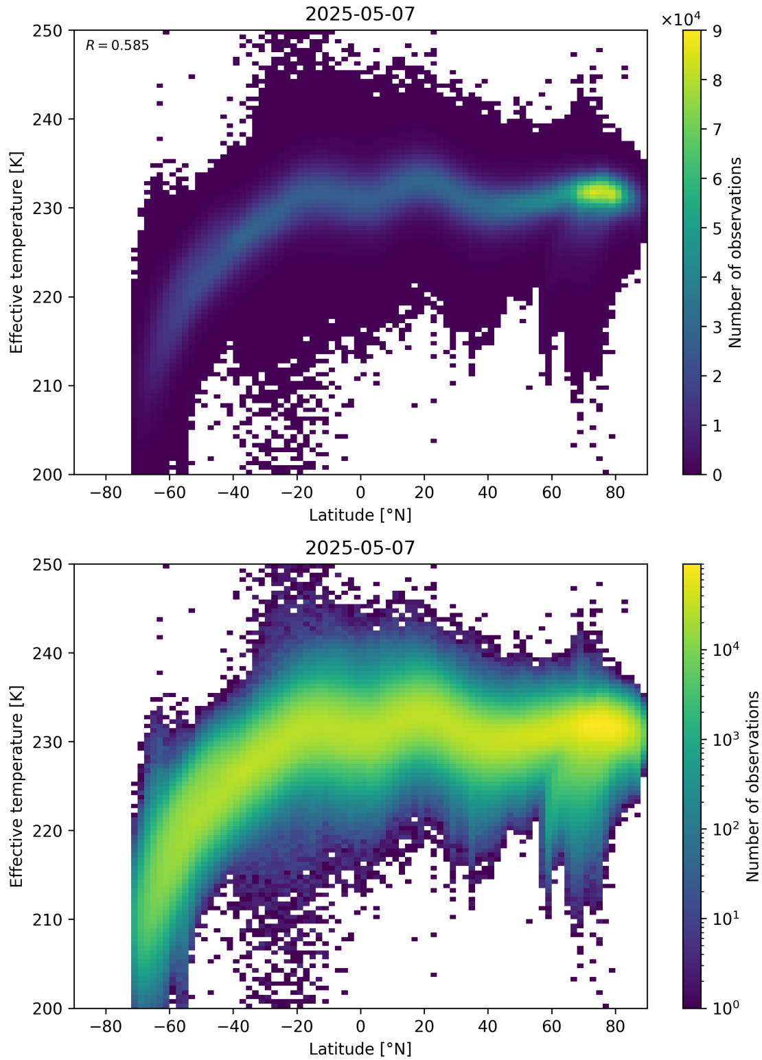
Figure 34: Scatter density plot of “Latitude” against “Effective temperature” for 2025-05-06 to 2025-05-08.
