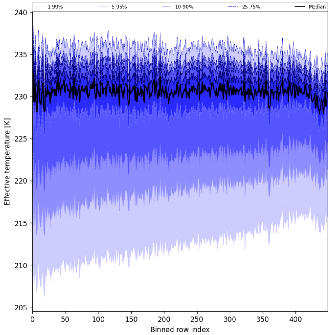
Figure 31: Along track statistics of “Effective temperature” for 2025-05-06 to 2025-05-08
