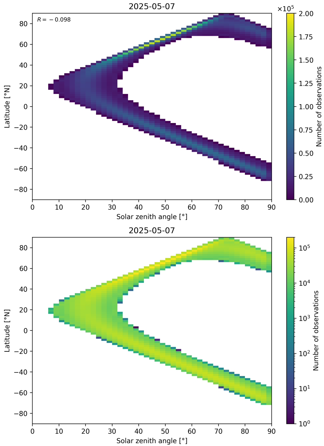
Figure 44: Scatter density plot of “Solar zenith angle” against “Latitude” for 2025-05-06 to 2025-05-08.
