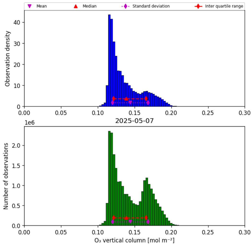
Figure 21: Histogram of “O 3 vertical column” for 2025-05-06 to 2025-05-08
