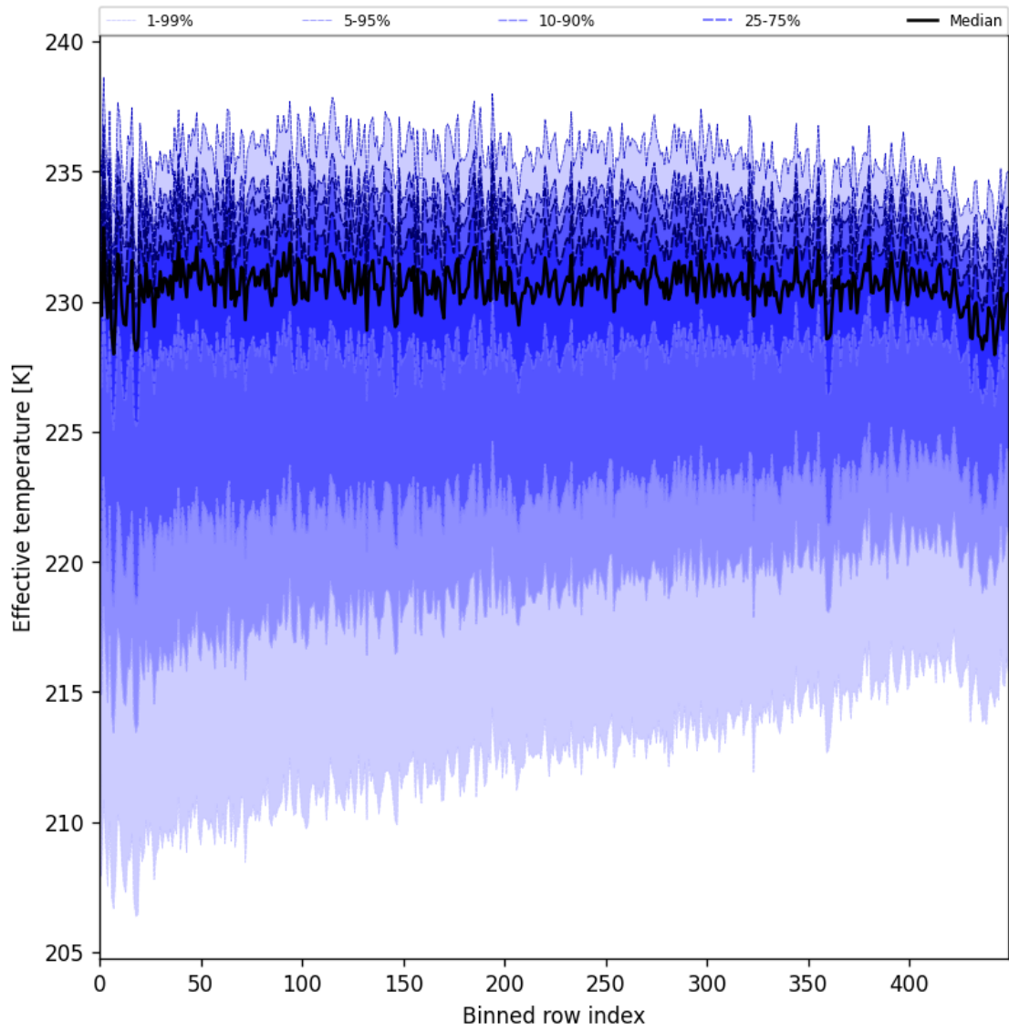
Figure 31: Along track statistics of “Effective temperature” for 2025-05-07 to 2025-05-09
