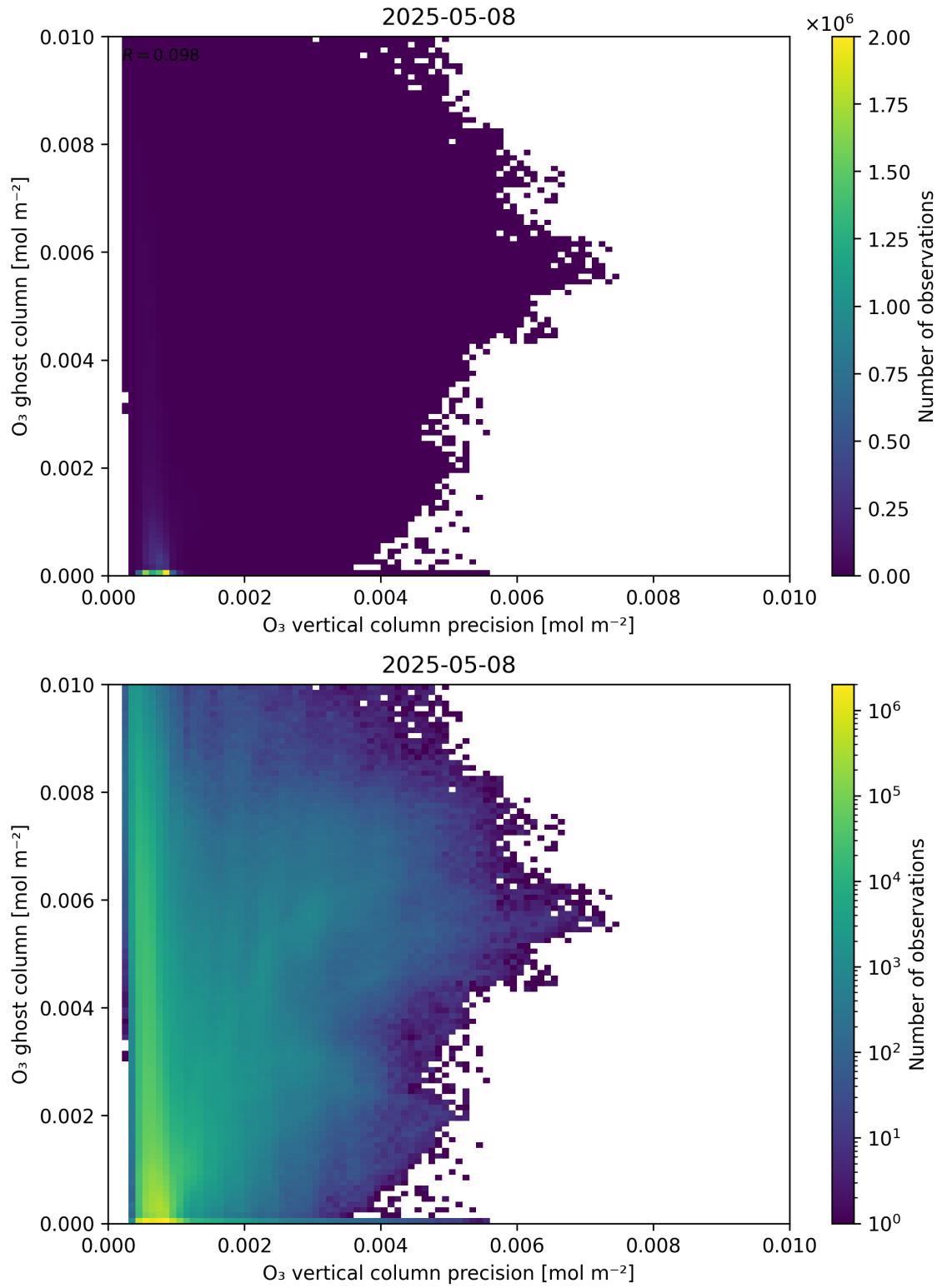
Figure 43: Scatter density plot of “O 3 vertical column precision” against “O 3 ghost column” for 2025-05-07 to 2025-05-09.
