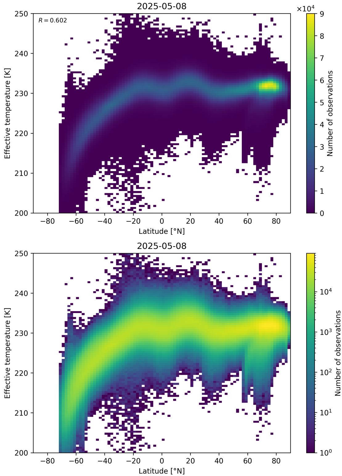
Figure 34: Scatter density plot of “Latitude” against “Effective temperature” for 2025-05-07 to 2025-05-09.
