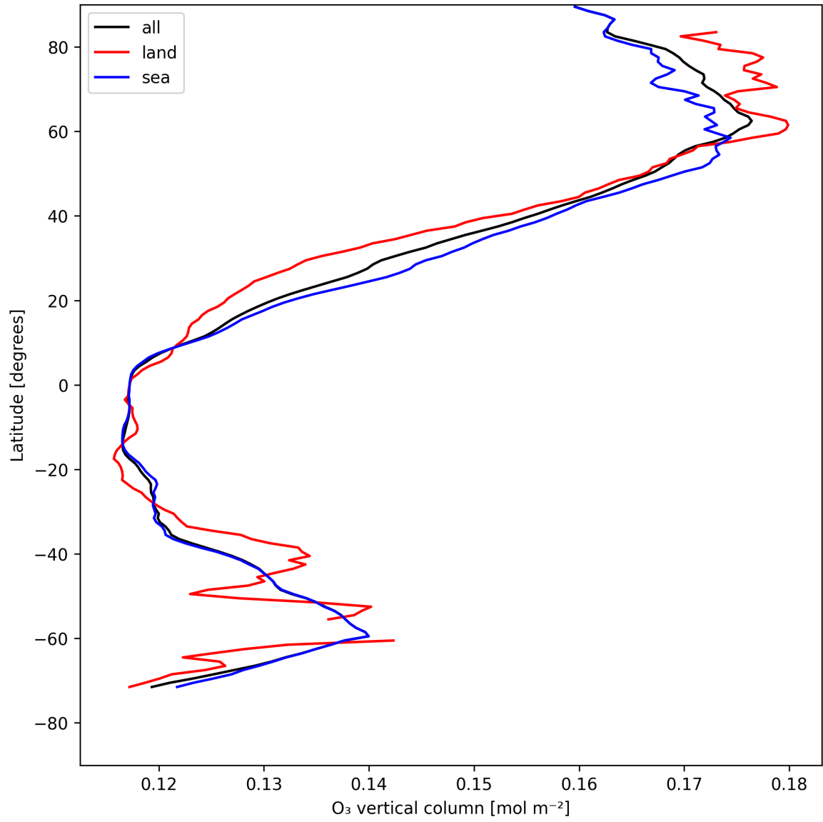
Figure 14: Zonal average of “O 3 vertical column” for 2025-05-07 to 2025-05-09.
