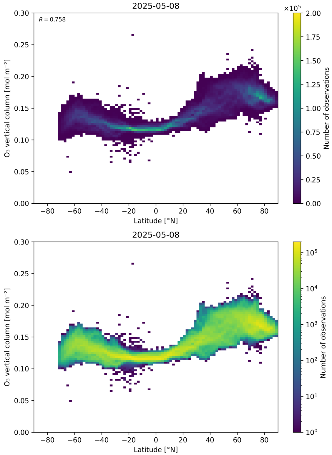
Figure 36: Scatter density plot of “Latitude” against “O 3 vertical column” for 2025-05-07 to 2025-05-09.
