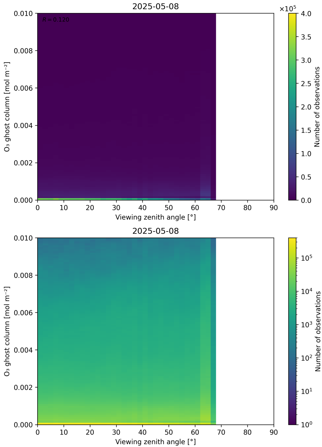
Figure 51: Scatter density plot of “Viewing zenith angle” against “O 3 ghost column” for 2025-05-07 to 2025-05-09.
