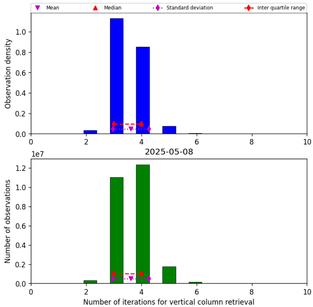
Figure 26: Histogram of “Number of iterations for vertical column retrieval” for 2025-05-07 to 2025-05-09
