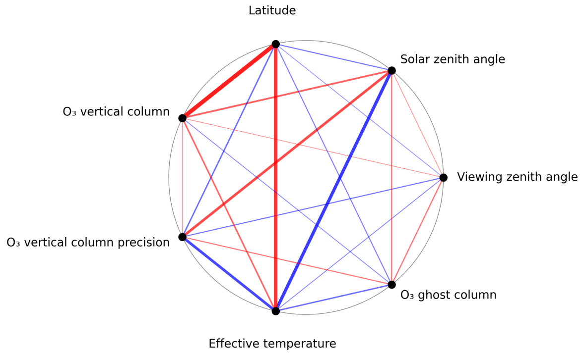
Figure 1: Map of correlation graph for 2025-05-07 to 2025-05-09.
