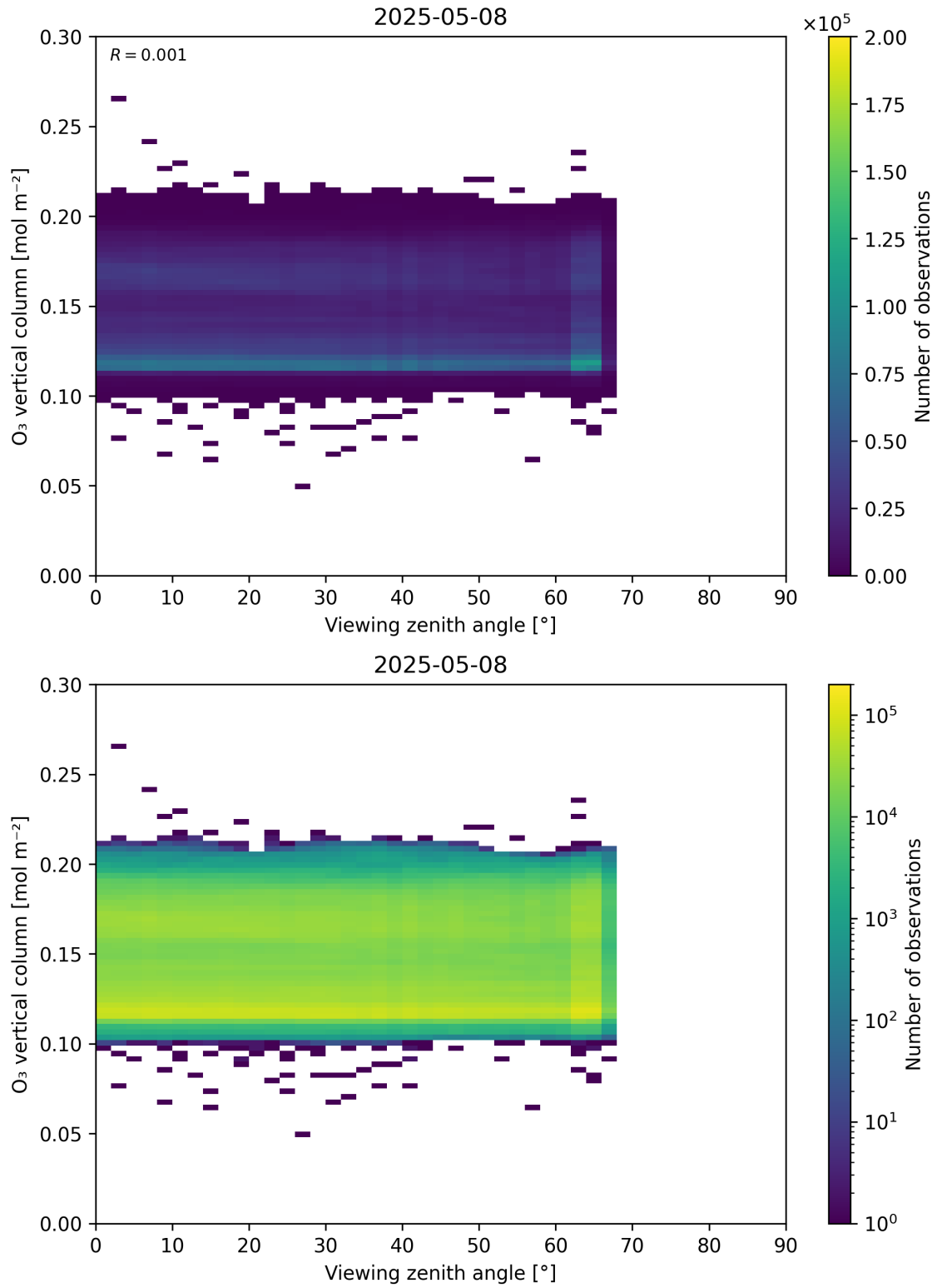
Figure 52: Scatter density plot of “Viewing zenith angle” against “O 3 vertical column” for 2025-05-07 to 2025-05-09.
