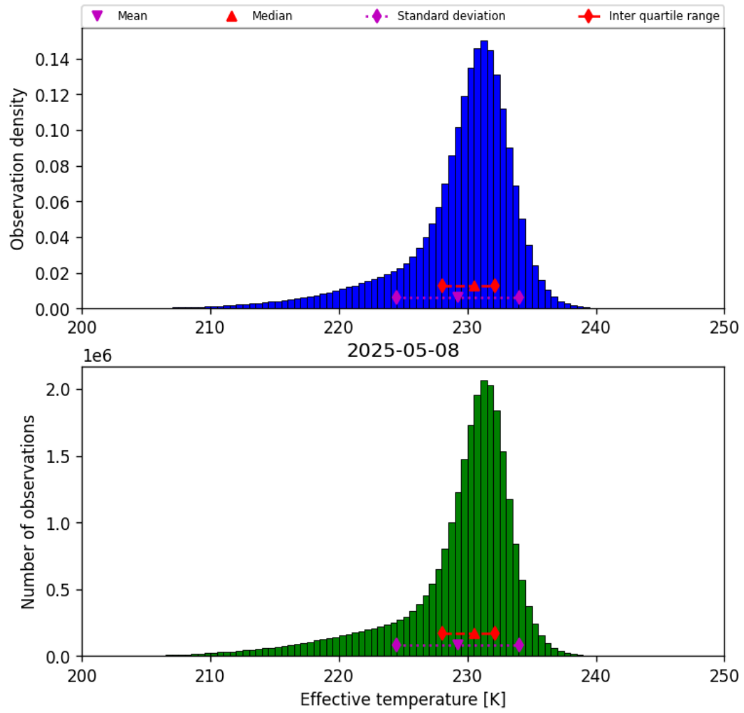
Figure 24: Histogram of “Effective temperature” for 2025-05-07 to 2025-05-09
