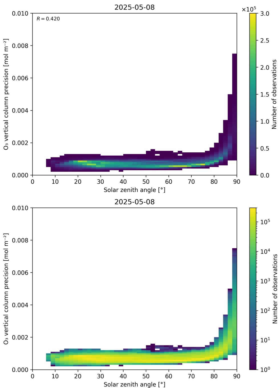
Figure 48: Scatter density plot of “Solar zenith angle” against “O 3 vertical column precision” for 2025-05-07 to 2025-05-09.
