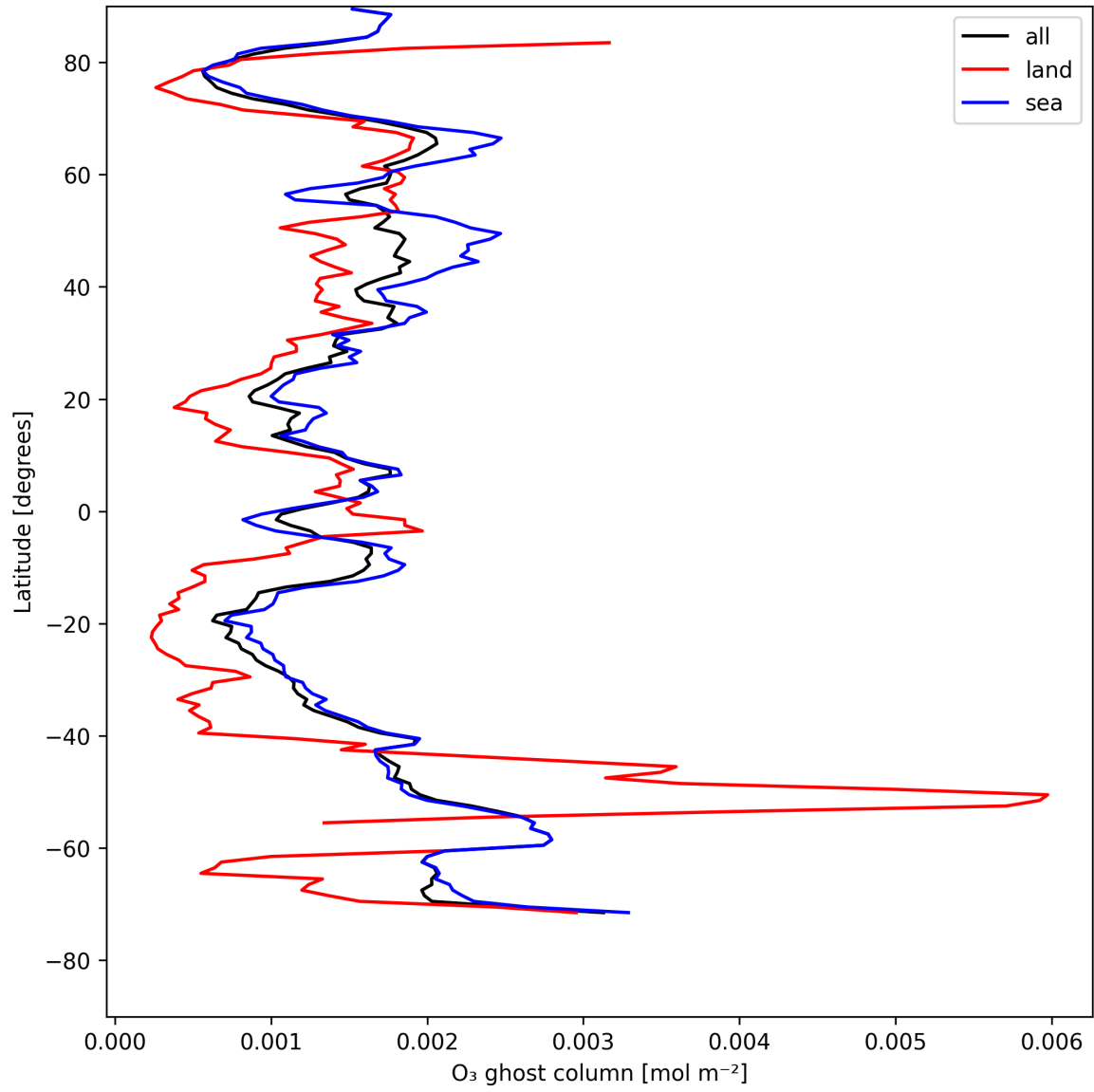
Figure 18: Zonal average of "O 3 ghost column" for 2025-05-07 to 2025-05-09.
