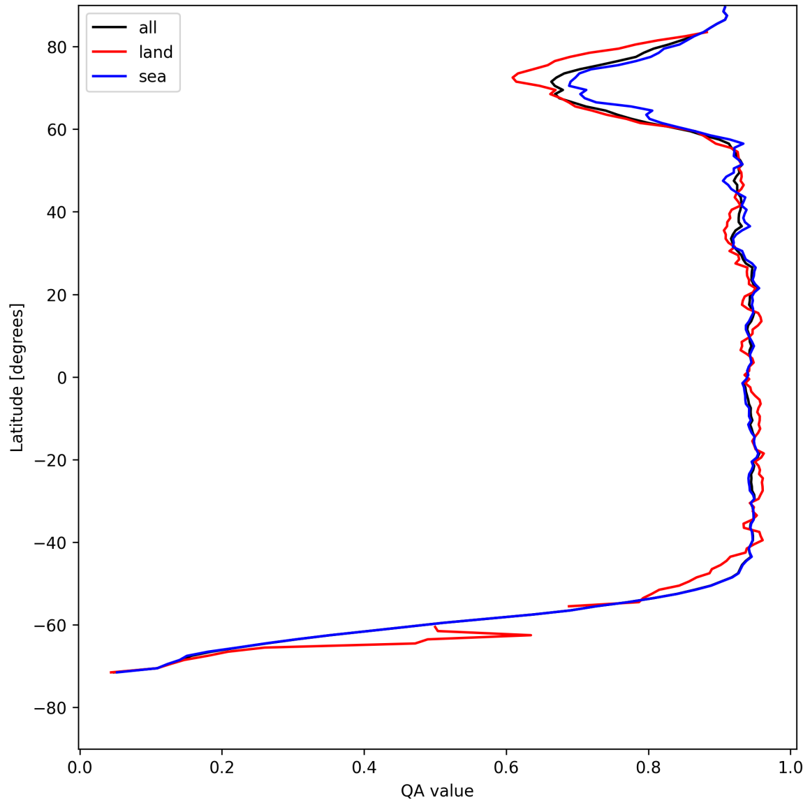
Figure 13: Zonal average of “QA value” for 2025-05-07 to 2025-05-09.
