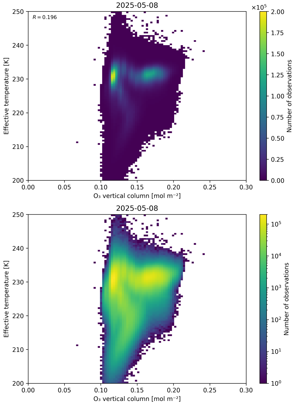
Figure 39: Scatter density plot of “O 3 vertical column” against “Effective temperature” for 2025-05-07 to 2025-05-09.
