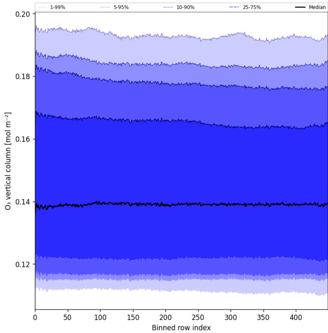
Figure 28: Along track statistics of “ \text{O}_3 vertical column” for 2025-05-07 to 2025-05-09
