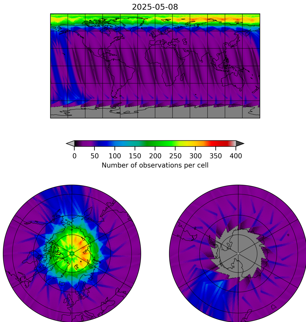
Figure 12: Map of the number of observations for 2025-05-07 to 2025-05-09
