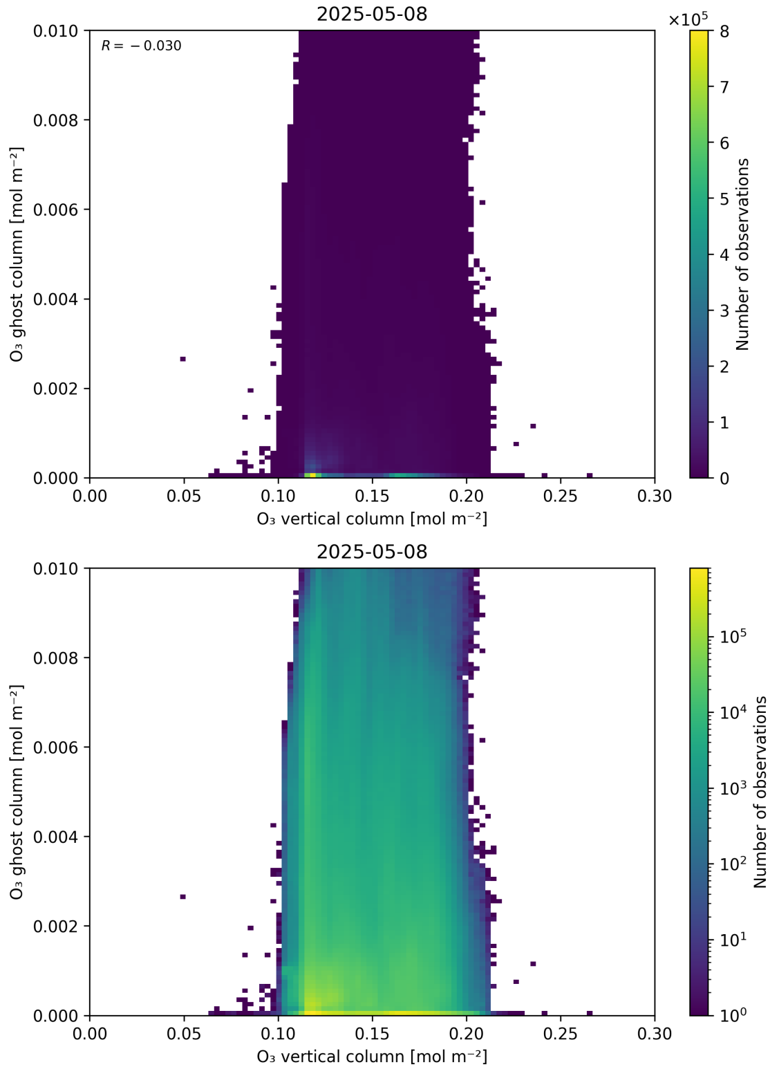
Figure 40: Scatter density plot of “O 3 vertical column” against “O 3 ghost column” for 2025-05-07 to 2025-05-09.
