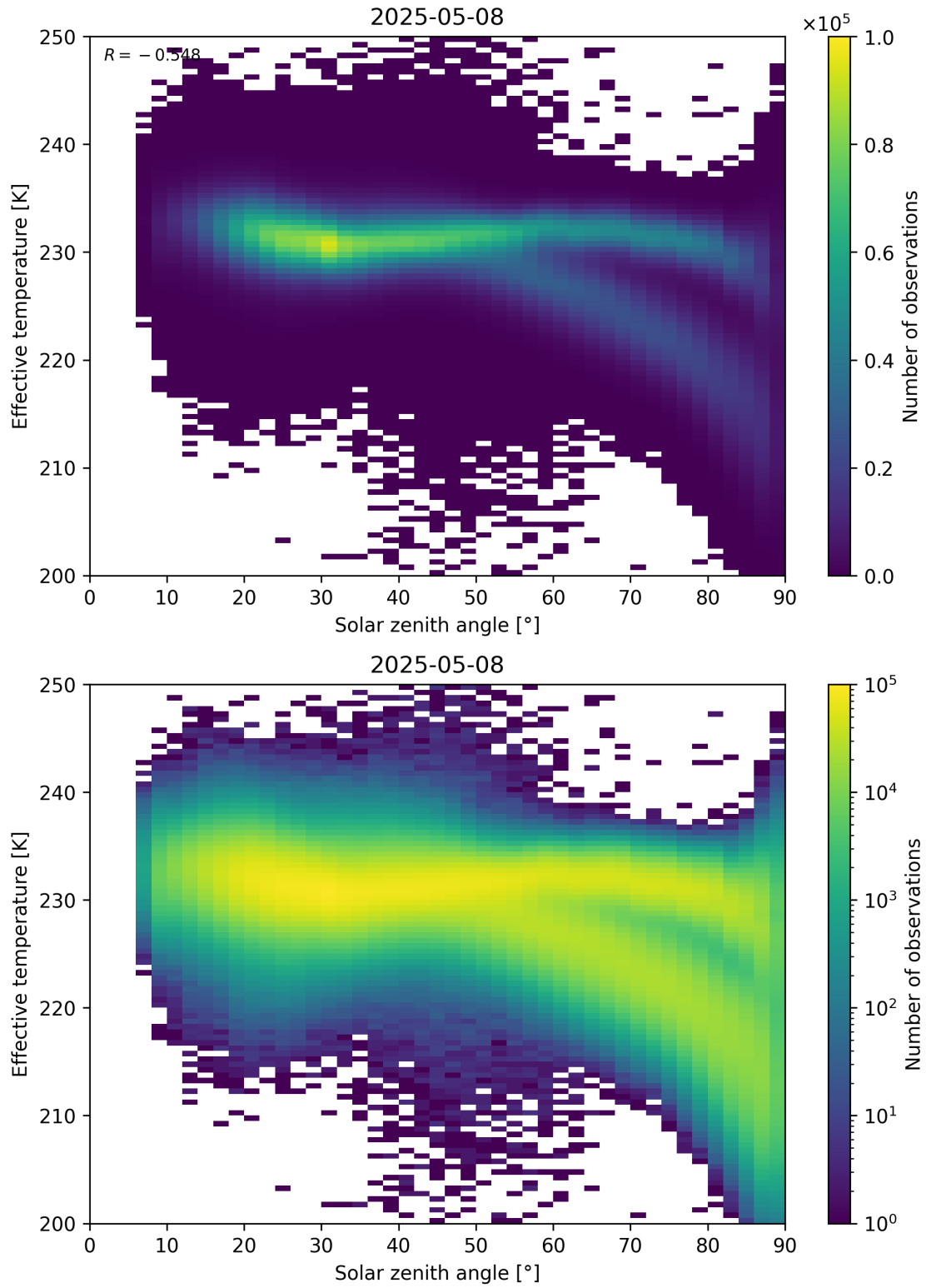
Figure 45: Scatter density plot of “Solar zenith angle” against “Effective temperature” for 2025-05-07 to 2025-05-09.
