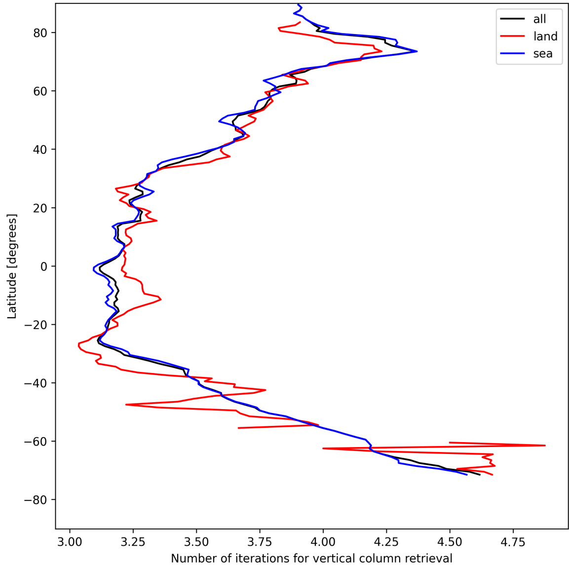
Figure 19: Zonal average of “Number of iterations for vertical column retrieval” for 2025-05-07 to 2025-05-09.
