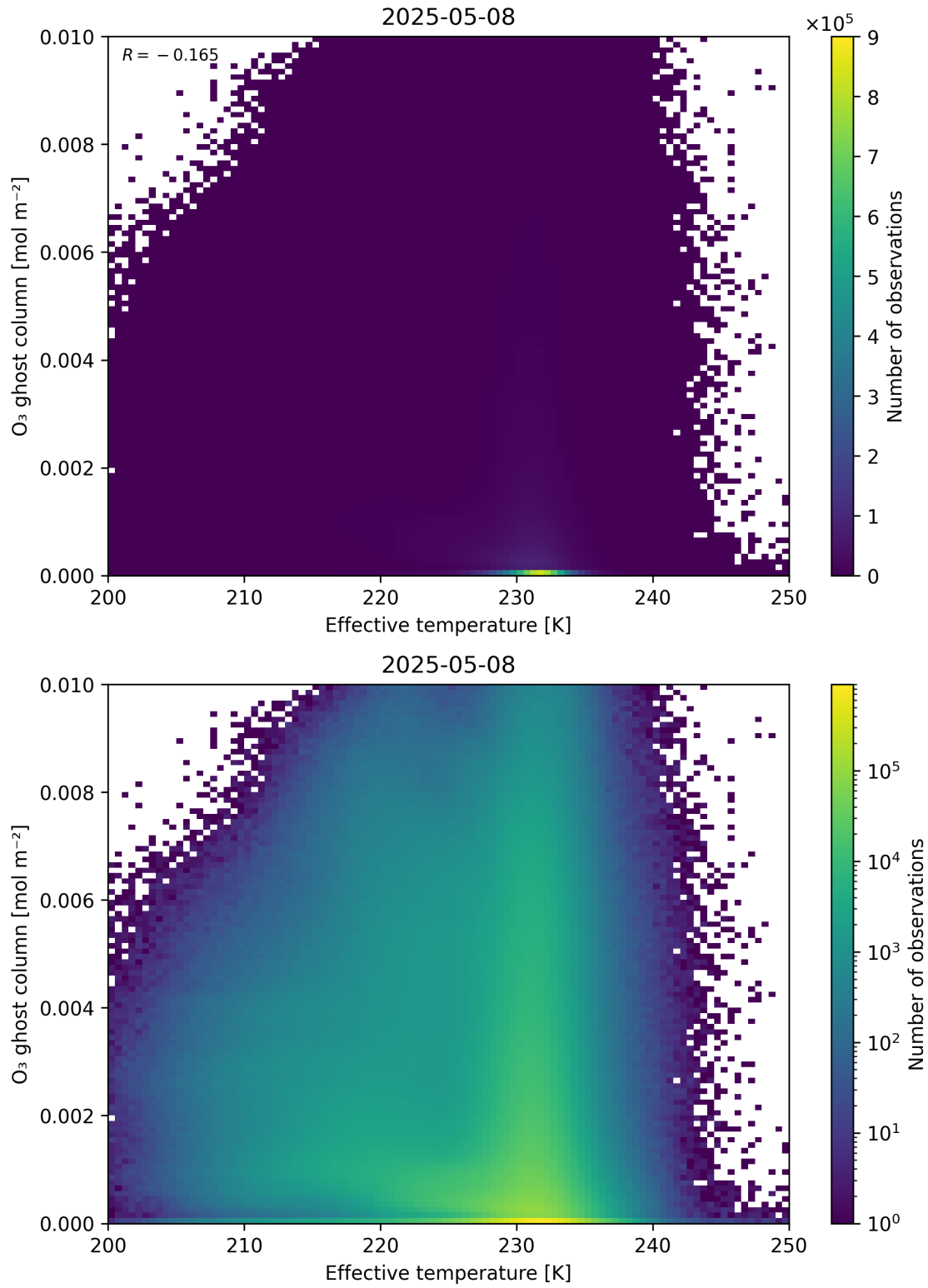
Figure 38: Scatter density plot of “Effective temperature” against “O 3 ghost column” for 2025-05-07 to 2025-05-09.
