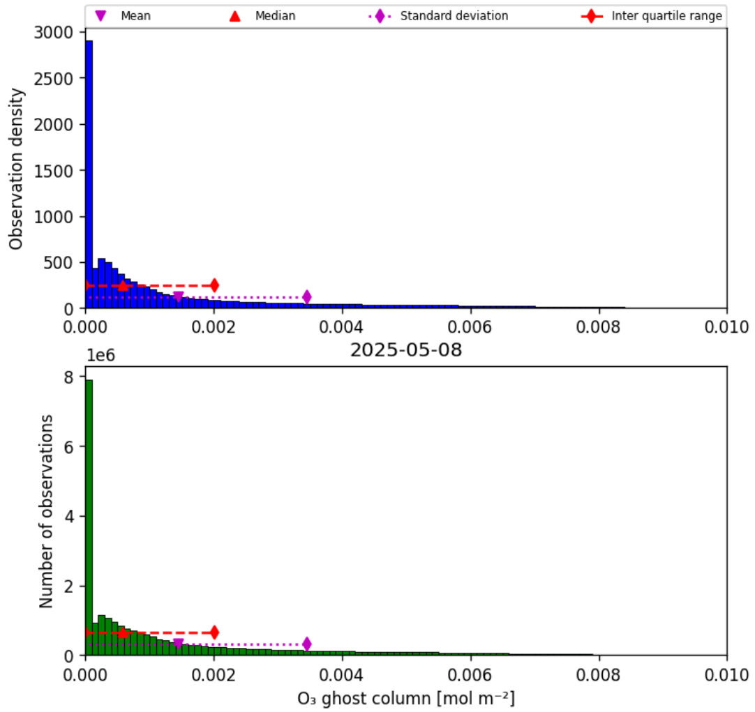
Figure 25: Histogram of “O 3 ghost column” for 2025-05-07 to 2025-05-09
