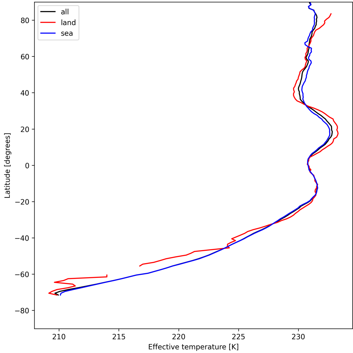
Figure 17: Zonal average of "Effective temperature" for 2025-05-07 to 2025-05-09.
