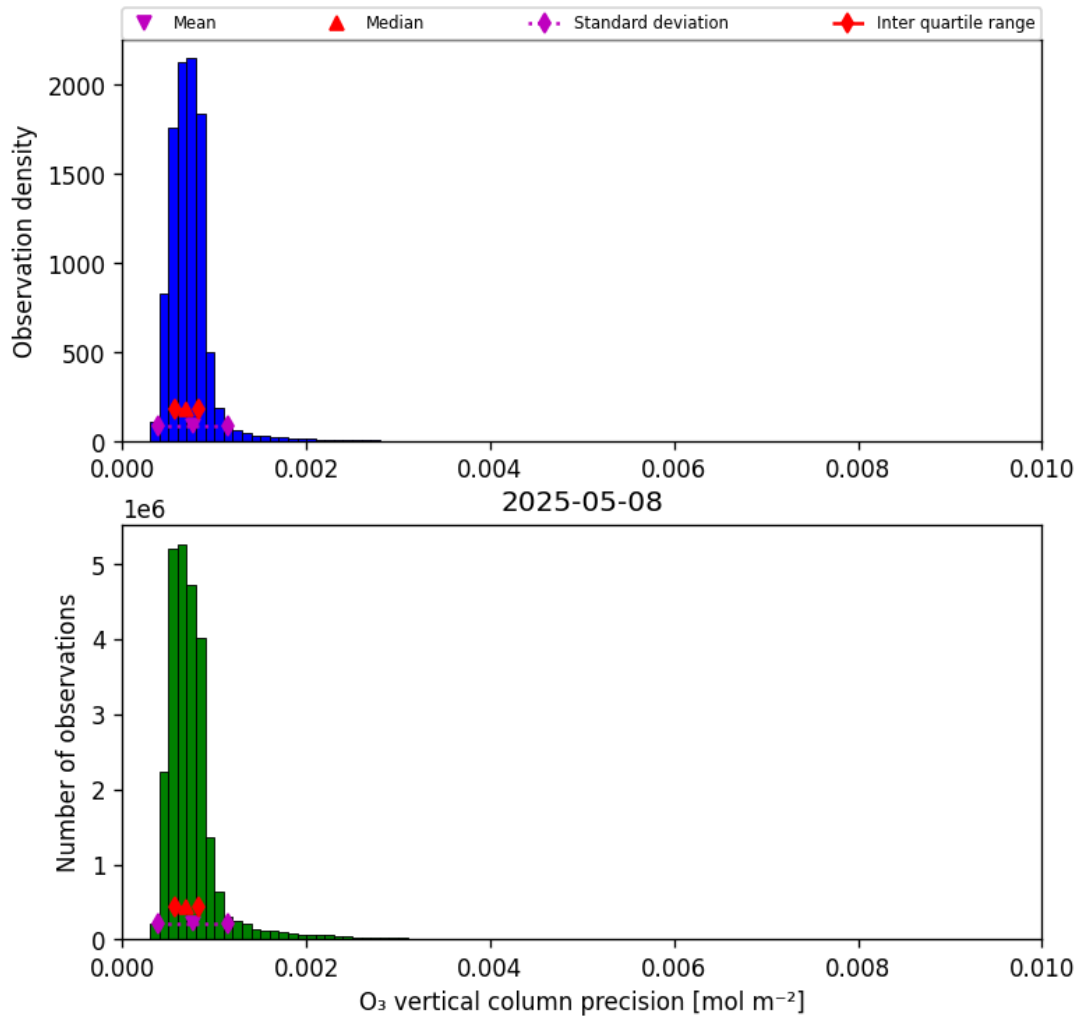
Figure 22: Histogram of “O 3 vertical column precision” for 2025-05-07 to 2025-05-09
