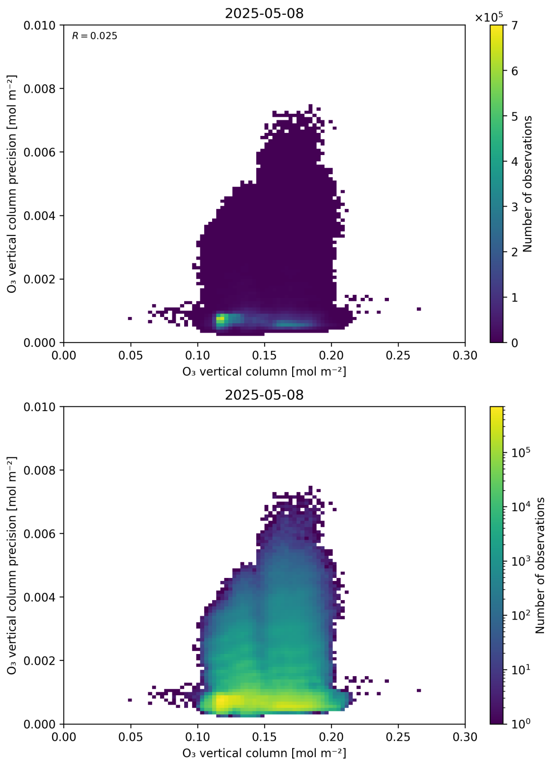
Figure 41: Scatter density plot of “O 3 vertical column” against “O 3 vertical column precision” for 2025-05-07 to 2025-05-09.
