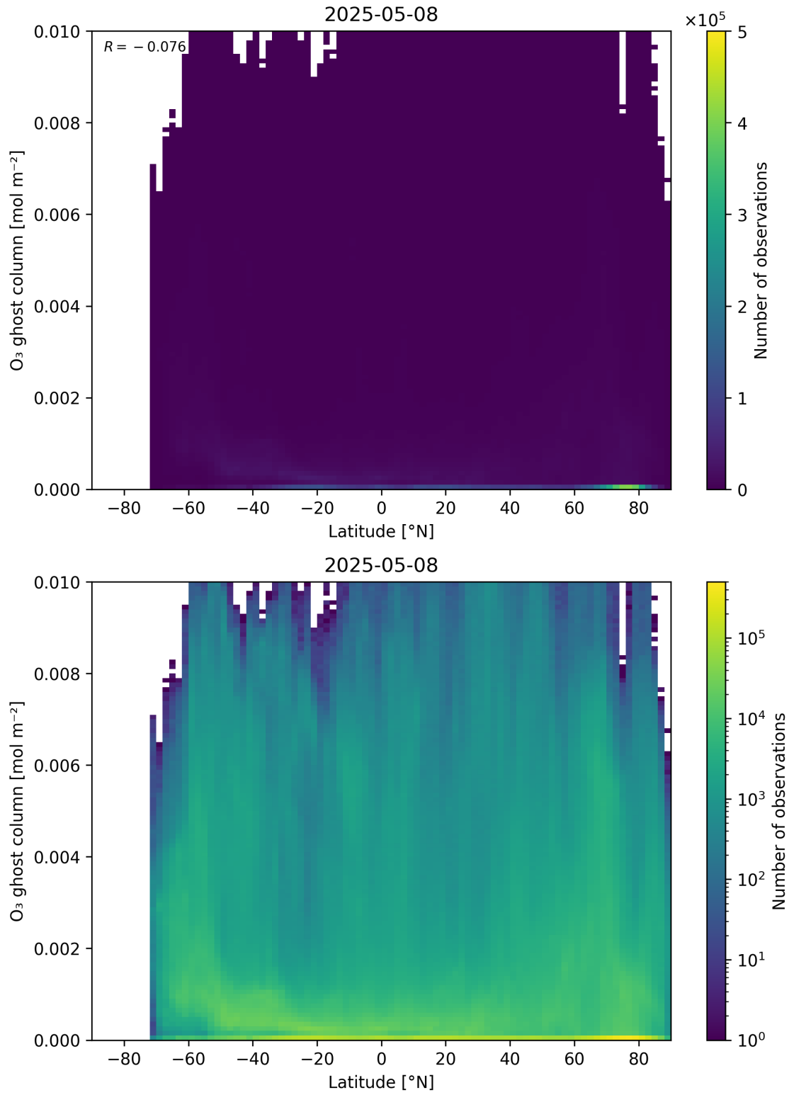
Figure 35: Scatter density plot of “Latitude” against “O 3 ghost column” for 2025-05-07 to 2025-05-09.
