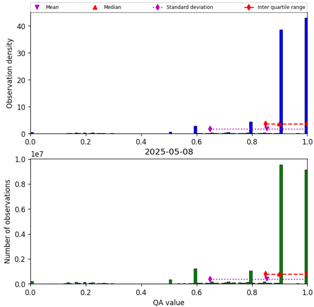
Figure 20: Histogram of “QA value” for 2025-05-07 to 2025-05-09
