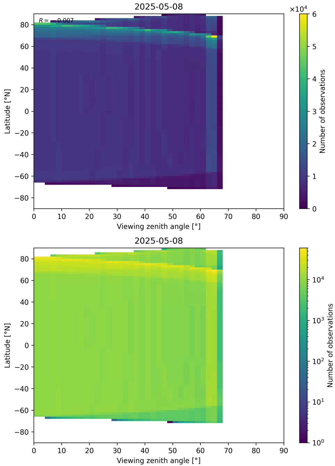
Figure 49: Scatter density plot of “Viewing zenith angle” against “Latitude” for 2025-05-07 to 2025-05-09.
