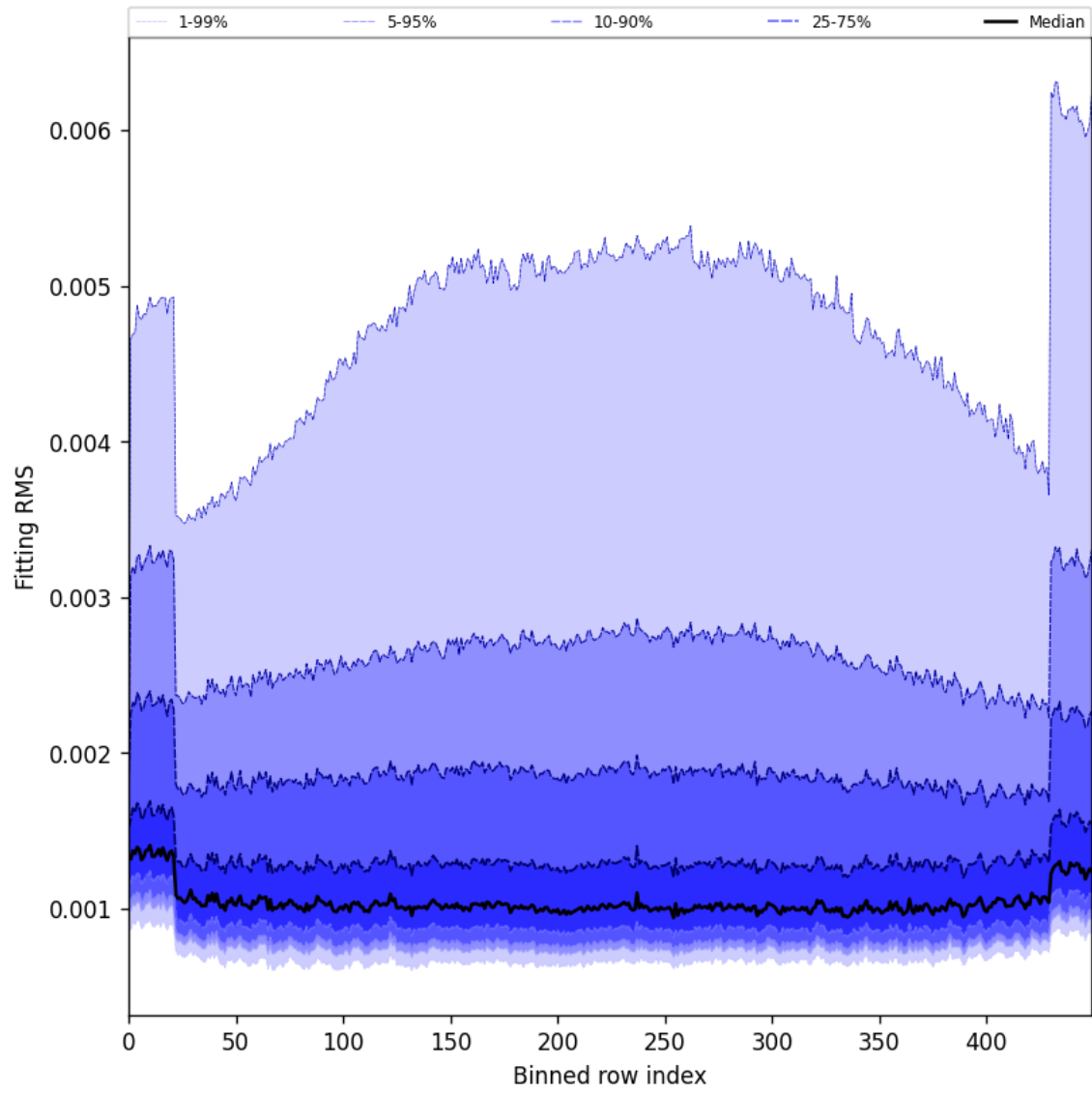
Figure 30: Along track statistics of “Fitting RMS” for 2025-05-07 to 2025-05-09
