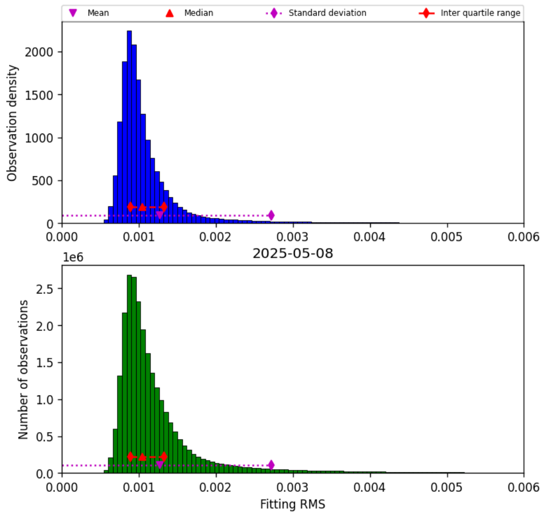
Figure 23: Histogram of “Fitting RMS” for 2025-05-07 to 2025-05-09
