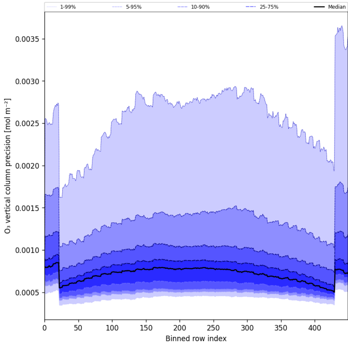
Figure 29: Along track statistics of “O 3 vertical column precision” for 2025-05-07 to 2025-05-09
