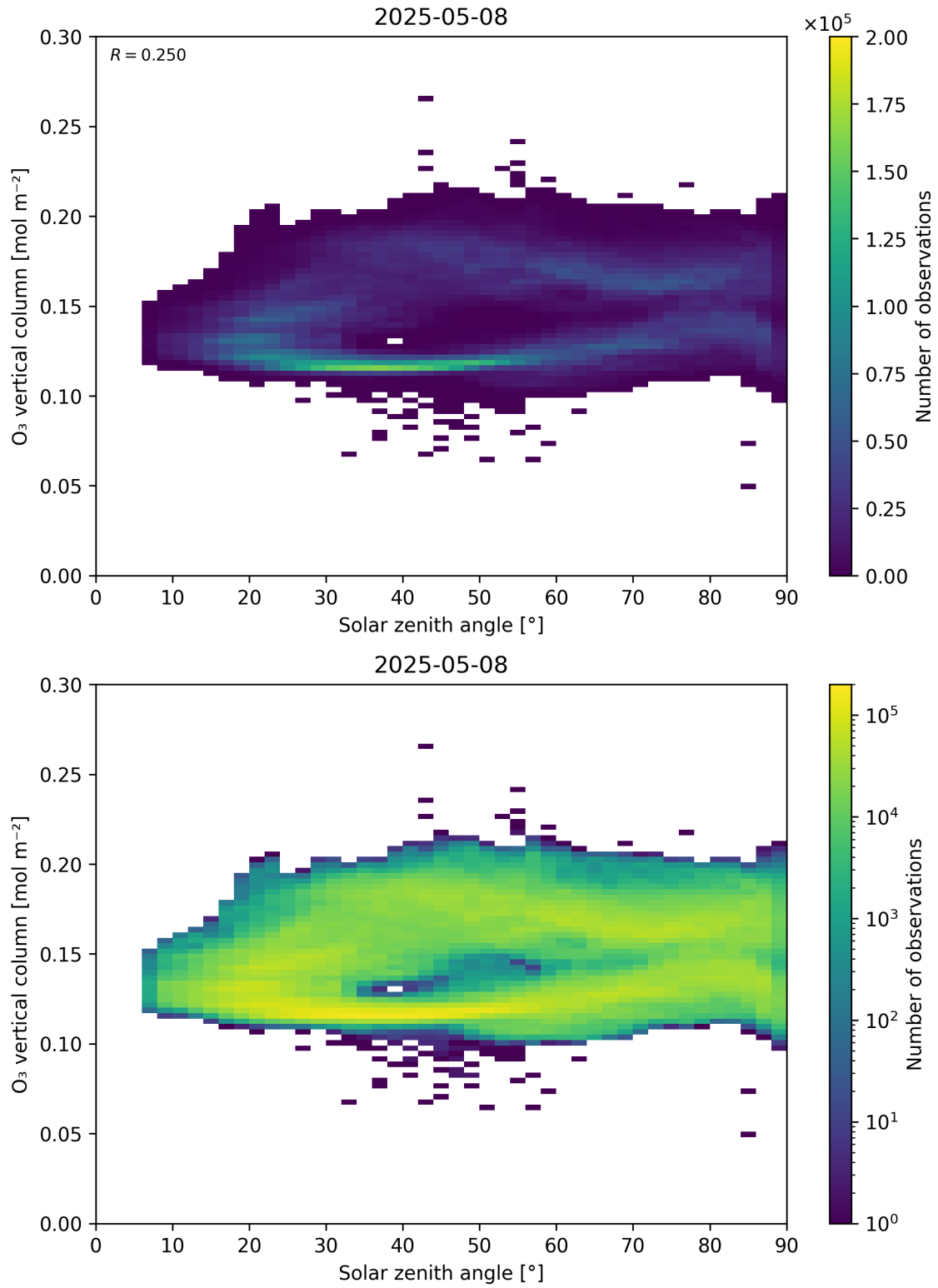
Figure 47: Scatter density plot of “Solar zenith angle” against “O 3 vertical column” for 2025-05-07 to 2025-05-09.
