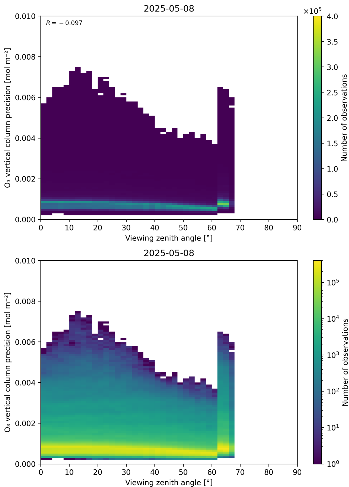
Figure 53: Scatter density plot of “Viewing zenith angle” against “O 3 vertical column precision” for 2025-05-07 to 2025-05-09.
