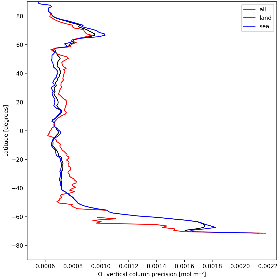
Figure 15: Zonal average of “O 3 vertical column precision” for 2025-05-07 to 2025-05-09.
