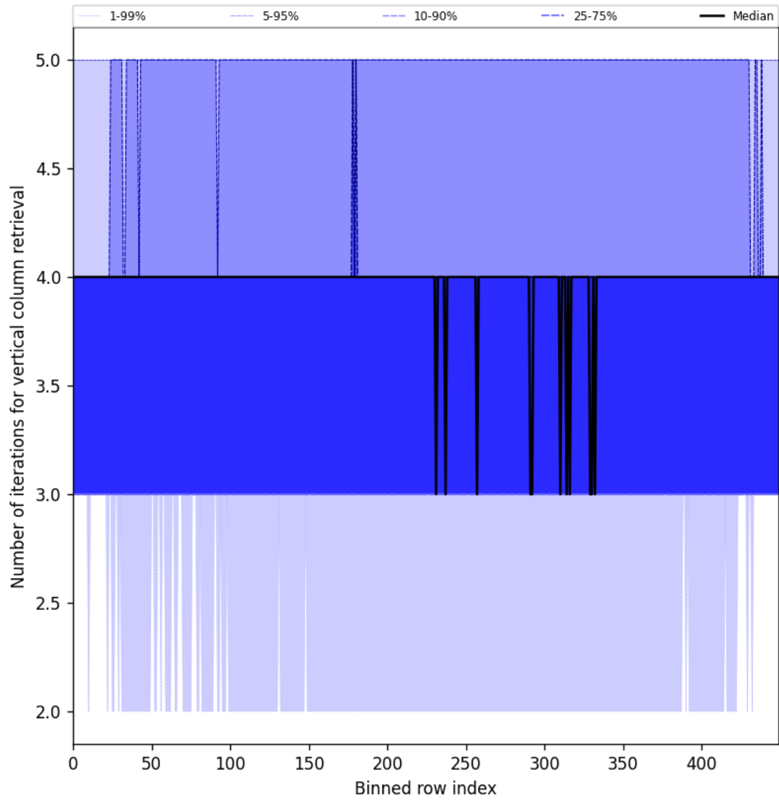
Figure 33: Along track statistics of “Number of iterations for vertical column retrieval” for 2025-05-07 to 2025-05-09
