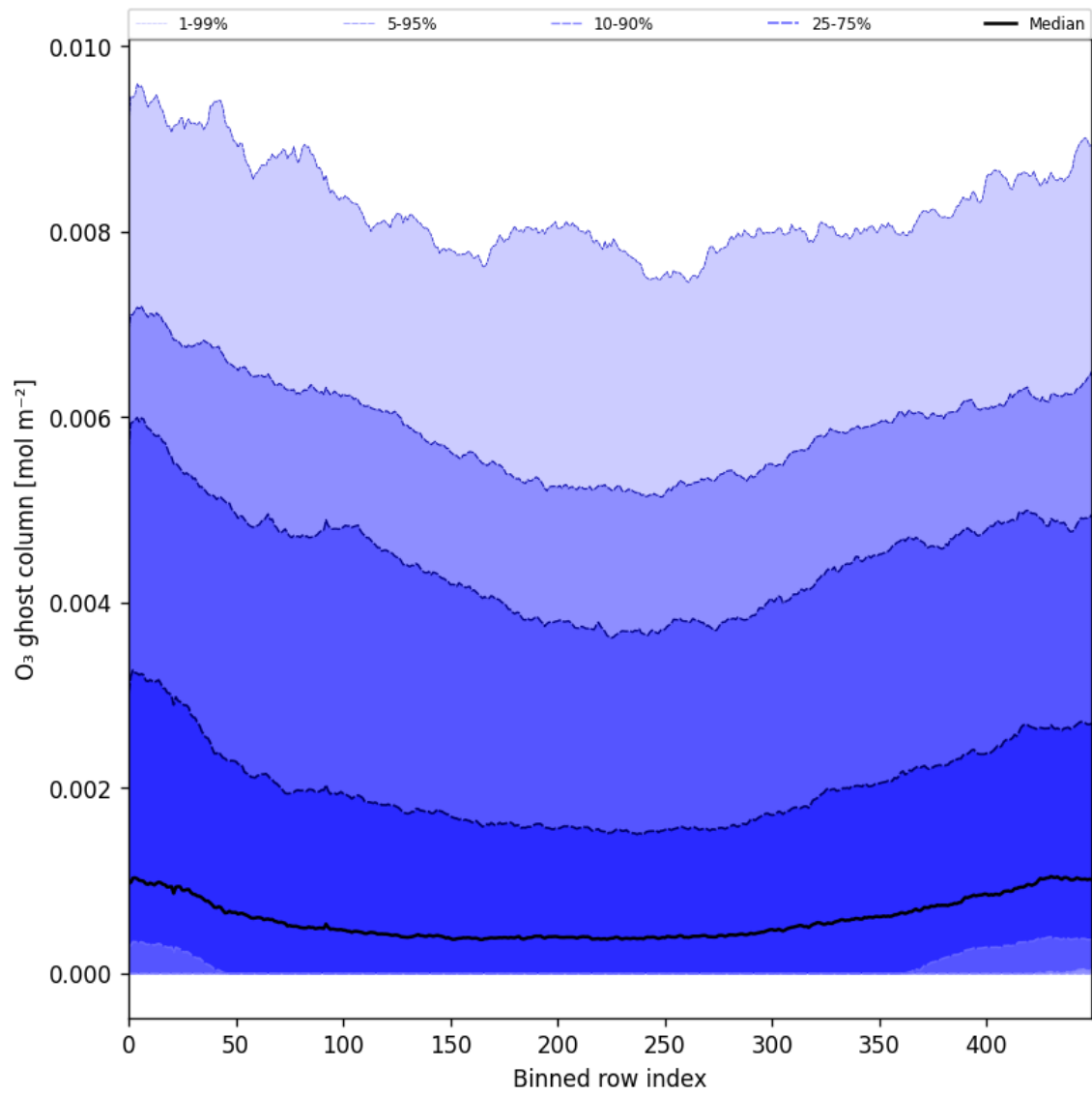
Figure 32: Along track statistics of “O 3 ghost column” for 2025-05-07 to 2025-05-09
