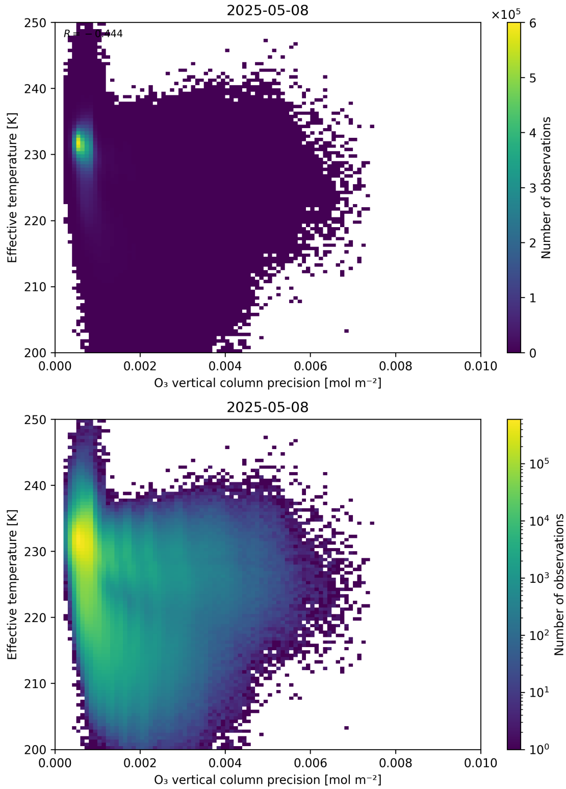
Figure 42: Scatter density plot of “O 3 vertical column precision” against “Effective temperature” for 2025-05-07 to 2025-05-09.
