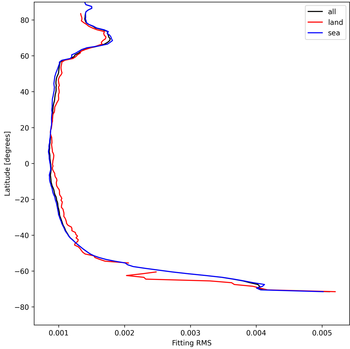
Figure 16: Zonal average of “Fitting RMS” for 2025-05-07 to 2025-05-09.
