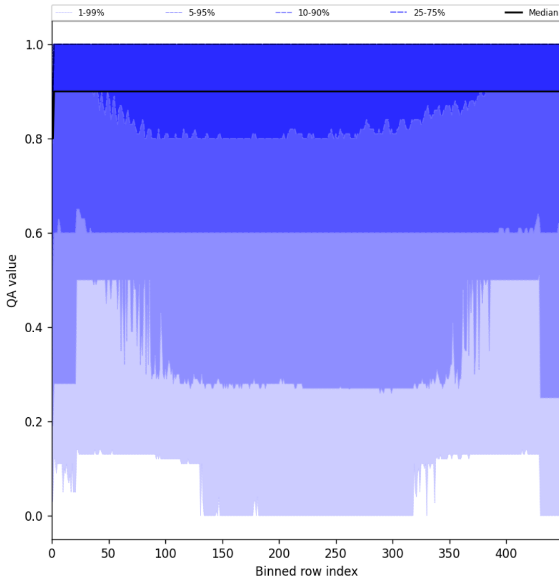
Figure 27: Along track statistics of “QA value” for 2025-05-07 to 2025-05-09
