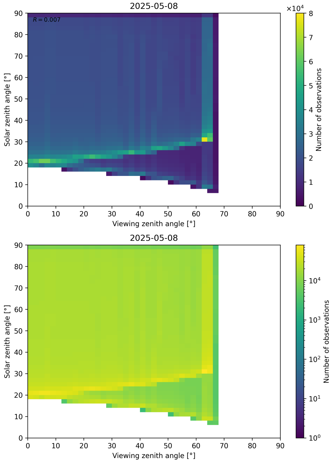
Figure 54: Scatter density plot of “Viewing zenith angle” against “Solar zenith angle” for 2025-05-07 to 2025-05-09.
