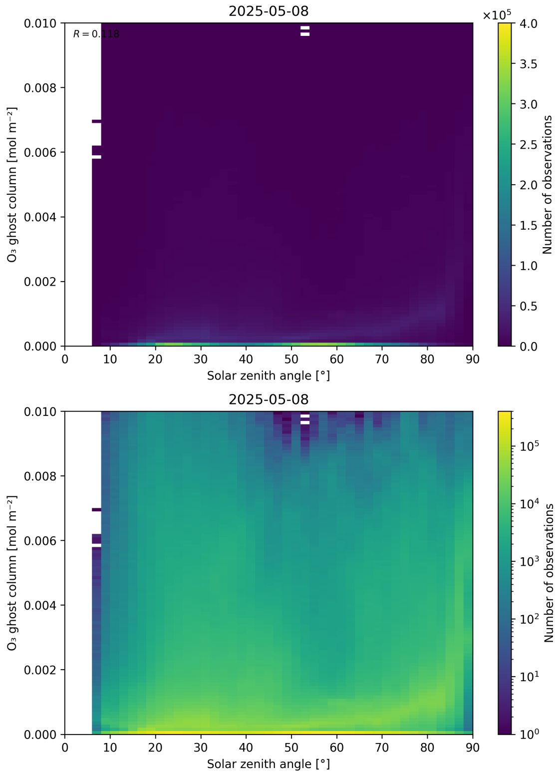
Figure 46: Scatter density plot of “Solar zenith angle” against “O 3 ghost column” for 2025-05-07 to 2025-05-09.
