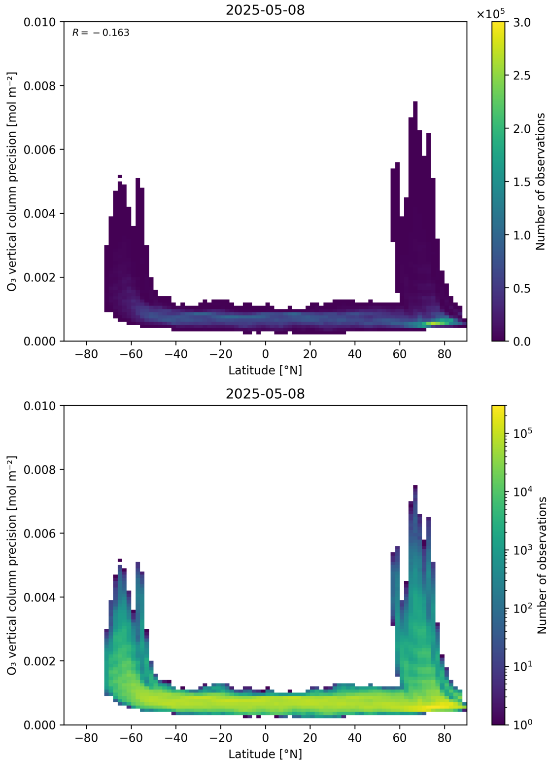
Figure 37: Scatter density plot of “Latitude” against “O 3 vertical column precision” for 2025-05-07 to 2025-05-09.
