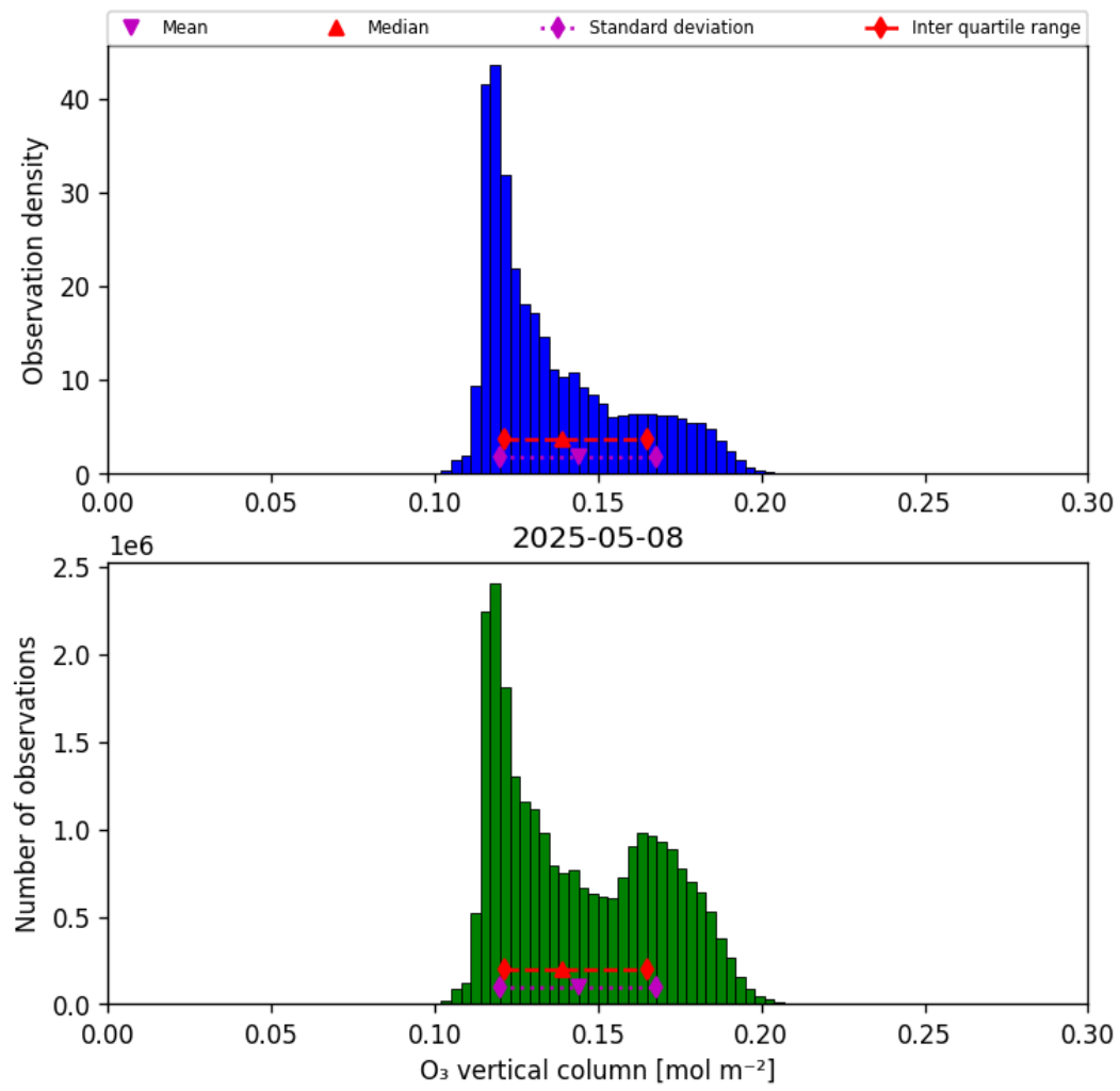
Figure 21: Histogram of “O 3 vertical column” for 2025-05-07 to 2025-05-09
