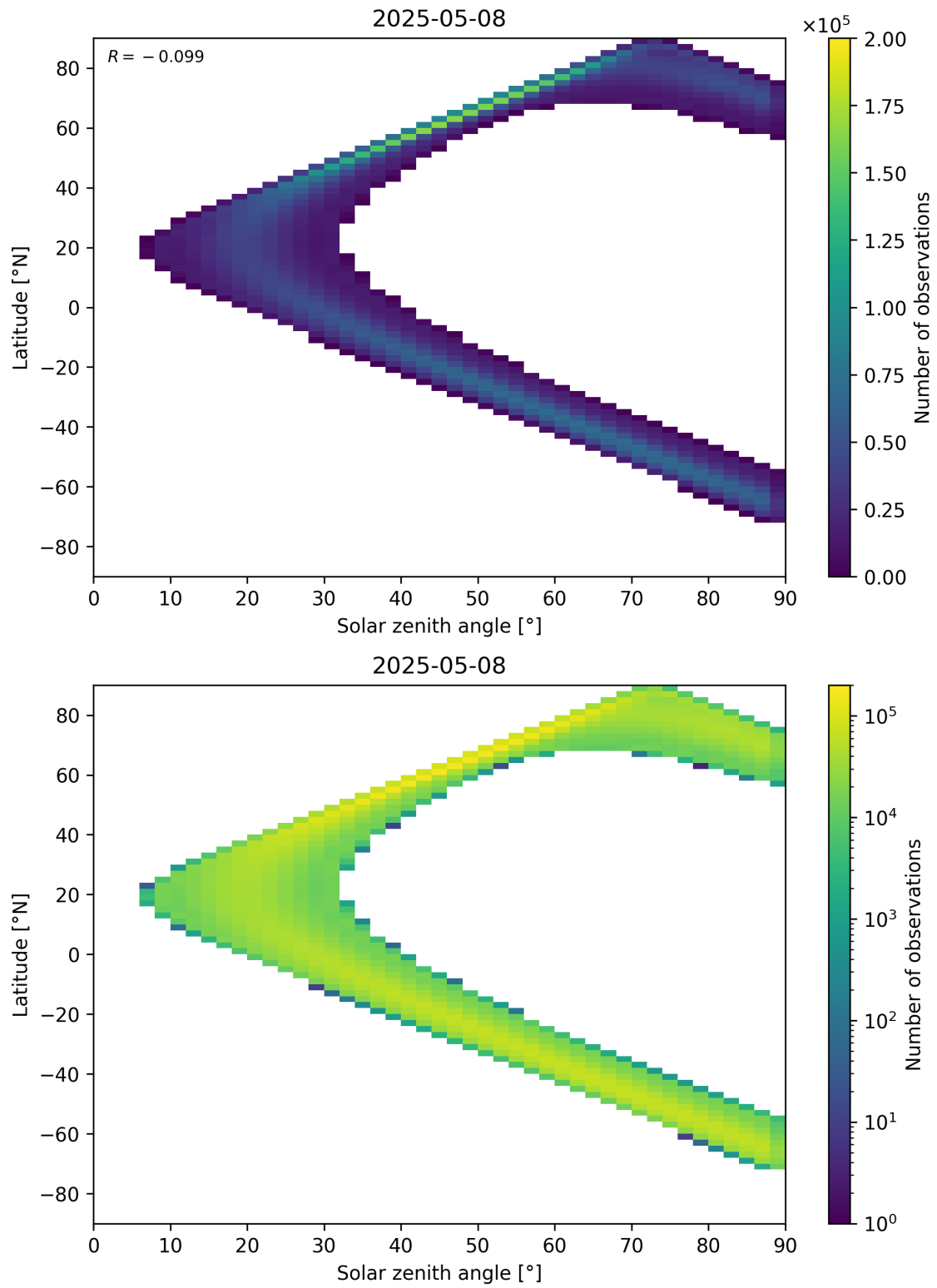
Figure 44: Scatter density plot of “Solar zenith angle” against “Latitude” for 2025-05-07 to 2025-05-09.
