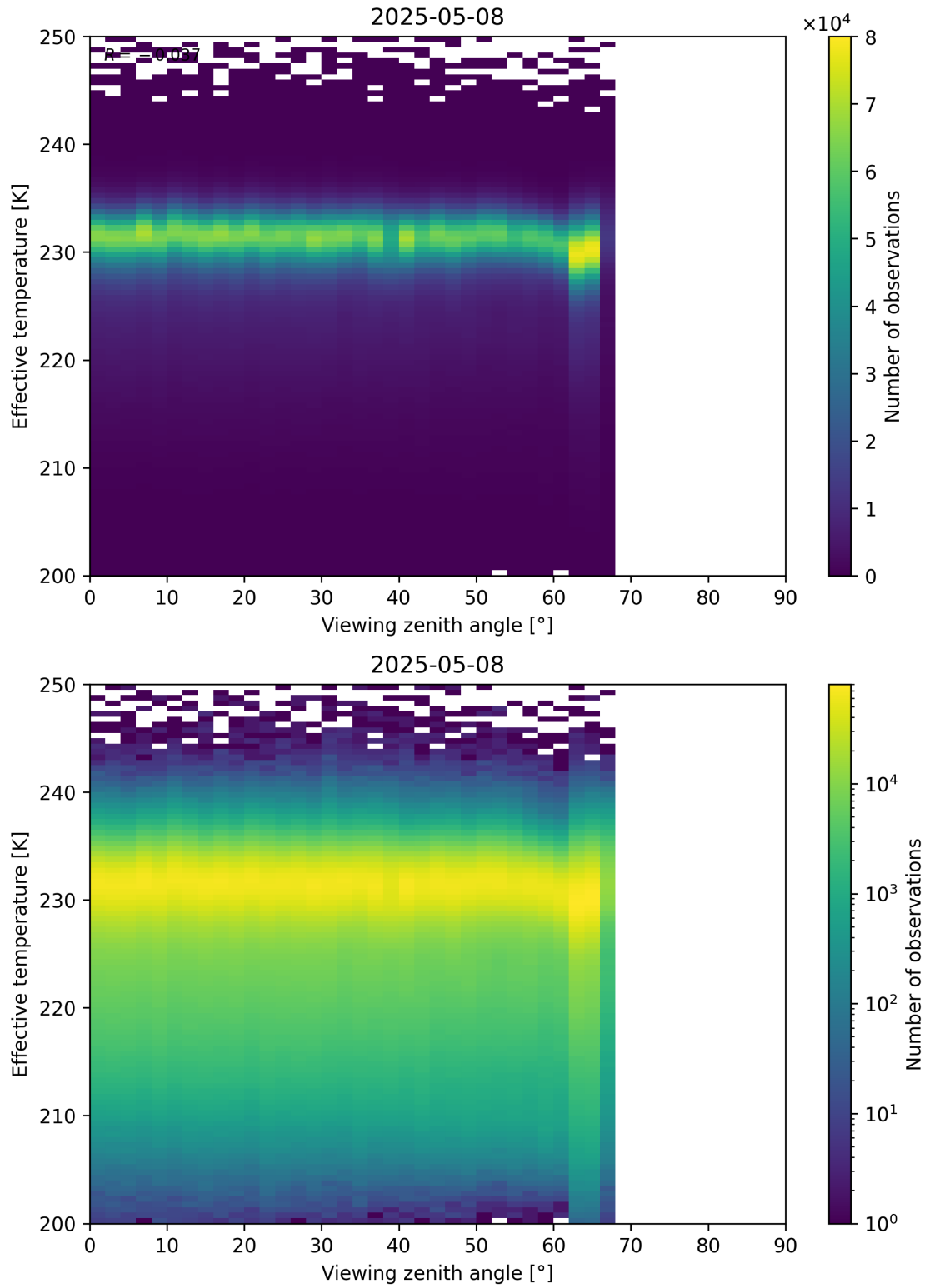
Figure 50: Scatter density plot of “Viewing zenith angle” against “Effective temperature” for 2025-05-07 to 2025-05-09.
