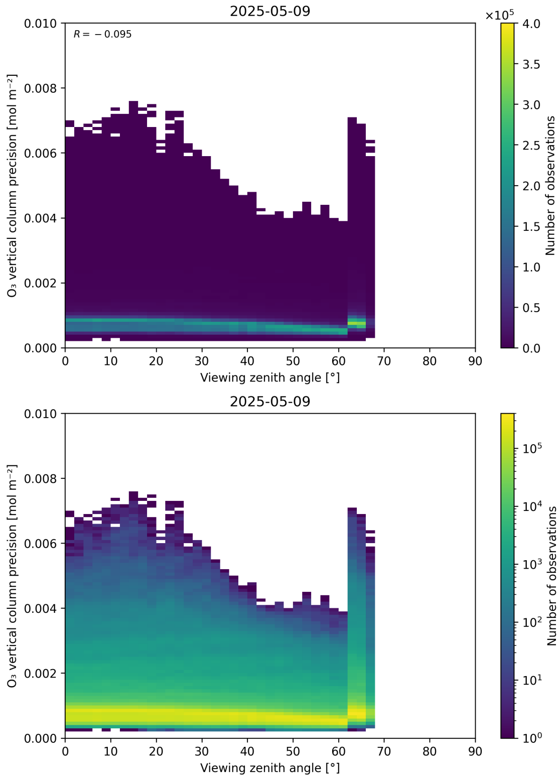
Figure 53: Scatter density plot of “Viewing zenith angle” against “O 3 vertical column precision” for 2025-05-08 to 2025-05-10.
