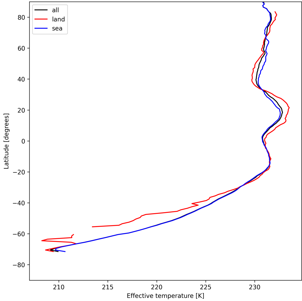
Figure 17: Zonal average of "Effective temperature" for 2025-05-08 to 2025-05-10.
