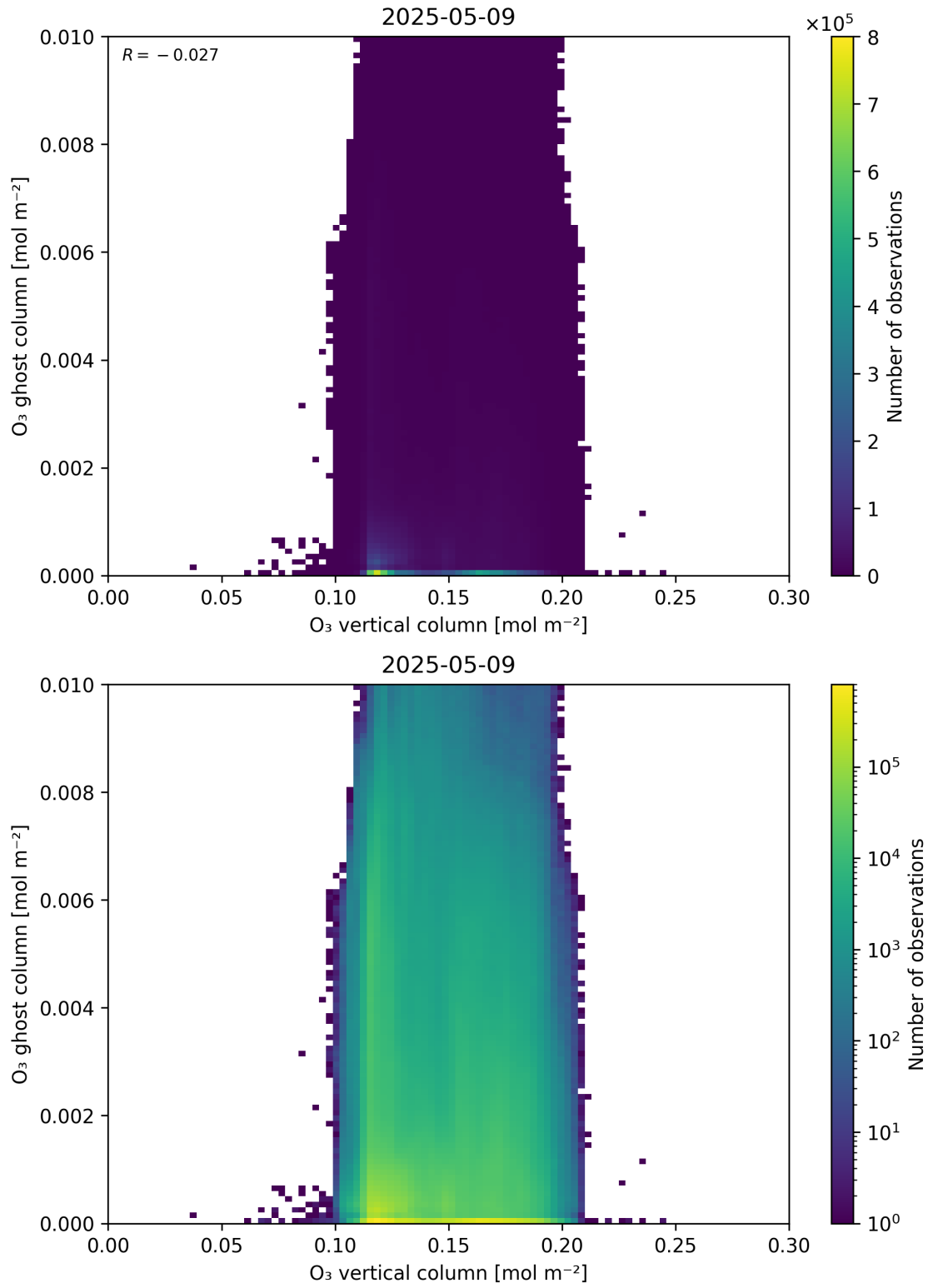
Figure 40: Scatter density plot of “O 3 vertical column” against “O 3 ghost column” for 2025-05-08 to 2025-05-10.
