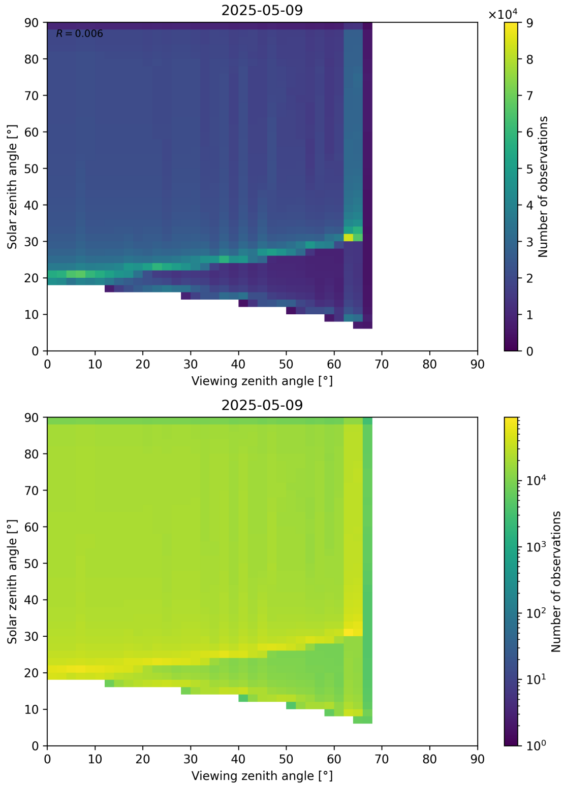
Figure 54: Scatter density plot of “Viewing zenith angle” against “Solar zenith angle” for 2025-05-08 to 2025-05-10.
