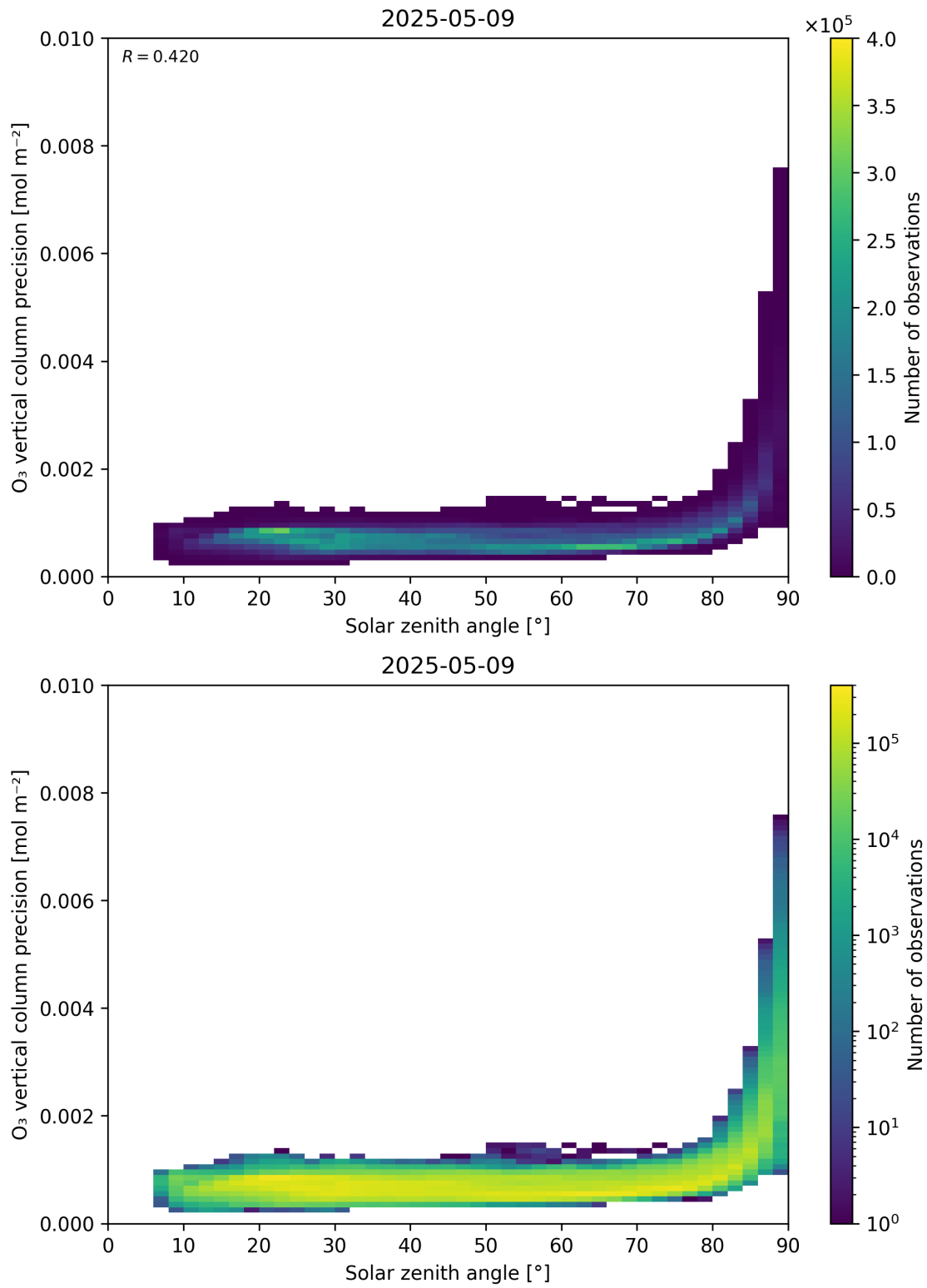
Figure 48: Scatter density plot of “Solar zenith angle” against “O 3 vertical column precision” for 2025-05-08 to 2025-05-10.
