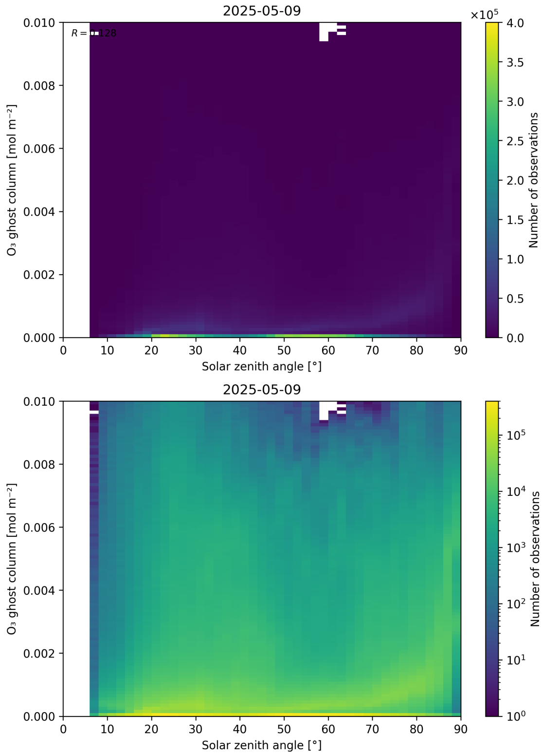
Figure 46: Scatter density plot of “Solar zenith angle” against “O 3 ghost column” for 2025-05-08 to 2025-05-10.
