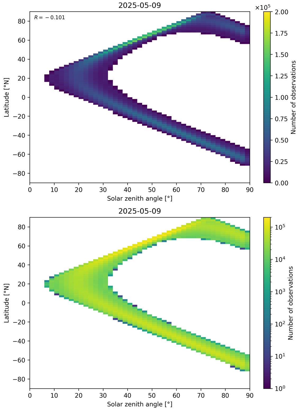
Figure 44: Scatter density plot of “Solar zenith angle” against “Latitude” for 2025-05-08 to 2025-05-10.
