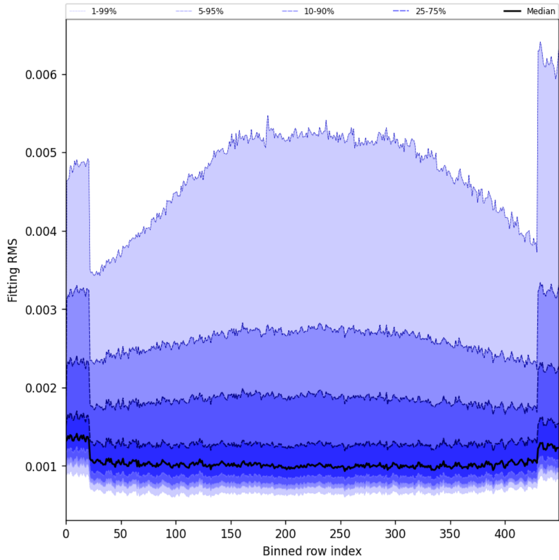
Figure 30: Along track statistics of “Fitting RMS” for 2025-05-08 to 2025-05-10
