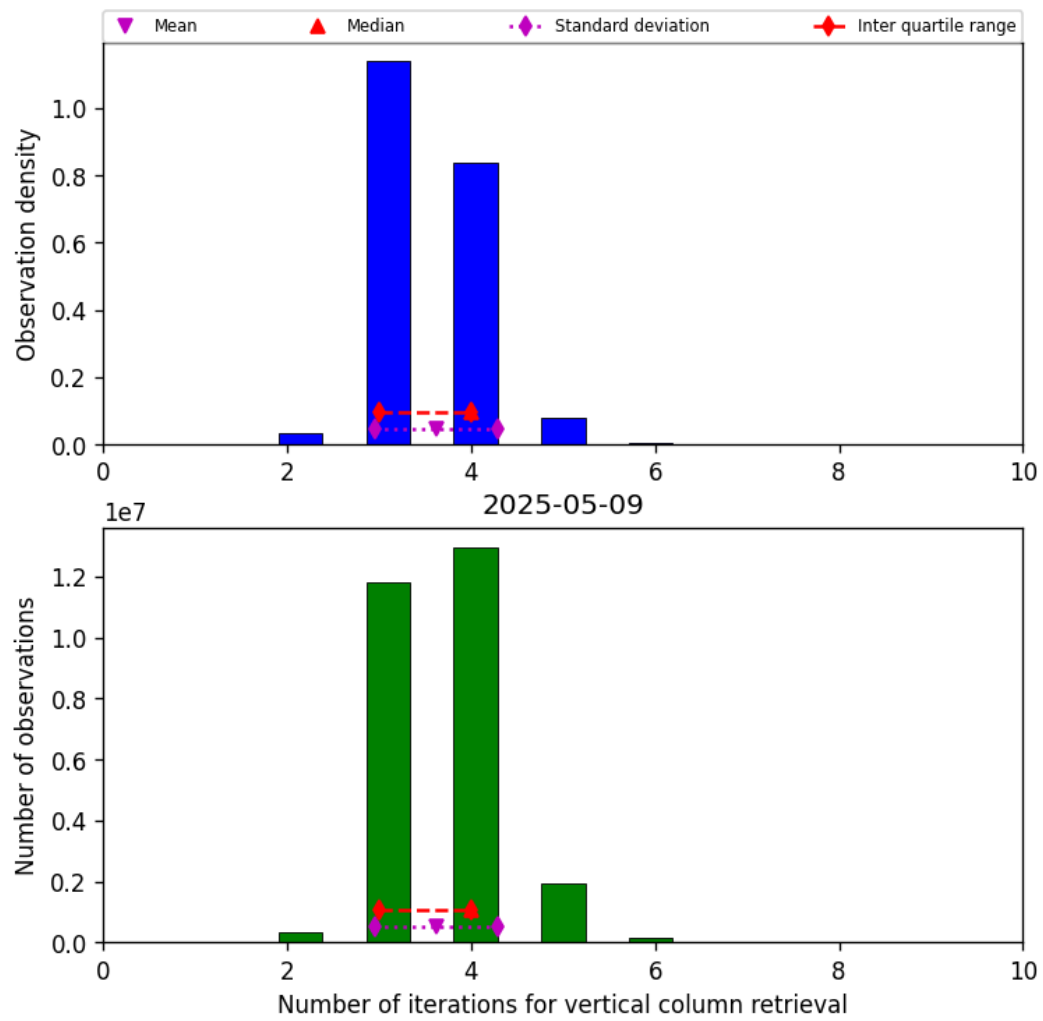
Figure 26: Histogram of “Number of iterations for vertical column retrieval” for 2025-05-08 to 2025-05-10
