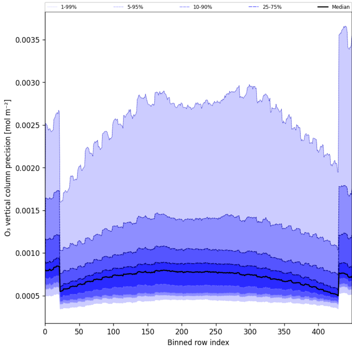
Figure 29: Along track statistics of “O 3 vertical column precision” for 2025-05-08 to 2025-05-10
