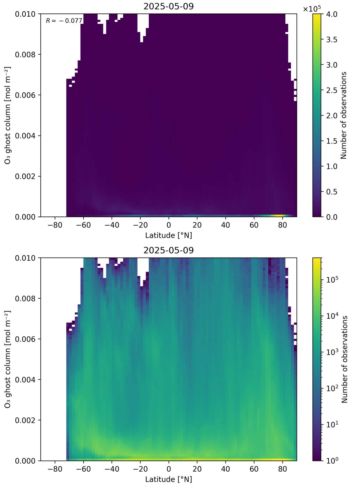
Figure 35: Scatter density plot of “Latitude” against “O 3 ghost column” for 2025-05-08 to 2025-05-10.
