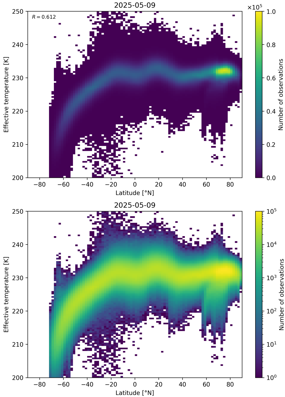
Figure 34: Scatter density plot of “Latitude” against “Effective temperature” for 2025-05-08 to 2025-05-10.
