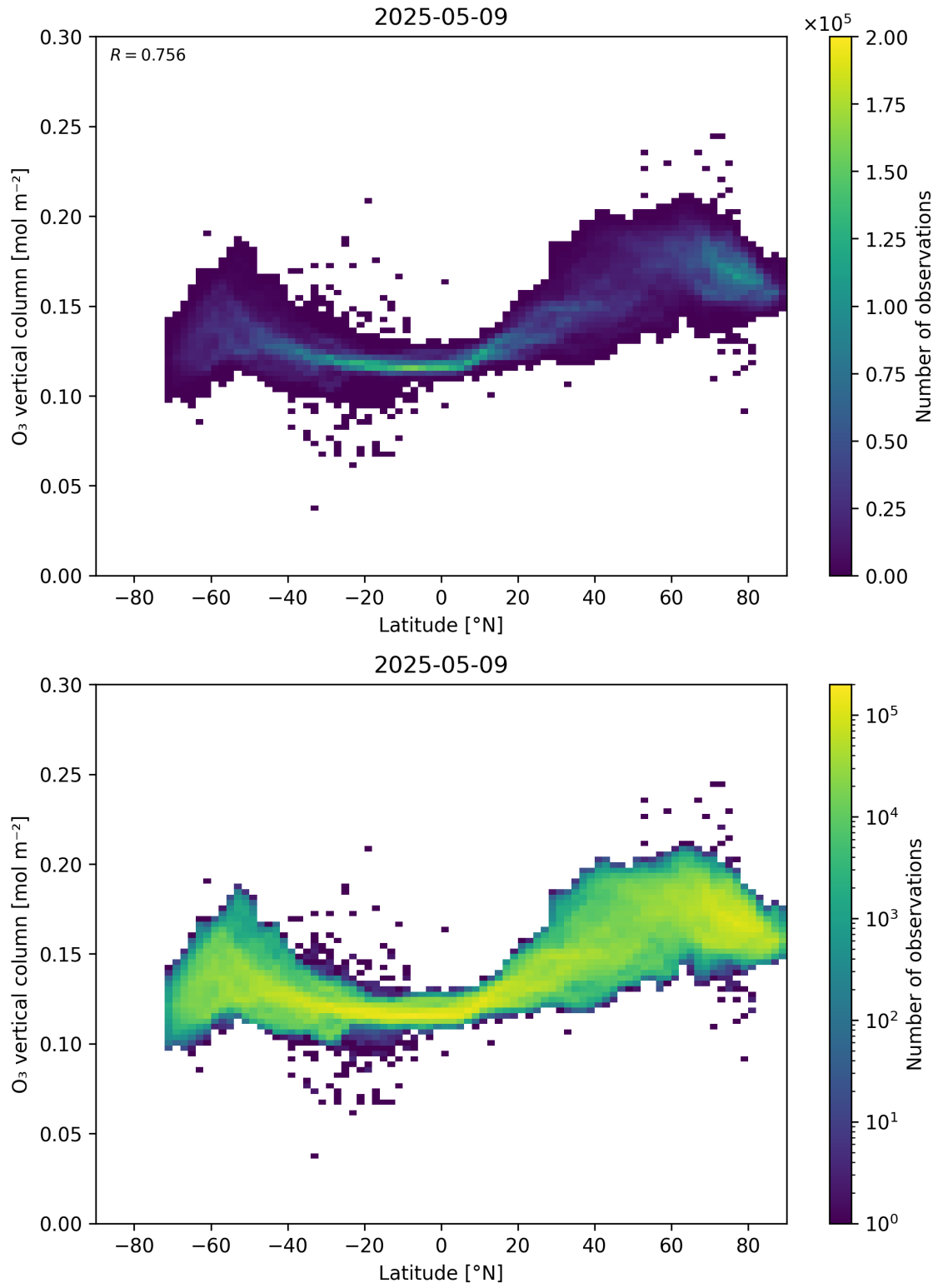
Figure 36: Scatter density plot of “Latitude” against “O 3 vertical column” for 2025-05-08 to 2025-05-10.
