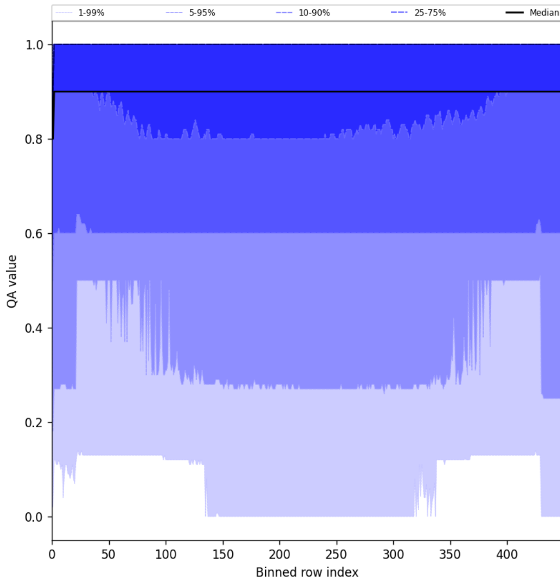
Figure 27: Along track statistics of “QA value” for 2025-05-08 to 2025-05-10
