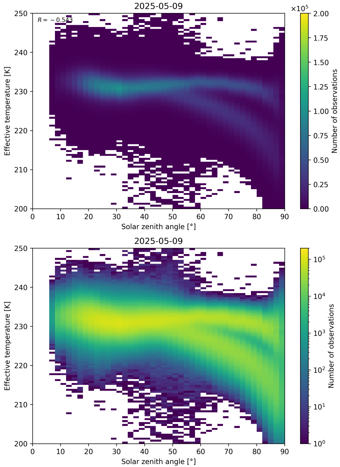
Figure 45: Scatter density plot of “Solar zenith angle” against “Effective temperature” for 2025-05-08 to 2025-05-10.
