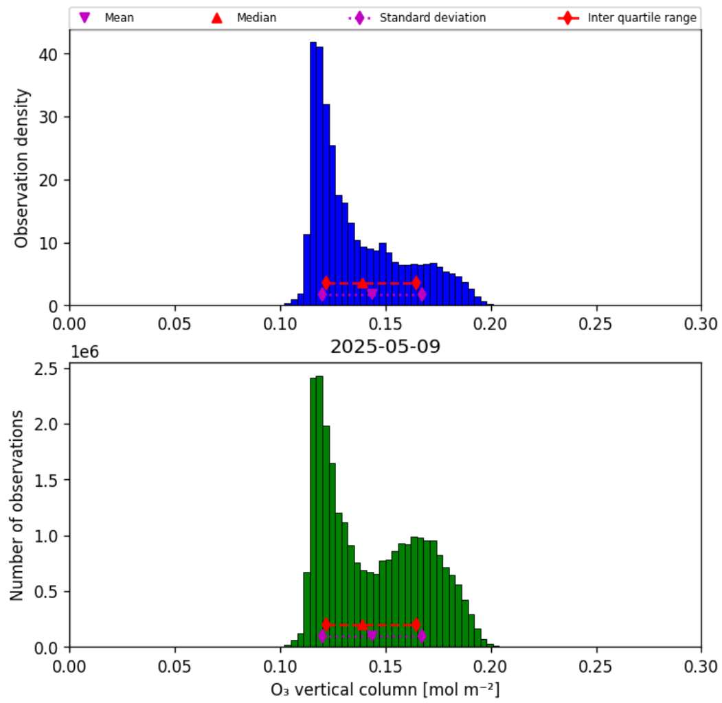
Figure 21: Histogram of “O 3 vertical column” for 2025-05-08 to 2025-05-10
