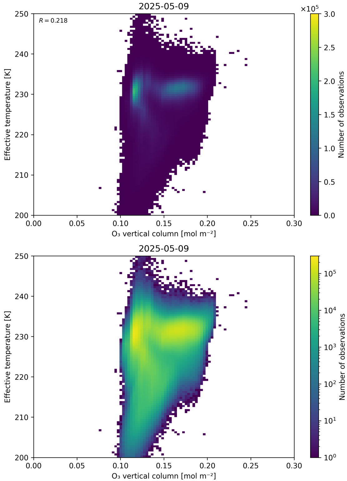
Figure 39: Scatter density plot of “O 3 vertical column” against “Effective temperature” for 2025-05-08 to 2025-05-10.
