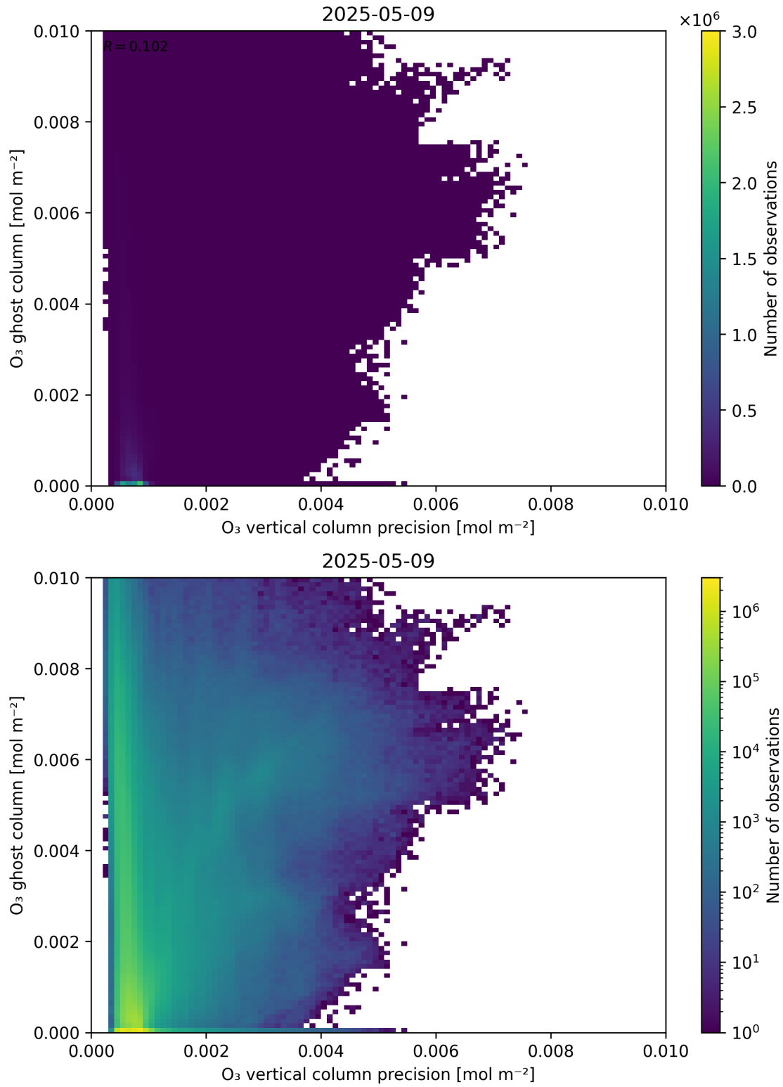
Figure 43: Scatter density plot of “O 3 vertical column precision” against “O 3 ghost column” for 2025-05-08 to 2025-05-10.
