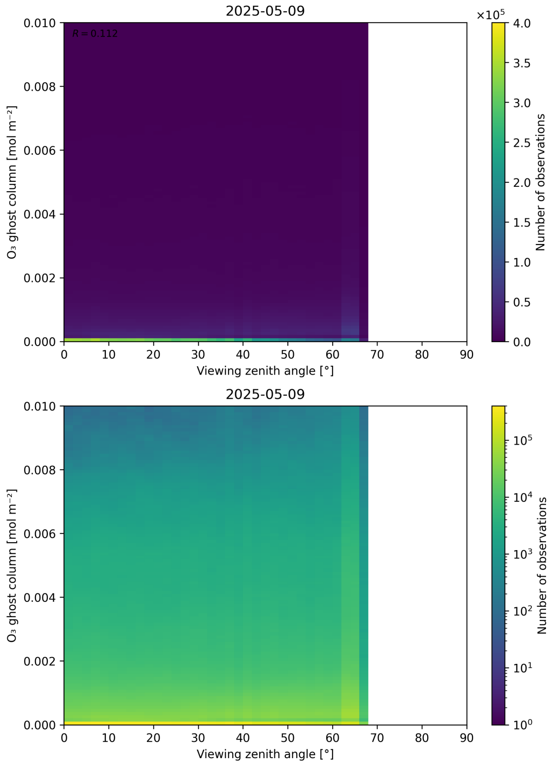
Figure 51: Scatter density plot of “Viewing zenith angle” against “O 3 ghost column” for 2025-05-08 to 2025-05-10.
