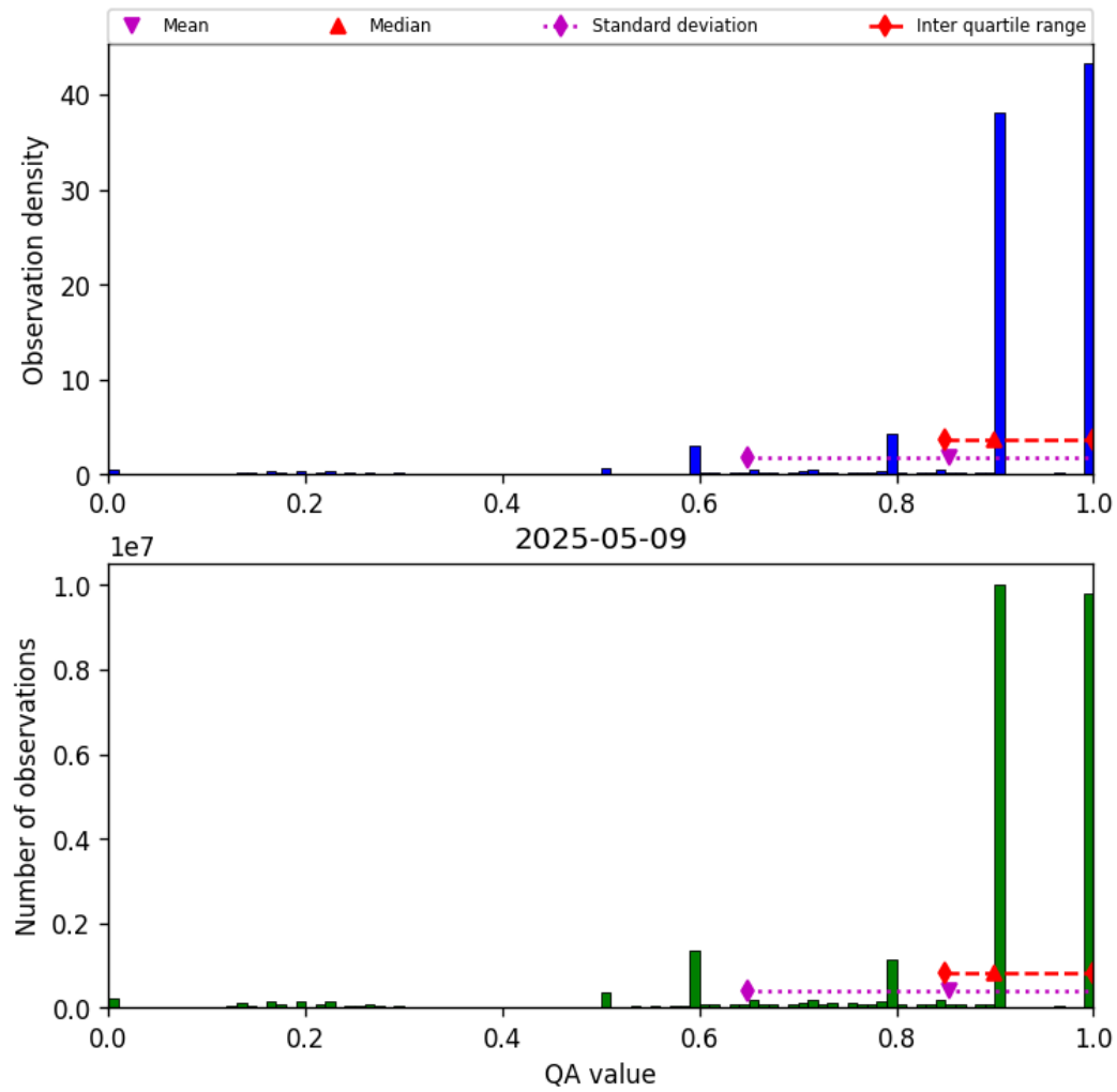
Figure 20: Histogram of “QA value” for 2025-05-08 to 2025-05-10
