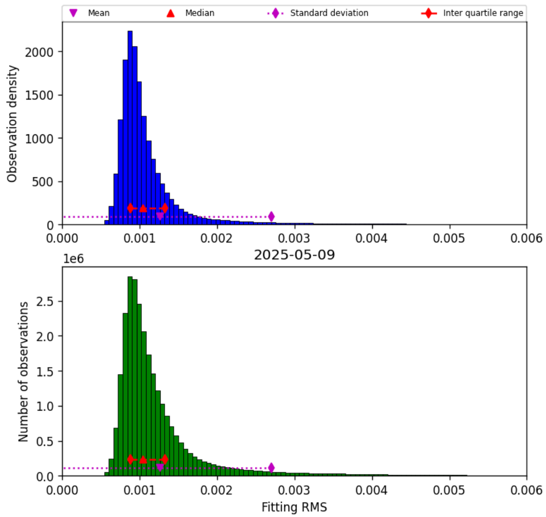
Figure 23: Histogram of “Fitting RMS” for 2025-05-08 to 2025-05-10
