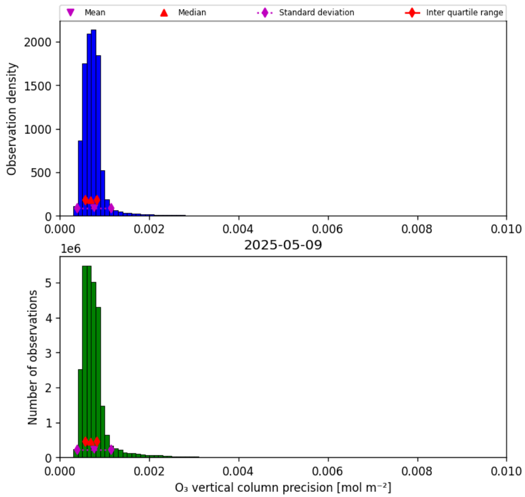
Figure 22: Histogram of “O 3 vertical column precision” for 2025-05-08 to 2025-05-10
