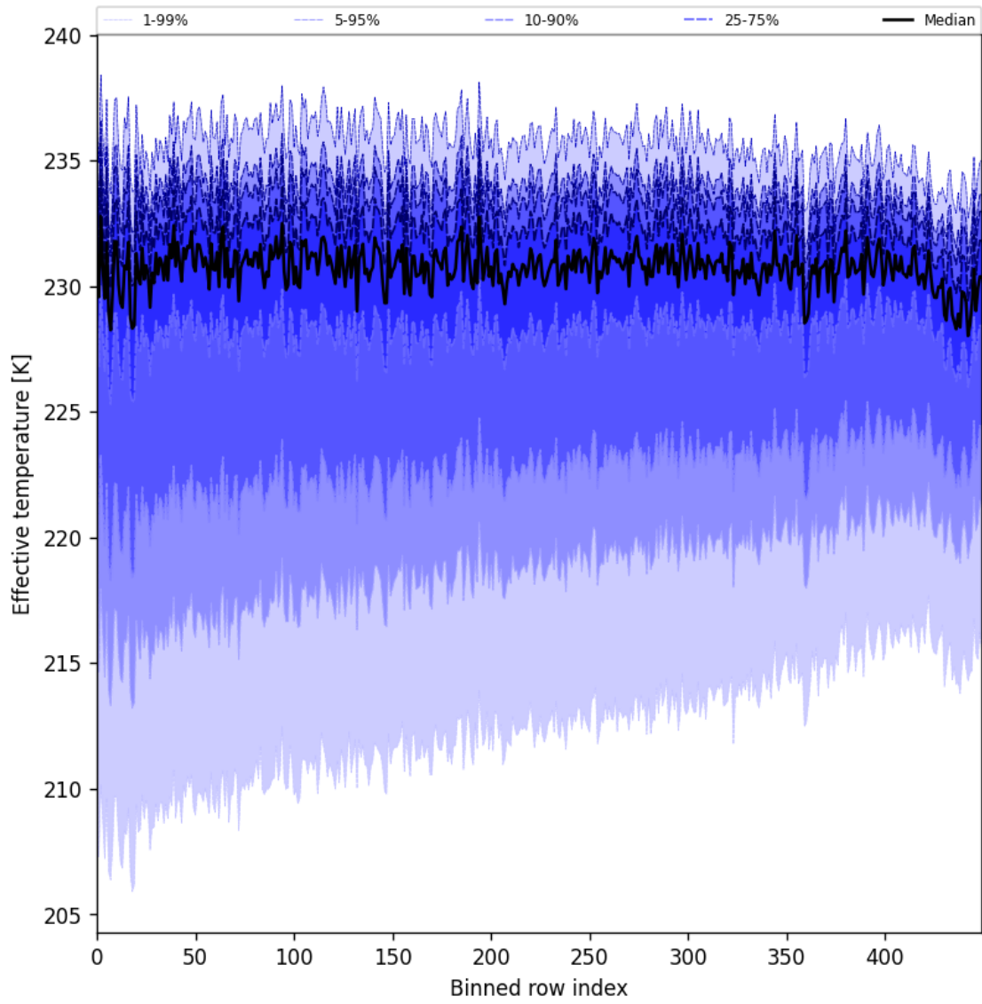
Figure 31: Along track statistics of “Effective temperature” for 2025-05-08 to 2025-05-10
