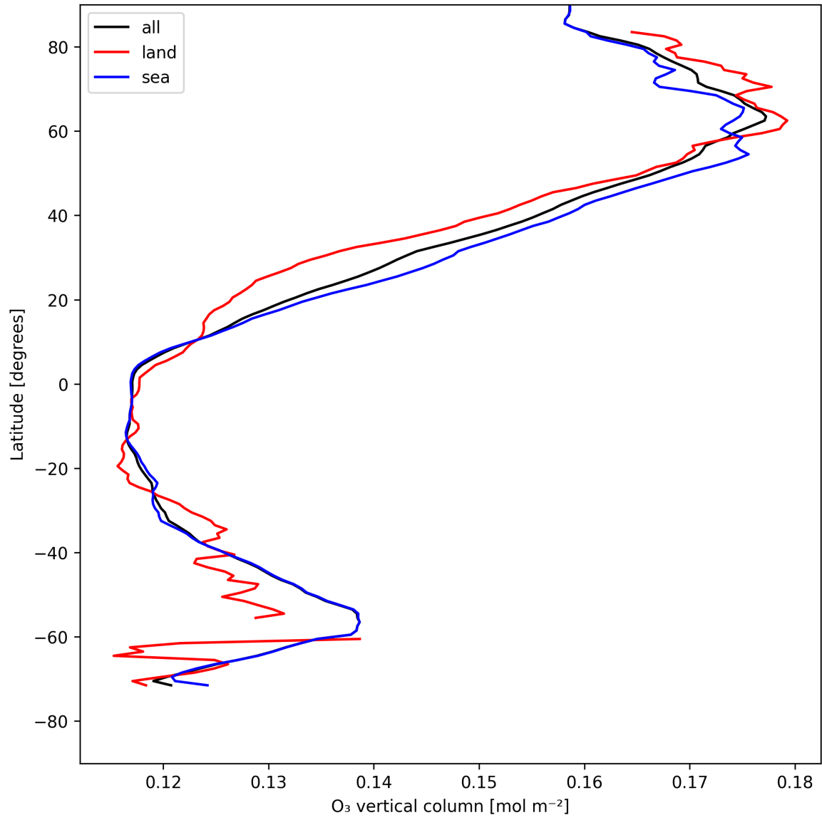
Figure 14: Zonal average of “O 3 vertical column” for 2025-05-08 to 2025-05-10.
