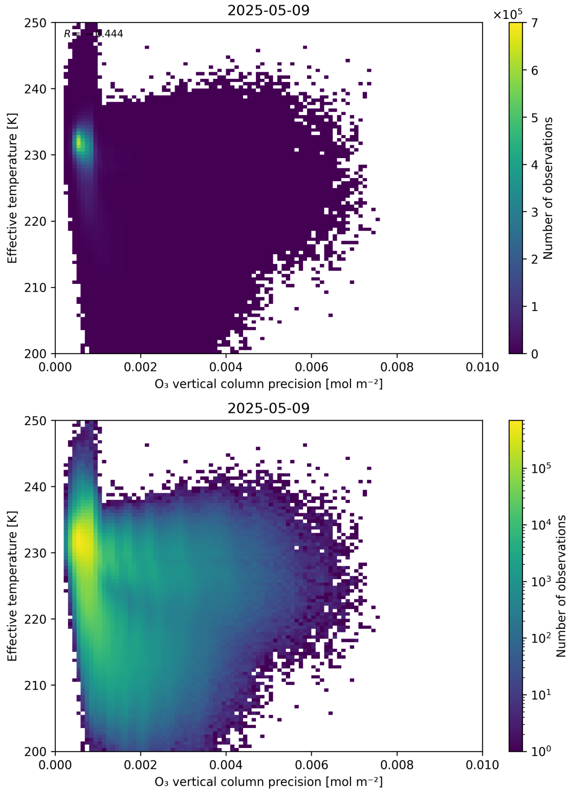
Figure 42: Scatter density plot of “O 3 vertical column precision” against “Effective temperature” for 2025-05-08 to 2025-05-10.
