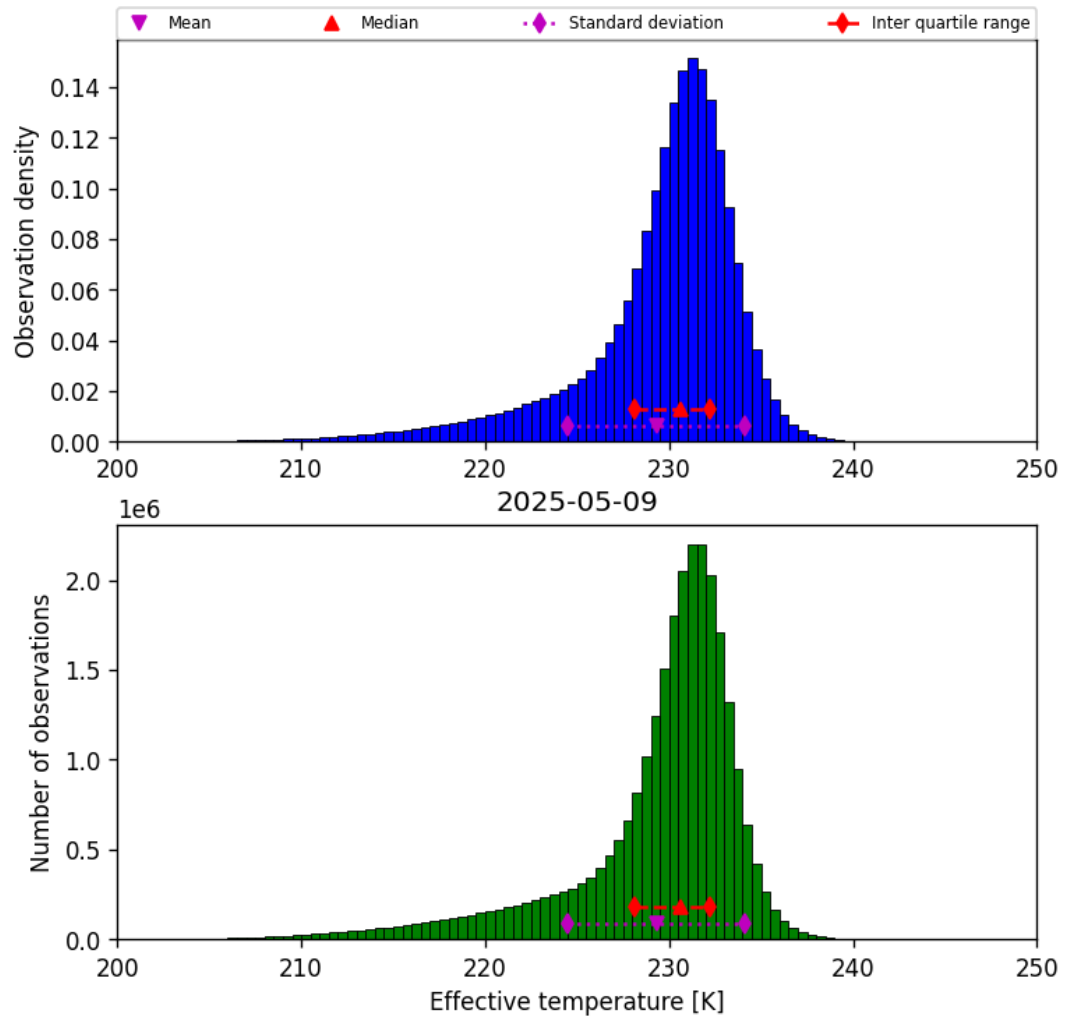
Figure 24: Histogram of “Effective temperature” for 2025-05-08 to 2025-05-10
