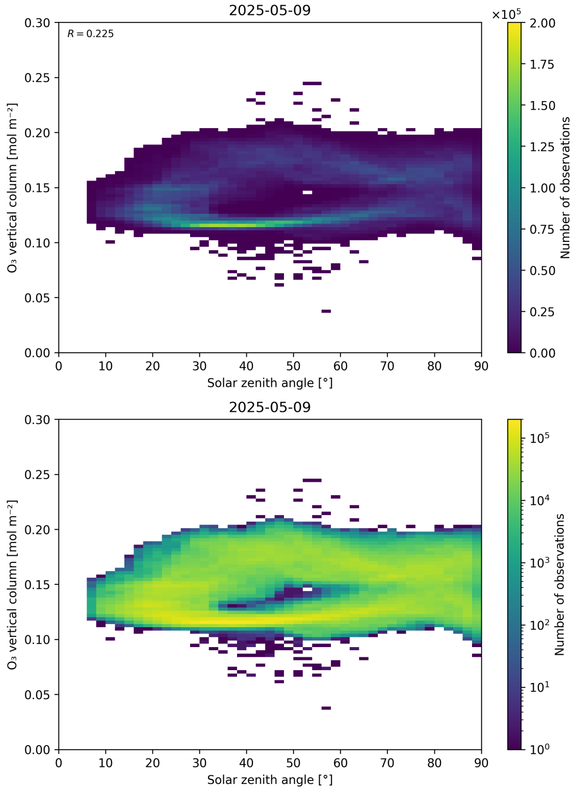
Figure 47: Scatter density plot of “Solar zenith angle” against “O 3 vertical column” for 2025-05-08 to 2025-05-10.
