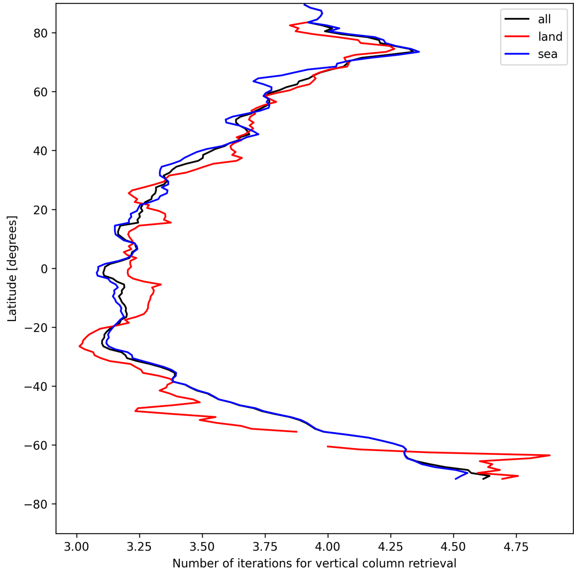
Figure 19: Zonal average of “Number of iterations for vertical column retrieval” for 2025-05-08 to 2025-05-10.
