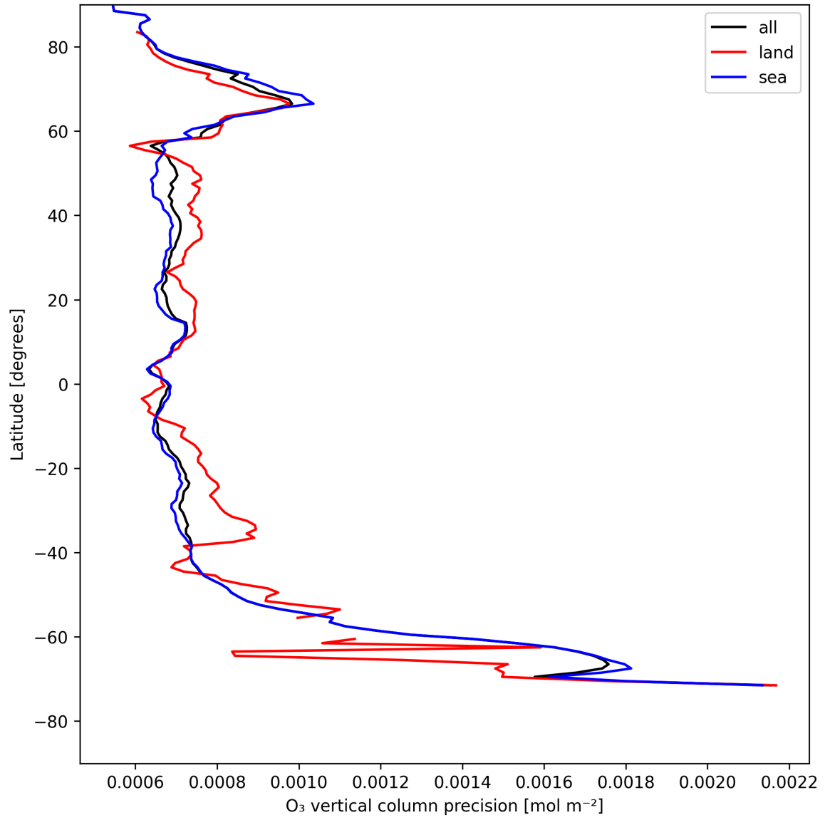
Figure 15: Zonal average of “O 3 vertical column precision” for 2025-05-08 to 2025-05-10.
