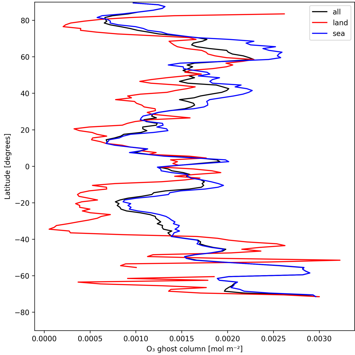
Figure 18: Zonal average of "O 3 ghost column" for 2025-05-08 to 2025-05-10.
