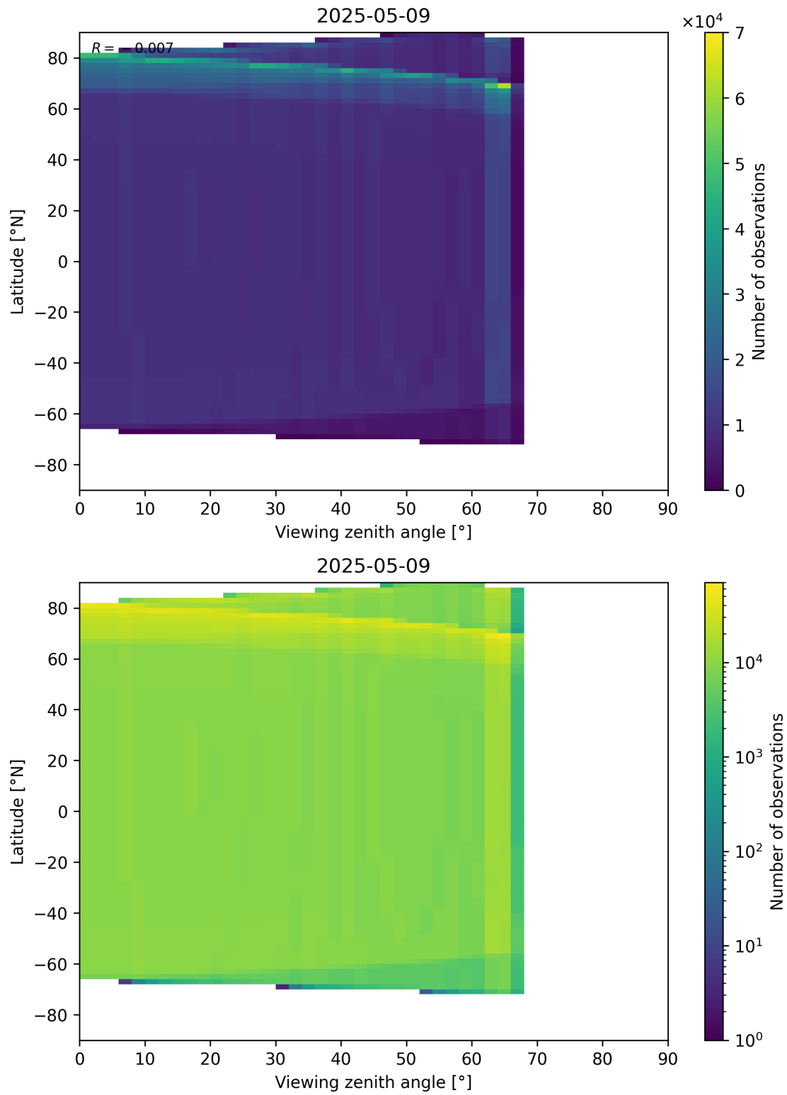
Figure 49: Scatter density plot of “Viewing zenith angle” against “Latitude” for 2025-05-08 to 2025-05-10.
