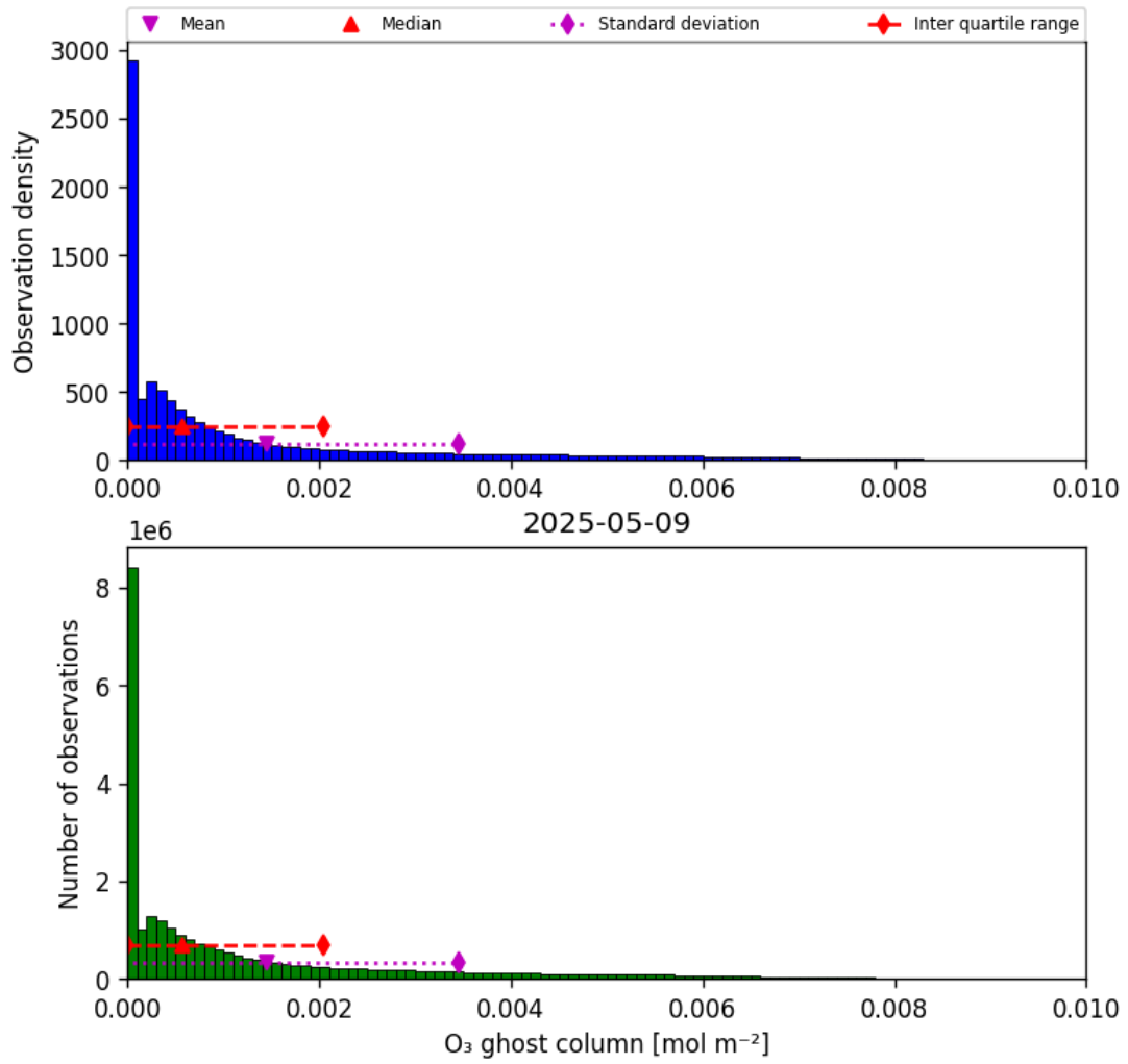
Figure 25: Histogram of “O 3 ghost column” for 2025-05-08 to 2025-05-10
