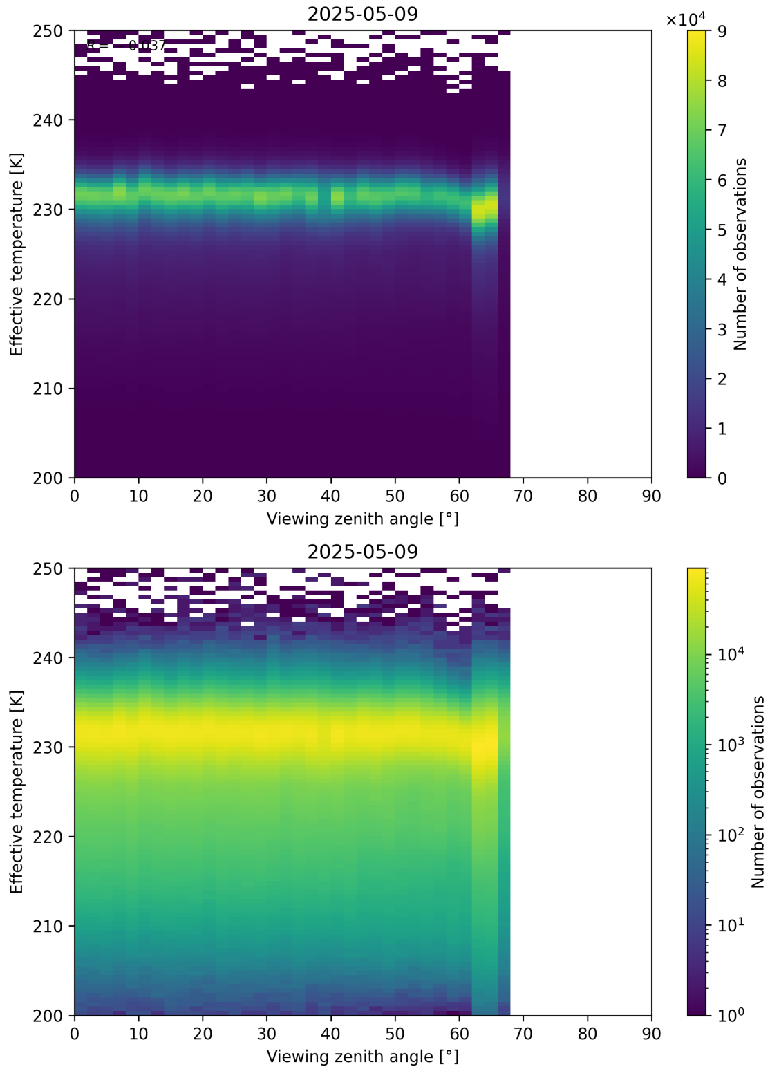
Figure 50: Scatter density plot of “Viewing zenith angle” against “Effective temperature” for 2025-05-08 to 2025-05-10.
