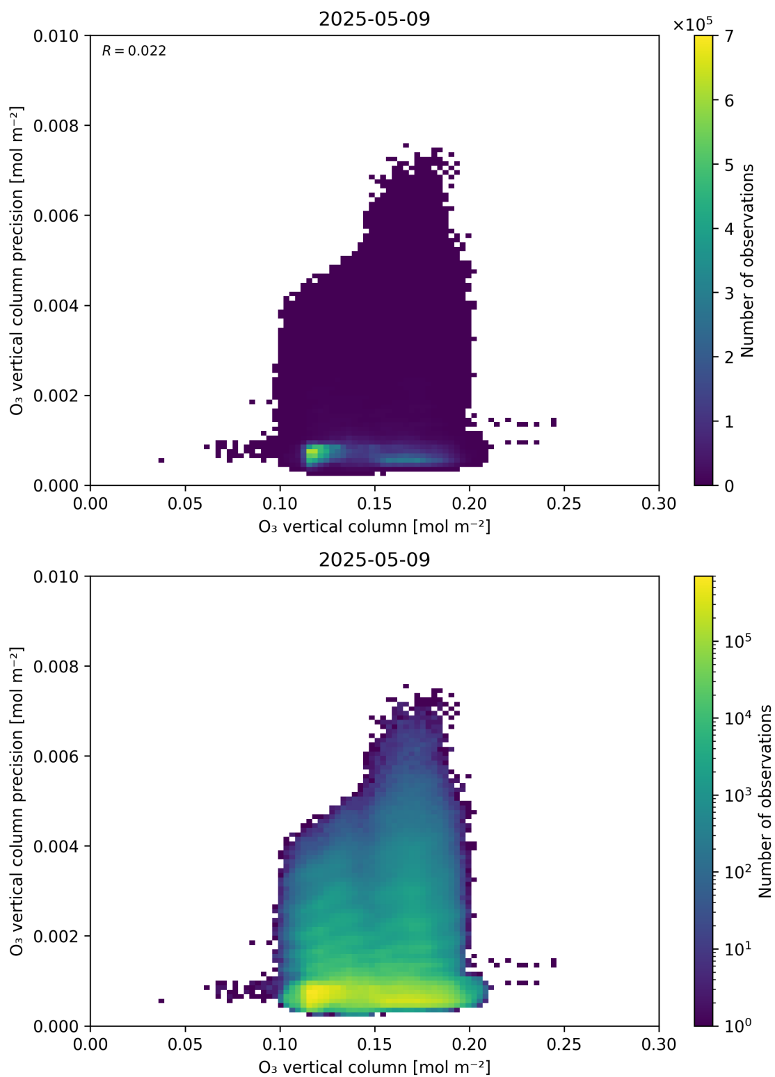
Figure 41: Scatter density plot of “O 3 vertical column” against “O 3 vertical column precision” for 2025-05-08 to 2025-05-10.
