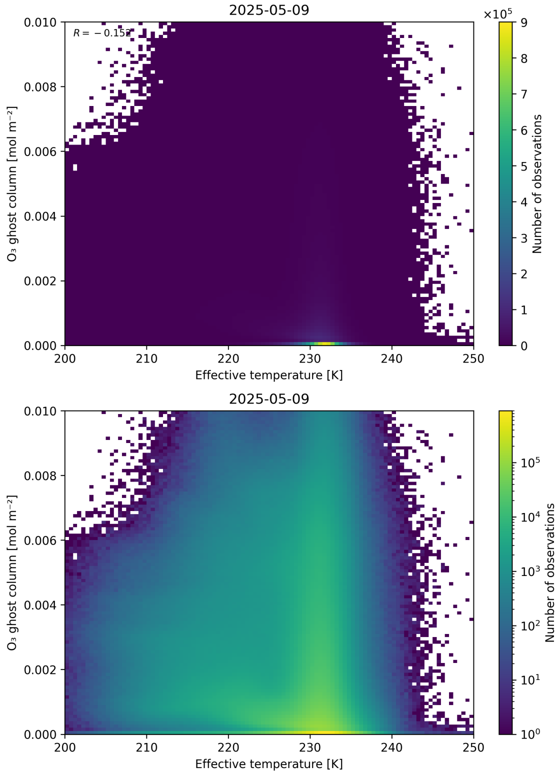
Figure 38: Scatter density plot of “Effective temperature” against “O 3 ghost column” for 2025-05-08 to 2025-05-10.
