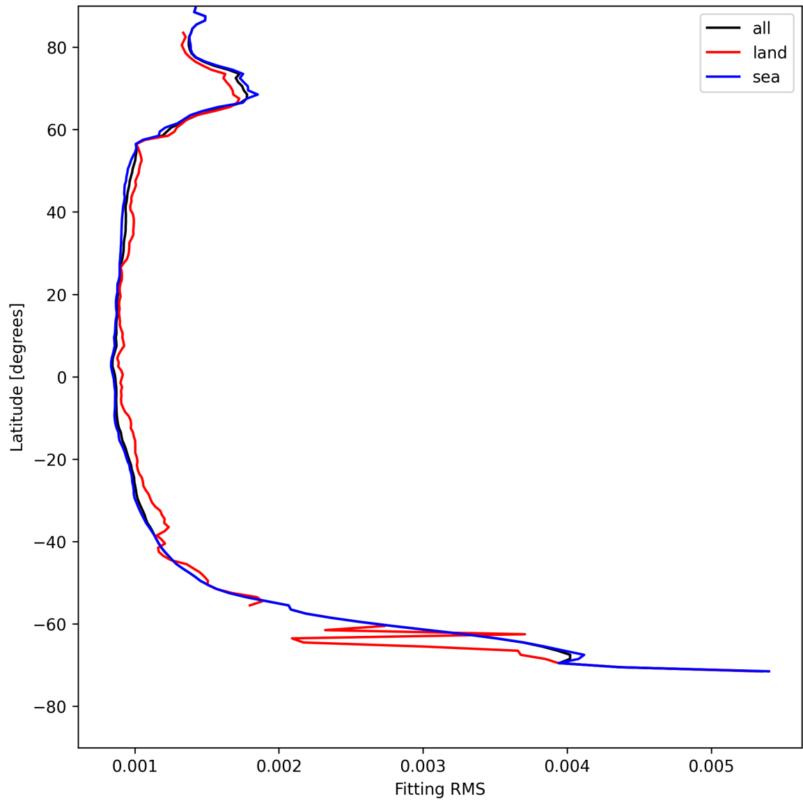
Figure 16: Zonal average of “Fitting RMS” for 2025-05-08 to 2025-05-10.
