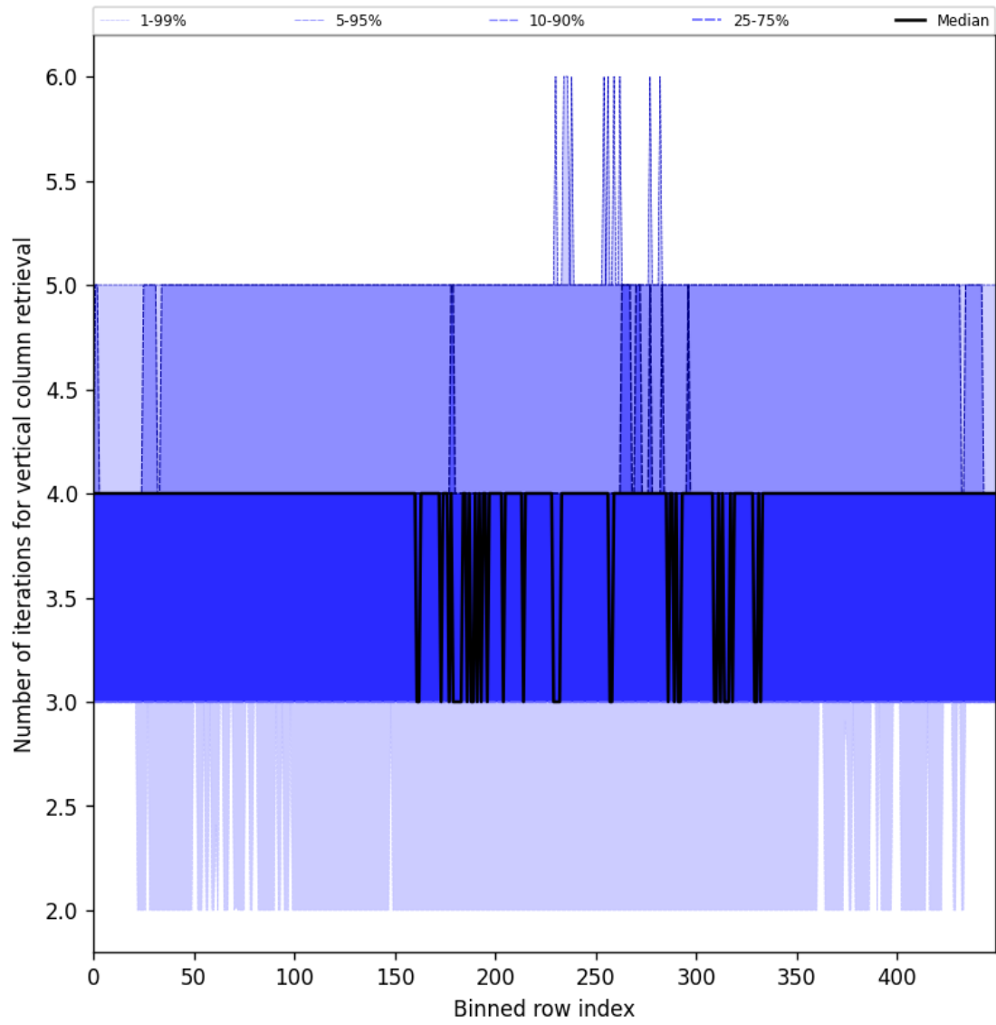
Figure 33: Along track statistics of “Number of iterations for vertical column retrieval” for 2025-05-08 to 2025-05-10
