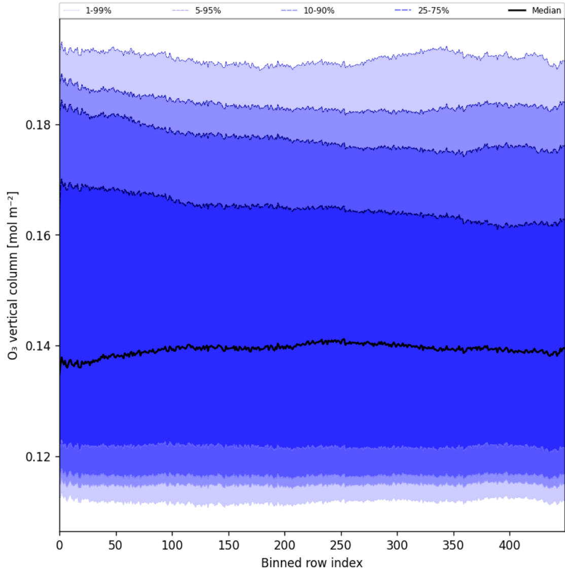
Figure 28: Along track statistics of “O 3 vertical column” for 2025-05-08 to 2025-05-10
