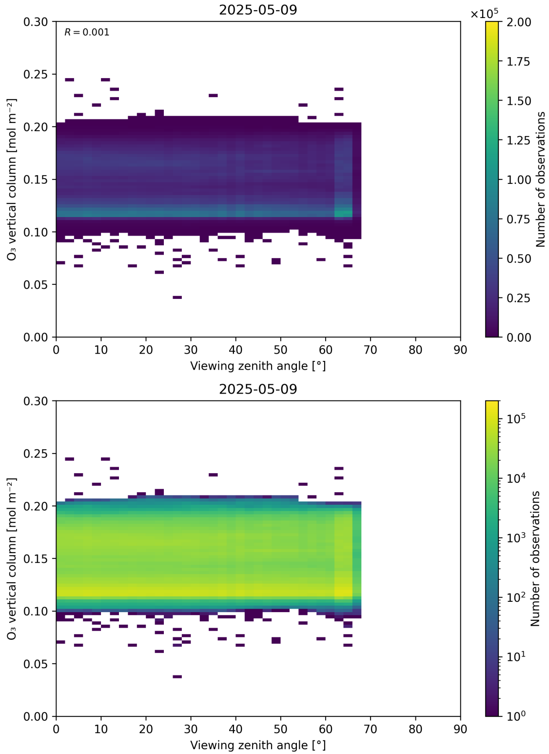
Figure 52: Scatter density plot of “Viewing zenith angle” against “O 3 vertical column” for 2025-05-08 to 2025-05-10.
