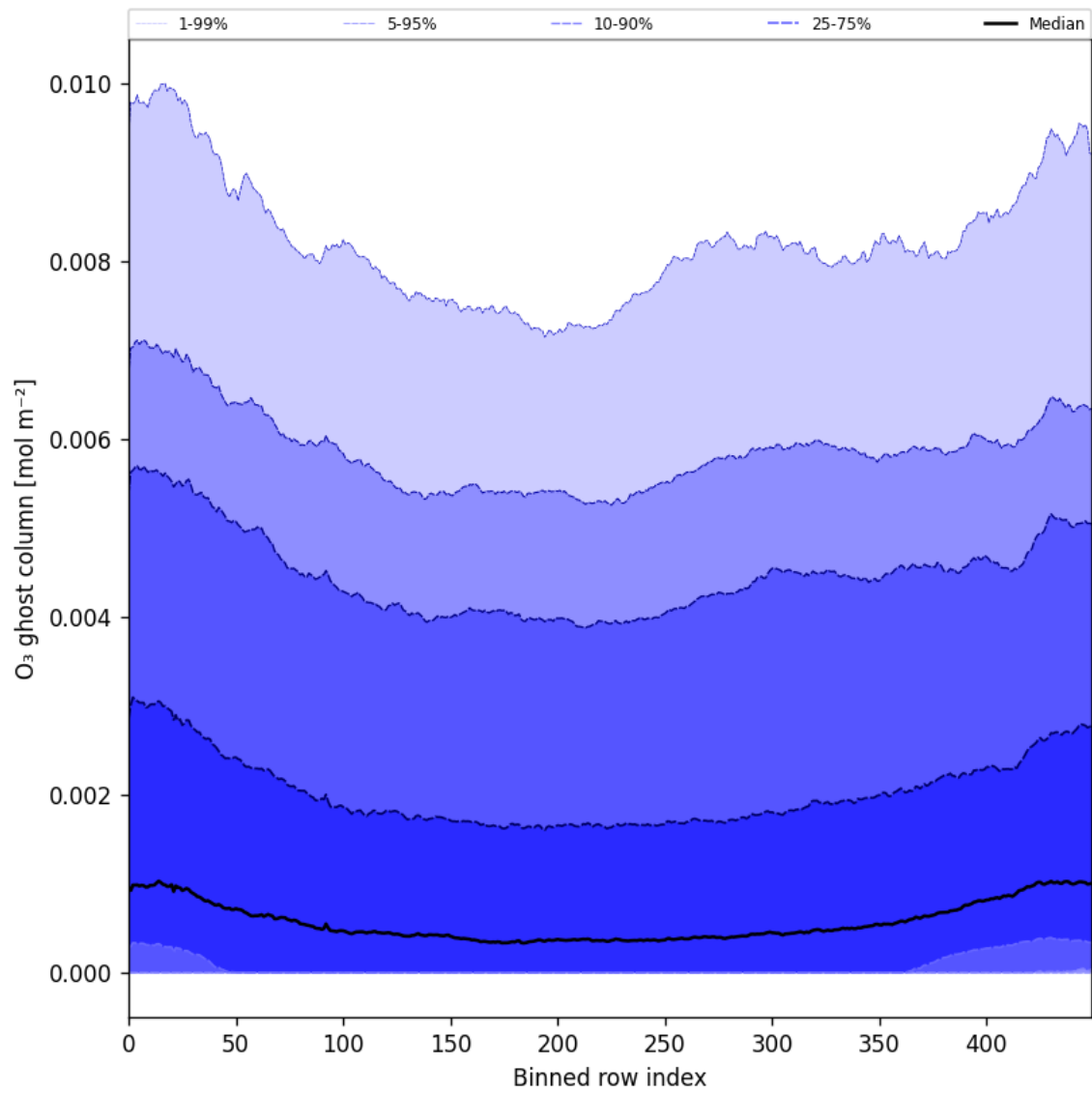
Figure 32: Along track statistics of “O 3 ghost column” for 2025-05-08 to 2025-05-10
