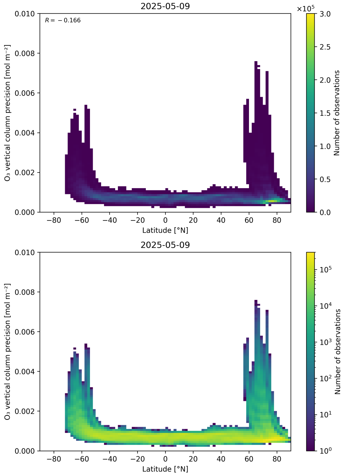
Figure 37: Scatter density plot of “Latitude” against “O 3 vertical column precision” for 2025-05-08 to 2025-05-10.
