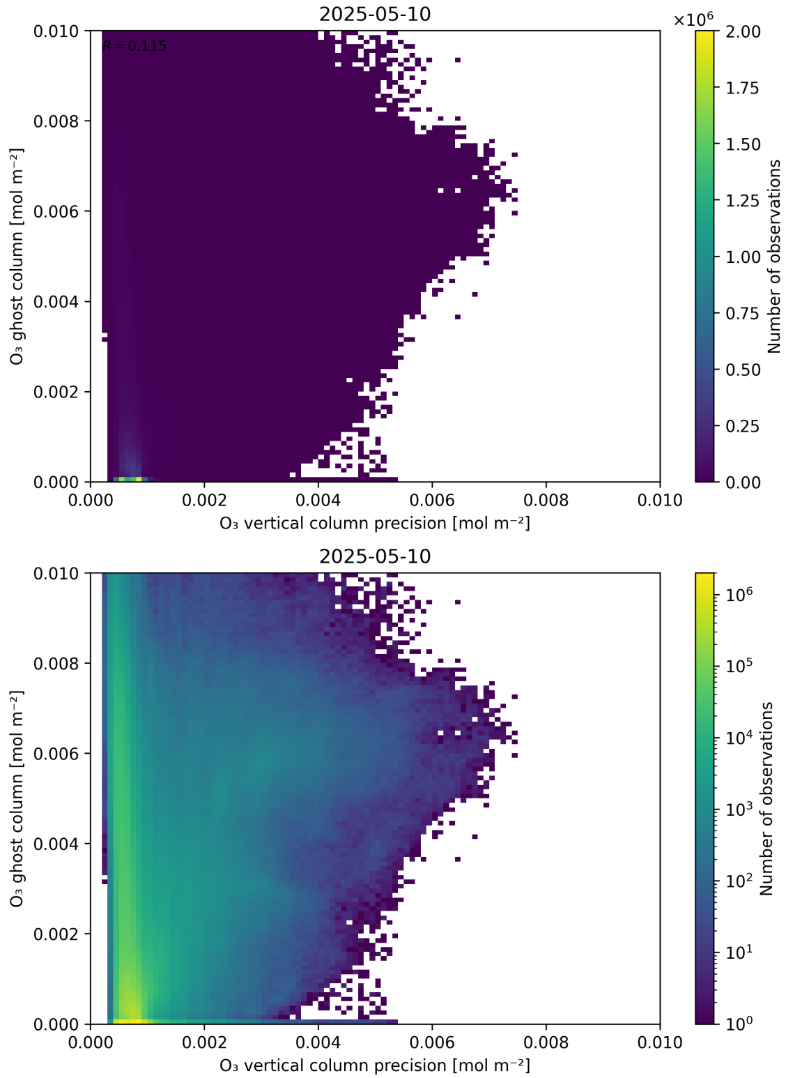
Figure 43: Scatter density plot of “O 3 vertical column precision” against “O 3 ghost column” for 2025-05-10 to 2025-05-11.
