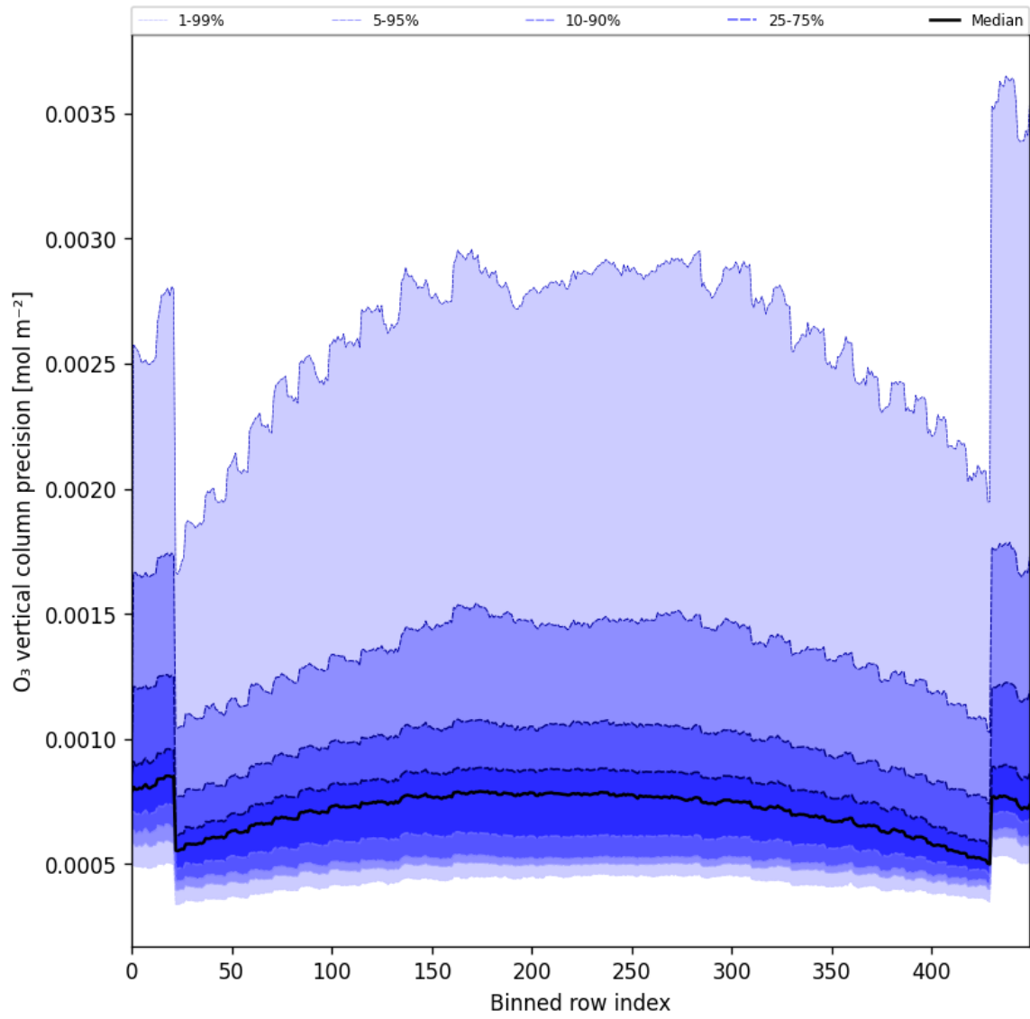
Figure 29: Along track statistics of “O 3 vertical column precision” for 2025-05-10 to 2025-05-11
