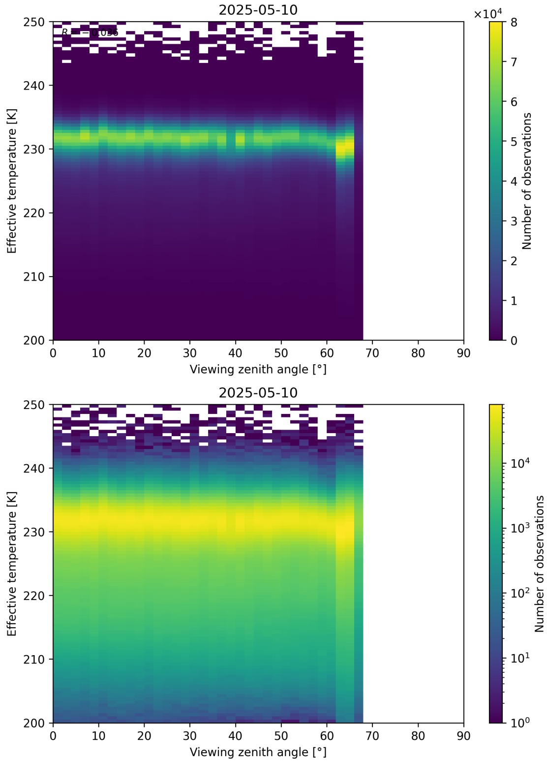
Figure 50: Scatter density plot of “Viewing zenith angle” against “Effective temperature” for 2025-05-10 to 2025-05-11.
