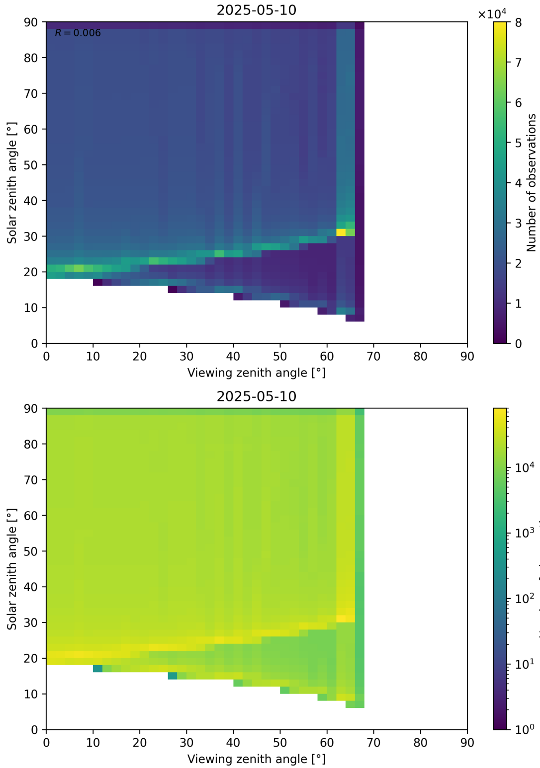
Figure 54: Scatter density plot of “Viewing zenith angle” against “Solar zenith angle” for 2025-05-10 to 2025-05-11.
