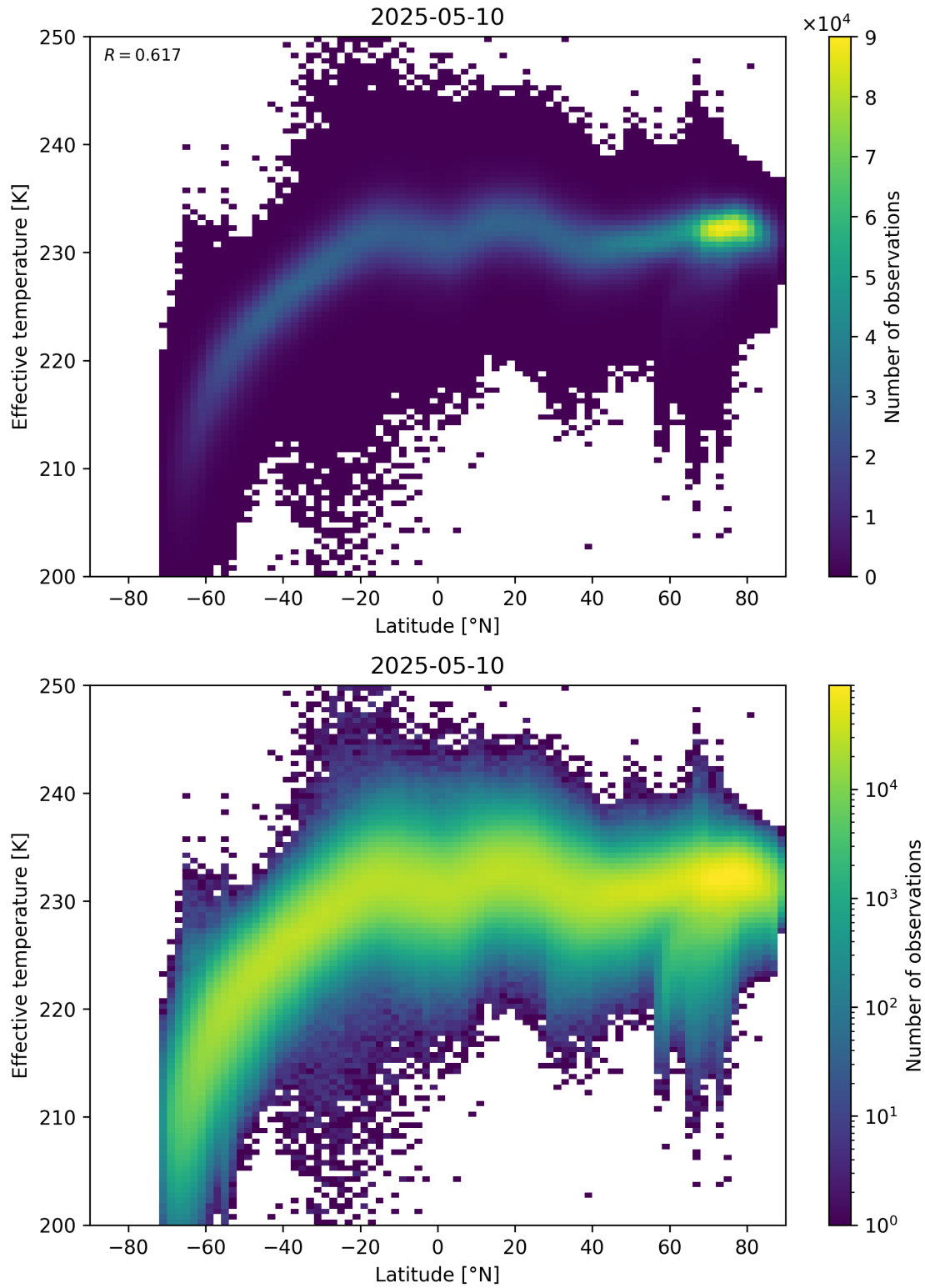
Figure 34: Scatter density plot of “Latitude” against “Effective temperature” for 2025-05-10 to 2025-05-11.
