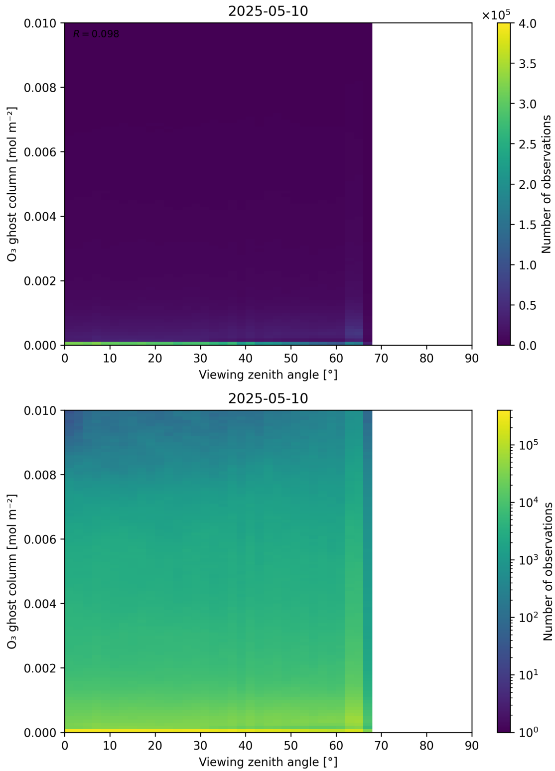
Figure 51: Scatter density plot of “Viewing zenith angle” against “O 3 ghost column” for 2025-05-10 to 2025-05-11.
