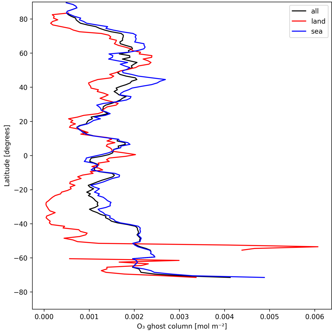
Figure 18: Zonal average of “O 3 ghost column” for 2025-05-10 to 2025-05-11.
