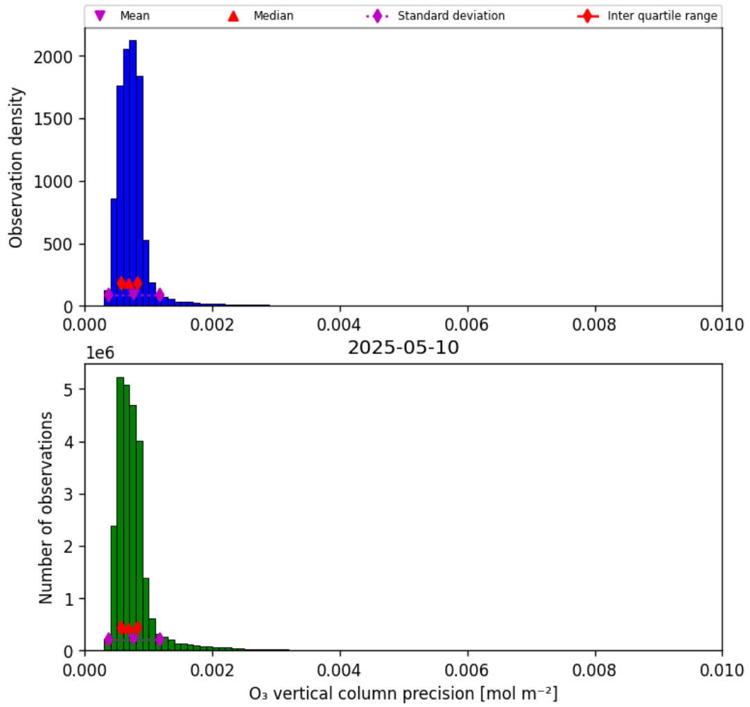
Figure 22: Histogram of “O 3 vertical column precision” for 2025-05-10 to 2025-05-11
