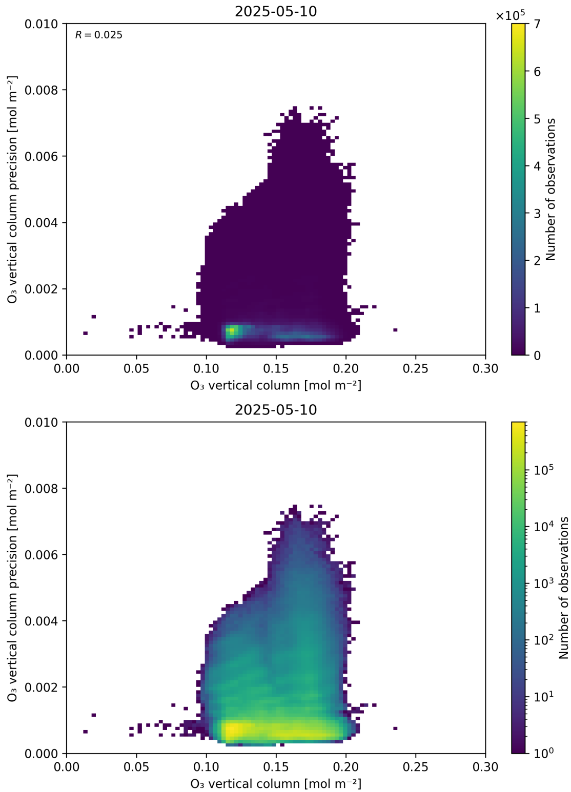
Figure 41: Scatter density plot of “O 3 vertical column” against “O 3 vertical column precision” for 2025-05-10 to 2025-05-11.
