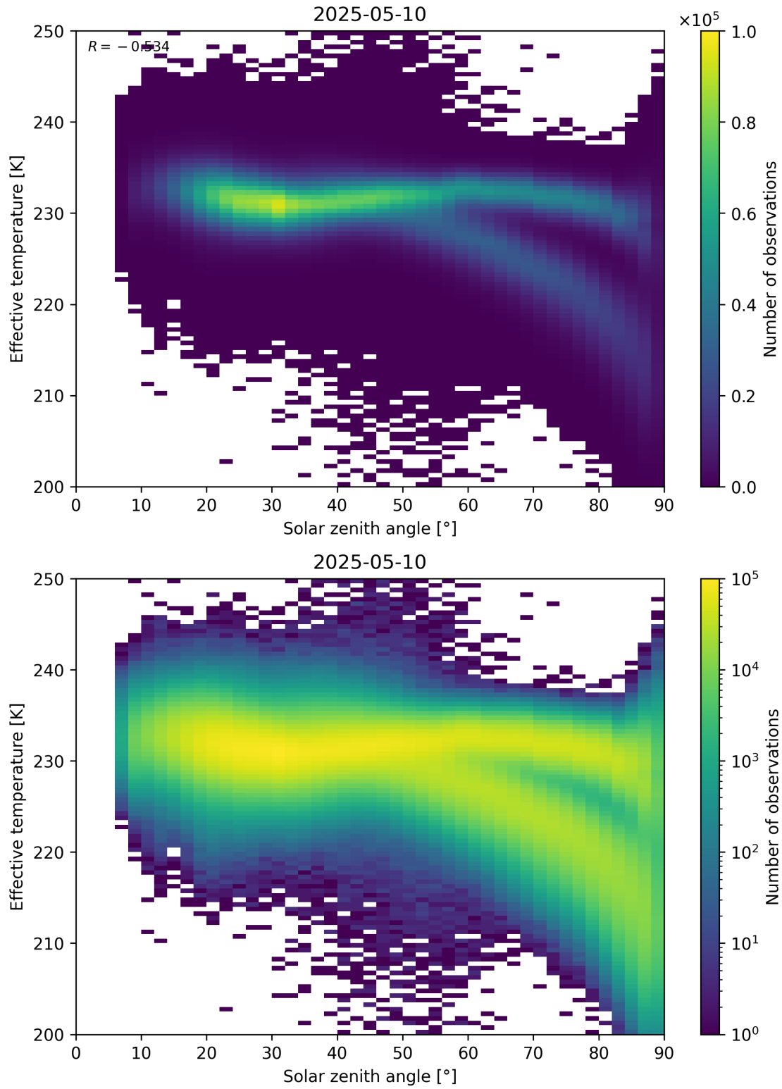
Figure 45: Scatter density plot of “Solar zenith angle” against “Effective temperature” for 2025-05-10 to 2025-05-11.
