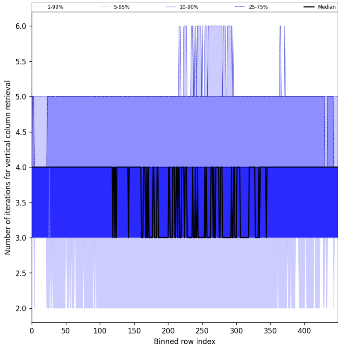
Figure 33: Along track statistics of “Number of iterations for vertical column retrieval” for 2025-05-10 to 2025-05-11
