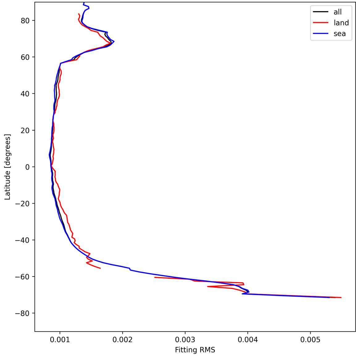
Figure 16: Zonal average of “Fitting RMS” for 2025-05-10 to 2025-05-11.
