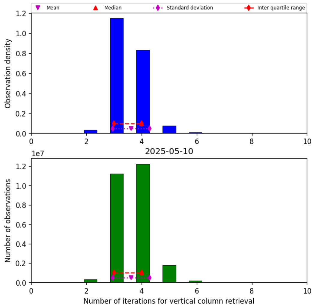
Figure 26: Histogram of “Number of iterations for vertical column retrieval” for 2025-05-10 to 2025-05-11
