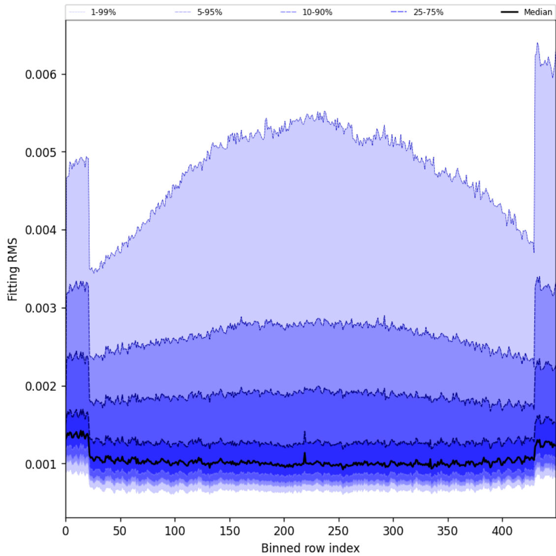
Figure 30: Along track statistics of “Fitting RMS” for 2025-05-10 to 2025-05-11
