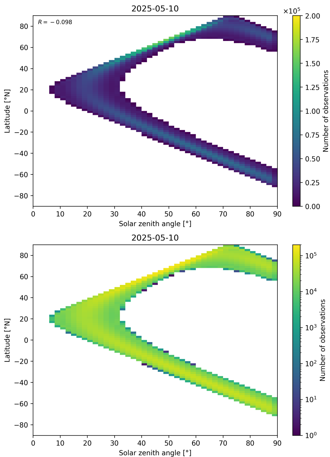
Figure 44: Scatter density plot of “Solar zenith angle” against “Latitude” for 2025-05-10 to 2025-05-11.
