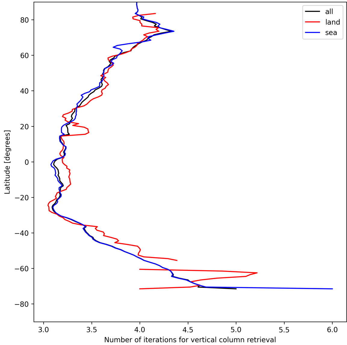
Figure 19: Zonal average of “Number of iterations for vertical column retrieval” for 2025-05-10 to 2025-05-11.
