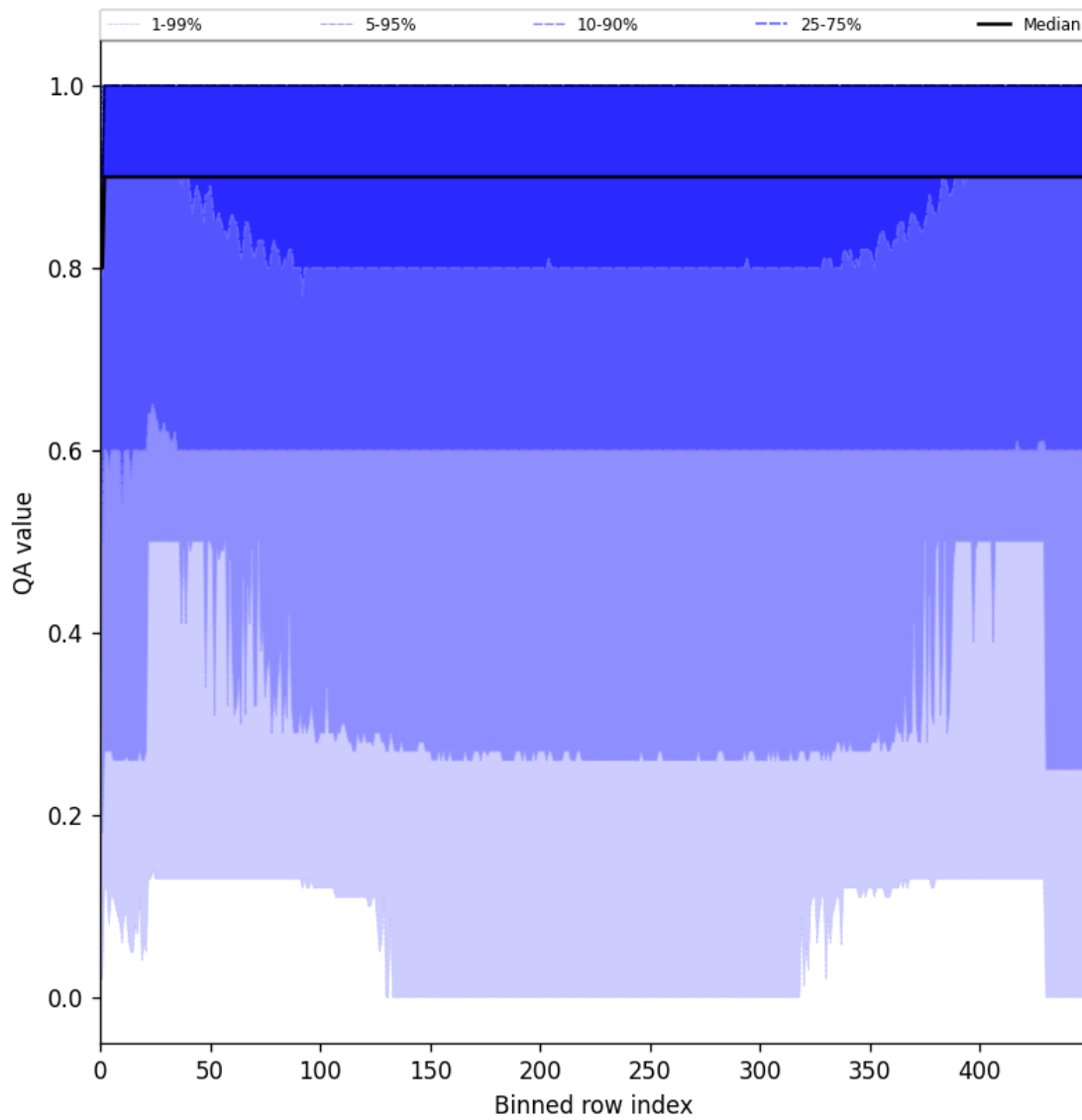
Figure 27: Along track statistics of “QA value” for 2025-05-10 to 2025-05-11
