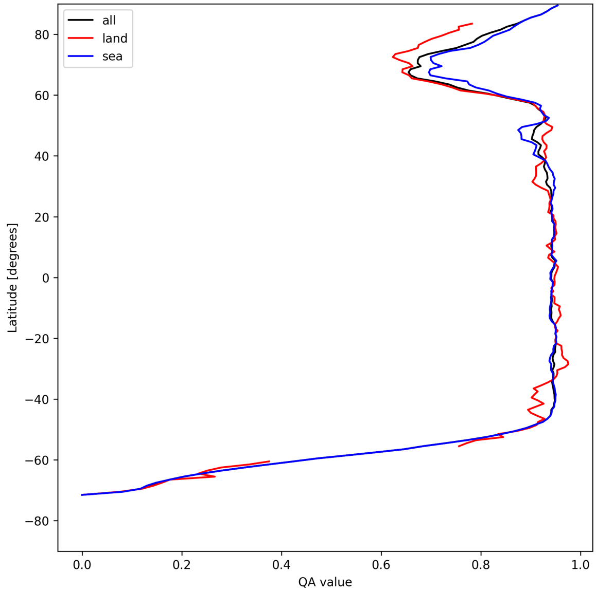
Figure 13: Zonal average of “QA value” for 2025-05-10 to 2025-05-11.
