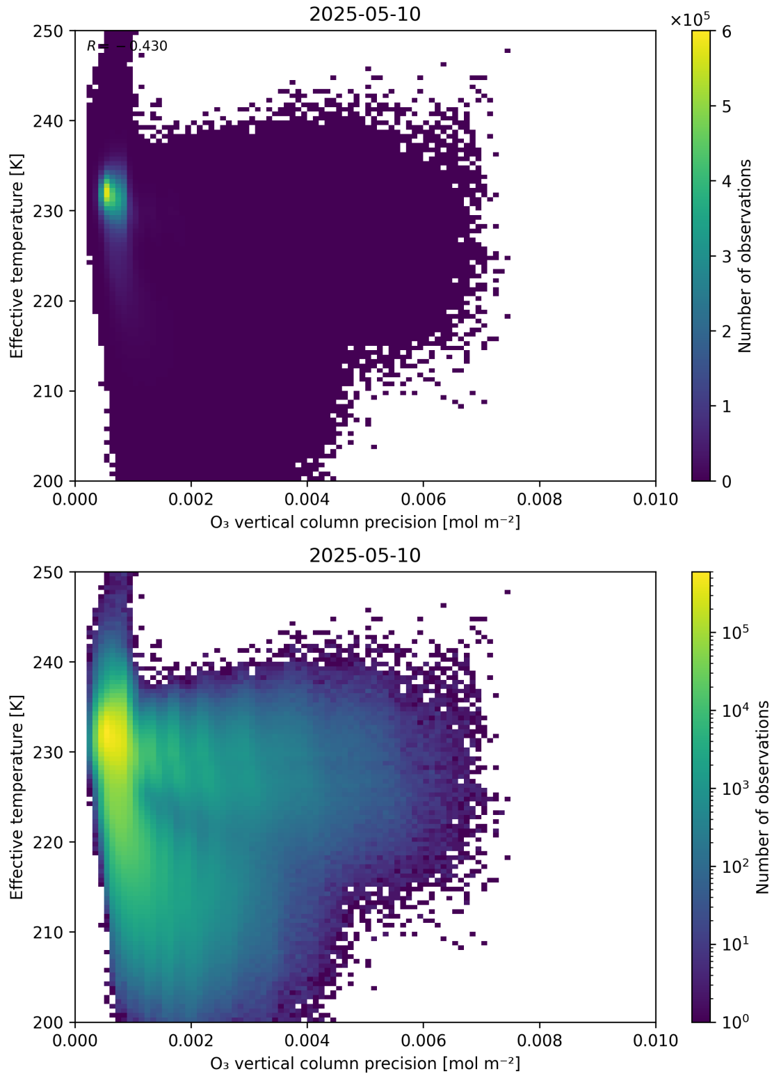
Figure 42: Scatter density plot of “O 3 vertical column precision” against “Effective temperature” for 2025-05-10 to 2025-05-11.
