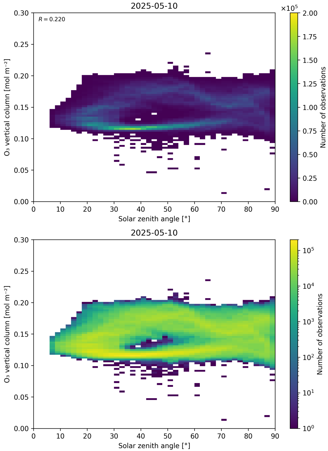
Figure 47: Scatter density plot of “Solar zenith angle” against “O 3 vertical column” for 2025-05-10 to 2025-05-11.
