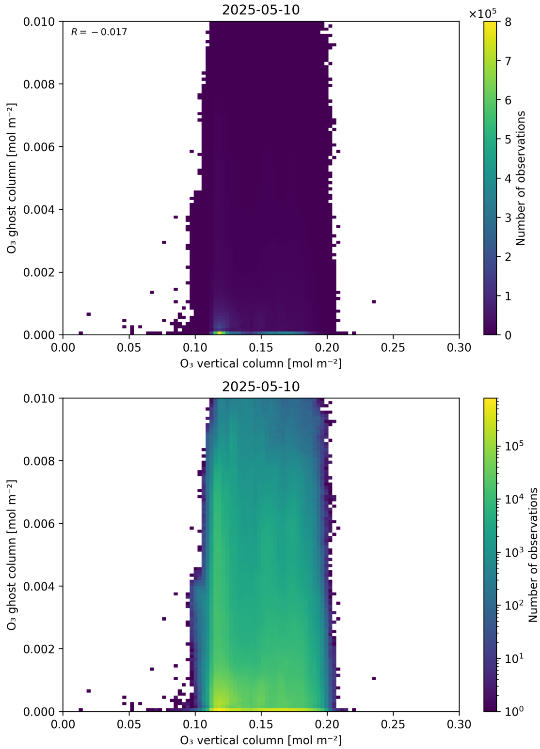
Figure 40: Scatter density plot of “O 3 vertical column” against “O 3 ghost column” for 2025-05-10 to 2025-05-11.
