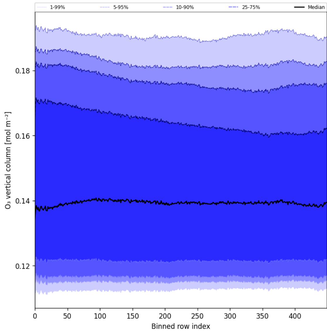
Figure 28: Along track statistics of “O 3 vertical column” for 2025-05-10 to 2025-05-11
