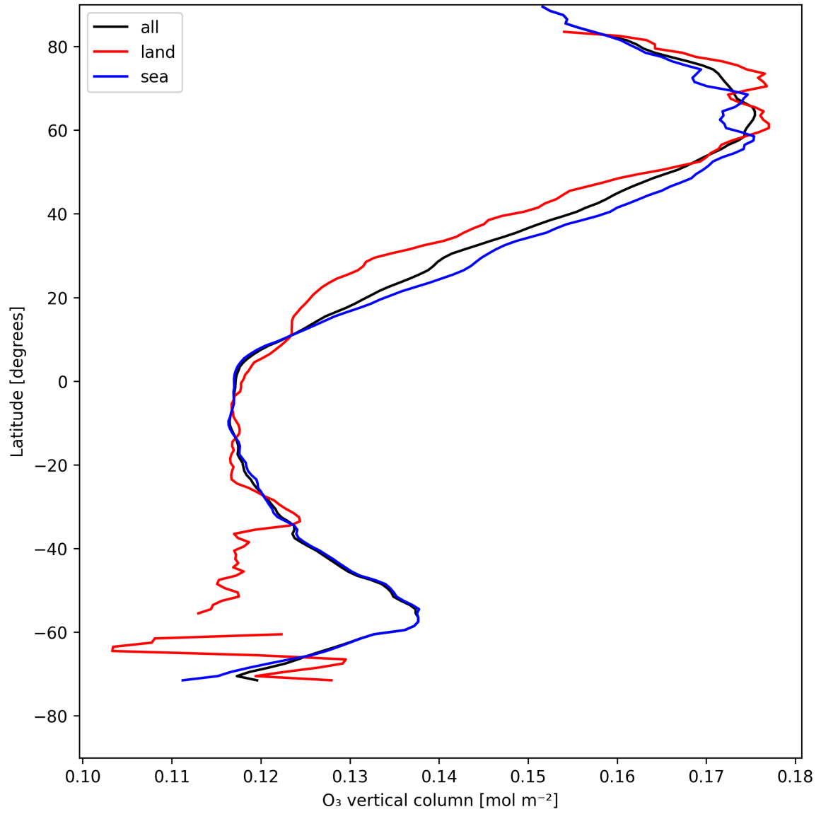
Figure 14: Zonal average of “O 3 vertical column” for 2025-05-10 to 2025-05-11.
