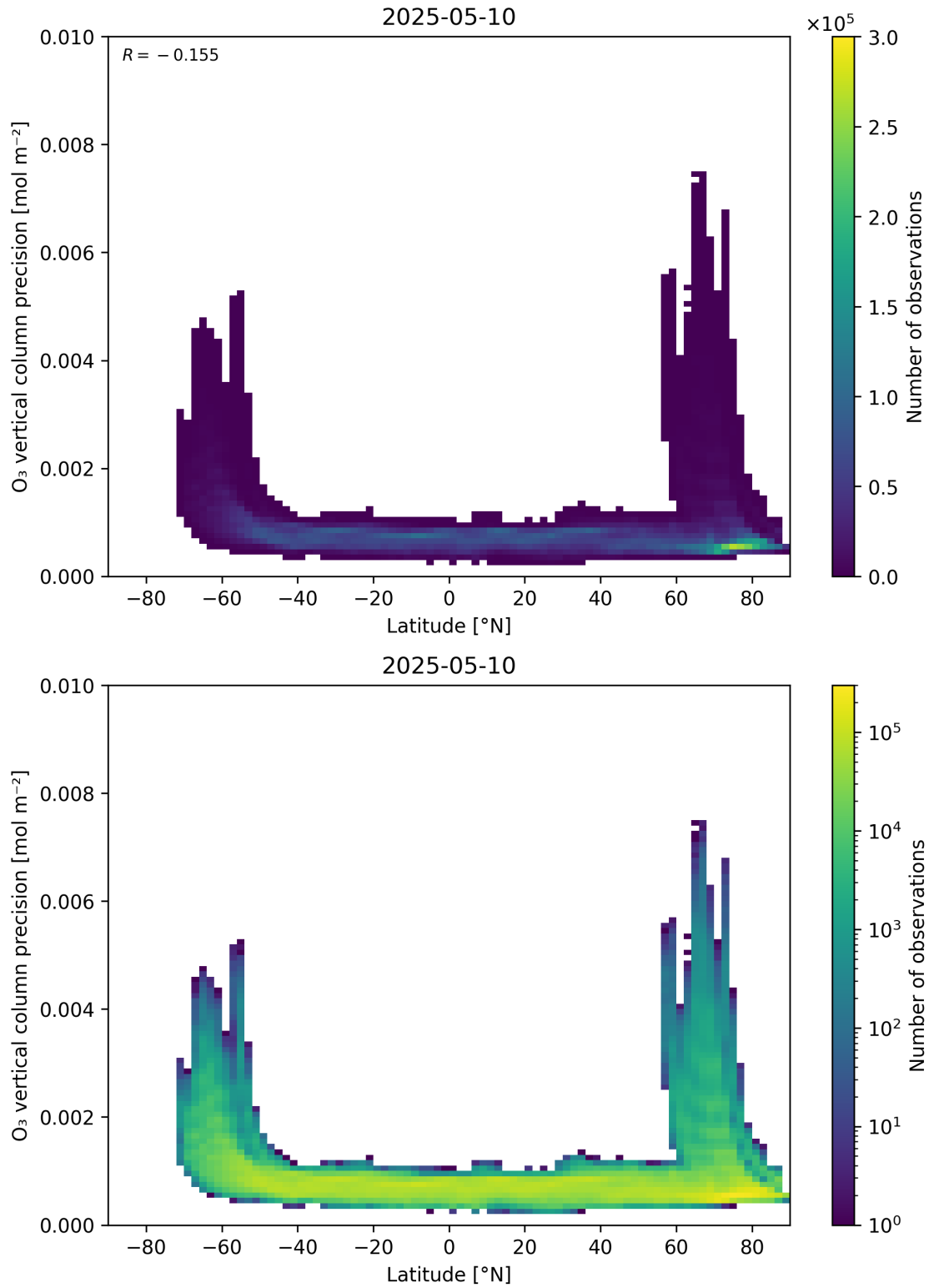
Figure 37: Scatter density plot of “Latitude” against “O 3 vertical column precision” for 2025-05-10 to 2025-05-11.
