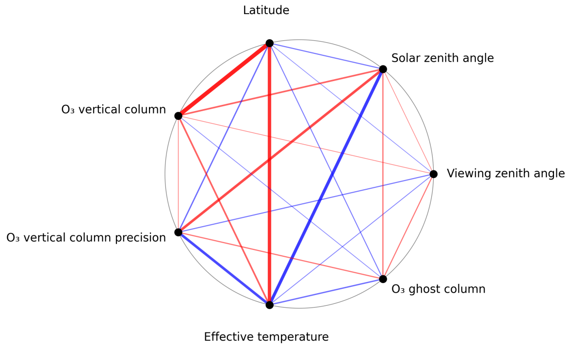
Figure 1: Map of correlation graph for 2025-05-10 to 2025-05-11.
