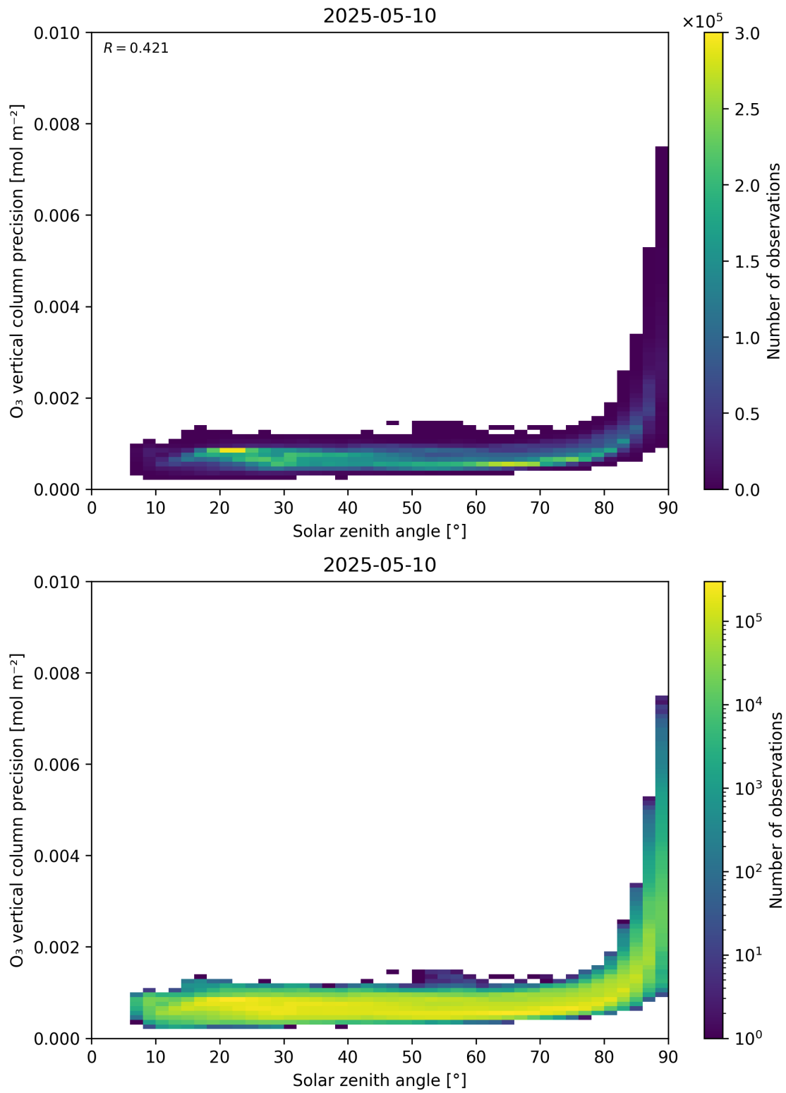
Figure 48: Scatter density plot of “Solar zenith angle” against “O 3 vertical column precision” for 2025-05-10 to 2025-05-11.
