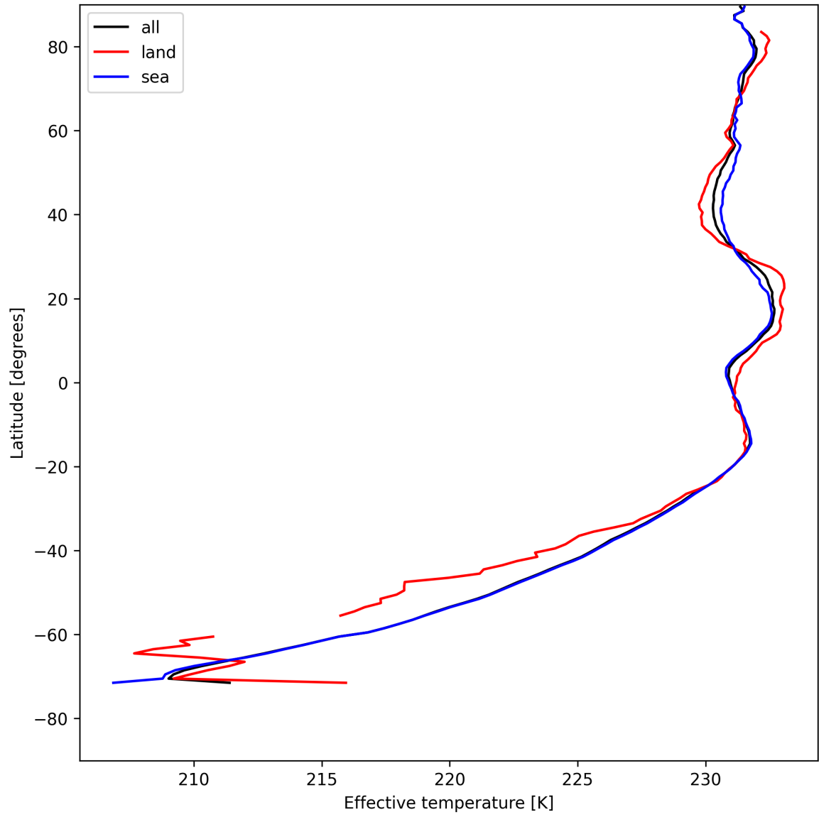
Figure 17: Zonal average of "Effective temperature" for 2025-05-10 to 2025-05-11.
