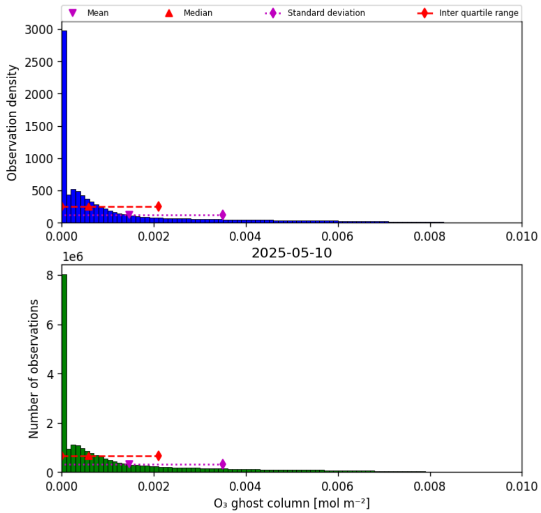
Figure 25: Histogram of “O 3 ghost column” for 2025-05-10 to 2025-05-11
