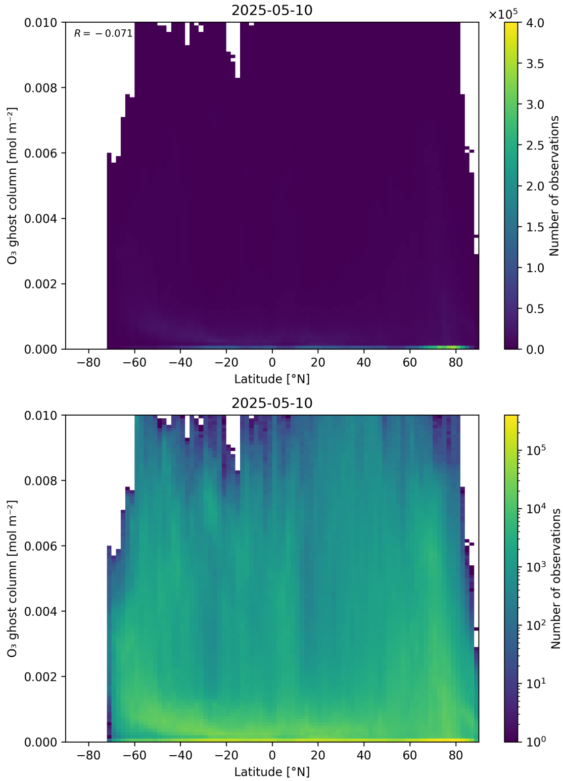
Figure 35: Scatter density plot of “Latitude” against “O 3 ghost column” for 2025-05-10 to 2025-05-11.
