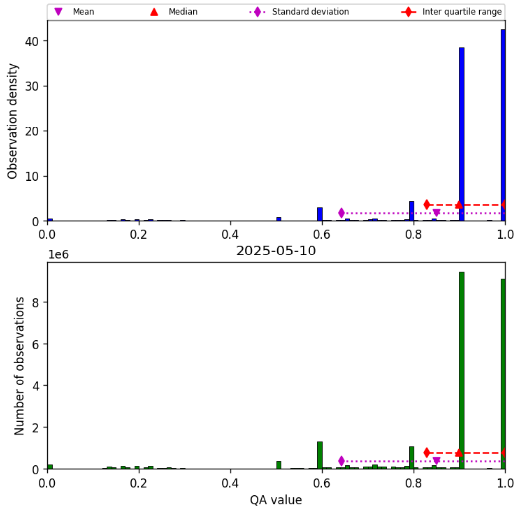
Figure 20: Histogram of “QA value” for 2025-05-10 to 2025-05-11
