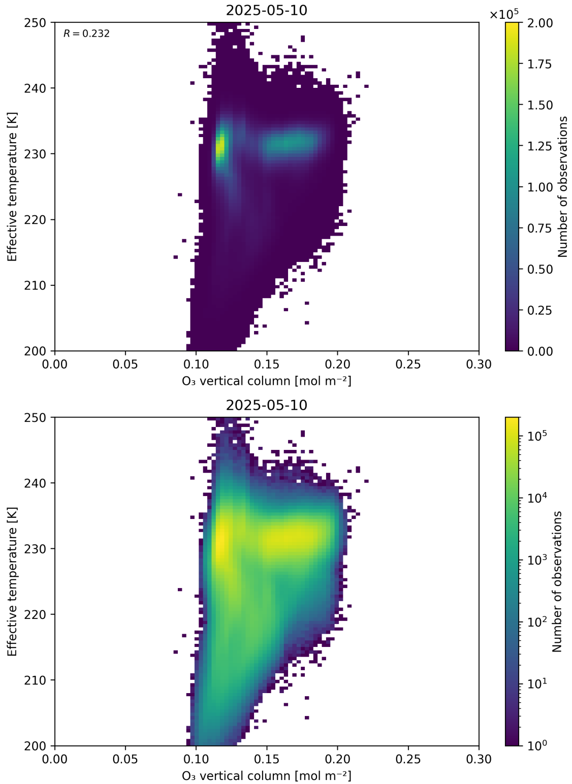
Figure 39: Scatter density plot of “O 3 vertical column” against “Effective temperature” for 2025-05-10 to 2025-05-11.
