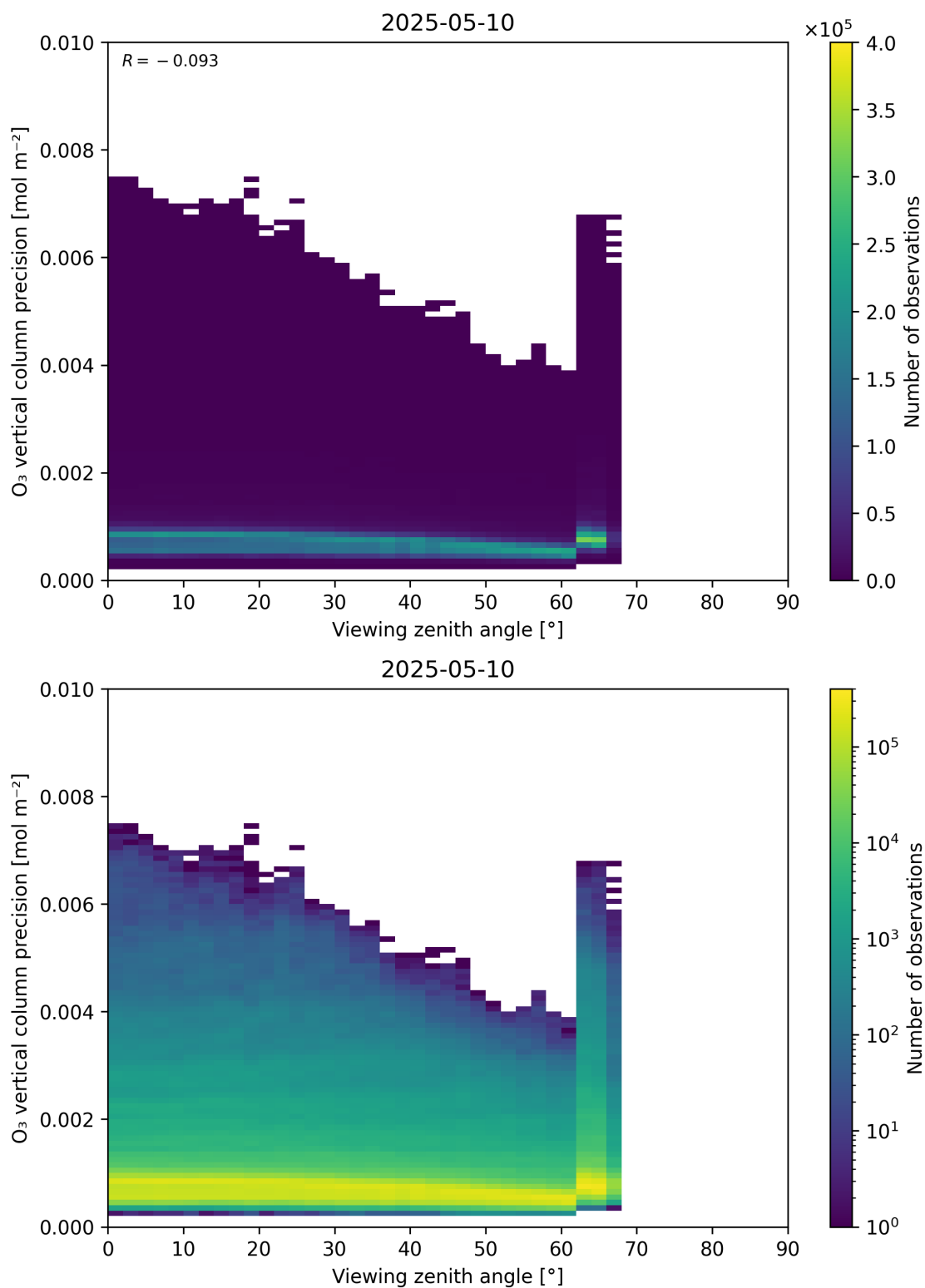
Figure 53: Scatter density plot of “Viewing zenith angle” against “O 3 vertical column precision” for 2025-05-10 to 2025-05-11.
