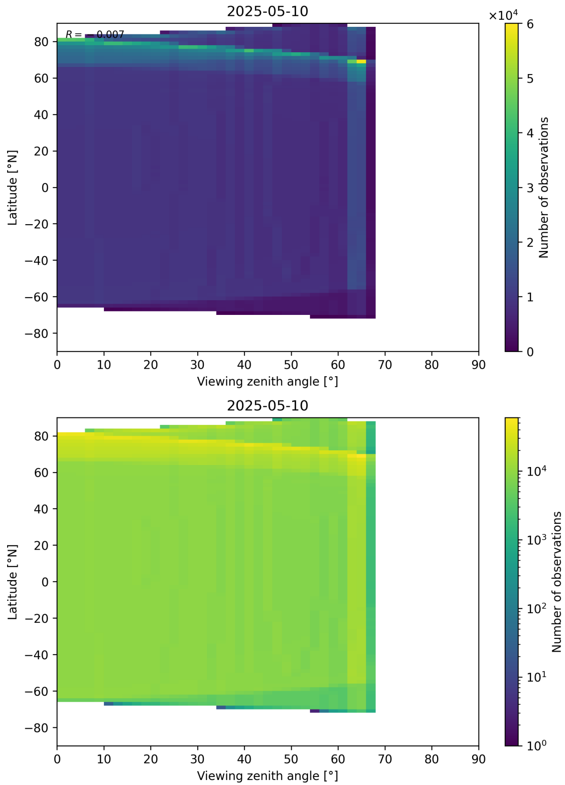
Figure 49: Scatter density plot of “Viewing zenith angle” against “Latitude” for 2025-05-10 to 2025-05-11.
