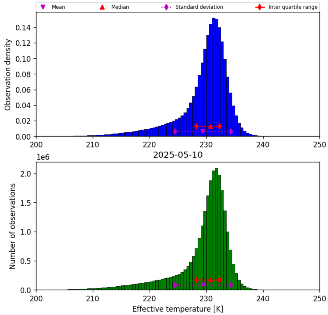
Figure 24: Histogram of “Effective temperature” for 2025-05-10 to 2025-05-11
