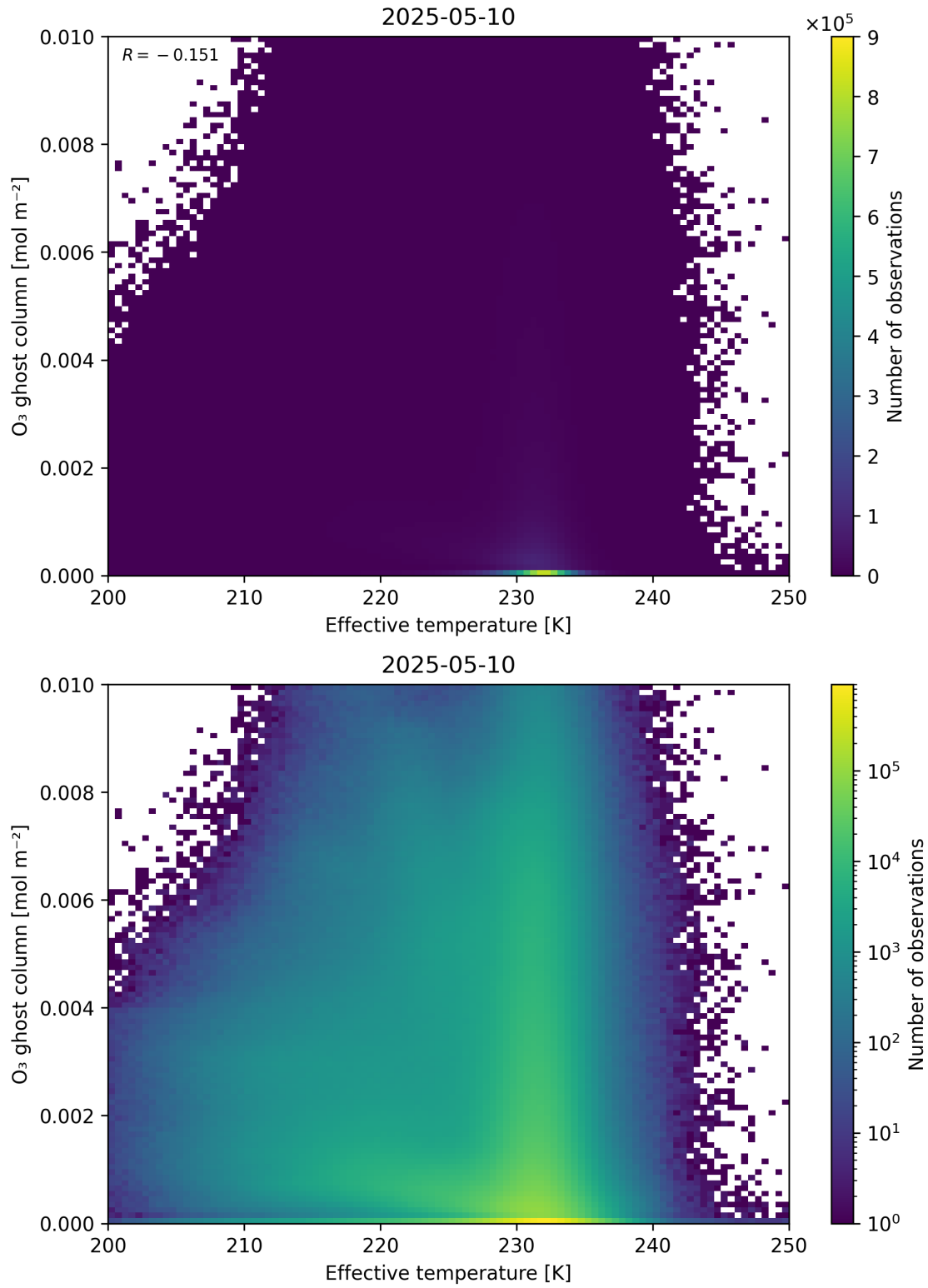
Figure 38: Scatter density plot of “Effective temperature” against “O 3 ghost column” for 2025-05-10 to 2025-05-11.
