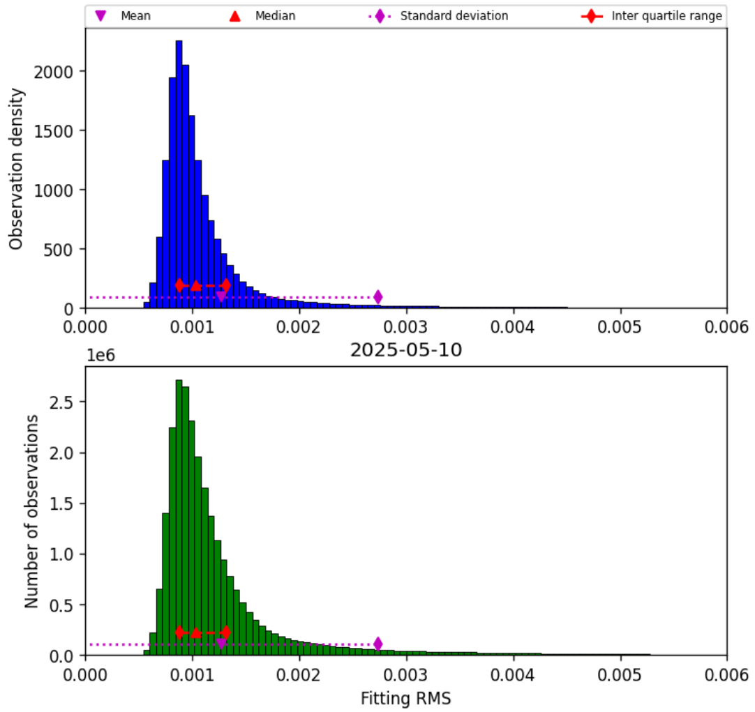
Figure 23: Histogram of “Fitting RMS” for 2025-05-10 to 2025-05-11
