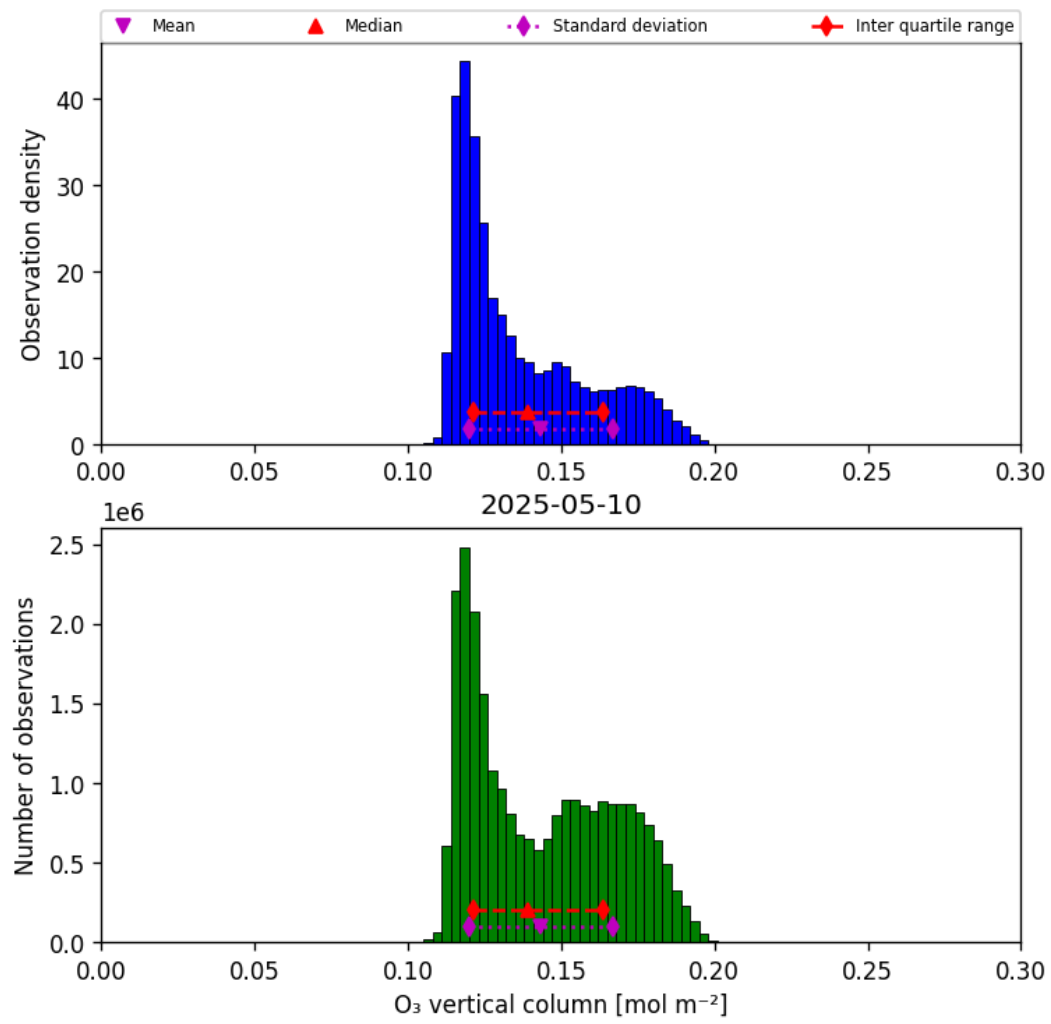
Figure 21: Histogram of “O 3 vertical column” for 2025-05-10 to 2025-05-11
