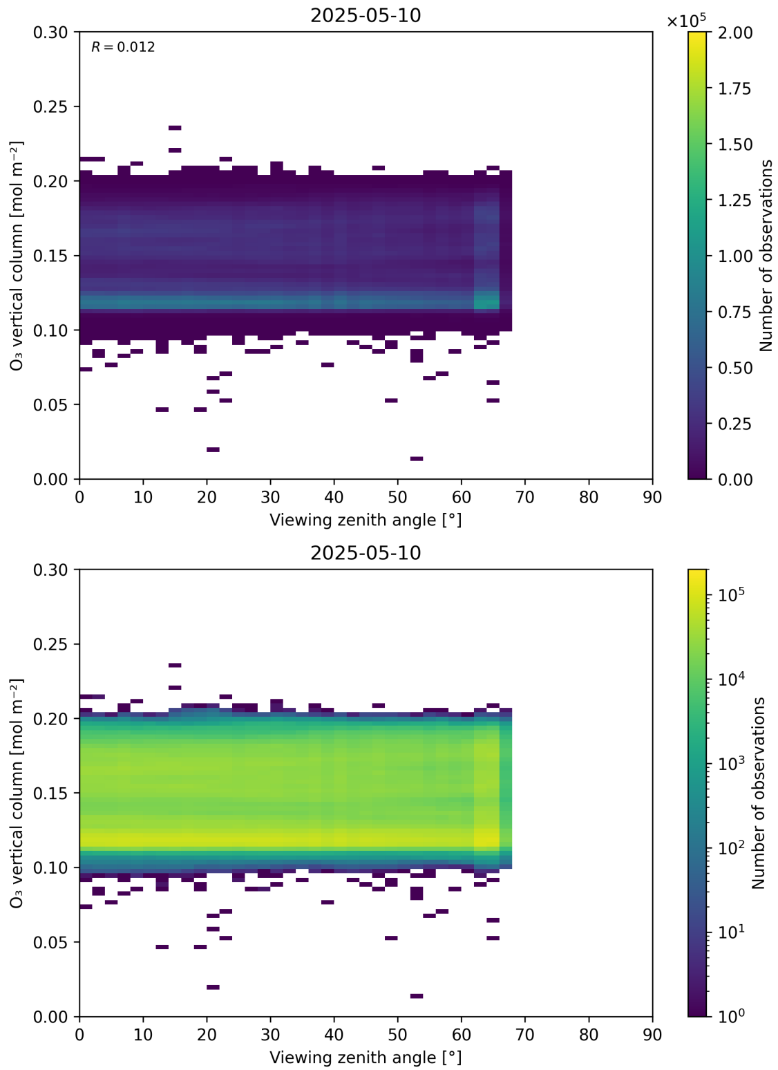
Figure 52: Scatter density plot of “Viewing zenith angle” against “O 3 vertical column” for 2025-05-10 to 2025-05-11.
