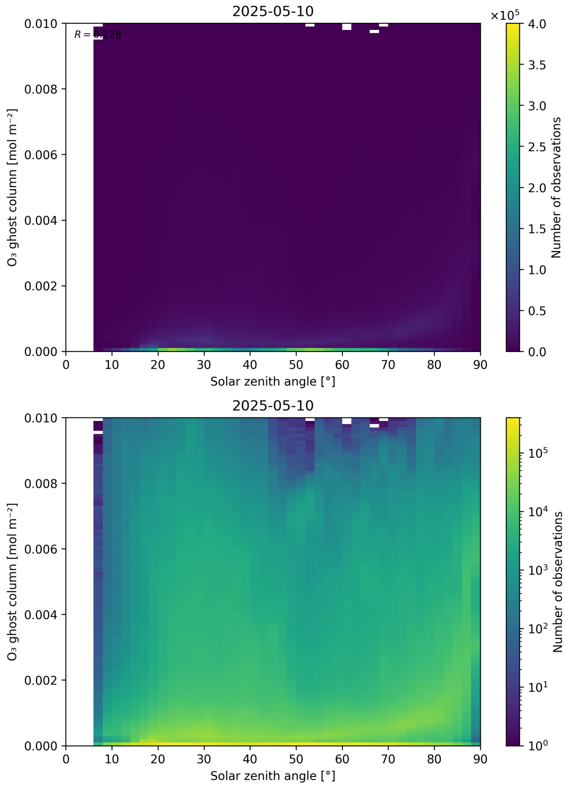
Figure 46: Scatter density plot of “Solar zenith angle” against “O 3 ghost column” for 2025-05-10 to 2025-05-11.
