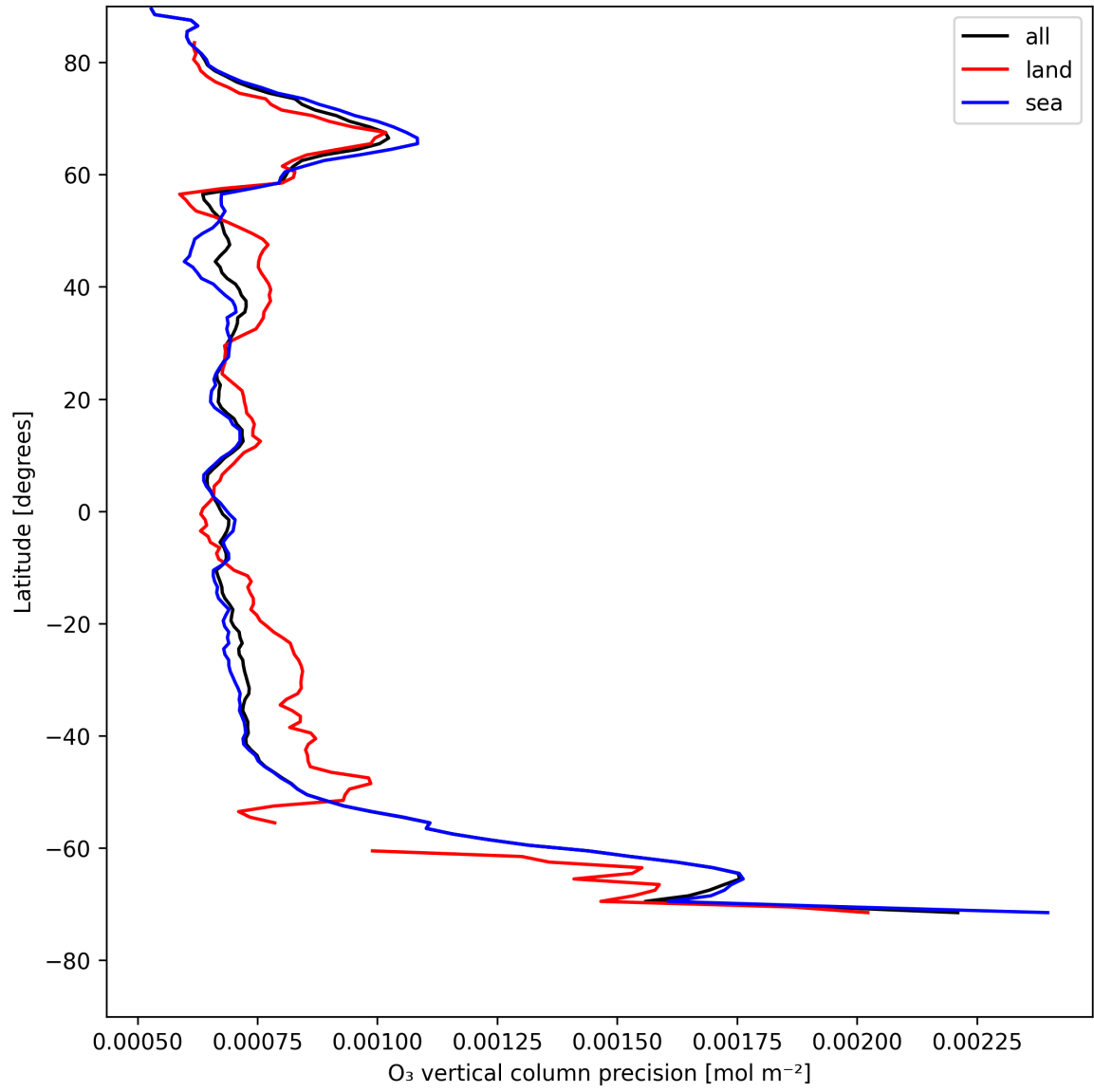
Figure 15: Zonal average of “O 3 vertical column precision” for 2025-05-10 to 2025-05-11.
