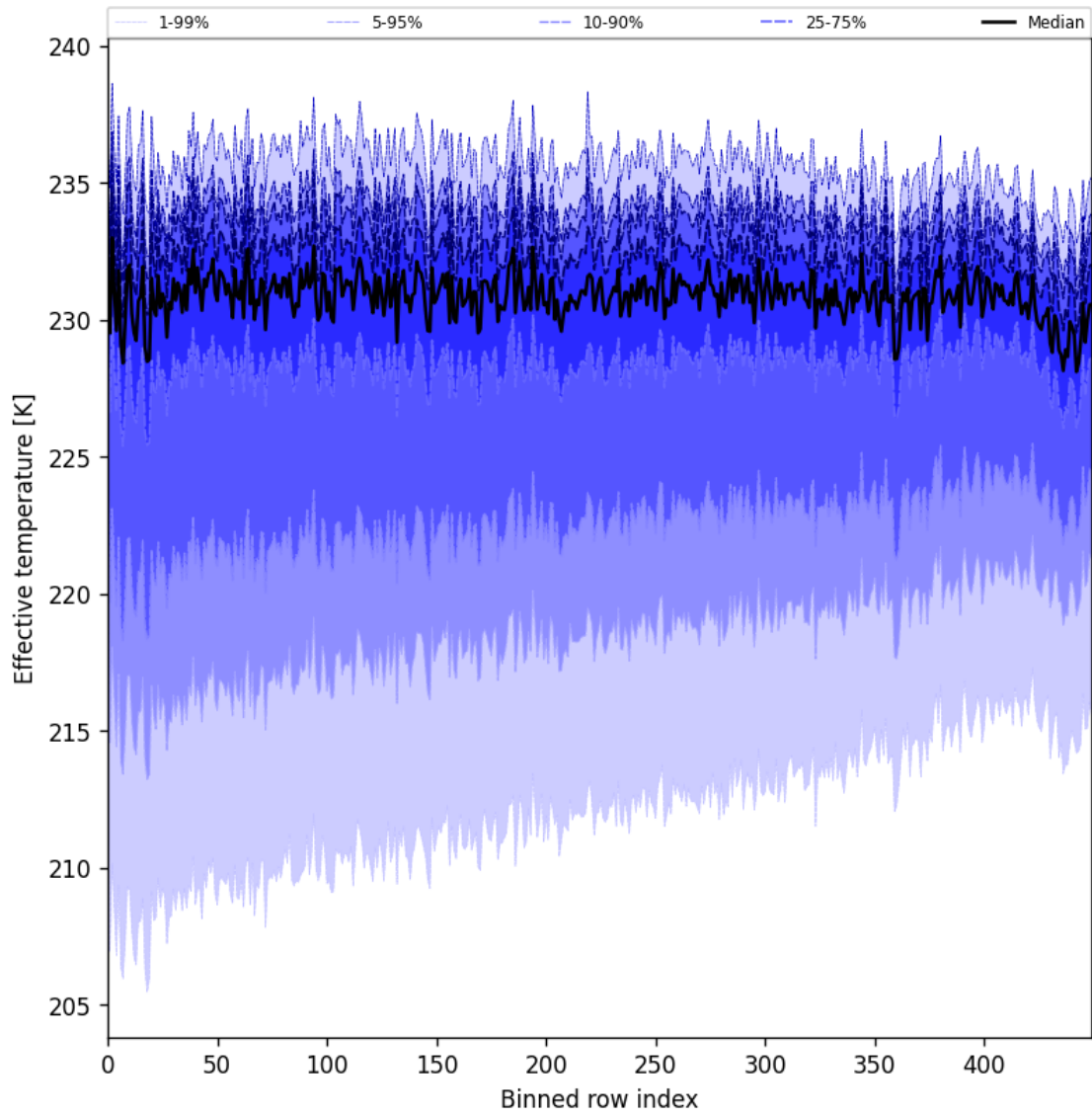
Figure 31: Along track statistics of “Effective temperature” for 2025-05-10 to 2025-05-11
