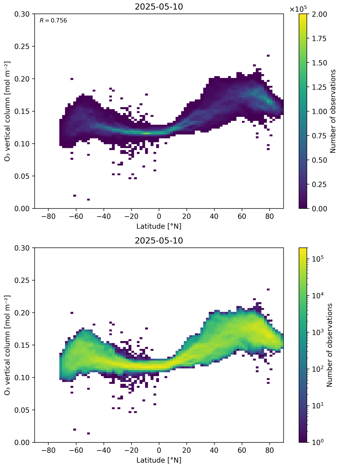
Figure 36: Scatter density plot of “Latitude” against “O 3 vertical column” for 2025-05-10 to 2025-05-11.
