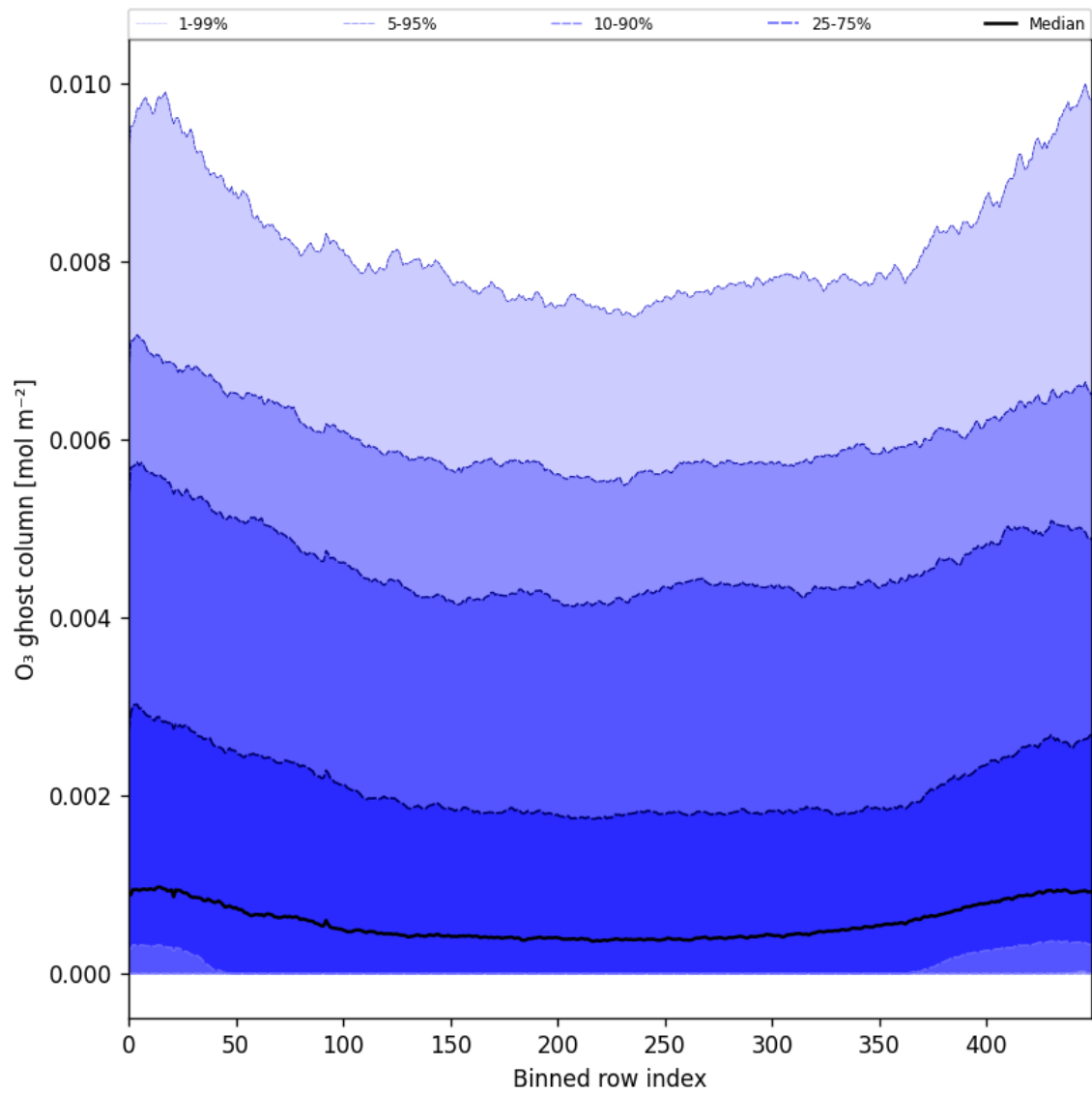
Figure 32: Along track statistics of “O 3 ghost column” for 2025-05-10 to 2025-05-11
