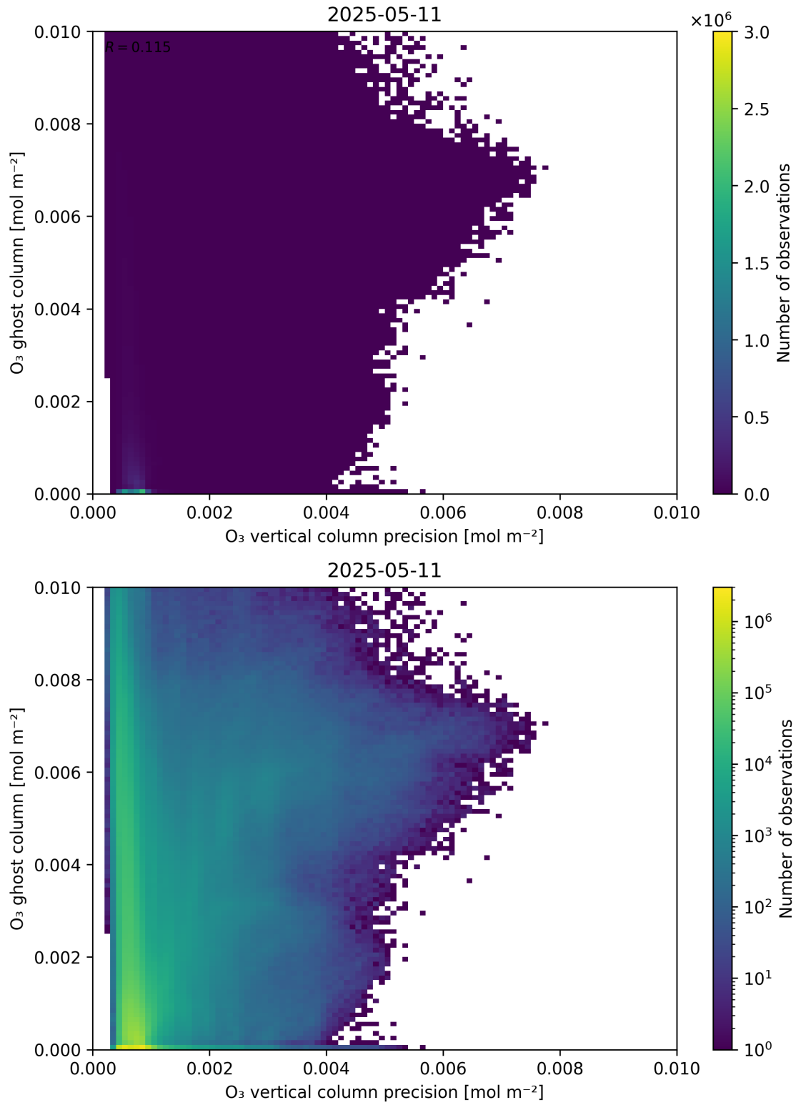
Figure 43: Scatter density plot of “ \text{O}_3 vertical column precision” against “ \text{O}_3 ghost column” for 2025-05-10 to 2025-05-12.
