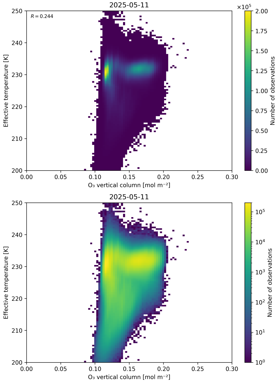
Figure 39: Scatter density plot of “O 3 vertical column” against “Effective temperature” for 2025-05-10 to 2025-05-12.
