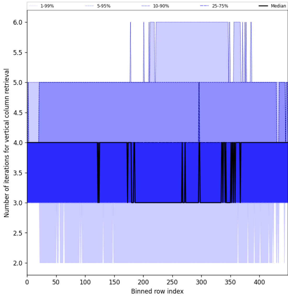
Figure 33: Along track statistics of “Number of iterations for vertical column retrieval” for 2025-05-10 to 2025-05-12
