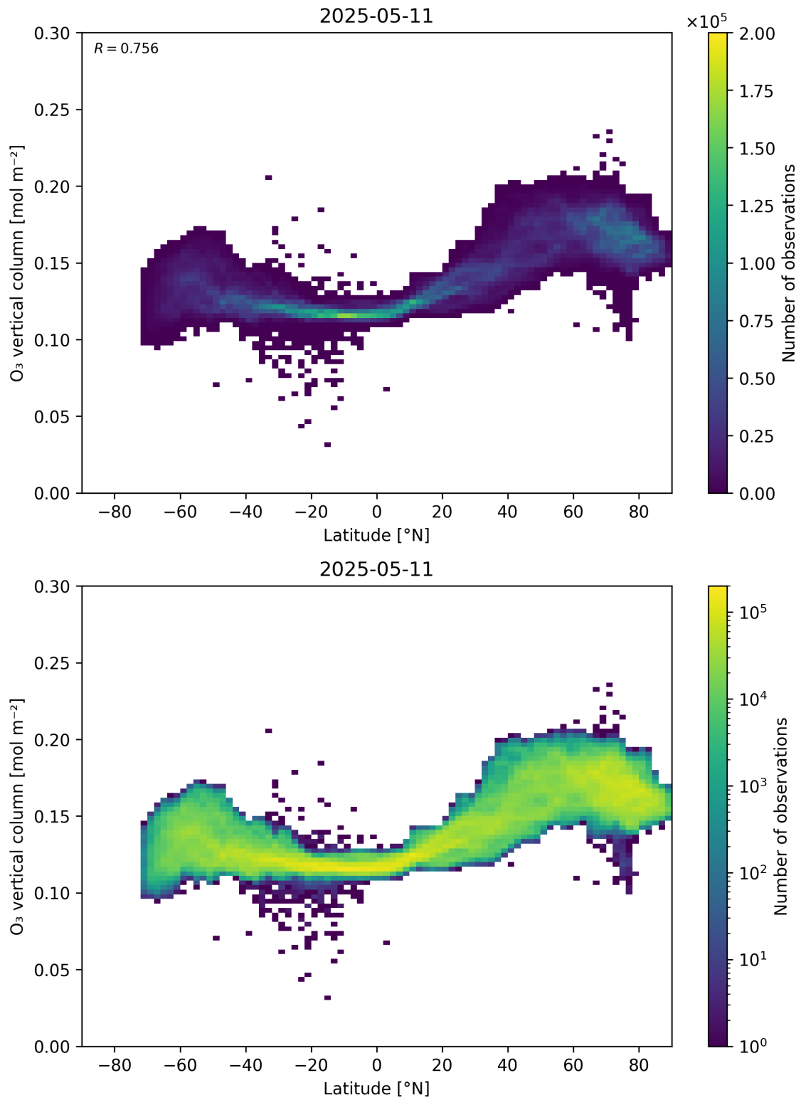
Figure 36: Scatter density plot of “Latitude” against “O 3 vertical column” for 2025-05-10 to 2025-05-12.
