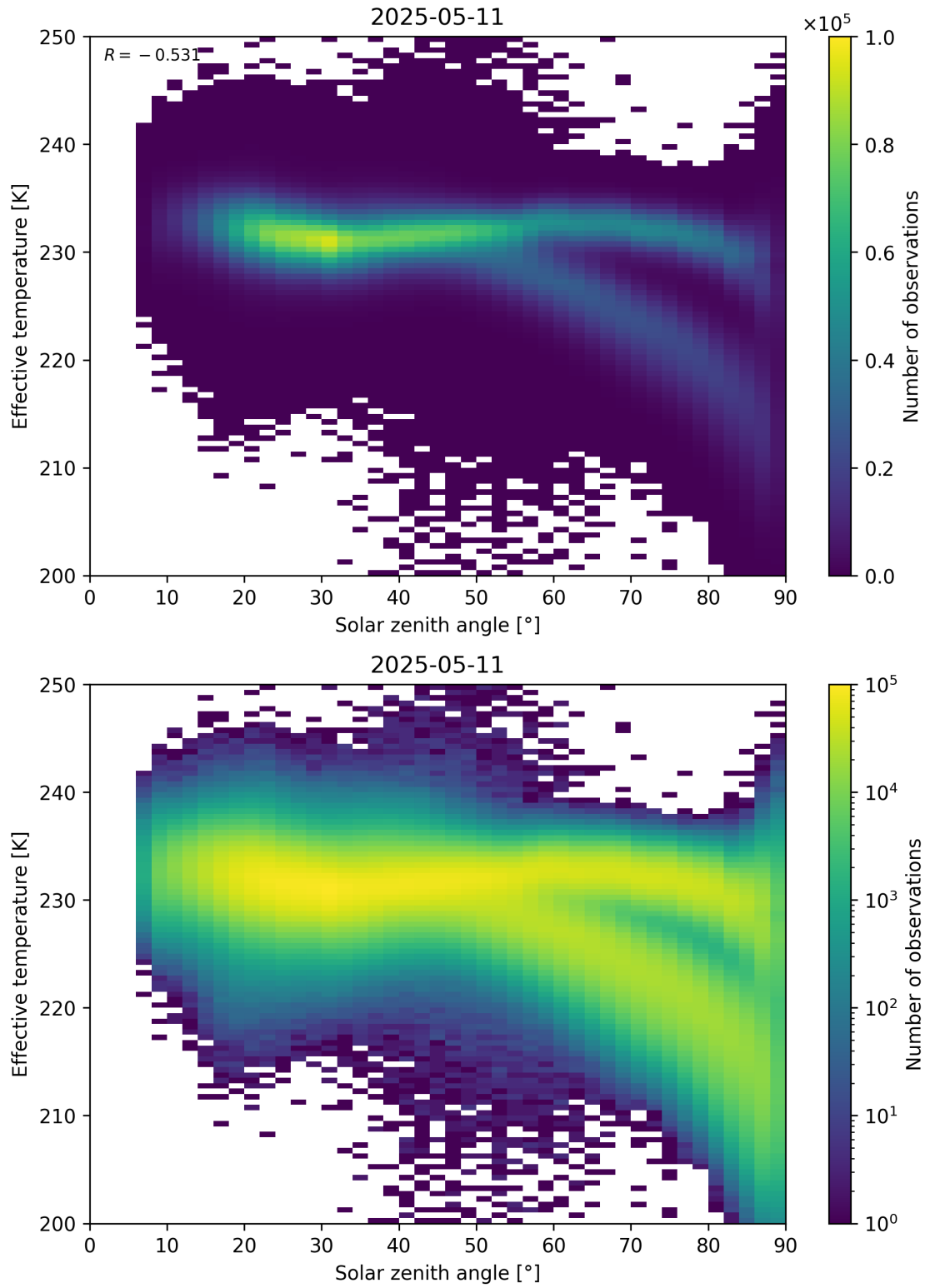
Figure 45: Scatter density plot of “Solar zenith angle” against “Effective temperature” for 2025-05-10 to 2025-05-12.
