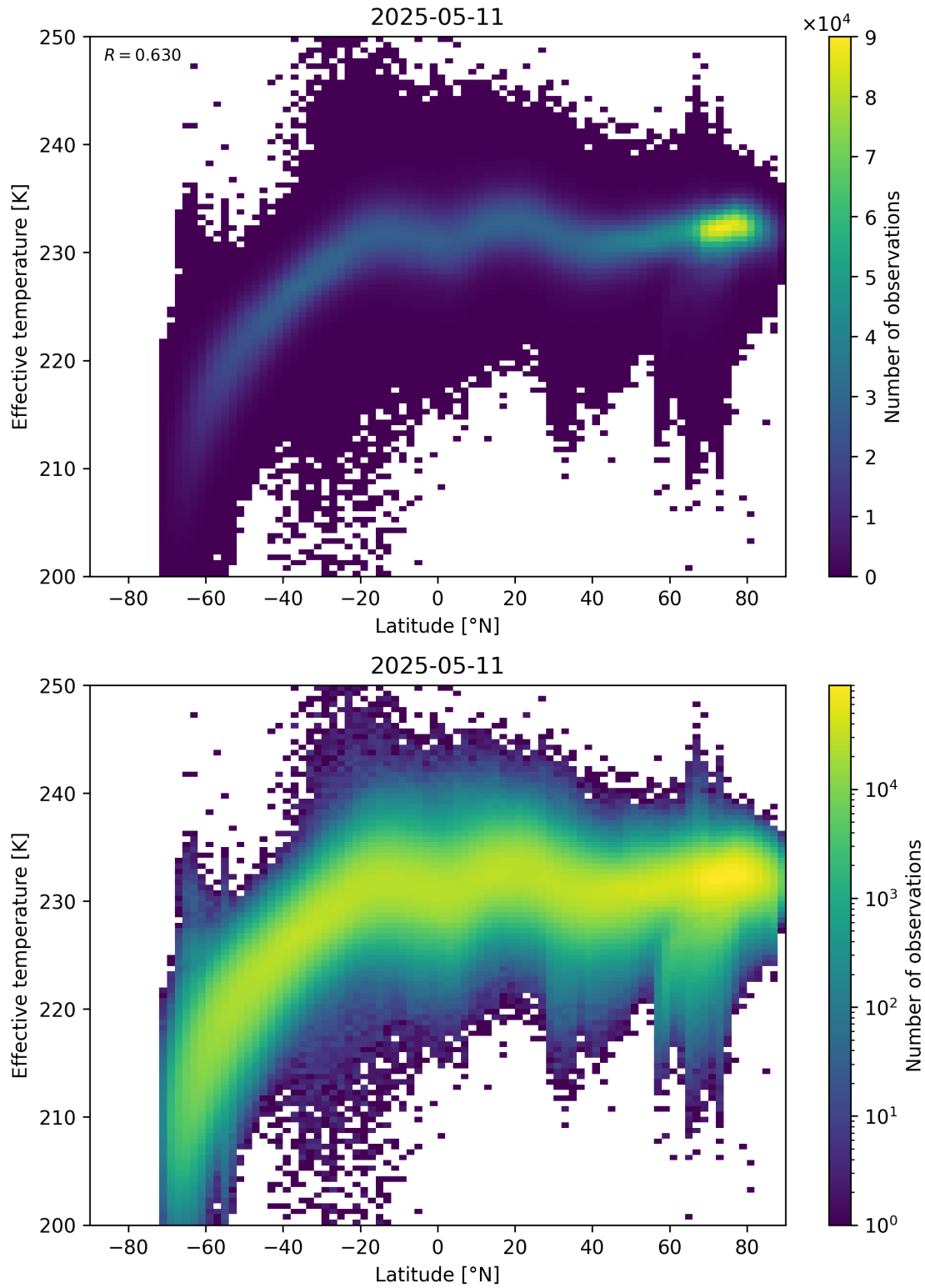
Figure 34: Scatter density plot of “Latitude” against “Effective temperature” for 2025-05-10 to 2025-05-12.
