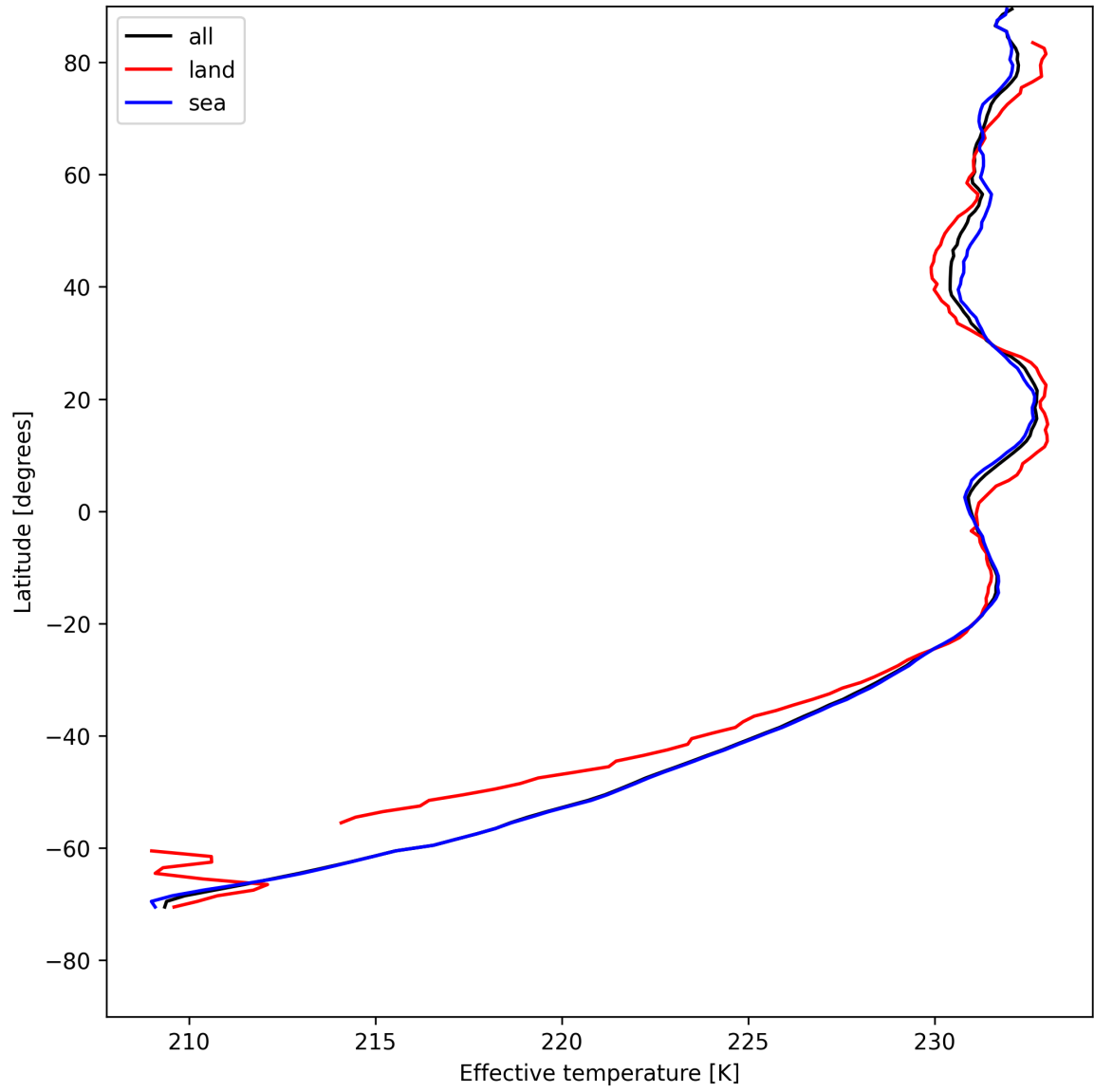
Figure 17: Zonal average of "Effective temperature" for 2025-05-10 to 2025-05-12.
