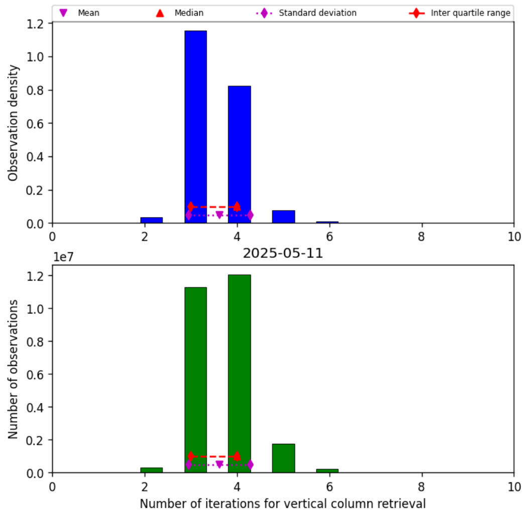
Figure 26: Histogram of “Number of iterations for vertical column retrieval” for 2025-05-10 to 2025-05-12
