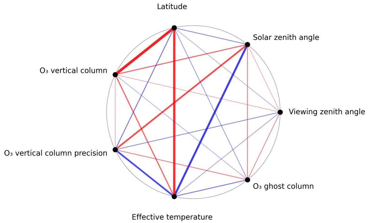
Figure 1: Map of correlation graph for 2025-05-10 to 2025-05-12.
