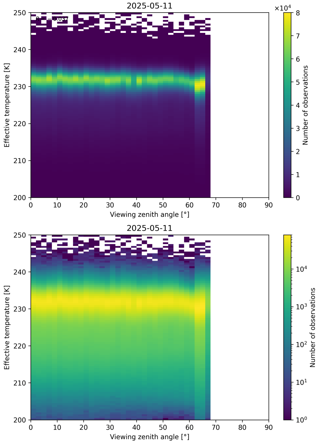
Figure 50: Scatter density plot of “Viewing zenith angle” against “Effective temperature” for 2025-05-10 to 2025-05-12.
