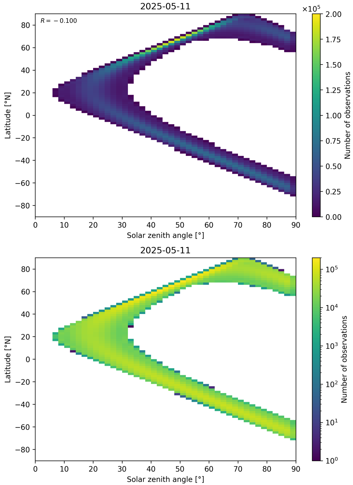
Figure 44: Scatter density plot of “Solar zenith angle” against “Latitude” for 2025-05-10 to 2025-05-12.
