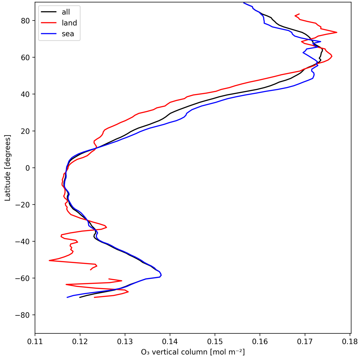
Figure 14: Zonal average of “O 3 vertical column” for 2025-05-10 to 2025-05-12.
