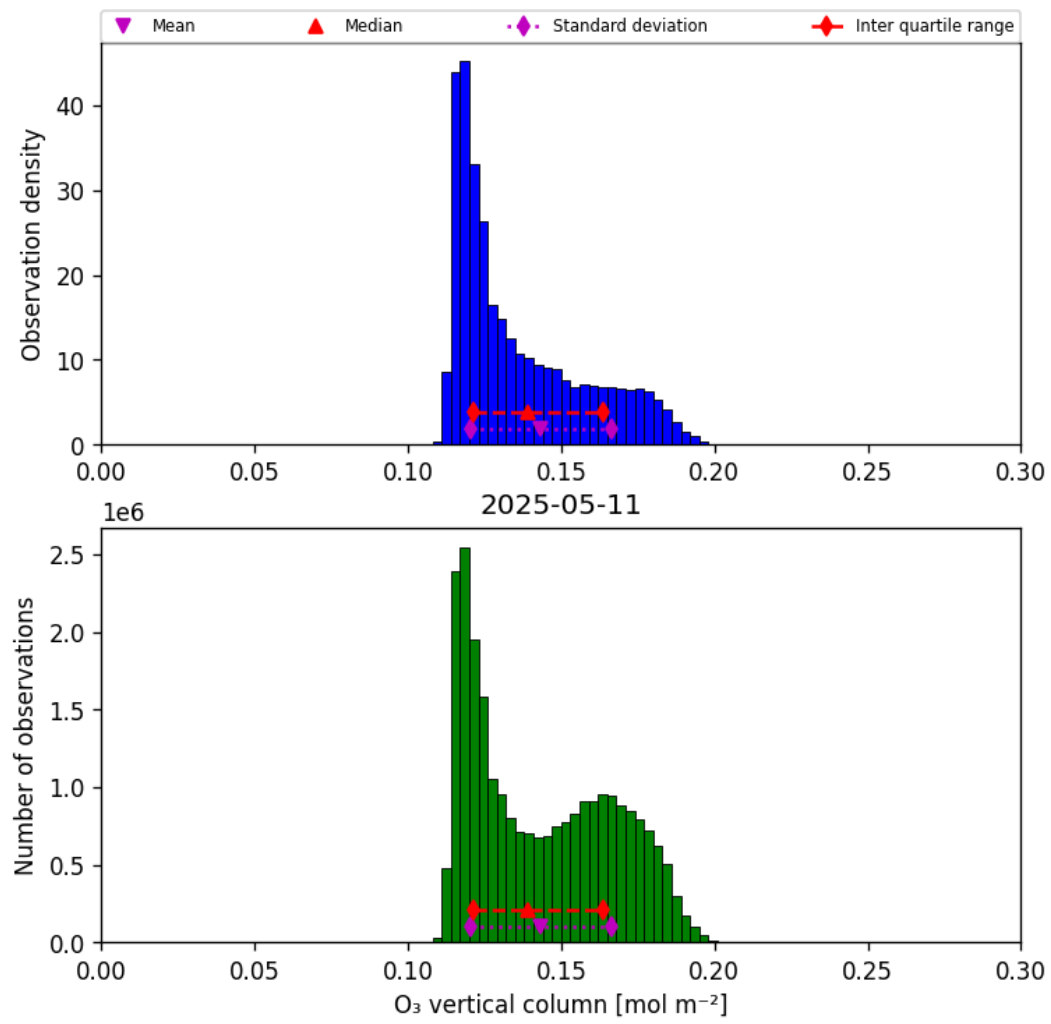
Figure 21: Histogram of “O 3 vertical column” for 2025-05-10 to 2025-05-12
