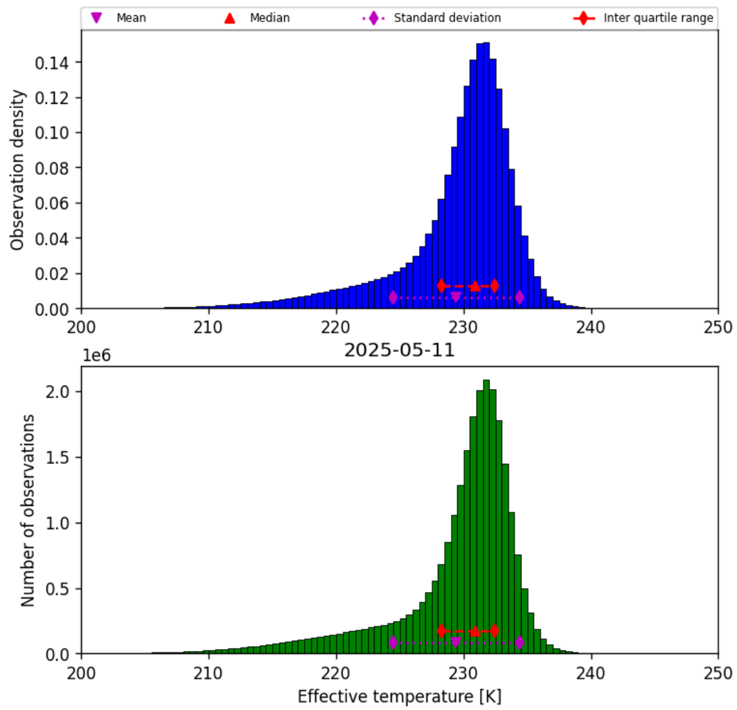
Figure 24: Histogram of “Effective temperature” for 2025-05-10 to 2025-05-12
