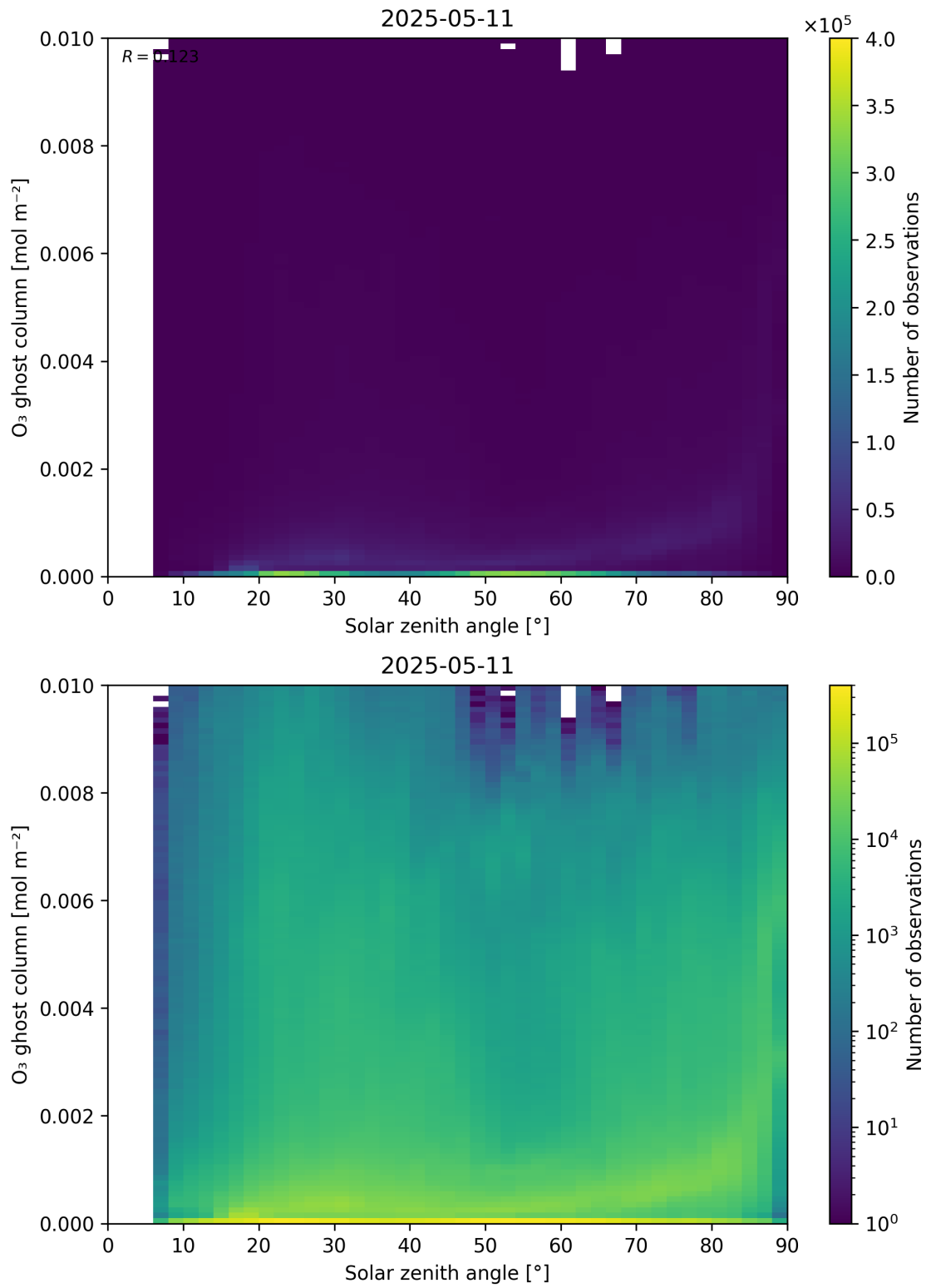
Figure 46: Scatter density plot of “Solar zenith angle” against “O 3 ghost column” for 2025-05-10 to 2025-05-12.
