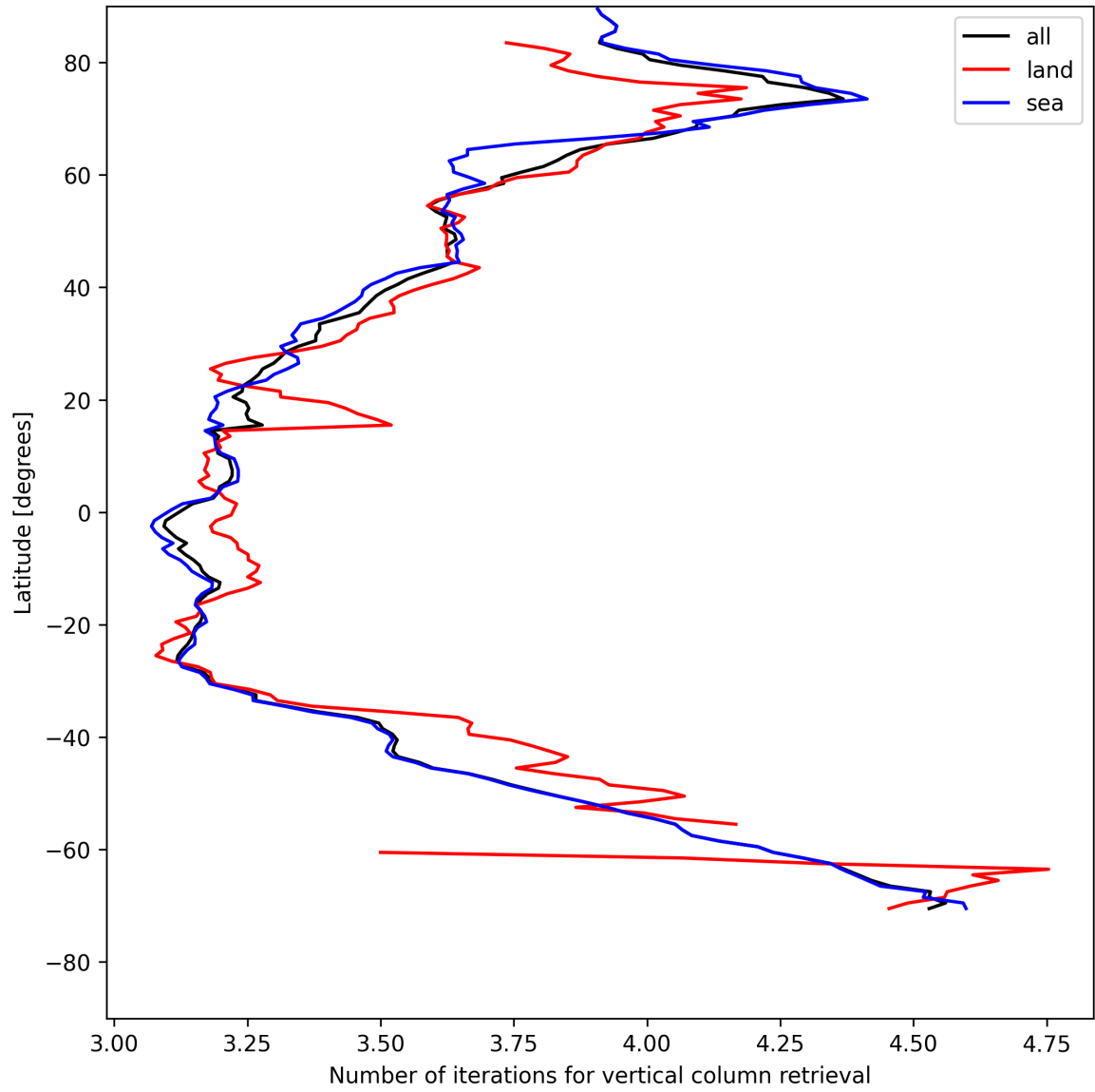
Figure 19: Zonal average of “Number of iterations for vertical column retrieval” for 2025-05-10 to 2025-05-12.
