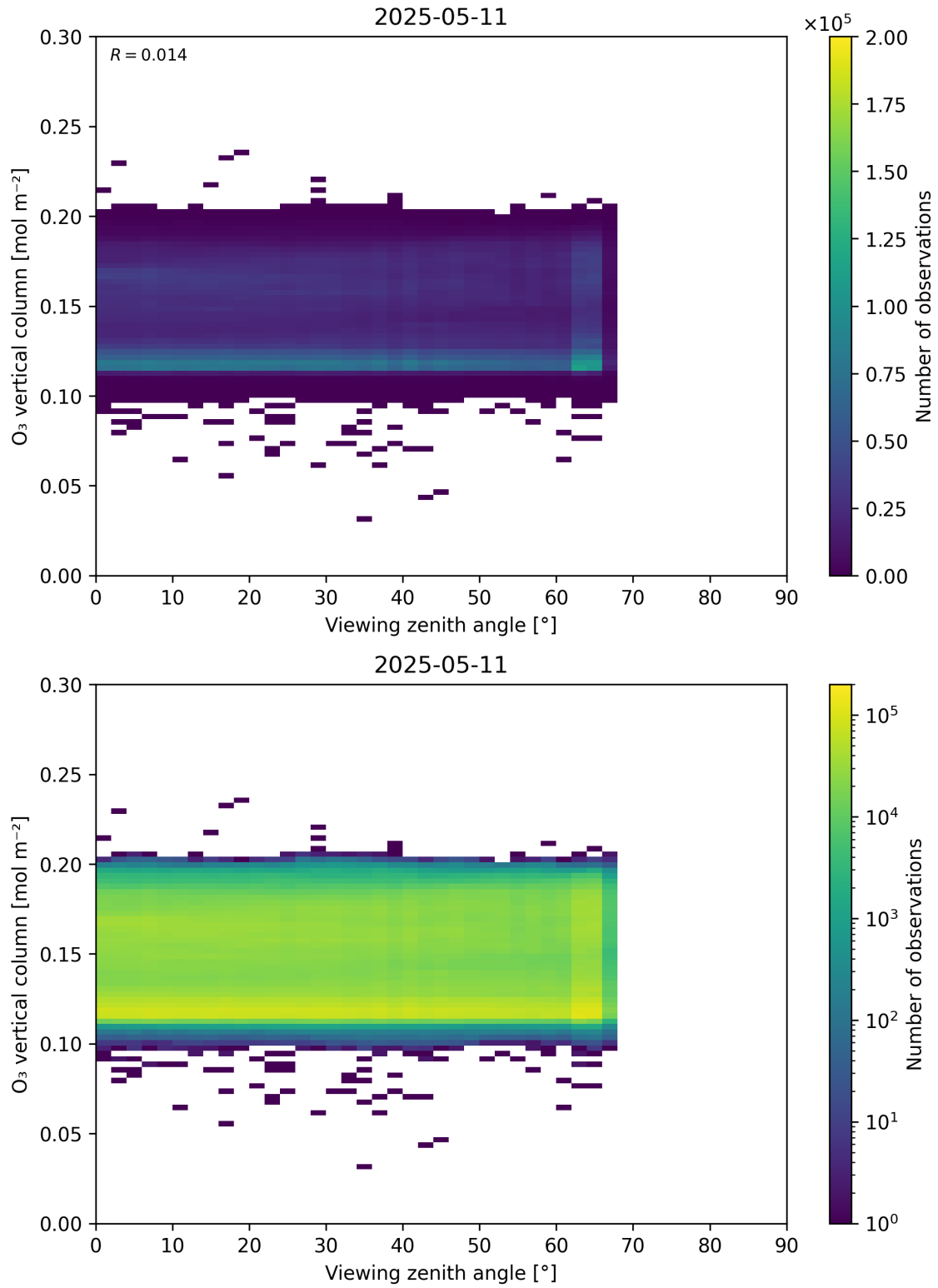
Figure 52: Scatter density plot of “Viewing zenith angle” against “O 3 vertical column” for 2025-05-10 to 2025-05-12.
