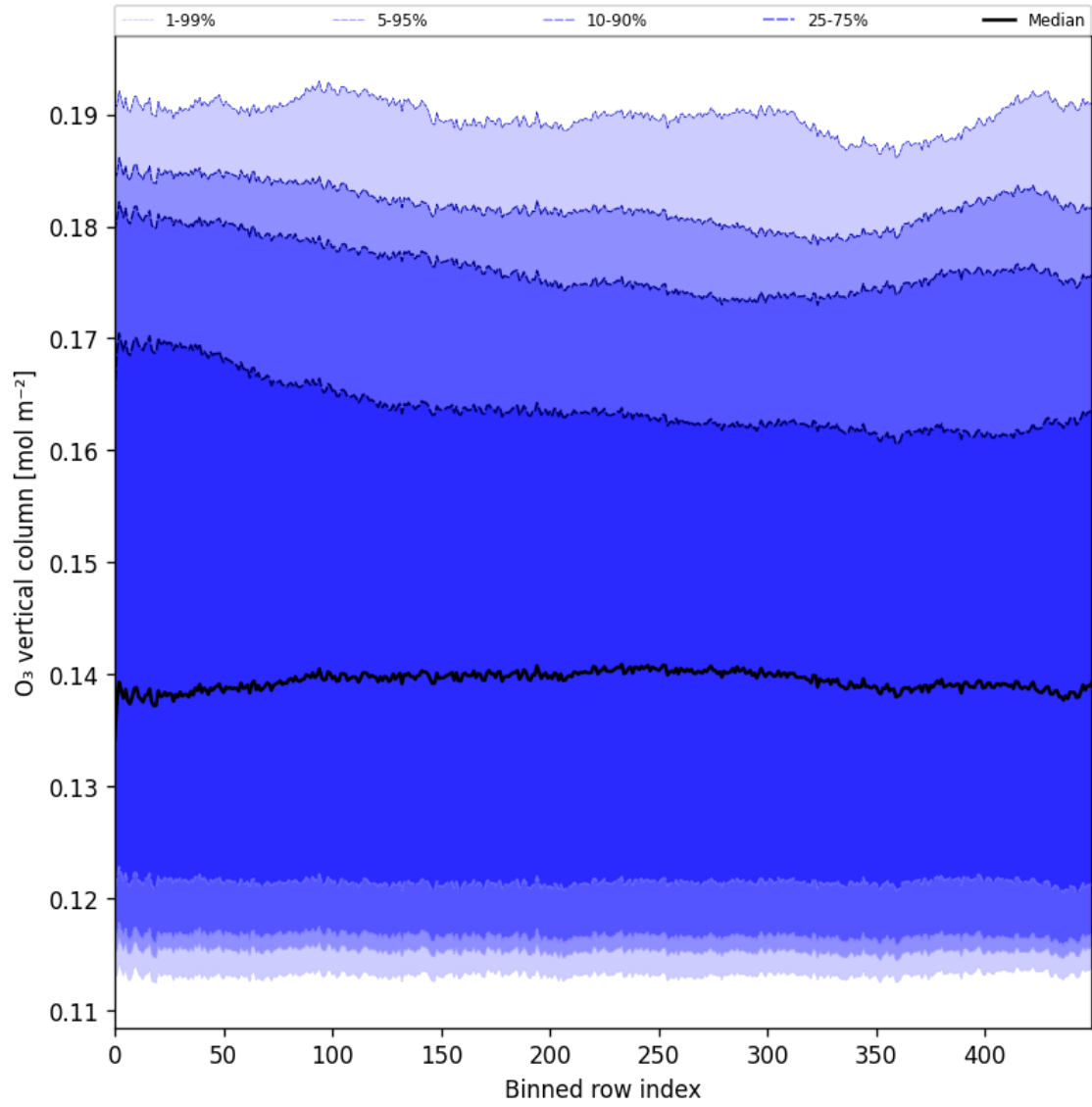
Figure 28: Along track statistics of “O 3 vertical column” for 2025-05-10 to 2025-05-12
