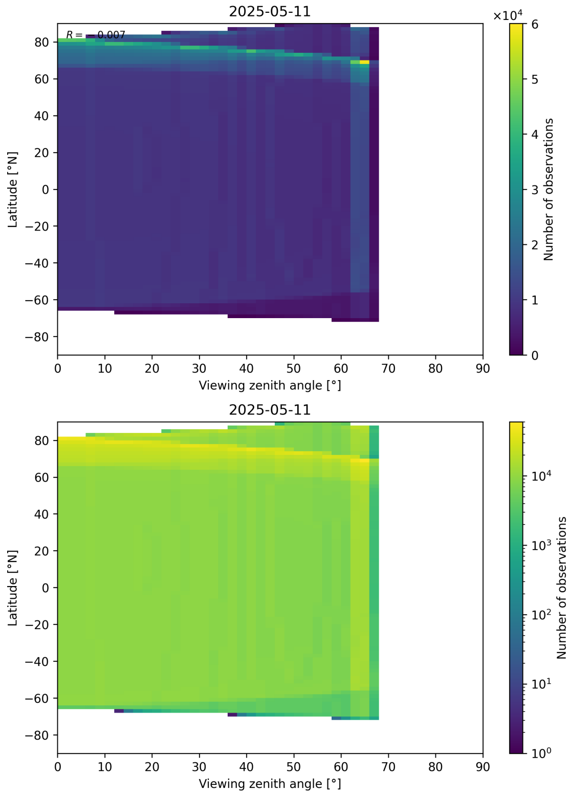
Figure 49: Scatter density plot of “Viewing zenith angle” against “Latitude” for 2025-05-10 to 2025-05-12.
