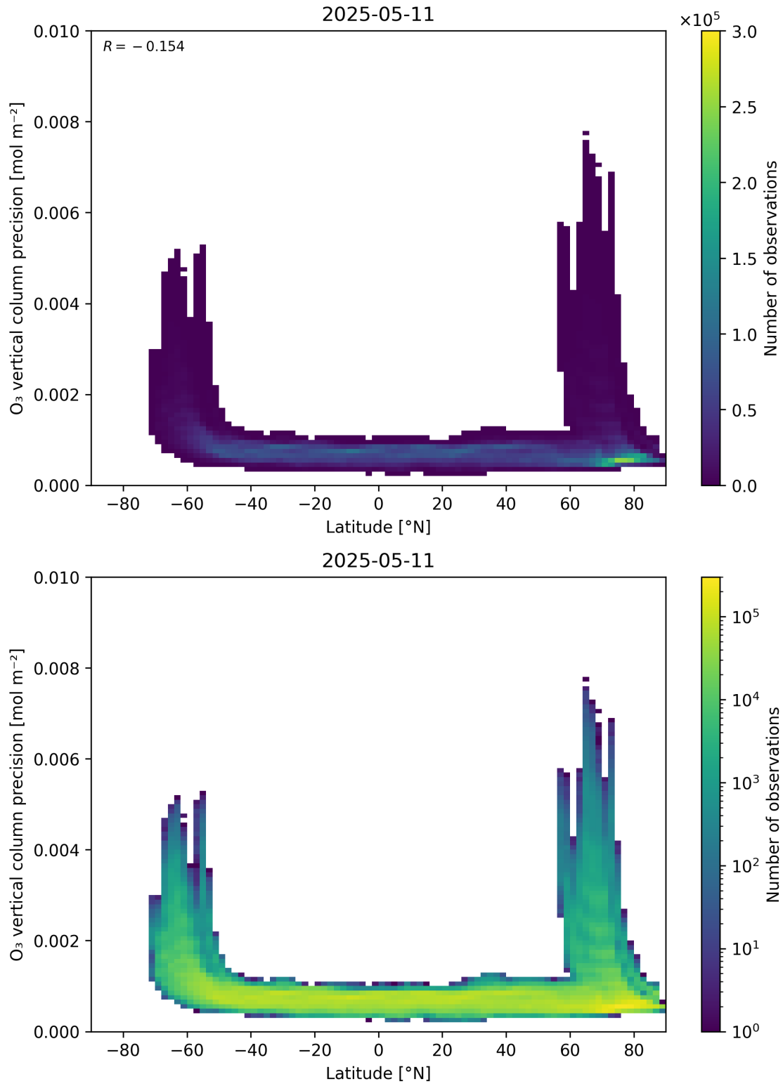
Figure 37: Scatter density plot of “Latitude” against “O 3 vertical column precision” for 2025-05-10 to 2025-05-12.
