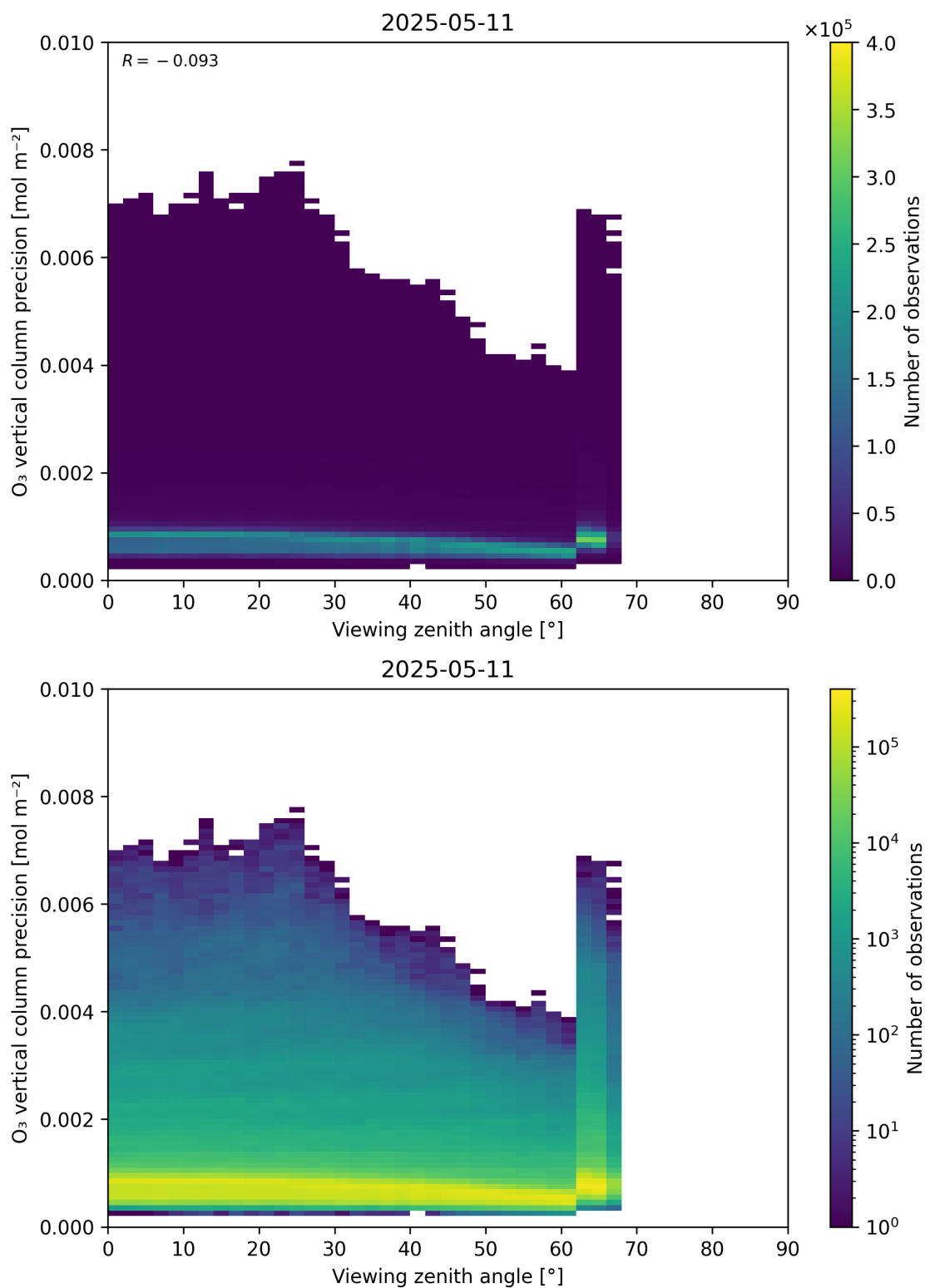
Figure 53: Scatter density plot of “Viewing zenith angle” against “O 3 vertical column precision” for 2025-05-10 to 2025-05-12.
