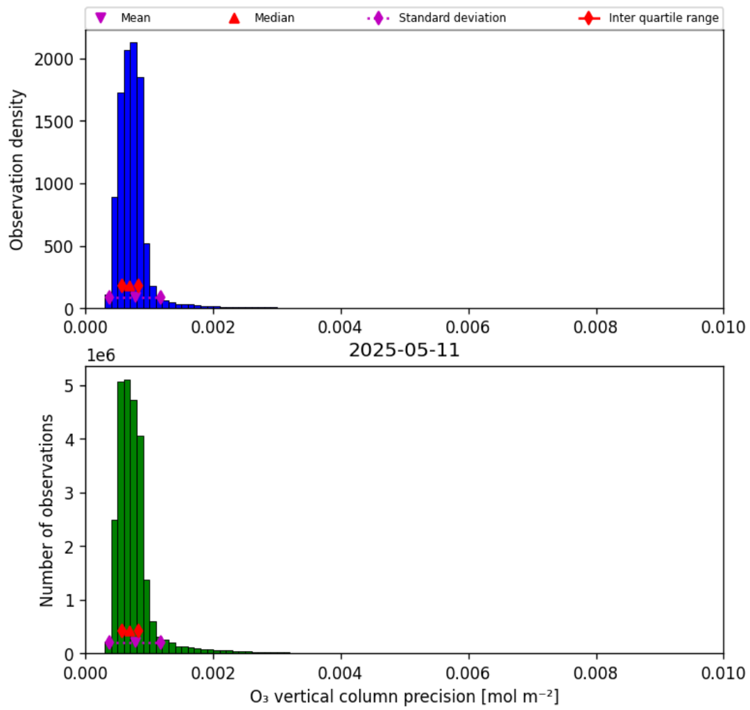
Figure 22: Histogram of “O 3 vertical column precision” for 2025-05-10 to 2025-05-12
