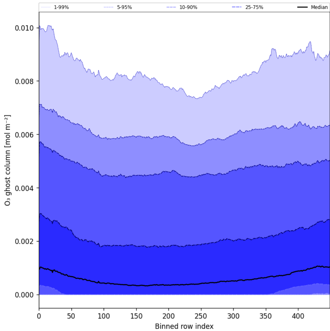
Figure 32: Along track statistics of “O 3 ghost column” for 2025-05-10 to 2025-05-12
