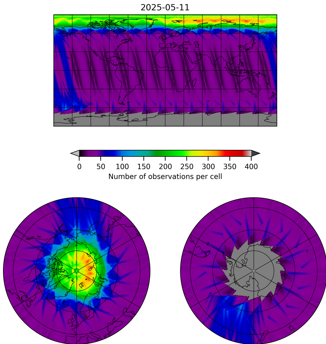
Figure 12: Map of the number of observations for 2025-05-10 to 2025-05-12
