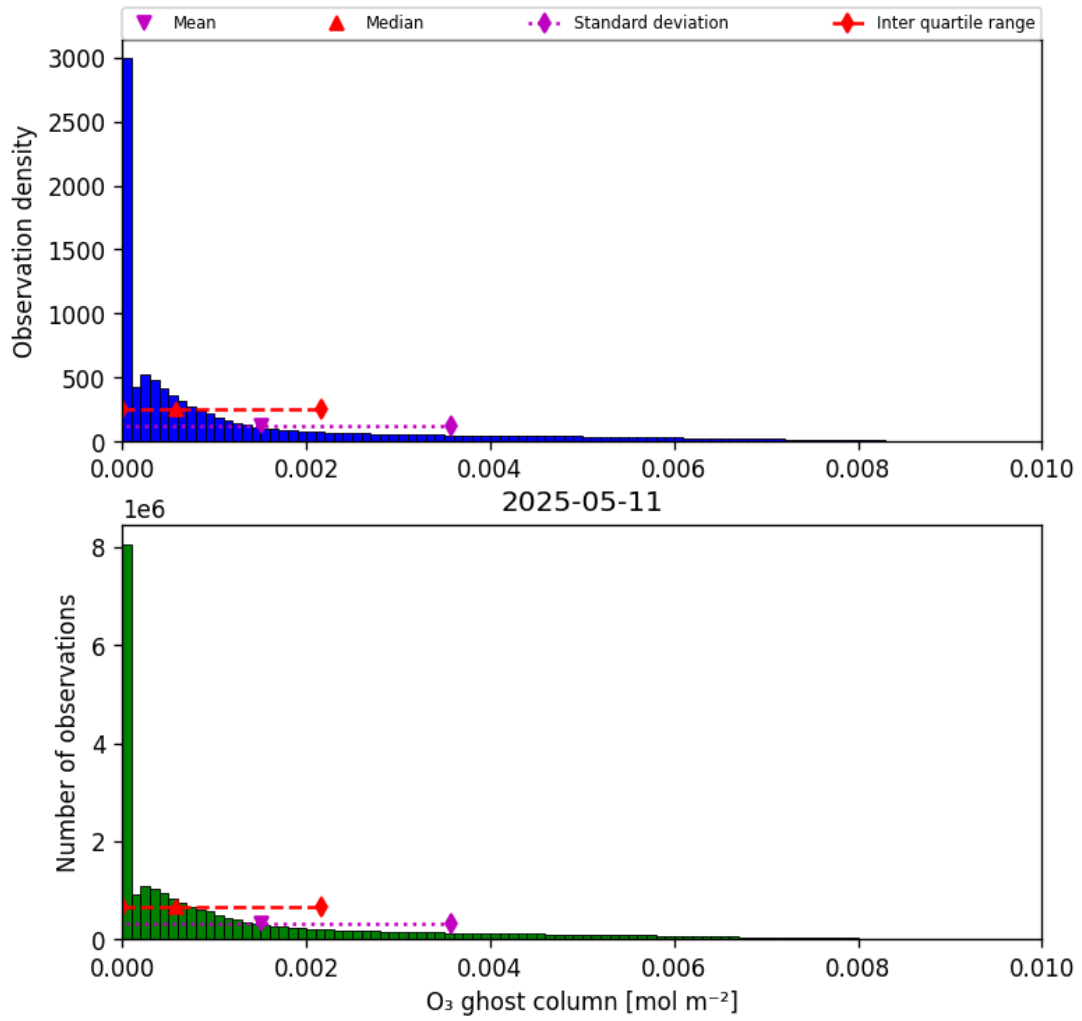
Figure 25: Histogram of “O 3 ghost column” for 2025-05-10 to 2025-05-12
