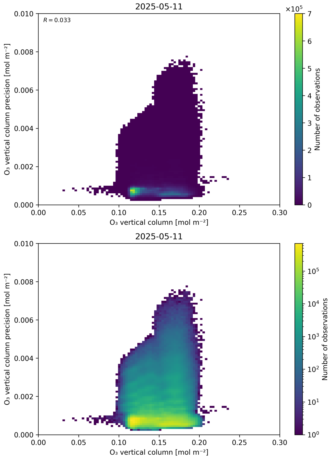
Figure 41: Scatter density plot of “O 3 vertical column” against “O 3 vertical column precision” for 2025-05-10 to 2025-05-12.
