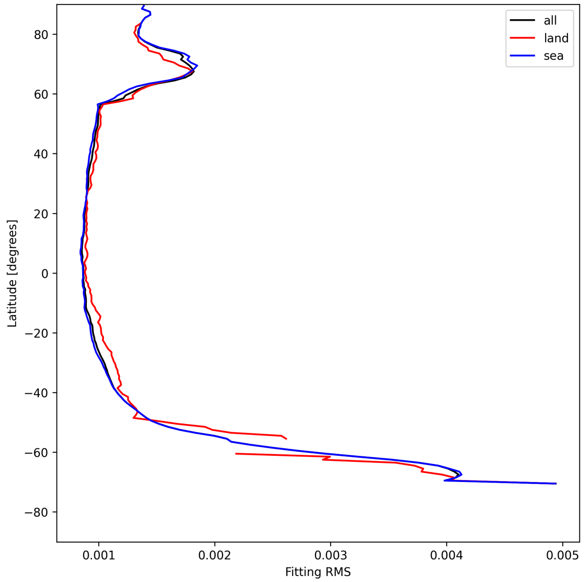
Figure 16: Zonal average of “Fitting RMS” for 2025-05-10 to 2025-05-12.
