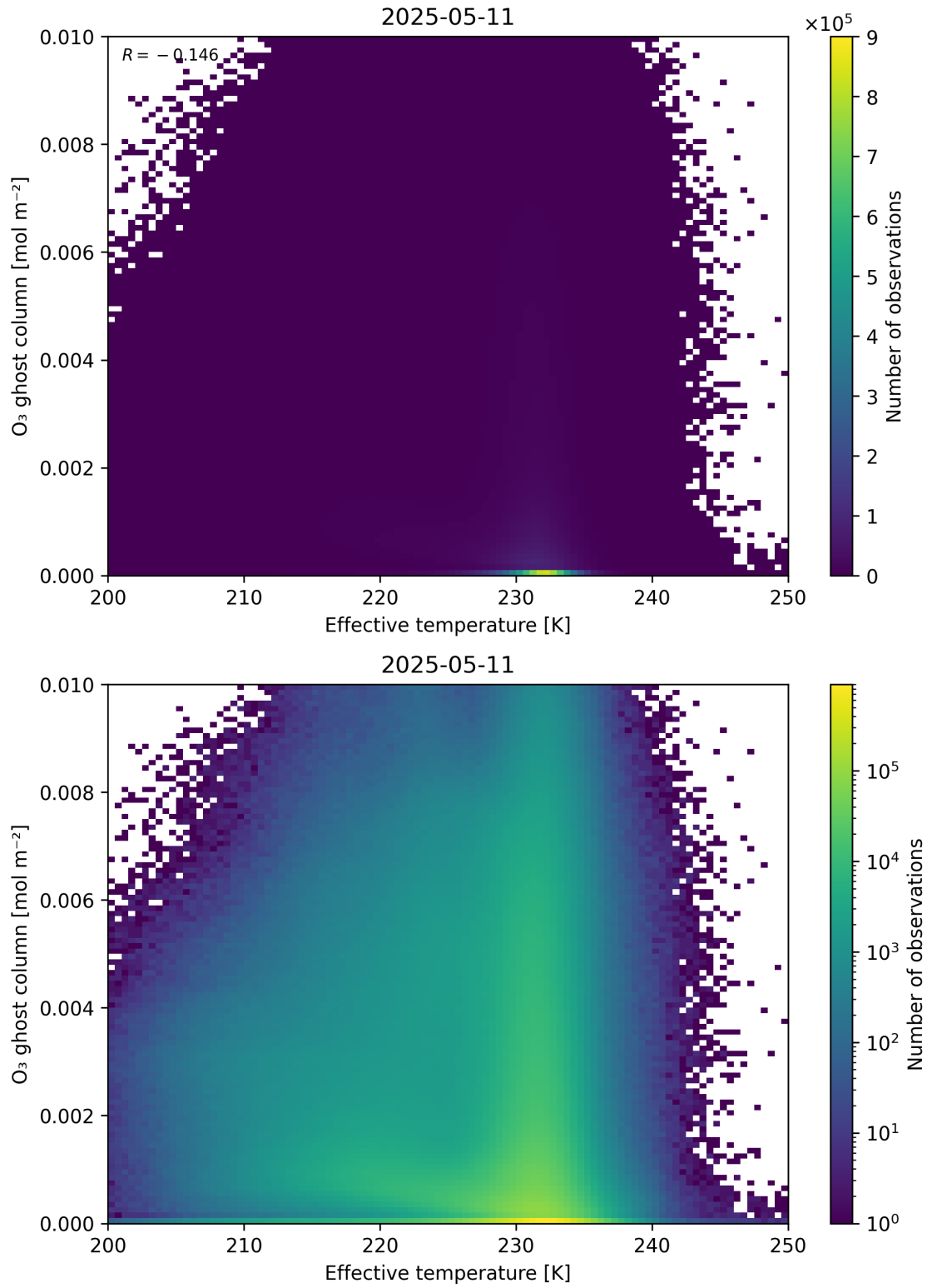
Figure 38: Scatter density plot of “Effective temperature” against “O 3 ghost column” for 2025-05-10 to 2025-05-12.
