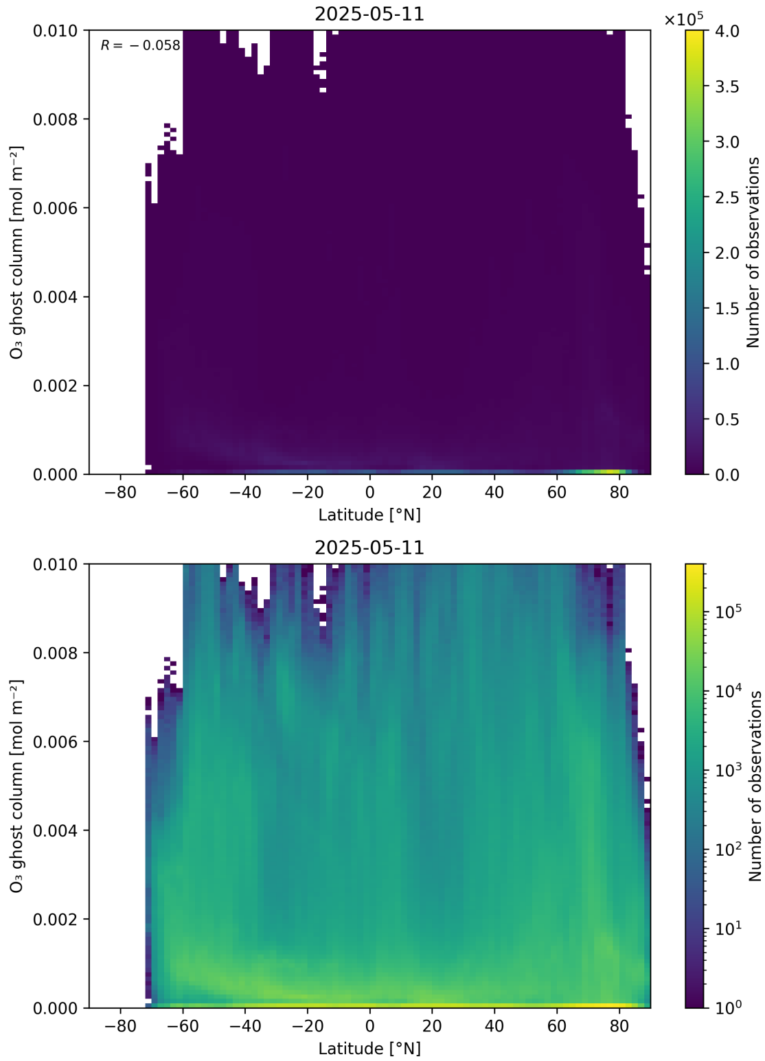
Figure 35: Scatter density plot of “Latitude” against “O 3 ghost column” for 2025-05-10 to 2025-05-12.
