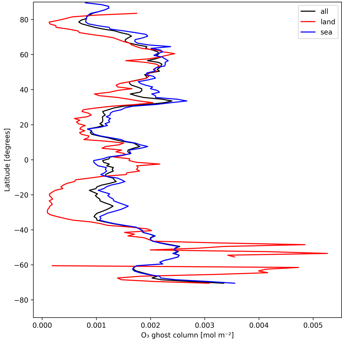
Figure 18: Zonal average of "O 3 ghost column" for 2025-05-10 to 2025-05-12.
