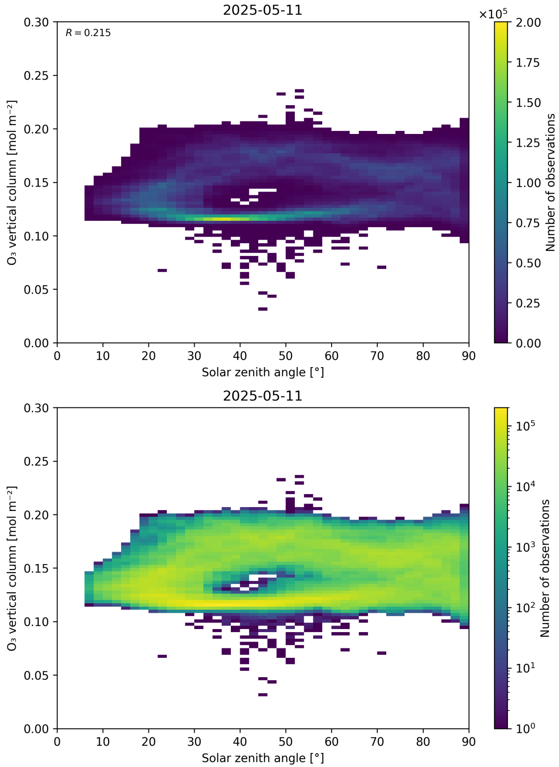
Figure 47: Scatter density plot of “Solar zenith angle” against “O 3 vertical column” for 2025-05-10 to 2025-05-12.
