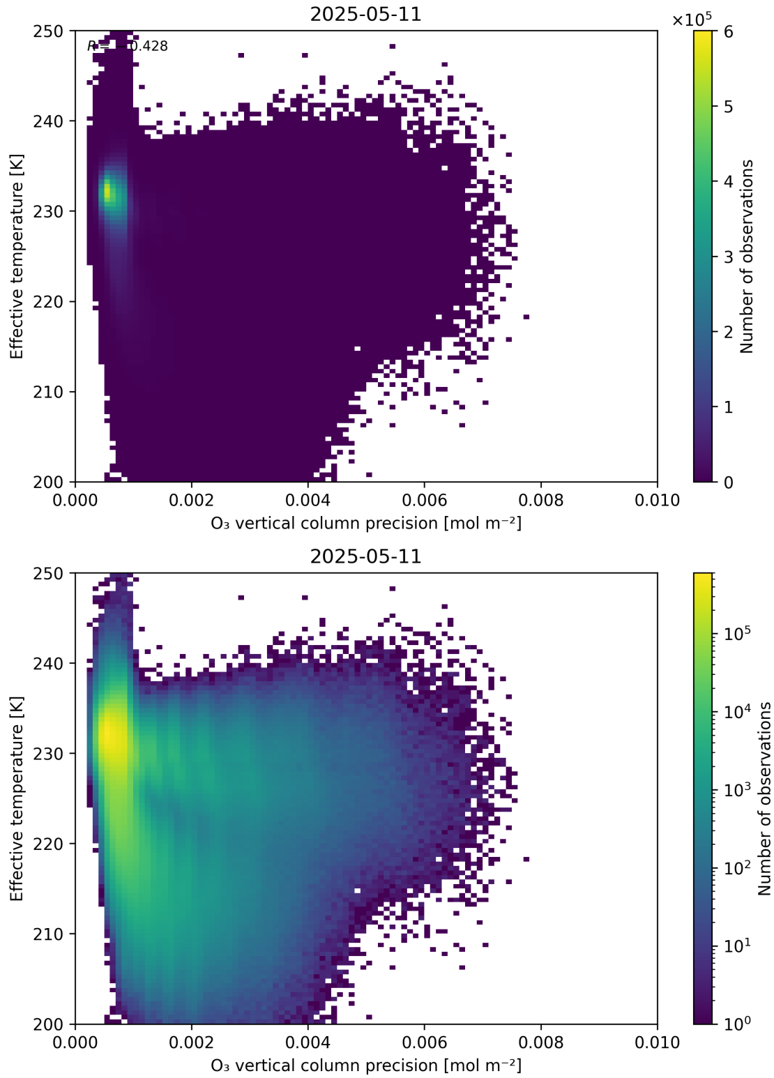
Figure 42: Scatter density plot of “O 3 vertical column precision” against “Effective temperature” for 2025-05-10 to 2025-05-12.
