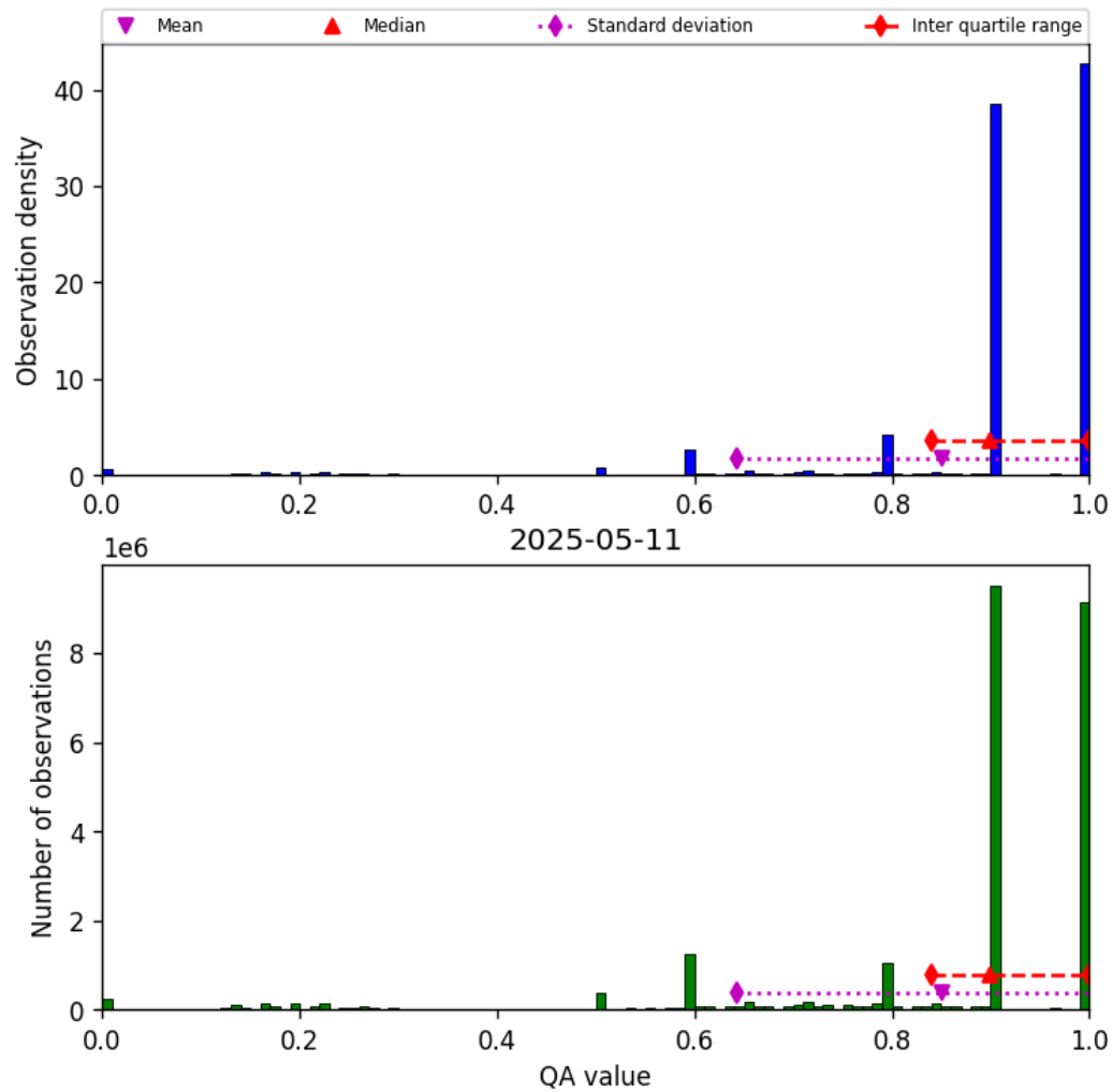
Figure 20: Histogram of “QA value” for 2025-05-10 to 2025-05-12
