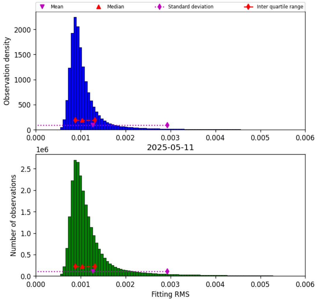
Figure 23: Histogram of “Fitting RMS” for 2025-05-10 to 2025-05-12
