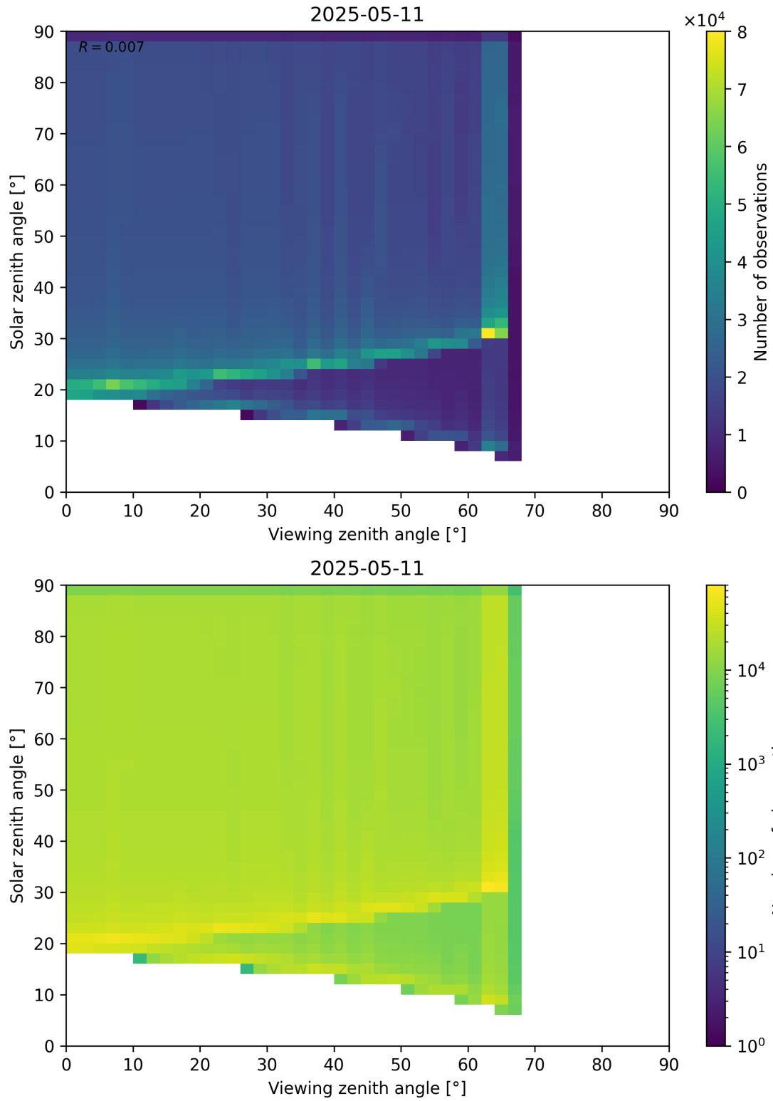
Figure 54: Scatter density plot of “Viewing zenith angle” against “Solar zenith angle” for 2025-05-10 to 2025-05-12.
