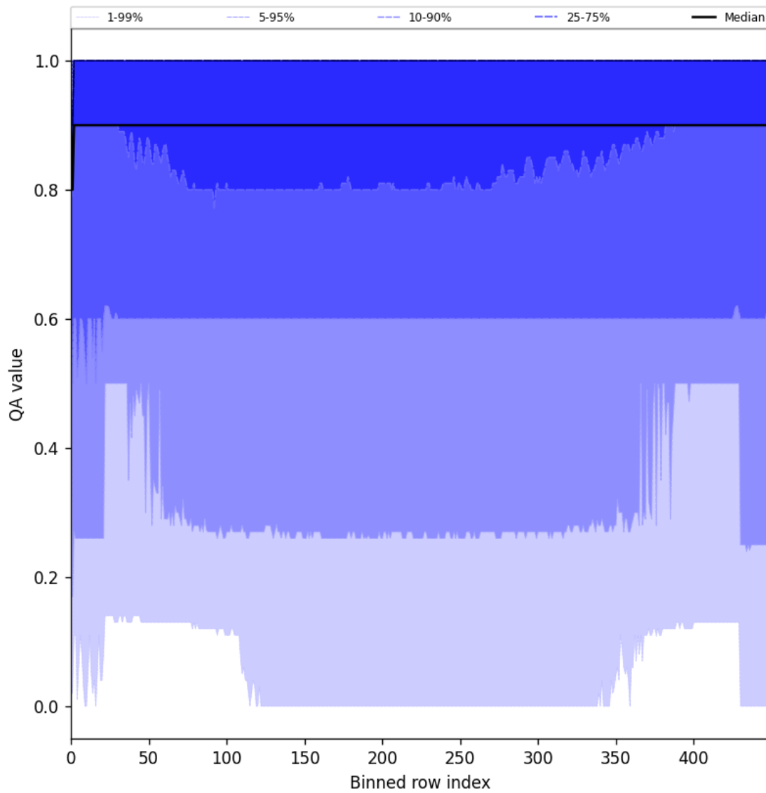
Figure 27: Along track statistics of “QA value” for 2025-05-10 to 2025-05-12
