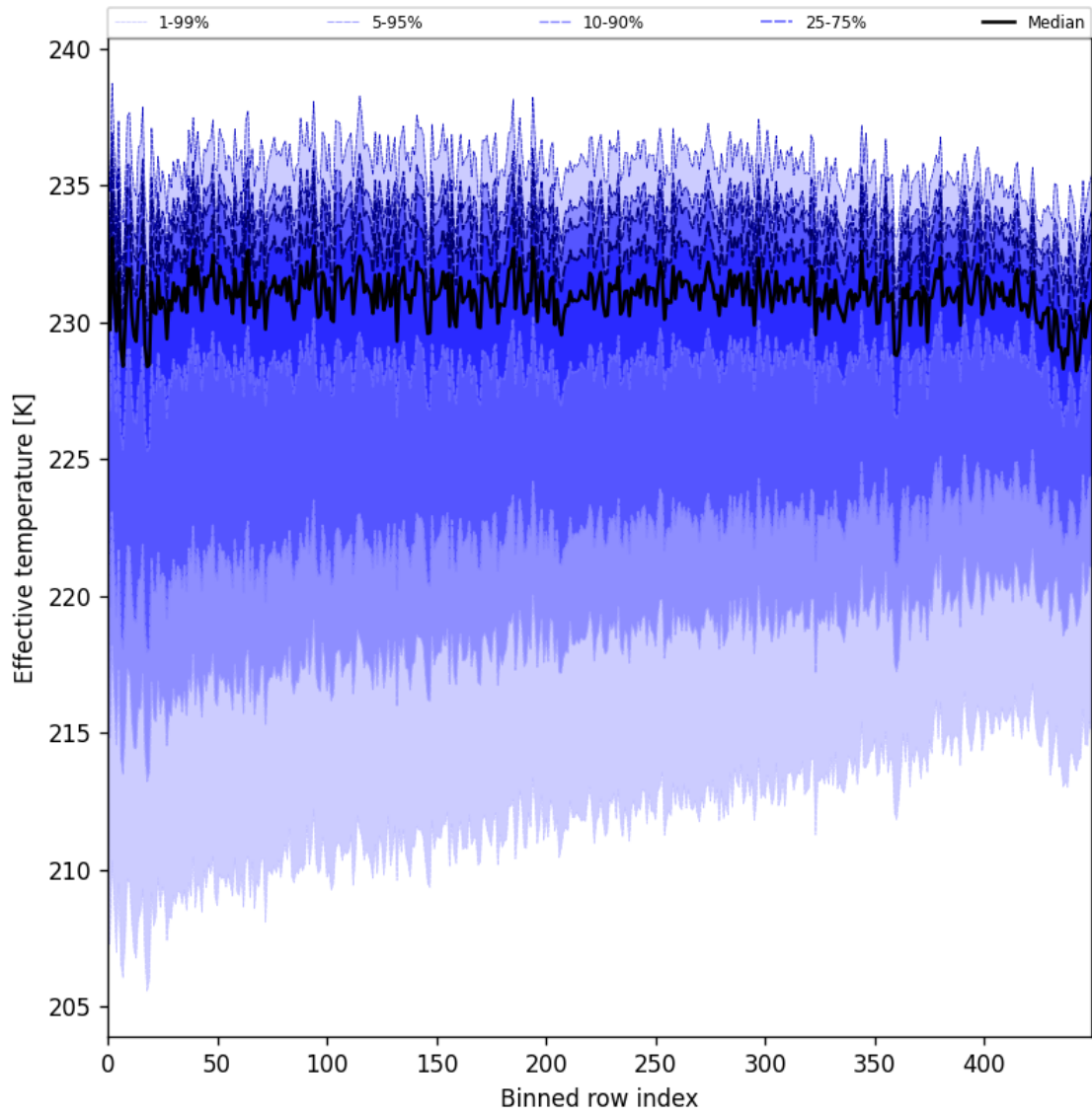
Figure 31: Along track statistics of “Effective temperature” for 2025-05-10 to 2025-05-12
