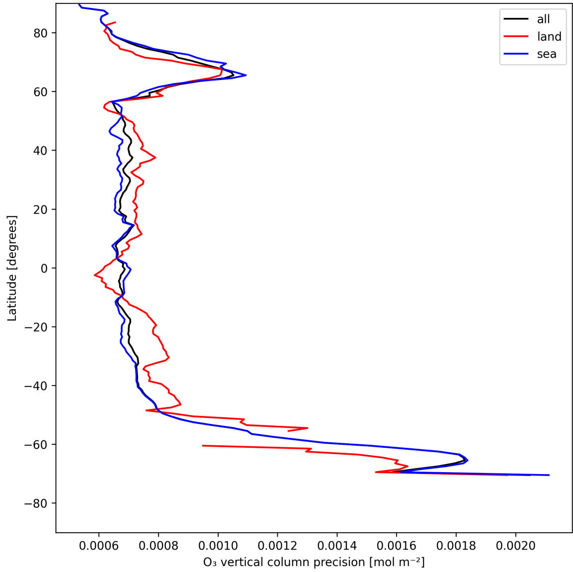
Figure 15: Zonal average of “O 3 vertical column precision” for 2025-05-10 to 2025-05-12.
