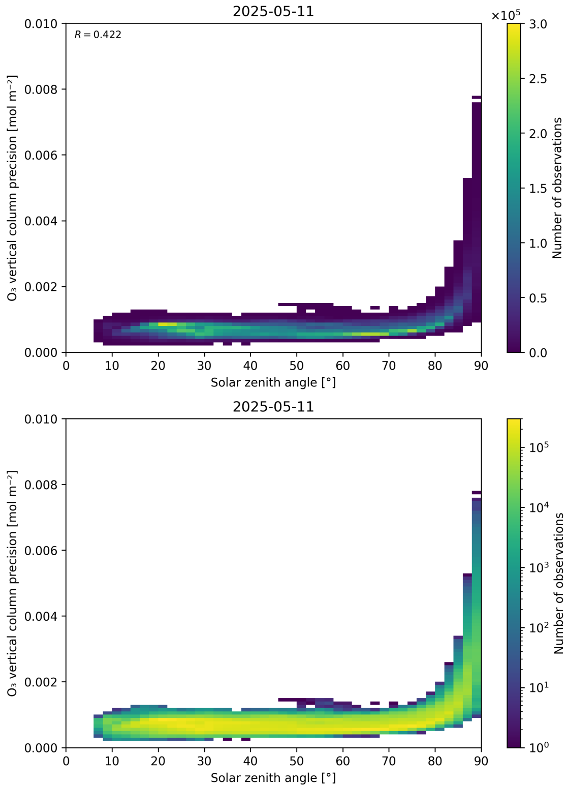
Figure 48: Scatter density plot of “Solar zenith angle” against “O 3 vertical column precision” for 2025-05-10 to 2025-05-12.
