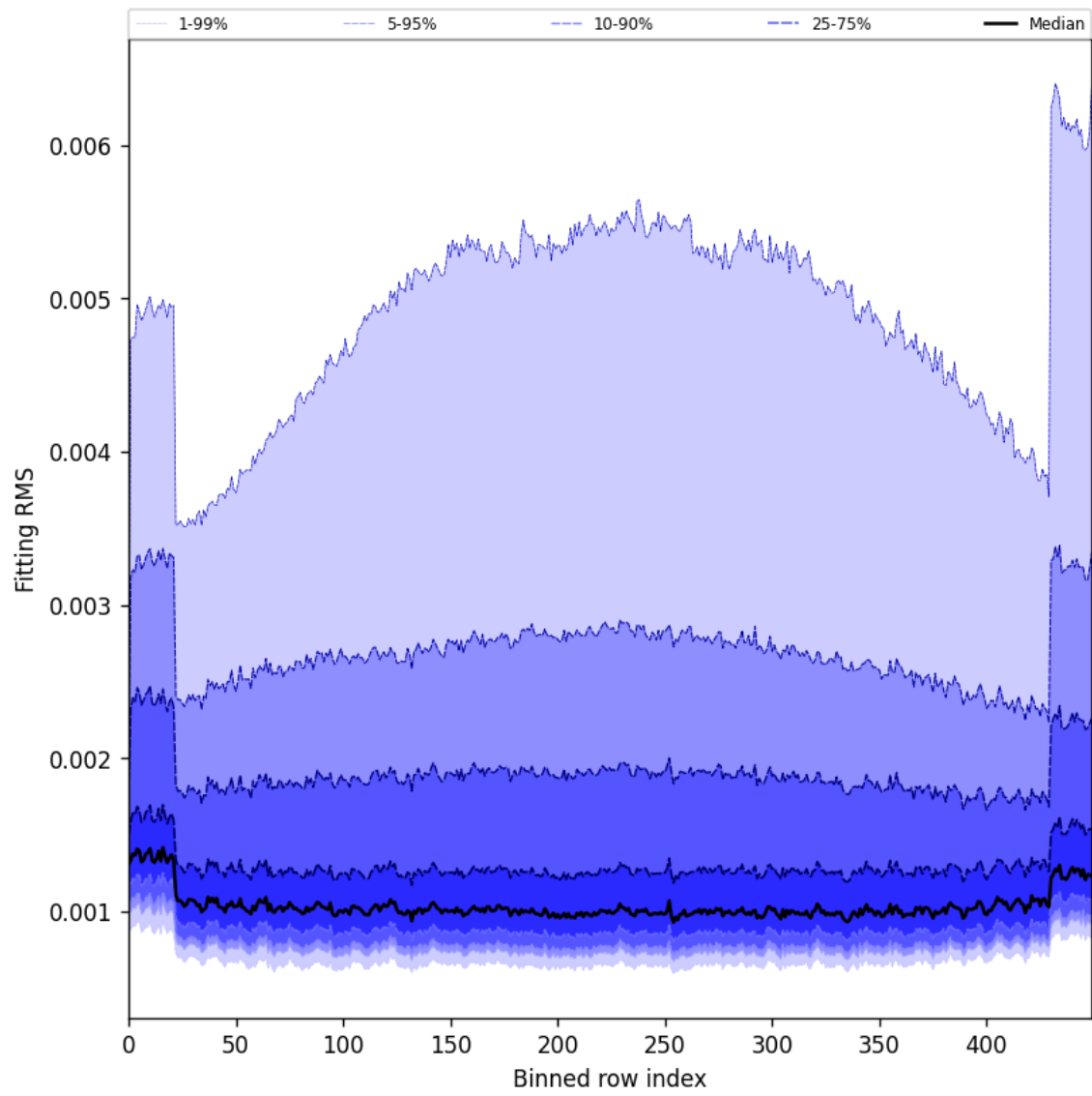
Figure 30: Along track statistics of “Fitting RMS” for 2025-05-10 to 2025-05-12
