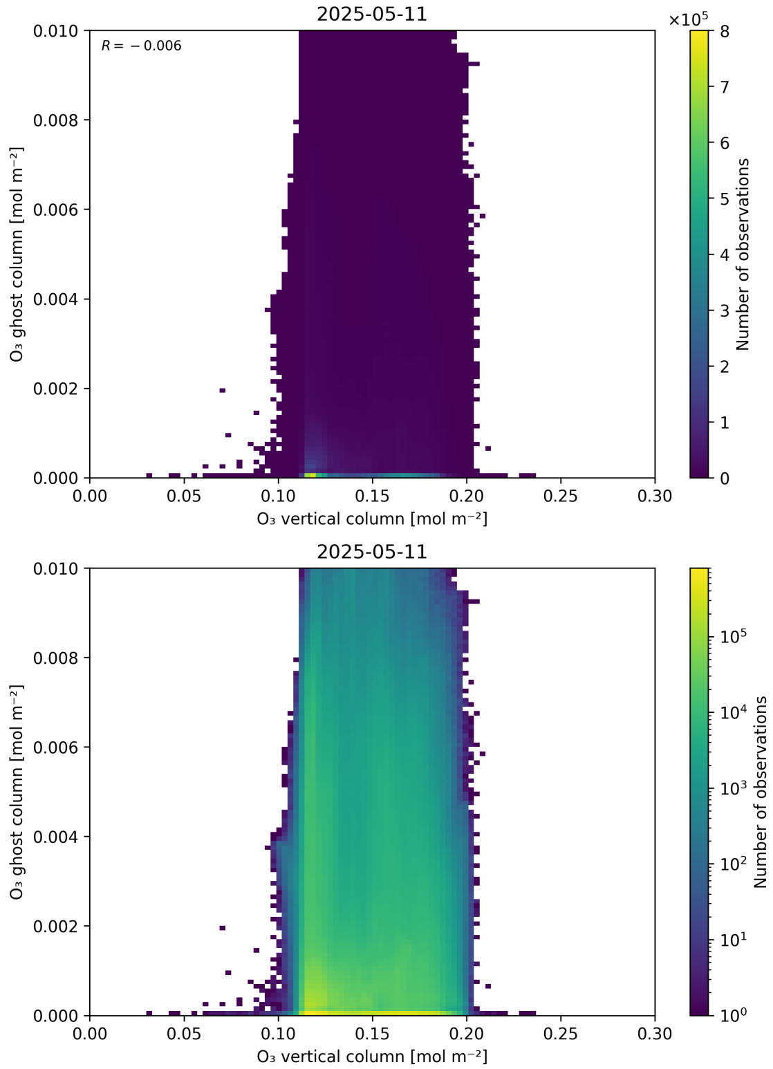
Figure 40: Scatter density plot of “O 3 vertical column” against “O 3 ghost column” for 2025-05-10 to 2025-05-12.
