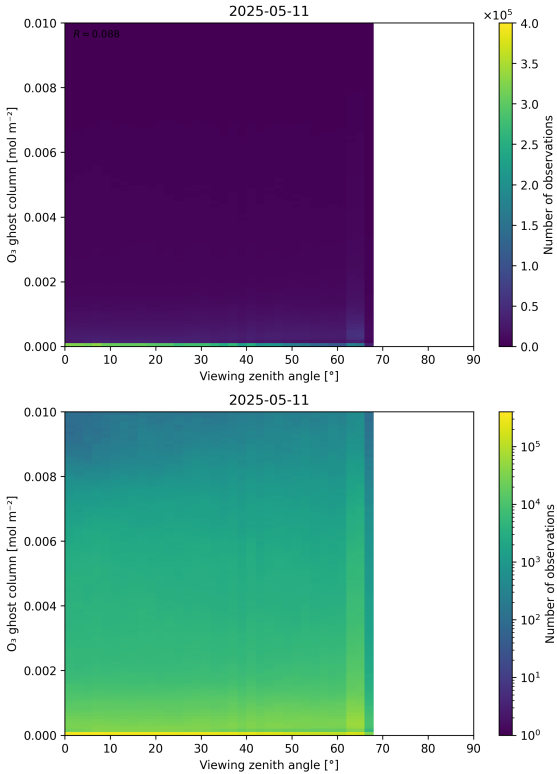
Figure 51: Scatter density plot of “Viewing zenith angle” against “O 3 ghost column” for 2025-05-10 to 2025-05-12.
