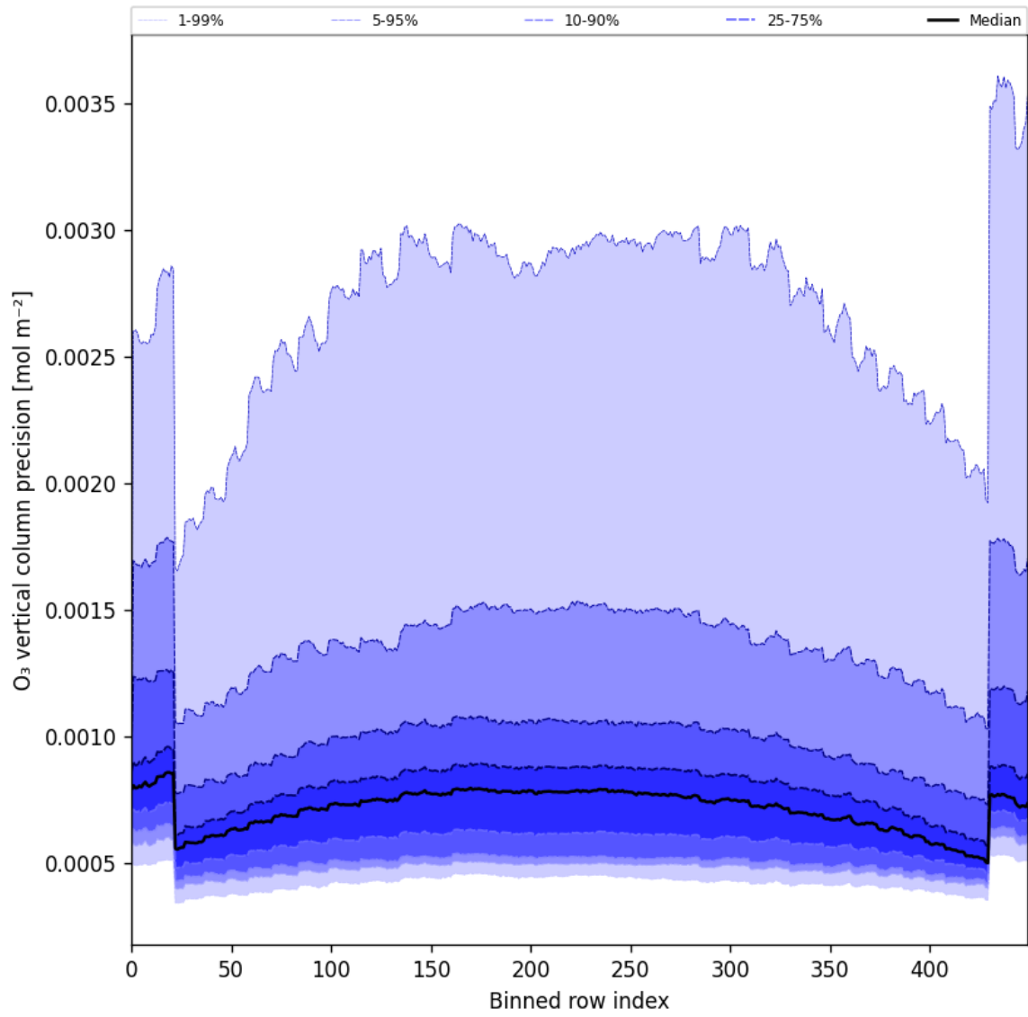
Figure 29: Along track statistics of “O 3 vertical column precision” for 2025-05-10 to 2025-05-12
