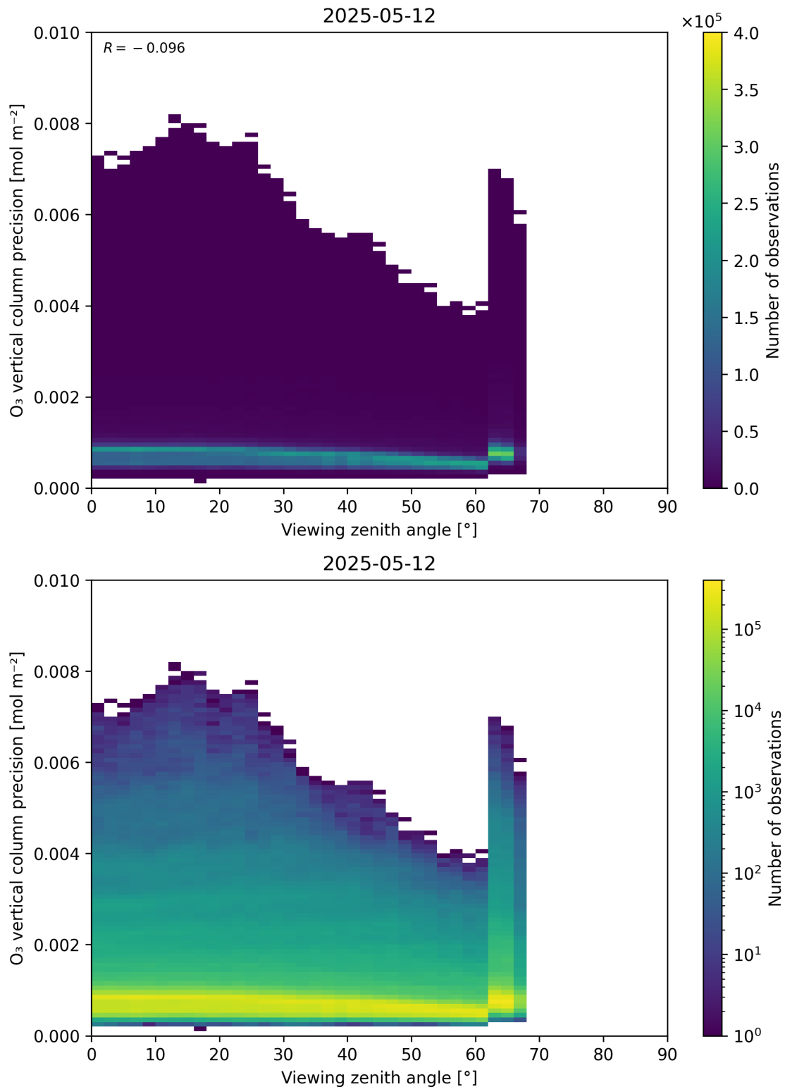
Figure 53: Scatter density plot of “Viewing zenith angle” against “O 3 vertical column precision” for 2025-05-11 to 2025-05-13.
