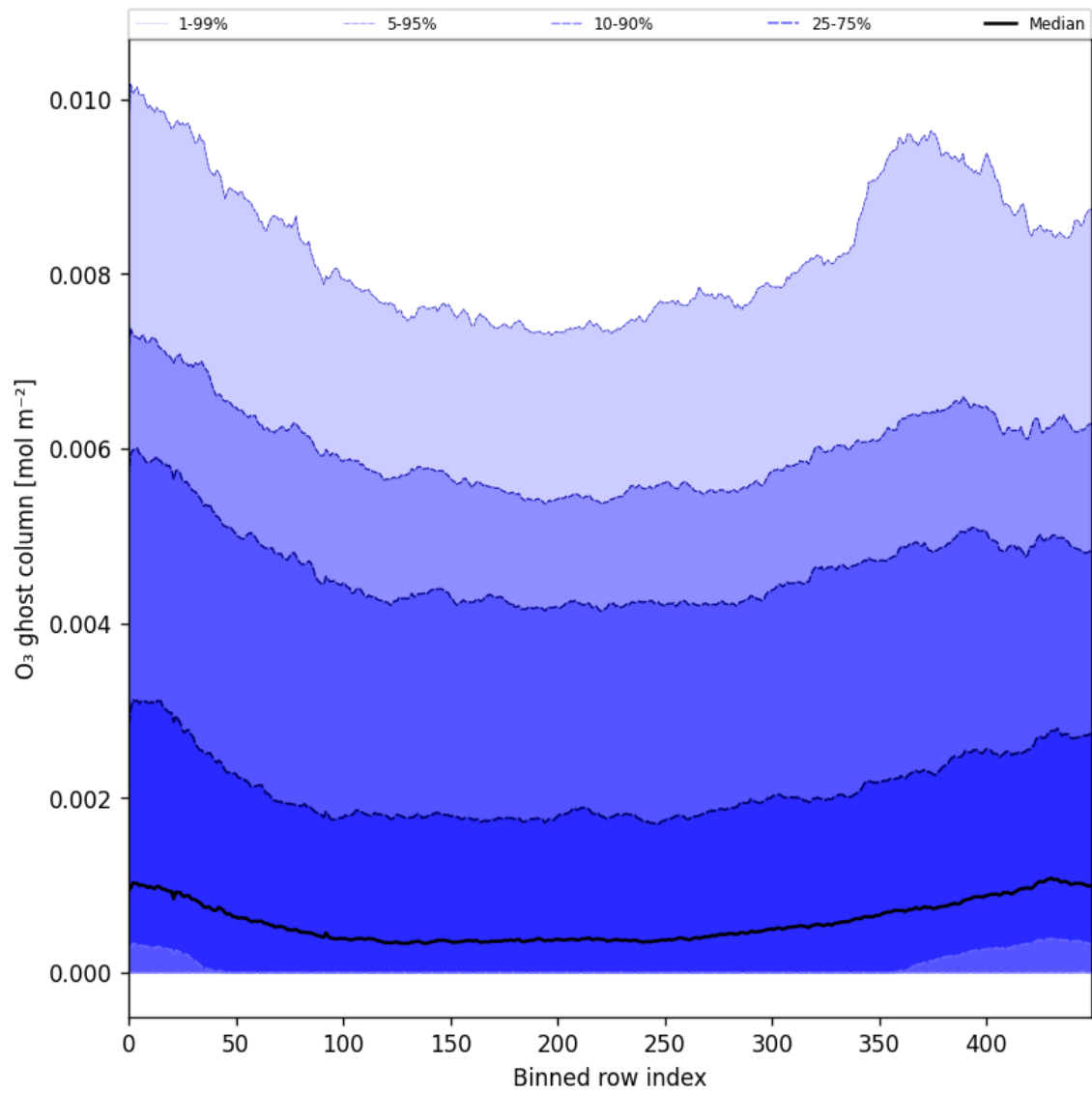
Figure 32: Along track statistics of “O 3 ghost column” for 2025-05-11 to 2025-05-13
