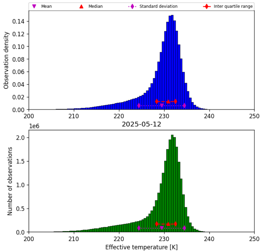
Figure 24: Histogram of “Effective temperature” for 2025-05-11 to 2025-05-13
