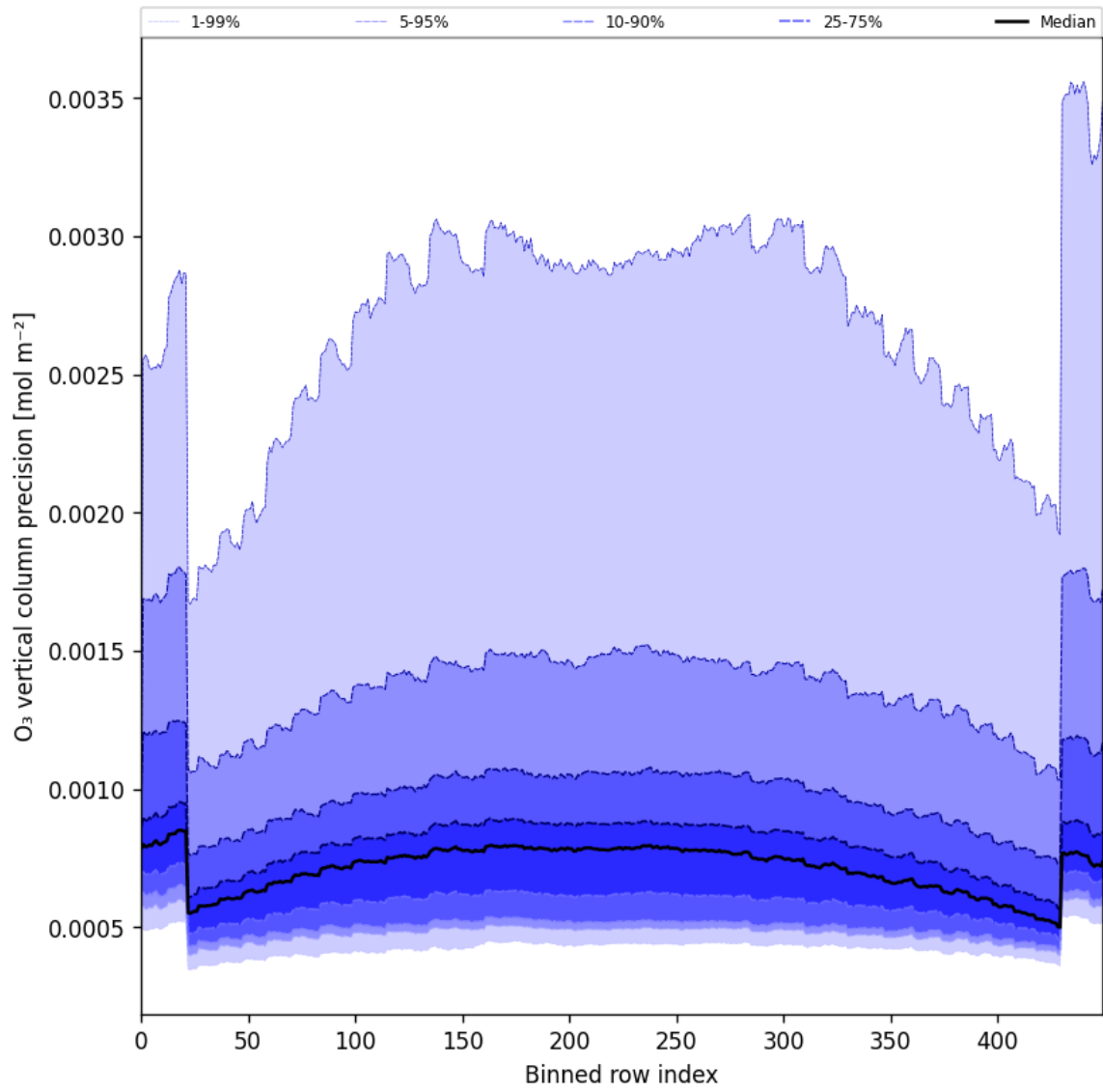
Figure 29: Along track statistics of “O 3 vertical column precision” for 2025-05-11 to 2025-05-13
