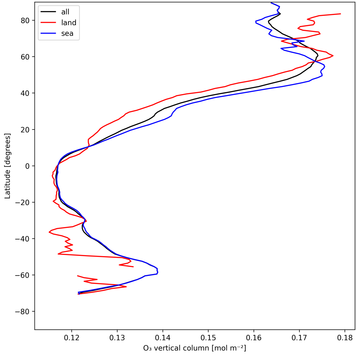
Figure 14: Zonal average of “O 3 vertical column” for 2025-05-11 to 2025-05-13.
