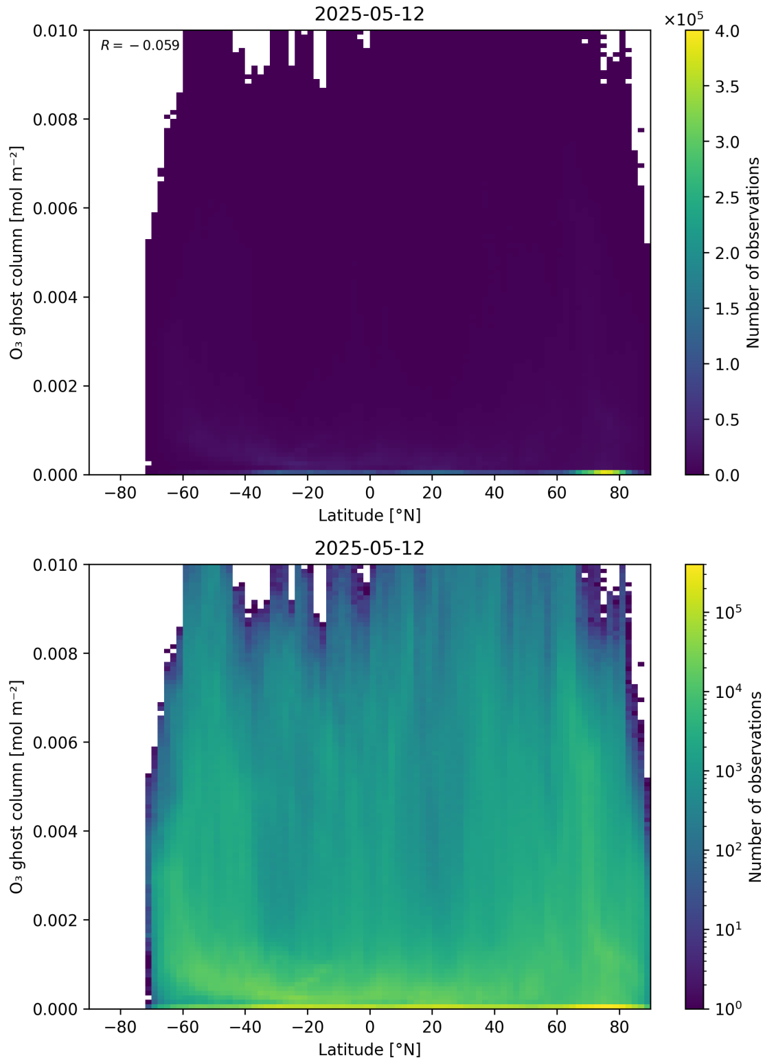
Figure 35: Scatter density plot of “Latitude” against “O 3 ghost column” for 2025-05-11 to 2025-05-13.
