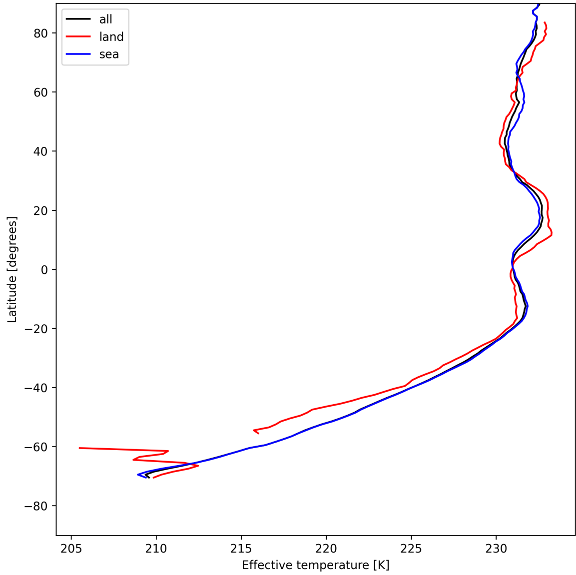
Figure 17: Zonal average of "Effective temperature" for 2025-05-11 to 2025-05-13.
