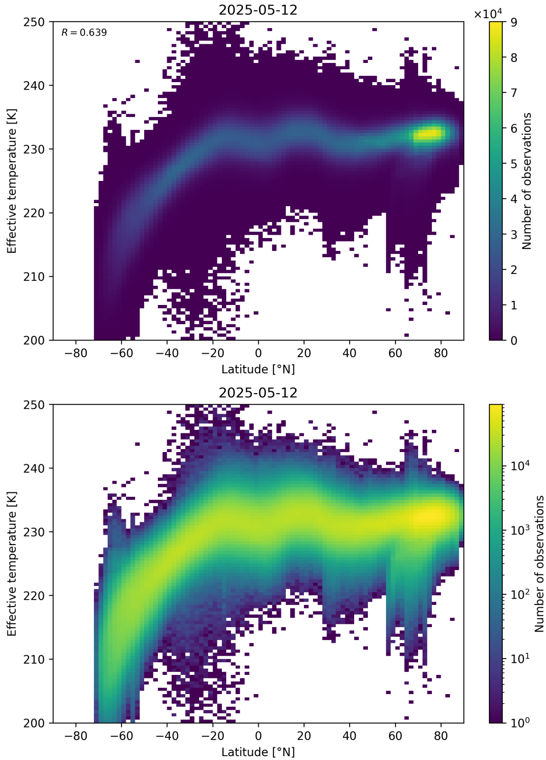
Figure 34: Scatter density plot of “Latitude” against “Effective temperature” for 2025-05-11 to 2025-05-13.
