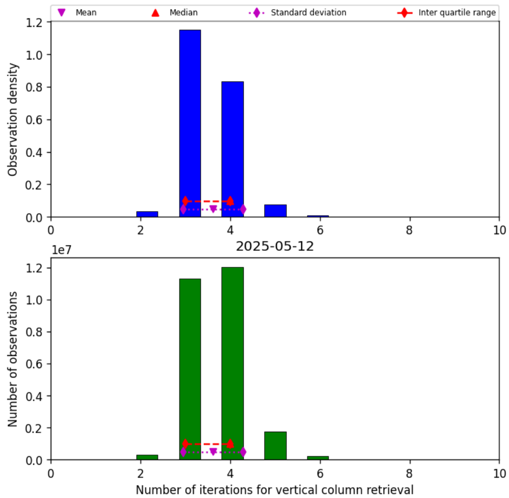
Figure 26: Histogram of “Number of iterations for vertical column retrieval” for 2025-05-11 to 2025-05-13
