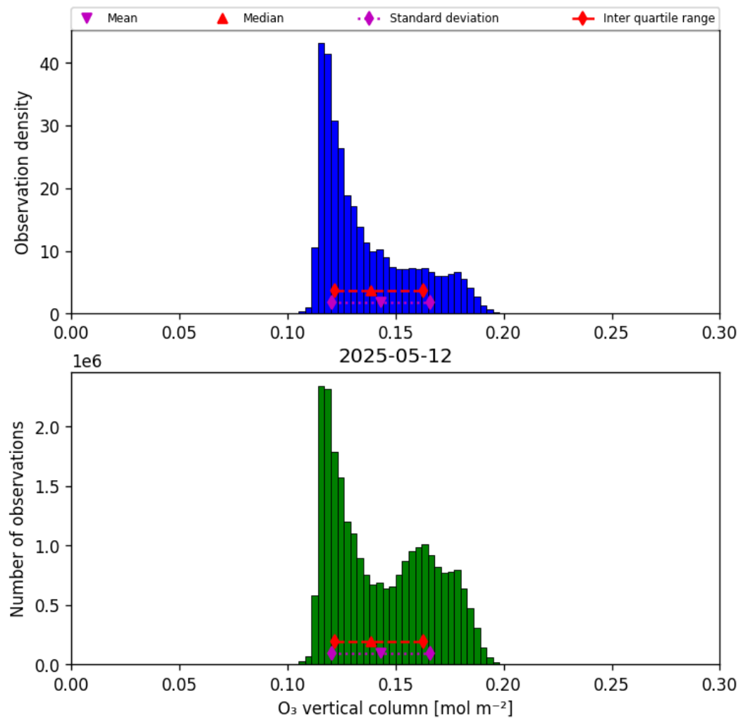
Figure 21: Histogram of “O 3 vertical column” for 2025-05-11 to 2025-05-13
