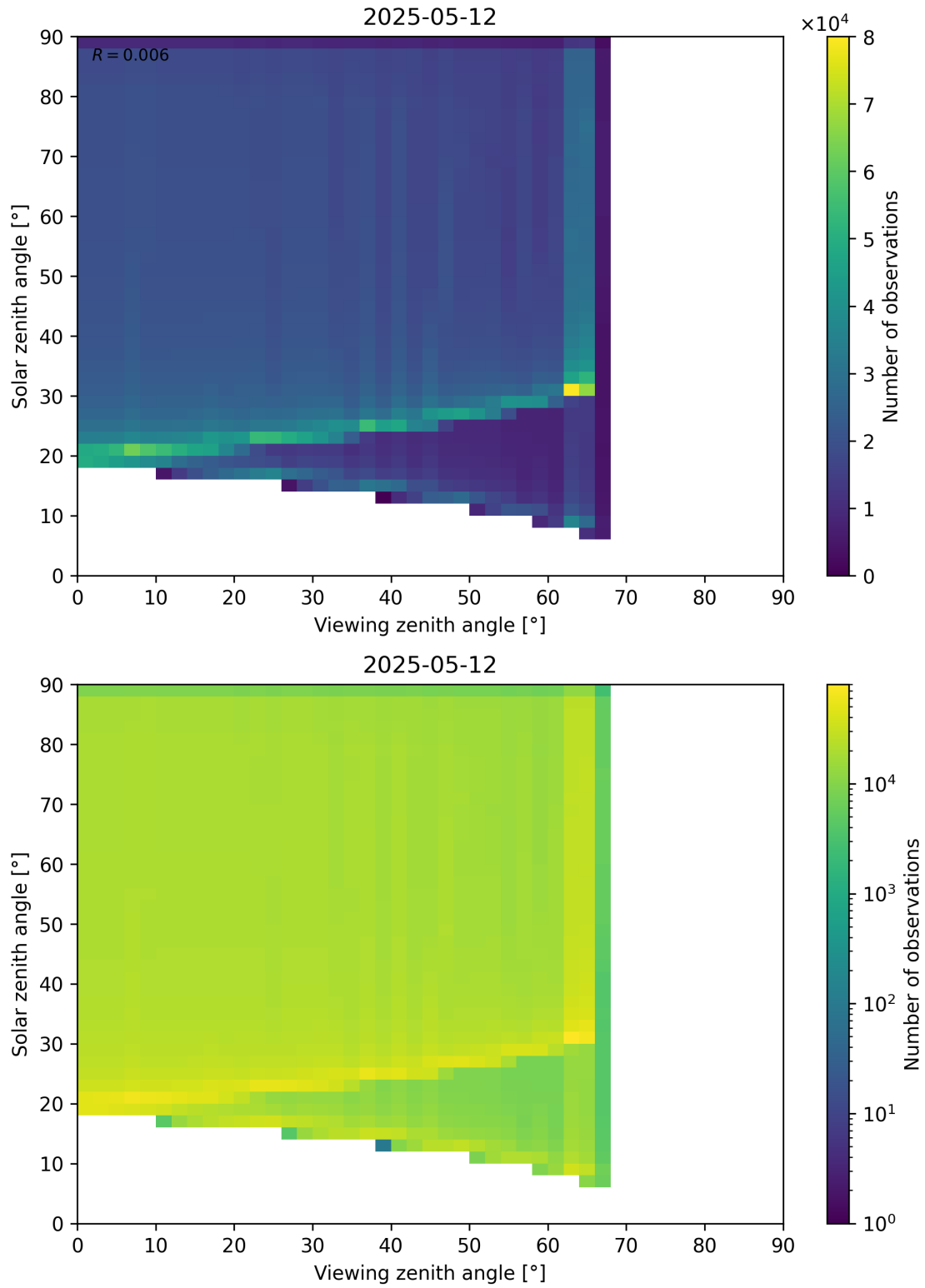
Figure 54: Scatter density plot of “Viewing zenith angle” against “Solar zenith angle” for 2025-05-11 to 2025-05-13.
