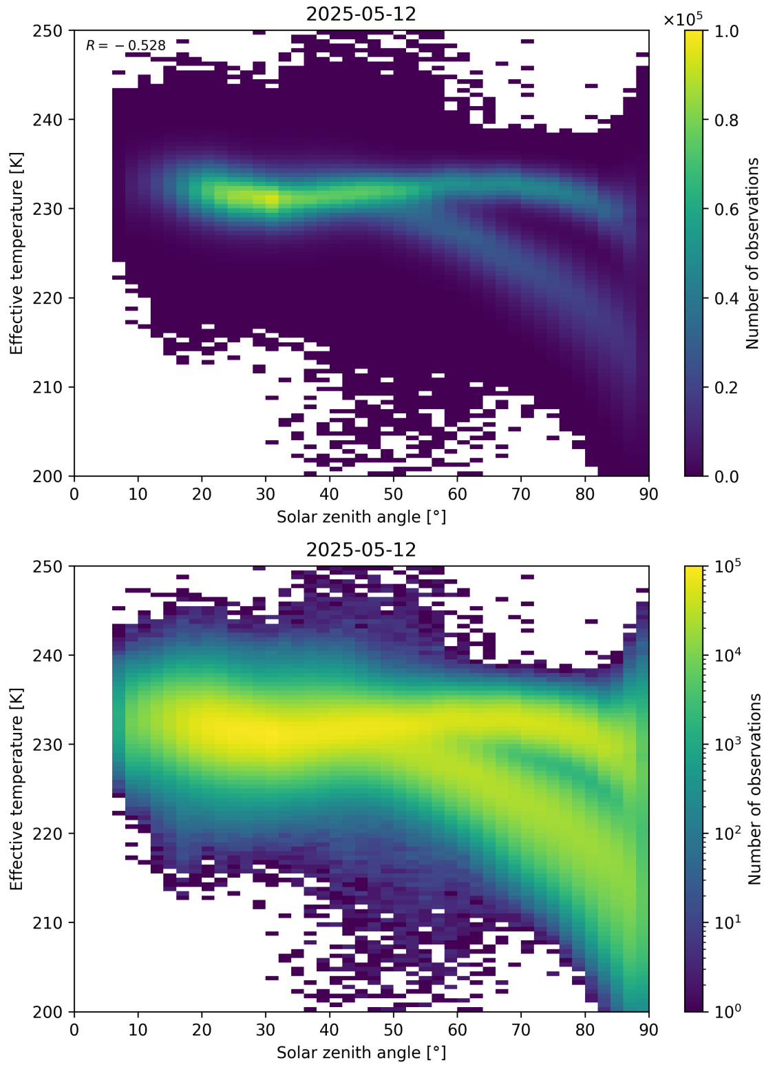
Figure 45: Scatter density plot of “Solar zenith angle” against “Effective temperature” for 2025-05-11 to 2025-05-13.
