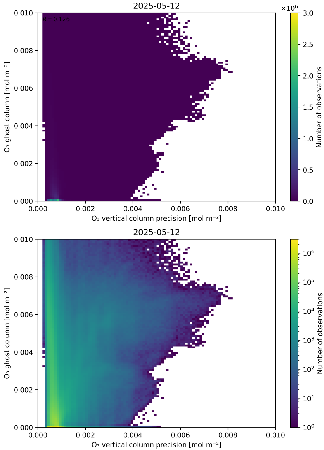
Figure 43: Scatter density plot of “O 3 vertical column precision” against “O 3 ghost column” for 2025-05-11 to 2025-05-13.
