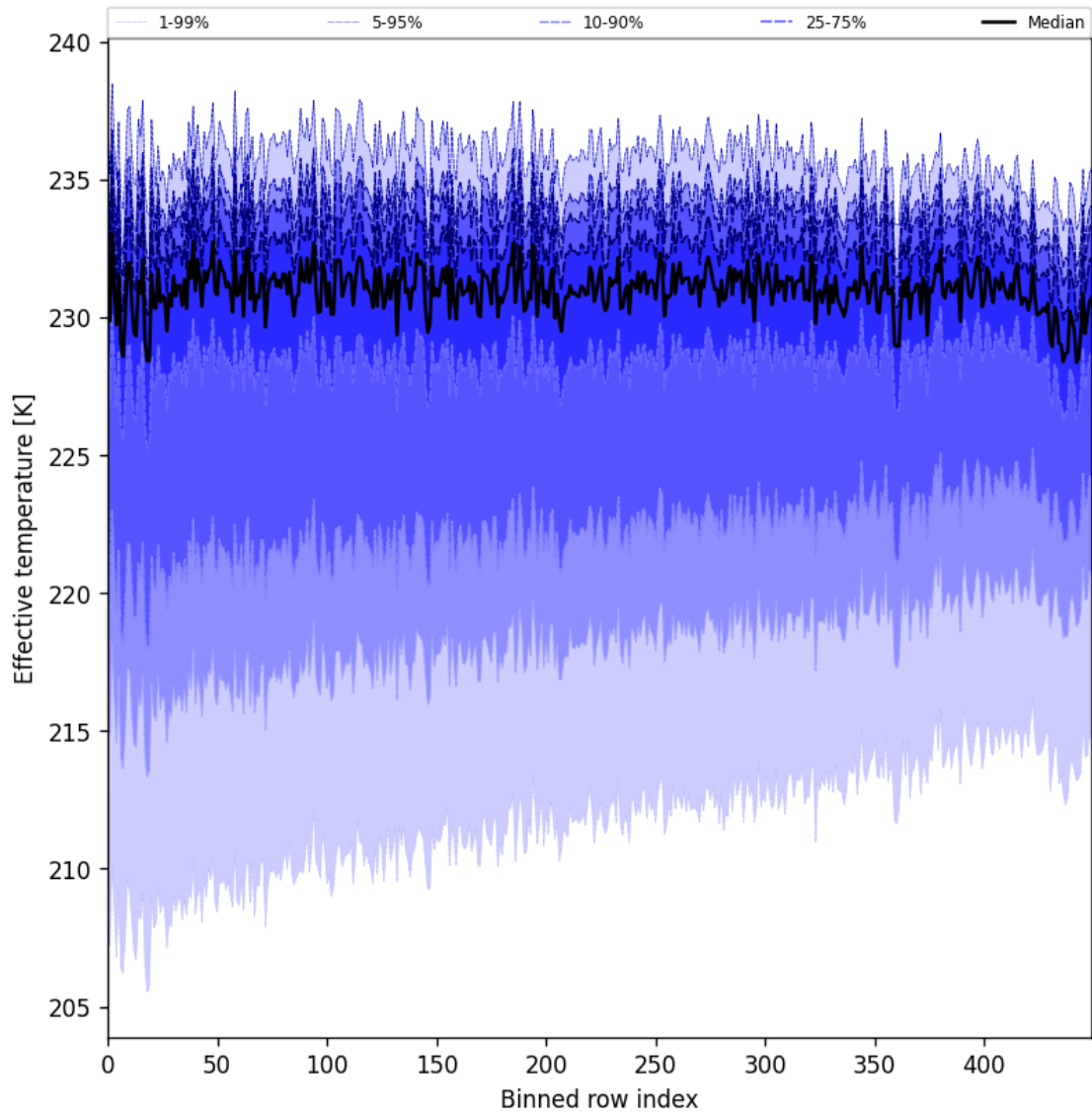
Figure 31: Along track statistics of "Effective temperature" for 2025-05-11 to 2025-05-13
