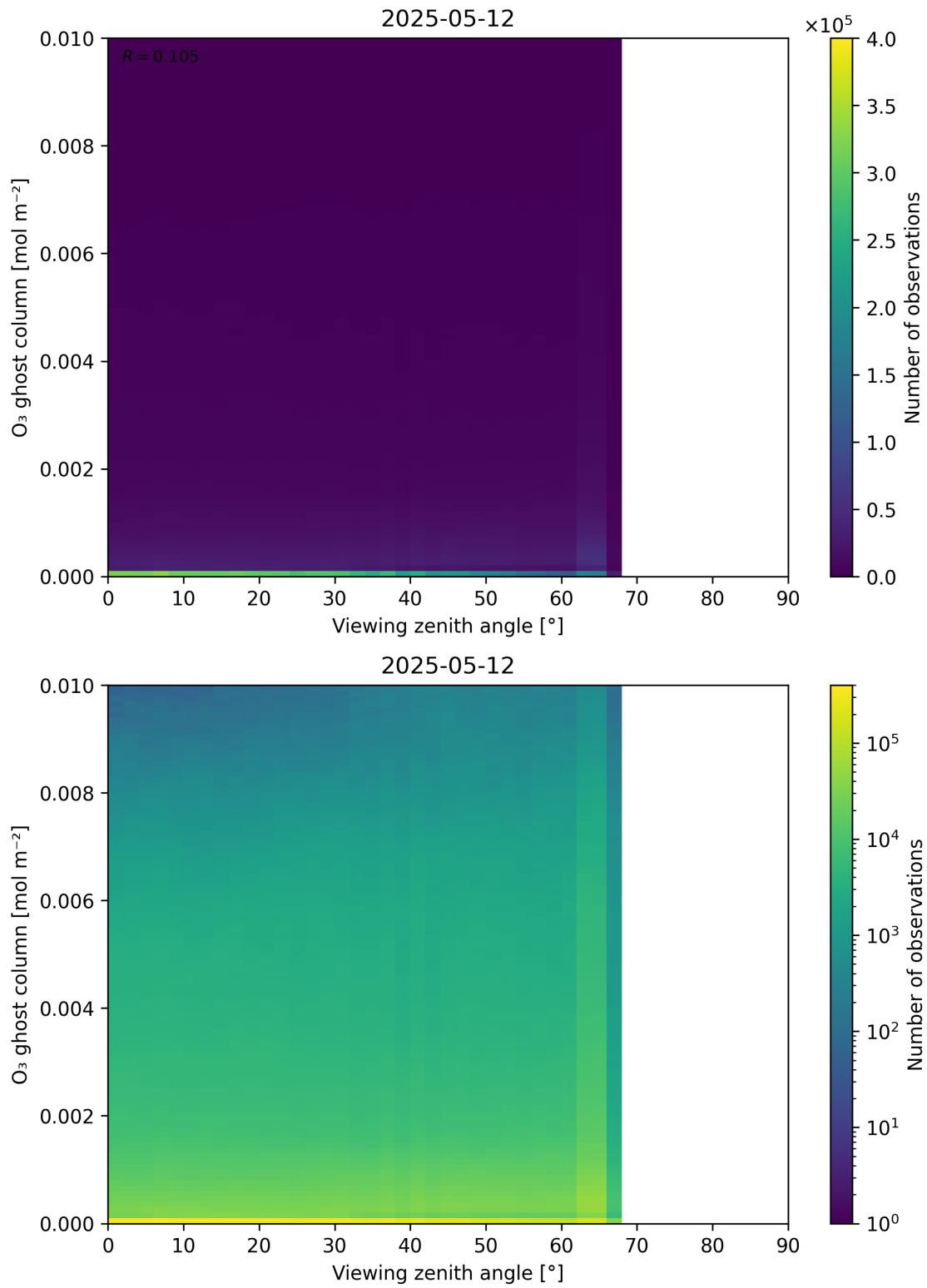
Figure 51: Scatter density plot of “Viewing zenith angle” against “O 3 ghost column” for 2025-05-11 to 2025-05-13.
