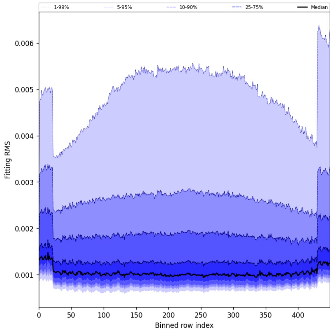
Figure 30: Along track statistics of “Fitting RMS” for 2025-05-11 to 2025-05-13
