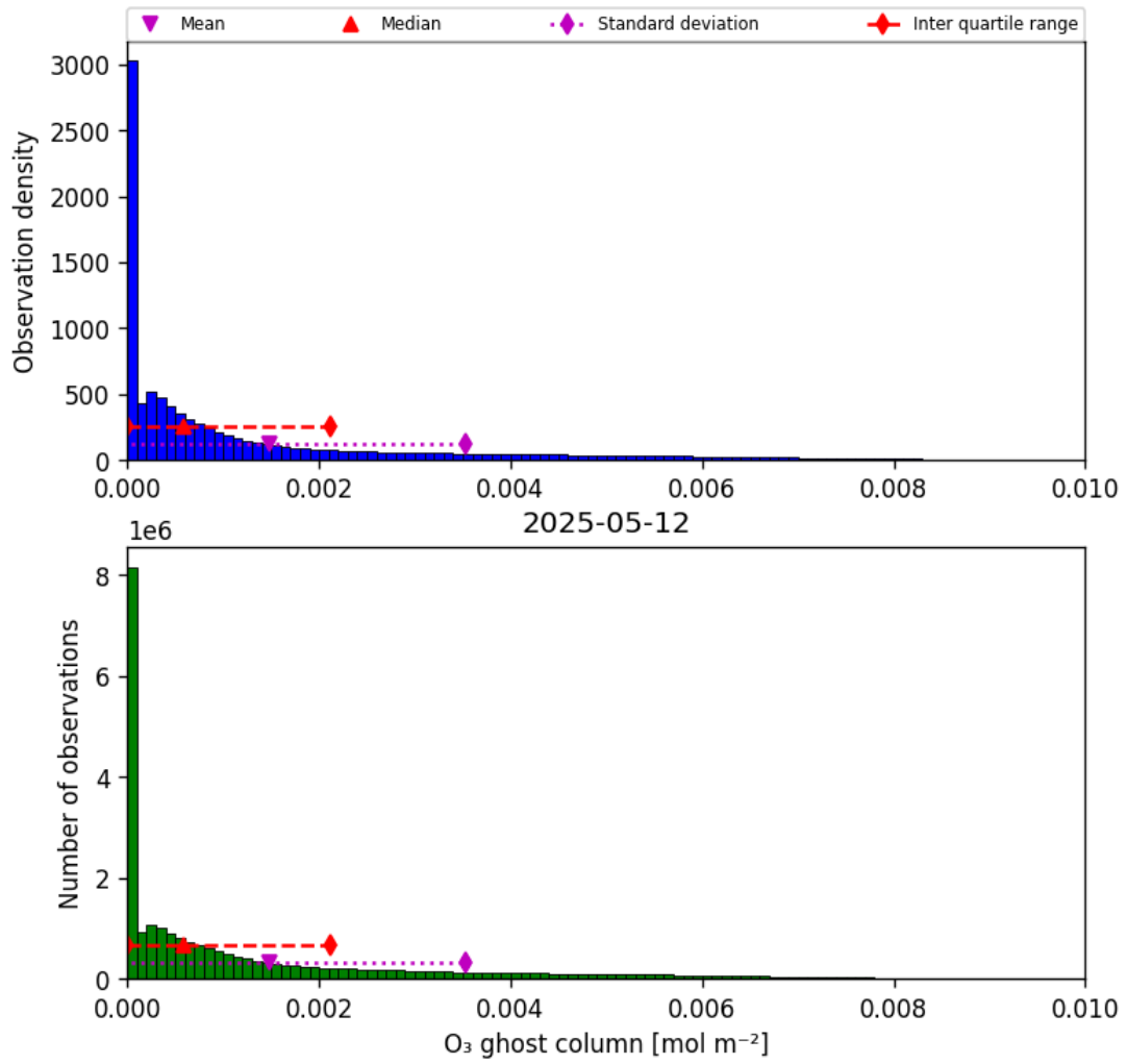
Figure 25: Histogram of “O 3 ghost column” for 2025-05-11 to 2025-05-13
