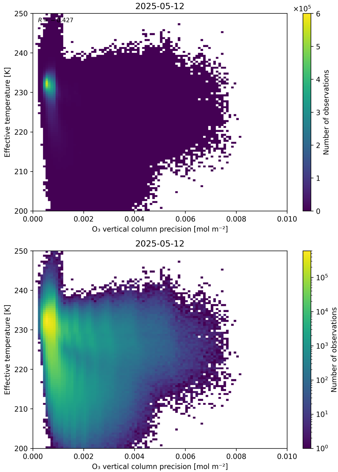
Figure 42: Scatter density plot of “O 3 vertical column precision” against “Effective temperature” for 2025-05-11 to 2025-05-13.
