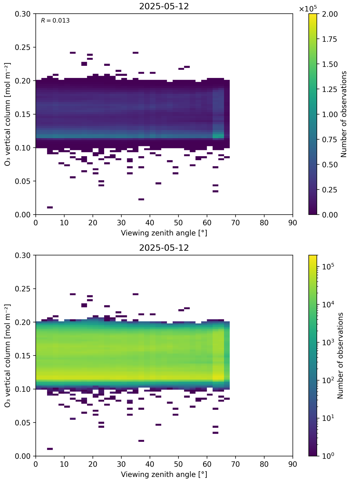
Figure 52: Scatter density plot of “Viewing zenith angle” against “O 3 vertical column” for 2025-05-11 to 2025-05-13.
