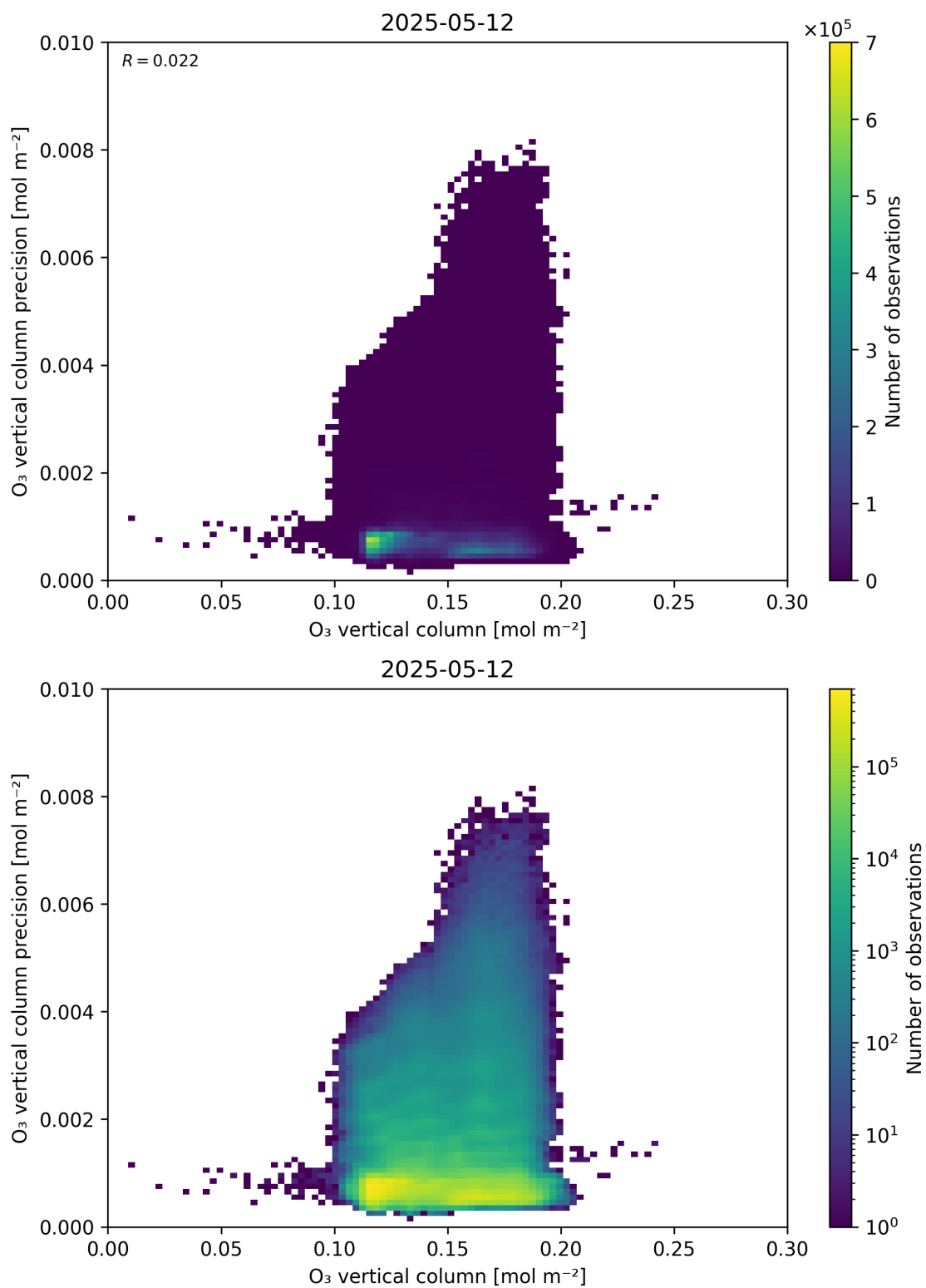
Figure 41: Scatter density plot of “O 3 vertical column” against “O 3 vertical column precision” for 2025-05-11 to 2025-05-13.
