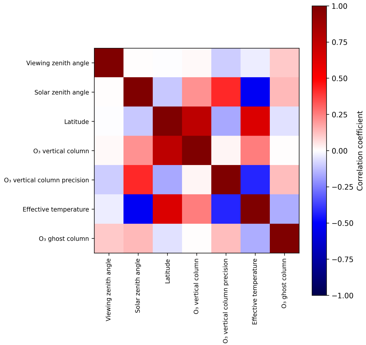
Figure 2: Map of correlation matrix for 2025-05-11 to 2025-05-13.
