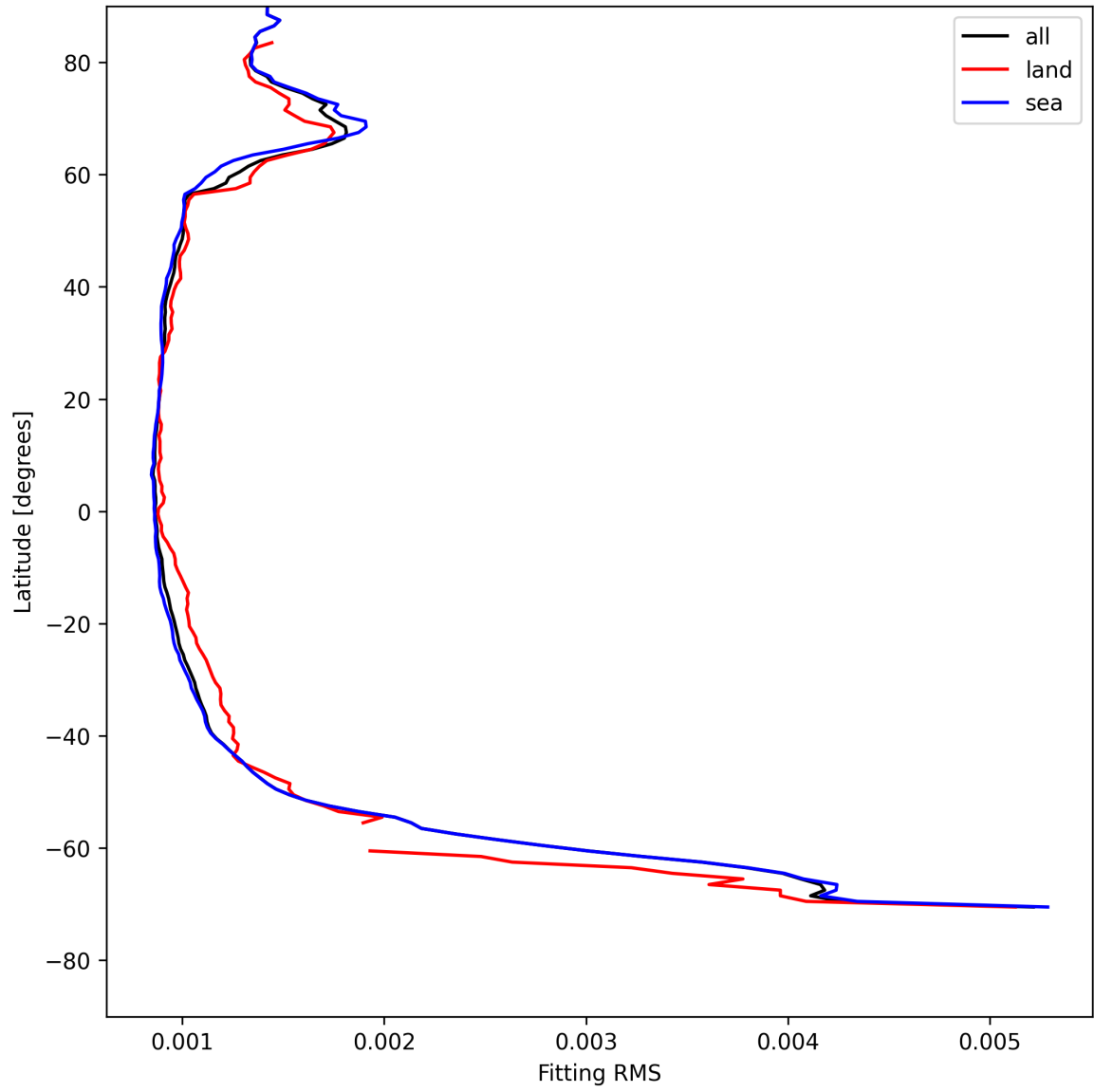
Figure 16: Zonal average of “Fitting RMS” for 2025-05-11 to 2025-05-13.
