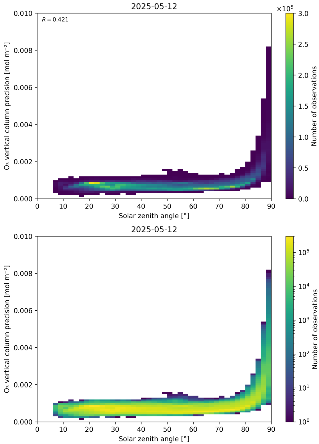
Figure 48: Scatter density plot of “Solar zenith angle” against “O 3 vertical column precision” for 2025-05-11 to 2025-05-13.
