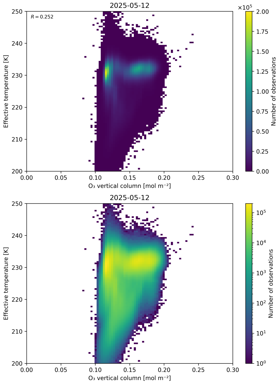
Figure 39: Scatter density plot of “O 3 vertical column” against “Effective temperature” for 2025-05-11 to 2025-05-13.
