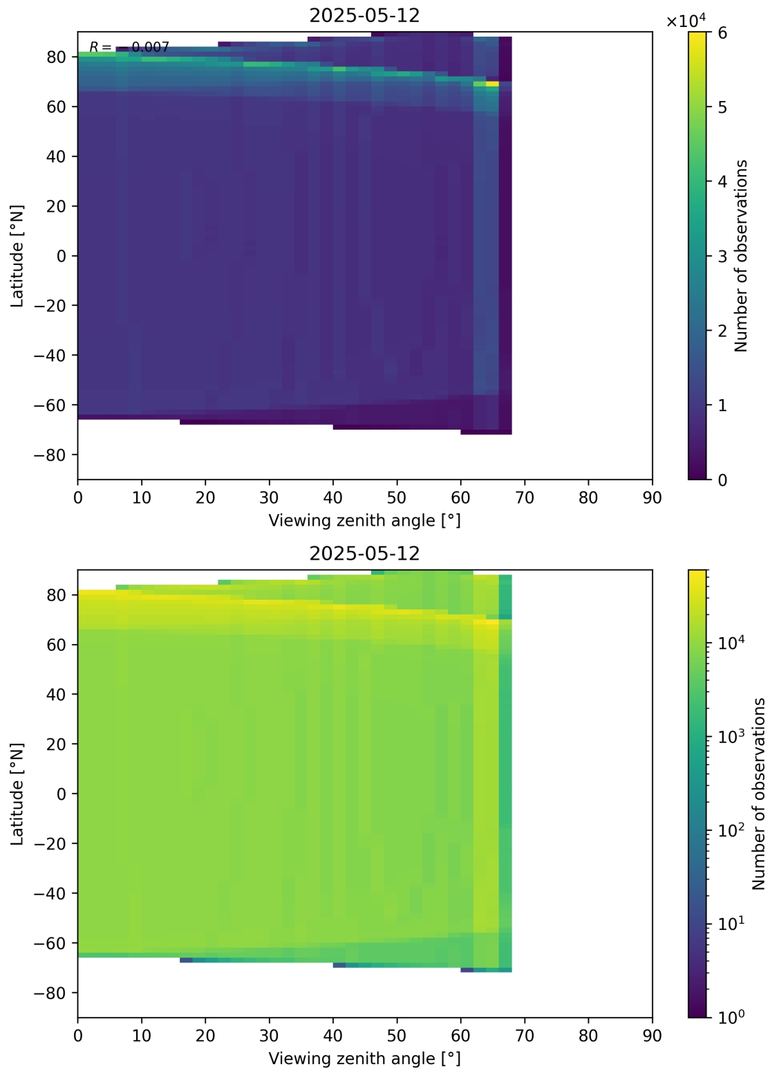
Figure 49: Scatter density plot of “Viewing zenith angle” against “Latitude” for 2025-05-11 to 2025-05-13.
