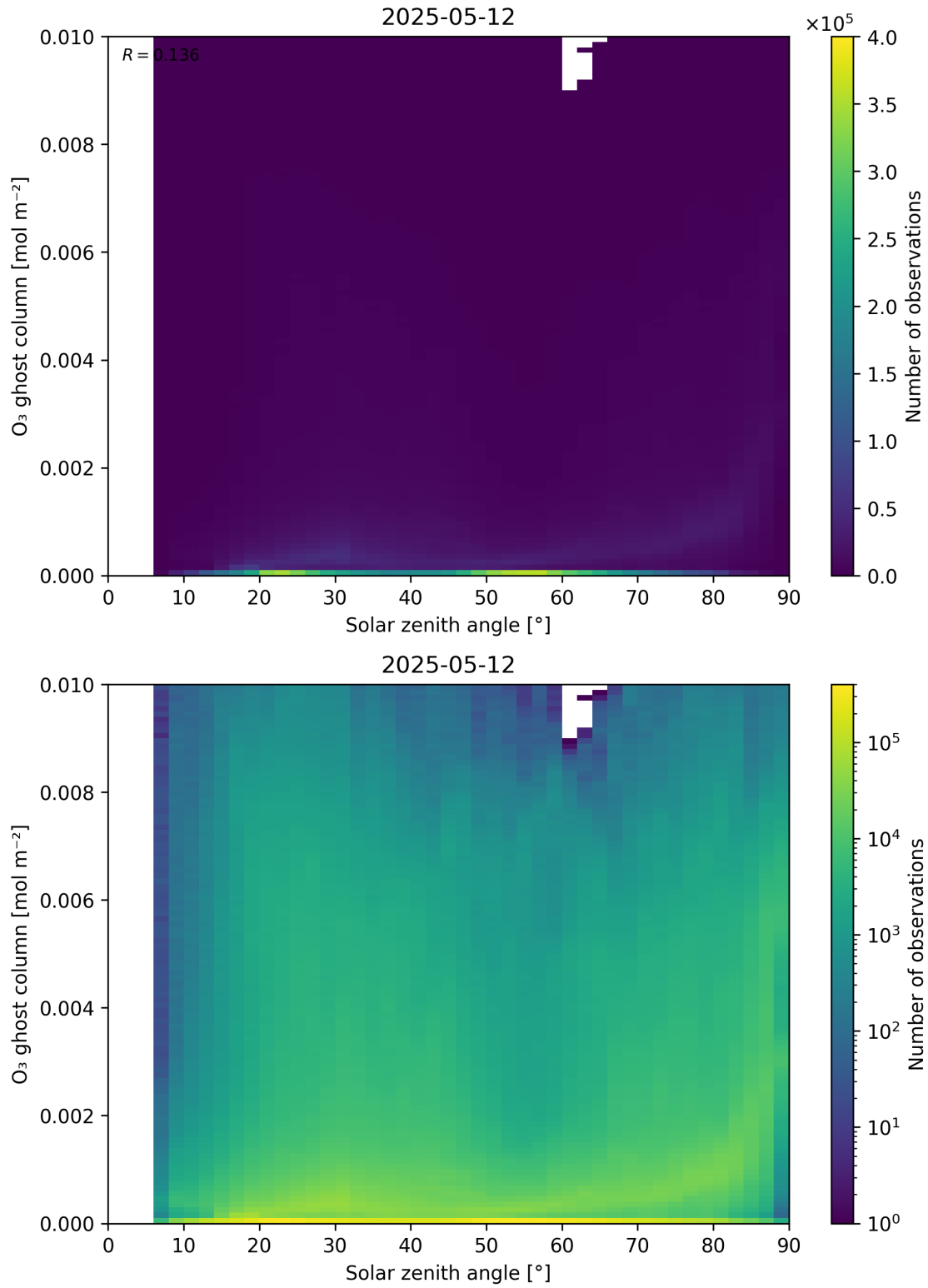
Figure 46: Scatter density plot of “Solar zenith angle” against “O 3 ghost column” for 2025-05-11 to 2025-05-13.
