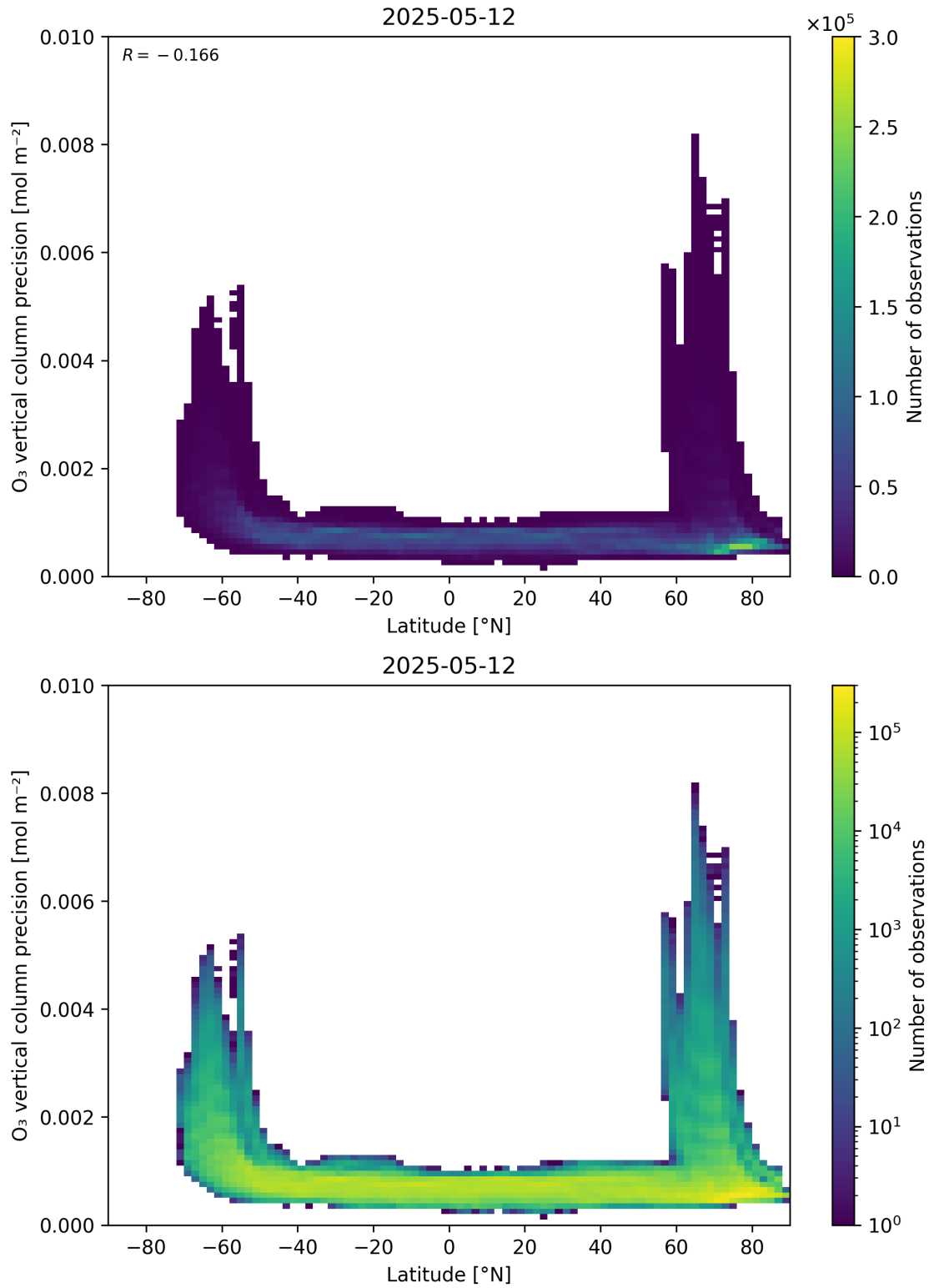
Figure 37: Scatter density plot of “Latitude” against “O 3 vertical column precision” for 2025-05-11 to 2025-05-13.
