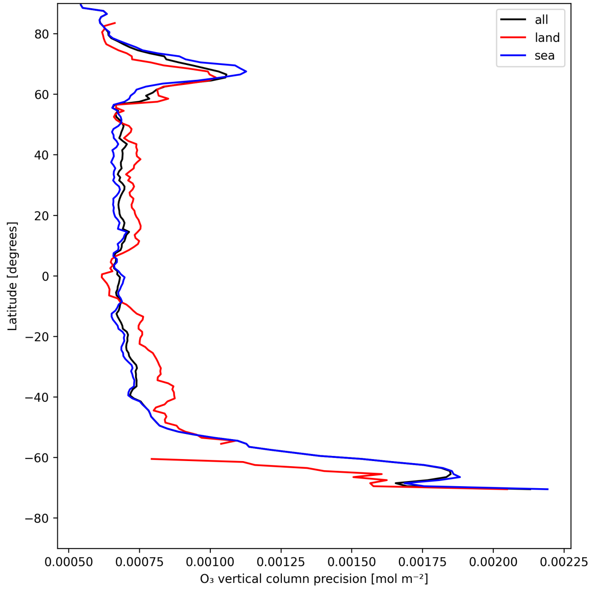
Figure 15: Zonal average of “O 3 vertical column precision” for 2025-05-11 to 2025-05-13.
