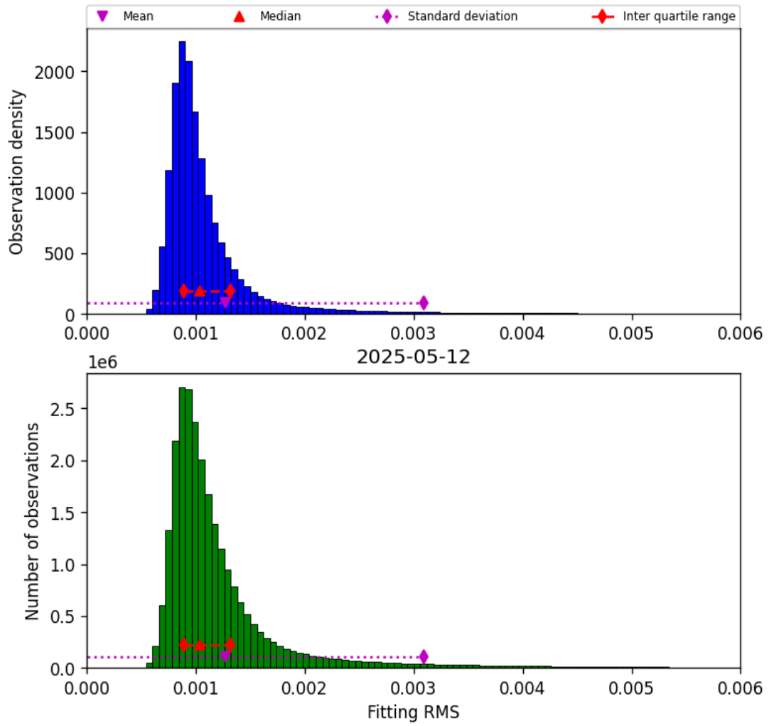
Figure 23: Histogram of “Fitting RMS” for 2025-05-11 to 2025-05-13
