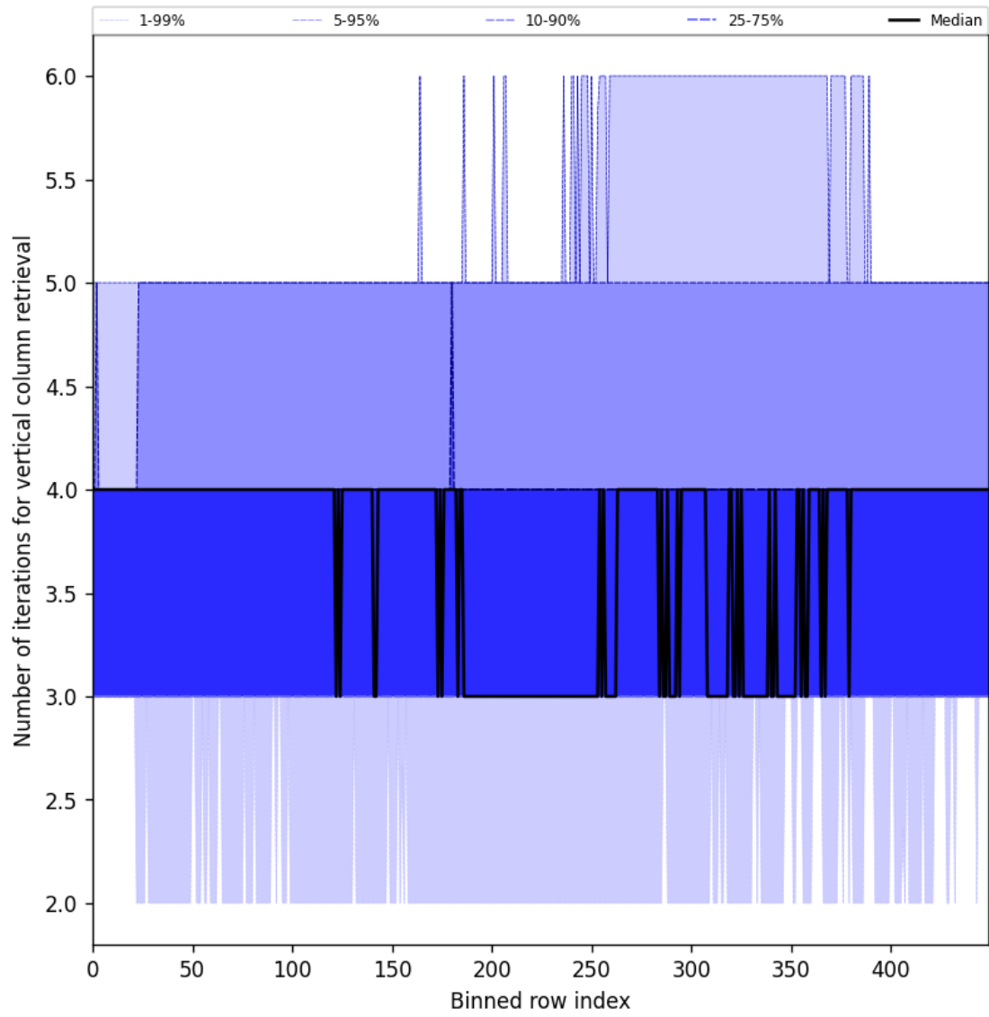
Figure 33: Along track statistics of “Number of iterations for vertical column retrieval” for 2025-05-11 to 2025-05-13
