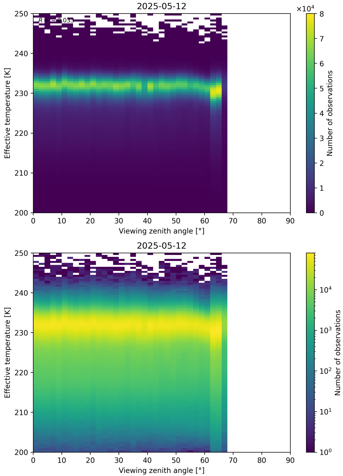
Figure 50: Scatter density plot of “Viewing zenith angle” against “Effective temperature” for 2025-05-11 to 2025-05-13.
