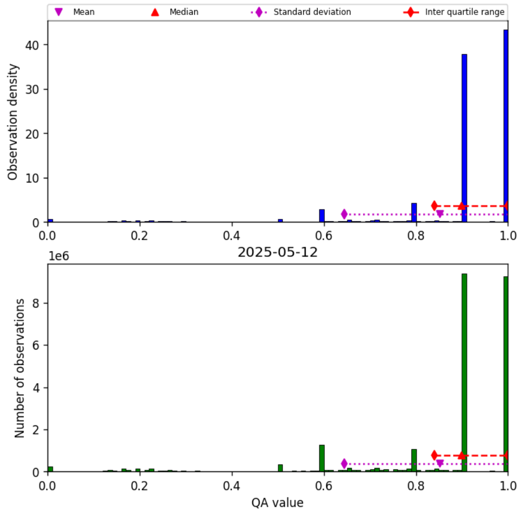
Figure 20: Histogram of “QA value” for 2025-05-11 to 2025-05-13
