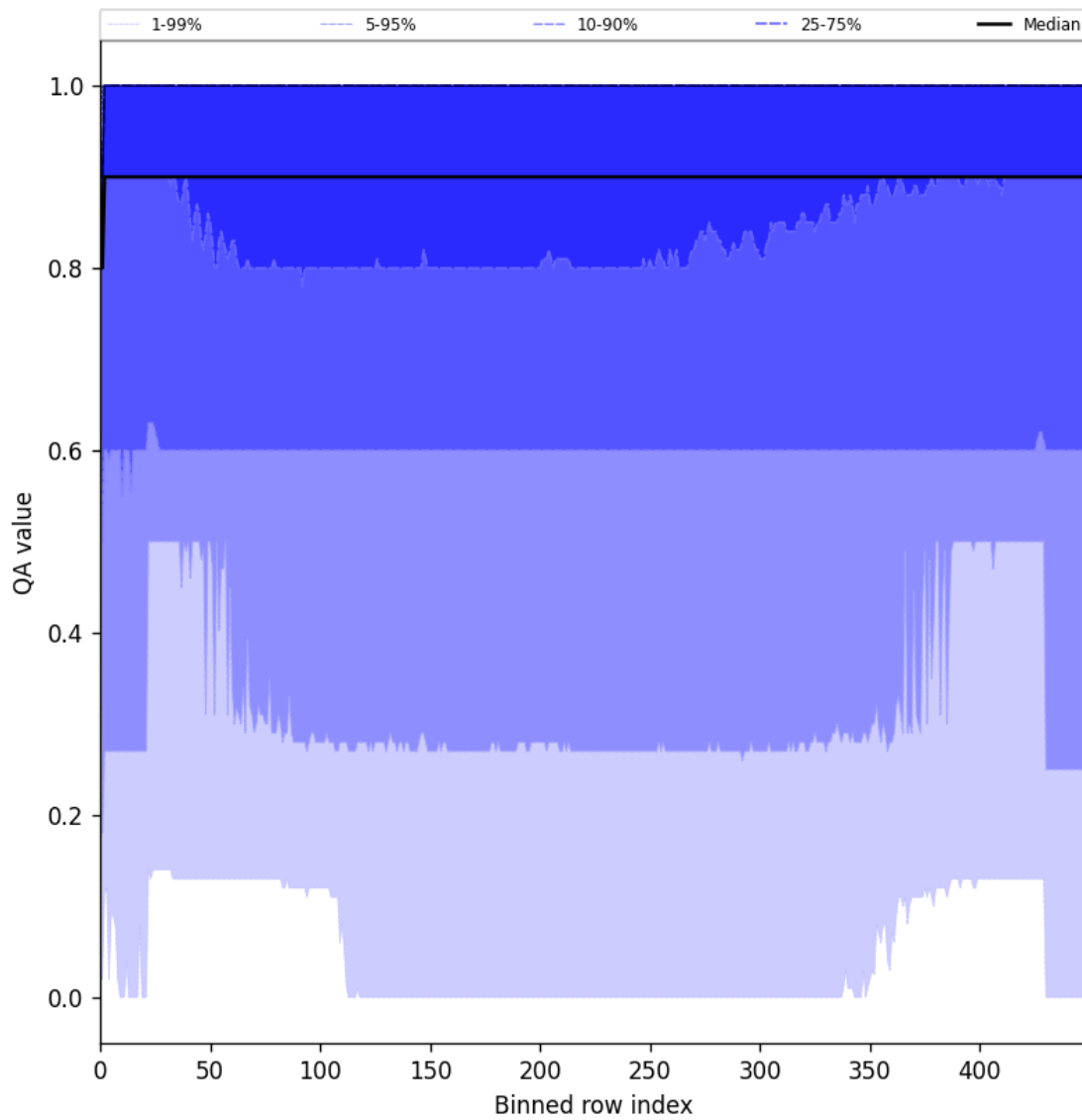
Figure 27: Along track statistics of “QA value” for 2025-05-11 to 2025-05-13
