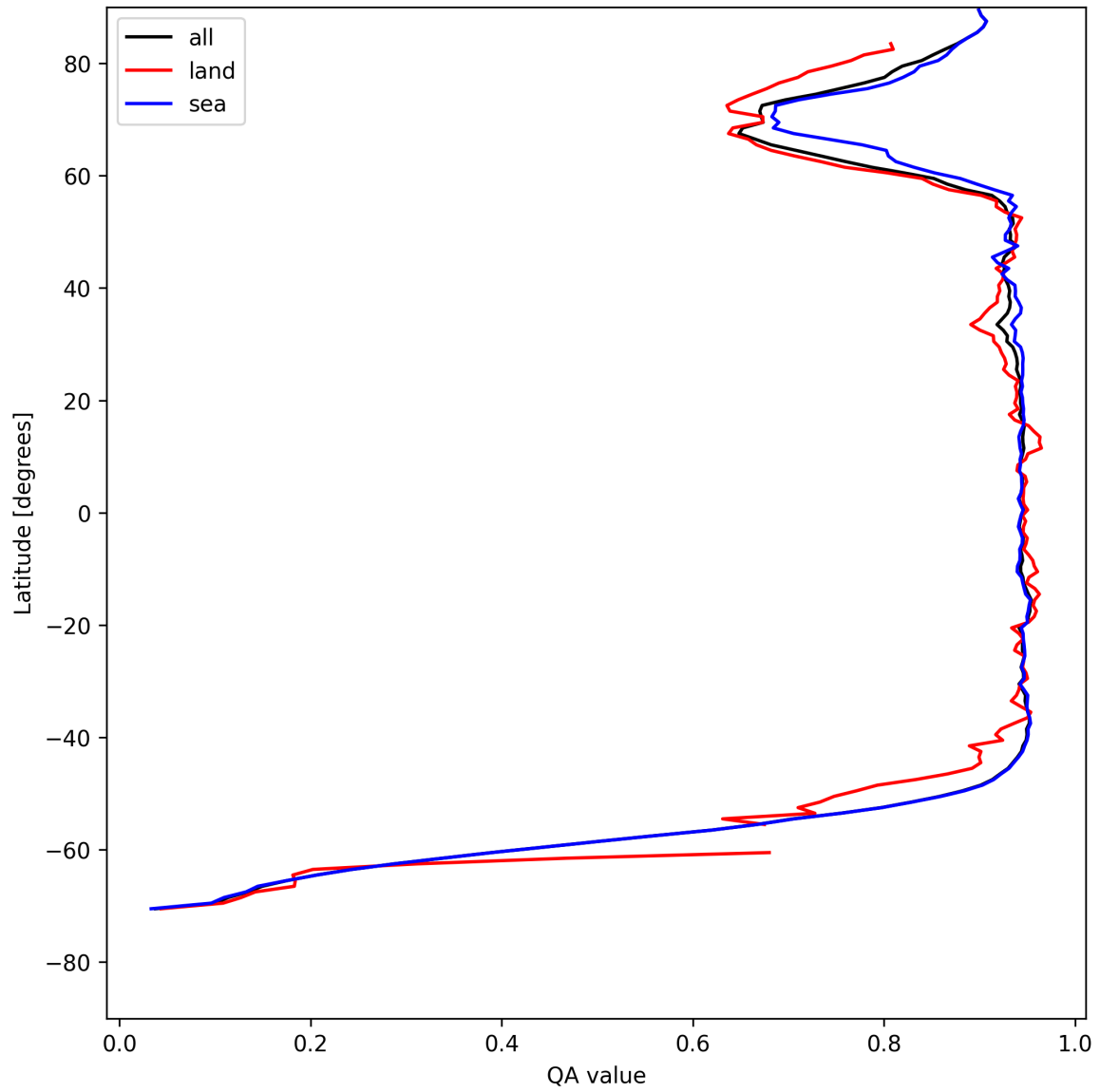
Figure 13: Zonal average of “QA value” for 2025-05-11 to 2025-05-13.
