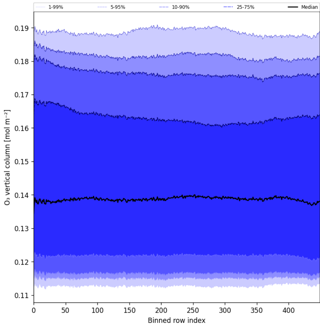
Figure 28: Along track statistics of “O 3 vertical column” for 2025-05-11 to 2025-05-13
