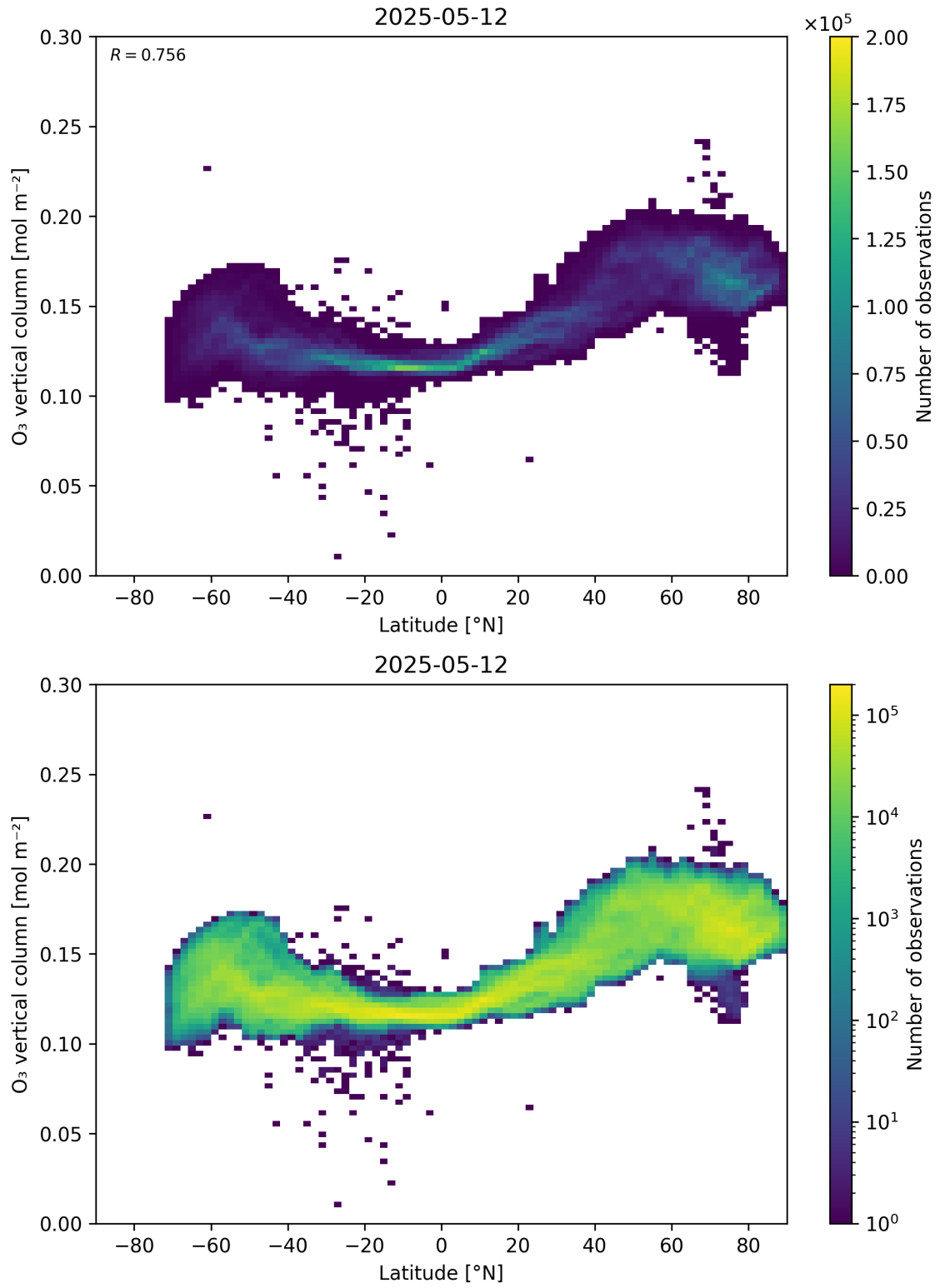
Figure 36: Scatter density plot of “Latitude” against “O 3 vertical column” for 2025-05-11 to 2025-05-13.
