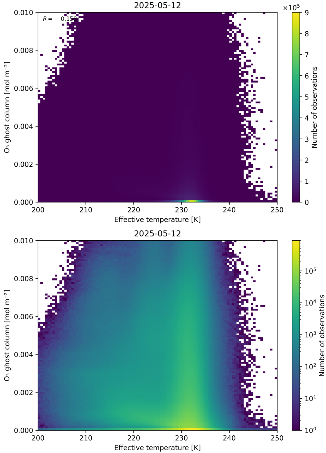
Figure 38: Scatter density plot of “Effective temperature” against “O 3 ghost column” for 2025-05-11 to 2025-05-13.
