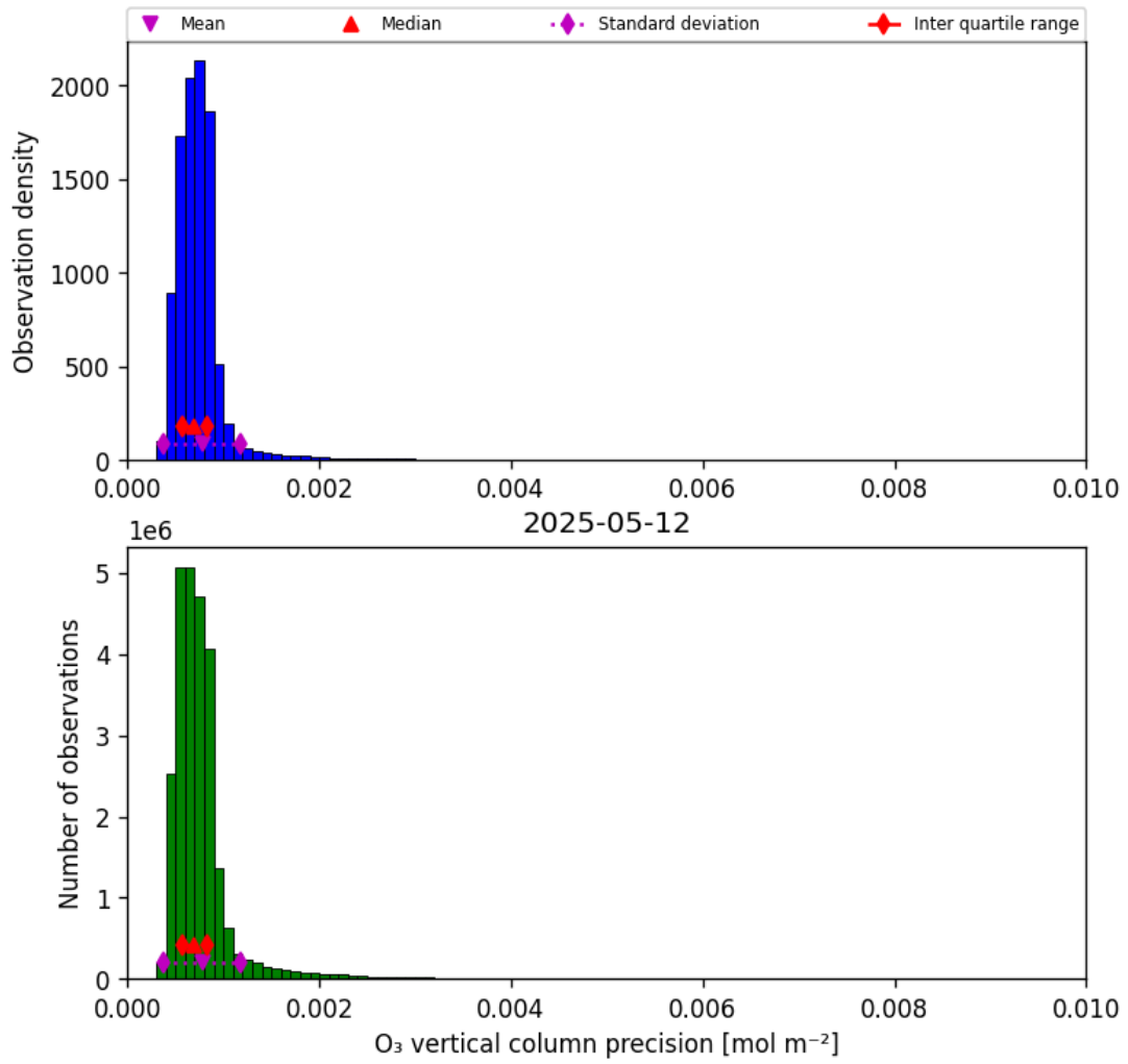
Figure 22: Histogram of “O 3 vertical column precision” for 2025-05-11 to 2025-05-13
