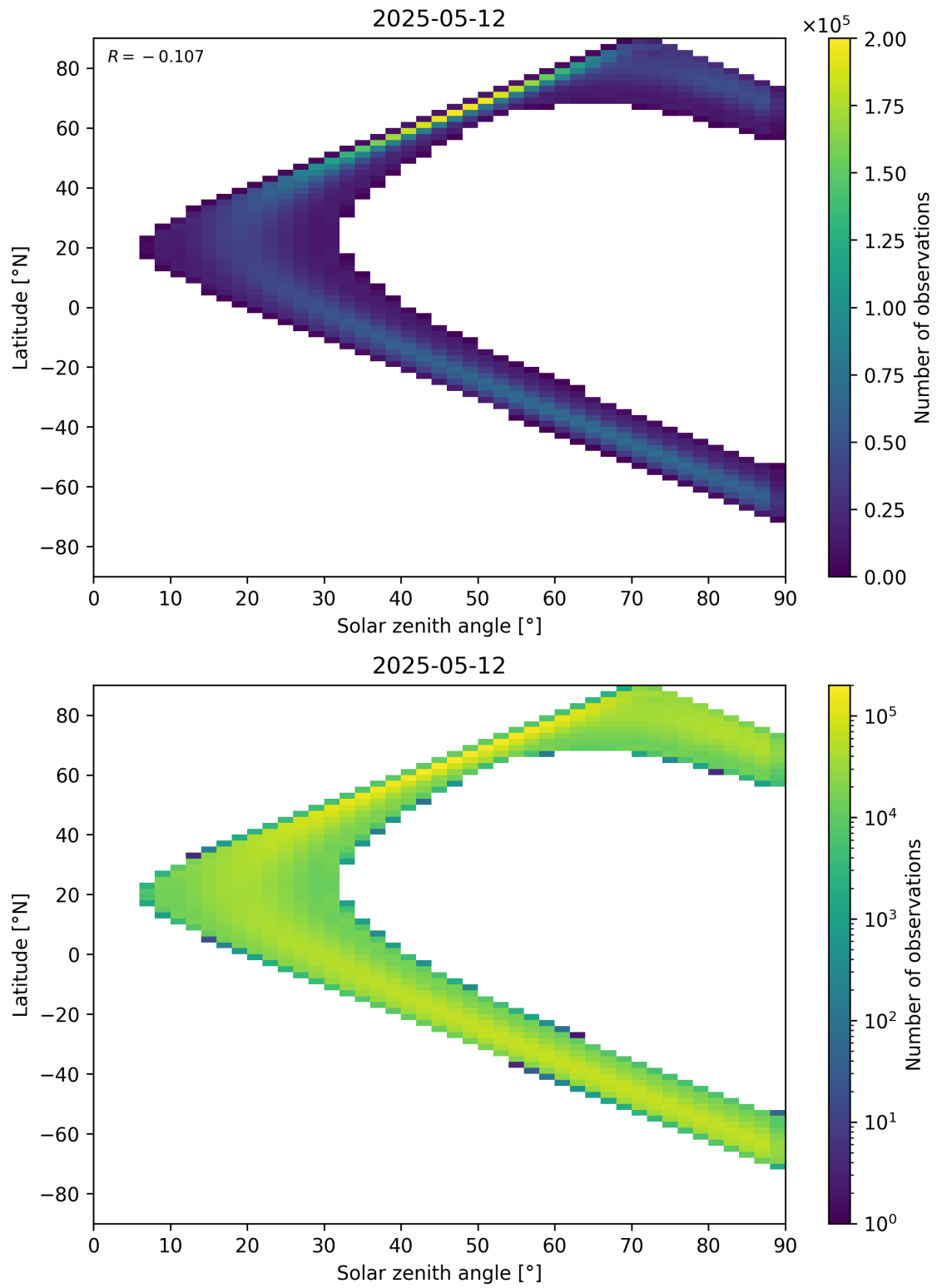
Figure 44: Scatter density plot of “Solar zenith angle” against “Latitude” for 2025-05-11 to 2025-05-13.
