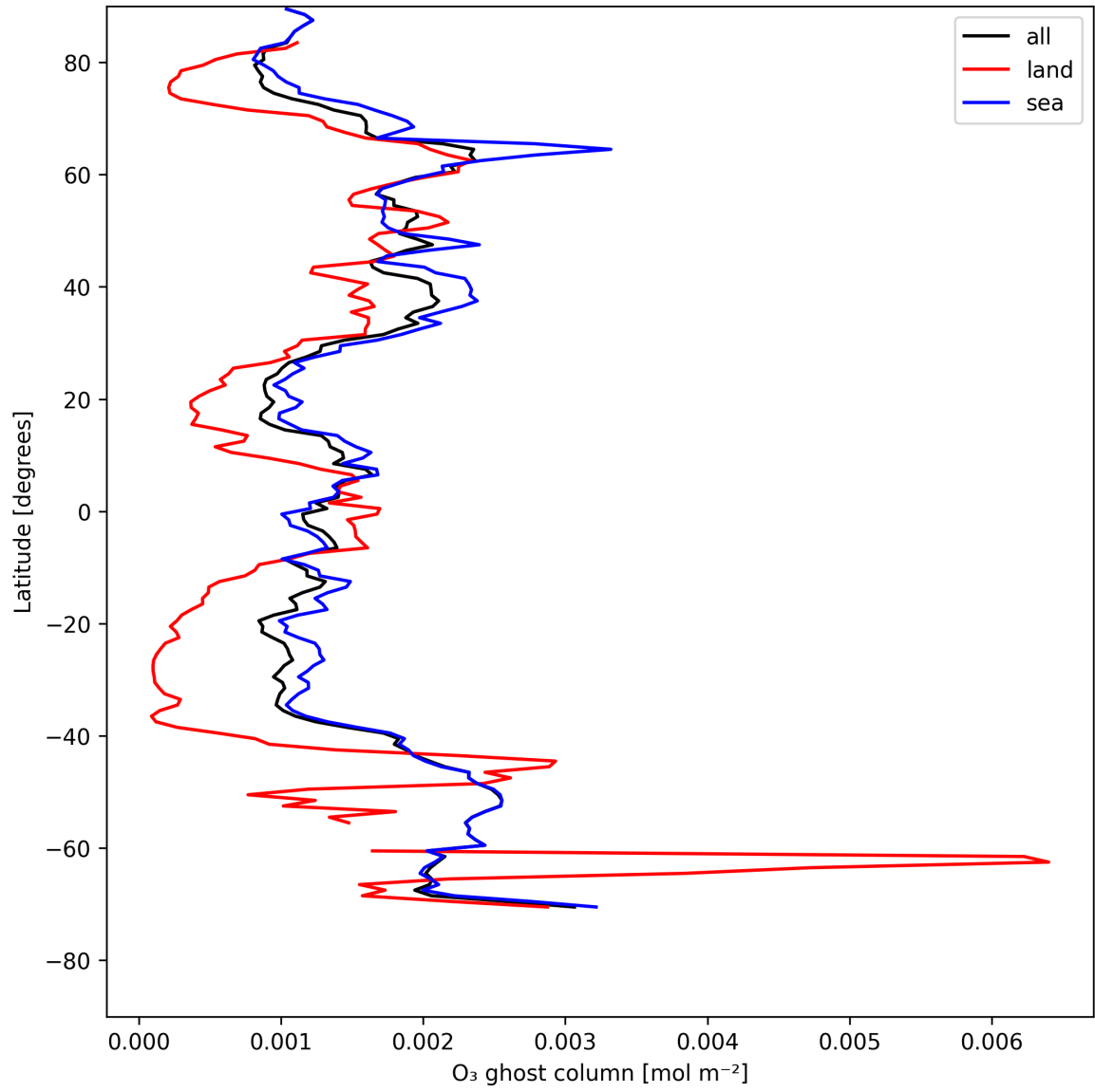
Figure 18: Zonal average of "O 3 ghost column" for 2025-05-11 to 2025-05-13.
