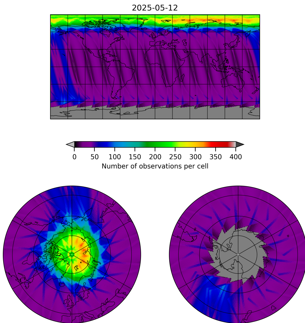
Figure 12: Map of the number of observations for 2025-05-11 to 2025-05-13
