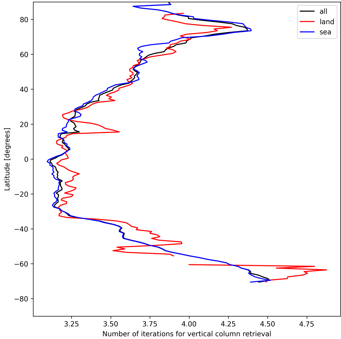
Figure 19: Zonal average of “Number of iterations for vertical column retrieval” for 2025-05-11 to 2025-05-13.
