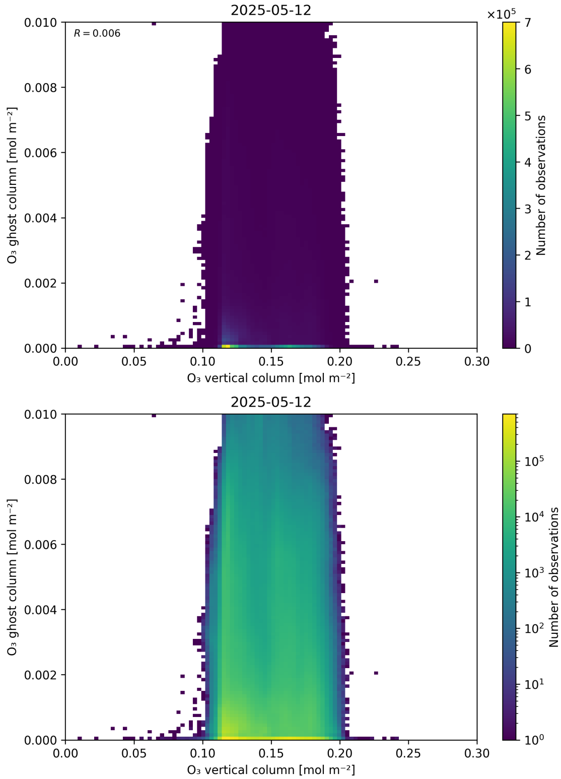
Figure 40: Scatter density plot of “O 3 vertical column” against “O 3 ghost column” for 2025-05-11 to 2025-05-13.
