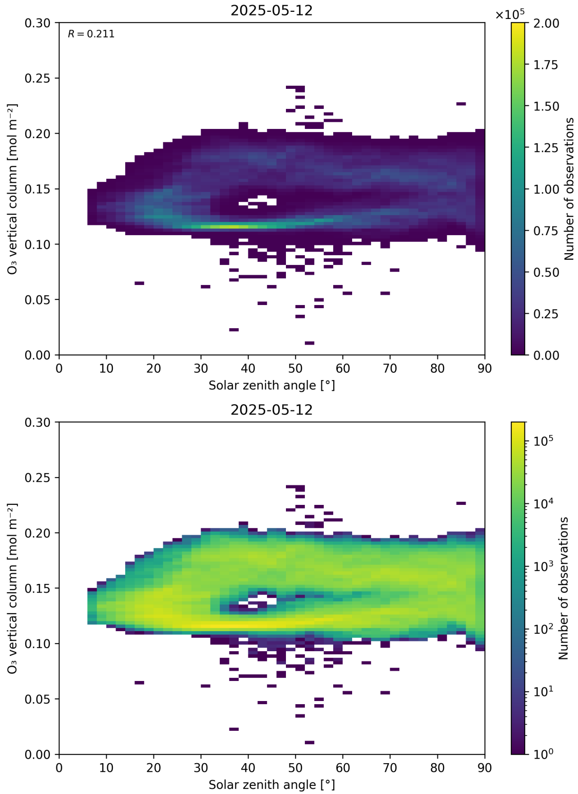
Figure 47: Scatter density plot of “Solar zenith angle” against “O 3 vertical column” for 2025-05-11 to 2025-05-13.
