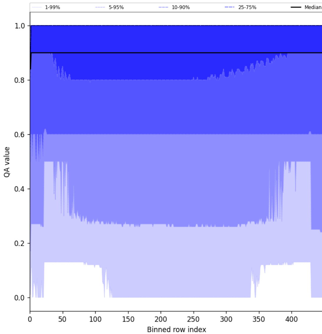
Figure 27: Along track statistics of “QA value” for 2025-05-12 to 2025-05-14
