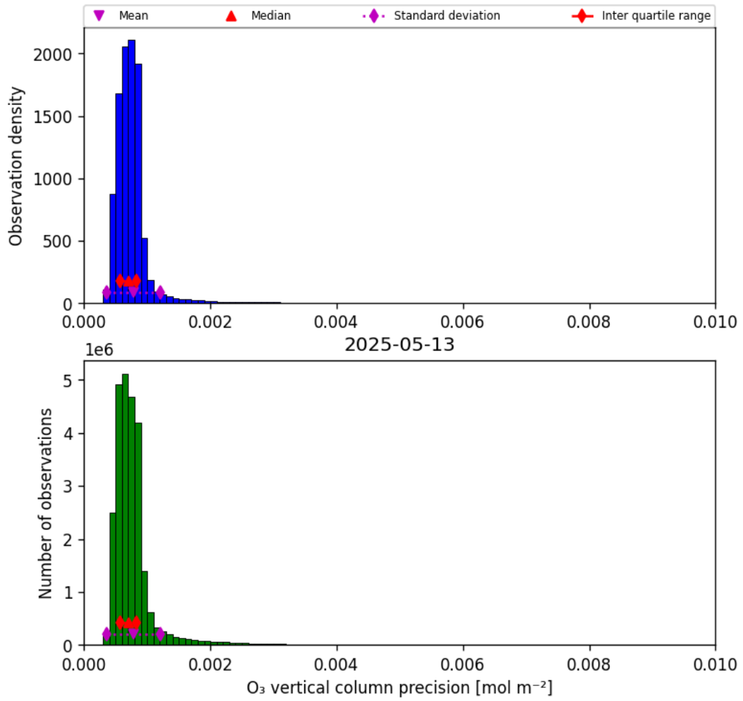
Figure 22: Histogram of “O 3 vertical column precision” for 2025-05-12 to 2025-05-14
