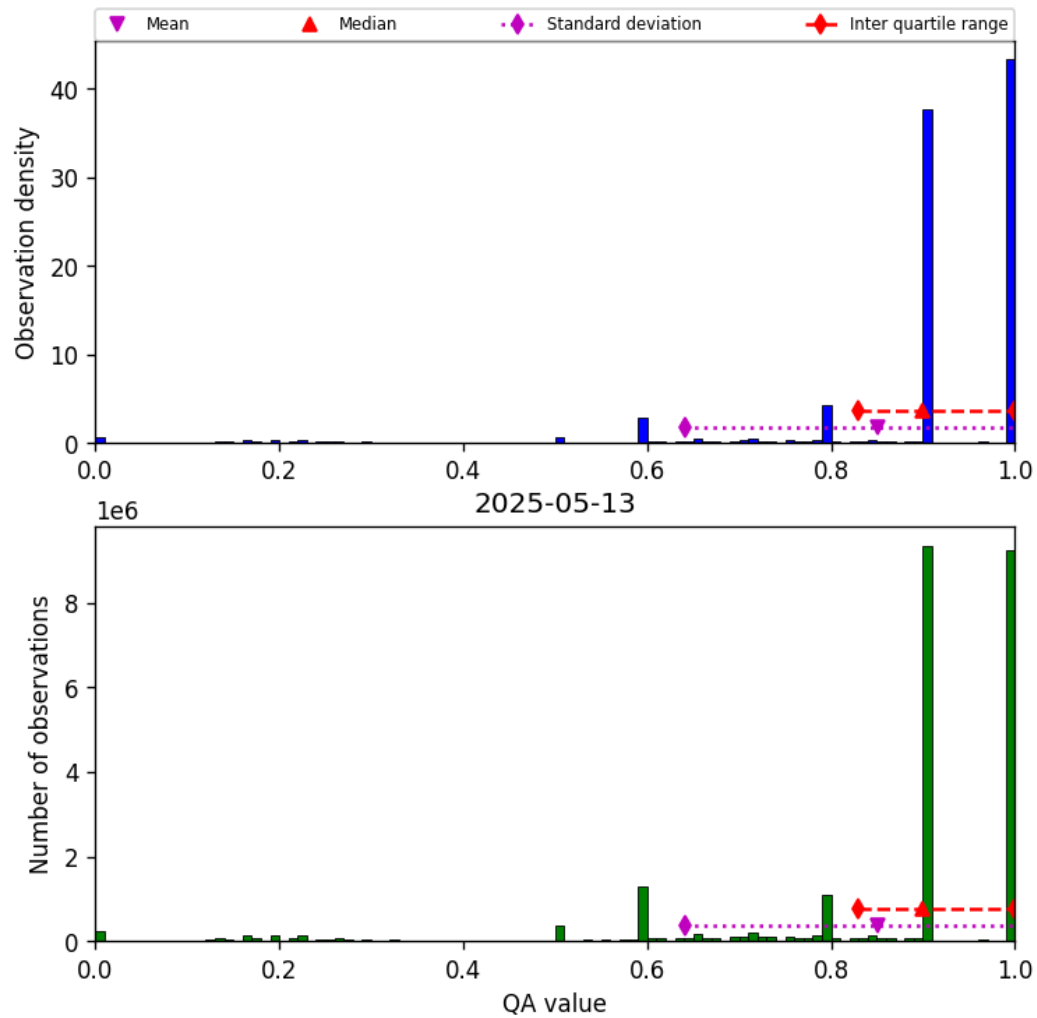
Figure 20: Histogram of “QA value” for 2025-05-12 to 2025-05-14
