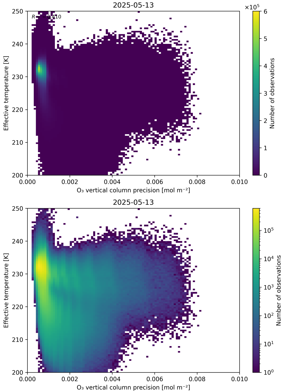
Figure 42: Scatter density plot of “O 3 vertical column precision” against “Effective temperature” for 2025-05-12 to 2025-05-14.
