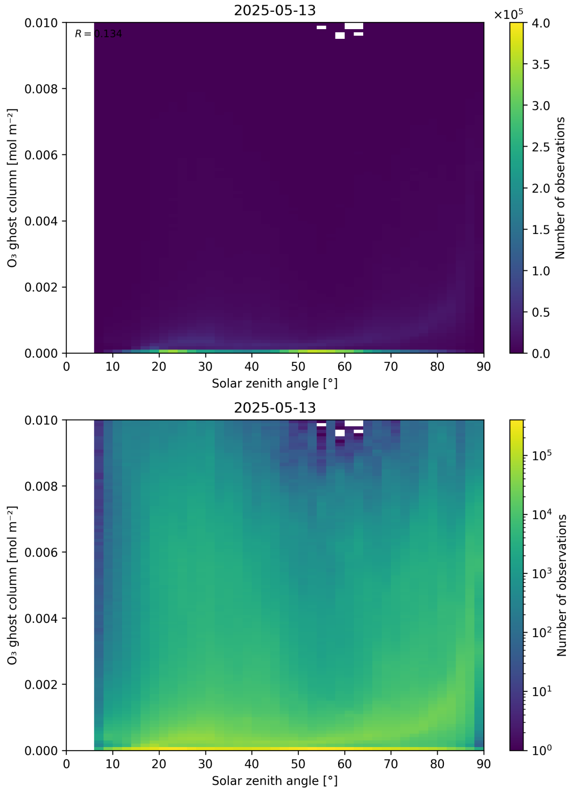
Figure 46: Scatter density plot of “Solar zenith angle” against “O 3 ghost column” for 2025-05-12 to 2025-05-14.
