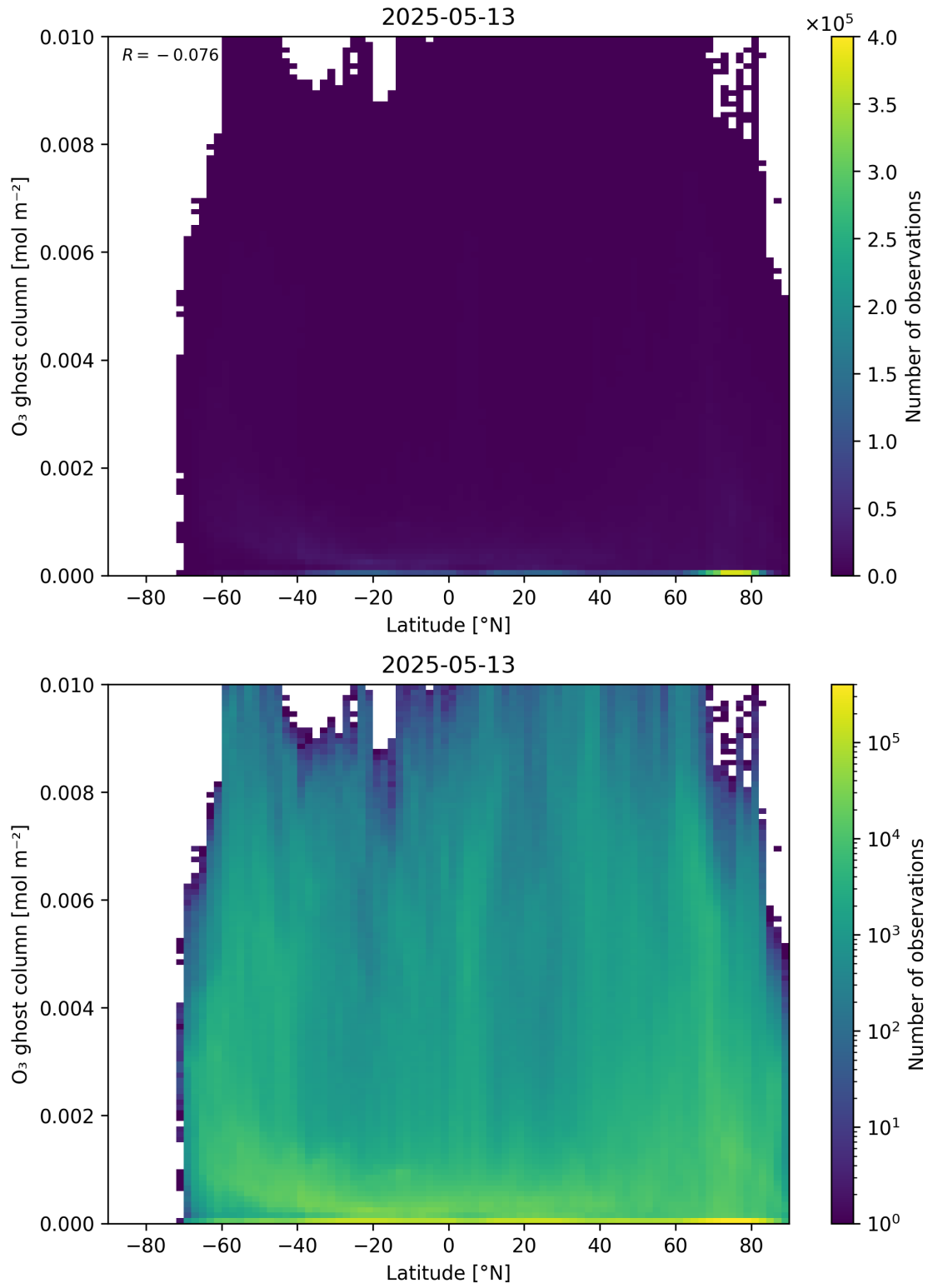
Figure 35: Scatter density plot of “Latitude” against “O 3 ghost column” for 2025-05-12 to 2025-05-14.
