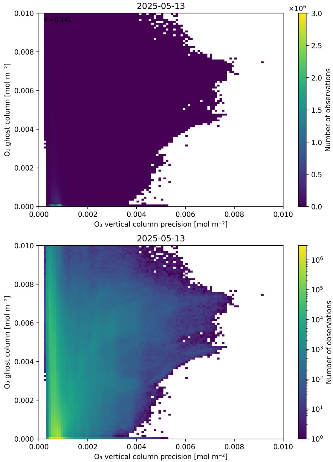
Figure 43: Scatter density plot of “ \text{O}_3 vertical column precision” against “ \text{O}_3 ghost column” for 2025-05-12 to 2025-05-14.
