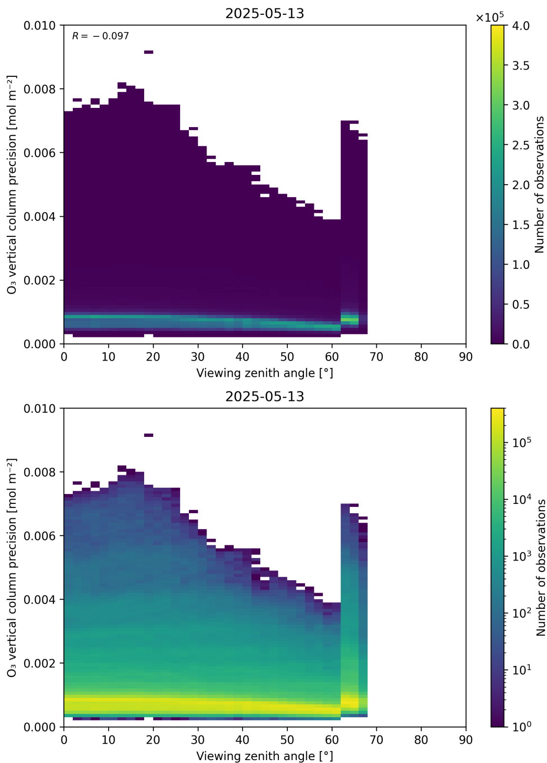
Figure 53: Scatter density plot of “Viewing zenith angle” against “O 3 vertical column precision” for 2025-05-12 to 2025-05-14.
