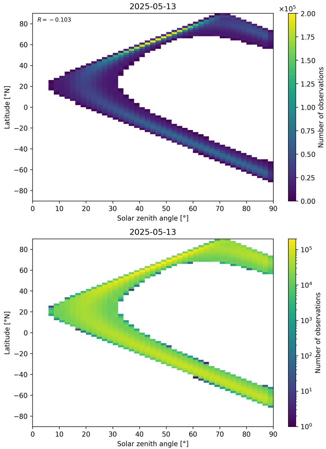
Figure 44: Scatter density plot of “Solar zenith angle” against “Latitude” for 2025-05-12 to 2025-05-14.
