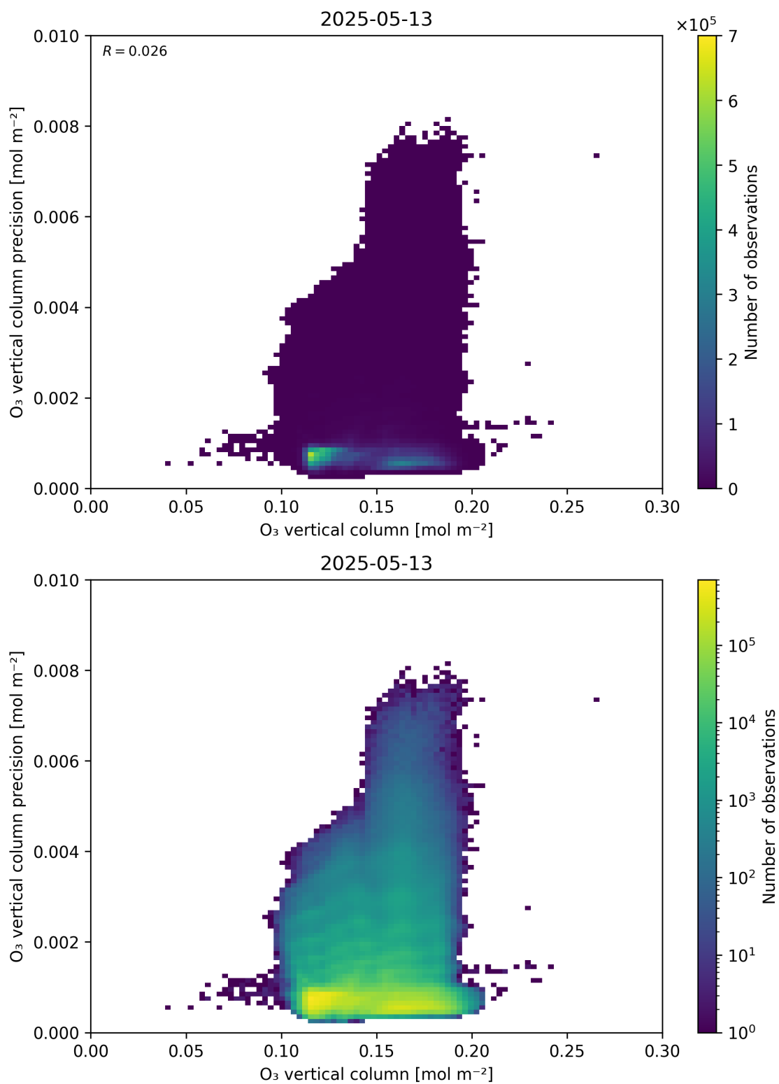
Figure 41: Scatter density plot of “O 3 vertical column” against “O 3 vertical column precision” for 2025-05-12 to 2025-05-14.
