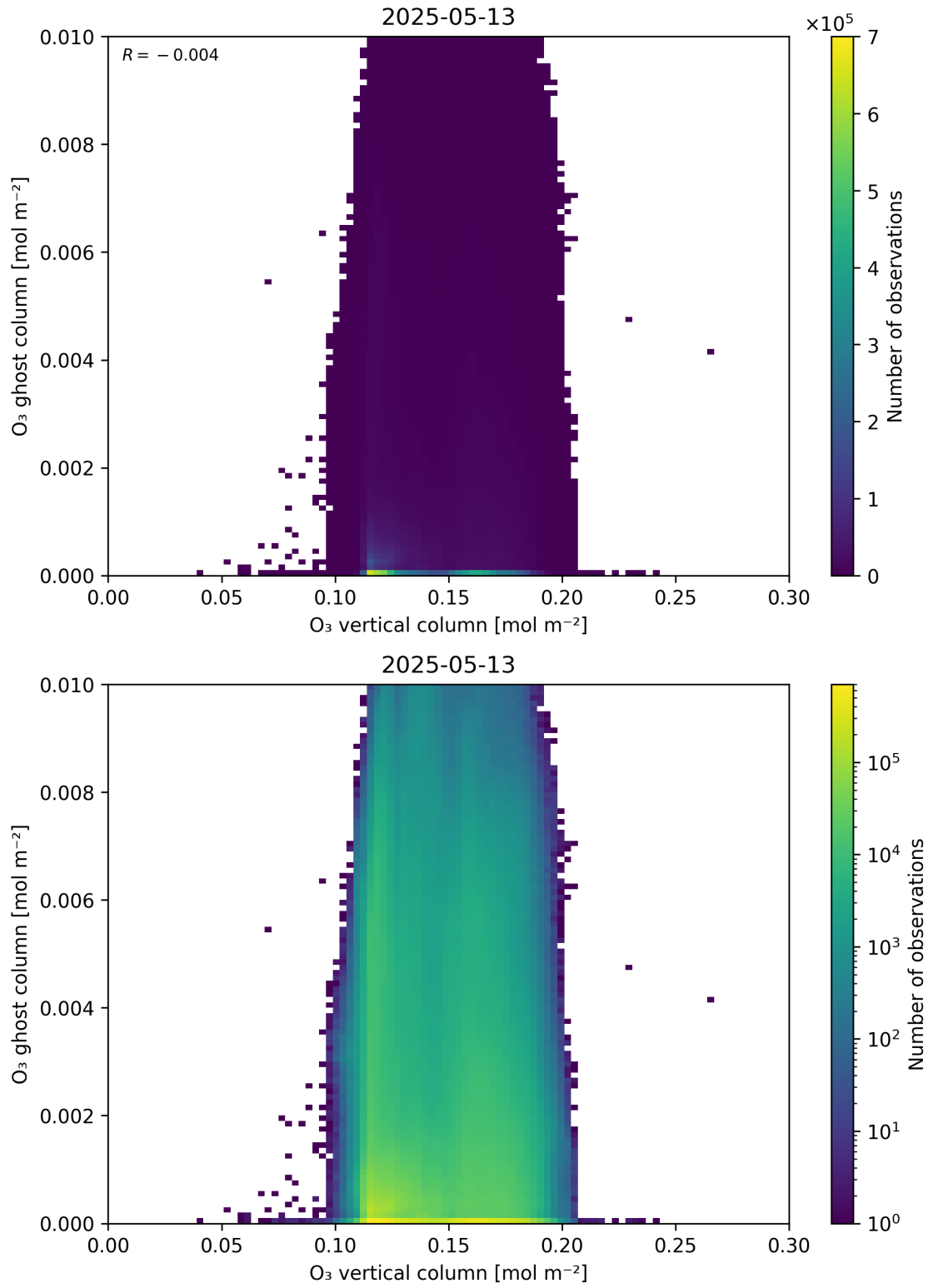
Figure 40: Scatter density plot of “O 3 vertical column” against “O 3 ghost column” for 2025-05-12 to 2025-05-14.
