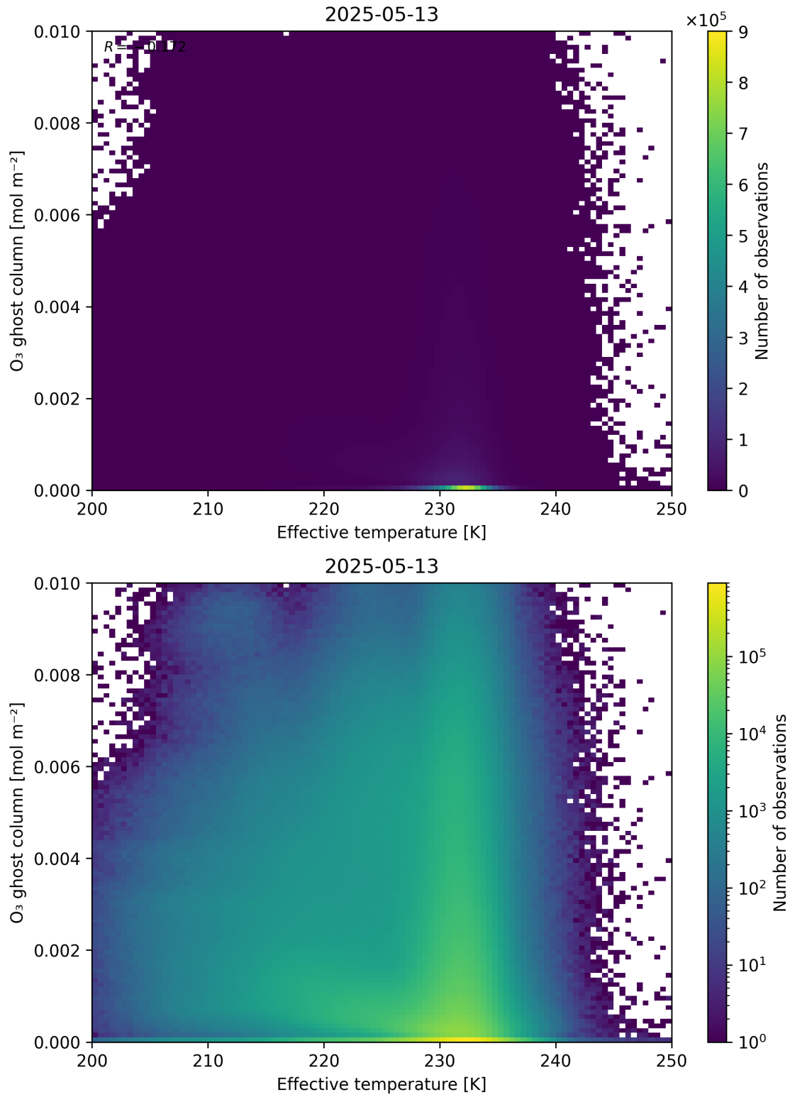
Figure 38: Scatter density plot of “Effective temperature” against “O 3 ghost column” for 2025-05-12 to 2025-05-14.
