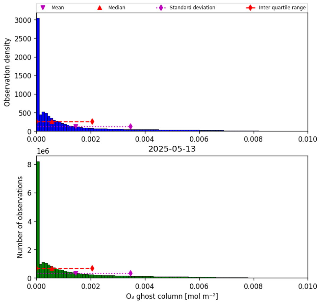
Figure 25: Histogram of “O 3 ghost column” for 2025-05-12 to 2025-05-14
