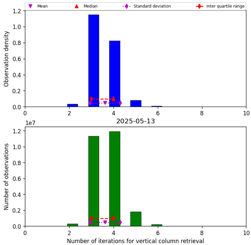
Figure 26: Histogram of “Number of iterations for vertical column retrieval” for 2025-05-12 to 2025-05-14
