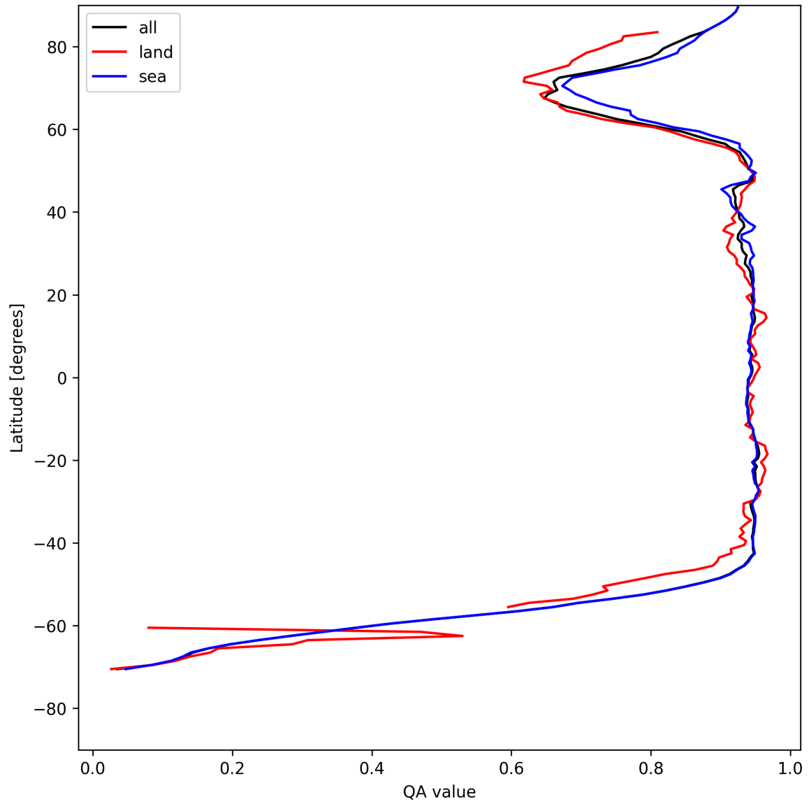
Figure 13: Zonal average of “QA value” for 2025-05-12 to 2025-05-14.
