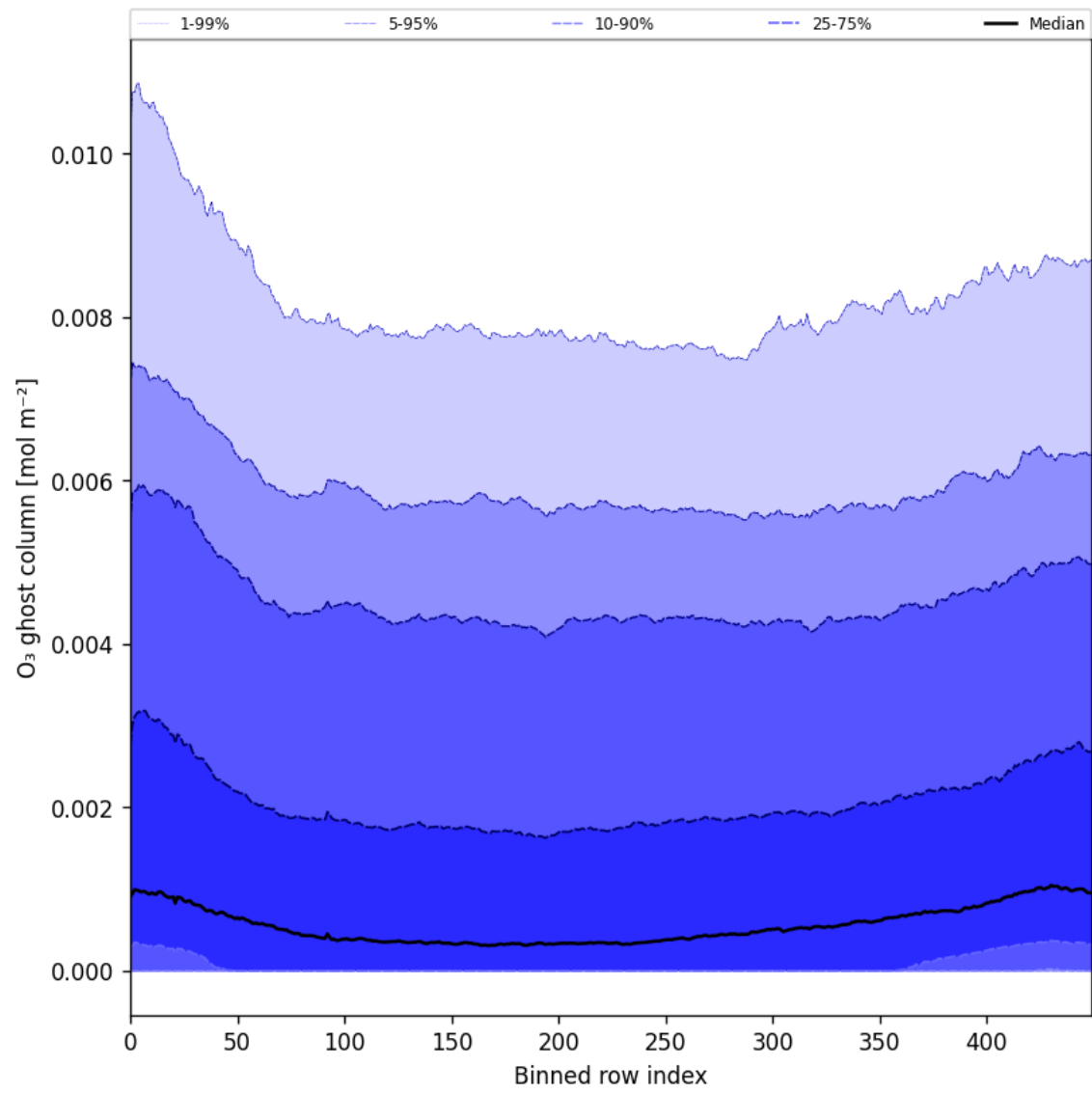
Figure 32: Along track statistics of “O 3 ghost column” for 2025-05-12 to 2025-05-14
