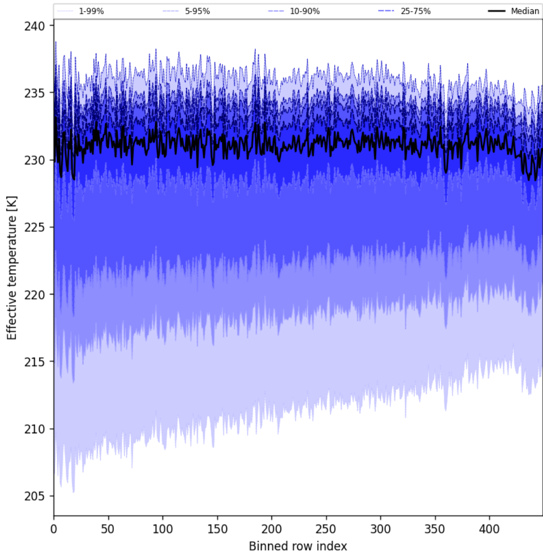
Figure 31: Along track statistics of “Effective temperature” for 2025-05-12 to 2025-05-14
