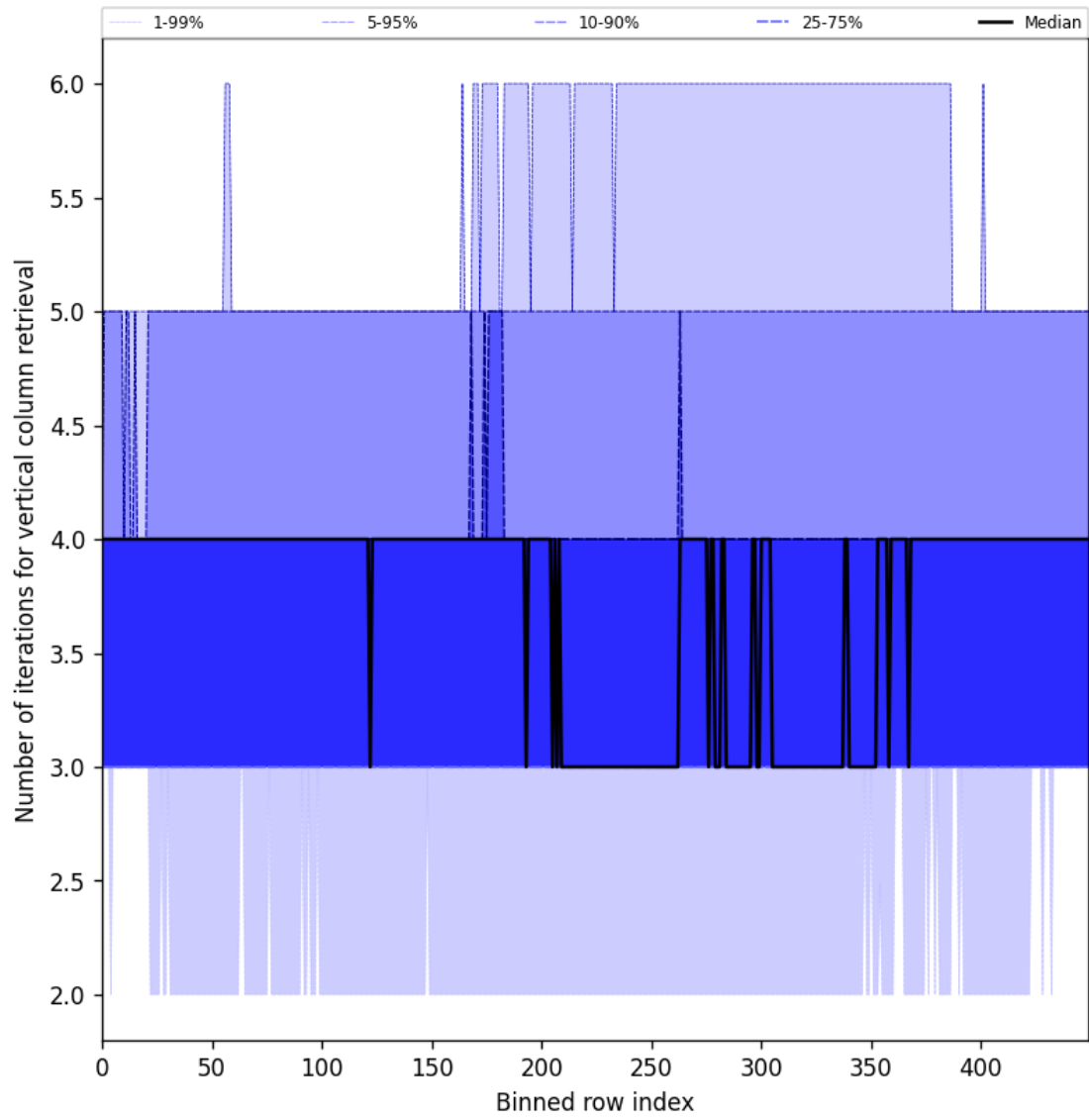
Figure 33: Along track statistics of “Number of iterations for vertical column retrieval” for 2025-05-12 to 2025-05-14
