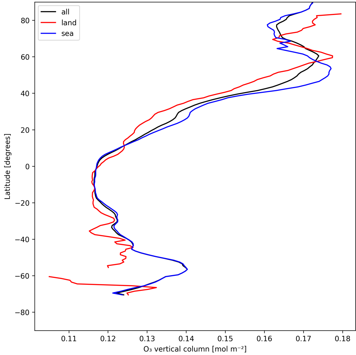
Figure 14: Zonal average of “O 3 vertical column” for 2025-05-12 to 2025-05-14.
