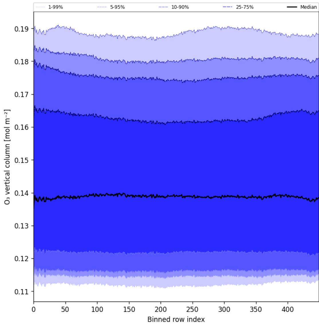
Figure 28: Along track statistics of “O 3 vertical column” for 2025-05-12 to 2025-05-14
