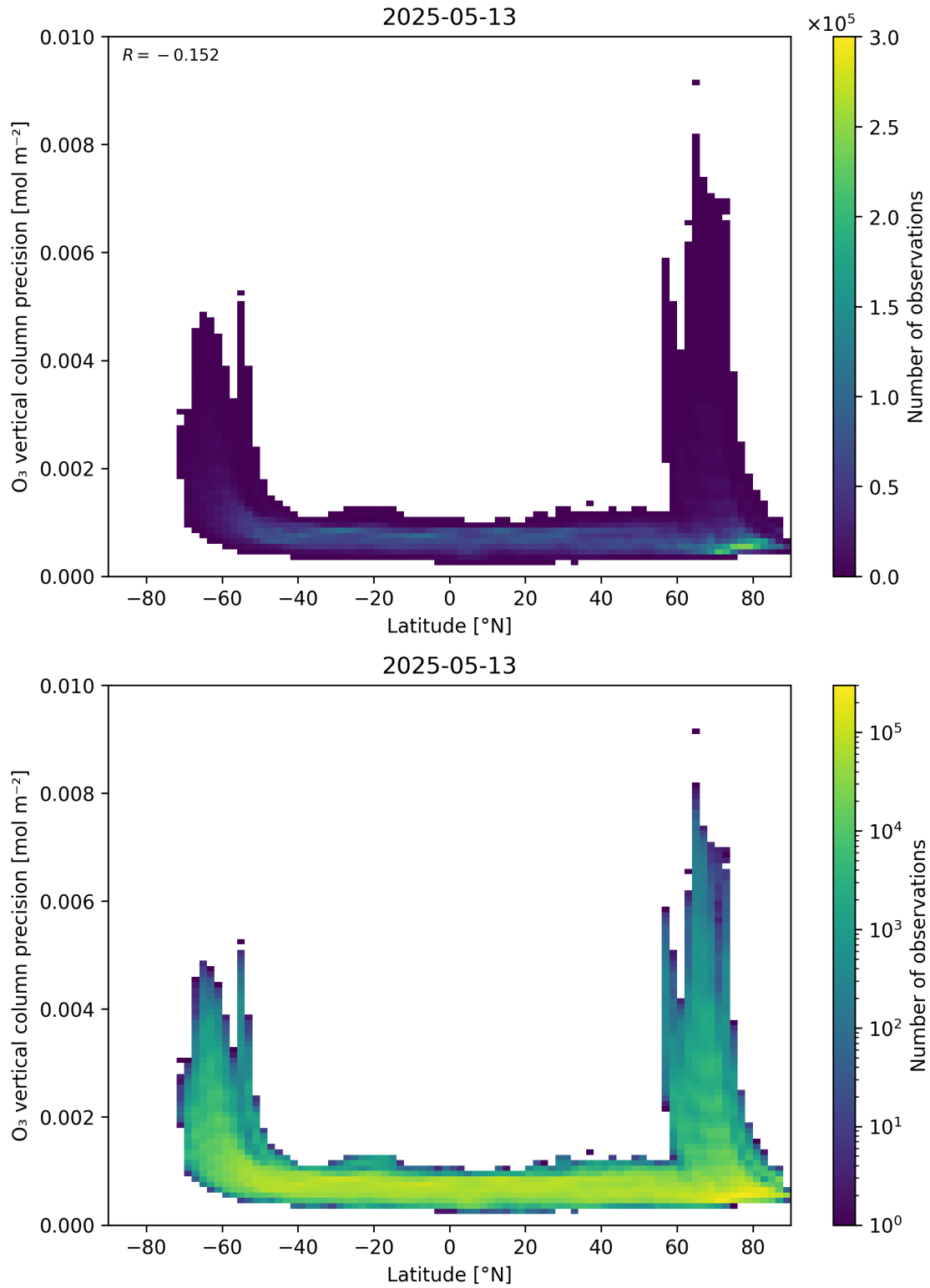
Figure 37: Scatter density plot of “Latitude” against “O 3 vertical column precision” for 2025-05-12 to 2025-05-14.
