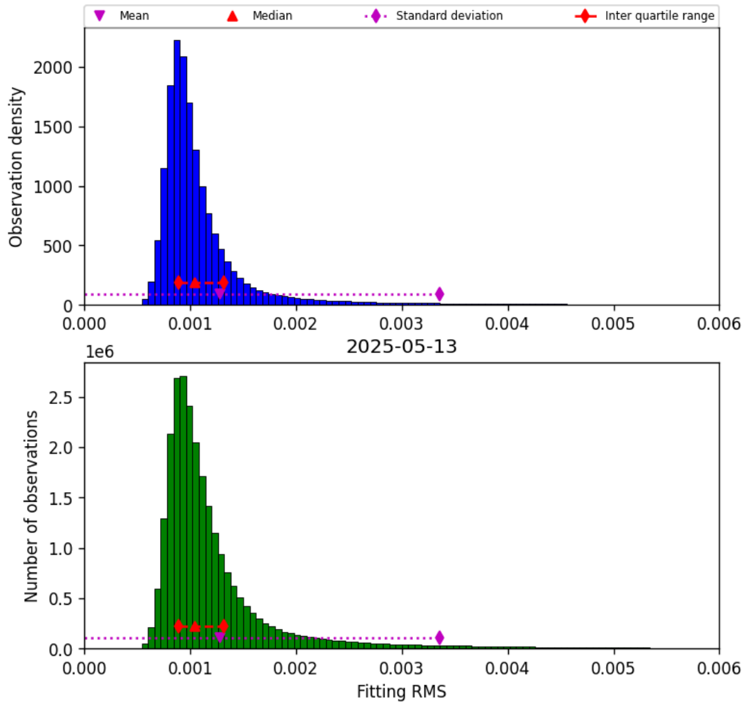
Figure 23: Histogram of “Fitting RMS” for 2025-05-12 to 2025-05-14
