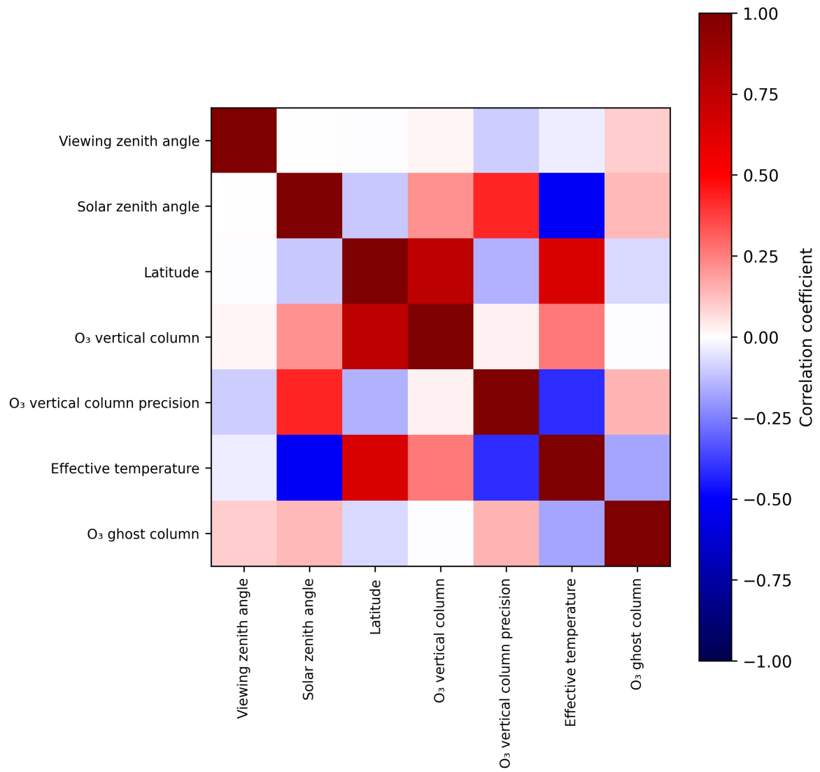
Figure 2: Map of correlation matrix for 2025-05-12 to 2025-05-14.
