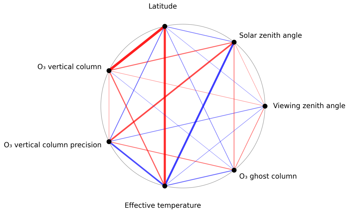
Figure 1: Map of correlation graph for 2025-05-12 to 2025-05-14.
