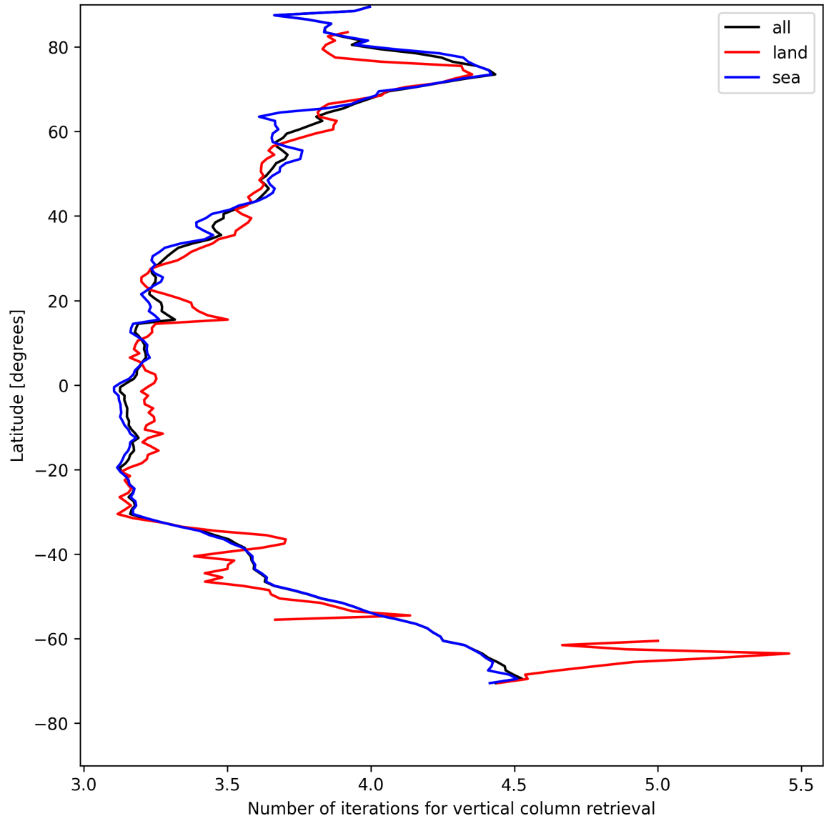
Figure 19: Zonal average of “Number of iterations for vertical column retrieval” for 2025-05-12 to 2025-05-14.
