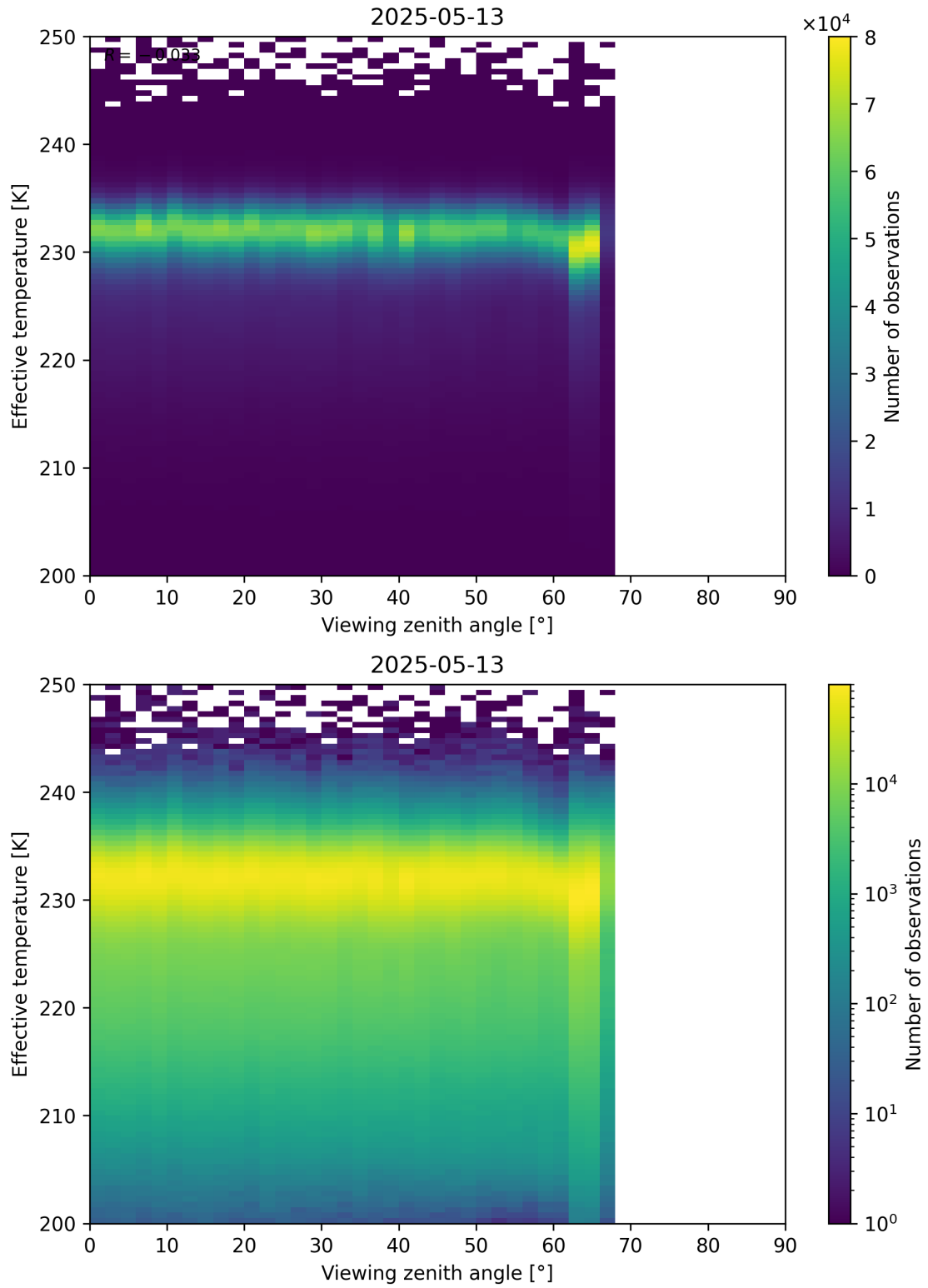
Figure 50: Scatter density plot of “Viewing zenith angle” against “Effective temperature” for 2025-05-12 to 2025-05-14.
