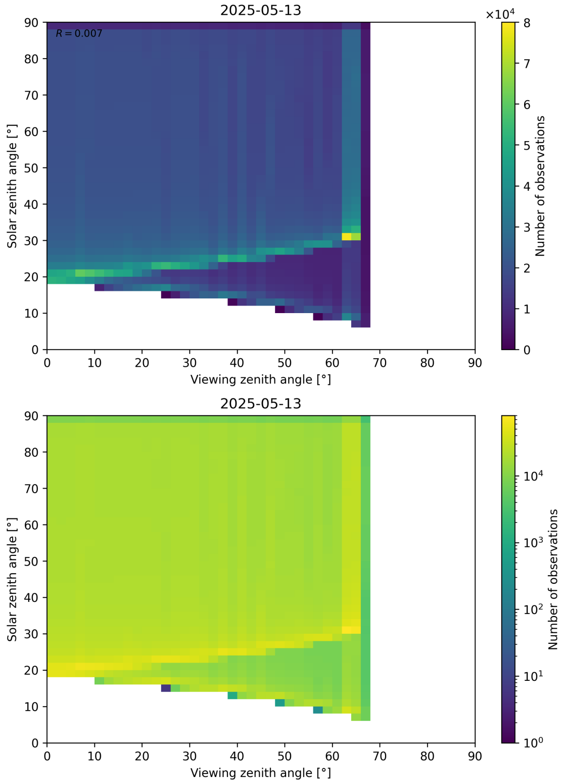
Figure 54: Scatter density plot of “Viewing zenith angle” against “Solar zenith angle” for 2025-05-12 to 2025-05-14.
