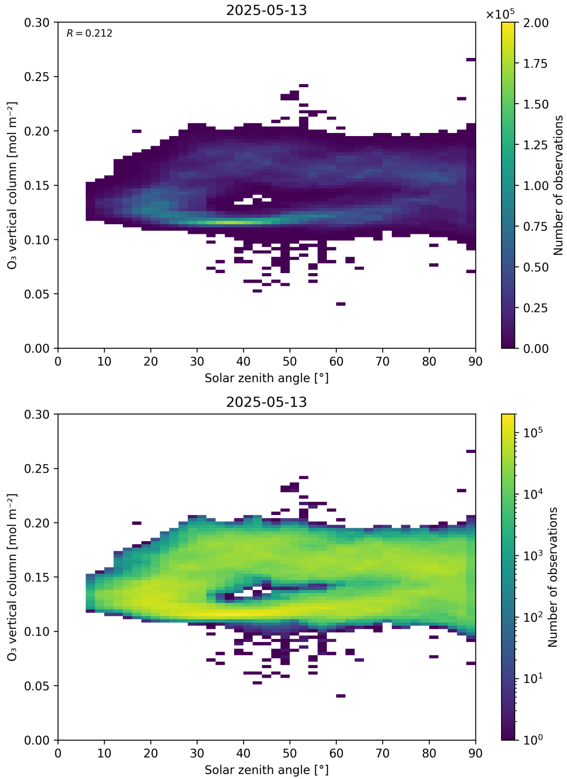
Figure 47: Scatter density plot of “Solar zenith angle” against “O 3 vertical column” for 2025-05-12 to 2025-05-14.
