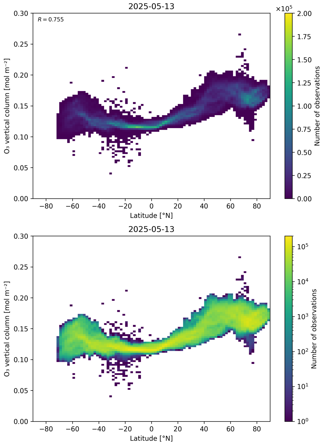
Figure 36: Scatter density plot of “Latitude” against “O 3 vertical column” for 2025-05-12 to 2025-05-14.
