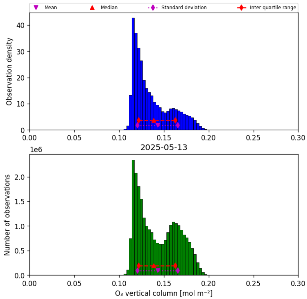
Figure 21: Histogram of “O 3 vertical column” for 2025-05-12 to 2025-05-14
