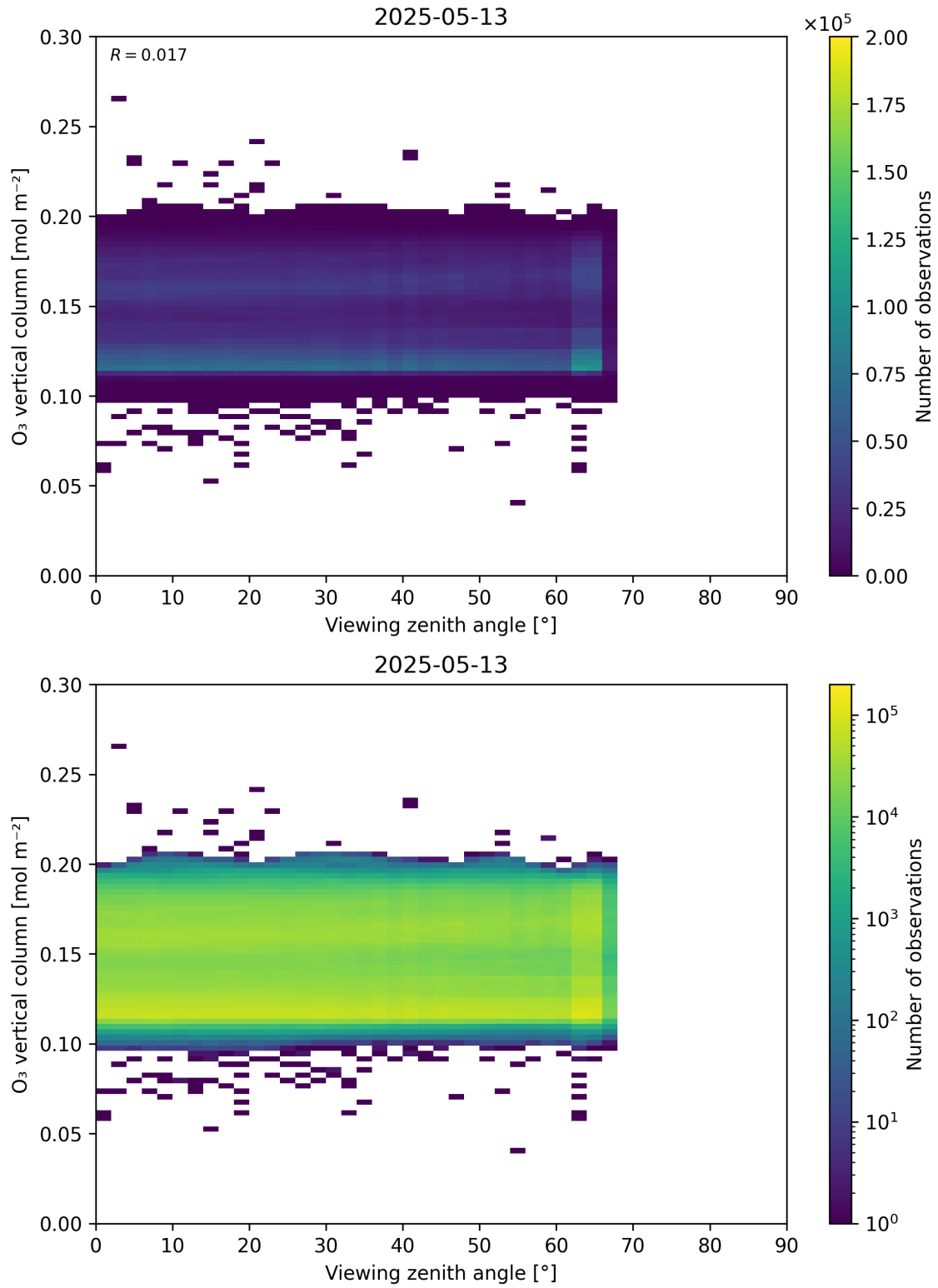
Figure 52: Scatter density plot of “Viewing zenith angle” against “O 3 vertical column” for 2025-05-12 to 2025-05-14.
