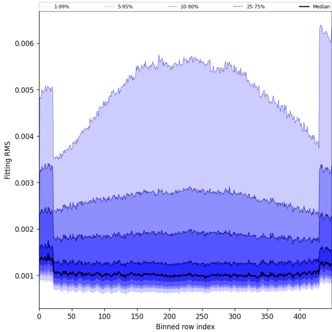
Figure 30: Along track statistics of “Fitting RMS” for 2025-05-12 to 2025-05-14
