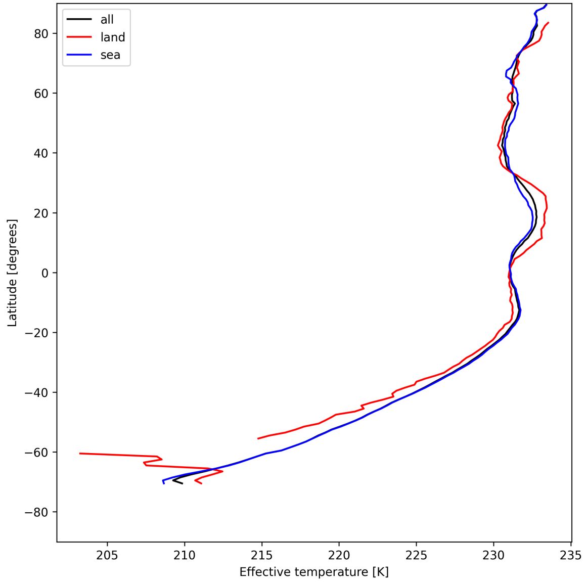
Figure 17: Zonal average of "Effective temperature" for 2025-05-12 to 2025-05-14.
