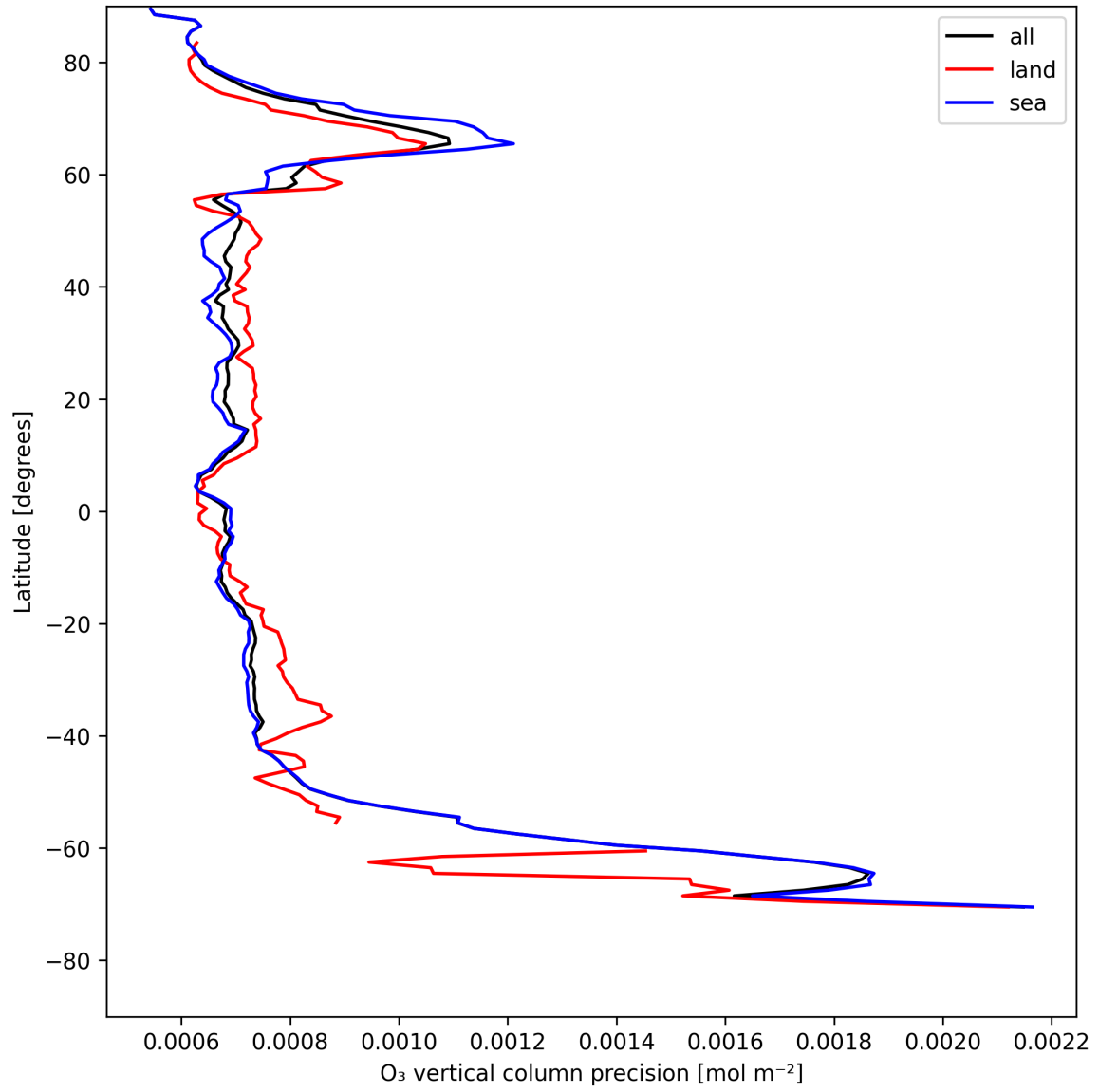
Figure 15: Zonal average of “O 3 vertical column precision” for 2025-05-12 to 2025-05-14.
