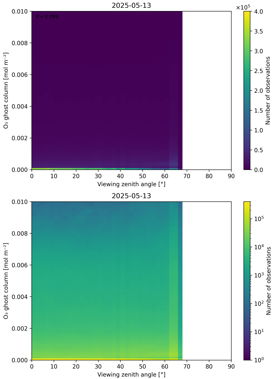
Figure 51: Scatter density plot of “Viewing zenith angle” against “O 3 ghost column” for 2025-05-12 to 2025-05-14.
