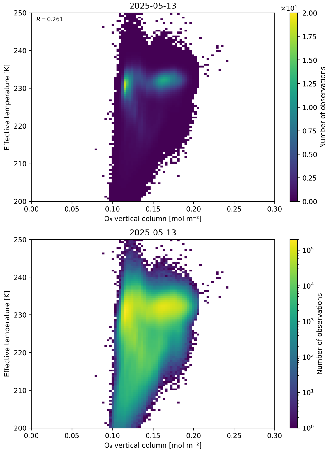
Figure 39: Scatter density plot of “O 3 vertical column” against “Effective temperature” for 2025-05-12 to 2025-05-14.
