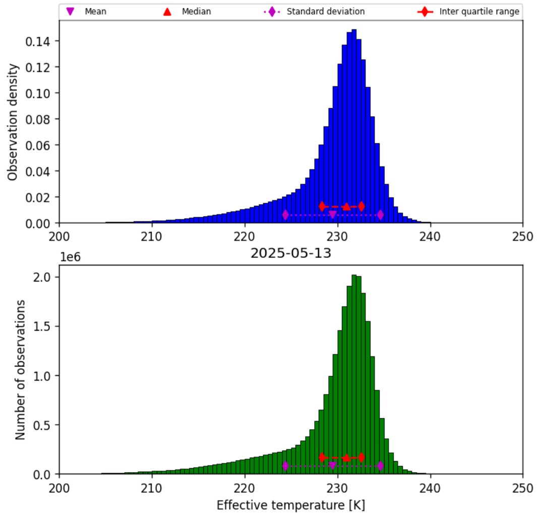
Figure 24: Histogram of “Effective temperature” for 2025-05-12 to 2025-05-14
