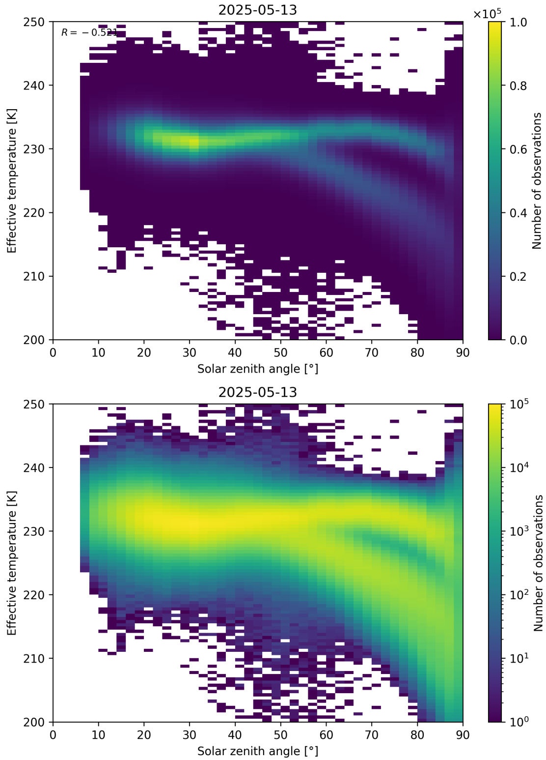
Figure 45: Scatter density plot of “Solar zenith angle” against “Effective temperature” for 2025-05-12 to 2025-05-14.
