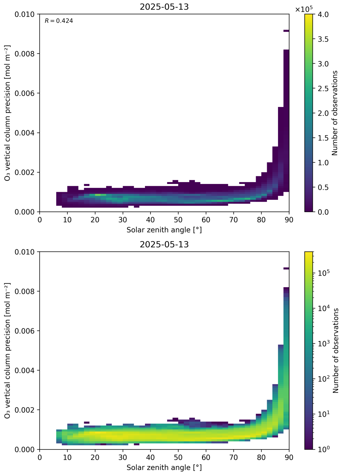
Figure 48: Scatter density plot of “Solar zenith angle” against “O 3 vertical column precision” for 2025-05-12 to 2025-05-14.
