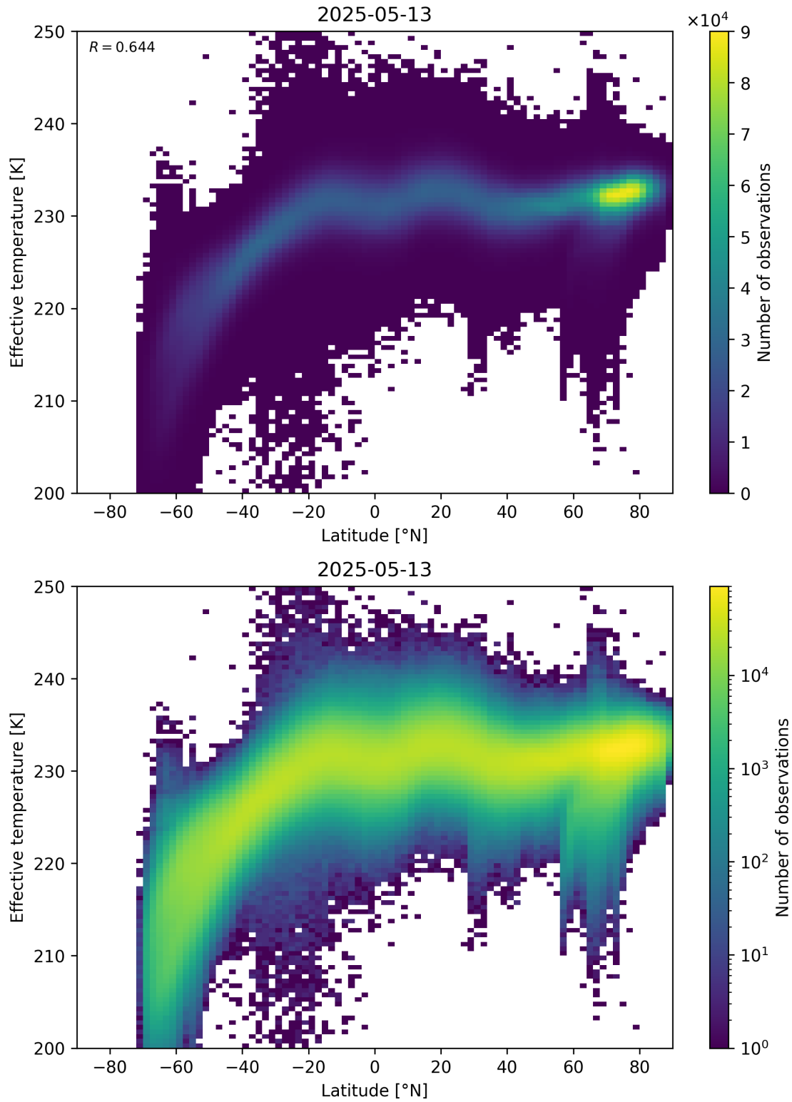
Figure 34: Scatter density plot of “Latitude” against “Effective temperature” for 2025-05-12 to 2025-05-14.
