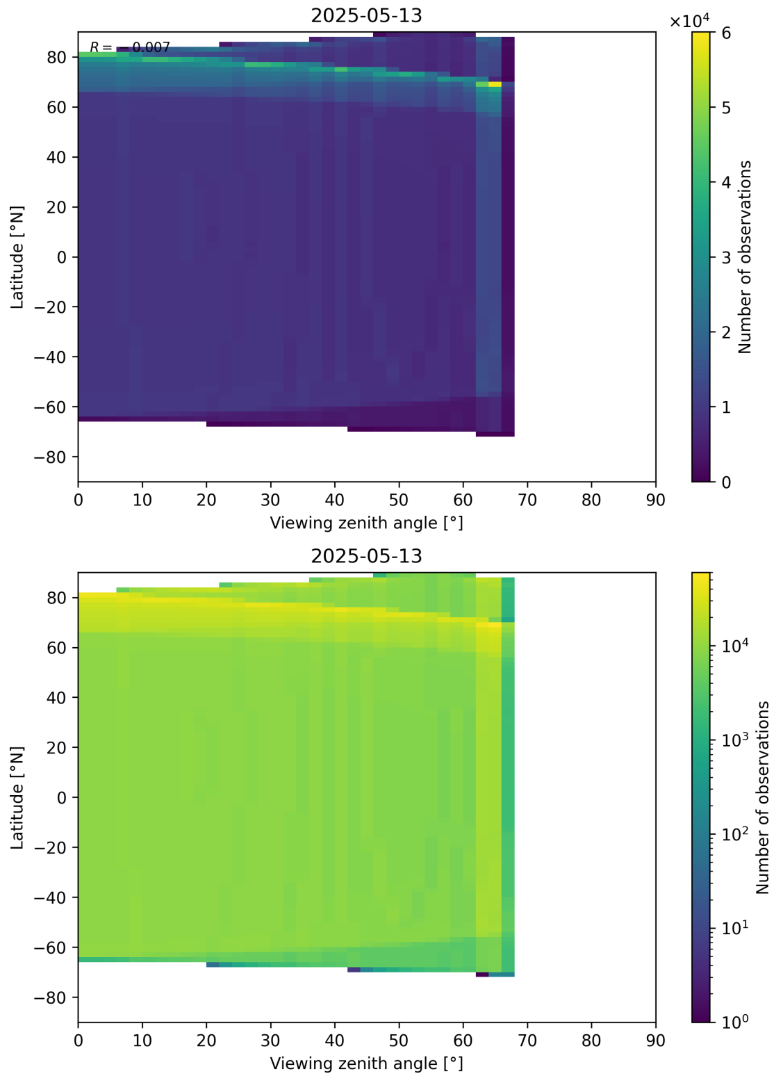
Figure 49: Scatter density plot of “Viewing zenith angle” against “Latitude” for 2025-05-12 to 2025-05-14.
