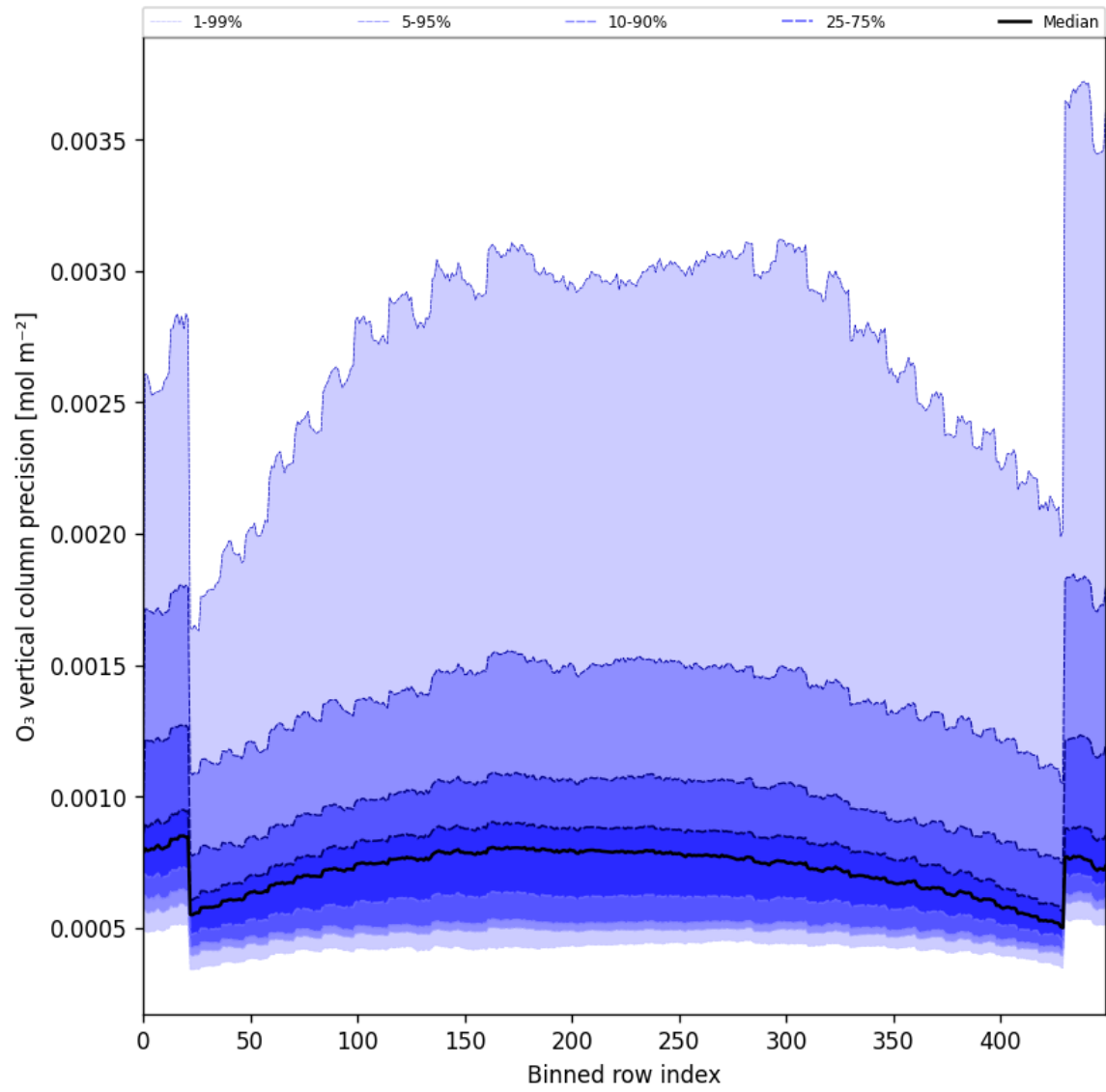
Figure 29: Along track statistics of “O 3 vertical column precision” for 2025-05-12 to 2025-05-14
