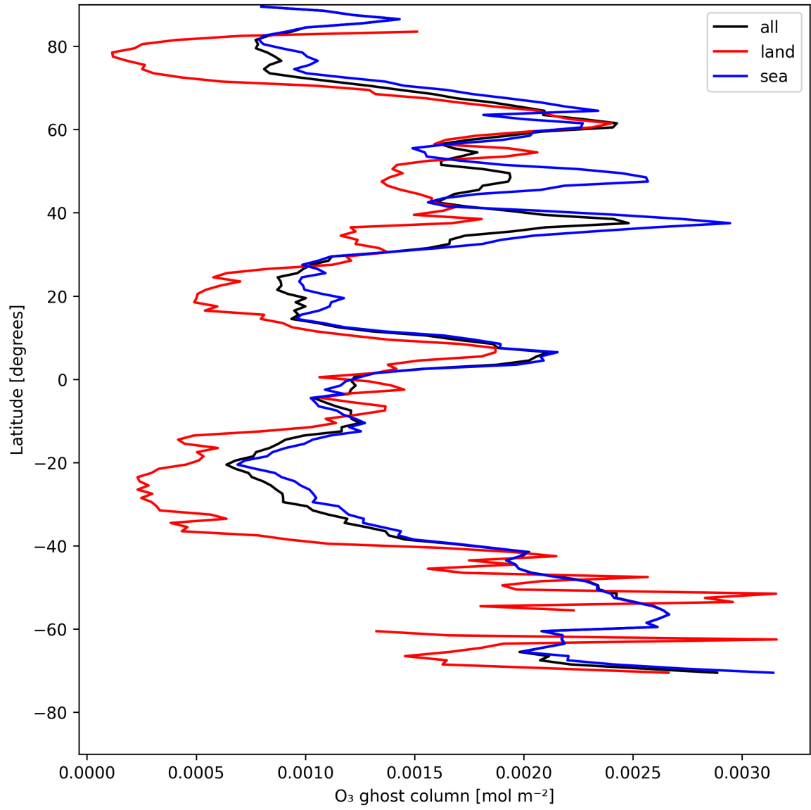
Figure 18: Zonal average of “O 3 ghost column” for 2025-05-12 to 2025-05-14.
