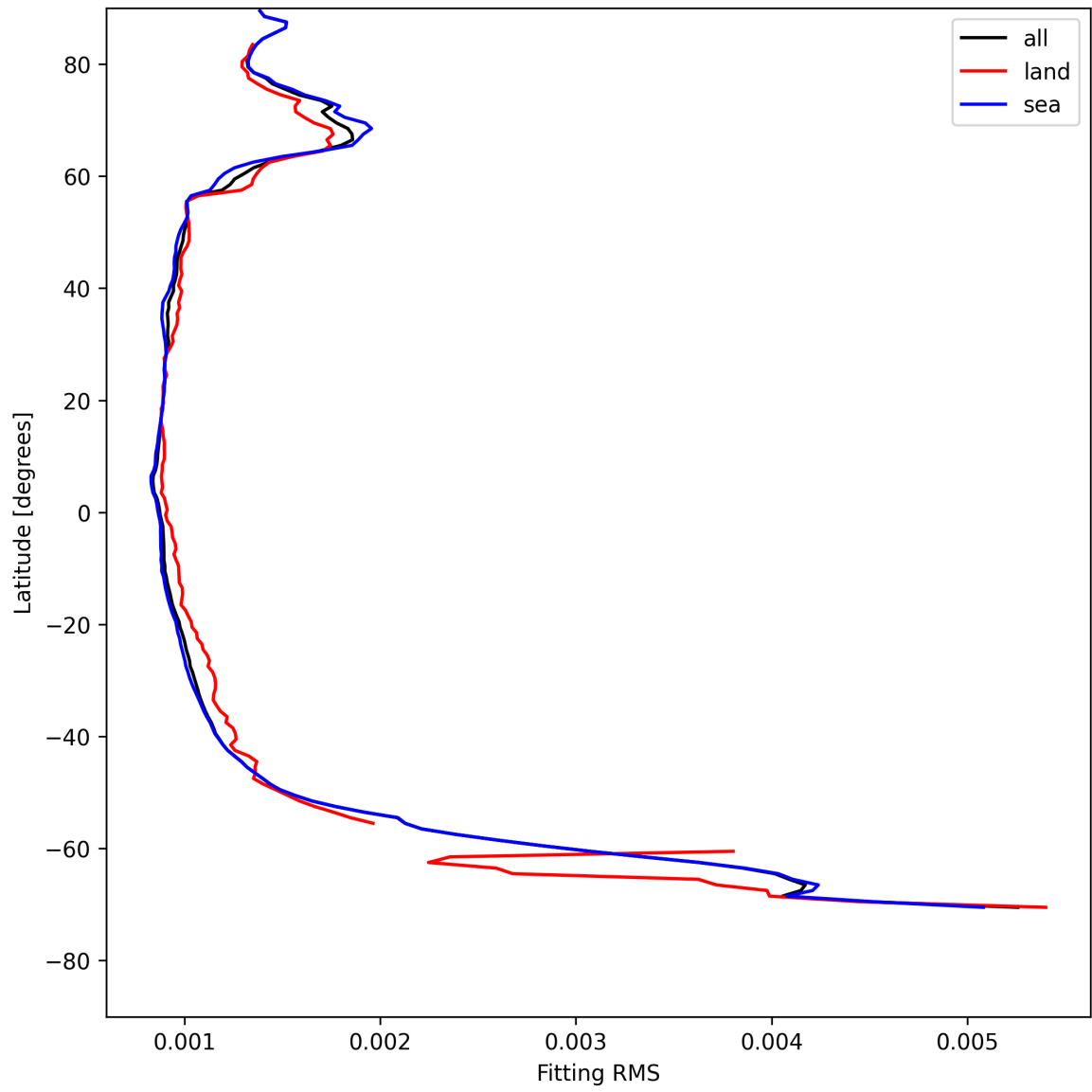
Figure 16: Zonal average of “Fitting RMS” for 2025-05-12 to 2025-05-14.
