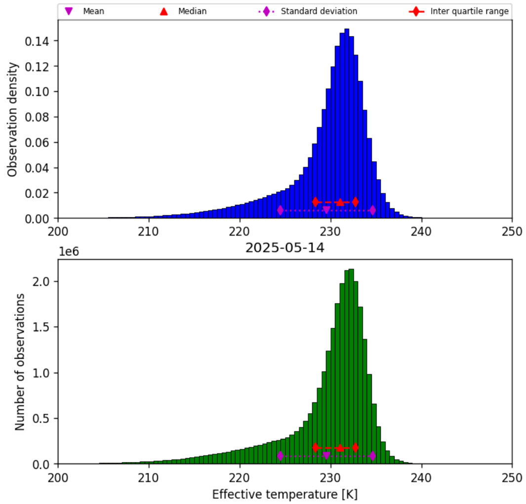
Figure 24: Histogram of “Effective temperature” for 2025-05-13 to 2025-05-15
