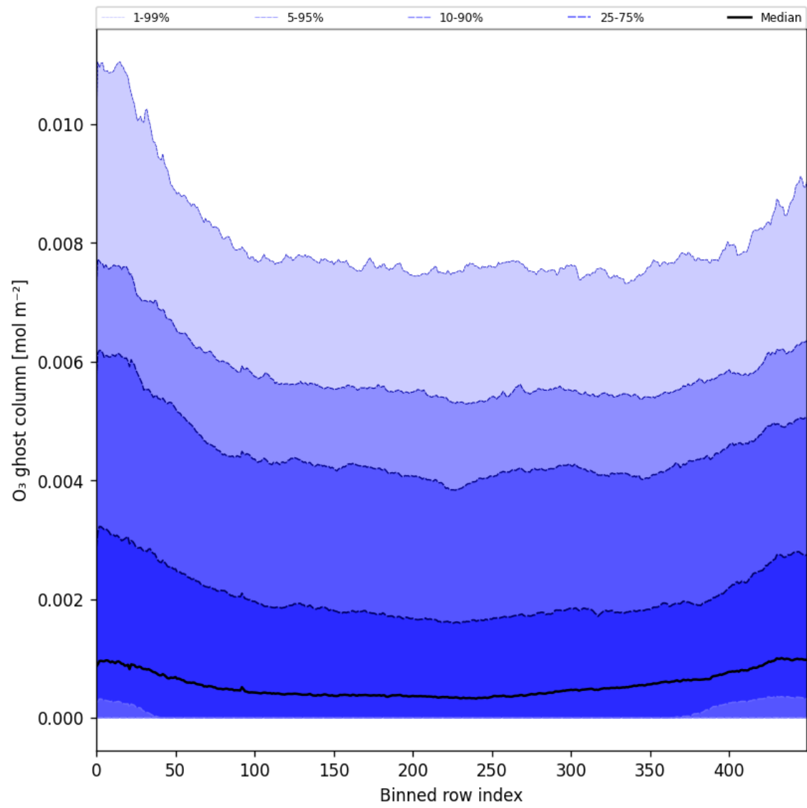
Figure 32: Along track statistics of “O 3 ghost column” for 2025-05-13 to 2025-05-15
