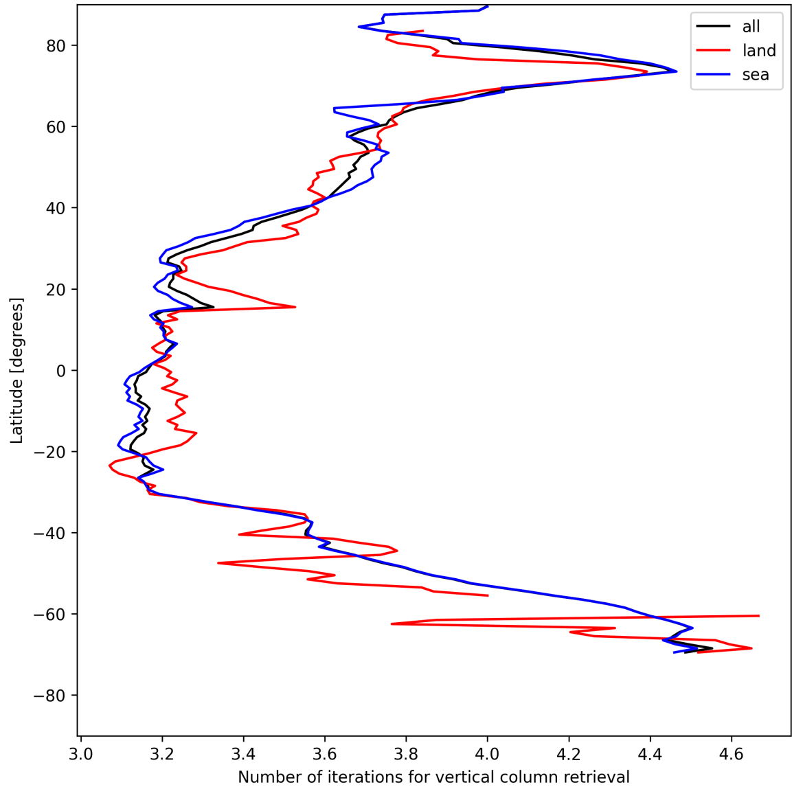
Figure 19: Zonal average of “Number of iterations for vertical column retrieval” for 2025-05-13 to 2025-05-15.
