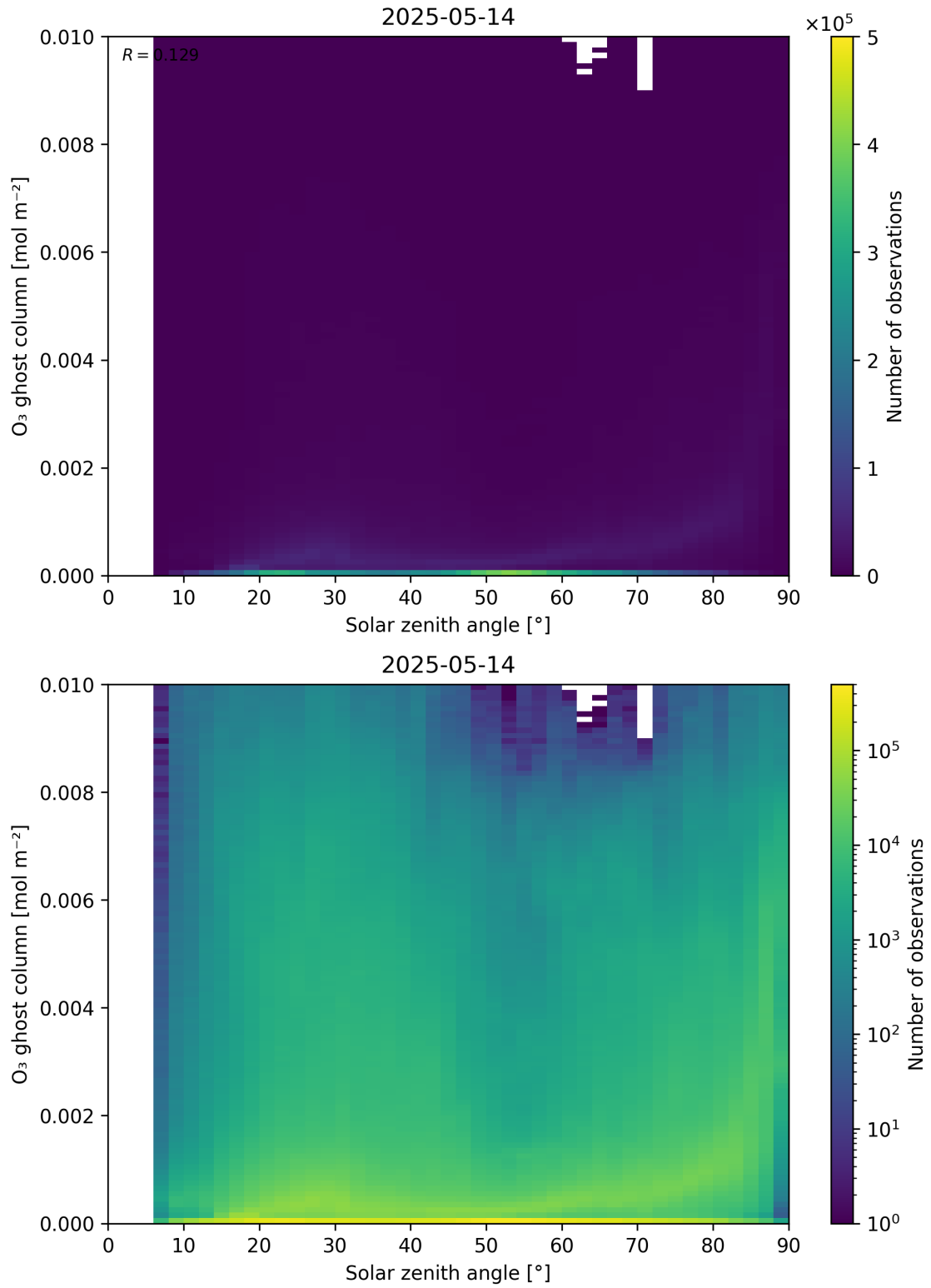
Figure 46: Scatter density plot of “Solar zenith angle” against “O 3 ghost column” for 2025-05-13 to 2025-05-15.
