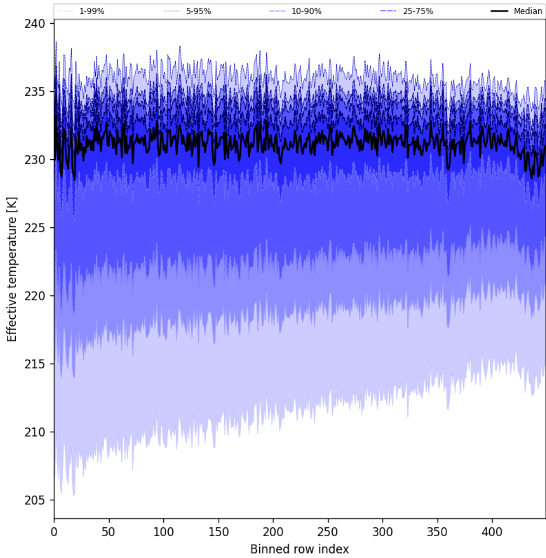
Figure 31: Along track statistics of “Effective temperature” for 2025-05-13 to 2025-05-15
