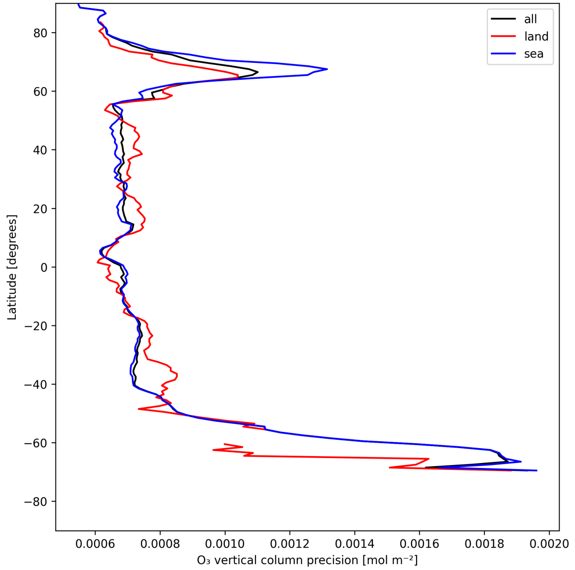
Figure 15: Zonal average of “O 3 vertical column precision” for 2025-05-13 to 2025-05-15.
