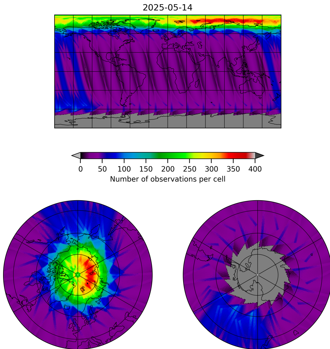
Figure 12: Map of the number of observations for 2025-05-13 to 2025-05-15
