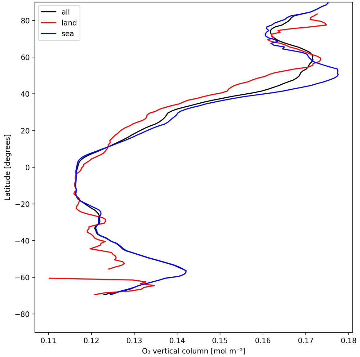
Figure 14: Zonal average of “O 3 vertical column” for 2025-05-13 to 2025-05-15.
