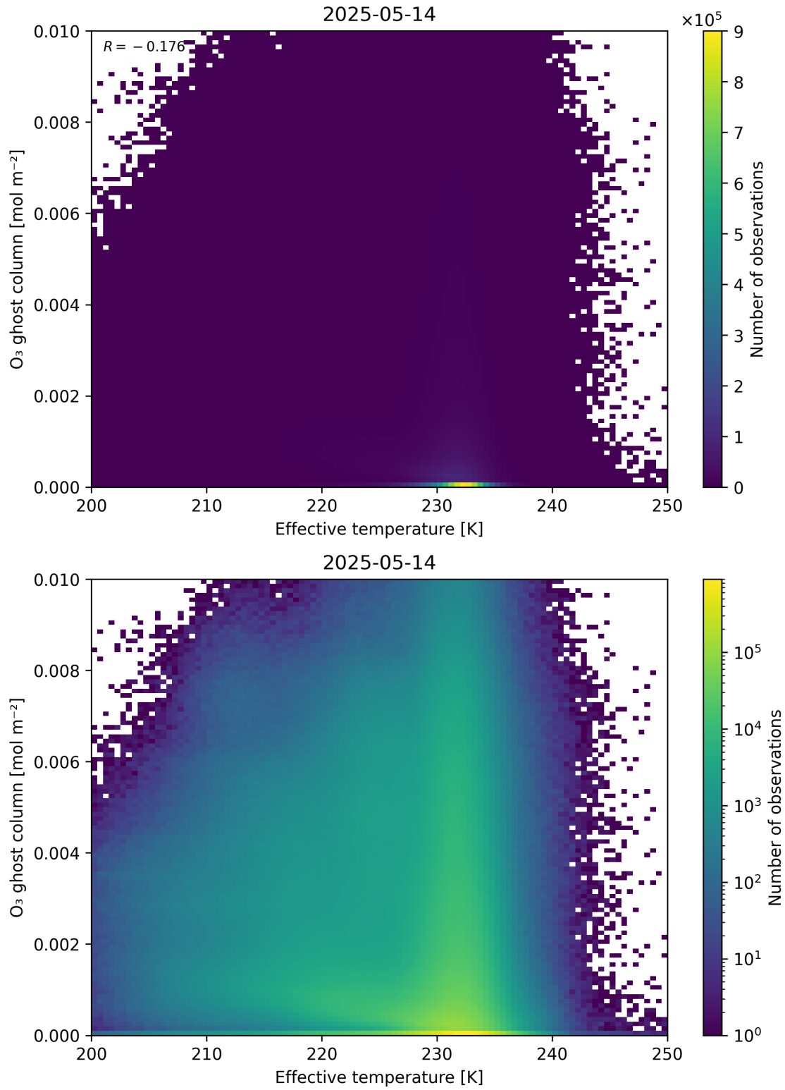
Figure 38: Scatter density plot of “Effective temperature” against “O 3 ghost column” for 2025-05-13 to 2025-05-15.
