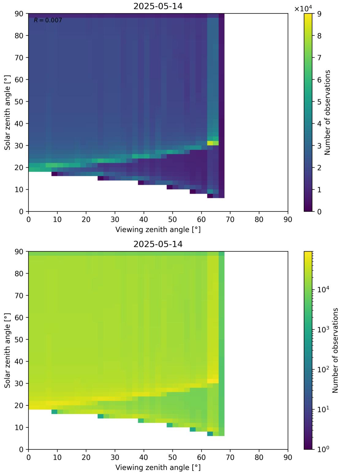
Figure 54: Scatter density plot of “Viewing zenith angle” against “Solar zenith angle” for 2025-05-13 to 2025-05-15.
