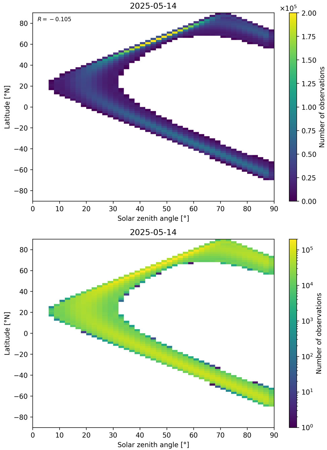
Figure 44: Scatter density plot of “Solar zenith angle” against “Latitude” for 2025-05-13 to 2025-05-15.
