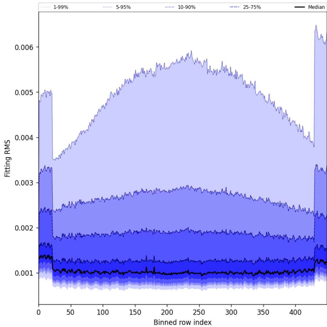
Figure 30: Along track statistics of “Fitting RMS” for 2025-05-13 to 2025-05-15
