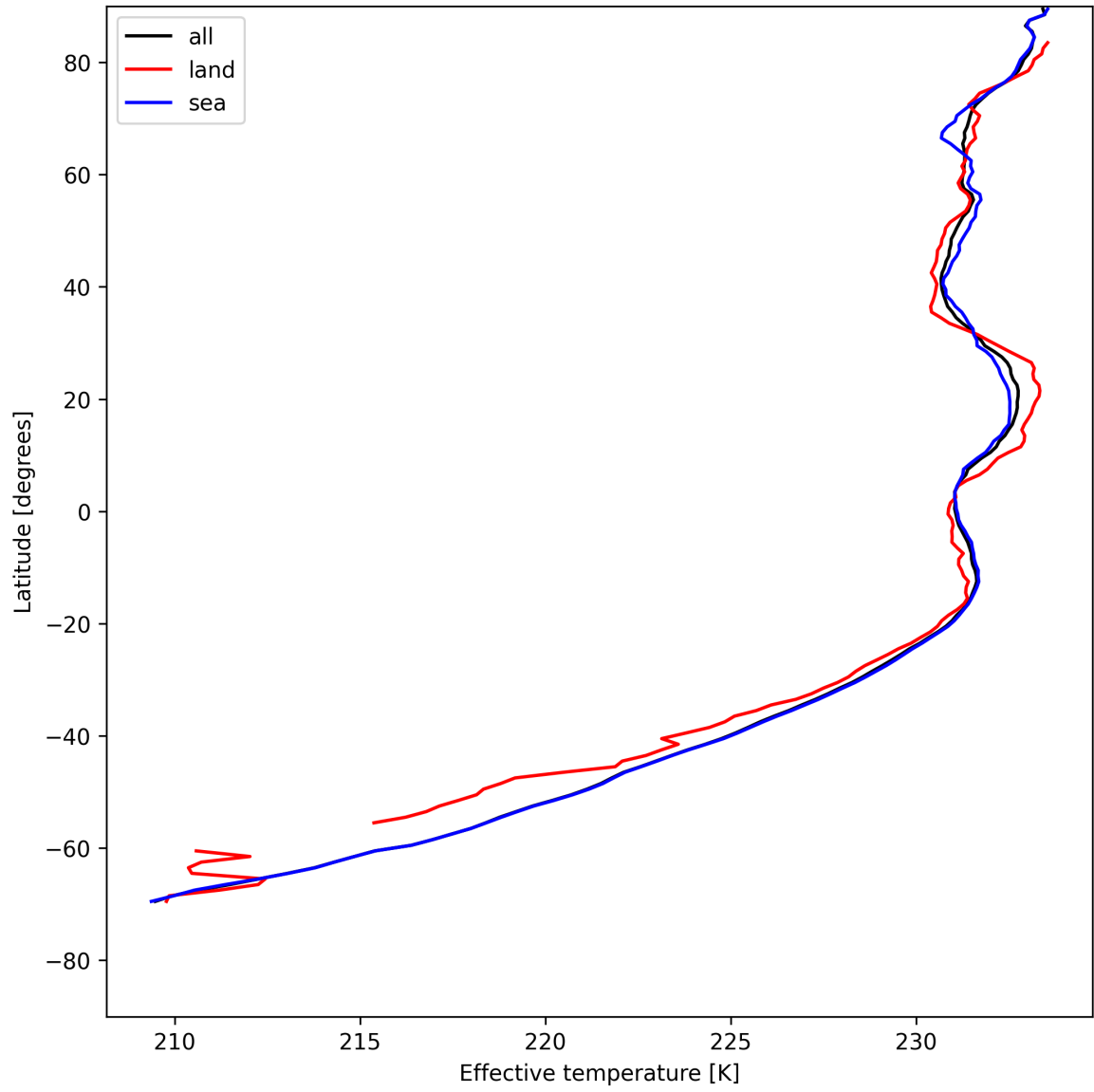
Figure 17: Zonal average of "Effective temperature" for 2025-05-13 to 2025-05-15.
