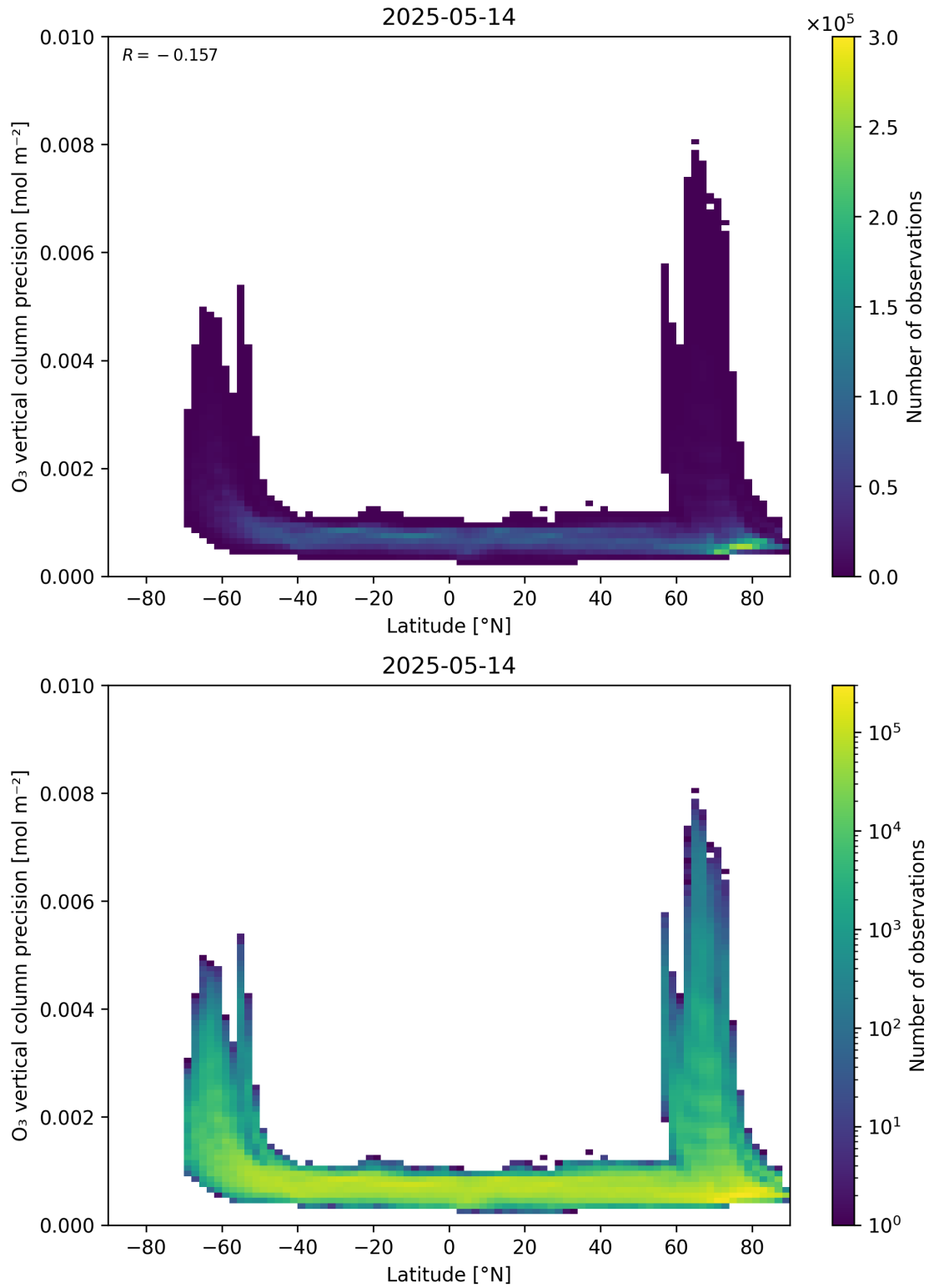
Figure 37: Scatter density plot of “Latitude” against “O 3 vertical column precision” for 2025-05-13 to 2025-05-15.
