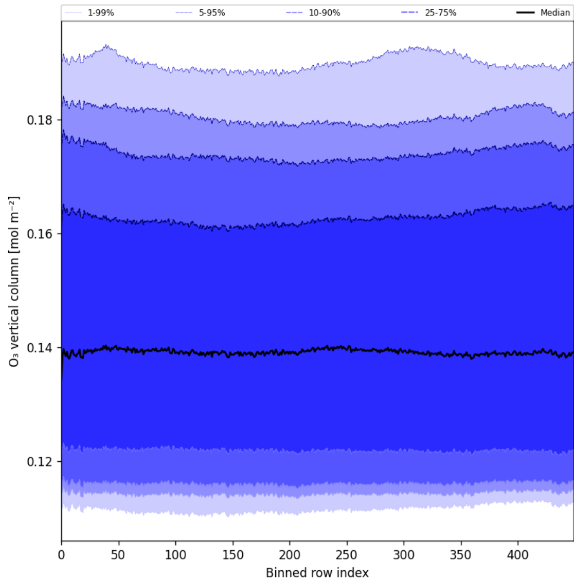
Figure 28: Along track statistics of “O 3 vertical column” for 2025-05-13 to 2025-05-15
