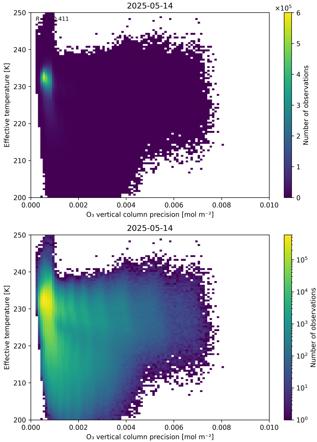
Figure 42: Scatter density plot of “O 3 vertical column precision” against “Effective temperature” for 2025-05-13 to 2025-05-15.
