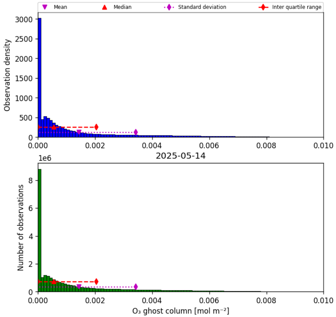
Figure 25: Histogram of “O 3 ghost column” for 2025-05-13 to 2025-05-15
