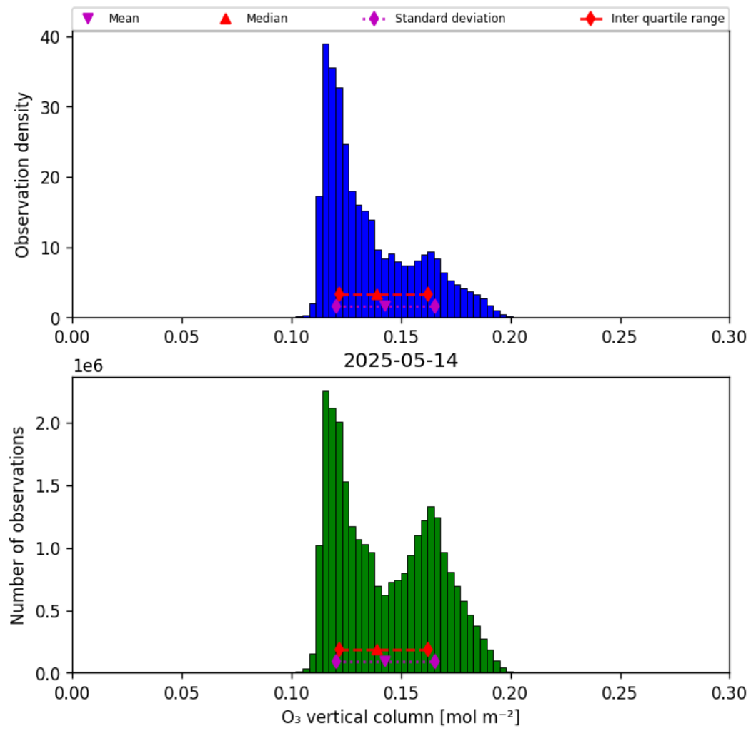
Figure 21: Histogram of “O 3 vertical column” for 2025-05-13 to 2025-05-15
