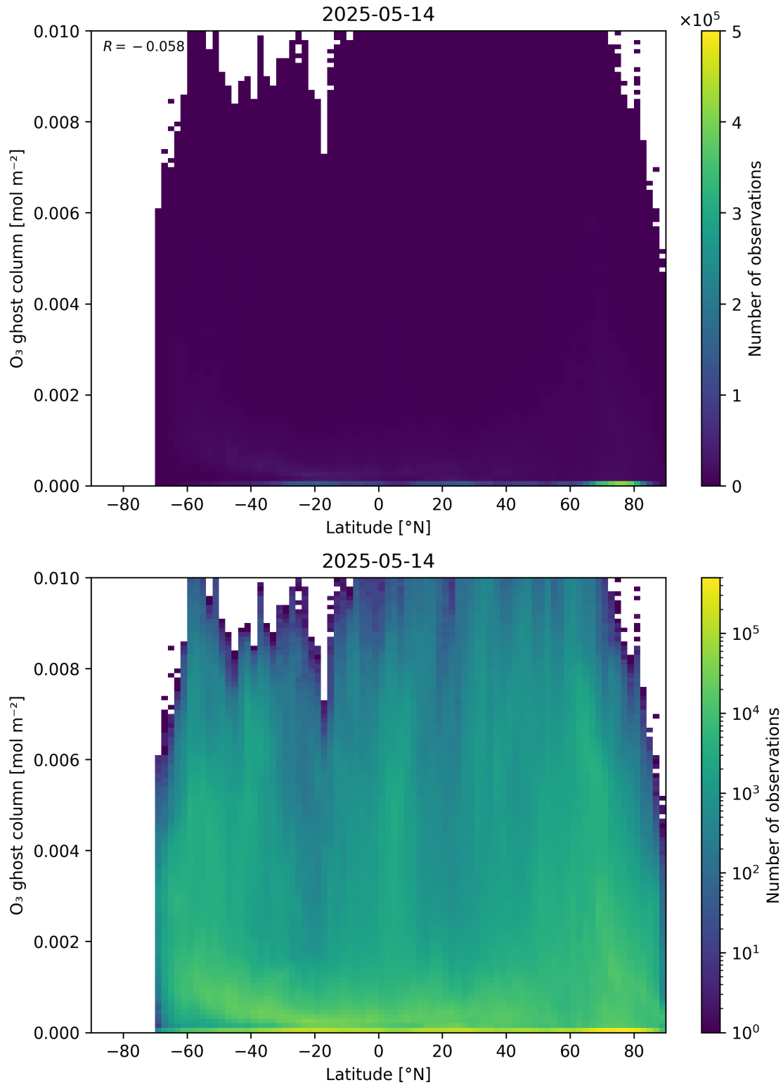
Figure 35: Scatter density plot of “Latitude” against “O 3 ghost column” for 2025-05-13 to 2025-05-15.
