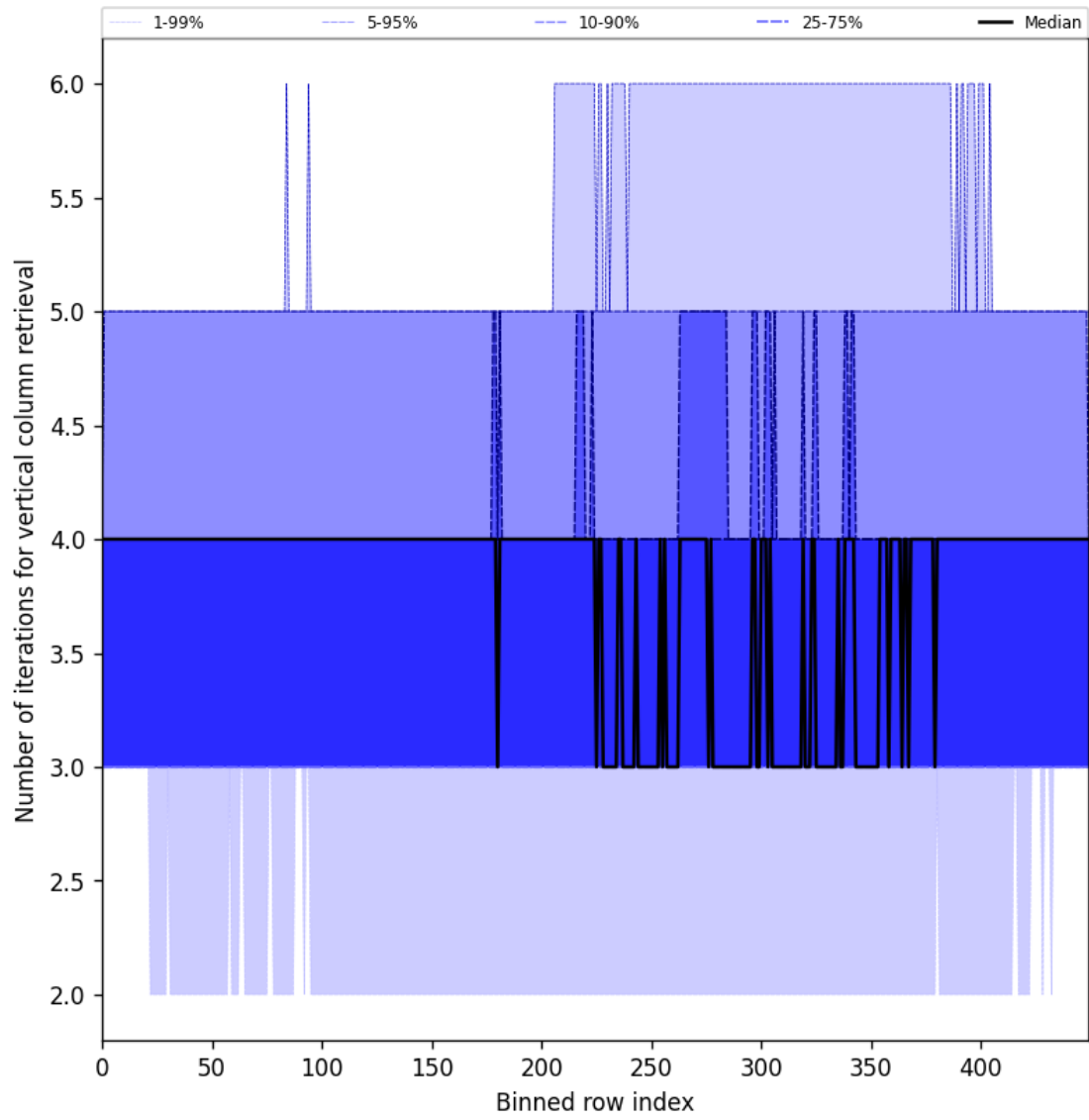
Figure 33: Along track statistics of “Number of iterations for vertical column retrieval” for 2025-05-13 to 2025-05-15
