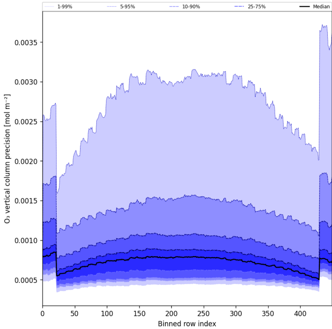
Figure 29: Along track statistics of “O 3 vertical column precision” for 2025-05-13 to 2025-05-15
