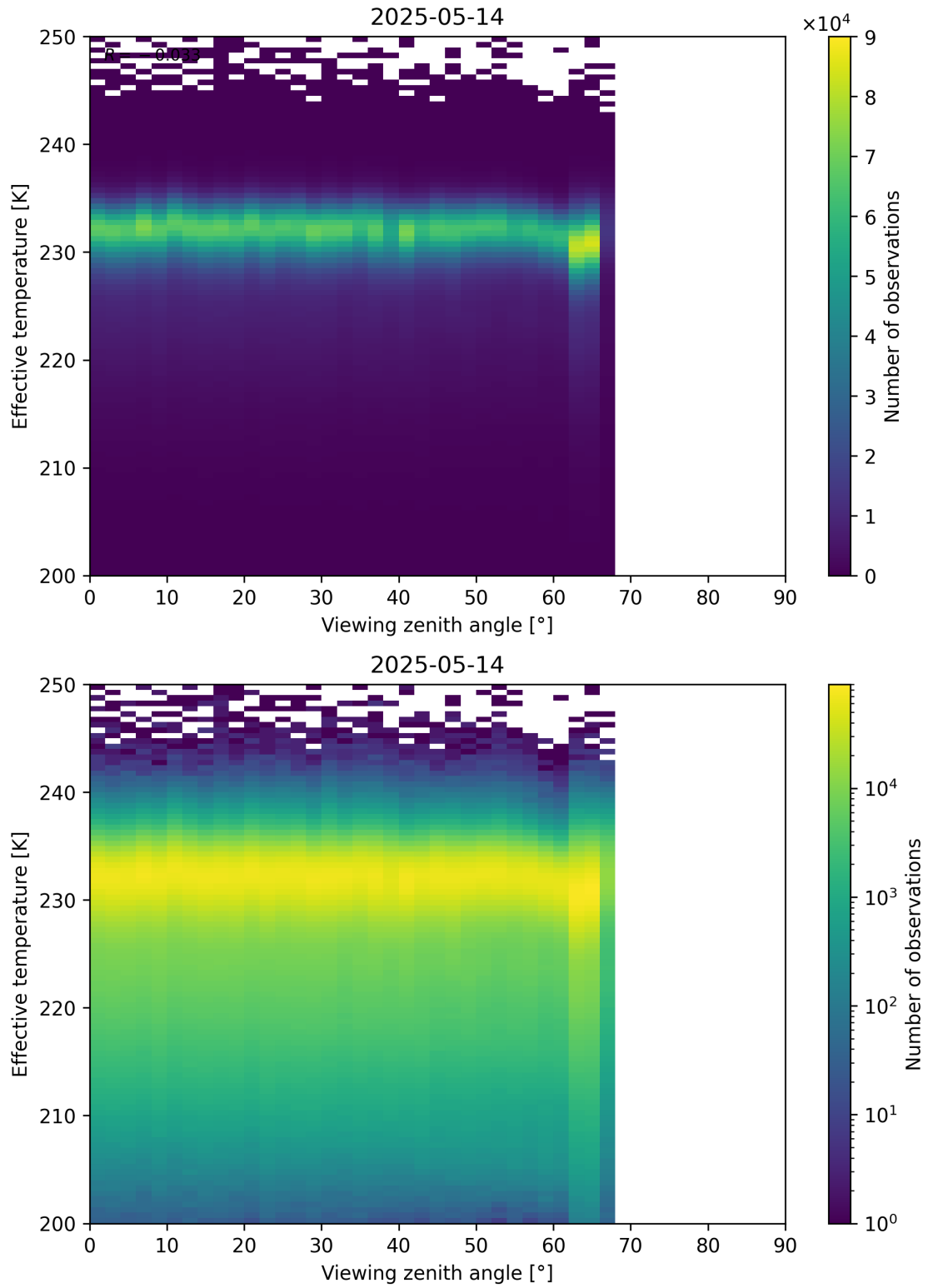
Figure 50: Scatter density plot of “Viewing zenith angle” against “Effective temperature” for 2025-05-13 to 2025-05-15.
