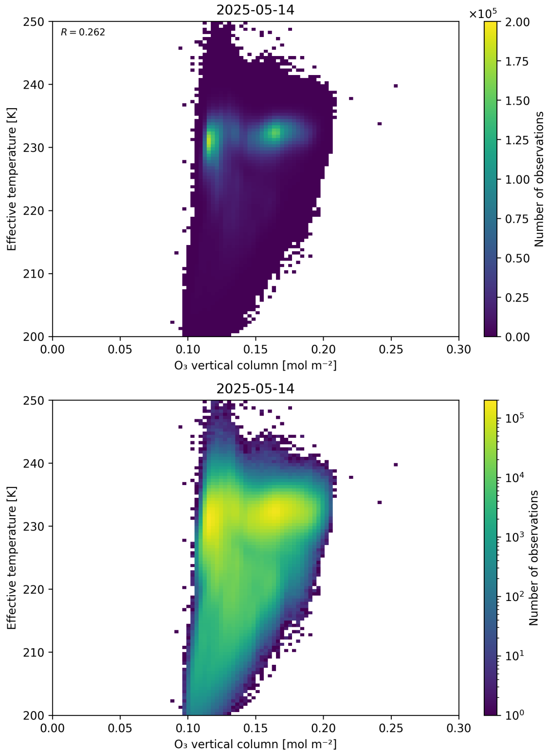
Figure 39: Scatter density plot of “O 3 vertical column” against “Effective temperature” for 2025-05-13 to 2025-05-15.
