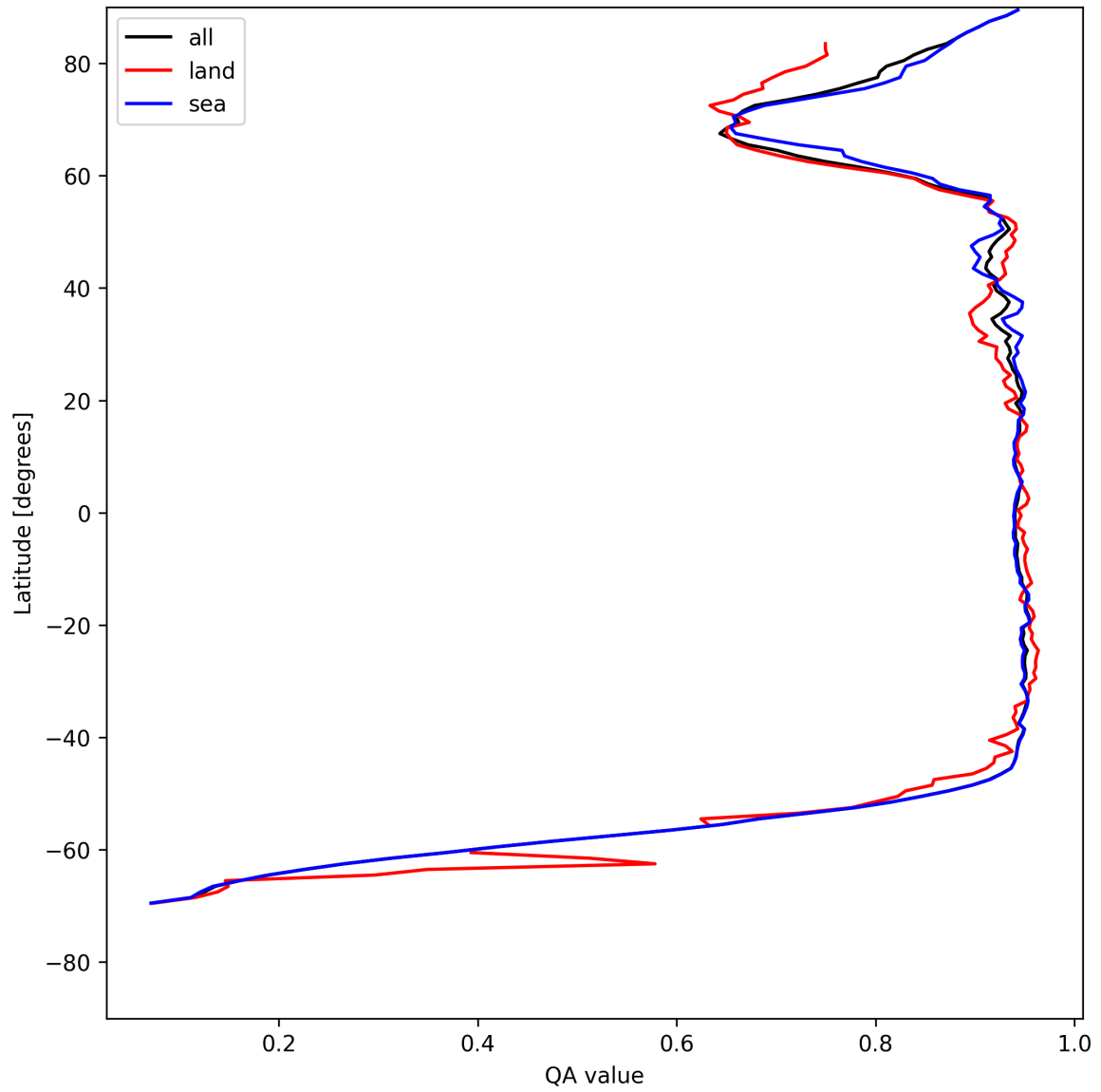
Figure 13: Zonal average of “QA value” for 2025-05-13 to 2025-05-15.
