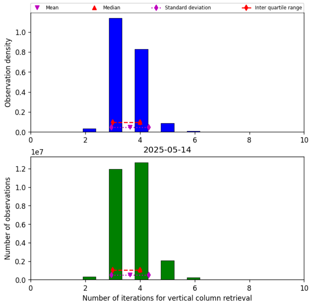
Figure 26: Histogram of “Number of iterations for vertical column retrieval” for 2025-05-13 to 2025-05-15
