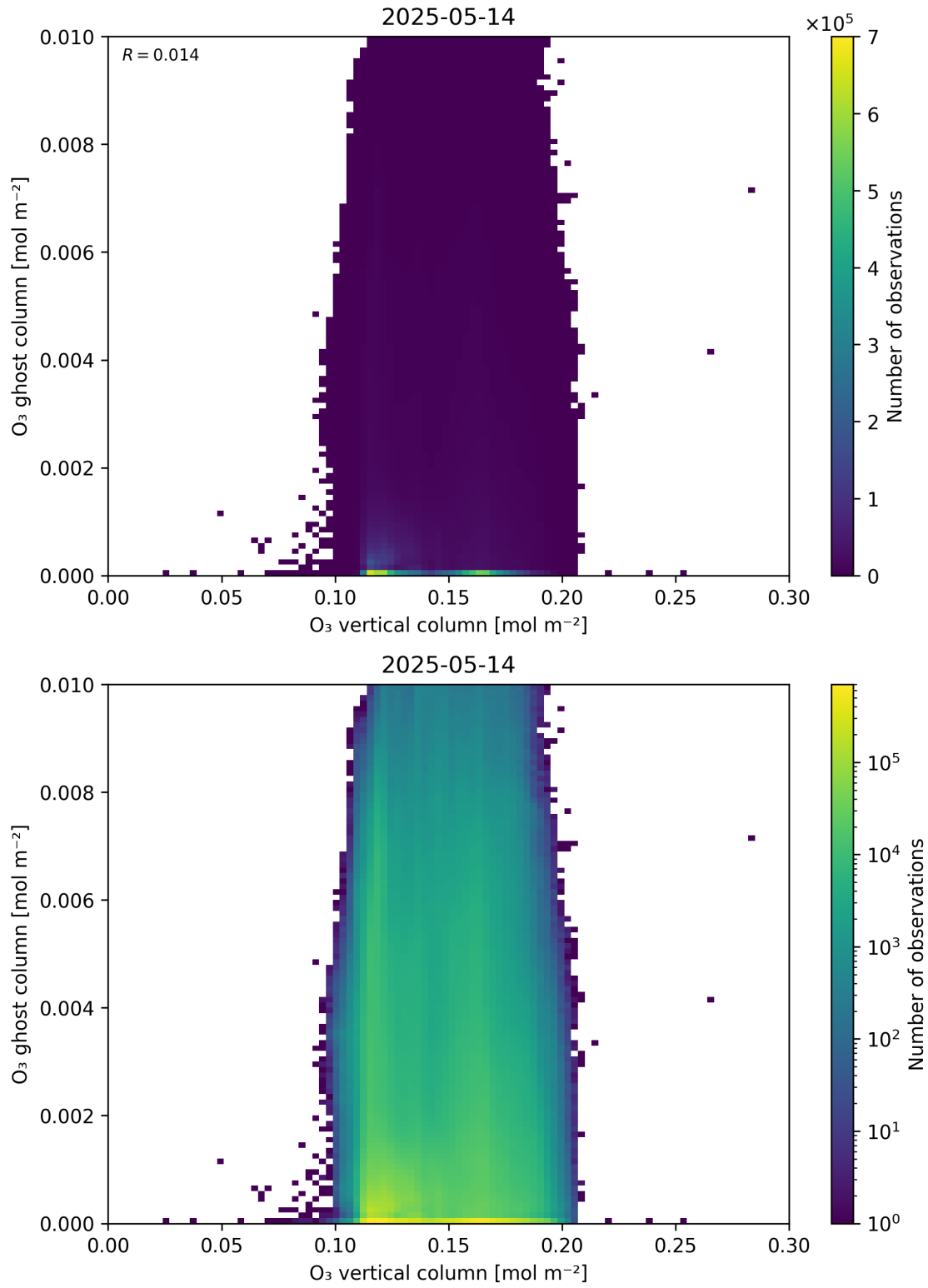
Figure 40: Scatter density plot of “O 3 vertical column” against “O 3 ghost column” for 2025-05-13 to 2025-05-15.
