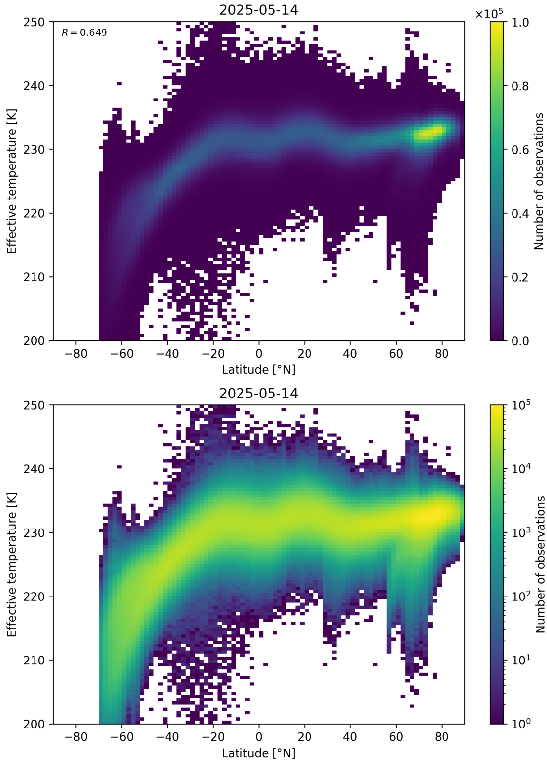
Figure 34: Scatter density plot of “Latitude” against “Effective temperature” for 2025-05-13 to 2025-05-15.
