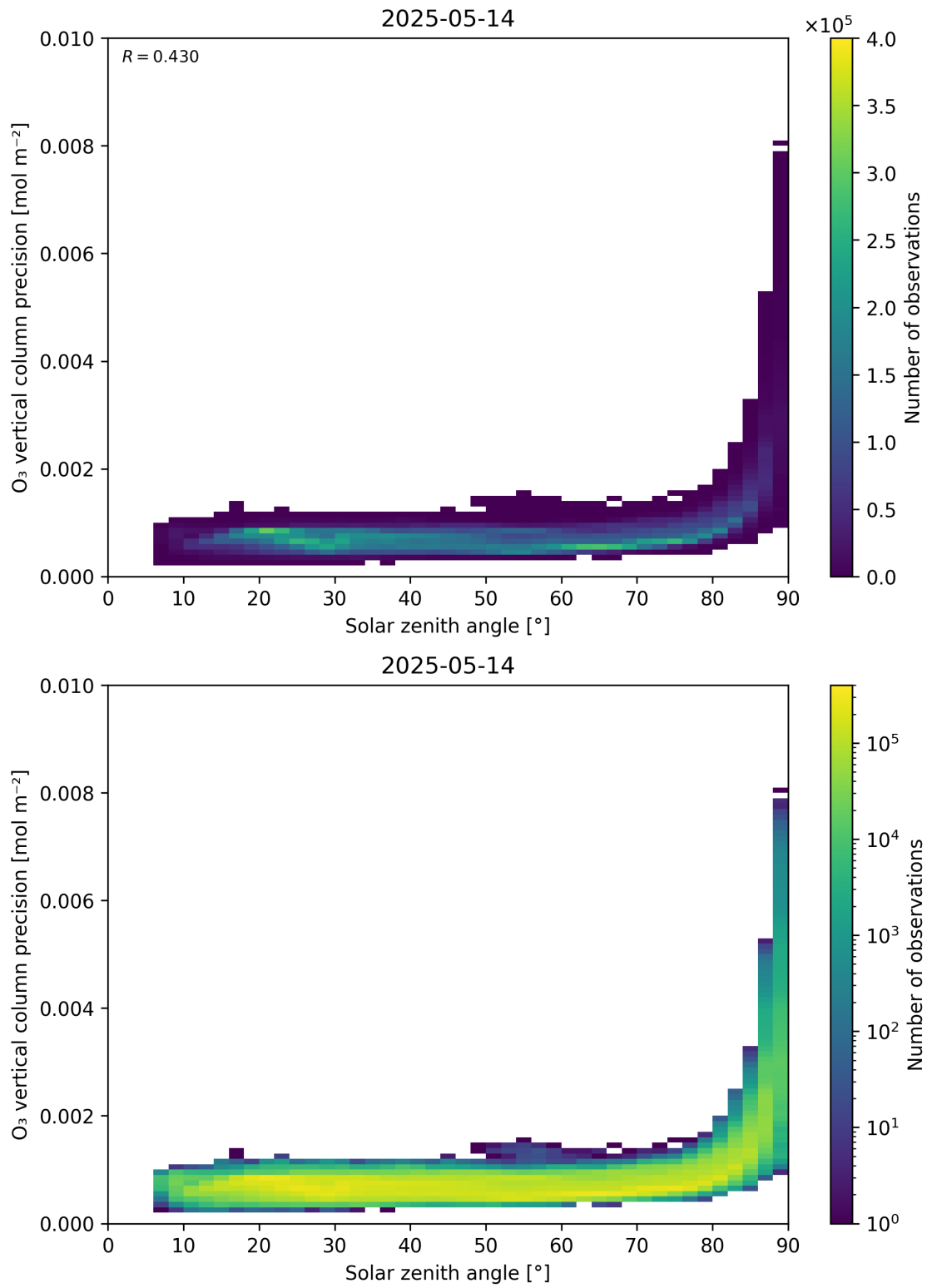
Figure 48: Scatter density plot of “Solar zenith angle” against “O 3 vertical column precision” for 2025-05-13 to 2025-05-15.
