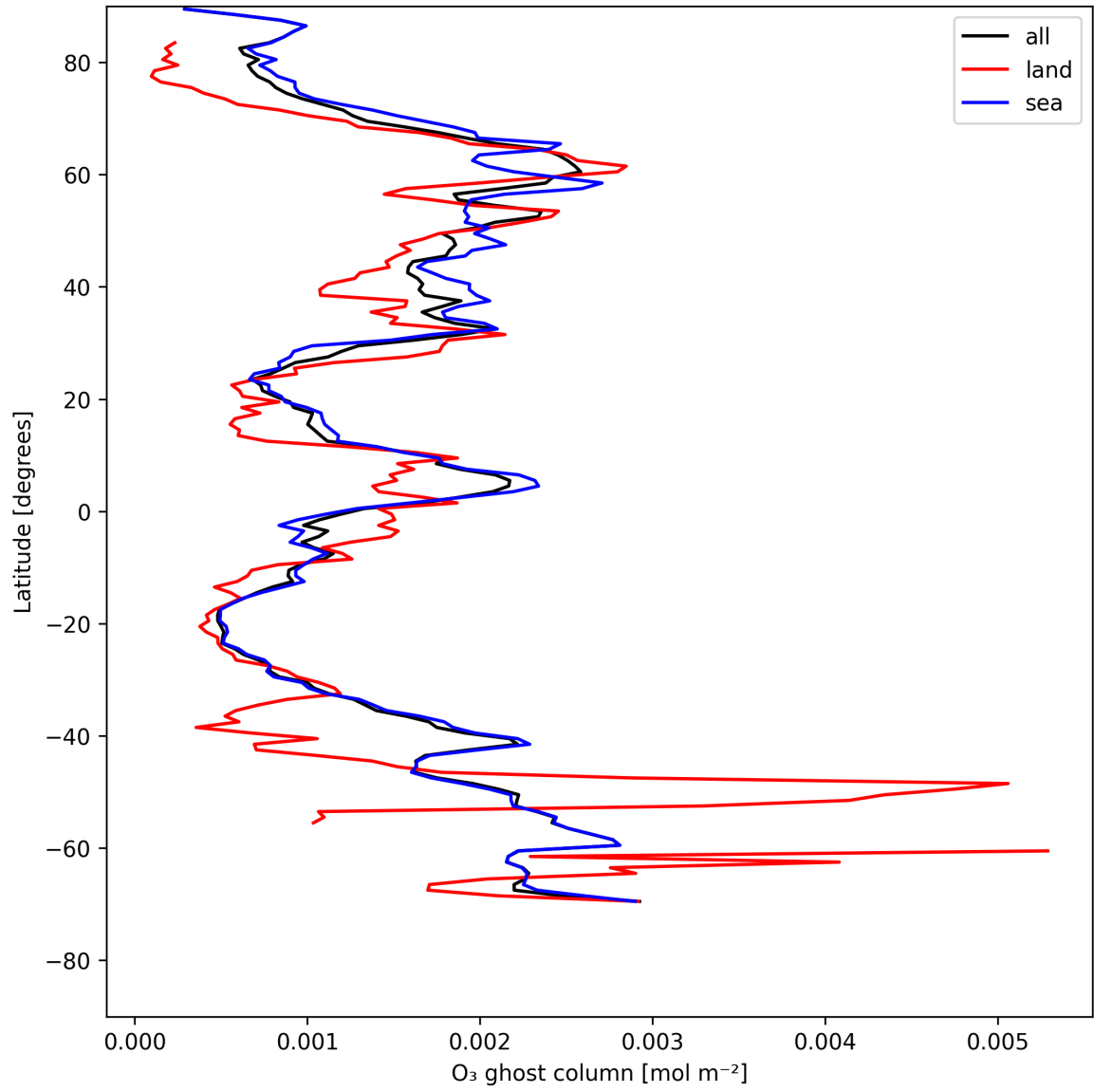
Figure 18: Zonal average of “O 3 ghost column” for 2025-05-13 to 2025-05-15.
