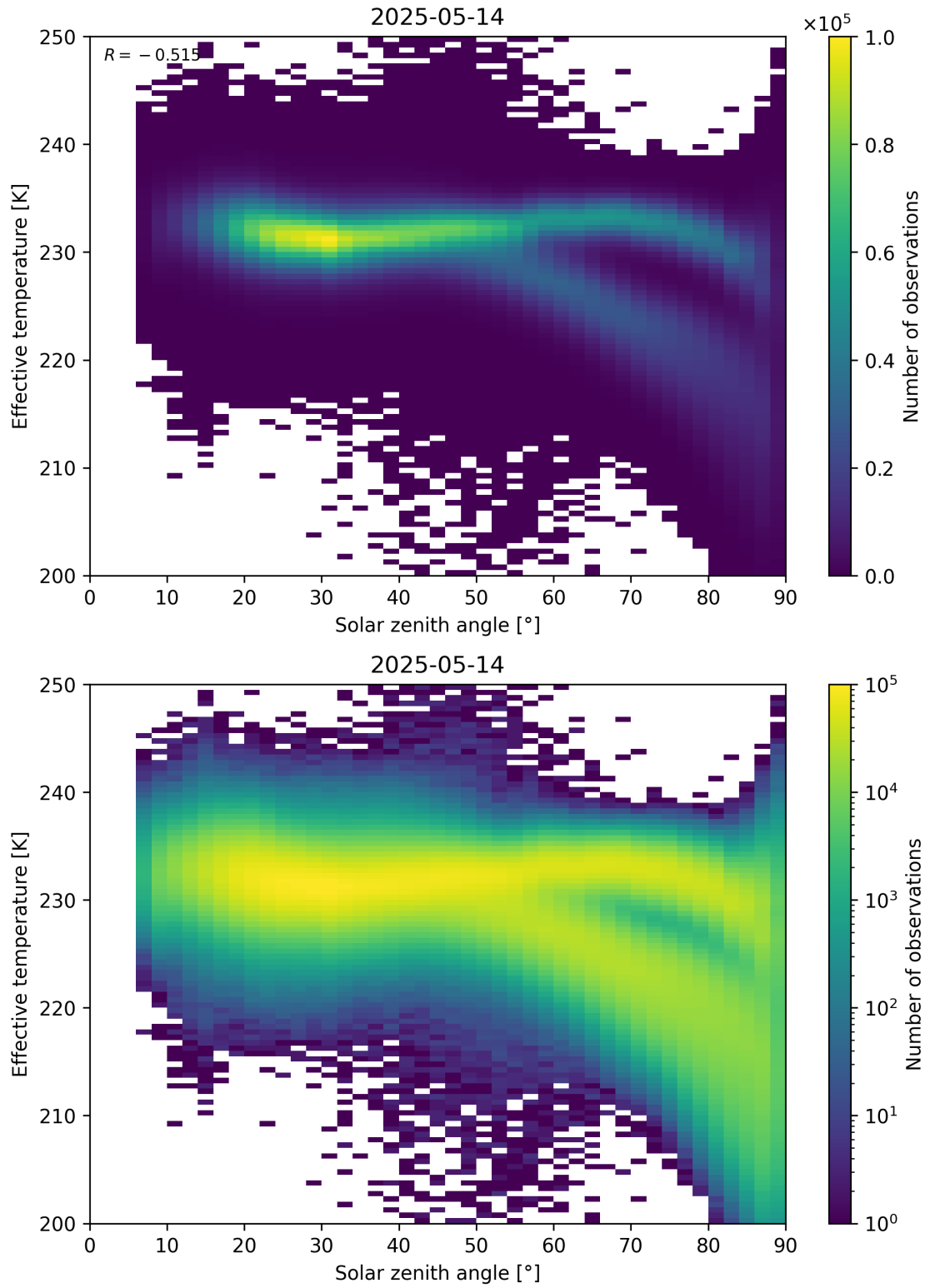
Figure 45: Scatter density plot of “Solar zenith angle” against “Effective temperature” for 2025-05-13 to 2025-05-15.
