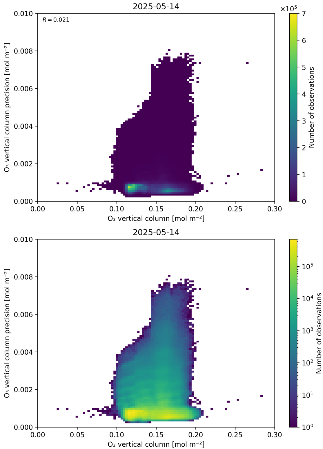
Figure 41: Scatter density plot of “O 3 vertical column” against “O 3 vertical column precision” for 2025-05-13 to 2025-05-15.
