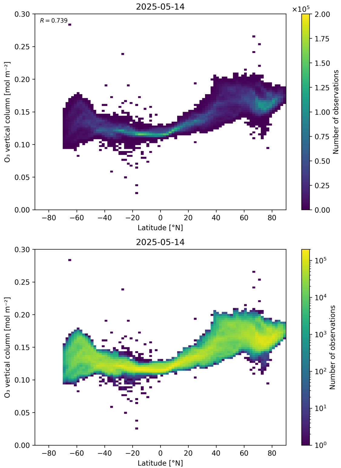
Figure 36: Scatter density plot of “Latitude” against “O 3 vertical column” for 2025-05-13 to 2025-05-15.
