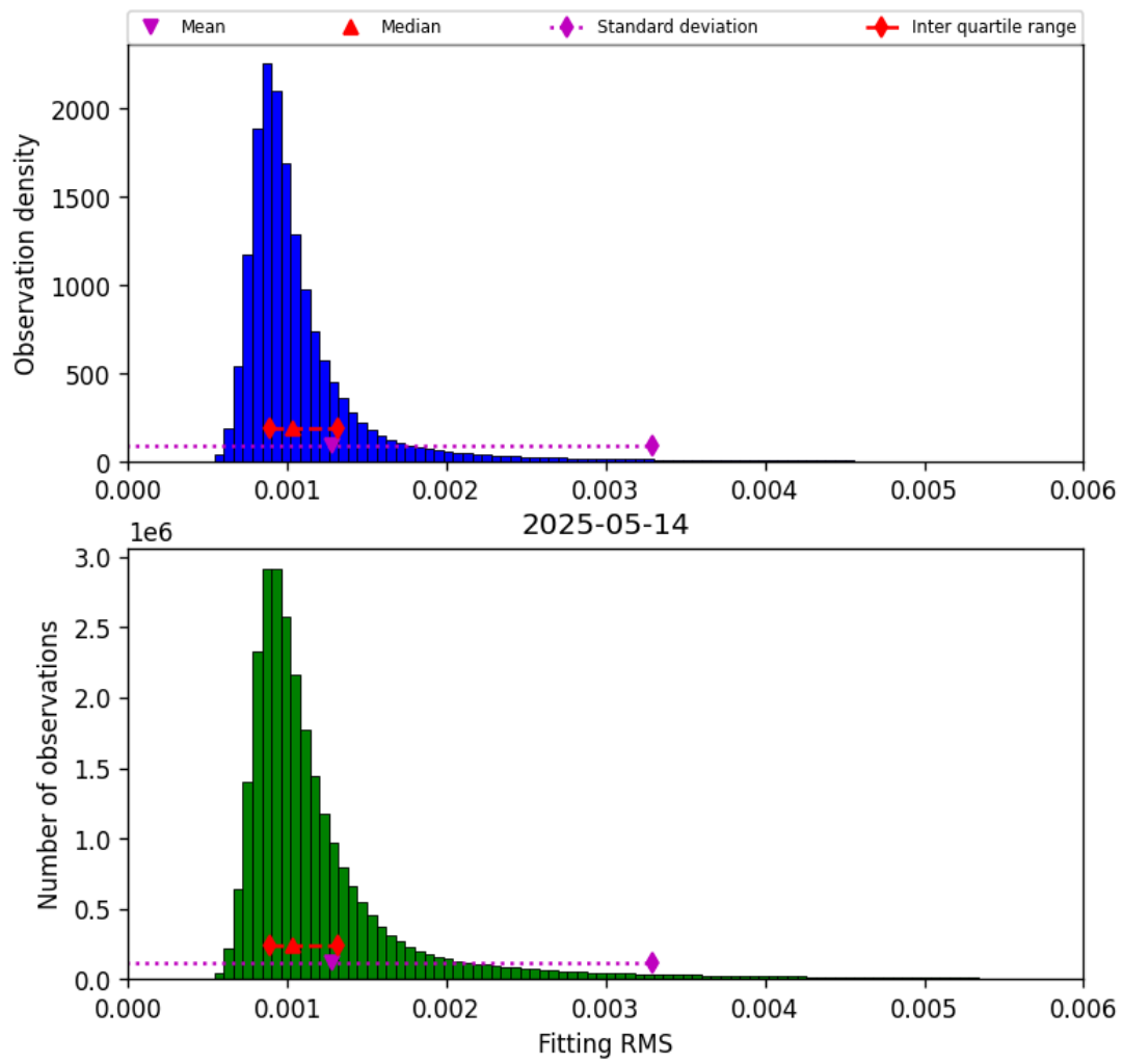
Figure 23: Histogram of “Fitting RMS” for 2025-05-13 to 2025-05-15
