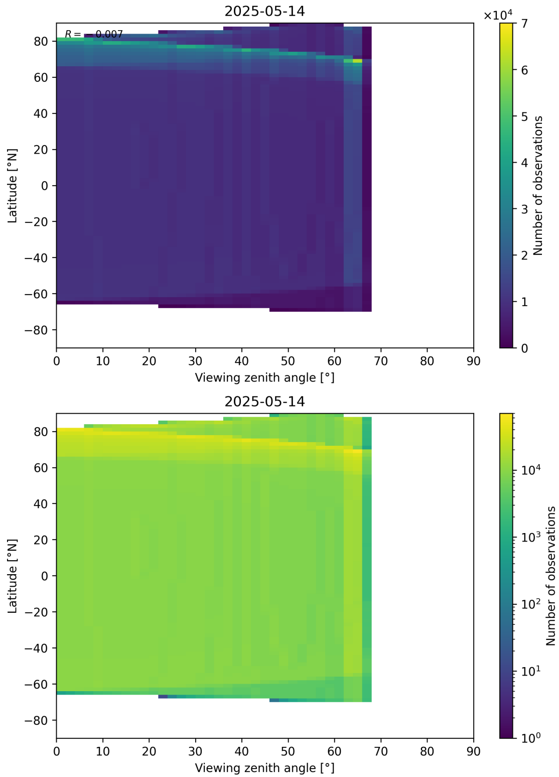
Figure 49: Scatter density plot of “Viewing zenith angle” against “Latitude” for 2025-05-13 to 2025-05-15.
