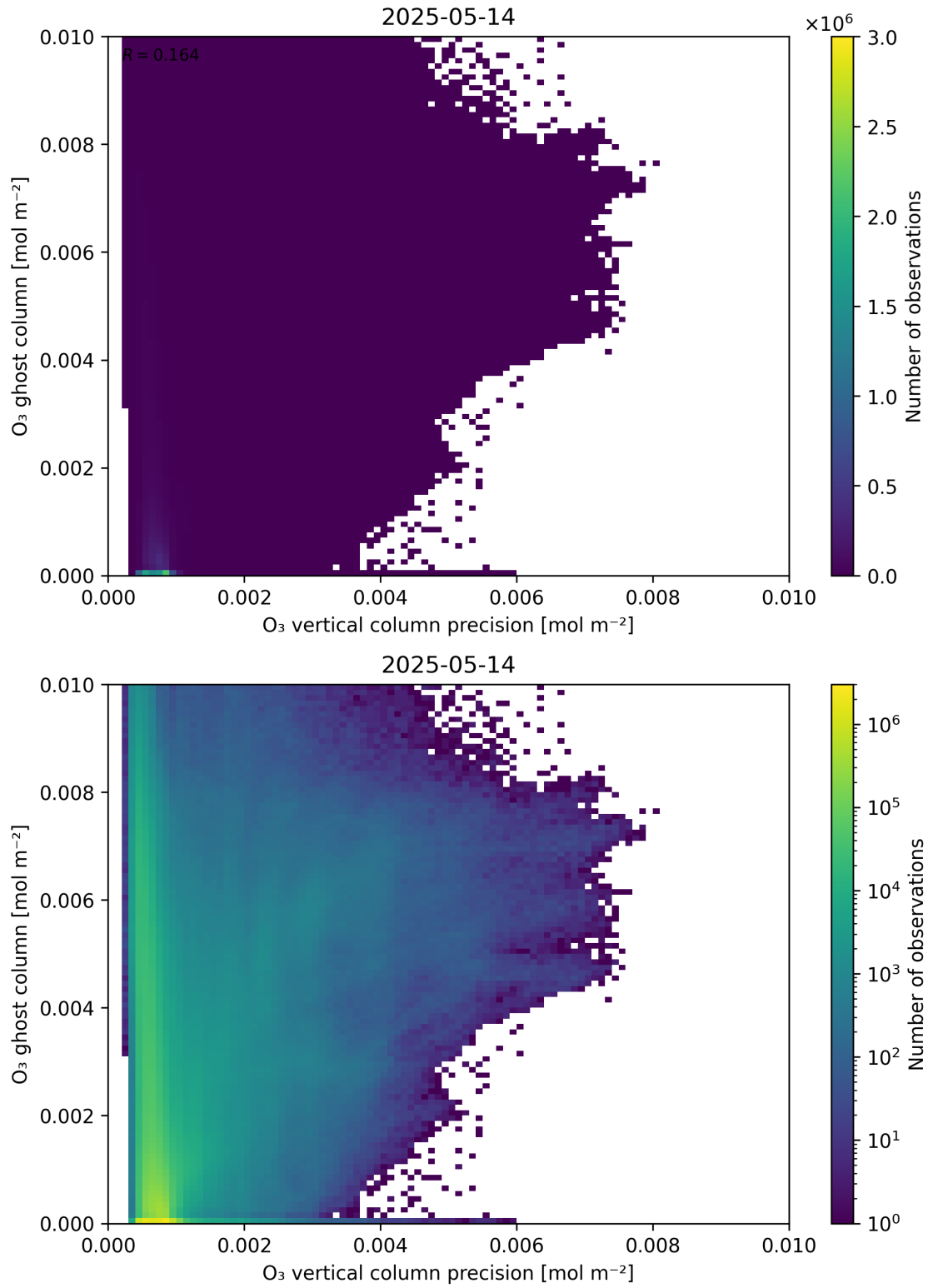
Figure 43: Scatter density plot of “ O_3 vertical column precision” against “ O_3 ghost column” for 2025-05-13 to 2025-05-15.
