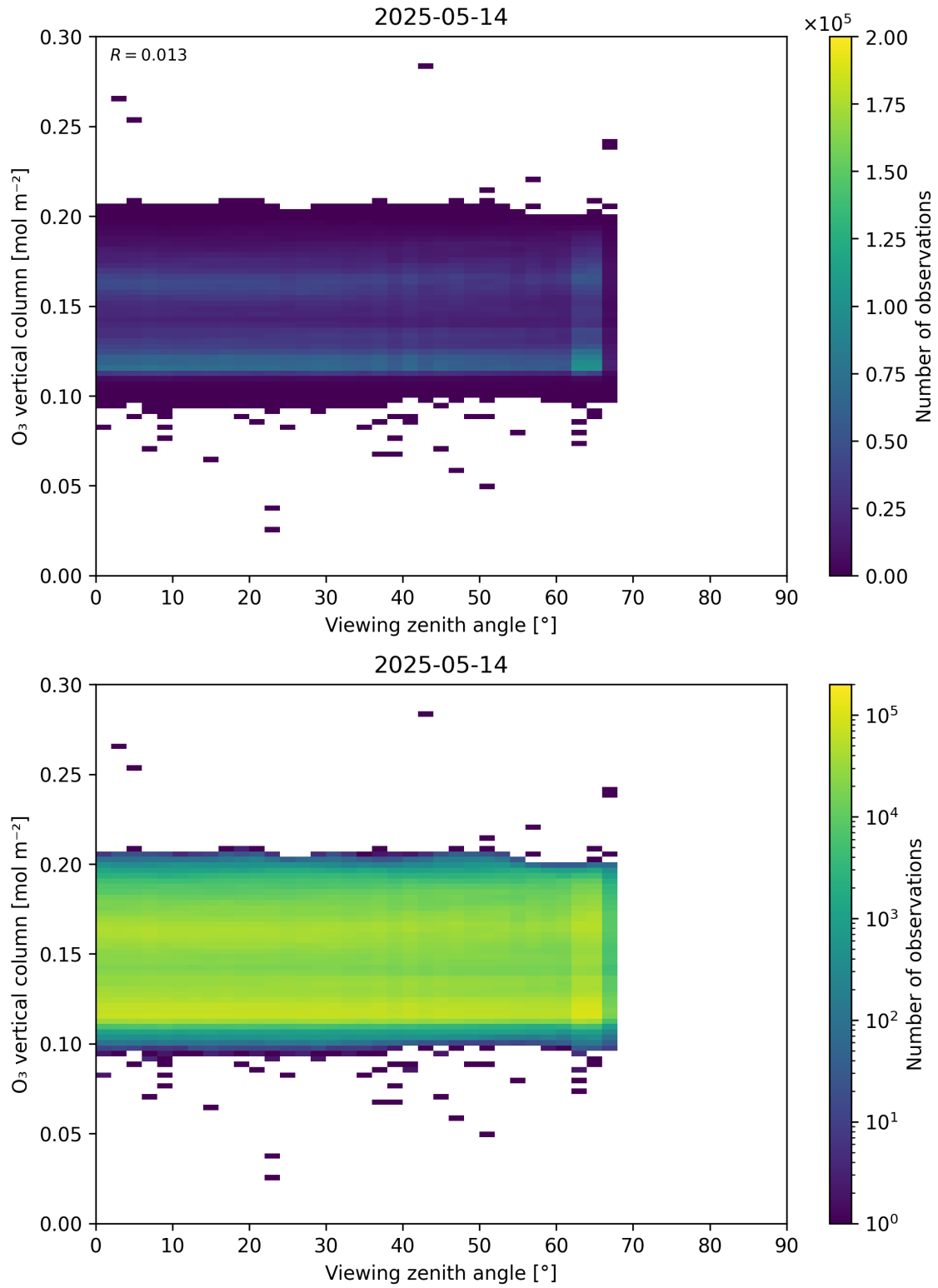
Figure 52: Scatter density plot of “Viewing zenith angle” against “O 3 vertical column” for 2025-05-13 to 2025-05-15.
