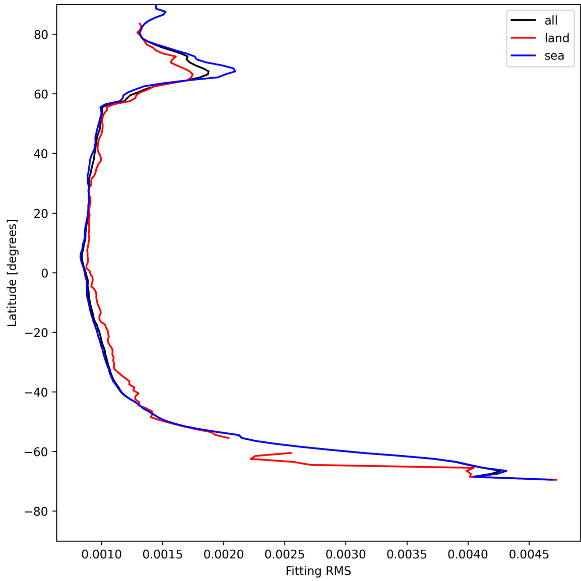
Figure 16: Zonal average of “Fitting RMS” for 2025-05-13 to 2025-05-15.
