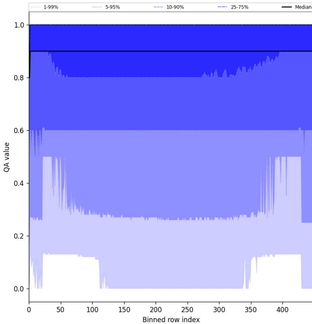
Figure 27: Along track statistics of “QA value” for 2025-05-13 to 2025-05-15
