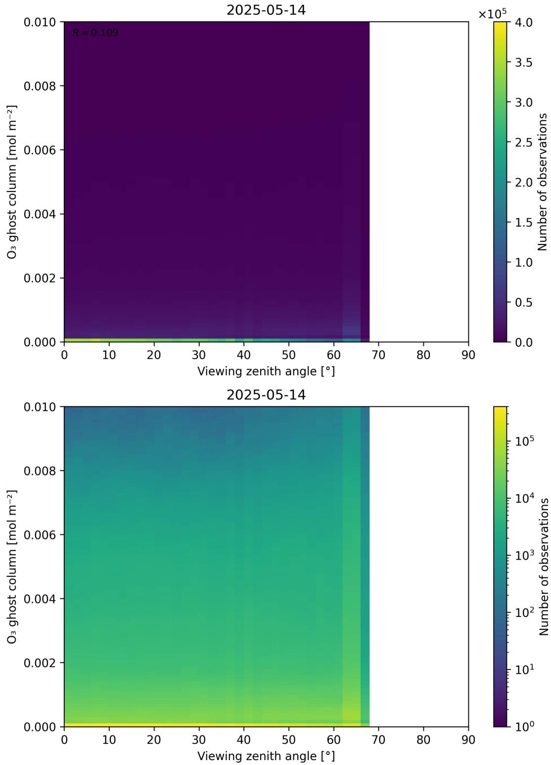
Figure 51: Scatter density plot of “Viewing zenith angle” against “O 3 ghost column” for 2025-05-13 to 2025-05-15.
