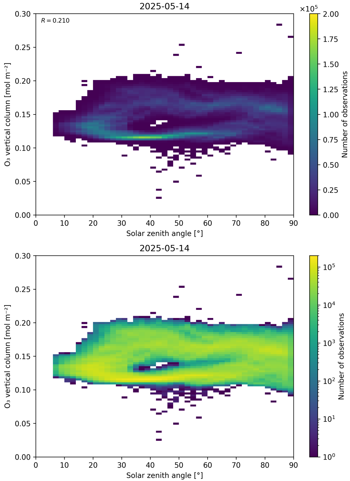
Figure 47: Scatter density plot of “Solar zenith angle” against “O 3 vertical column” for 2025-05-13 to 2025-05-15.
