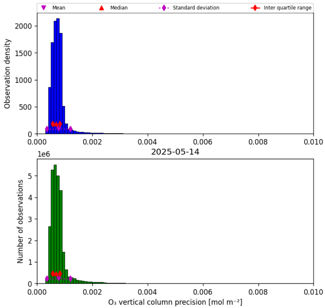
Figure 22: Histogram of “O 3 vertical column precision” for 2025-05-13 to 2025-05-15
