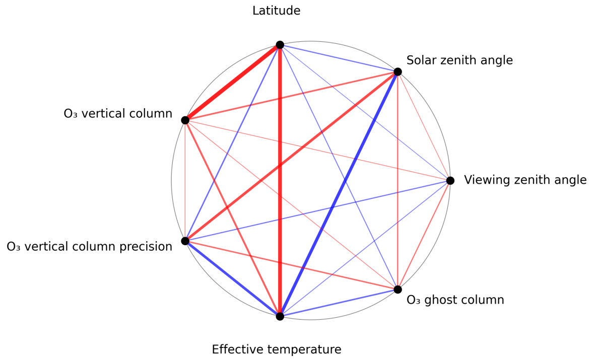
Figure 1: Map of correlation graph for 2025-05-13 to 2025-05-15.
