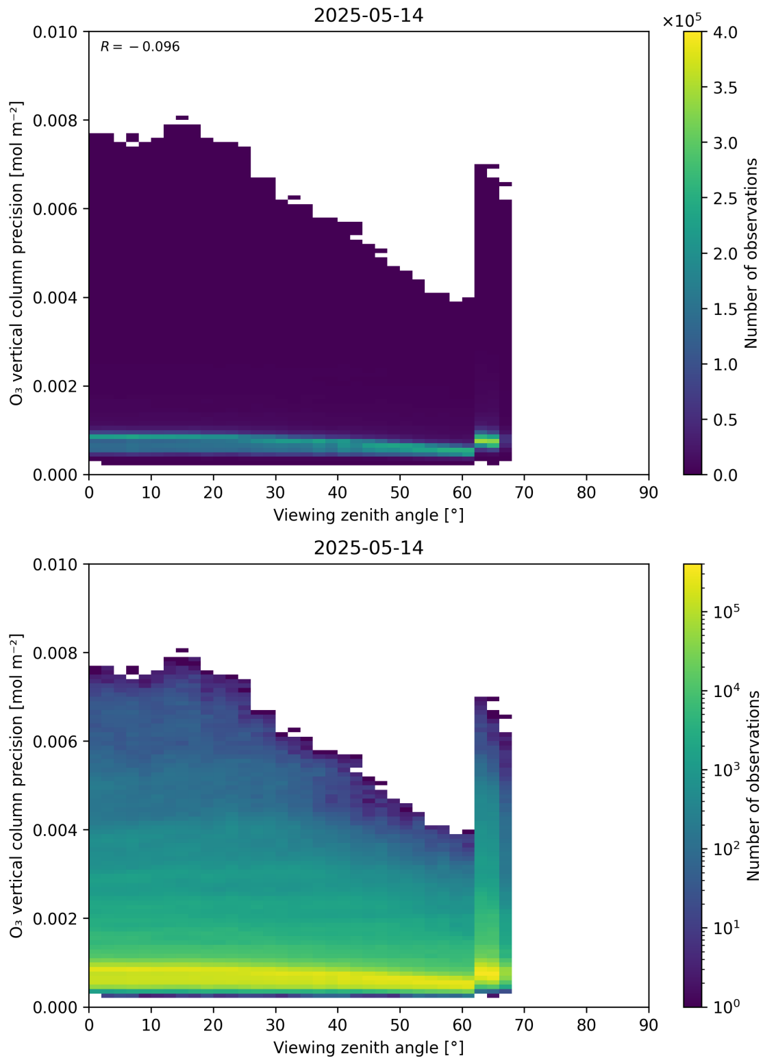
Figure 53: Scatter density plot of “Viewing zenith angle” against “O 3 vertical column precision” for 2025-05-13 to 2025-05-15.
