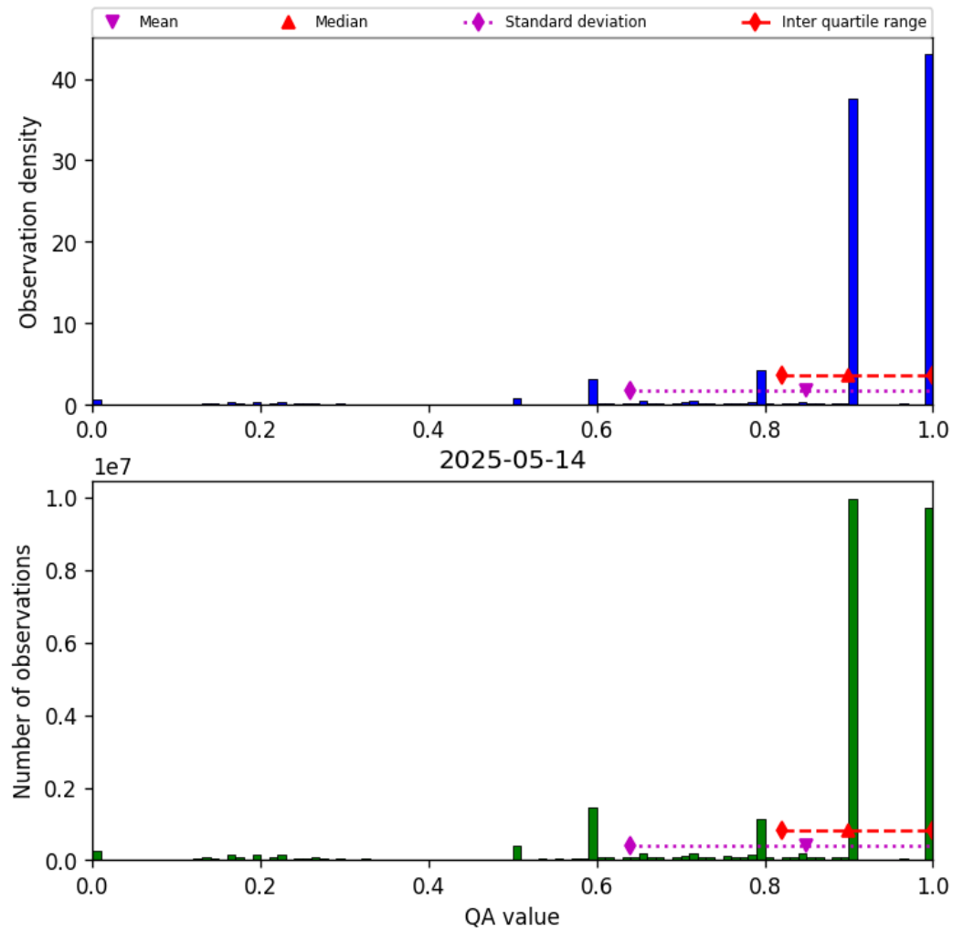
Figure 20: Histogram of “QA value” for 2025-05-13 to 2025-05-15
