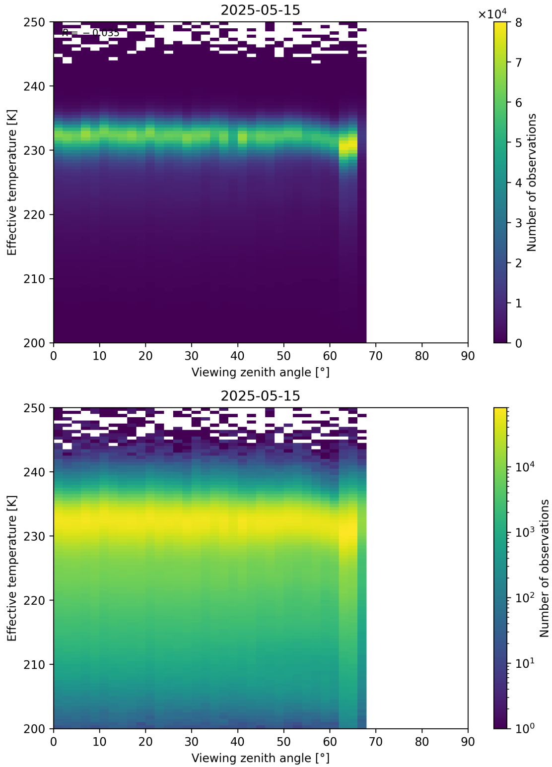
Figure 50: Scatter density plot of “Viewing zenith angle” against “Effective temperature” for 2025-05-15 to 2025-05-16.
