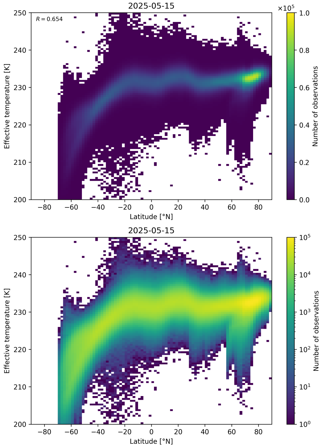
Figure 34: Scatter density plot of “Latitude” against “Effective temperature” for 2025-05-15 to 2025-05-16.
