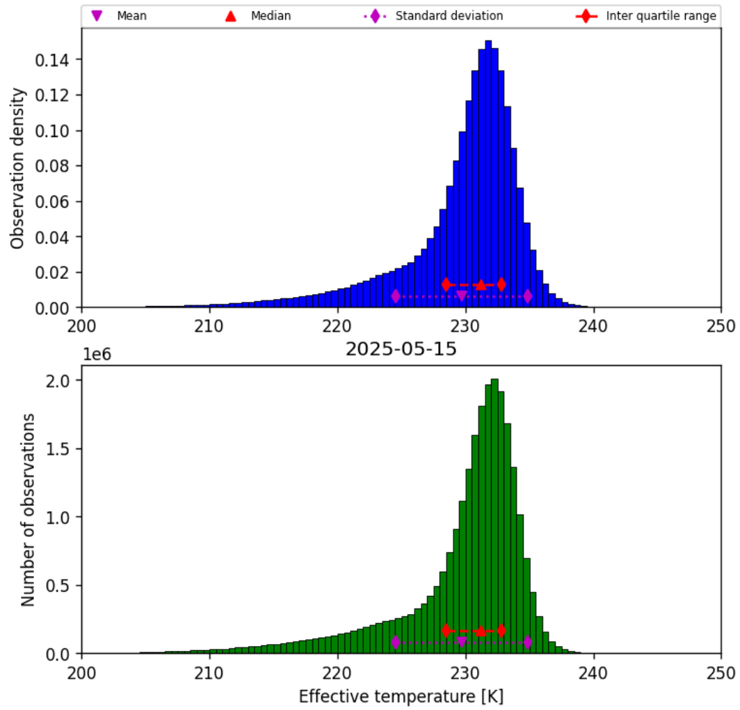
Figure 24: Histogram of “Effective temperature” for 2025-05-15 to 2025-05-16
