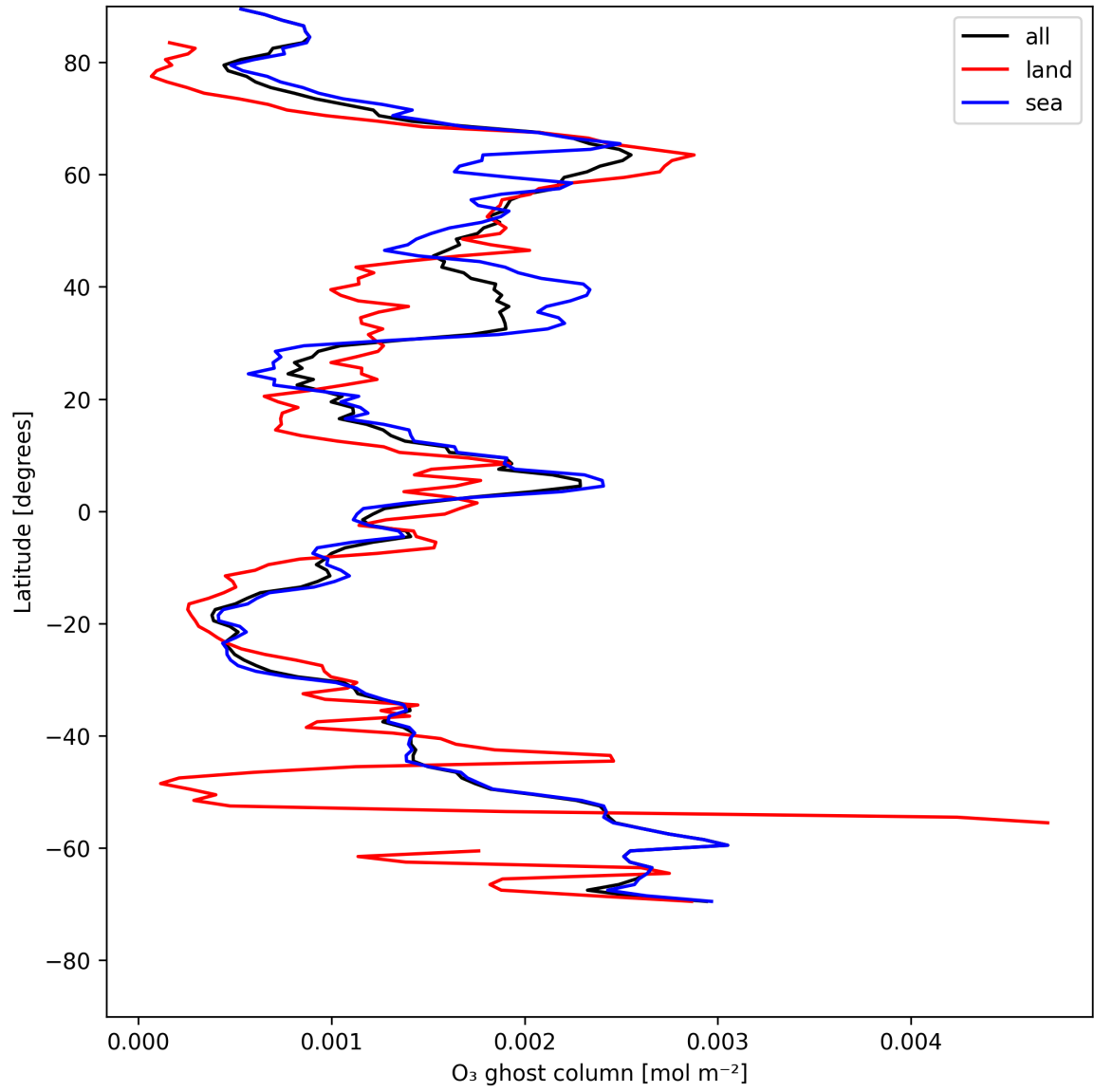
Figure 18: Zonal average of "O 3 ghost column" for 2025-05-15 to 2025-05-16.
