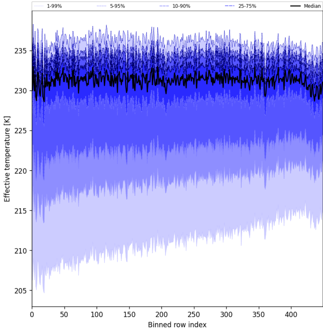
Figure 31: Along track statistics of “Effective temperature” for 2025-05-15 to 2025-05-16
