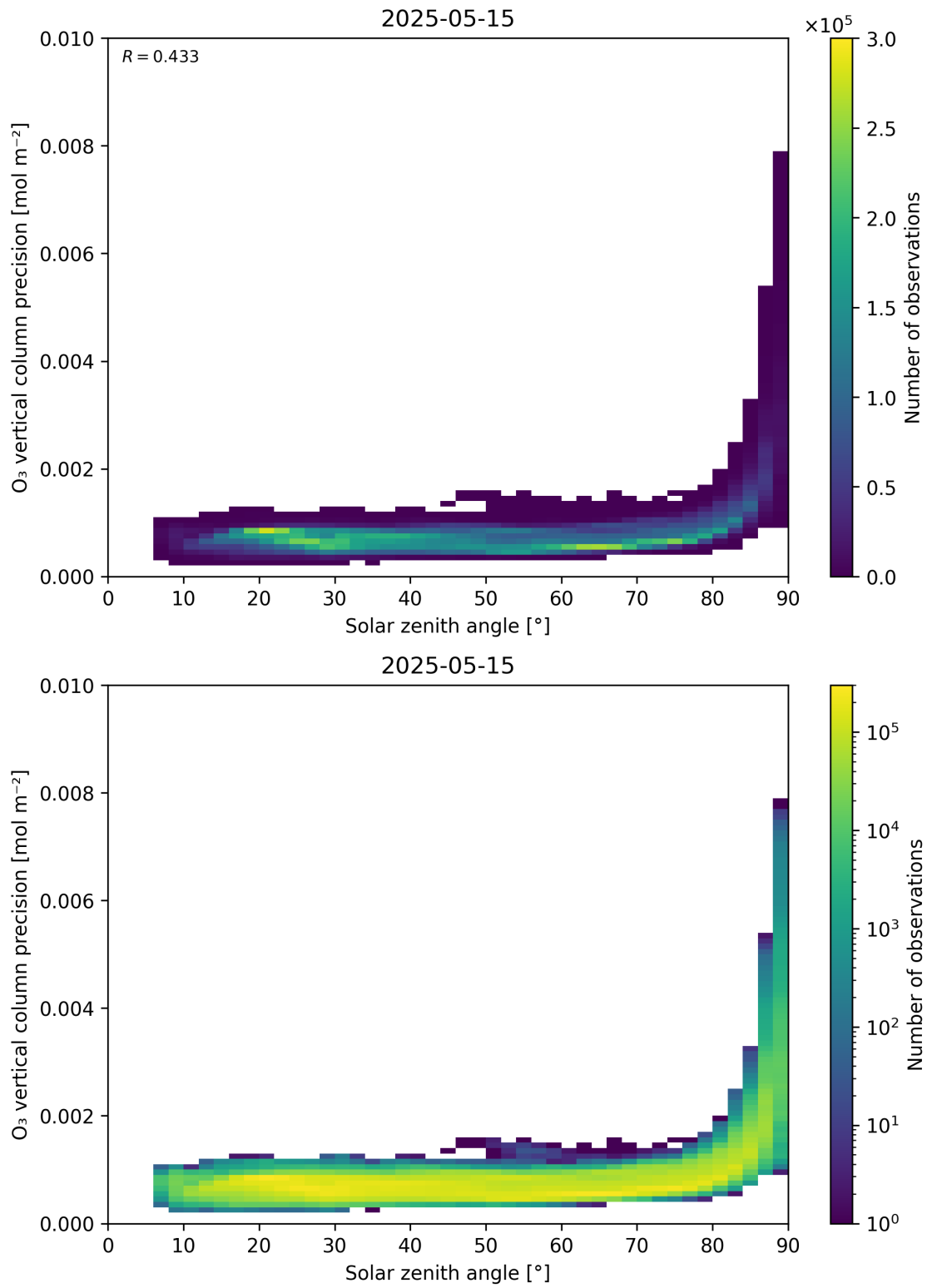
Figure 48: Scatter density plot of “Solar zenith angle” against “O 3 vertical column precision” for 2025-05-15 to 2025-05-16.
