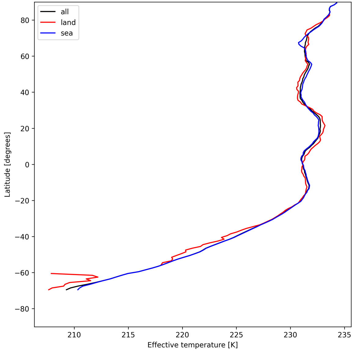
Figure 17: Zonal average of "Effective temperature" for 2025-05-15 to 2025-05-16.
