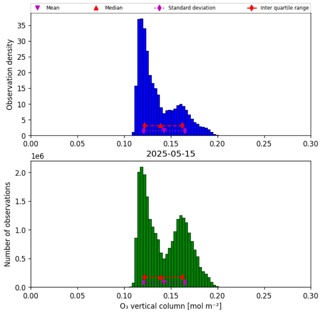
Figure 21: Histogram of “O 3 vertical column” for 2025-05-15 to 2025-05-16
