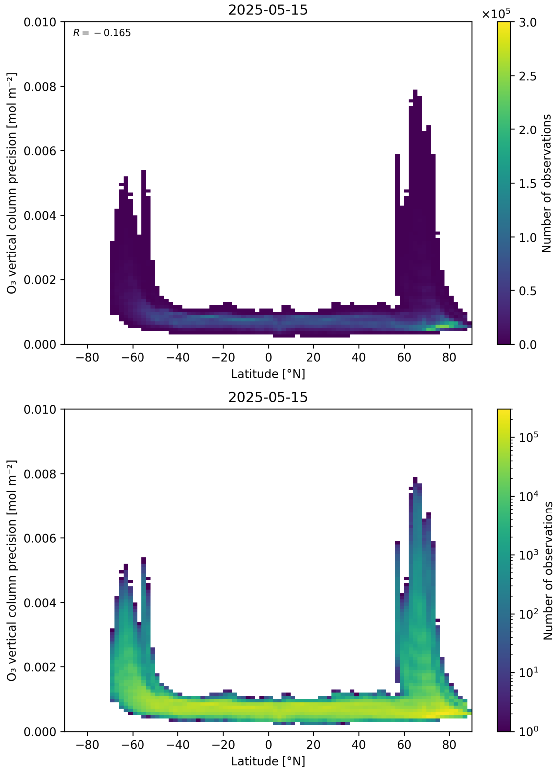
Figure 37: Scatter density plot of “Latitude” against “O 3 vertical column precision” for 2025-05-15 to 2025-05-16.
