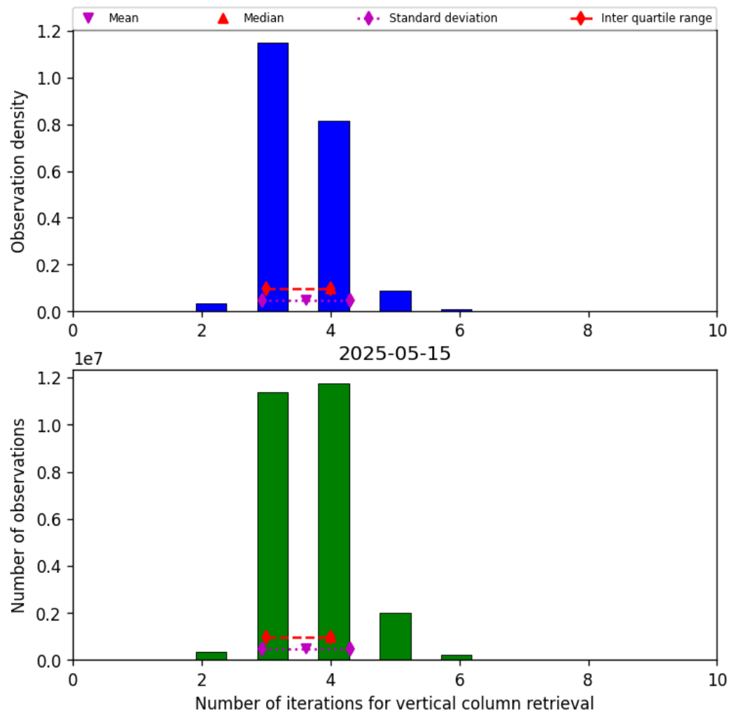
Figure 26: Histogram of “Number of iterations for vertical column retrieval” for 2025-05-15 to 2025-05-16
