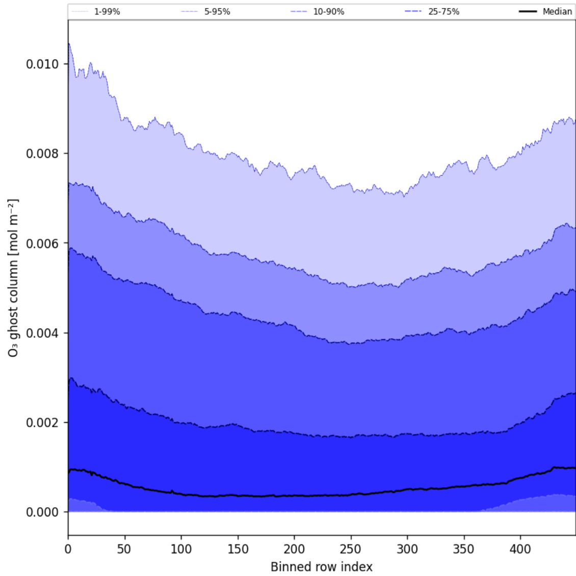
Figure 32: Along track statistics of “O 3 ghost column” for 2025-05-15 to 2025-05-16
