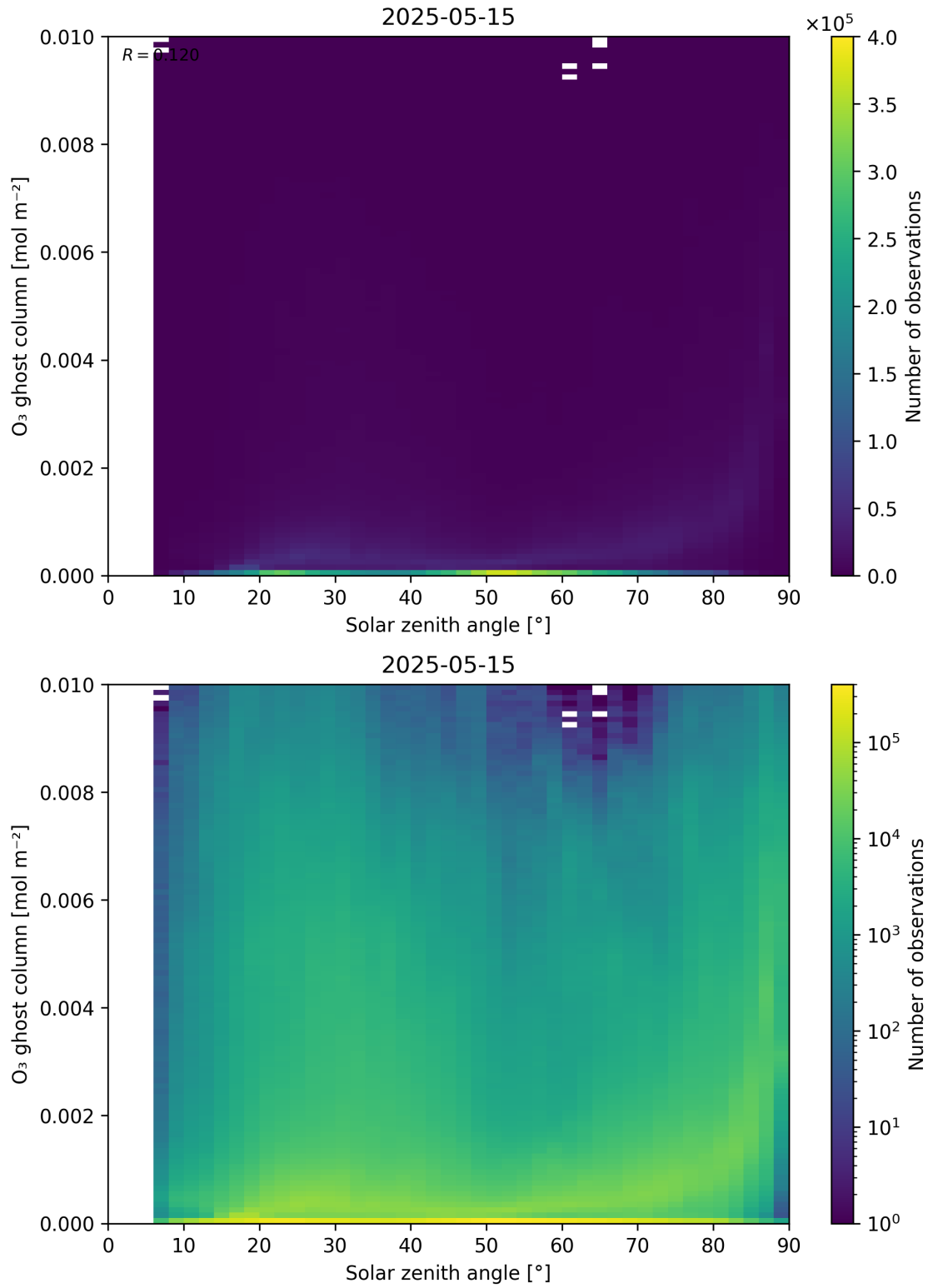
Figure 46: Scatter density plot of “Solar zenith angle” against “O 3 ghost column” for 2025-05-15 to 2025-05-16.
