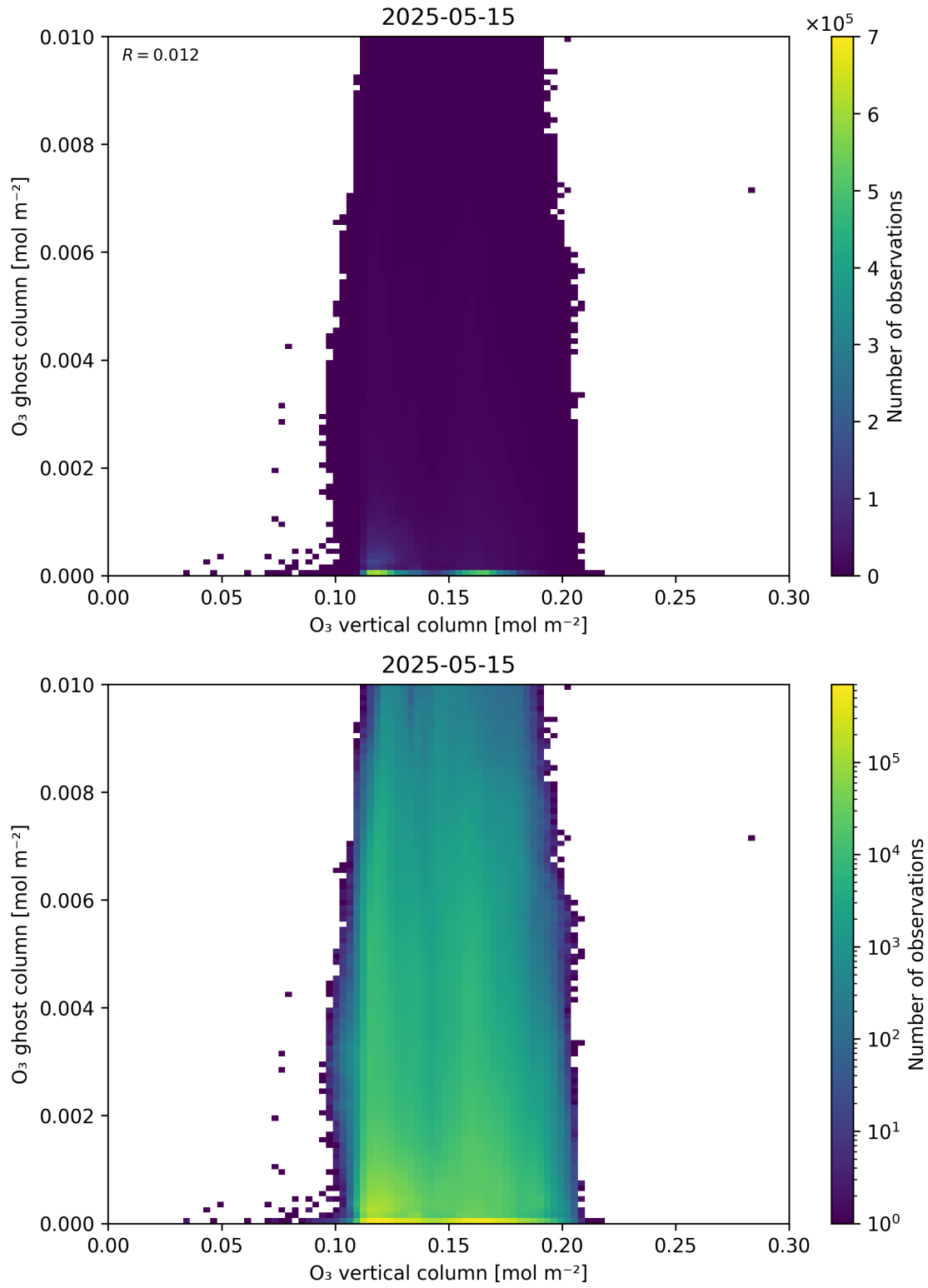
Figure 40: Scatter density plot of “O 3 vertical column” against “O 3 ghost column” for 2025-05-15 to 2025-05-16.
