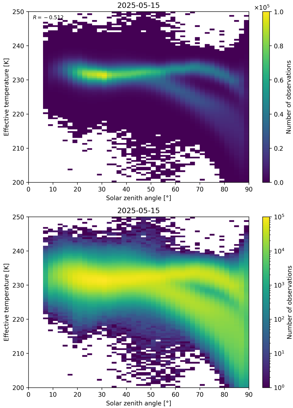
Figure 45: Scatter density plot of “Solar zenith angle” against “Effective temperature” for 2025-05-15 to 2025-05-16.
