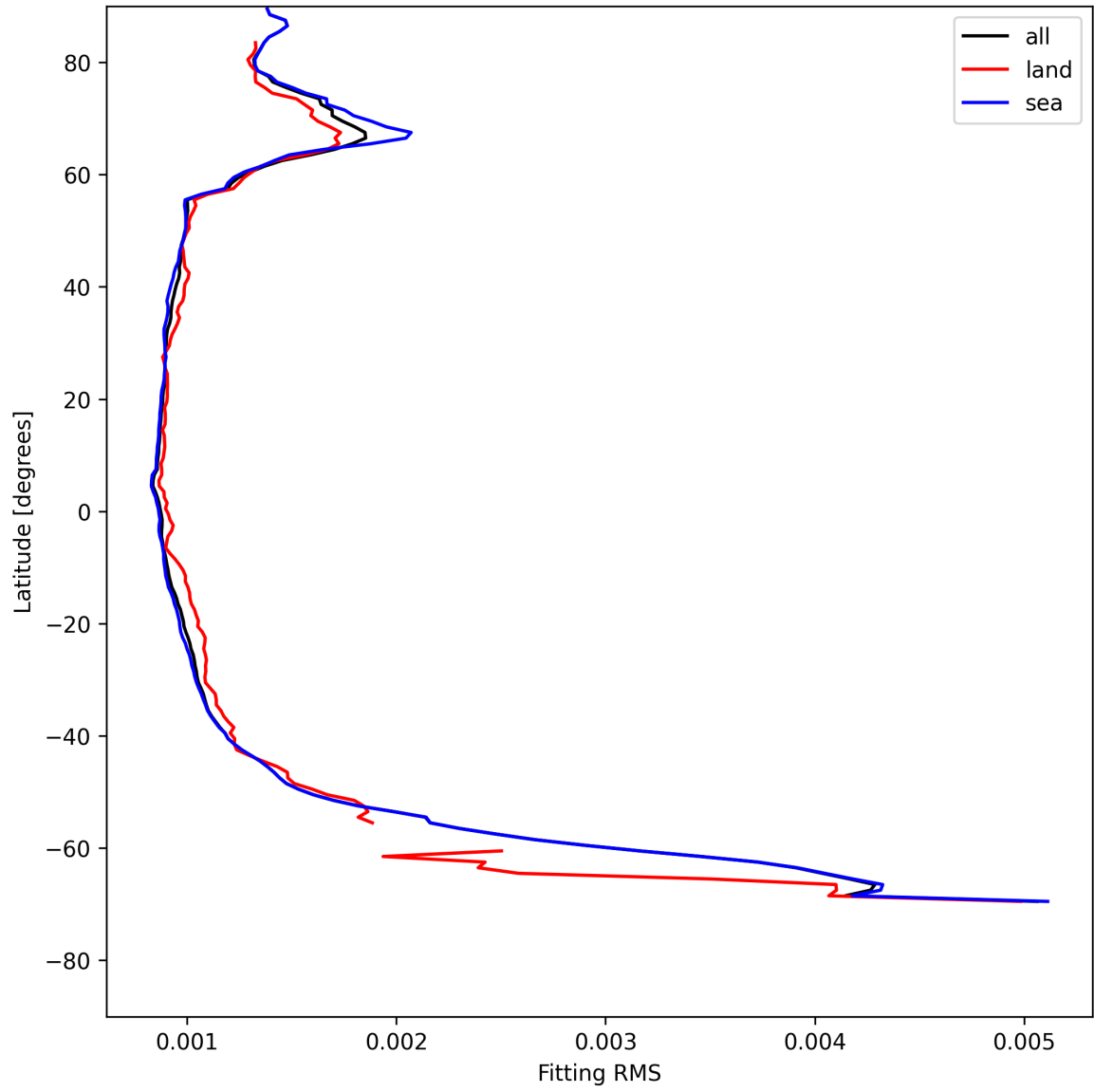
Figure 16: Zonal average of “Fitting RMS” for 2025-05-15 to 2025-05-16.
