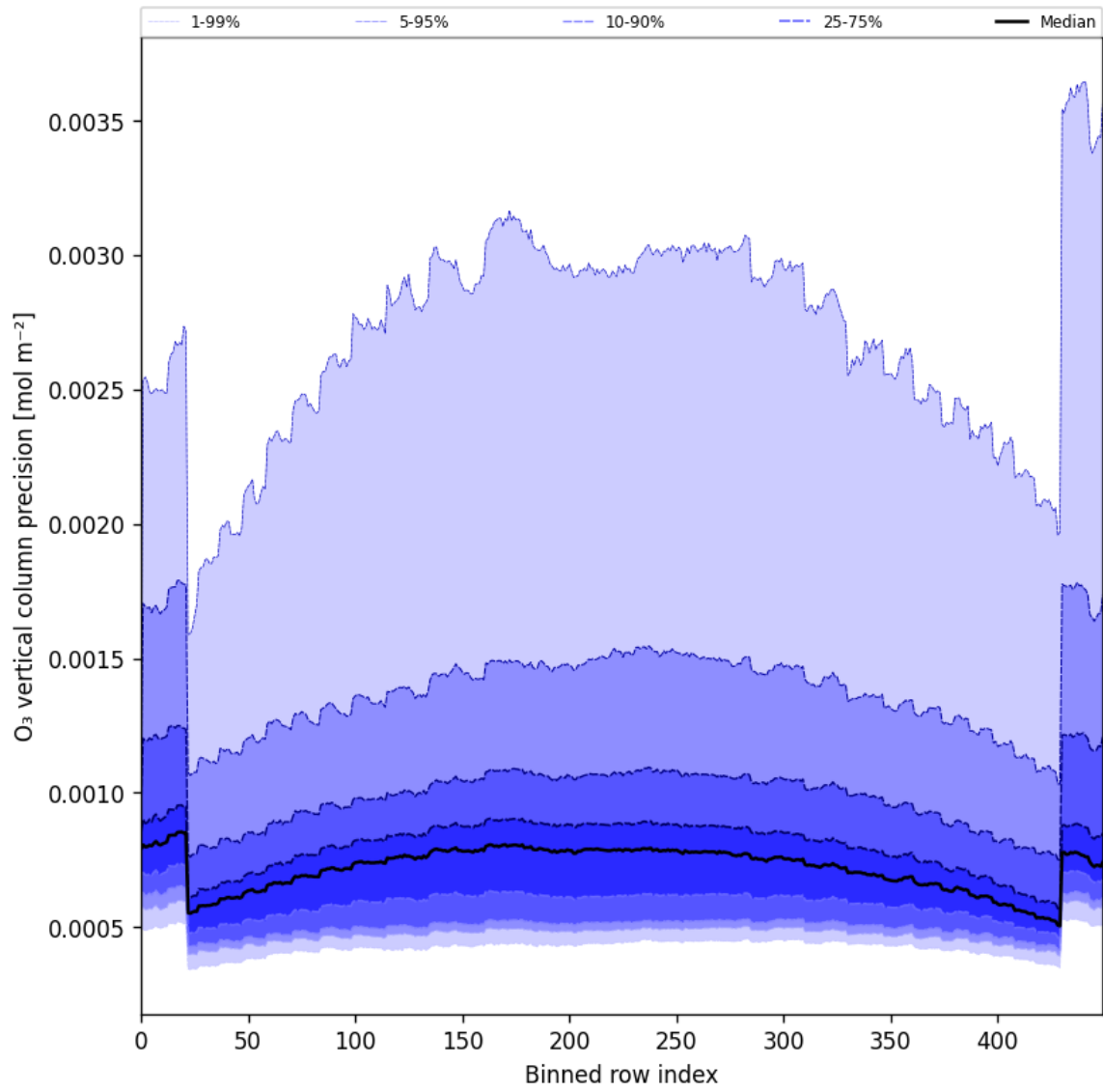
Figure 29: Along track statistics of “O 3 vertical column precision” for 2025-05-15 to 2025-05-16
