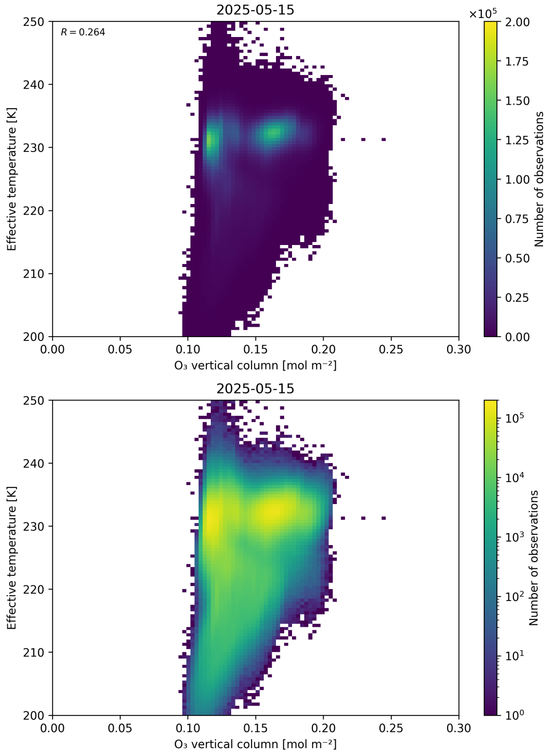
Figure 39: Scatter density plot of “O 3 vertical column” against “Effective temperature” for 2025-05-15 to 2025-05-16.
