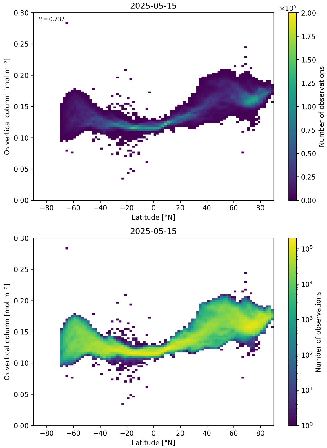
Figure 36: Scatter density plot of “Latitude” against “O 3 vertical column” for 2025-05-15 to 2025-05-16.
