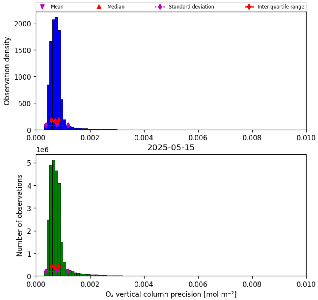
Figure 22: Histogram of “O 3 vertical column precision” for 2025-05-15 to 2025-05-16
