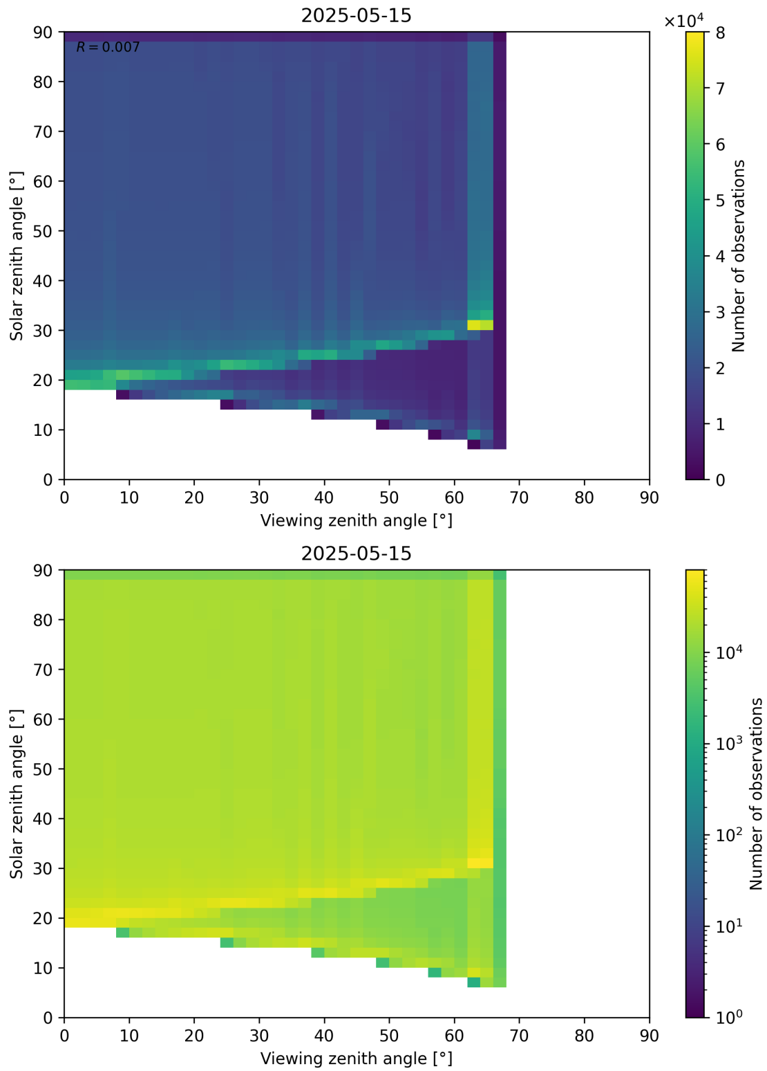
Figure 54: Scatter density plot of “Viewing zenith angle” against “Solar zenith angle” for 2025-05-15 to 2025-05-16.
