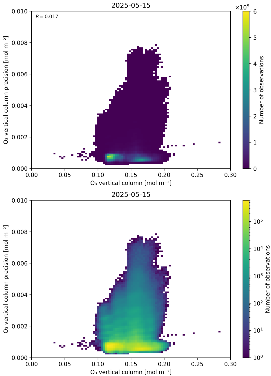
Figure 41: Scatter density plot of “O 3 vertical column” against “O 3 vertical column precision” for 2025-05-15 to 2025-05-16.
