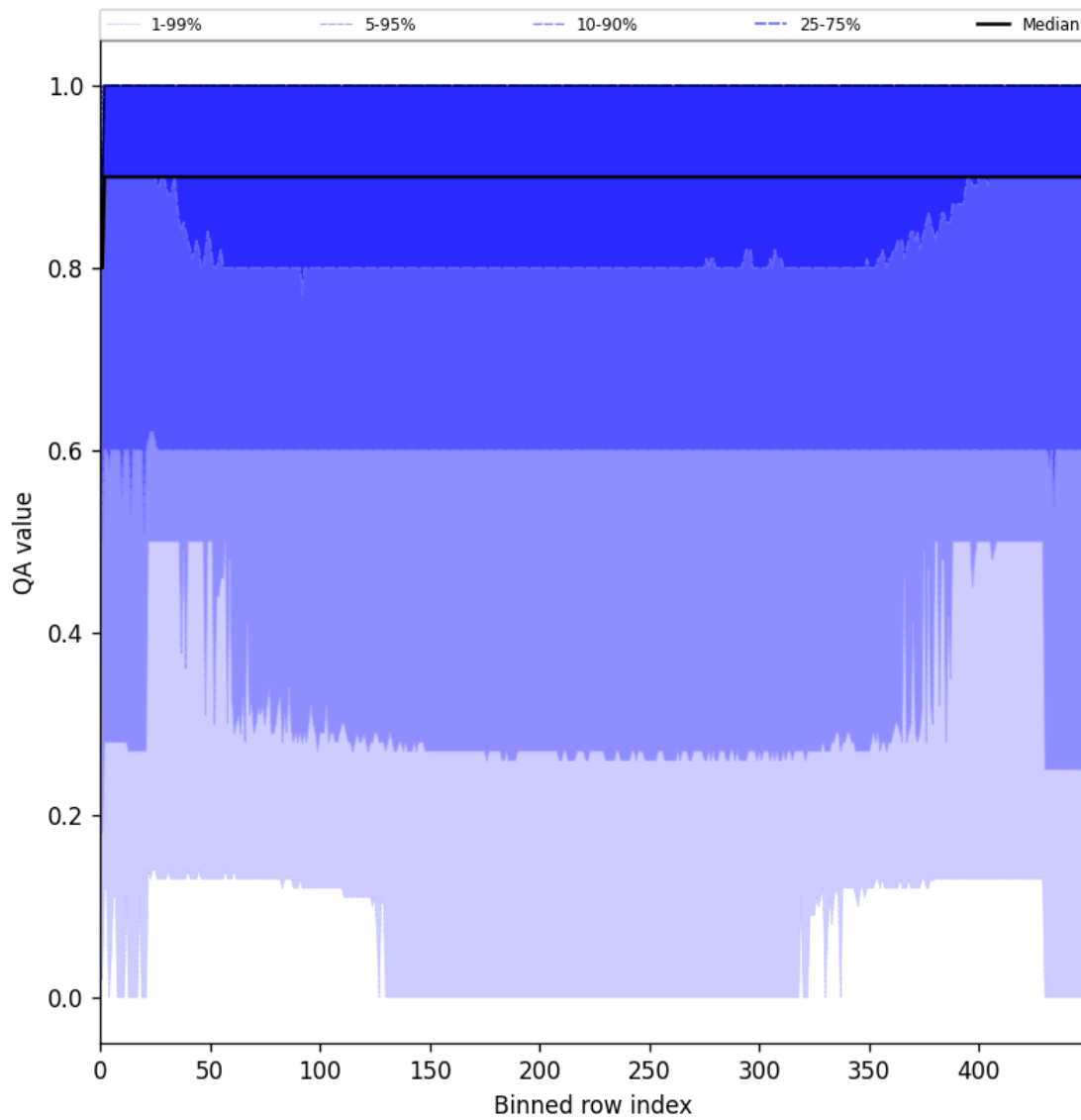
Figure 27: Along track statistics of “QA value” for 2025-05-15 to 2025-05-16
