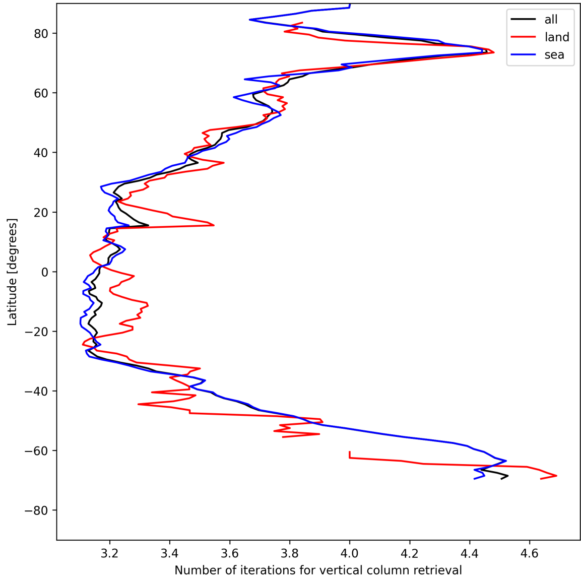
Figure 19: Zonal average of “Number of iterations for vertical column retrieval” for 2025-05-15 to 2025-05-16.
