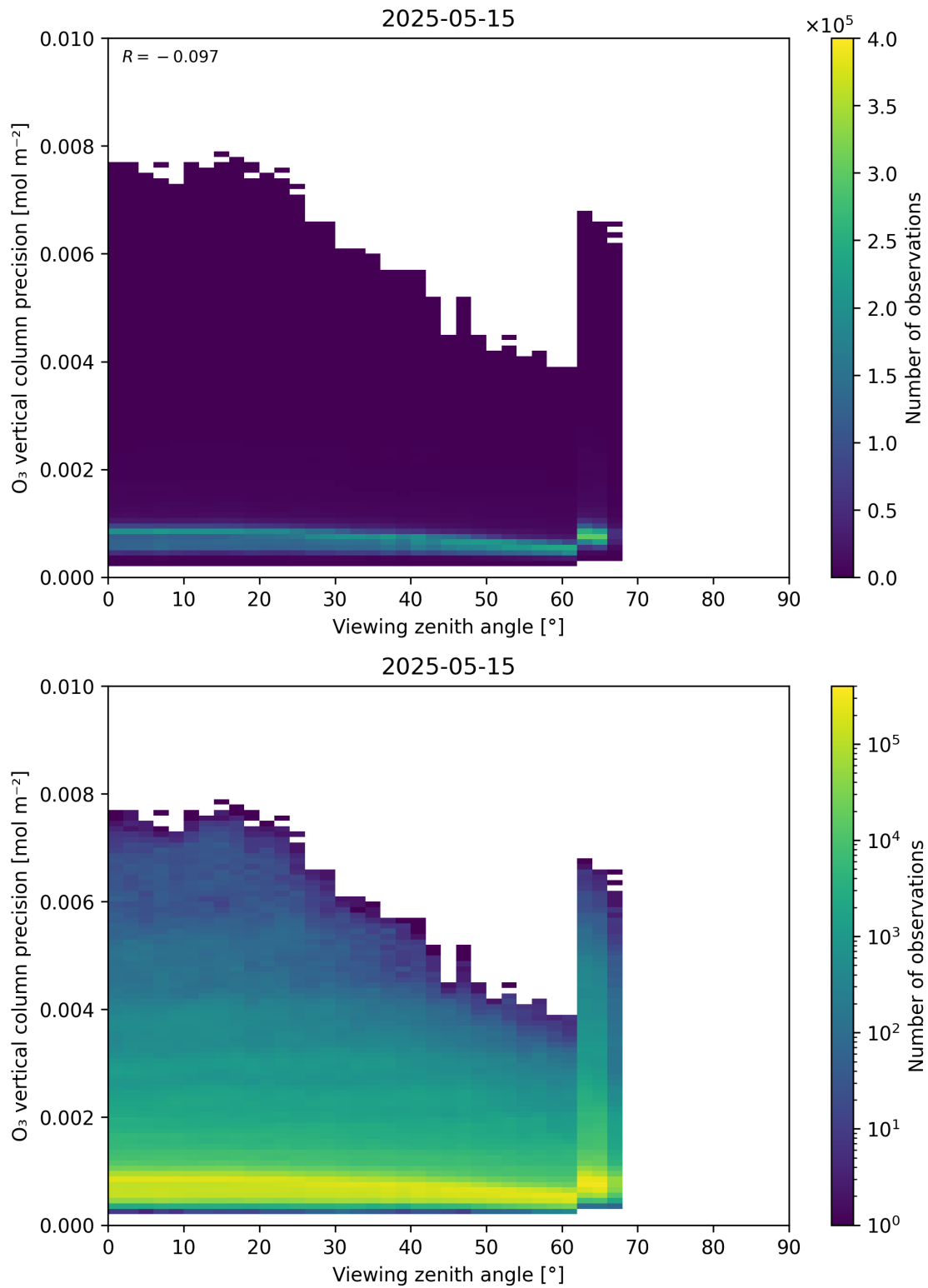
Figure 53: Scatter density plot of “Viewing zenith angle” against “O 3 vertical column precision” for 2025-05-15 to 2025-05-16.
