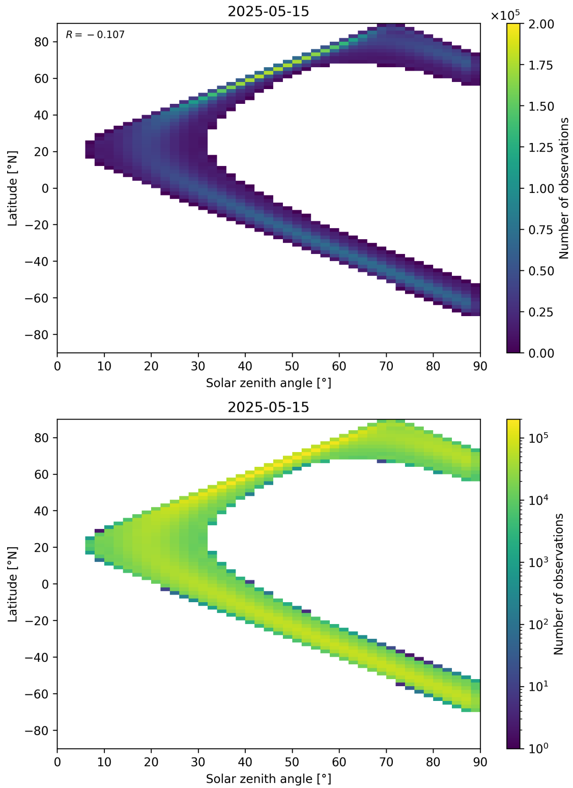
Figure 44: Scatter density plot of “Solar zenith angle” against “Latitude” for 2025-05-15 to 2025-05-16.
