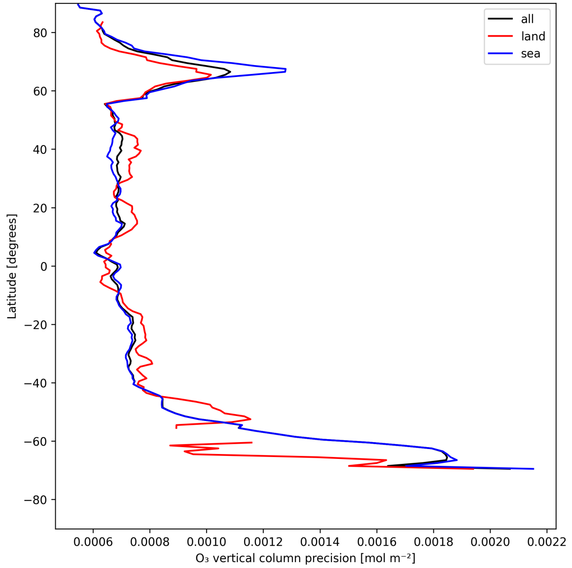
Figure 15: Zonal average of “O 3 vertical column precision” for 2025-05-15 to 2025-05-16.
