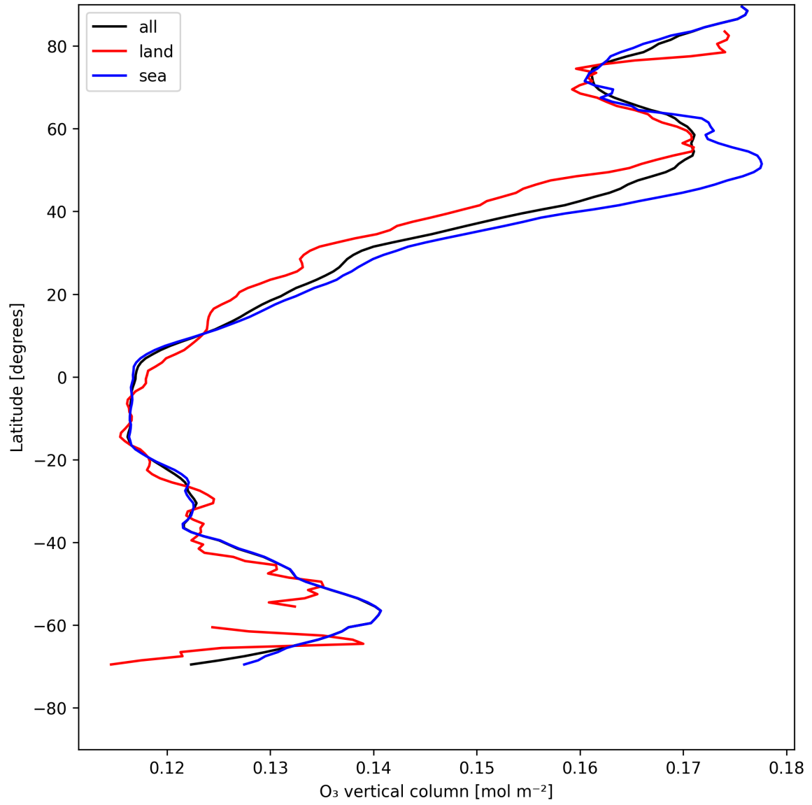
Figure 14: Zonal average of “O 3 vertical column” for 2025-05-15 to 2025-05-16.
