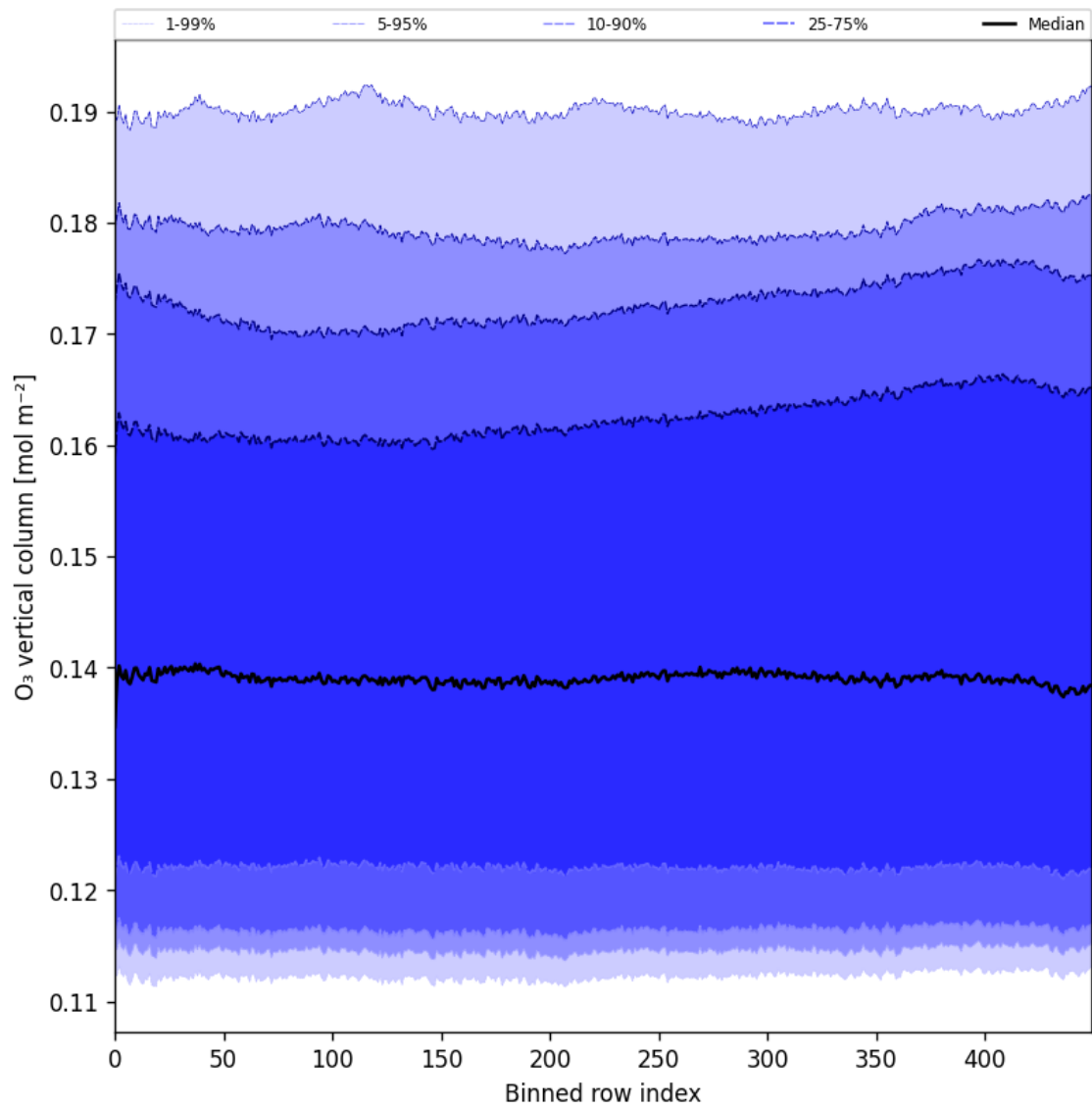
Figure 28: Along track statistics of “O 3 vertical column” for 2025-05-15 to 2025-05-16
