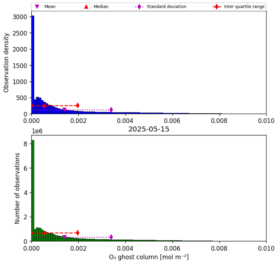
Figure 25: Histogram of “O 3 ghost column” for 2025-05-15 to 2025-05-16
