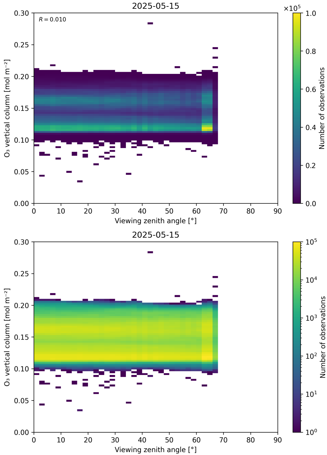
Figure 52: Scatter density plot of “Viewing zenith angle” against “O 3 vertical column” for 2025-05-15 to 2025-05-16.
