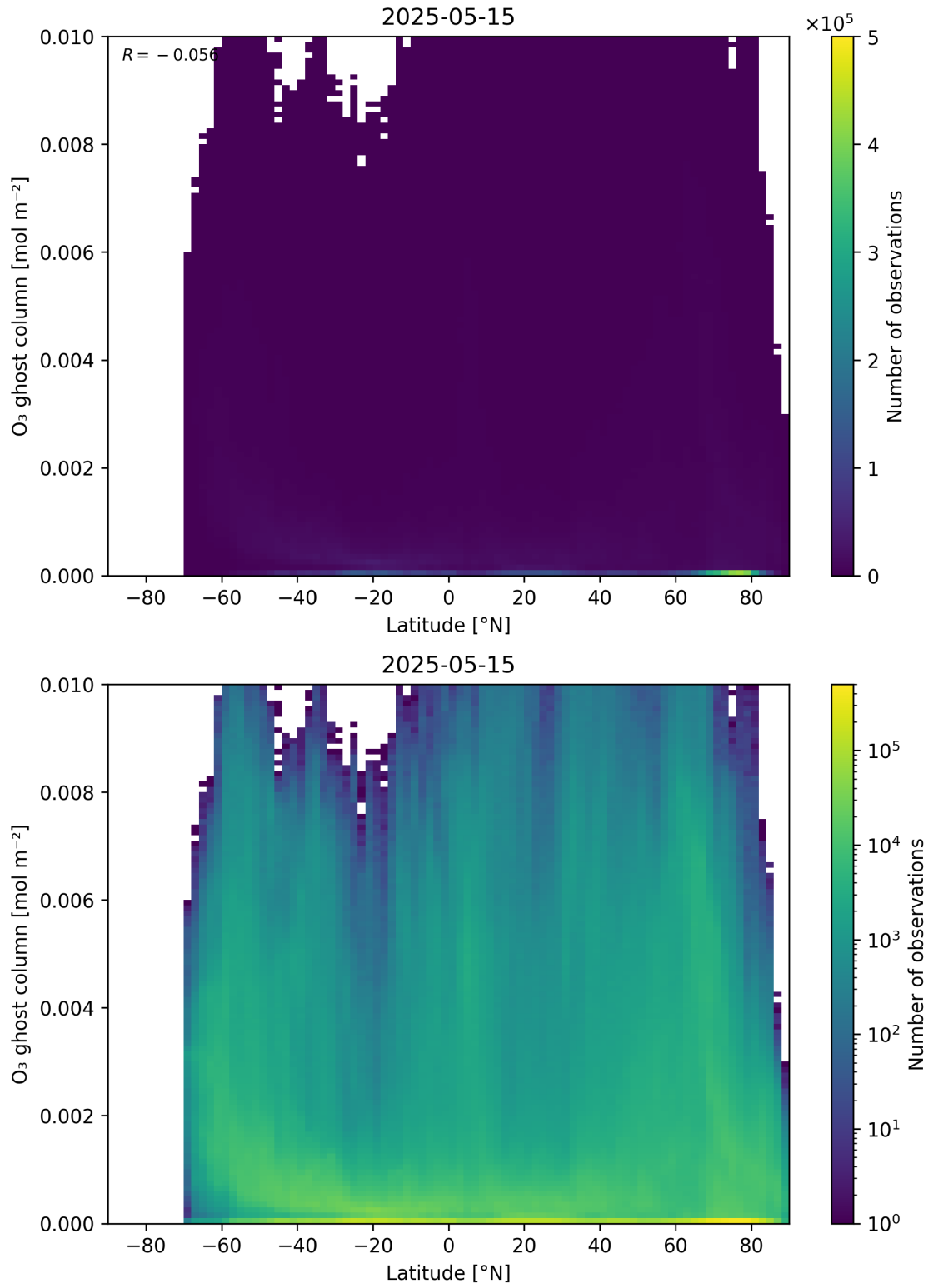
Figure 35: Scatter density plot of “Latitude” against “O 3 ghost column” for 2025-05-15 to 2025-05-16.
