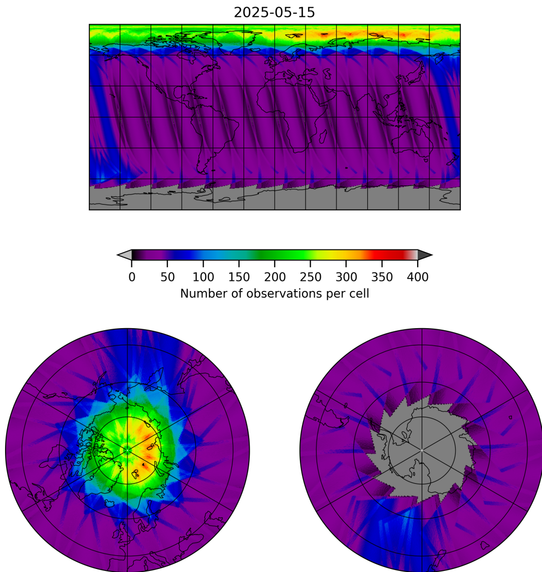
Figure 12: Map of the number of observations for 2025-05-15 to 2025-05-16
