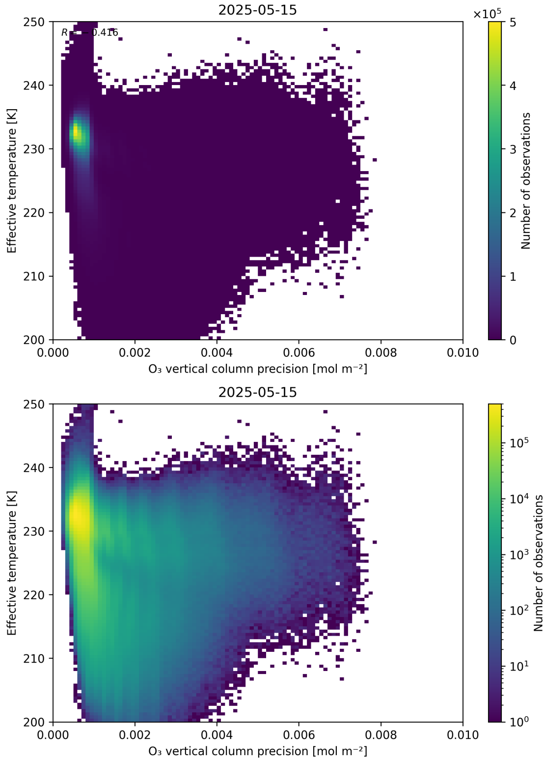
Figure 42: Scatter density plot of “O 3 vertical column precision” against “Effective temperature” for 2025-05-15 to 2025-05-16.
