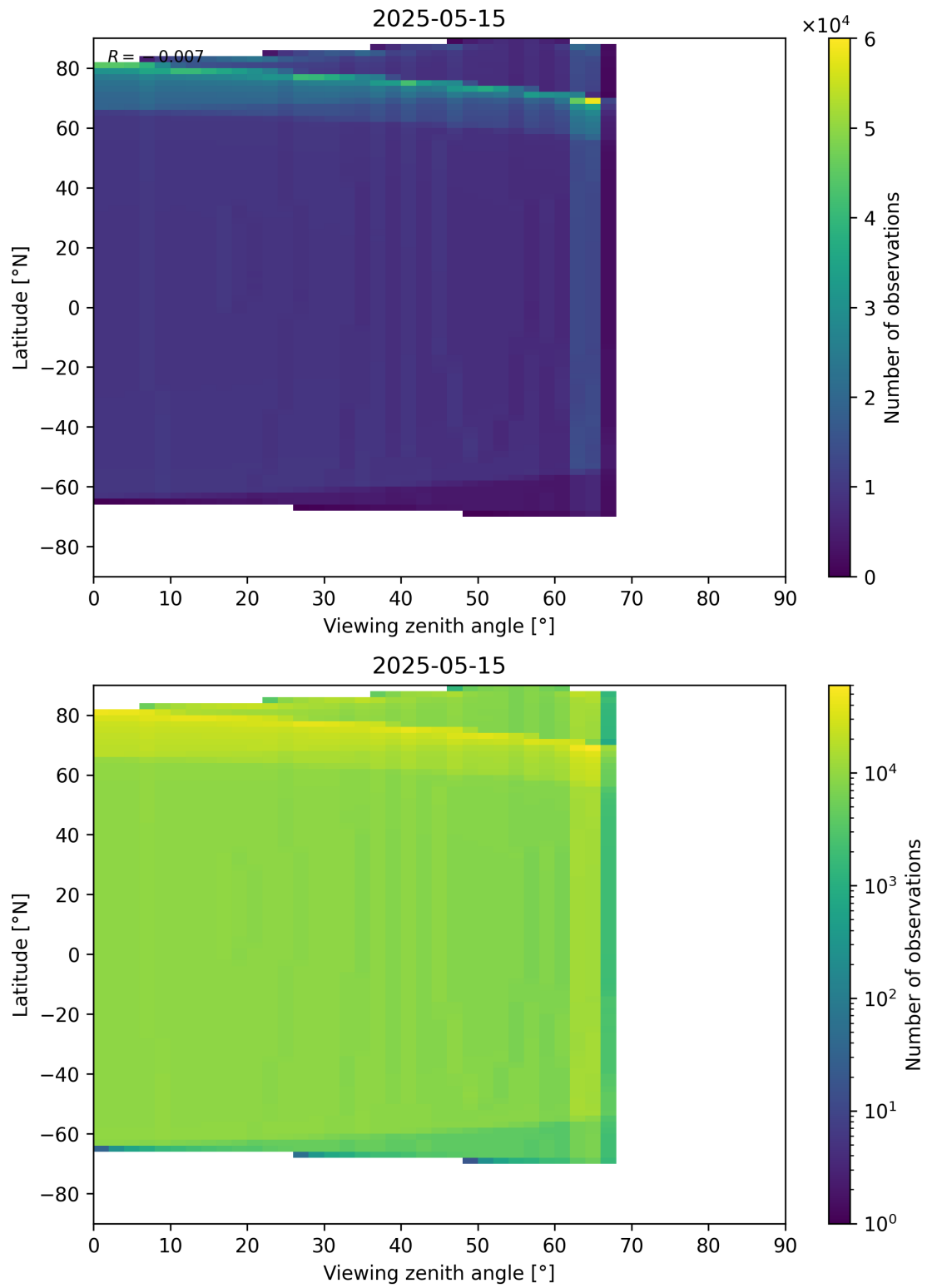
Figure 49: Scatter density plot of “Viewing zenith angle” against “Latitude” for 2025-05-15 to 2025-05-16.
