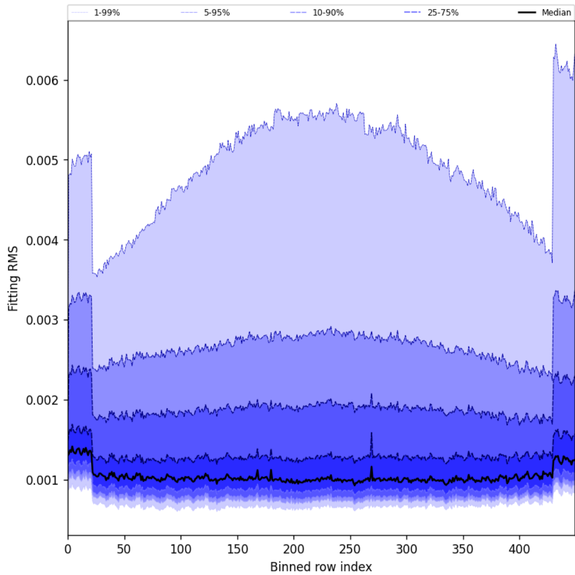
Figure 30: Along track statistics of “Fitting RMS” for 2025-05-15 to 2025-05-16
