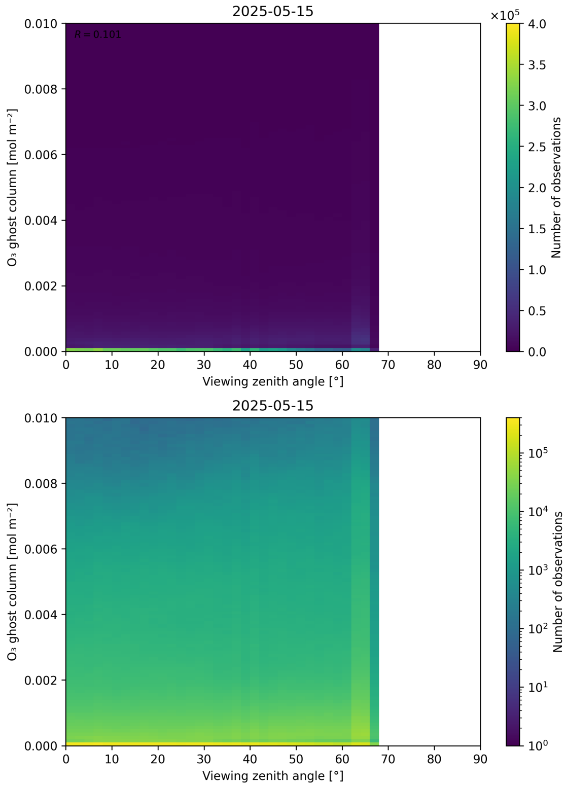
Figure 51: Scatter density plot of “Viewing zenith angle” against “O 3 ghost column” for 2025-05-15 to 2025-05-16.
