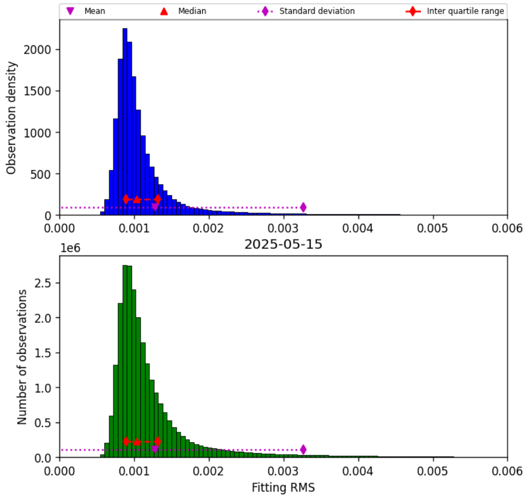
Figure 23: Histogram of “Fitting RMS” for 2025-05-15 to 2025-05-16
