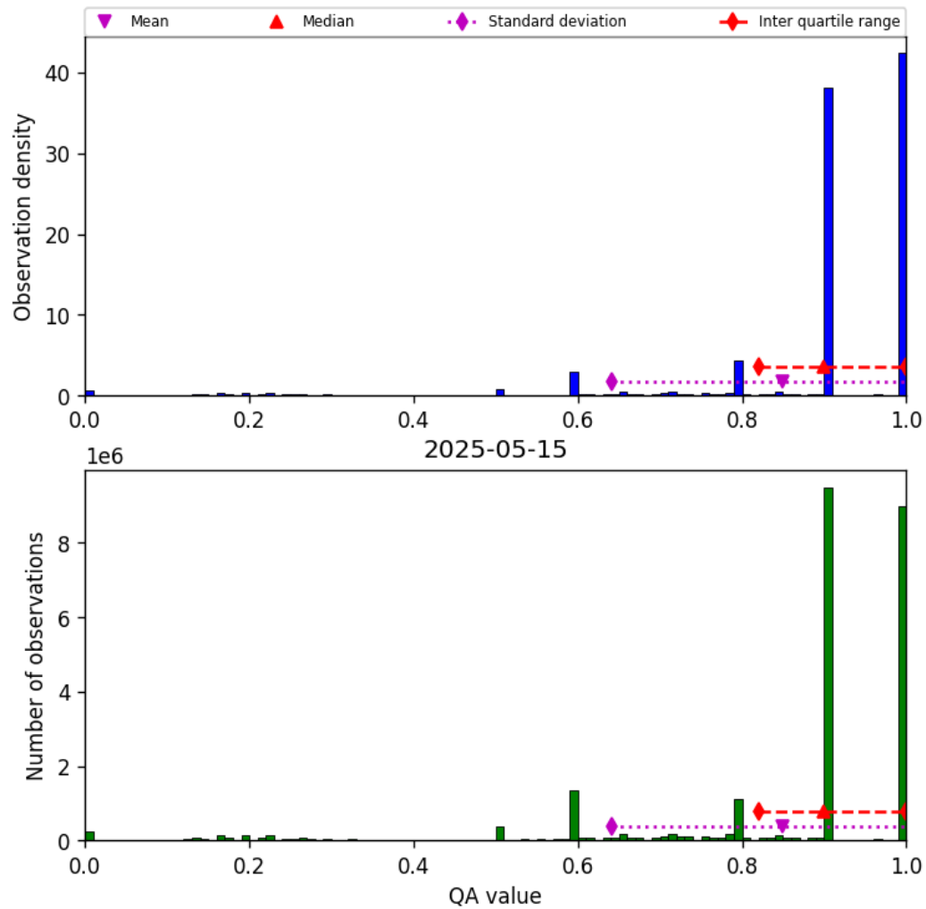
Figure 20: Histogram of “QA value” for 2025-05-15 to 2025-05-16
