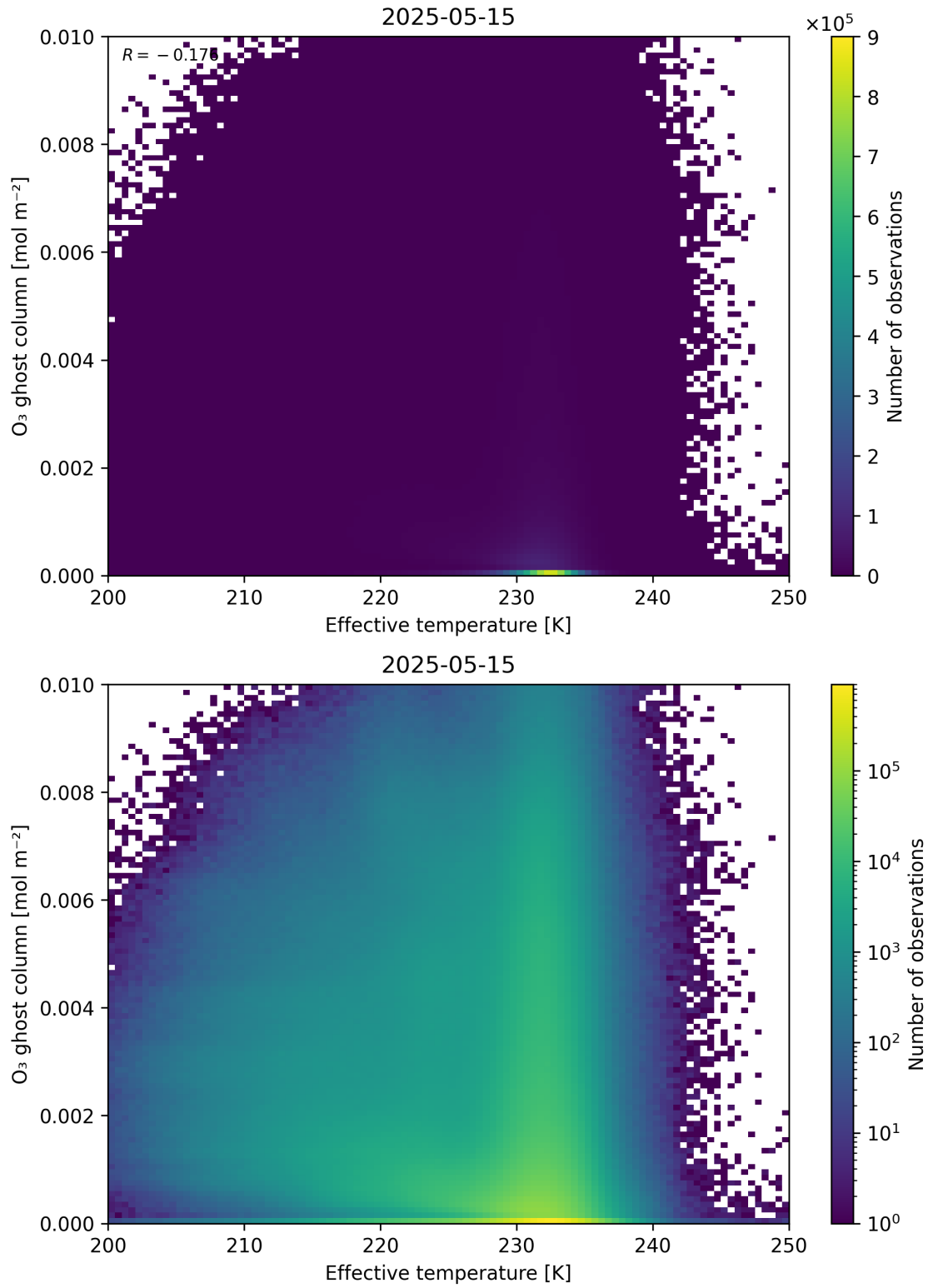
Figure 38: Scatter density plot of “Effective temperature” against “O 3 ghost column” for 2025-05-15 to 2025-05-16.
