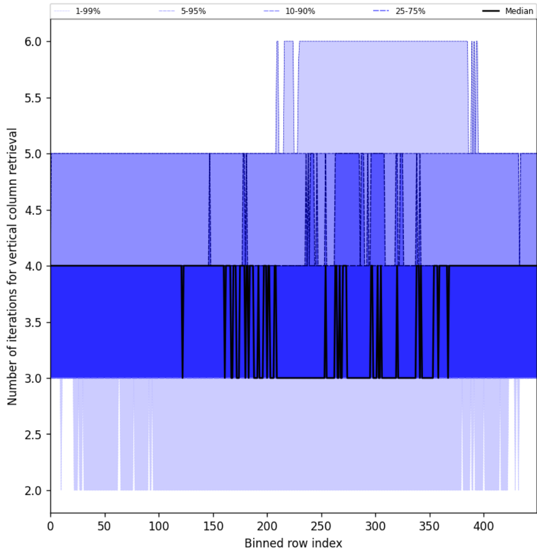
Figure 33: Along track statistics of “Number of iterations for vertical column retrieval” for 2025-05-15 to 2025-05-16
