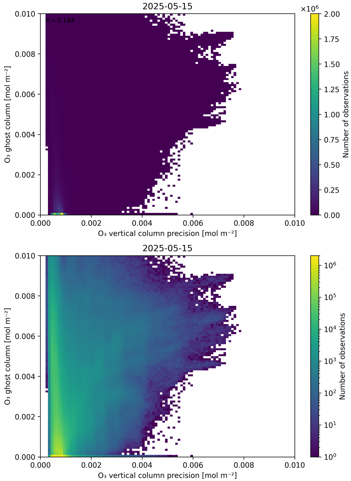
Figure 43: Scatter density plot of “O 3 vertical column precision” against “O 3 ghost column” for 2025-05-15 to 2025-05-16.
