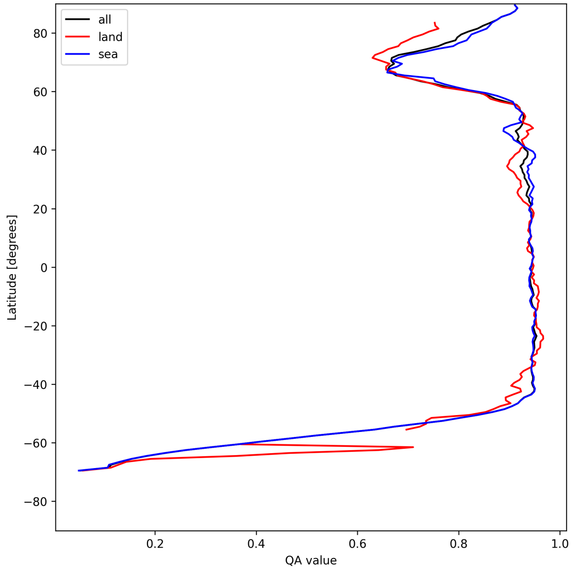
Figure 13: Zonal average of “QA value” for 2025-05-15 to 2025-05-16.
