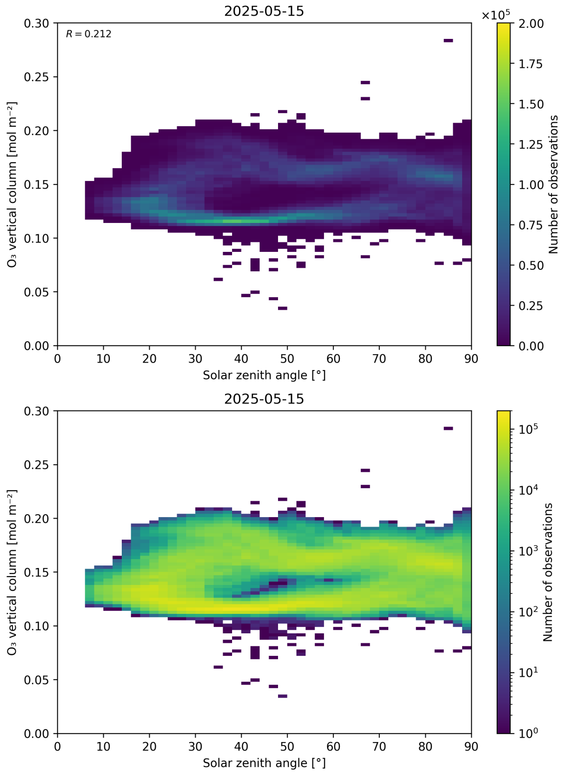
Figure 47: Scatter density plot of “Solar zenith angle” against “O 3 vertical column” for 2025-05-15 to 2025-05-16.
