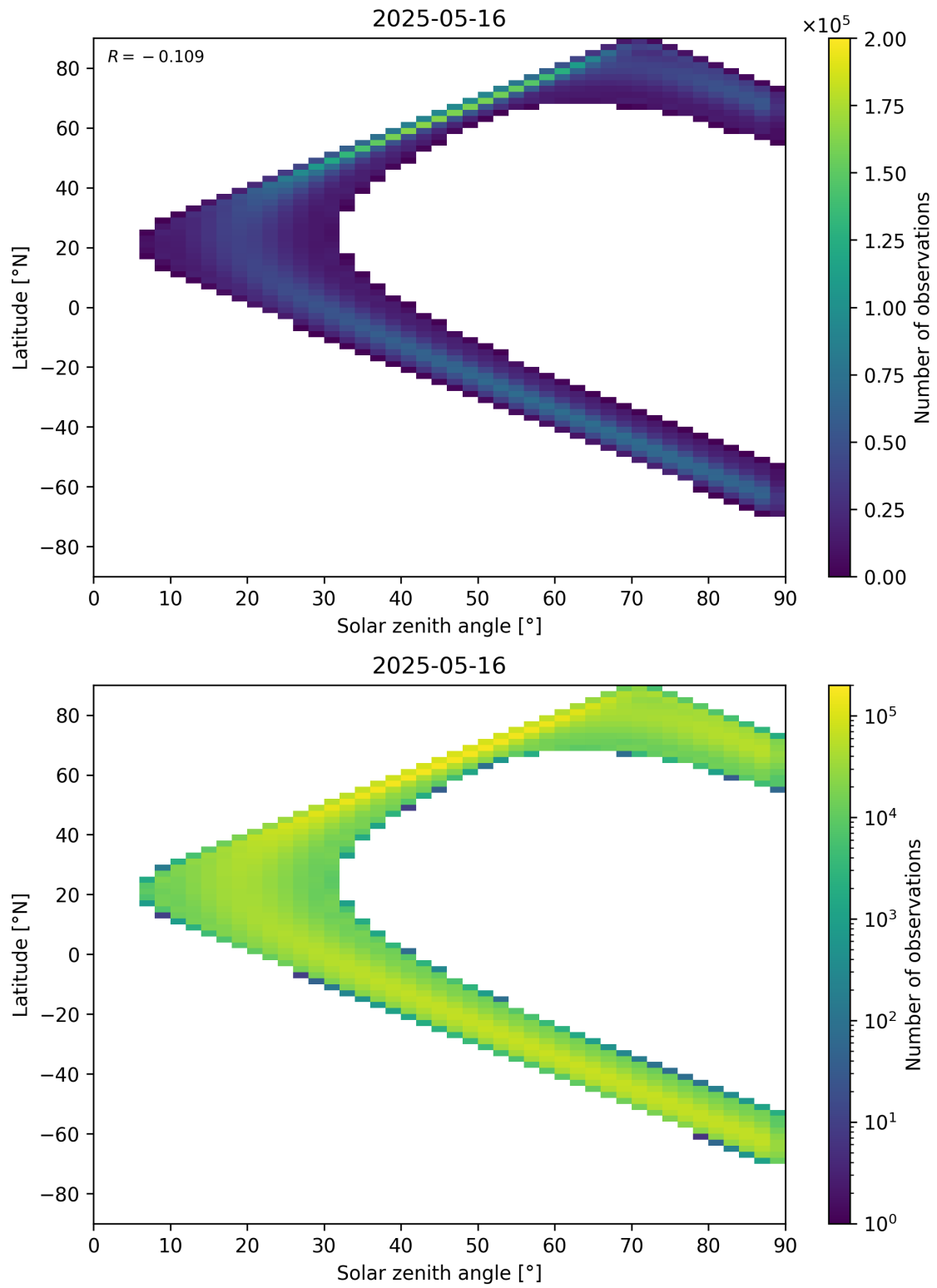
Figure 44: Scatter density plot of “Solar zenith angle” against “Latitude” for 2025-05-15 to 2025-05-17.
