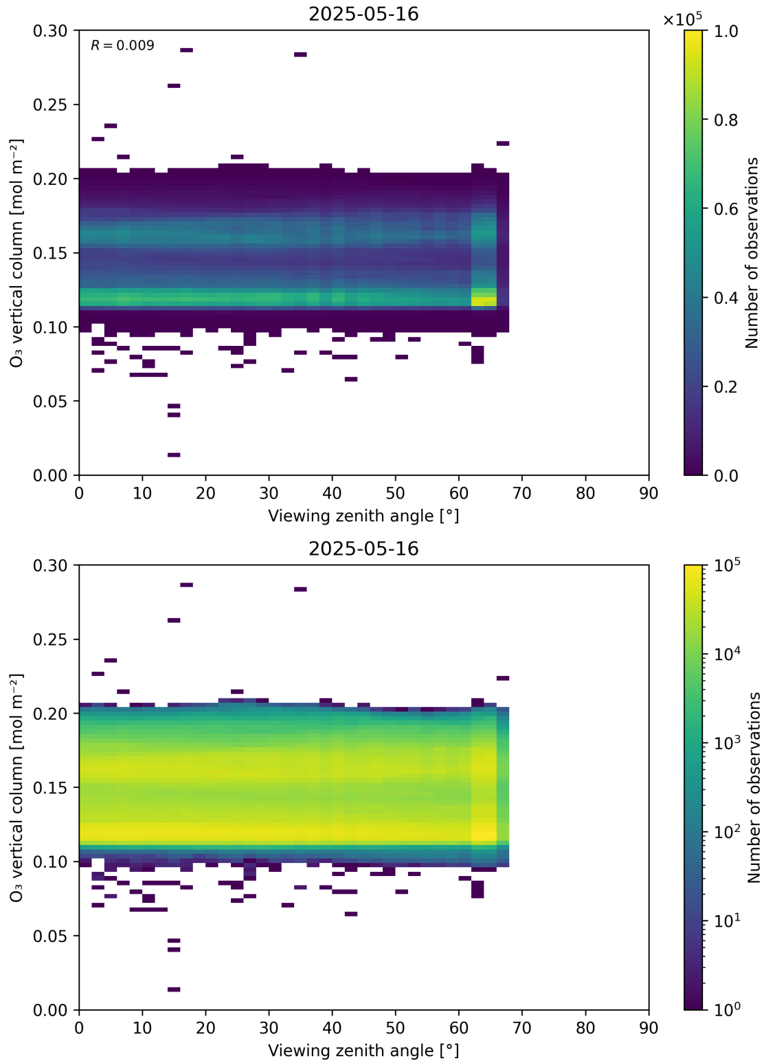
Figure 52: Scatter density plot of “Viewing zenith angle” against “O 3 vertical column” for 2025-05-15 to 2025-05-17.
