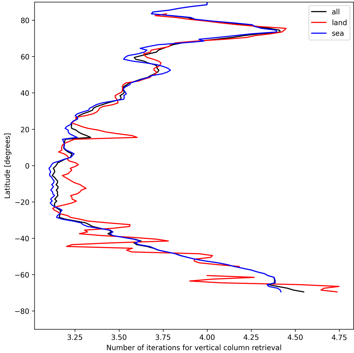
Figure 19: Zonal average of “Number of iterations for vertical column retrieval” for 2025-05-15 to 2025-05-17.
