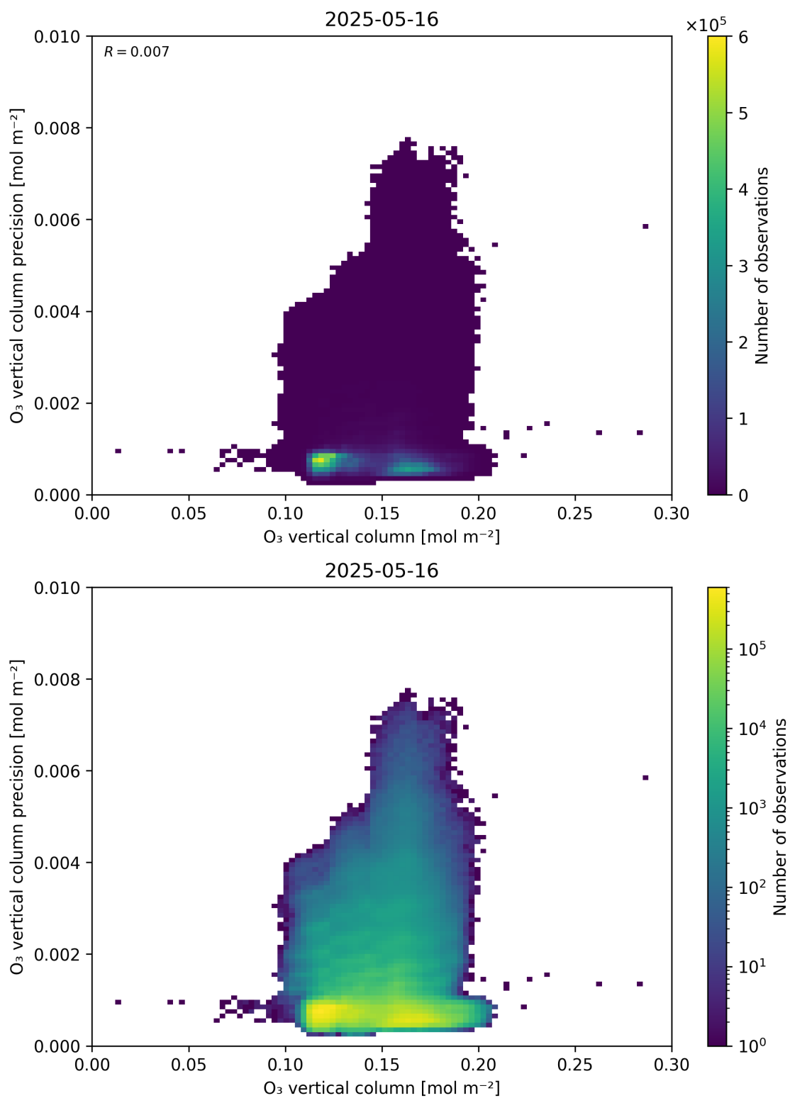
Figure 41: Scatter density plot of “O 3 vertical column” against “O 3 vertical column precision” for 2025-05-15 to 2025-05-17.
