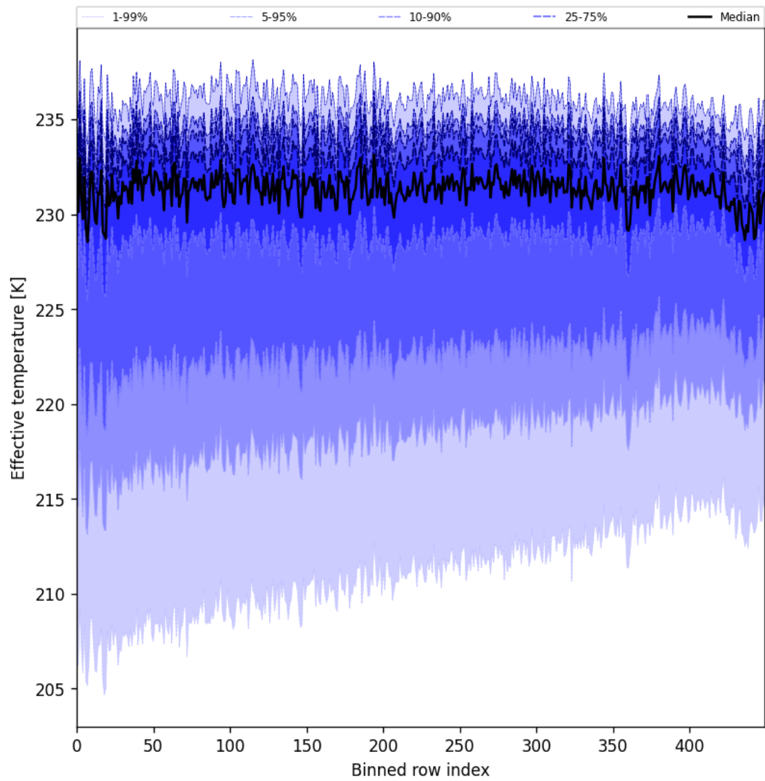
Figure 31: Along track statistics of “Effective temperature” for 2025-05-15 to 2025-05-17
