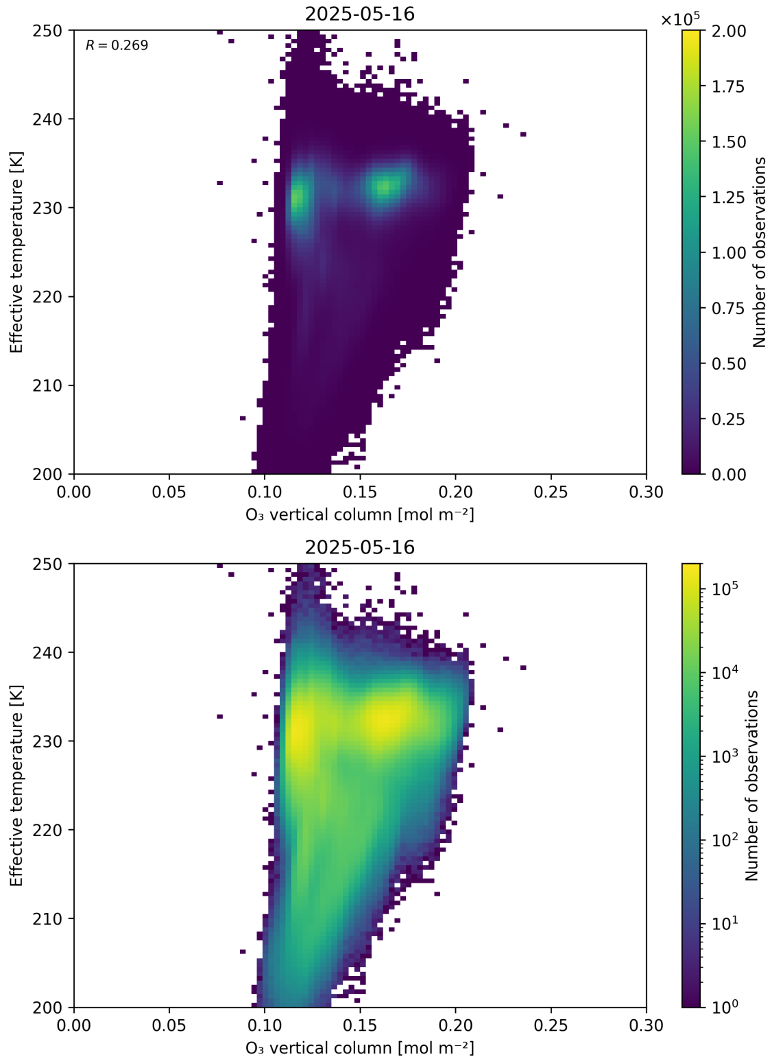
Figure 39: Scatter density plot of “O 3 vertical column” against “Effective temperature” for 2025-05-15 to 2025-05-17.
