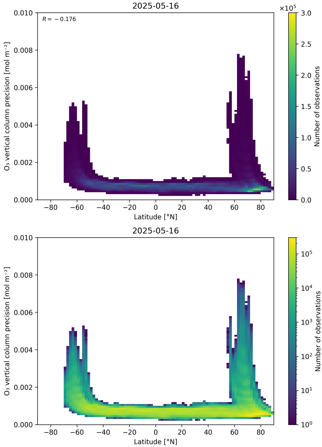
Figure 37: Scatter density plot of “Latitude” against “O 3 vertical column precision” for 2025-05-15 to 2025-05-17.
