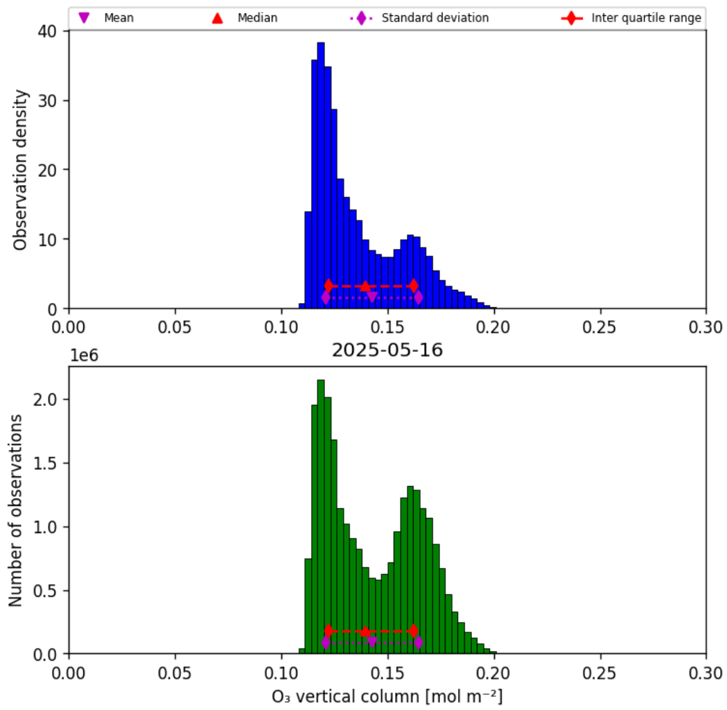
Figure 21: Histogram of “O 3 vertical column” for 2025-05-15 to 2025-05-17
