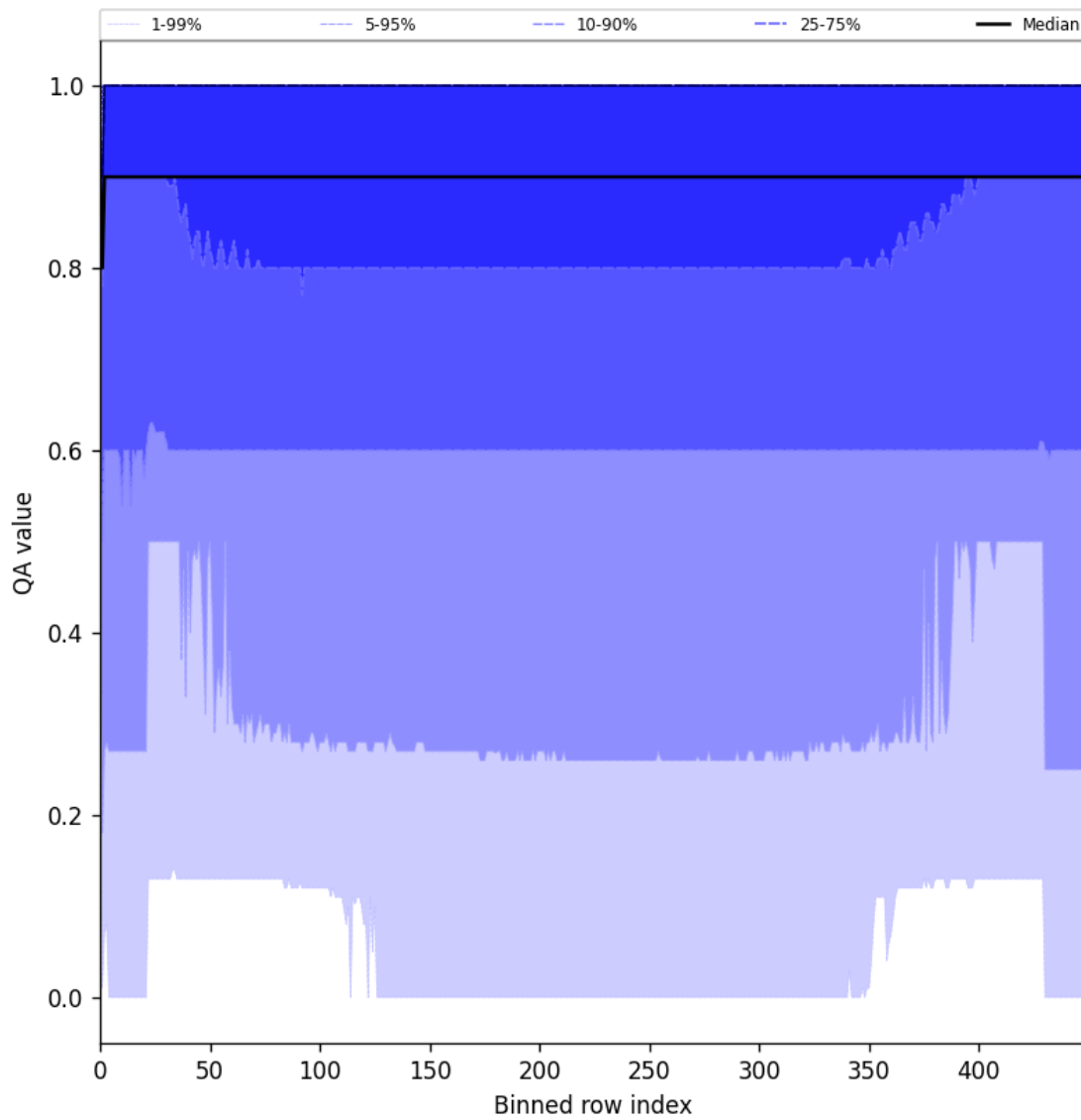
Figure 27: Along track statistics of “QA value” for 2025-05-15 to 2025-05-17
