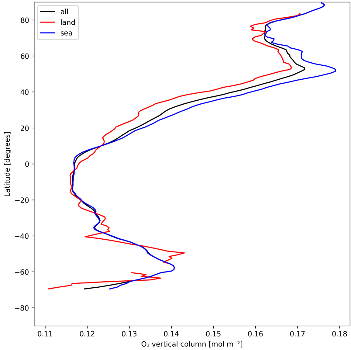
Figure 14: Zonal average of “O 3 vertical column” for 2025-05-15 to 2025-05-17.
