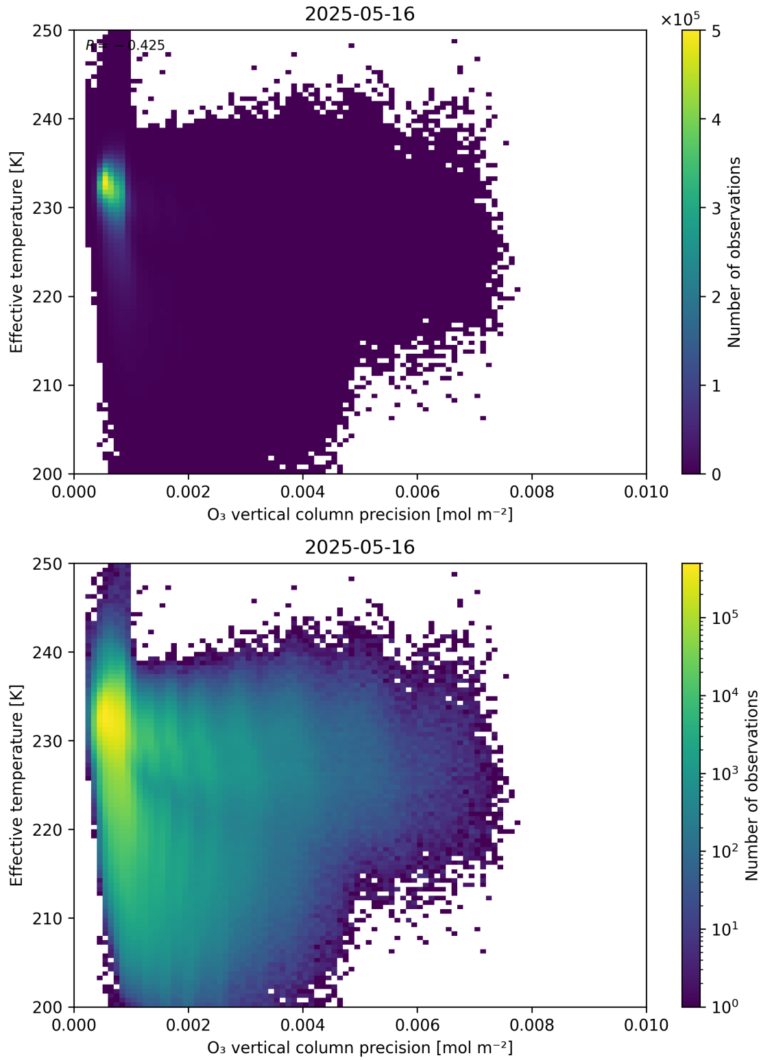
Figure 42: Scatter density plot of “O 3 vertical column precision” against “Effective temperature” for 2025-05-15 to 2025-05-17.
