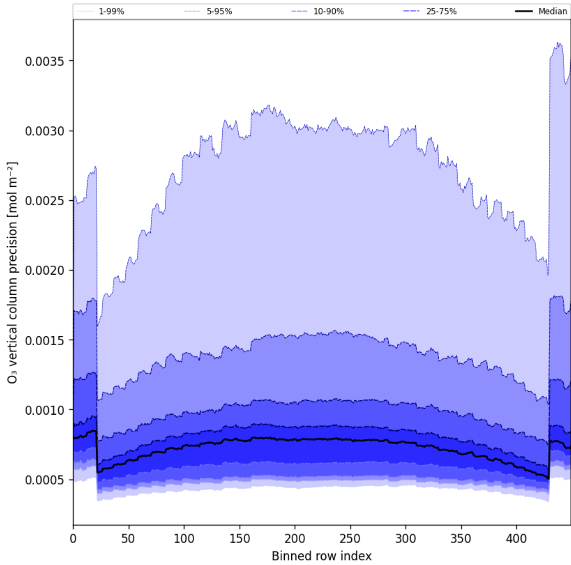
Figure 29: Along track statistics of “O 3 vertical column precision” for 2025-05-15 to 2025-05-17
