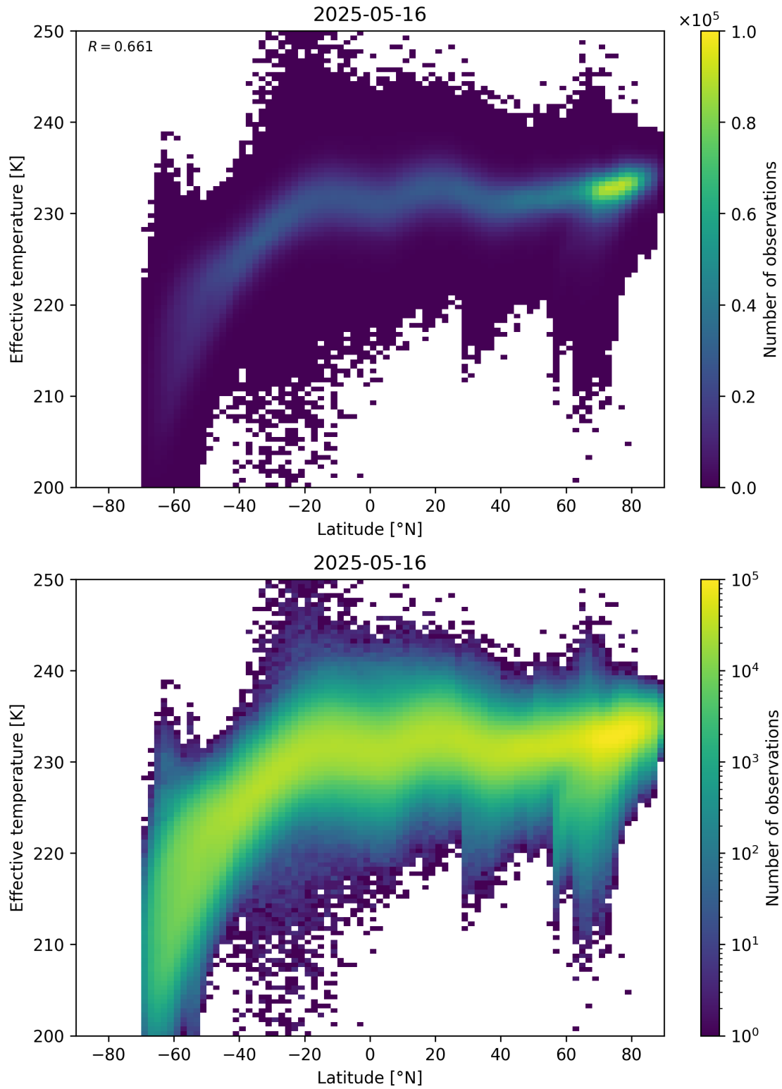
Figure 34: Scatter density plot of “Latitude” against “Effective temperature” for 2025-05-15 to 2025-05-17.
