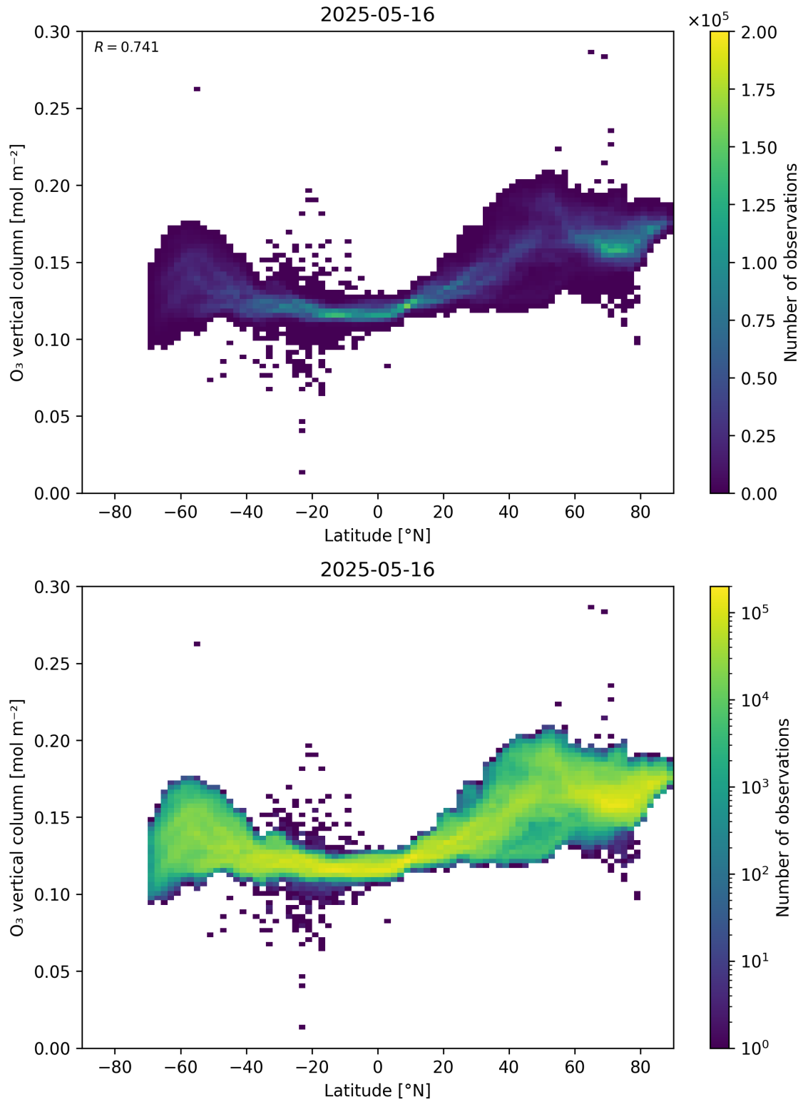
Figure 36: Scatter density plot of “Latitude” against “O 3 vertical column” for 2025-05-15 to 2025-05-17.
