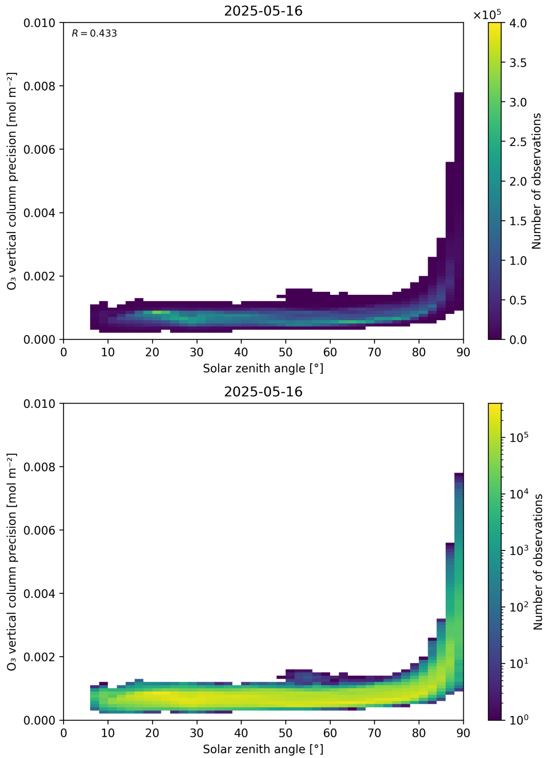
Figure 48: Scatter density plot of “Solar zenith angle” against “O 3 vertical column precision” for 2025-05-15 to 2025-05-17.
