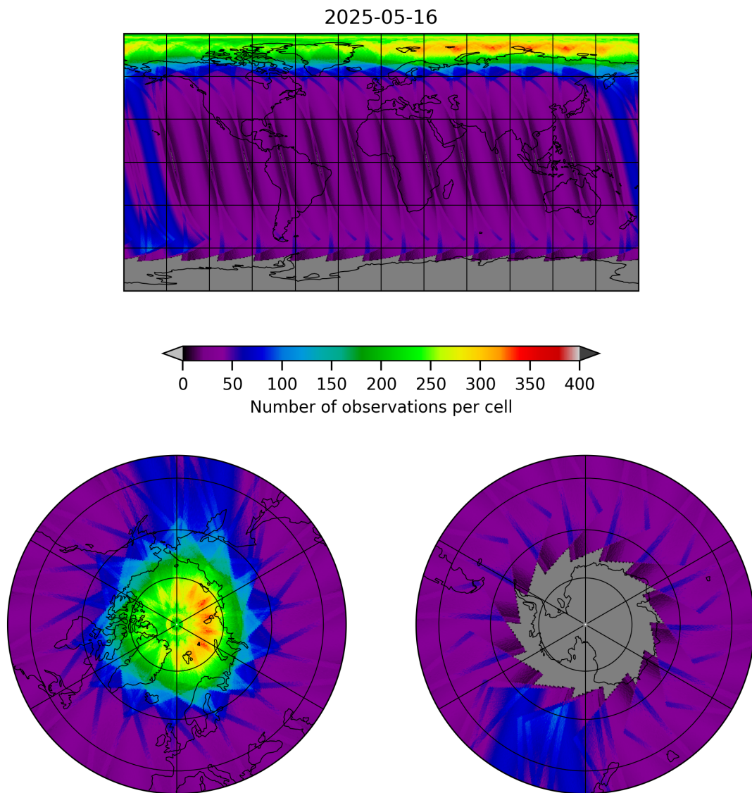
Figure 12: Map of the number of observations for 2025-05-15 to 2025-05-17
