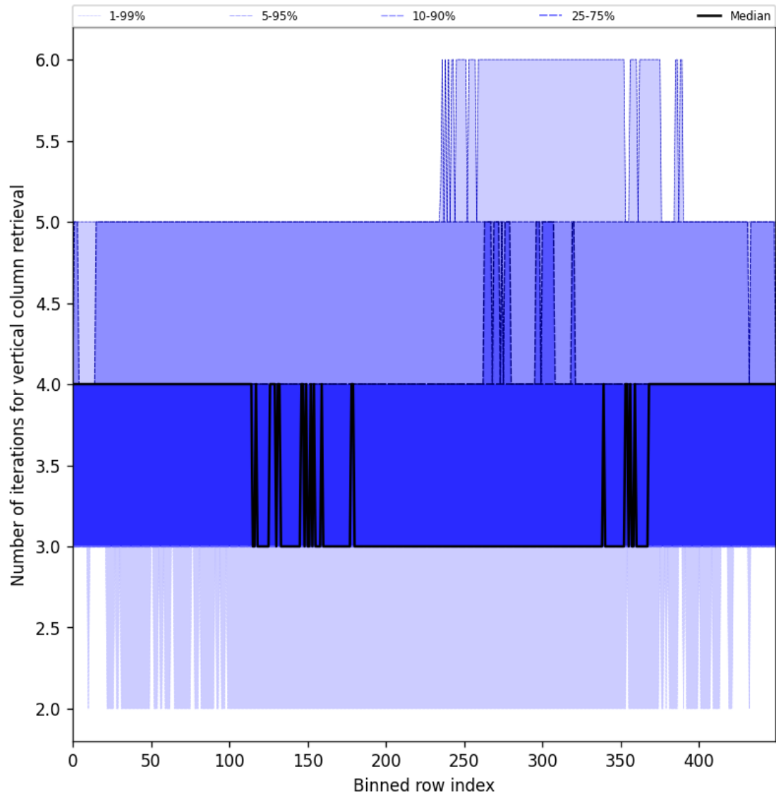
Figure 33: Along track statistics of “Number of iterations for vertical column retrieval” for 2025-05-15 to 2025-05-17
