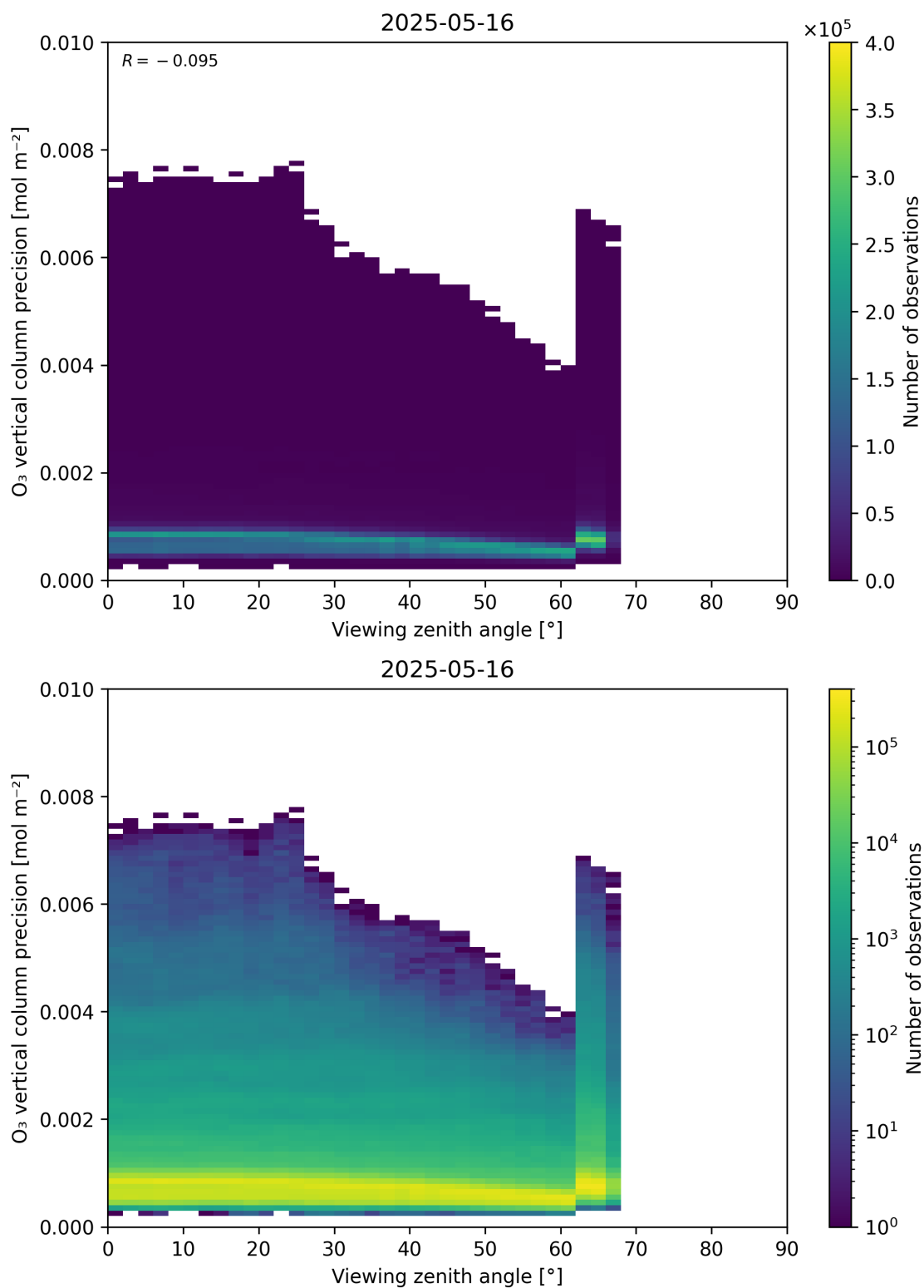
Figure 53: Scatter density plot of “Viewing zenith angle” against “O 3 vertical column precision” for 2025-05-15 to 2025-05-17.
