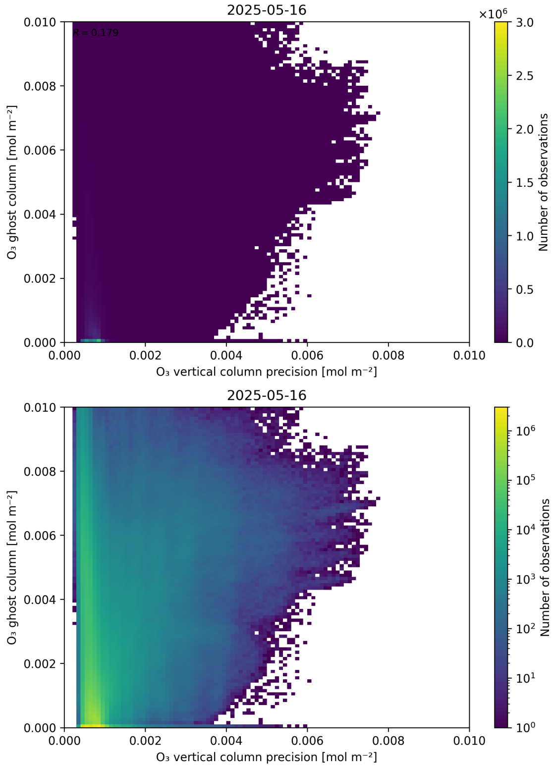
Figure 43: Scatter density plot of “ \text{O}_3 vertical column precision” against “ \text{O}_3 ghost column” for 2025-05-15 to 2025-05-17.
