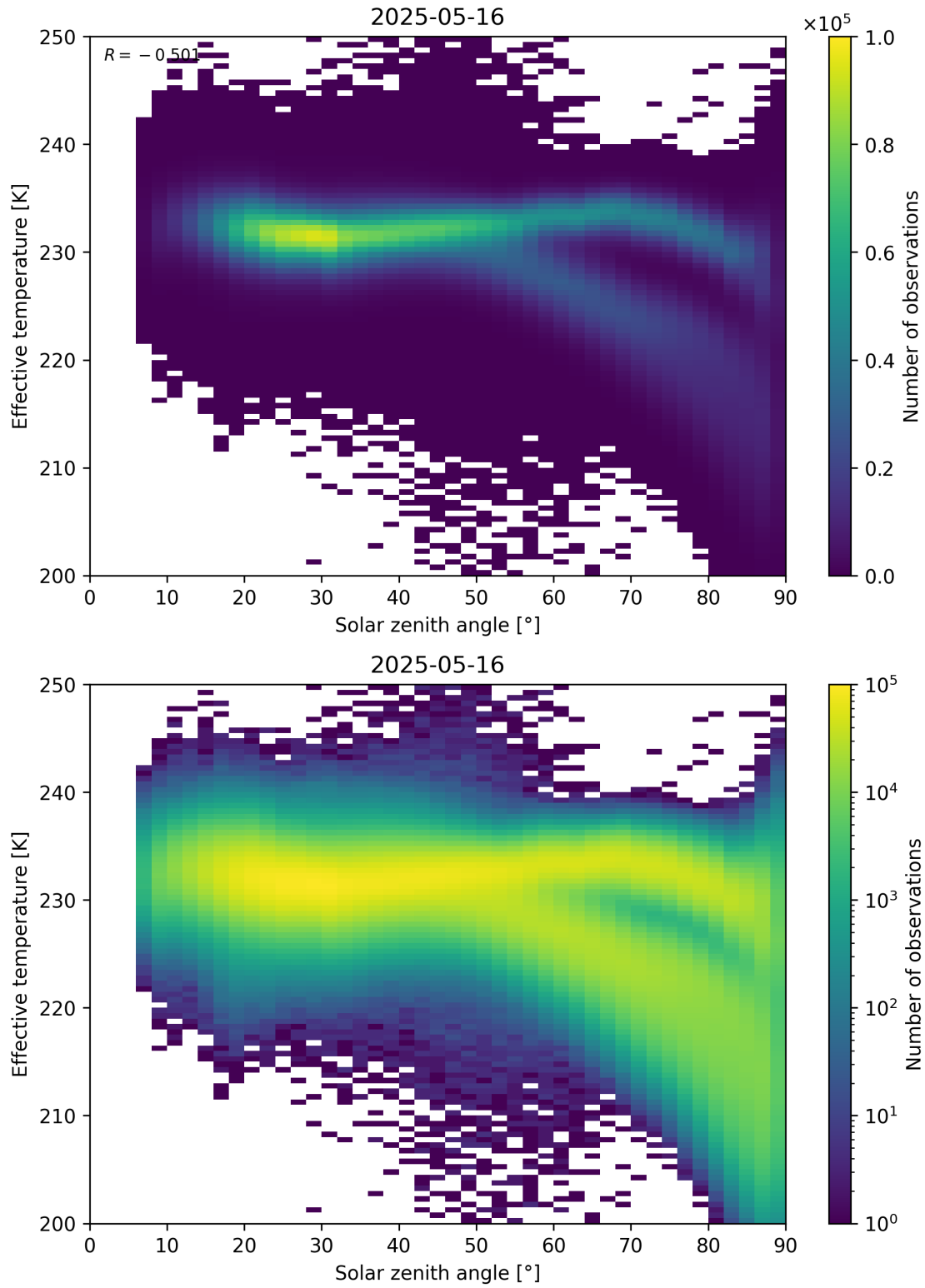
Figure 45: Scatter density plot of “Solar zenith angle” against “Effective temperature” for 2025-05-15 to 2025-05-17.
