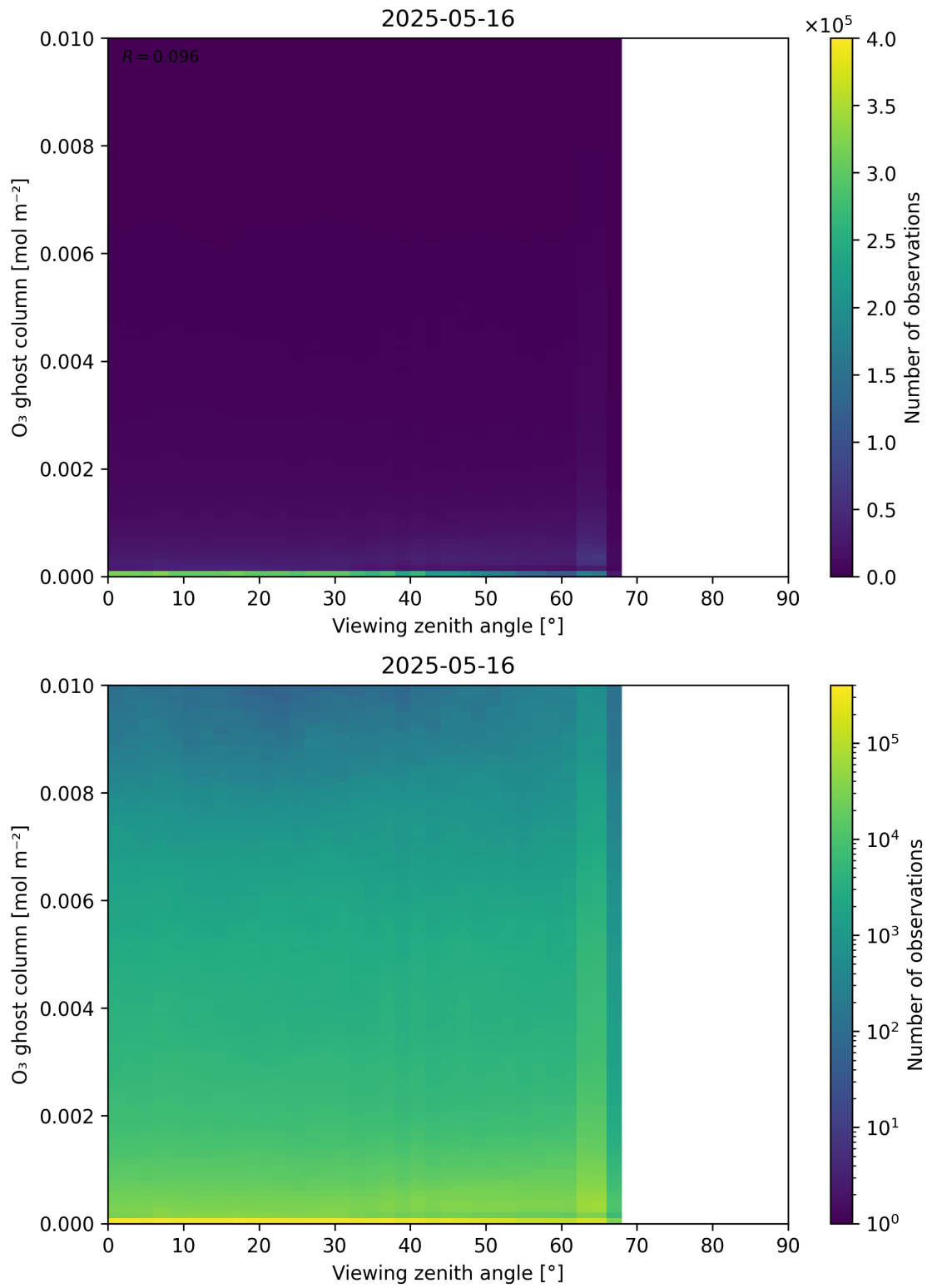
Figure 51: Scatter density plot of “Viewing zenith angle” against “O 3 ghost column” for 2025-05-15 to 2025-05-17.
