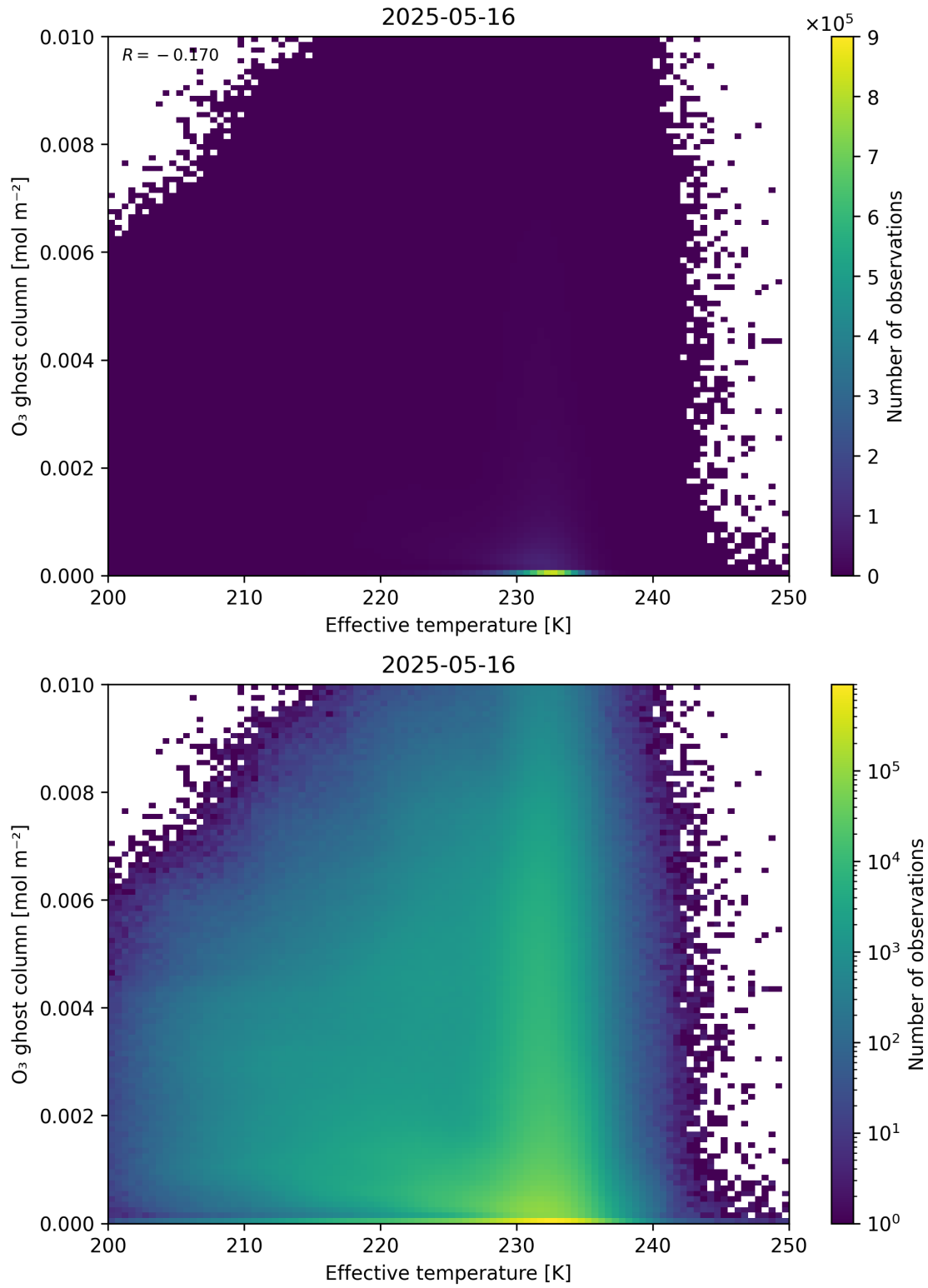
Figure 38: Scatter density plot of “Effective temperature” against “O 3 ghost column” for 2025-05-15 to 2025-05-17.
