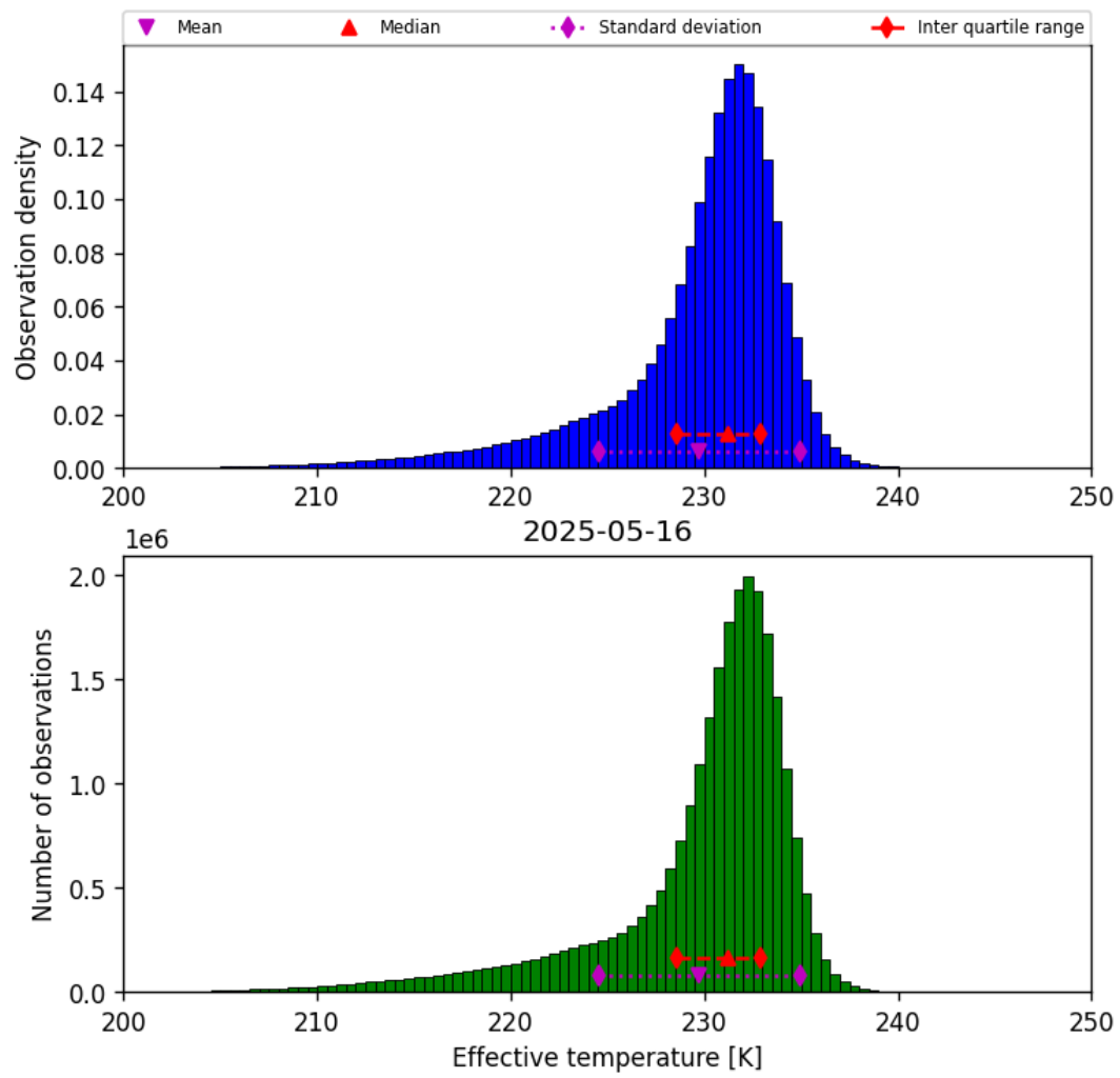
Figure 24: Histogram of “Effective temperature” for 2025-05-15 to 2025-05-17
