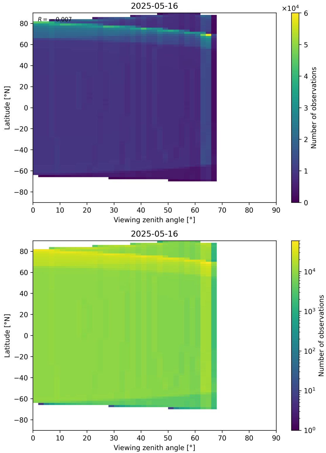
Figure 49: Scatter density plot of “Viewing zenith angle” against “Latitude” for 2025-05-15 to 2025-05-17.
