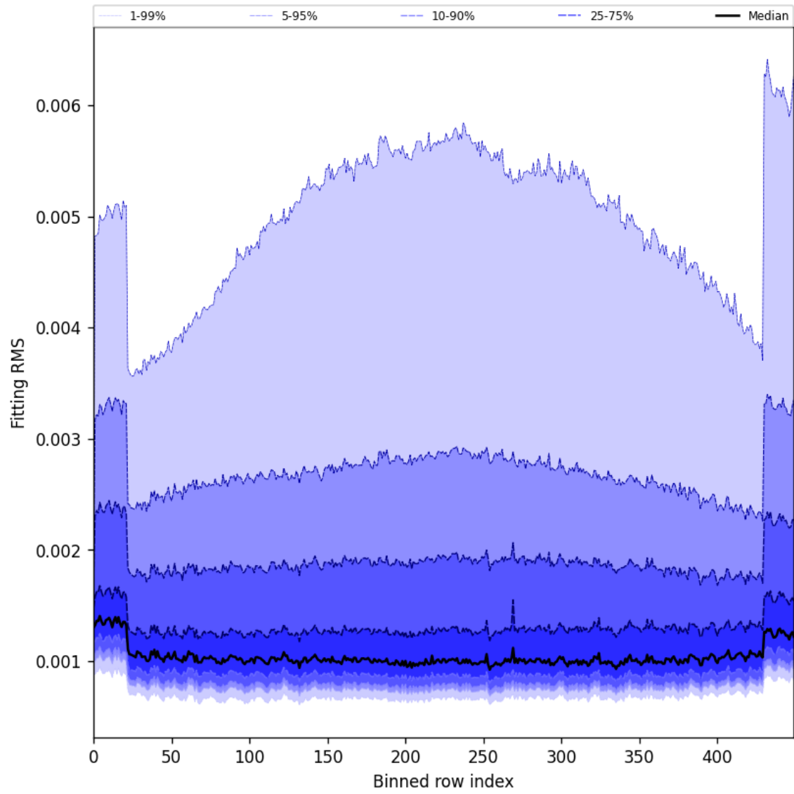
Figure 30: Along track statistics of “Fitting RMS” for 2025-05-15 to 2025-05-17
