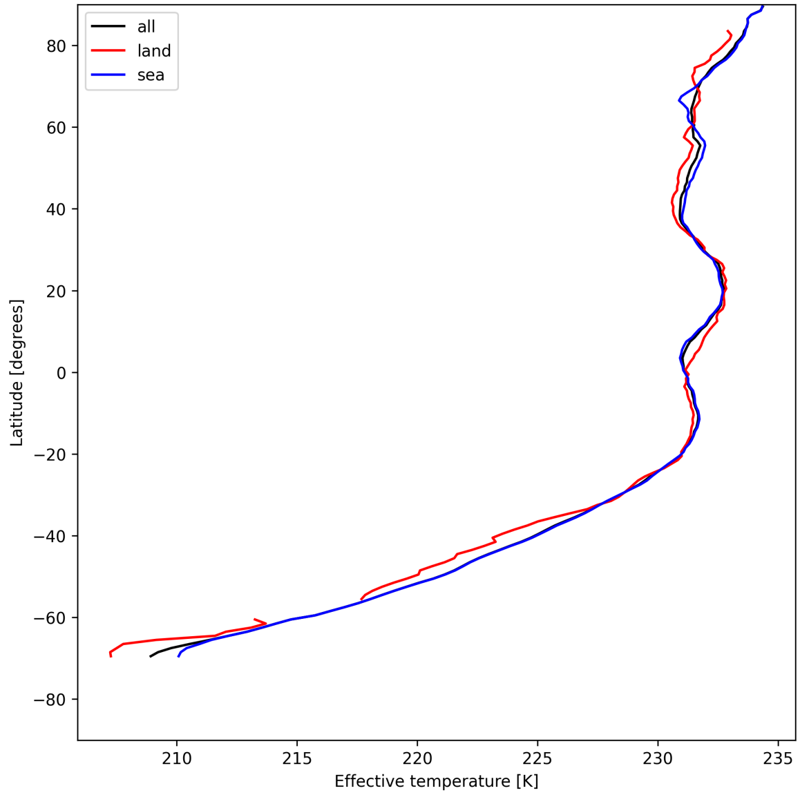
Figure 17: Zonal average of “Effective temperature” for 2025-05-15 to 2025-05-17.
