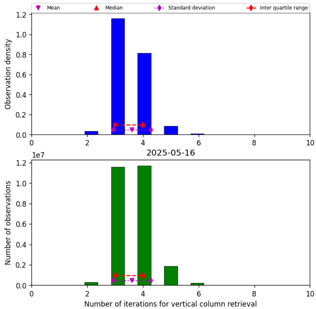
Figure 26: Histogram of “Number of iterations for vertical column retrieval” for 2025-05-15 to 2025-05-17
