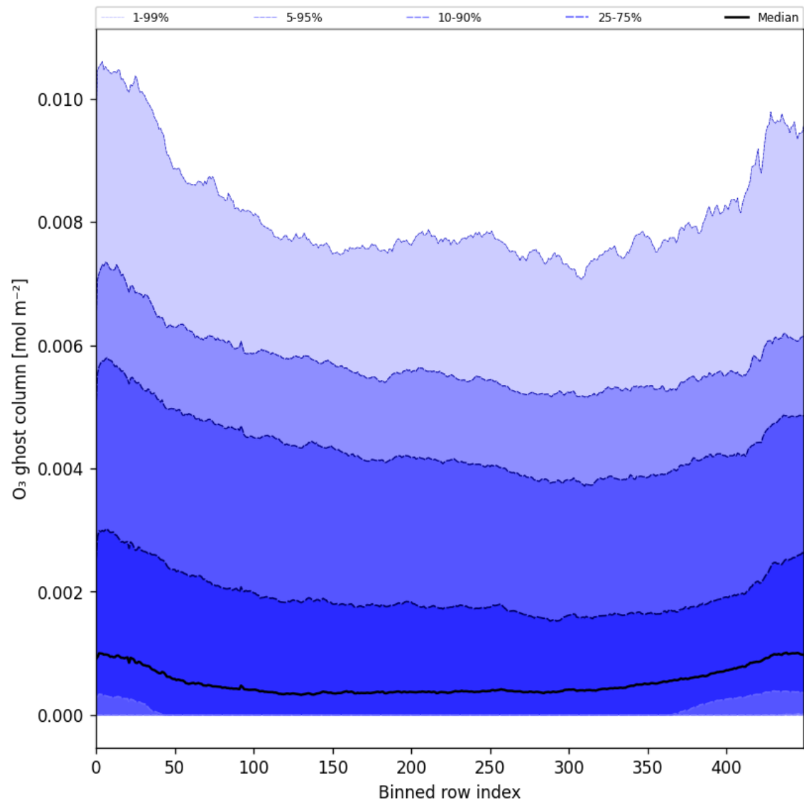
Figure 32: Along track statistics of “O 3 ghost column” for 2025-05-15 to 2025-05-17
