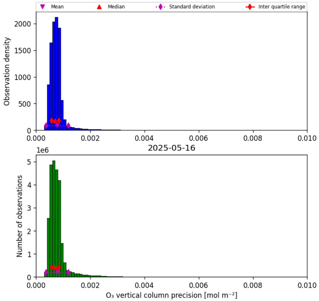
Figure 22: Histogram of “O 3 vertical column precision” for 2025-05-15 to 2025-05-17
