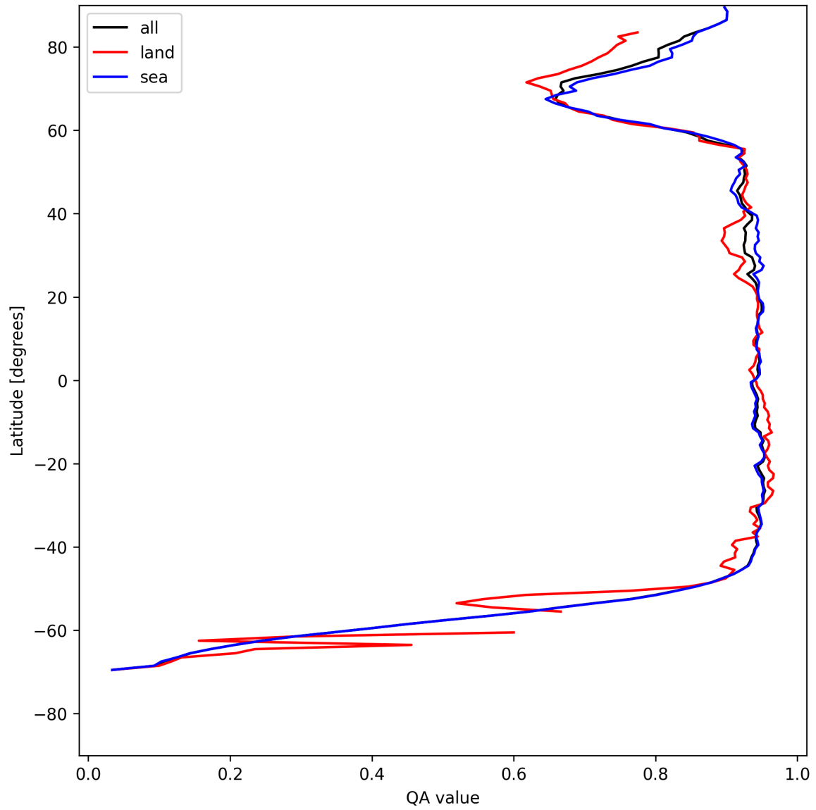
Figure 13: Zonal average of “QA value” for 2025-05-15 to 2025-05-17.
