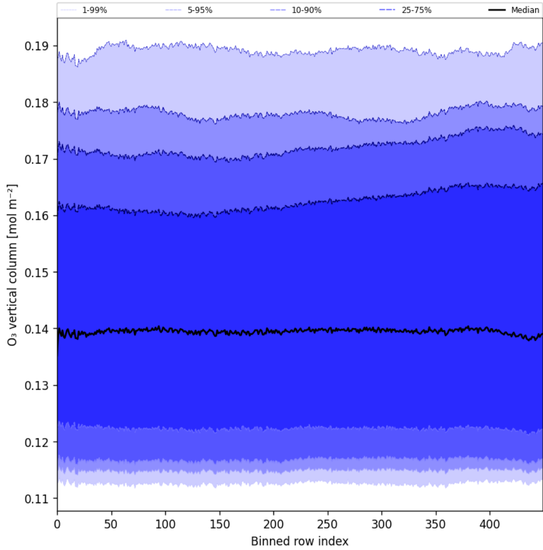
Figure 28: Along track statistics of “O 3 vertical column” for 2025-05-15 to 2025-05-17
