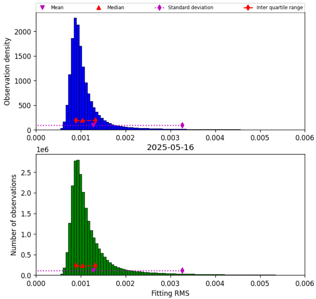
Figure 23: Histogram of “Fitting RMS” for 2025-05-15 to 2025-05-17
