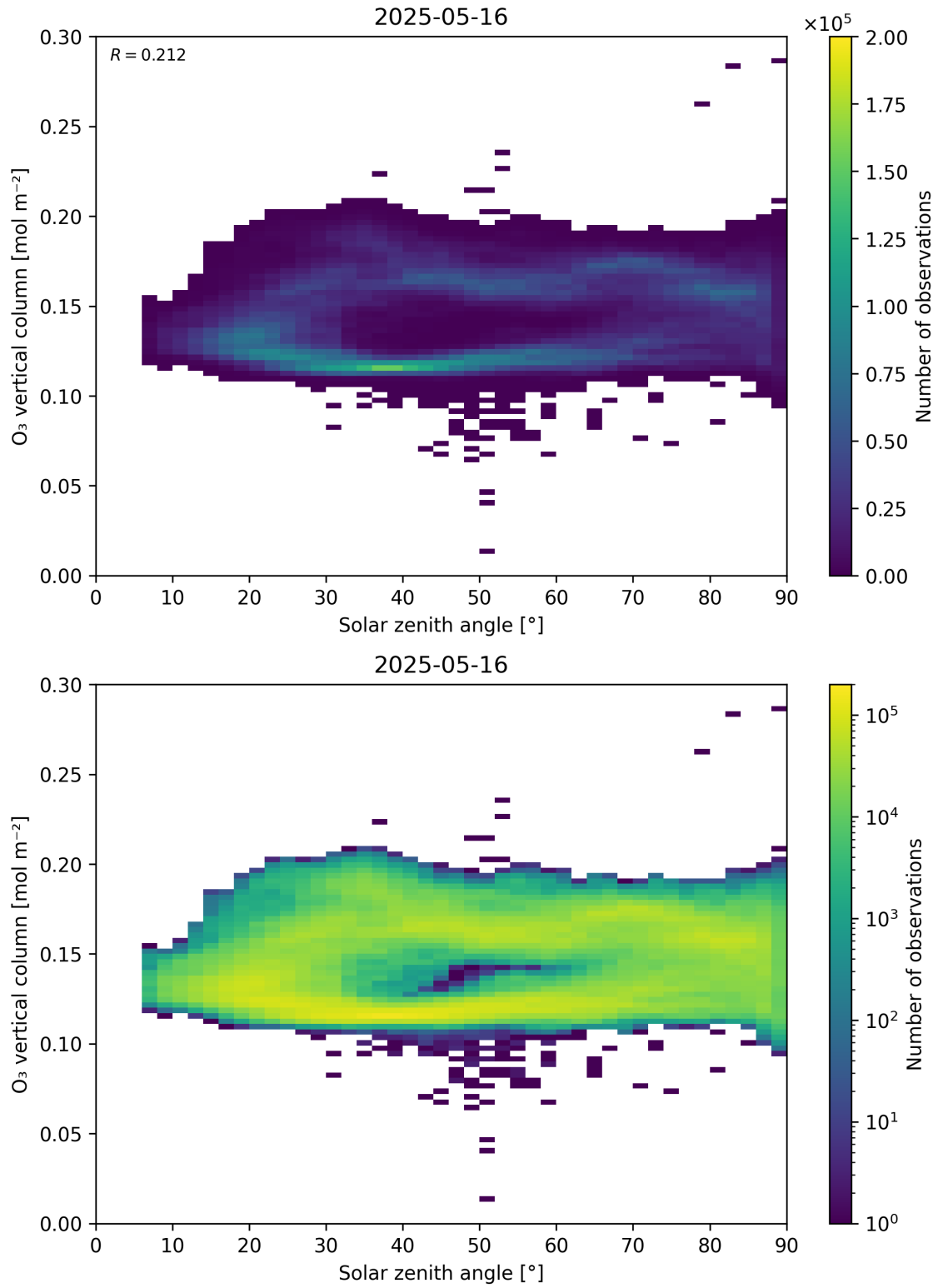
Figure 47: Scatter density plot of “Solar zenith angle” against “O 3 vertical column” for 2025-05-15 to 2025-05-17.
