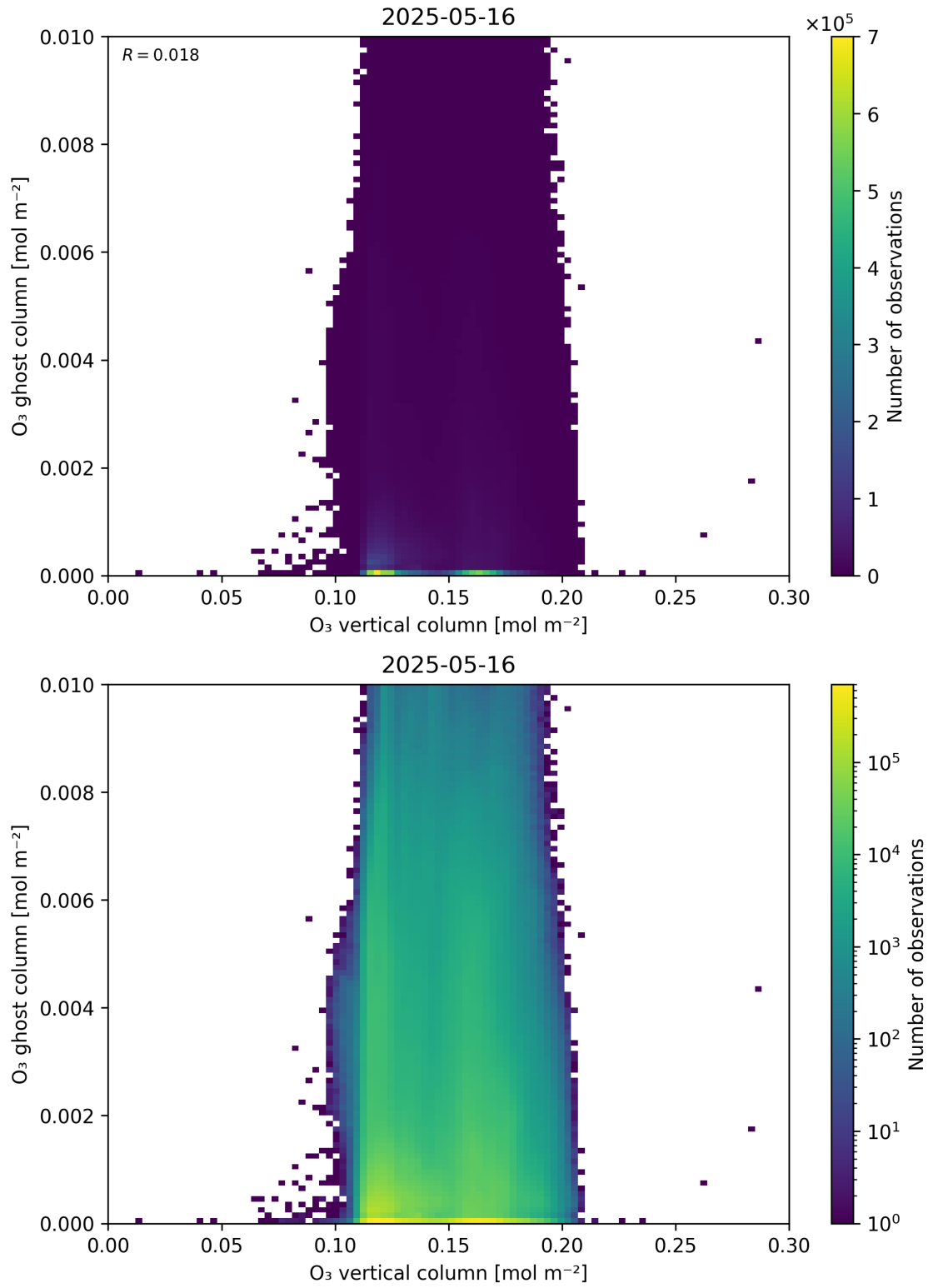
Figure 40: Scatter density plot of “O 3 vertical column” against “O 3 ghost column” for 2025-05-15 to 2025-05-17.
