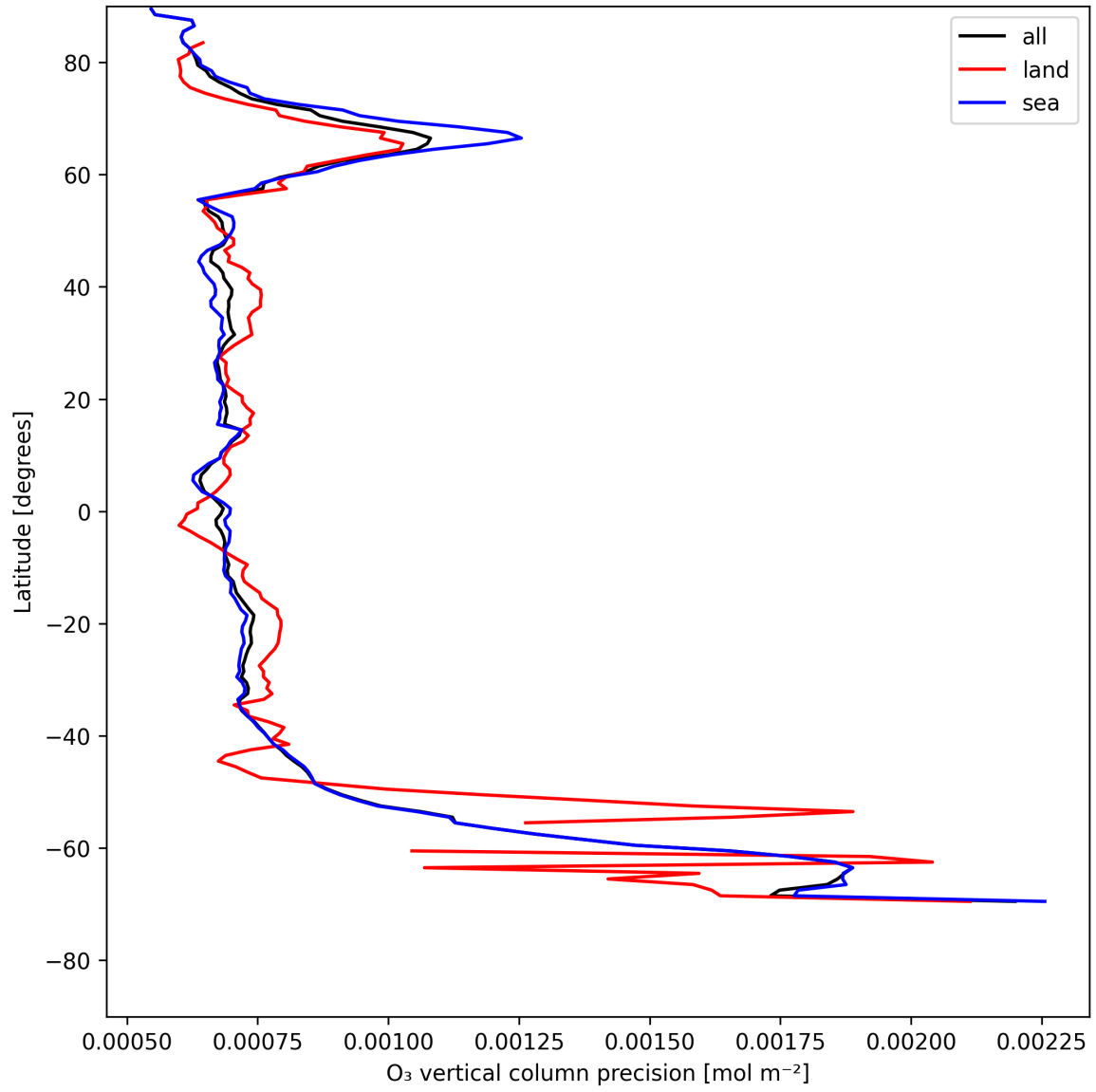
Figure 15: Zonal average of "O 3 vertical column precision" for 2025-05-15 to 2025-05-17.
