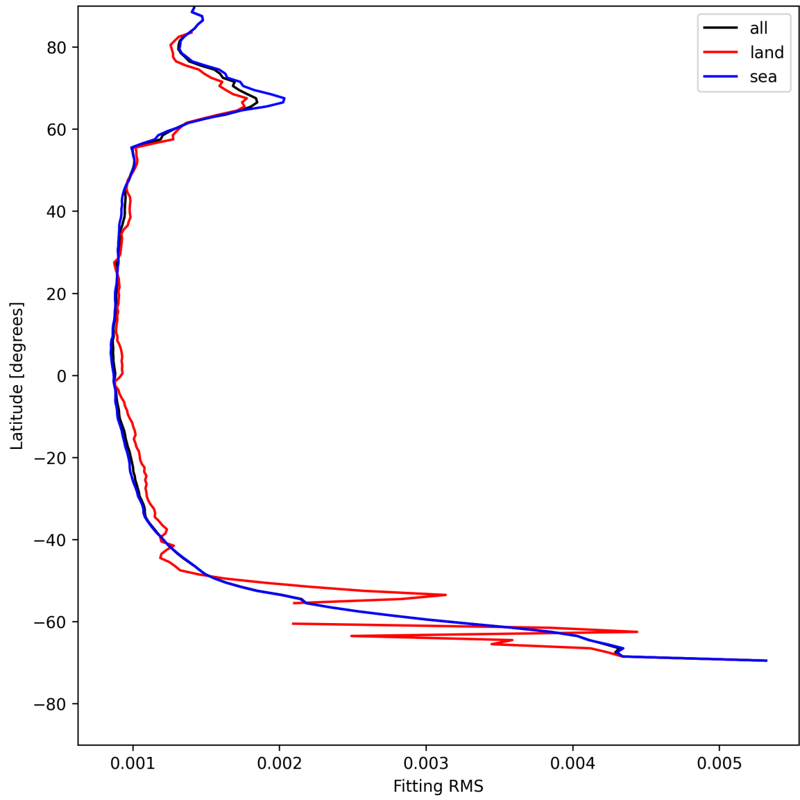
Figure 16: Zonal average of “Fitting RMS” for 2025-05-15 to 2025-05-17.
