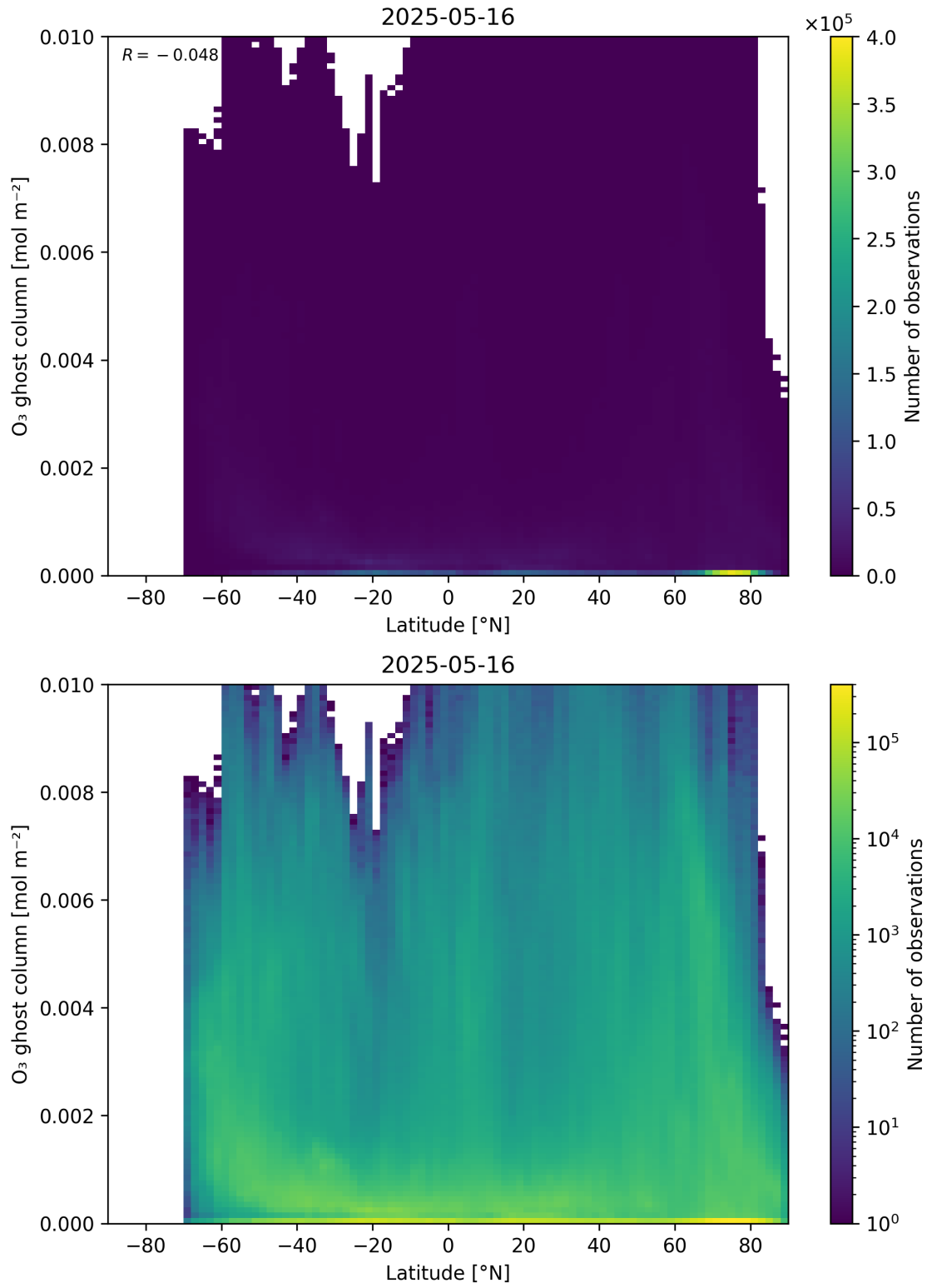
Figure 35: Scatter density plot of “Latitude” against “O 3 ghost column” for 2025-05-15 to 2025-05-17.
