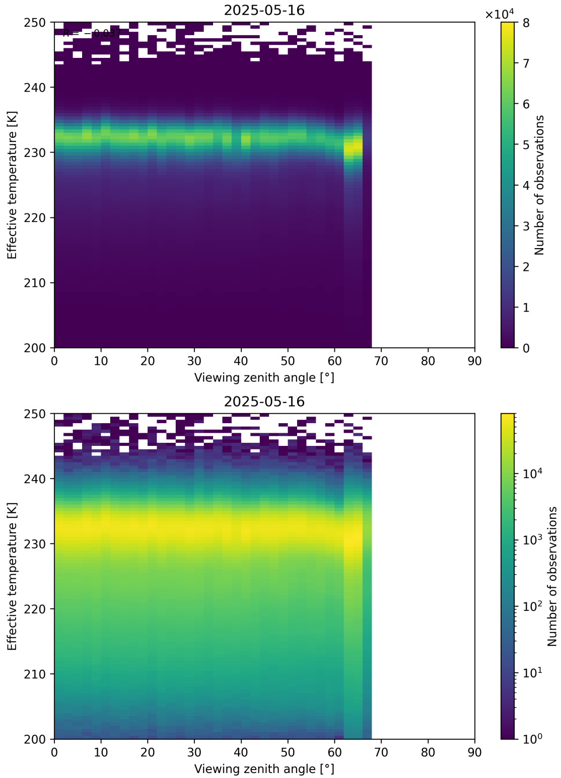
Figure 50: Scatter density plot of “Viewing zenith angle” against “Effective temperature” for 2025-05-15 to 2025-05-17.
