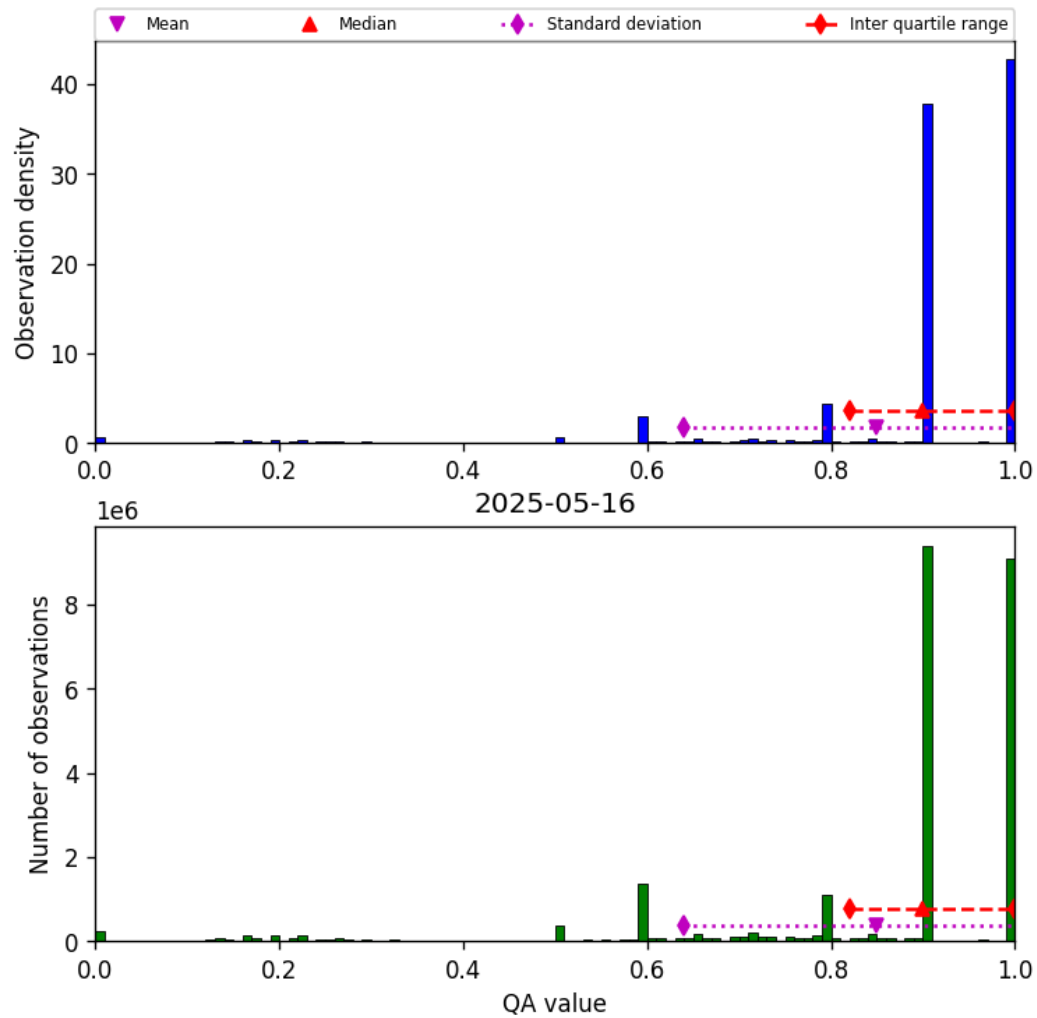
Figure 20: Histogram of “QA value” for 2025-05-15 to 2025-05-17
