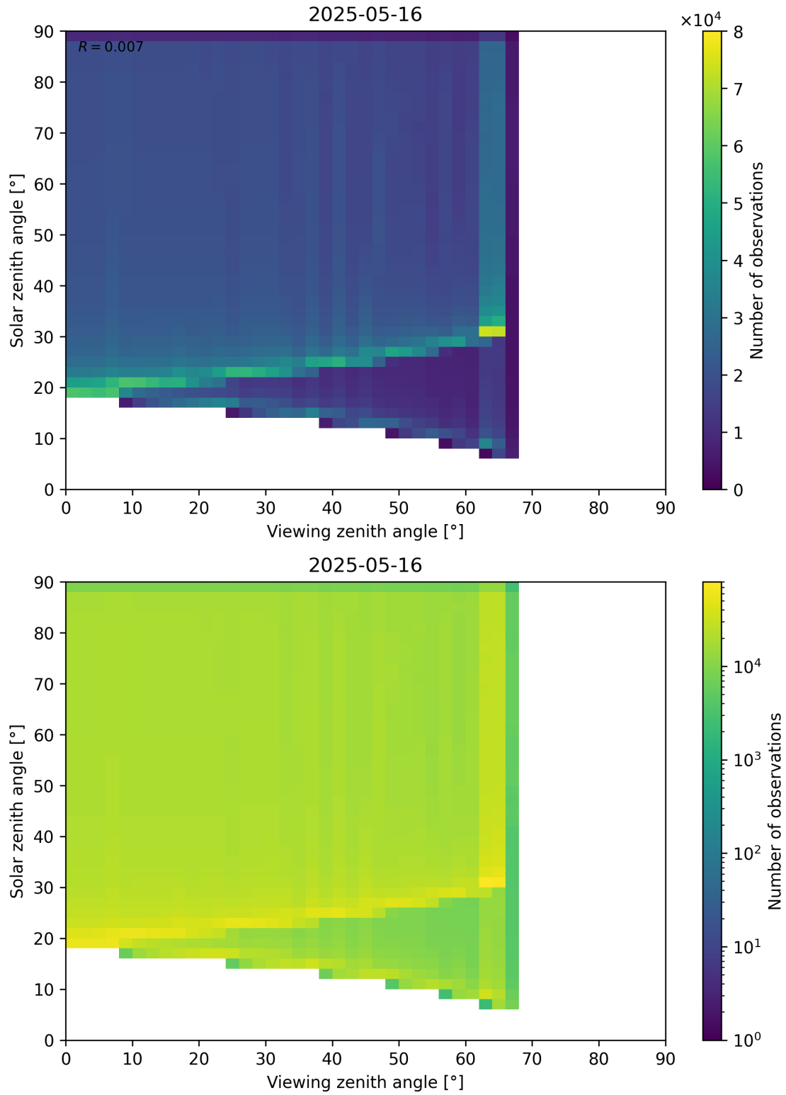
Figure 54: Scatter density plot of “Viewing zenith angle” against “Solar zenith angle” for 2025-05-15 to 2025-05-17.
