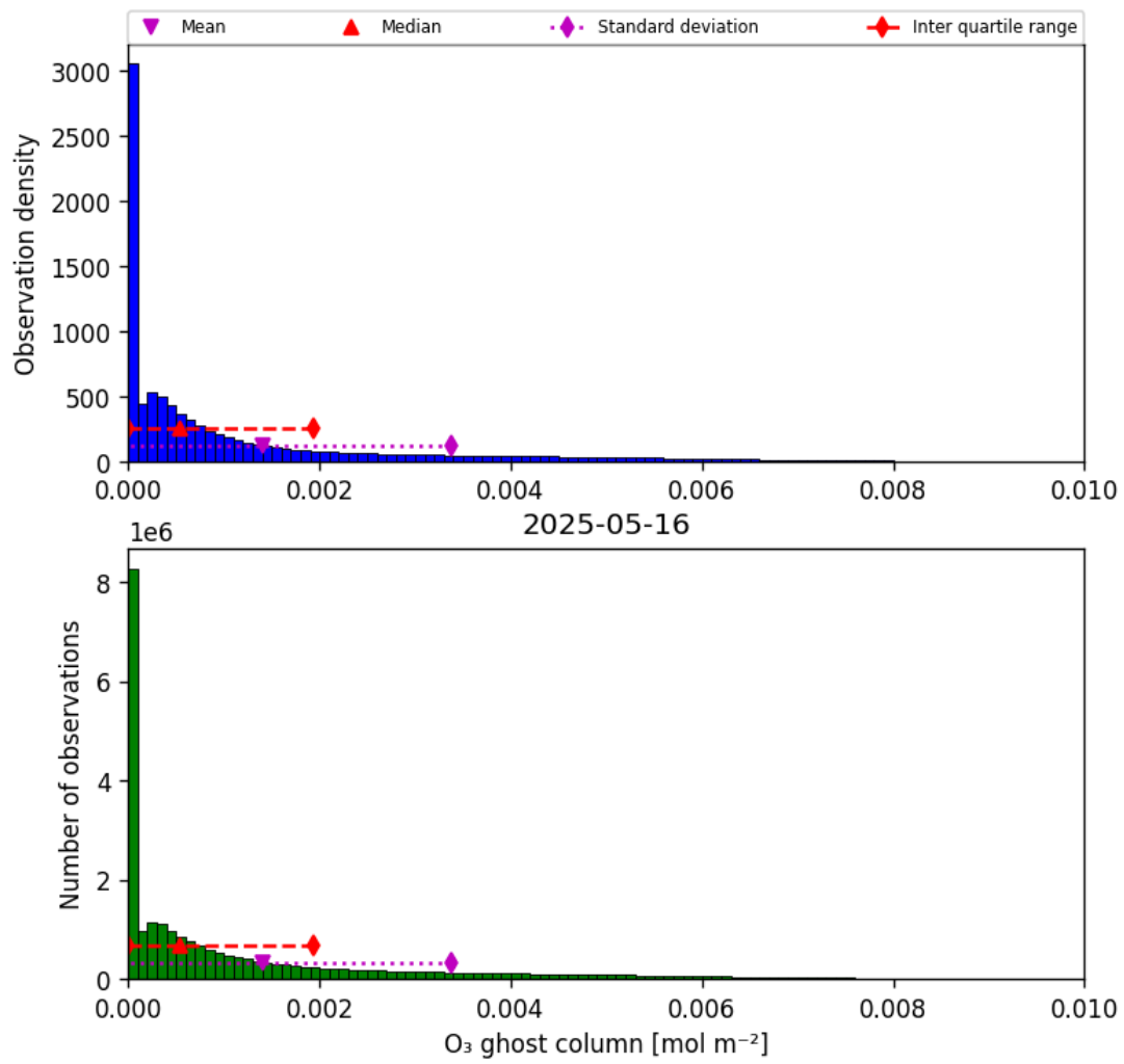
Figure 25: Histogram of “O 3 ghost column” for 2025-05-15 to 2025-05-17
