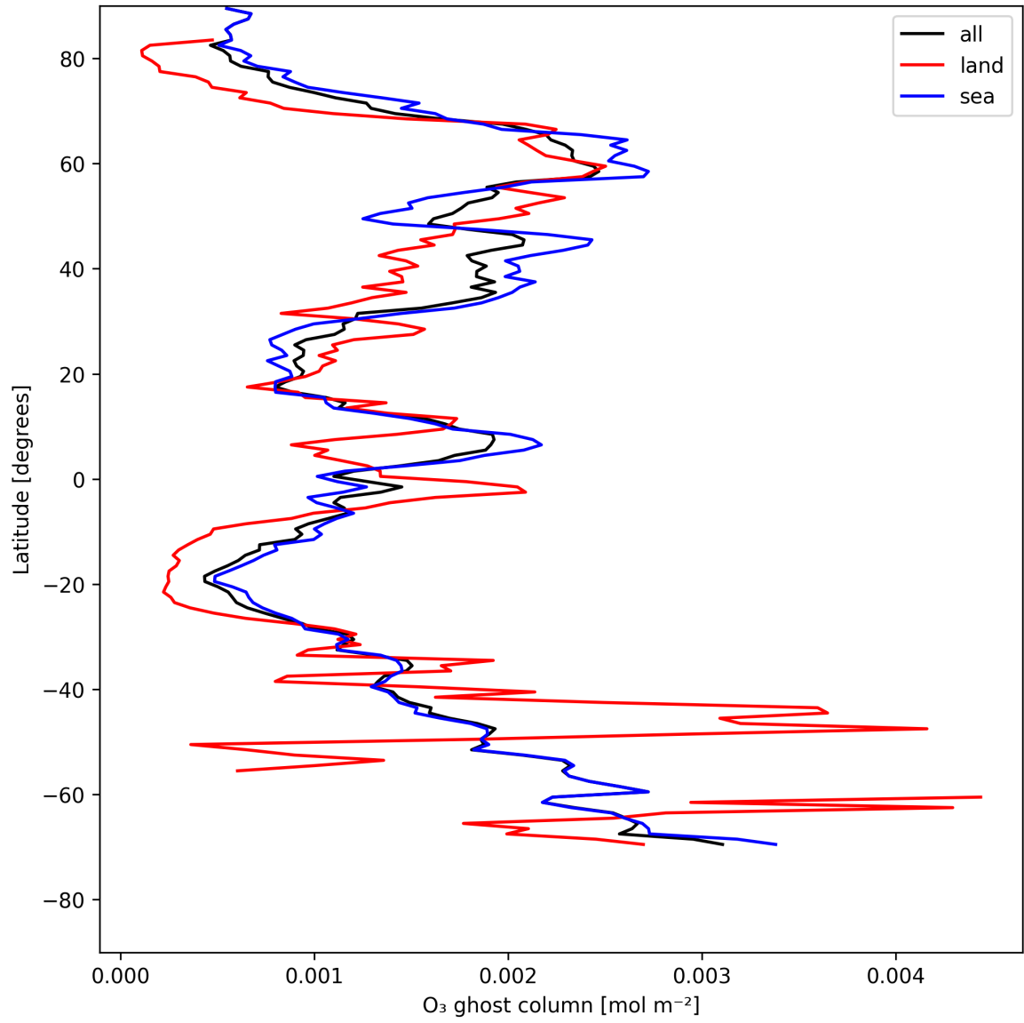
Figure 18: Zonal average of "O 3 ghost column" for 2025-05-15 to 2025-05-17.
