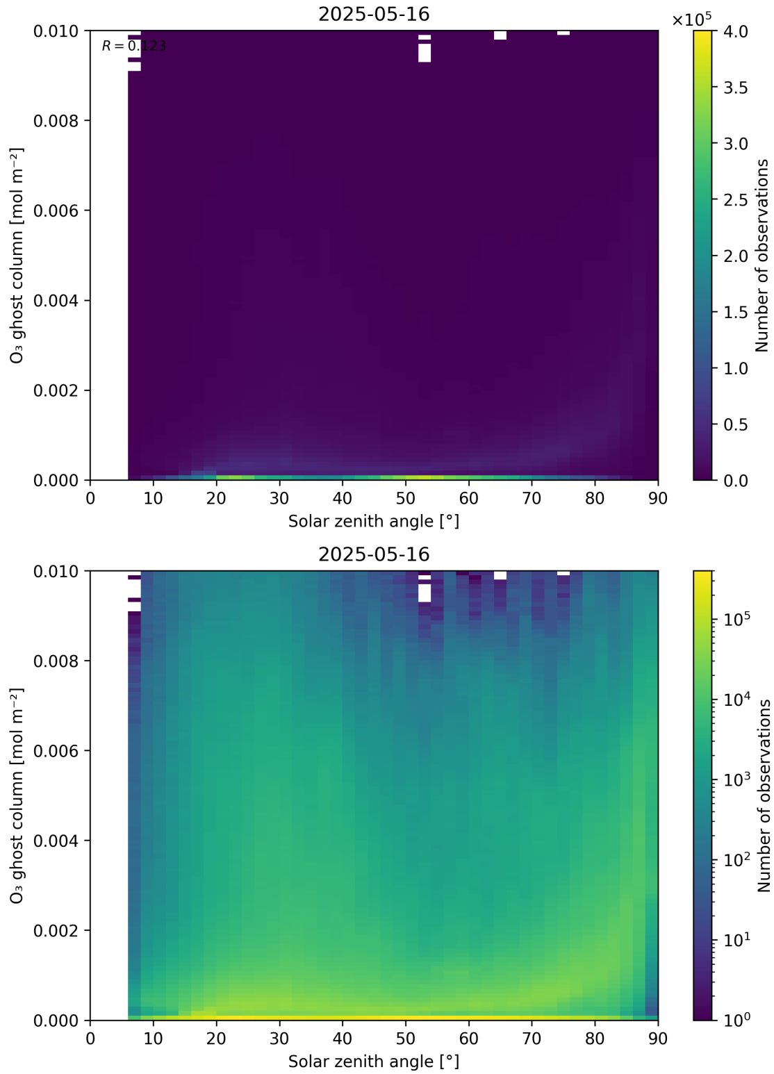
Figure 46: Scatter density plot of “Solar zenith angle” against “O 3 ghost column” for 2025-05-15 to 2025-05-17.
