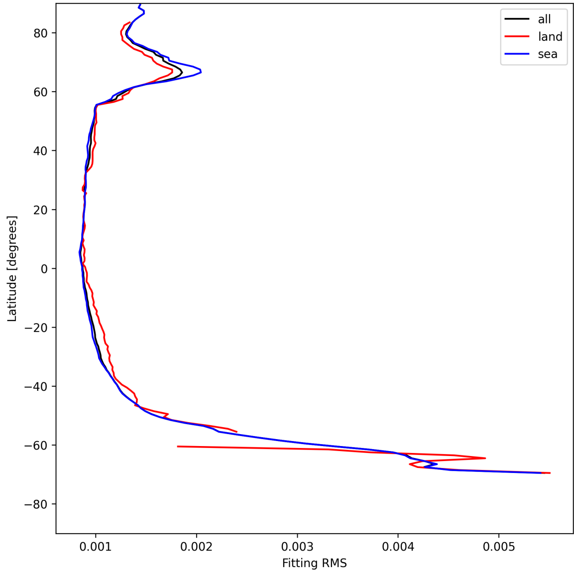
Figure 16: Zonal average of “Fitting RMS” for 2025-05-16 to 2025-05-18.
