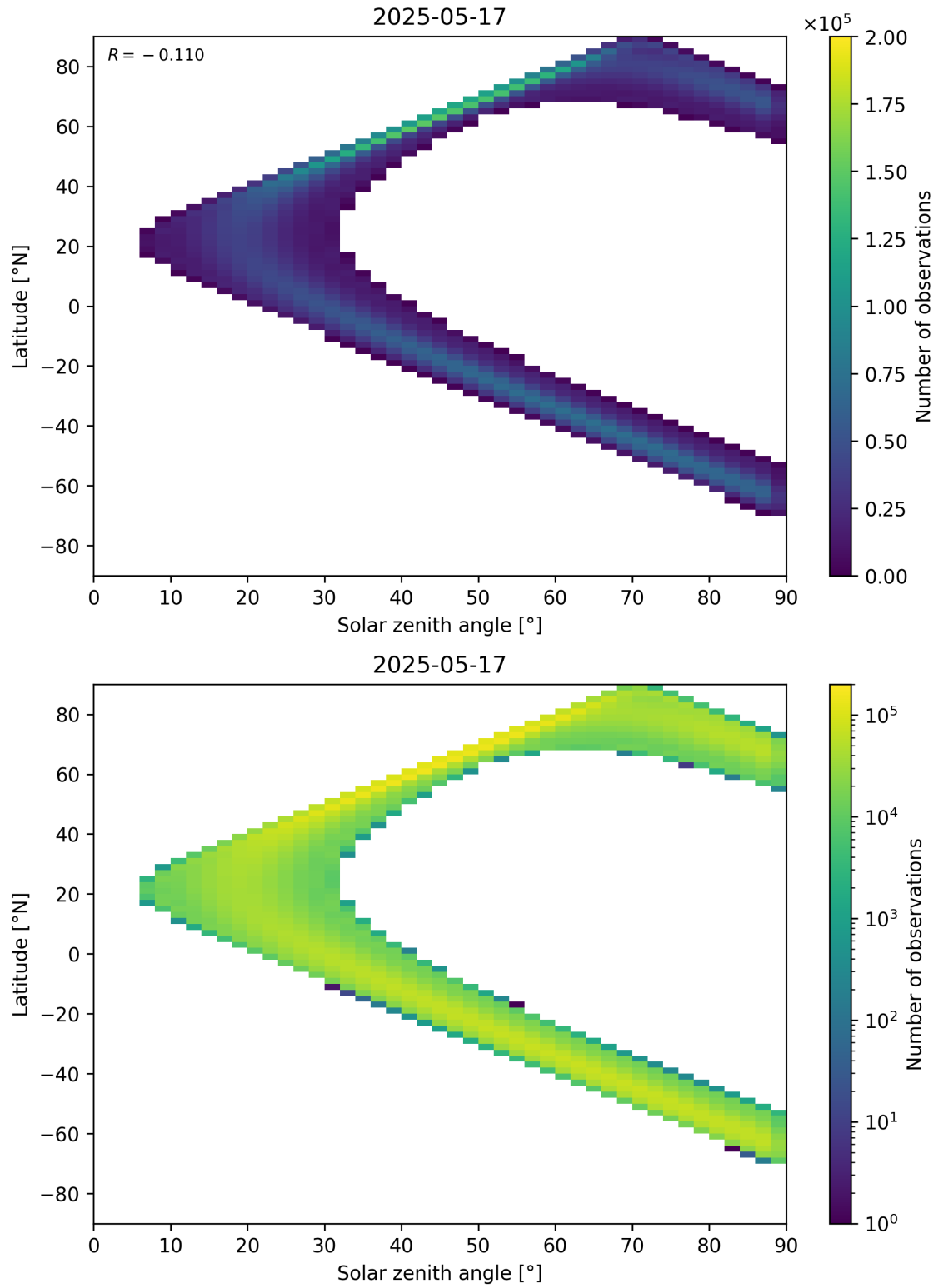
Figure 44: Scatter density plot of “Solar zenith angle” against “Latitude” for 2025-05-16 to 2025-05-18.
