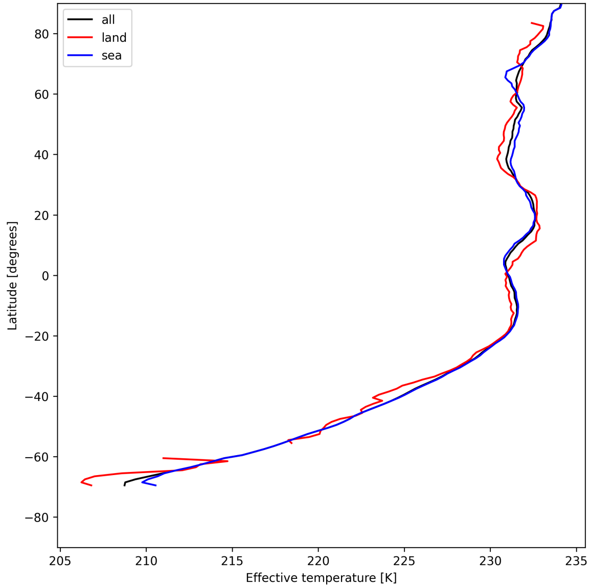
Figure 17: Zonal average of "Effective temperature" for 2025-05-16 to 2025-05-18.
