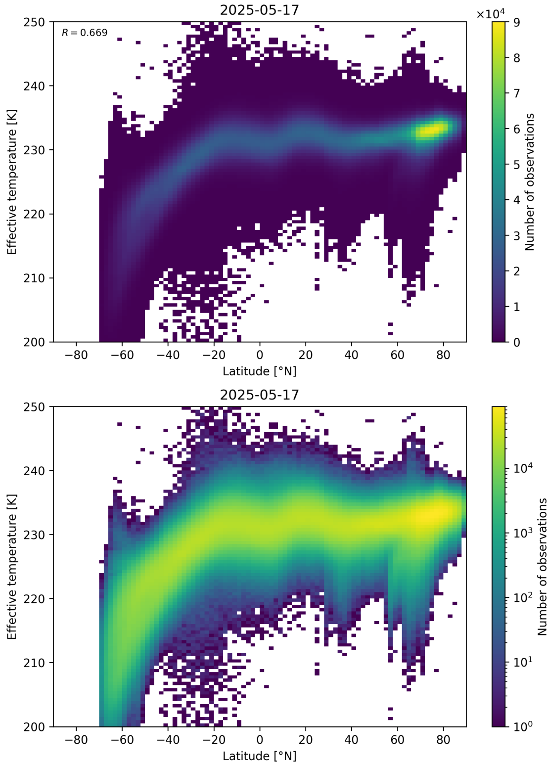
Figure 34: Scatter density plot of “Latitude” against “Effective temperature” for 2025-05-16 to 2025-05-18.
