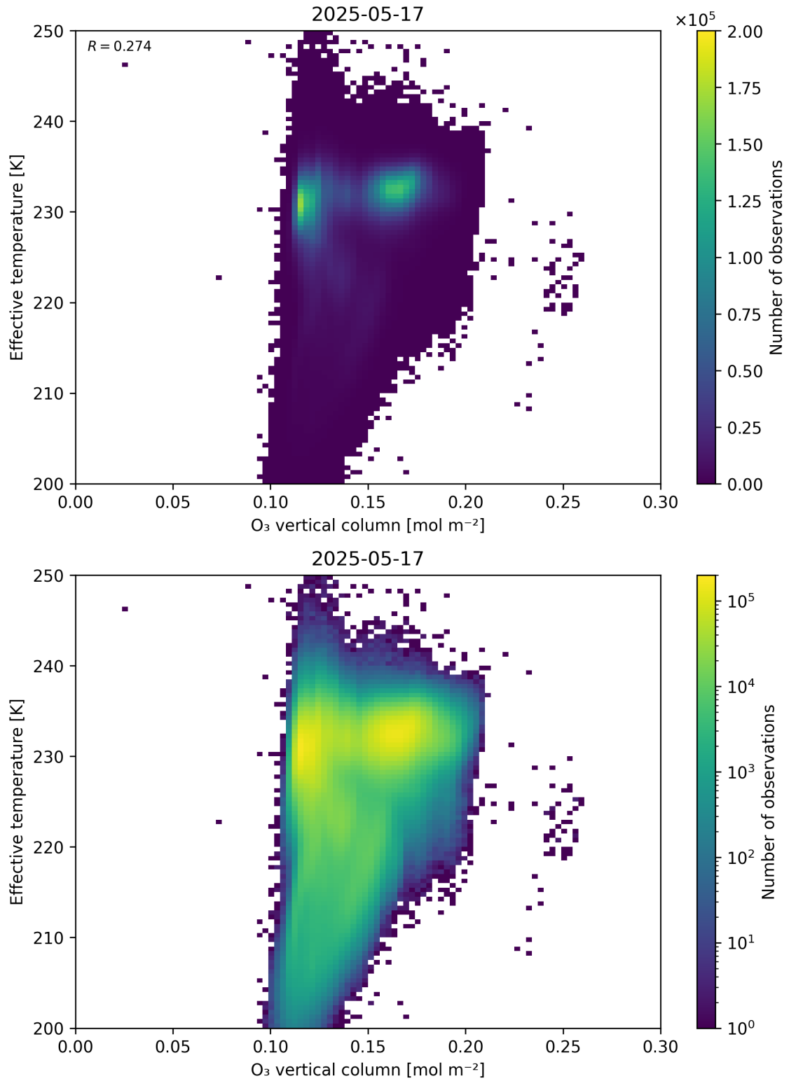
Figure 39: Scatter density plot of “O 3 vertical column” against “Effective temperature” for 2025-05-16 to 2025-05-18.
