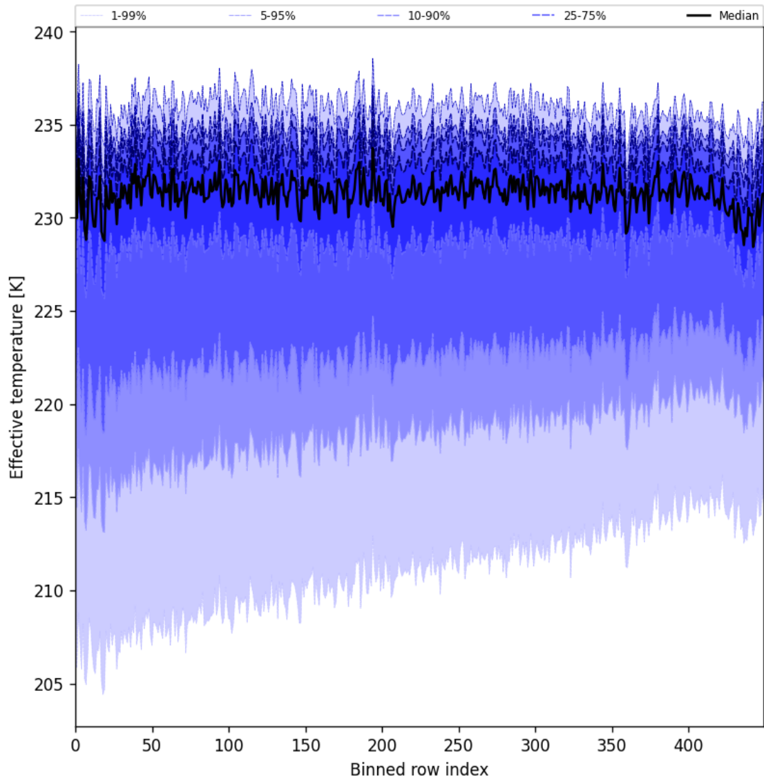
Figure 31: Along track statistics of “Effective temperature” for 2025-05-16 to 2025-05-18
