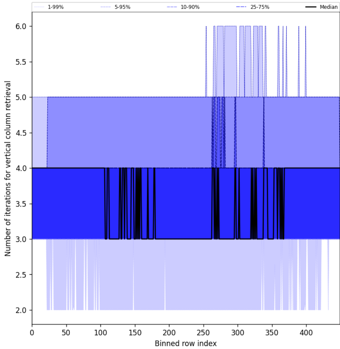
Figure 33: Along track statistics of “Number of iterations for vertical column retrieval” for 2025-05-16 to 2025-05-18
