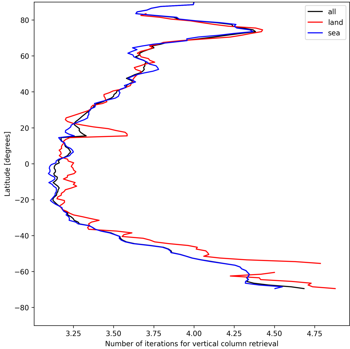
Figure 19: Zonal average of “Number of iterations for vertical column retrieval” for 2025-05-16 to 2025-05-18.
