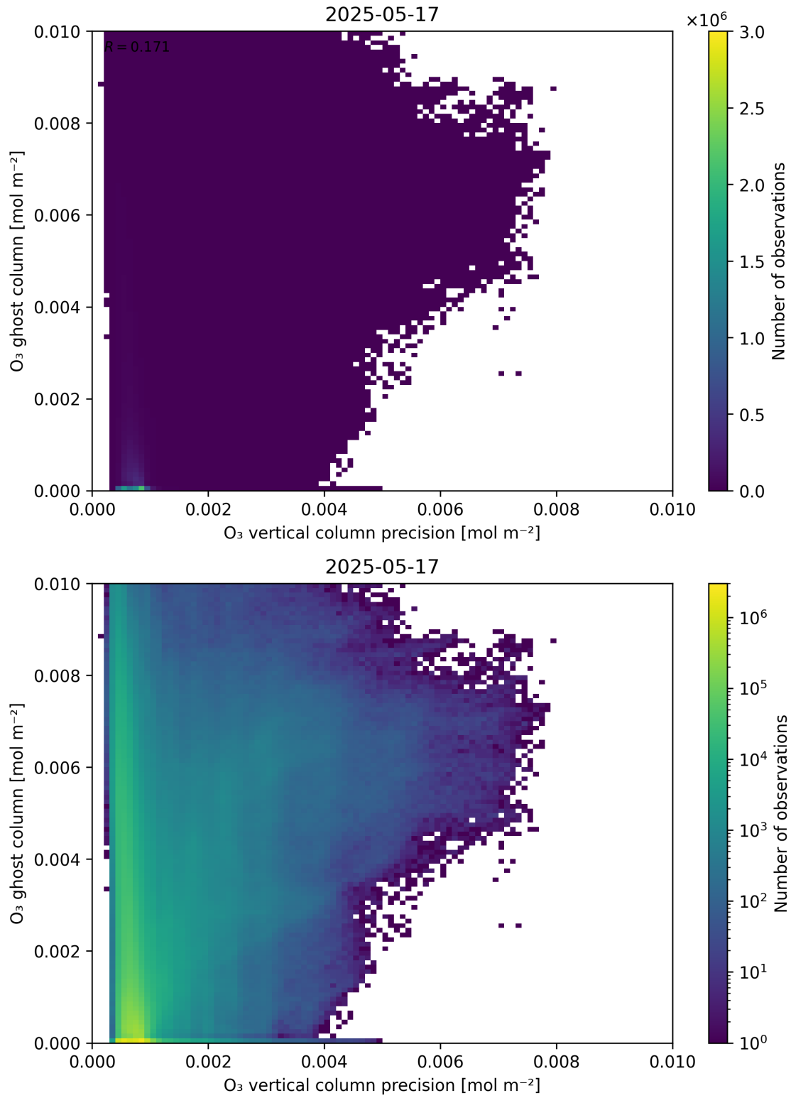
Figure 43: Scatter density plot of “ \text{O}_3 vertical column precision” against “ \text{O}_3 ghost column” for 2025-05-16 to 2025-05-18.
