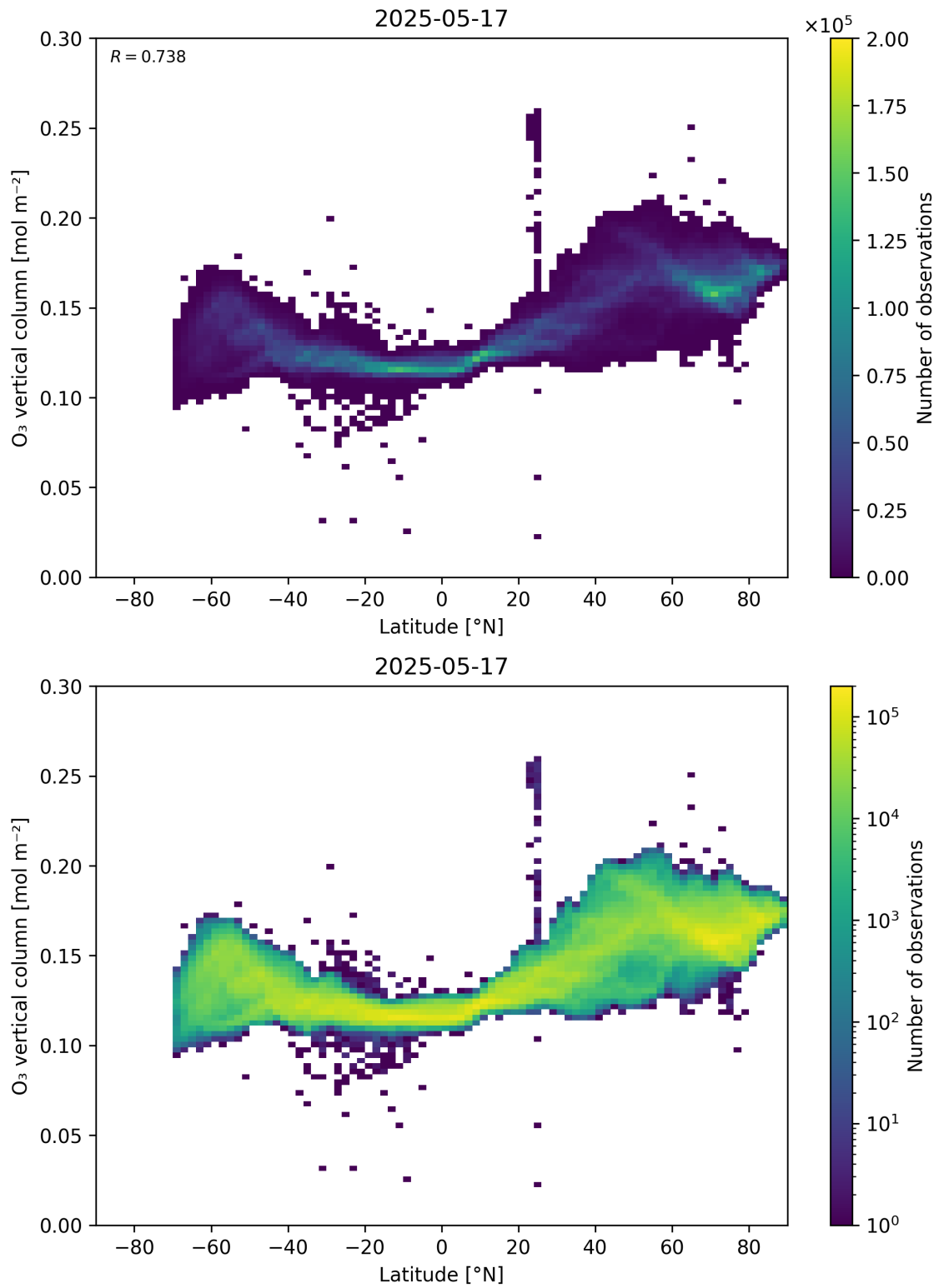
Figure 36: Scatter density plot of “Latitude” against “O 3 vertical column” for 2025-05-16 to 2025-05-18.
