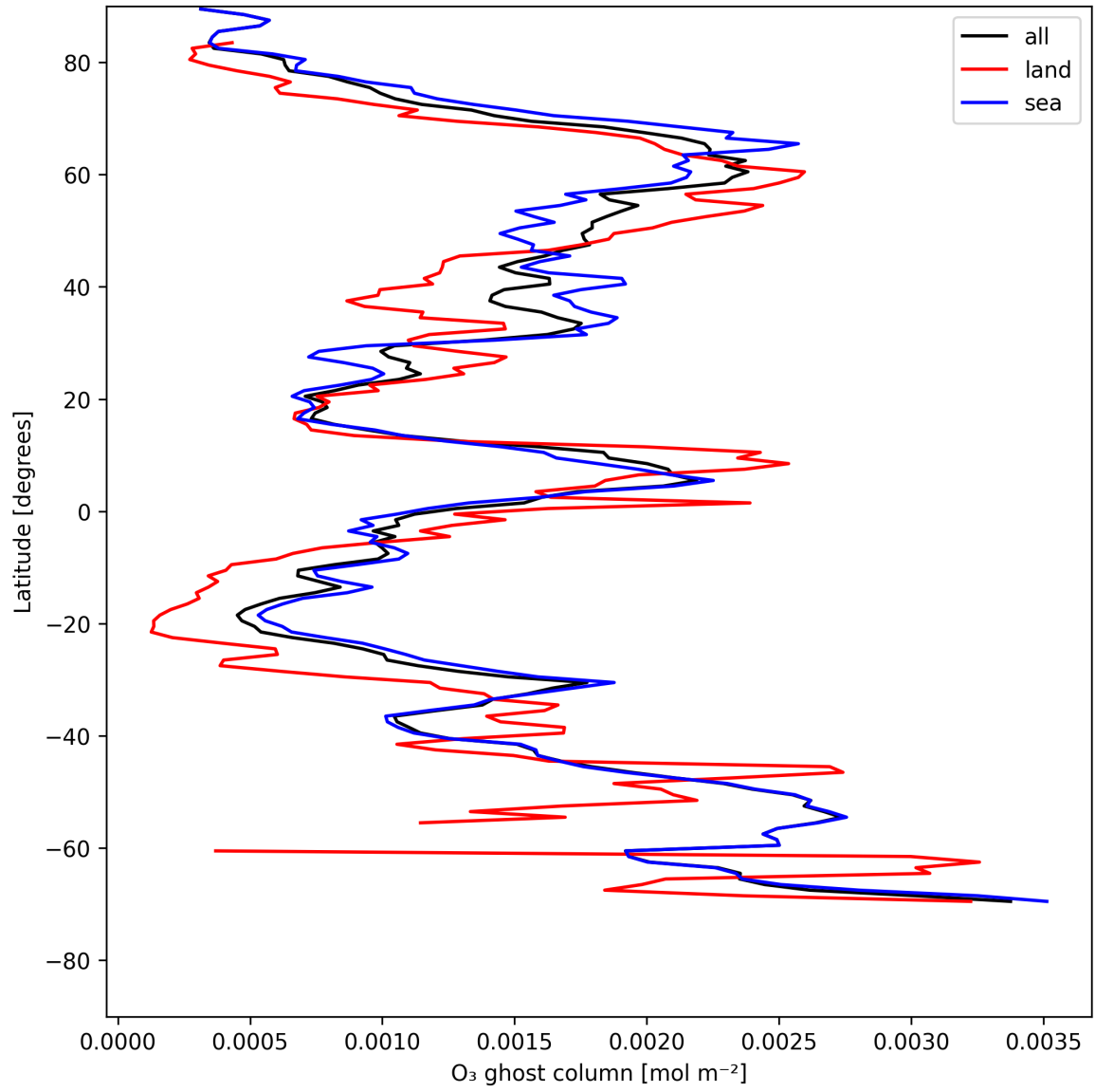
Figure 18: Zonal average of “O 3 ghost column” for 2025-05-16 to 2025-05-18.
