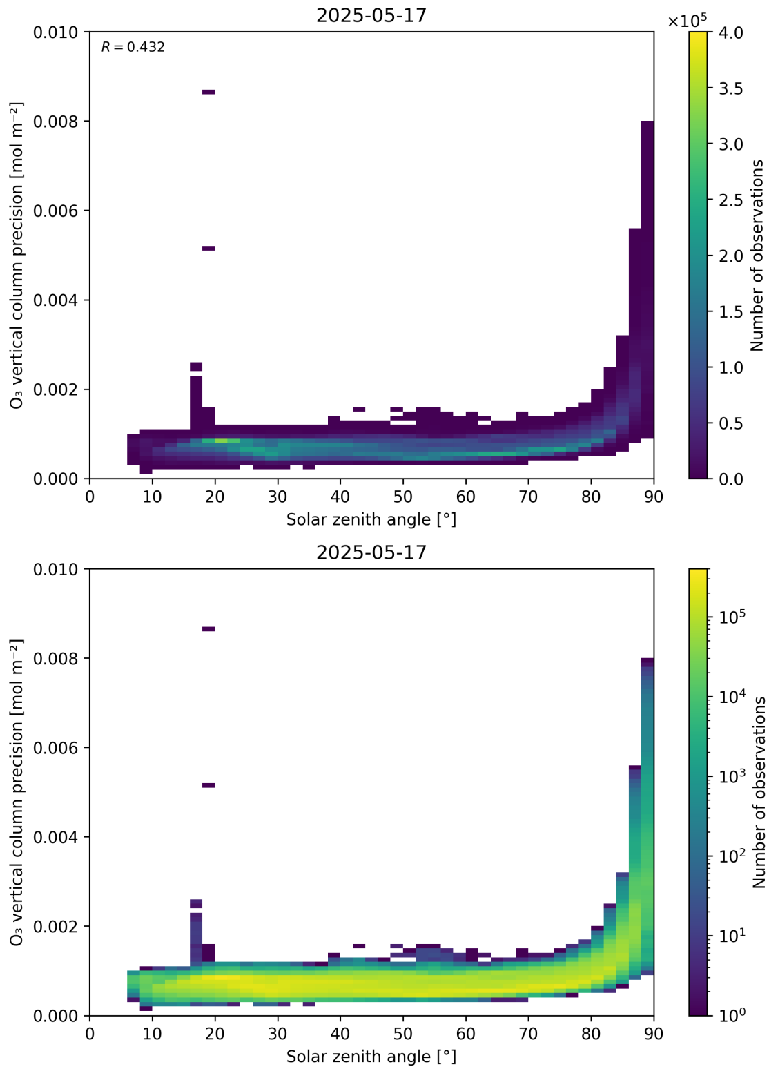
Figure 48: Scatter density plot of “Solar zenith angle” against “O 3 vertical column precision” for 2025-05-16 to 2025-05-18.
