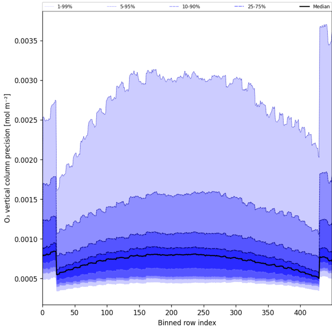
Figure 29: Along track statistics of “O 3 vertical column precision” for 2025-05-16 to 2025-05-18
