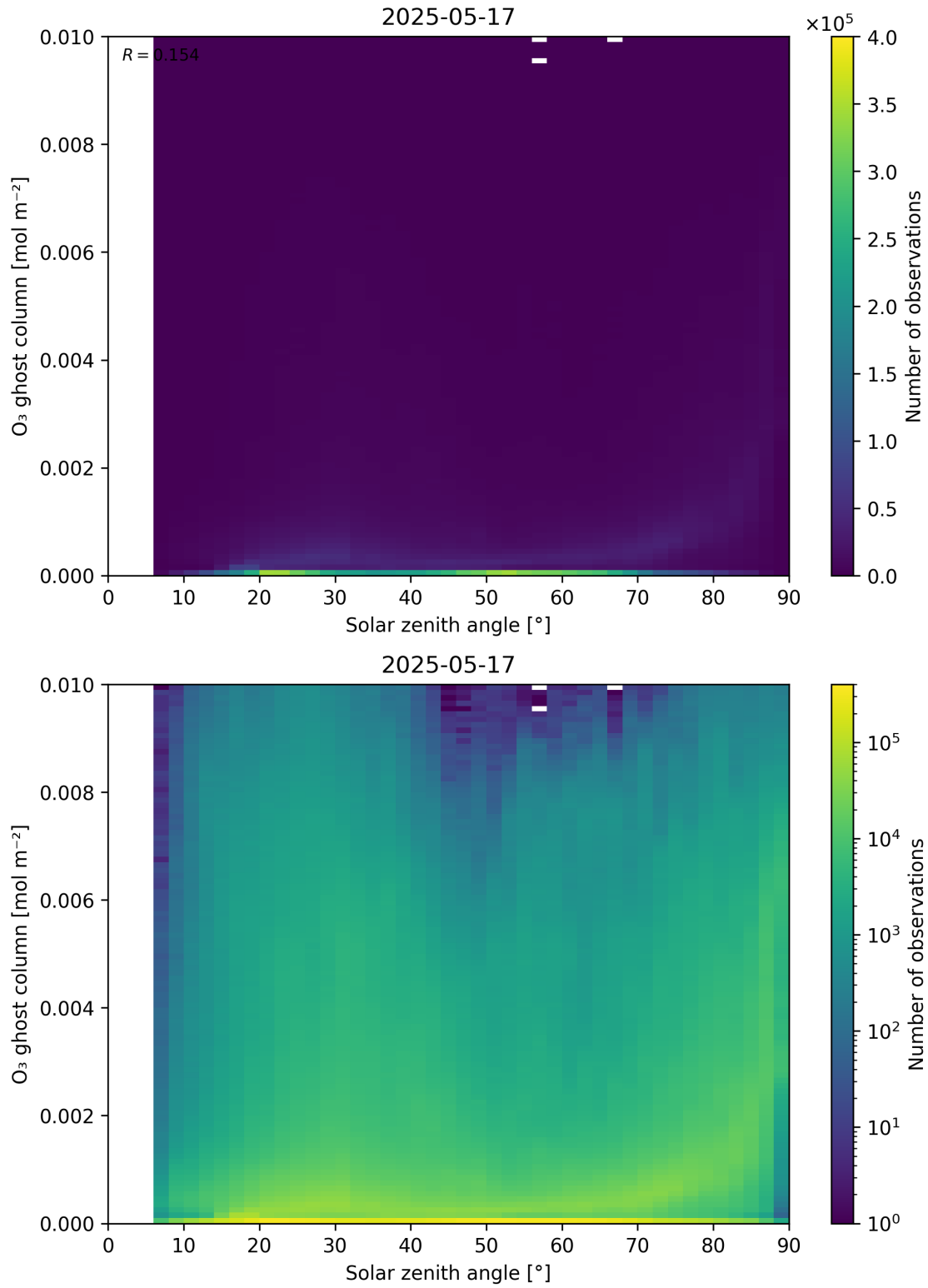
Figure 46: Scatter density plot of “Solar zenith angle” against “O 3 ghost column” for 2025-05-16 to 2025-05-18.
