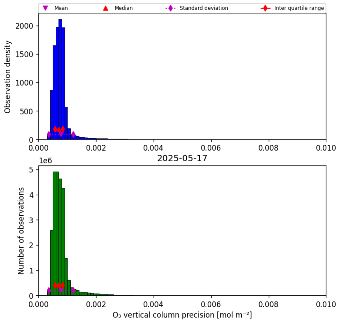
Figure 22: Histogram of “O 3 vertical column precision” for 2025-05-16 to 2025-05-18
