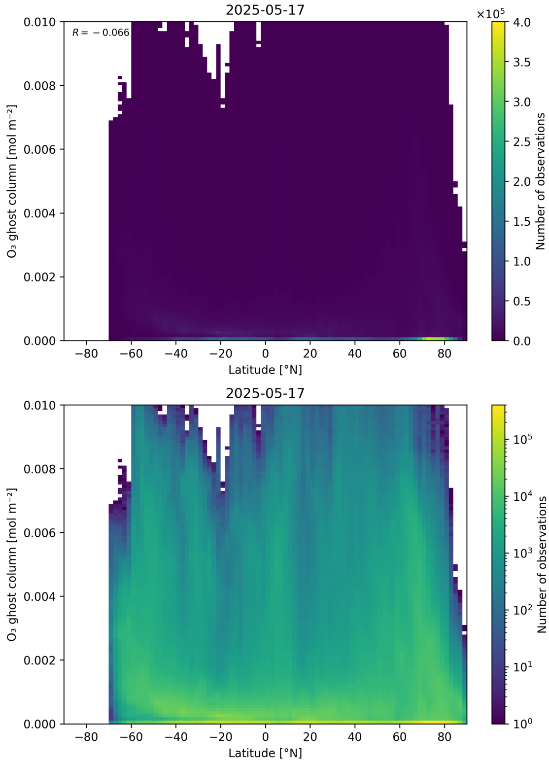
Figure 35: Scatter density plot of “Latitude” against “O 3 ghost column” for 2025-05-16 to 2025-05-18.
