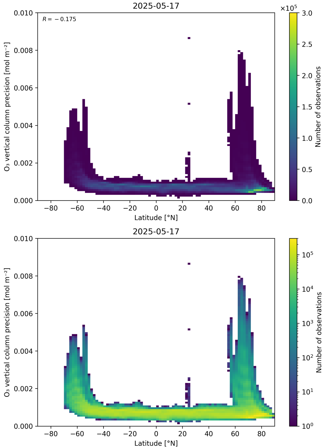
Figure 37: Scatter density plot of “Latitude” against “O 3 vertical column precision” for 2025-05-16 to 2025-05-18.
