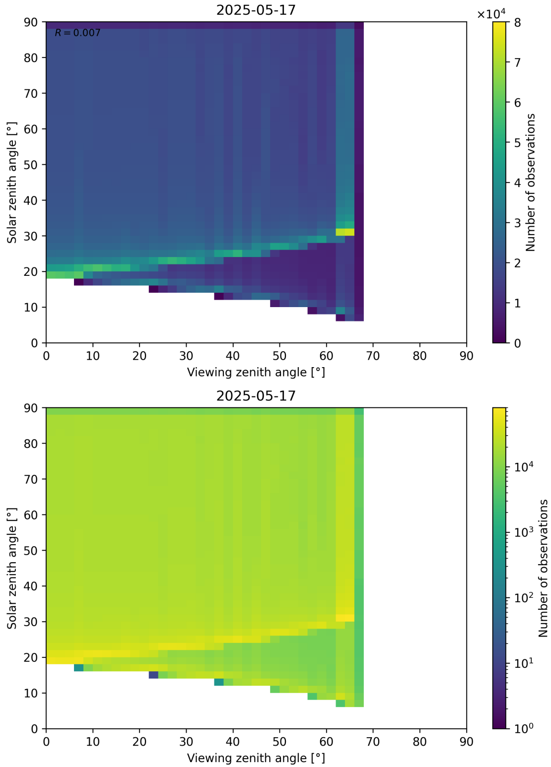
Figure 54: Scatter density plot of “Viewing zenith angle” against “Solar zenith angle” for 2025-05-16 to 2025-05-18.
