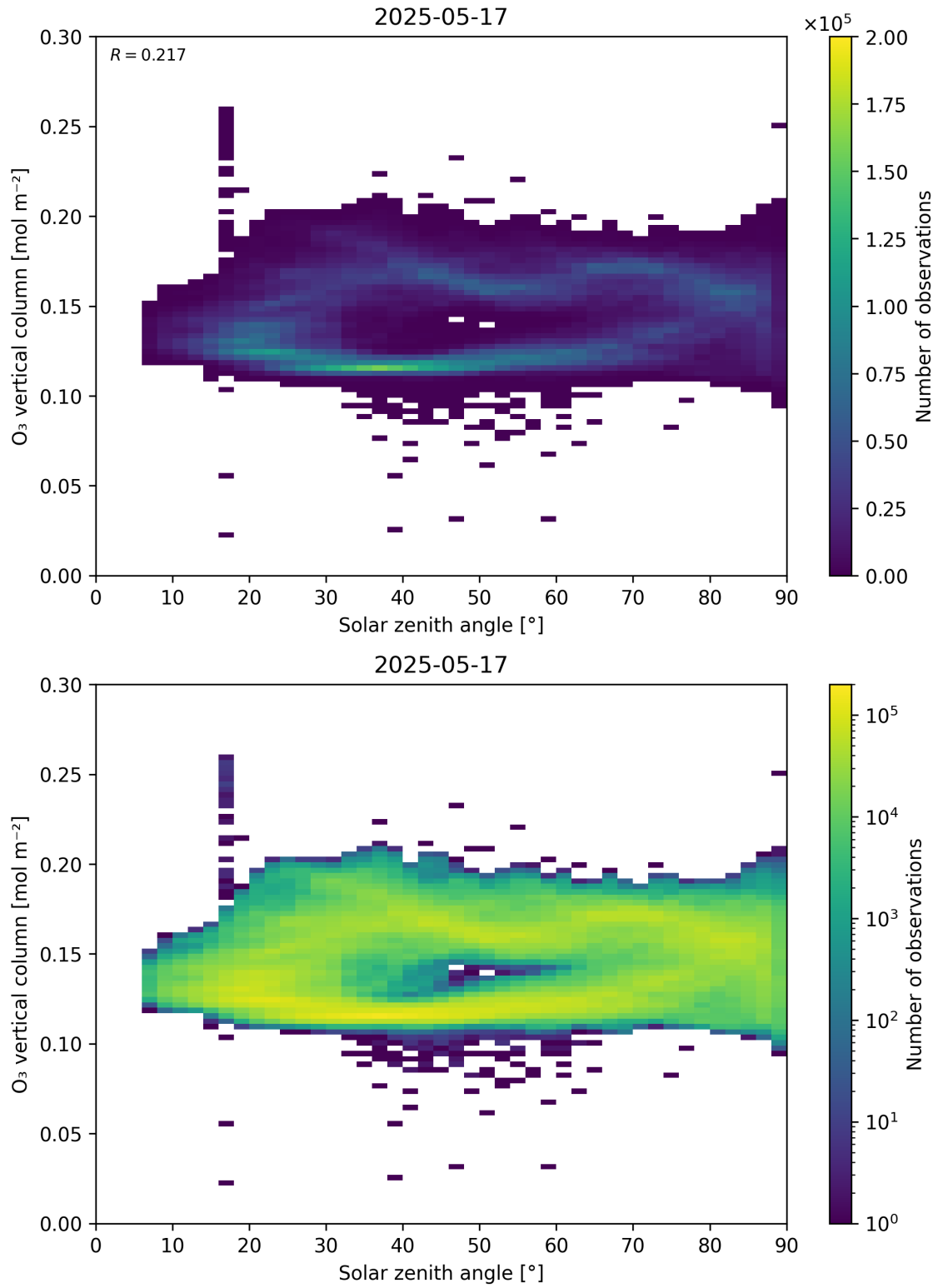
Figure 47: Scatter density plot of “Solar zenith angle” against “O 3 vertical column” for 2025-05-16 to 2025-05-18.
