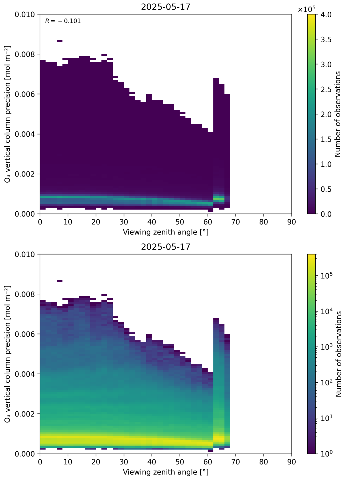
Figure 53: Scatter density plot of “Viewing zenith angle” against “O 3 vertical column precision” for 2025-05-16 to 2025-05-18.
