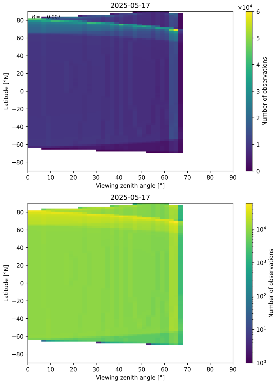
Figure 49: Scatter density plot of “Viewing zenith angle” against “Latitude” for 2025-05-16 to 2025-05-18.
