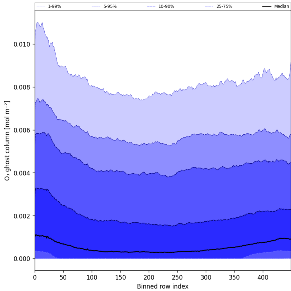
Figure 32: Along track statistics of “O 3 ghost column” for 2025-05-16 to 2025-05-18
