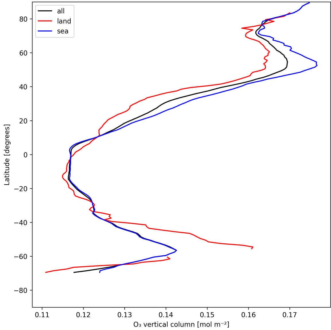
Figure 14: Zonal average of “O 3 vertical column” for 2025-05-16 to 2025-05-18.
