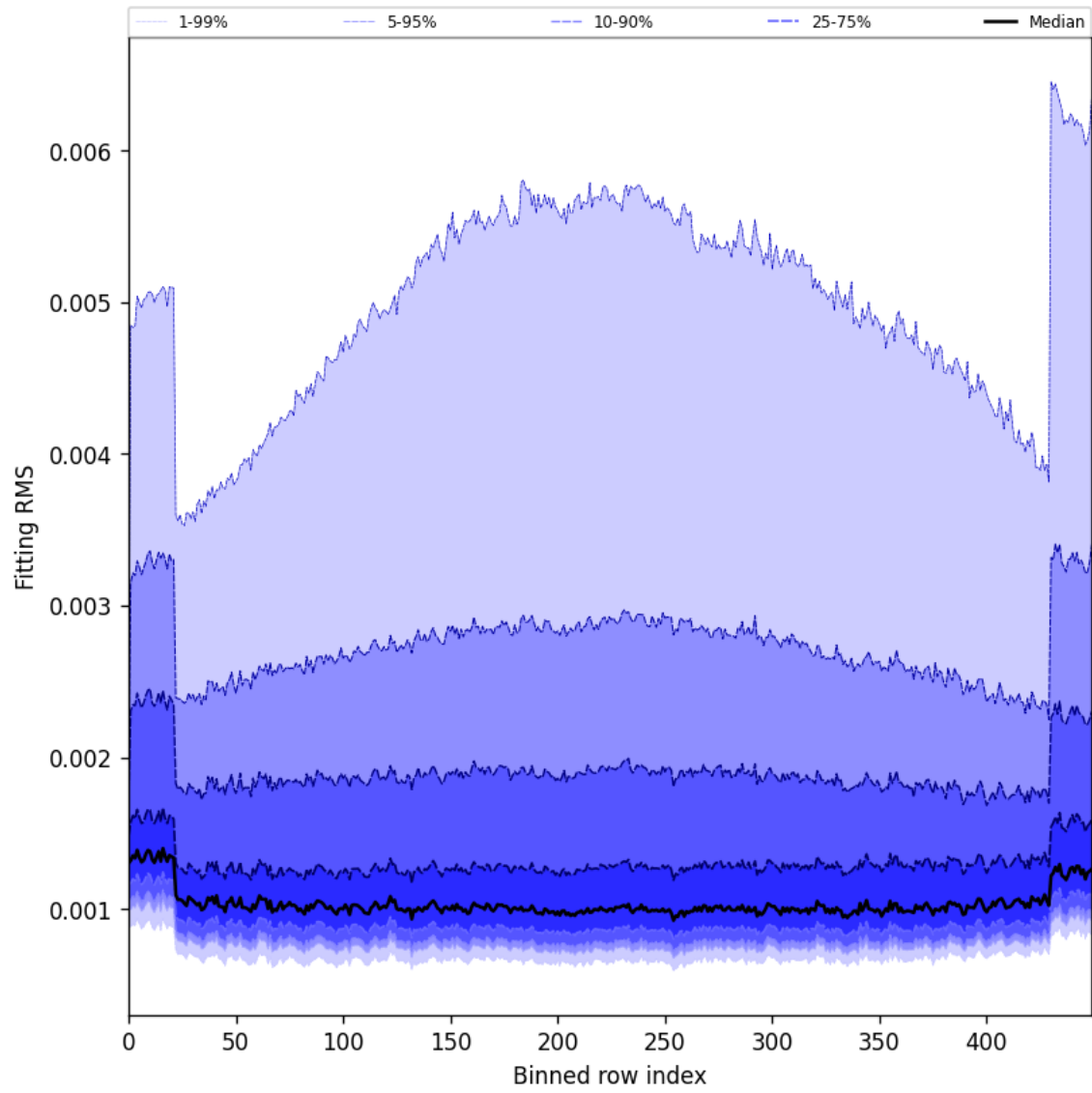
Figure 30: Along track statistics of “Fitting RMS” for 2025-05-16 to 2025-05-18
