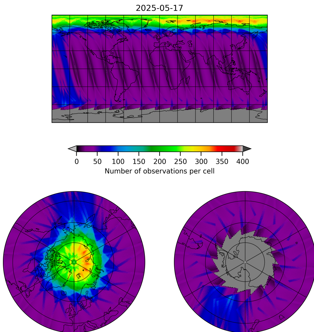
Figure 12: Map of the number of observations for 2025-05-16 to 2025-05-18
