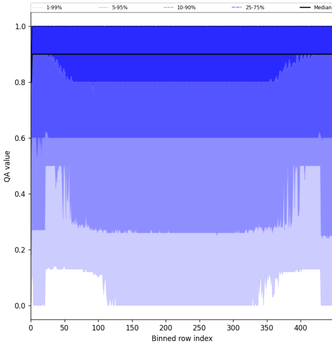
Figure 27: Along track statistics of “QA value” for 2025-05-16 to 2025-05-18
