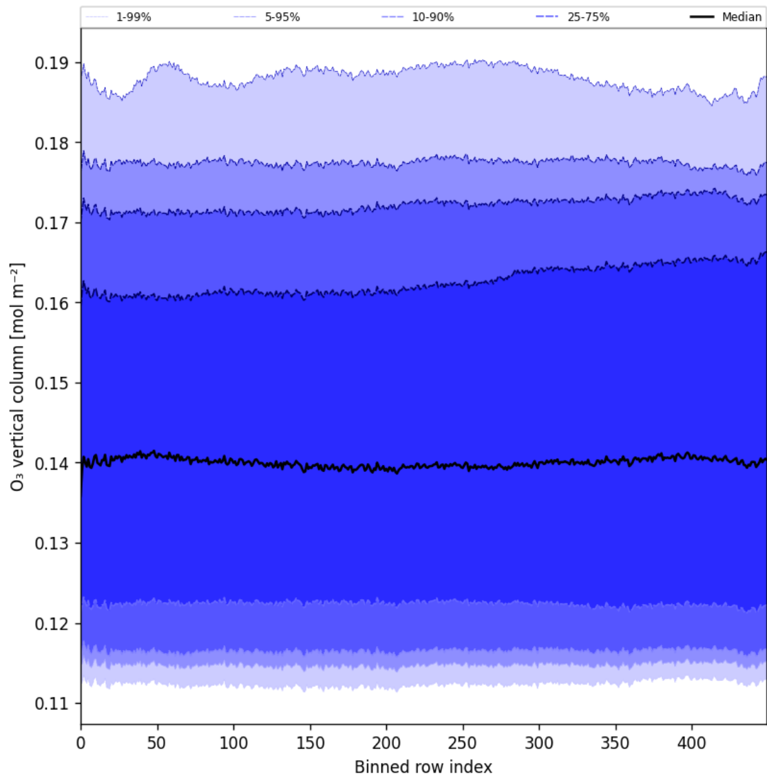
Figure 28: Along track statistics of “ \text{O}_3 vertical column” for 2025-05-16 to 2025-05-18
