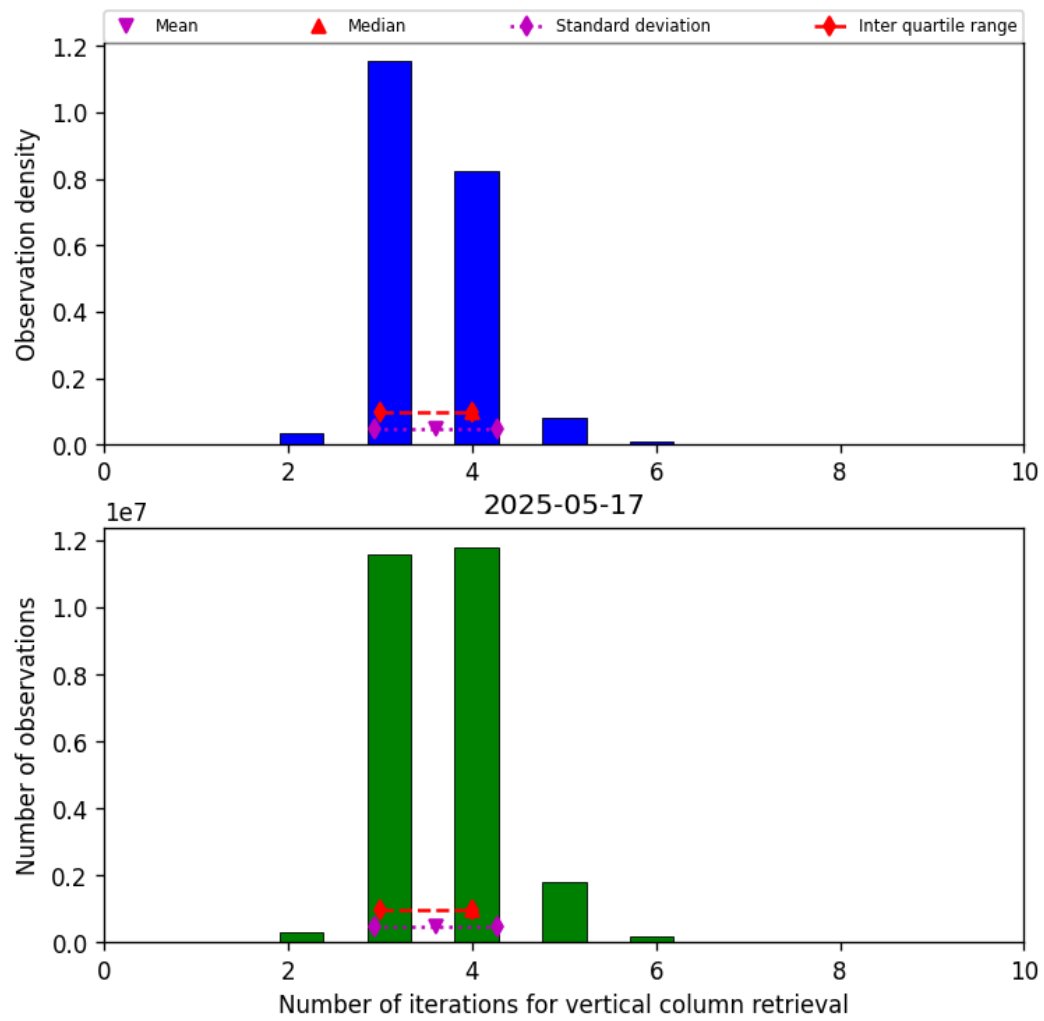
Figure 26: Histogram of “Number of iterations for vertical column retrieval” for 2025-05-16 to 2025-05-18
