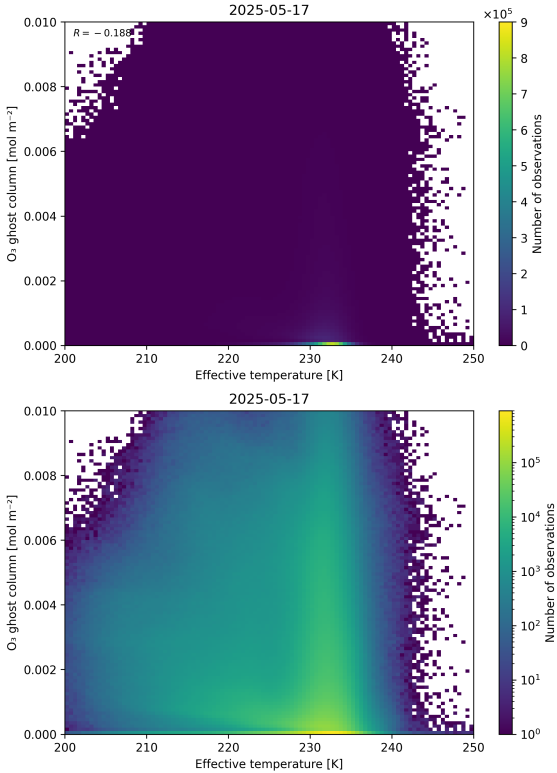
Figure 38: Scatter density plot of “Effective temperature” against “O 3 ghost column” for 2025-05-16 to 2025-05-18.
