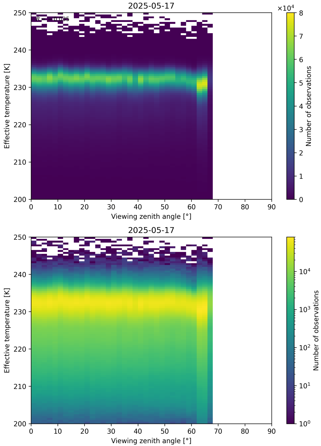
Figure 50: Scatter density plot of “Viewing zenith angle” against “Effective temperature” for 2025-05-16 to 2025-05-18.
