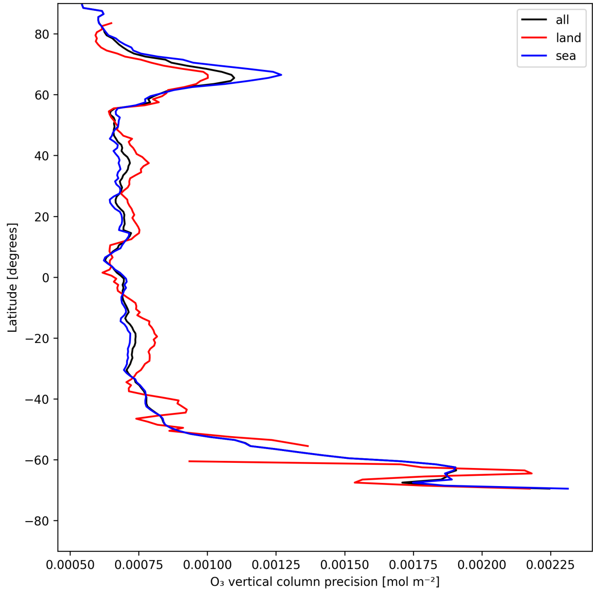
Figure 15: Zonal average of “O 3 vertical column precision” for 2025-05-16 to 2025-05-18.
