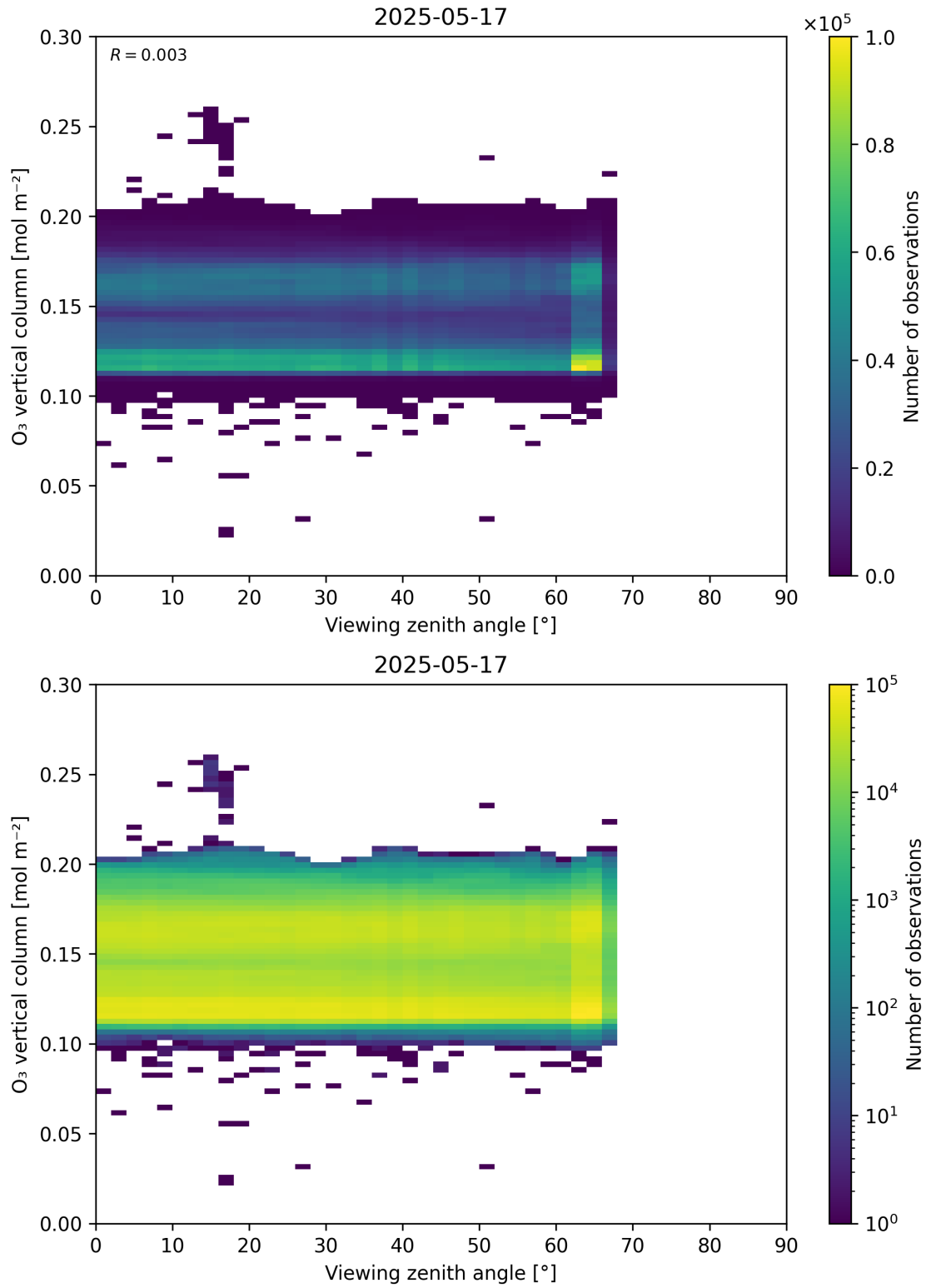
Figure 52: Scatter density plot of “Viewing zenith angle” against “O 3 vertical column” for 2025-05-16 to 2025-05-18.
