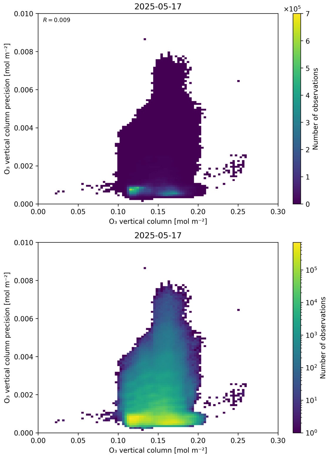
Figure 41: Scatter density plot of “O 3 vertical column” against “O 3 vertical column precision” for 2025-05-16 to 2025-05-18.
