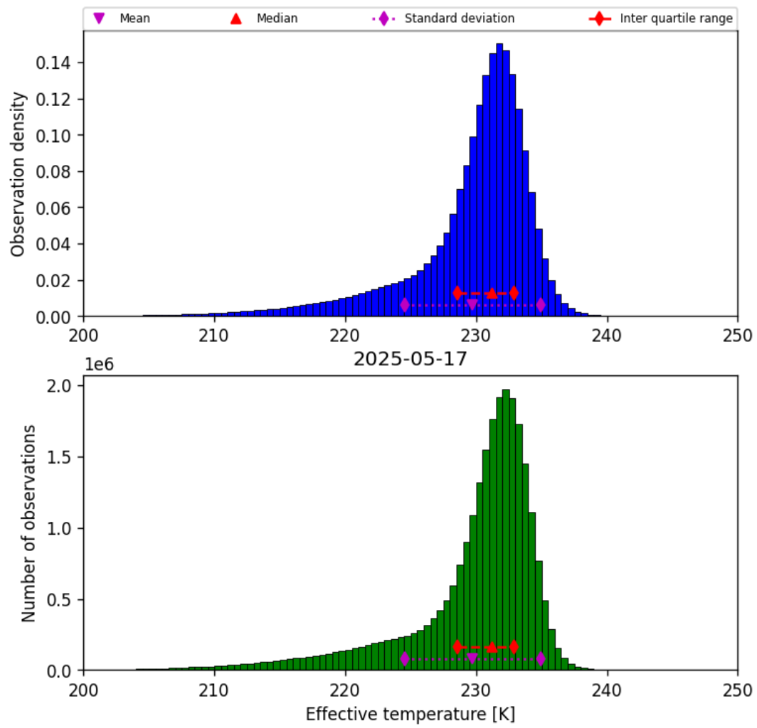
Figure 24: Histogram of “Effective temperature” for 2025-05-16 to 2025-05-18
