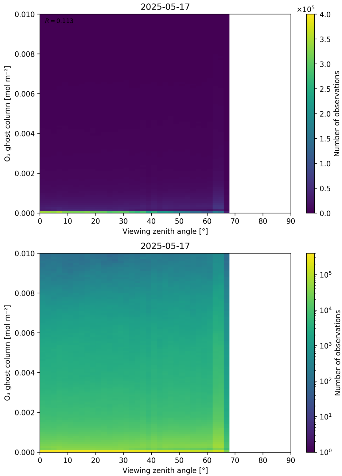
Figure 51: Scatter density plot of “Viewing zenith angle” against “O 3 ghost column” for 2025-05-16 to 2025-05-18.
