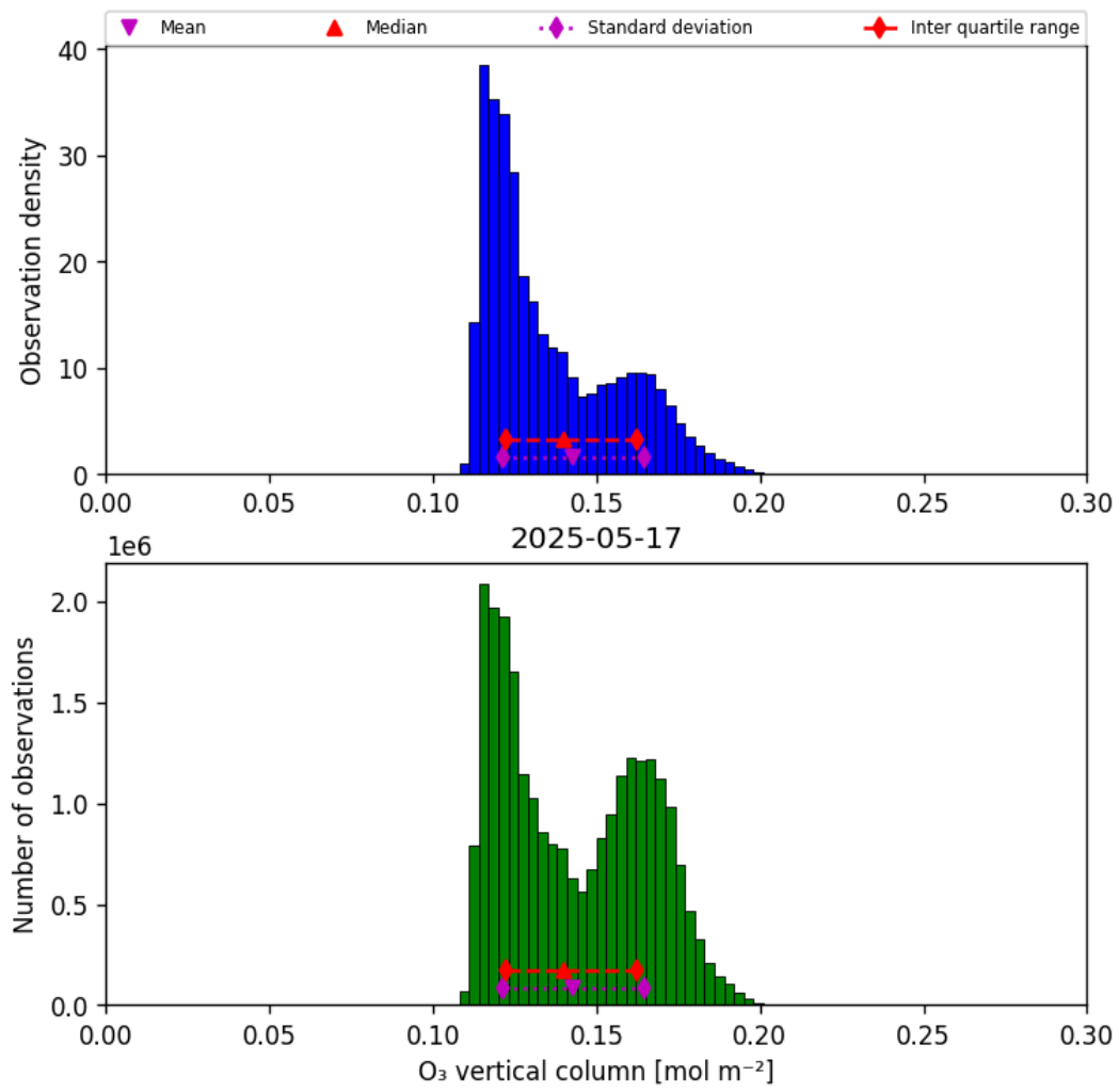
Figure 21: Histogram of “O 3 vertical column” for 2025-05-16 to 2025-05-18
