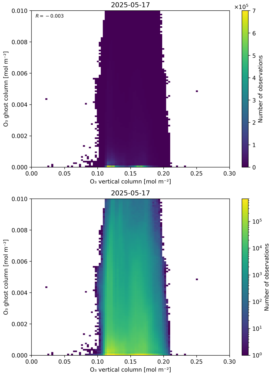
Figure 40: Scatter density plot of “O 3 vertical column” against “O 3 ghost column” for 2025-05-16 to 2025-05-18.
