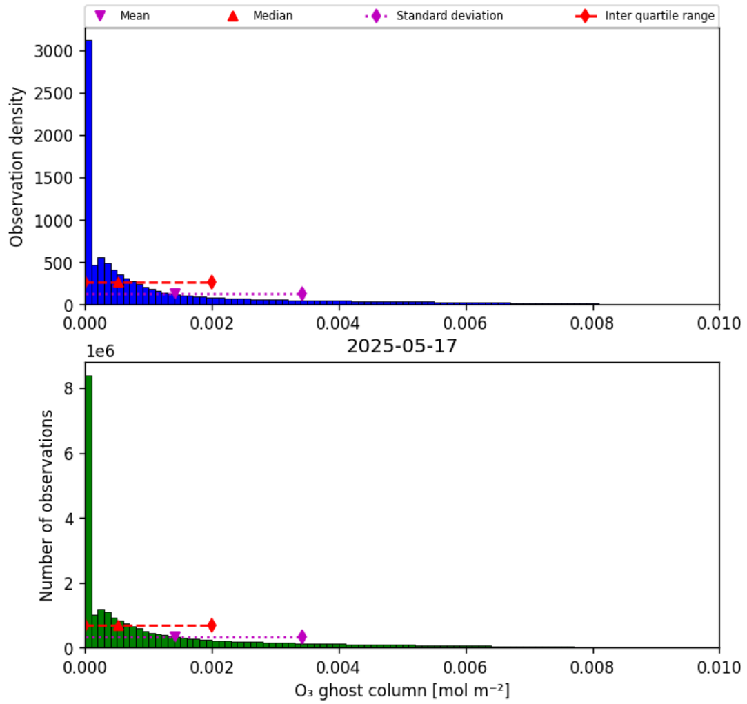
Figure 25: Histogram of “O 3 ghost column” for 2025-05-16 to 2025-05-18
