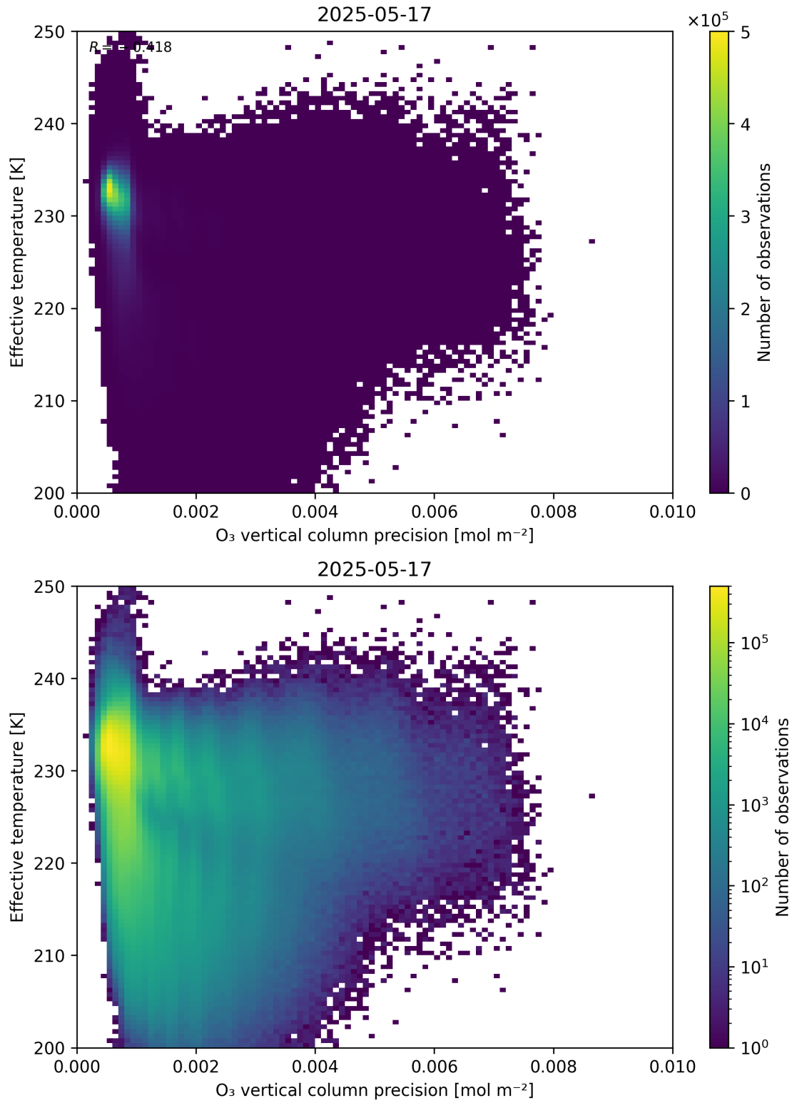
Figure 42: Scatter density plot of “O 3 vertical column precision” against “Effective temperature” for 2025-05-16 to 2025-05-18.
