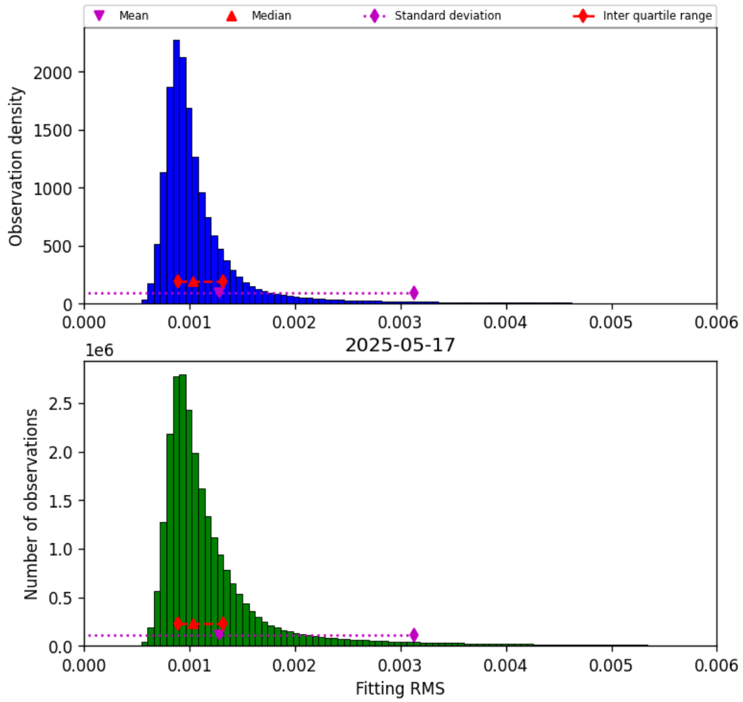
Figure 23: Histogram of “Fitting RMS” for 2025-05-16 to 2025-05-18
