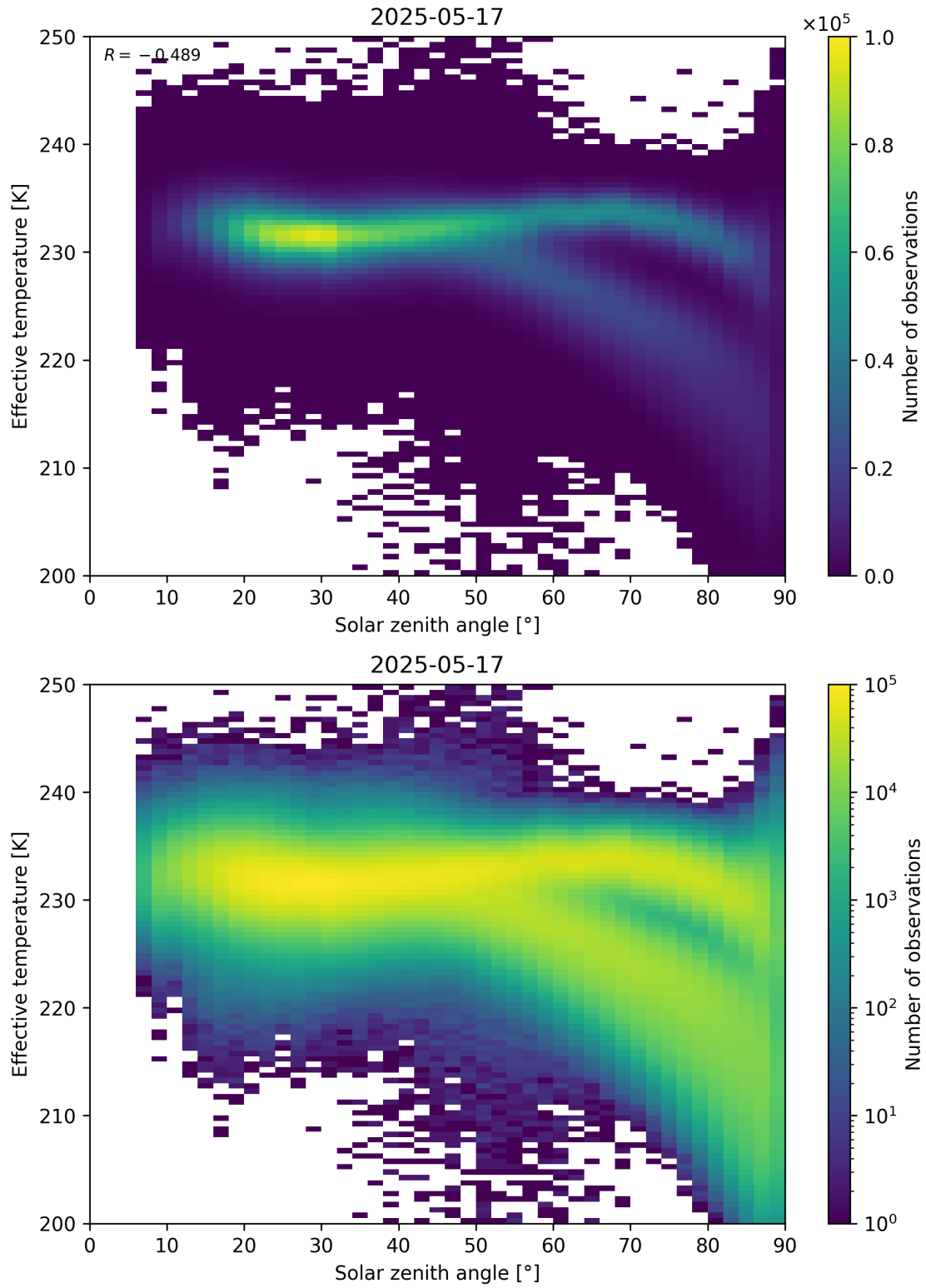
Figure 45: Scatter density plot of “Solar zenith angle” against “Effective temperature” for 2025-05-16 to 2025-05-18.
