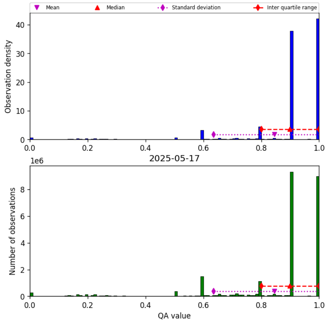
Figure 20: Histogram of “QA value” for 2025-05-16 to 2025-05-18
