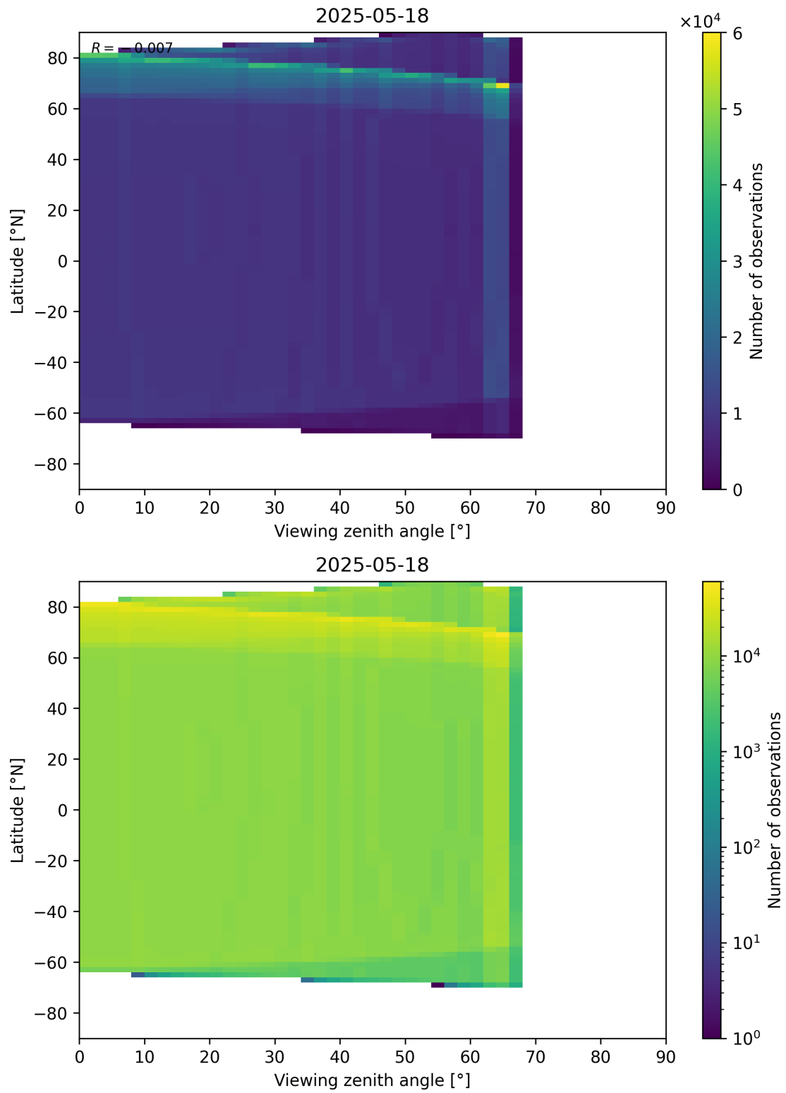
Figure 49: Scatter density plot of “Viewing zenith angle” against “Latitude” for 2025-05-17 to 2025-05-19.
