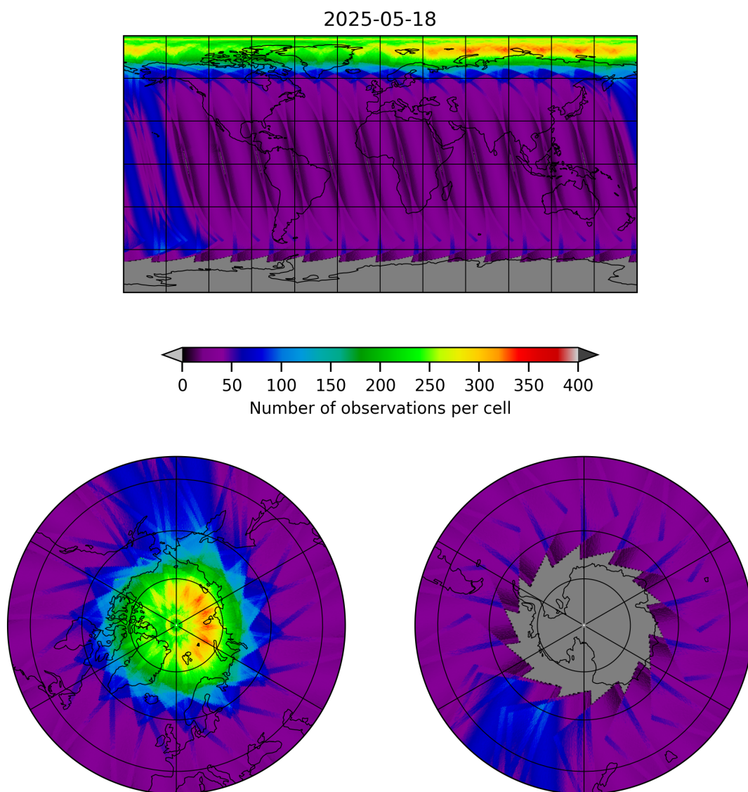
Figure 12: Map of the number of observations for 2025-05-17 to 2025-05-19
