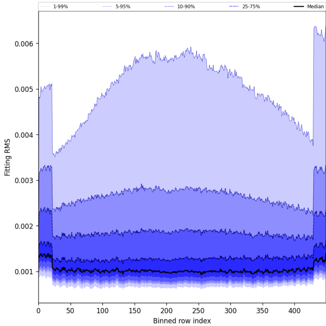
Figure 30: Along track statistics of “Fitting RMS” for 2025-05-17 to 2025-05-19
