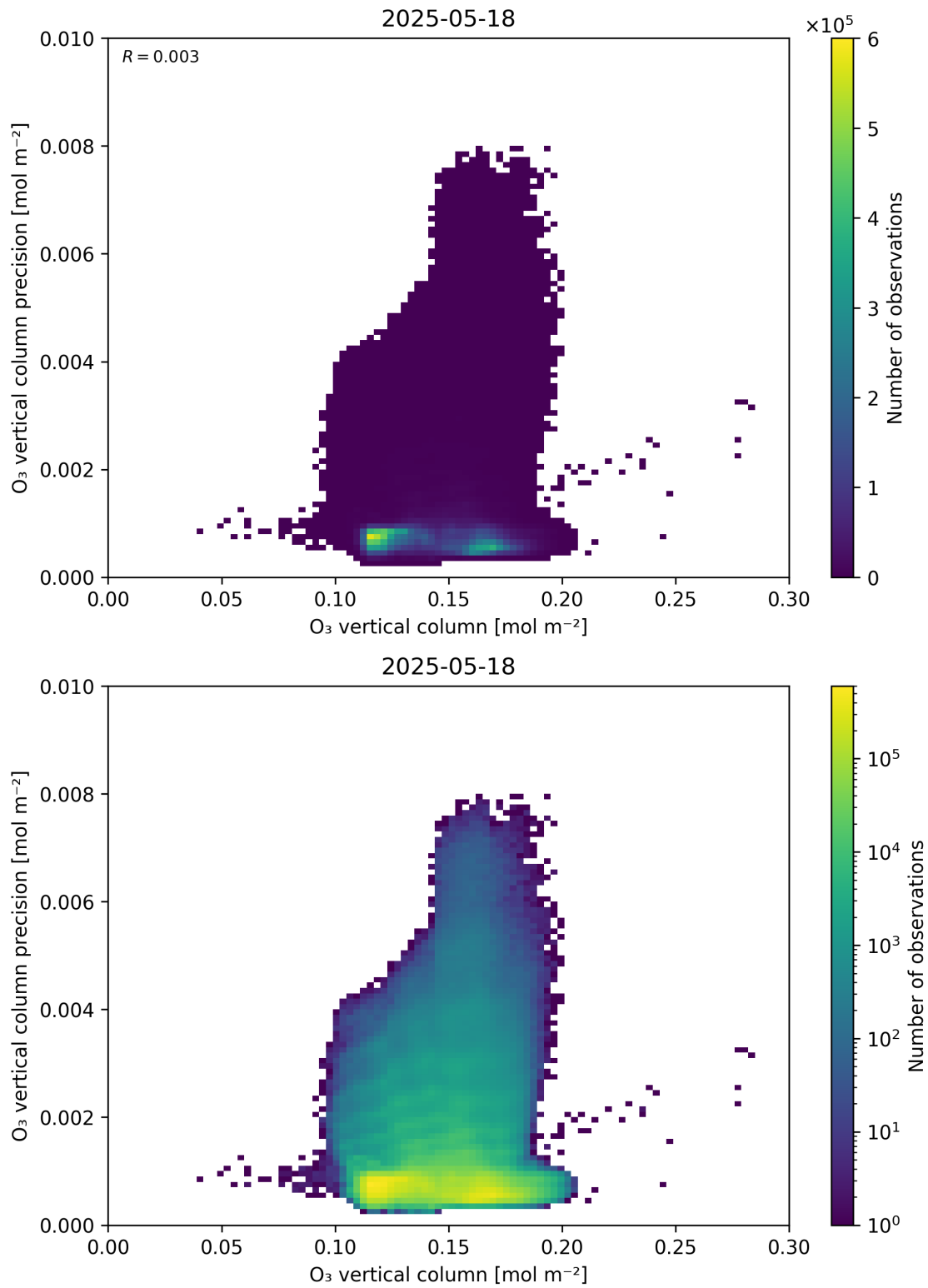
Figure 41: Scatter density plot of “O 3 vertical column” against “O 3 vertical column precision” for 2025-05-17 to 2025-05-19.
