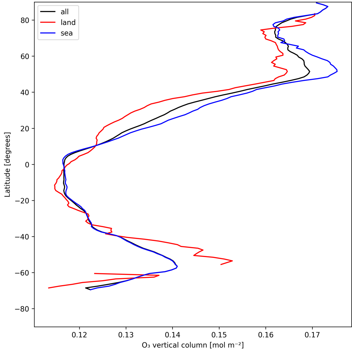
Figure 14: Zonal average of “O 3 vertical column” for 2025-05-17 to 2025-05-19.
