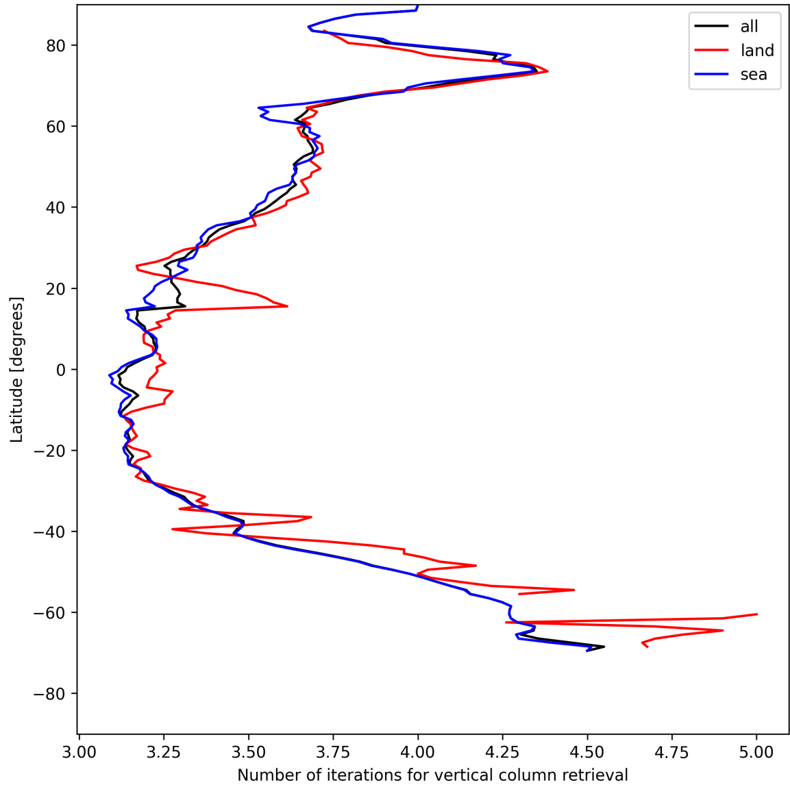
Figure 19: Zonal average of “Number of iterations for vertical column retrieval” for 2025-05-17 to 2025-05-19.
