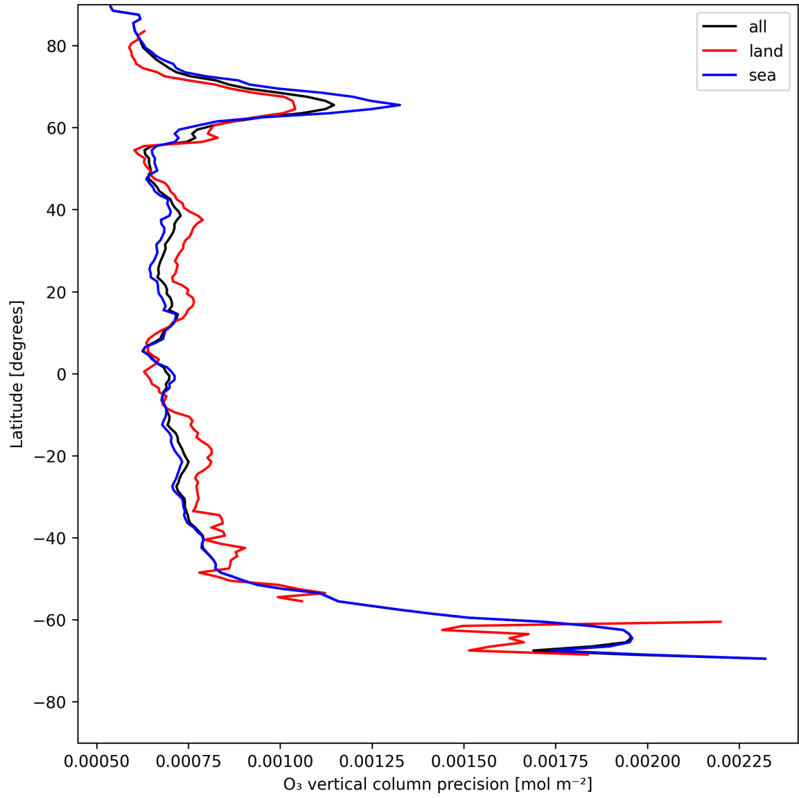
Figure 15: Zonal average of "O 3 vertical column precision" for 2025-05-17 to 2025-05-19.
