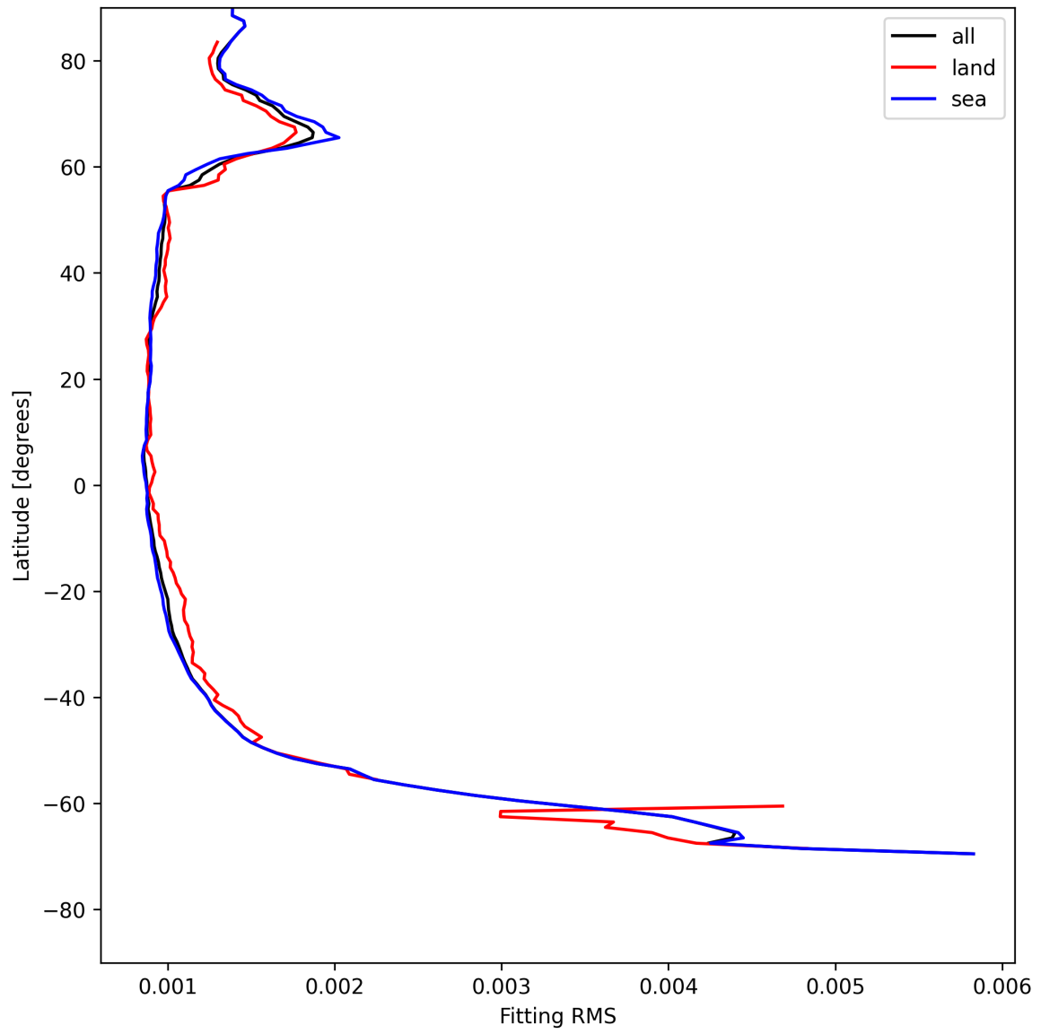
Figure 16: Zonal average of “Fitting RMS” for 2025-05-17 to 2025-05-19.
