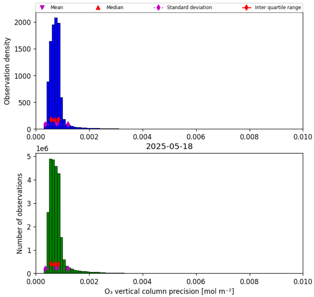
Figure 22: Histogram of “O 3 vertical column precision” for 2025-05-17 to 2025-05-19
