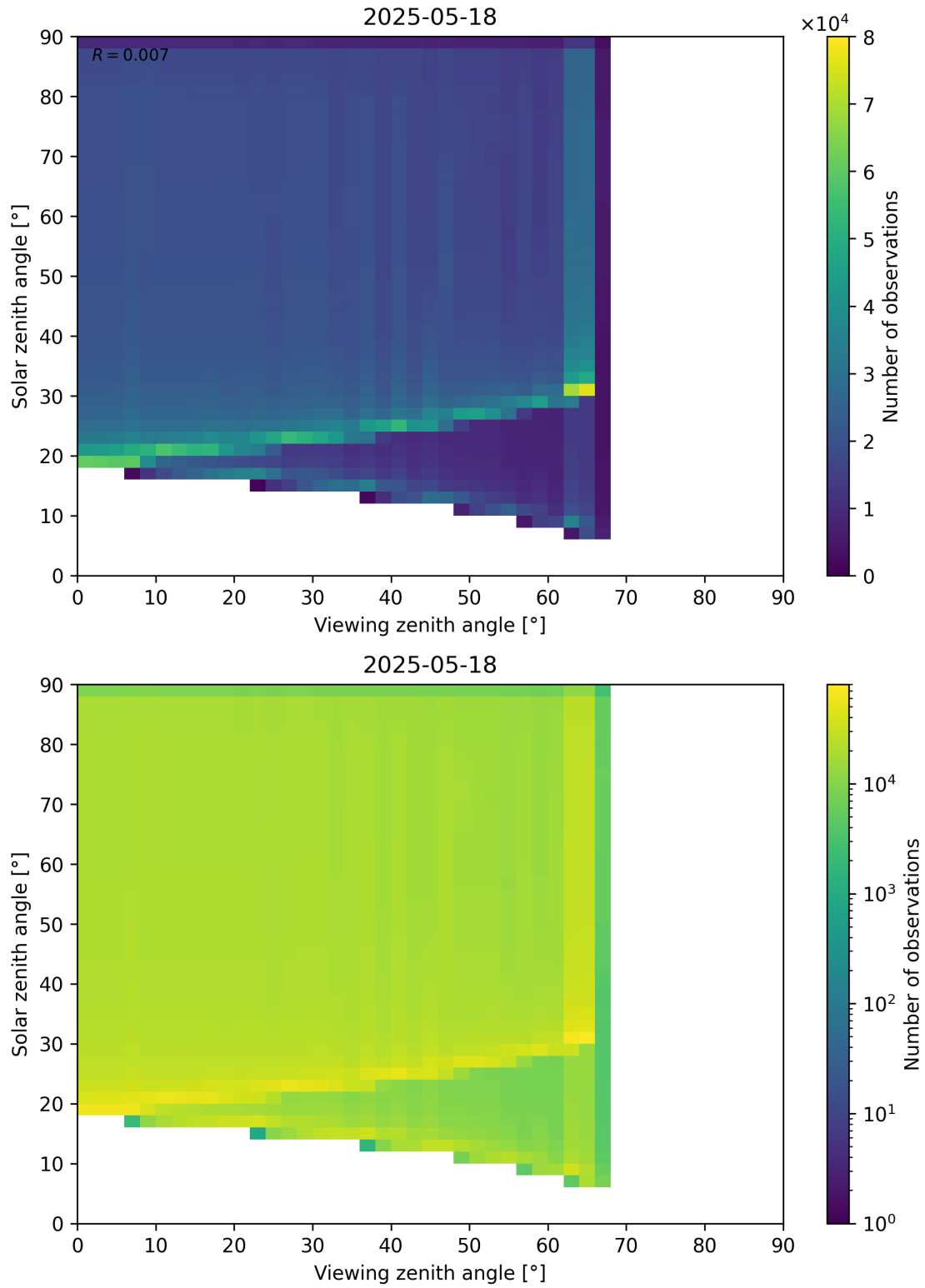
Figure 54: Scatter density plot of “Viewing zenith angle” against “Solar zenith angle” for 2025-05-17 to 2025-05-19.
