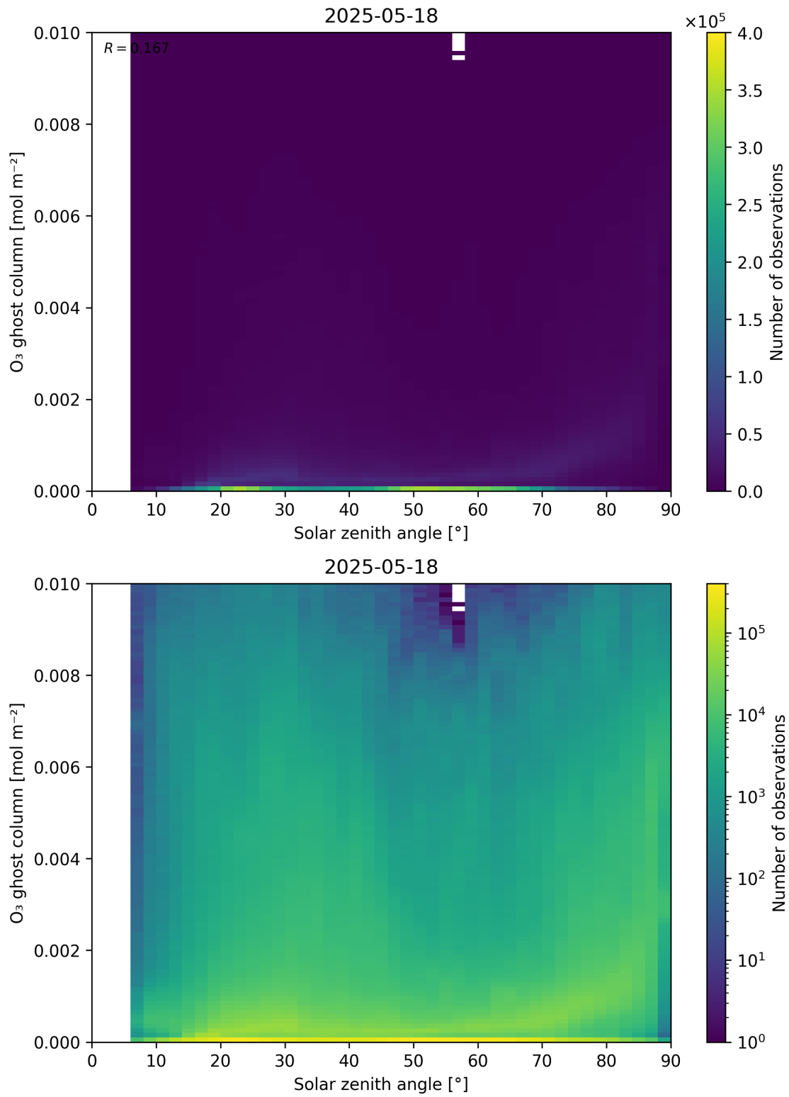
Figure 46: Scatter density plot of “Solar zenith angle” against “O 3 ghost column” for 2025-05-17 to 2025-05-19.
