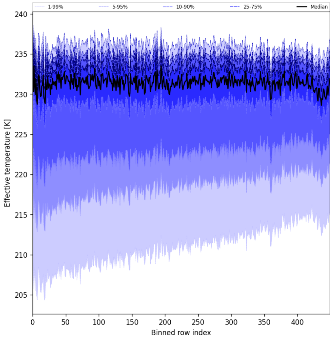
Figure 31: Along track statistics of “Effective temperature” for 2025-05-17 to 2025-05-19
