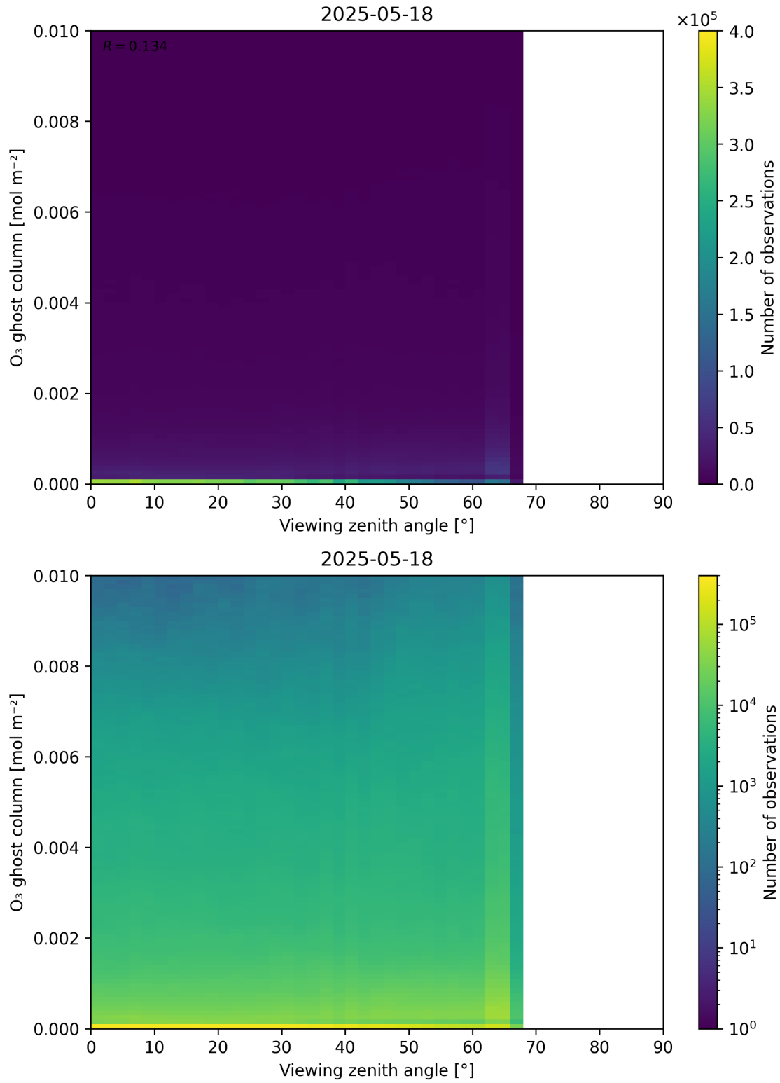
Figure 51: Scatter density plot of “Viewing zenith angle” against “O 3 ghost column” for 2025-05-17 to 2025-05-19.
