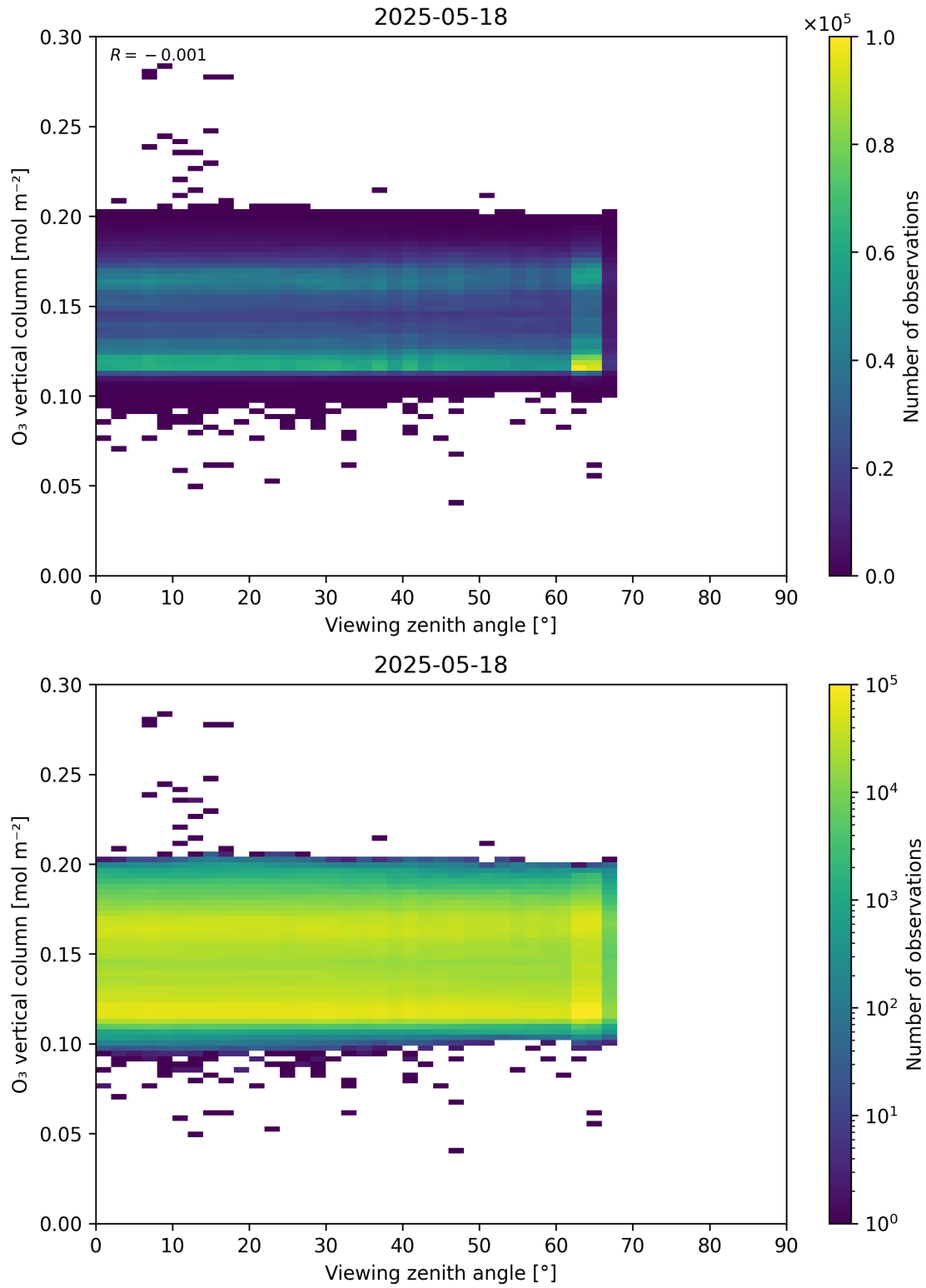
Figure 52: Scatter density plot of “Viewing zenith angle” against “O 3 vertical column” for 2025-05-17 to 2025-05-19.
