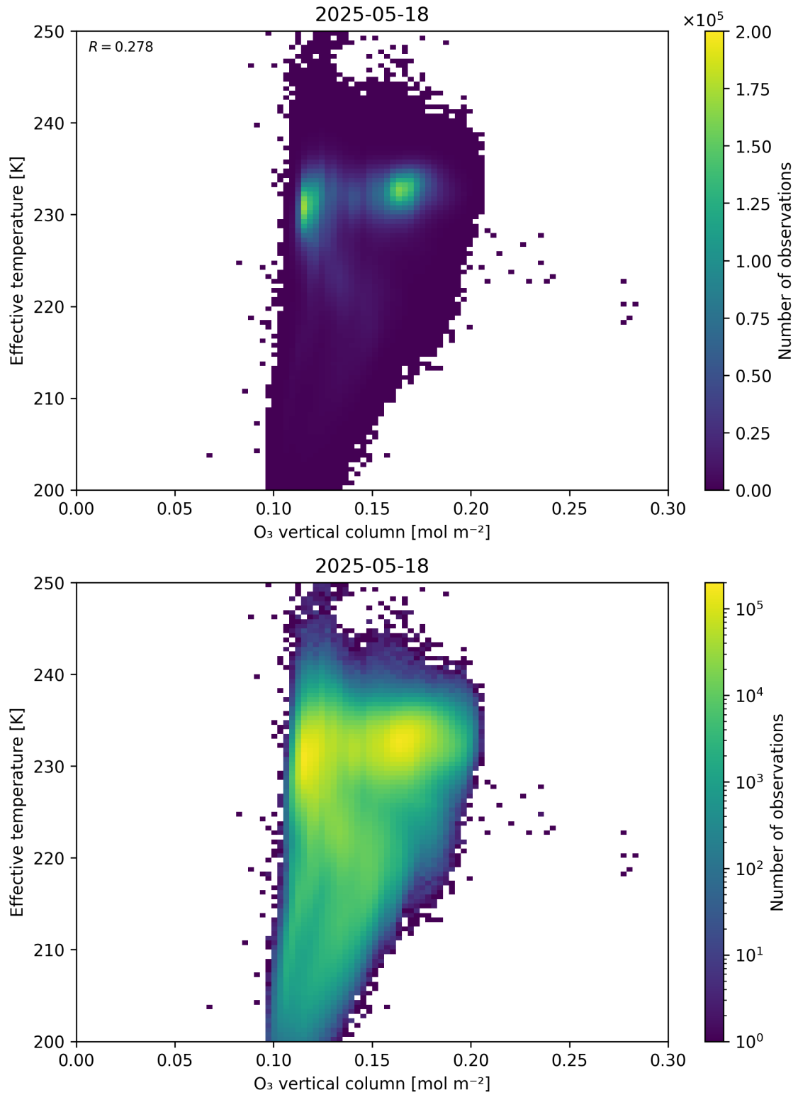
Figure 39: Scatter density plot of “O 3 vertical column” against “Effective temperature” for 2025-05-17 to 2025-05-19.
