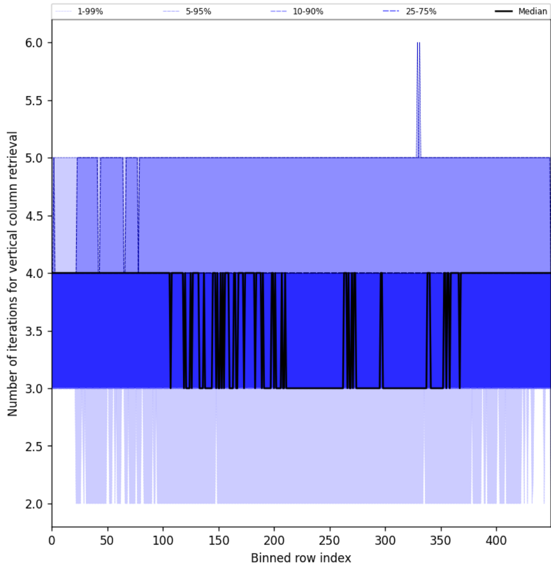
Figure 33: Along track statistics of “Number of iterations for vertical column retrieval” for 2025-05-17 to 2025-05-19
