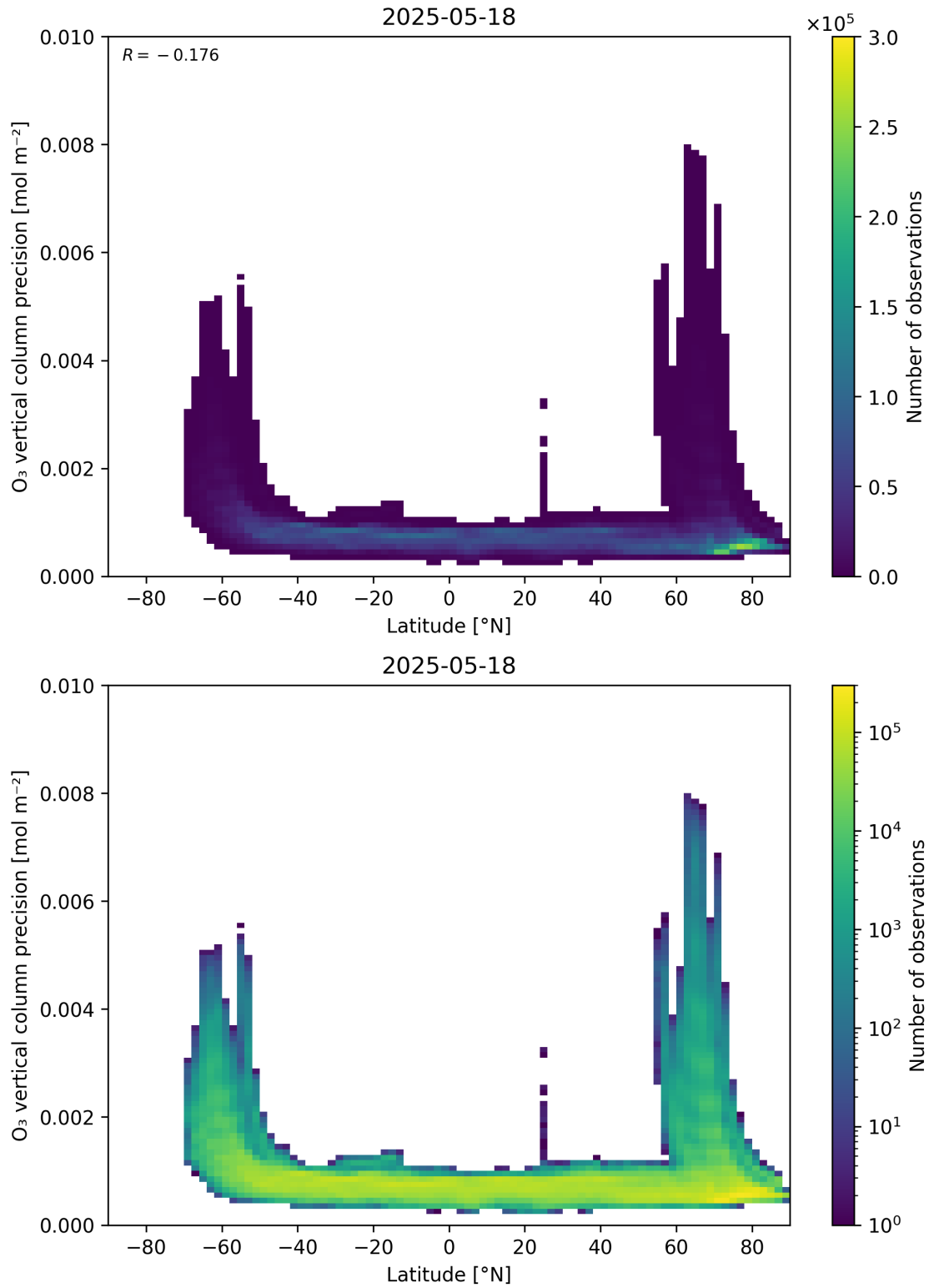
Figure 37: Scatter density plot of “Latitude” against “O 3 vertical column precision” for 2025-05-17 to 2025-05-19.
