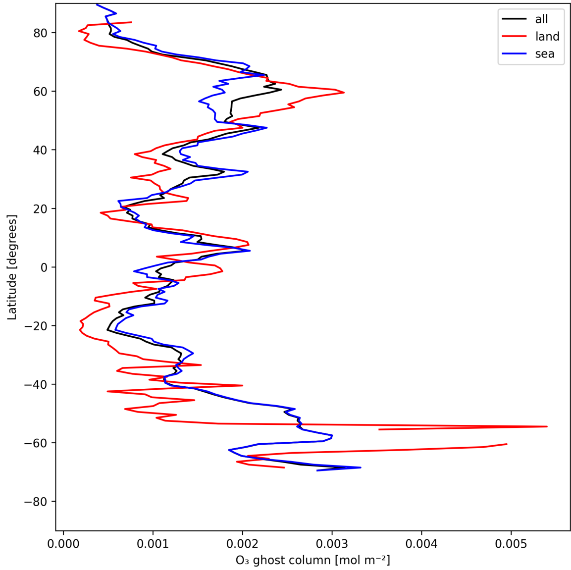
Figure 18: Zonal average of "O 3 ghost column" for 2025-05-17 to 2025-05-19.
