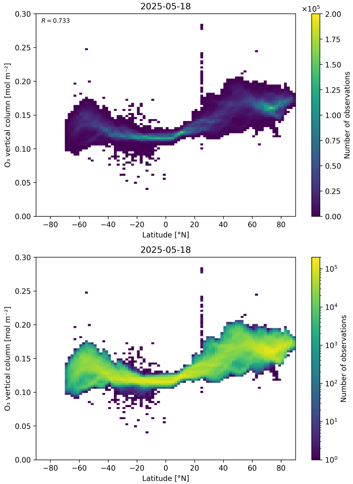
Figure 36: Scatter density plot of “Latitude” against “O 3 vertical column” for 2025-05-17 to 2025-05-19.
