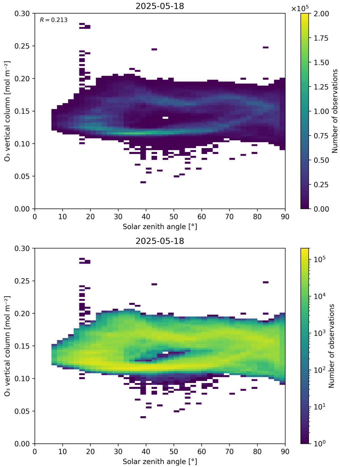
Figure 47: Scatter density plot of “Solar zenith angle” against “O 3 vertical column” for 2025-05-17 to 2025-05-19.
