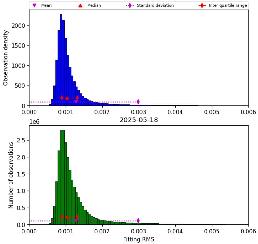
Figure 23: Histogram of “Fitting RMS” for 2025-05-17 to 2025-05-19
