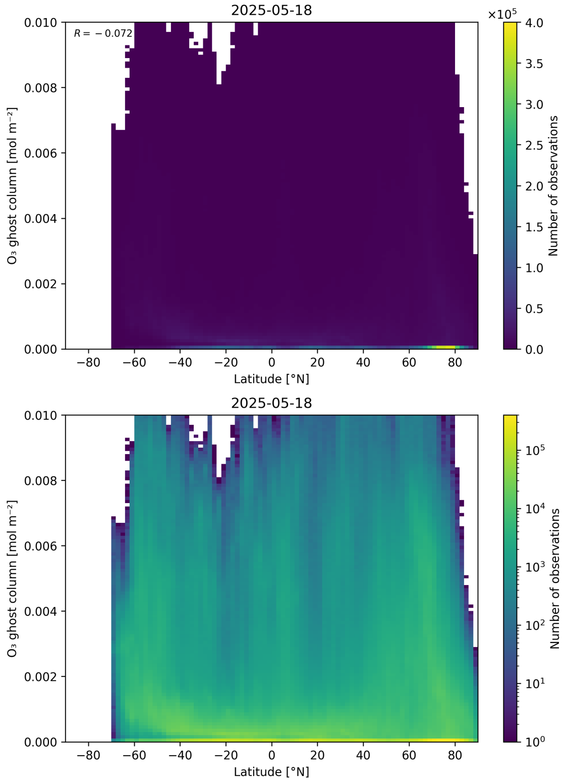
Figure 35: Scatter density plot of “Latitude” against “O 3 ghost column” for 2025-05-17 to 2025-05-19.
