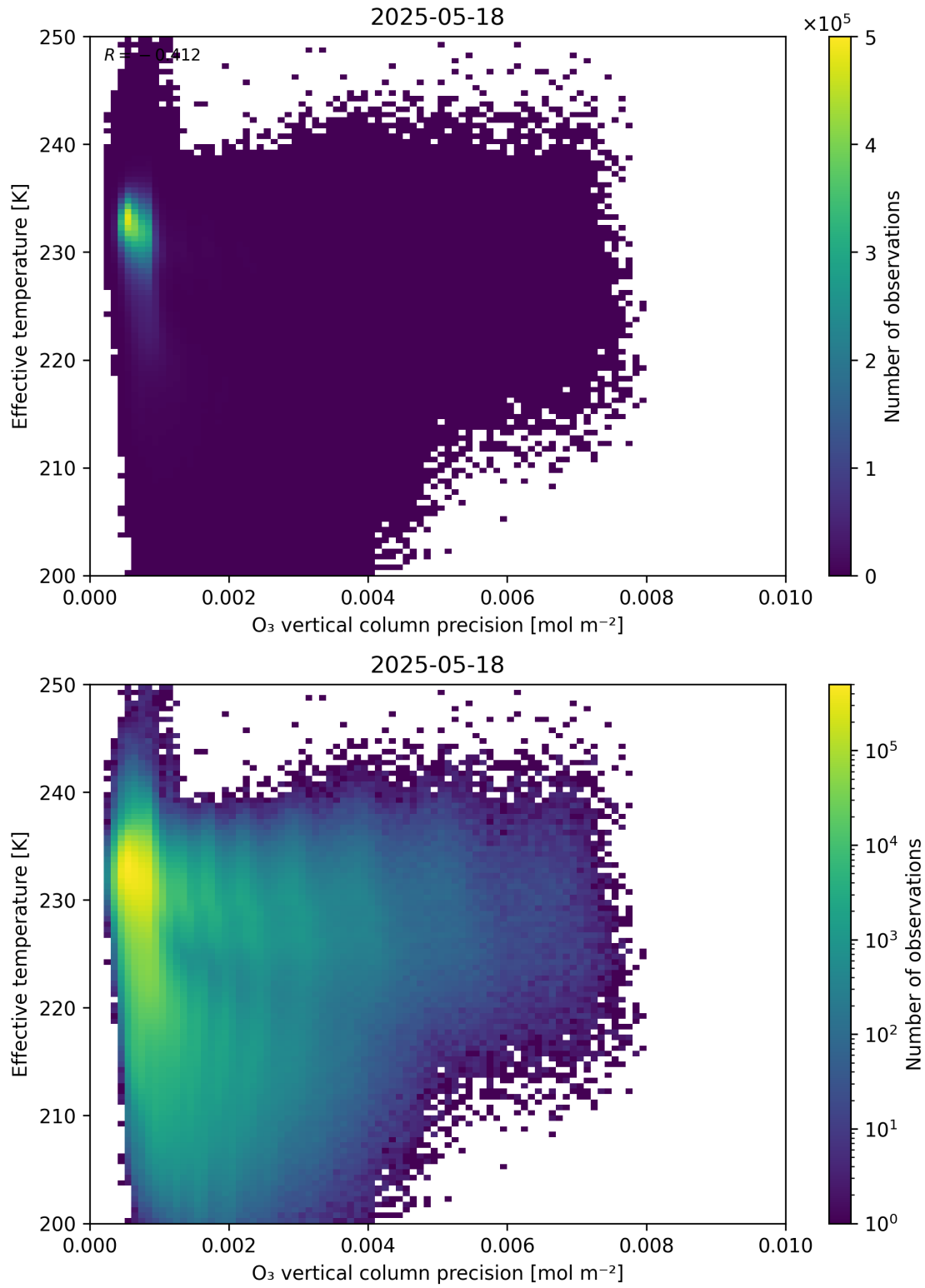
Figure 42: Scatter density plot of “O 3 vertical column precision” against “Effective temperature” for 2025-05-17 to 2025-05-19.
