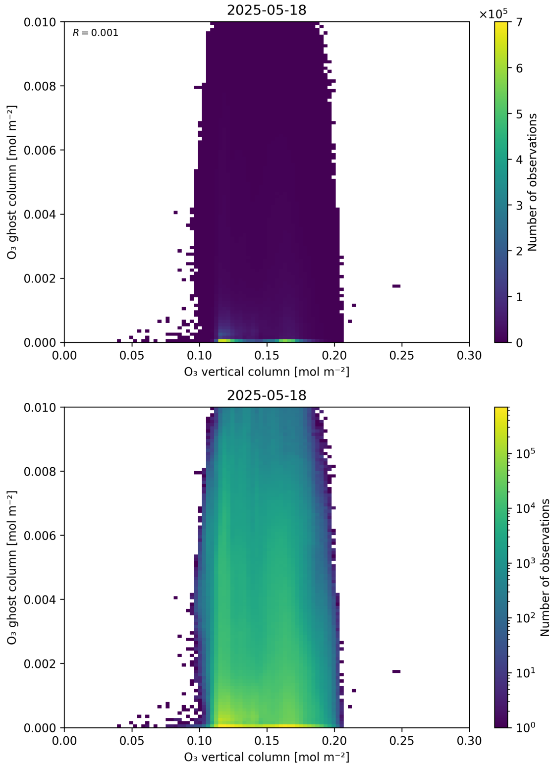
Figure 40: Scatter density plot of “O 3 vertical column” against “O 3 ghost column” for 2025-05-17 to 2025-05-19.
