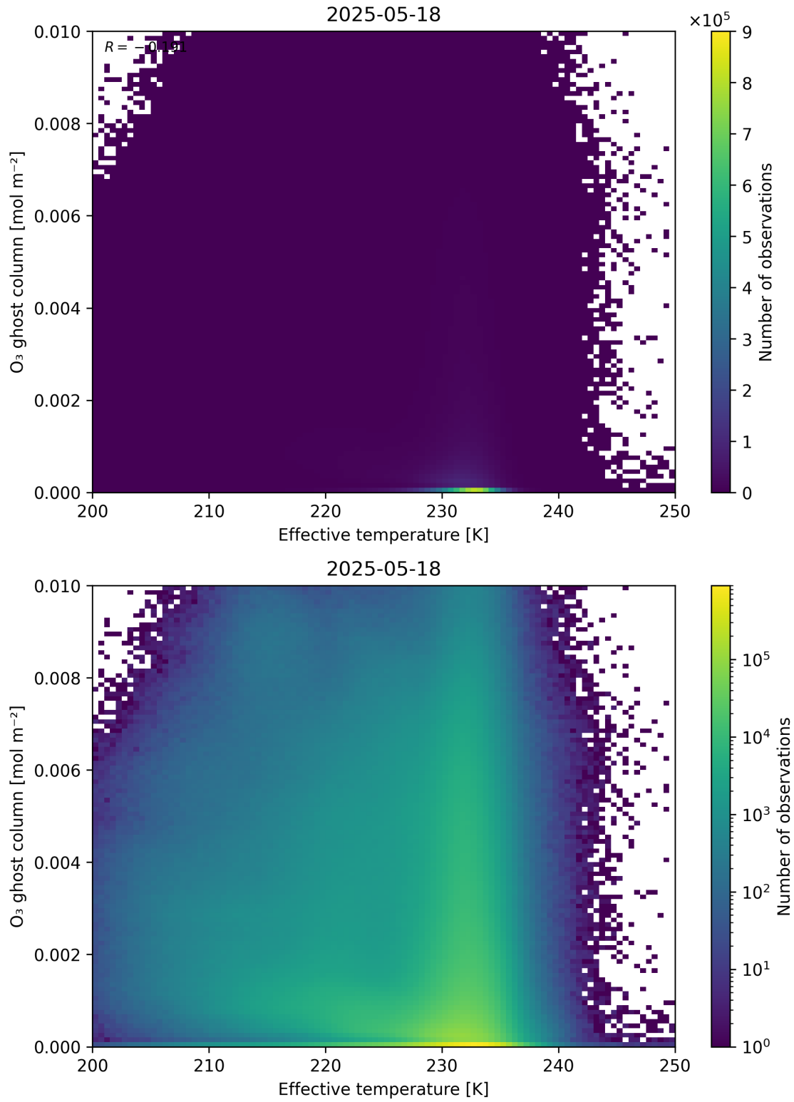
Figure 38: Scatter density plot of “Effective temperature” against “O 3 ghost column” for 2025-05-17 to 2025-05-19.
