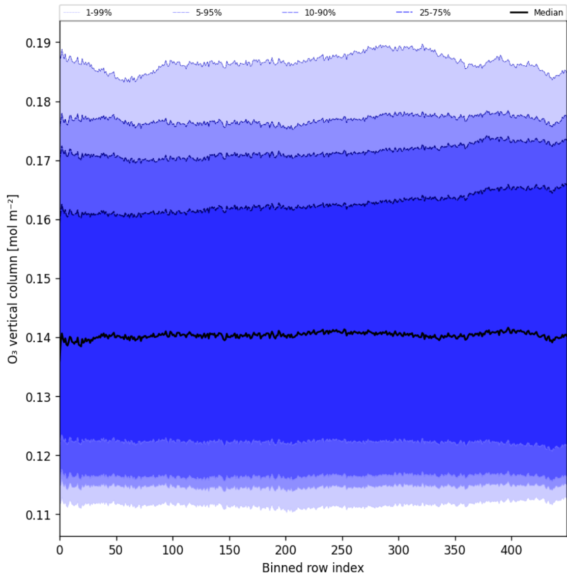
Figure 28: Along track statistics of “ O_3 vertical column” for 2025-05-17 to 2025-05-19
