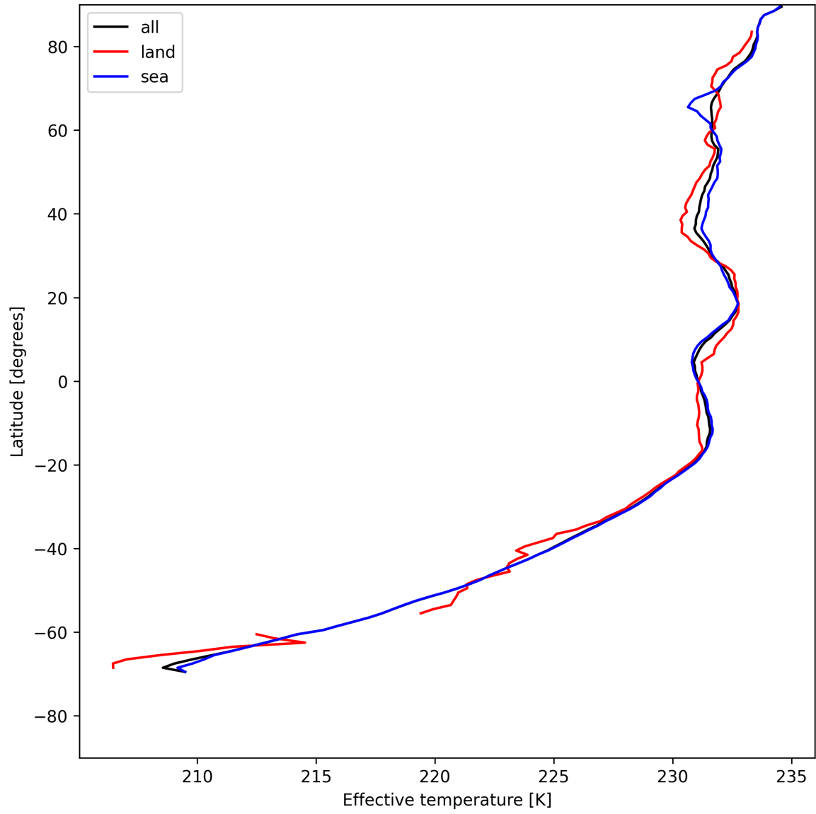
Figure 17: Zonal average of "Effective temperature" for 2025-05-17 to 2025-05-19.
