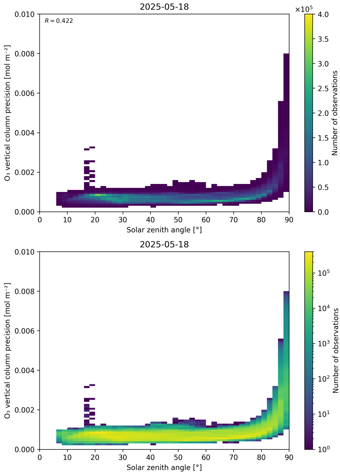
Figure 48: Scatter density plot of “Solar zenith angle” against “O 3 vertical column precision” for 2025-05-17 to 2025-05-19.
