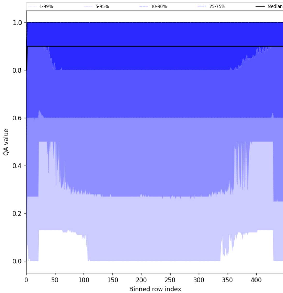
Figure 27: Along track statistics of “QA value” for 2025-05-17 to 2025-05-19
