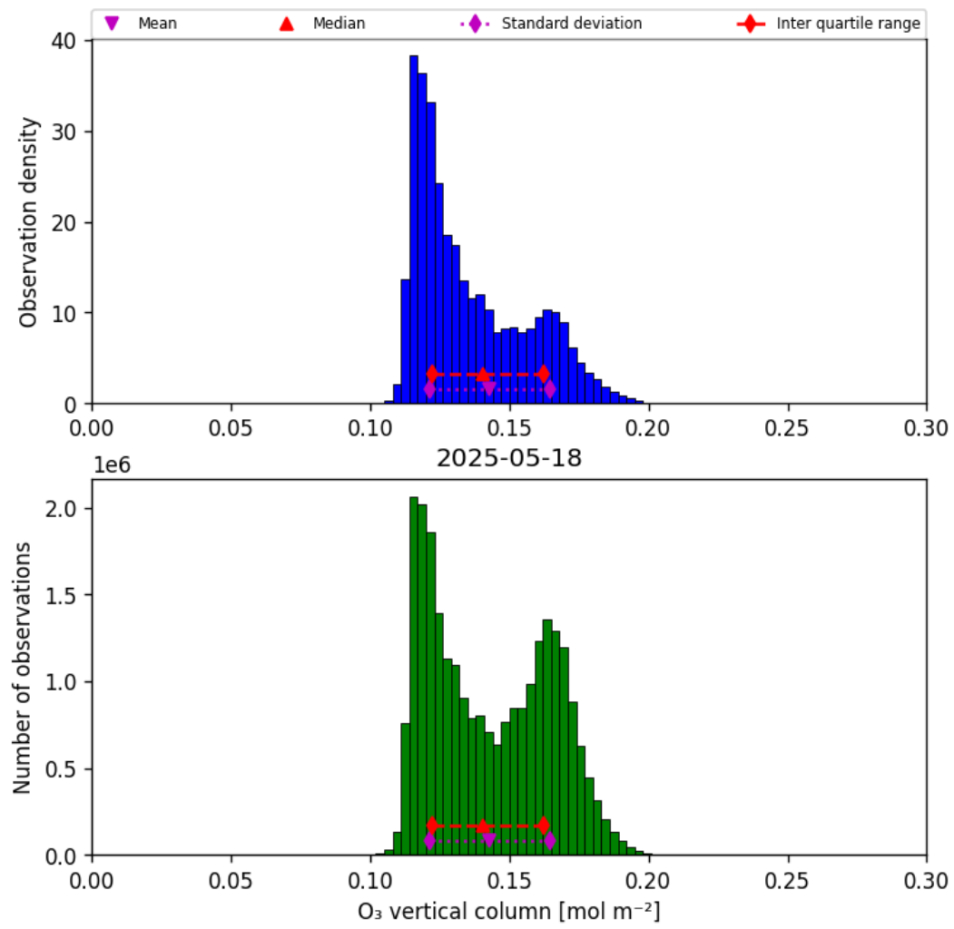
Figure 21: Histogram of “O 3 vertical column” for 2025-05-17 to 2025-05-19
