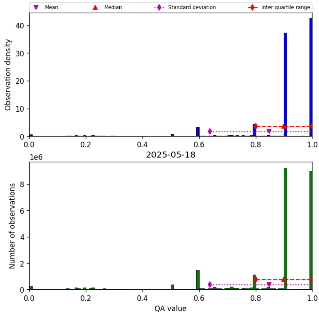
Figure 20: Histogram of “QA value” for 2025-05-17 to 2025-05-19
