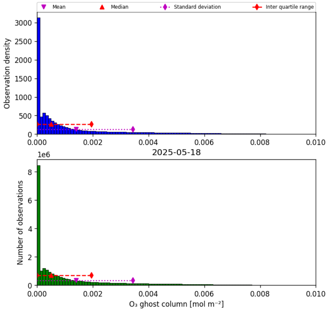
Figure 25: Histogram of “O 3 ghost column” for 2025-05-17 to 2025-05-19
