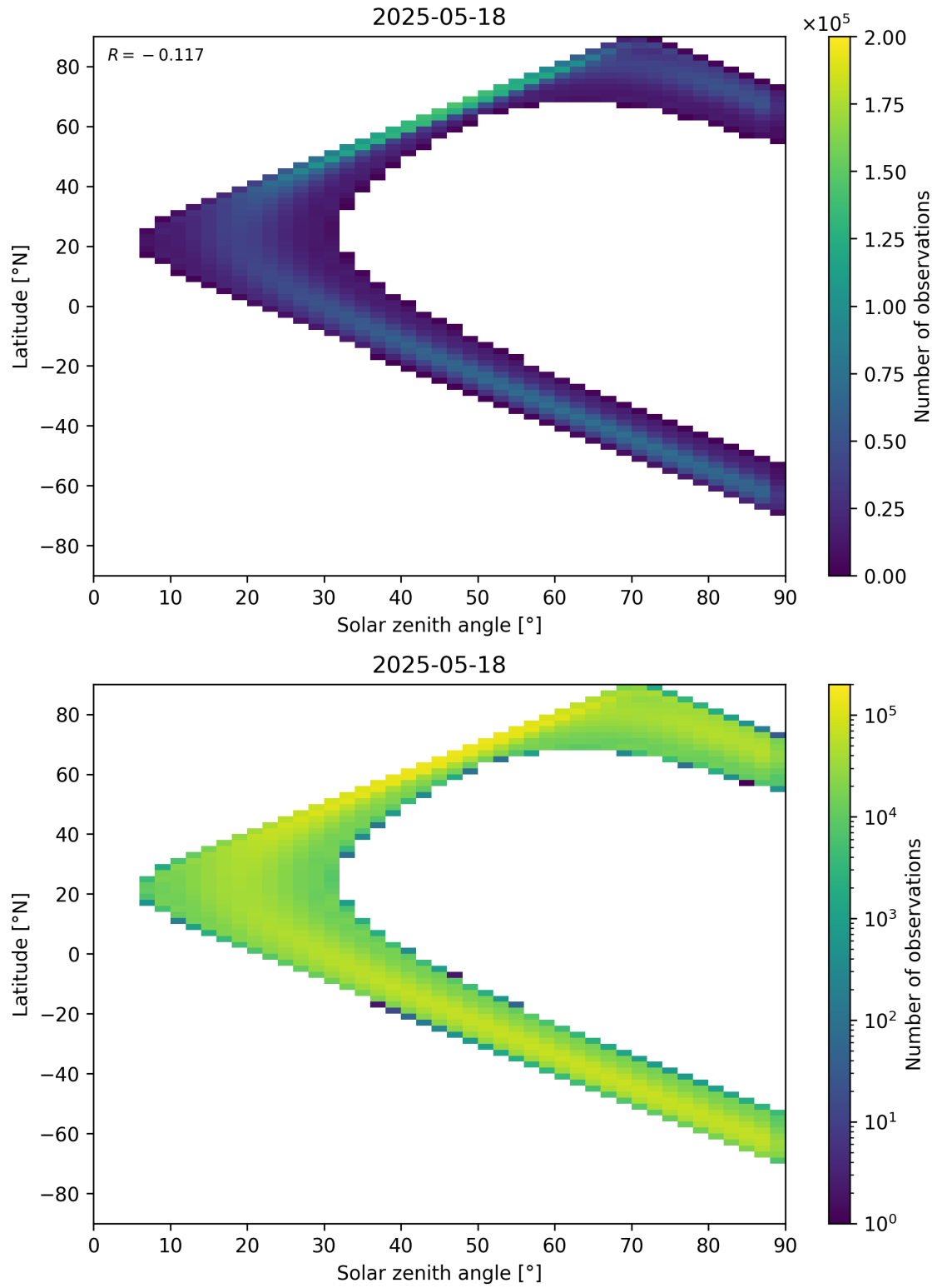
Figure 44: Scatter density plot of “Solar zenith angle” against “Latitude” for 2025-05-17 to 2025-05-19.
