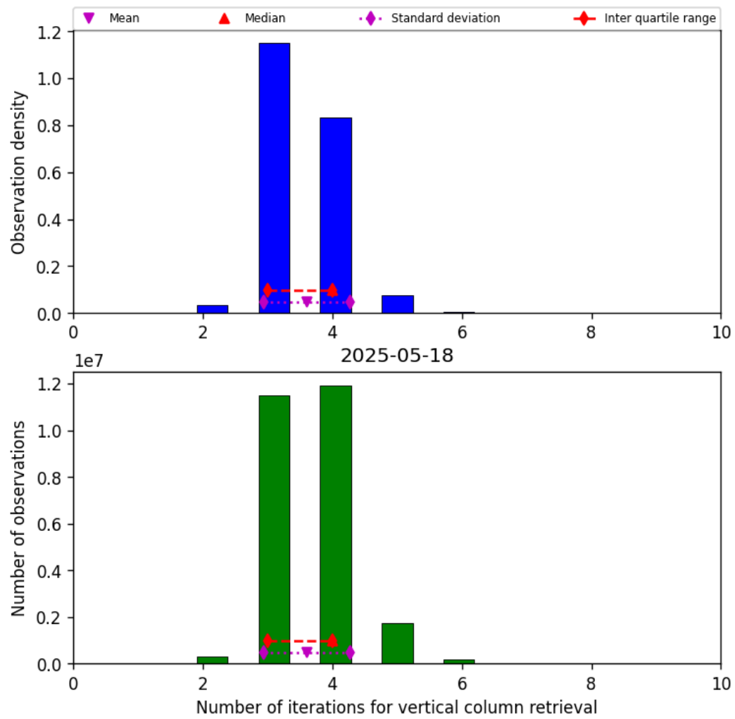
Figure 26: Histogram of “Number of iterations for vertical column retrieval” for 2025-05-17 to 2025-05-19
