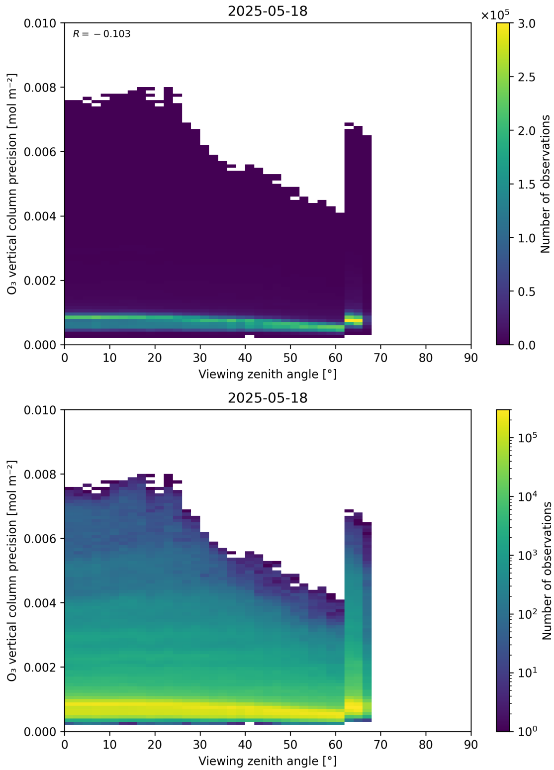
Figure 53: Scatter density plot of “Viewing zenith angle” against “O 3 vertical column precision” for 2025-05-17 to 2025-05-19.
