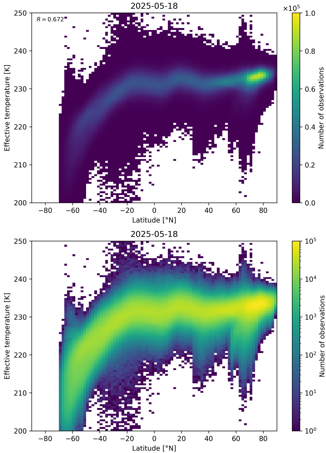
Figure 34: Scatter density plot of “Latitude” against “Effective temperature” for 2025-05-17 to 2025-05-19.
