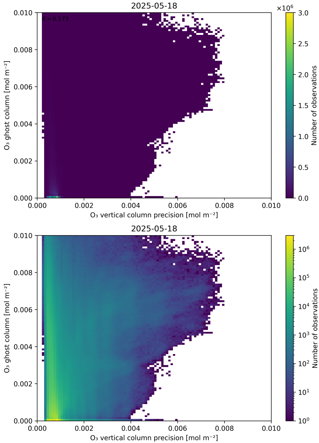
Figure 43: Scatter density plot of “ \text{O}_3 vertical column precision” against “ \text{O}_3 ghost column” for 2025-05-17 to 2025-05-19.
