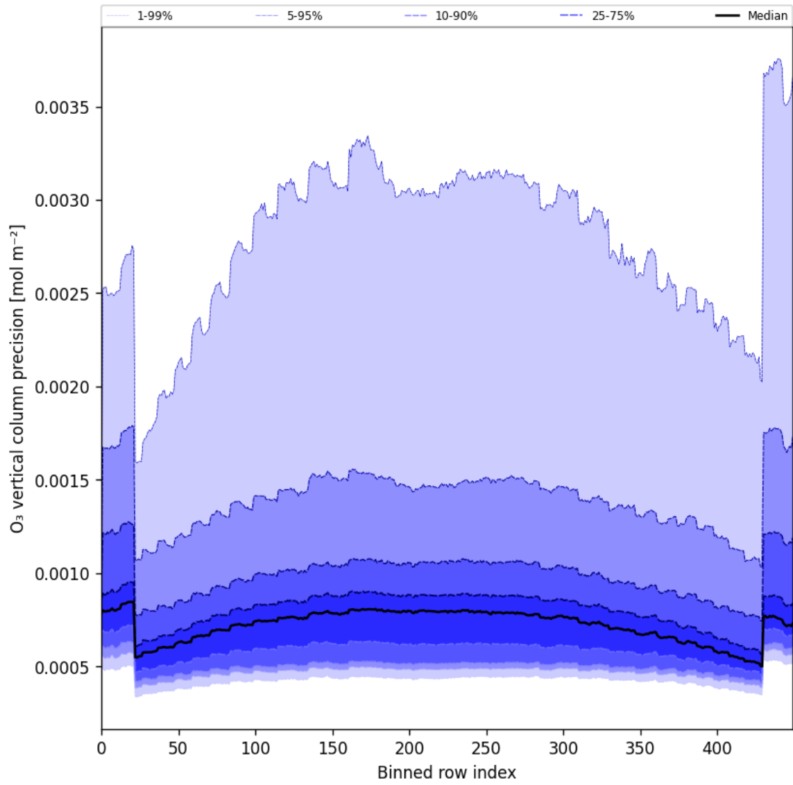
Figure 29: Along track statistics of “O 3 vertical column precision” for 2025-05-17 to 2025-05-19
