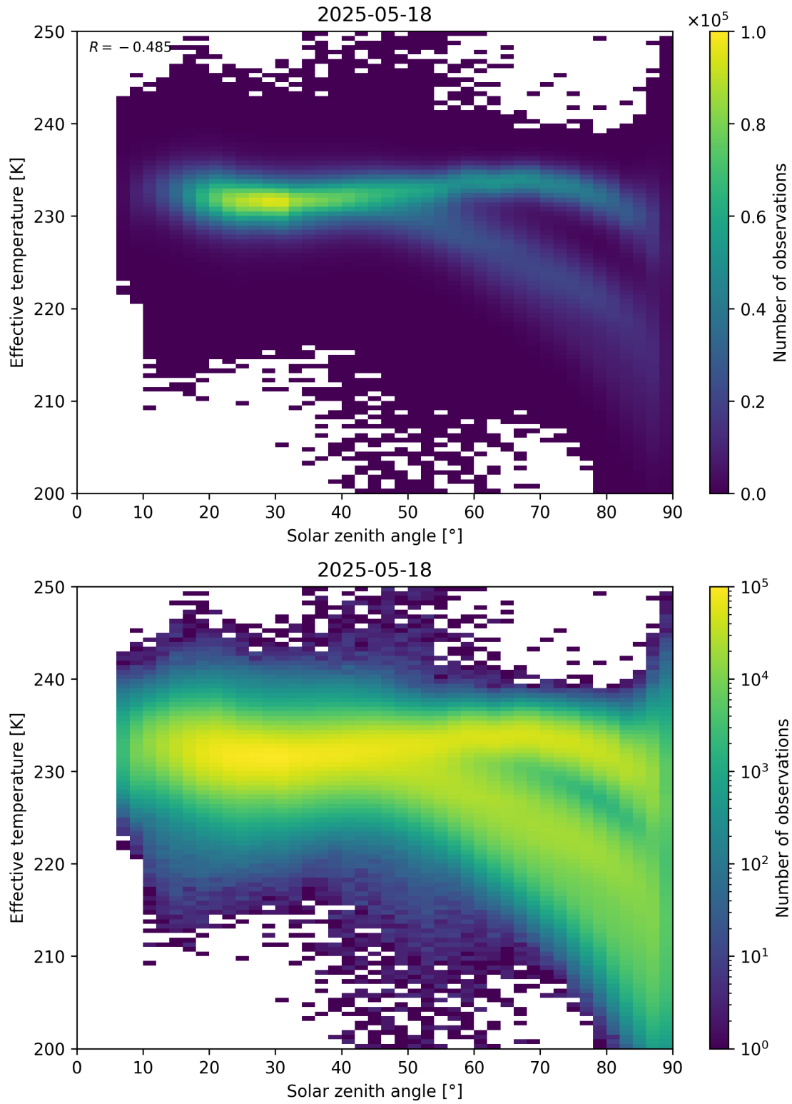
Figure 45: Scatter density plot of “Solar zenith angle” against “Effective temperature” for 2025-05-17 to 2025-05-19.
