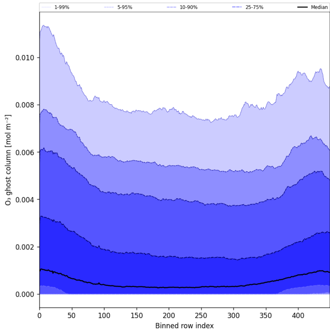
Figure 32: Along track statistics of “O 3 ghost column” for 2025-05-17 to 2025-05-19
