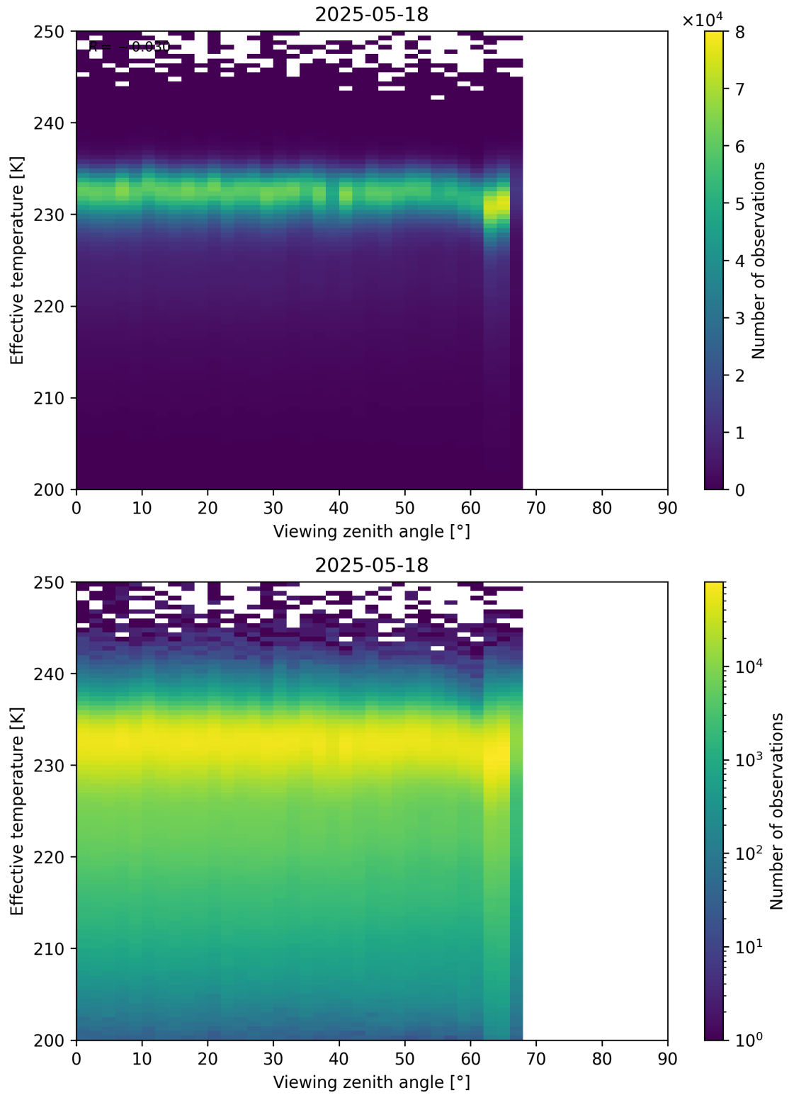
Figure 50: Scatter density plot of “Viewing zenith angle” against “Effective temperature” for 2025-05-17 to 2025-05-19.
