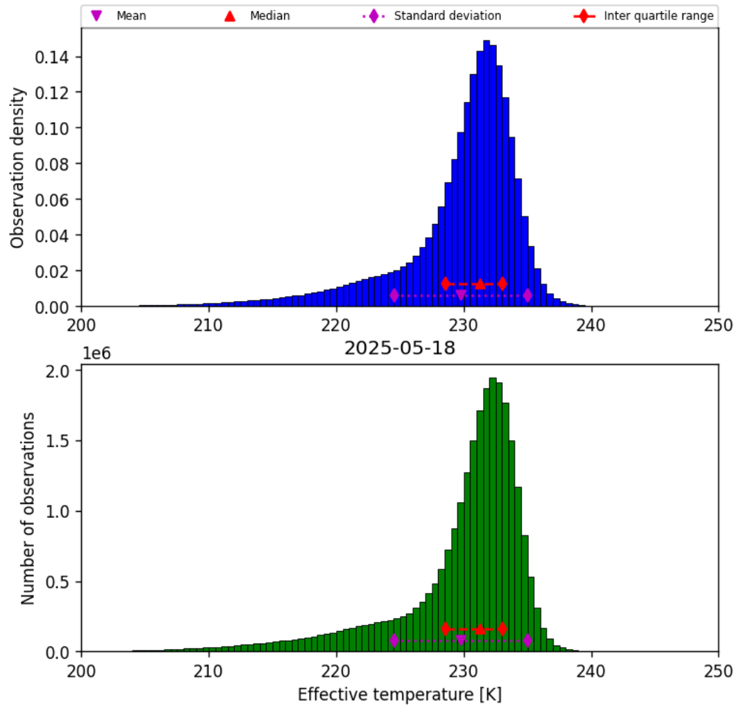
Figure 24: Histogram of “Effective temperature” for 2025-05-17 to 2025-05-19
