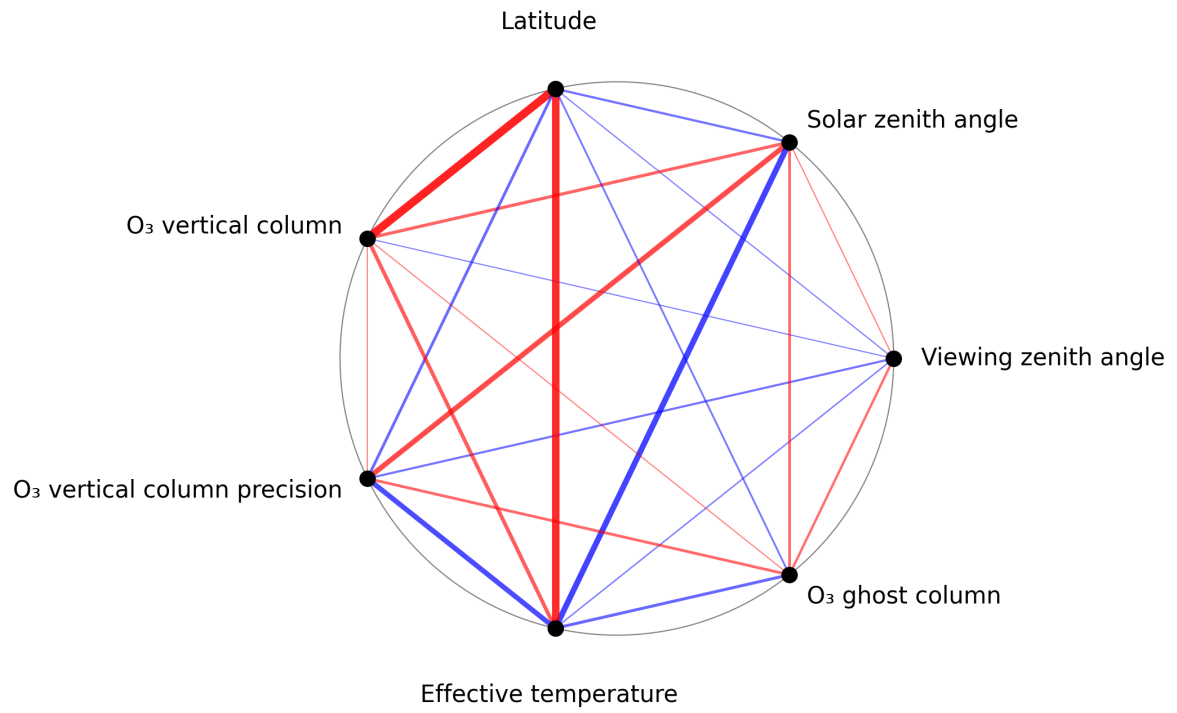
Figure 1: Map of correlation graph for 2025-05-17 to 2025-05-19.
