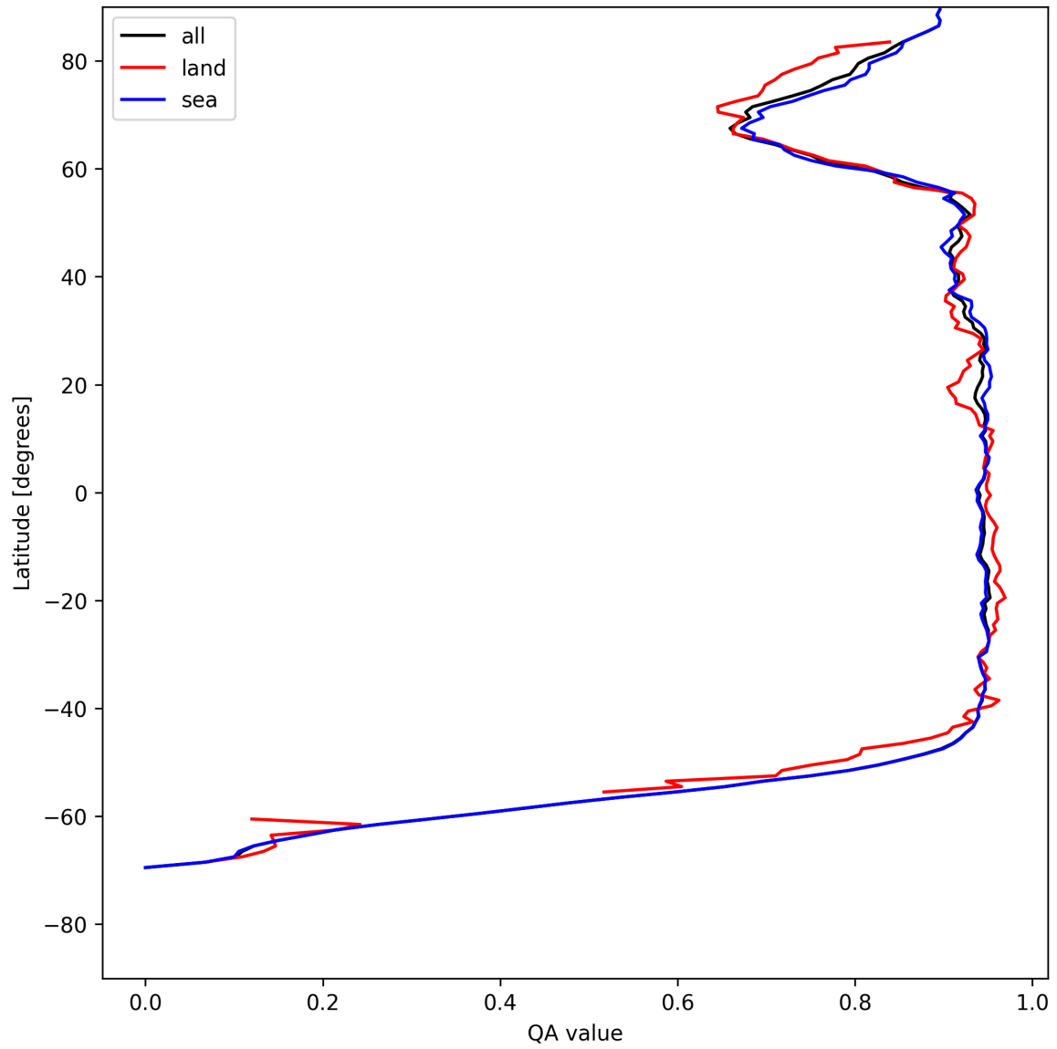
Figure 13: Zonal average of “QA value” for 2025-05-17 to 2025-05-19.
