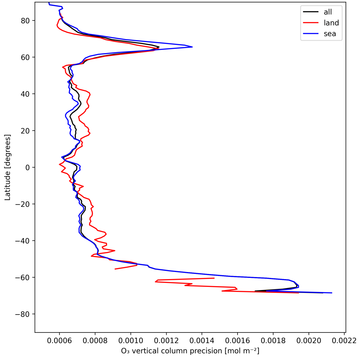
Figure 15: Zonal average of “O 3 vertical column precision” for 2025-05-18 to 2025-05-20.
