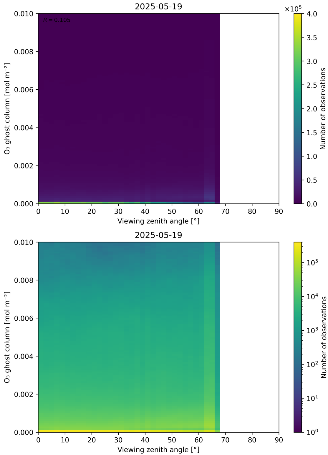
Figure 51: Scatter density plot of “Viewing zenith angle” against “O 3 ghost column” for 2025-05-18 to 2025-05-20.
