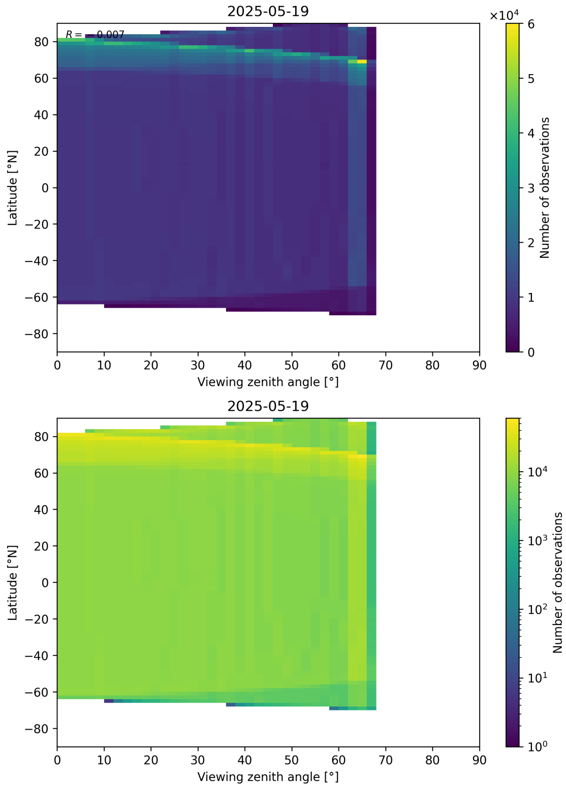
Figure 49: Scatter density plot of “Viewing zenith angle” against “Latitude” for 2025-05-18 to 2025-05-20.
