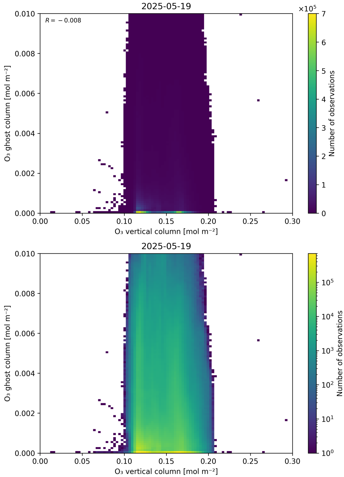
Figure 40: Scatter density plot of “O 3 vertical column” against “O 3 ghost column” for 2025-05-18 to 2025-05-20.
