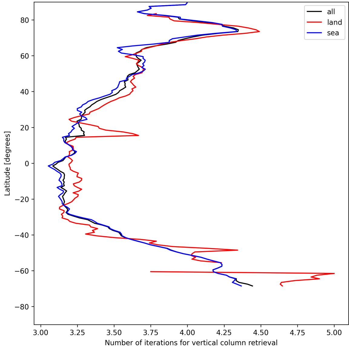
Figure 19: Zonal average of “Number of iterations for vertical column retrieval” for 2025-05-18 to 2025-05-20.
