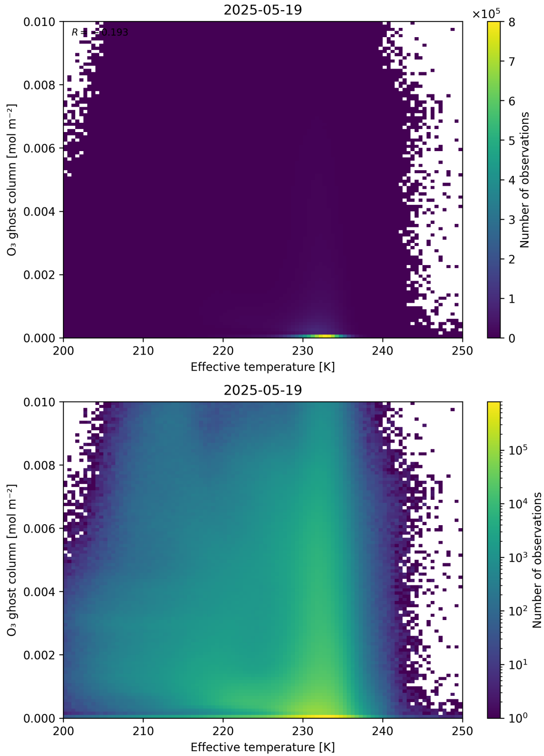
Figure 38: Scatter density plot of “Effective temperature” against “O 3 ghost column” for 2025-05-18 to 2025-05-20.
