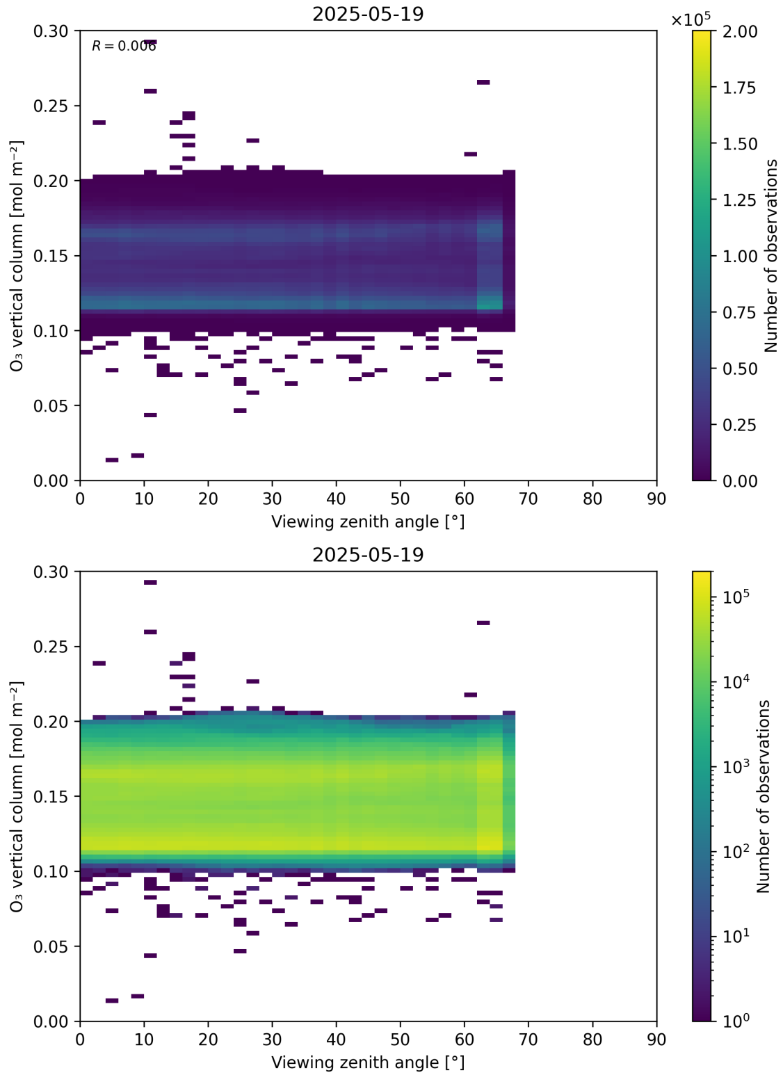
Figure 52: Scatter density plot of “Viewing zenith angle” against “O 3 vertical column” for 2025-05-18 to 2025-05-20.
