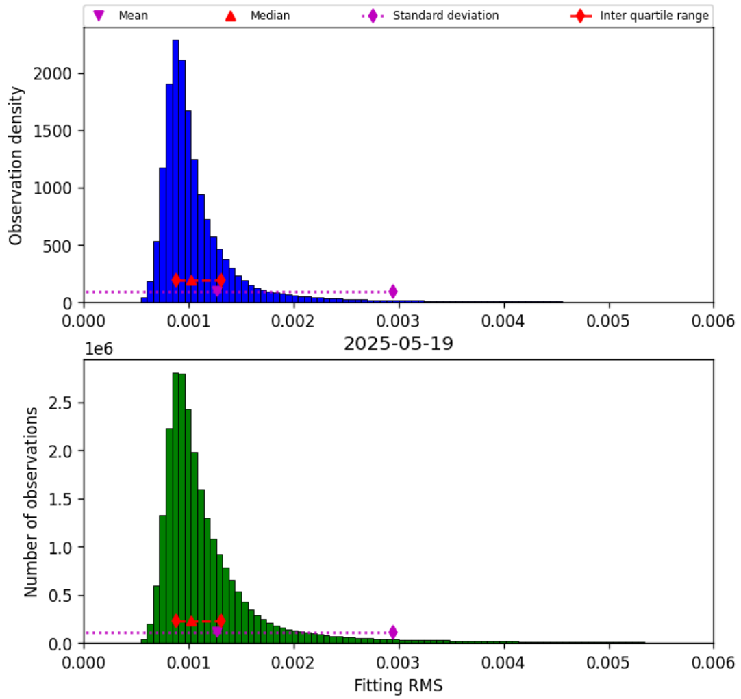
Figure 23: Histogram of “Fitting RMS” for 2025-05-18 to 2025-05-20
