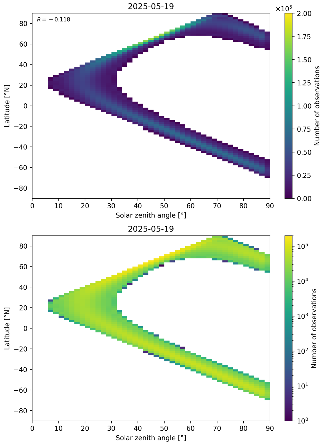
Figure 44: Scatter density plot of “Solar zenith angle” against “Latitude” for 2025-05-18 to 2025-05-20.
