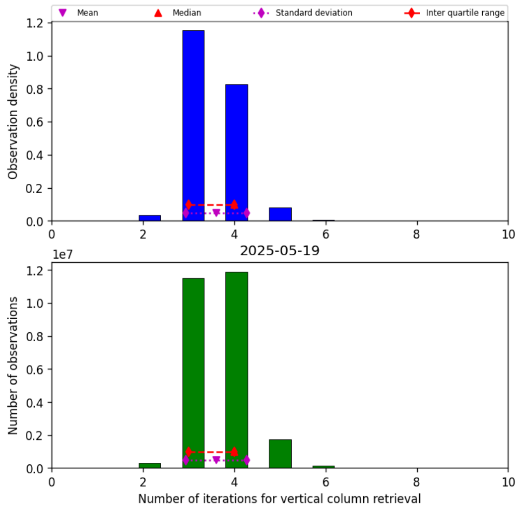
Figure 26: Histogram of “Number of iterations for vertical column retrieval” for 2025-05-18 to 2025-05-20
