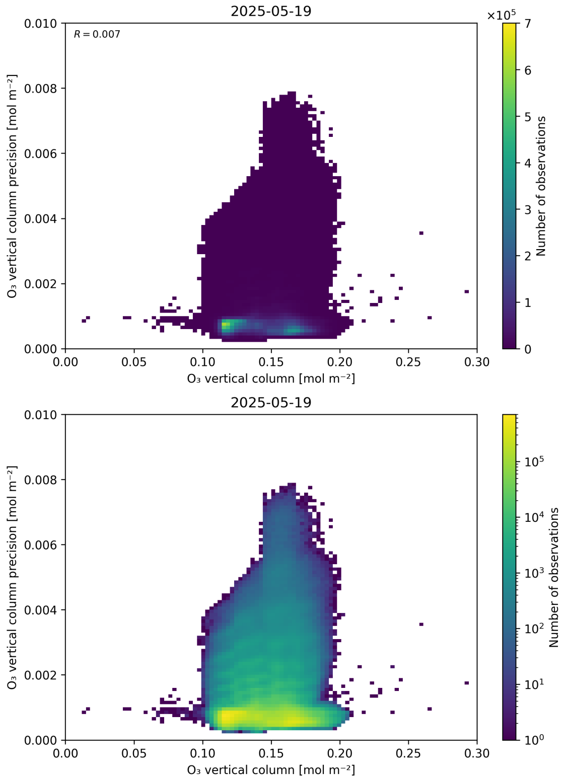
Figure 41: Scatter density plot of “O 3 vertical column” against “O 3 vertical column precision” for 2025-05-18 to 2025-05-20.
