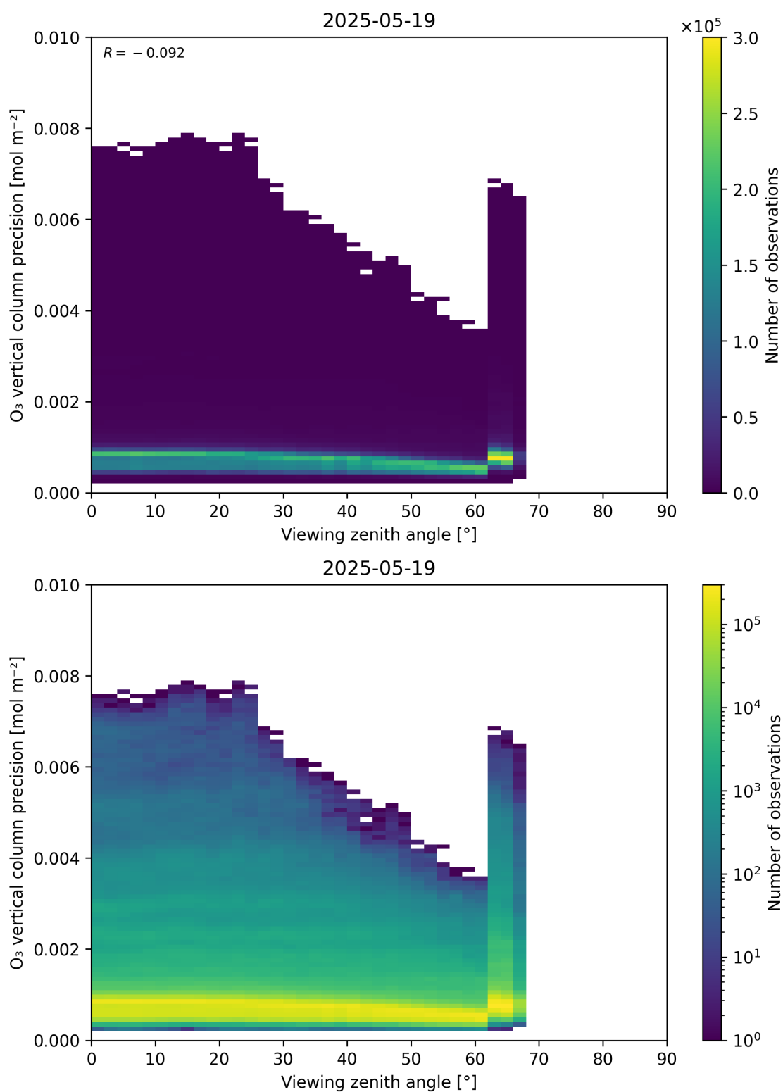
Figure 53: Scatter density plot of “Viewing zenith angle” against “O 3 vertical column precision” for 2025-05-18 to 2025-05-20.
