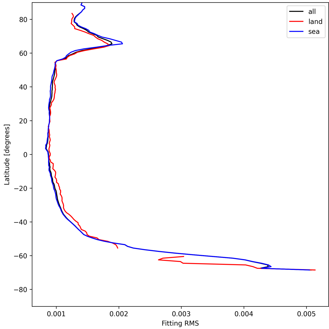
Figure 16: Zonal average of “Fitting RMS” for 2025-05-18 to 2025-05-20.
