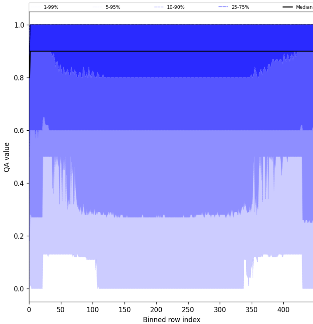
Figure 27: Along track statistics of “QA value” for 2025-05-18 to 2025-05-20
