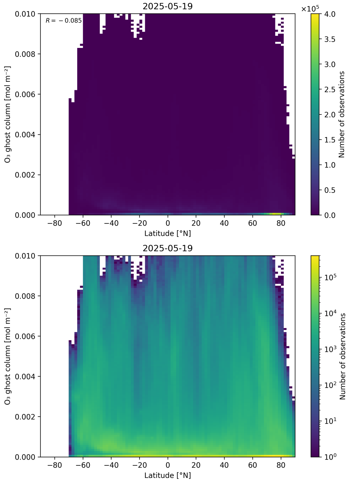
Figure 35: Scatter density plot of “Latitude” against “O 3 ghost column” for 2025-05-18 to 2025-05-20.
