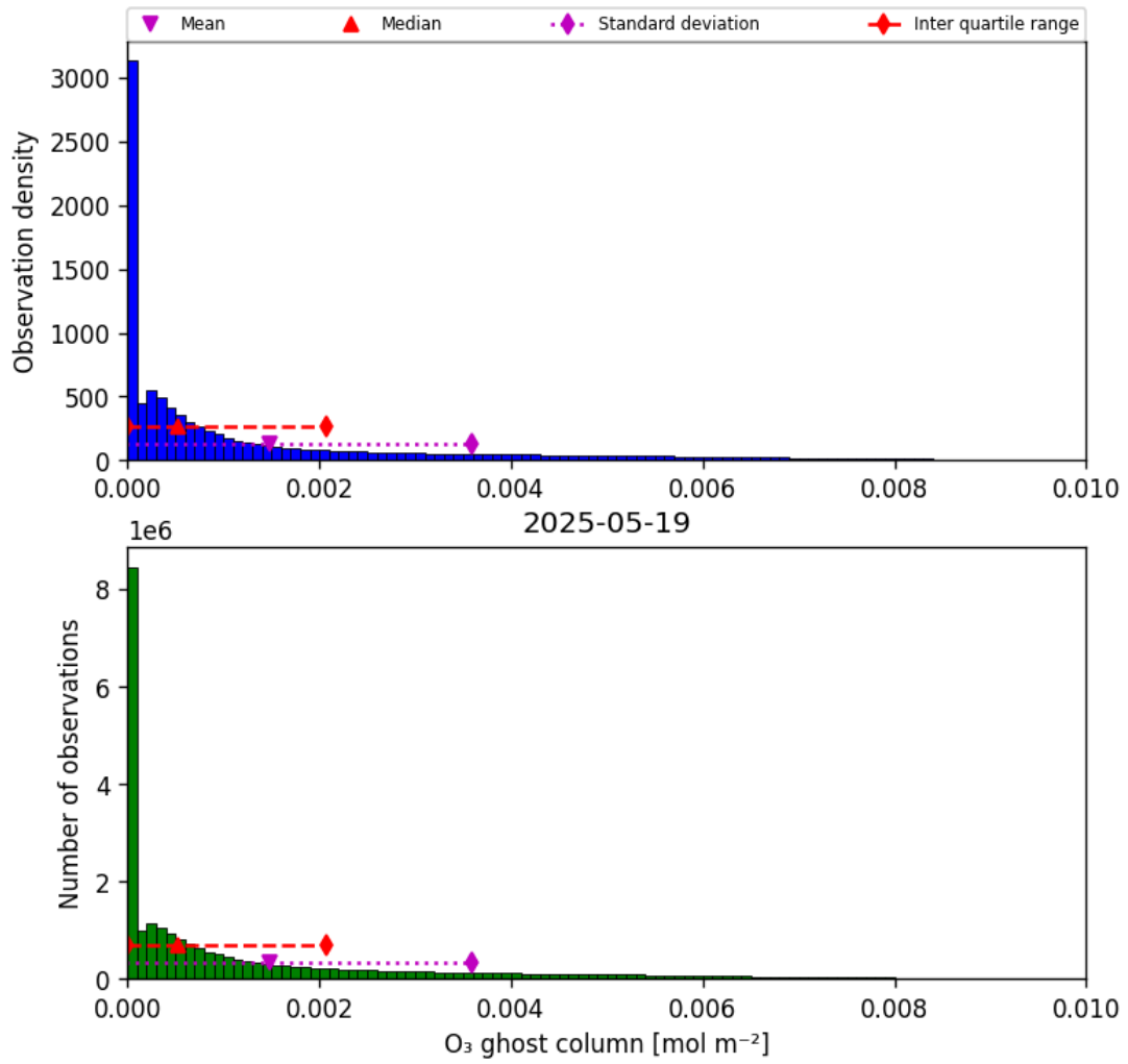
Figure 25: Histogram of “O 3 ghost column” for 2025-05-18 to 2025-05-20
