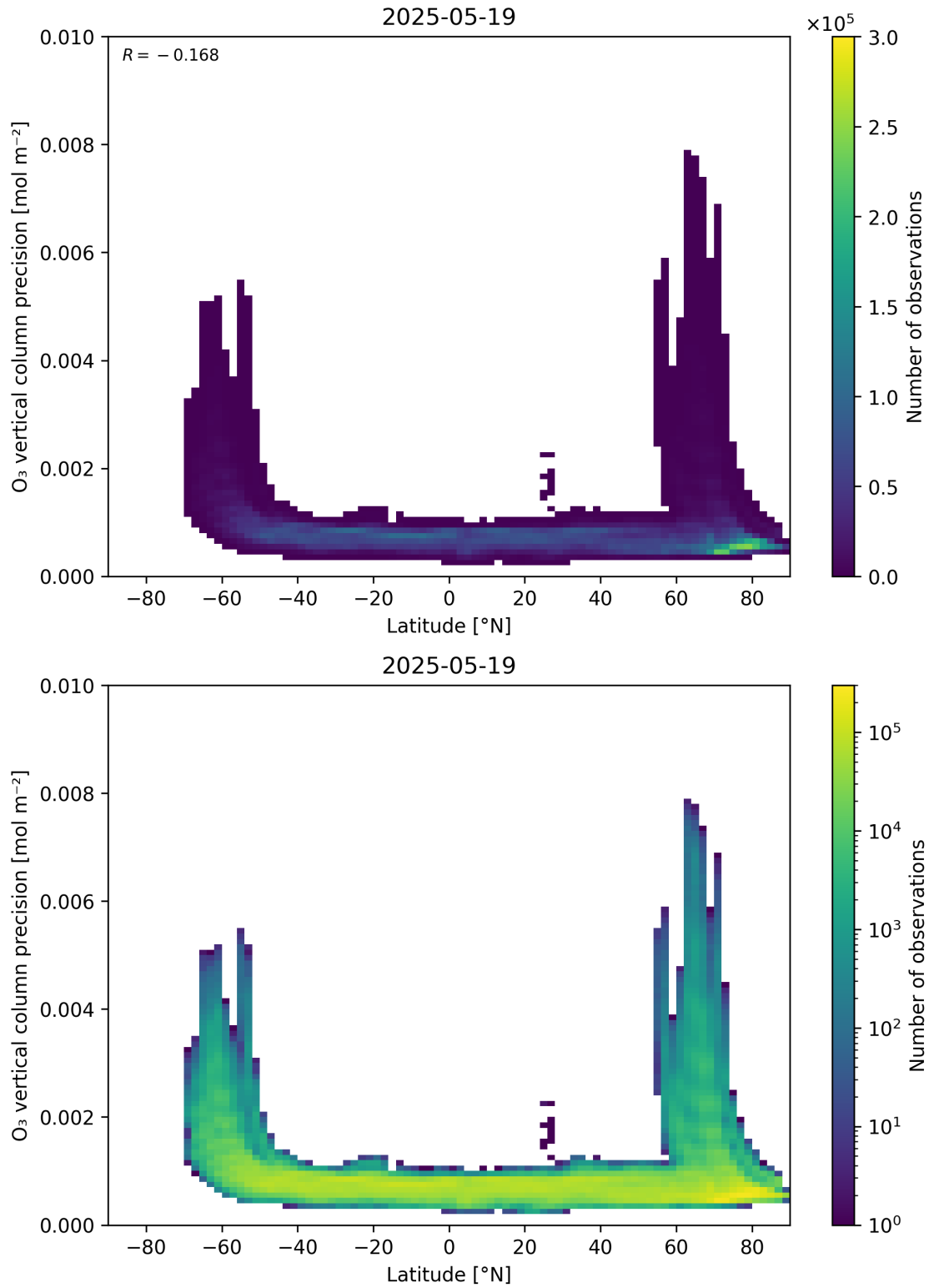
Figure 37: Scatter density plot of “Latitude” against “O 3 vertical column precision” for 2025-05-18 to 2025-05-20.
