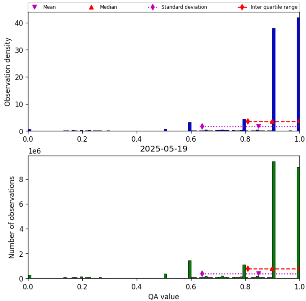
Figure 20: Histogram of “QA value” for 2025-05-18 to 2025-05-20
