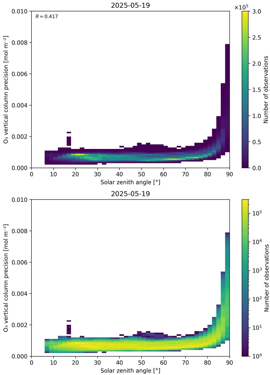
Figure 48: Scatter density plot of “Solar zenith angle” against “O 3 vertical column precision” for 2025-05-18 to 2025-05-20.
