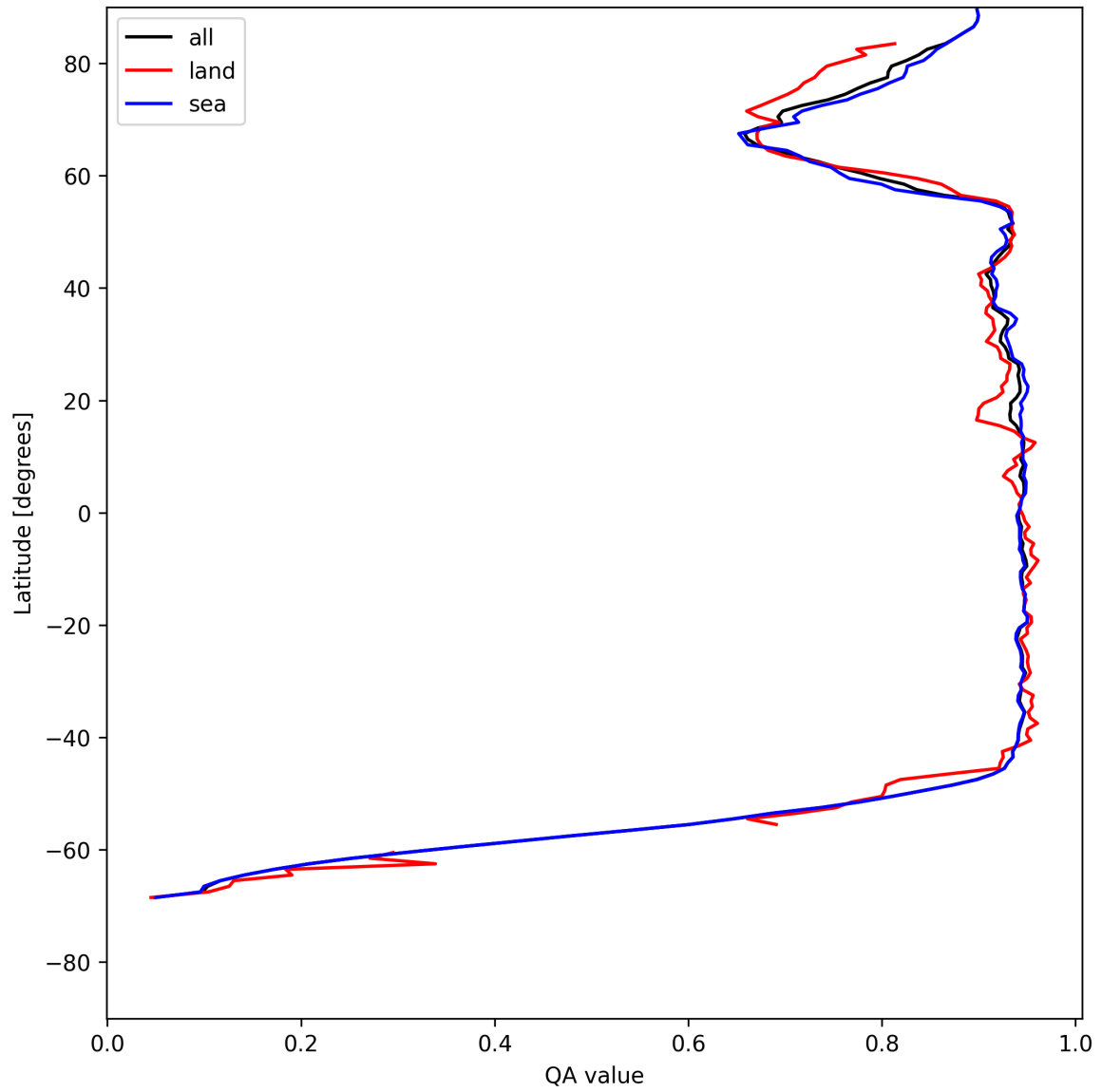
Figure 13: Zonal average of “QA value” for 2025-05-18 to 2025-05-20.
