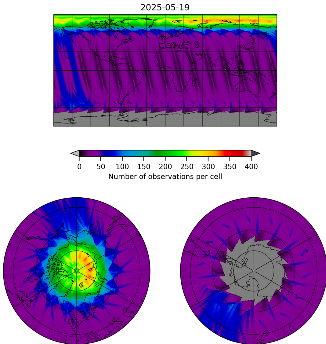
Figure 12: Map of the number of observations for 2025-05-18 to 2025-05-20
