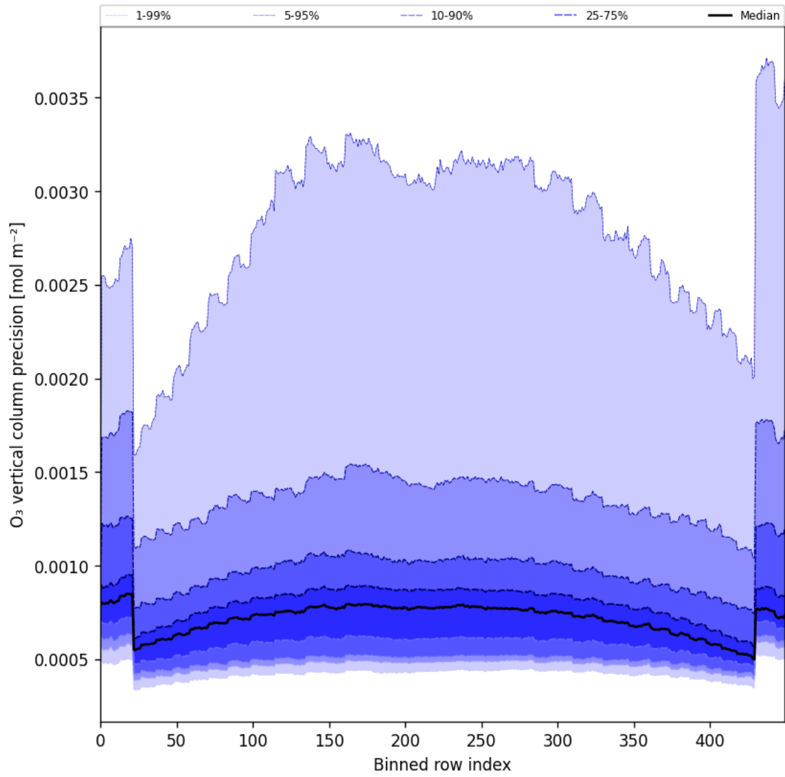
Figure 29: Along track statistics of “O 3 vertical column precision” for 2025-05-18 to 2025-05-20
