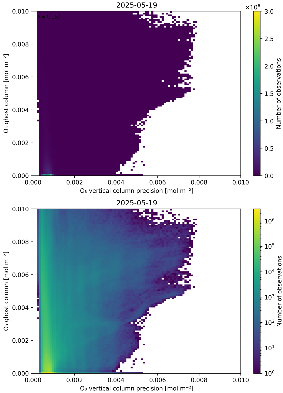
Figure 43: Scatter density plot of “ \text{O}_3 vertical column precision” against “ \text{O}_3 ghost column” for 2025-05-18 to 2025-05-20.
