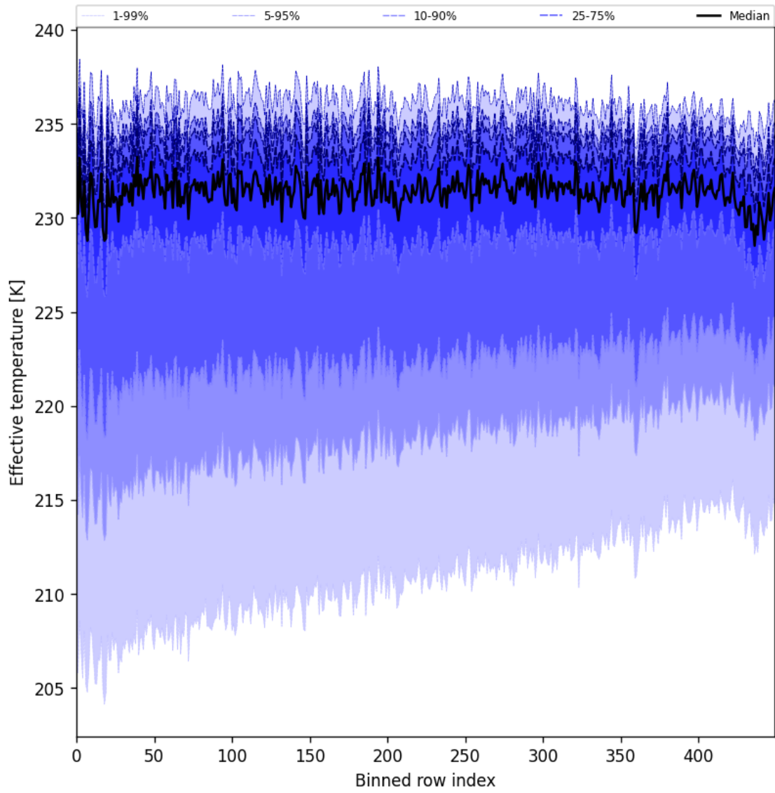
Figure 31: Along track statistics of “Effective temperature” for 2025-05-18 to 2025-05-20
