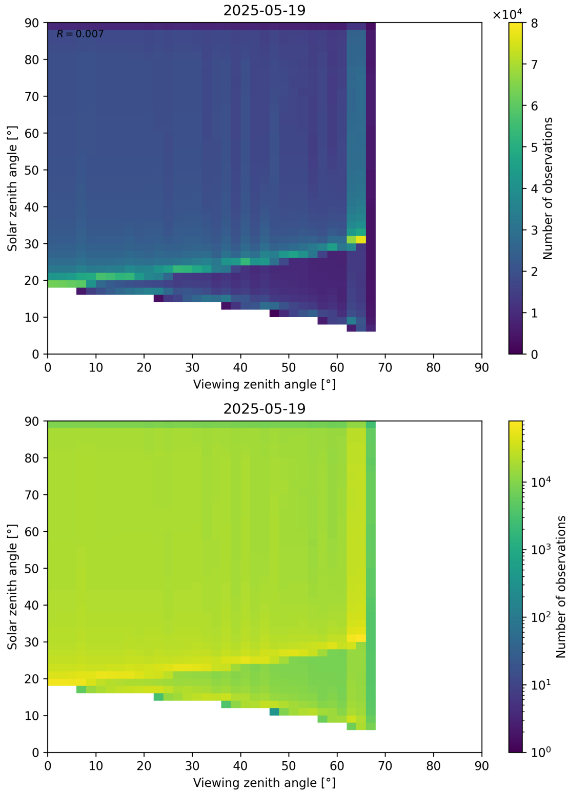
Figure 54: Scatter density plot of “Viewing zenith angle” against “Solar zenith angle” for 2025-05-18 to 2025-05-20.
