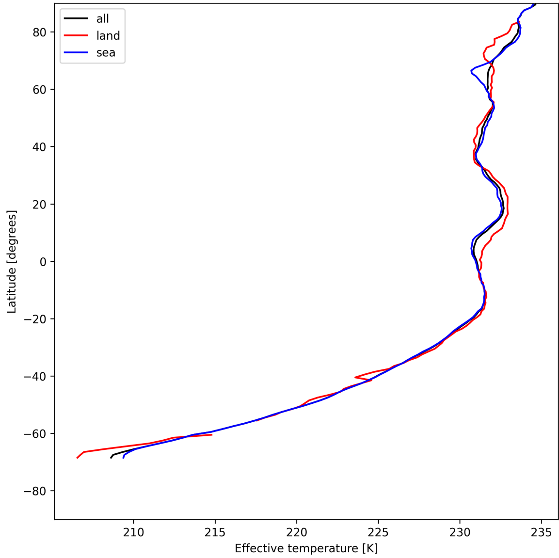
Figure 17: Zonal average of "Effective temperature" for 2025-05-18 to 2025-05-20.
