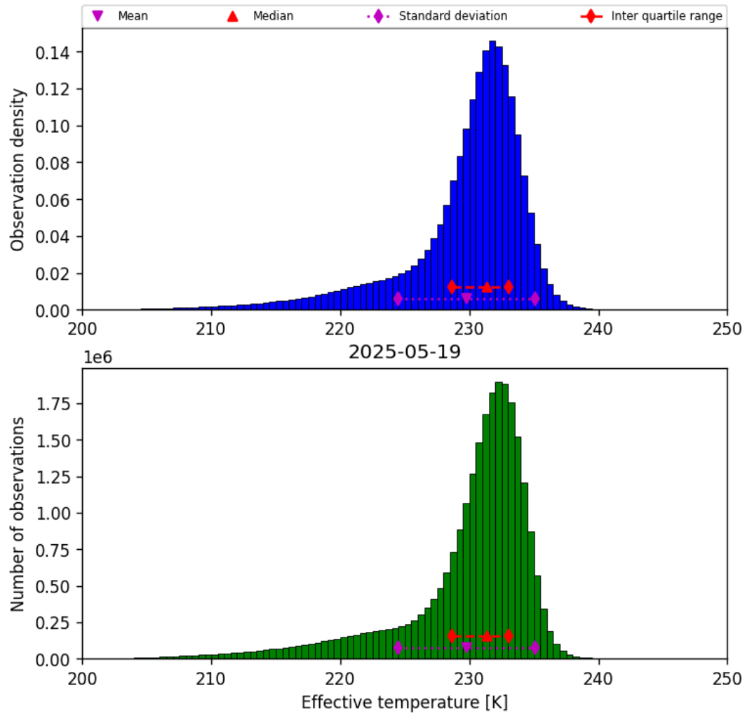
Figure 24: Histogram of “Effective temperature” for 2025-05-18 to 2025-05-20
