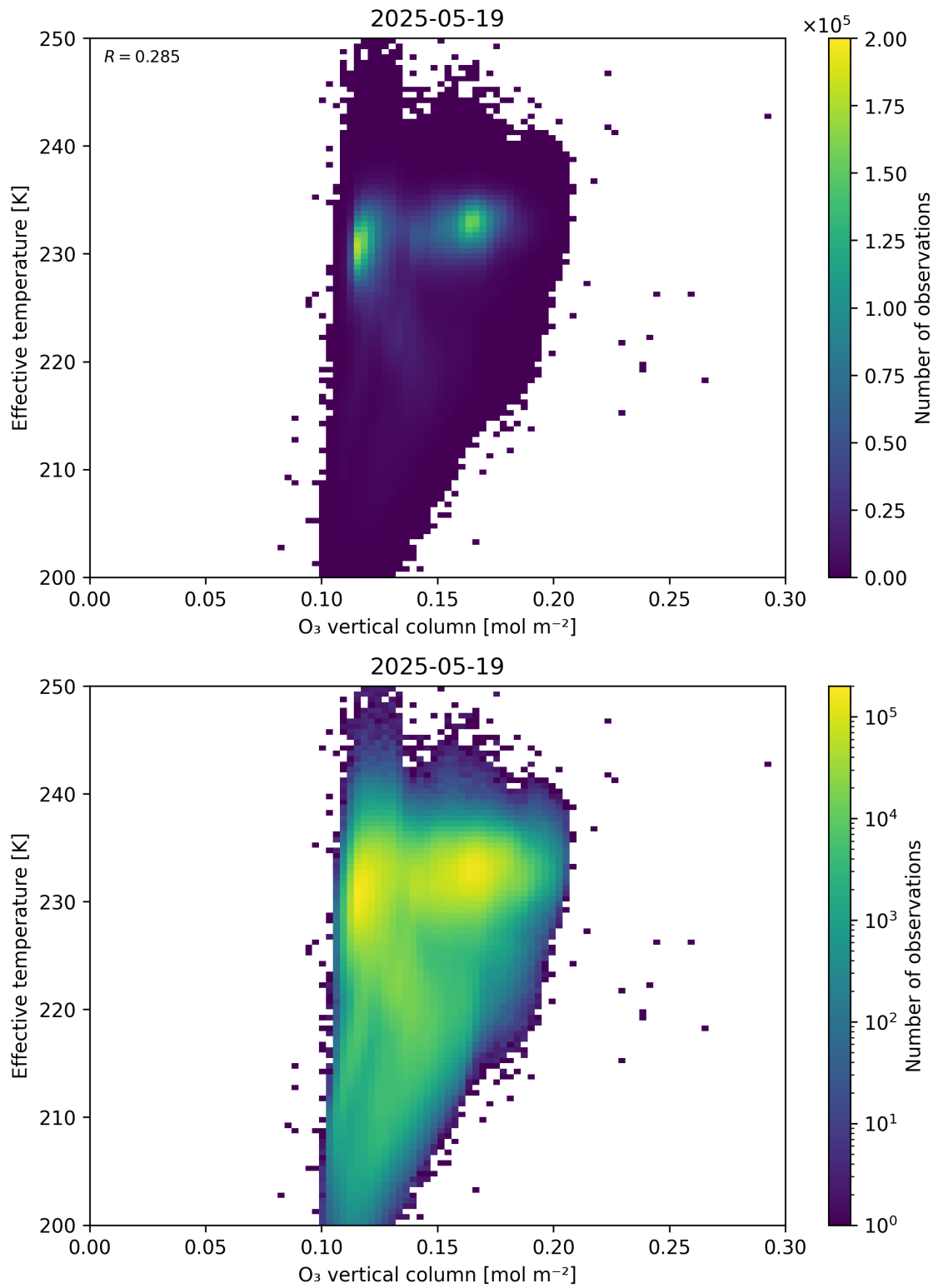
Figure 39: Scatter density plot of “O 3 vertical column” against “Effective temperature” for 2025-05-18 to 2025-05-20.
