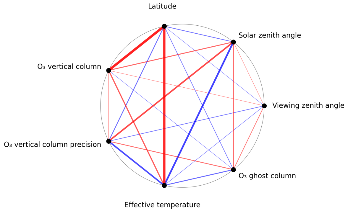
Figure 1: Map of correlation graph for 2025-05-18 to 2025-05-20.
