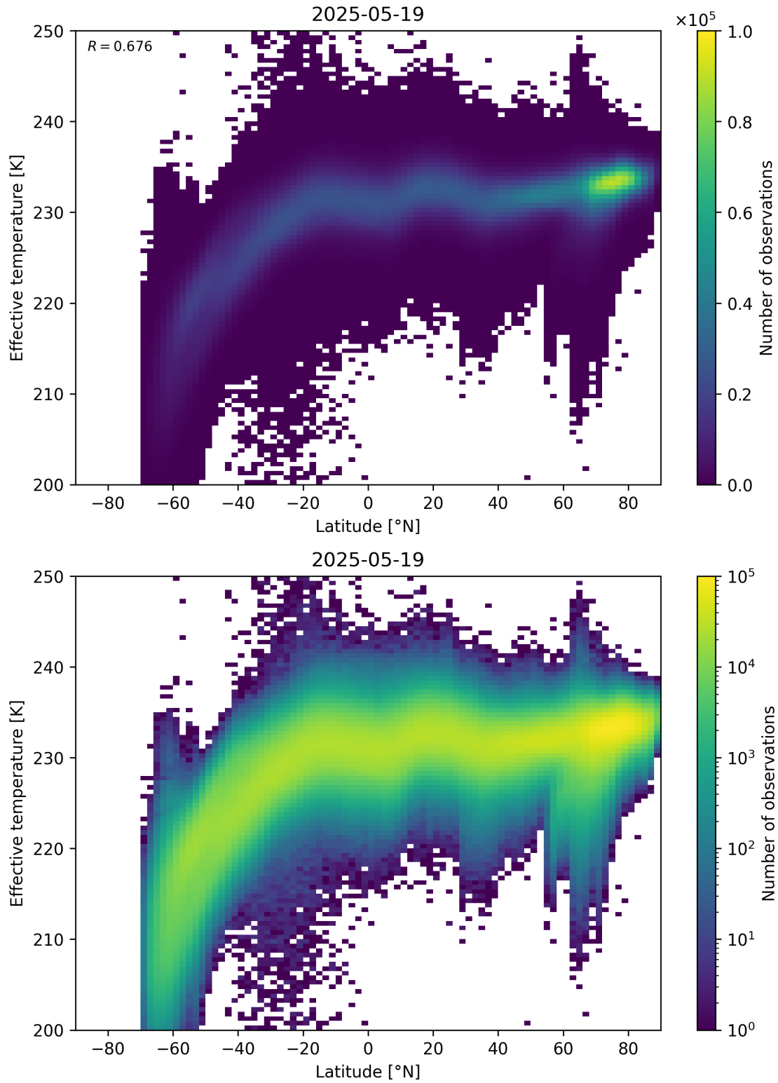
Figure 34: Scatter density plot of “Latitude” against “Effective temperature” for 2025-05-18 to 2025-05-20.
