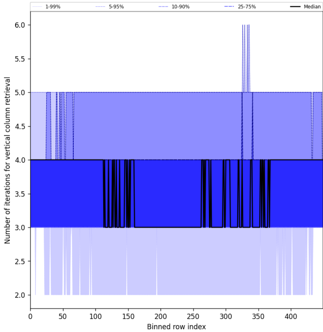
Figure 33: Along track statistics of “Number of iterations for vertical column retrieval” for 2025-05-18 to 2025-05-20
