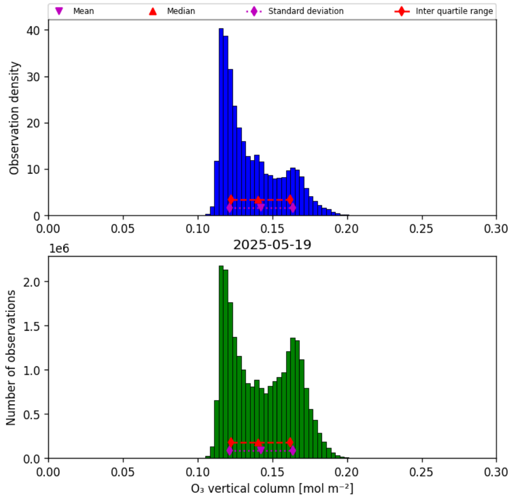
Figure 21: Histogram of “O 3 vertical column” for 2025-05-18 to 2025-05-20
