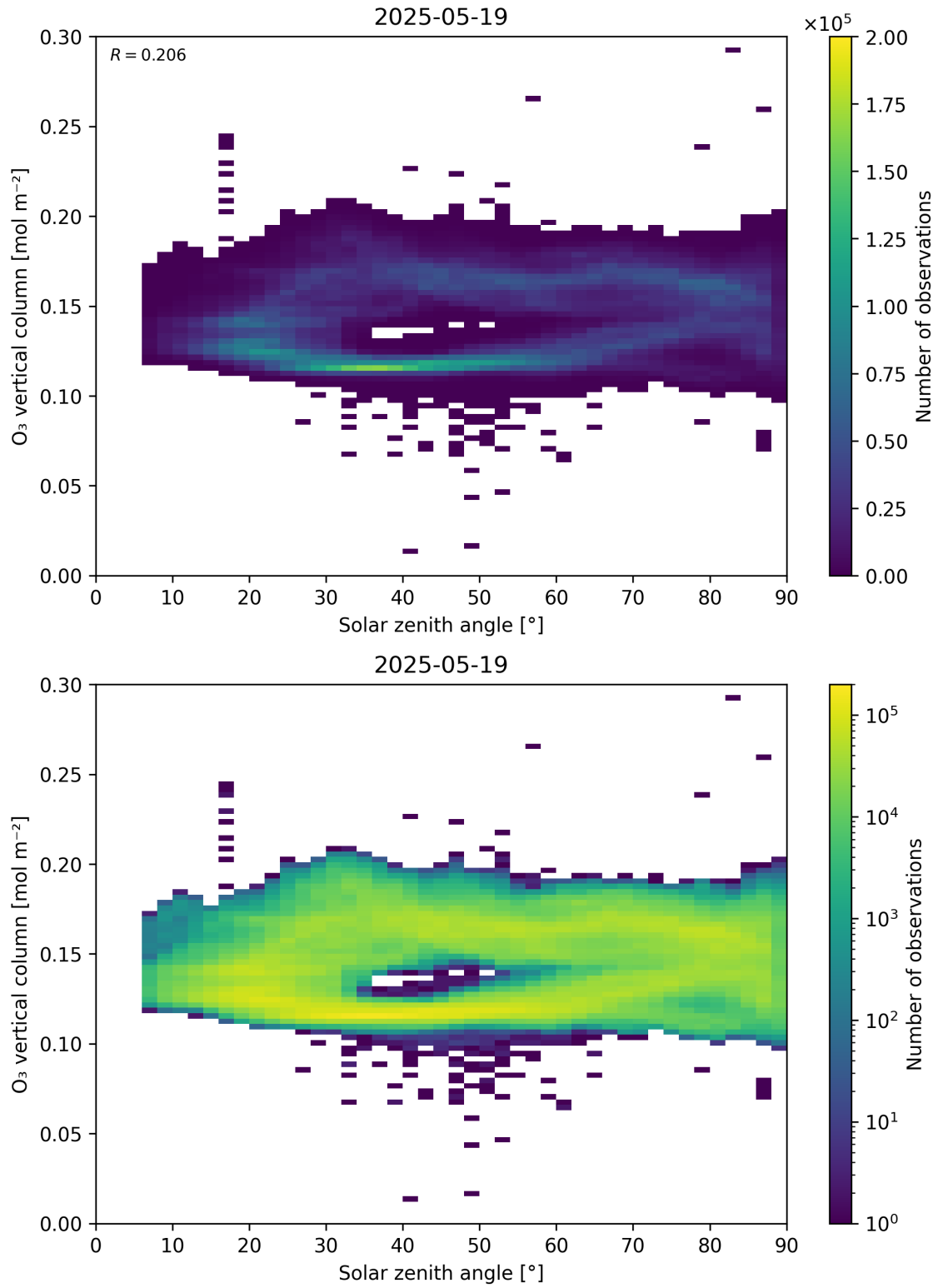
Figure 47: Scatter density plot of “Solar zenith angle” against “O 3 vertical column” for 2025-05-18 to 2025-05-20.
