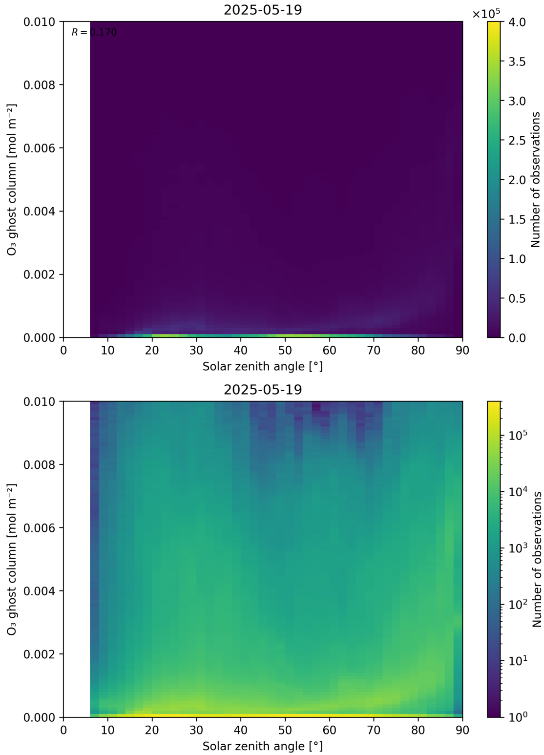
Figure 46: Scatter density plot of “Solar zenith angle” against “O 3 ghost column” for 2025-05-18 to 2025-05-20.
