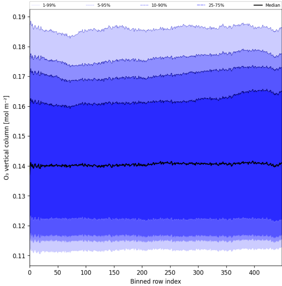
Figure 28: Along track statistics of “O 3 vertical column” for 2025-05-18 to 2025-05-20
