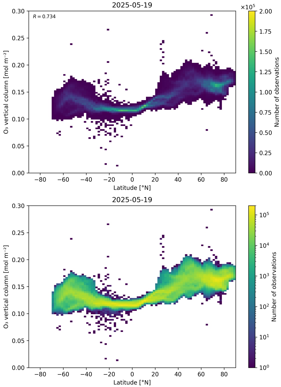
Figure 36: Scatter density plot of “Latitude” against “O 3 vertical column” for 2025-05-18 to 2025-05-20.
