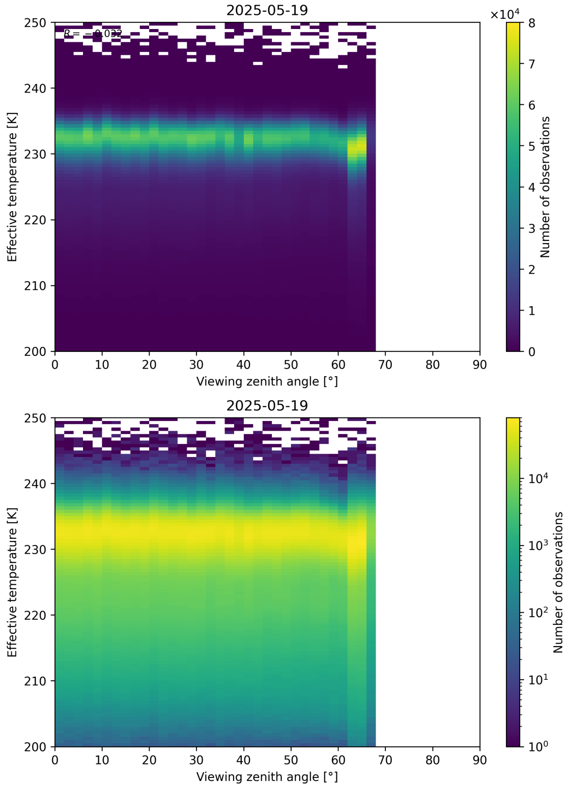
Figure 50: Scatter density plot of “Viewing zenith angle” against “Effective temperature” for 2025-05-18 to 2025-05-20.
