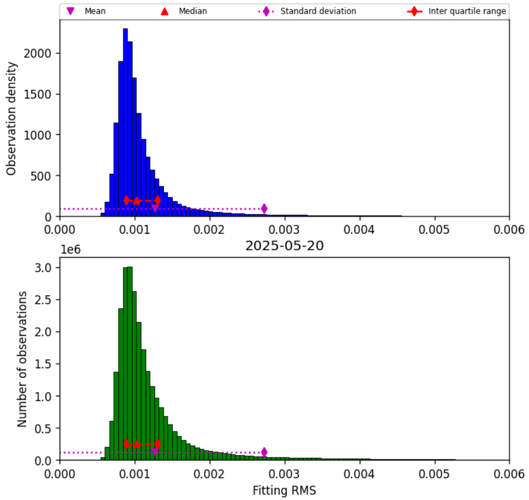
Figure 23: Histogram of “Fitting RMS” for 2025-05-19 to 2025-05-21
