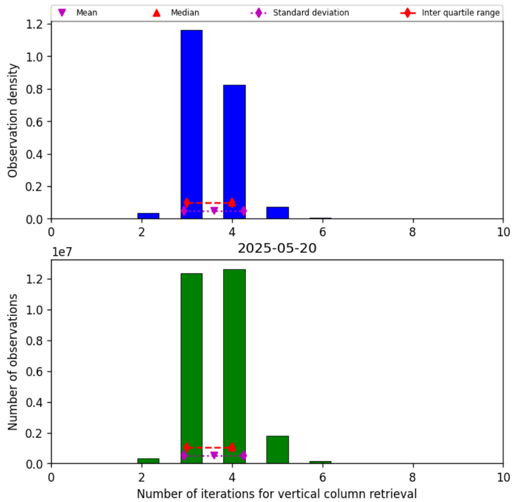
Figure 26: Histogram of “Number of iterations for vertical column retrieval” for 2025-05-19 to 2025-05-21
