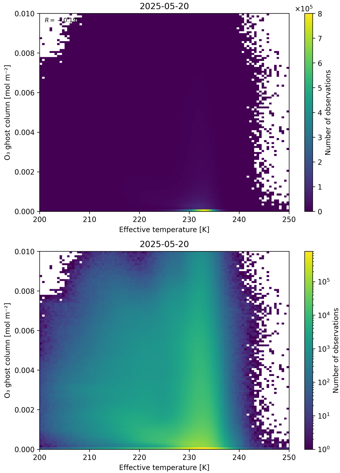
Figure 38: Scatter density plot of “Effective temperature” against “O 3 ghost column” for 2025-05-19 to 2025-05-21.
