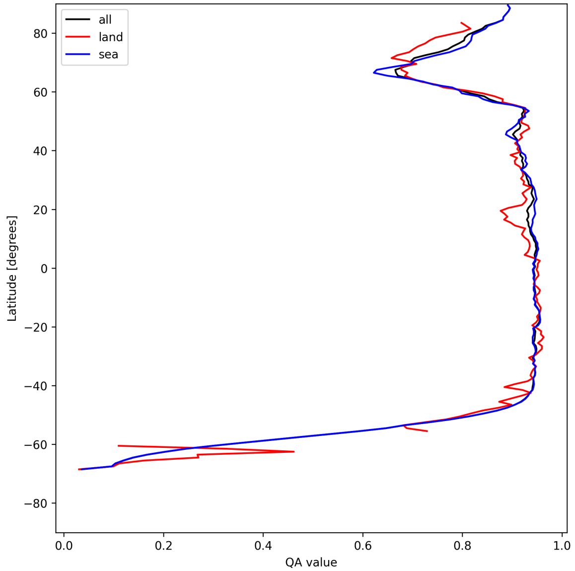
Figure 13: Zonal average of “QA value” for 2025-05-19 to 2025-05-21.
