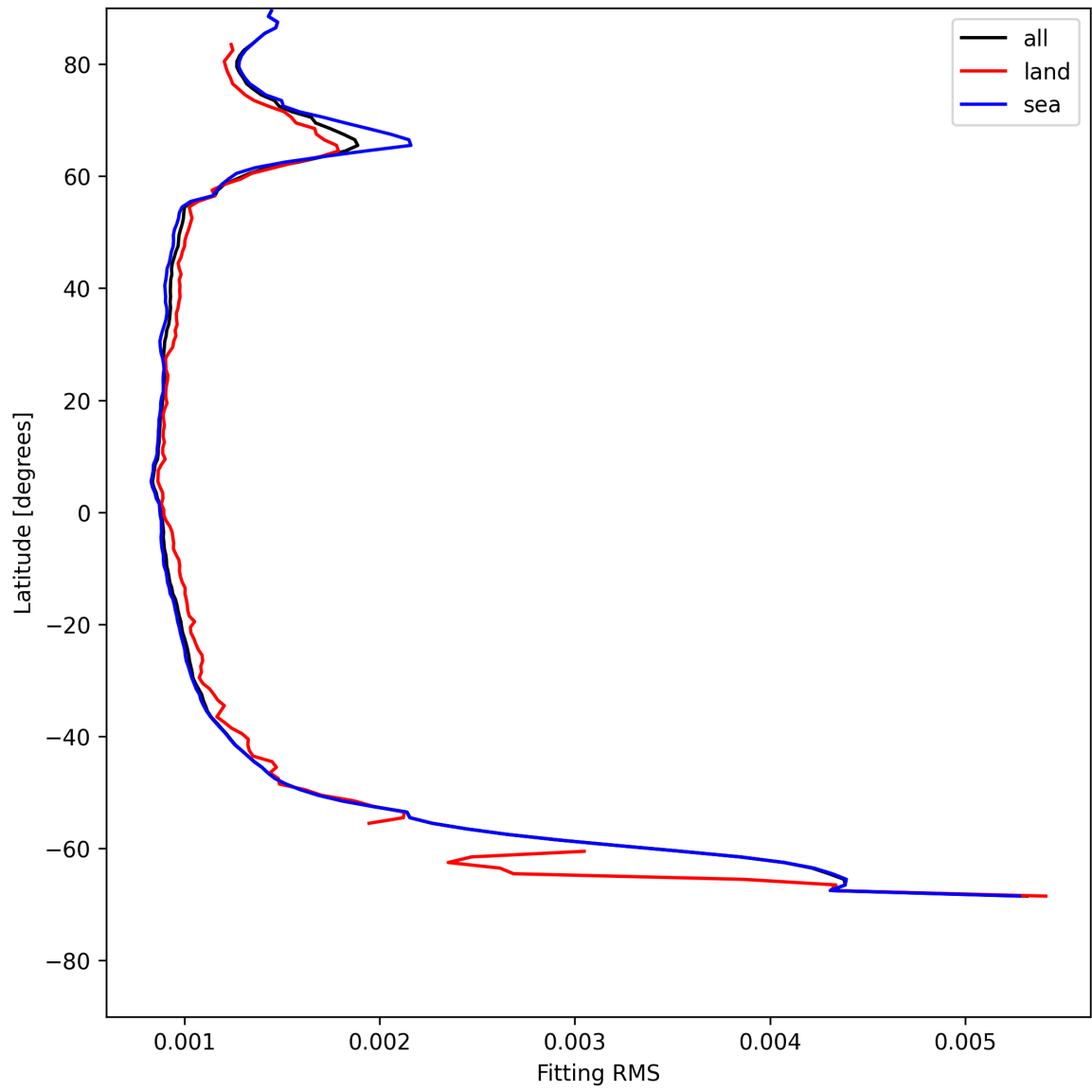
Figure 16: Zonal average of “Fitting RMS” for 2025-05-19 to 2025-05-21.
