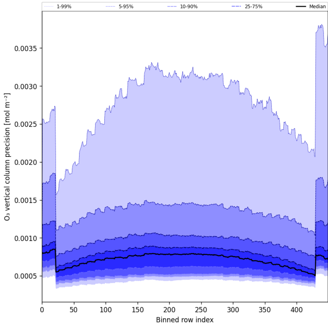
Figure 29: Along track statistics of “O 3 vertical column precision” for 2025-05-19 to 2025-05-21
