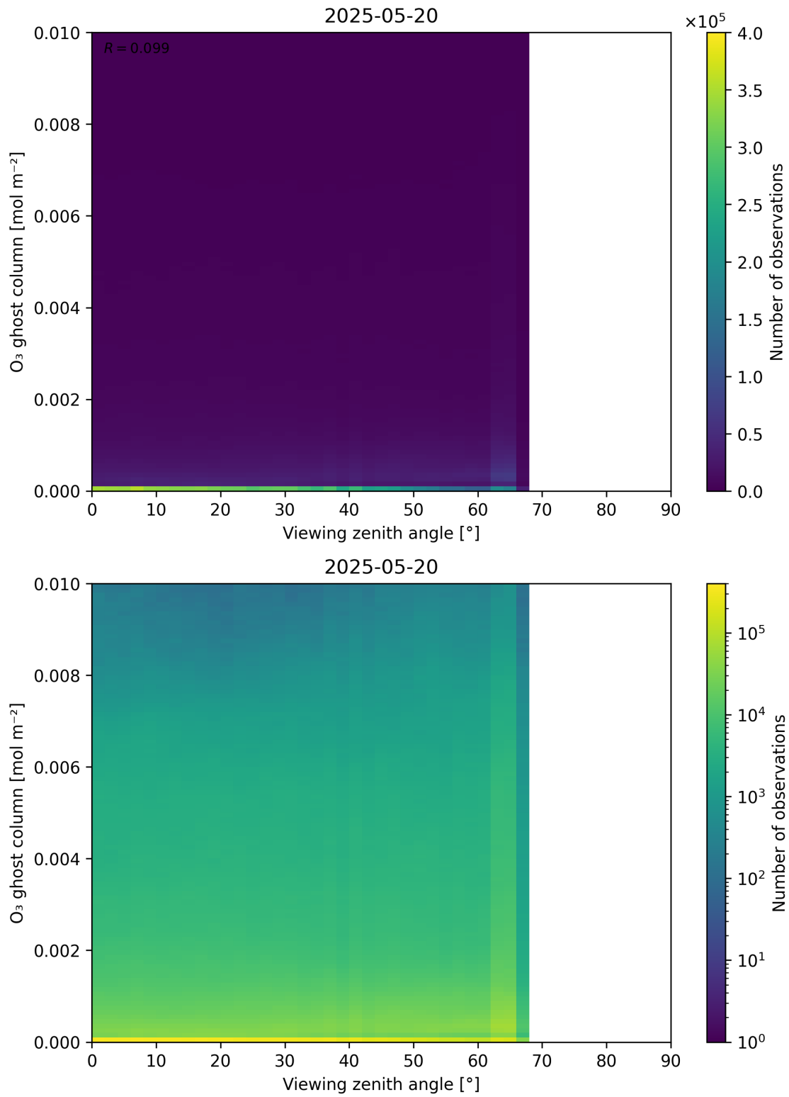
Figure 51: Scatter density plot of “Viewing zenith angle” against “O 3 ghost column” for 2025-05-19 to 2025-05-21.
