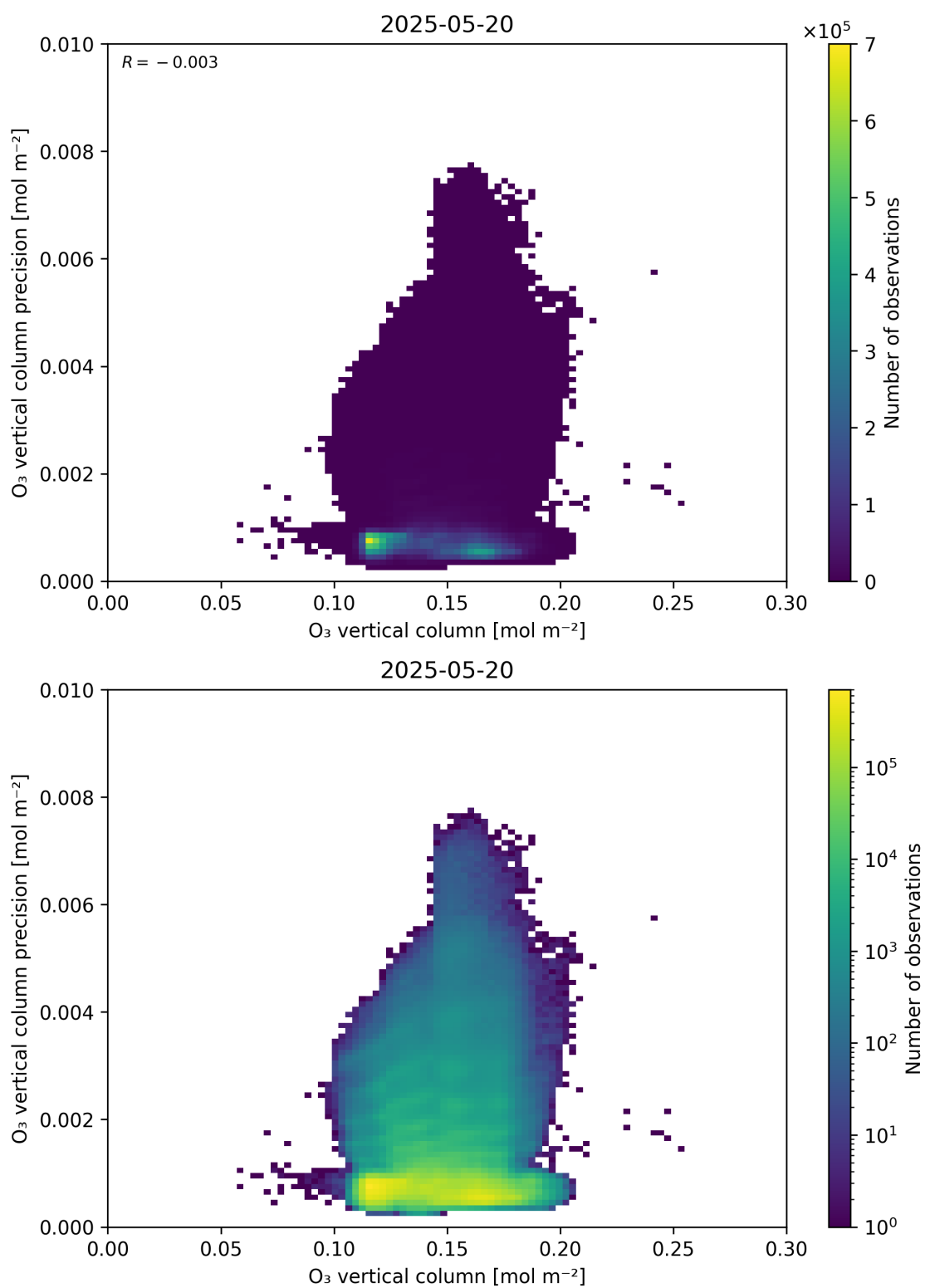
Figure 41: Scatter density plot of “O 3 vertical column” against “O 3 vertical column precision” for 2025-05-19 to 2025-05-21.
