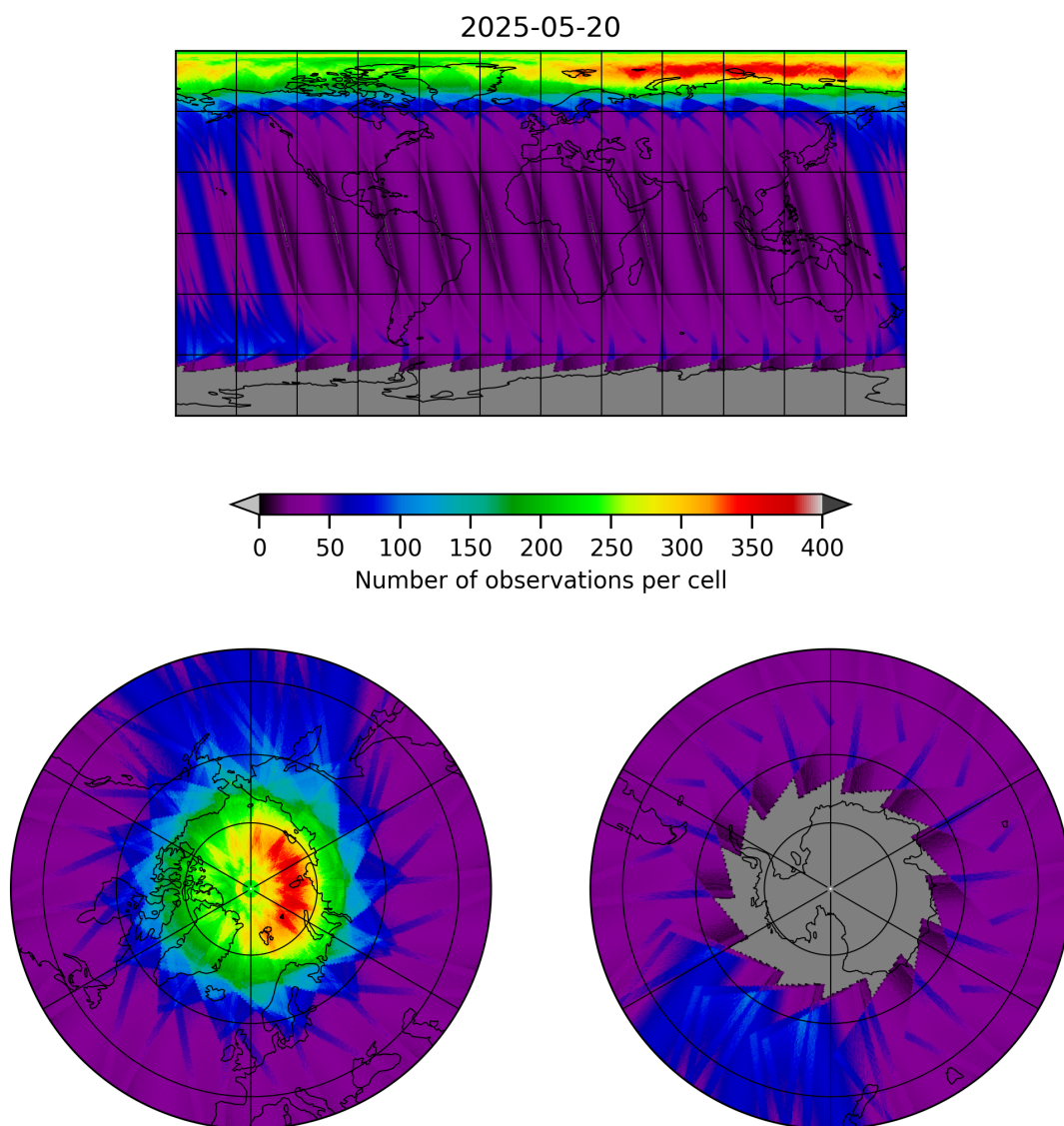
Figure 12: Map of the number of observations for 2025-05-19 to 2025-05-21
