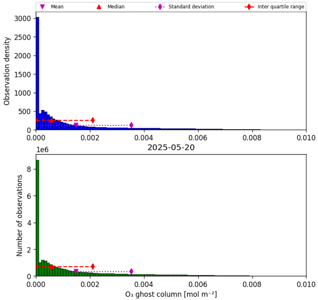
Figure 25: Histogram of “O 3 ghost column” for 2025-05-19 to 2025-05-21
