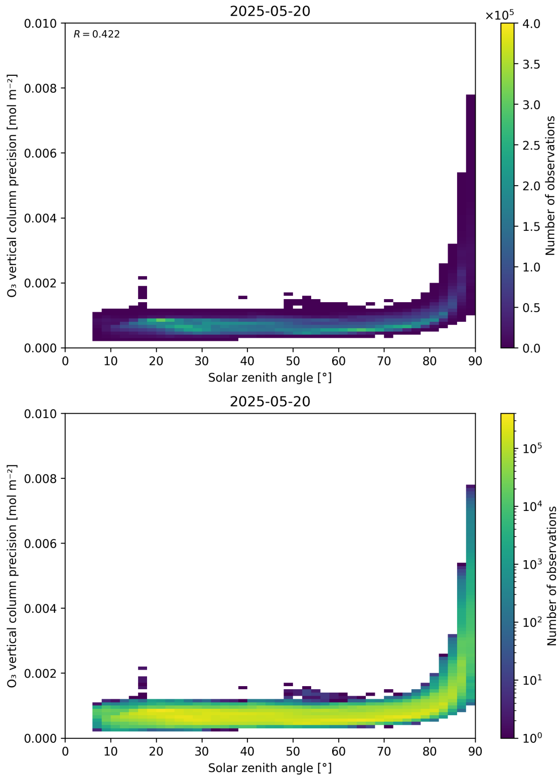
Figure 48: Scatter density plot of “Solar zenith angle” against “O 3 vertical column precision” for 2025-05-19 to 2025-05-21.
