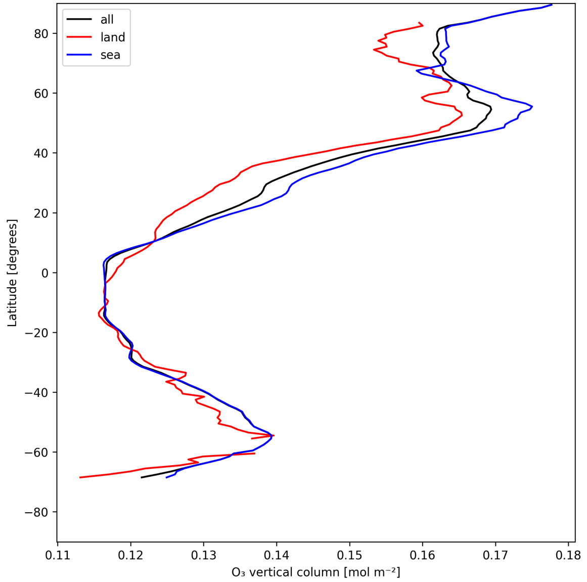
Figure 14: Zonal average of “O 3 vertical column” for 2025-05-19 to 2025-05-21.
