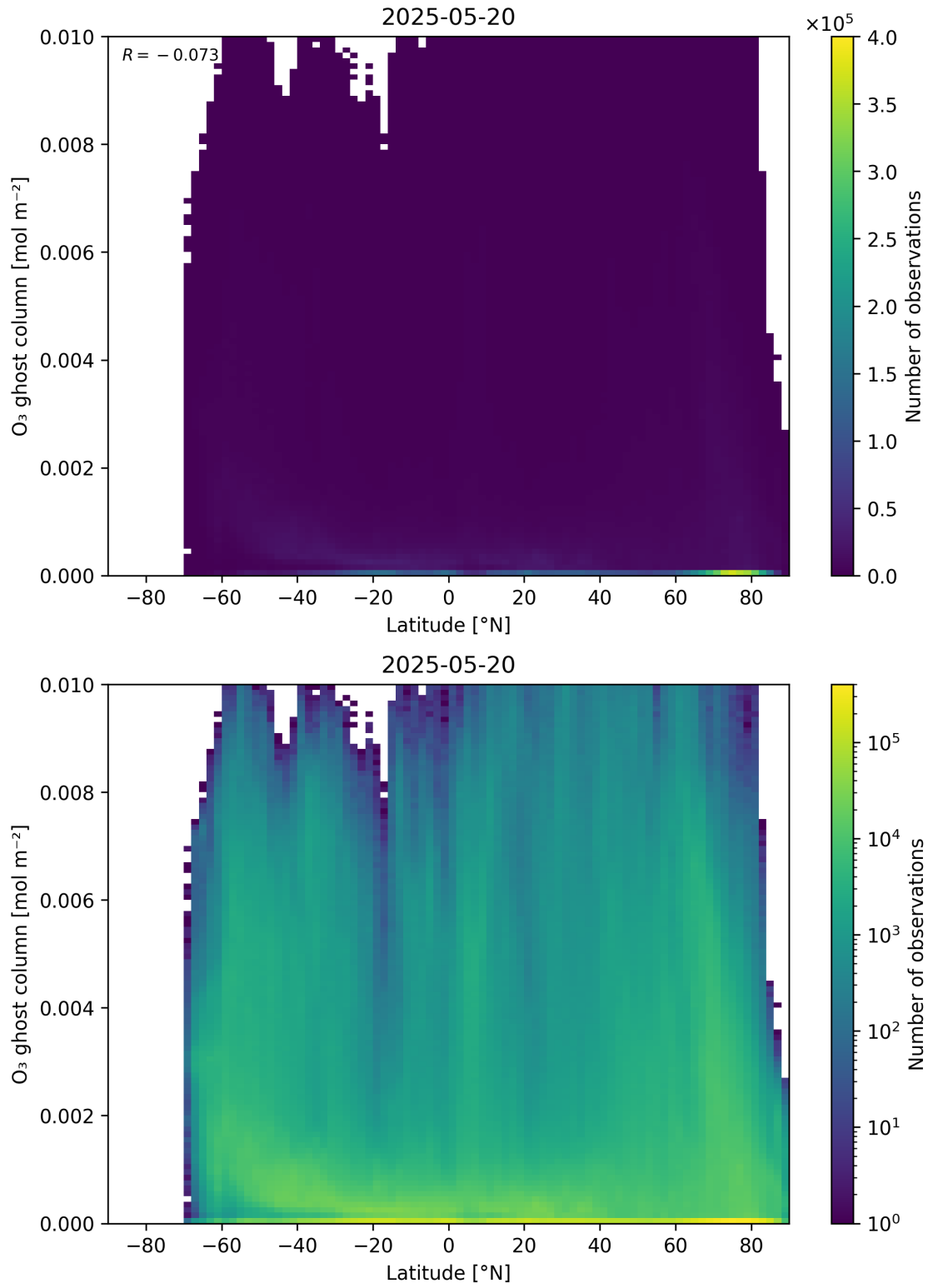
Figure 35: Scatter density plot of “Latitude” against “O 3 ghost column” for 2025-05-19 to 2025-05-21.
