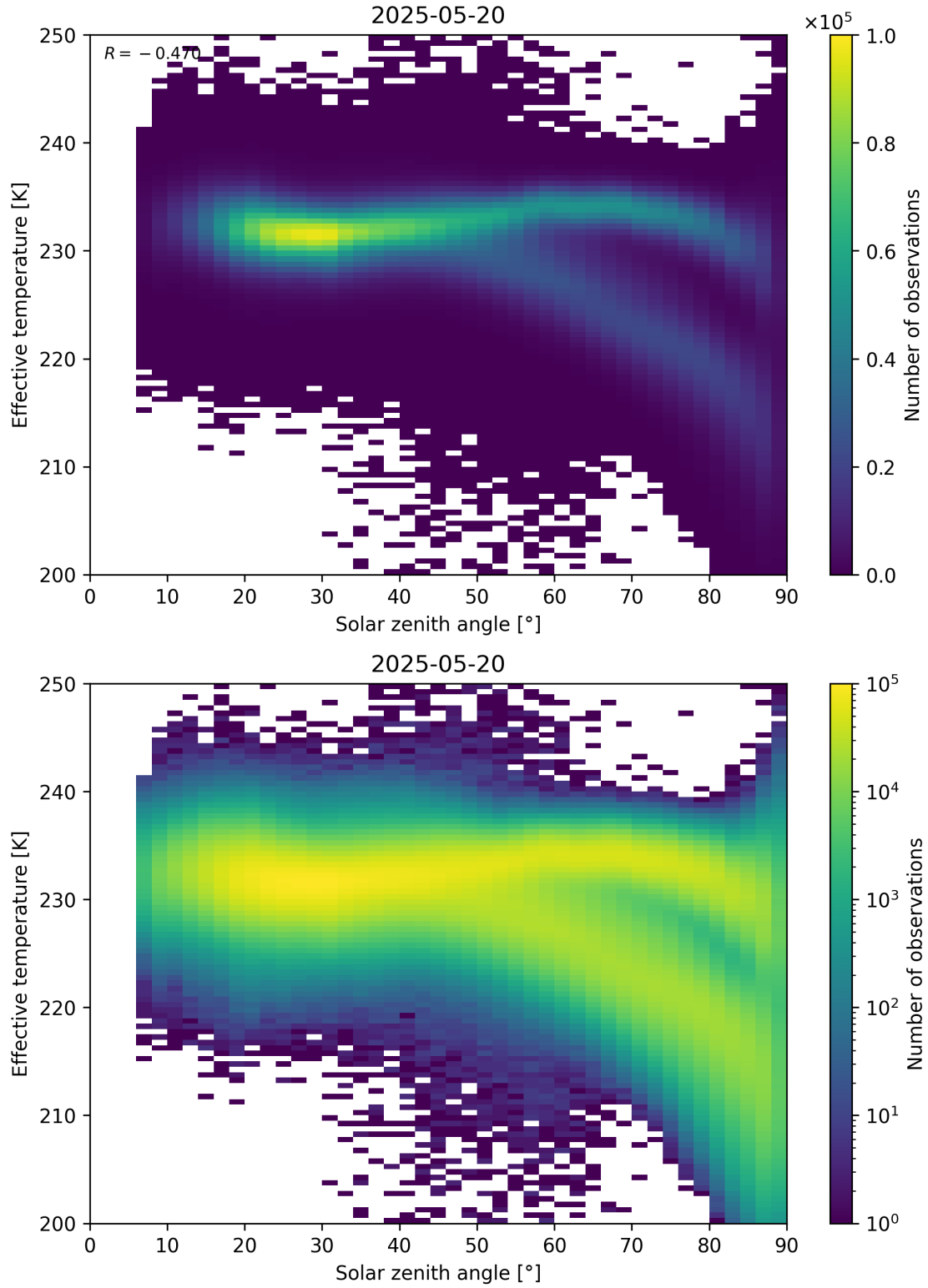
Figure 45: Scatter density plot of “Solar zenith angle” against “Effective temperature” for 2025-05-19 to 2025-05-21.
