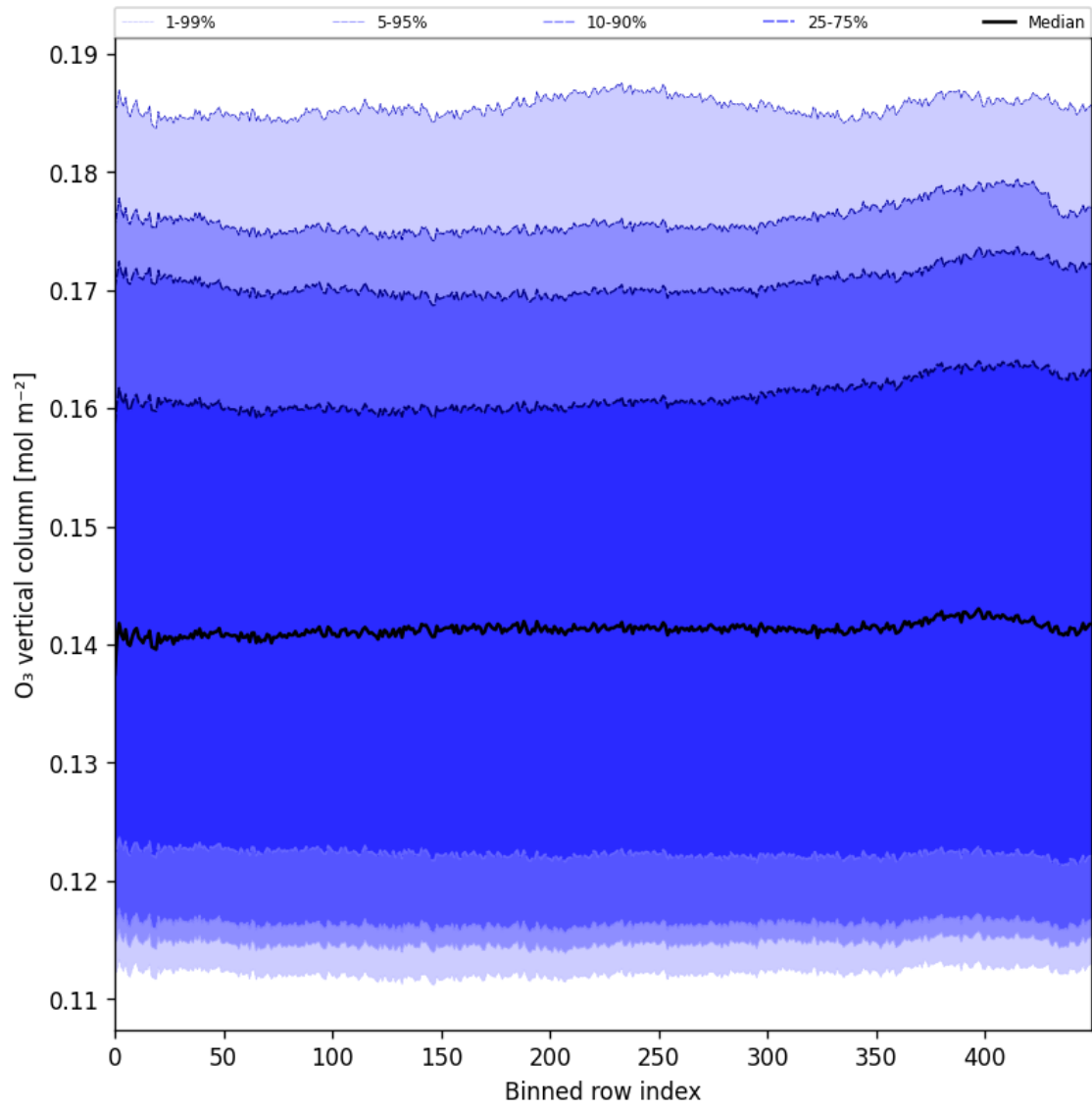
Figure 28: Along track statistics of “ O_3 vertical column” for 2025-05-19 to 2025-05-21
