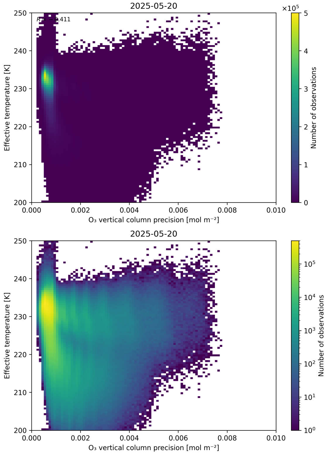
Figure 42: Scatter density plot of “O 3 vertical column precision” against “Effective temperature” for 2025-05-19 to 2025-05-21.
