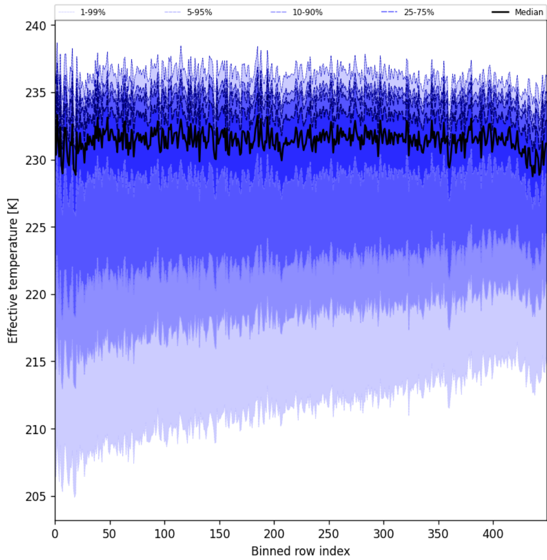
Figure 31: Along track statistics of “Effective temperature” for 2025-05-19 to 2025-05-21
