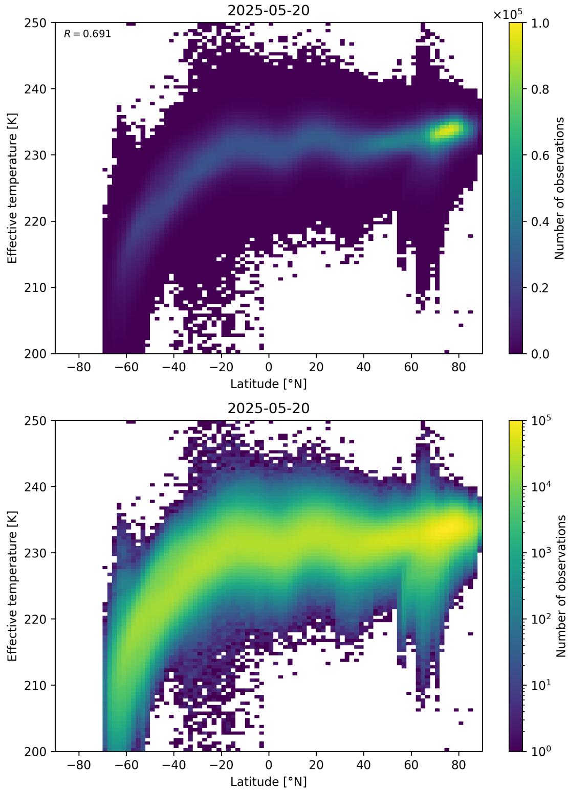
Figure 34: Scatter density plot of “Latitude” against “Effective temperature” for 2025-05-19 to 2025-05-21.
