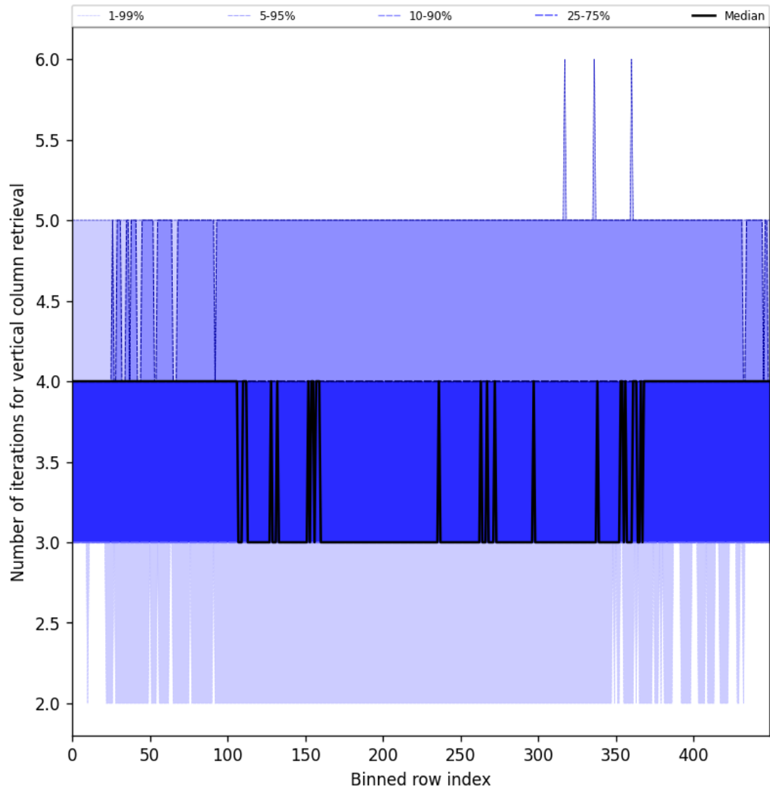
Figure 33: Along track statistics of “Number of iterations for vertical column retrieval” for 2025-05-19 to 2025-05-21
