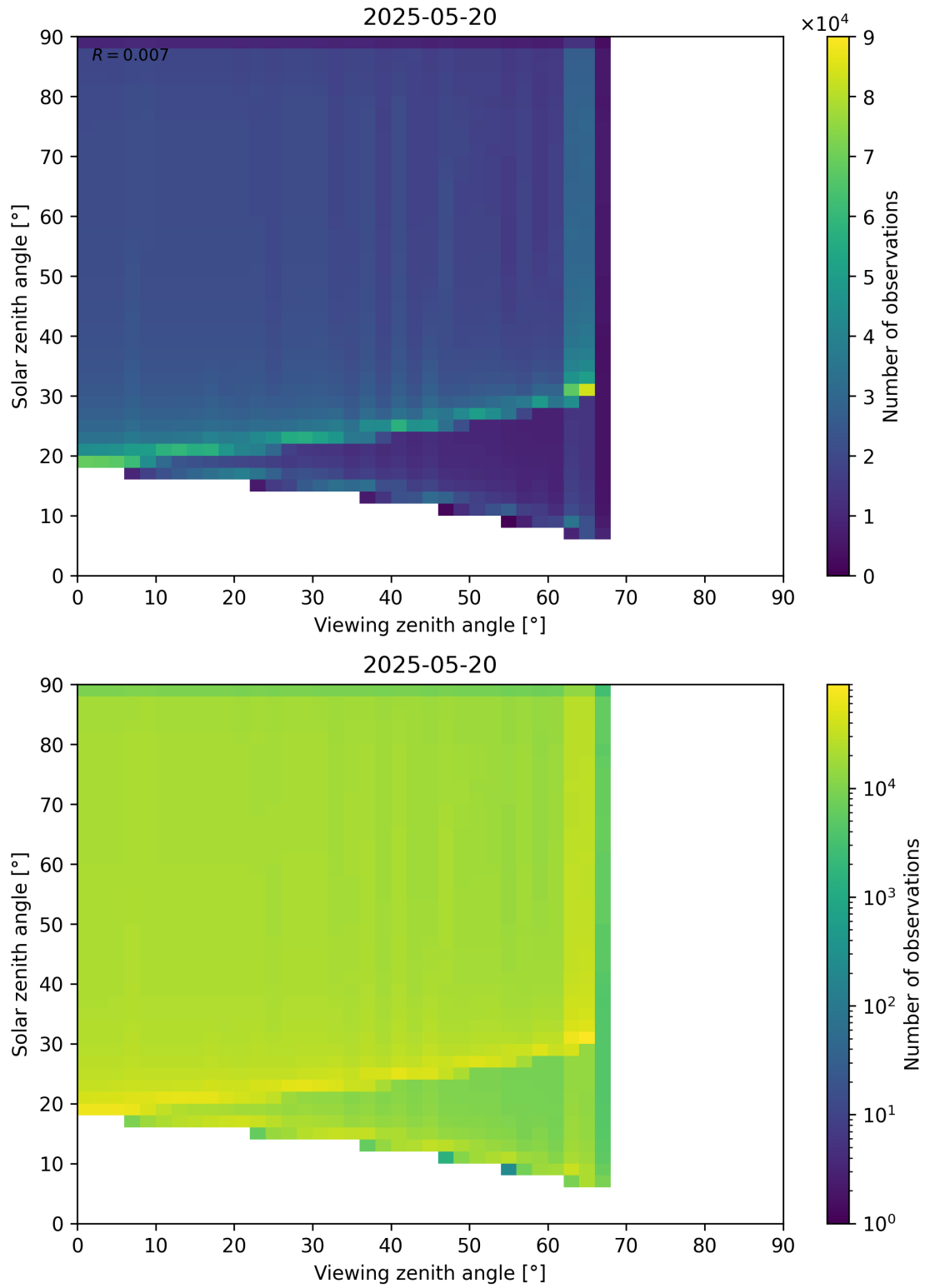
Figure 54: Scatter density plot of “Viewing zenith angle” against “Solar zenith angle” for 2025-05-19 to 2025-05-21.
