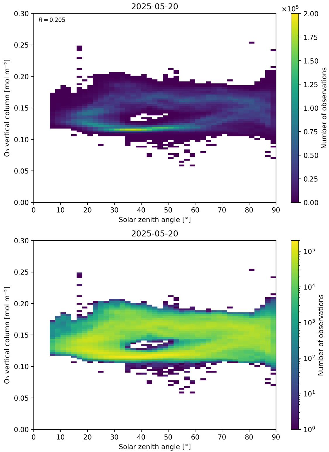
Figure 47: Scatter density plot of “Solar zenith angle” against “O 3 vertical column” for 2025-05-19 to 2025-05-21.
