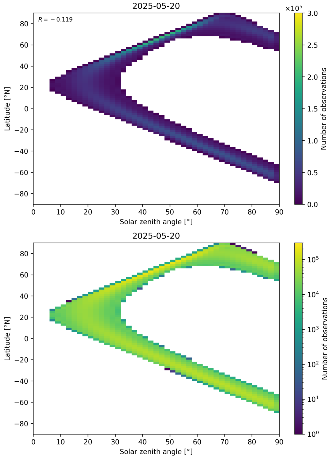
Figure 44: Scatter density plot of “Solar zenith angle” against “Latitude” for 2025-05-19 to 2025-05-21.
