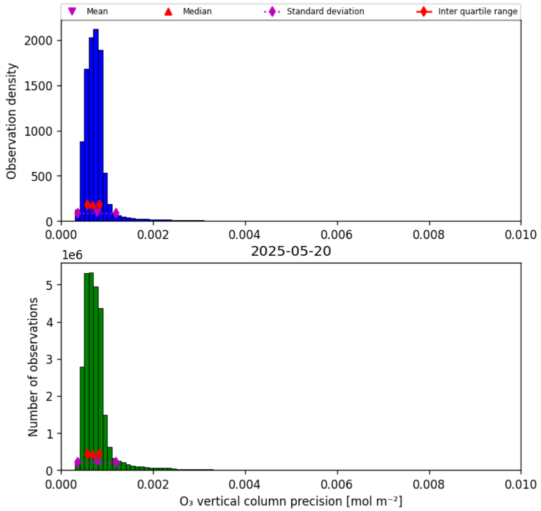
Figure 22: Histogram of “O 3 vertical column precision” for 2025-05-19 to 2025-05-21
