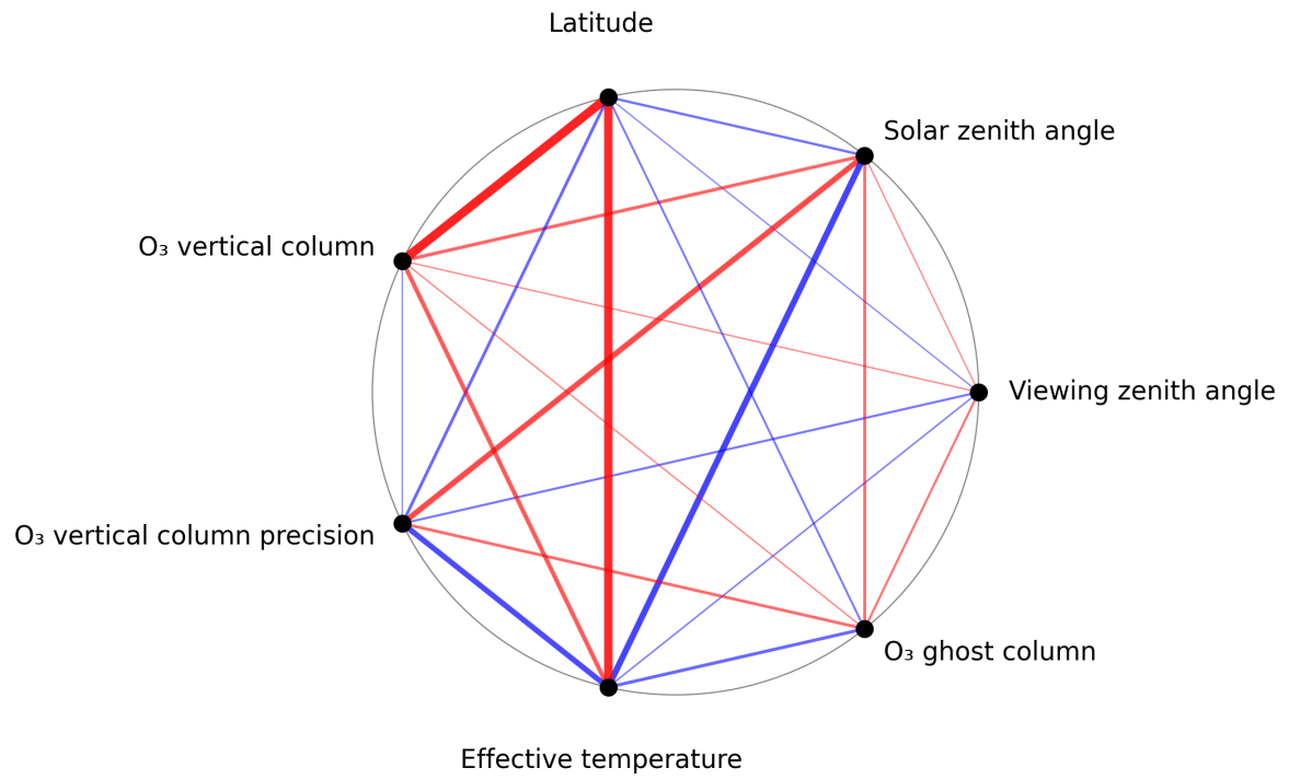
Figure 1: Map of correlation graph for 2025-05-19 to 2025-05-21.
