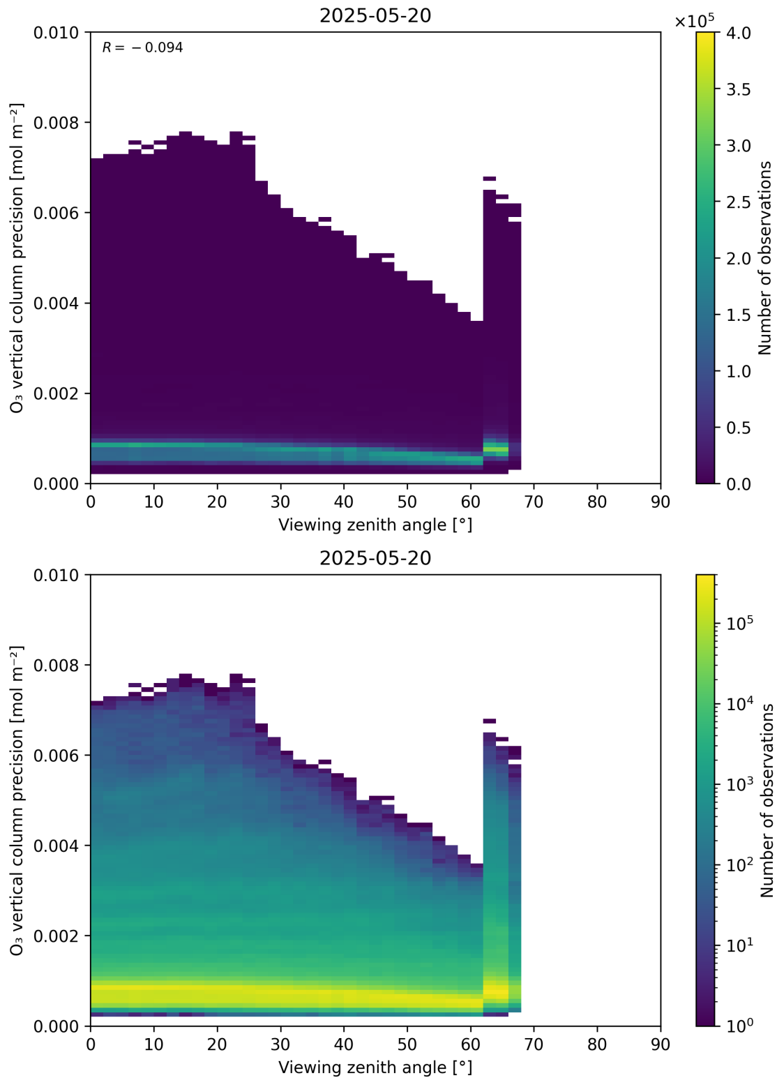
Figure 53: Scatter density plot of “Viewing zenith angle” against “O 3 vertical column precision” for 2025-05-19 to 2025-05-21.
