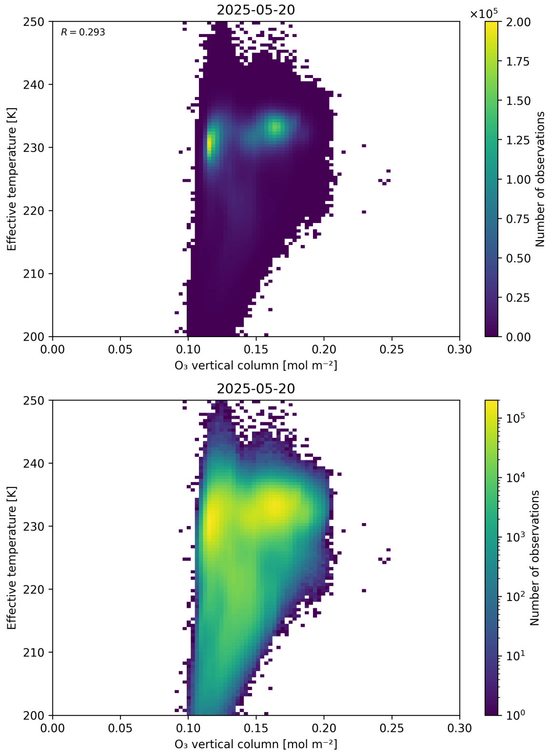
Figure 39: Scatter density plot of “O 3 vertical column” against “Effective temperature” for 2025-05-19 to 2025-05-21.
