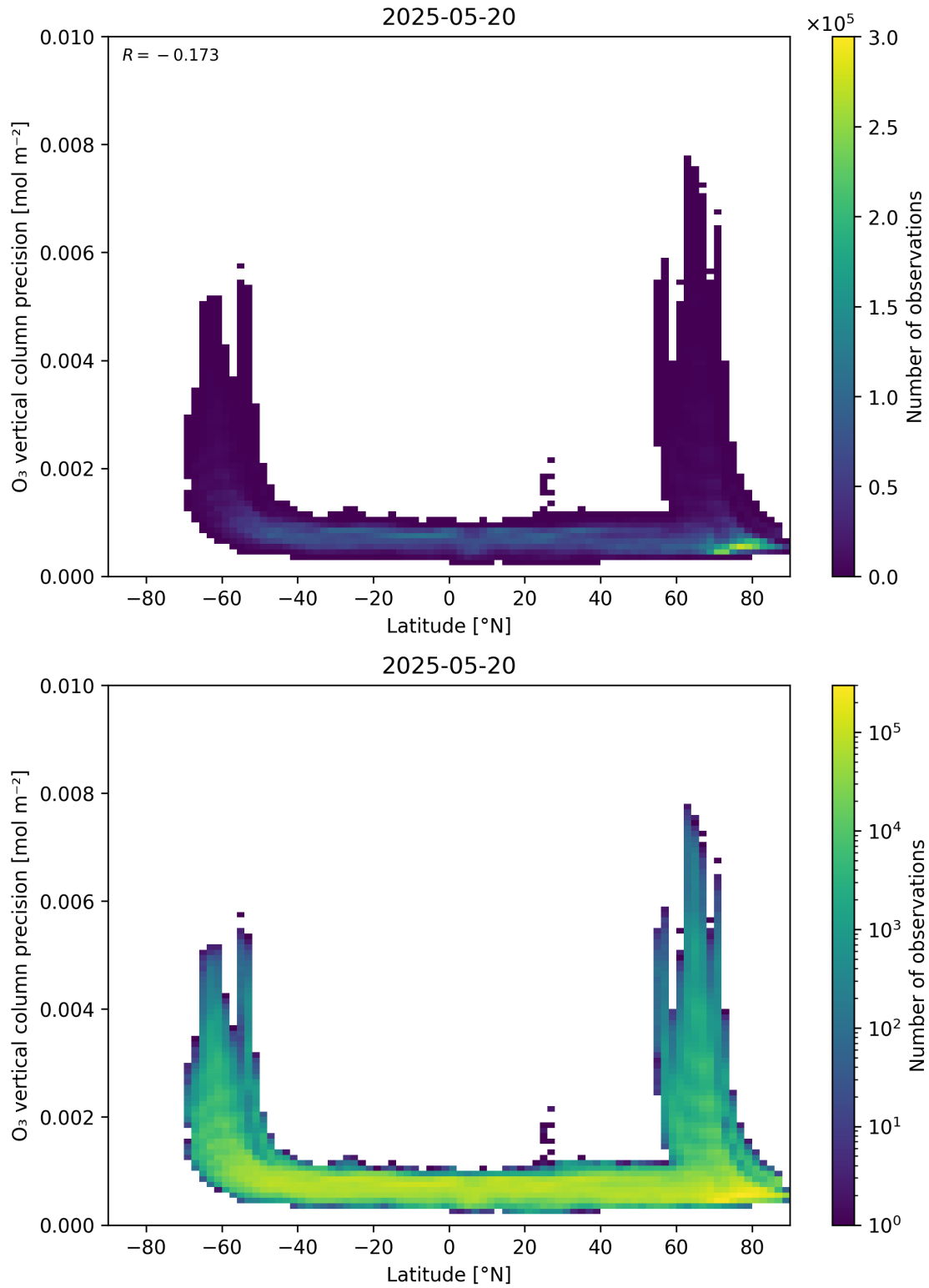
Figure 37: Scatter density plot of “Latitude” against “O 3 vertical column precision” for 2025-05-19 to 2025-05-21.
