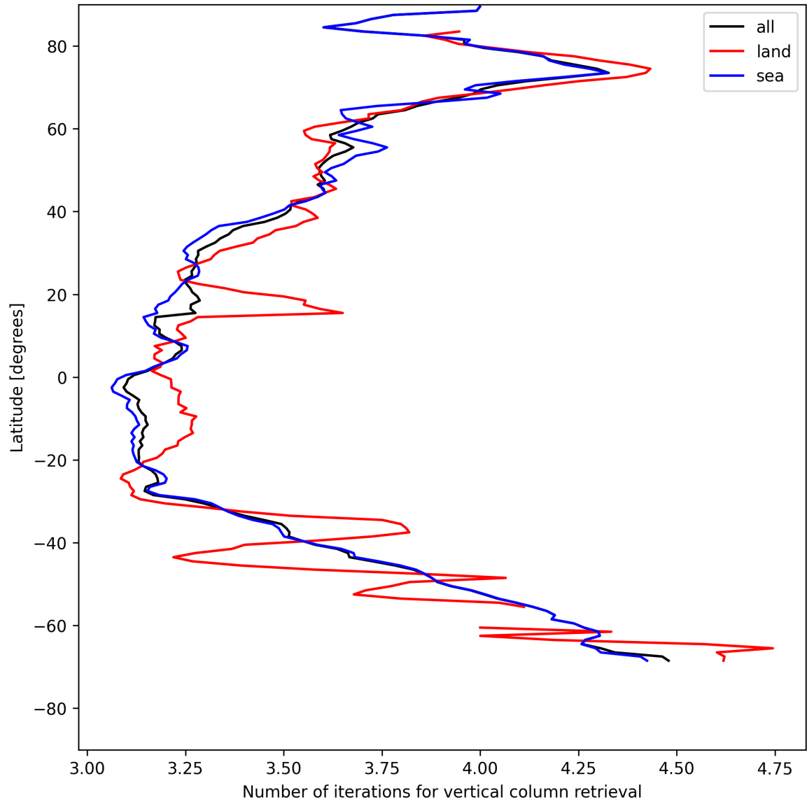
Figure 19: Zonal average of “Number of iterations for vertical column retrieval” for 2025-05-19 to 2025-05-21.
