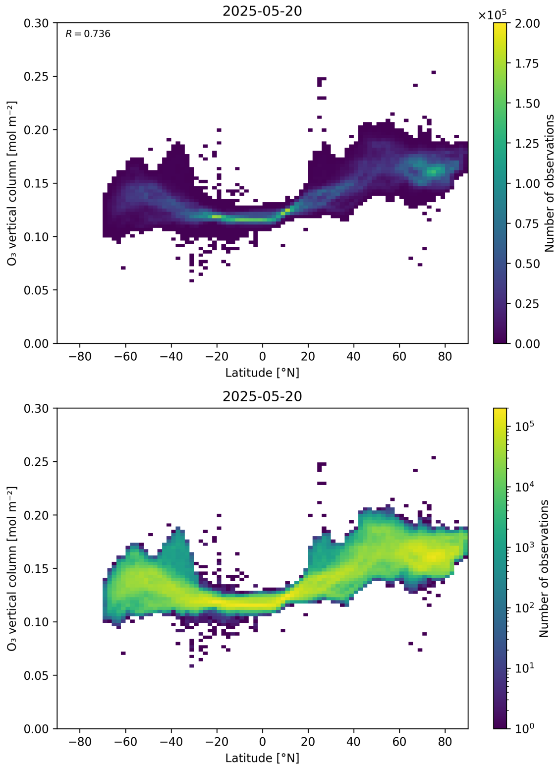
Figure 36: Scatter density plot of “Latitude” against “O 3 vertical column” for 2025-05-19 to 2025-05-21.
