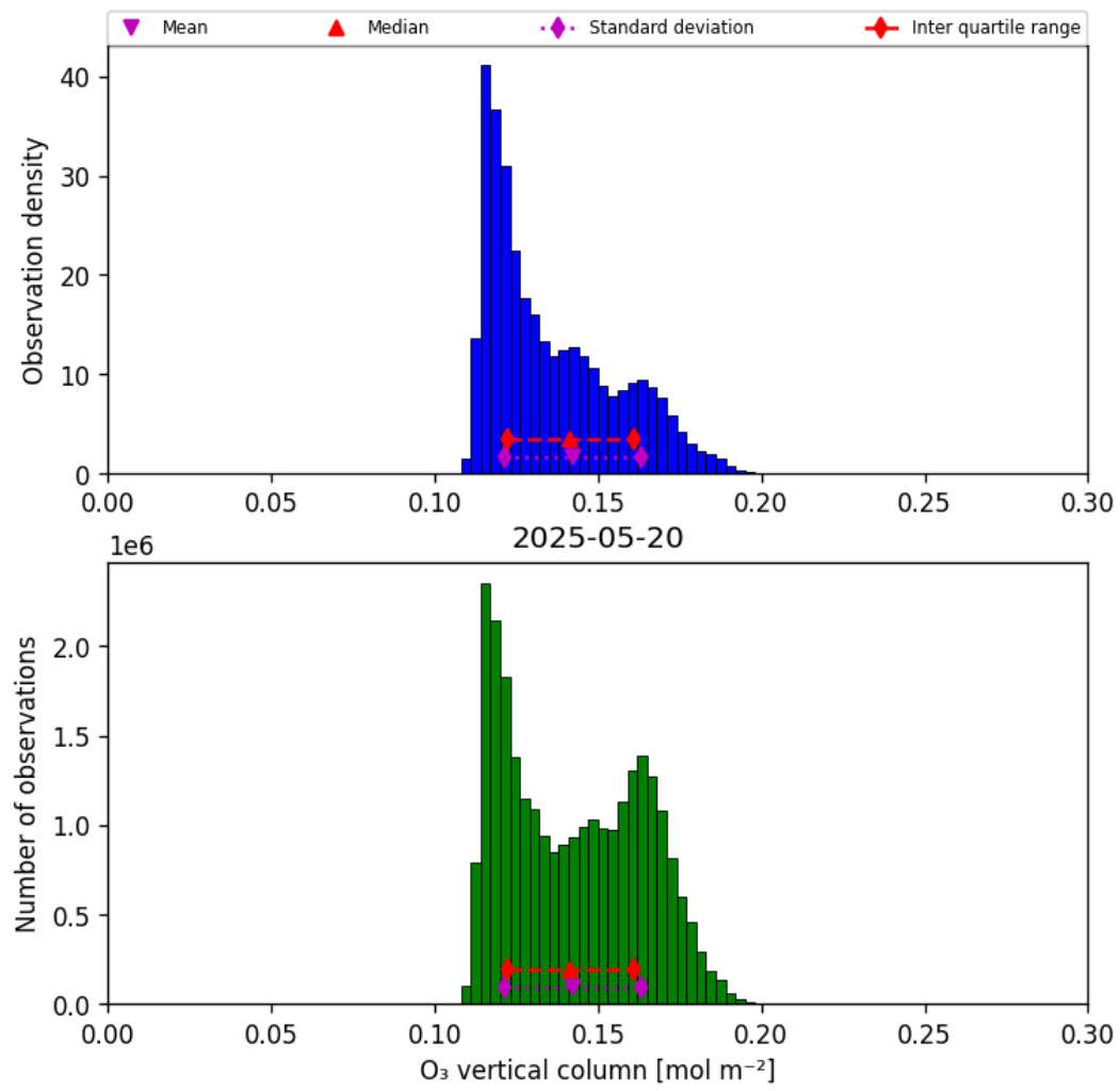
Figure 21: Histogram of “O 3 vertical column” for 2025-05-19 to 2025-05-21
