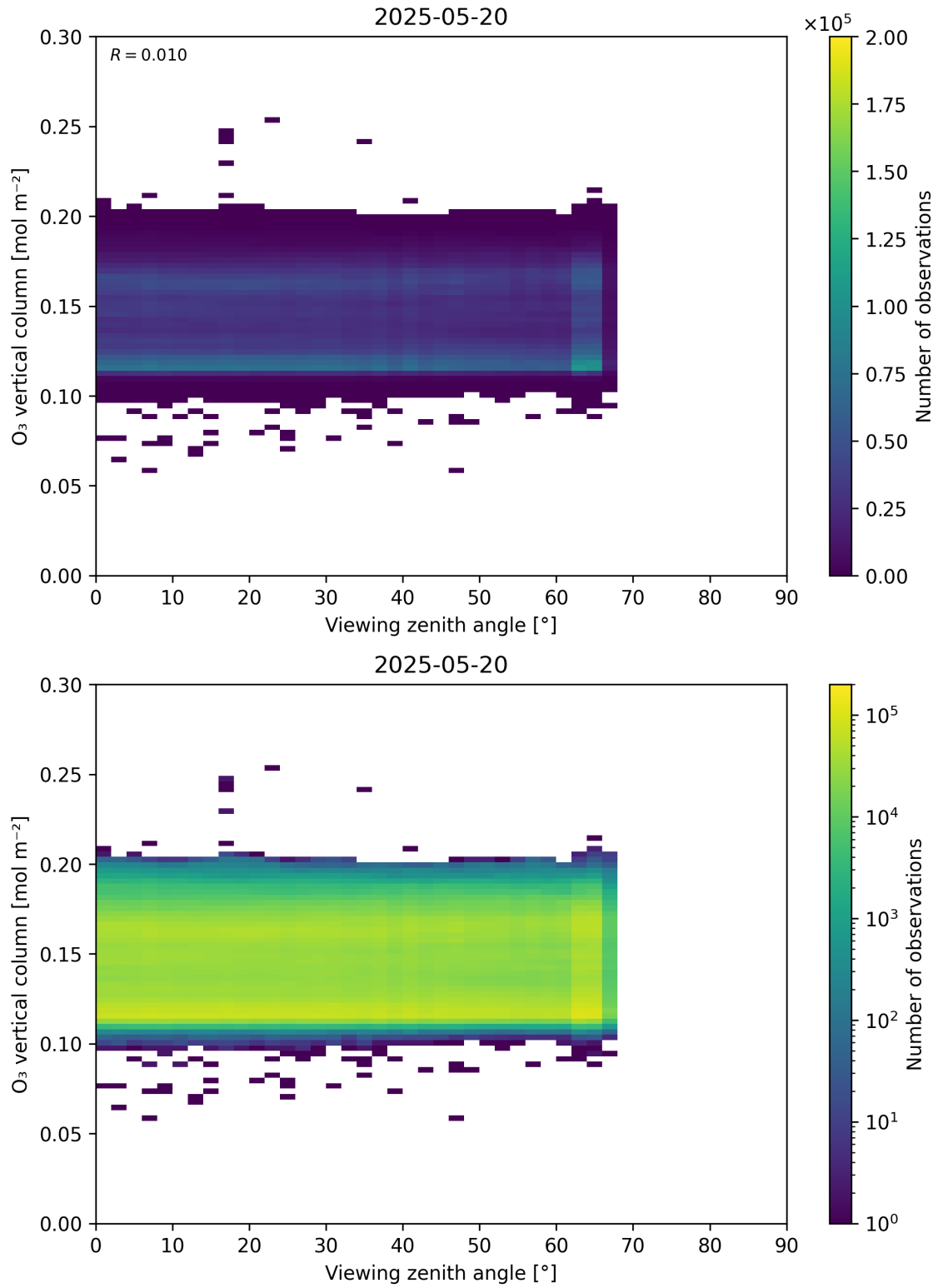
Figure 52: Scatter density plot of “Viewing zenith angle” against “O 3 vertical column” for 2025-05-19 to 2025-05-21.
