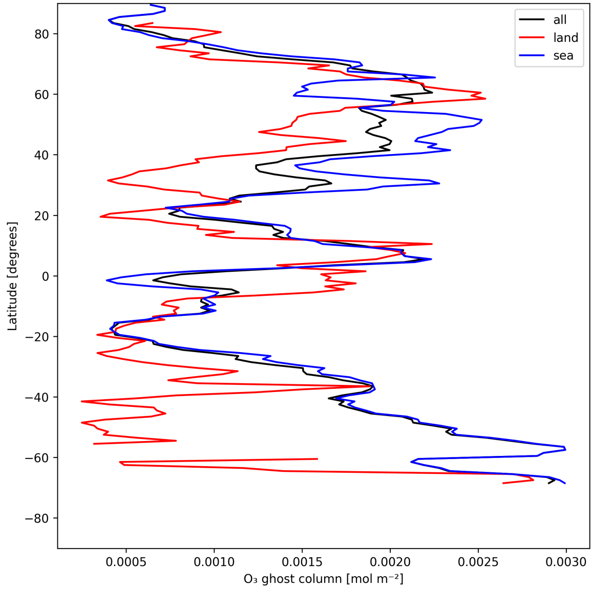
Figure 18: Zonal average of “O 3 ghost column” for 2025-05-19 to 2025-05-21.
