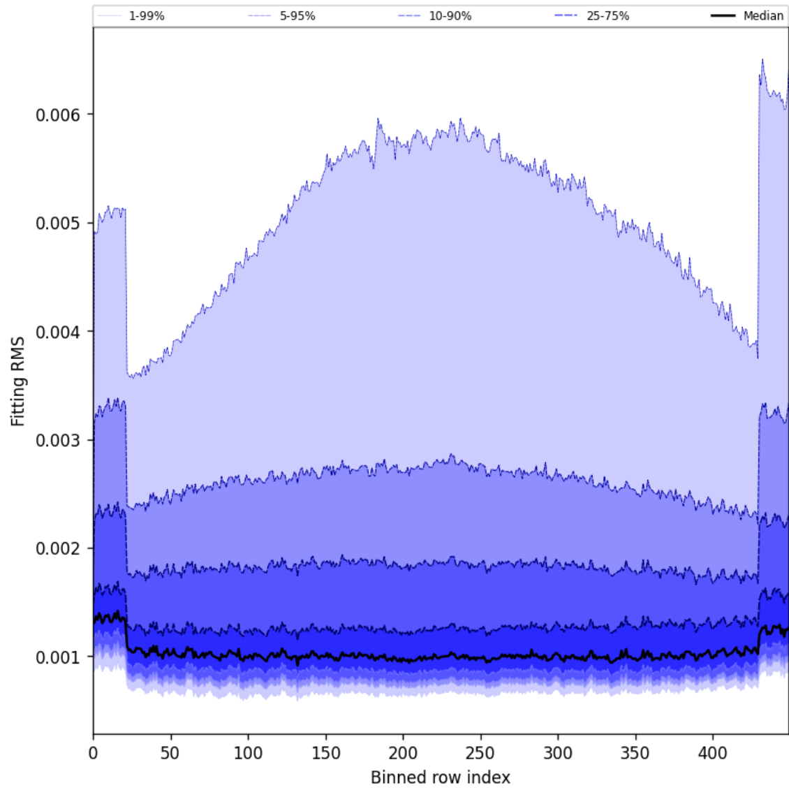
Figure 30: Along track statistics of “Fitting RMS” for 2025-05-19 to 2025-05-21
