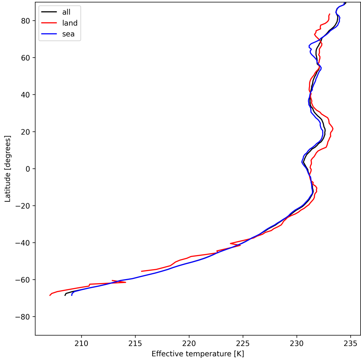
Figure 17: Zonal average of "Effective temperature" for 2025-05-19 to 2025-05-21.
