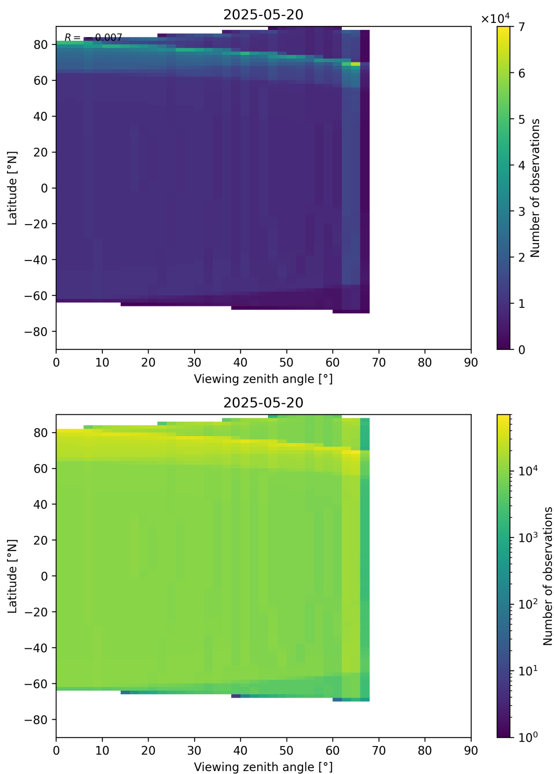
Figure 49: Scatter density plot of “Viewing zenith angle” against “Latitude” for 2025-05-19 to 2025-05-21.
