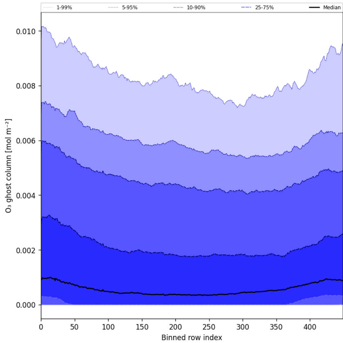
Figure 32: Along track statistics of “O 3 ghost column” for 2025-05-19 to 2025-05-21
