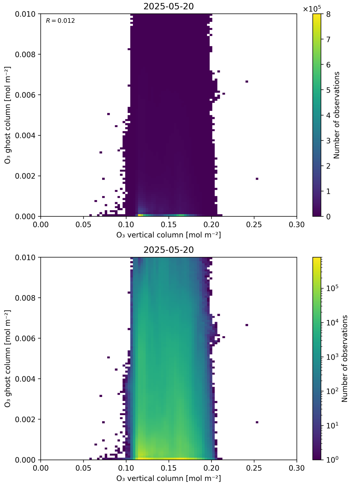
Figure 40: Scatter density plot of “O 3 vertical column” against “O 3 ghost column” for 2025-05-19 to 2025-05-21.
