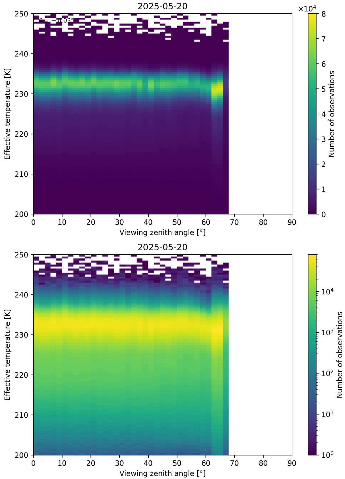
Figure 50: Scatter density plot of “Viewing zenith angle” against “Effective temperature” for 2025-05-19 to 2025-05-21.
