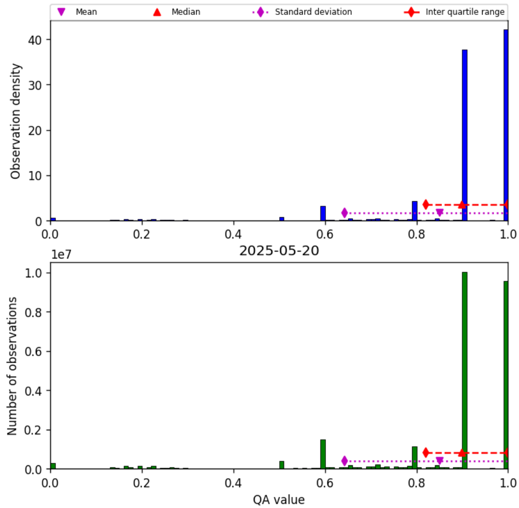
Figure 20: Histogram of “QA value” for 2025-05-19 to 2025-05-21
