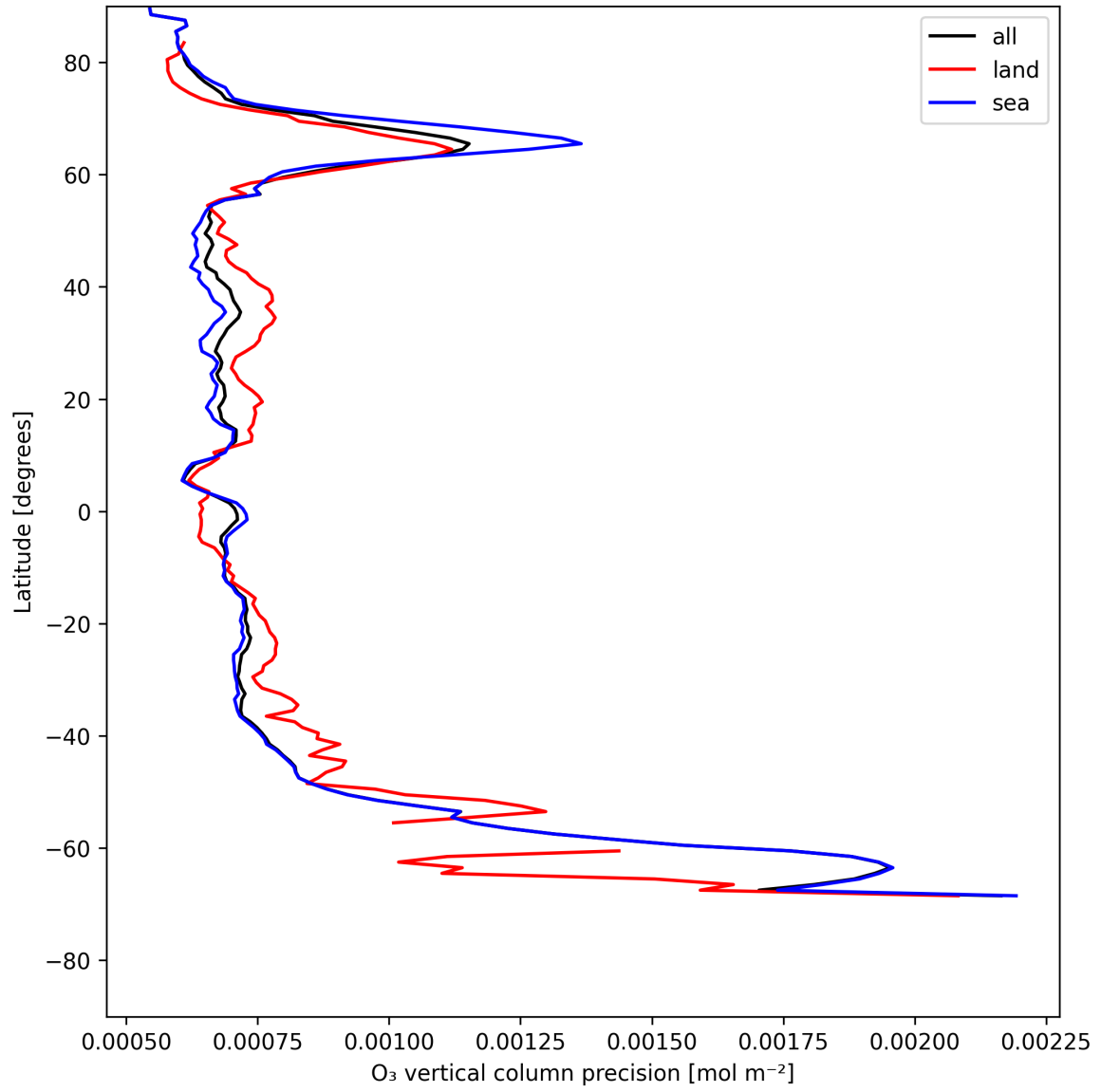
Figure 15: Zonal average of “O 3 vertical column precision” for 2025-05-19 to 2025-05-21.
