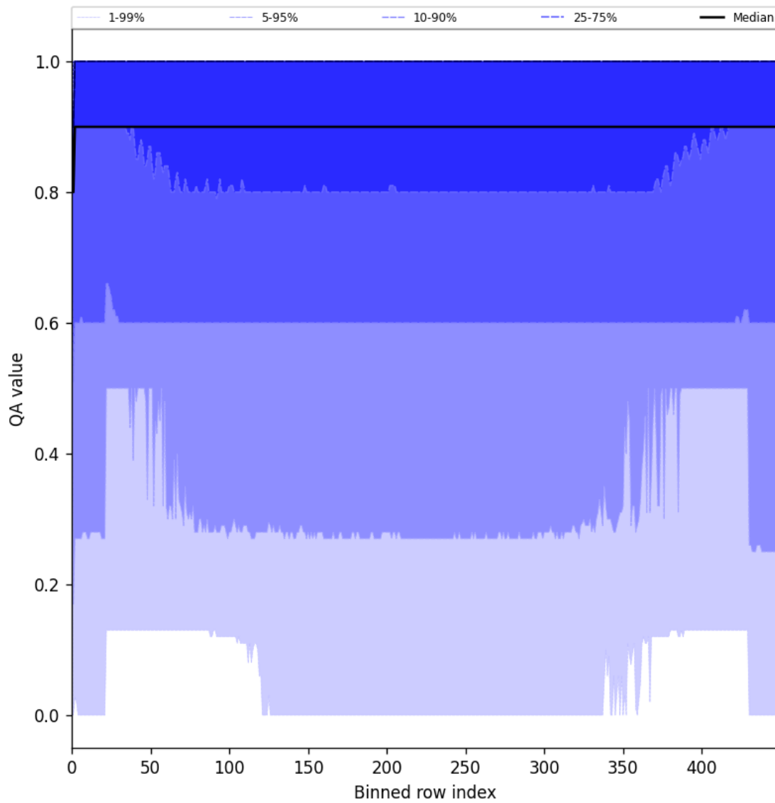
Figure 27: Along track statistics of “QA value” for 2025-05-19 to 2025-05-21
