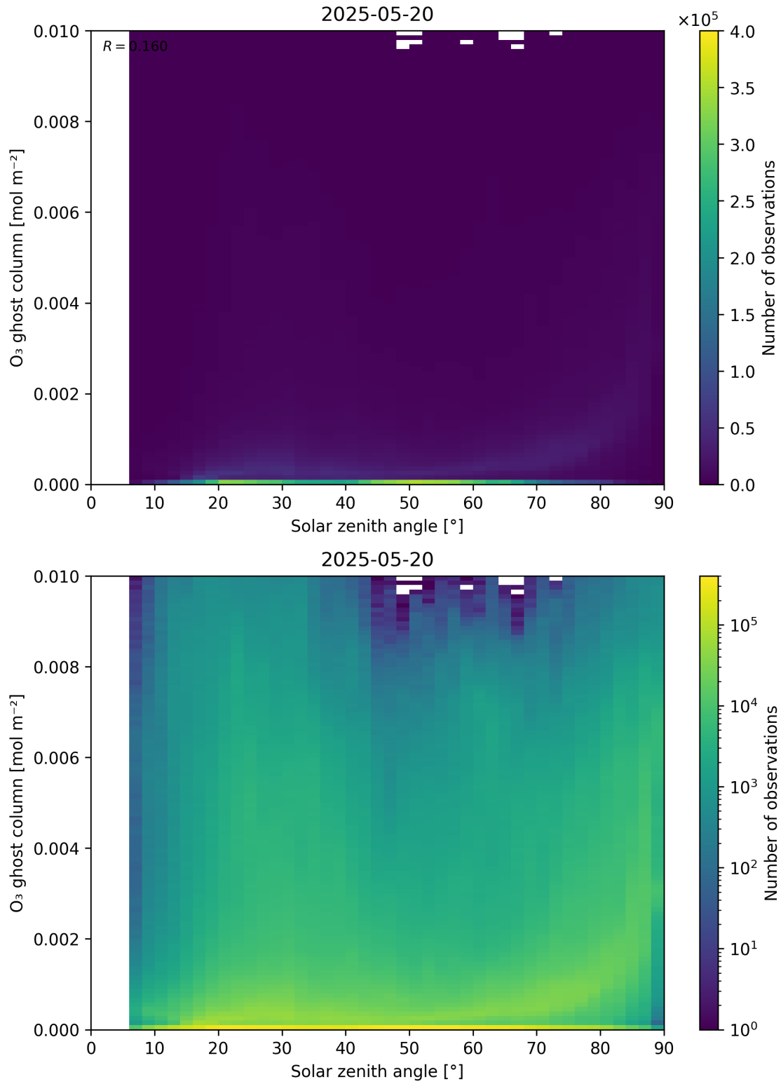
Figure 46: Scatter density plot of “Solar zenith angle” against “O 3 ghost column” for 2025-05-19 to 2025-05-21.
