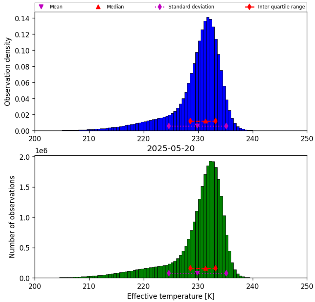
Figure 24: Histogram of “Effective temperature” for 2025-05-19 to 2025-05-21
