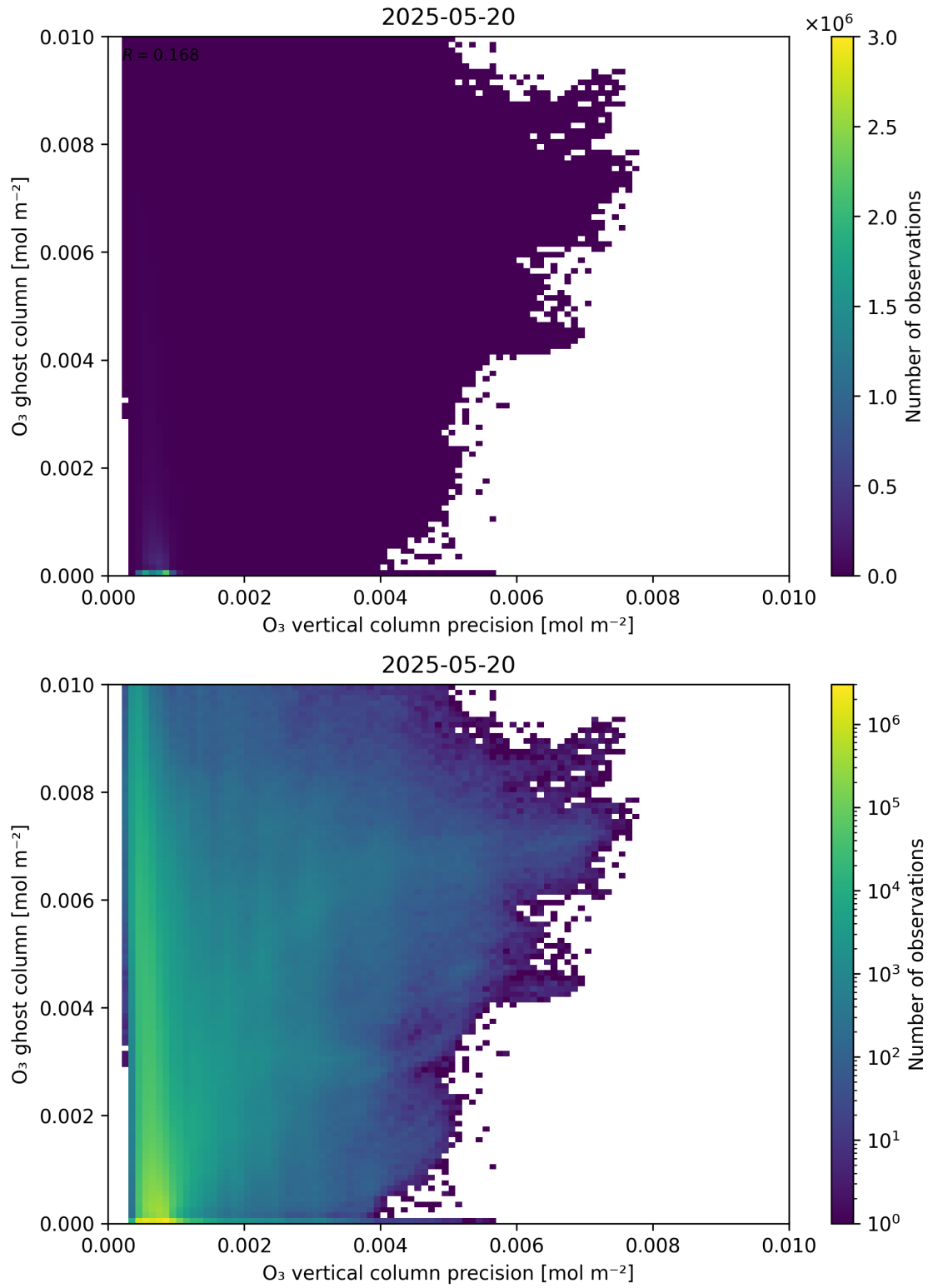
Figure 43: Scatter density plot of “ \text{O}_3 vertical column precision” against “ \text{O}_3 ghost column” for 2025-05-19 to 2025-05-21.
