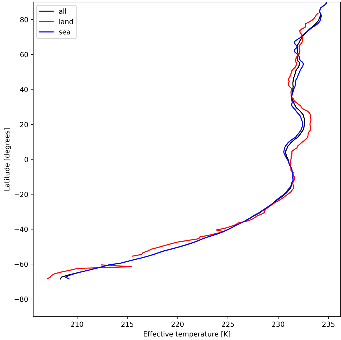
Figure 17: Zonal average of "Effective temperature" for 2025-05-21 to 2025-05-22.
