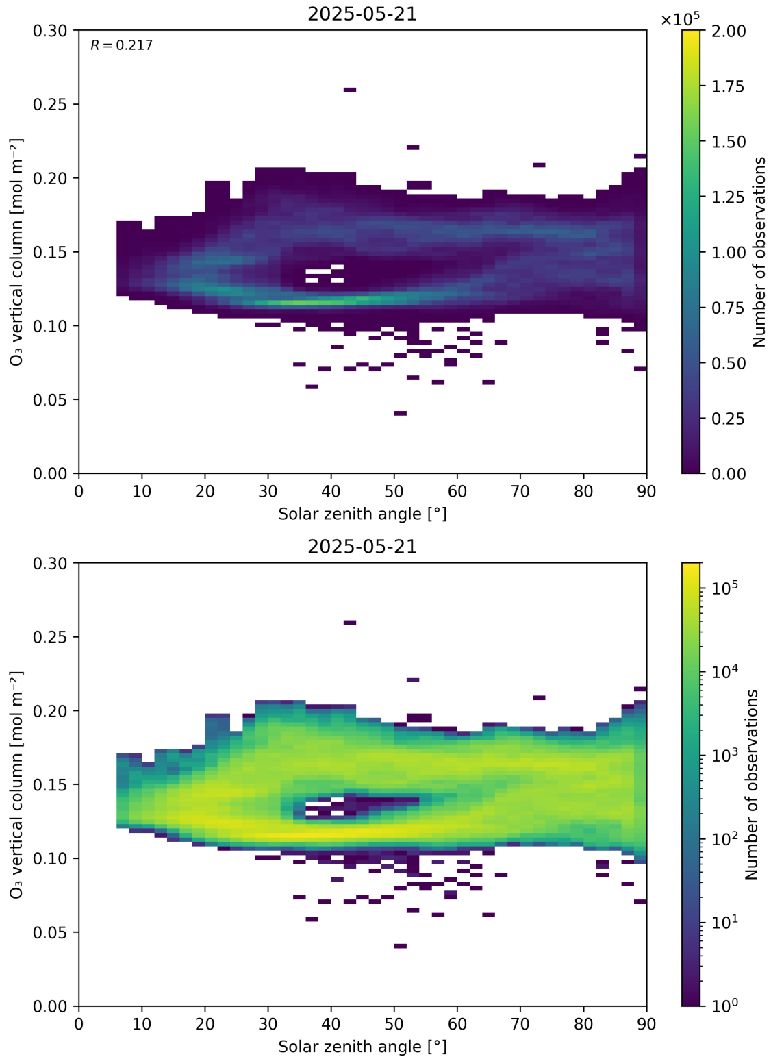
Figure 47: Scatter density plot of “Solar zenith angle” against “O 3 vertical column” for 2025-05-21 to 2025-05-22.
