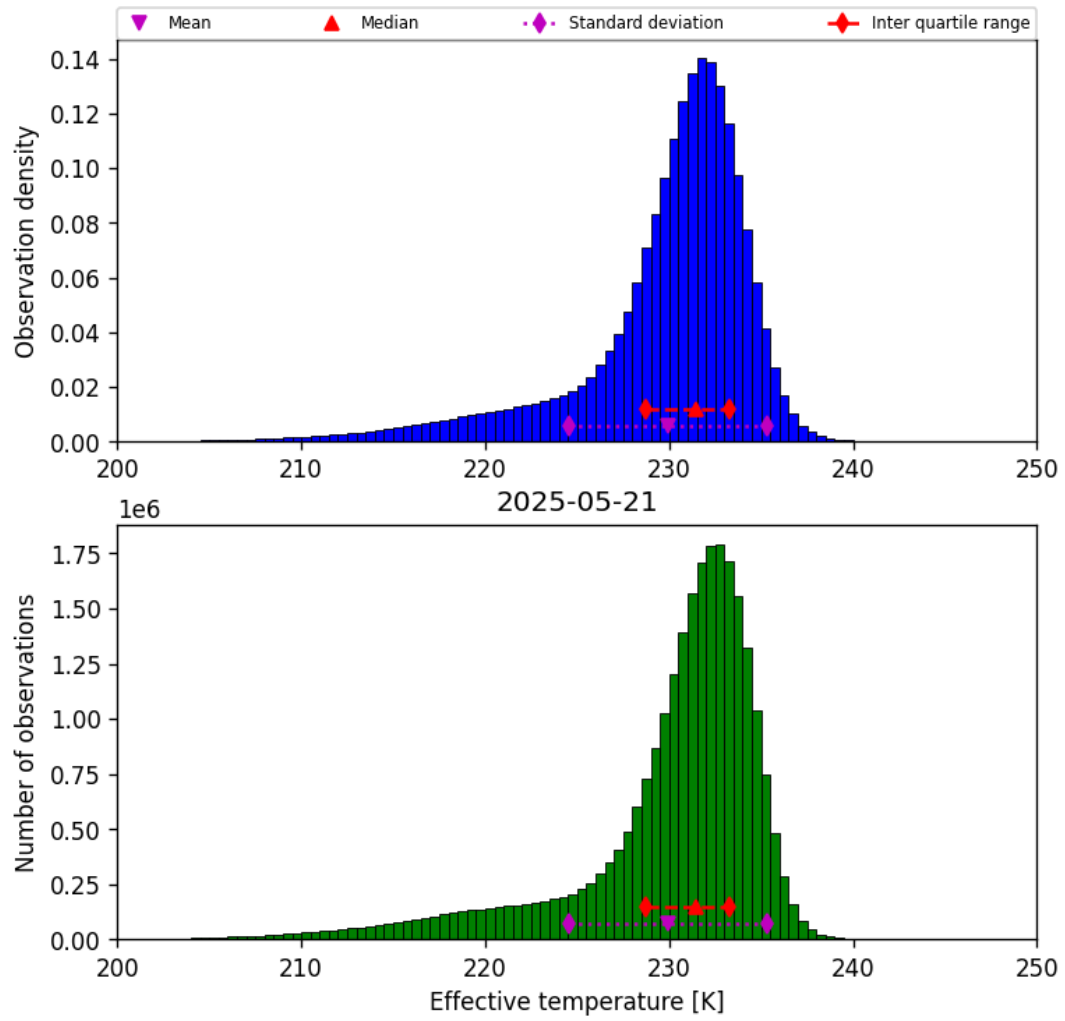
Figure 24: Histogram of “Effective temperature” for 2025-05-21 to 2025-05-22
