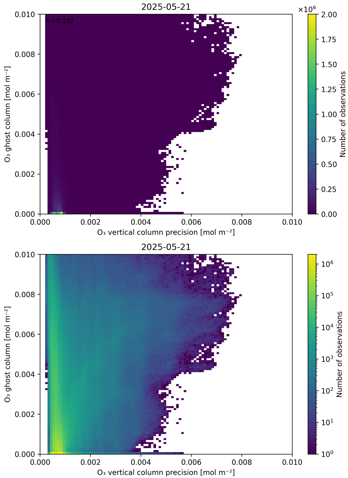
Figure 43: Scatter density plot of “O 3 vertical column precision” against “O 3 ghost column” for 2025-05-21 to 2025-05-22.
