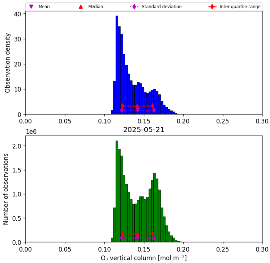
Figure 21: Histogram of “O 3 vertical column” for 2025-05-21 to 2025-05-22
