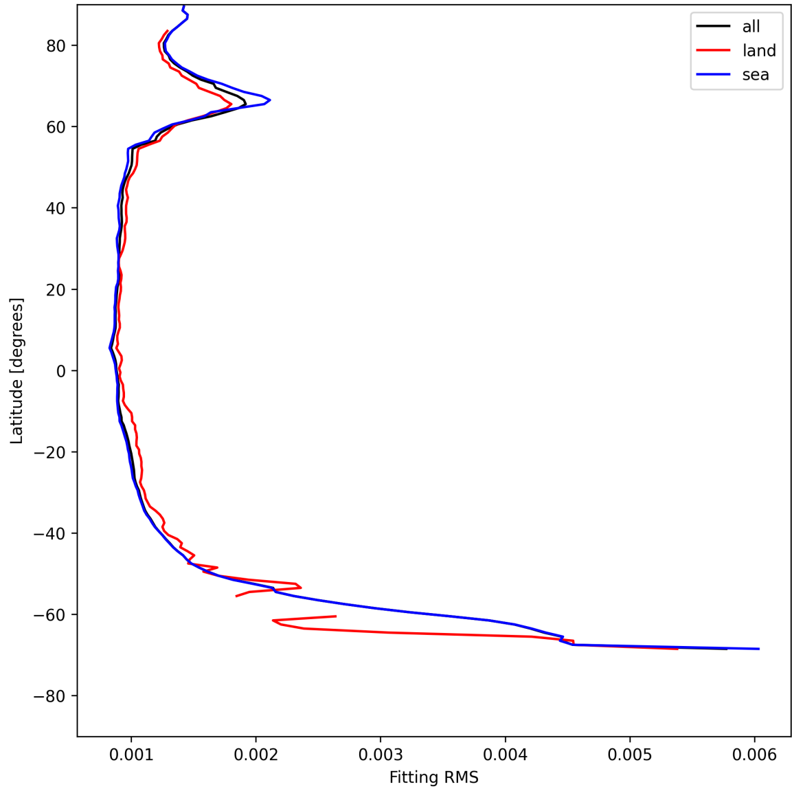
Figure 16: Zonal average of “Fitting RMS” for 2025-05-21 to 2025-05-22.
