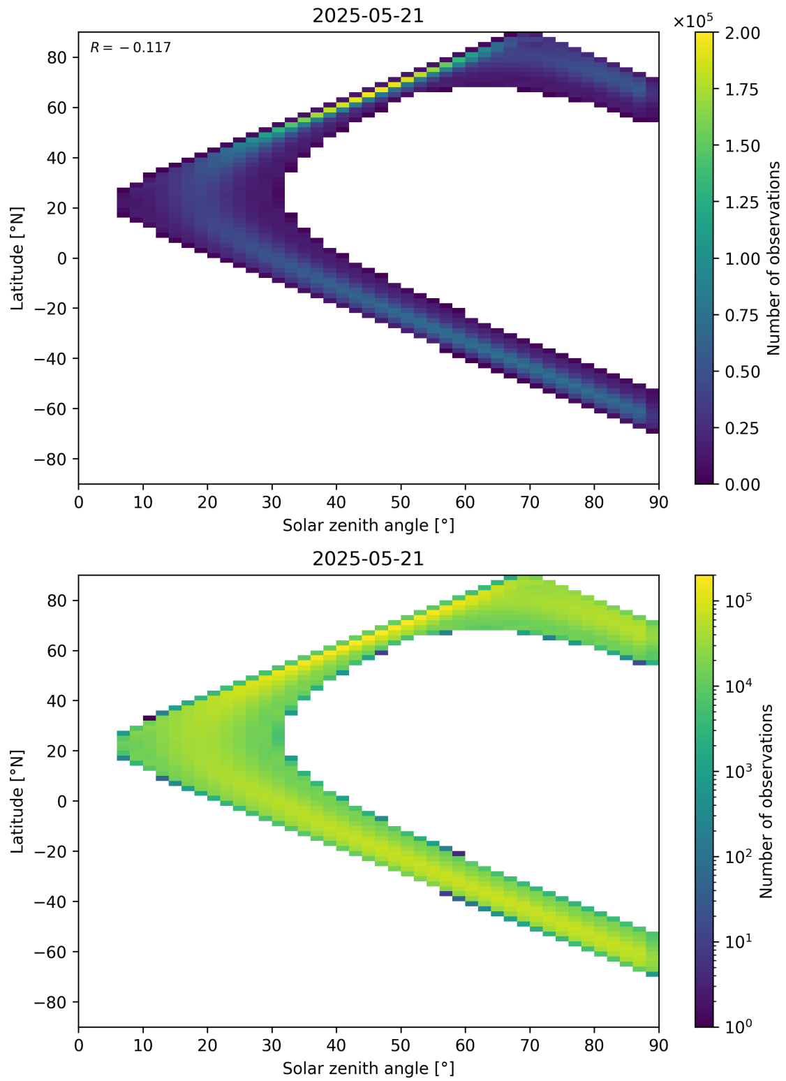
Figure 44: Scatter density plot of “Solar zenith angle” against “Latitude” for 2025-05-21 to 2025-05-22.
