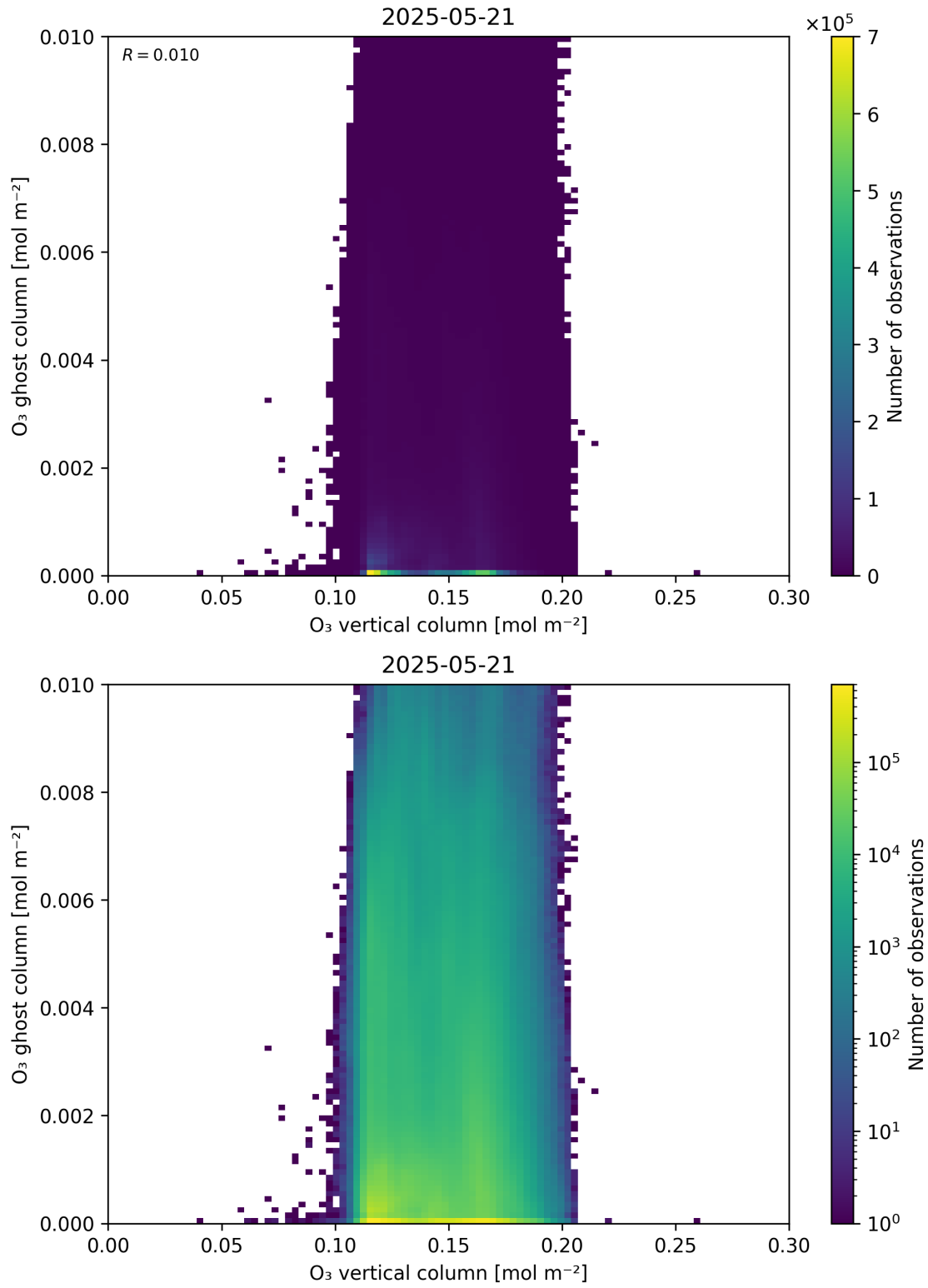
Figure 40: Scatter density plot of “O 3 vertical column” against “O 3 ghost column” for 2025-05-21 to 2025-05-22.
