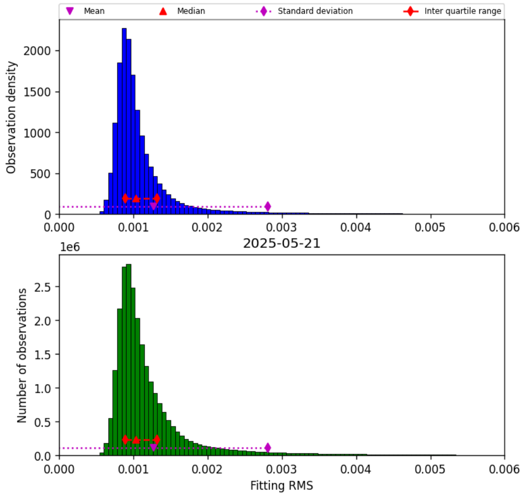
Figure 23: Histogram of “Fitting RMS” for 2025-05-21 to 2025-05-22
