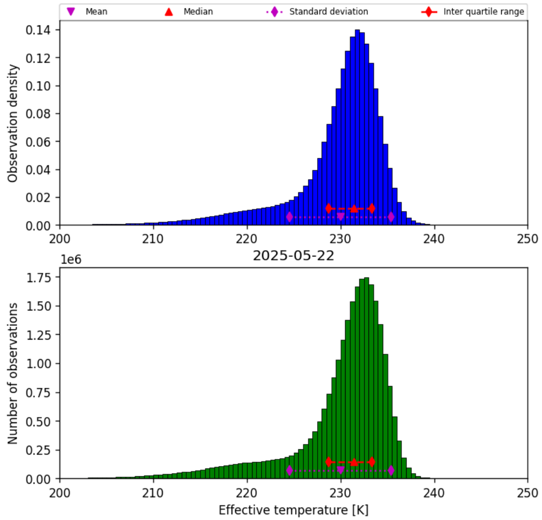
Figure 24: Histogram of “Effective temperature” for 2025-05-21 to 2025-05-23
