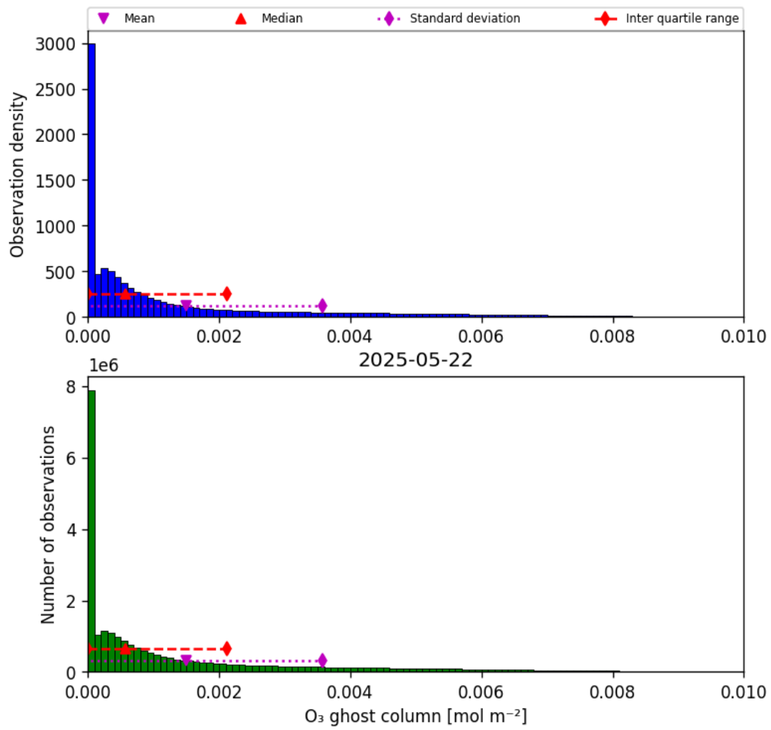
Figure 25: Histogram of “O 3 ghost column” for 2025-05-21 to 2025-05-23
