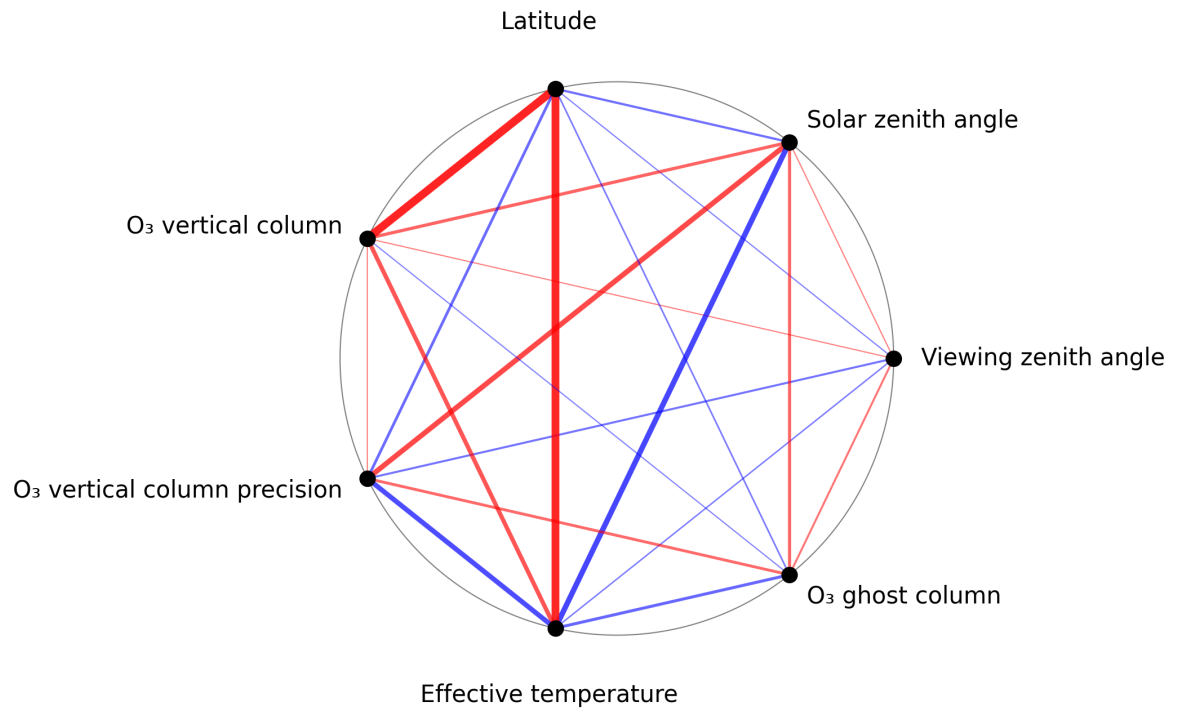
Figure 1: Map of correlation graph for 2025-05-21 to 2025-05-23.
