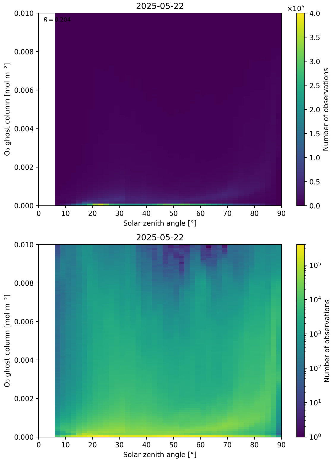
Figure 46: Scatter density plot of “Solar zenith angle” against “O 3 ghost column” for 2025-05-21 to 2025-05-23.
