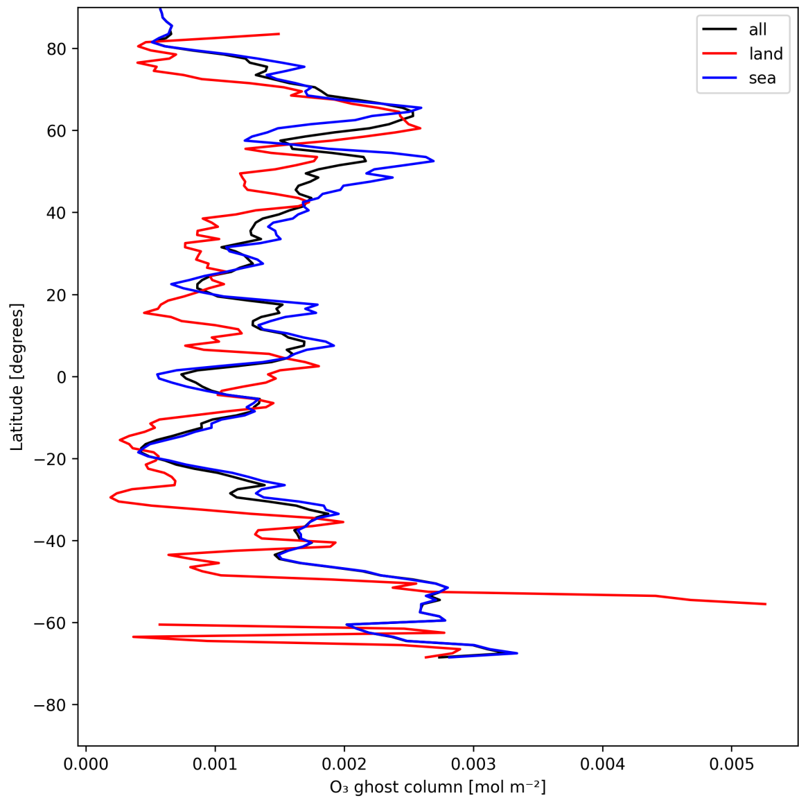
Figure 18: Zonal average of “O 3 ghost column” for 2025-05-21 to 2025-05-23.
