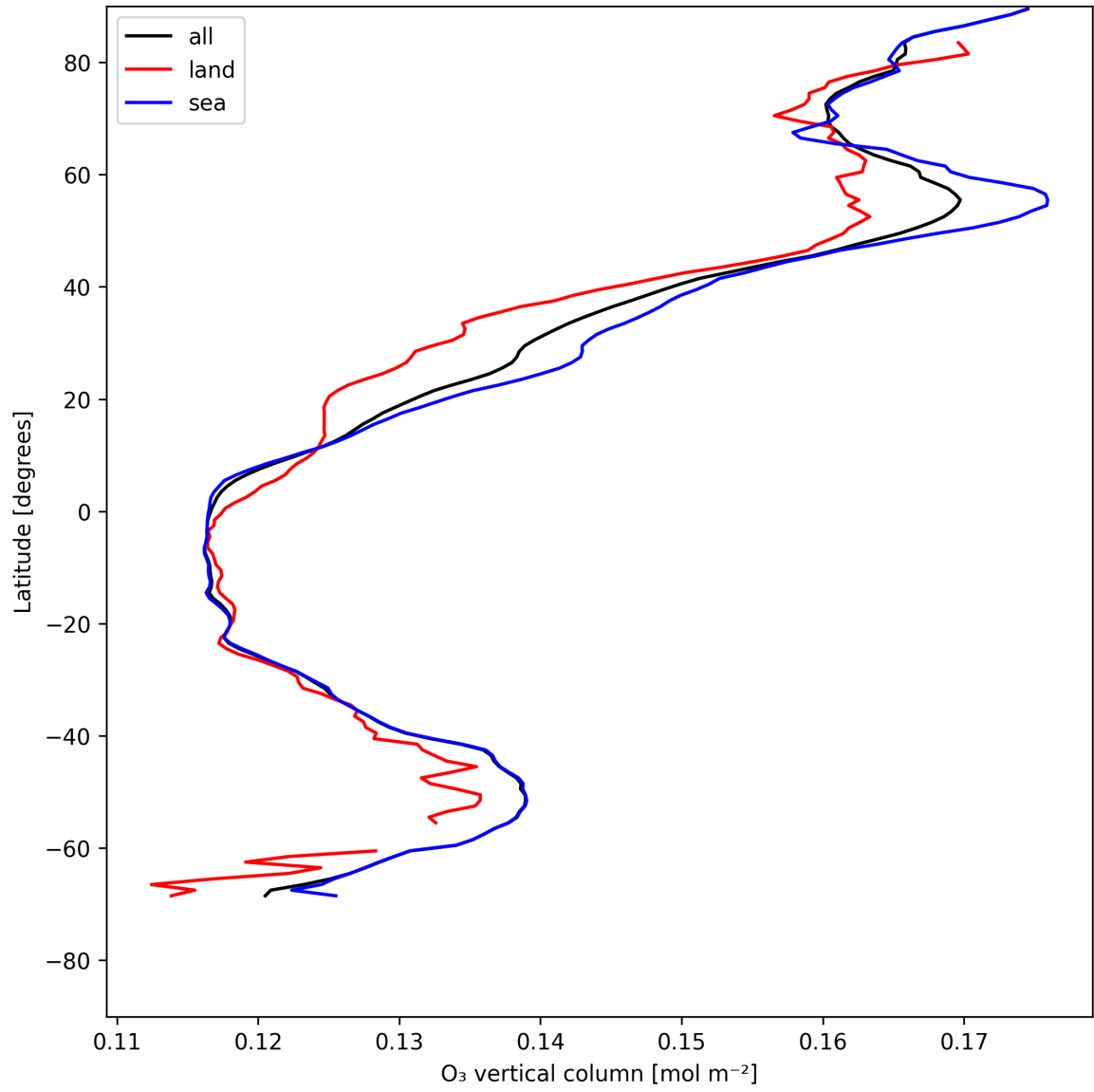
Figure 14: Zonal average of “O 3 vertical column” for 2025-05-21 to 2025-05-23.
