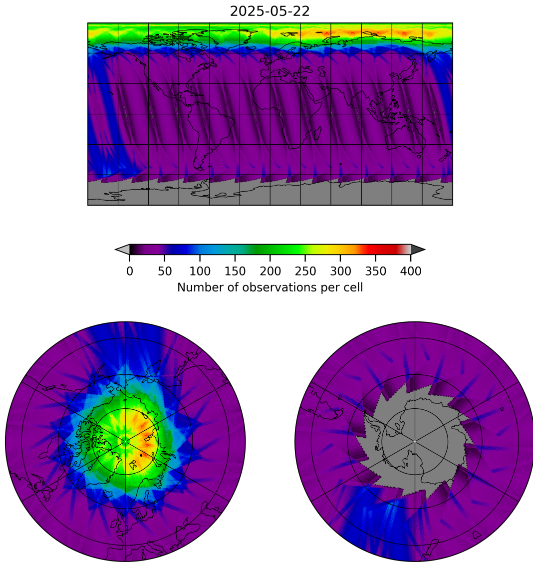
Figure 12: Map of the number of observations for 2025-05-21 to 2025-05-23
