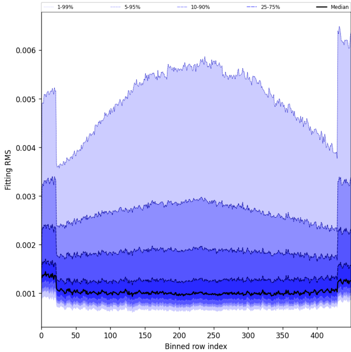
Figure 30: Along track statistics of “Fitting RMS” for 2025-05-21 to 2025-05-23
