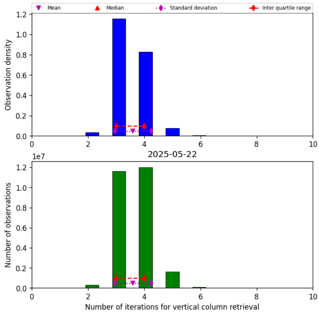
Figure 26: Histogram of “Number of iterations for vertical column retrieval” for 2025-05-21 to 2025-05-23
