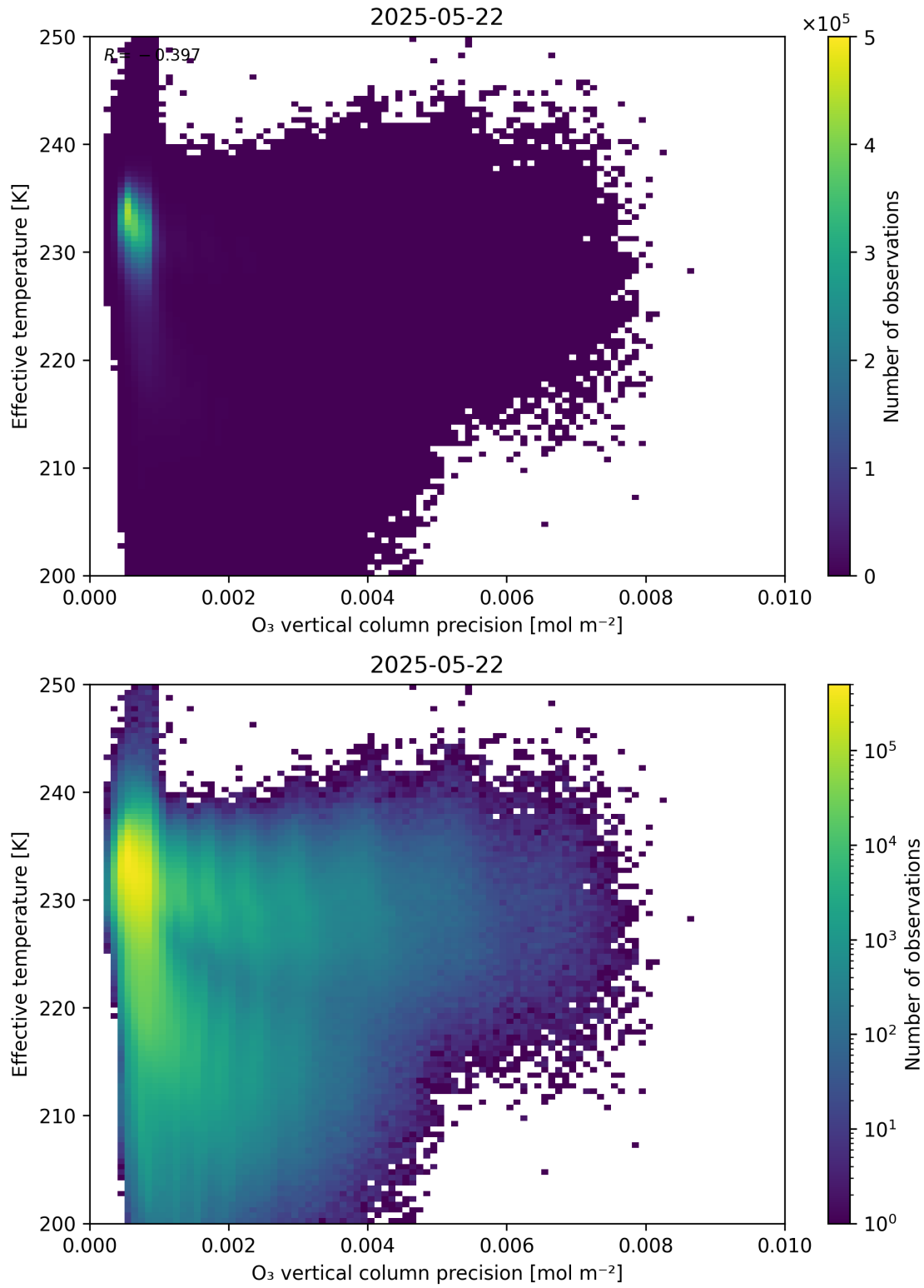
Figure 42: Scatter density plot of “O 3 vertical column precision” against “Effective temperature” for 2025-05-21 to 2025-05-23.
