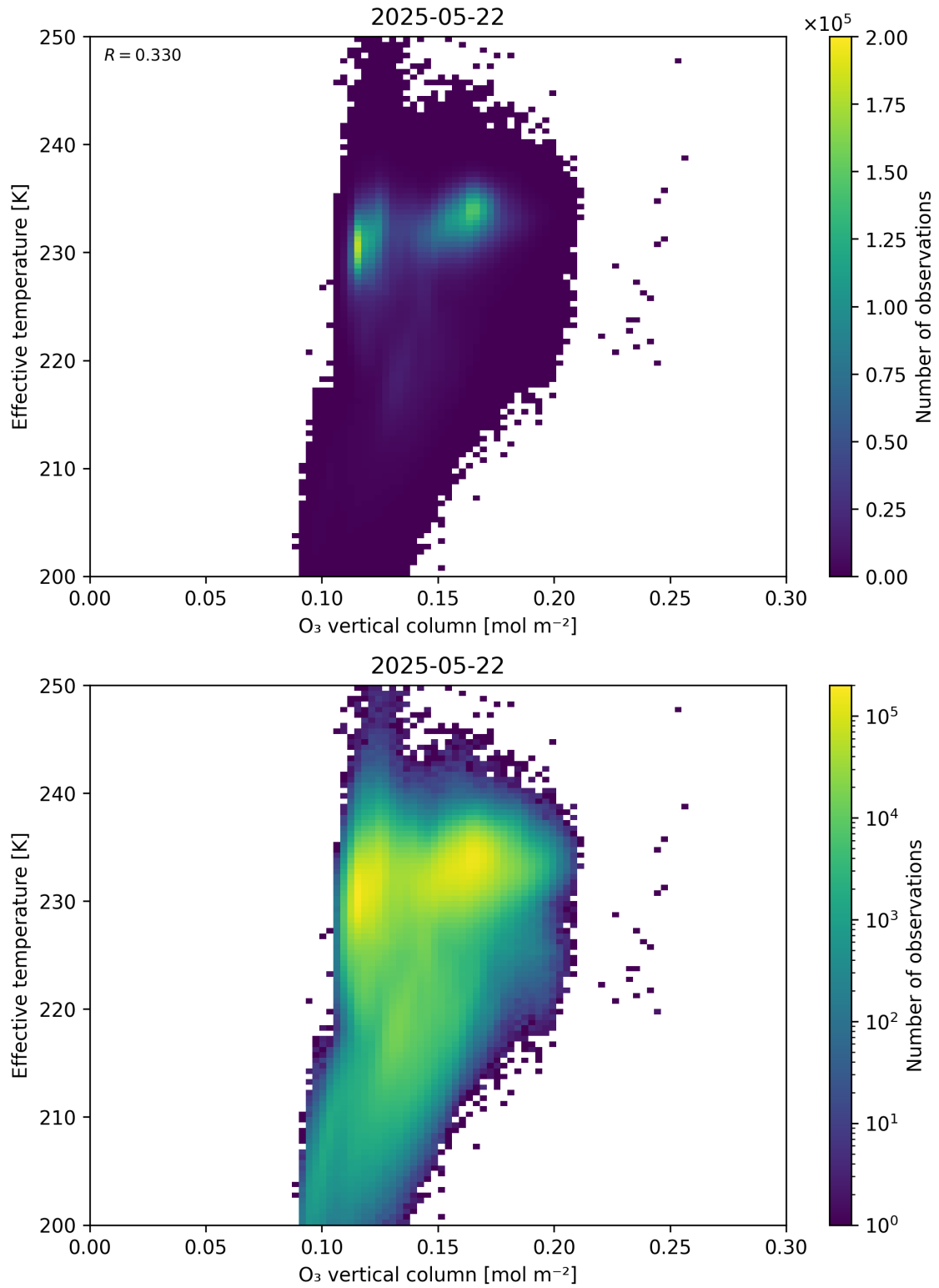
Figure 39: Scatter density plot of “O 3 vertical column” against “Effective temperature” for 2025-05-21 to 2025-05-23.
