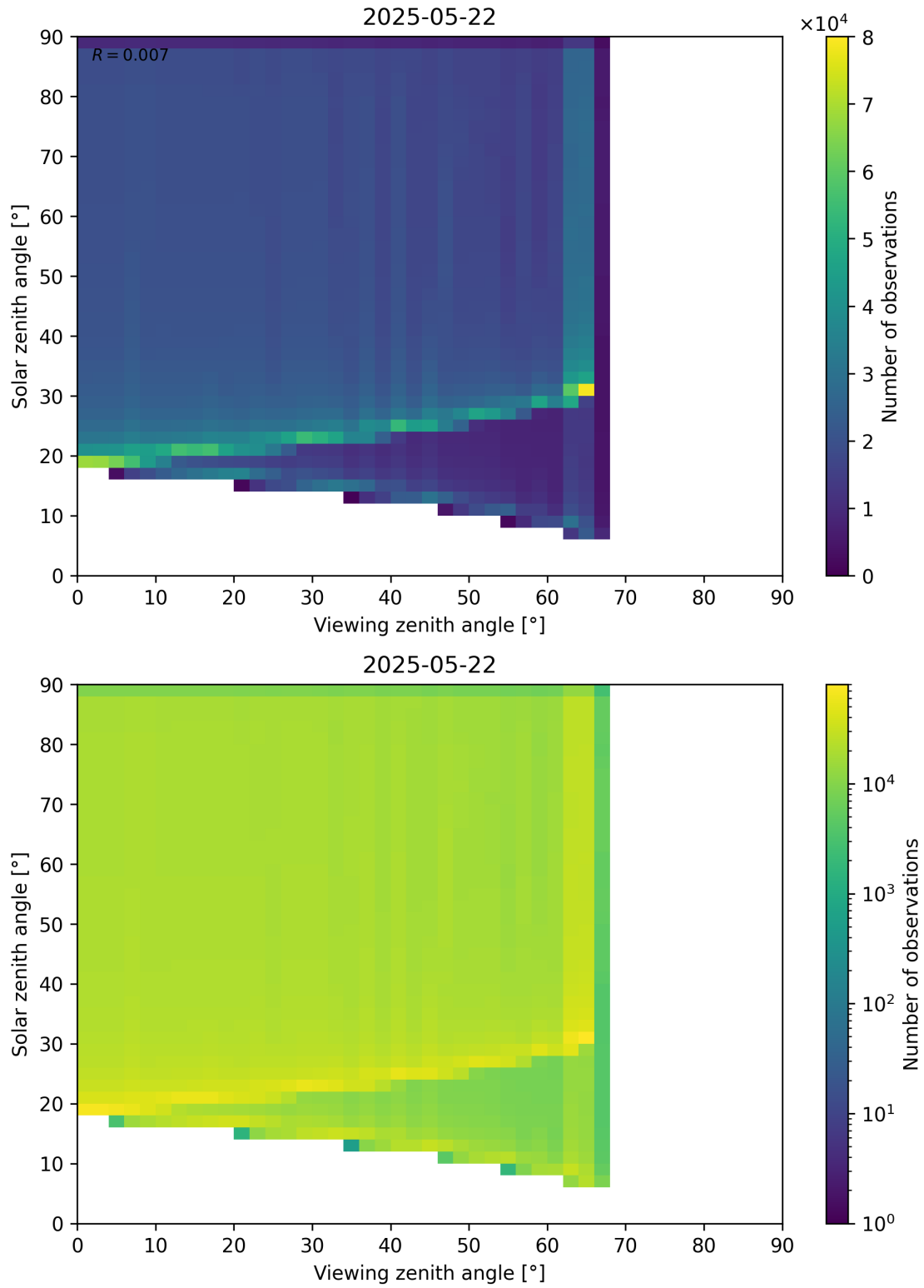
Figure 54: Scatter density plot of “Viewing zenith angle” against “Solar zenith angle” for 2025-05-21 to 2025-05-23.
