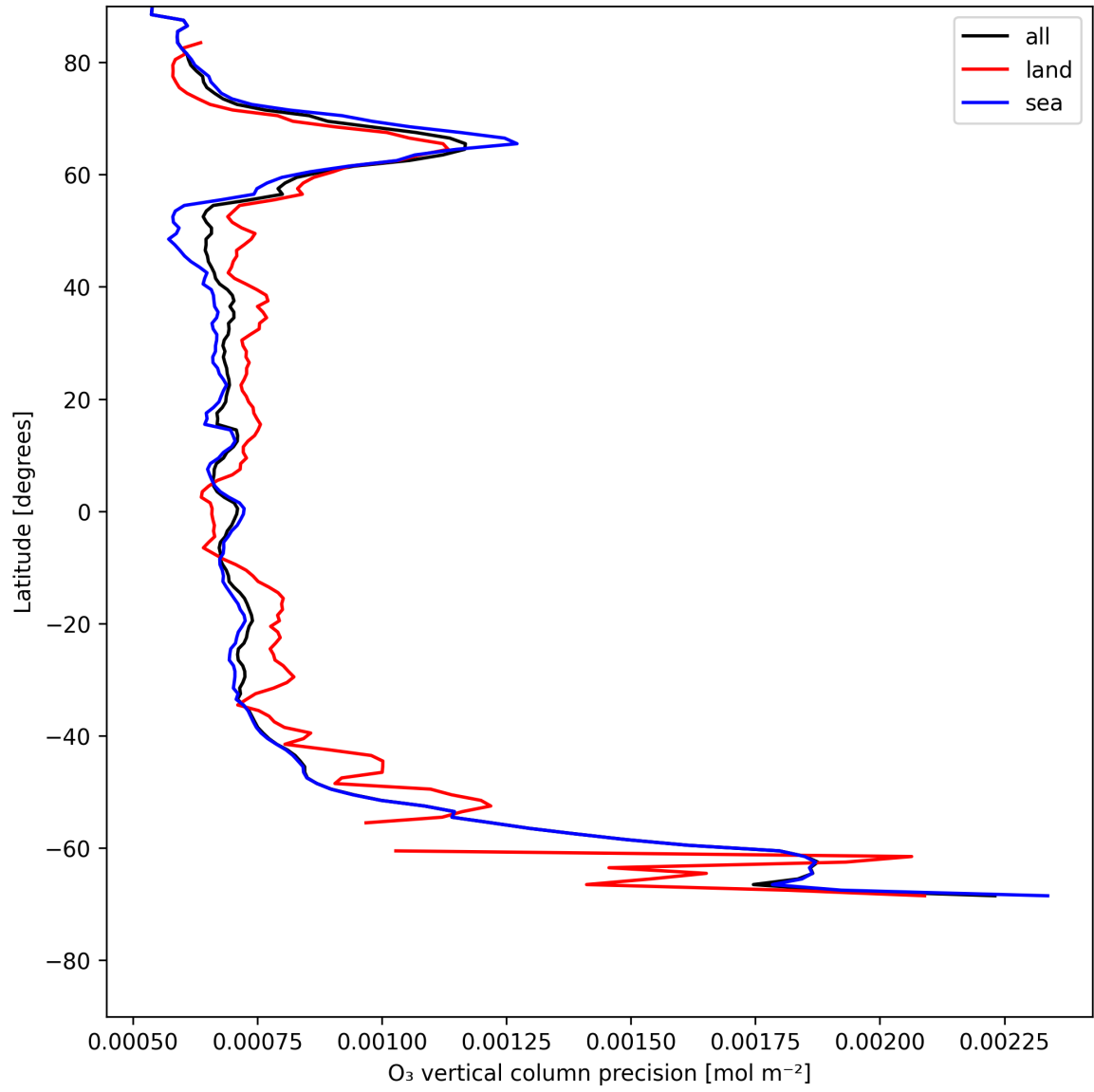
Figure 15: Zonal average of “O 3 vertical column precision” for 2025-05-21 to 2025-05-23.
