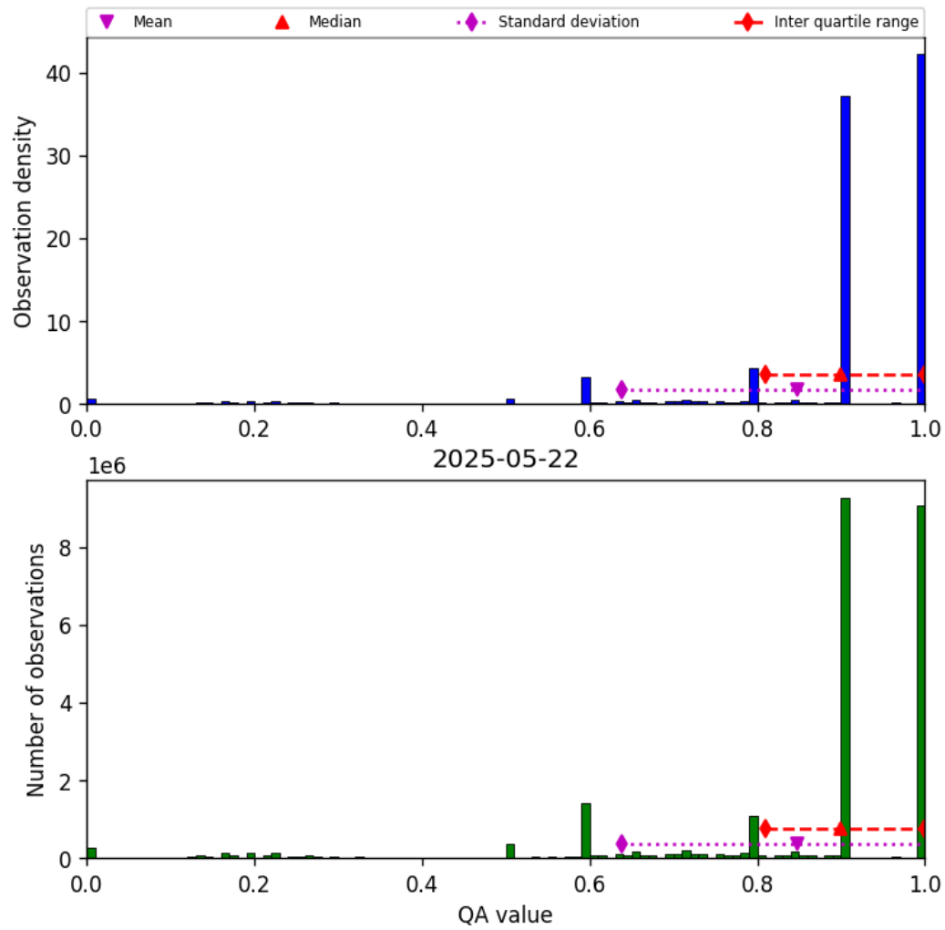
Figure 20: Histogram of “QA value” for 2025-05-21 to 2025-05-23
