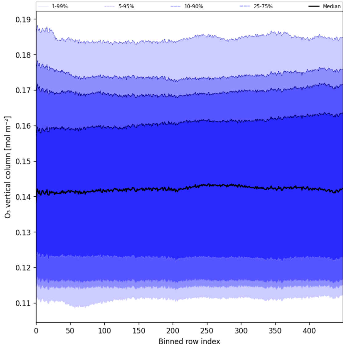
Figure 28: Along track statistics of “O 3 vertical column” for 2025-05-21 to 2025-05-23
