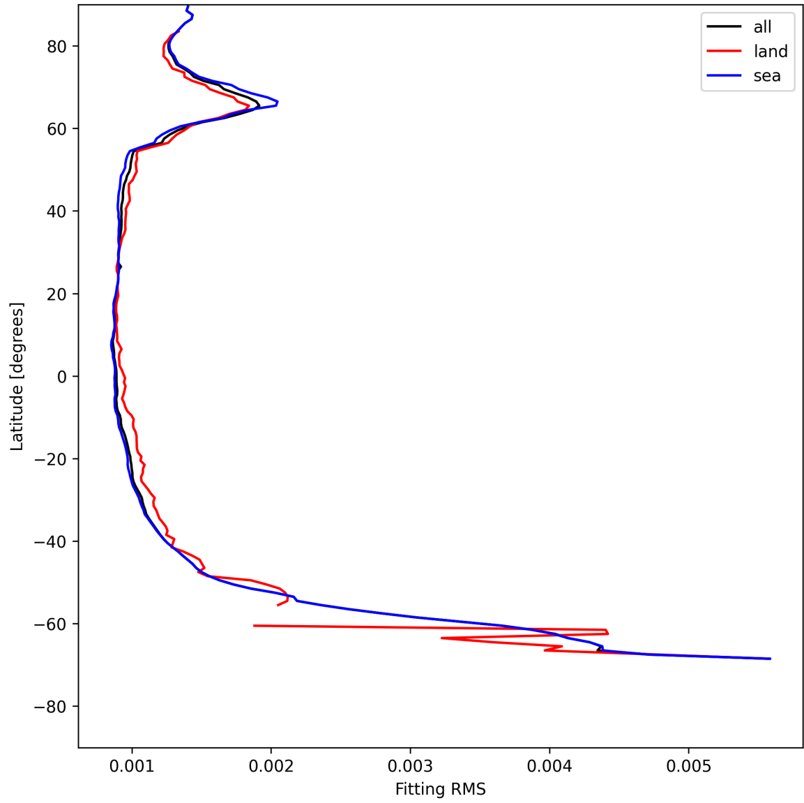
Figure 16: Zonal average of “Fitting RMS” for 2025-05-21 to 2025-05-23.
