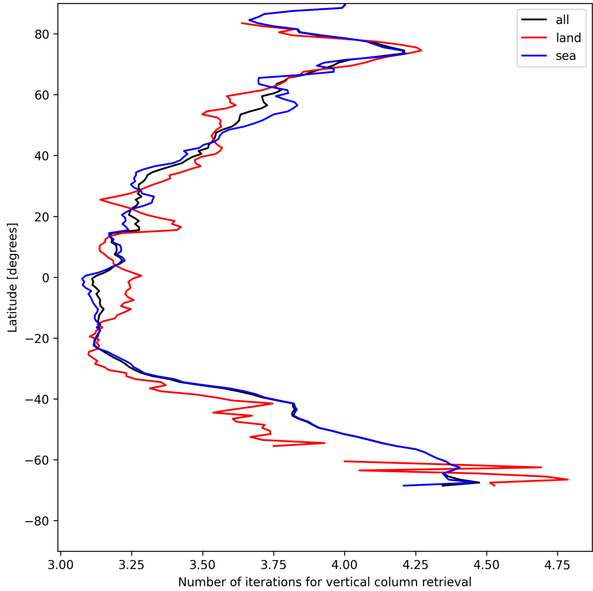
Figure 19: Zonal average of “Number of iterations for vertical column retrieval” for 2025-05-21 to 2025-05-23.
