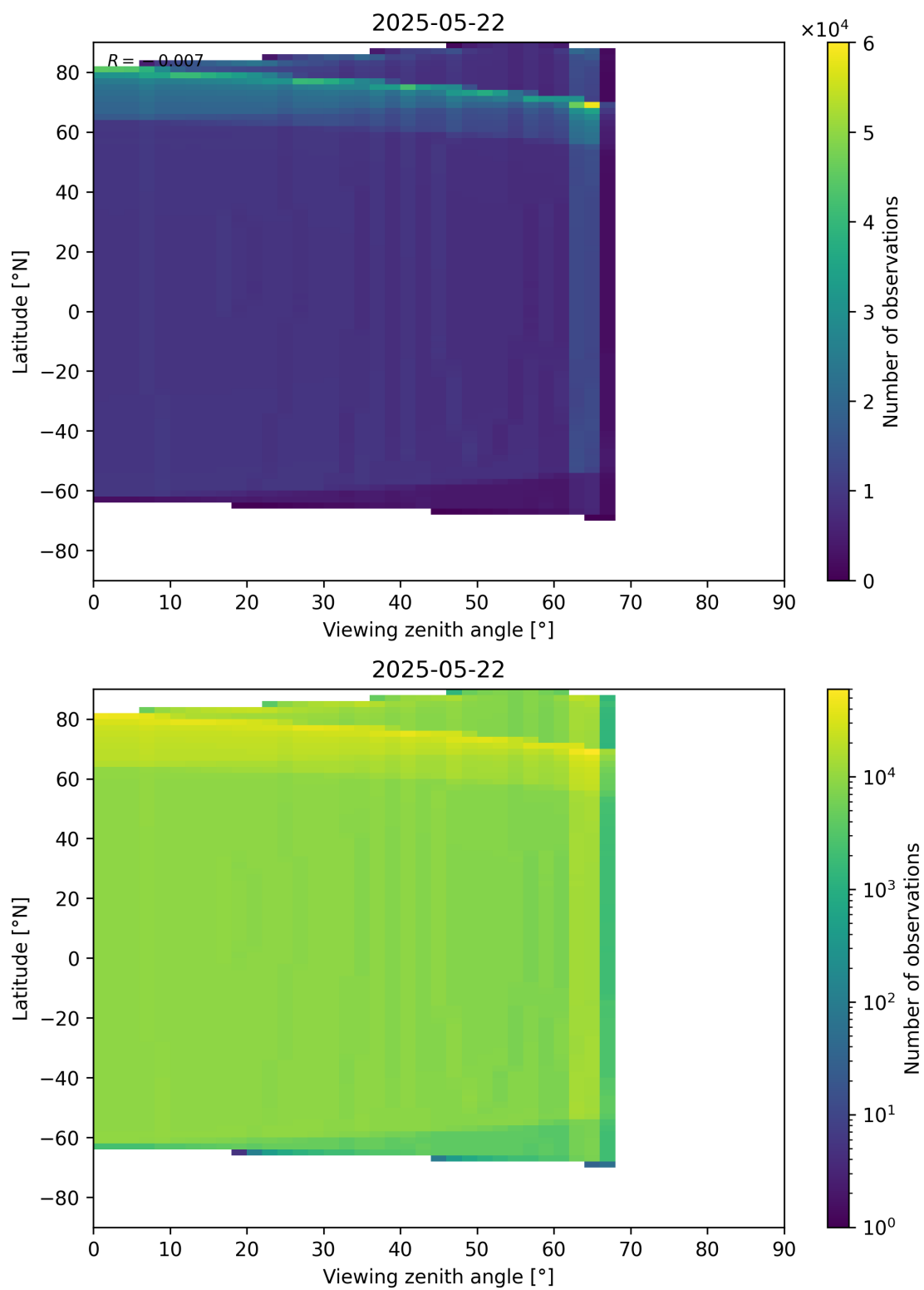
Figure 49: Scatter density plot of “Viewing zenith angle” against “Latitude” for 2025-05-21 to 2025-05-23.
