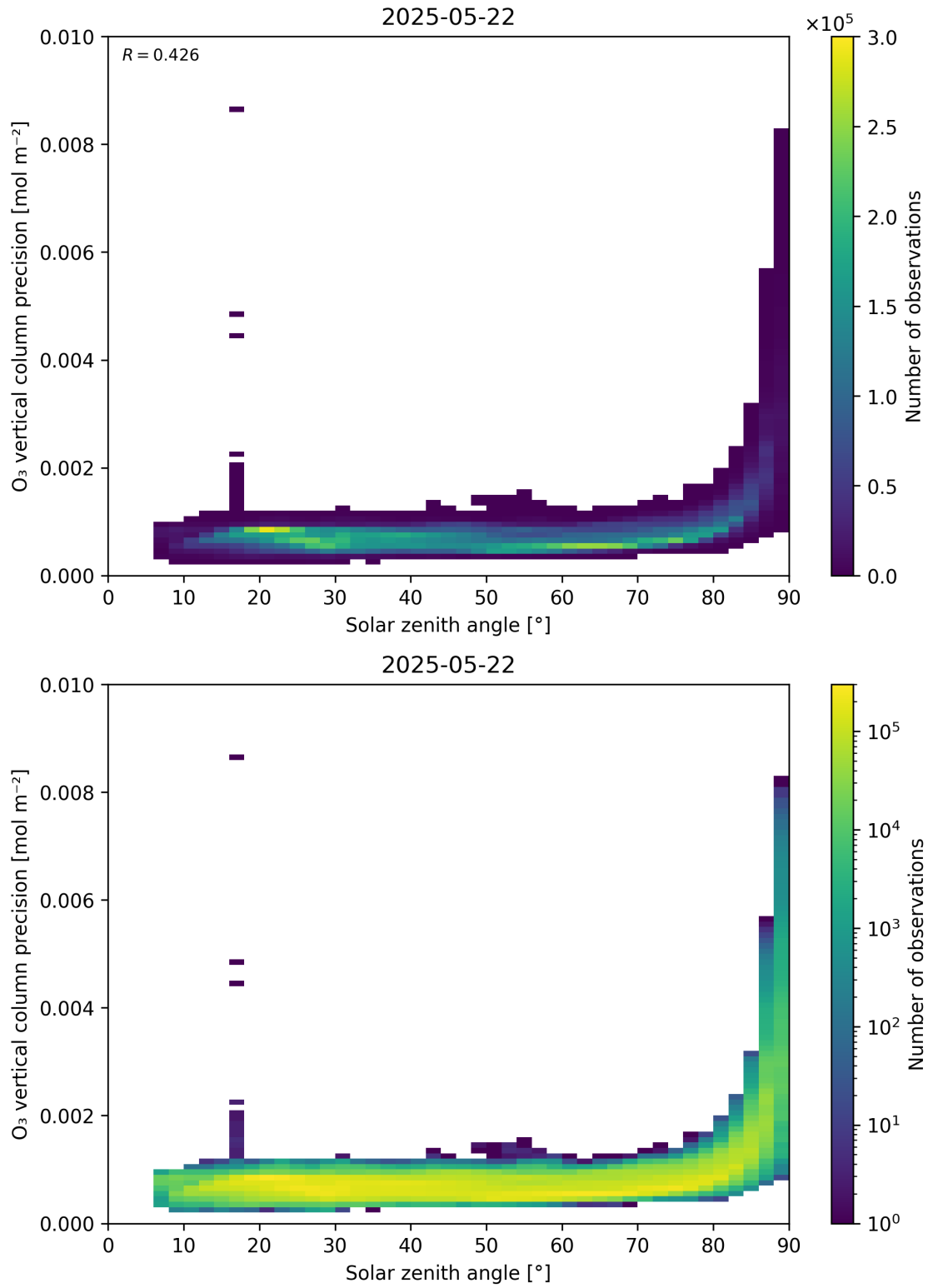
Figure 48: Scatter density plot of “Solar zenith angle” against “O 3 vertical column precision” for 2025-05-21 to 2025-05-23.
