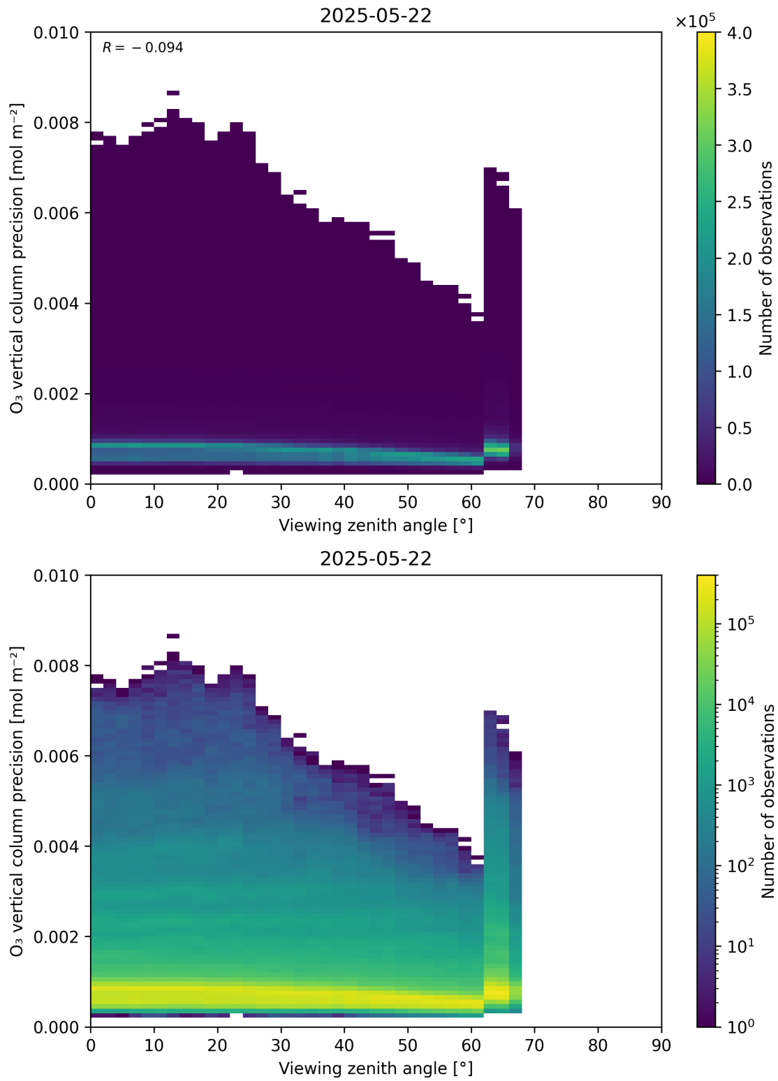
Figure 53: Scatter density plot of “Viewing zenith angle” against “O 3 vertical column precision” for 2025-05-21 to 2025-05-23.
