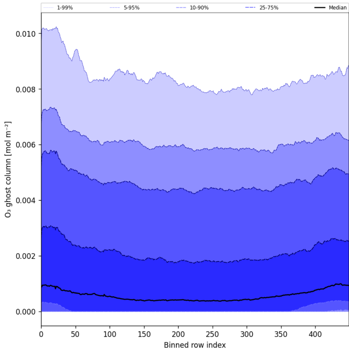
Figure 32: Along track statistics of “O 3 ghost column” for 2025-05-21 to 2025-05-23
