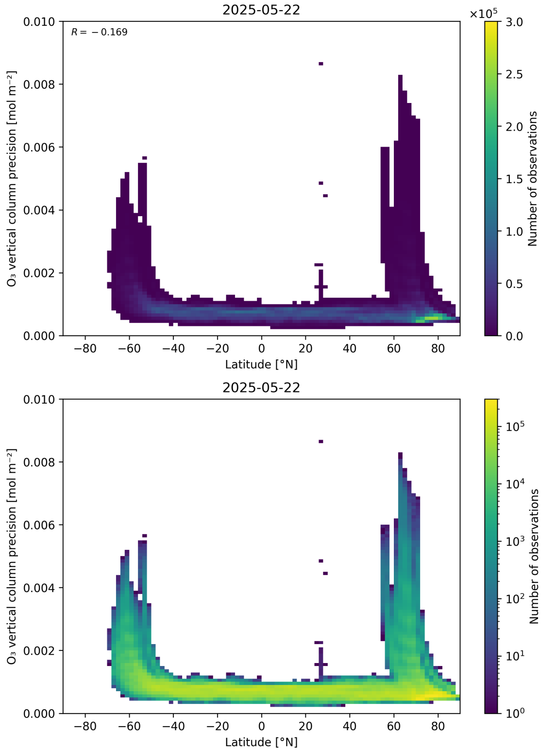
Figure 37: Scatter density plot of “Latitude” against “O 3 vertical column precision” for 2025-05-21 to 2025-05-23.
