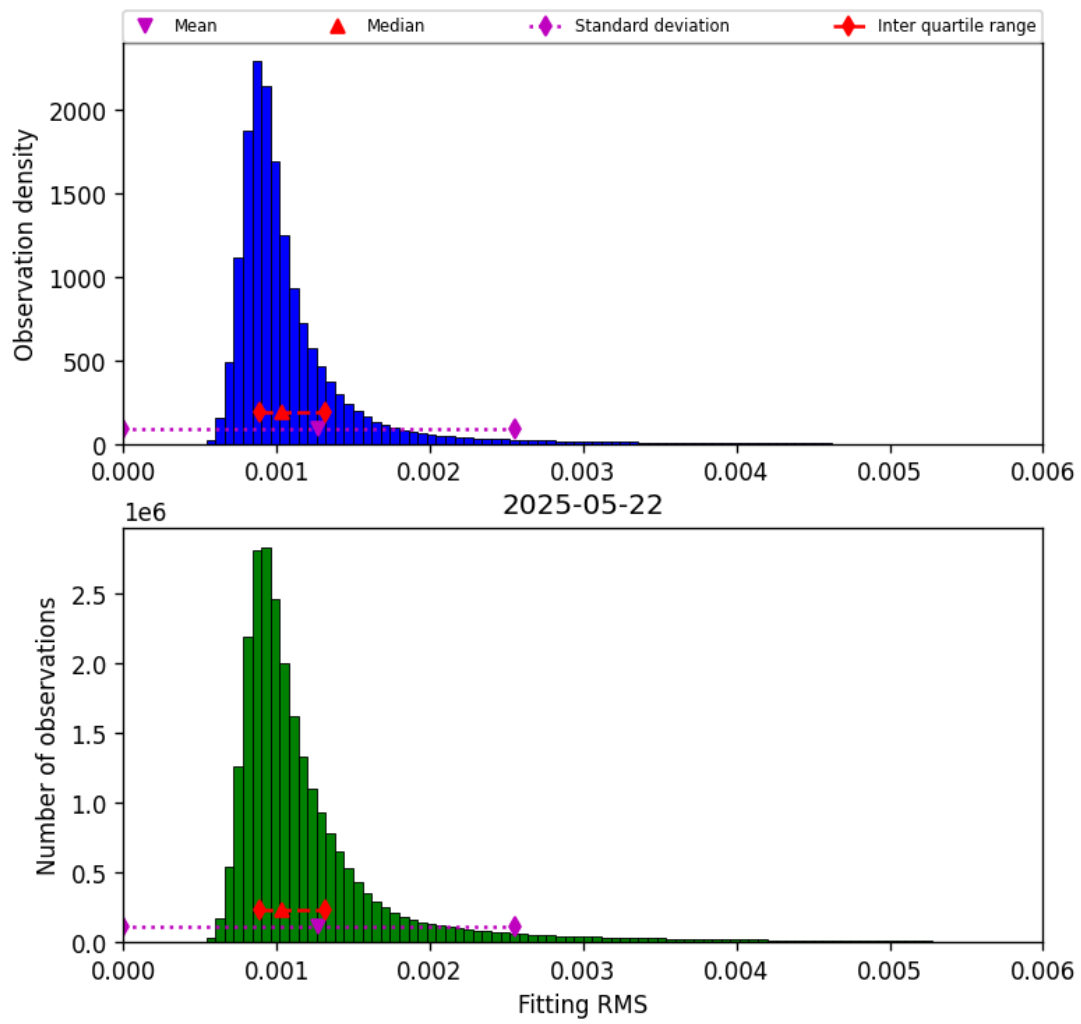
Figure 23: Histogram of “Fitting RMS” for 2025-05-21 to 2025-05-23
