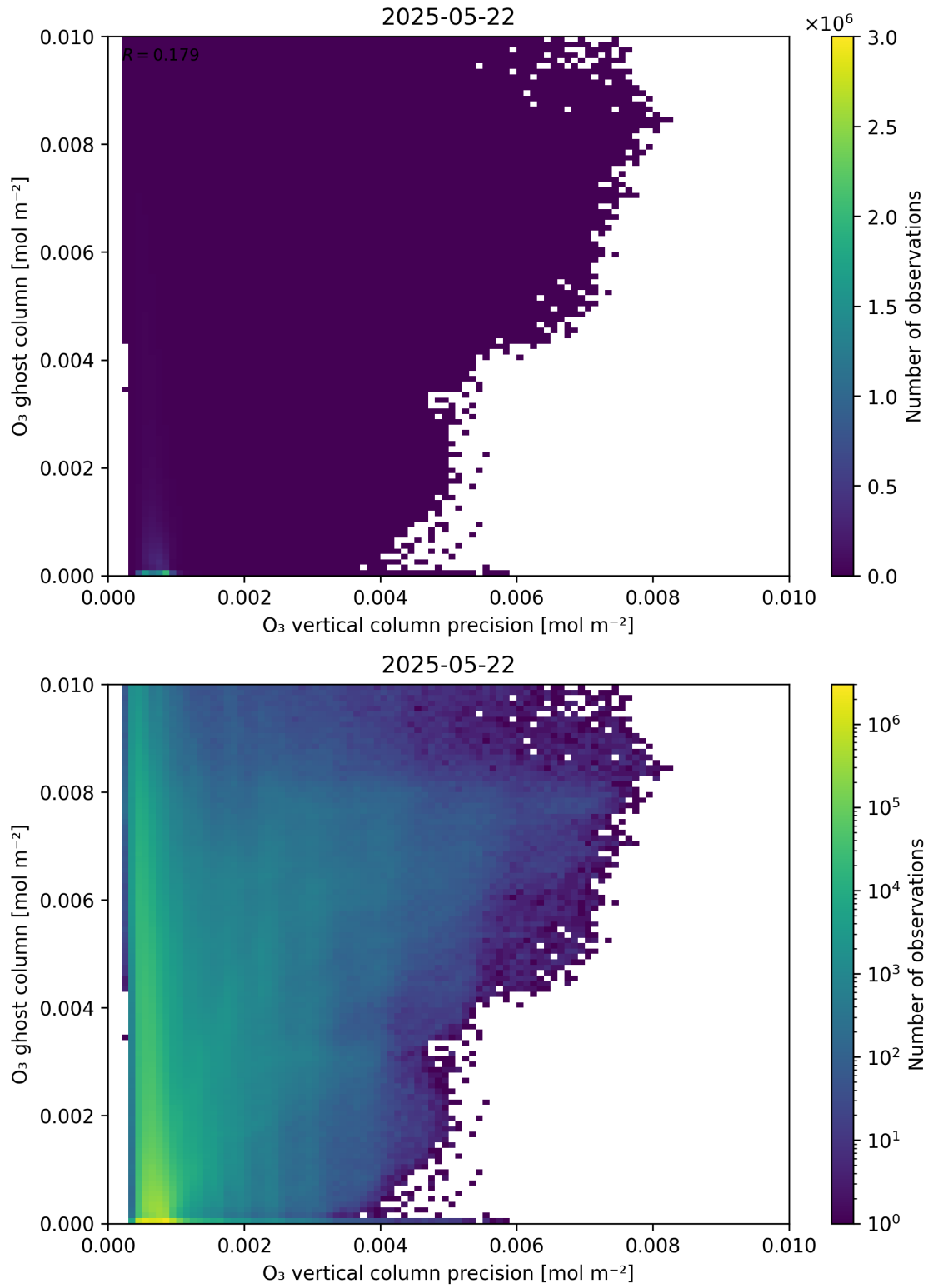
Figure 43: Scatter density plot of “ O_3 vertical column precision” against “ O_3 ghost column” for 2025-05-21 to 2025-05-23.
