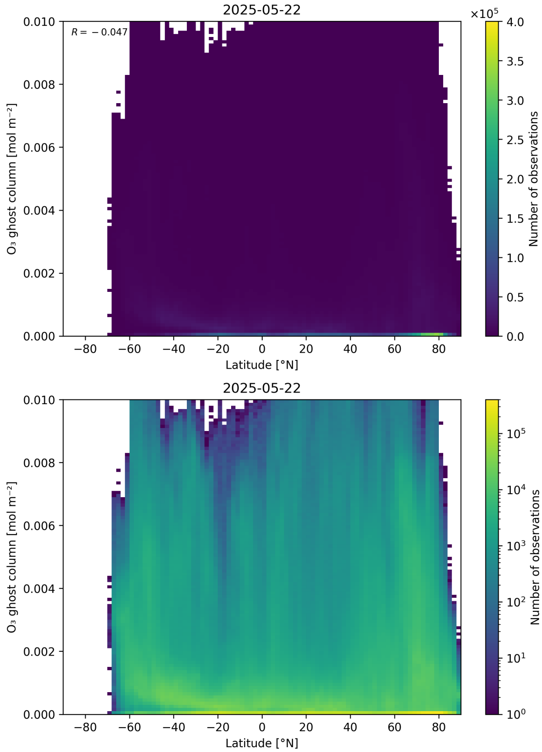
Figure 35: Scatter density plot of “Latitude” against “O 3 ghost column” for 2025-05-21 to 2025-05-23.
