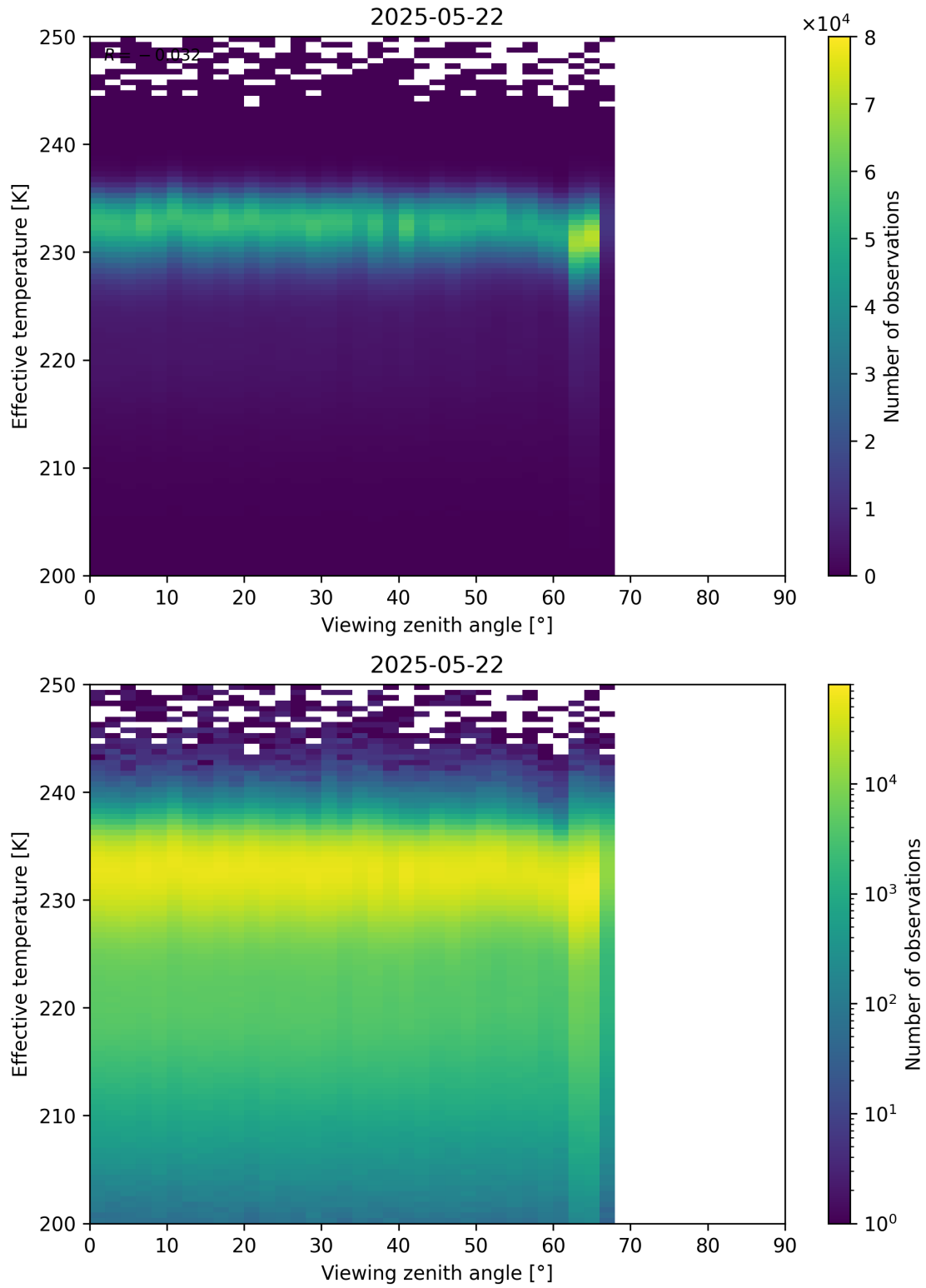
Figure 50: Scatter density plot of “Viewing zenith angle” against “Effective temperature” for 2025-05-21 to 2025-05-23.
