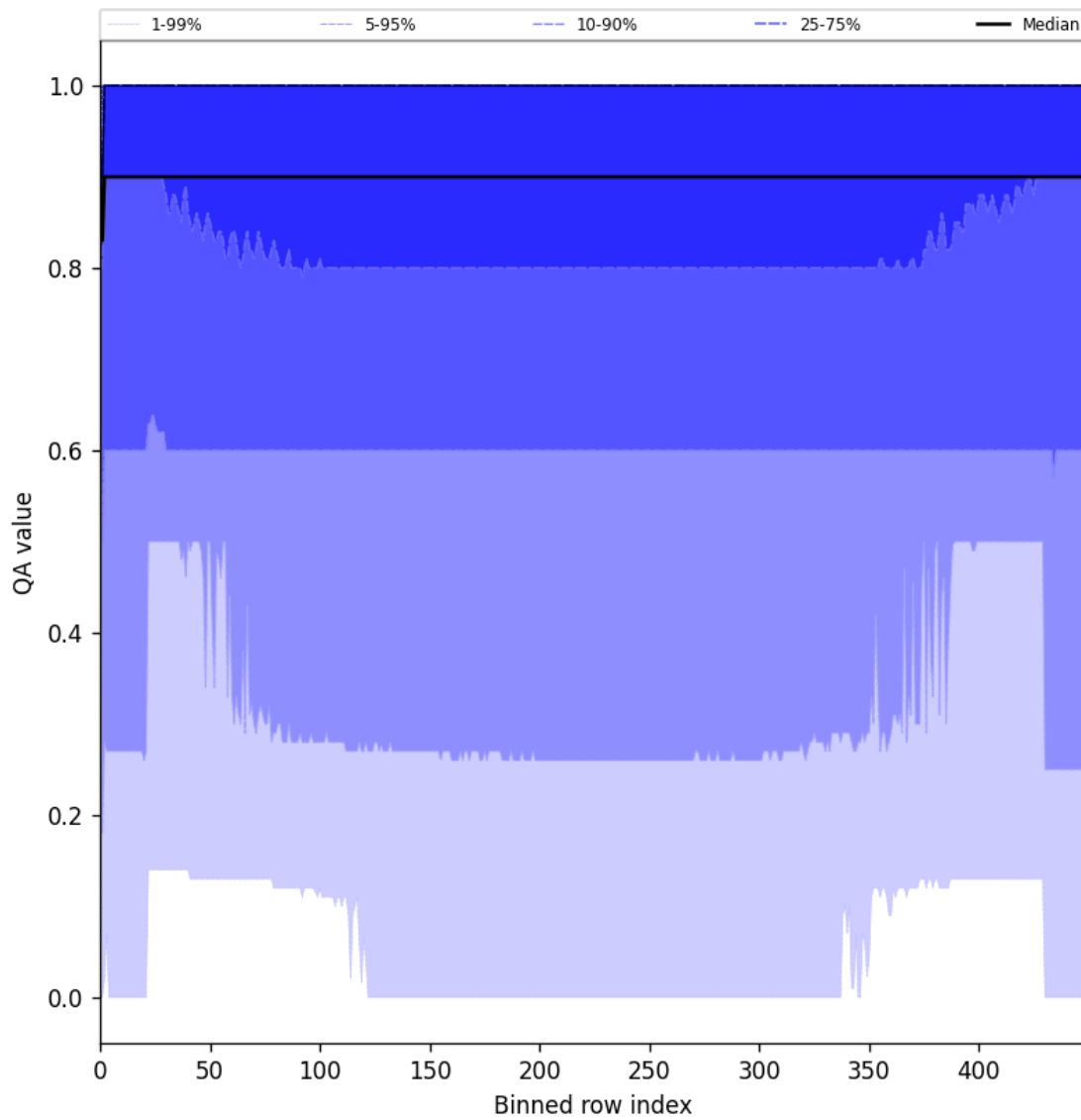
Figure 27: Along track statistics of “QA value” for 2025-05-21 to 2025-05-23
