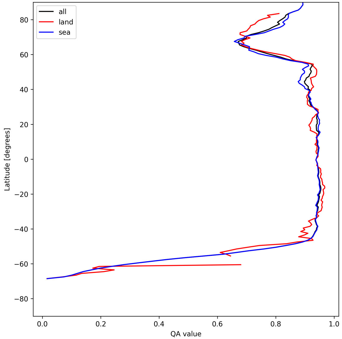
Figure 13: Zonal average of “QA value” for 2025-05-21 to 2025-05-23.
