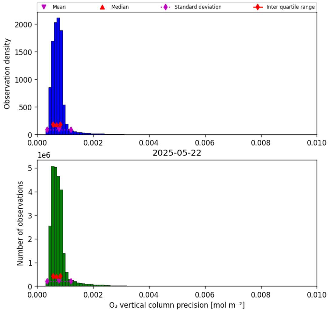
Figure 22: Histogram of “O 3 vertical column precision” for 2025-05-21 to 2025-05-23
