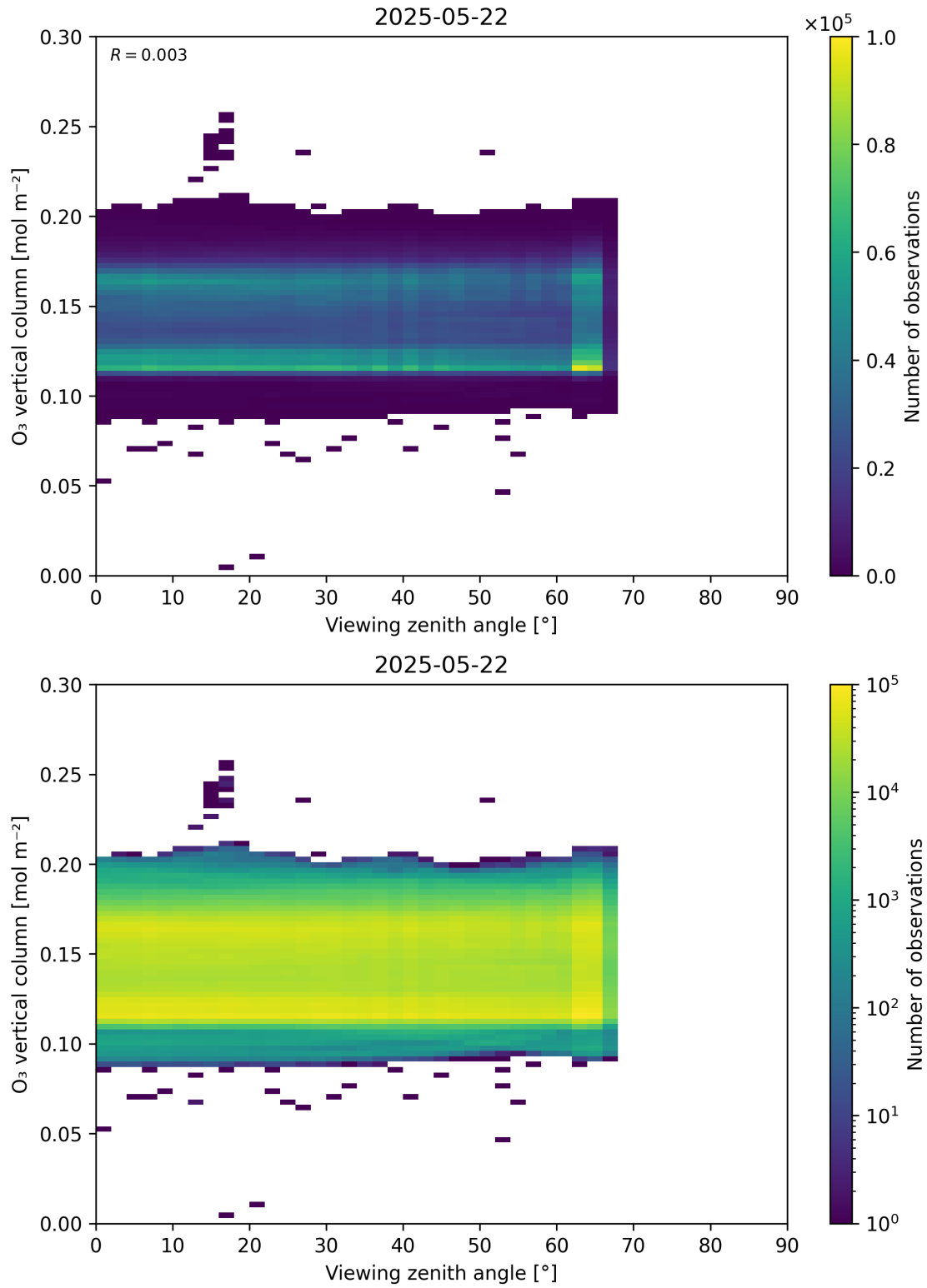
Figure 52: Scatter density plot of “Viewing zenith angle” against “O 3 vertical column” for 2025-05-21 to 2025-05-23.
