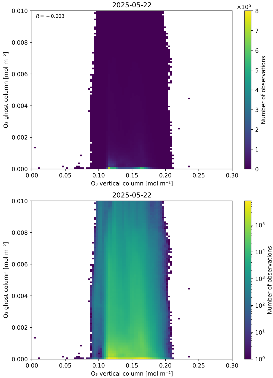
Figure 40: Scatter density plot of “O 3 vertical column” against “O 3 ghost column” for 2025-05-21 to 2025-05-23.
