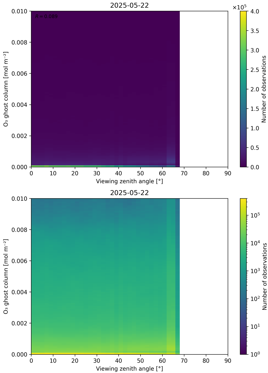
Figure 51: Scatter density plot of “Viewing zenith angle” against “O 3 ghost column” for 2025-05-21 to 2025-05-23.
