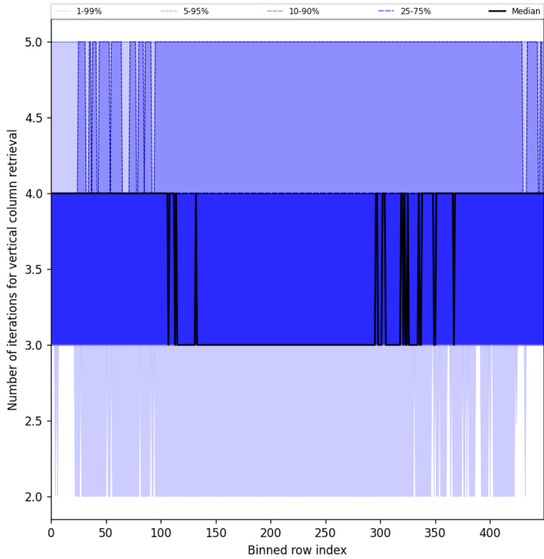
Figure 33: Along track statistics of “Number of iterations for vertical column retrieval” for 2025-05-21 to 2025-05-23
