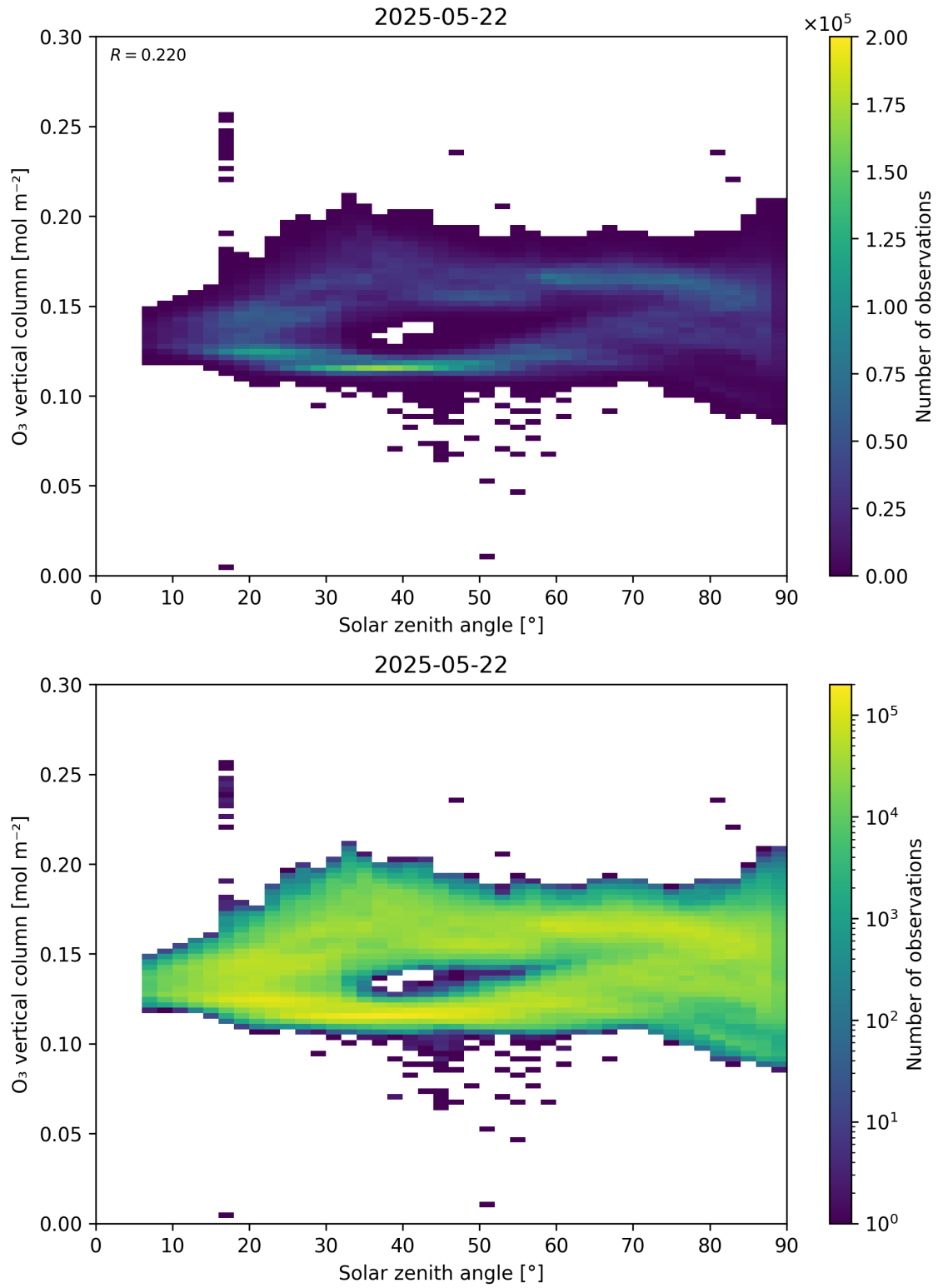
Figure 47: Scatter density plot of “Solar zenith angle” against “O 3 vertical column” for 2025-05-21 to 2025-05-23.
