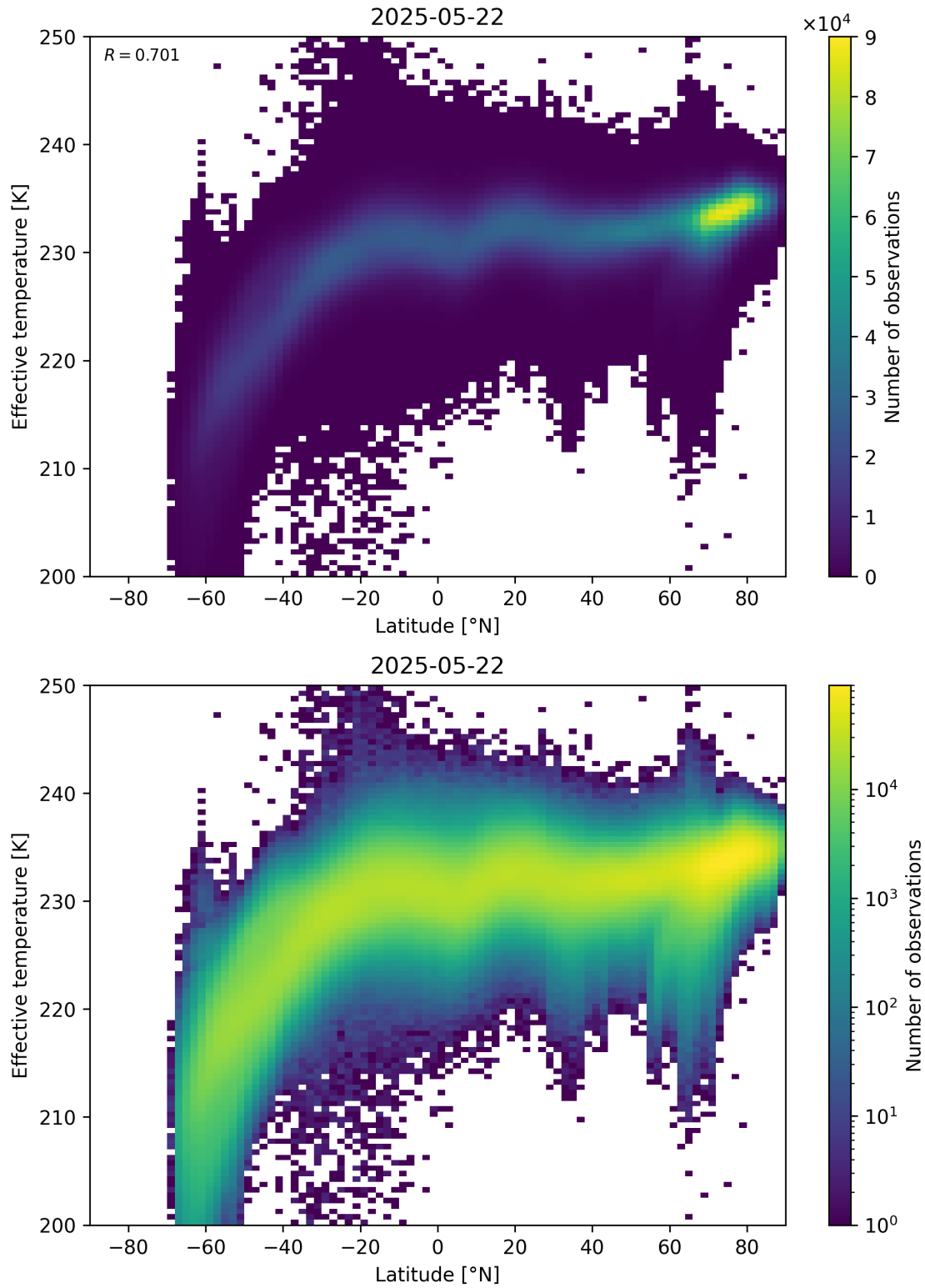
Figure 34: Scatter density plot of “Latitude” against “Effective temperature” for 2025-05-21 to 2025-05-23.
