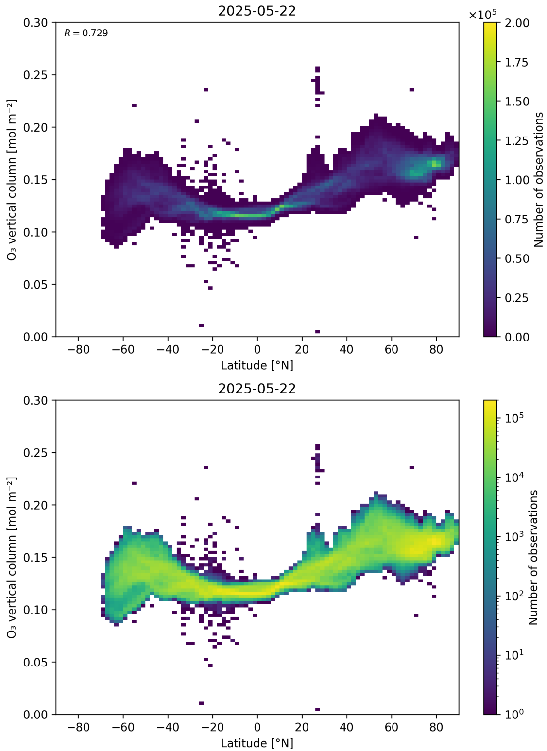
Figure 36: Scatter density plot of “Latitude” against “O 3 vertical column” for 2025-05-21 to 2025-05-23.
