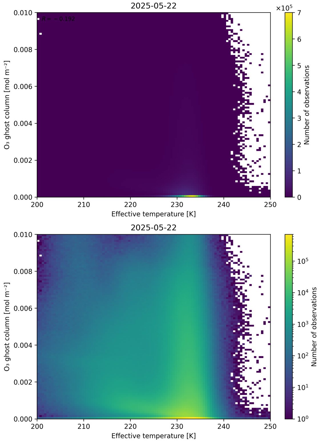
Figure 38: Scatter density plot of “Effective temperature” against “O 3 ghost column” for 2025-05-21 to 2025-05-23.
