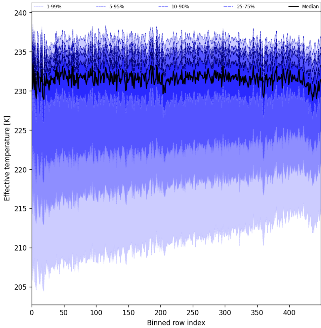
Figure 31: Along track statistics of “Effective temperature” for 2025-05-21 to 2025-05-23
