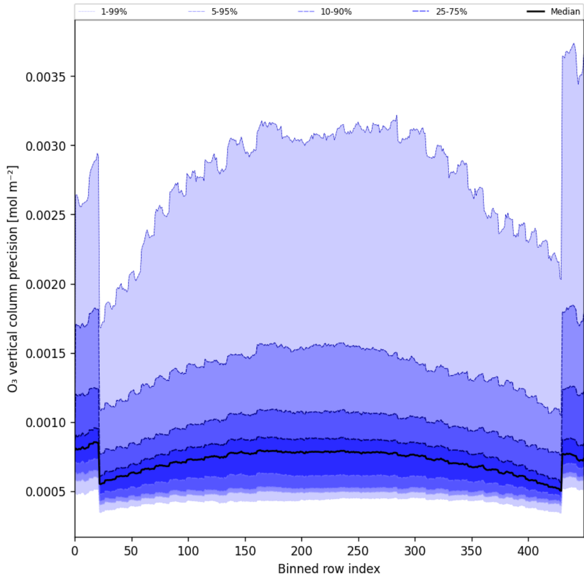
Figure 29: Along track statistics of “O 3 vertical column precision” for 2025-05-21 to 2025-05-23
