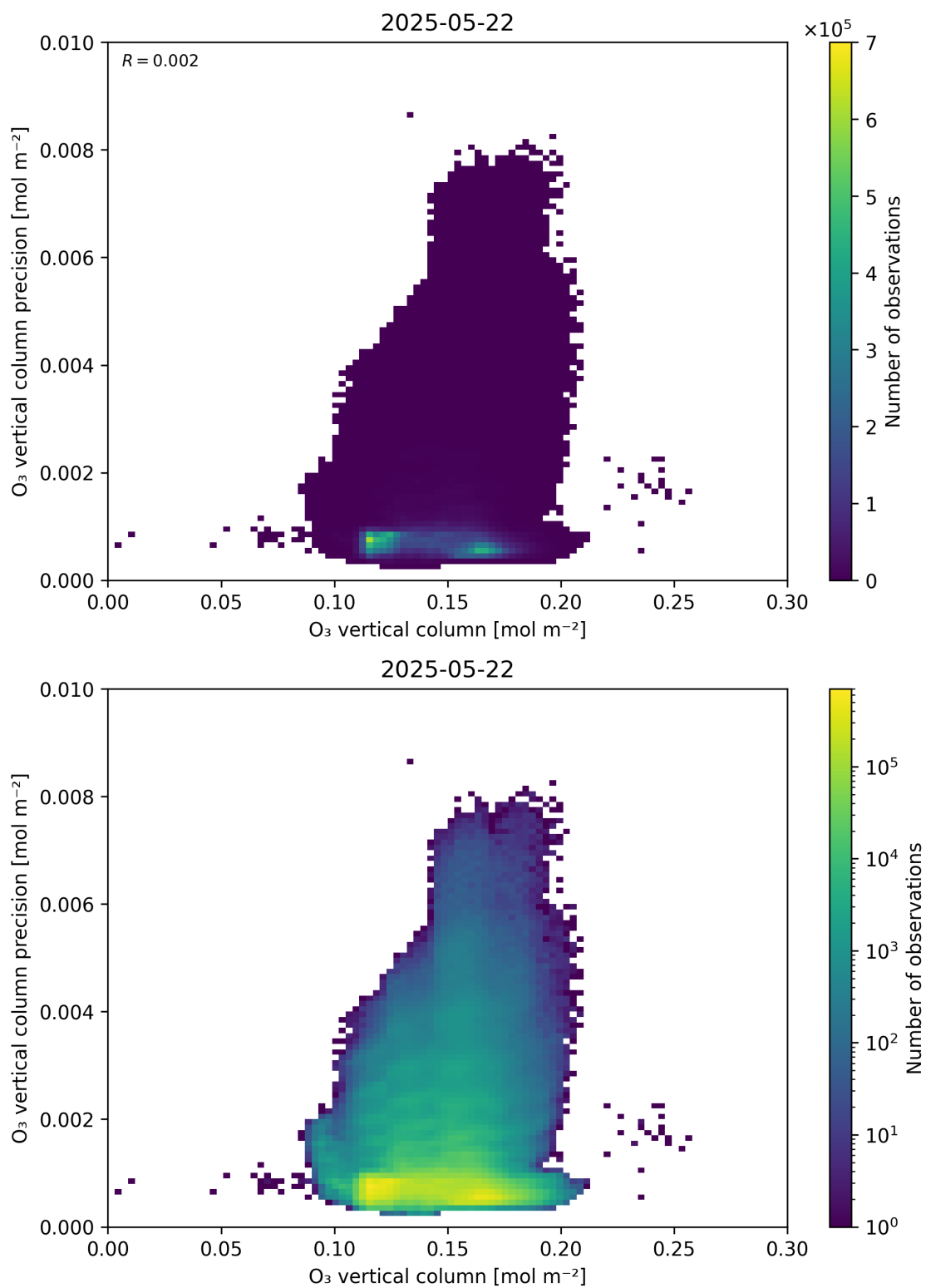
Figure 41: Scatter density plot of “O 3 vertical column” against “O 3 vertical column precision” for 2025-05-21 to 2025-05-23.
