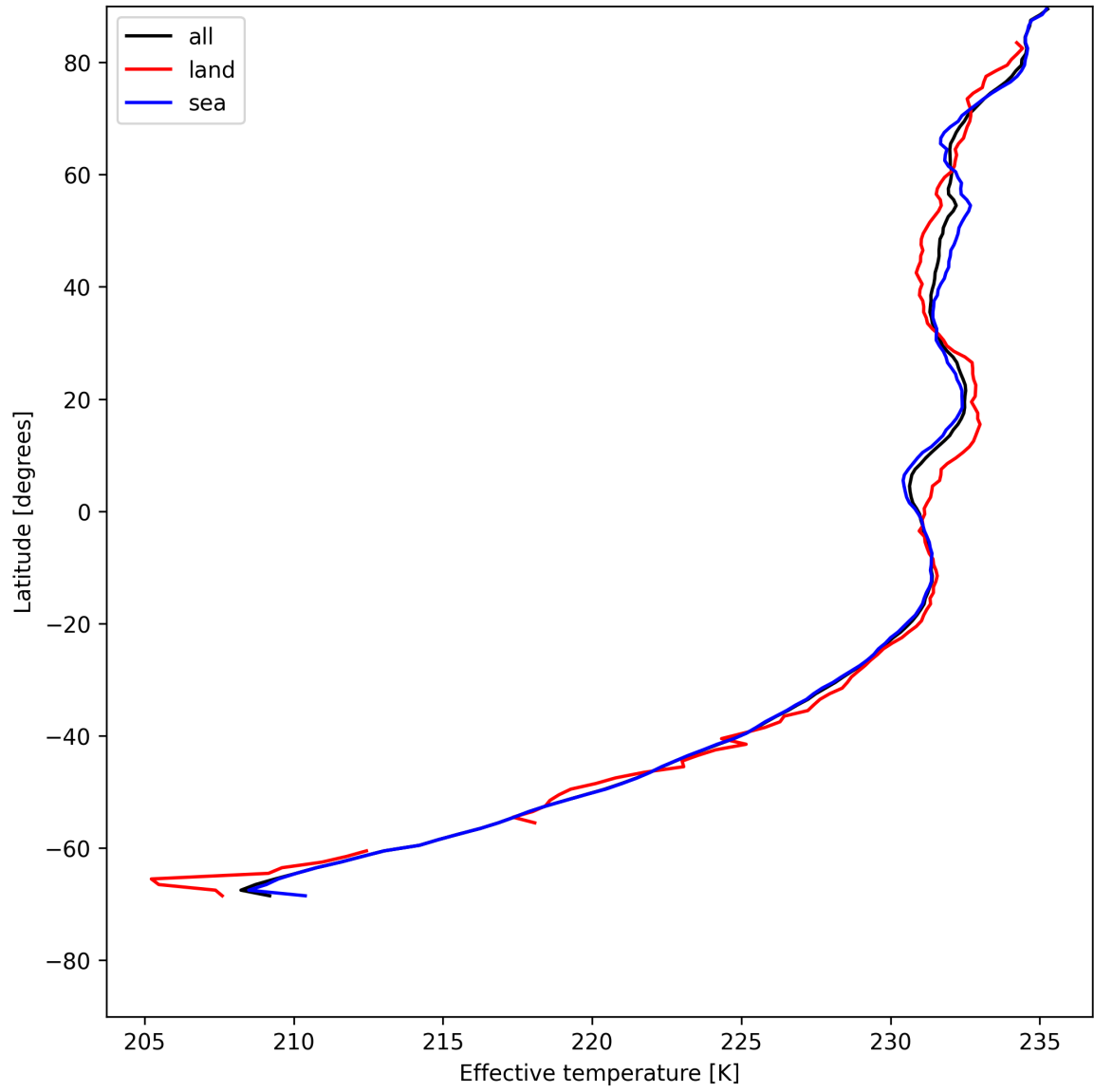
Figure 17: Zonal average of "Effective temperature" for 2025-05-21 to 2025-05-23.
