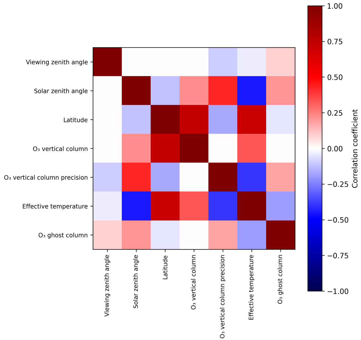
Figure 2: Map of correlation matrix for 2025-05-21 to 2025-05-23.
