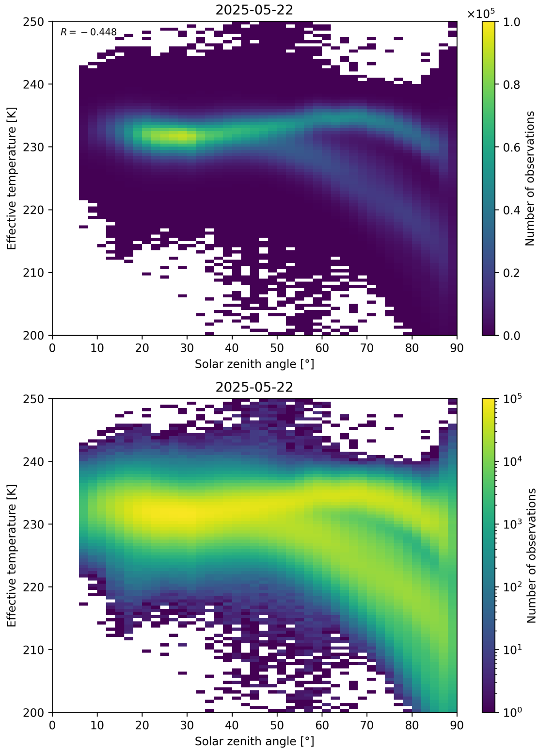
Figure 45: Scatter density plot of “Solar zenith angle” against “Effective temperature” for 2025-05-21 to 2025-05-23.
