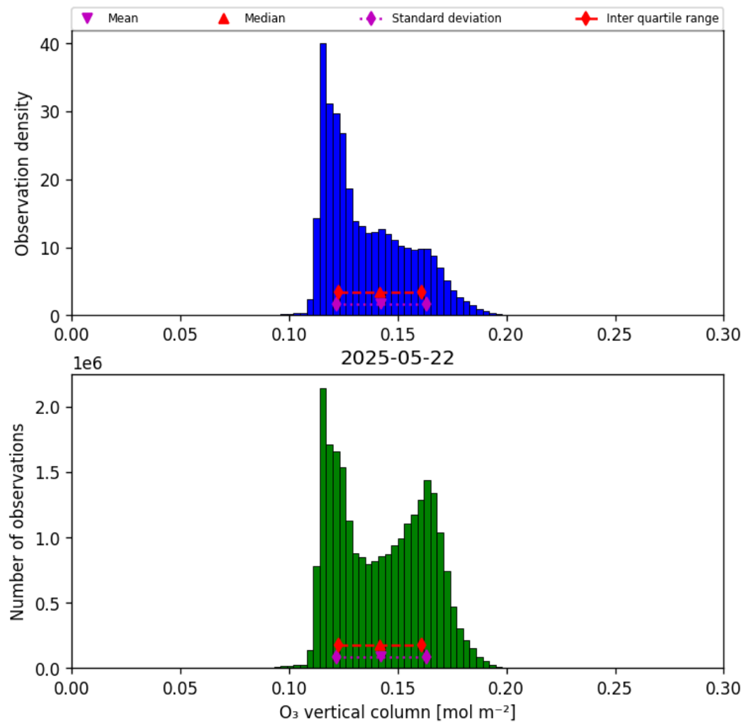
Figure 21: Histogram of “O 3 vertical column” for 2025-05-21 to 2025-05-23
