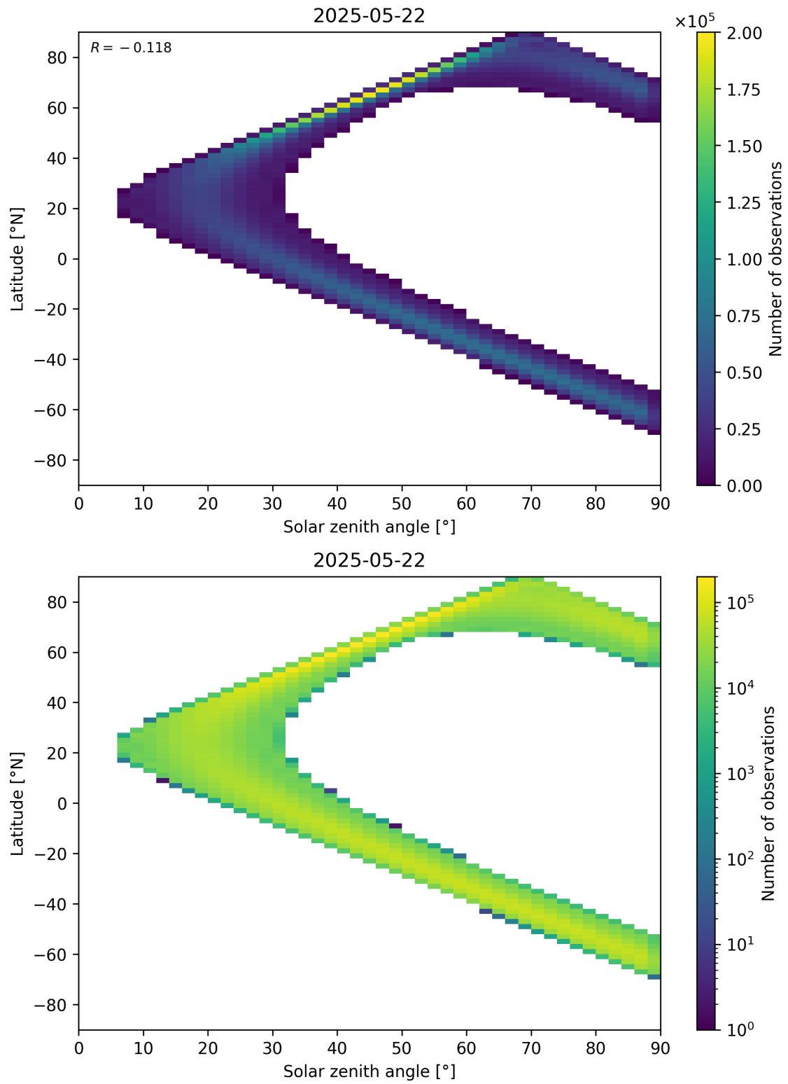
Figure 44: Scatter density plot of “Solar zenith angle” against “Latitude” for 2025-05-21 to 2025-05-23.
