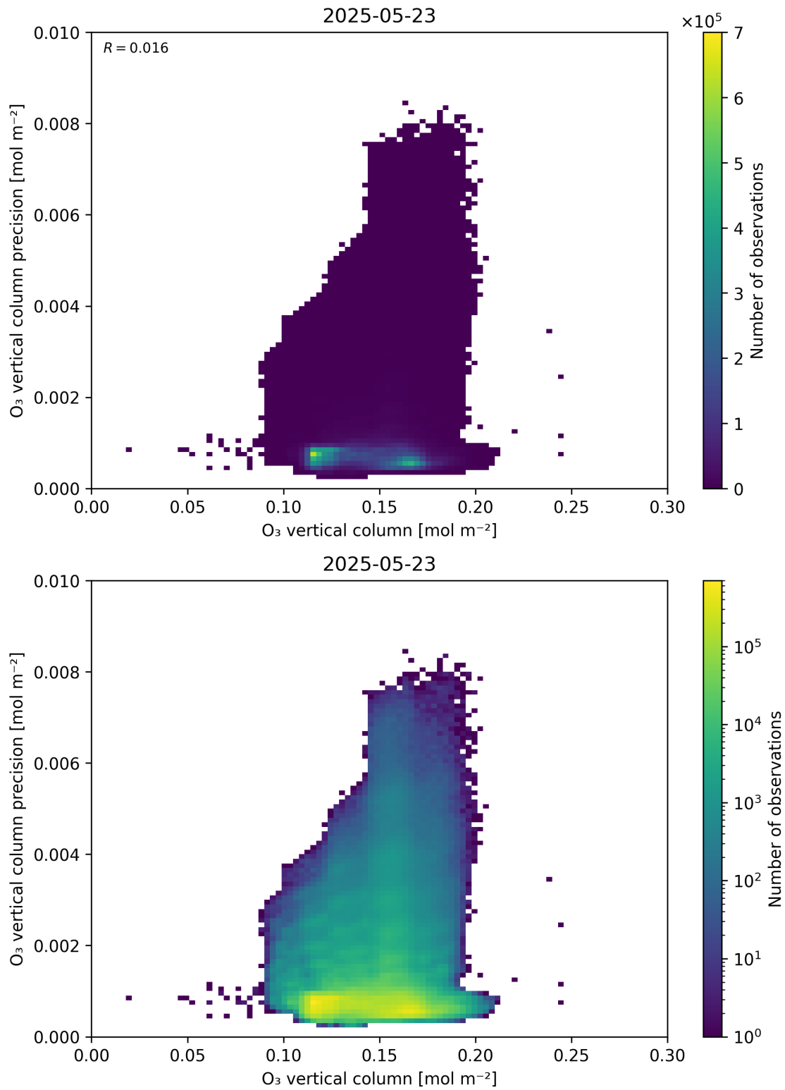
Figure 41: Scatter density plot of “O 3 vertical column” against “O 3 vertical column precision” for 2025-05-22 to 2025-05-24.
