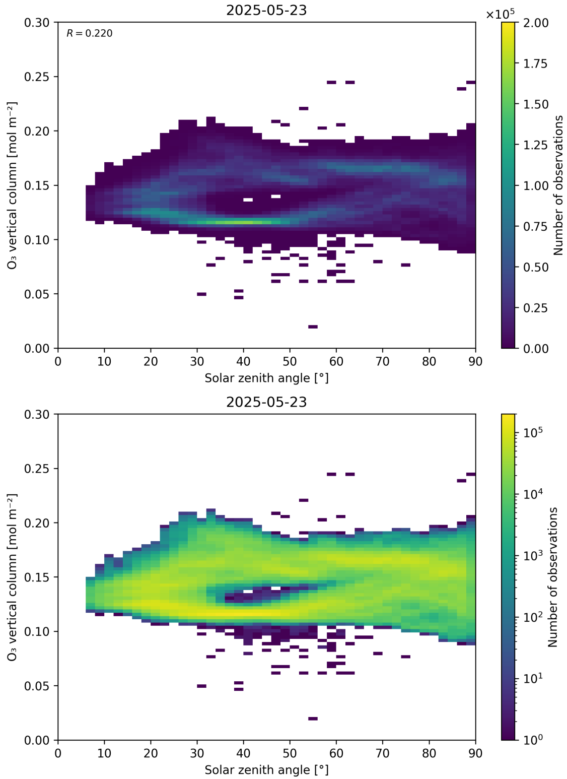
Figure 47: Scatter density plot of “Solar zenith angle” against “O 3 vertical column” for 2025-05-22 to 2025-05-24.
