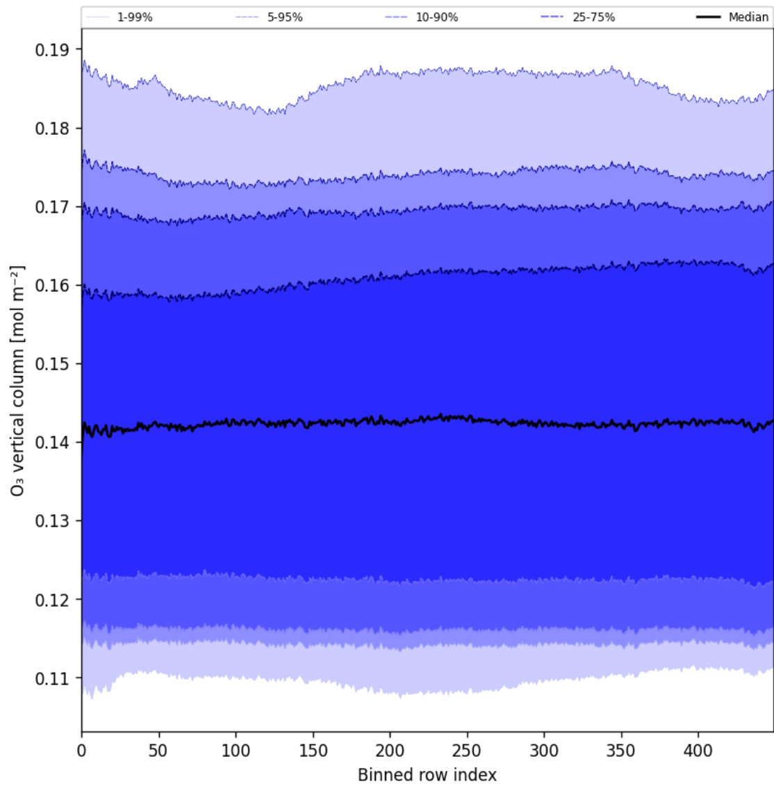
Figure 28: Along track statistics of “O 3 vertical column” for 2025-05-22 to 2025-05-24
