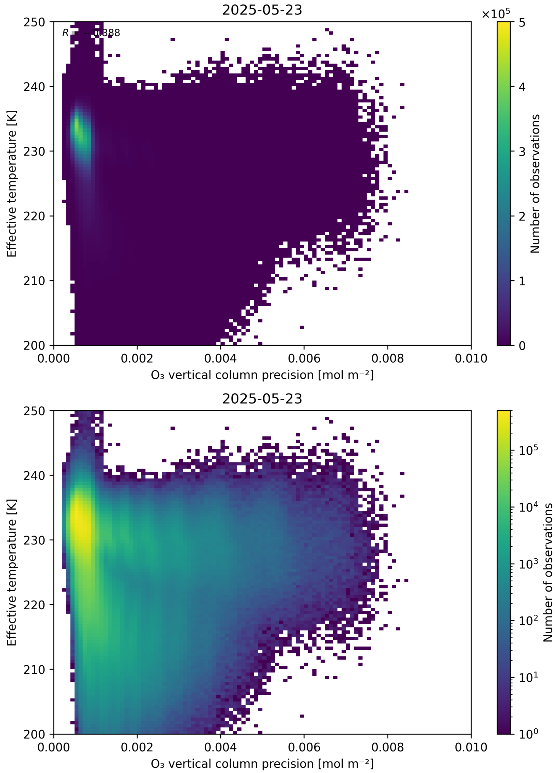
Figure 42: Scatter density plot of “O 3 vertical column precision” against “Effective temperature” for 2025-05-22 to 2025-05-24.
