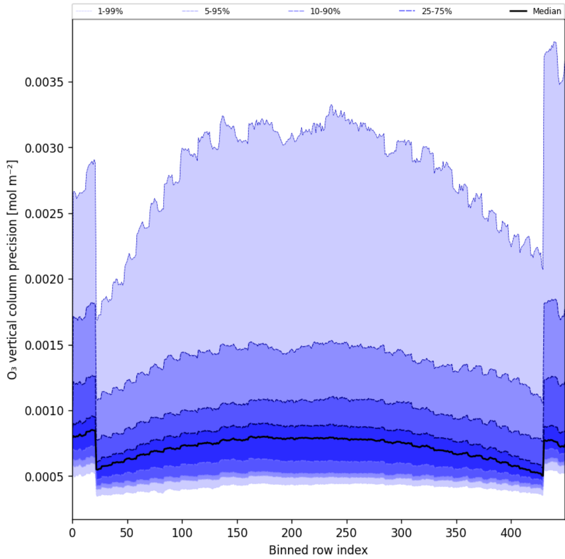
Figure 29: Along track statistics of “O 3 vertical column precision” for 2025-05-22 to 2025-05-24
