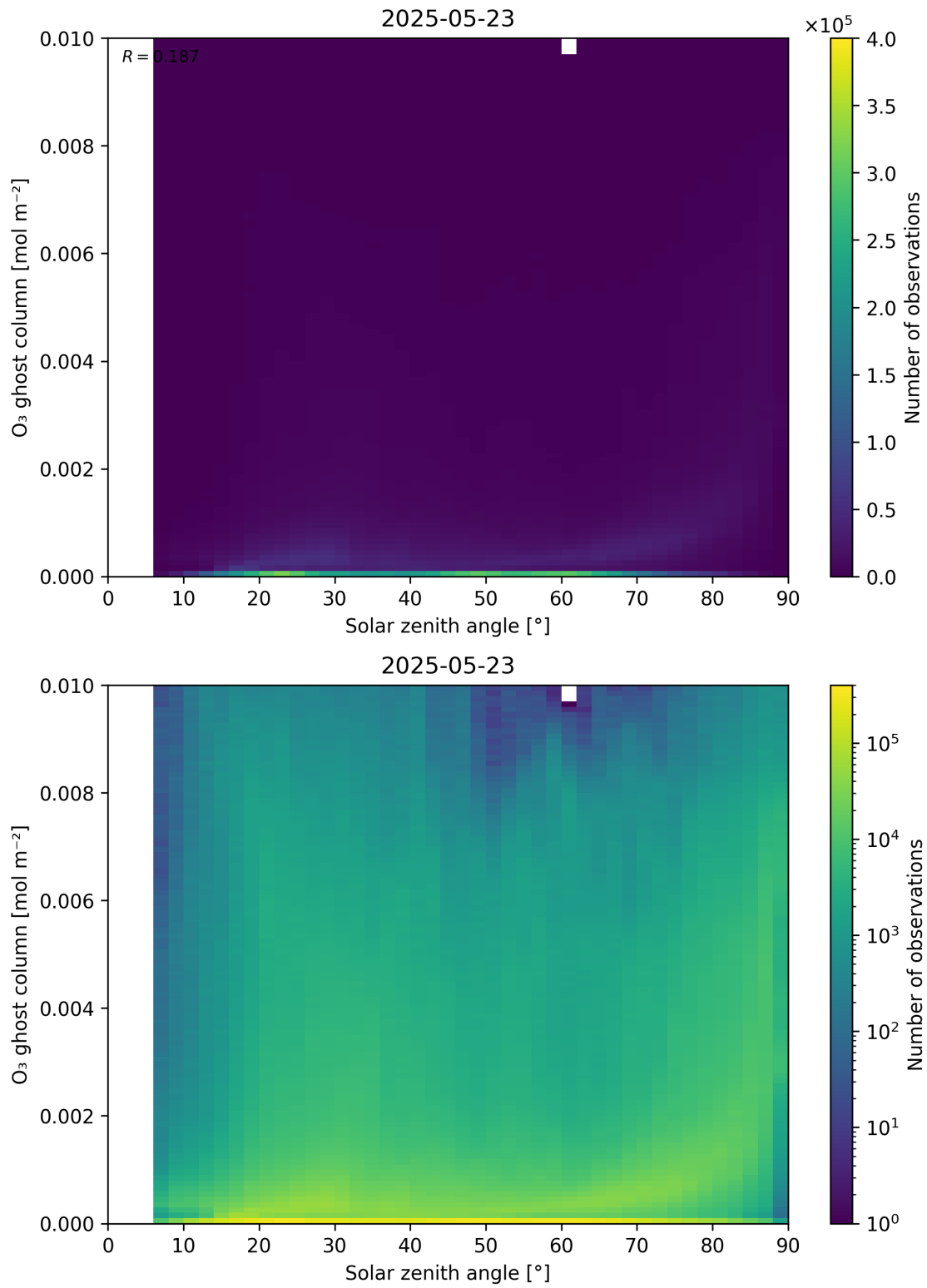
Figure 46: Scatter density plot of “Solar zenith angle” against “O 3 ghost column” for 2025-05-22 to 2025-05-24.
