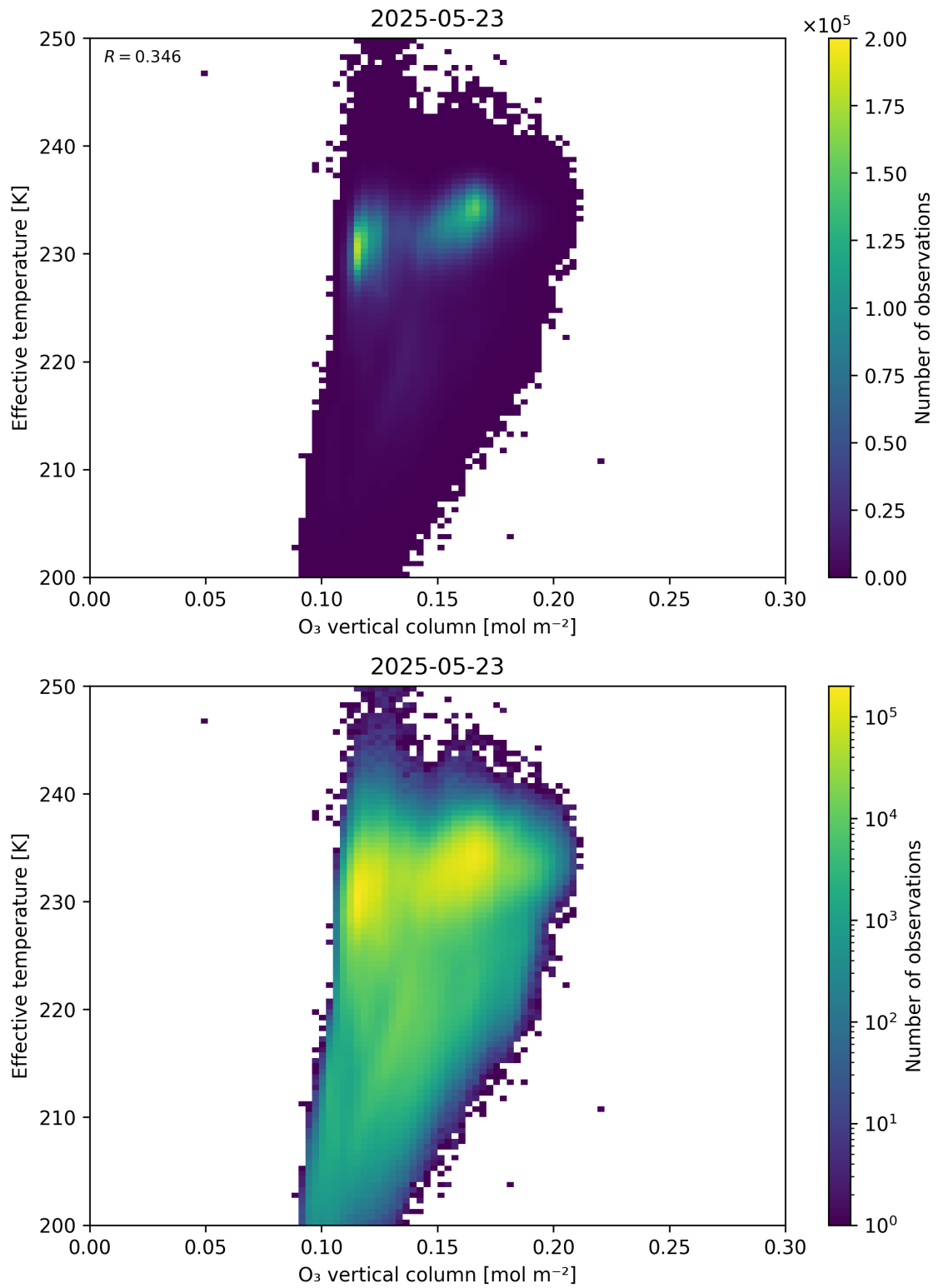
Figure 39: Scatter density plot of “O 3 vertical column” against “Effective temperature” for 2025-05-22 to 2025-05-24.
