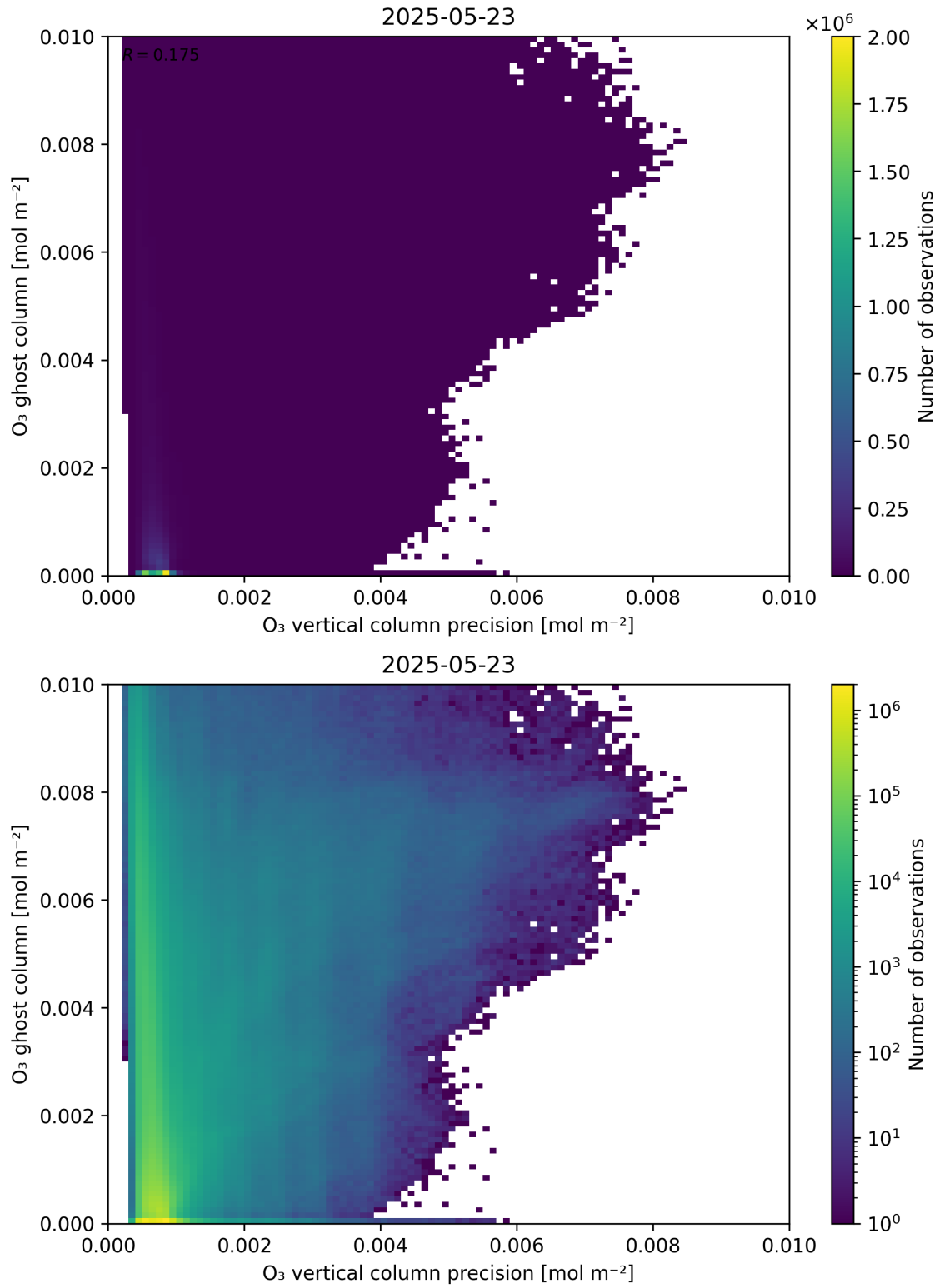
Figure 43: Scatter density plot of “ \text{O}_3 vertical column precision” against “ \text{O}_3 ghost column” for 2025-05-22 to 2025-05-24.
