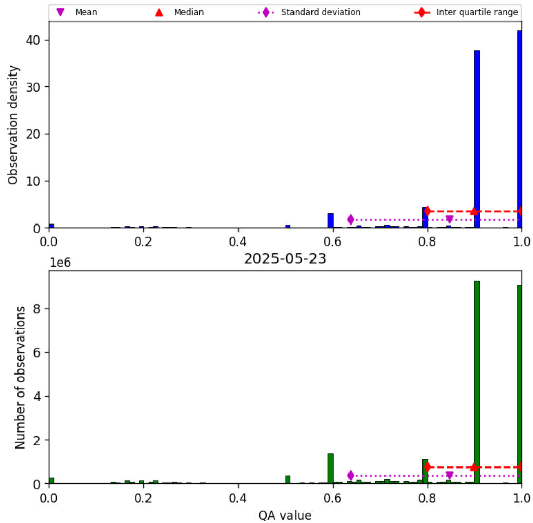
Figure 20: Histogram of “QA value” for 2025-05-22 to 2025-05-24
