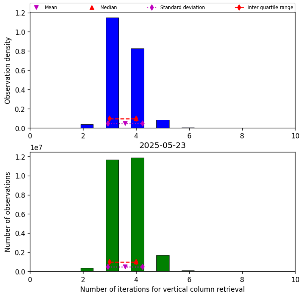
Figure 26: Histogram of “Number of iterations for vertical column retrieval” for 2025-05-22 to 2025-05-24
