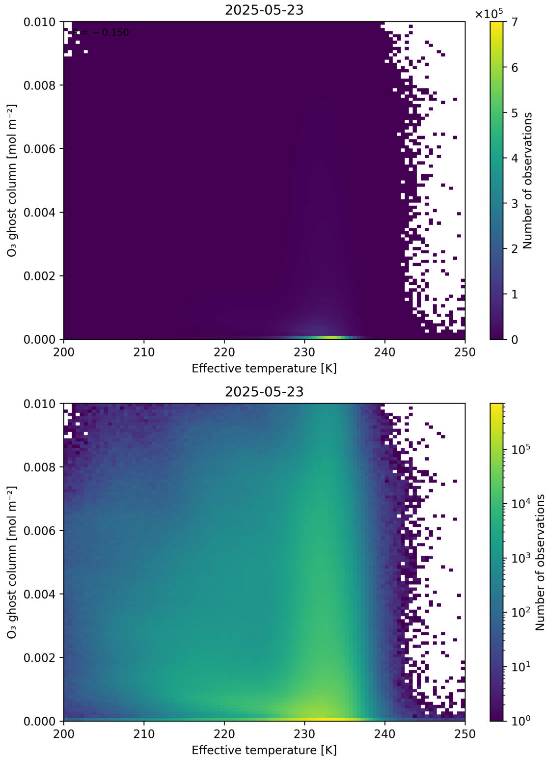
Figure 38: Scatter density plot of “Effective temperature” against “O 3 ghost column” for 2025-05-22 to 2025-05-24.
