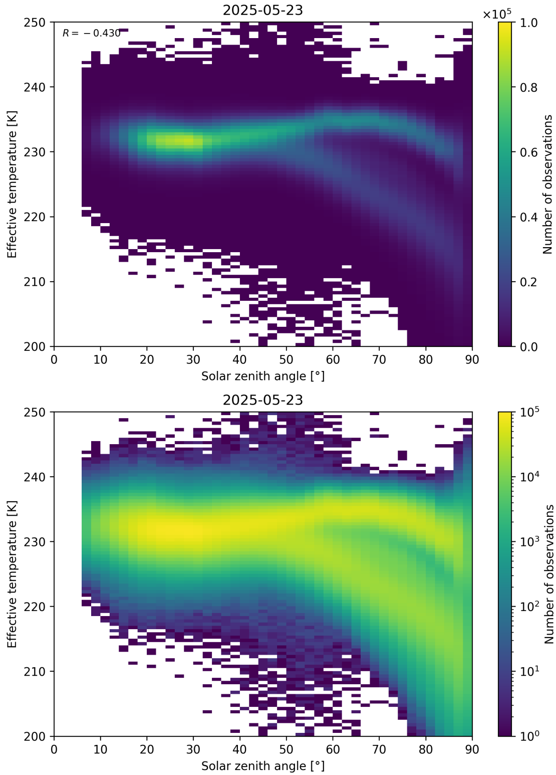
Figure 45: Scatter density plot of “Solar zenith angle” against “Effective temperature” for 2025-05-22 to 2025-05-24.
