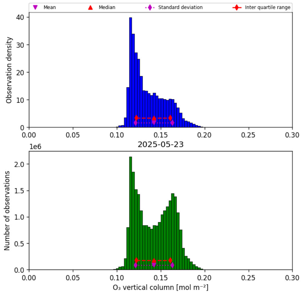
Figure 21: Histogram of “O 3 vertical column” for 2025-05-22 to 2025-05-24
