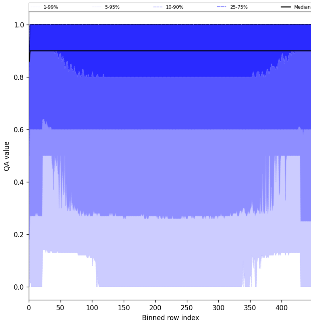
Figure 27: Along track statistics of “QA value” for 2025-05-22 to 2025-05-24
