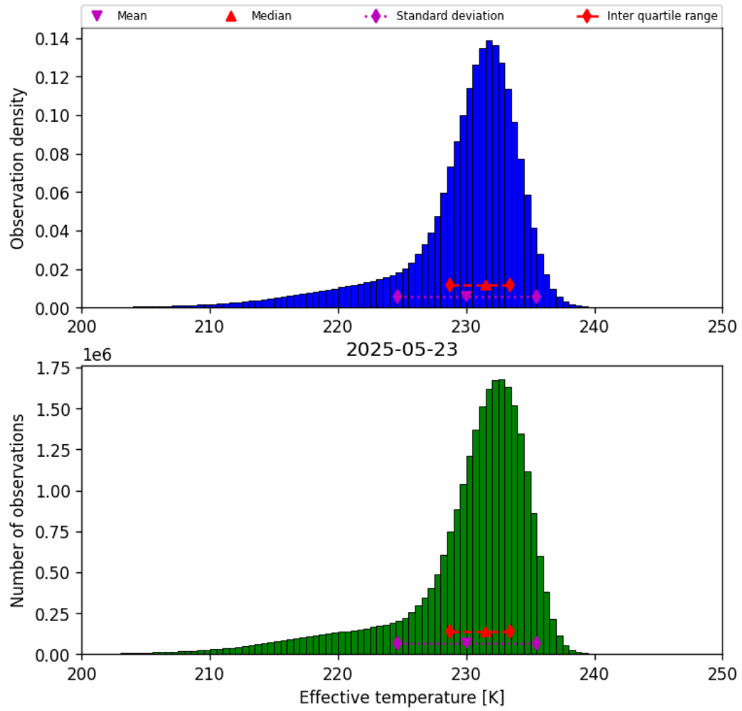
Figure 24: Histogram of “Effective temperature” for 2025-05-22 to 2025-05-24
