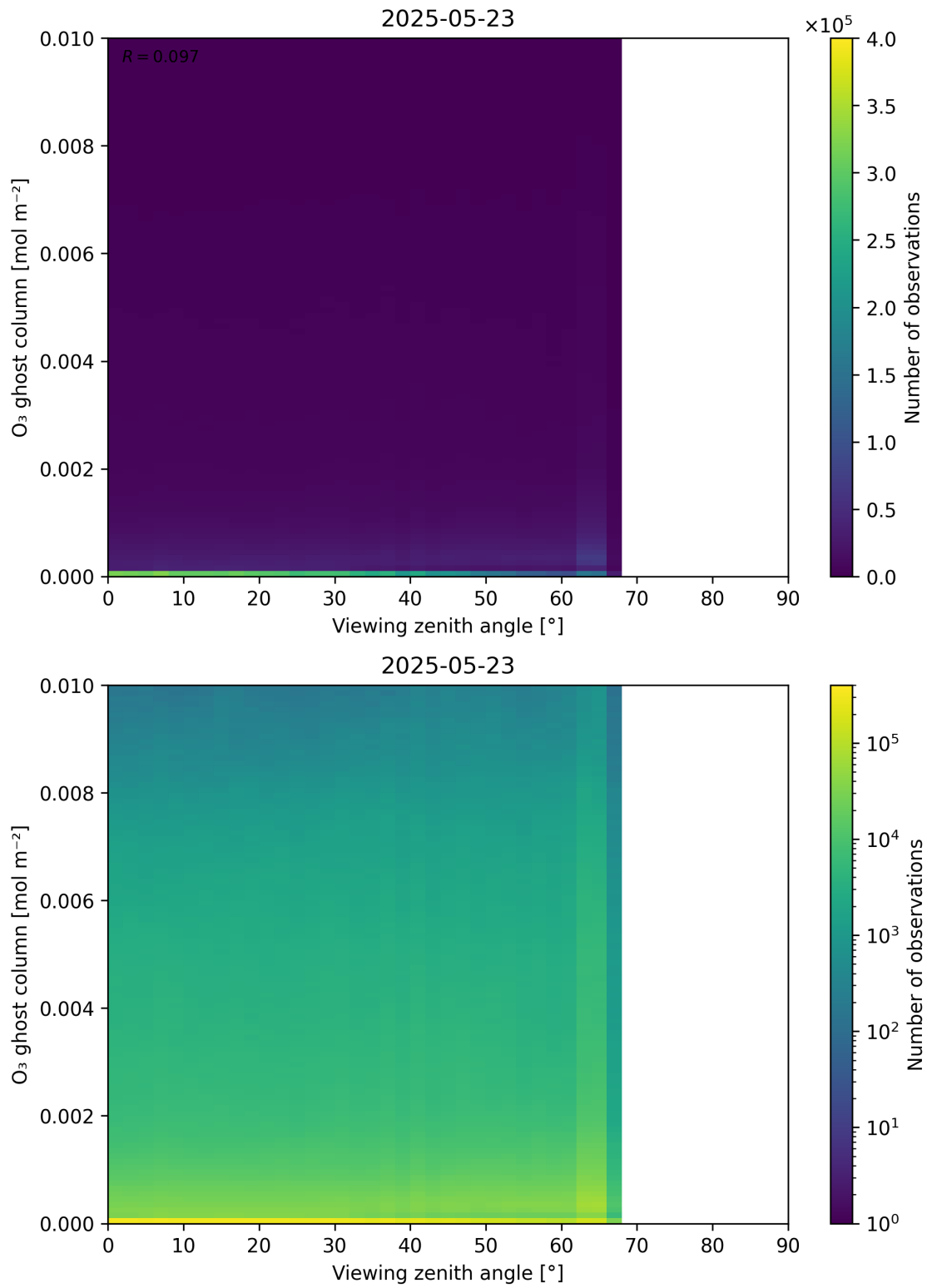
Figure 51: Scatter density plot of “Viewing zenith angle” against “O 3 ghost column” for 2025-05-22 to 2025-05-24.
