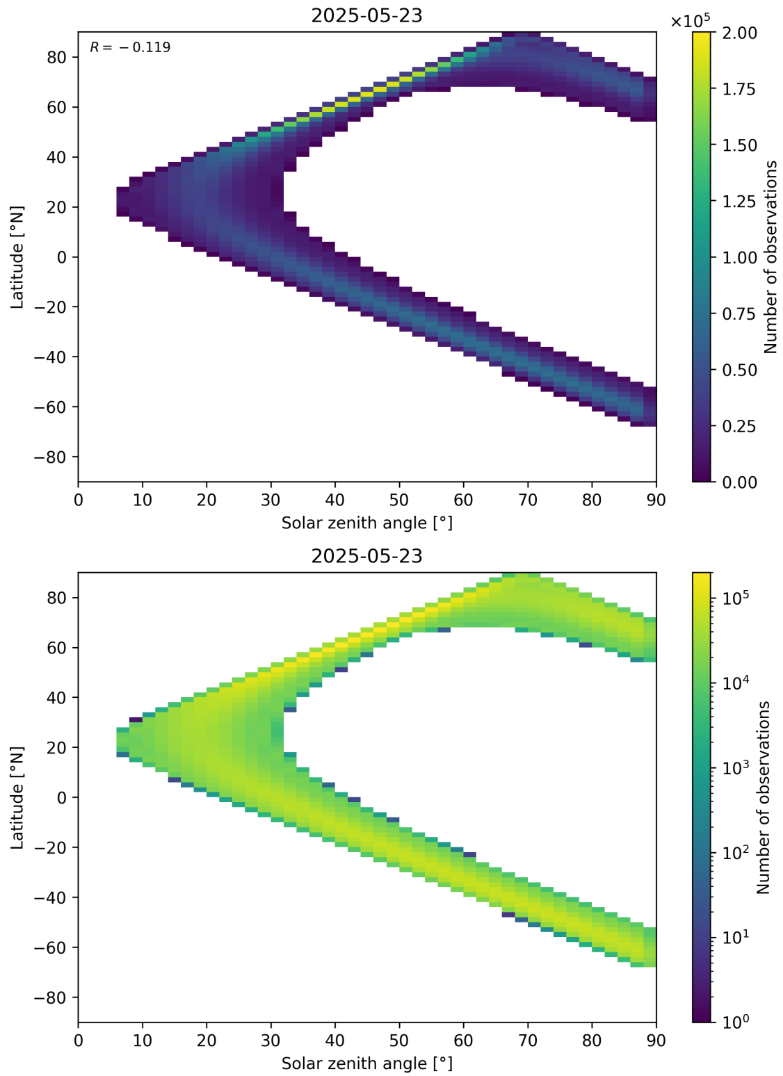
Figure 44: Scatter density plot of “Solar zenith angle” against “Latitude” for 2025-05-22 to 2025-05-24.
