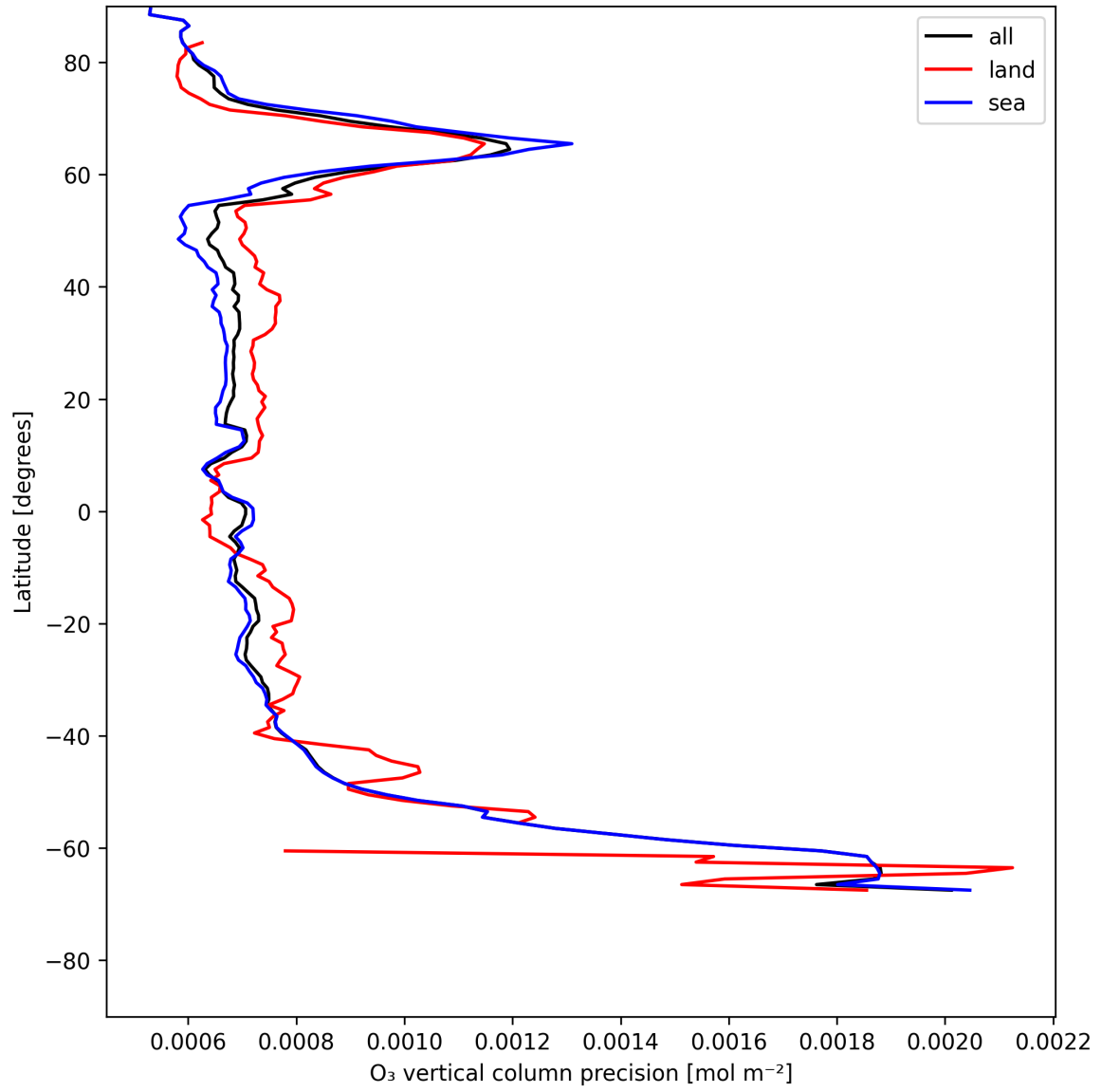
Figure 15: Zonal average of “O 3 vertical column precision” for 2025-05-22 to 2025-05-24.
