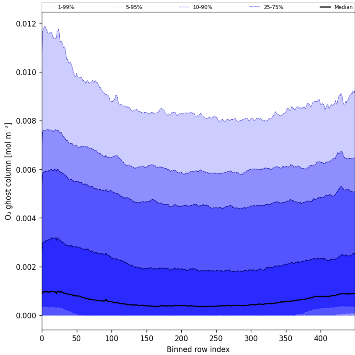
Figure 32: Along track statistics of "O 3 ghost column" for 2025-05-22 to 2025-05-24
