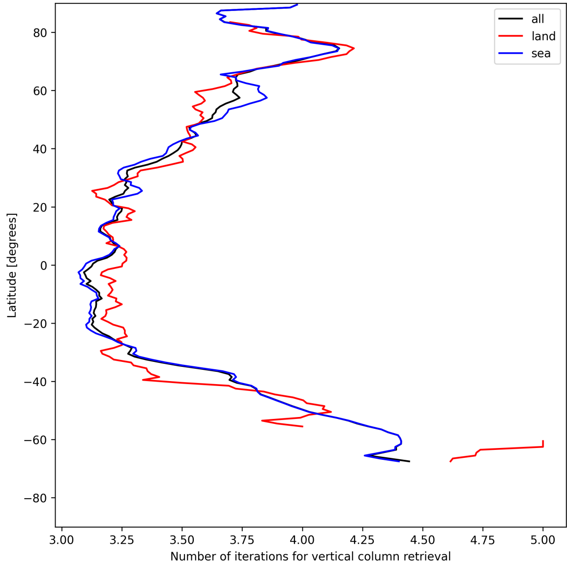
Figure 19: Zonal average of “Number of iterations for vertical column retrieval” for 2025-05-22 to 2025-05-24.
