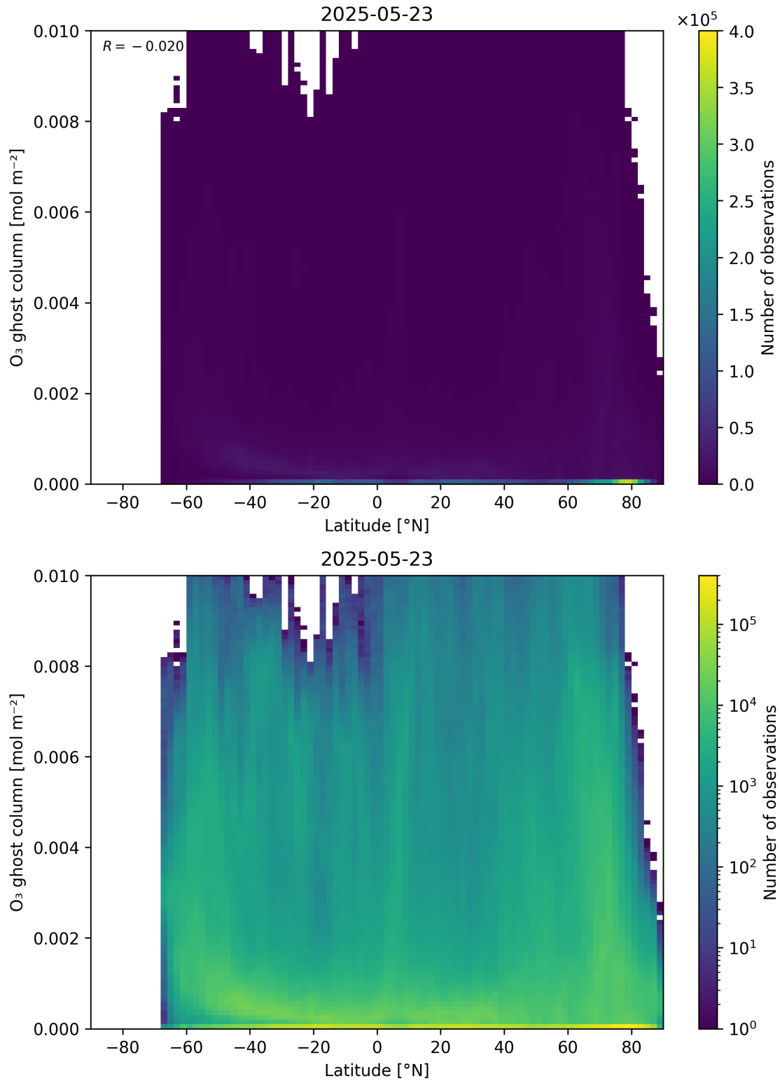
Figure 35: Scatter density plot of “Latitude” against “O 3 ghost column” for 2025-05-22 to 2025-05-24.
