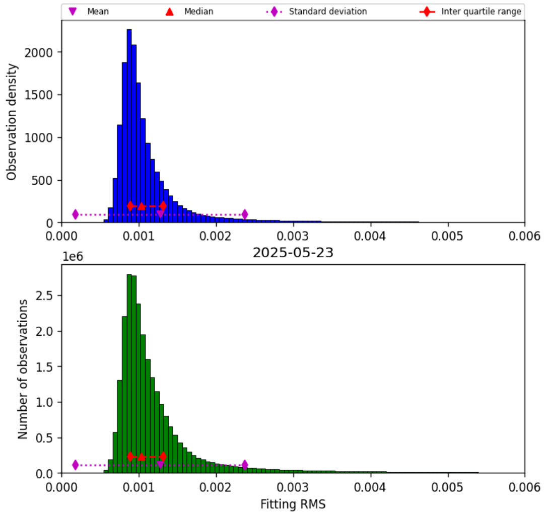
Figure 23: Histogram of “Fitting RMS” for 2025-05-22 to 2025-05-24
