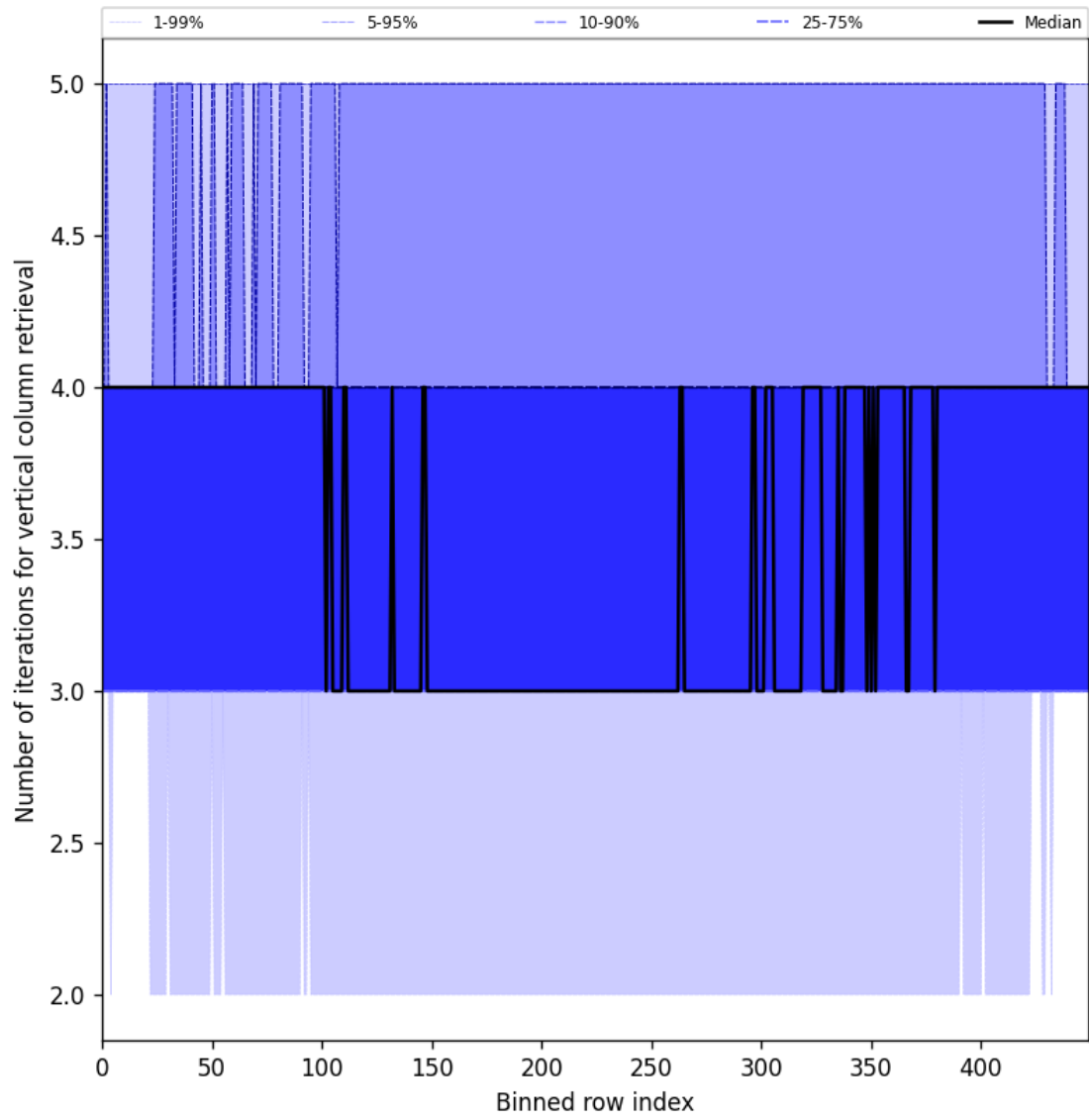
Figure 33: Along track statistics of “Number of iterations for vertical column retrieval” for 2025-05-22 to 2025-05-24
