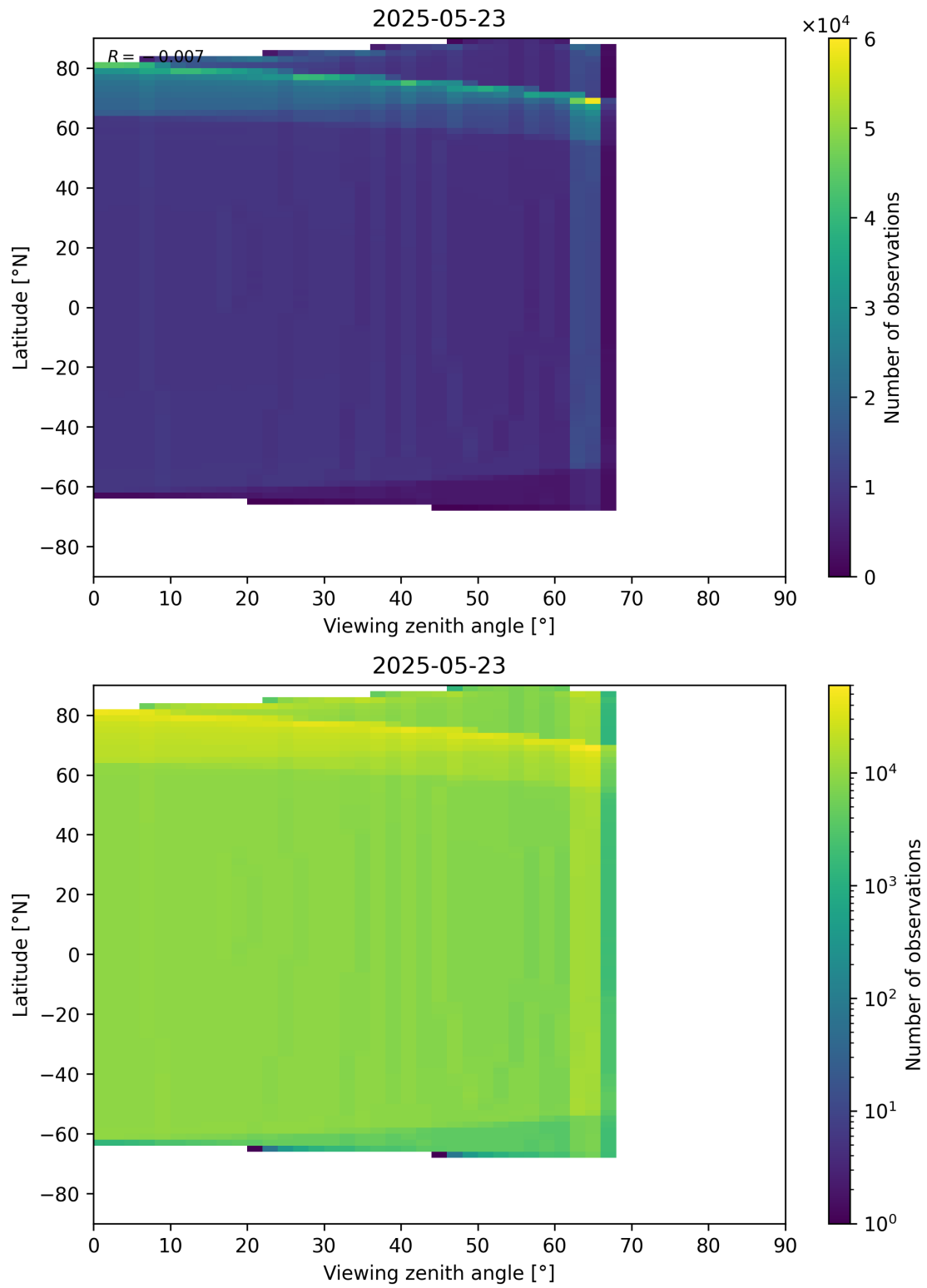
Figure 49: Scatter density plot of “Viewing zenith angle” against “Latitude” for 2025-05-22 to 2025-05-24.
