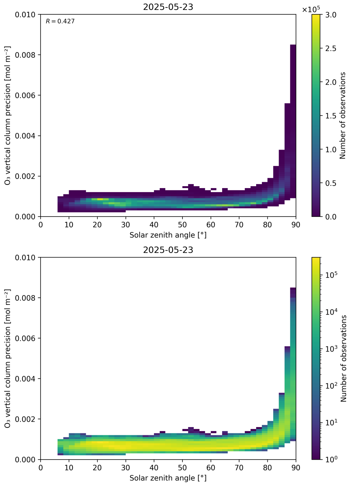
Figure 48: Scatter density plot of “Solar zenith angle” against “O 3 vertical column precision” for 2025-05-22 to 2025-05-24.
