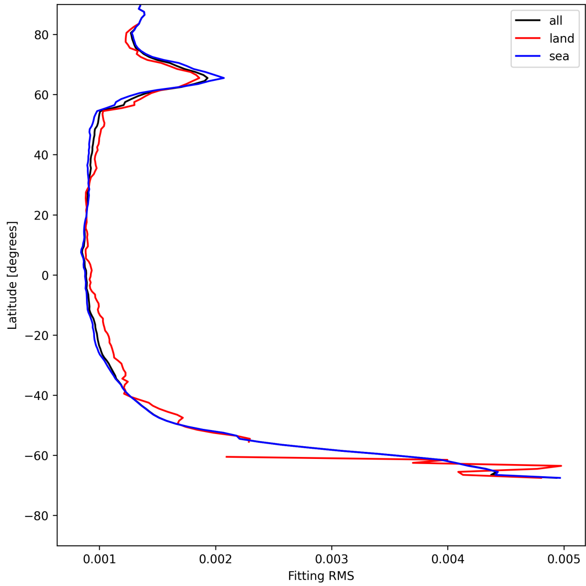
Figure 16: Zonal average of “Fitting RMS” for 2025-05-22 to 2025-05-24.
