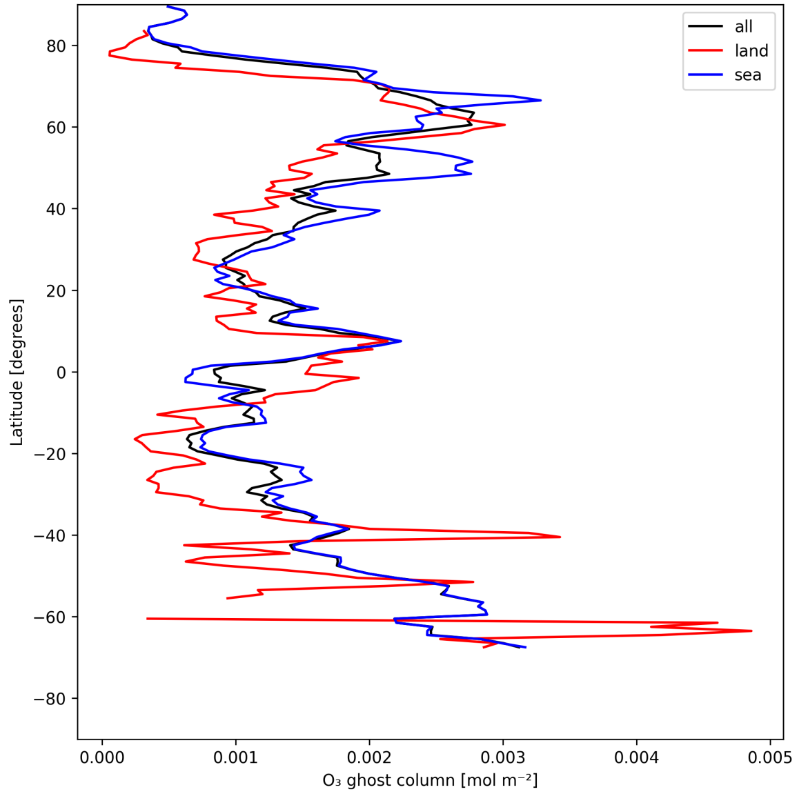
Figure 18: Zonal average of “O 3 ghost column” for 2025-05-22 to 2025-05-24.
