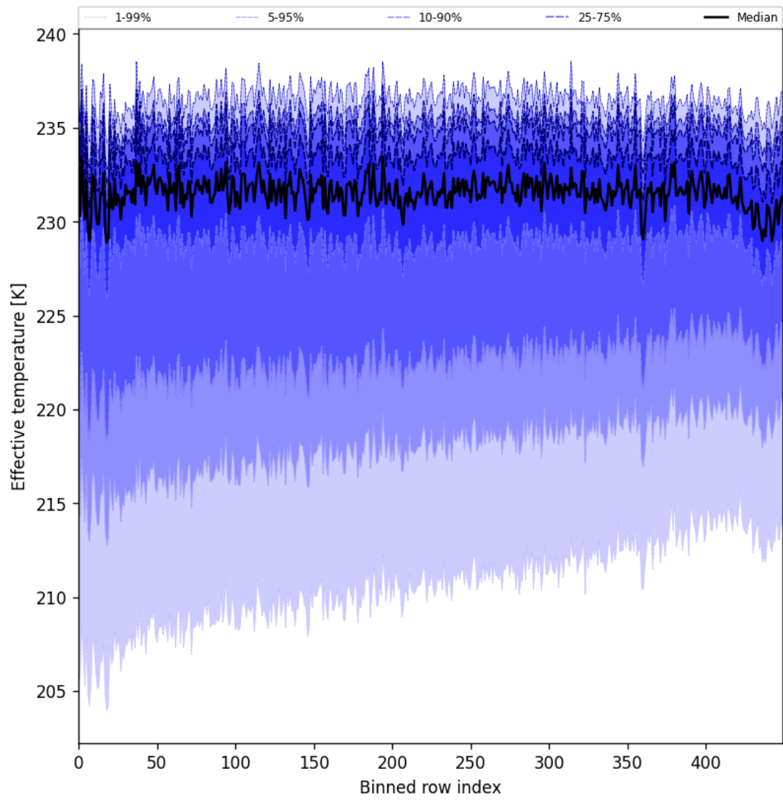
Figure 31: Along track statistics of “Effective temperature” for 2025-05-22 to 2025-05-24
