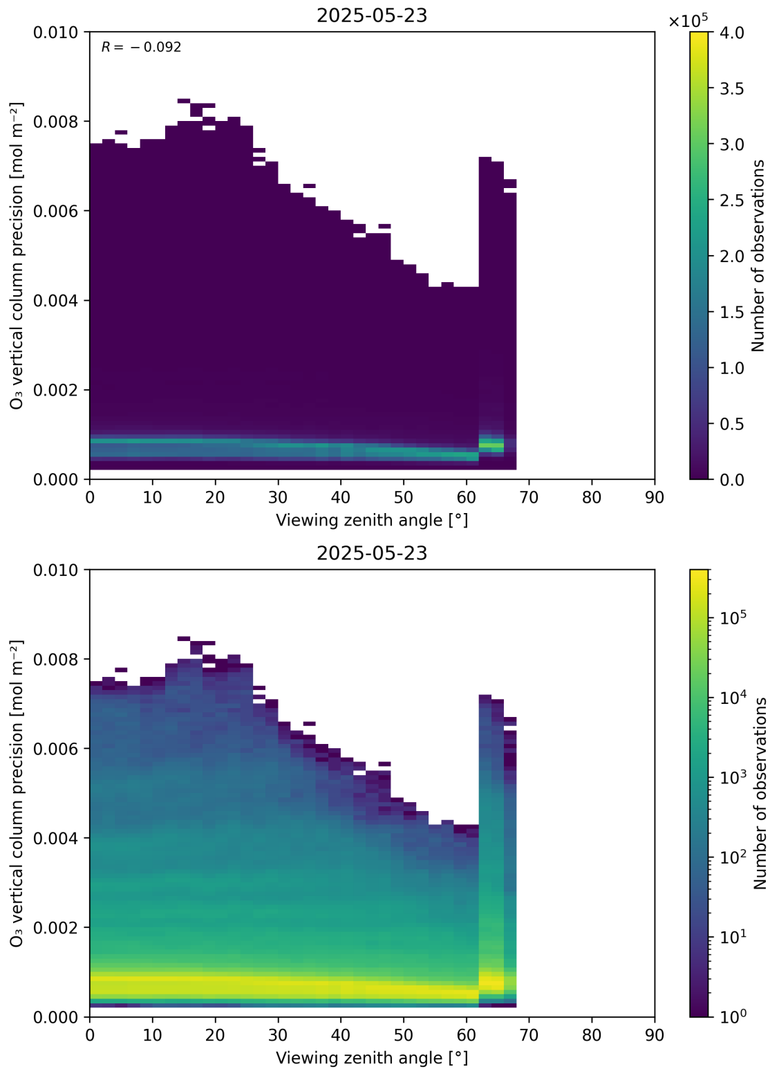
Figure 53: Scatter density plot of “Viewing zenith angle” against “O 3 vertical column precision” for 2025-05-22 to 2025-05-24.
