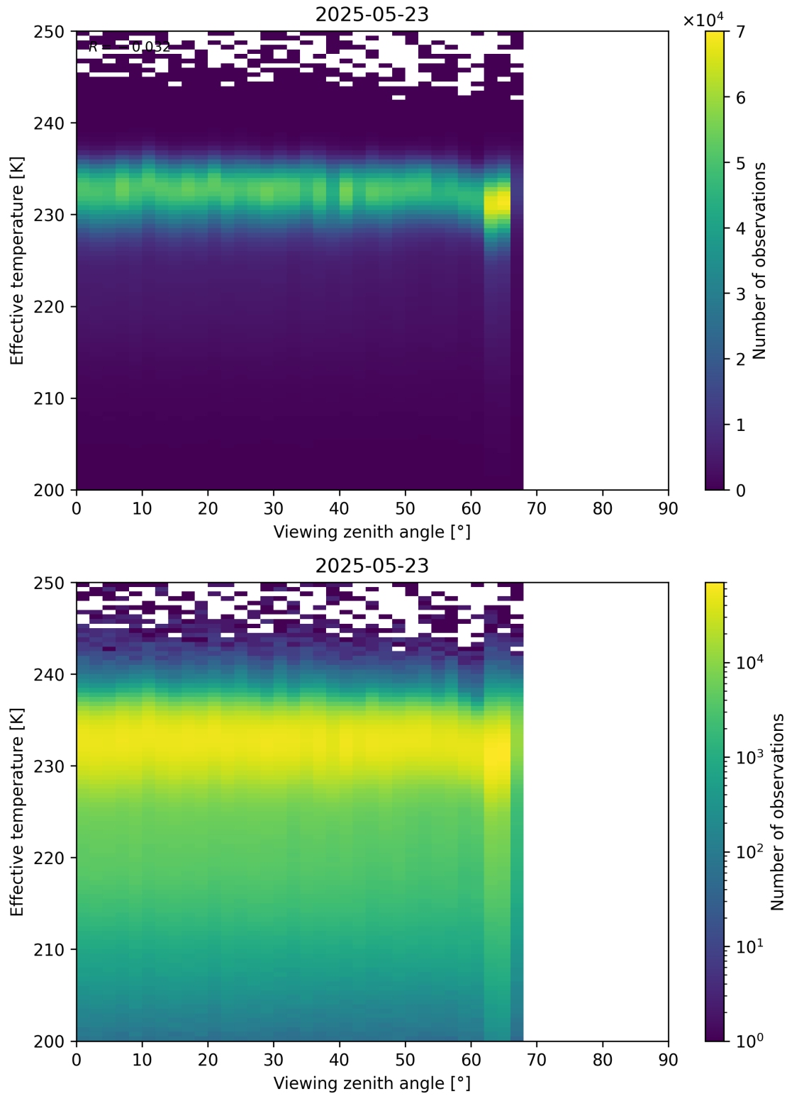
Figure 50: Scatter density plot of “Viewing zenith angle” against “Effective temperature” for 2025-05-22 to 2025-05-24.
