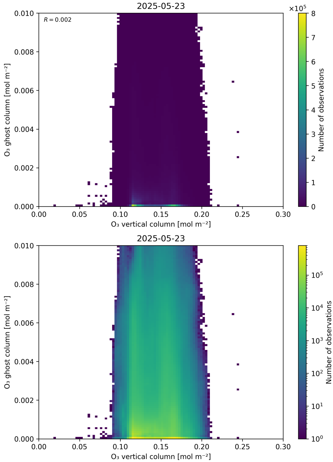
Figure 40: Scatter density plot of “O 3 vertical column” against “O 3 ghost column” for 2025-05-22 to 2025-05-24.
