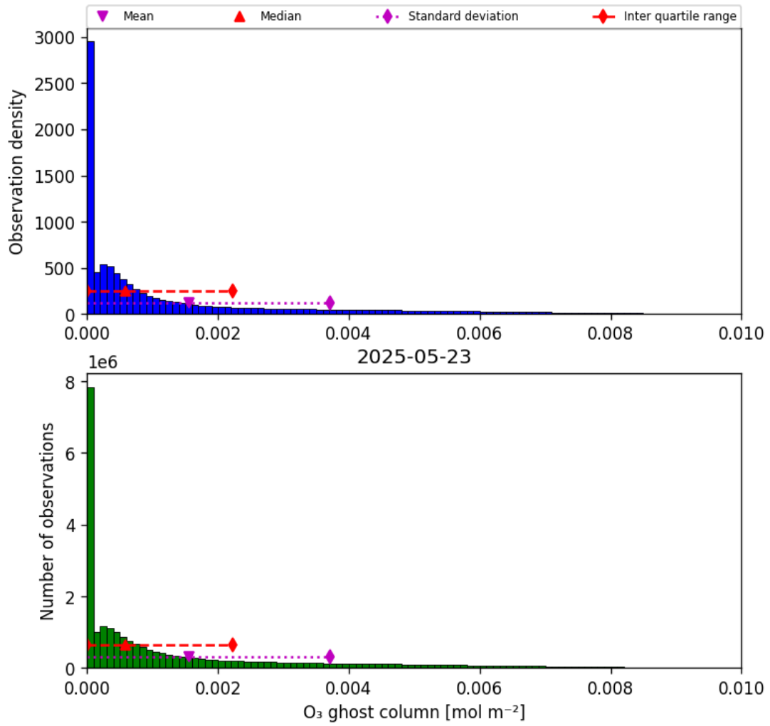
Figure 25: Histogram of “O 3 ghost column” for 2025-05-22 to 2025-05-24
