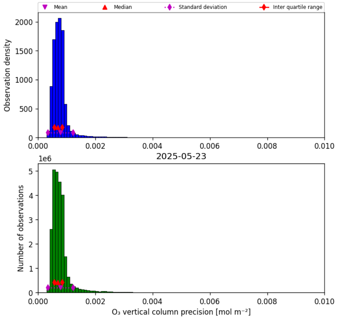
Figure 22: Histogram of “O 3 vertical column precision” for 2025-05-22 to 2025-05-24
