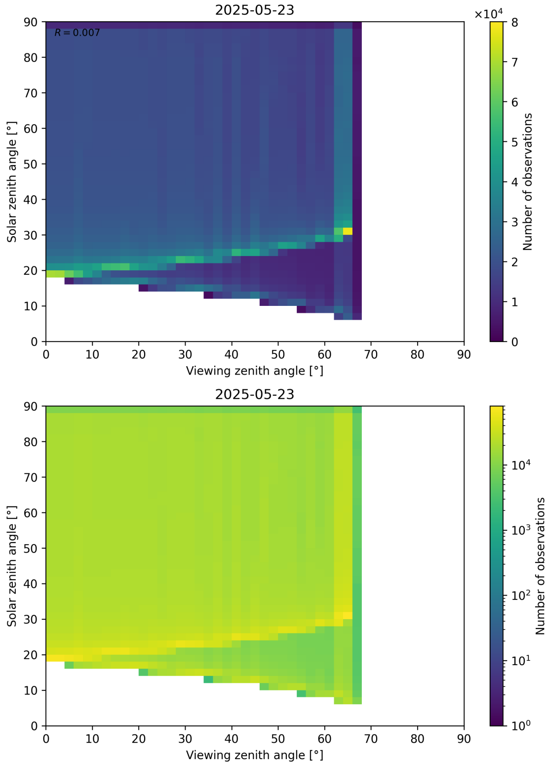
Figure 54: Scatter density plot of “Viewing zenith angle” against “Solar zenith angle” for 2025-05-22 to 2025-05-24.
