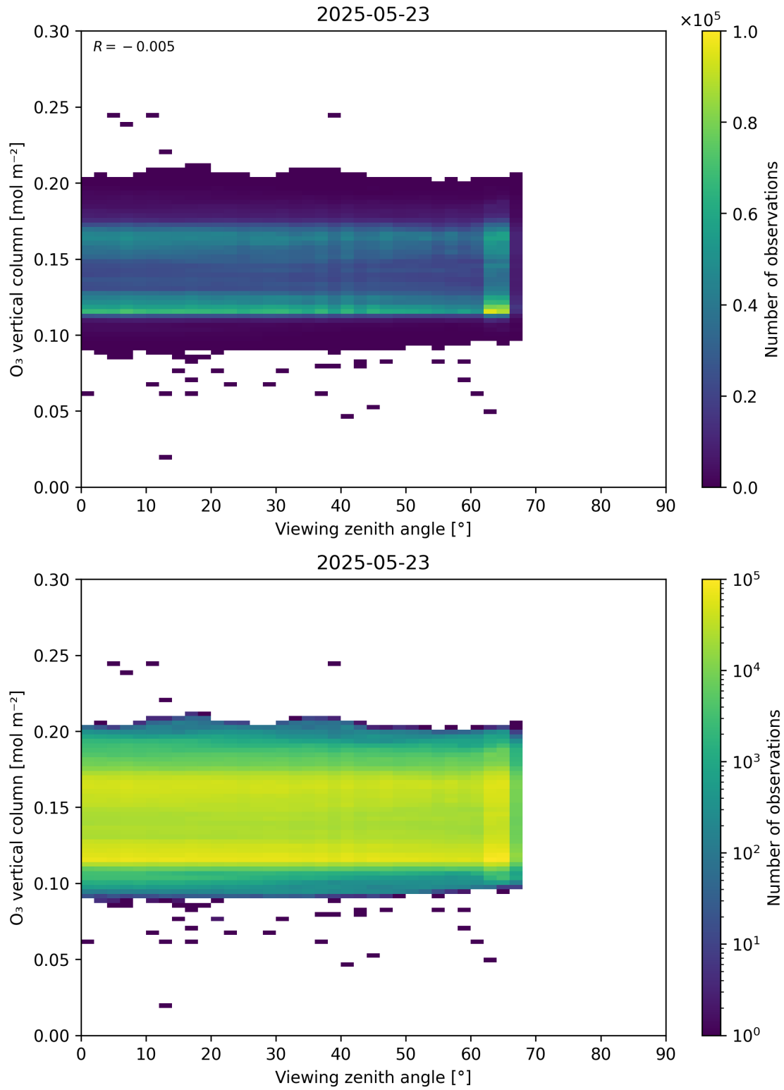
Figure 52: Scatter density plot of “Viewing zenith angle” against “O 3 vertical column” for 2025-05-22 to 2025-05-24.
