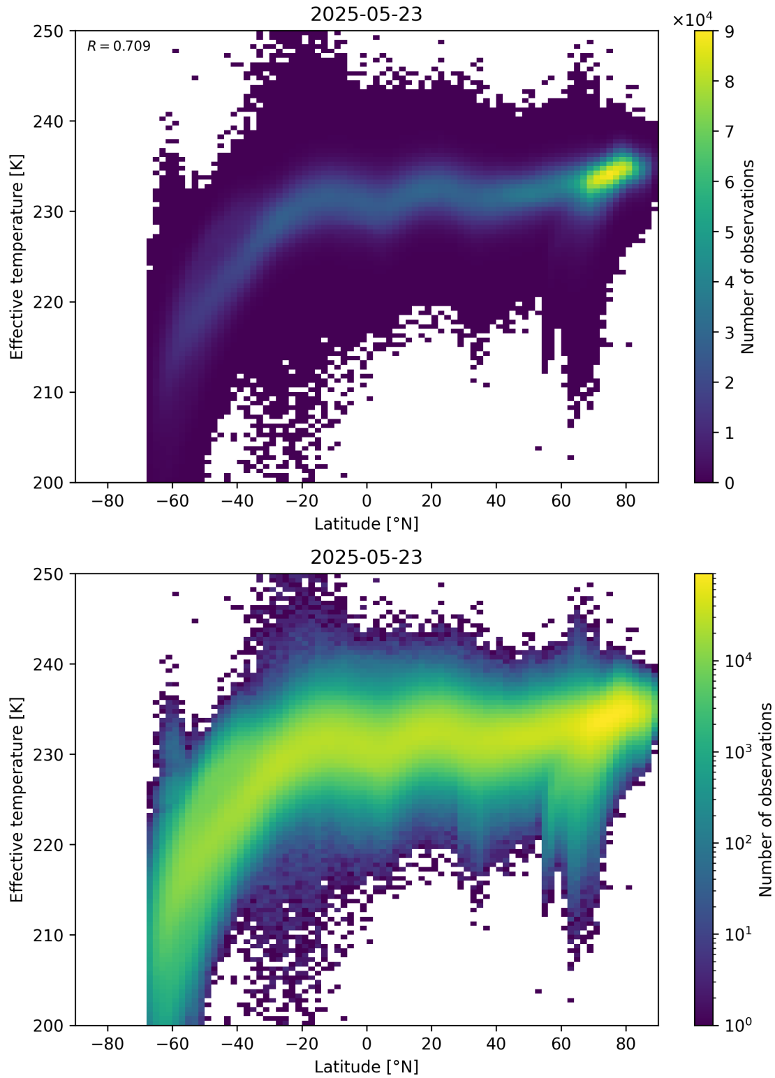
Figure 34: Scatter density plot of “Latitude” against “Effective temperature” for 2025-05-22 to 2025-05-24.
