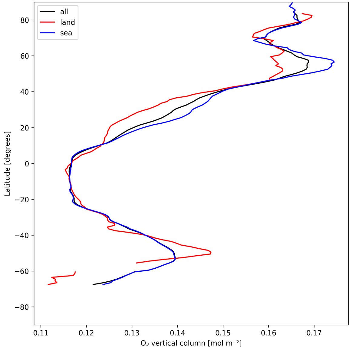
Figure 14: Zonal average of “O 3 vertical column” for 2025-05-22 to 2025-05-24.
