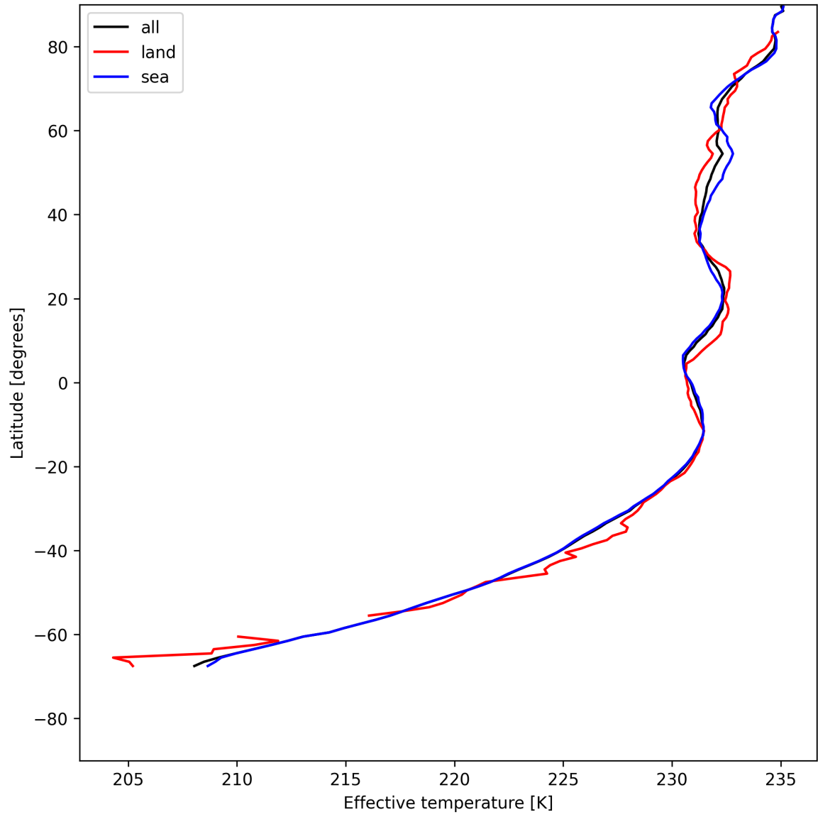
Figure 17: Zonal average of "Effective temperature" for 2025-05-22 to 2025-05-24.
