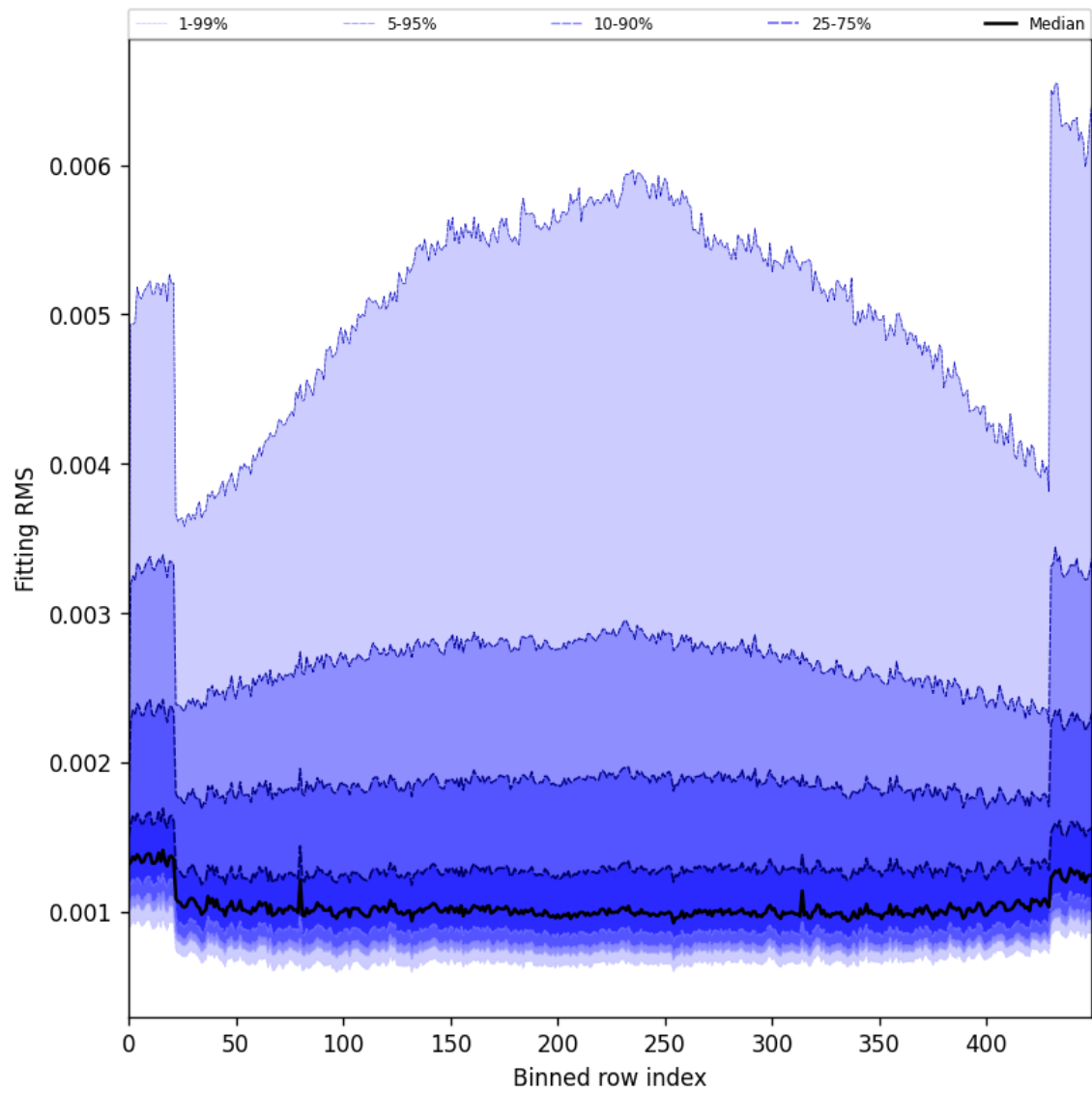
Figure 30: Along track statistics of “Fitting RMS” for 2025-05-22 to 2025-05-24
