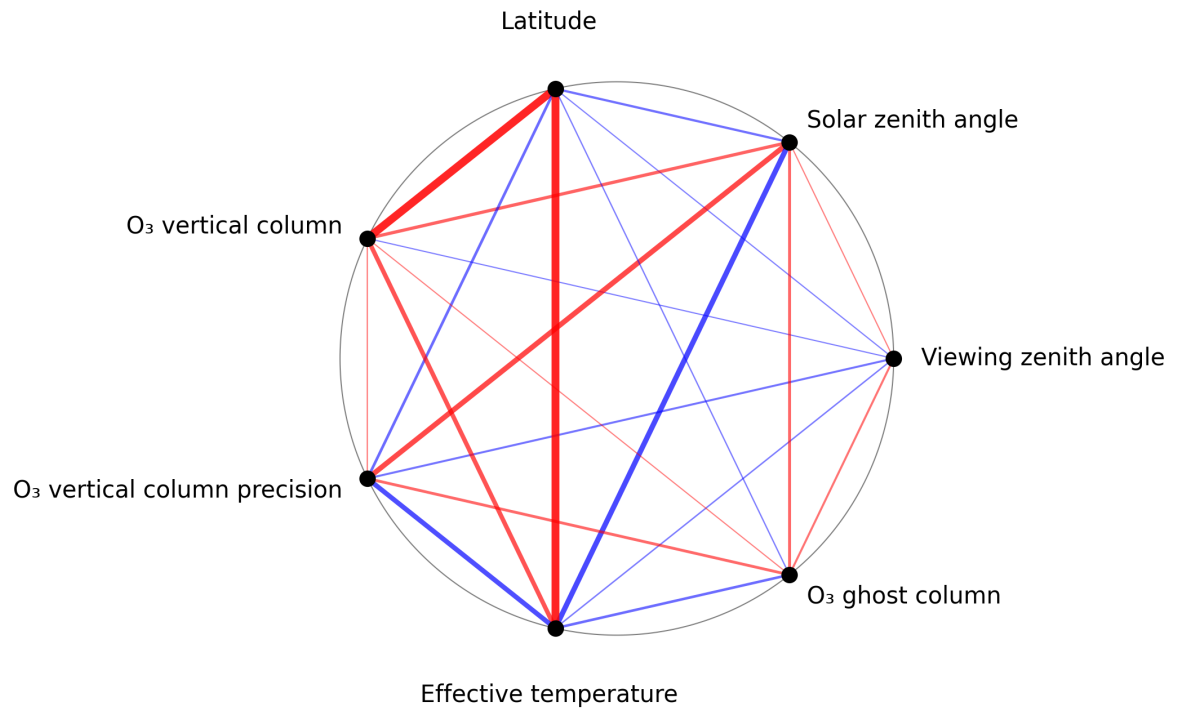
Figure 1: Map of correlation graph for 2025-05-22 to 2025-05-24.
