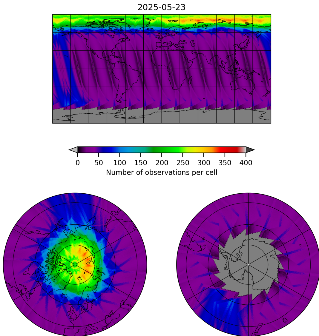
Figure 12: Map of the number of observations for 2025-05-22 to 2025-05-24
