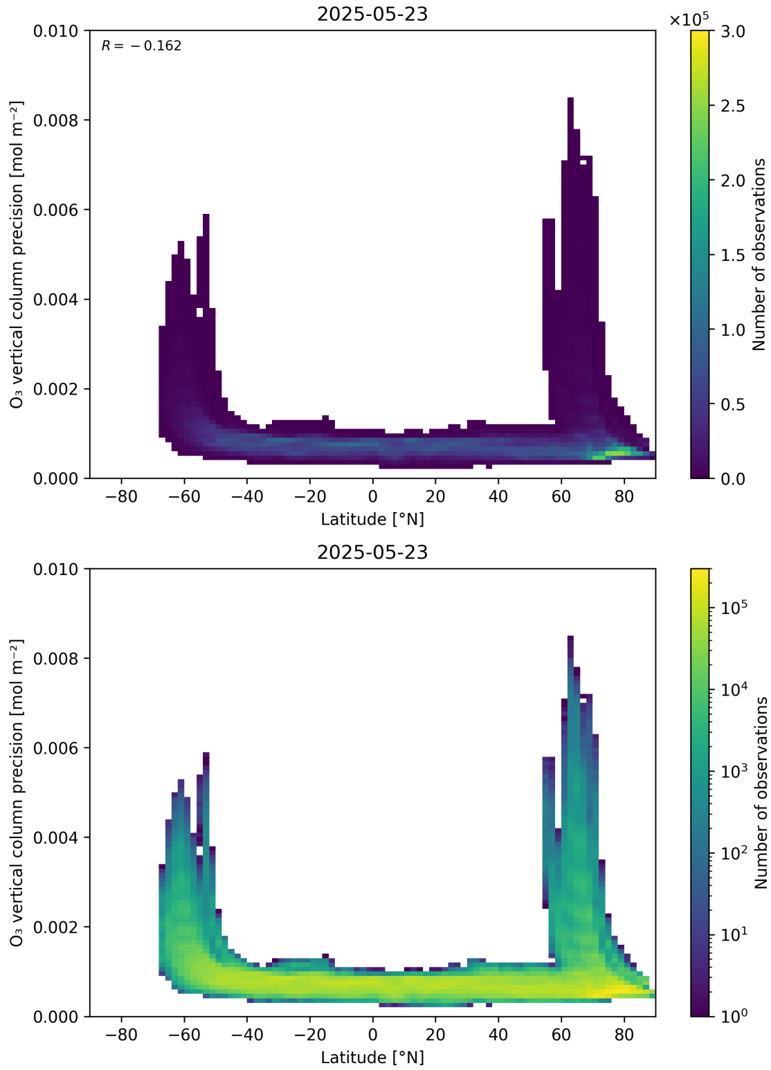
Figure 37: Scatter density plot of “Latitude” against “O 3 vertical column precision” for 2025-05-22 to 2025-05-24.
