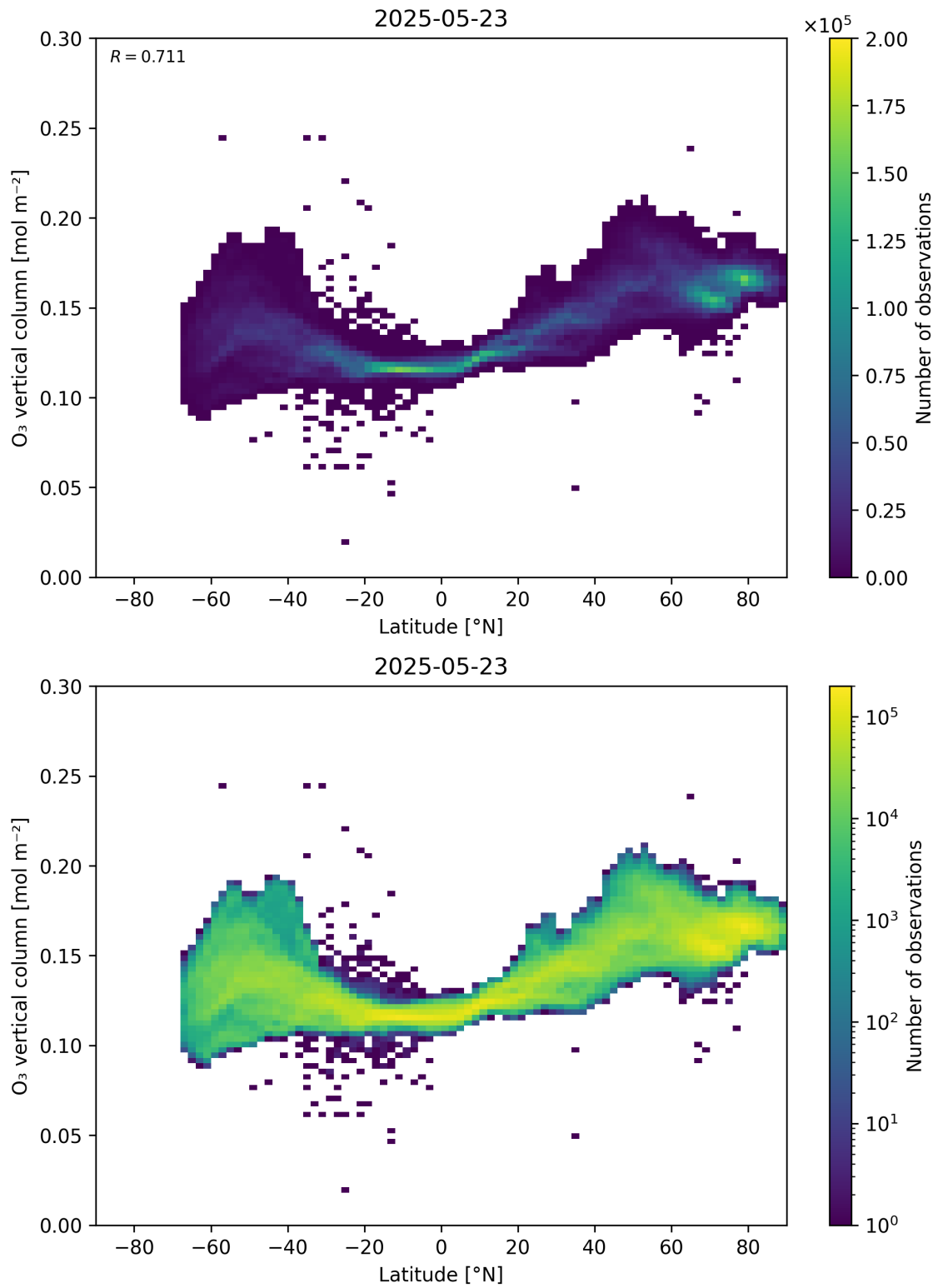
Figure 36: Scatter density plot of “Latitude” against “O 3 vertical column” for 2025-05-22 to 2025-05-24.
