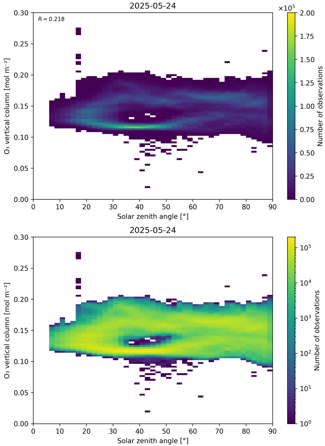
Figure 47: Scatter density plot of “Solar zenith angle” against “O 3 vertical column” for 2025-05-23 to 2025-05-25.
