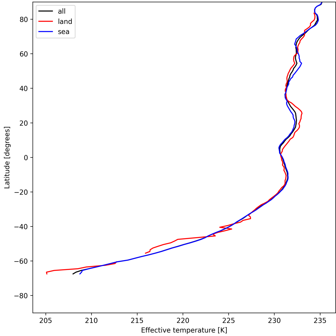
Figure 17: Zonal average of "Effective temperature" for 2025-05-23 to 2025-05-25.
