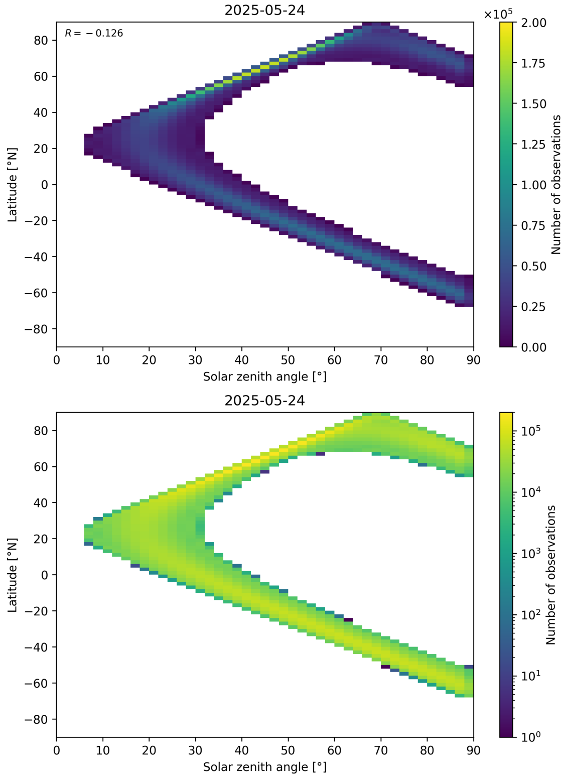
Figure 44: Scatter density plot of “Solar zenith angle” against “Latitude” for 2025-05-23 to 2025-05-25.
