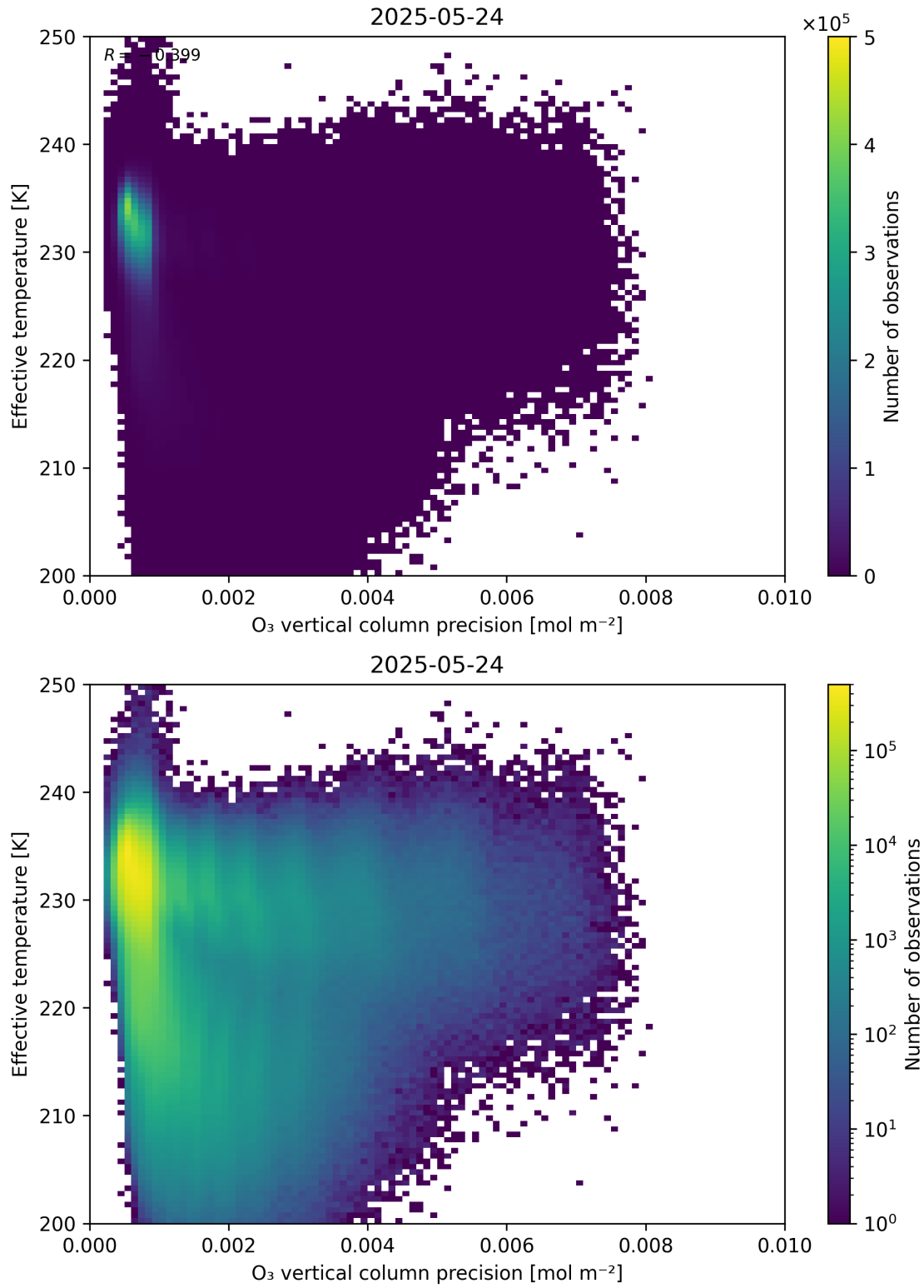
Figure 42: Scatter density plot of “ O_3 vertical column precision” against “Effective temperature” for 2025-05-23 to 2025-05-25.
