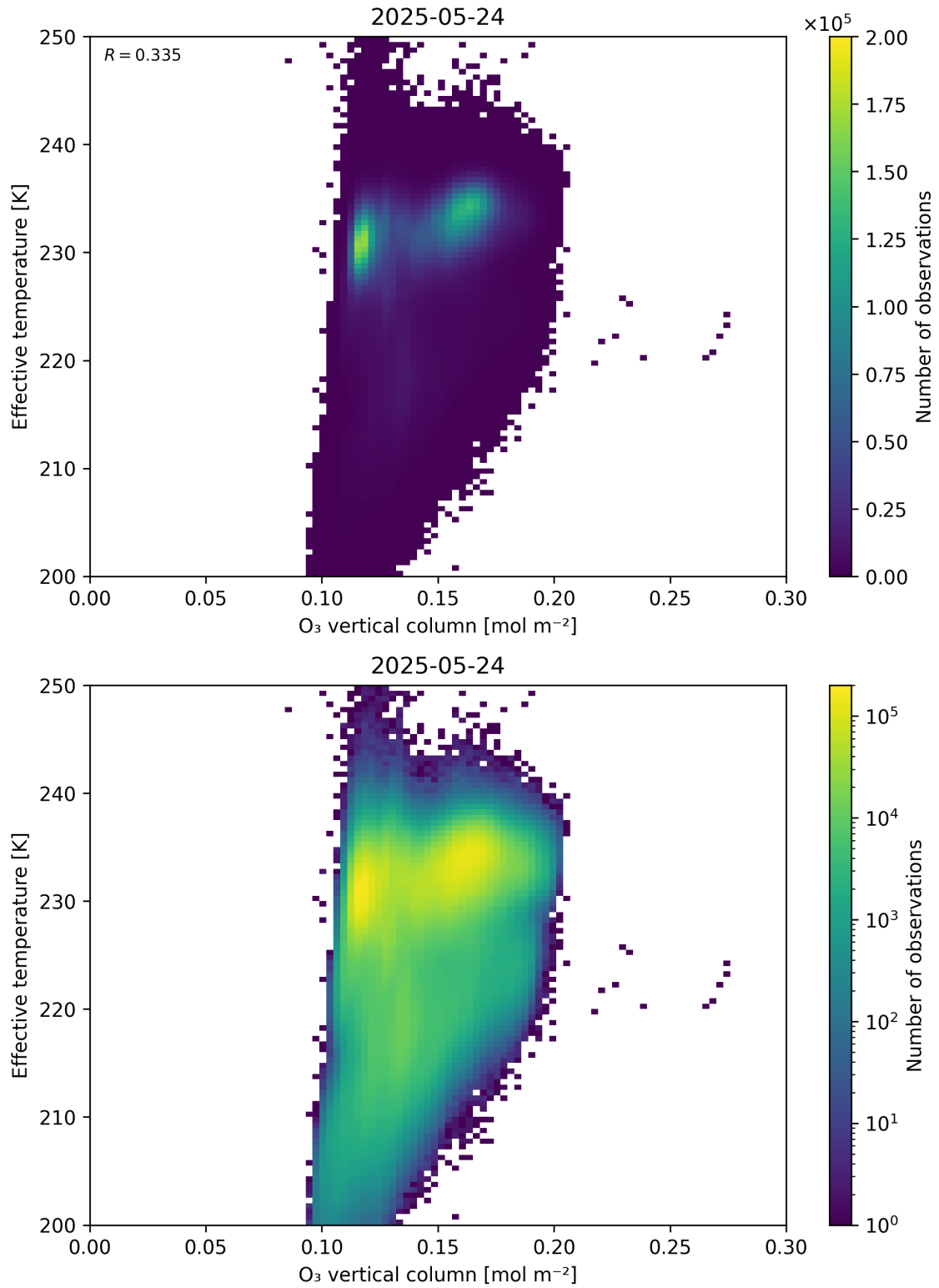
Figure 39: Scatter density plot of “O 3 vertical column” against “Effective temperature” for 2025-05-23 to 2025-05-25.
