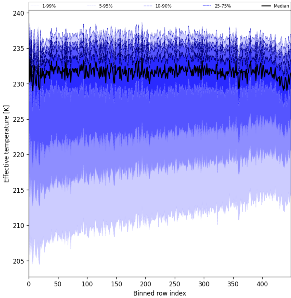
Figure 31: Along track statistics of “Effective temperature” for 2025-05-23 to 2025-05-25
