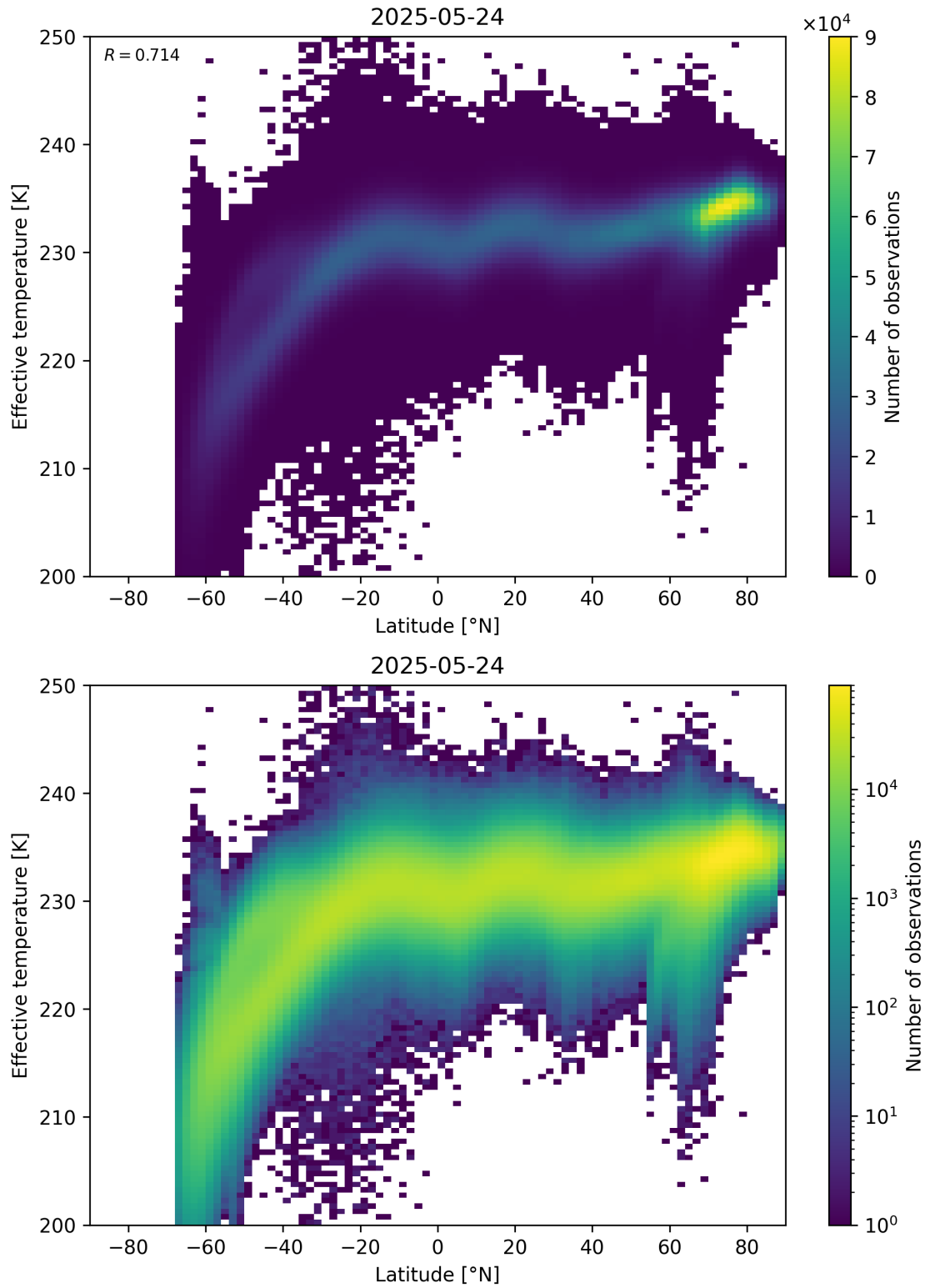
Figure 34: Scatter density plot of “Latitude” against “Effective temperature” for 2025-05-23 to 2025-05-25.
