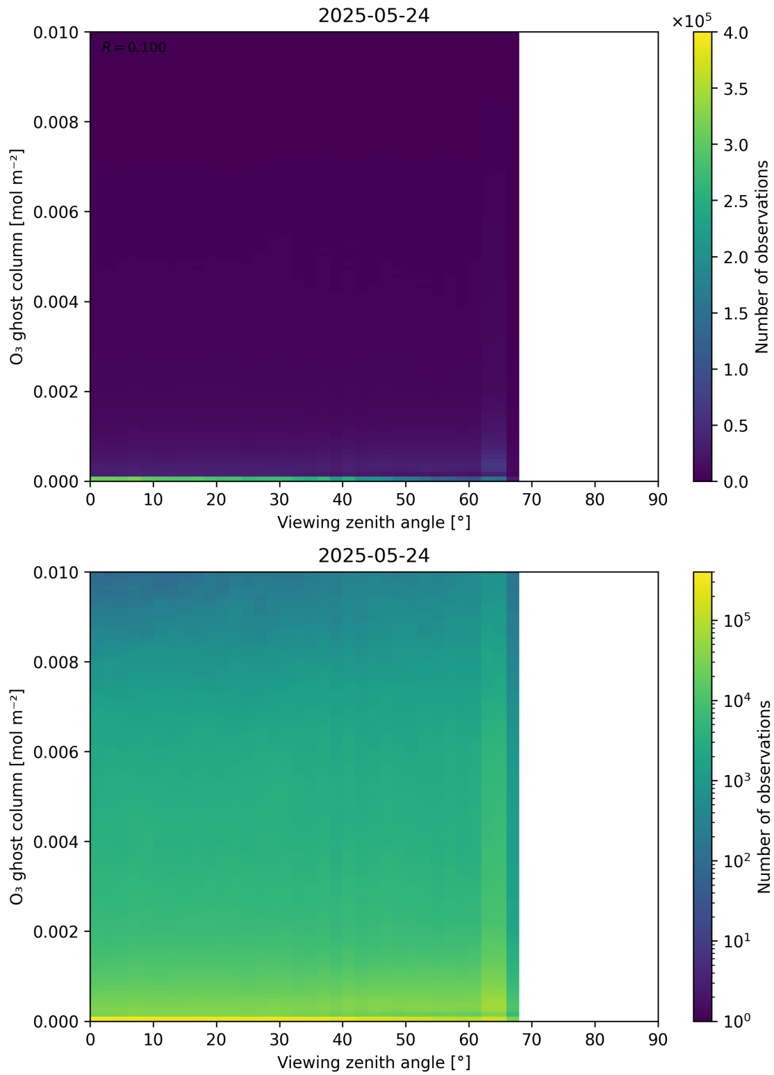
Figure 51: Scatter density plot of “Viewing zenith angle” against “O 3 ghost column” for 2025-05-23 to 2025-05-25.
