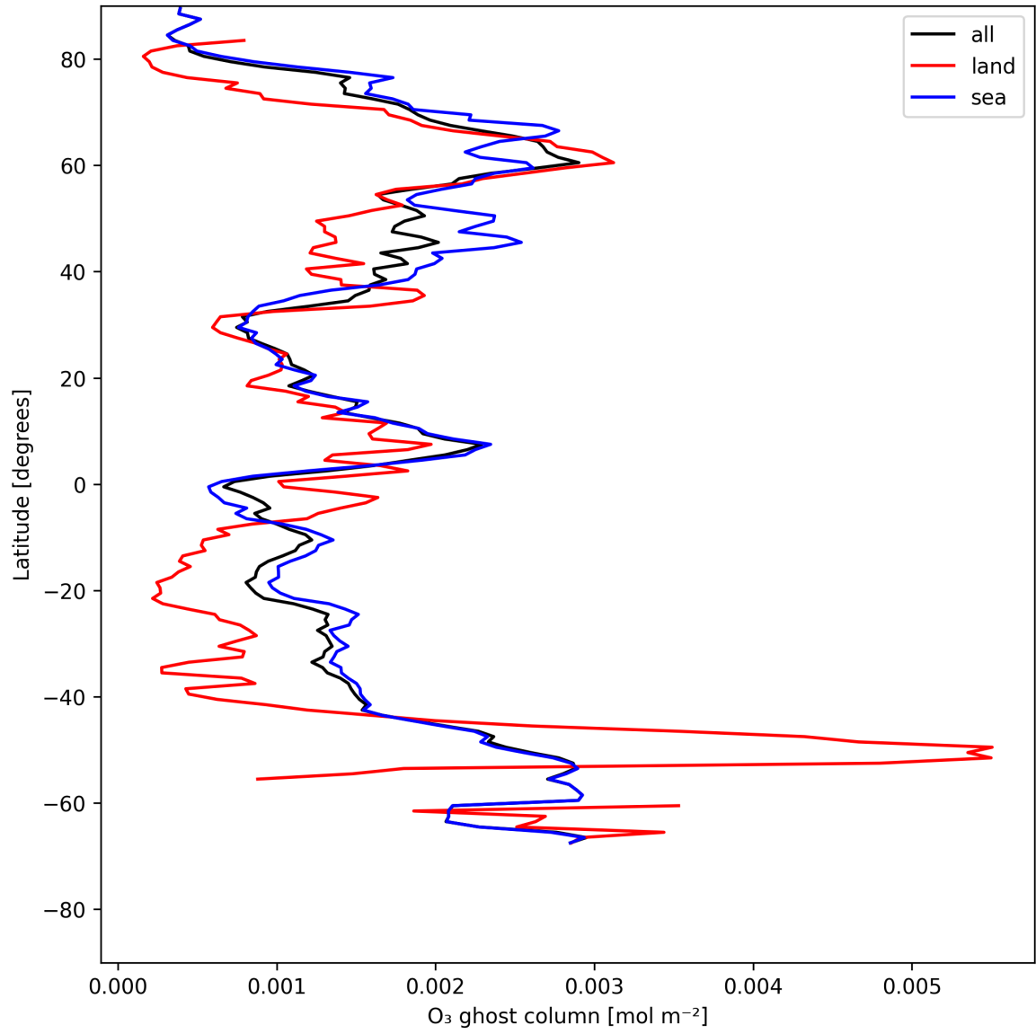
Figure 18: Zonal average of “O 3 ghost column” for 2025-05-23 to 2025-05-25.
