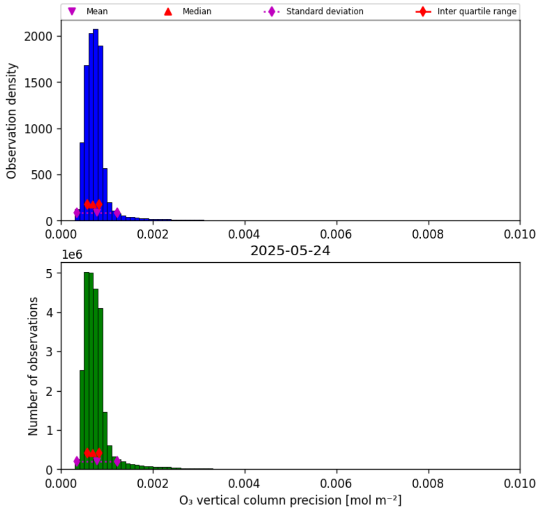
Figure 22: Histogram of “O 3 vertical column precision” for 2025-05-23 to 2025-05-25
