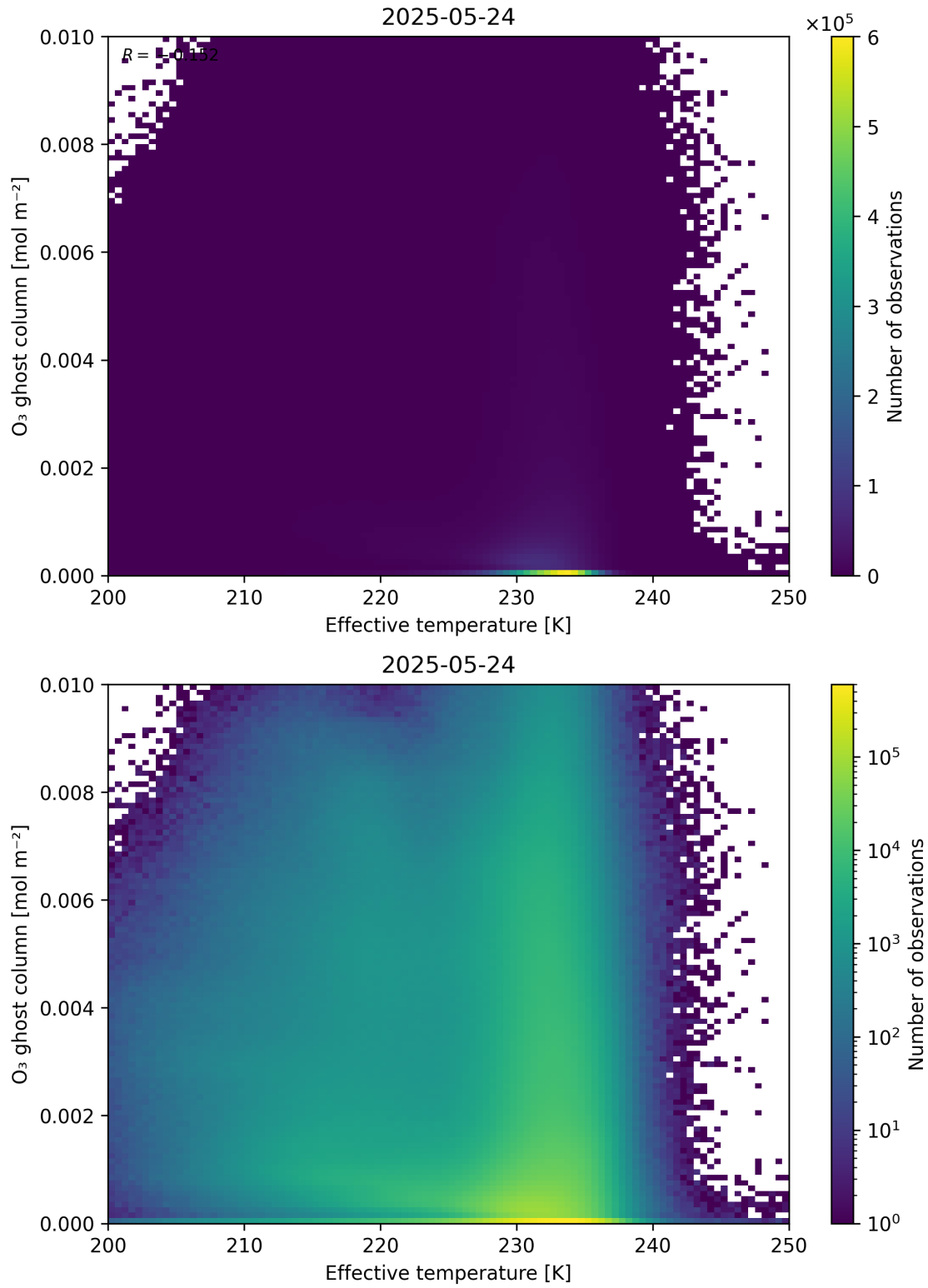
Figure 38: Scatter density plot of “Effective temperature” against “O 3 ghost column” for 2025-05-23 to 2025-05-25.
