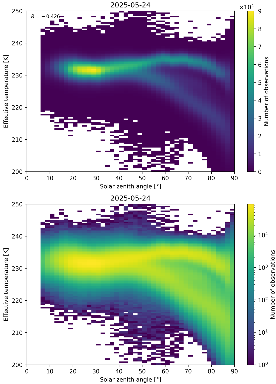
Figure 45: Scatter density plot of “Solar zenith angle” against “Effective temperature” for 2025-05-23 to 2025-05-25.
