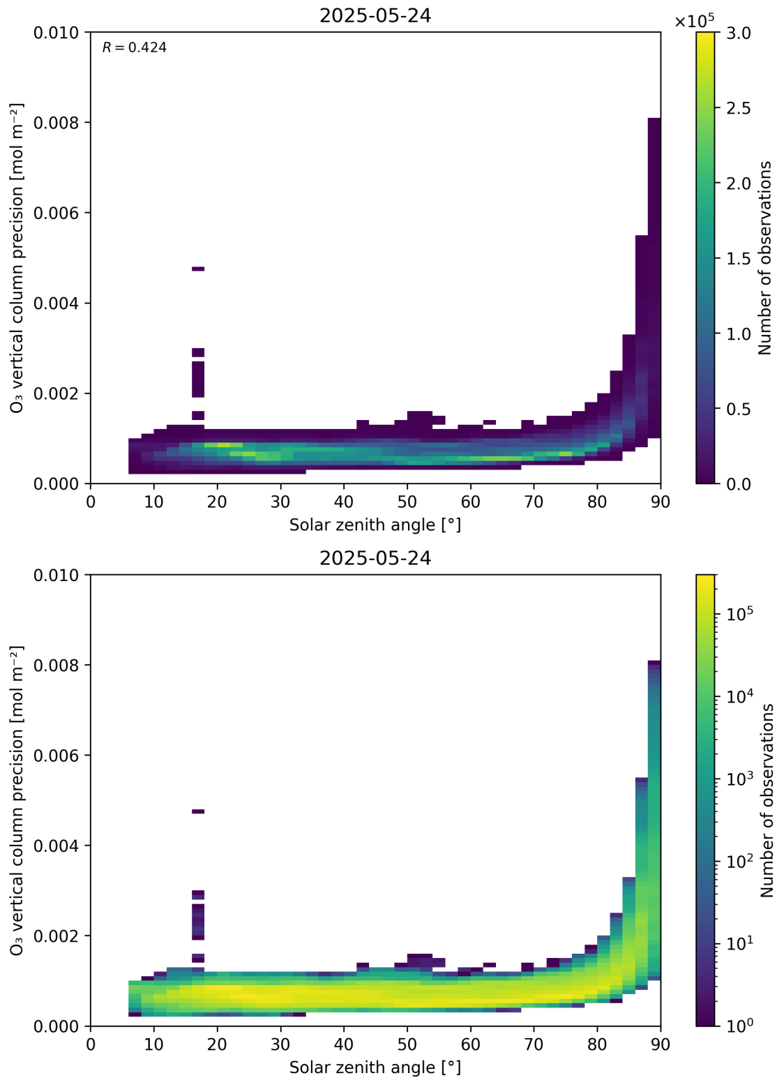
Figure 48: Scatter density plot of “Solar zenith angle” against “O 3 vertical column precision” for 2025-05-23 to 2025-05-25.
