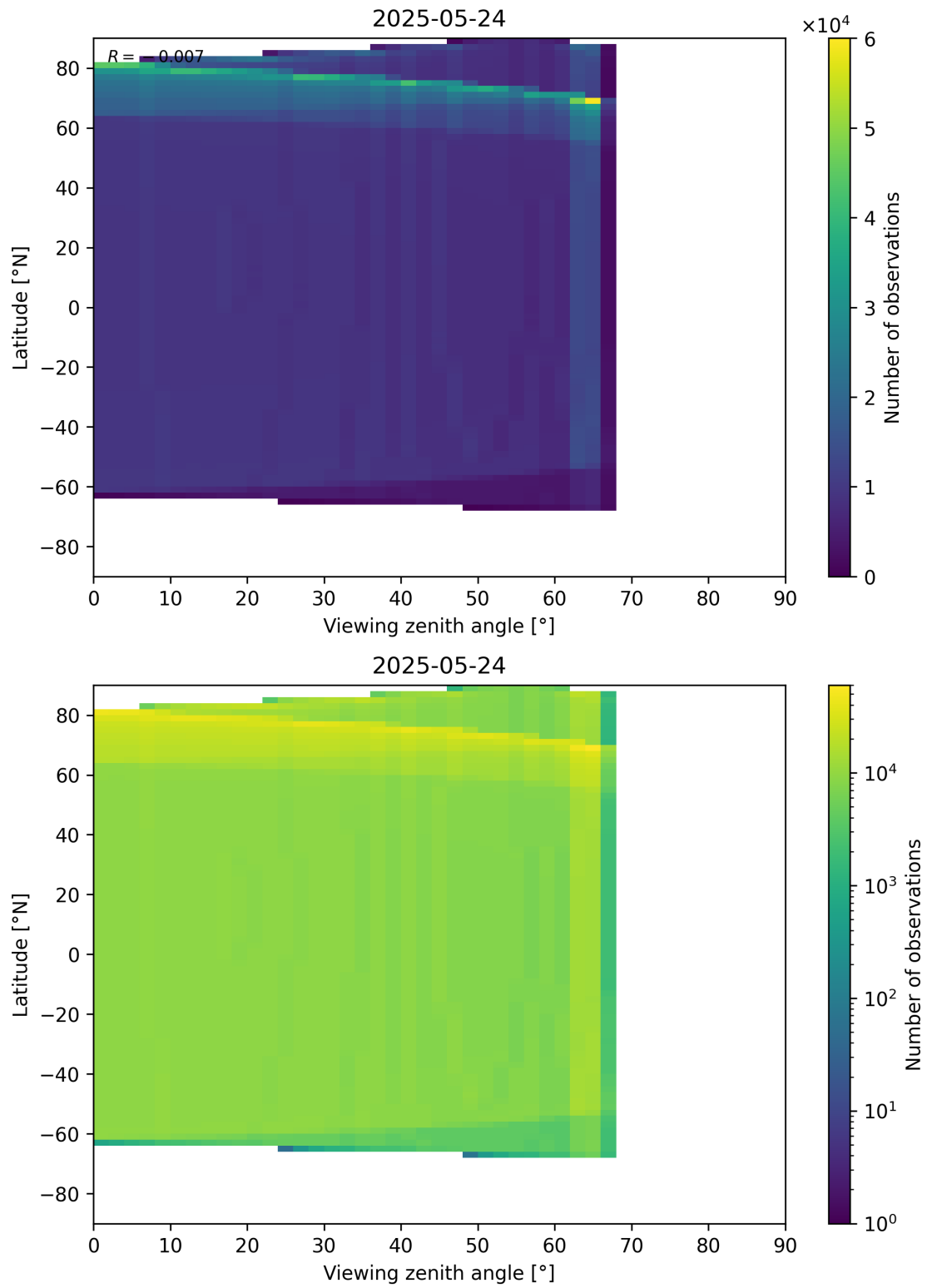
Figure 49: Scatter density plot of “Viewing zenith angle” against “Latitude” for 2025-05-23 to 2025-05-25.
