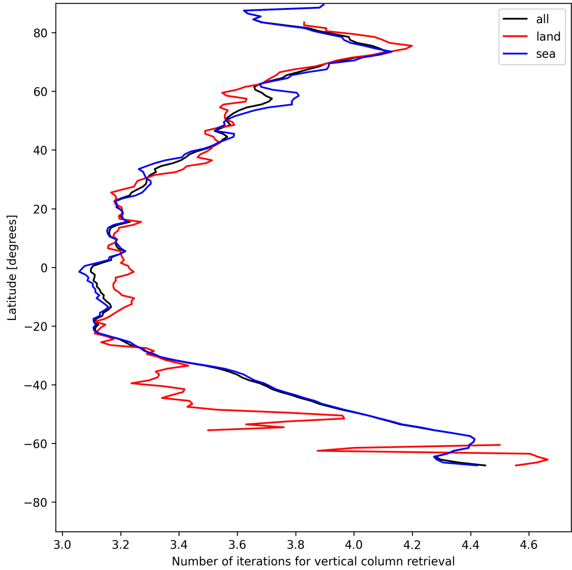
Figure 19: Zonal average of “Number of iterations for vertical column retrieval” for 2025-05-23 to 2025-05-25.
