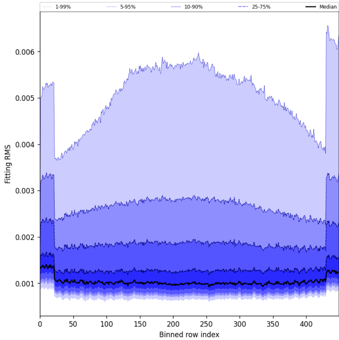
Figure 30: Along track statistics of “Fitting RMS” for 2025-05-23 to 2025-05-25
