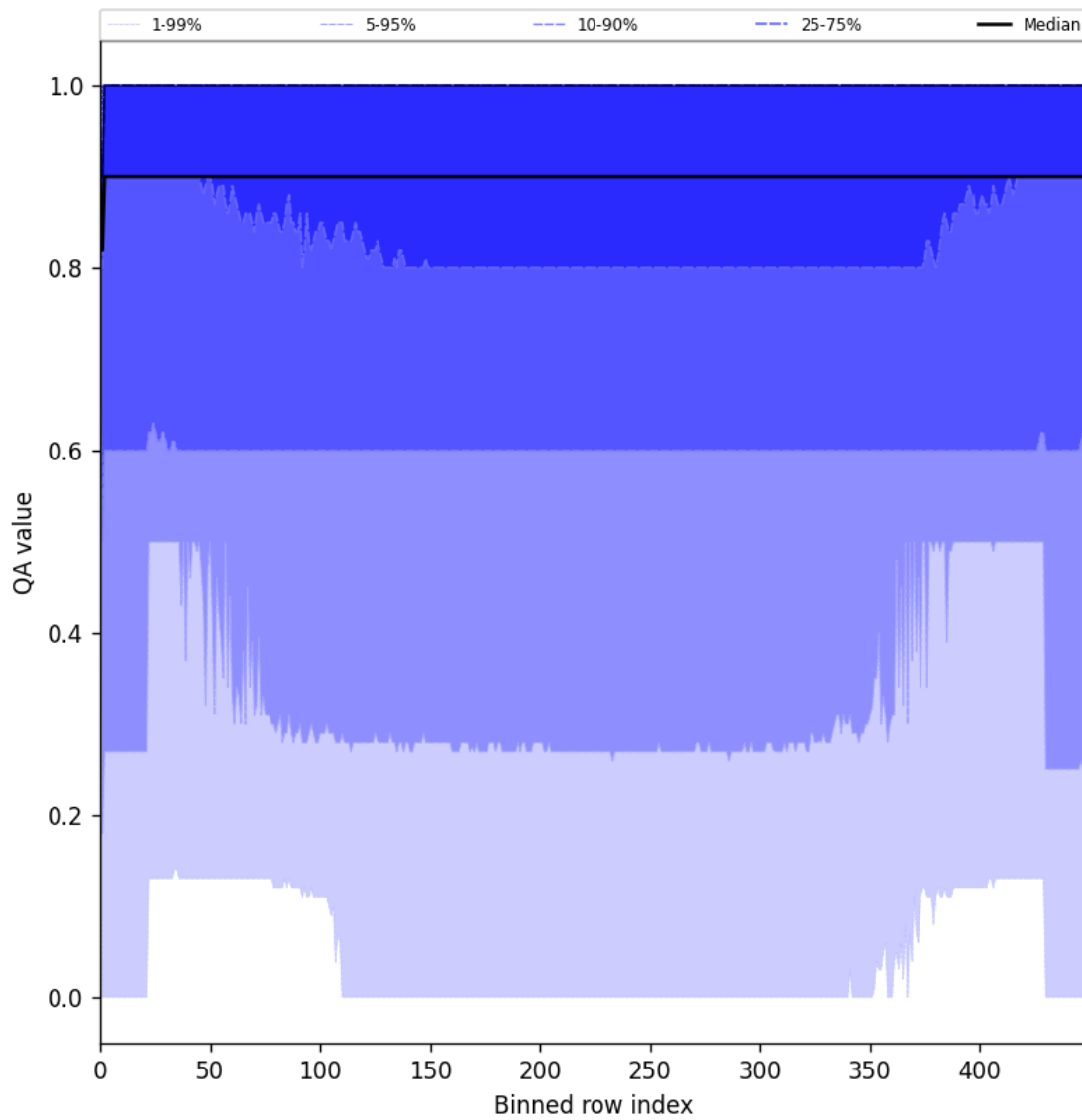
Figure 27: Along track statistics of “QA value” for 2025-05-23 to 2025-05-25
