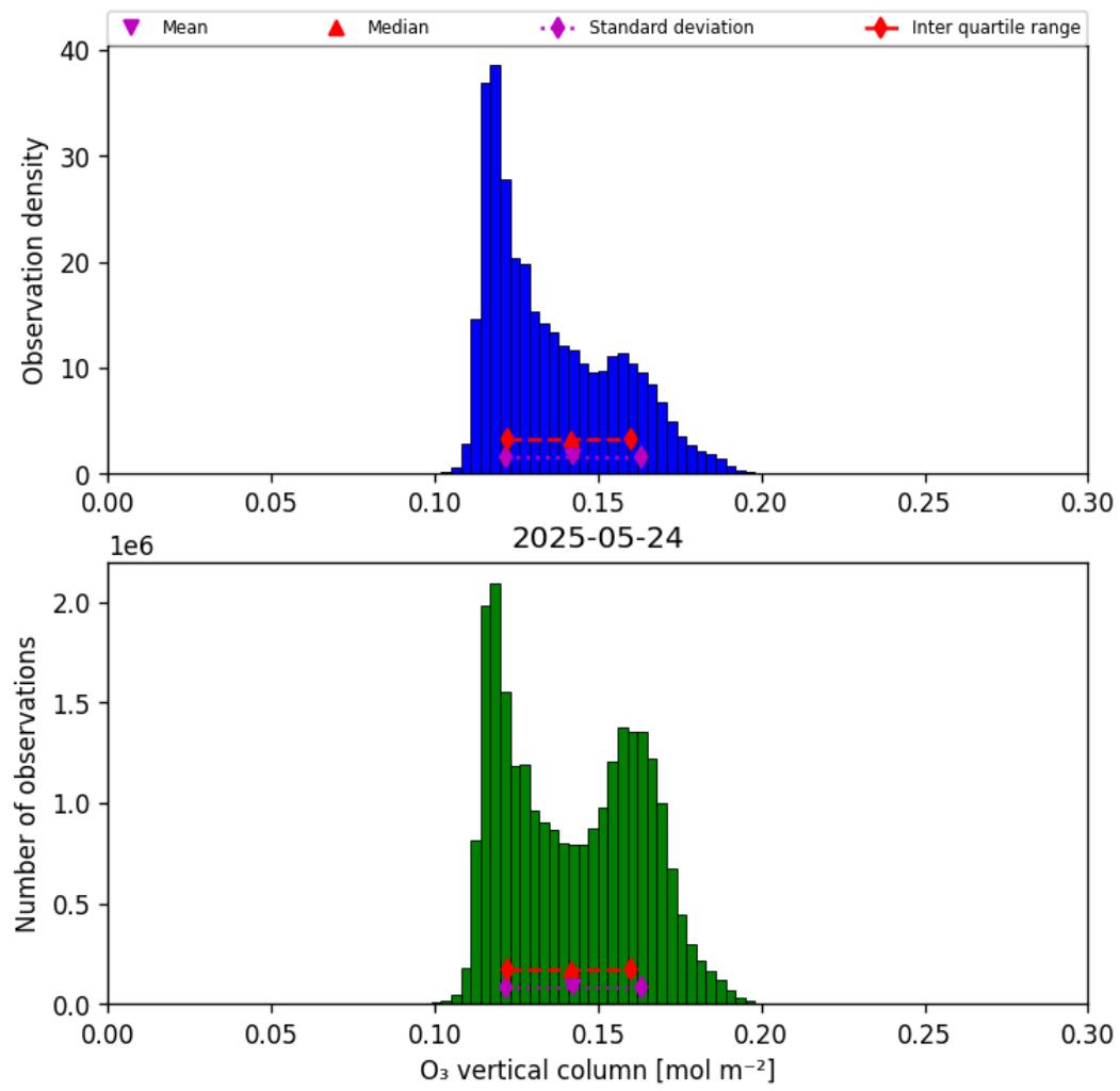
Figure 21: Histogram of “O 3 vertical column” for 2025-05-23 to 2025-05-25
