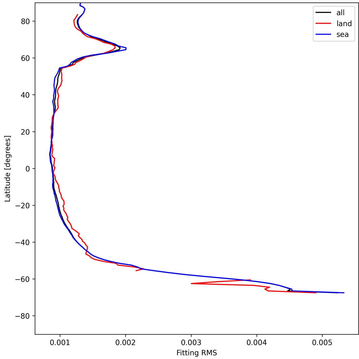
Figure 16: Zonal average of “Fitting RMS” for 2025-05-23 to 2025-05-25.
