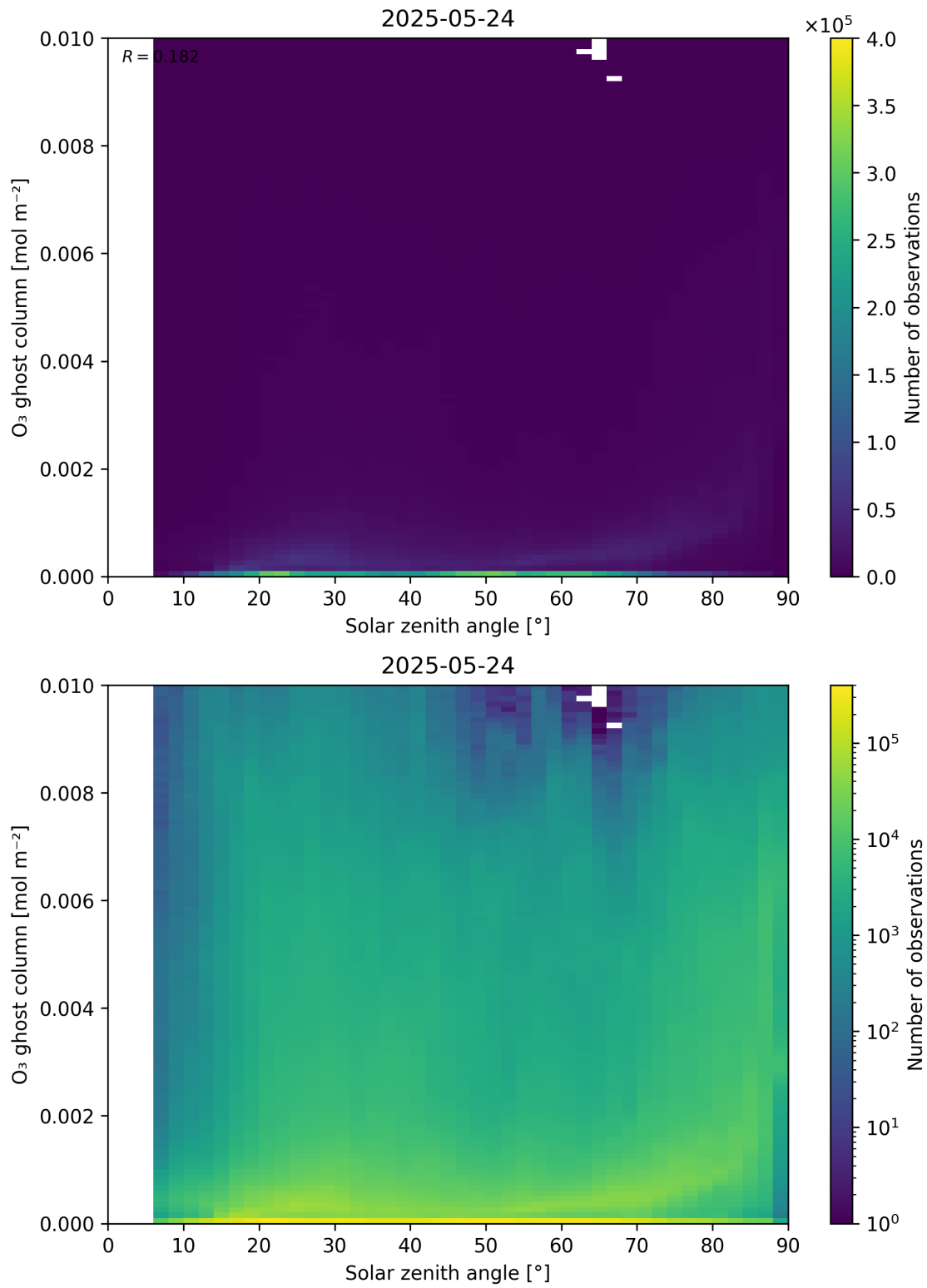
Figure 46: Scatter density plot of “Solar zenith angle” against “O 3 ghost column” for 2025-05-23 to 2025-05-25.
