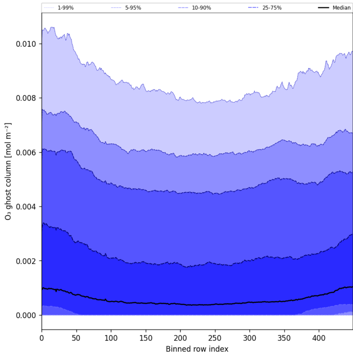
Figure 32: Along track statistics of “O 3 ghost column” for 2025-05-23 to 2025-05-25
