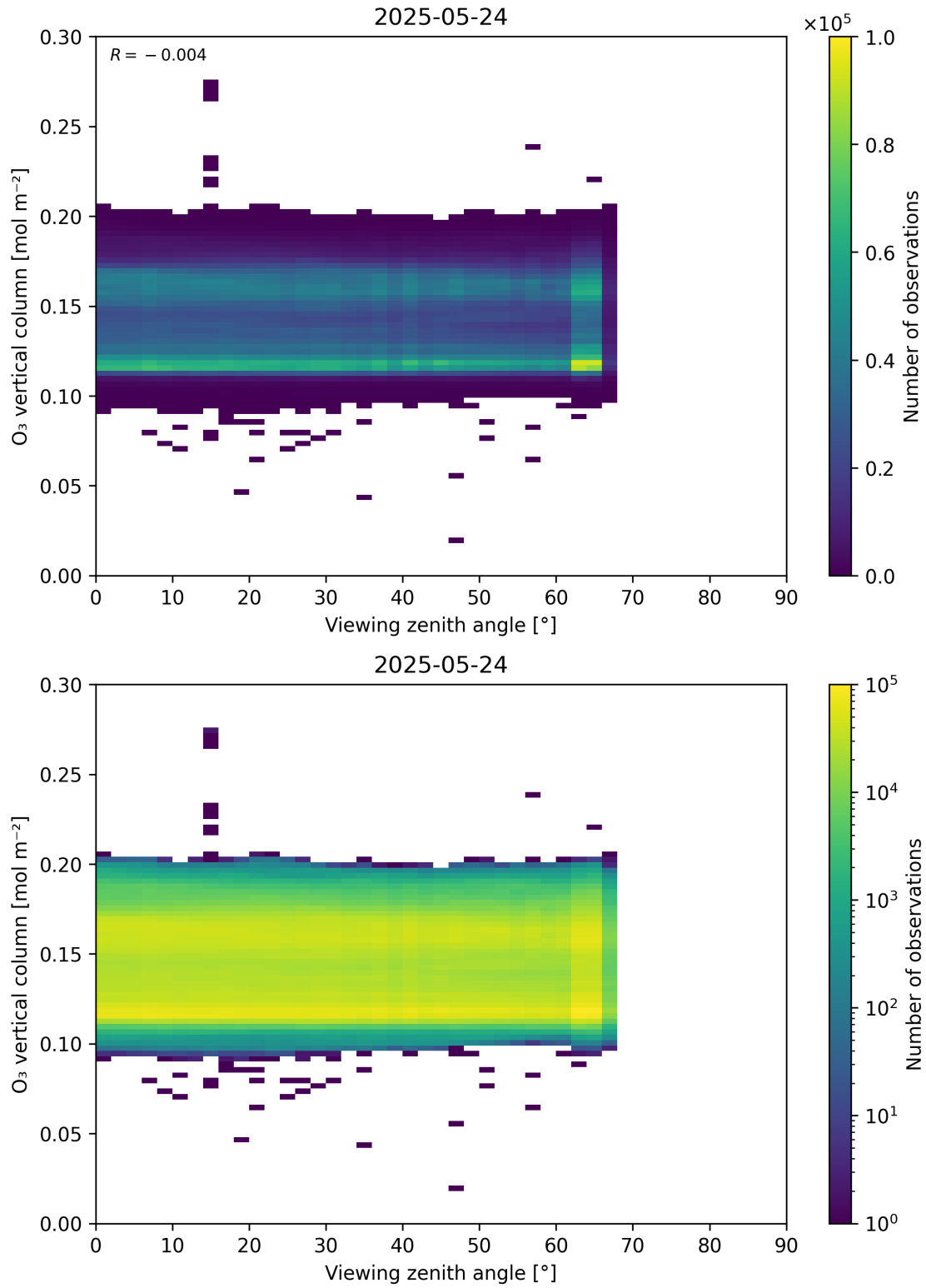
Figure 52: Scatter density plot of “Viewing zenith angle” against “O 3 vertical column” for 2025-05-23 to 2025-05-25.
