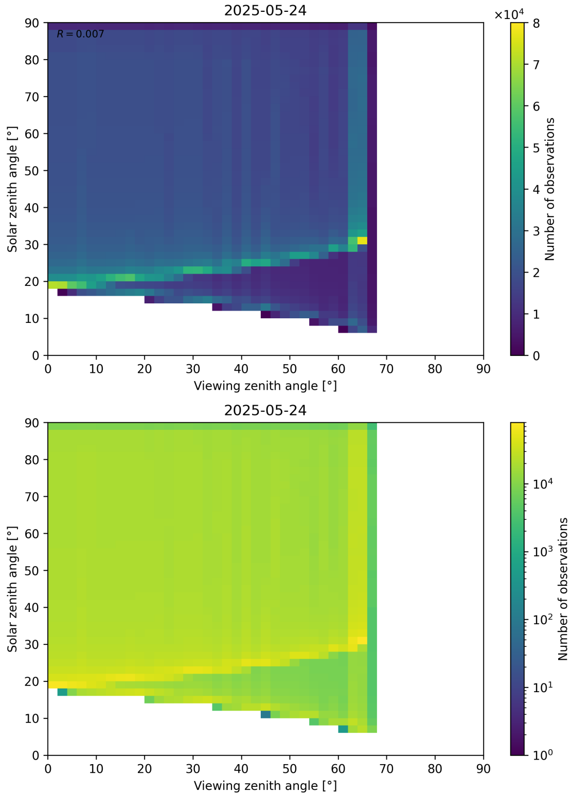
Figure 54: Scatter density plot of “Viewing zenith angle” against “Solar zenith angle” for 2025-05-23 to 2025-05-25.
