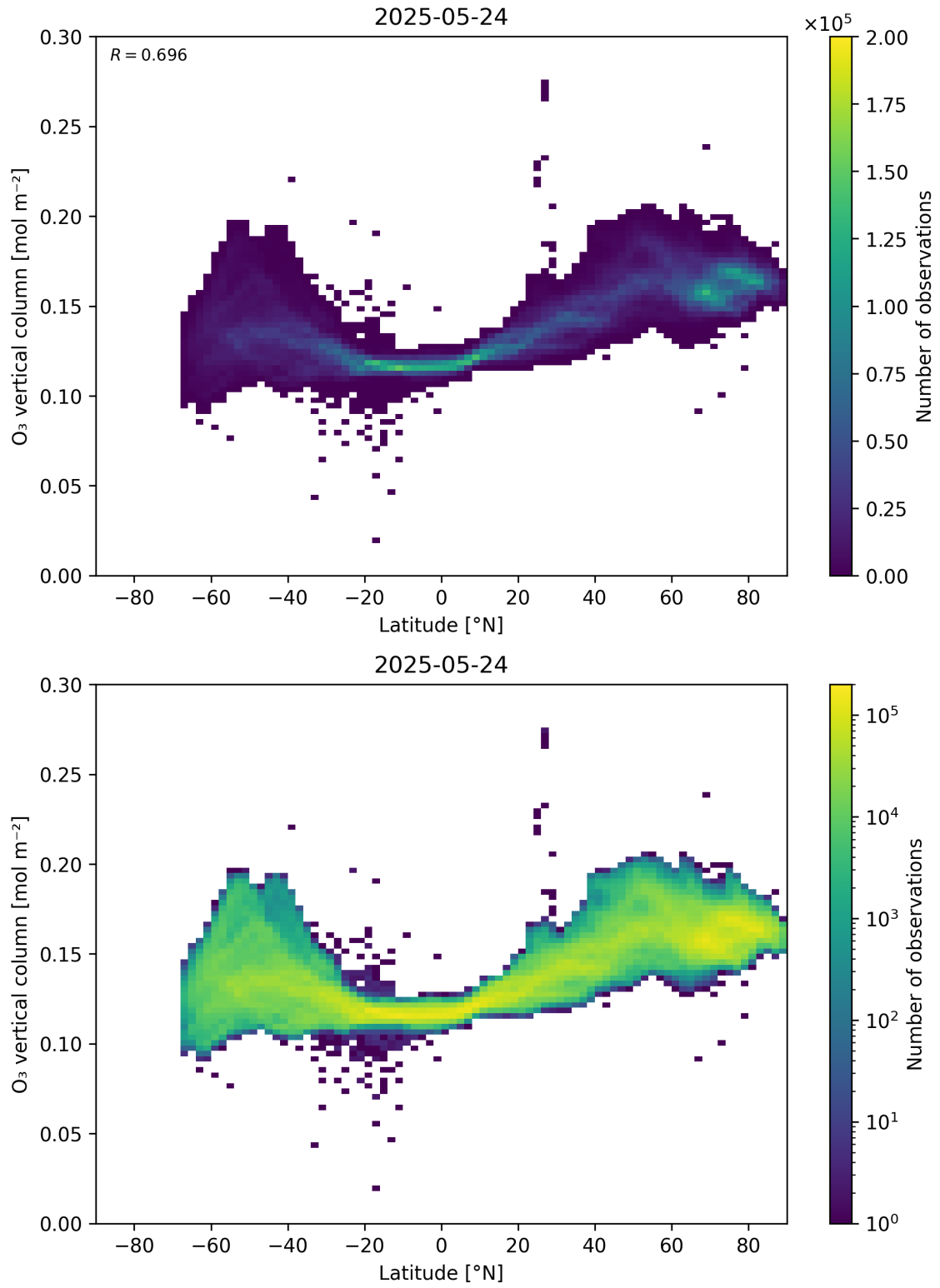
Figure 36: Scatter density plot of “Latitude” against “O 3 vertical column” for 2025-05-23 to 2025-05-25.
