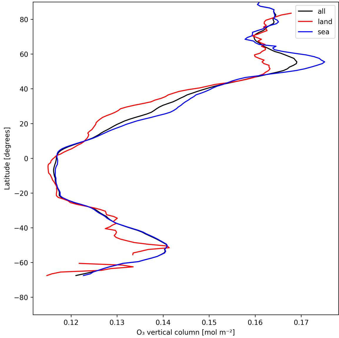
Figure 14: Zonal average of “O 3 vertical column” for 2025-05-23 to 2025-05-25.
