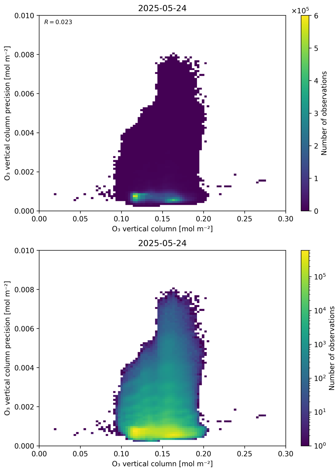
Figure 41: Scatter density plot of “O 3 vertical column” against “O 3 vertical column precision” for 2025-05-23 to 2025-05-25.
