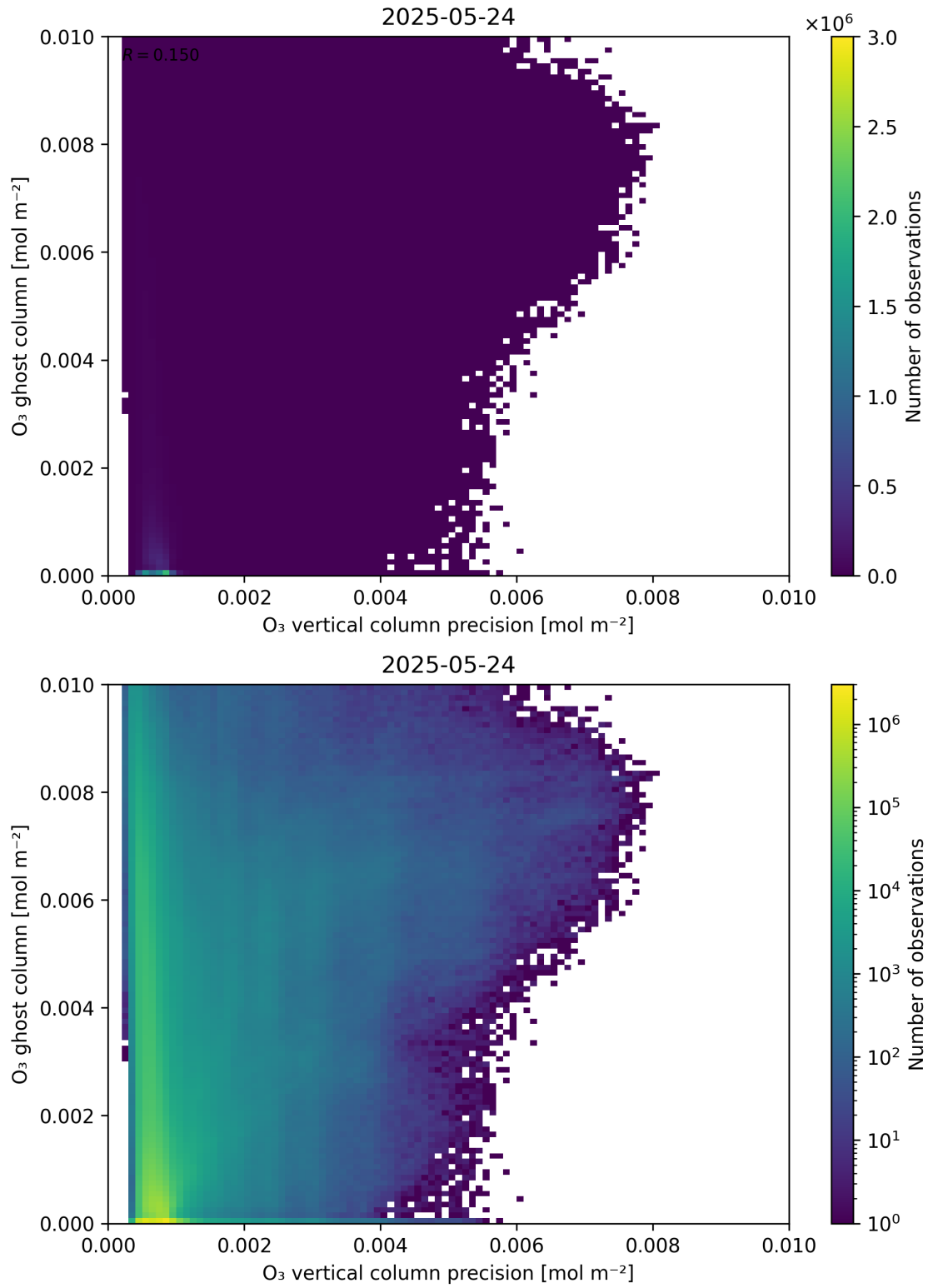
Figure 43: Scatter density plot of “ \text{O}_3 vertical column precision” against “ \text{O}_3 ghost column” for 2025-05-23 to 2025-05-25.
