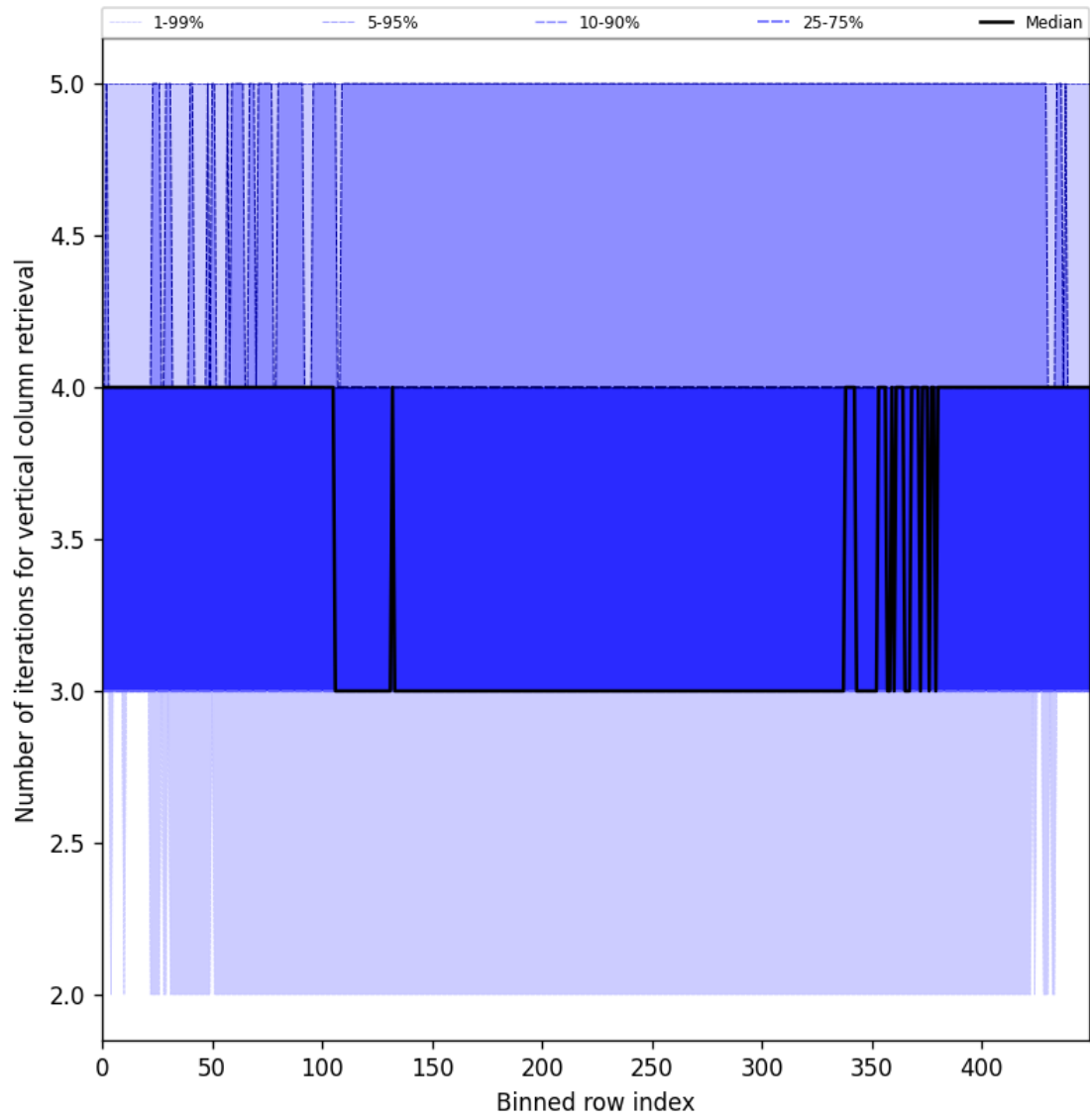
Figure 33: Along track statistics of “Number of iterations for vertical column retrieval” for 2025-05-23 to 2025-05-25
