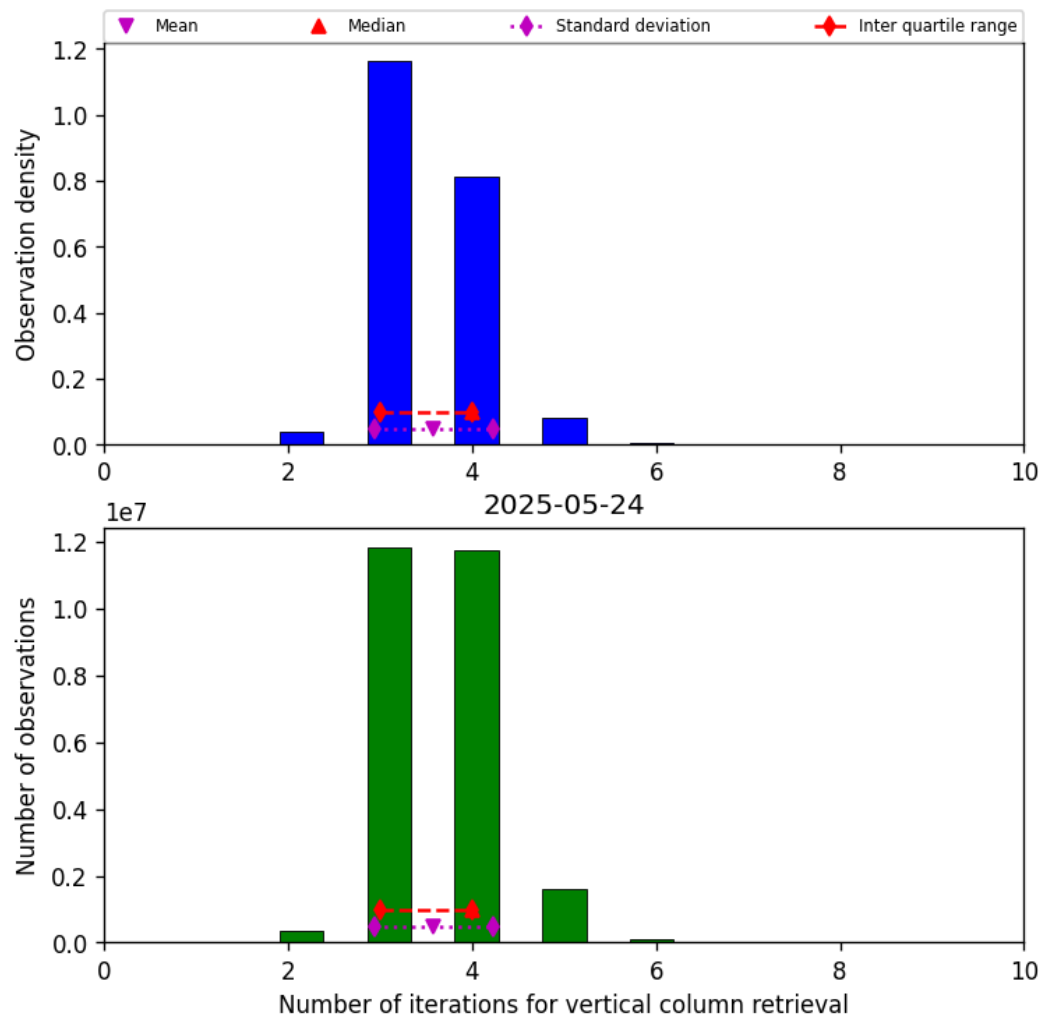
Figure 26: Histogram of “Number of iterations for vertical column retrieval” for 2025-05-23 to 2025-05-25
