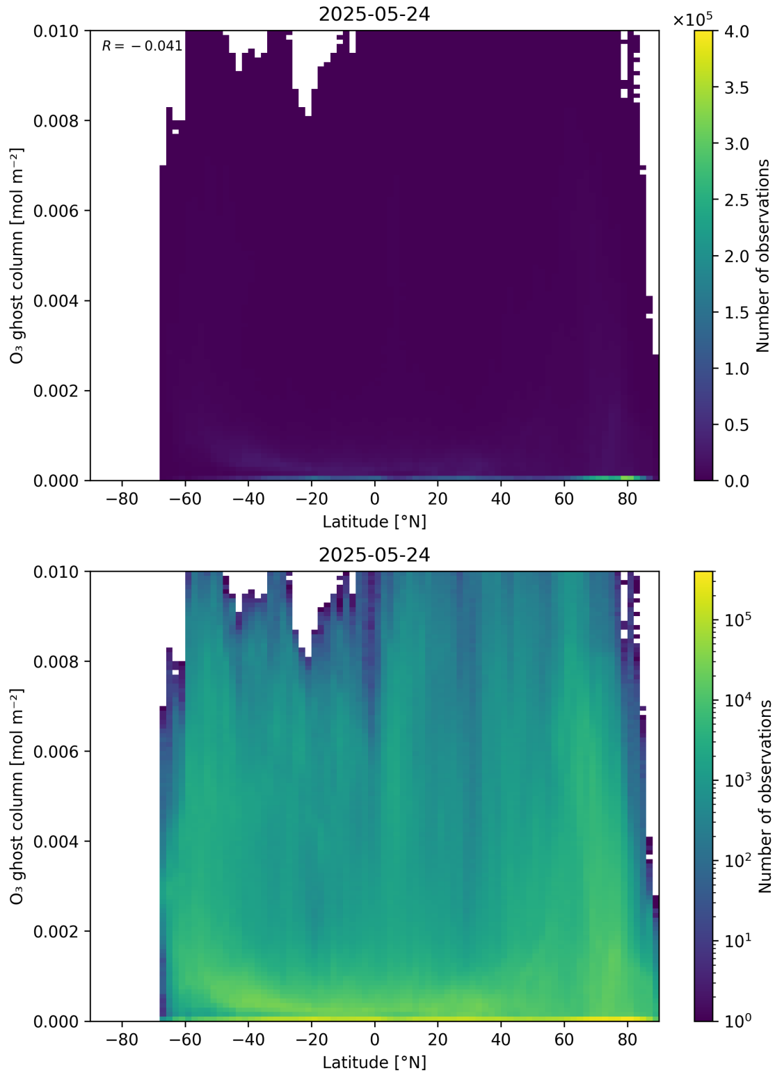
Figure 35: Scatter density plot of “Latitude” against “O 3 ghost column” for 2025-05-23 to 2025-05-25.
