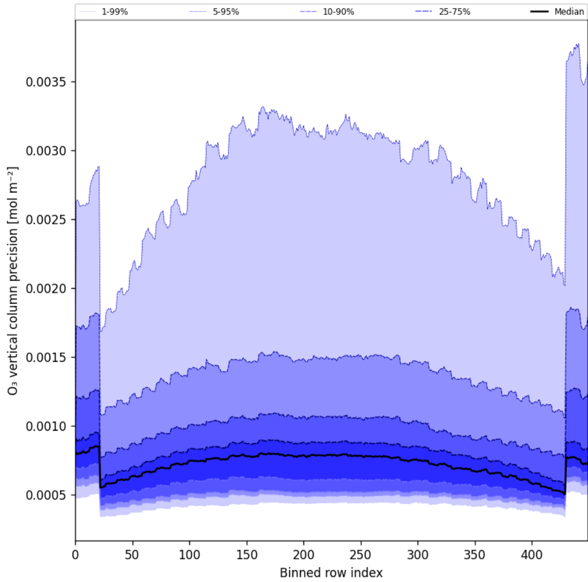
Figure 29: Along track statistics of “O 3 vertical column precision” for 2025-05-23 to 2025-05-25
