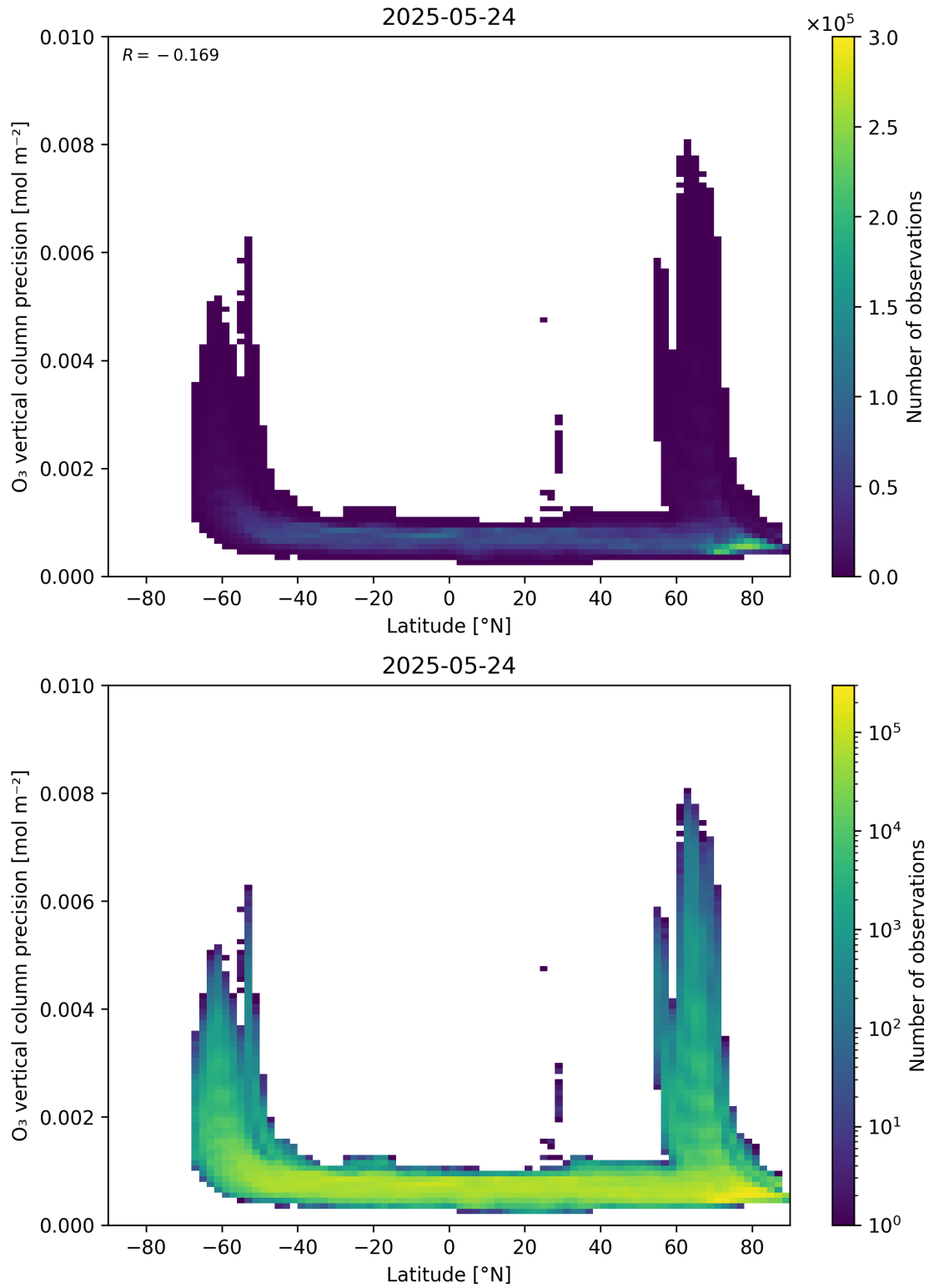
Figure 37: Scatter density plot of “Latitude” against “O 3 vertical column precision” for 2025-05-23 to 2025-05-25.
