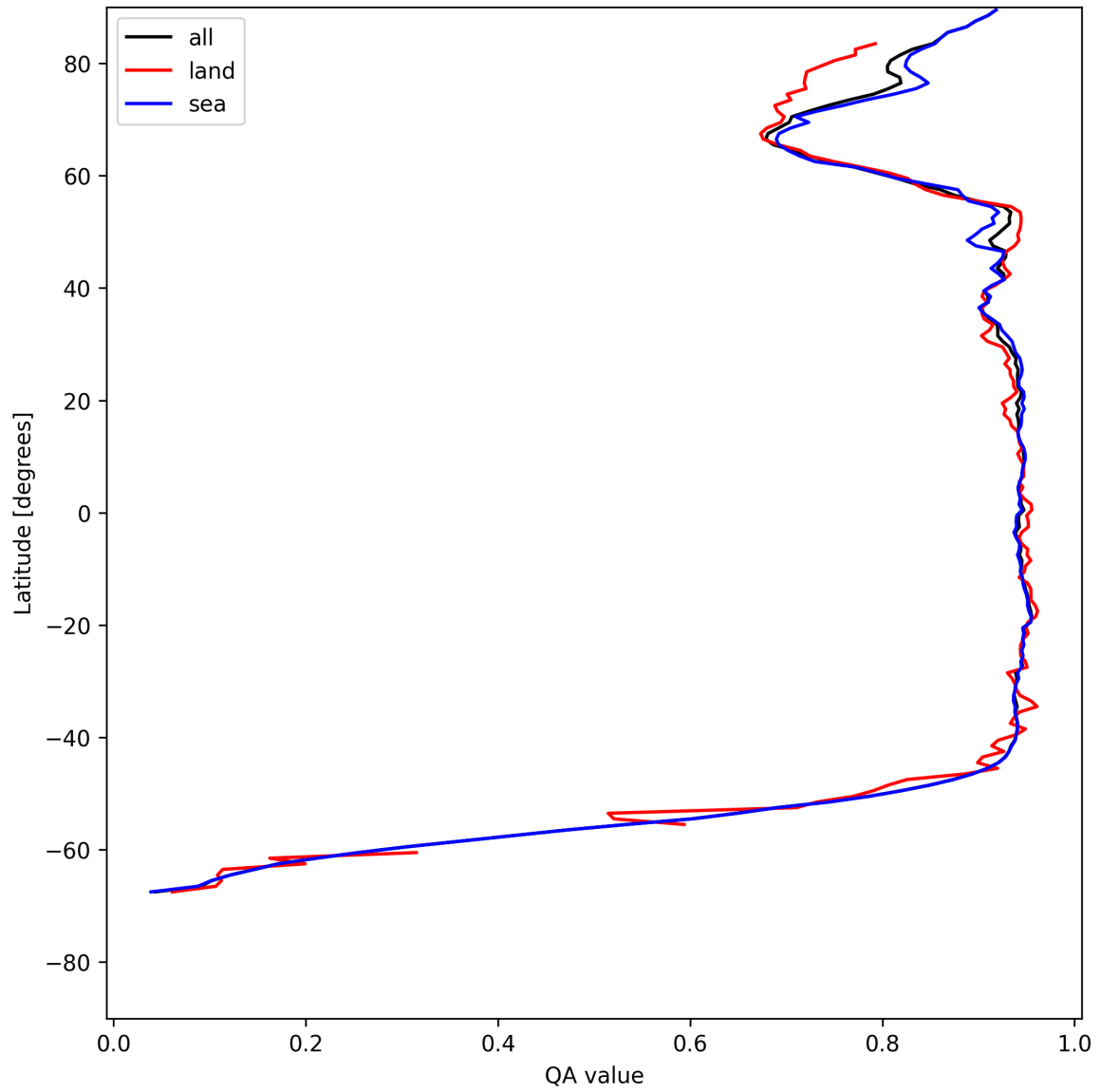
Figure 13: Zonal average of “QA value” for 2025-05-23 to 2025-05-25.
