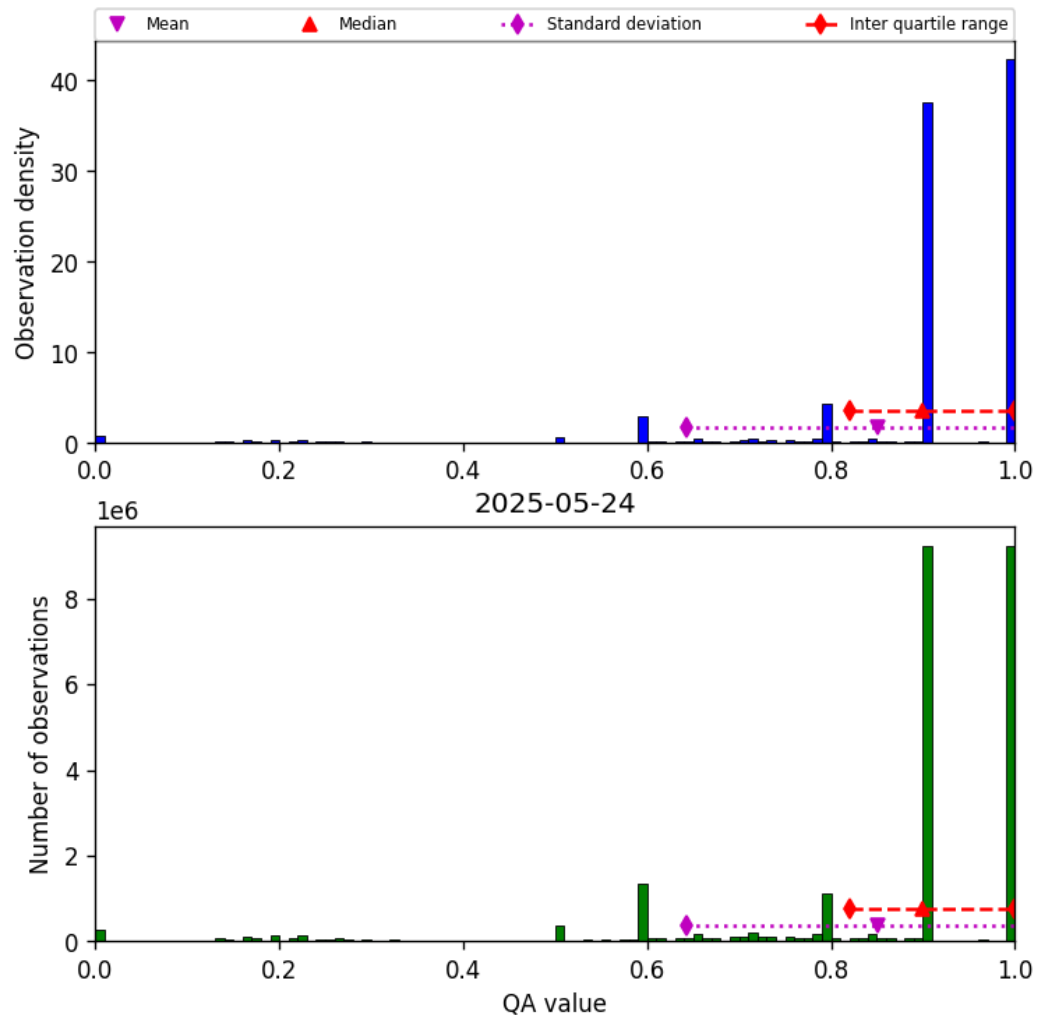
Figure 20: Histogram of “QA value” for 2025-05-23 to 2025-05-25
