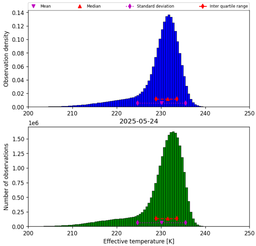
Figure 24: Histogram of “Effective temperature” for 2025-05-23 to 2025-05-25
