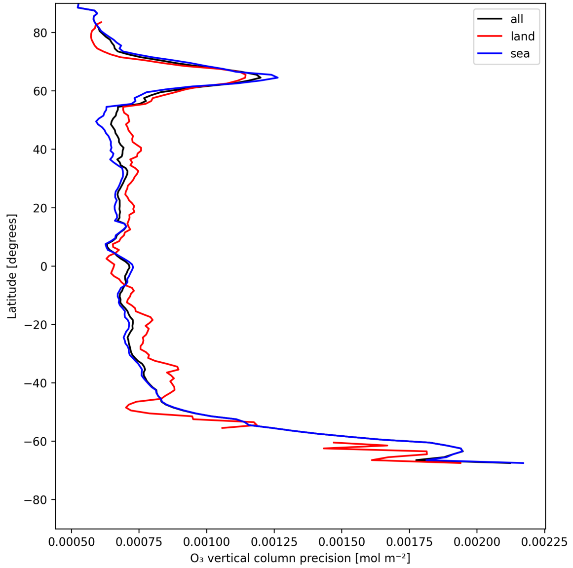
Figure 15: Zonal average of “O 3 vertical column precision” for 2025-05-23 to 2025-05-25.
