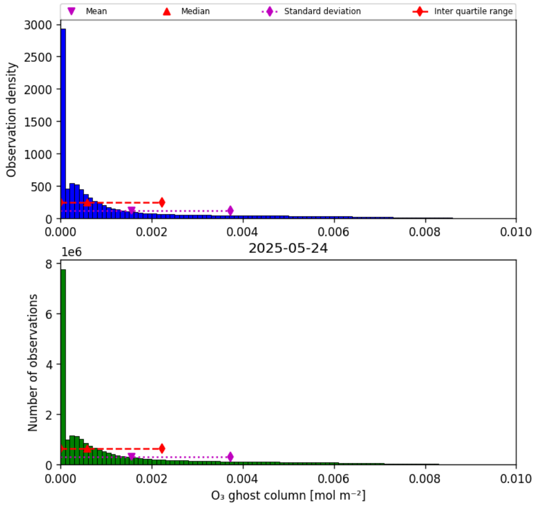
Figure 25: Histogram of “O 3 ghost column” for 2025-05-23 to 2025-05-25
