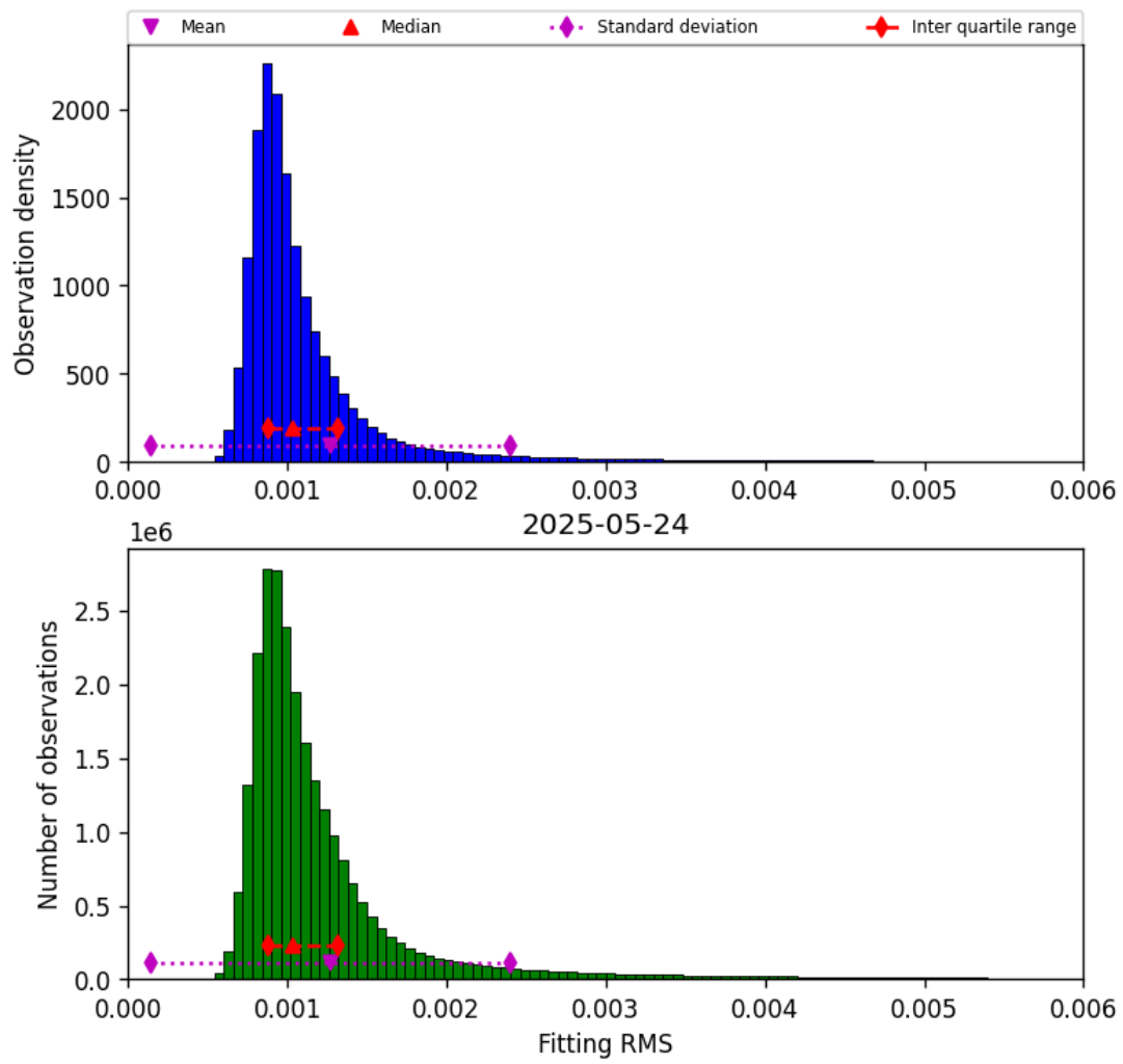
Figure 23: Histogram of “Fitting RMS” for 2025-05-23 to 2025-05-25
