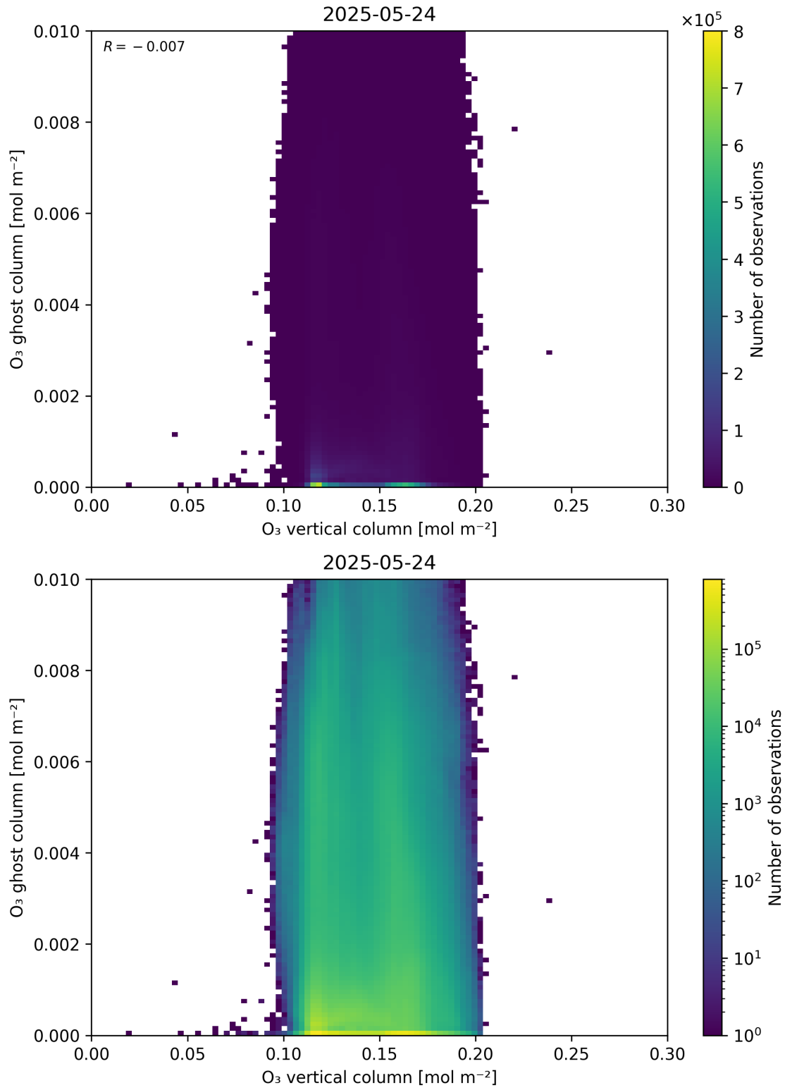
Figure 40: Scatter density plot of “O 3 vertical column” against “O 3 ghost column” for 2025-05-23 to 2025-05-25.
