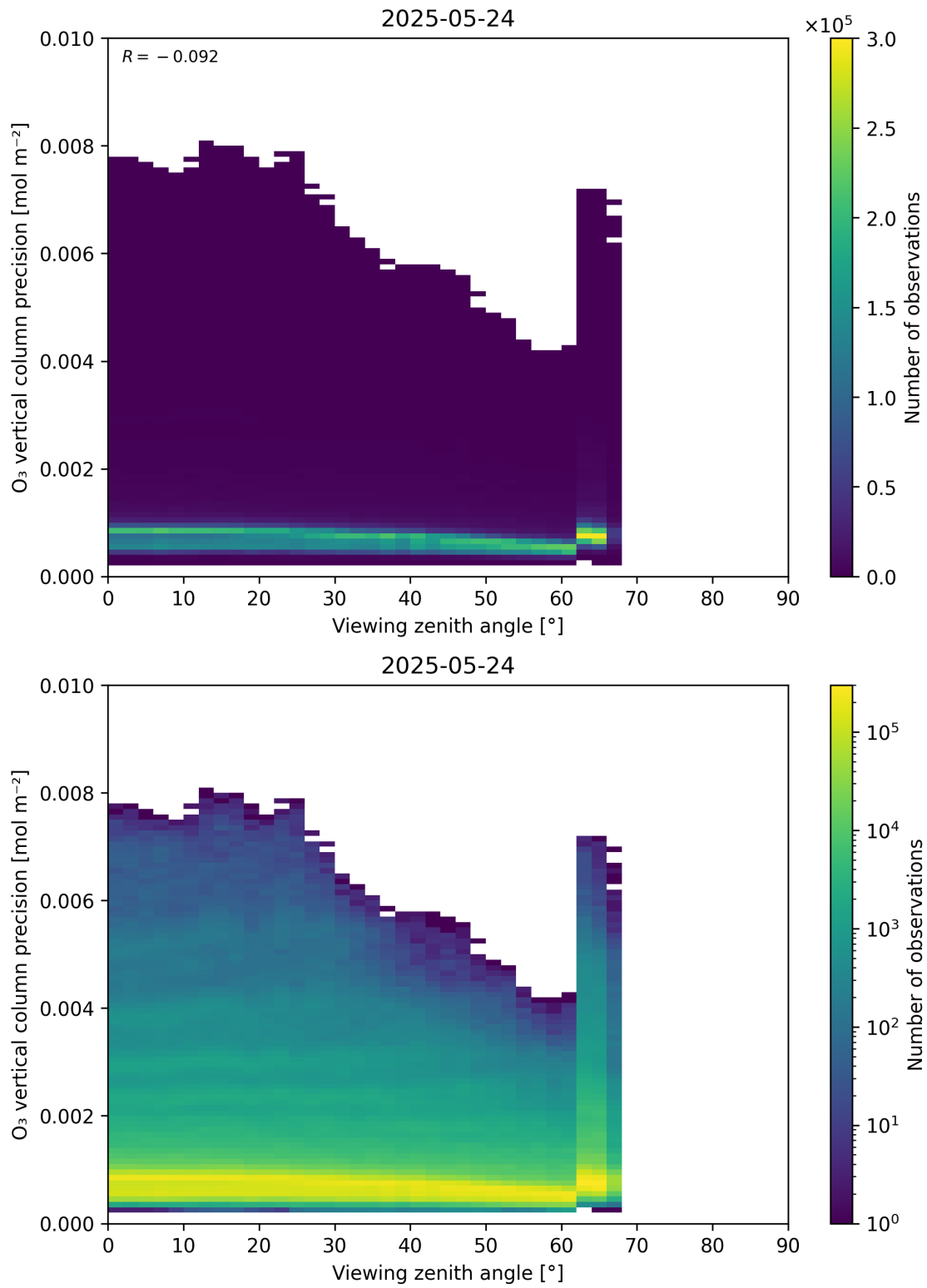
Figure 53: Scatter density plot of “Viewing zenith angle” against “O 3 vertical column precision” for 2025-05-23 to 2025-05-25.
