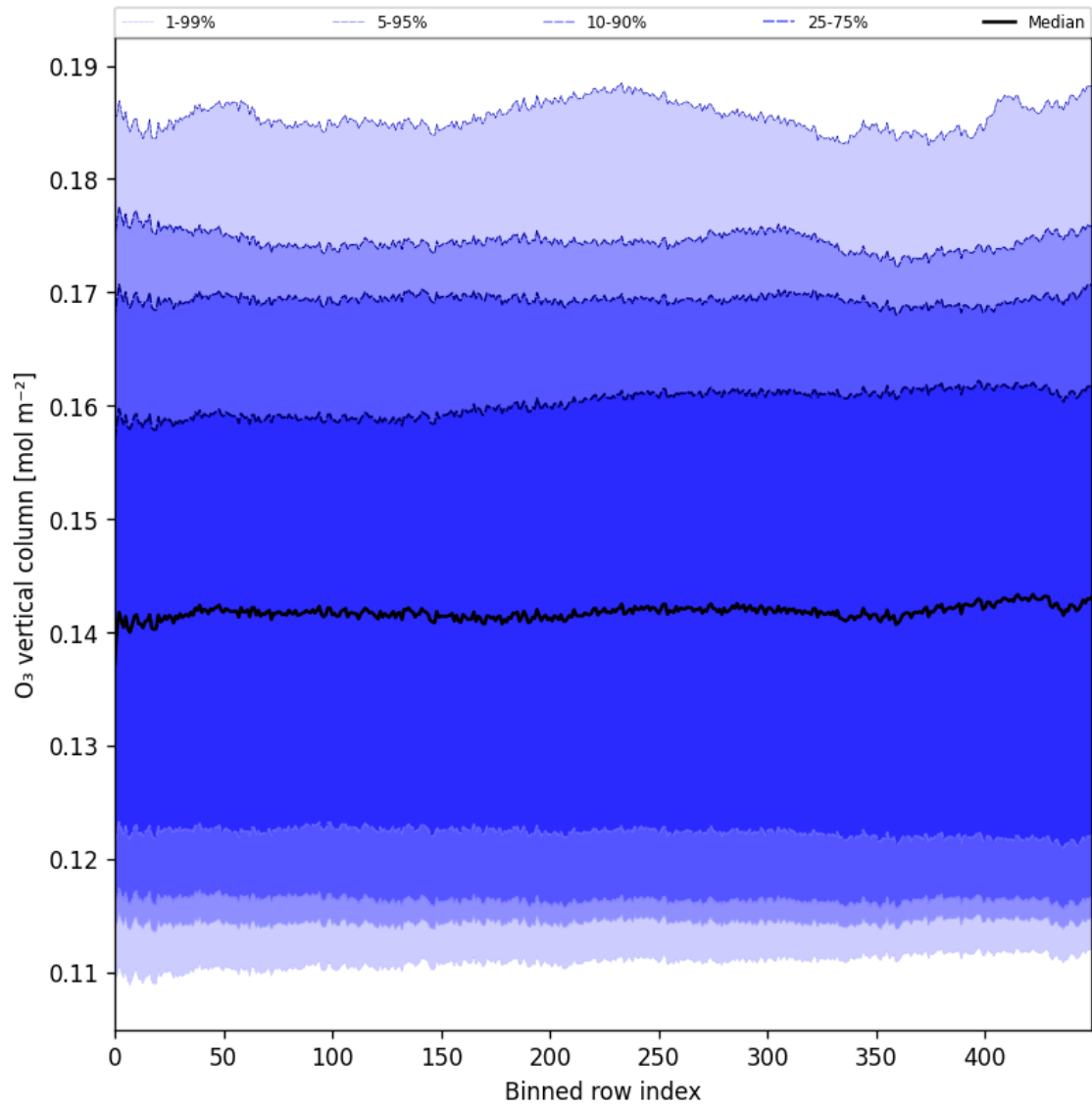
Figure 28: Along track statistics of “ \text{O}_3 vertical column” for 2025-05-23 to 2025-05-25
