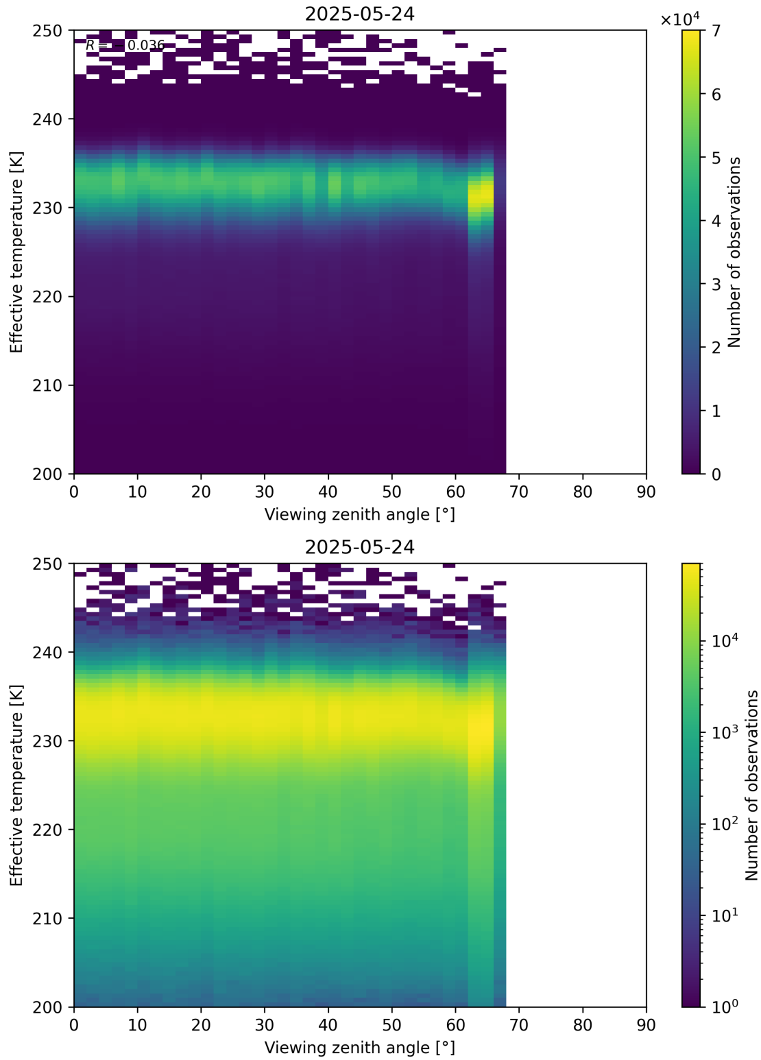
Figure 50: Scatter density plot of “Viewing zenith angle” against “Effective temperature” for 2025-05-23 to 2025-05-25.
