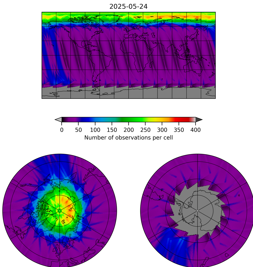
Figure 12: Map of the number of observations for 2025-05-23 to 2025-05-25
