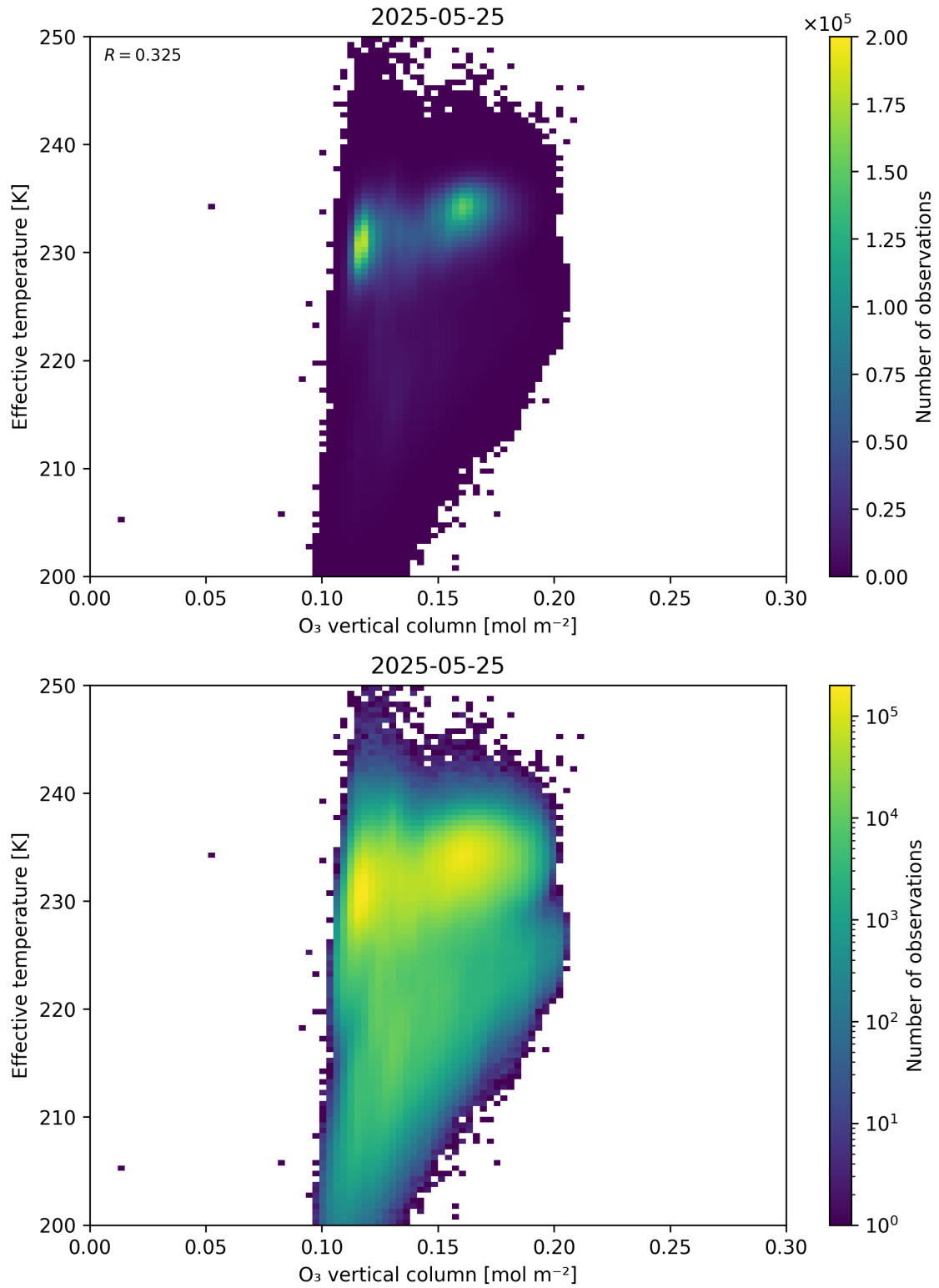
Figure 39: Scatter density plot of “O 3 vertical column” against “Effective temperature” for 2025-05-24 to 2025-05-26.
