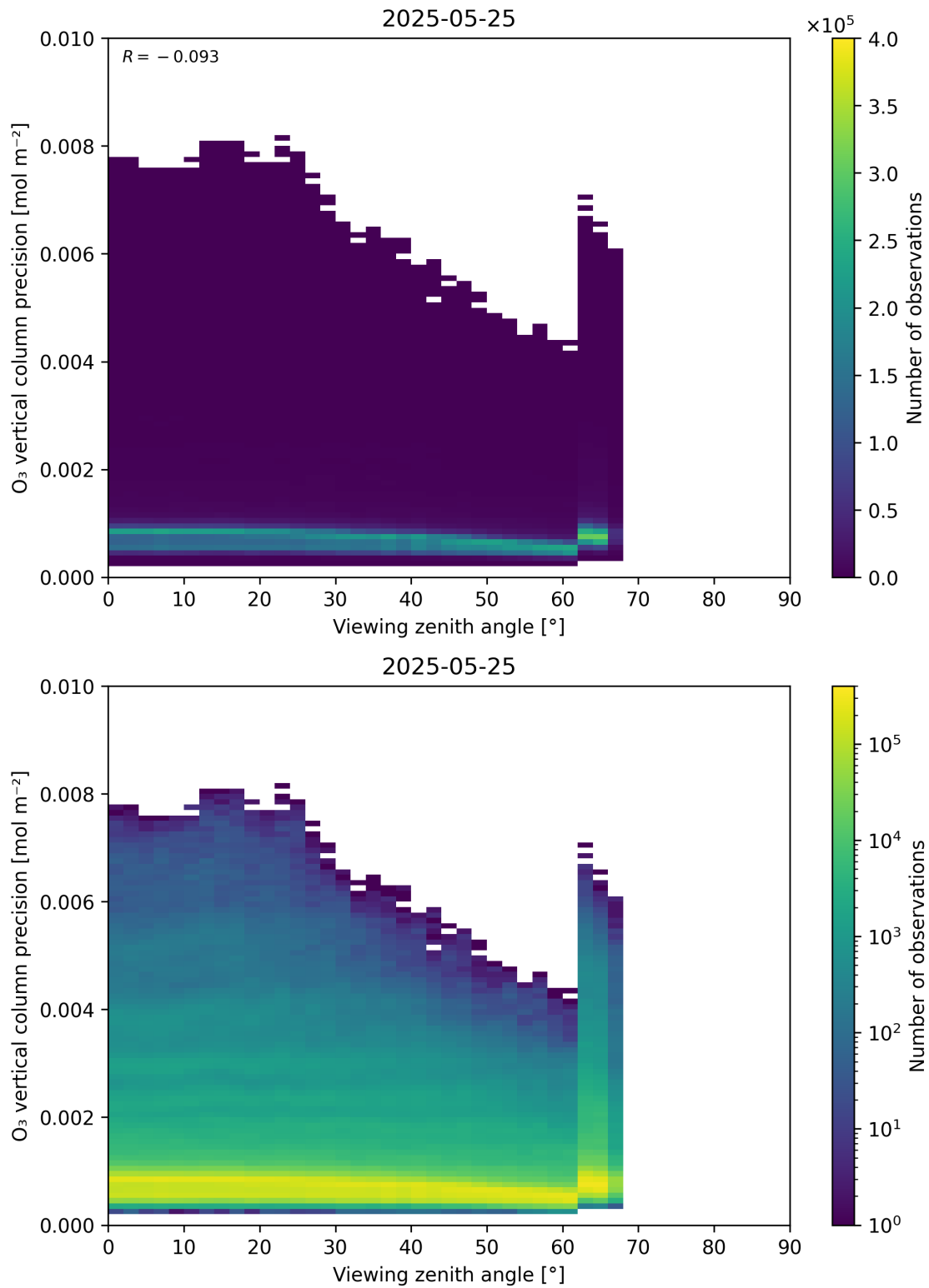
Figure 53: Scatter density plot of “Viewing zenith angle” against “O 3 vertical column precision” for 2025-05-24 to 2025-05-26.
