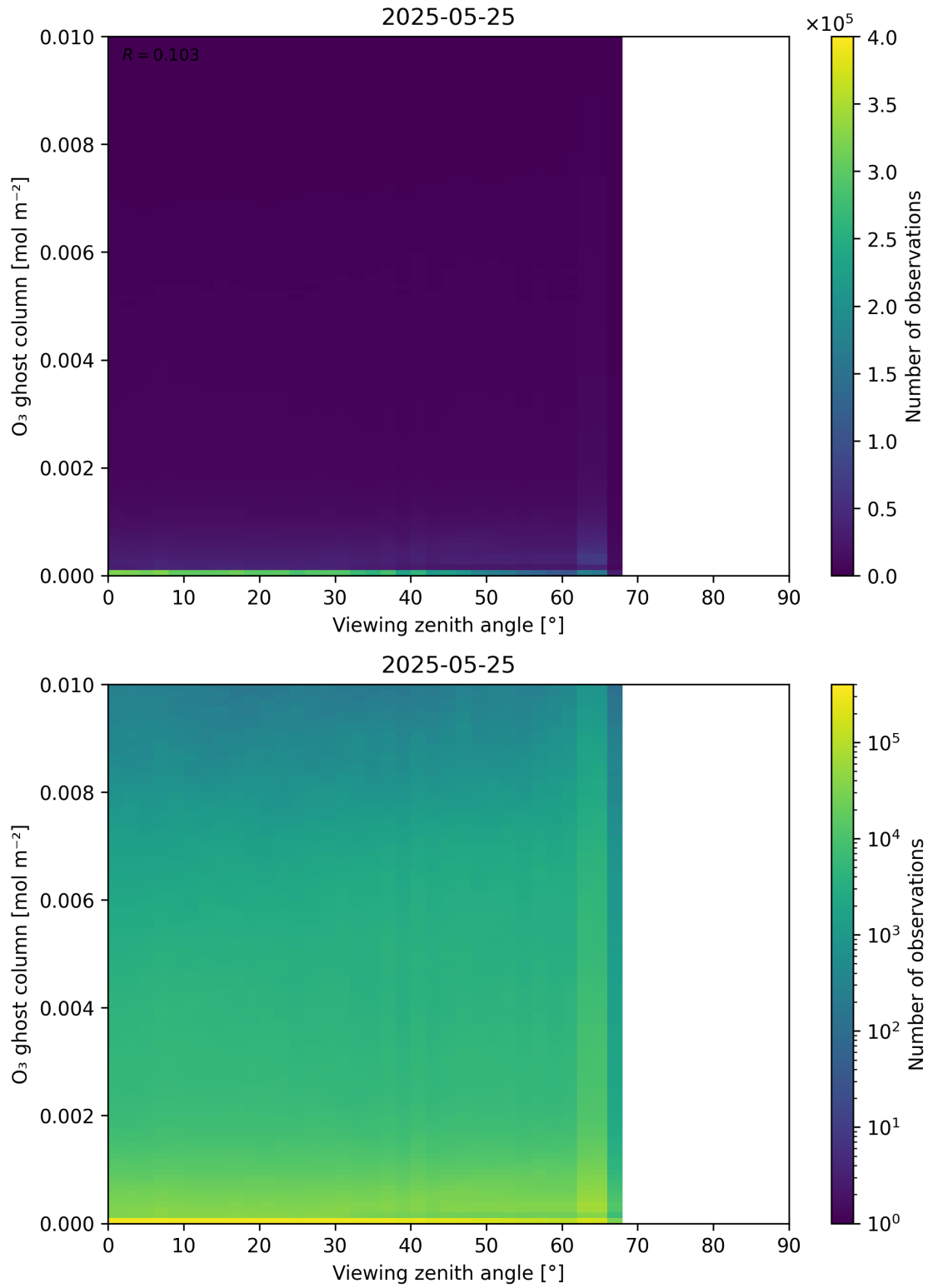
Figure 51: Scatter density plot of “Viewing zenith angle” against “O 3 ghost column” for 2025-05-24 to 2025-05-26.
