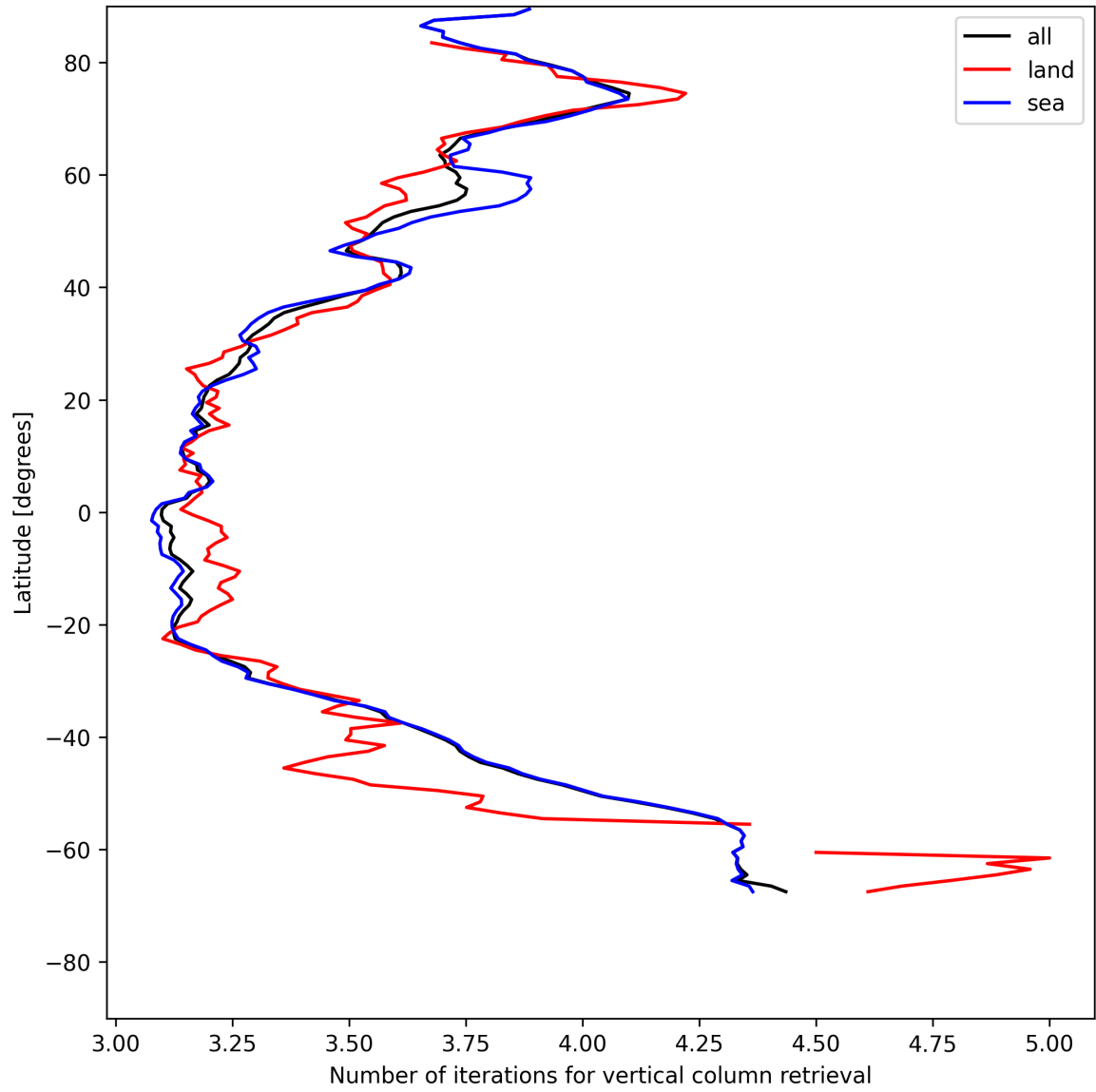
Figure 19: Zonal average of “Number of iterations for vertical column retrieval” for 2025-05-24 to 2025-05-26.
