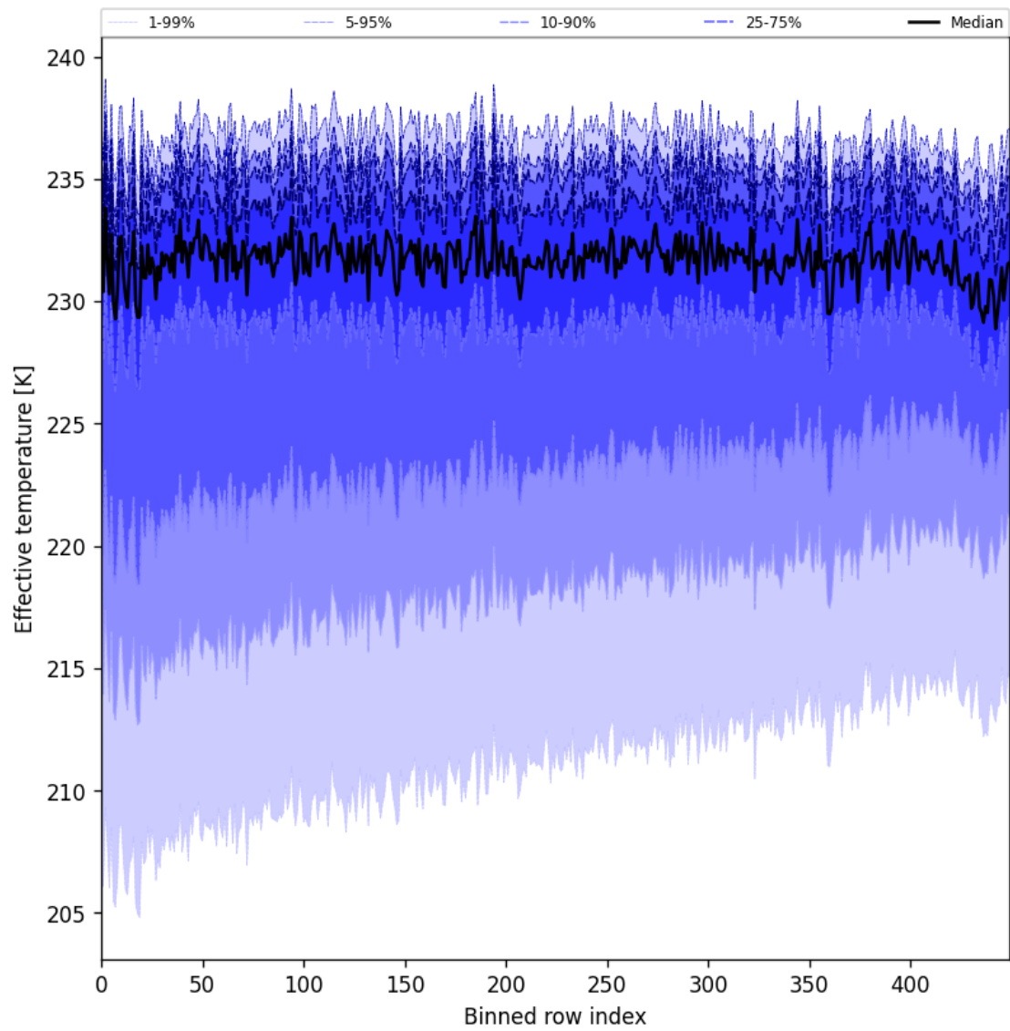
Figure 31: Along track statistics of “Effective temperature” for 2025-05-24 to 2025-05-26
