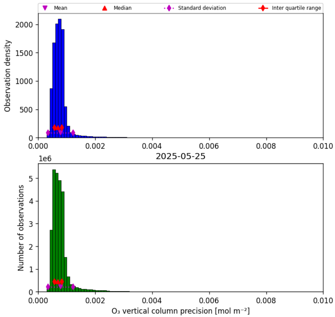
Figure 22: Histogram of “O 3 vertical column precision” for 2025-05-24 to 2025-05-26
