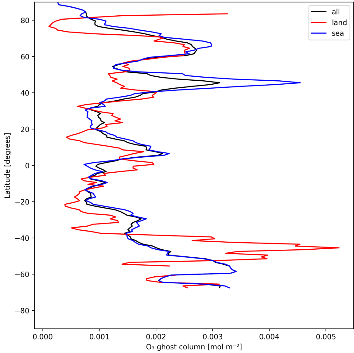
Figure 18: Zonal average of “O 3 ghost column” for 2025-05-24 to 2025-05-26.
