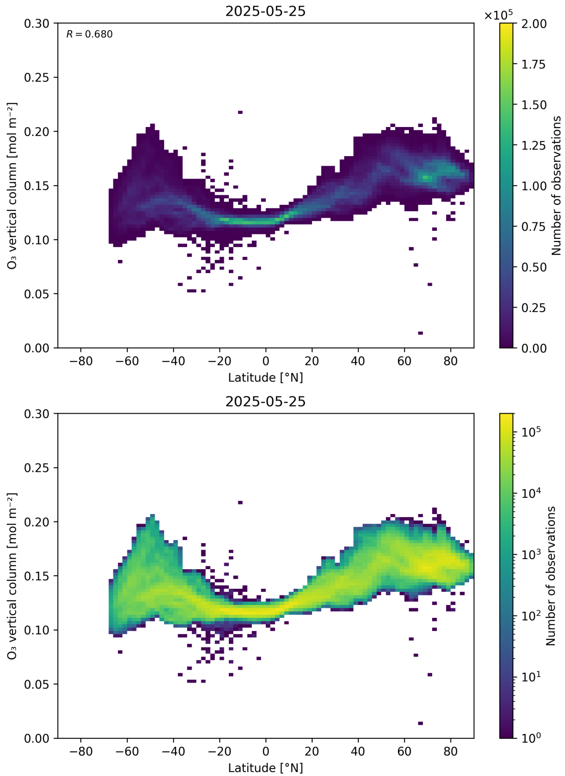
Figure 36: Scatter density plot of “Latitude” against “O 3 vertical column” for 2025-05-24 to 2025-05-26.
