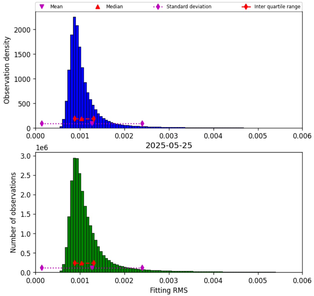
Figure 23: Histogram of “Fitting RMS” for 2025-05-24 to 2025-05-26
