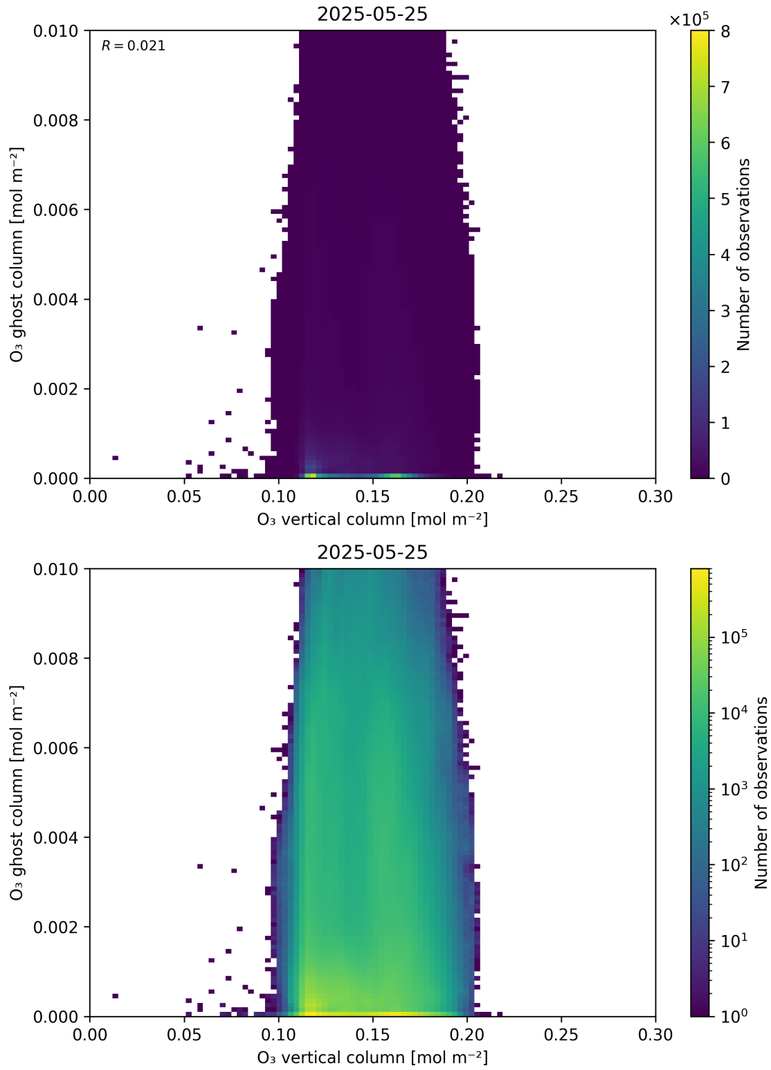
Figure 40: Scatter density plot of “O 3 vertical column” against “O 3 ghost column” for 2025-05-24 to 2025-05-26.
