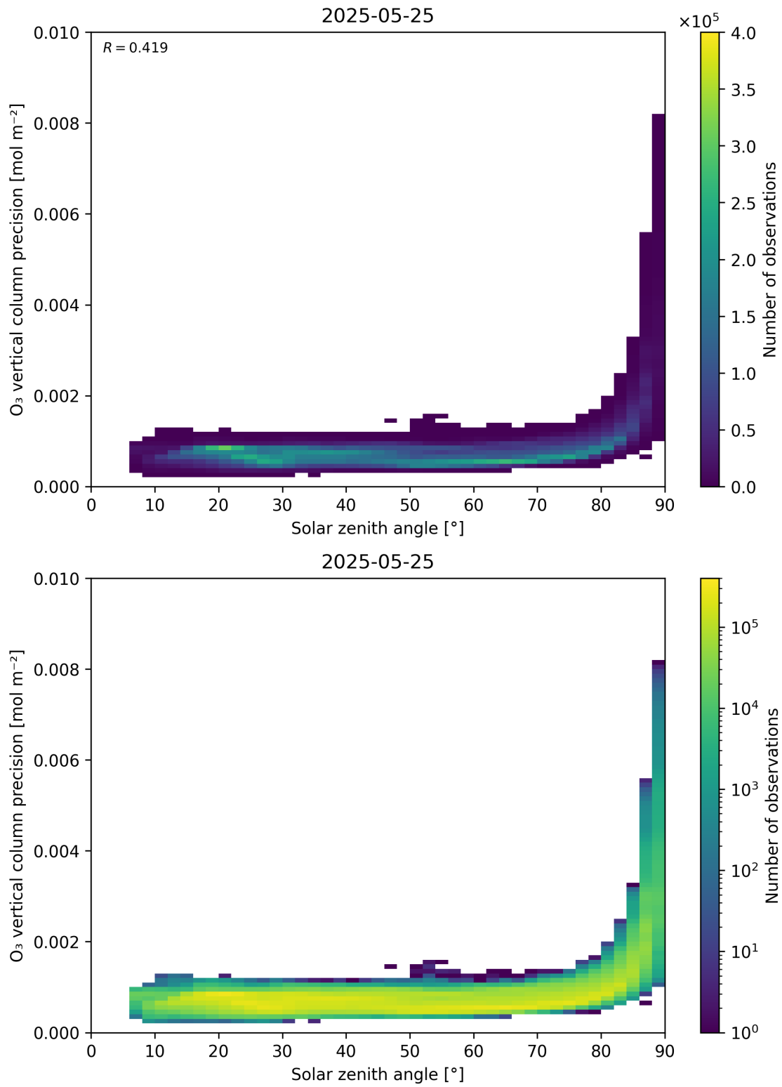
Figure 48: Scatter density plot of “Solar zenith angle” against “O 3 vertical column precision” for 2025-05-24 to 2025-05-26.
