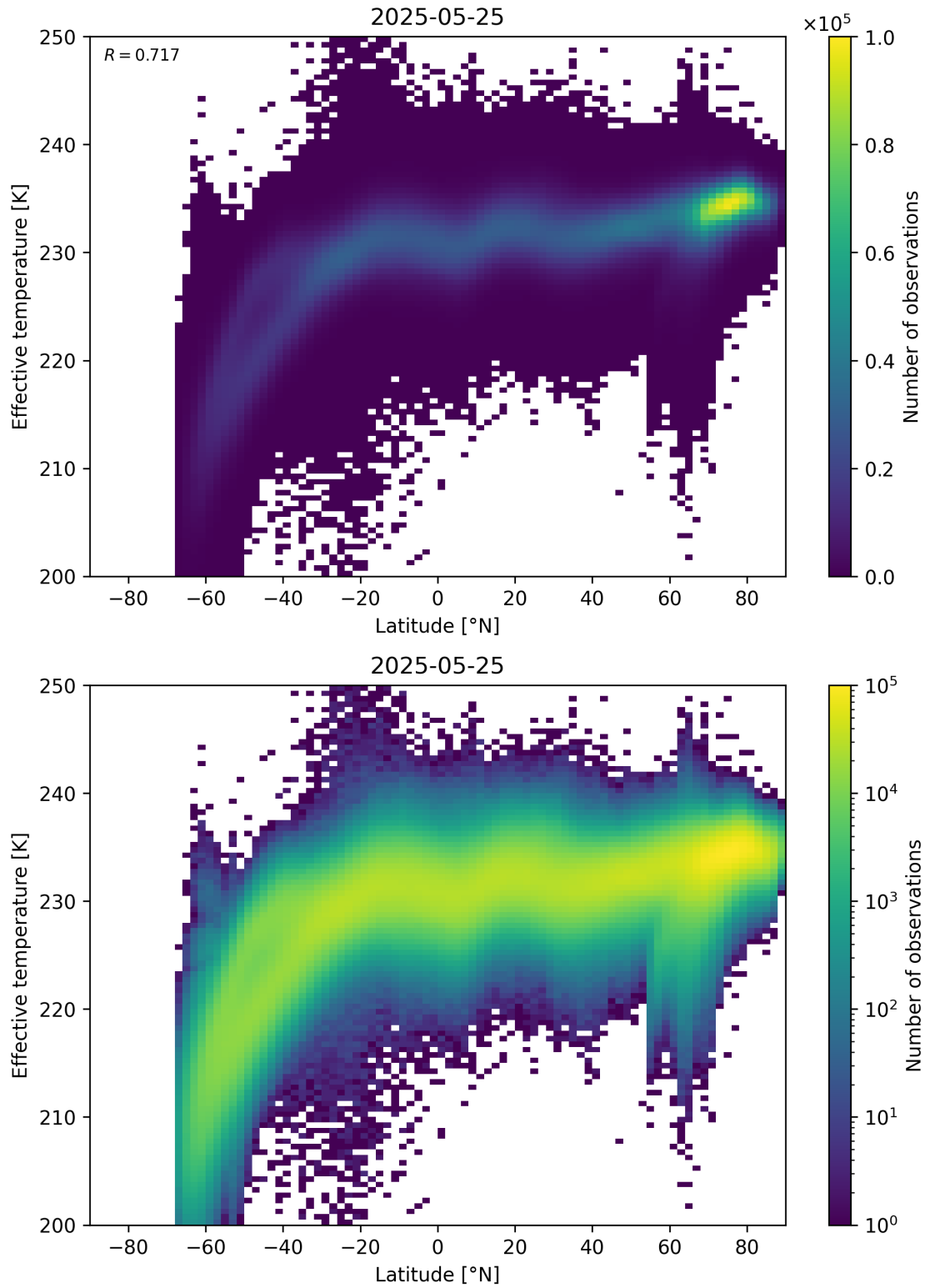
Figure 34: Scatter density plot of “Latitude” against “Effective temperature” for 2025-05-24 to 2025-05-26.
