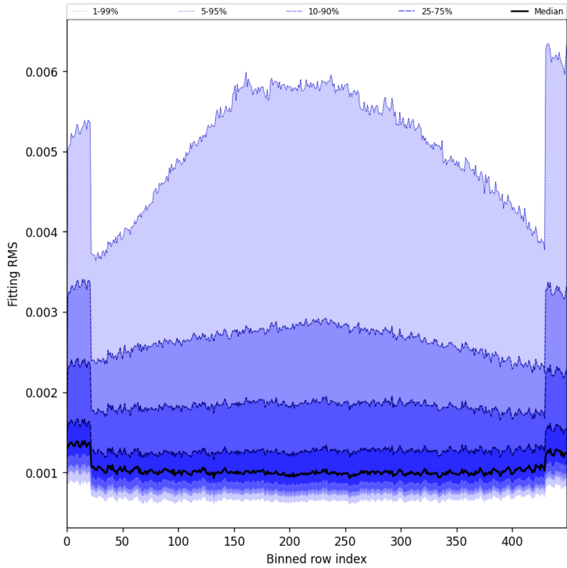
Figure 30: Along track statistics of “Fitting RMS” for 2025-05-24 to 2025-05-26
