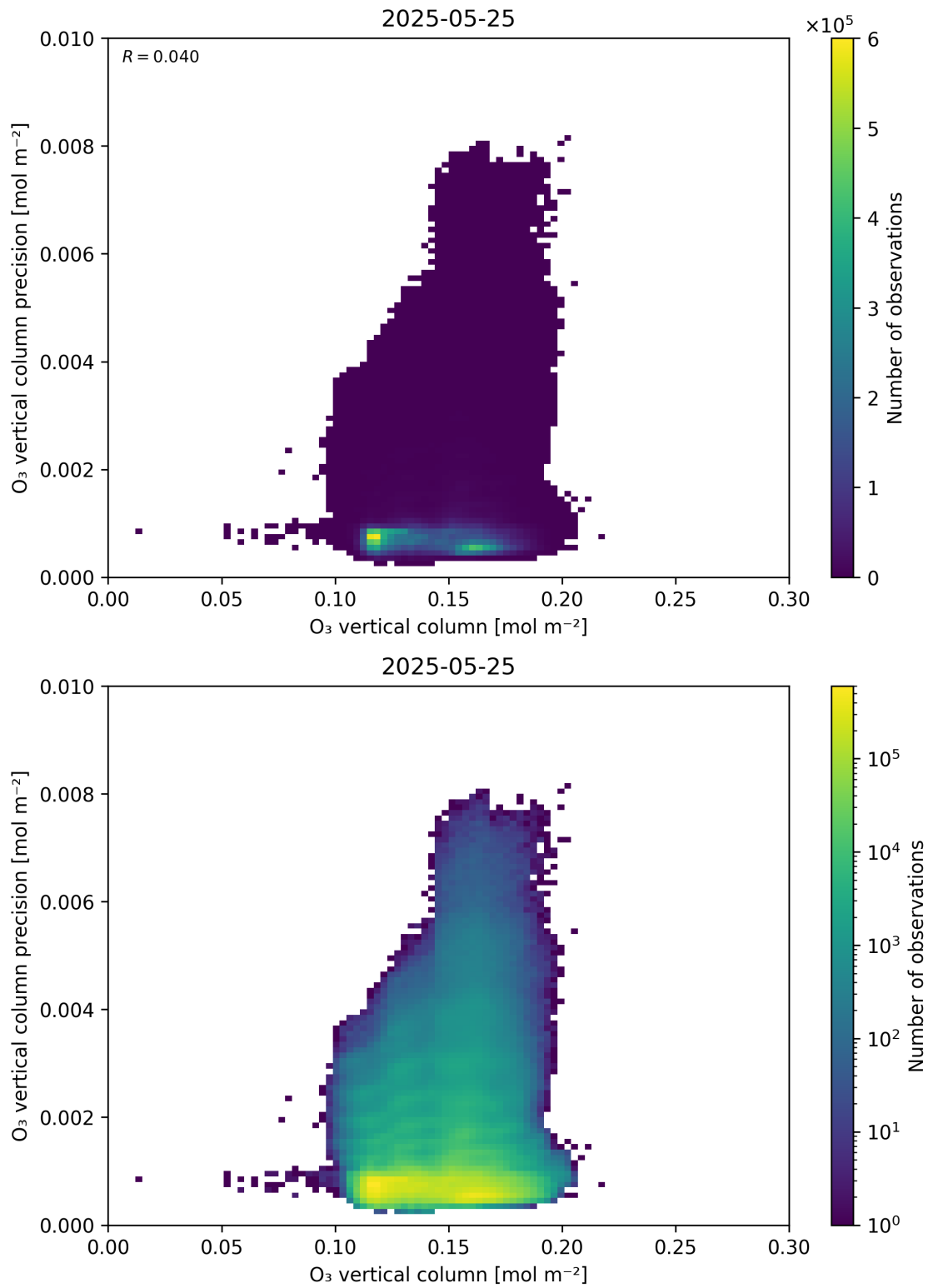
Figure 41: Scatter density plot of “O 3 vertical column” against “O 3 vertical column precision” for 2025-05-24 to 2025-05-26.
