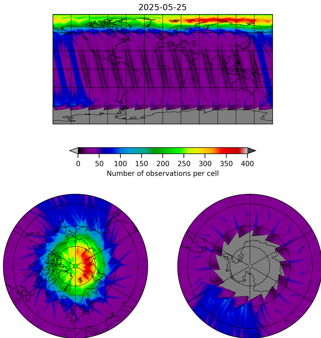
Figure 12: Map of the number of observations for 2025-05-24 to 2025-05-26
