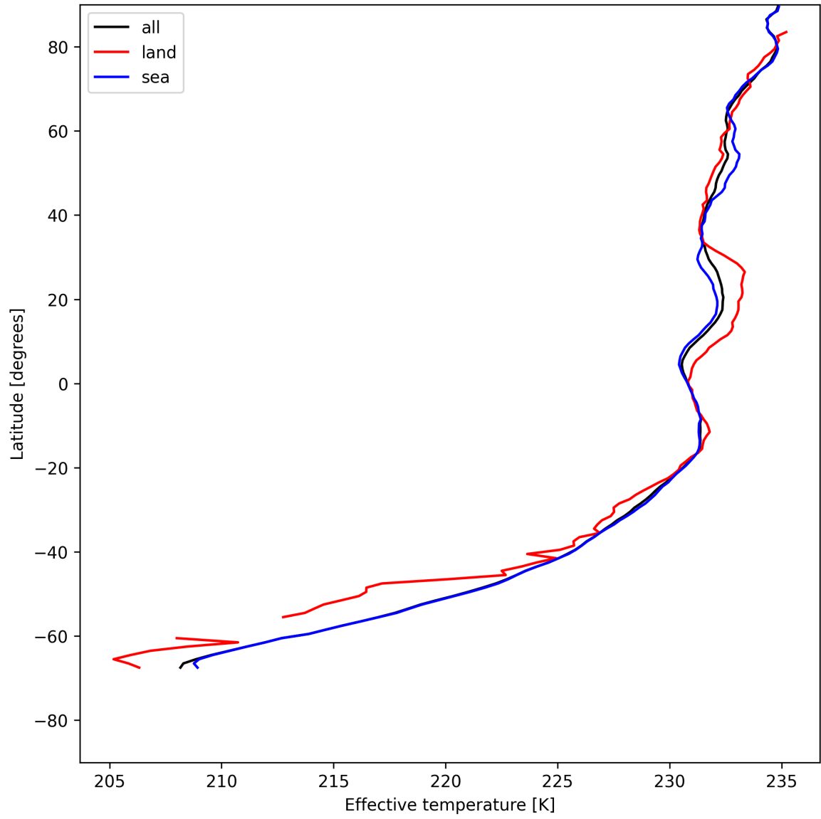
Figure 17: Zonal average of "Effective temperature" for 2025-05-24 to 2025-05-26.
