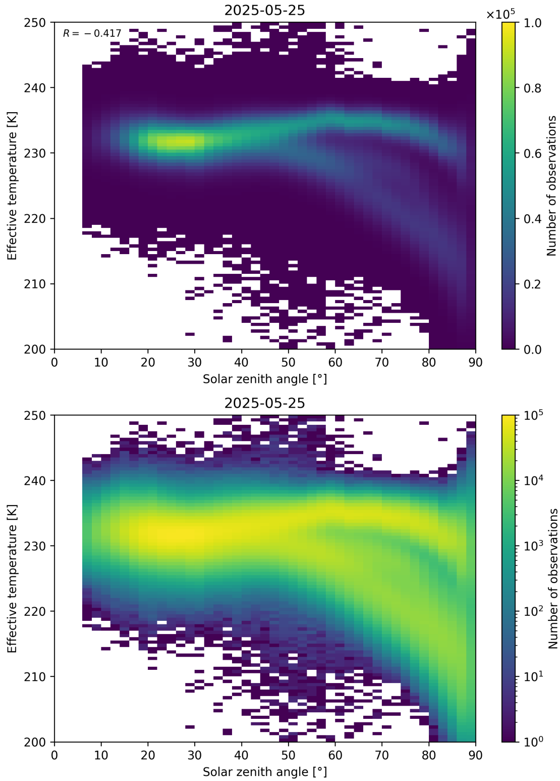
Figure 45: Scatter density plot of “Solar zenith angle” against “Effective temperature” for 2025-05-24 to 2025-05-26.
