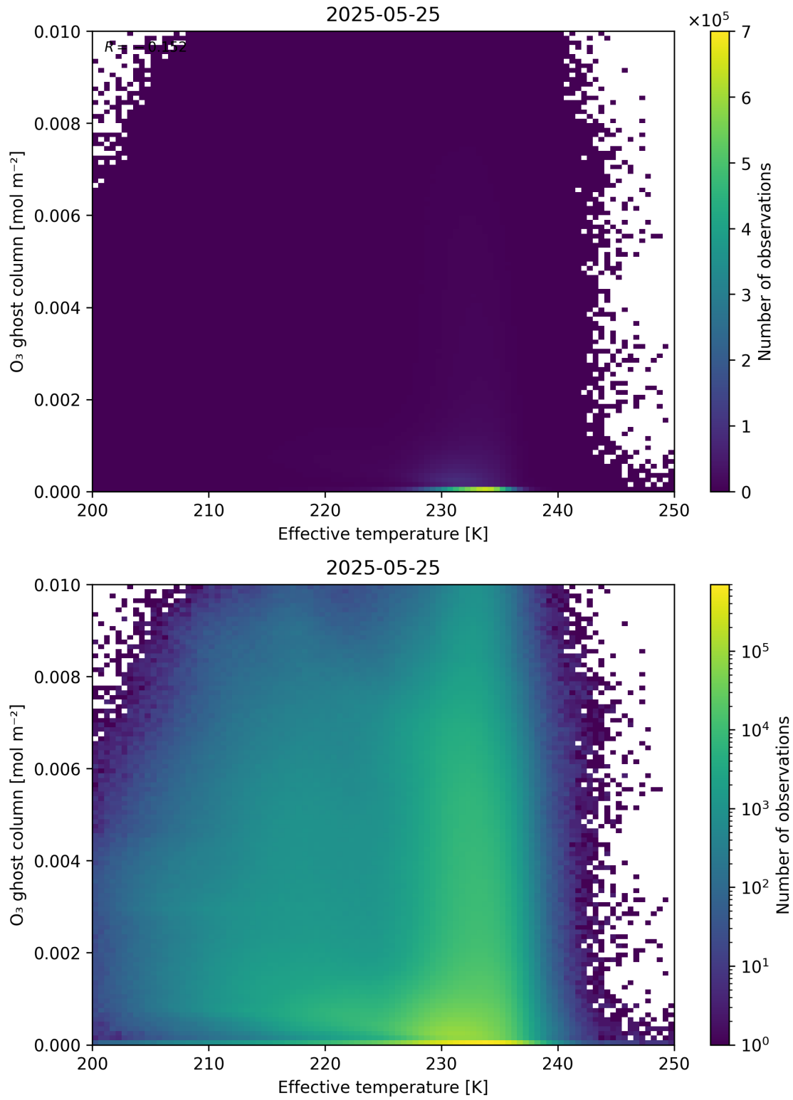
Figure 38: Scatter density plot of “Effective temperature” against “O 3 ghost column” for 2025-05-24 to 2025-05-26.
