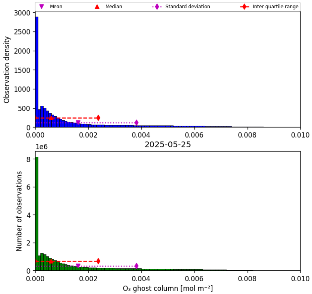
Figure 25: Histogram of “O 3 ghost column” for 2025-05-24 to 2025-05-26
