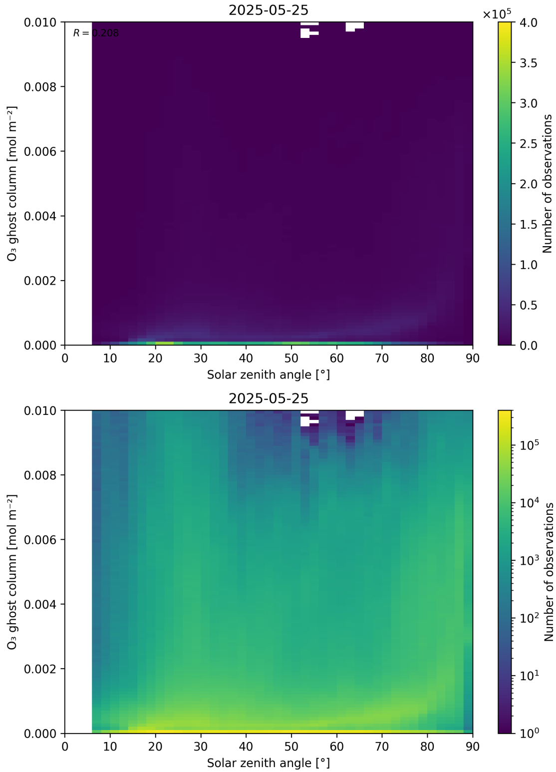
Figure 46: Scatter density plot of “Solar zenith angle” against “O 3 ghost column” for 2025-05-24 to 2025-05-26.
