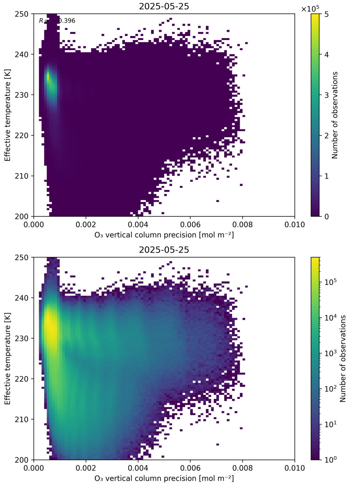
Figure 42: Scatter density plot of “O 3 vertical column precision” against “Effective temperature” for 2025-05-24 to 2025-05-26.
