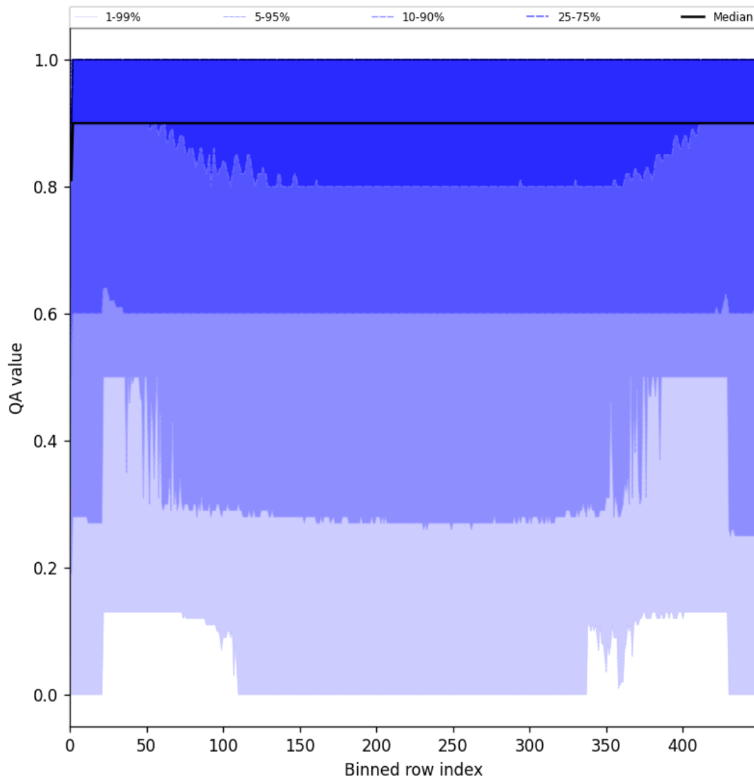
Figure 27: Along track statistics of “QA value” for 2025-05-24 to 2025-05-26
