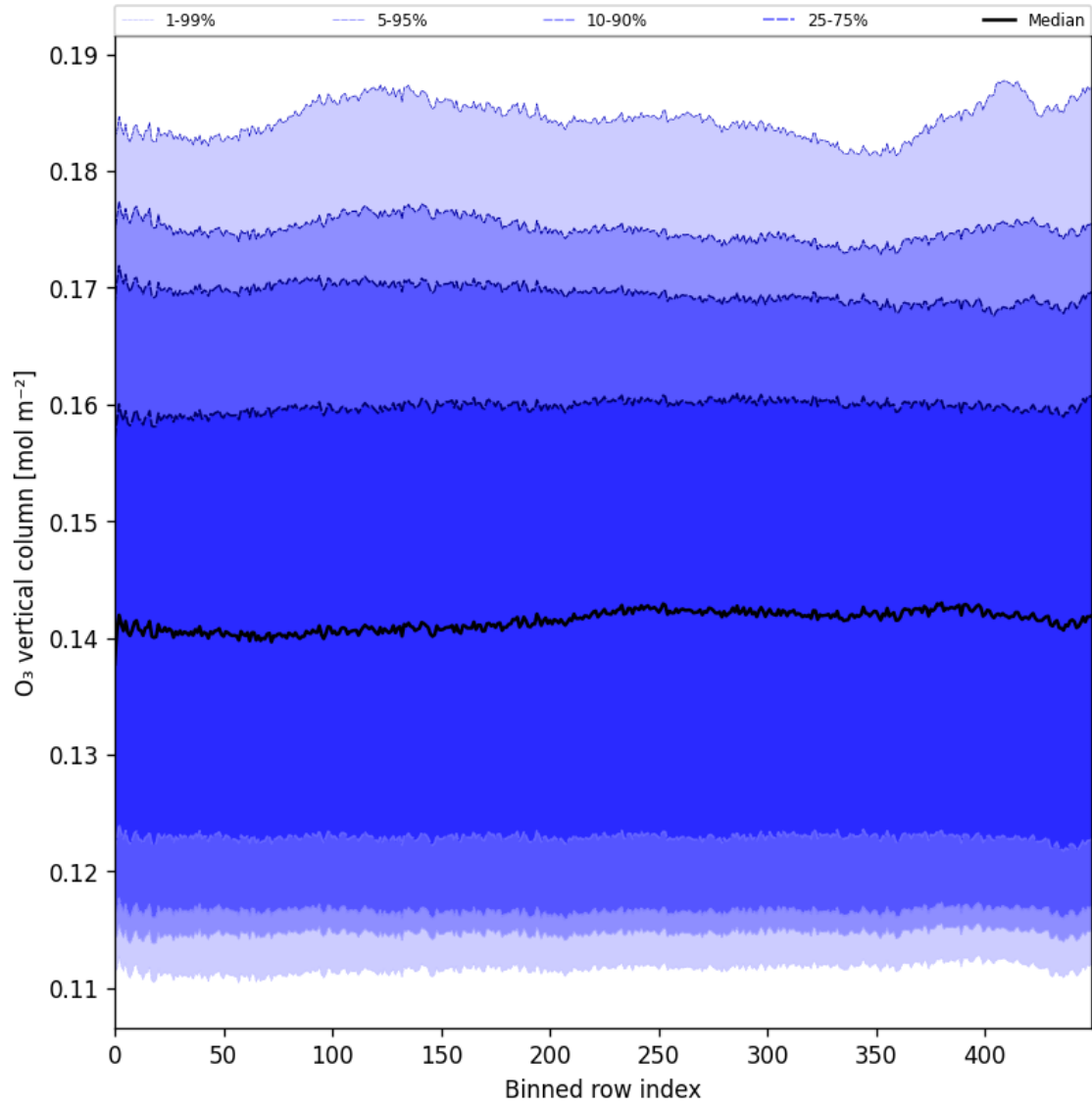
Figure 28: Along track statistics of “O 3 vertical column” for 2025-05-24 to 2025-05-26
