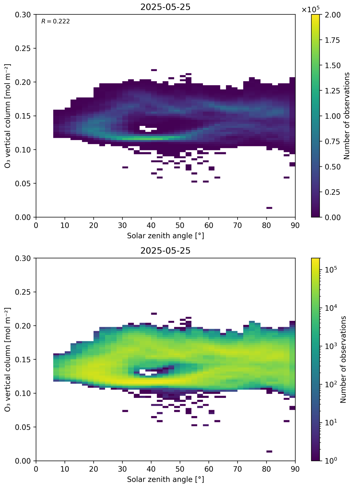
Figure 47: Scatter density plot of “Solar zenith angle” against “O 3 vertical column” for 2025-05-24 to 2025-05-26.
