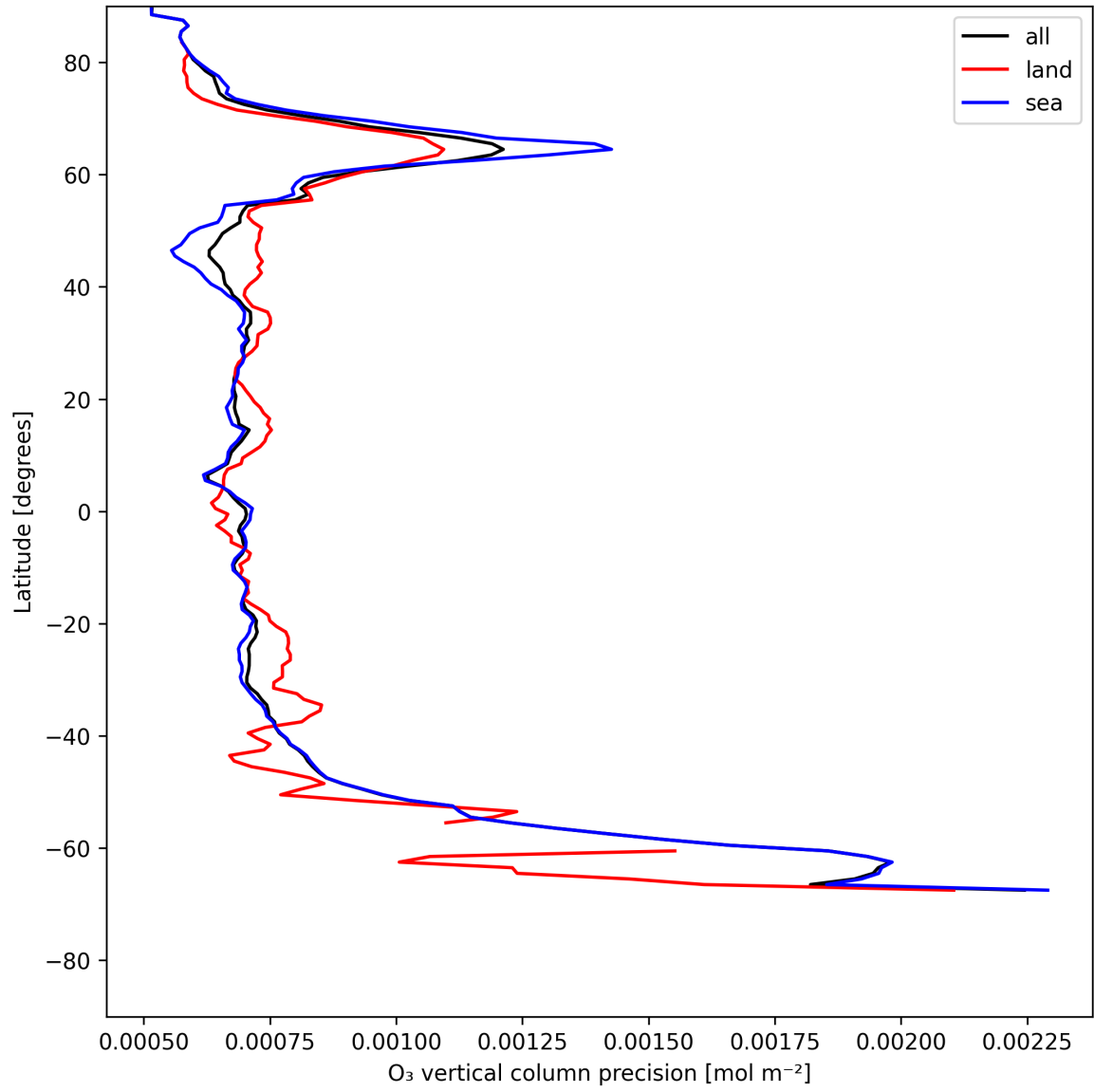
Figure 15: Zonal average of “O 3 vertical column precision” for 2025-05-24 to 2025-05-26.
