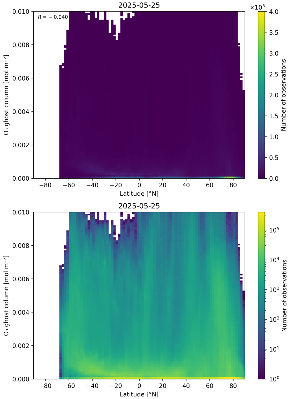
Figure 35: Scatter density plot of “Latitude” against “O 3 ghost column” for 2025-05-24 to 2025-05-26.
