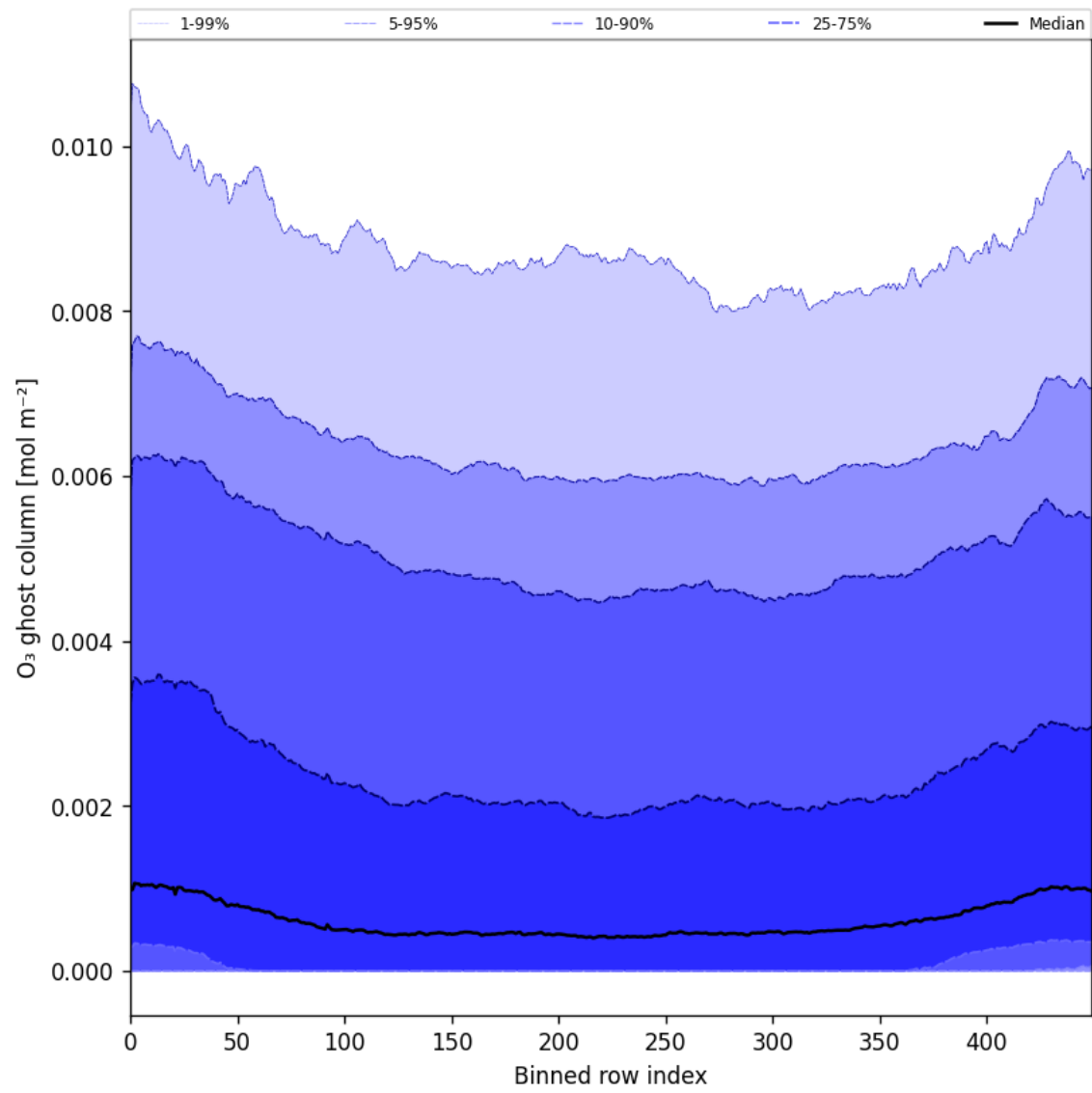
Figure 32: Along track statistics of “O 3 ghost column” for 2025-05-24 to 2025-05-26
