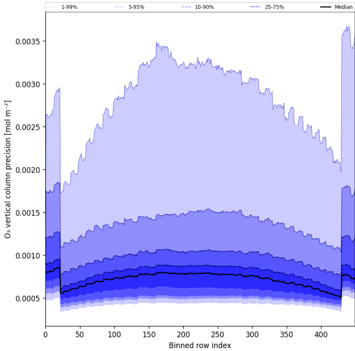
Figure 29: Along track statistics of “O 3 vertical column precision” for 2025-05-24 to 2025-05-26
