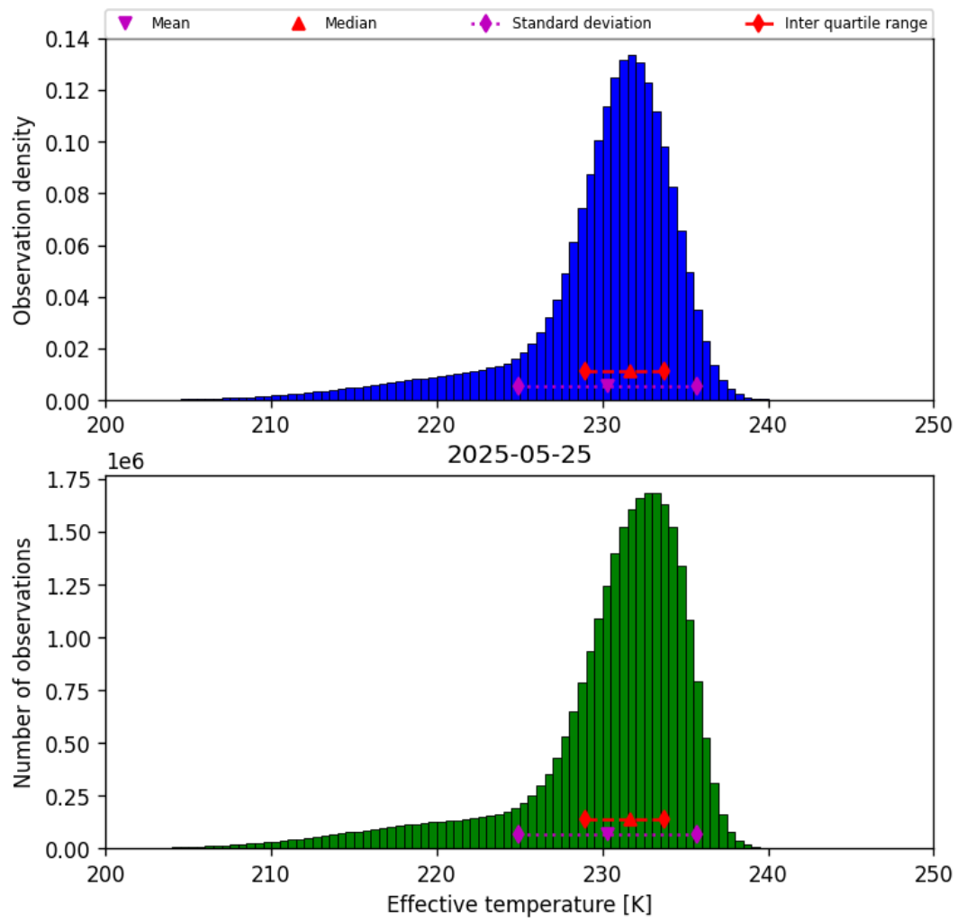
Figure 24: Histogram of “Effective temperature” for 2025-05-24 to 2025-05-26
