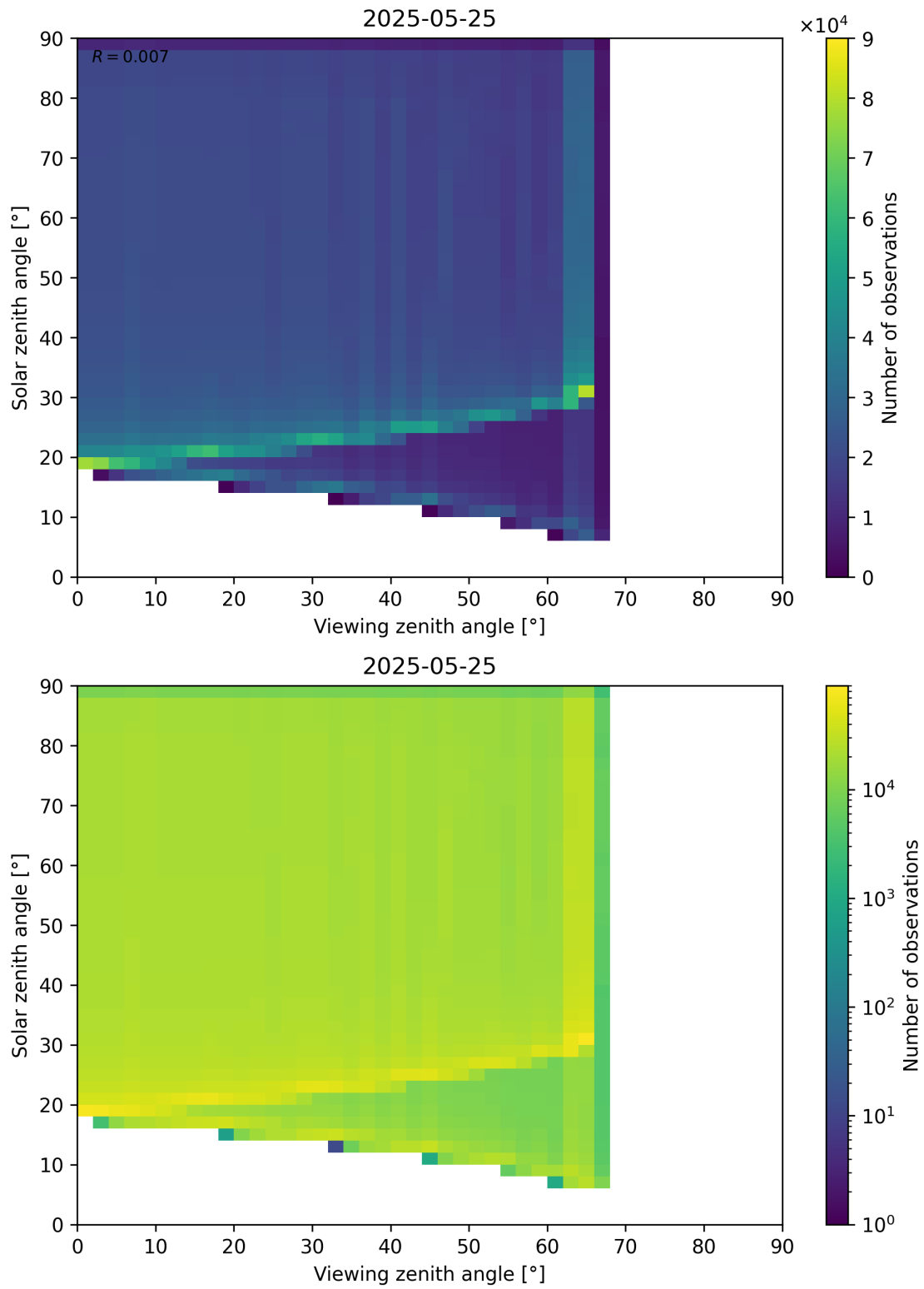
Figure 54: Scatter density plot of “Viewing zenith angle” against “Solar zenith angle” for 2025-05-24 to 2025-05-26.
