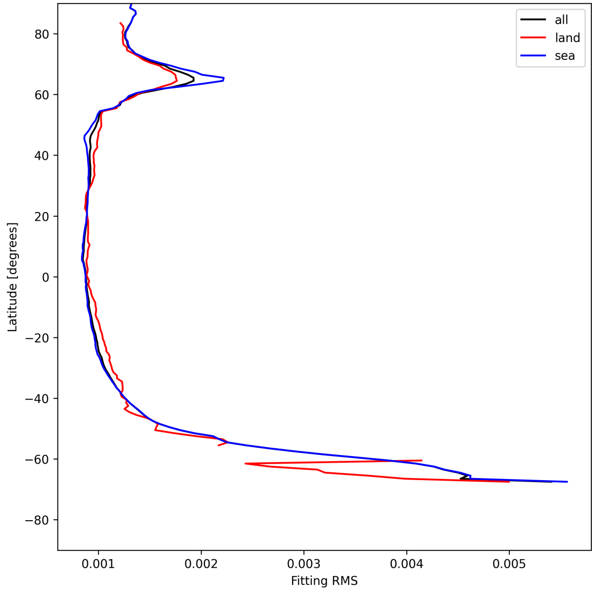
Figure 16: Zonal average of “Fitting RMS” for 2025-05-24 to 2025-05-26.
