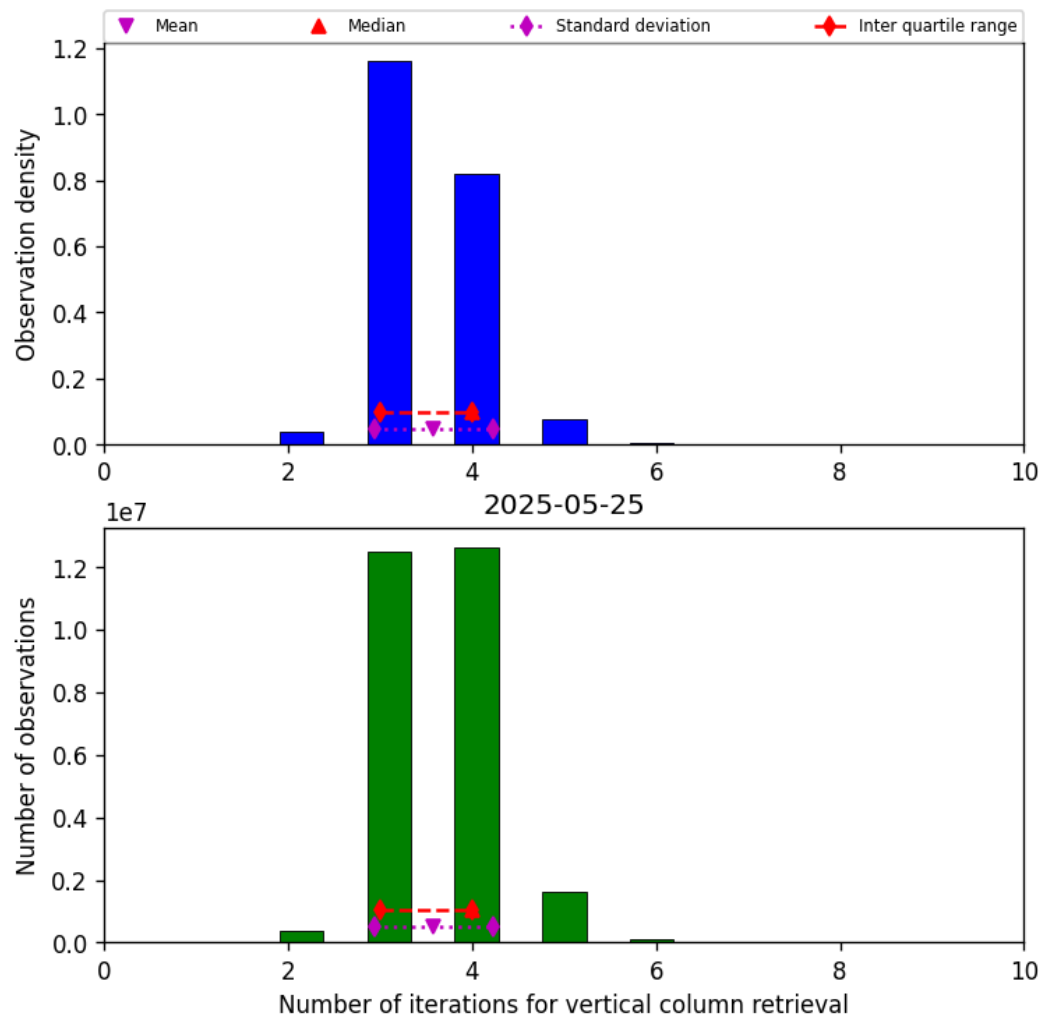
Figure 26: Histogram of “Number of iterations for vertical column retrieval” for 2025-05-24 to 2025-05-26
