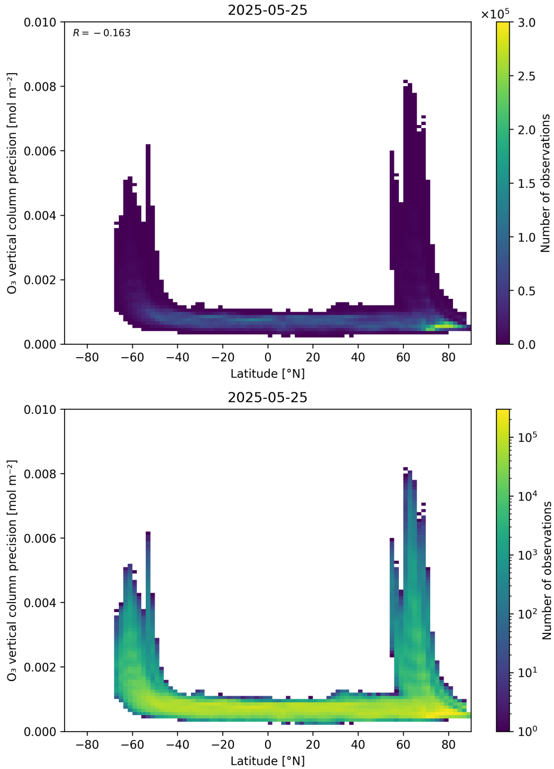
Figure 37: Scatter density plot of “Latitude” against “O 3 vertical column precision” for 2025-05-24 to 2025-05-26.
