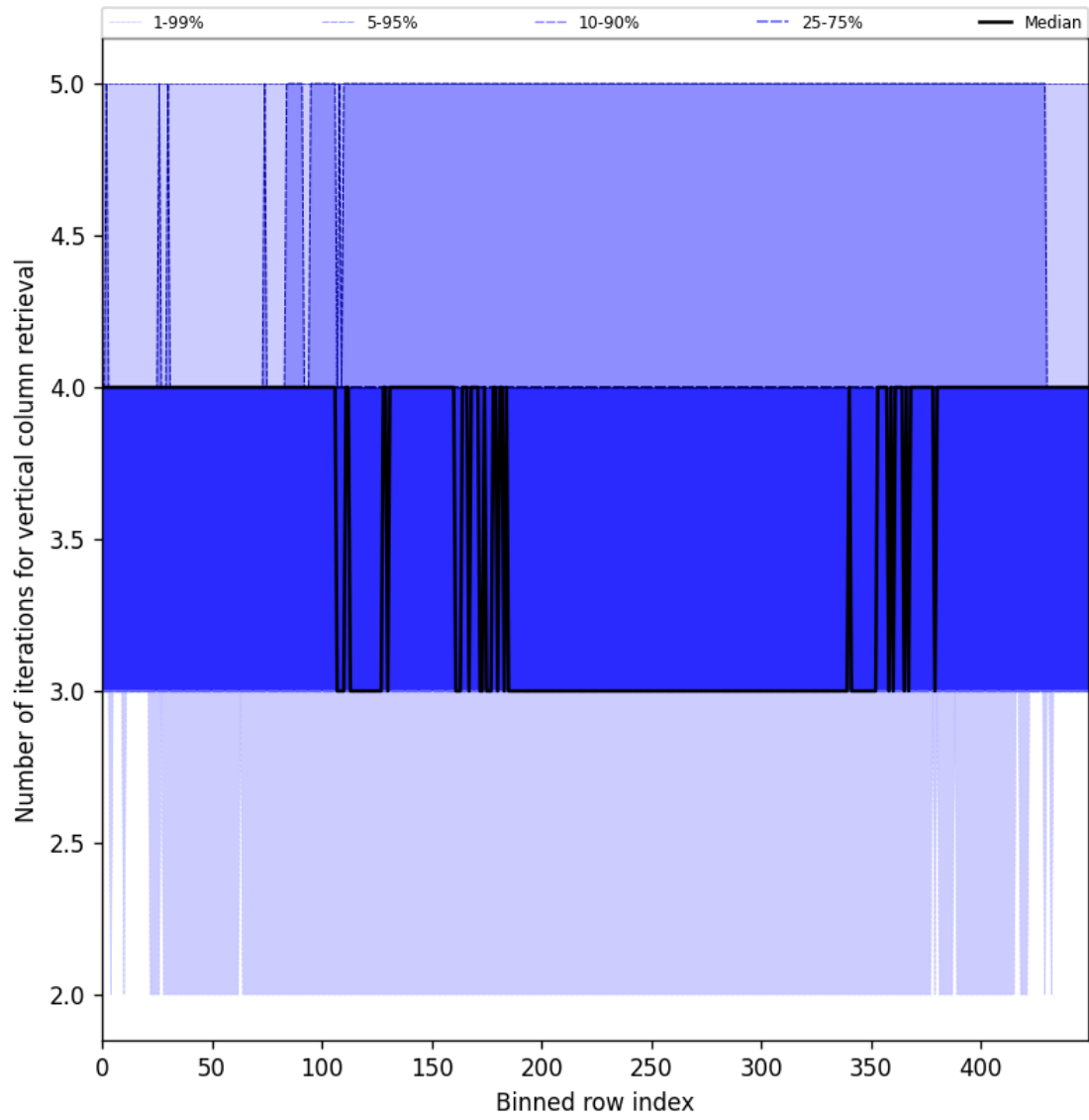
Figure 33: Along track statistics of “Number of iterations for vertical column retrieval” for 2025-05-24 to 2025-05-26
