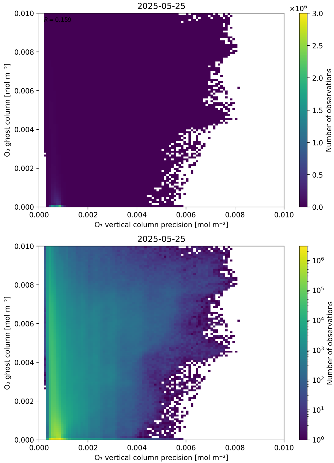
Figure 43: Scatter density plot of “ \text{O}_3 vertical column precision” against “ \text{O}_3 ghost column” for 2025-05-24 to 2025-05-26.
