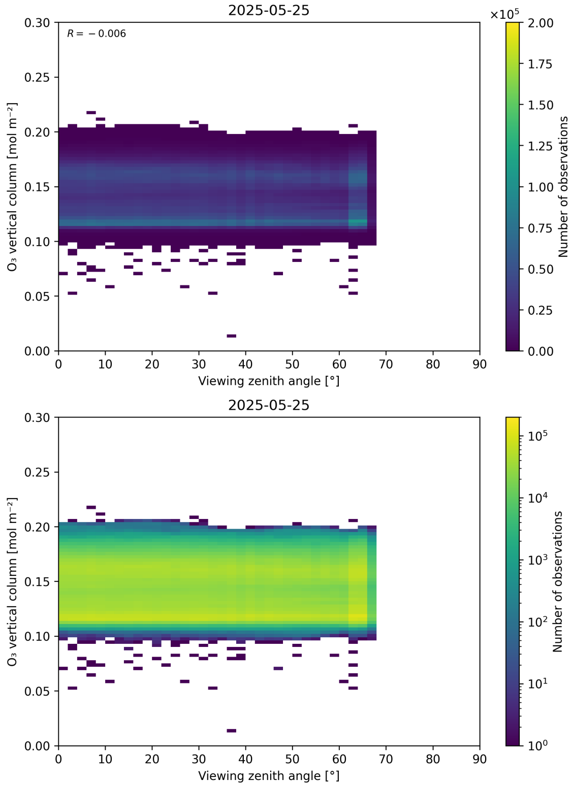
Figure 52: Scatter density plot of “Viewing zenith angle” against “O 3 vertical column” for 2025-05-24 to 2025-05-26.
