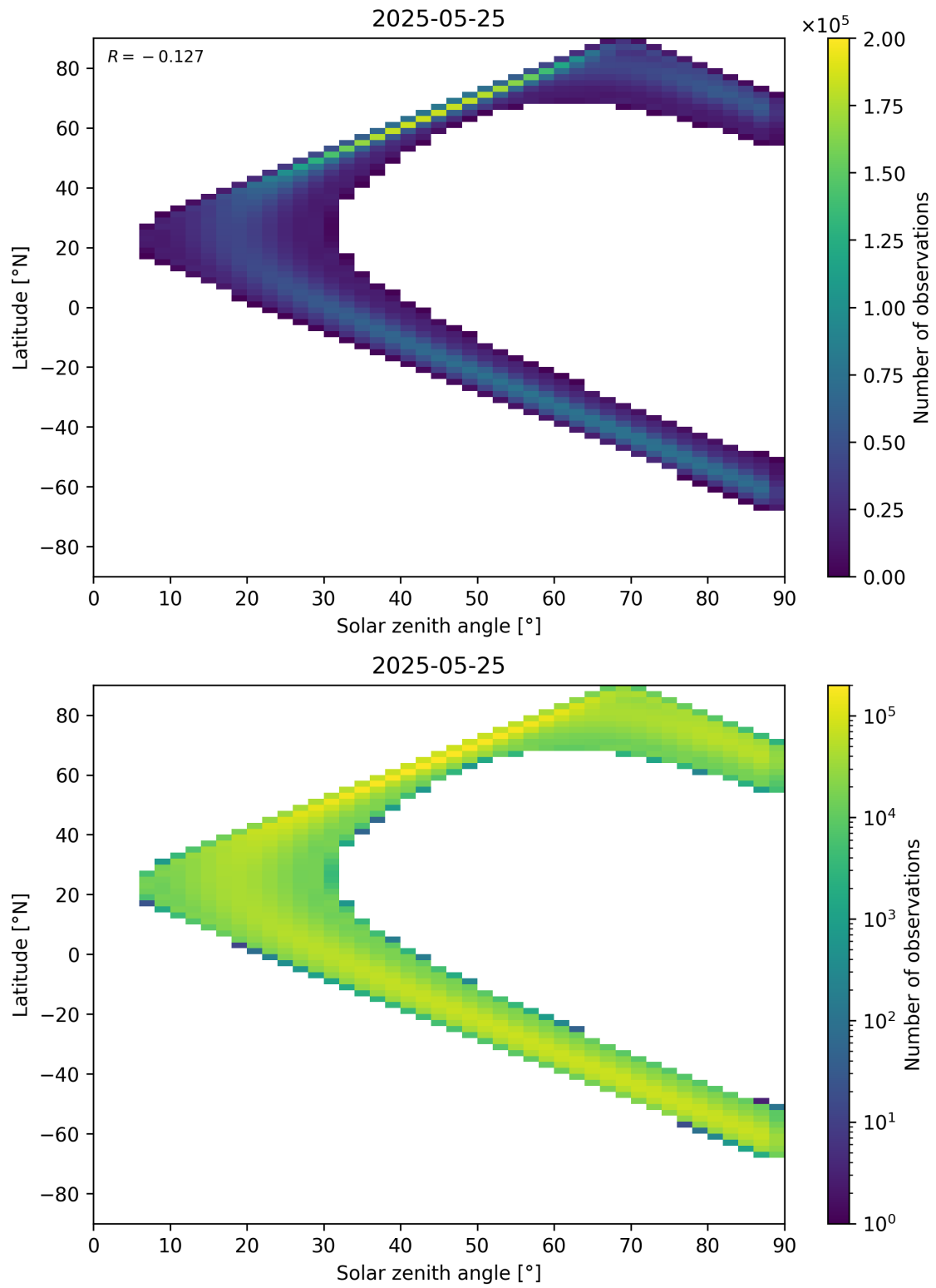
Figure 44: Scatter density plot of “Solar zenith angle” against “Latitude” for 2025-05-24 to 2025-05-26.
