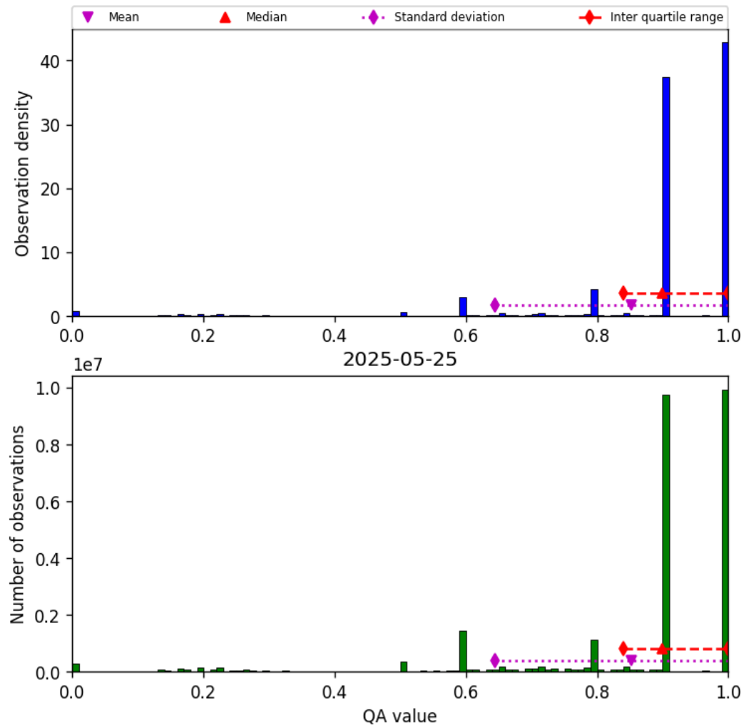
Figure 20: Histogram of “QA value” for 2025-05-24 to 2025-05-26
