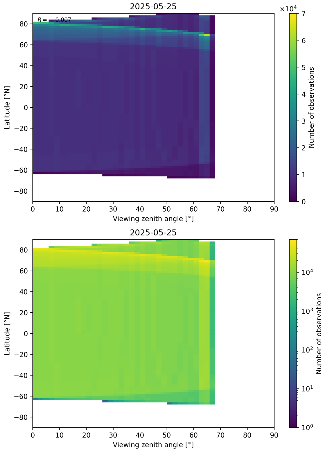
Figure 49: Scatter density plot of “Viewing zenith angle” against “Latitude” for 2025-05-24 to 2025-05-26.
