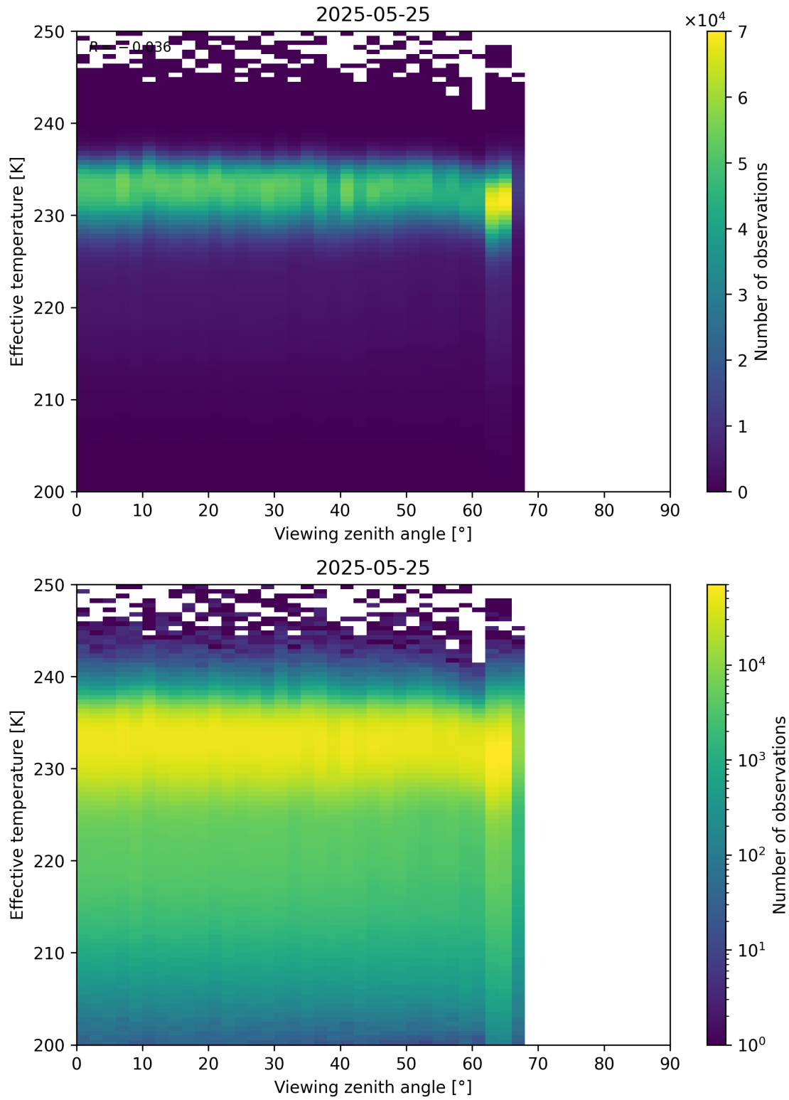
Figure 50: Scatter density plot of “Viewing zenith angle” against “Effective temperature” for 2025-05-24 to 2025-05-26.
