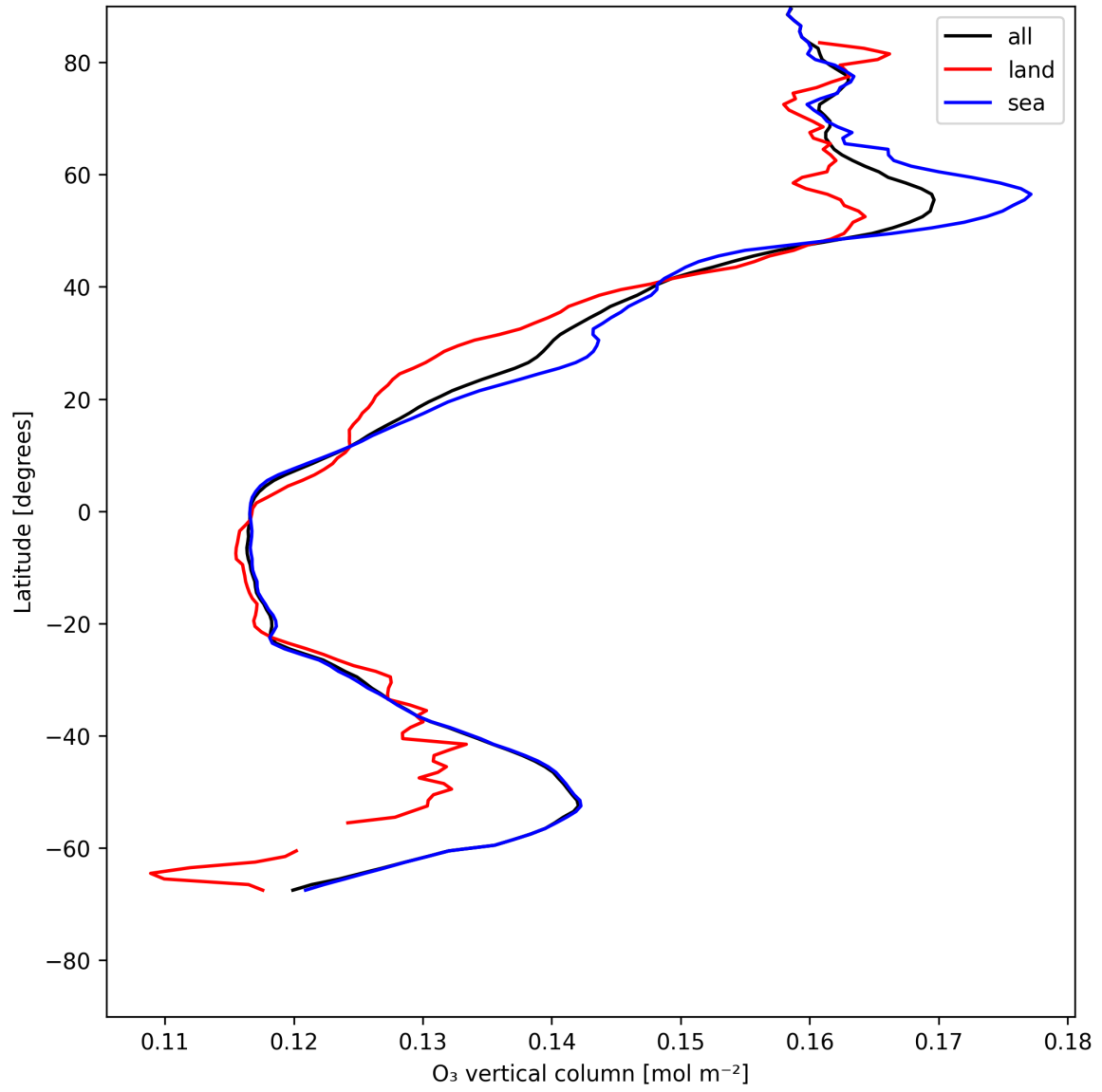
Figure 14: Zonal average of “O 3 vertical column” for 2025-05-24 to 2025-05-26.
