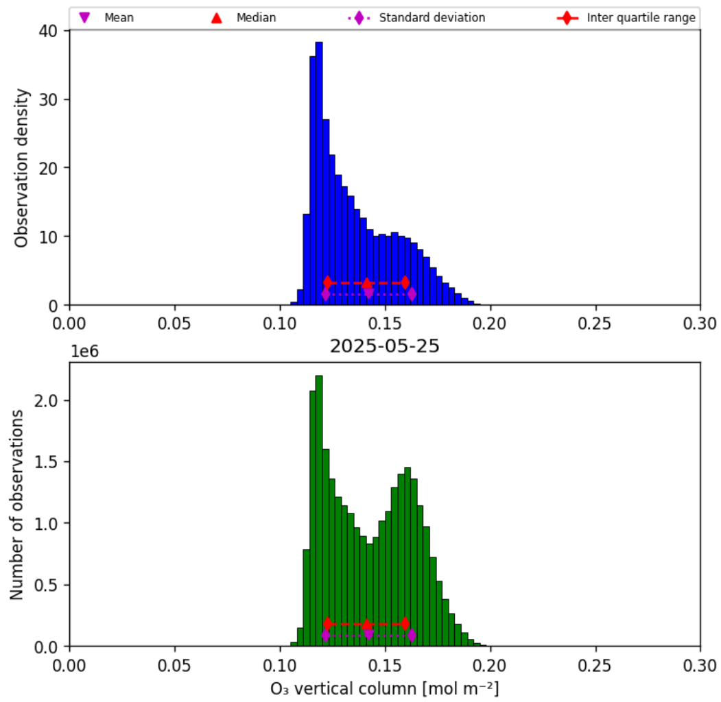
Figure 21: Histogram of “O 3 vertical column” for 2025-05-24 to 2025-05-26
