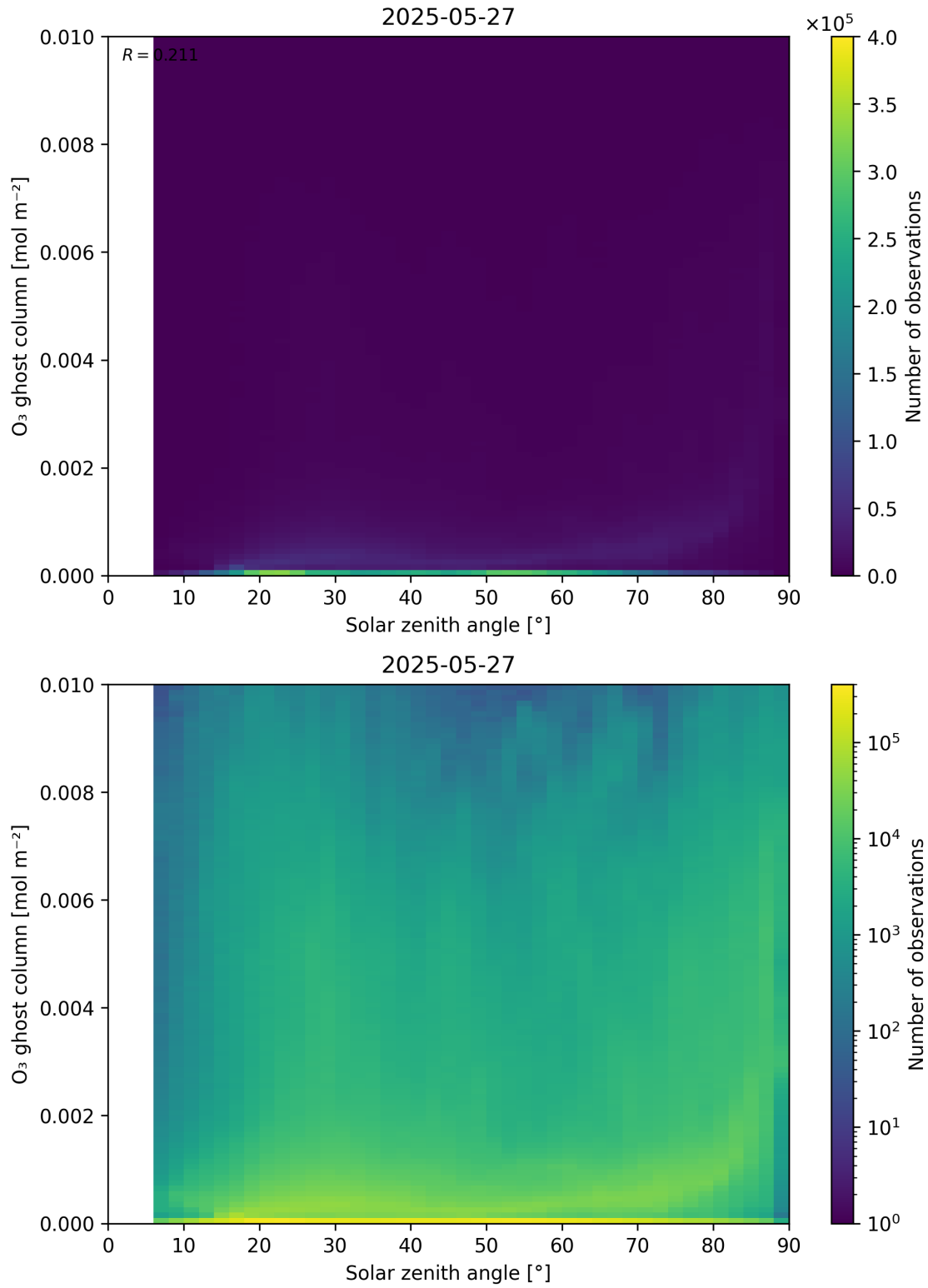
Figure 46: Scatter density plot of “Solar zenith angle” against “O 3 ghost column” for 2025-05-26 to 2025-05-28.
