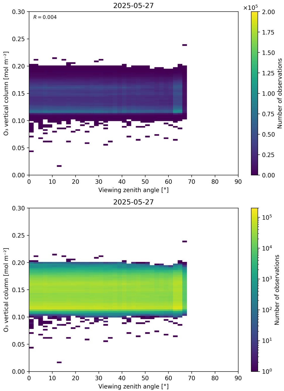
Figure 52: Scatter density plot of “Viewing zenith angle” against “O 3 vertical column” for 2025-05-26 to 2025-05-28.
