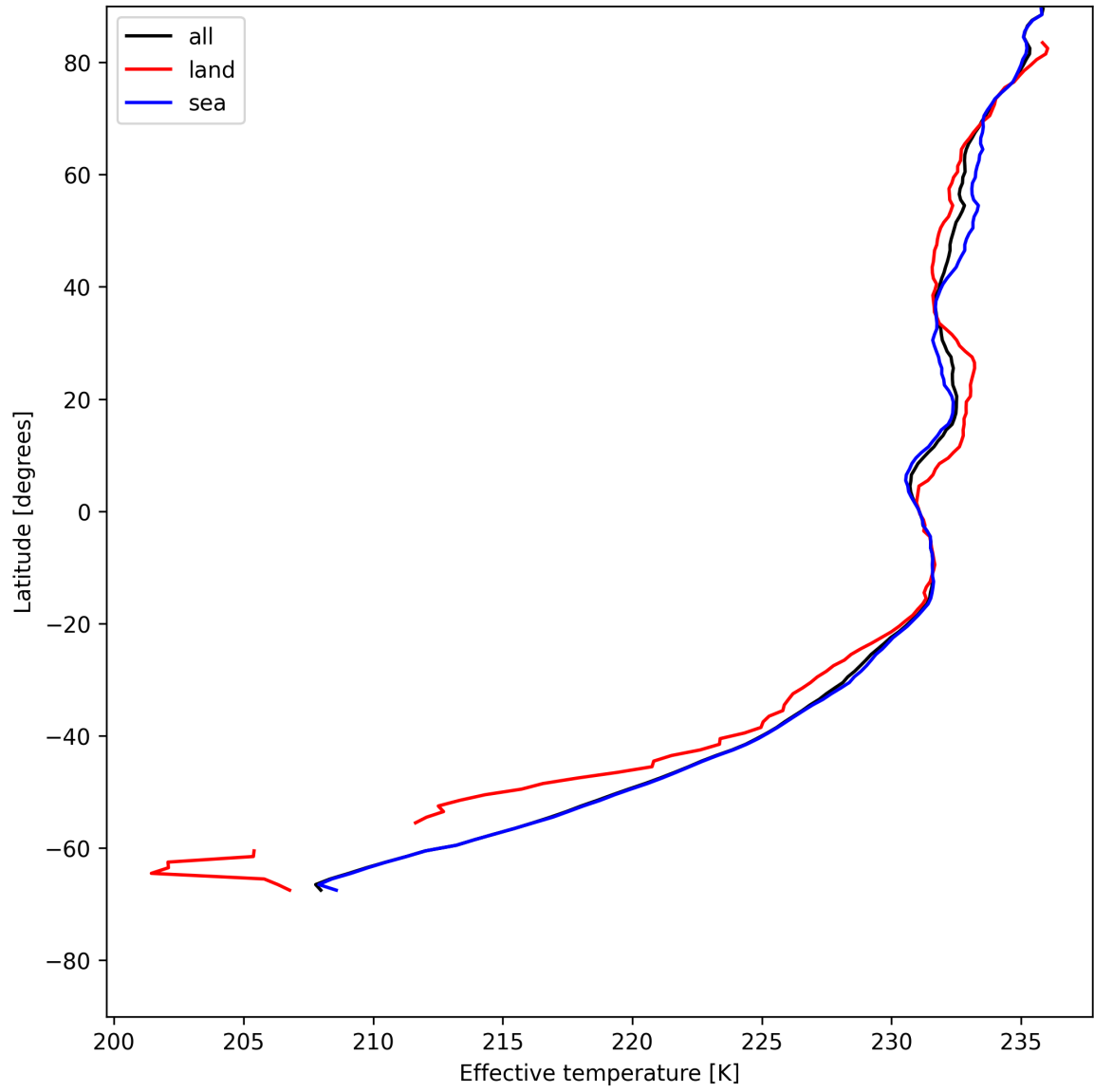
Figure 17: Zonal average of "Effective temperature" for 2025-05-26 to 2025-05-28.
