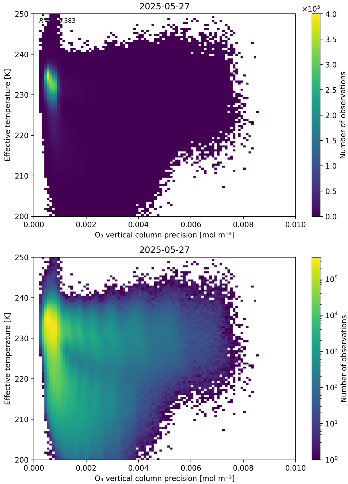
Figure 42: Scatter density plot of “O 3 vertical column precision” against “Effective temperature” for 2025-05-26 to 2025-05-28.
