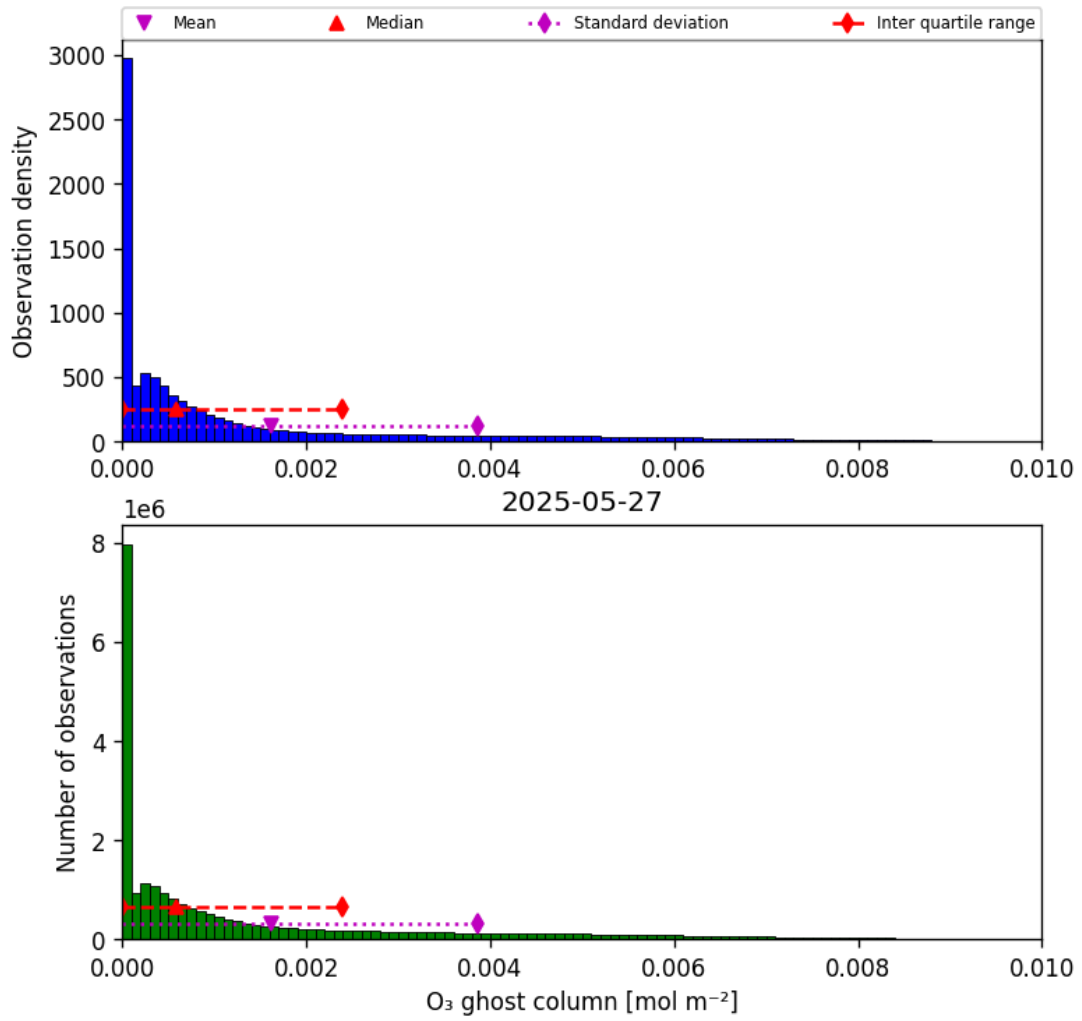
Figure 25: Histogram of “O 3 ghost column” for 2025-05-26 to 2025-05-28
