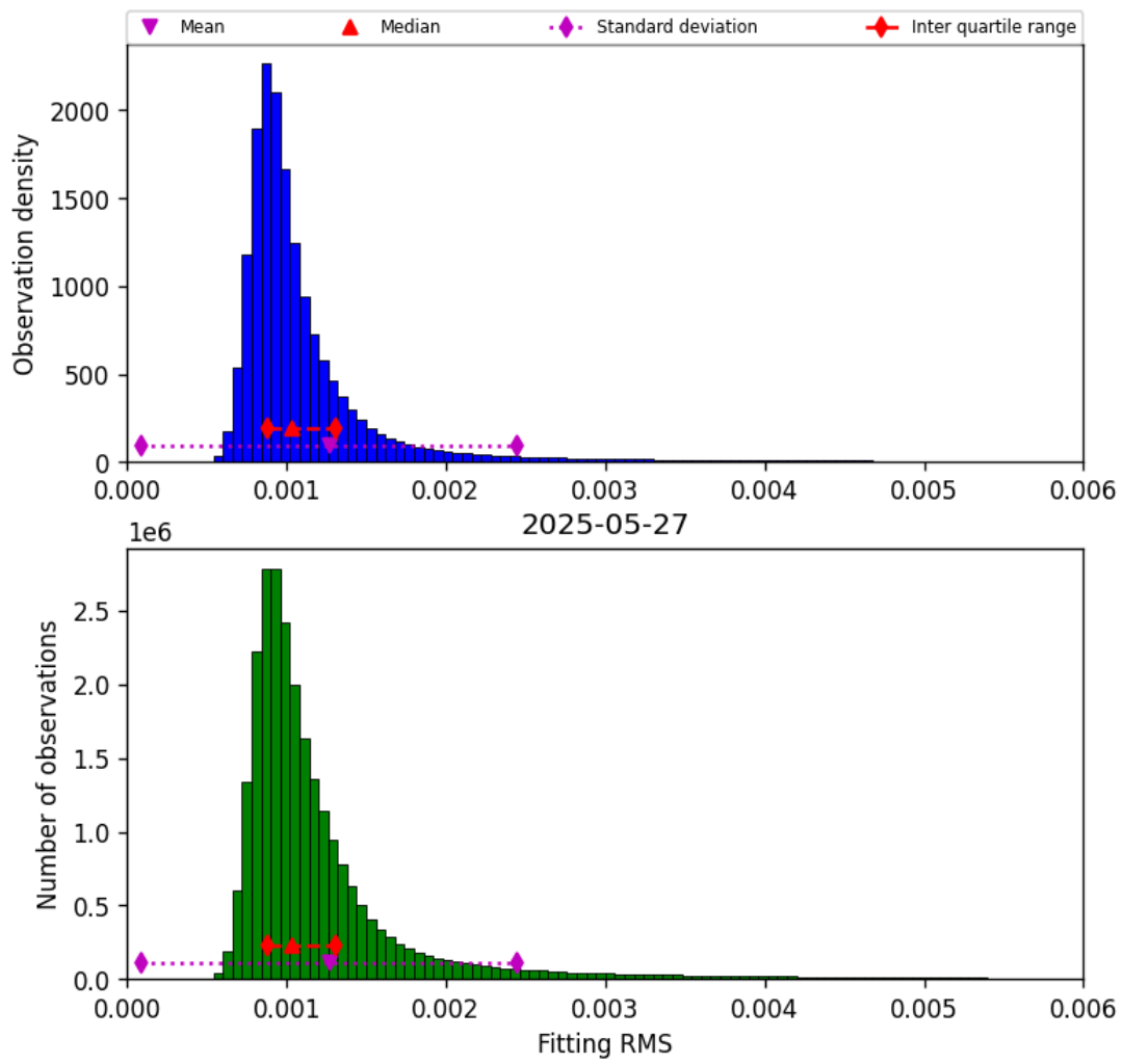
Figure 23: Histogram of “Fitting RMS” for 2025-05-26 to 2025-05-28
