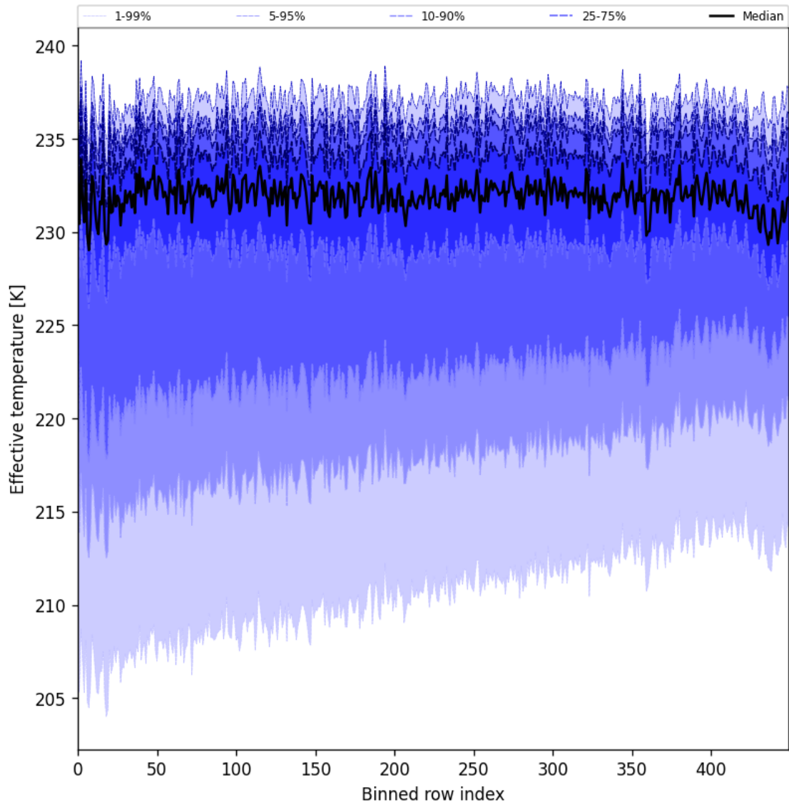
Figure 31: Along track statistics of “Effective temperature” for 2025-05-26 to 2025-05-28
