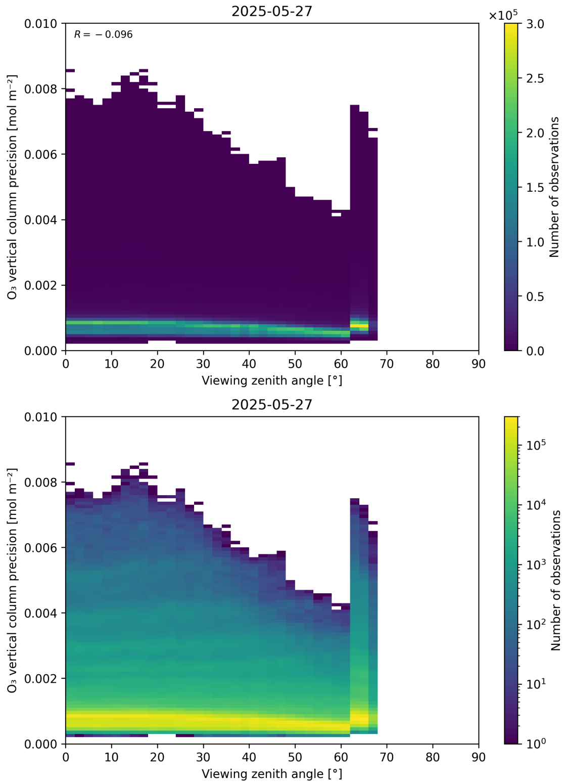
Figure 53: Scatter density plot of “Viewing zenith angle” against “O 3 vertical column precision” for 2025-05-26 to 2025-05-28.
