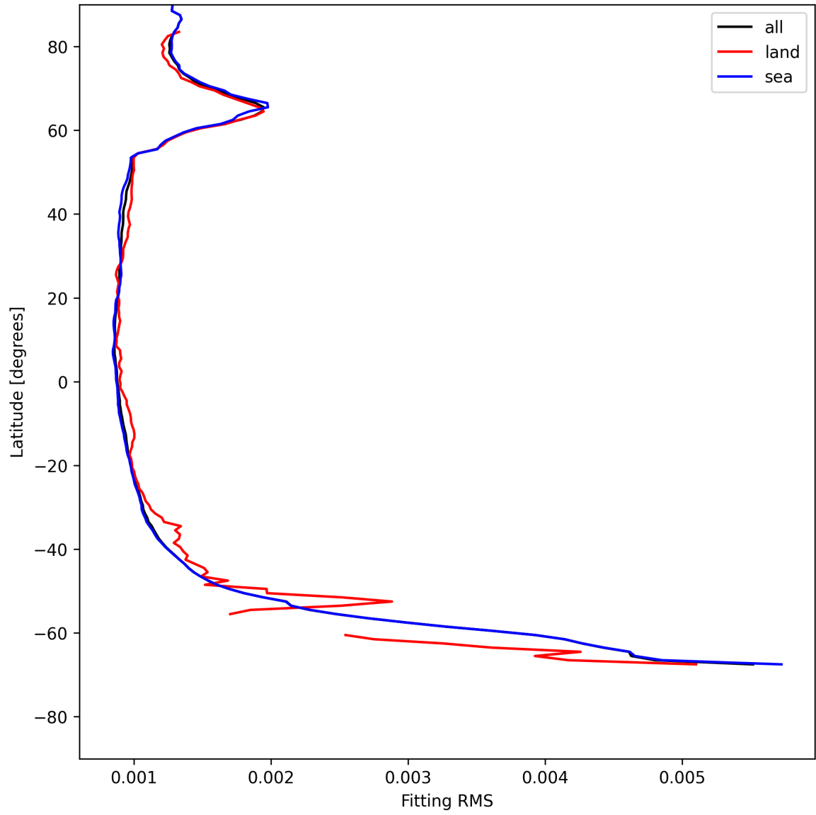
Figure 16: Zonal average of “Fitting RMS” for 2025-05-26 to 2025-05-28.
