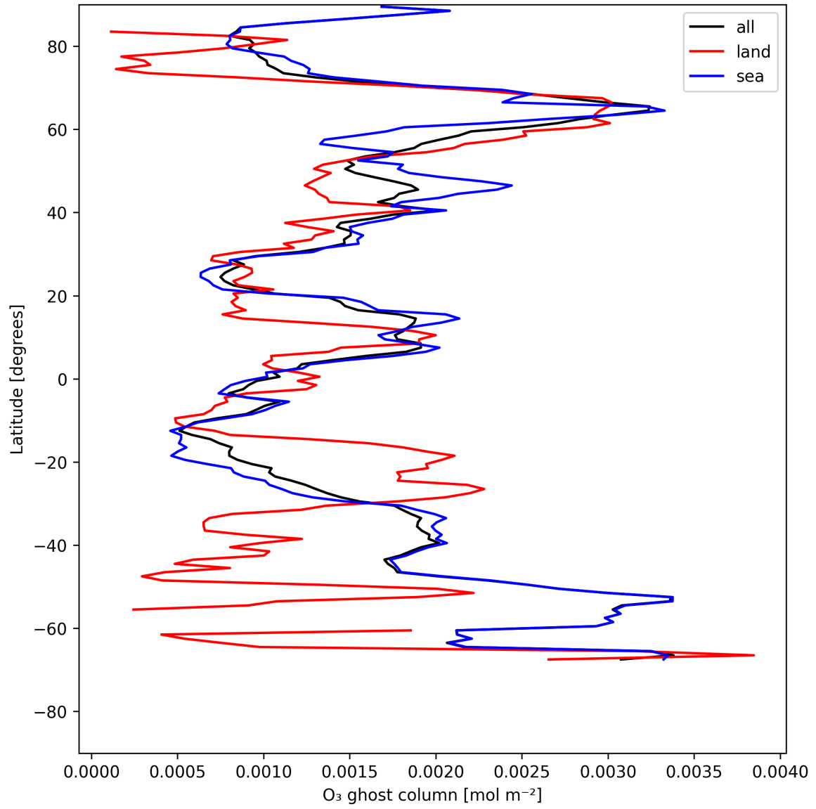
Figure 18: Zonal average of “O 3 ghost column” for 2025-05-26 to 2025-05-28.
