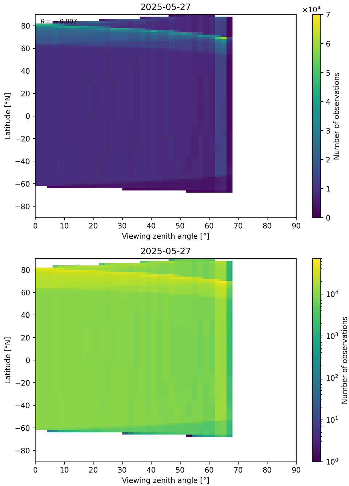
Figure 49: Scatter density plot of “Viewing zenith angle” against “Latitude” for 2025-05-26 to 2025-05-28.
