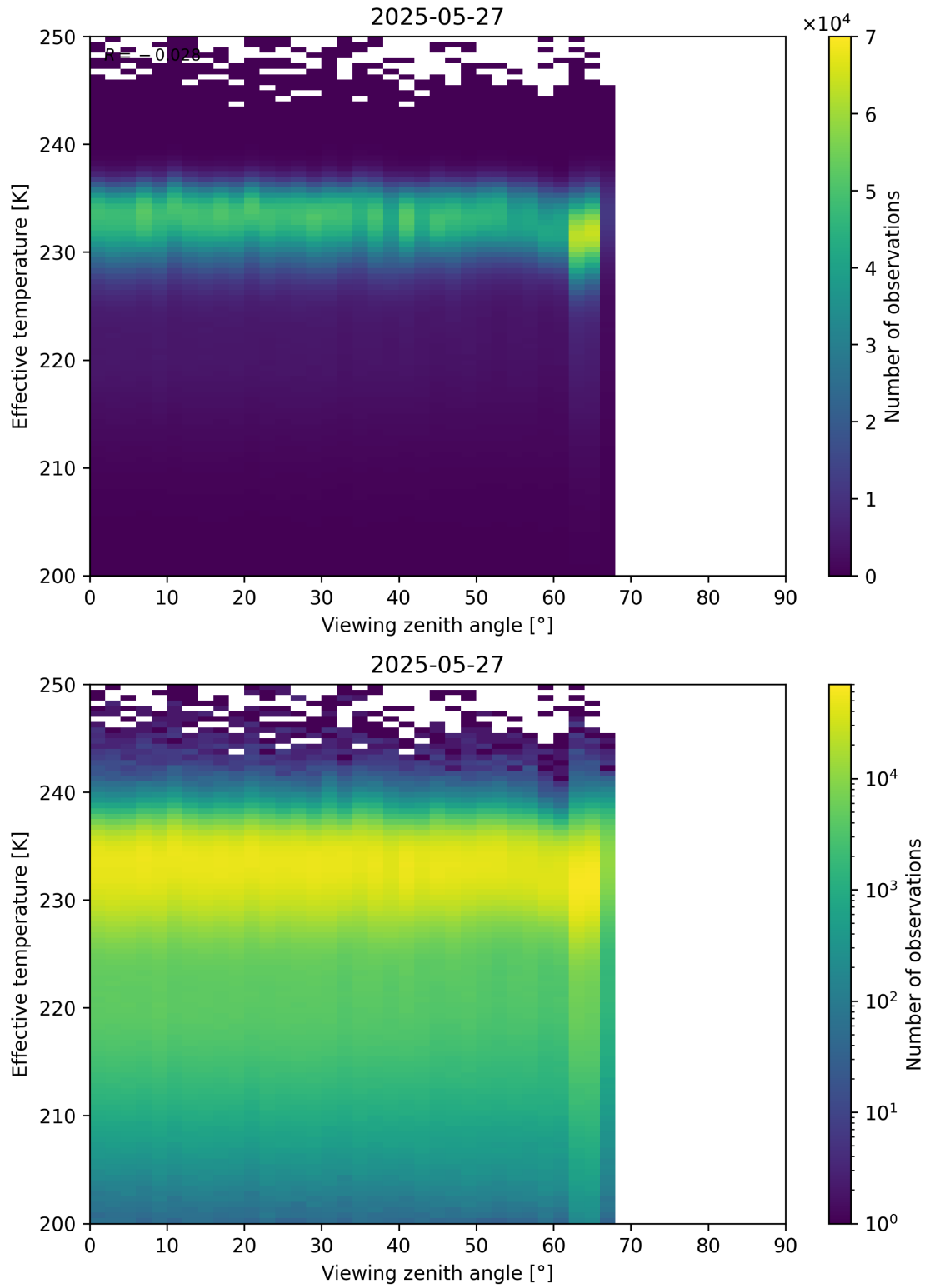
Figure 50: Scatter density plot of “Viewing zenith angle” against “Effective temperature” for 2025-05-26 to 2025-05-28.
