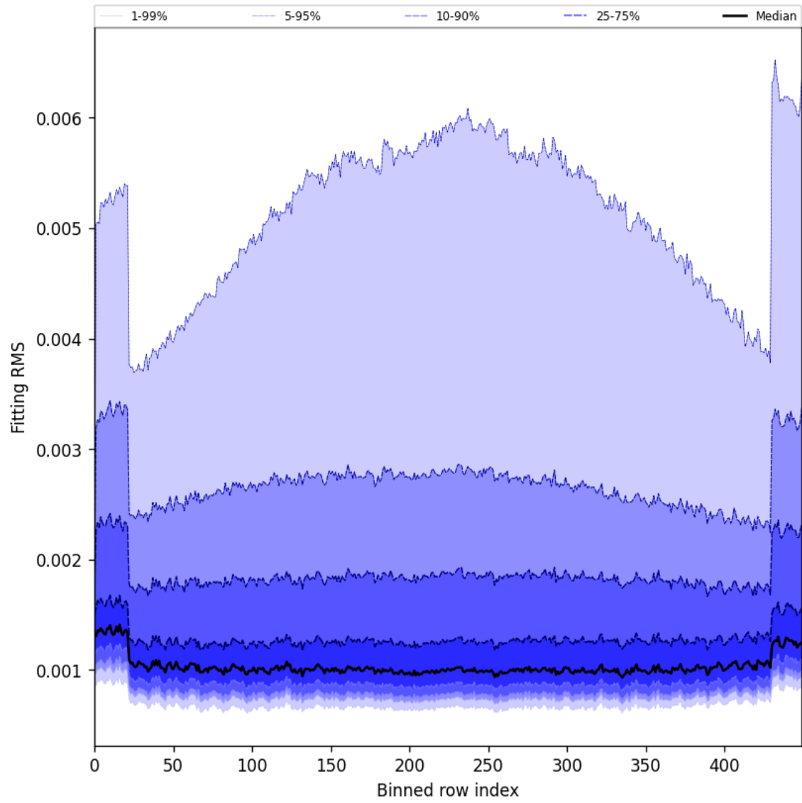
Figure 30: Along track statistics of “Fitting RMS” for 2025-05-26 to 2025-05-28
