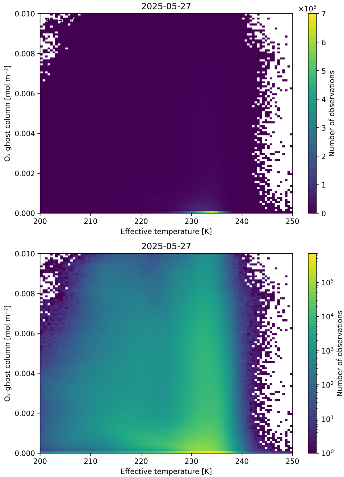
Figure 38: Scatter density plot of “Effective temperature” against “O 3 ghost column” for 2025-05-26 to 2025-05-28.
