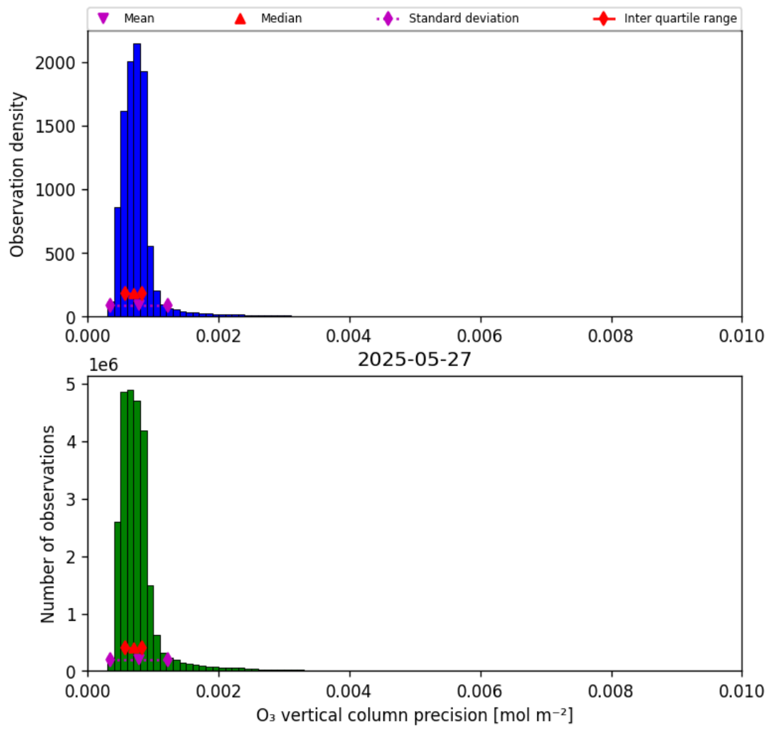
Figure 22: Histogram of “O 3 vertical column precision” for 2025-05-26 to 2025-05-28
