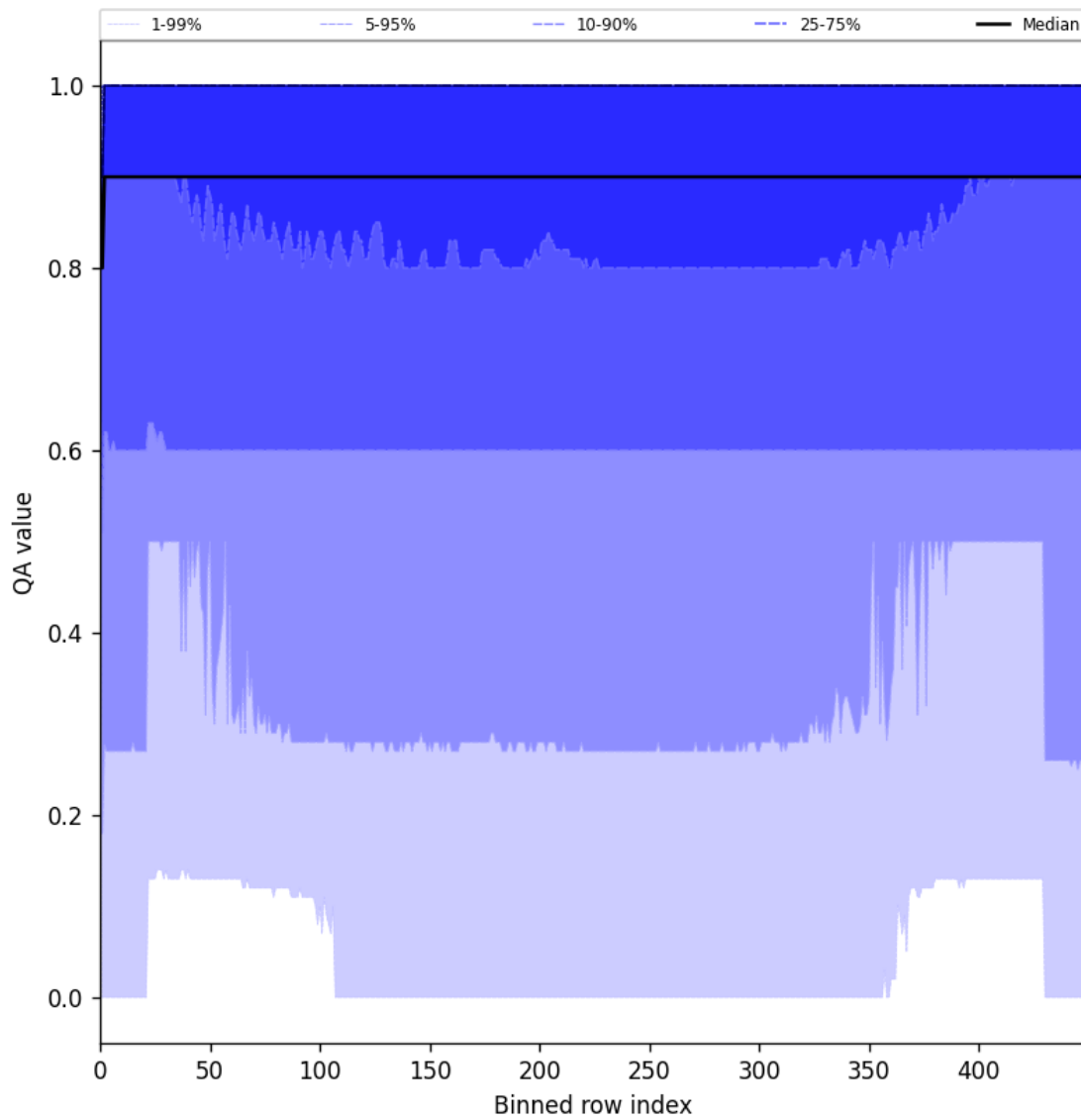
Figure 27: Along track statistics of “QA value” for 2025-05-26 to 2025-05-28
