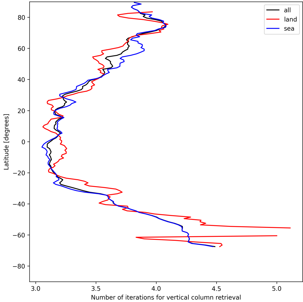
Figure 19: Zonal average of “Number of iterations for vertical column retrieval” for 2025-05-26 to 2025-05-28.
