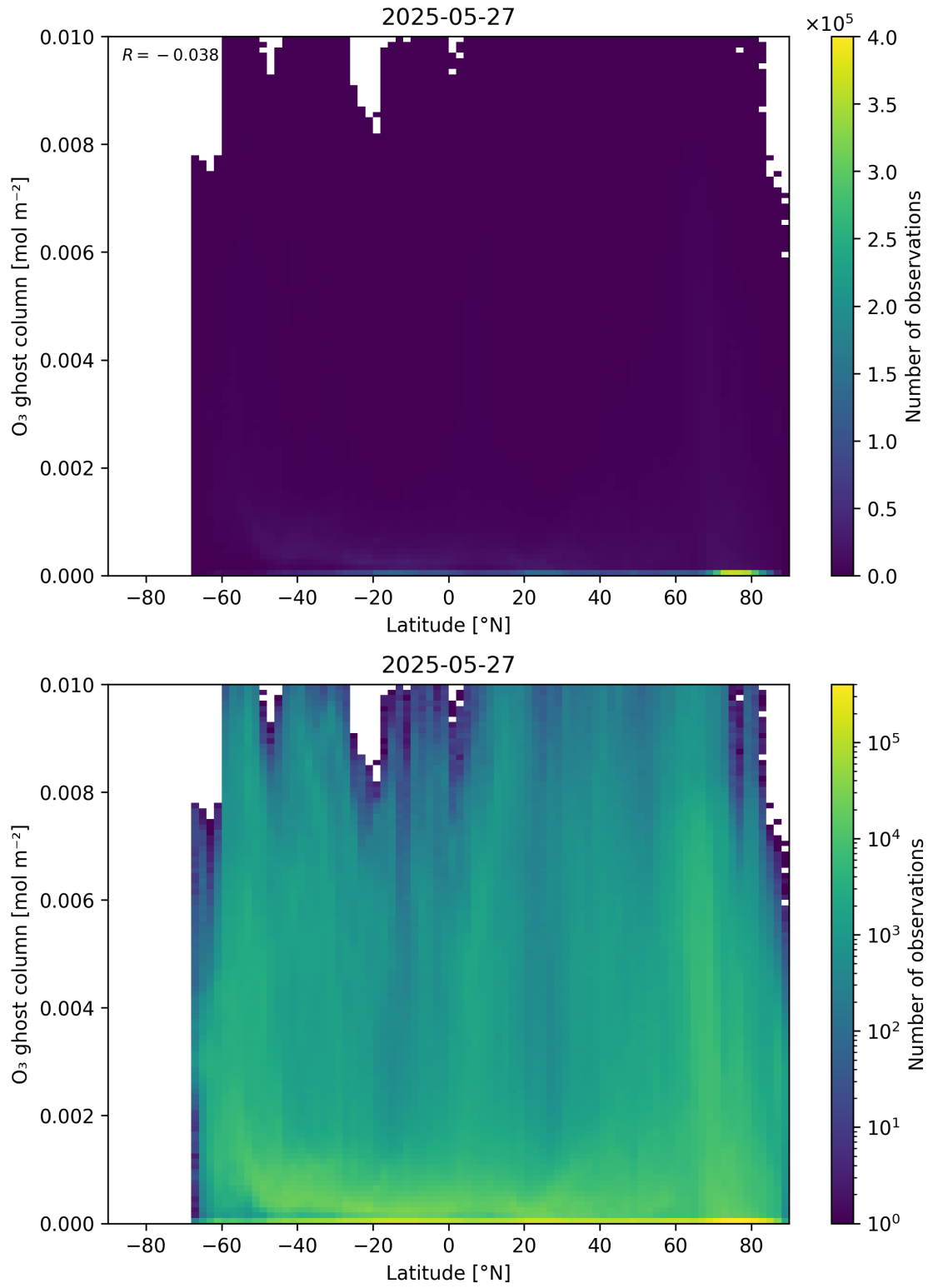
Figure 35: Scatter density plot of “Latitude” against “O 3 ghost column” for 2025-05-26 to 2025-05-28.
