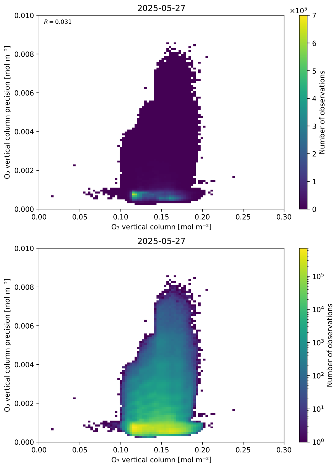
Figure 41: Scatter density plot of “O 3 vertical column” against “O 3 vertical column precision” for 2025-05-26 to 2025-05-28.
