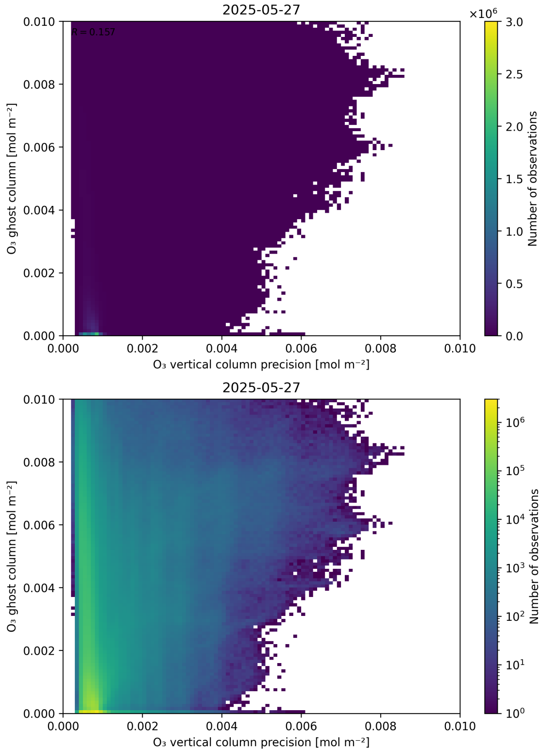
Figure 43: Scatter density plot of “ \text{O}_3 vertical column precision” against “ \text{O}_3 ghost column” for 2025-05-26 to 2025-05-28.
