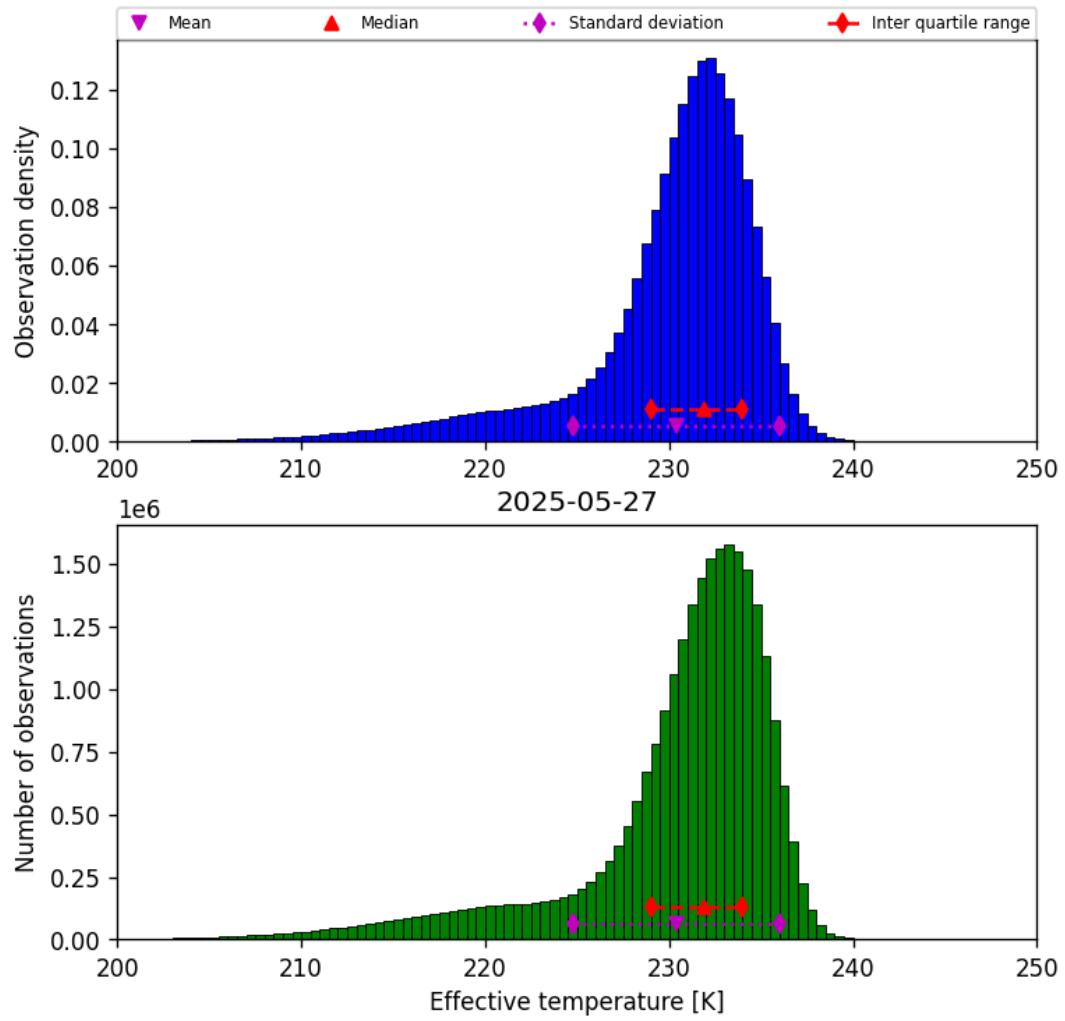
Figure 24: Histogram of “Effective temperature” for 2025-05-26 to 2025-05-28
