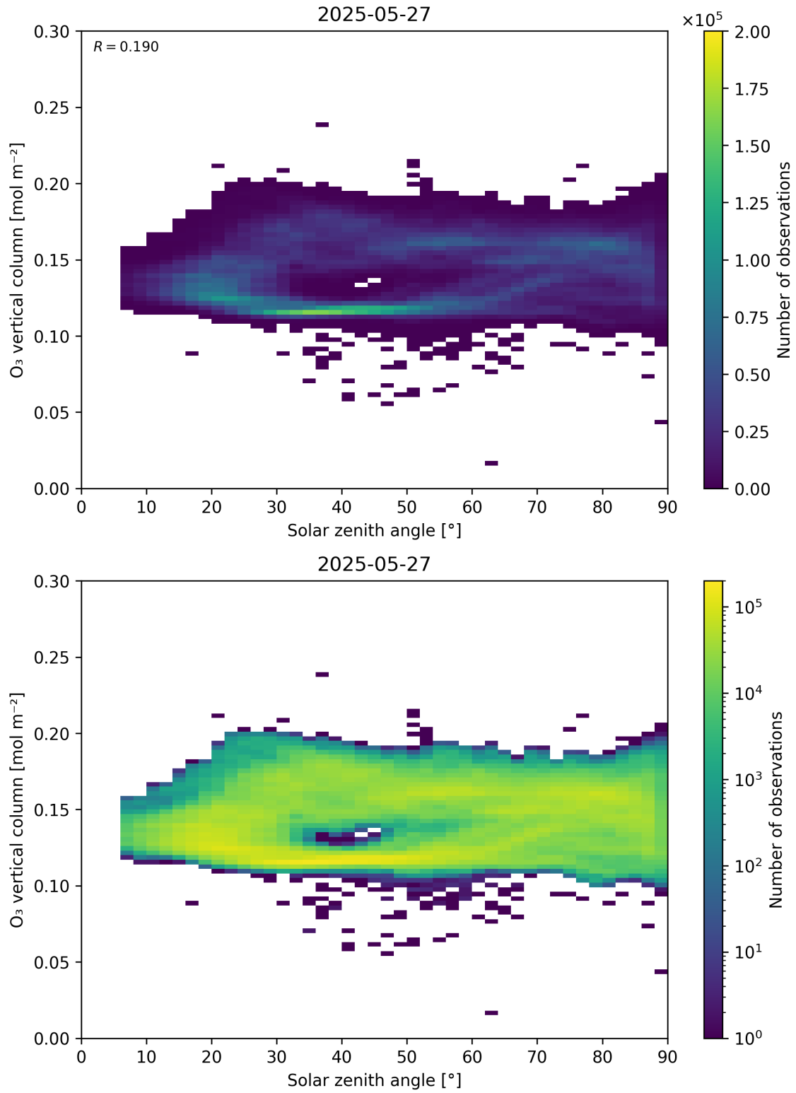
Figure 47: Scatter density plot of “Solar zenith angle” against “O 3 vertical column” for 2025-05-26 to 2025-05-28.
