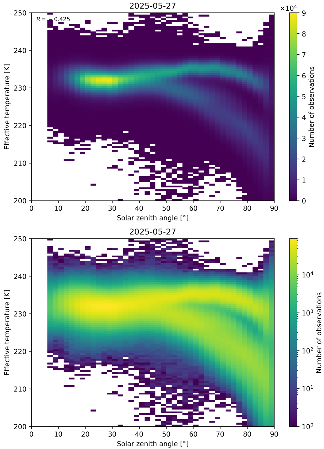
Figure 45: Scatter density plot of “Solar zenith angle” against “Effective temperature” for 2025-05-26 to 2025-05-28.
