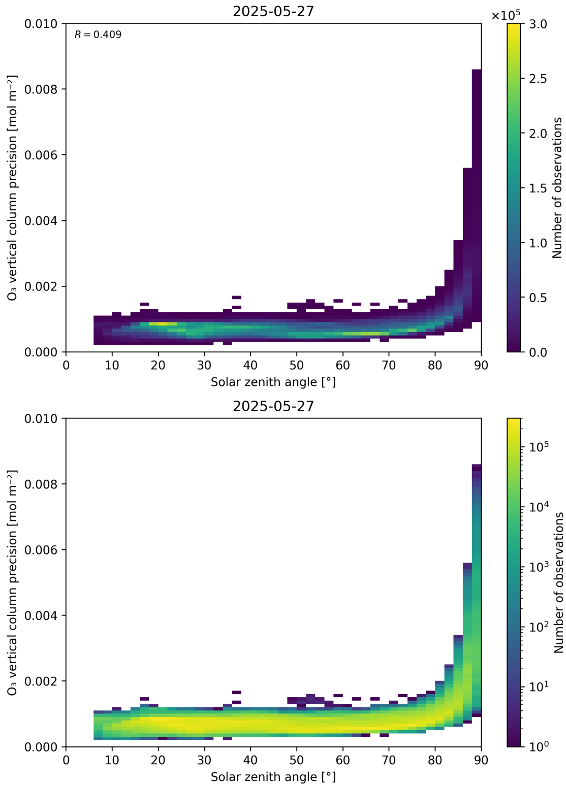
Figure 48: Scatter density plot of “Solar zenith angle” against “O 3 vertical column precision” for 2025-05-26 to 2025-05-28.
