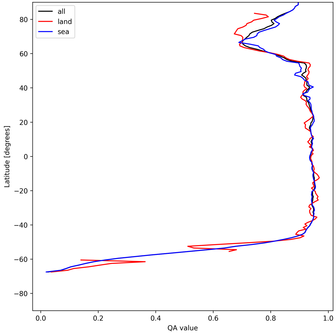
Figure 13: Zonal average of “QA value” for 2025-05-26 to 2025-05-28.
