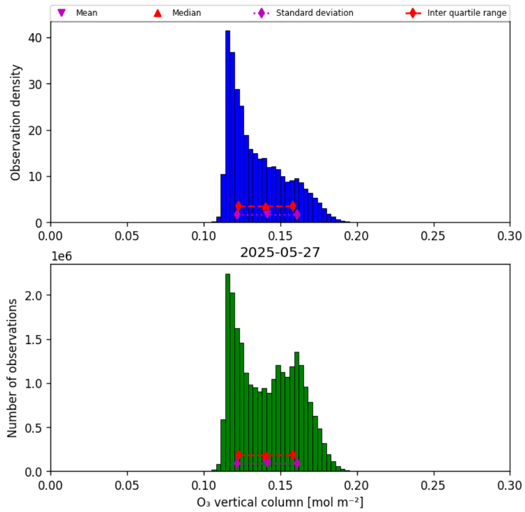
Figure 21: Histogram of “O 3 vertical column” for 2025-05-26 to 2025-05-28
