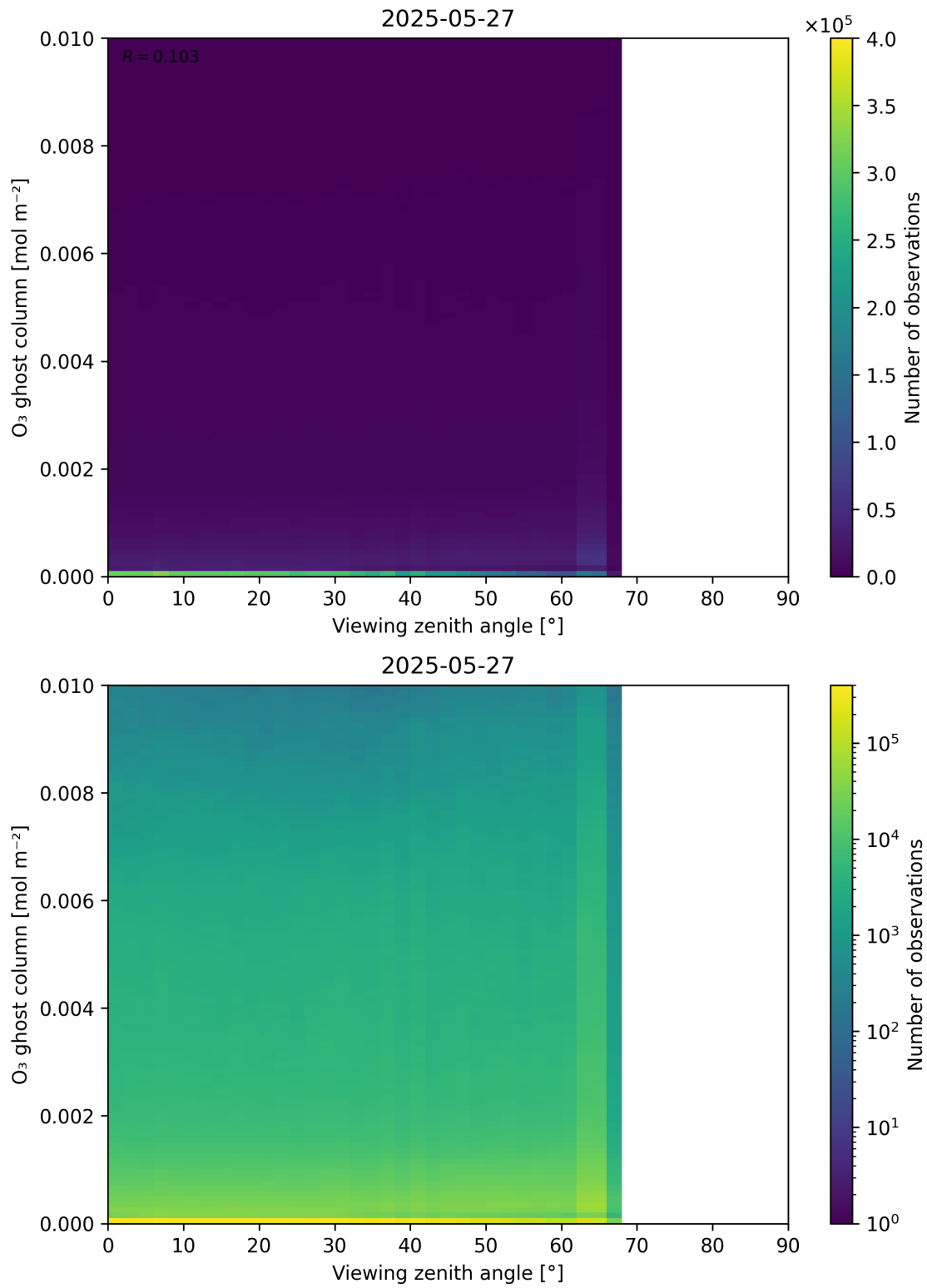
Figure 51: Scatter density plot of “Viewing zenith angle” against “O 3 ghost column” for 2025-05-26 to 2025-05-28.
