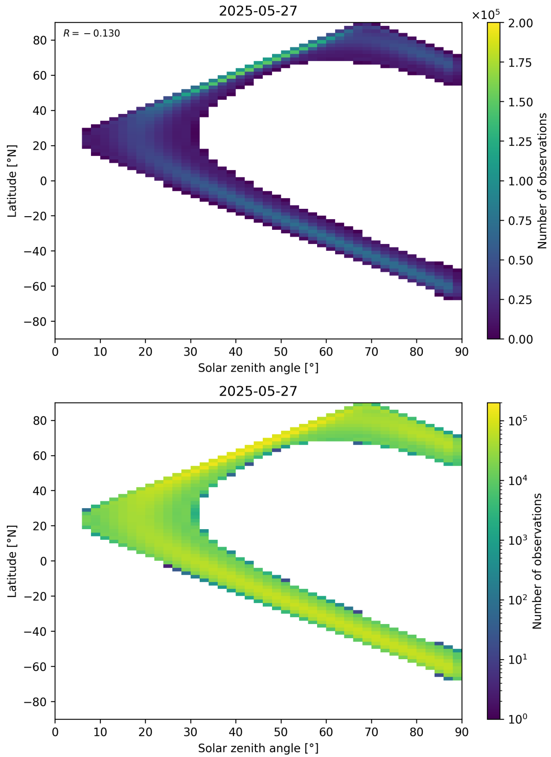
Figure 44: Scatter density plot of “Solar zenith angle” against “Latitude” for 2025-05-26 to 2025-05-28.
