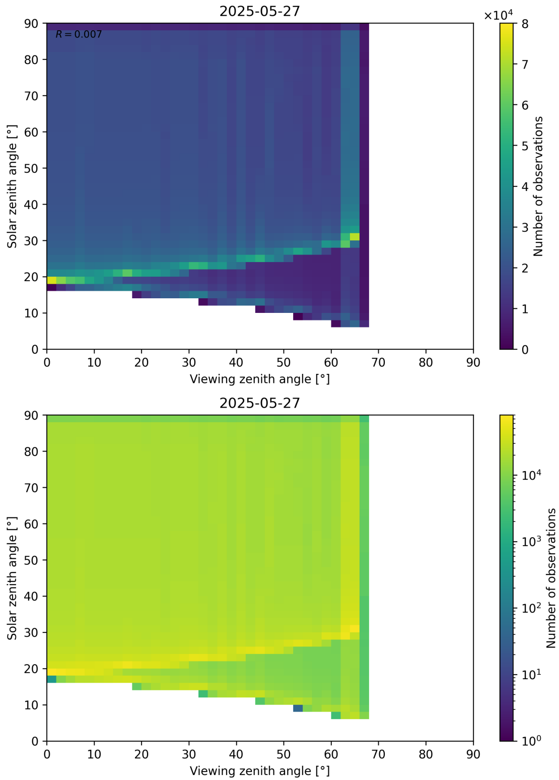
Figure 54: Scatter density plot of “Viewing zenith angle” against “Solar zenith angle” for 2025-05-26 to 2025-05-28.
