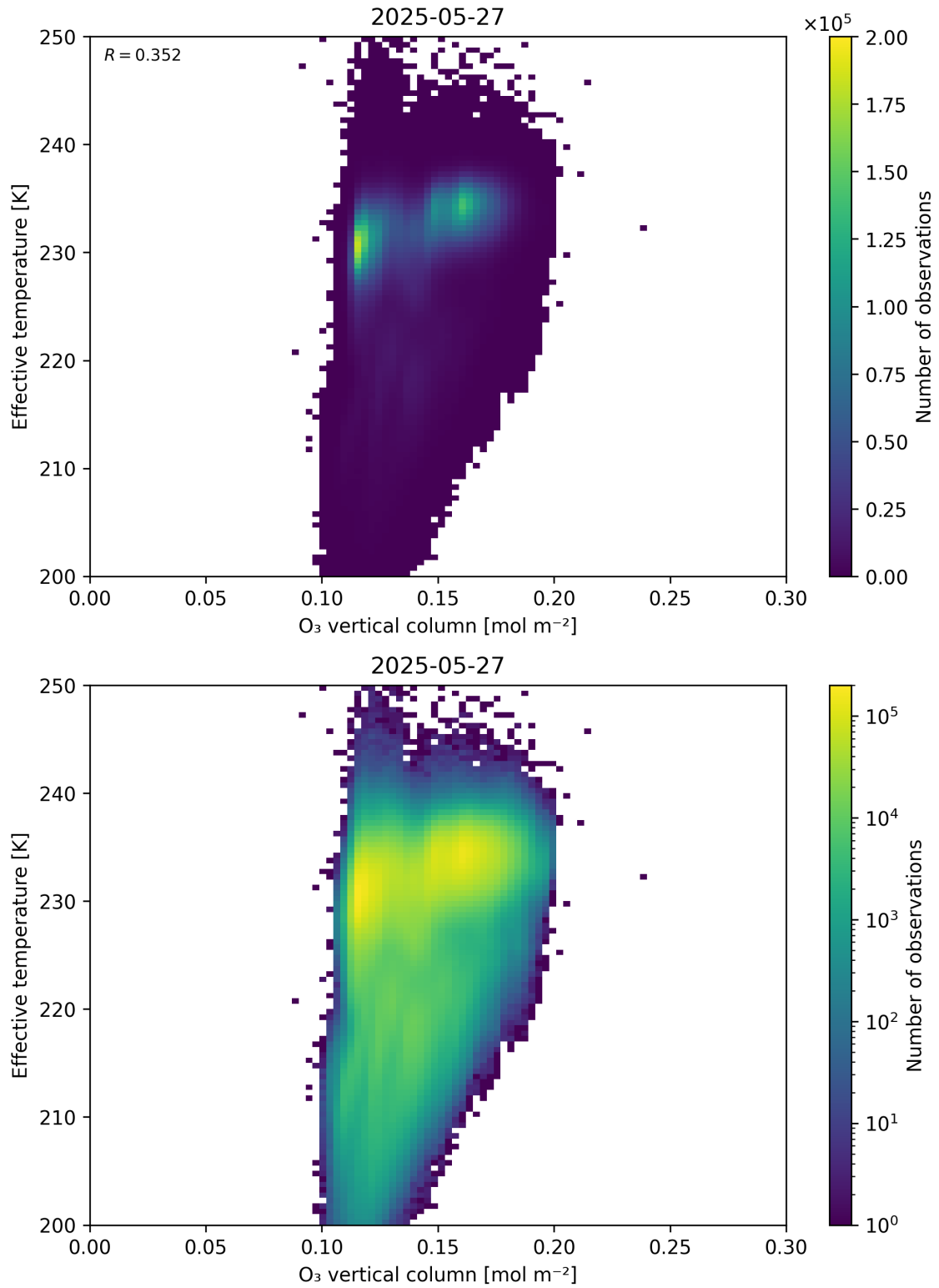
Figure 39: Scatter density plot of “O 3 vertical column” against “Effective temperature” for 2025-05-26 to 2025-05-28.
