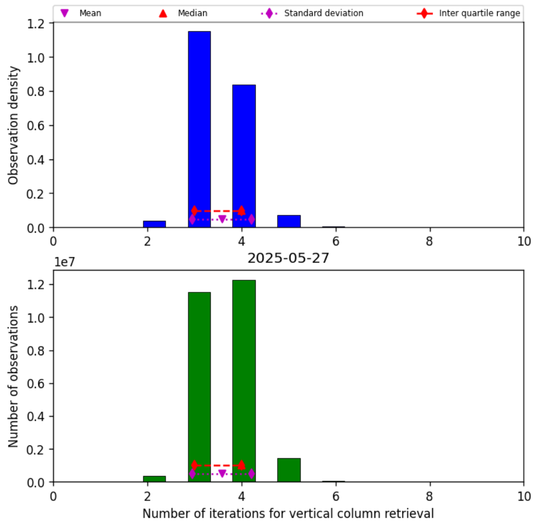
Figure 26: Histogram of “Number of iterations for vertical column retrieval” for 2025-05-26 to 2025-05-28
