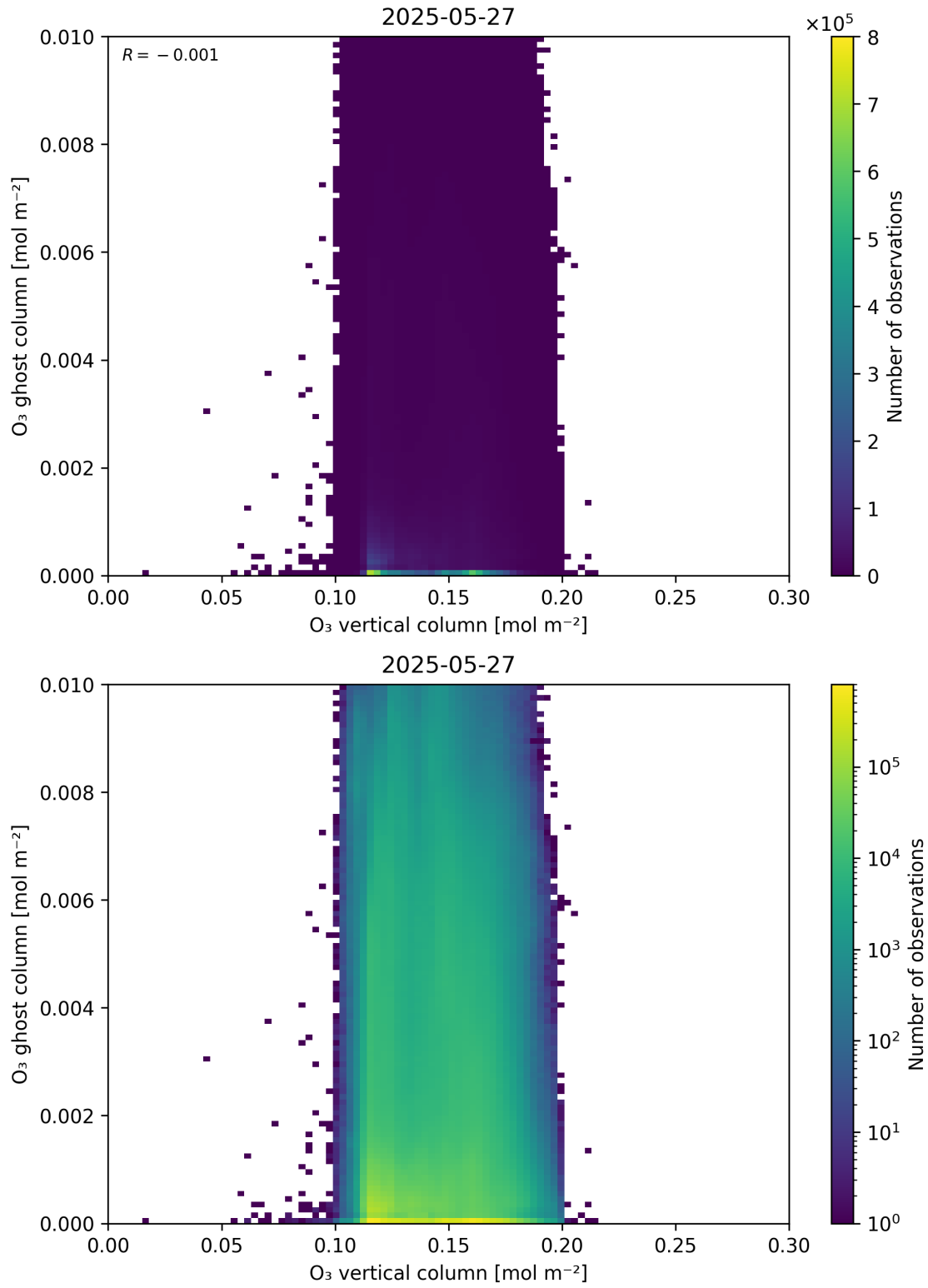
Figure 40: Scatter density plot of “O 3 vertical column” against “O 3 ghost column” for 2025-05-26 to 2025-05-28.
