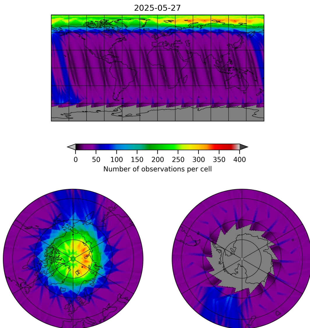
Figure 12: Map of the number of observations for 2025-05-26 to 2025-05-28
