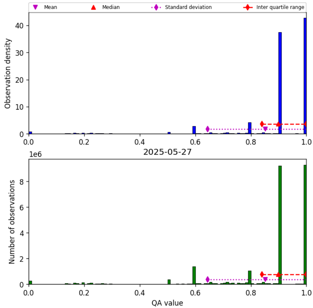
Figure 20: Histogram of “QA value” for 2025-05-26 to 2025-05-28
