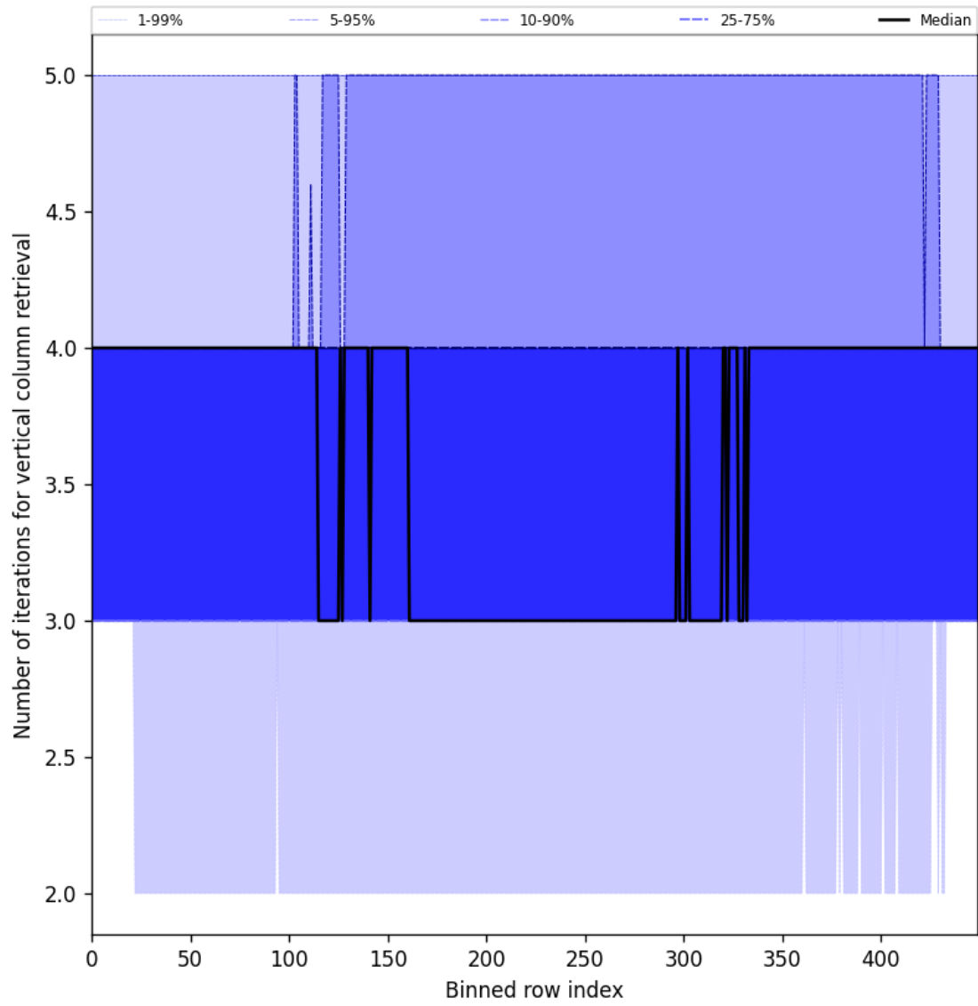
Figure 33: Along track statistics of “Number of iterations for vertical column retrieval” for 2025-05-26 to 2025-05-28
