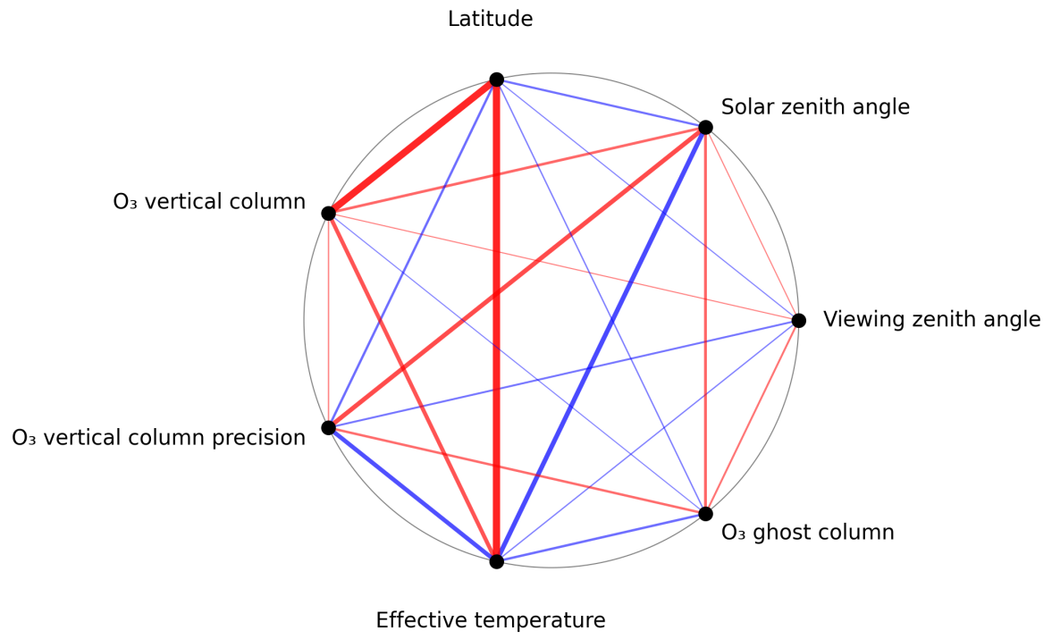
Figure 1: Map of correlation graph for 2025-05-26 to 2025-05-28.
