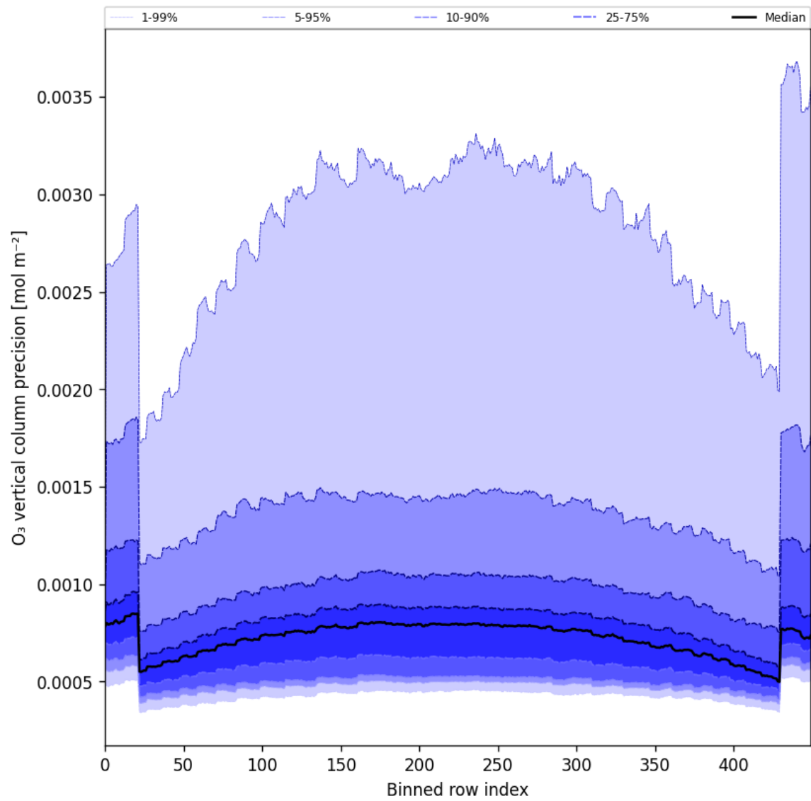
Figure 29: Along track statistics of “O 3 vertical column precision” for 2025-05-26 to 2025-05-28
