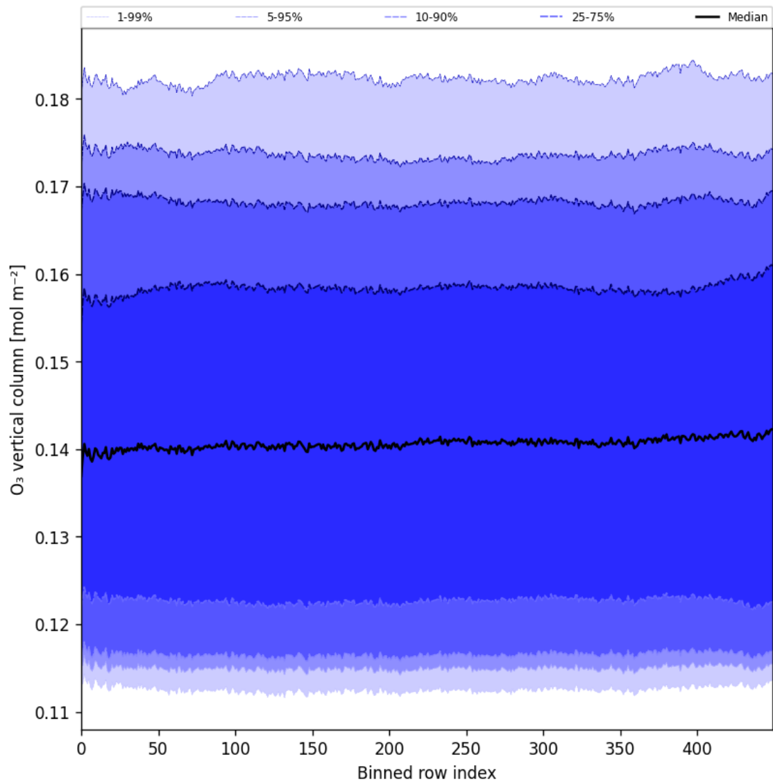
Figure 28: Along track statistics of “O 3 vertical column” for 2025-05-26 to 2025-05-28
