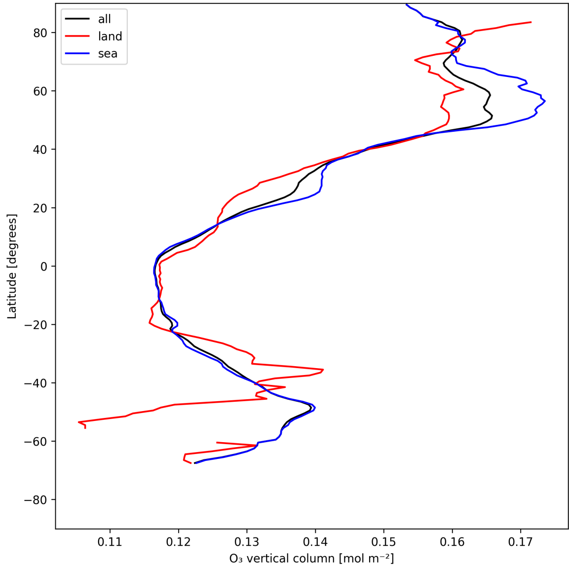
Figure 14: Zonal average of “O 3 vertical column” for 2025-05-26 to 2025-05-28.
