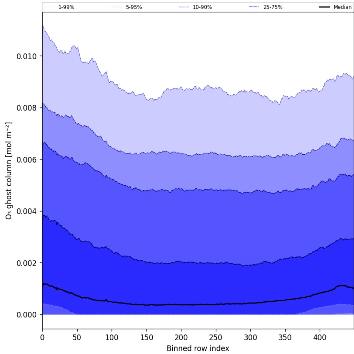
Figure 32: Along track statistics of “O 3 ghost column” for 2025-05-26 to 2025-05-28
