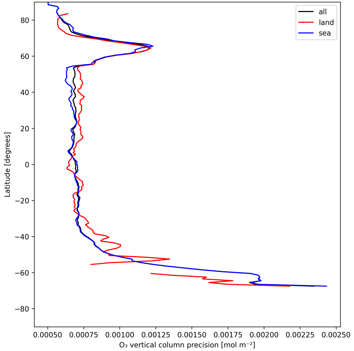
Figure 15: Zonal average of “O 3 vertical column precision” for 2025-05-26 to 2025-05-28.
