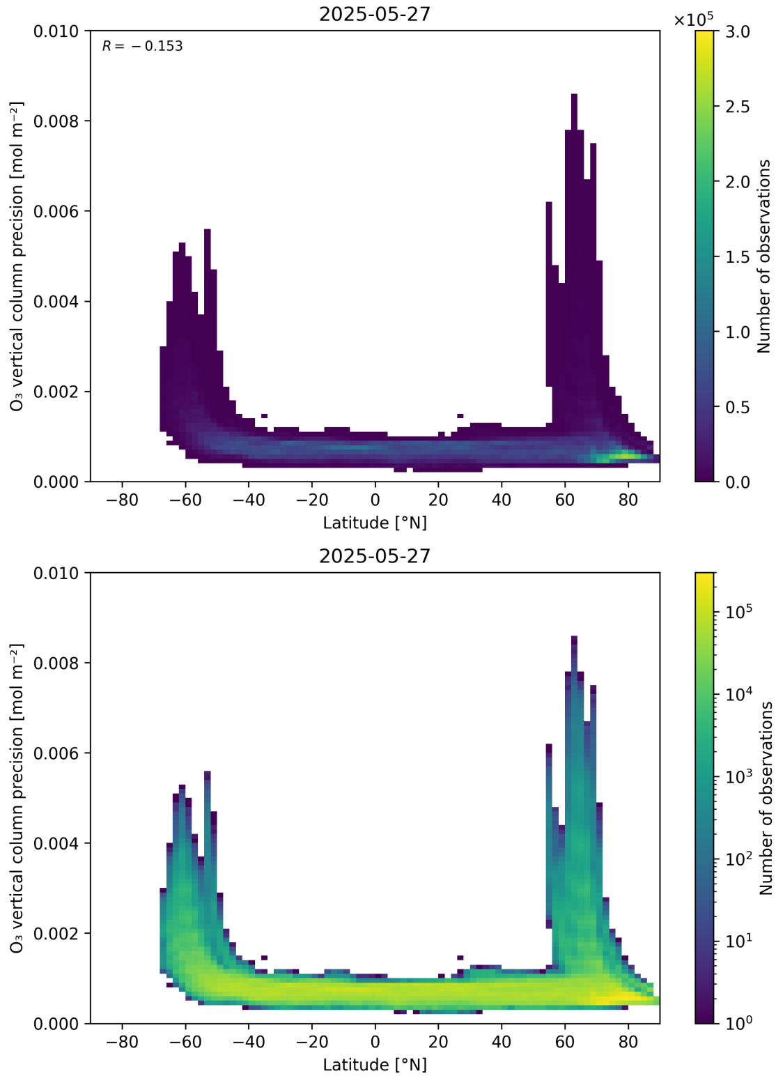
Figure 37: Scatter density plot of “Latitude” against “O 3 vertical column precision” for 2025-05-26 to 2025-05-28.
