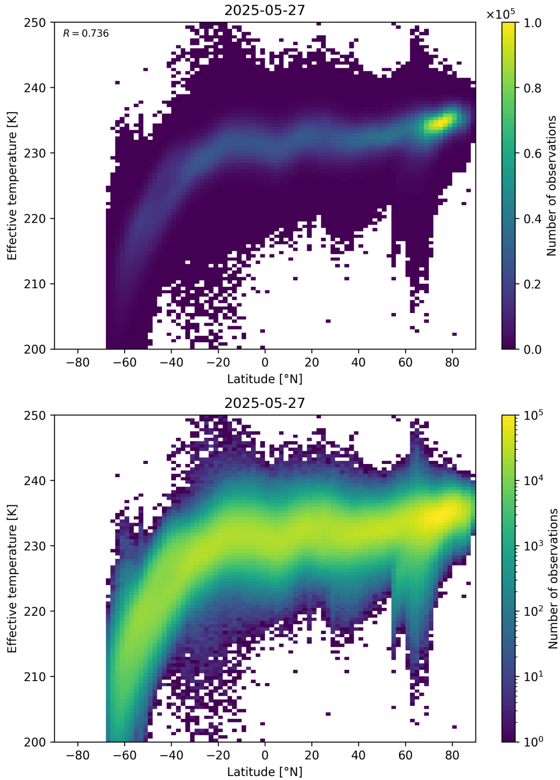
Figure 34: Scatter density plot of “Latitude” against “Effective temperature” for 2025-05-26 to 2025-05-28.
