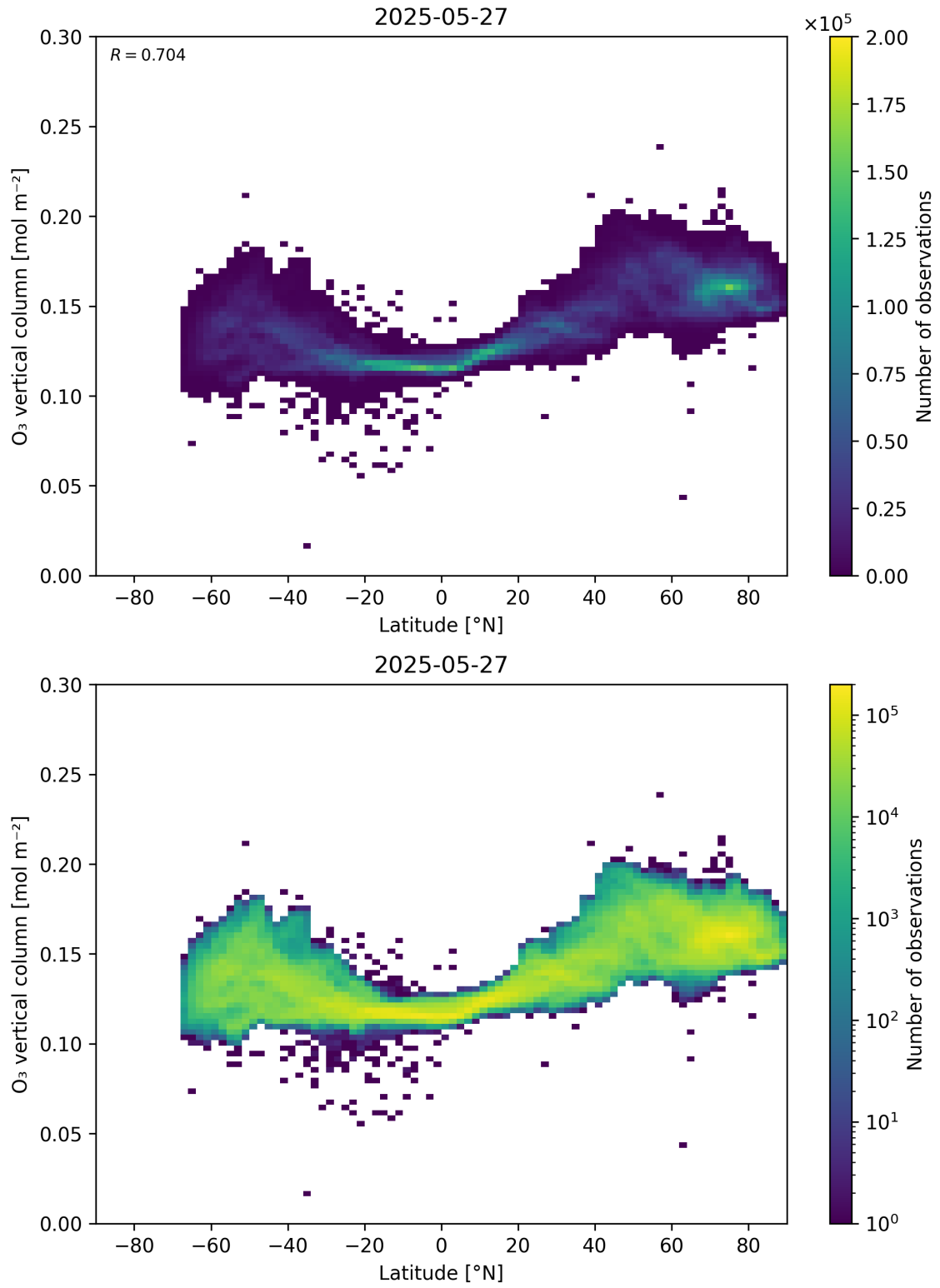
Figure 36: Scatter density plot of “Latitude” against “O 3 vertical column” for 2025-05-26 to 2025-05-28.
