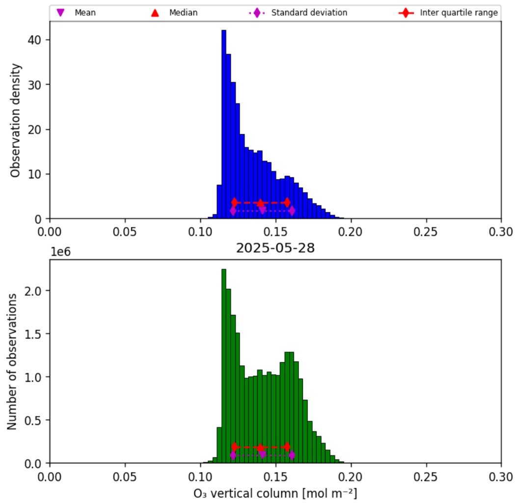
Figure 21: Histogram of “O 3 vertical column” for 2025-05-27 to 2025-05-29
