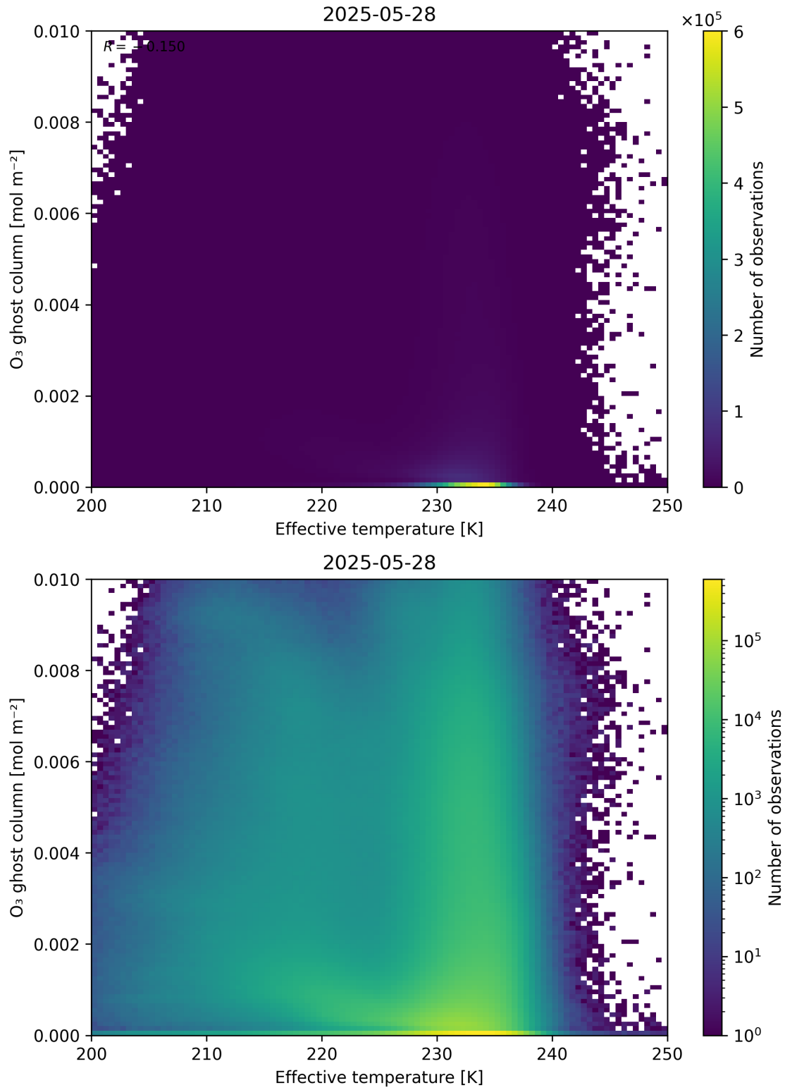
Figure 38: Scatter density plot of “Effective temperature” against “O 3 ghost column” for 2025-05-27 to 2025-05-29.
