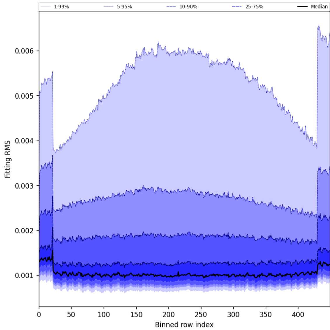
Figure 30: Along track statistics of “Fitting RMS” for 2025-05-27 to 2025-05-29
