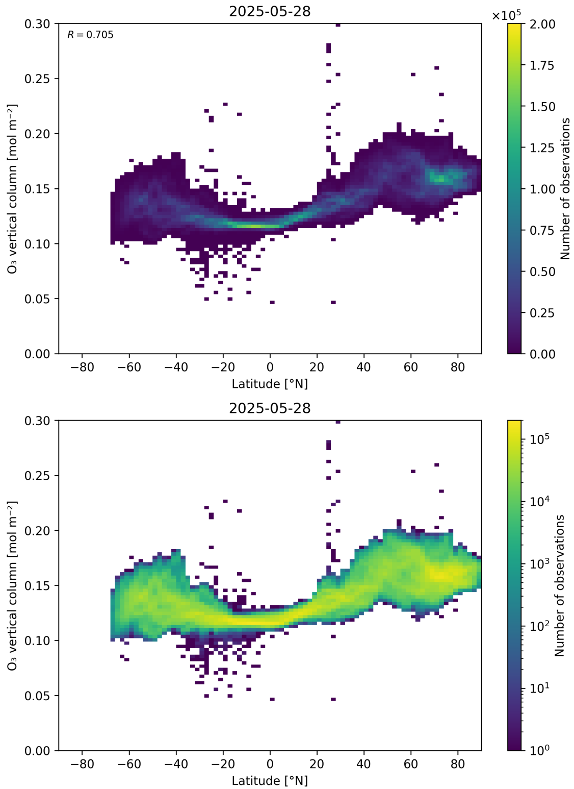
Figure 36: Scatter density plot of “Latitude” against “O 3 vertical column” for 2025-05-27 to 2025-05-29.
