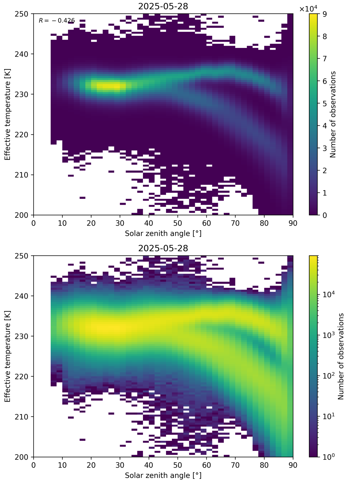
Figure 45: Scatter density plot of “Solar zenith angle” against “Effective temperature” for 2025-05-27 to 2025-05-29.
