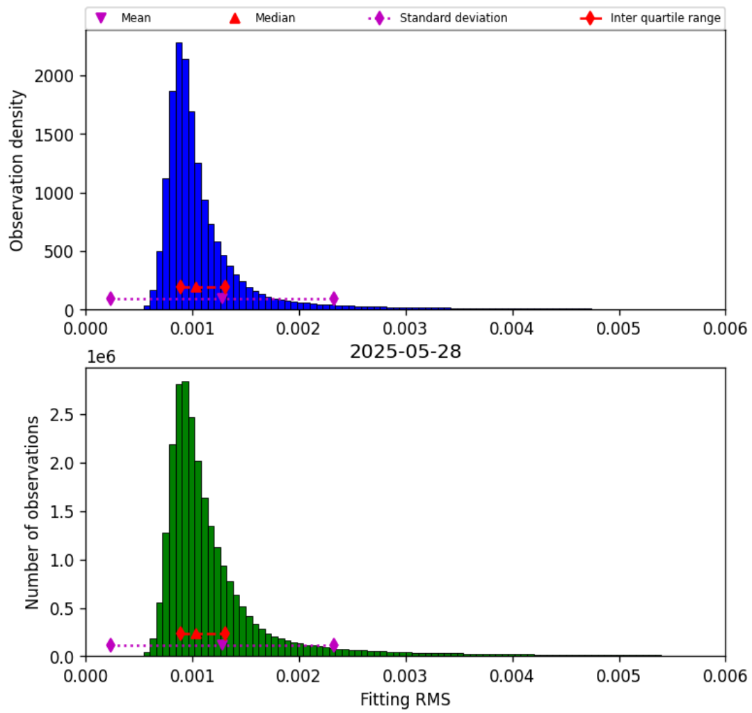
Figure 23: Histogram of “Fitting RMS” for 2025-05-27 to 2025-05-29
