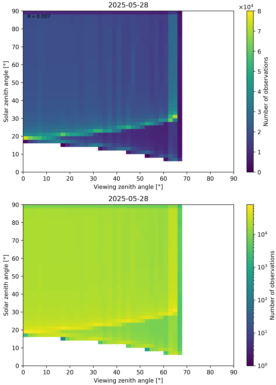
Figure 54: Scatter density plot of “Viewing zenith angle” against “Solar zenith angle” for 2025-05-27 to 2025-05-29.
