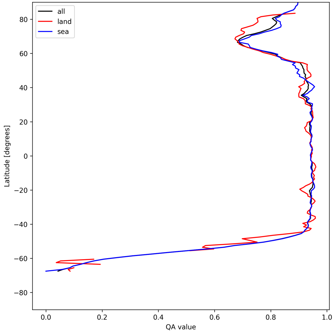
Figure 13: Zonal average of “QA value” for 2025-05-27 to 2025-05-29.
