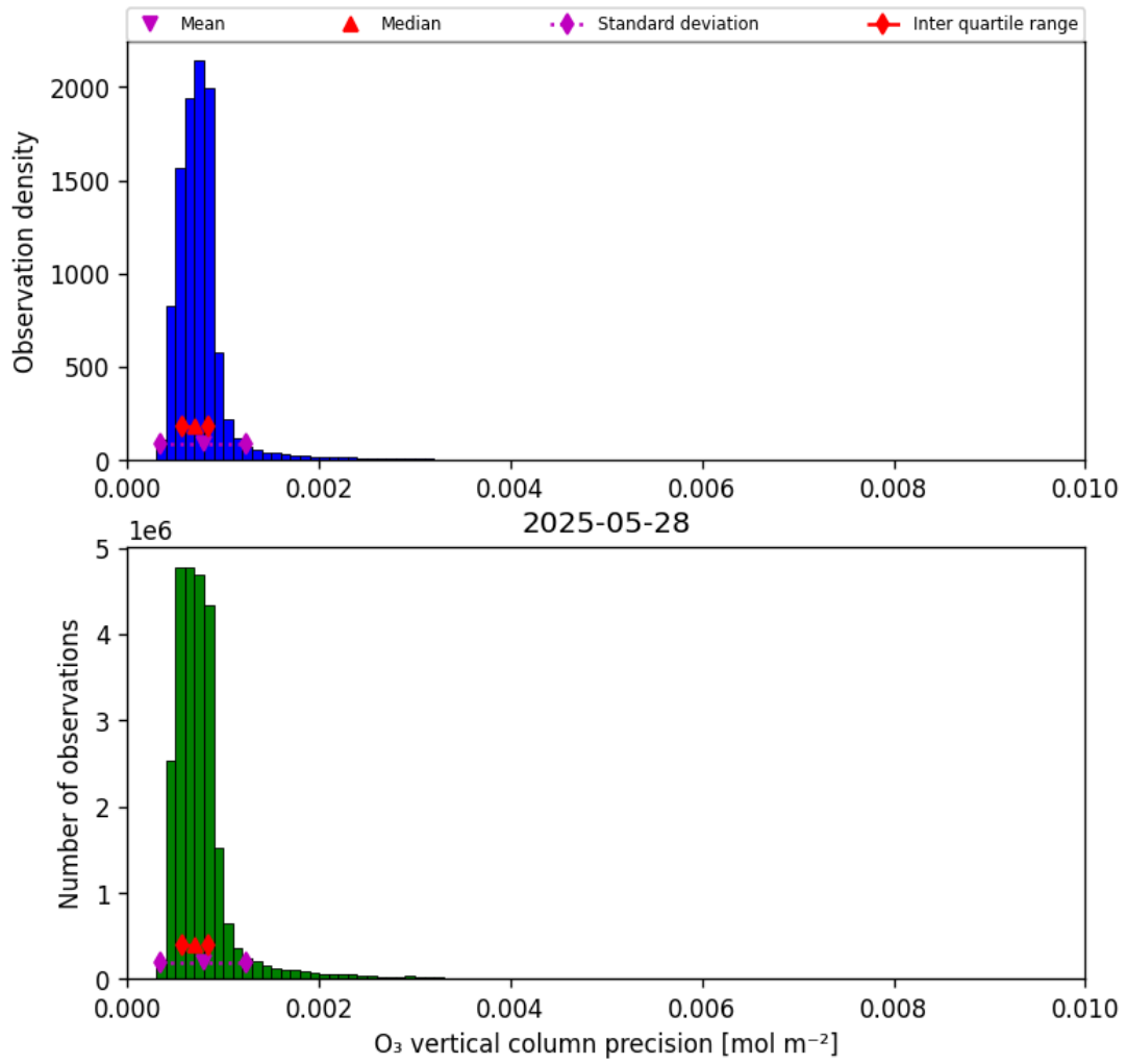
Figure 22: Histogram of “O 3 vertical column precision” for 2025-05-27 to 2025-05-29
