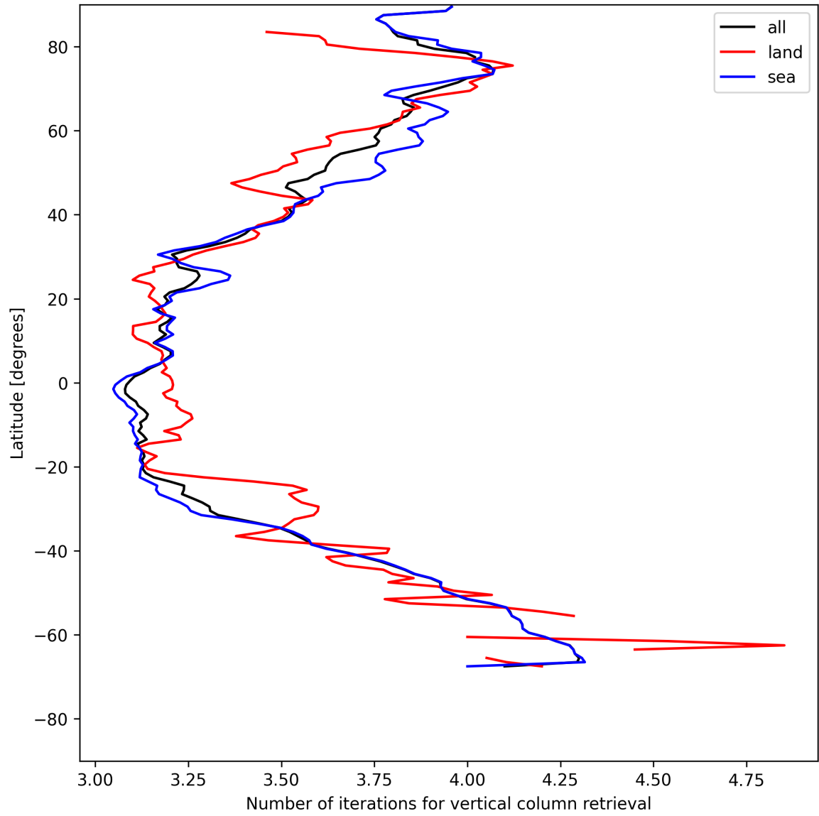
Figure 19: Zonal average of “Number of iterations for vertical column retrieval” for 2025-05-27 to 2025-05-29.
