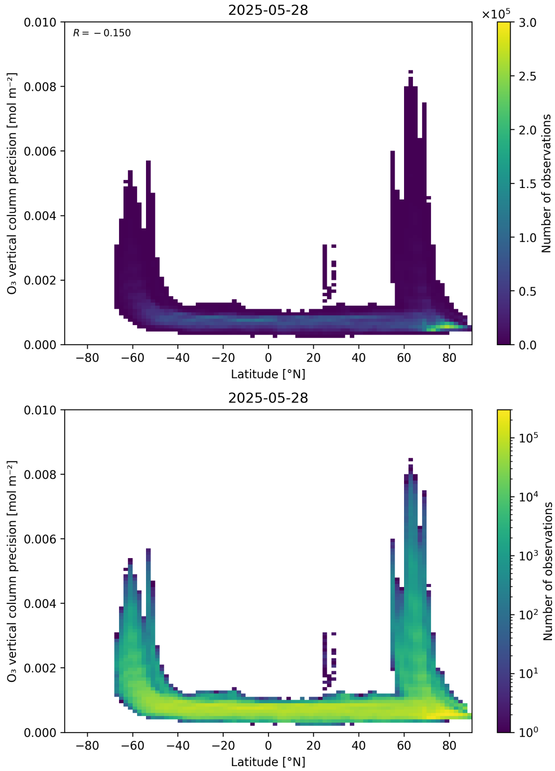
Figure 37: Scatter density plot of “Latitude” against “O 3 vertical column precision” for 2025-05-27 to 2025-05-29.
