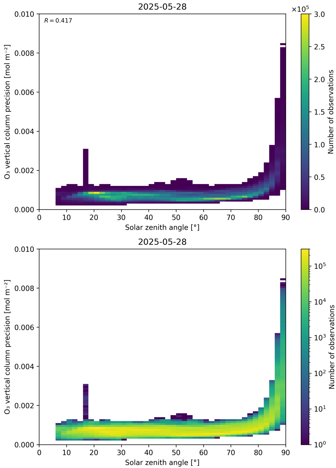
Figure 48: Scatter density plot of “Solar zenith angle” against “O 3 vertical column precision” for 2025-05-27 to 2025-05-29.
