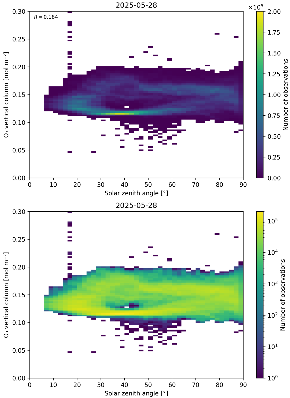
Figure 47: Scatter density plot of “Solar zenith angle” against “O 3 vertical column” for 2025-05-27 to 2025-05-29.
