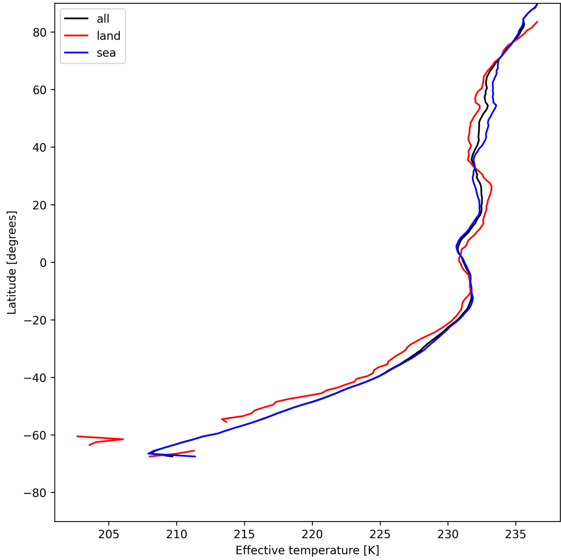
Figure 17: Zonal average of "Effective temperature" for 2025-05-27 to 2025-05-29.
