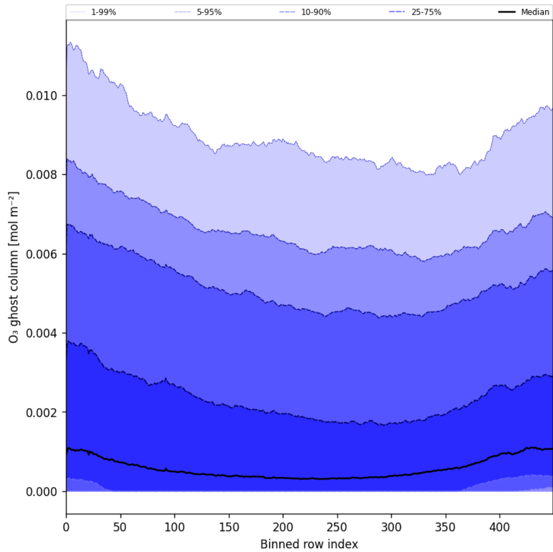
Figure 32: Along track statistics of “O 3 ghost column” for 2025-05-27 to 2025-05-29
