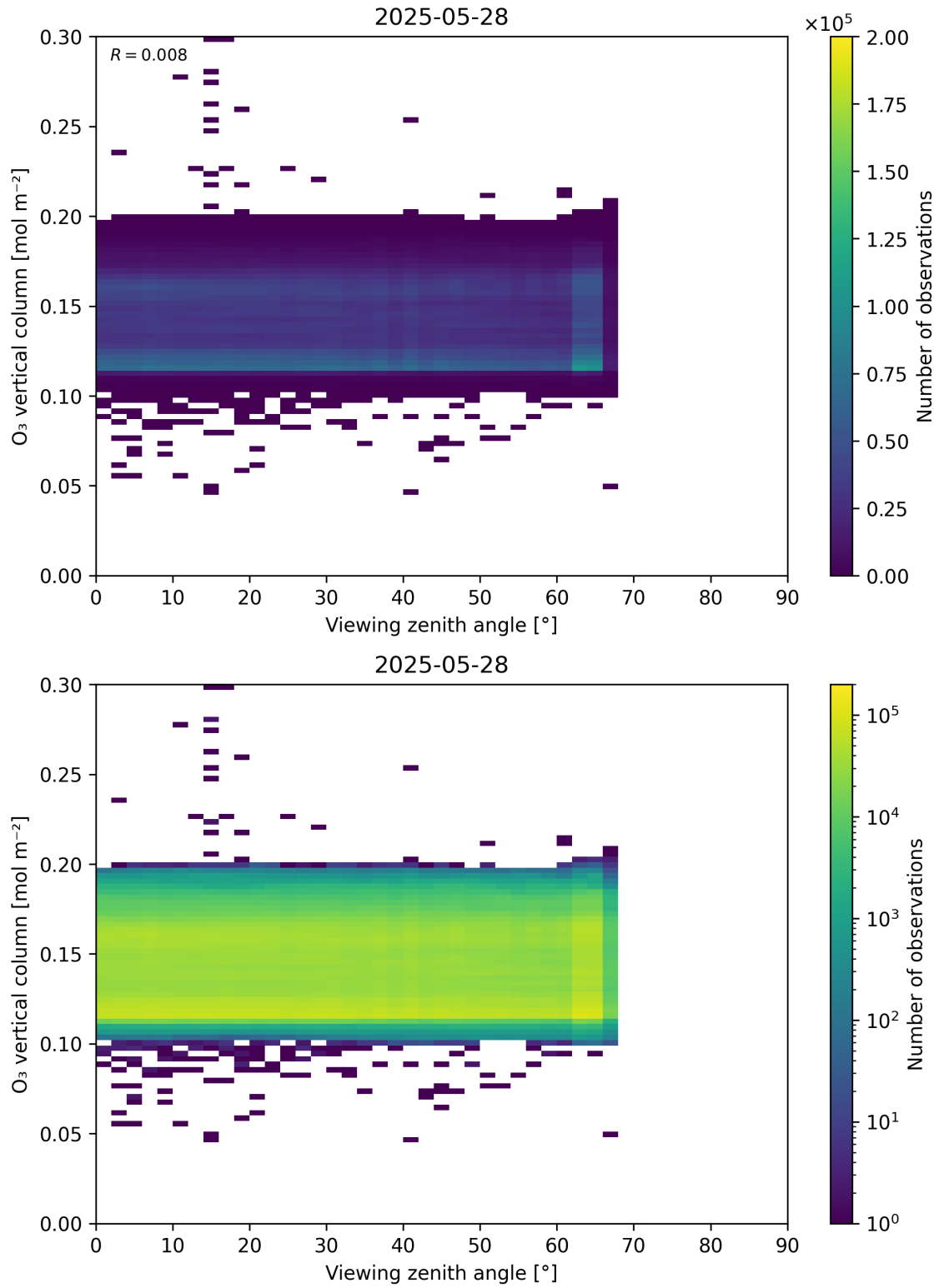
Figure 52: Scatter density plot of “Viewing zenith angle” against “O 3 vertical column” for 2025-05-27 to 2025-05-29.
