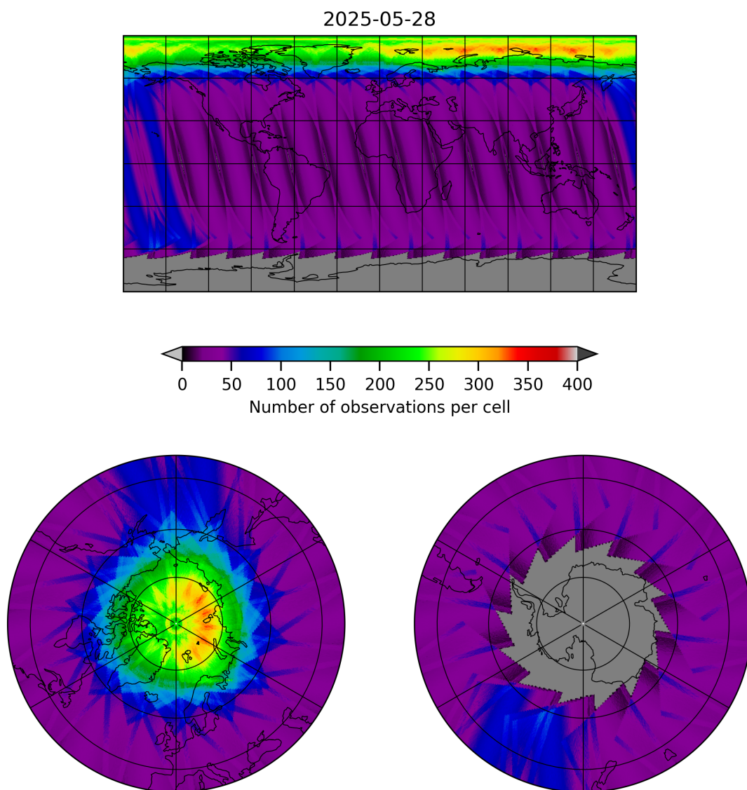
Figure 12: Map of the number of observations for 2025-05-27 to 2025-05-29
