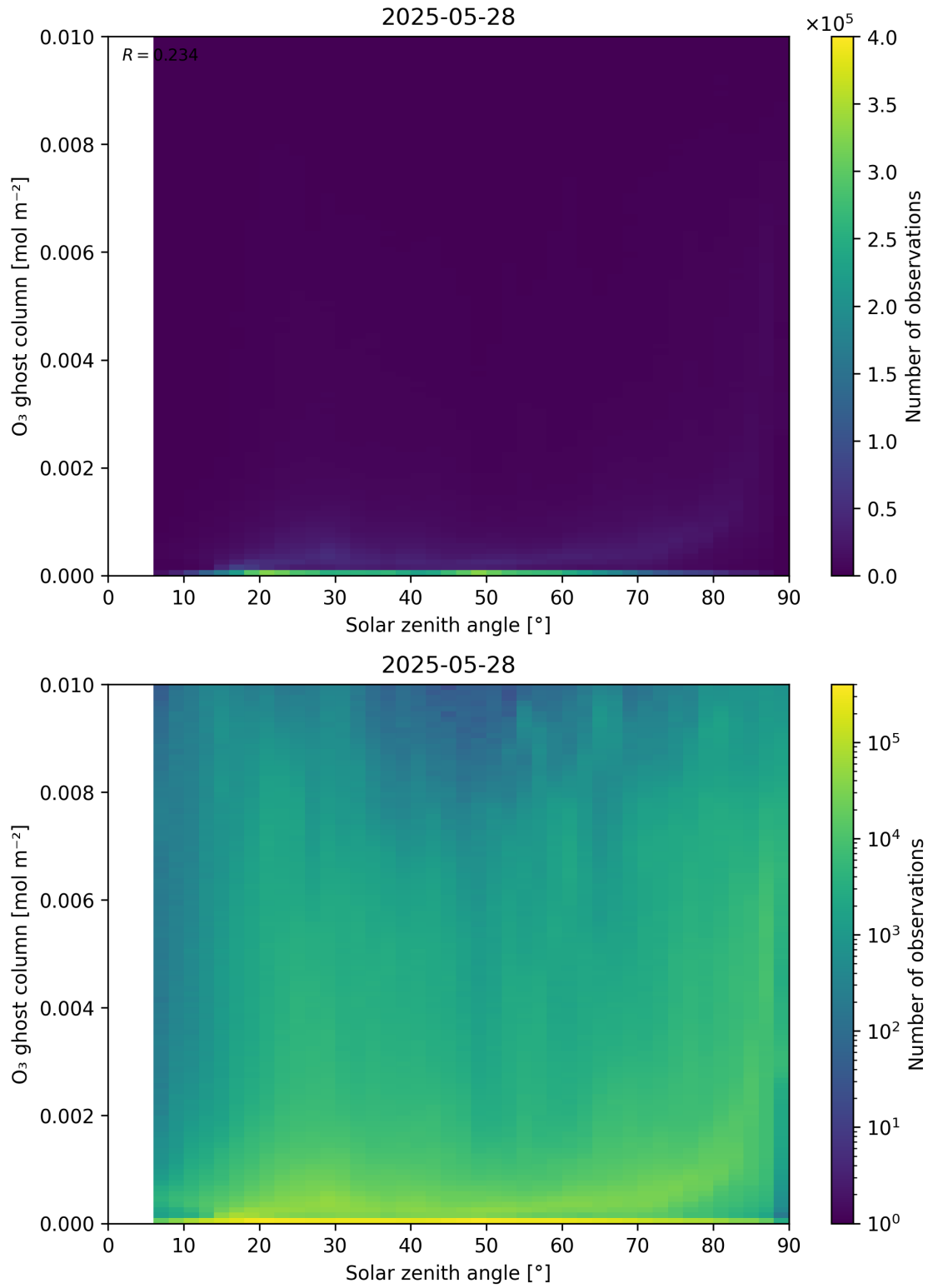
Figure 46: Scatter density plot of “Solar zenith angle” against “O 3 ghost column” for 2025-05-27 to 2025-05-29.
