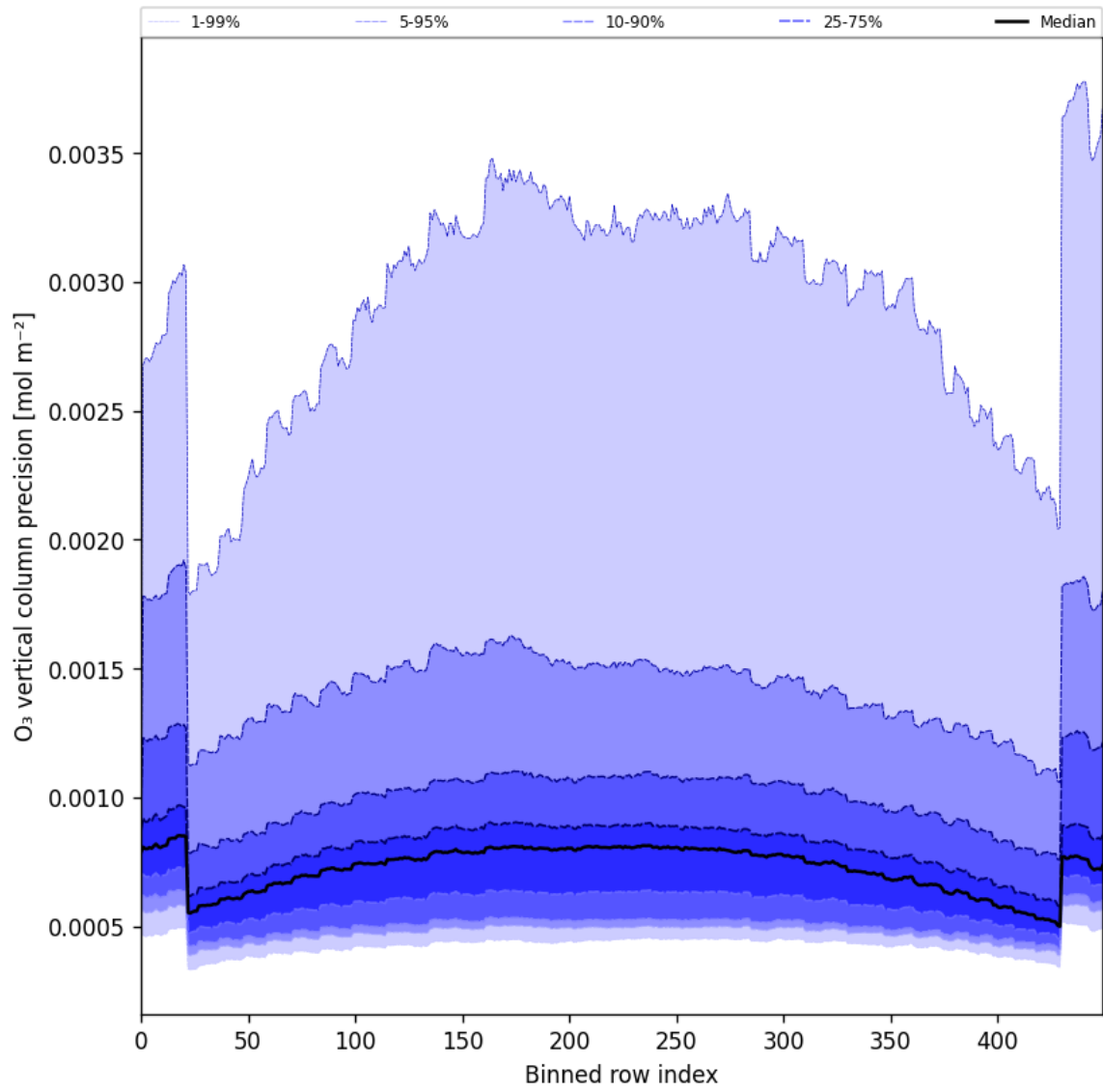
Figure 29: Along track statistics of “O 3 vertical column precision” for 2025-05-27 to 2025-05-29
