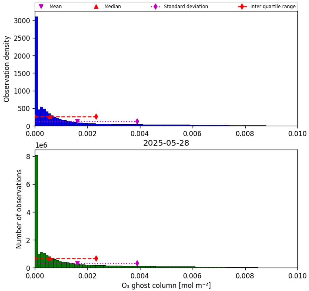
Figure 25: Histogram of “O 3 ghost column” for 2025-05-27 to 2025-05-29
