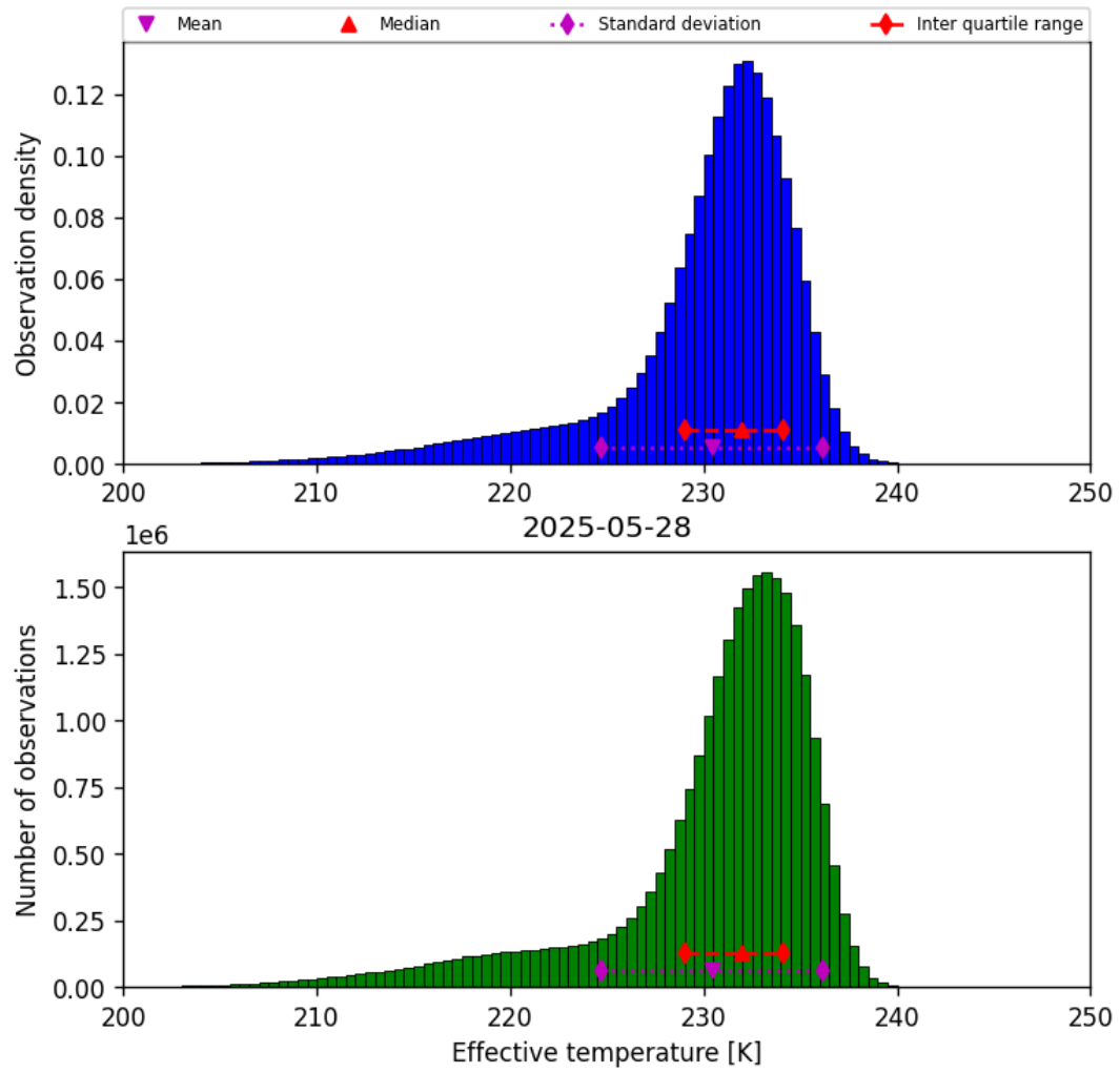
Figure 24: Histogram of “Effective temperature” for 2025-05-27 to 2025-05-29
