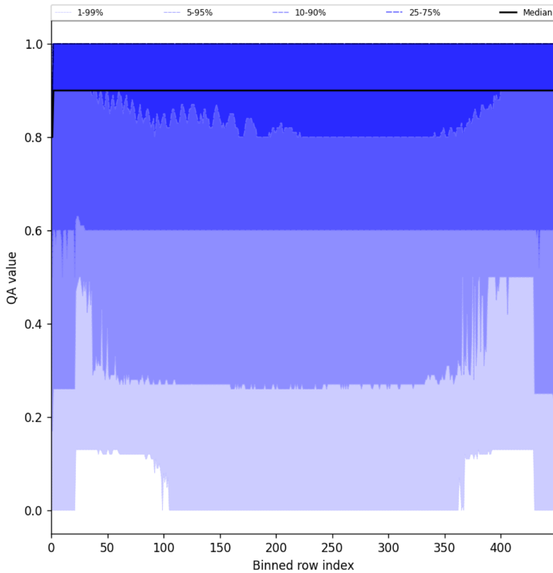
Figure 27: Along track statistics of “QA value” for 2025-05-27 to 2025-05-29
