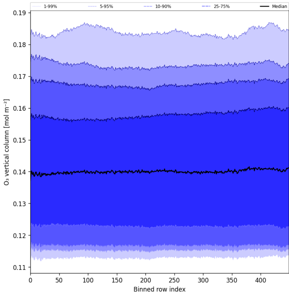
Figure 28: Along track statistics of “ \text{O}_3 vertical column” for 2025-05-27 to 2025-05-29
