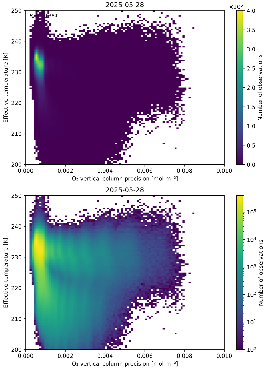
Figure 42: Scatter density plot of “O 3 vertical column precision” against “Effective temperature” for 2025-05-27 to 2025-05-29.
