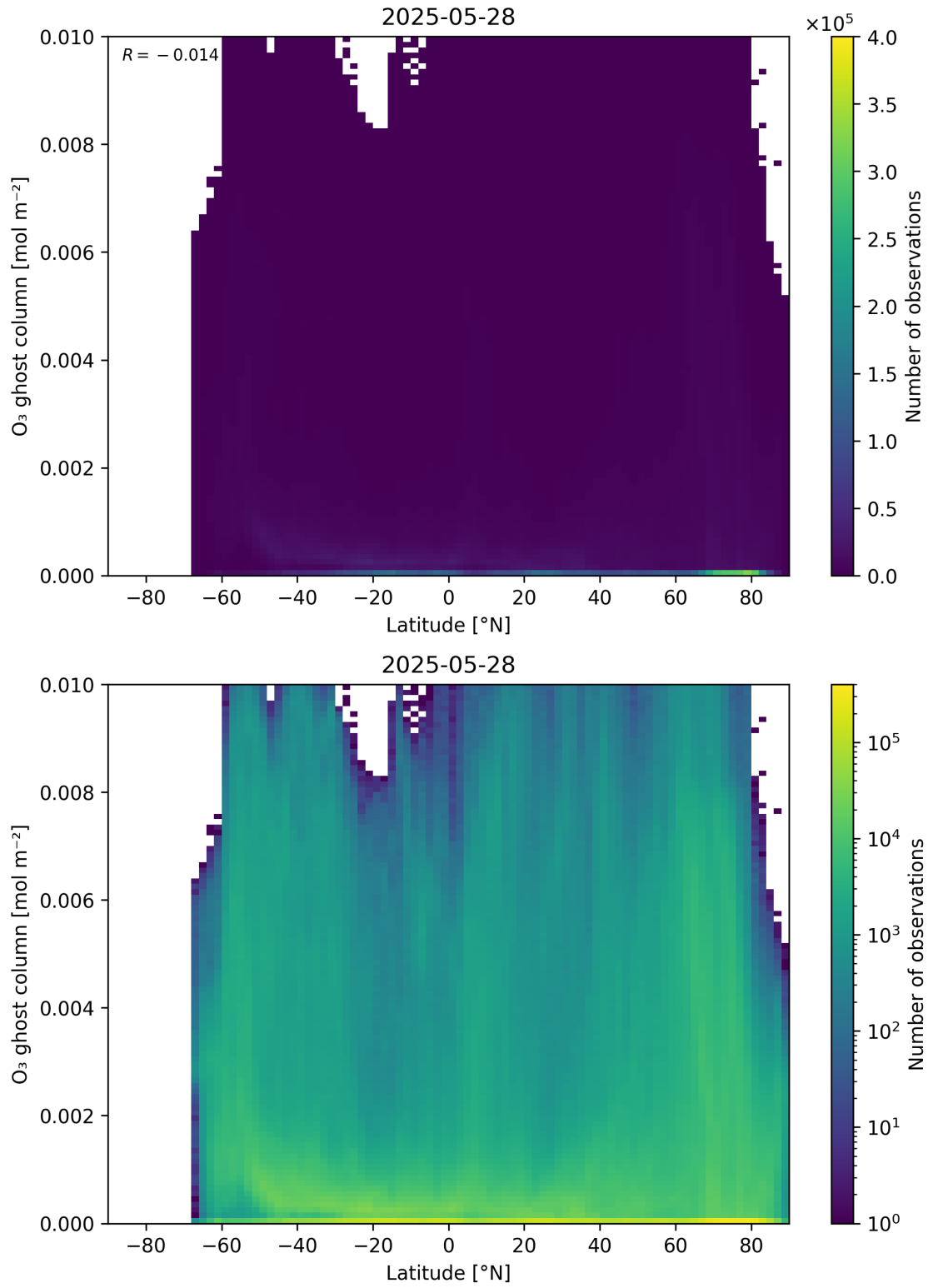
Figure 35: Scatter density plot of “Latitude” against “O 3 ghost column” for 2025-05-27 to 2025-05-29.
