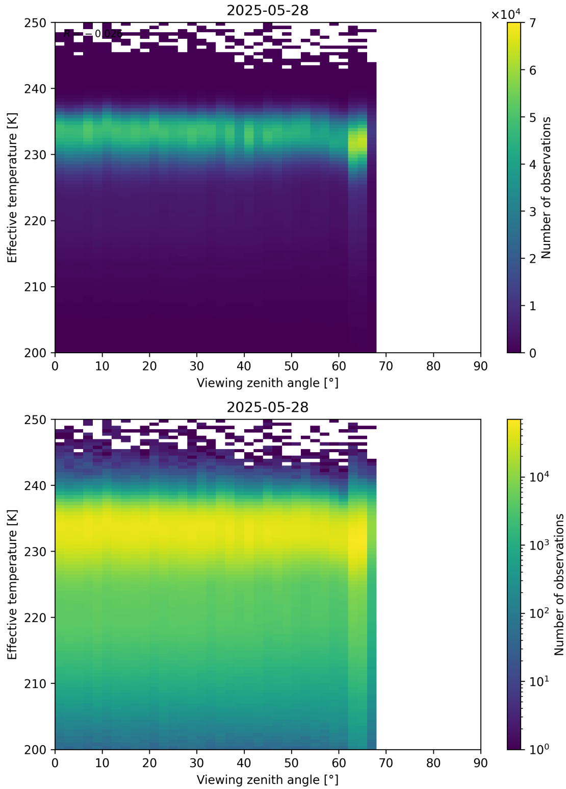
Figure 50: Scatter density plot of “Viewing zenith angle” against “Effective temperature” for 2025-05-27 to 2025-05-29.
