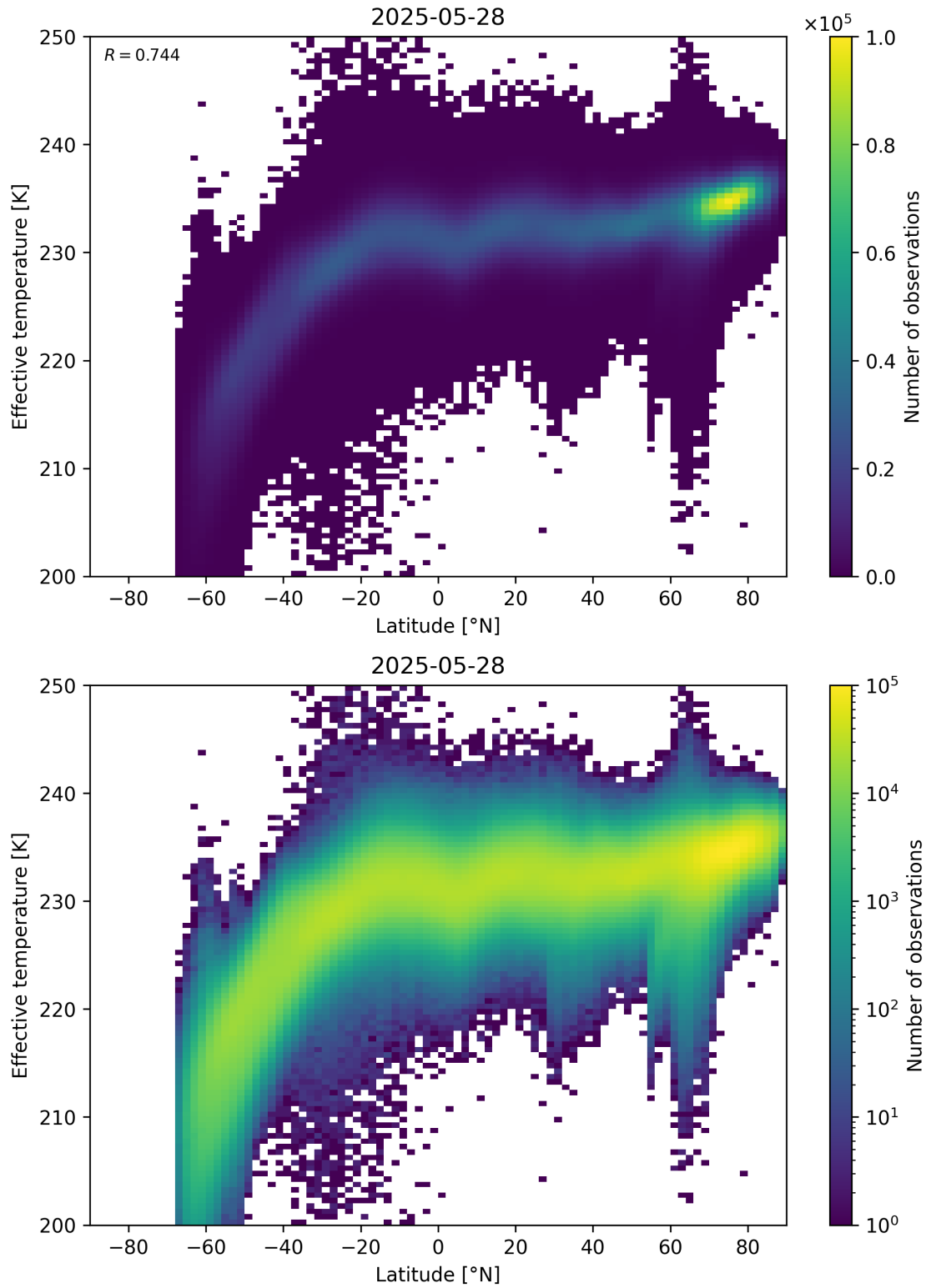
Figure 34: Scatter density plot of “Latitude” against “Effective temperature” for 2025-05-27 to 2025-05-29.
