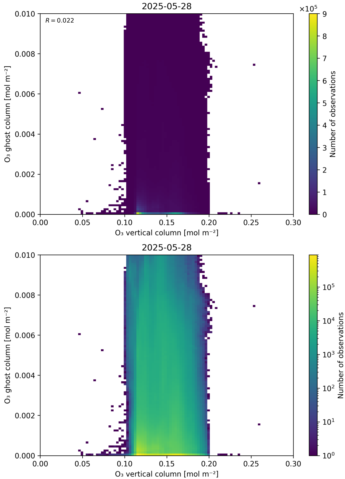
Figure 40: Scatter density plot of “O 3 vertical column” against “O 3 ghost column” for 2025-05-27 to 2025-05-29.
