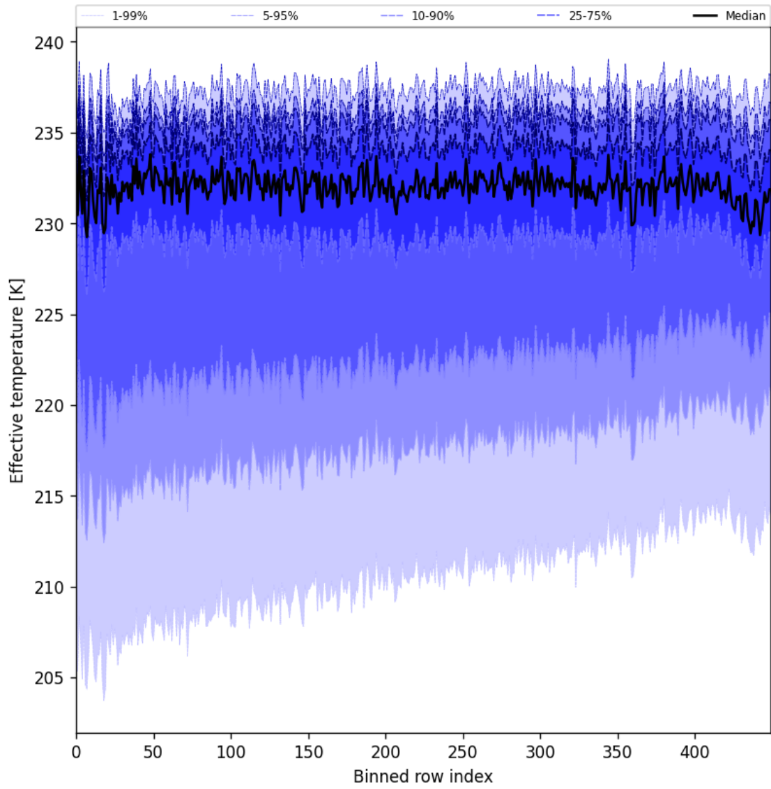
Figure 31: Along track statistics of “Effective temperature” for 2025-05-27 to 2025-05-29
