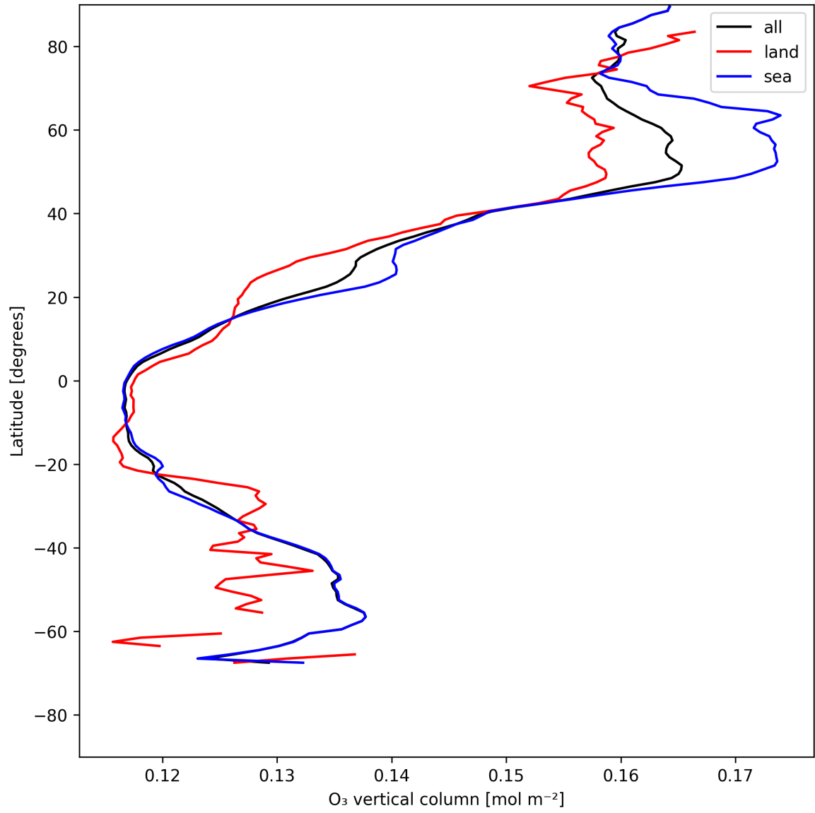
Figure 14: Zonal average of “O 3 vertical column” for 2025-05-27 to 2025-05-29.
