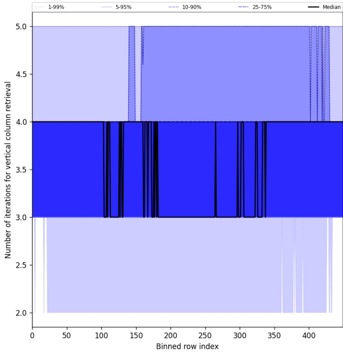
Figure 33: Along track statistics of “Number of iterations for vertical column retrieval” for 2025-05-27 to 2025-05-29
