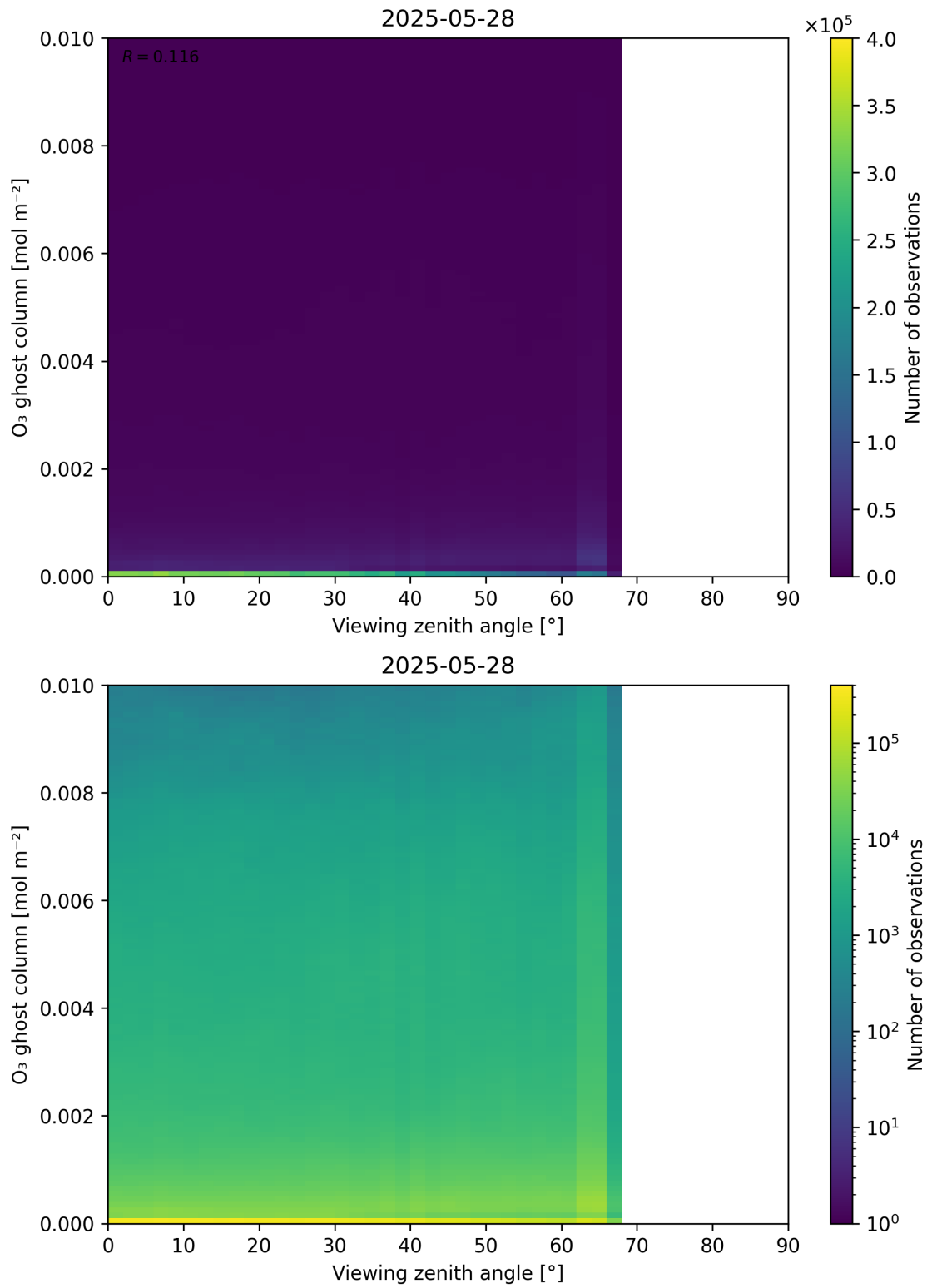
Figure 51: Scatter density plot of “Viewing zenith angle” against “O 3 ghost column” for 2025-05-27 to 2025-05-29.
