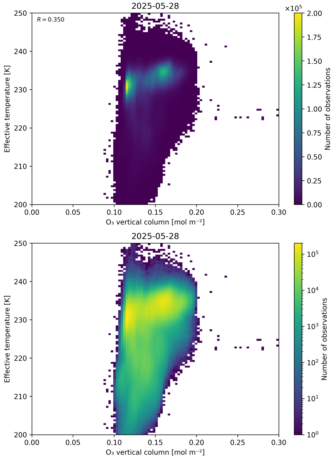
Figure 39: Scatter density plot of “O 3 vertical column” against “Effective temperature” for 2025-05-27 to 2025-05-29.
