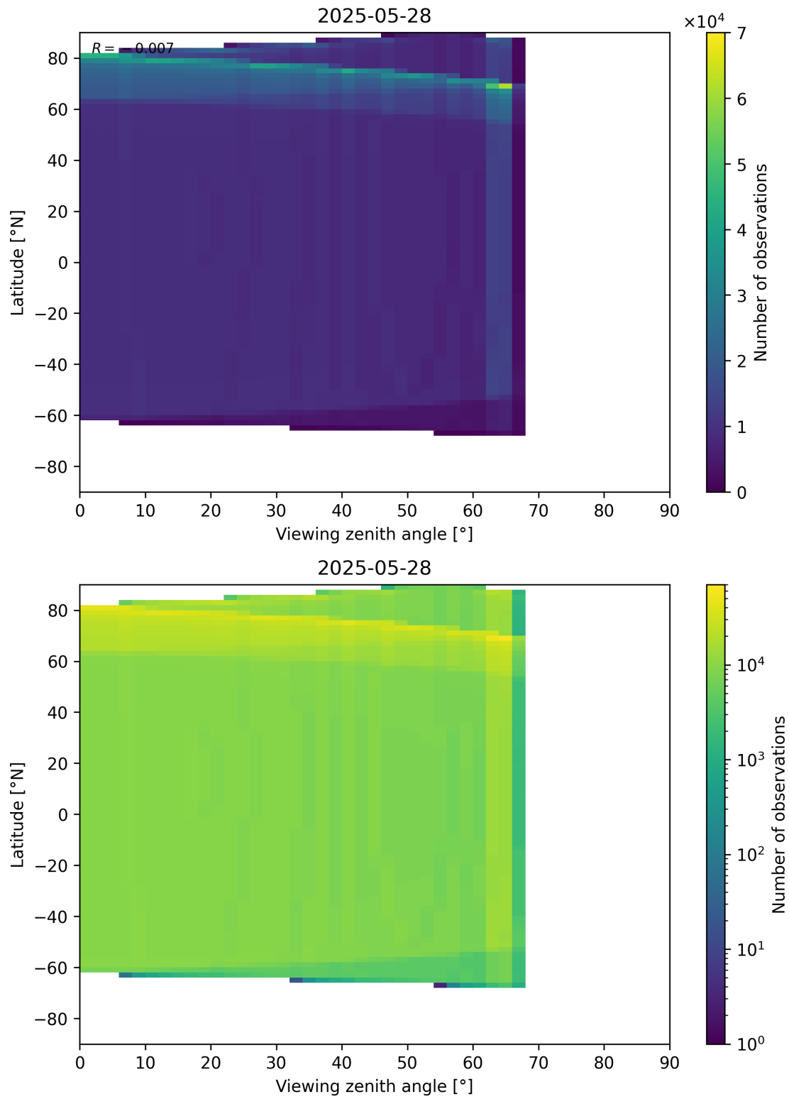
Figure 49: Scatter density plot of “Viewing zenith angle” against “Latitude” for 2025-05-27 to 2025-05-29.
