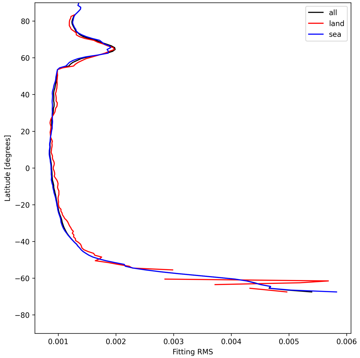
Figure 16: Zonal average of “Fitting RMS” for 2025-05-27 to 2025-05-29.
