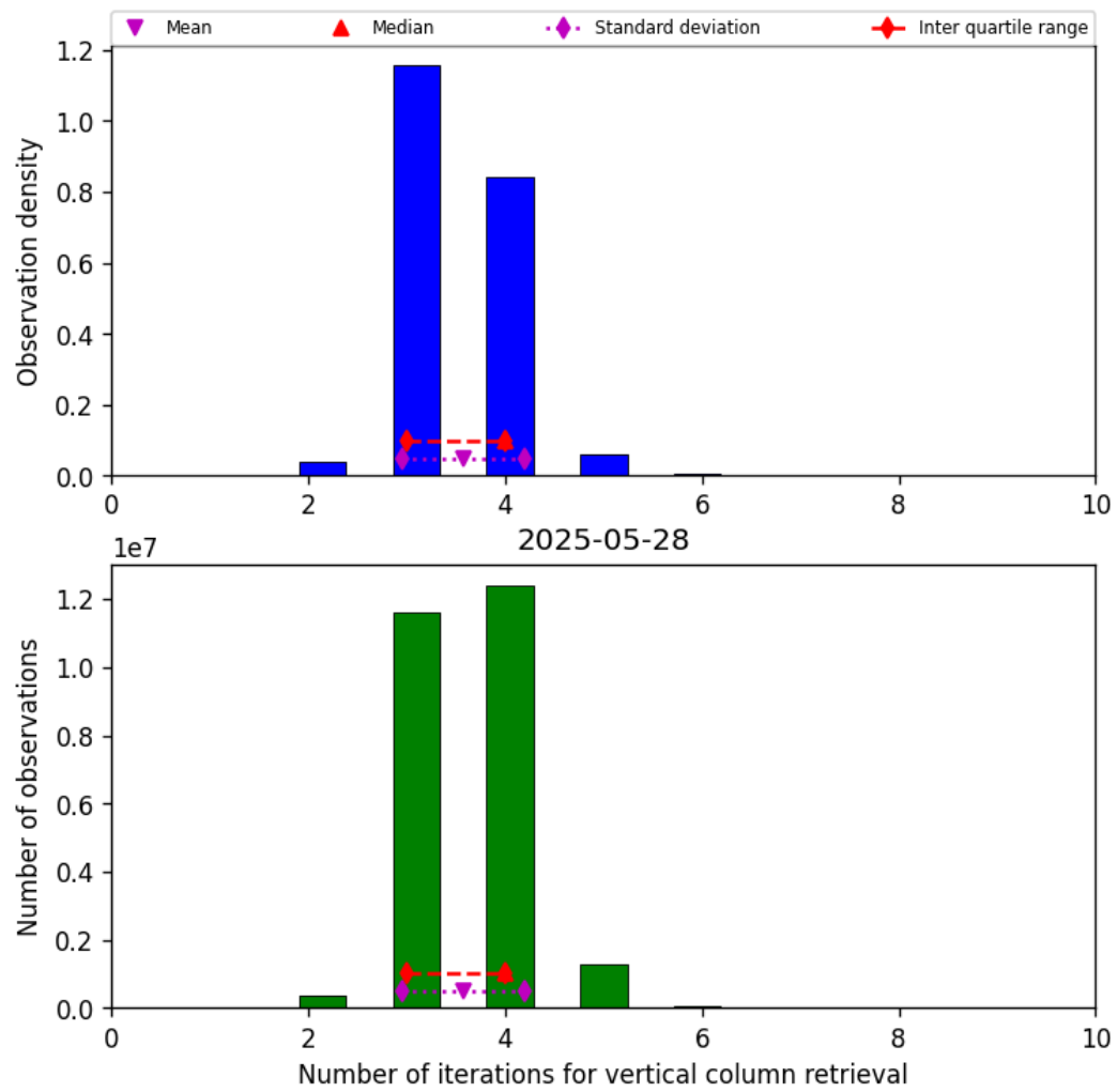
Figure 26: Histogram of “Number of iterations for vertical column retrieval” for 2025-05-27 to 2025-05-29
