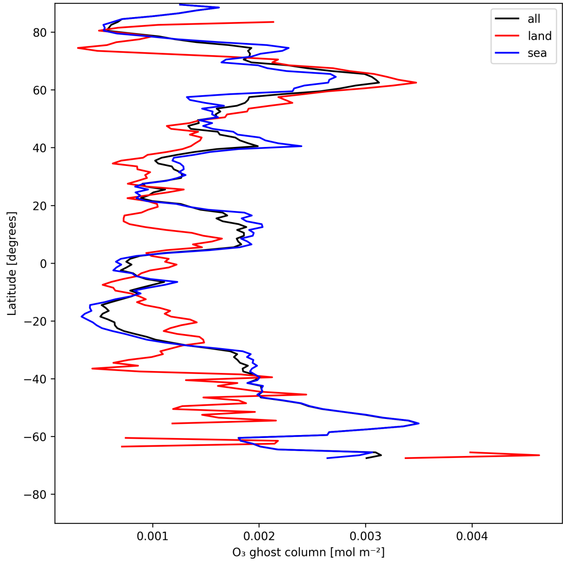
Figure 18: Zonal average of "O 3 ghost column" for 2025-05-27 to 2025-05-29.
