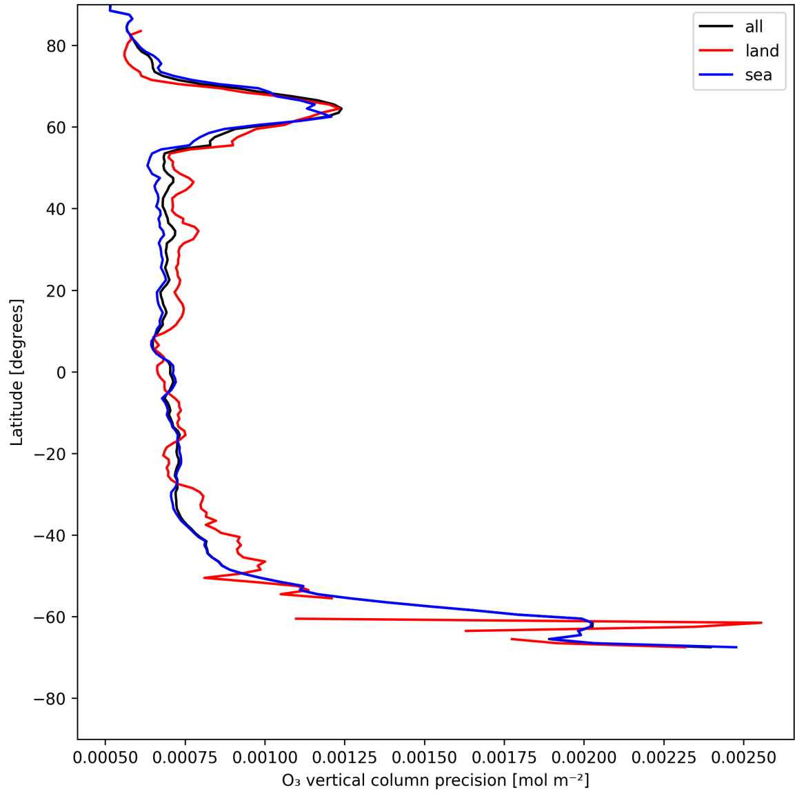
Figure 15: Zonal average of "O 3 vertical column precision" for 2025-05-27 to 2025-05-29.
