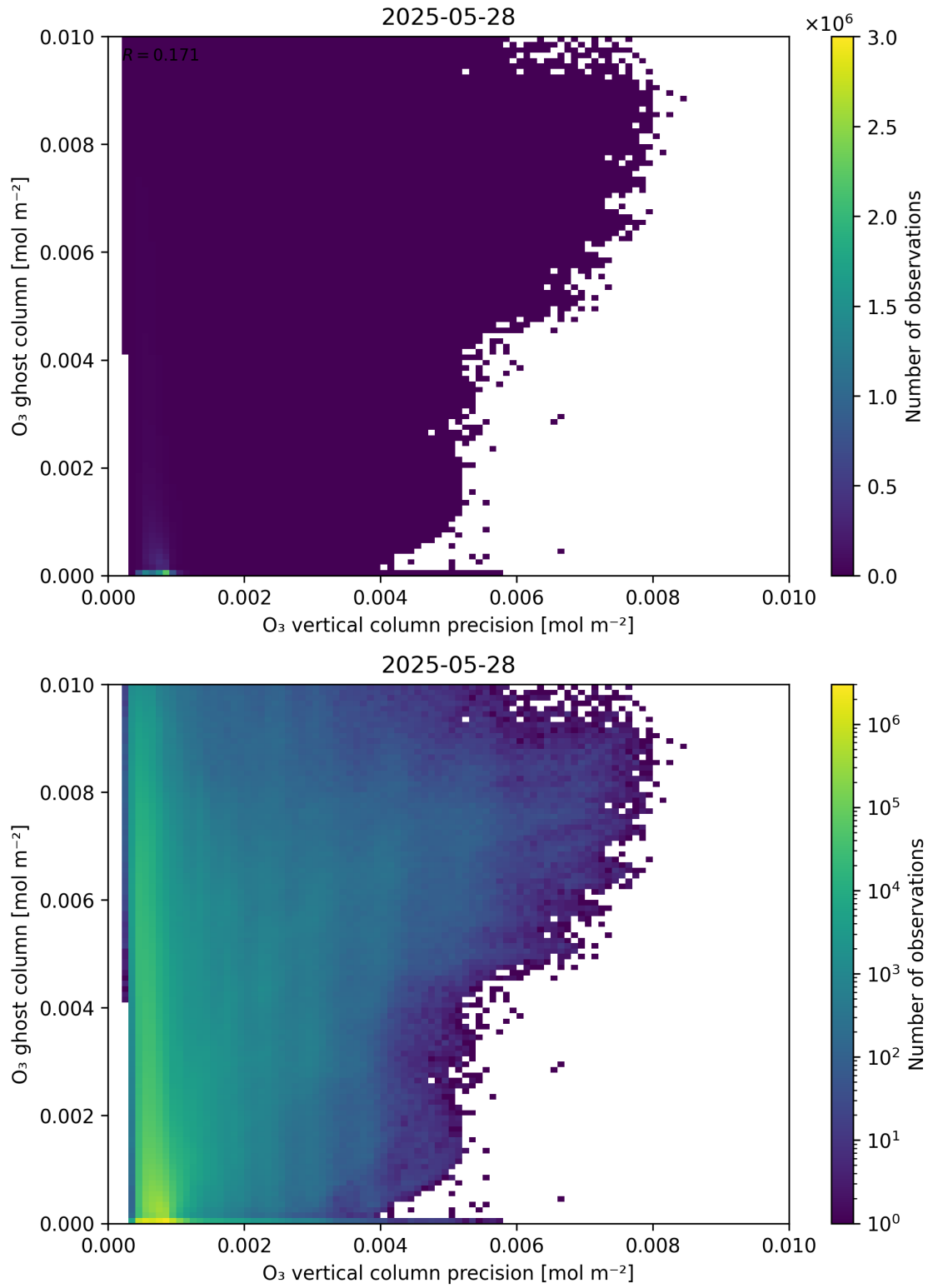
Figure 43: Scatter density plot of “ \text{O}_3 vertical column precision” against “ \text{O}_3 ghost column” for 2025-05-27 to 2025-05-29.
