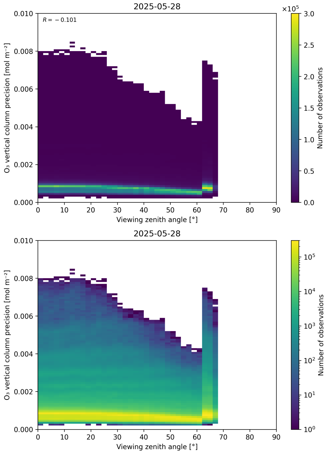
Figure 53: Scatter density plot of “Viewing zenith angle” against “O 3 vertical column precision” for 2025-05-27 to 2025-05-29.
