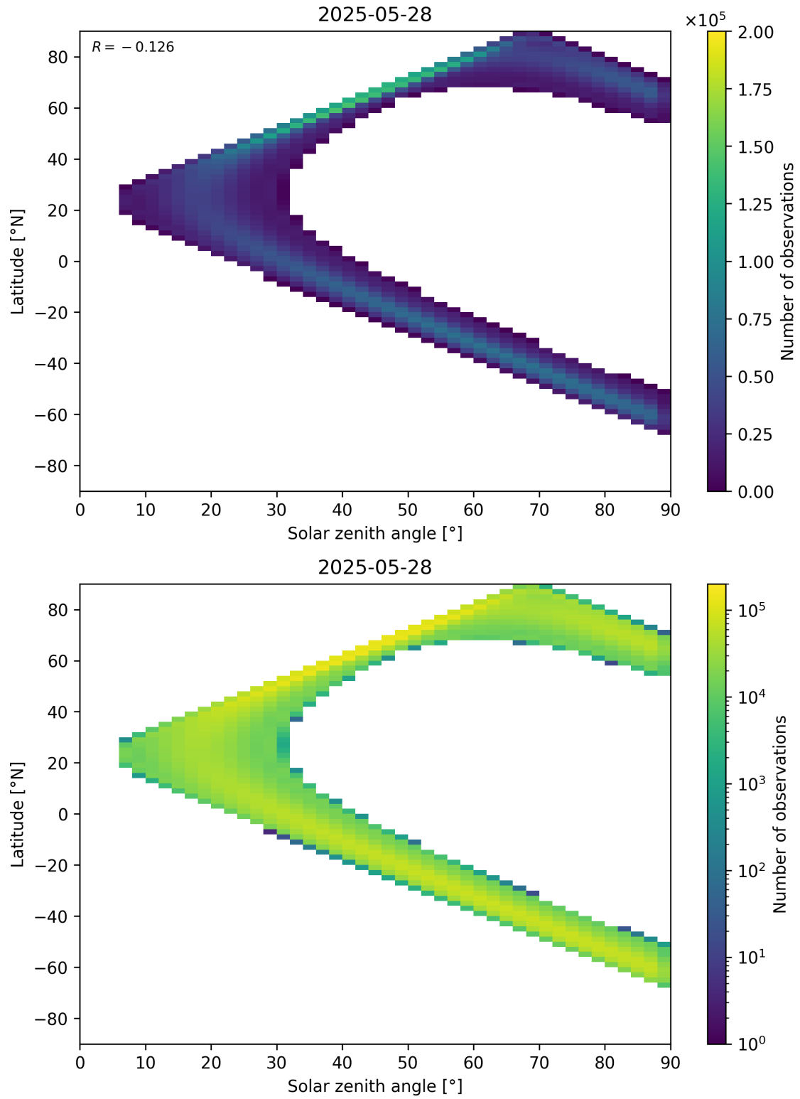
Figure 44: Scatter density plot of “Solar zenith angle” against “Latitude” for 2025-05-27 to 2025-05-29.
