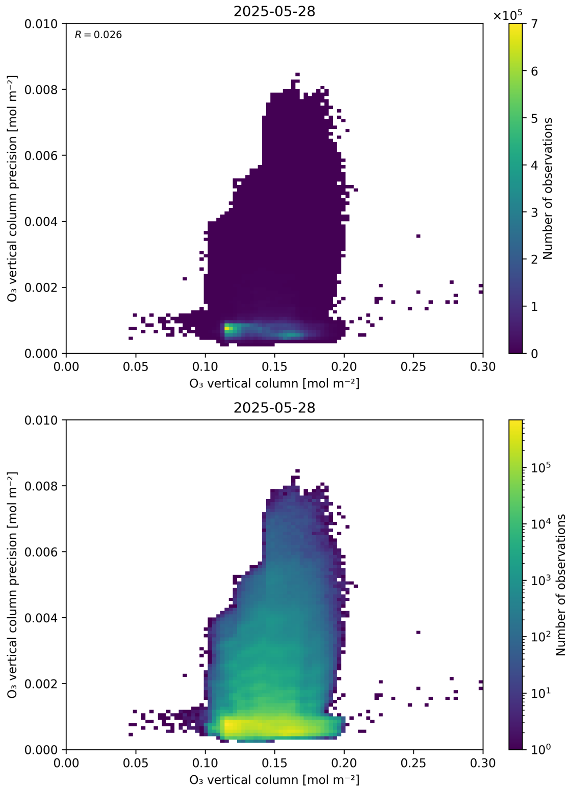
Figure 41: Scatter density plot of “O 3 vertical column” against “O 3 vertical column precision” for 2025-05-27 to 2025-05-29.
