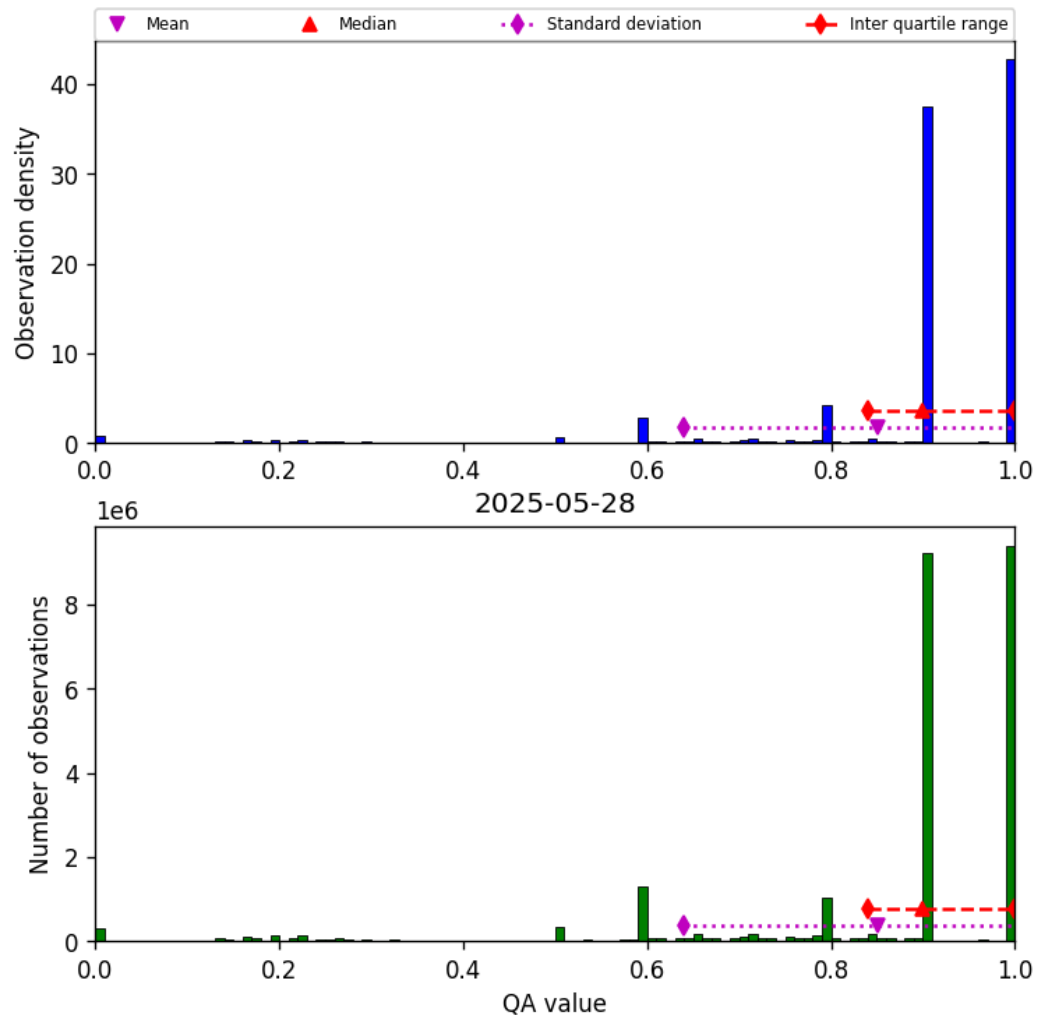
Figure 20: Histogram of “QA value” for 2025-05-27 to 2025-05-29
