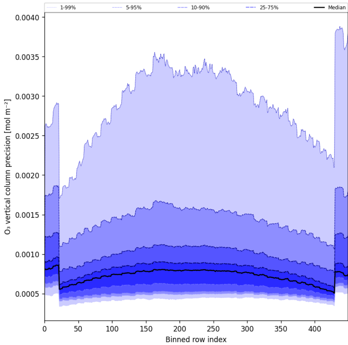
Figure 29: Along track statistics of "O 3 vertical column precision" for 2025-05-28 to 2025-05-30
