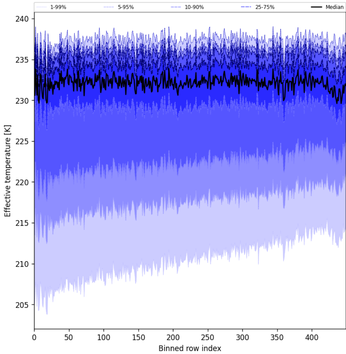
Figure 31: Along track statistics of “Effective temperature” for 2025-05-28 to 2025-05-30
