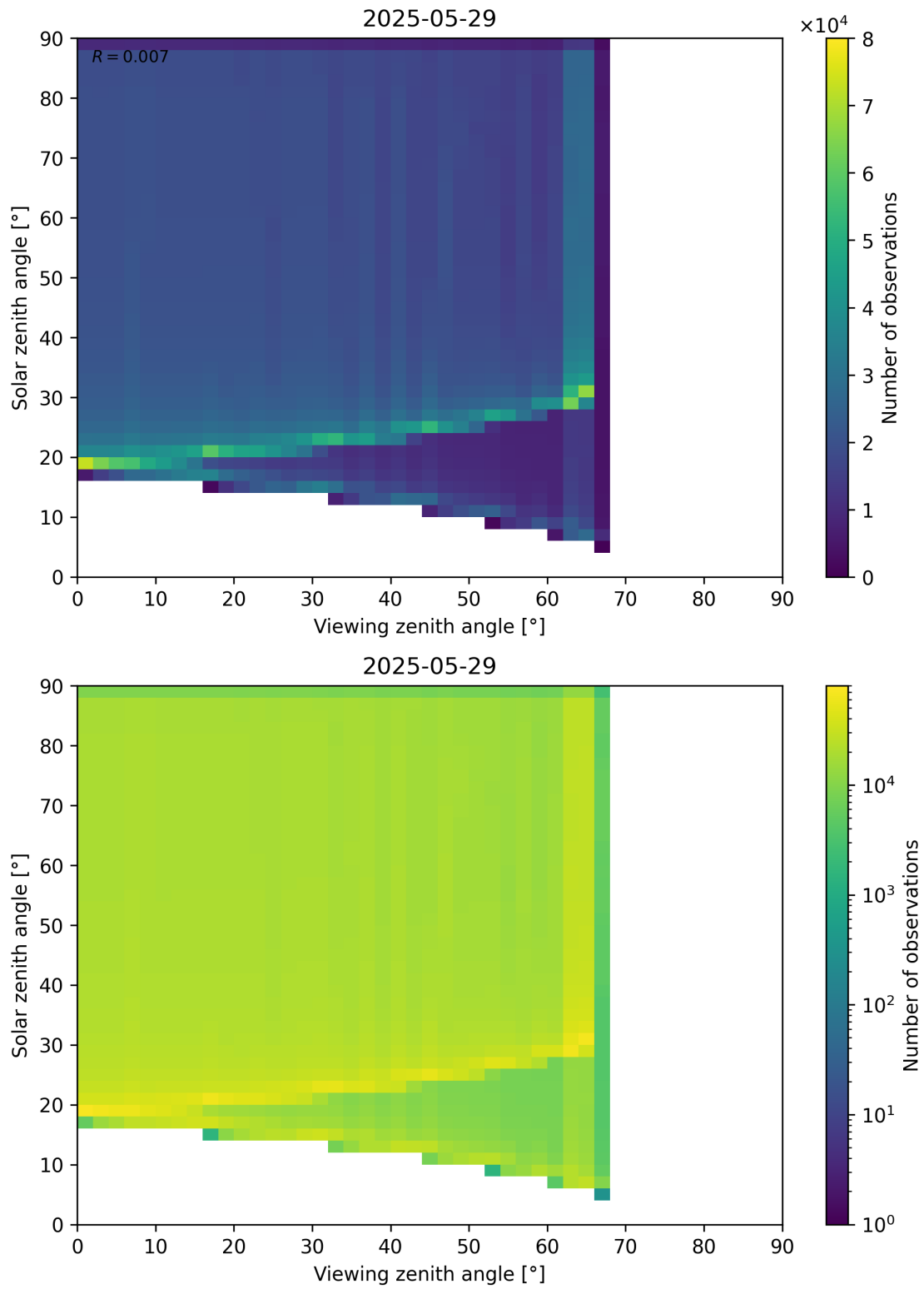
Figure 54: Scatter density plot of “Viewing zenith angle” against “Solar zenith angle” for 2025-05-28 to 2025-05-30.
