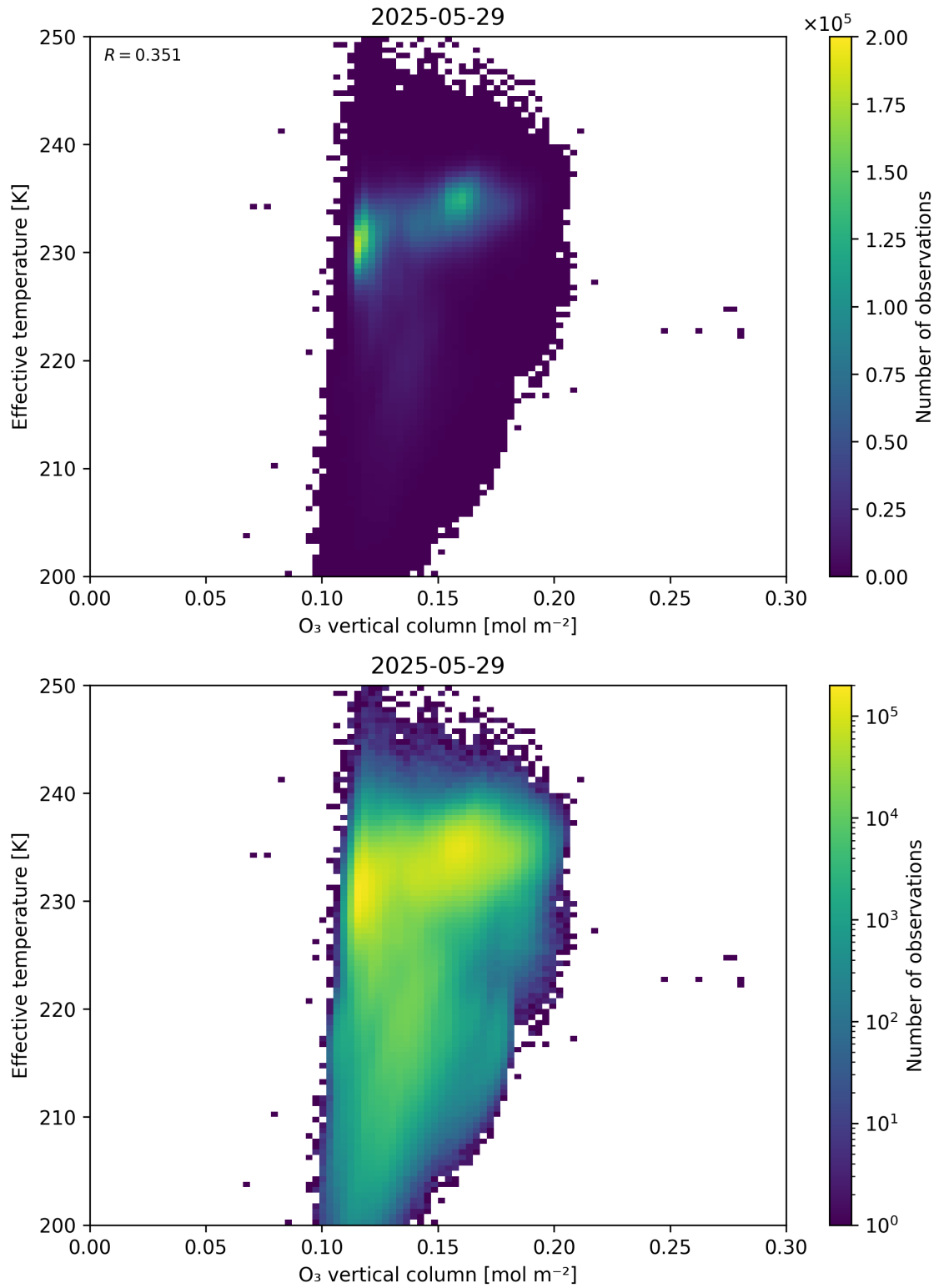
Figure 39: Scatter density plot of “O 3 vertical column” against “Effective temperature” for 2025-05-28 to 2025-05-30.
