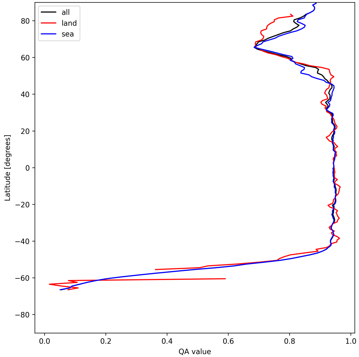
Figure 13: Zonal average of “QA value” for 2025-05-28 to 2025-05-30.
