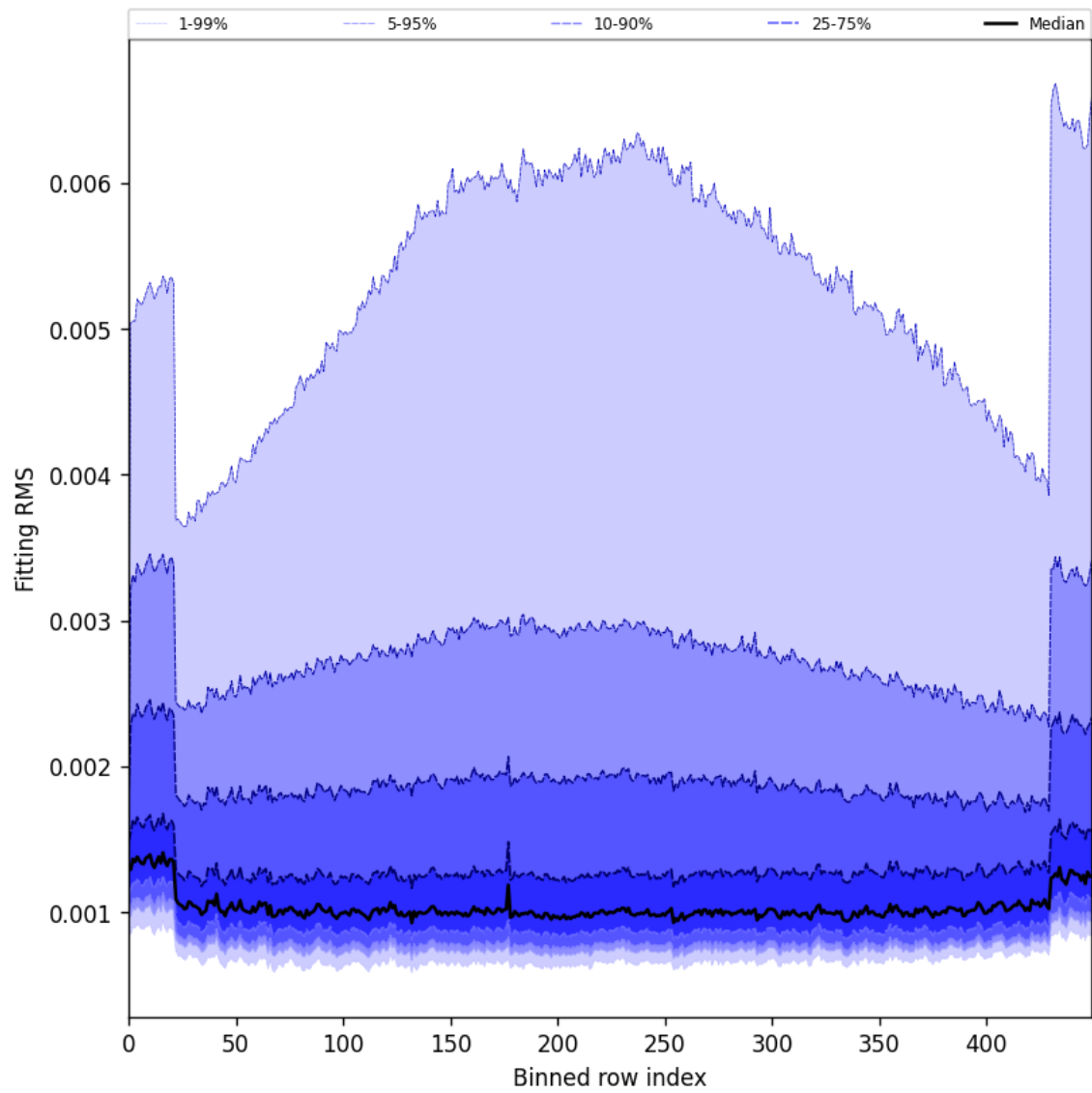
Figure 30: Along track statistics of “Fitting RMS” for 2025-05-28 to 2025-05-30
