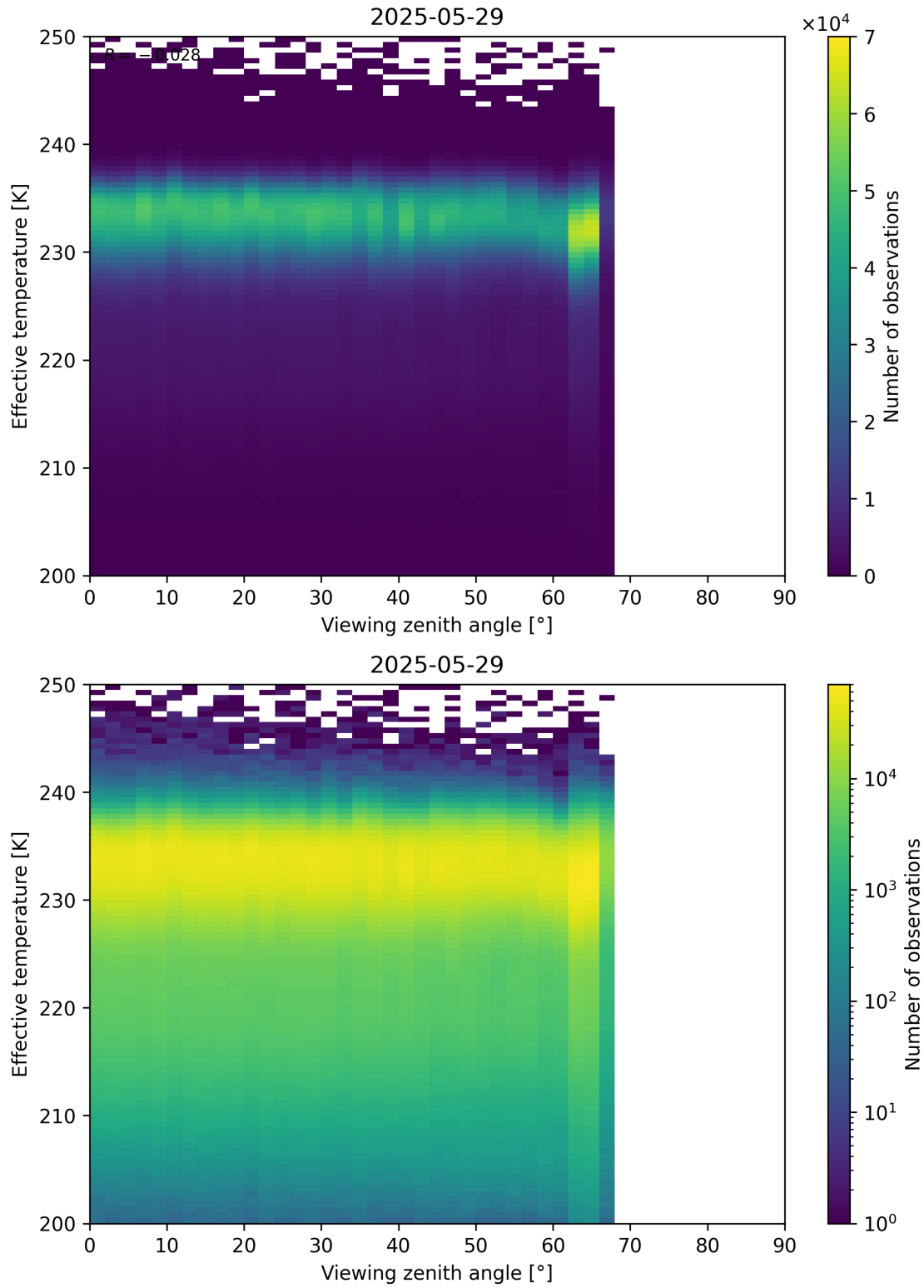
Figure 50: Scatter density plot of “Viewing zenith angle” against “Effective temperature” for 2025-05-28 to 2025-05-30.
