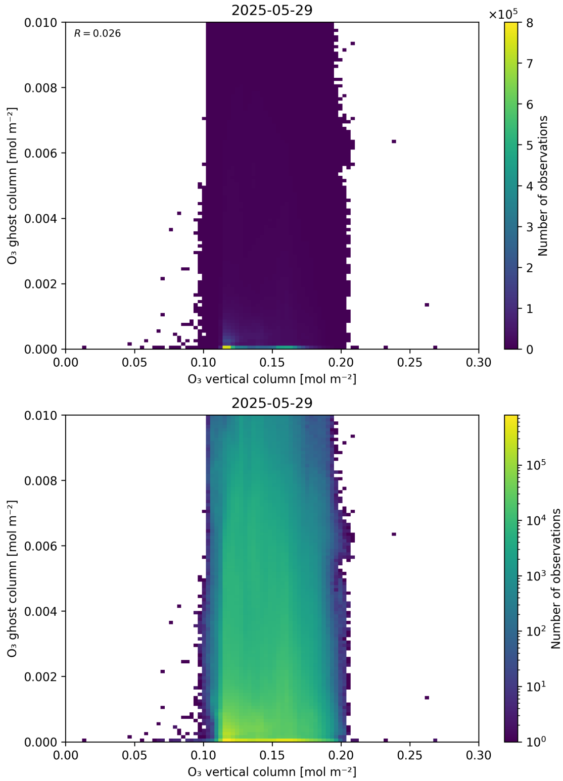
Figure 40: Scatter density plot of “O 3 vertical column” against “O 3 ghost column” for 2025-05-28 to 2025-05-30.
