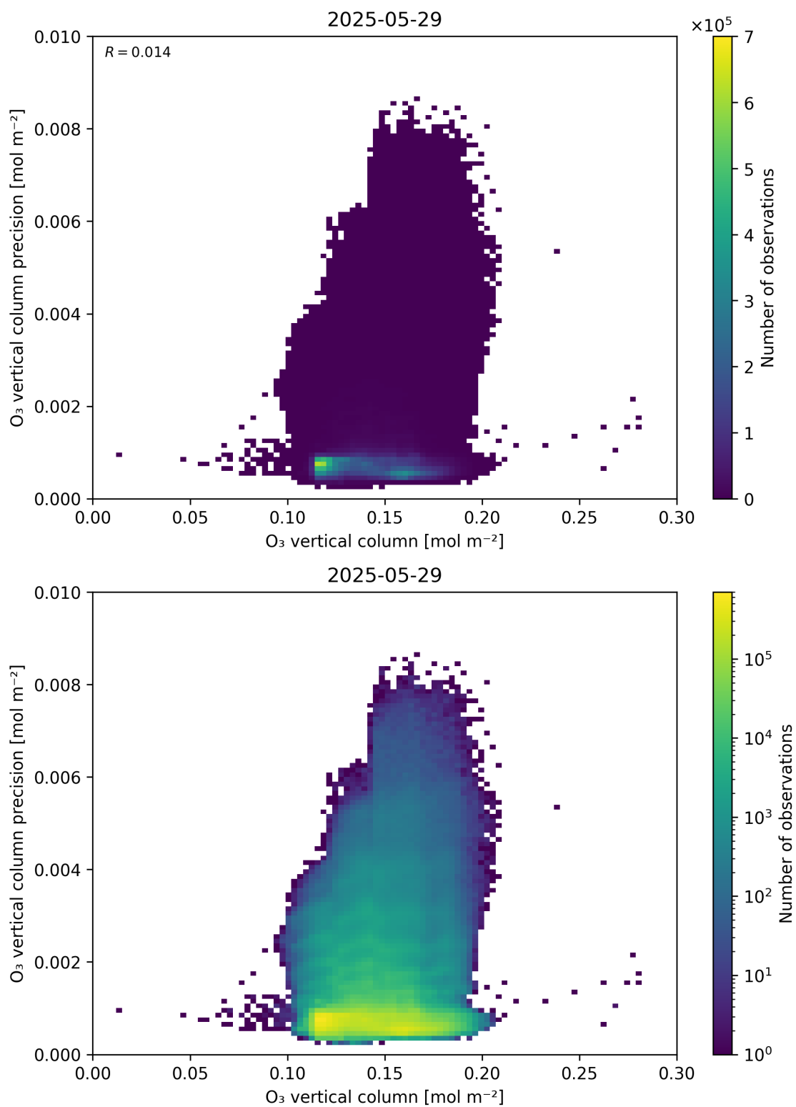
Figure 41: Scatter density plot of “O 3 vertical column” against “O 3 vertical column precision” for 2025-05-28 to 2025-05-30.
