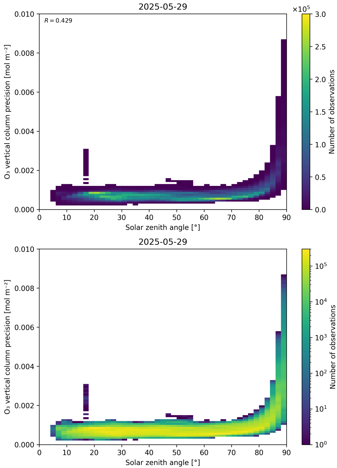
Figure 48: Scatter density plot of “Solar zenith angle” against “O 3 vertical column precision” for 2025-05-28 to 2025-05-30.
