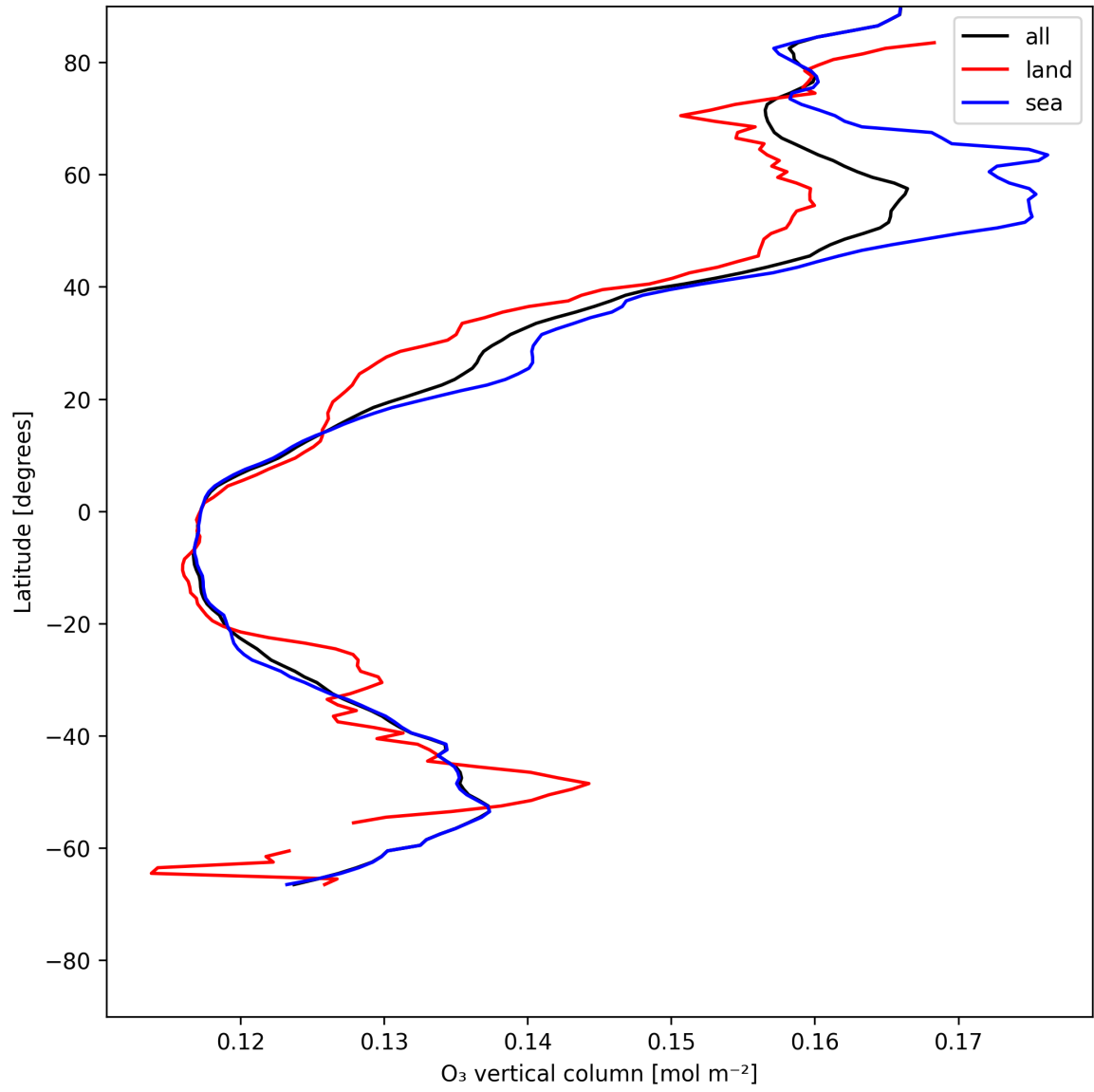
Figure 14: Zonal average of “O 3 vertical column” for 2025-05-28 to 2025-05-30.
