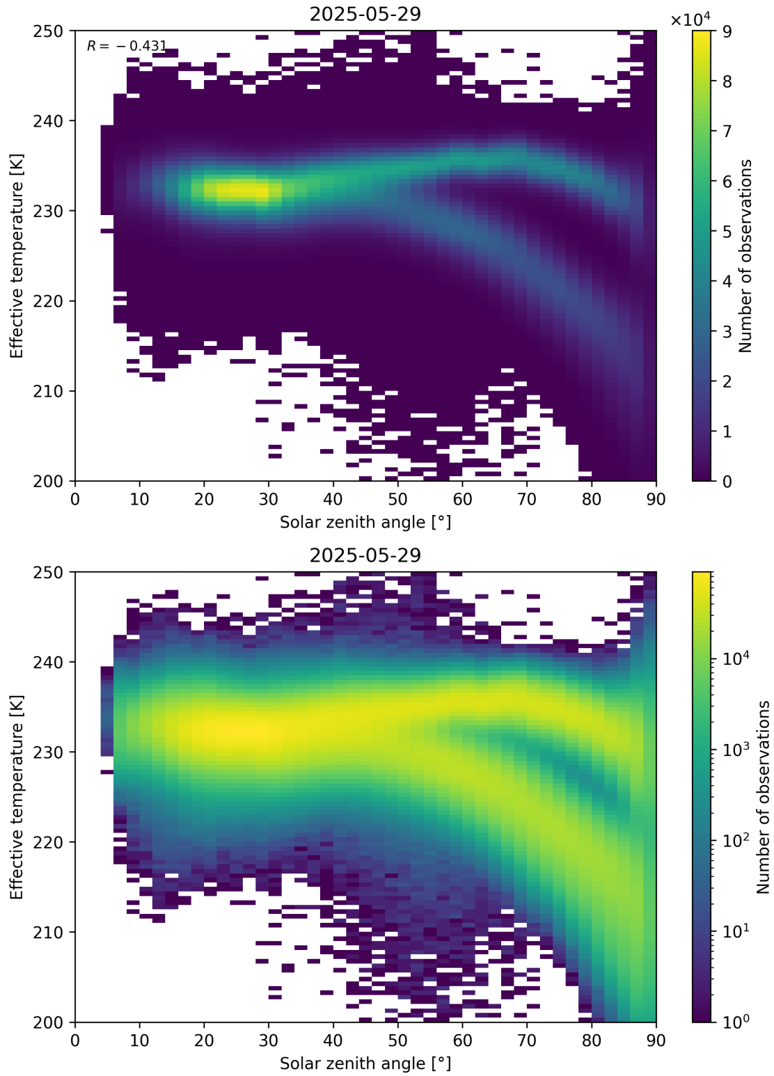
Figure 45: Scatter density plot of “Solar zenith angle” against “Effective temperature” for 2025-05-28 to 2025-05-30.
