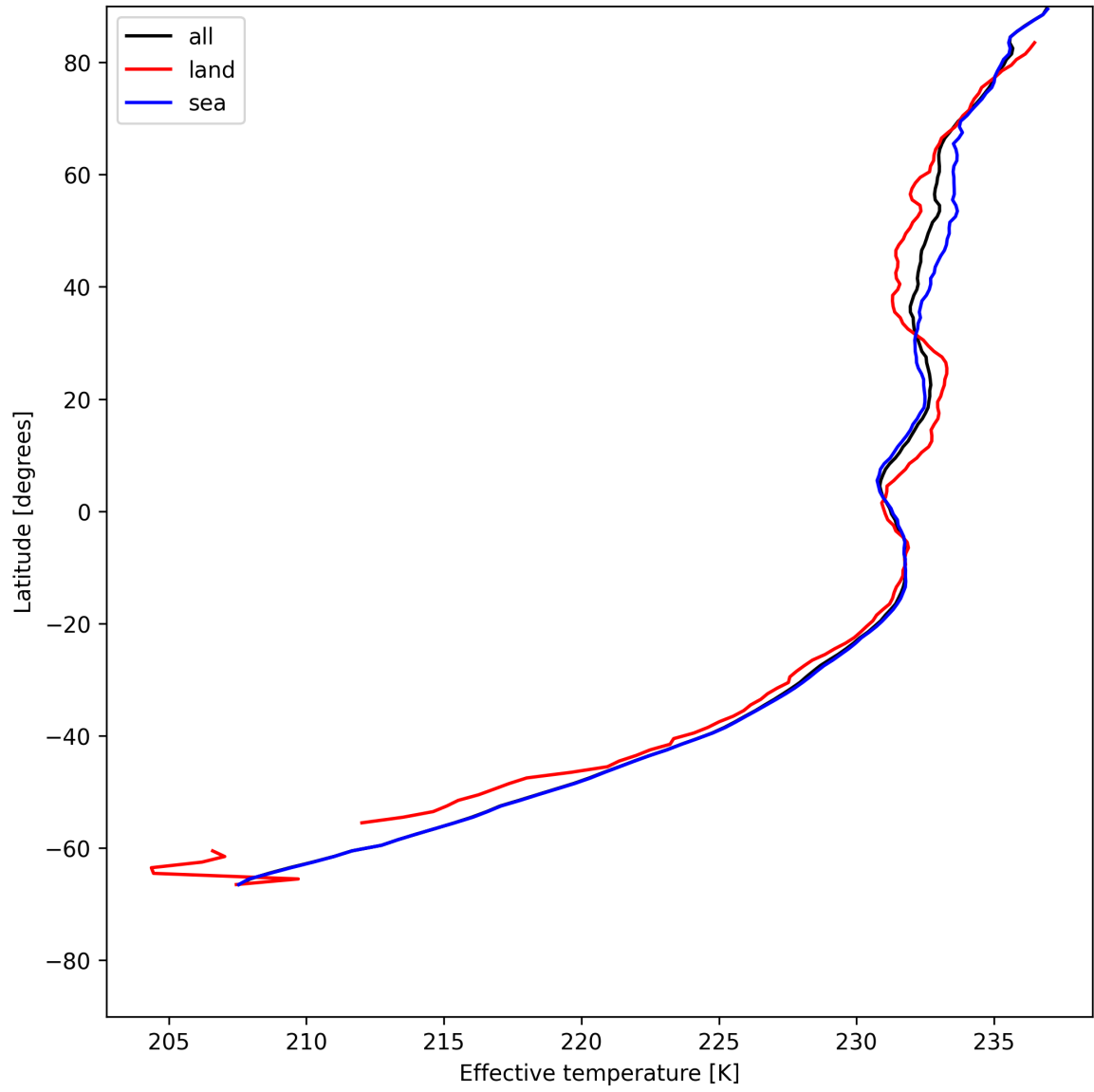
Figure 17: Zonal average of “Effective temperature” for 2025-05-28 to 2025-05-30.
