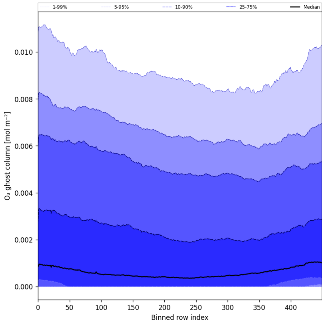
Figure 32: Along track statistics of “O 3 ghost column” for 2025-05-28 to 2025-05-30
