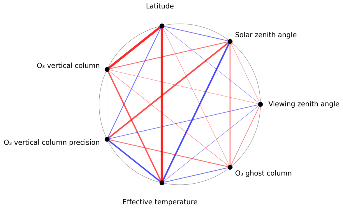
Figure 1: Map of correlation graph for 2025-05-28 to 2025-05-30.
