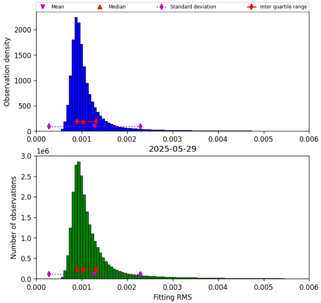
Figure 23: Histogram of “Fitting RMS” for 2025-05-28 to 2025-05-30
