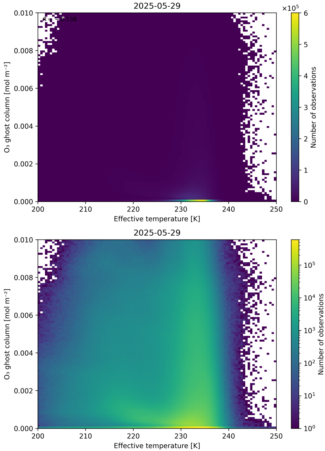
Figure 38: Scatter density plot of “Effective temperature” against “O 3 ghost column” for 2025-05-28 to 2025-05-30.
