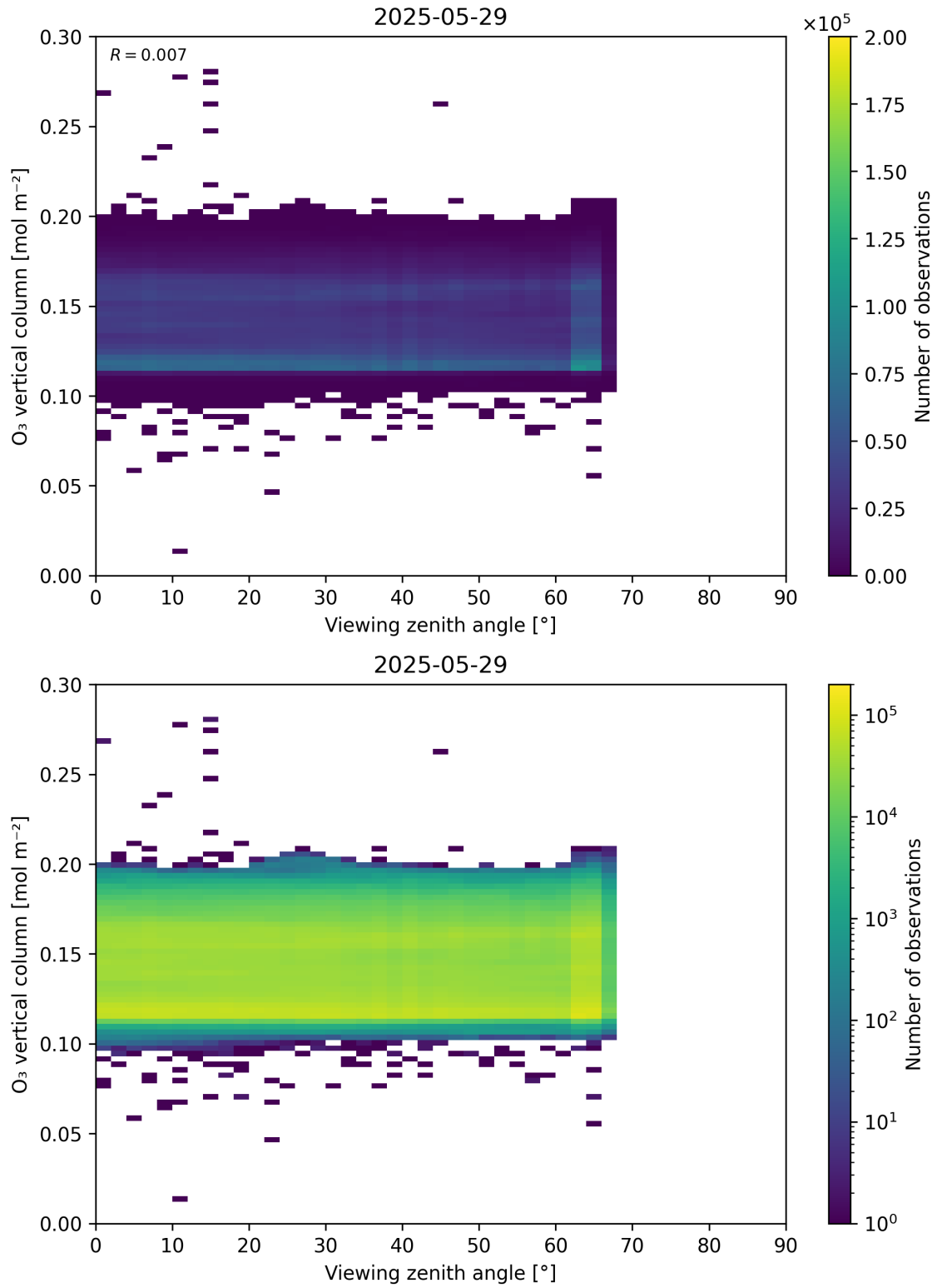
Figure 52: Scatter density plot of “Viewing zenith angle” against “O 3 vertical column” for 2025-05-28 to 2025-05-30.
