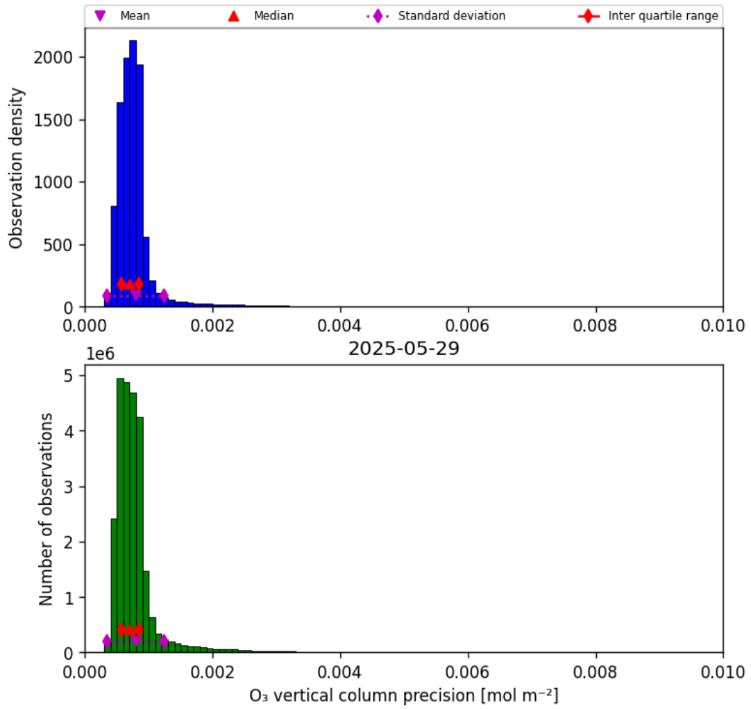
Figure 22: Histogram of “O 3 vertical column precision” for 2025-05-28 to 2025-05-30
