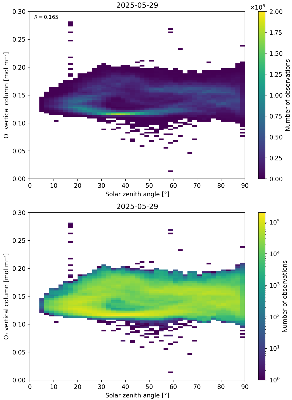
Figure 47: Scatter density plot of “Solar zenith angle” against “O 3 vertical column” for 2025-05-28 to 2025-05-30.
