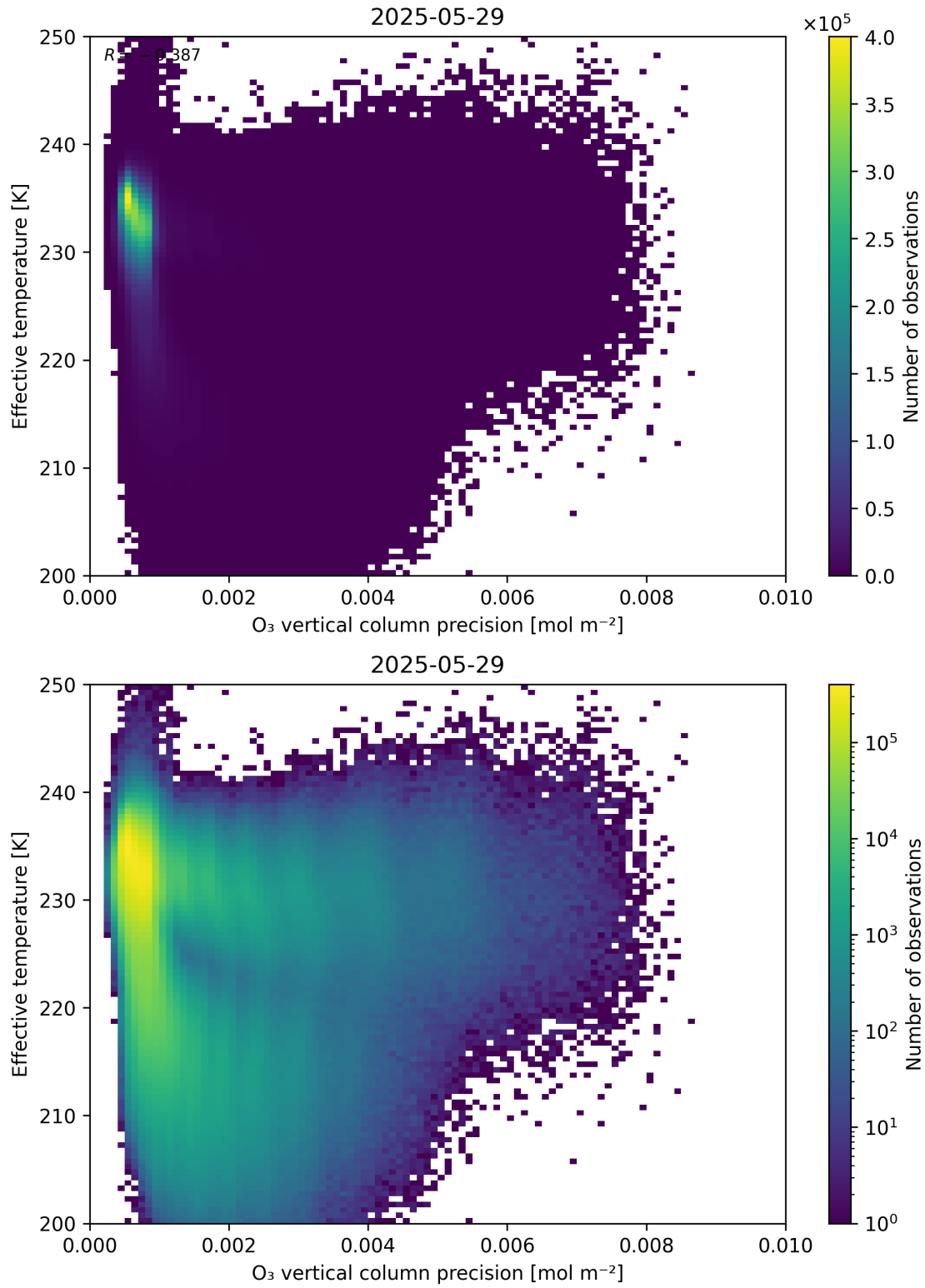
Figure 42: Scatter density plot of “O 3 vertical column precision” against “Effective temperature” for 2025-05-28 to 2025-05-30.
