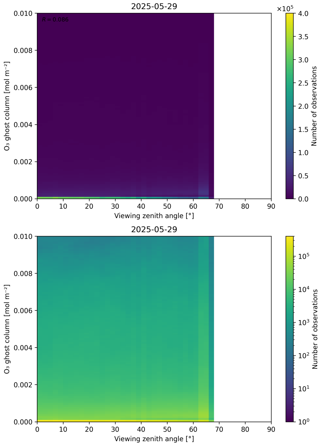
Figure 51: Scatter density plot of “Viewing zenith angle” against “O 3 ghost column” for 2025-05-28 to 2025-05-30.
