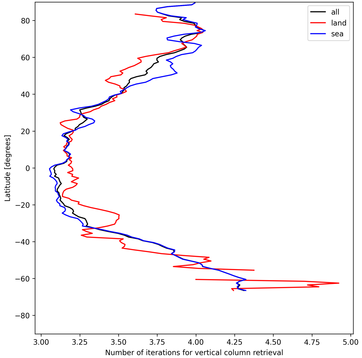
Figure 19: Zonal average of “Number of iterations for vertical column retrieval” for 2025-05-28 to 2025-05-30.
