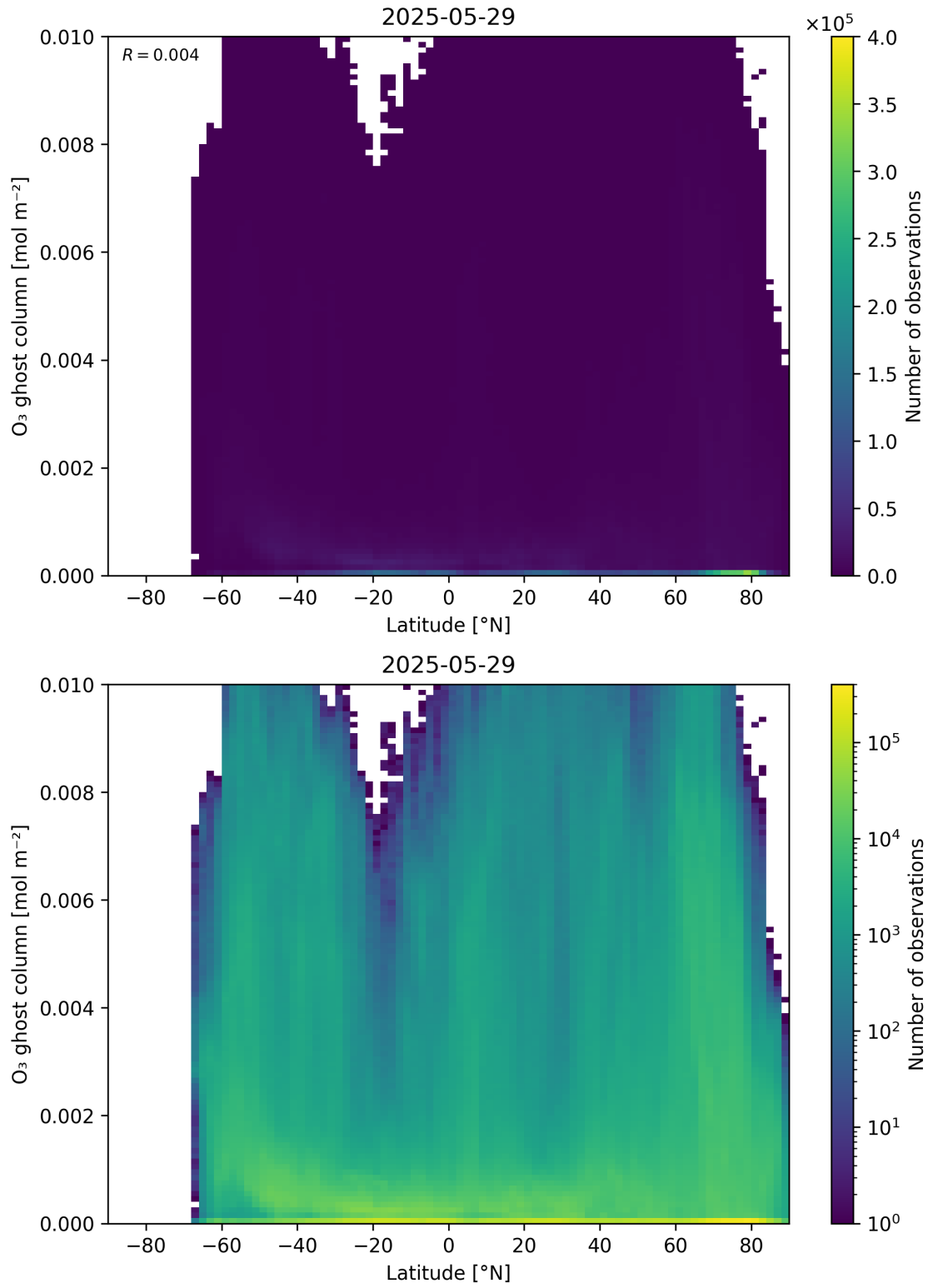
Figure 35: Scatter density plot of “Latitude” against “O 3 ghost column” for 2025-05-28 to 2025-05-30.
