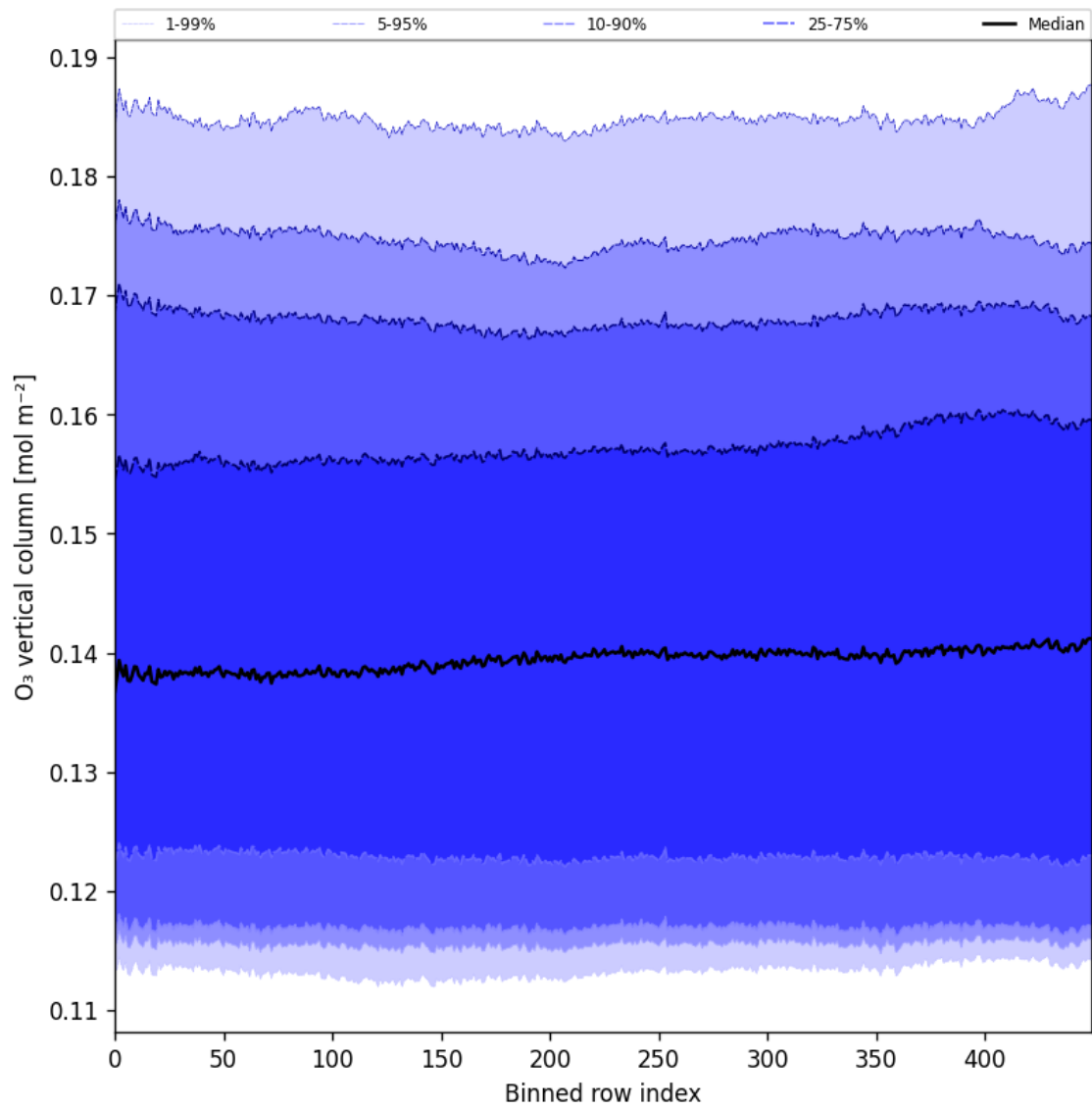
Figure 28: Along track statistics of “O 3 vertical column” for 2025-05-28 to 2025-05-30
