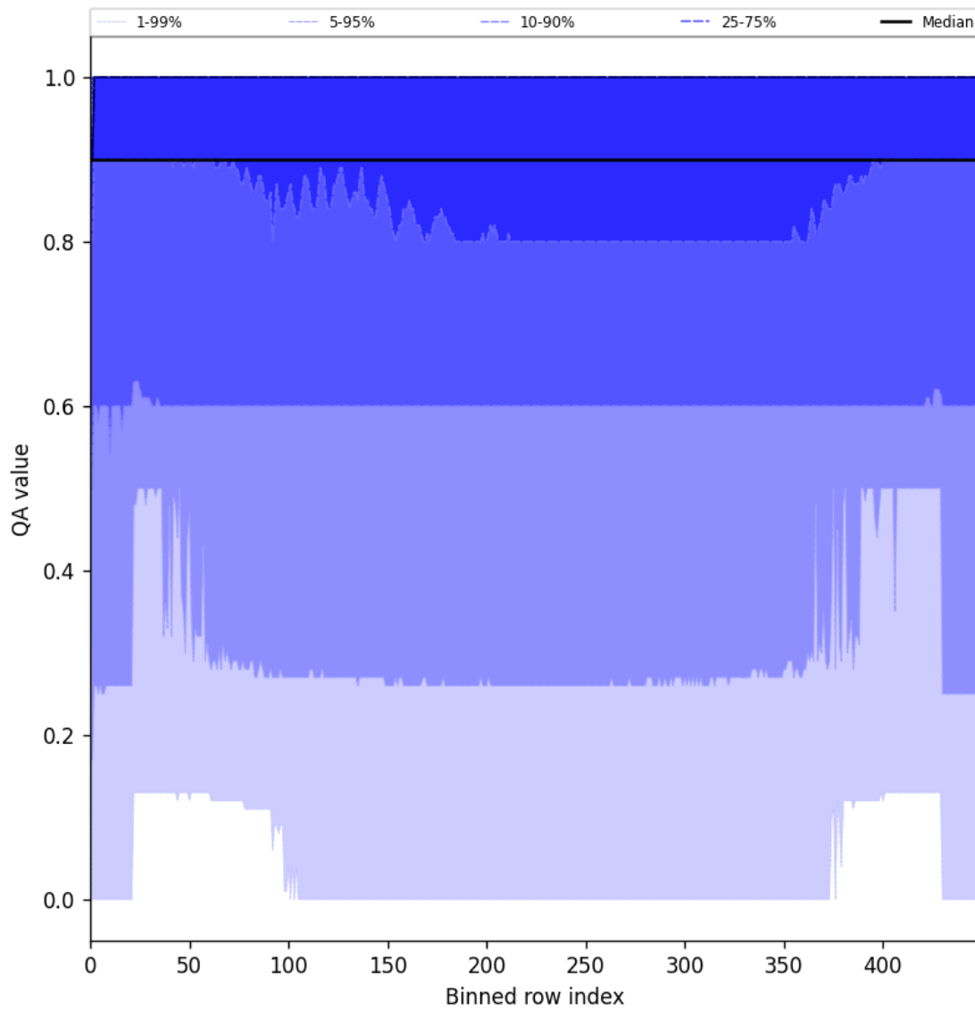
Figure 27: Along track statistics of “QA value” for 2025-05-28 to 2025-05-30
