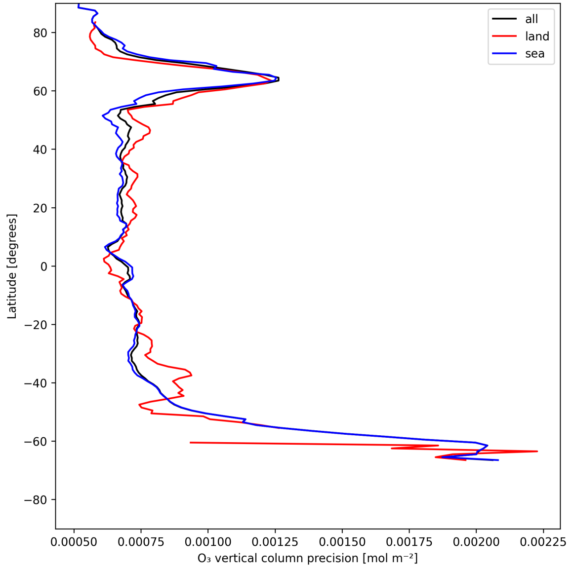
Figure 15: Zonal average of “O 3 vertical column precision” for 2025-05-28 to 2025-05-30.
