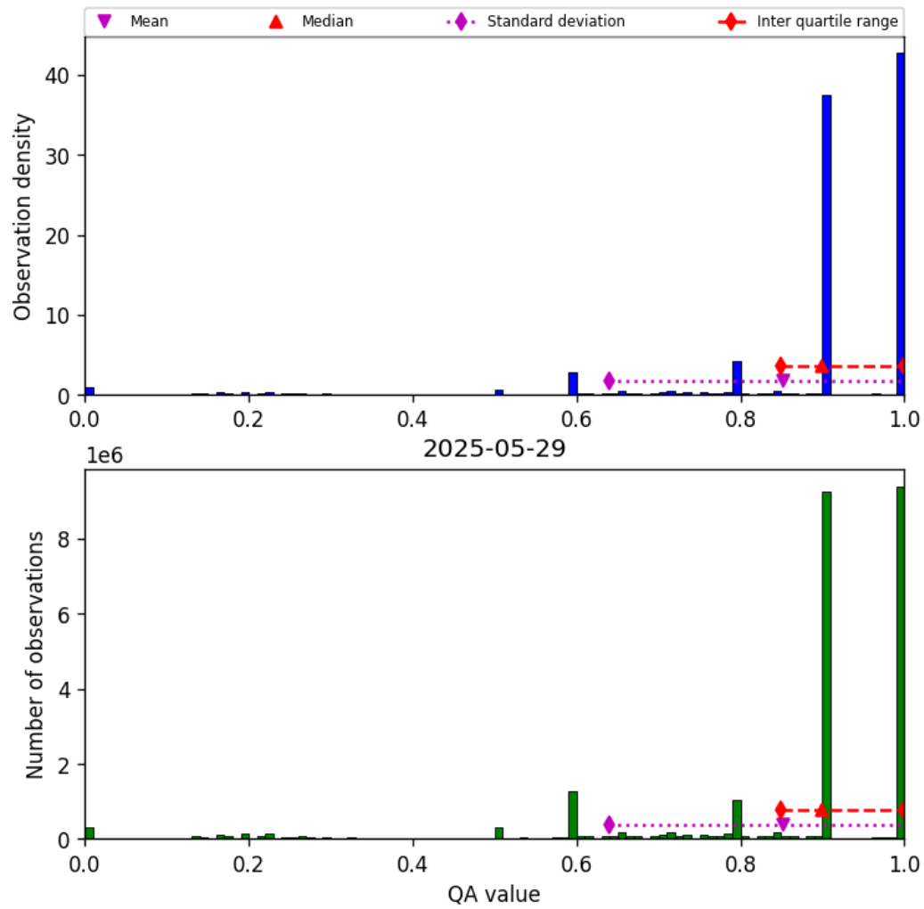
Figure 20: Histogram of “QA value” for 2025-05-28 to 2025-05-30
