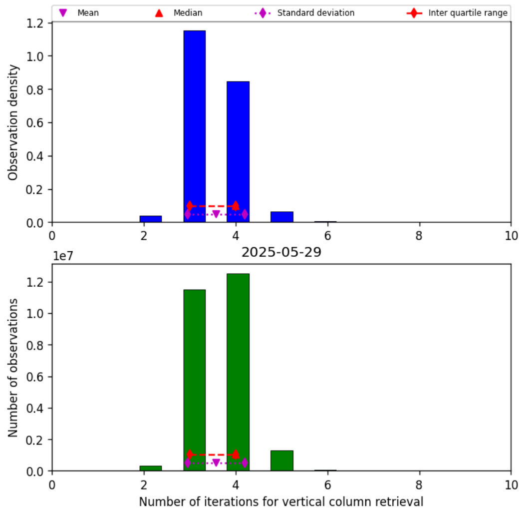
Figure 26: Histogram of “Number of iterations for vertical column retrieval” for 2025-05-28 to 2025-05-30
