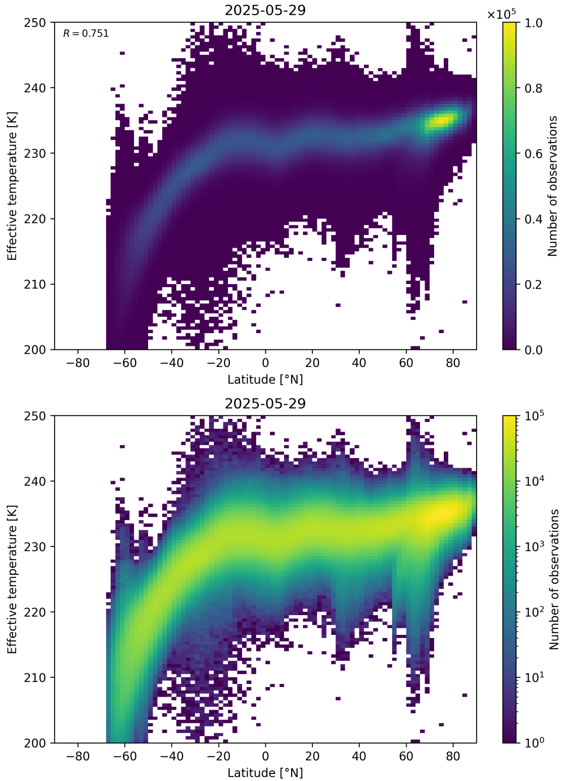
Figure 34: Scatter density plot of “Latitude” against “Effective temperature” for 2025-05-28 to 2025-05-30.
