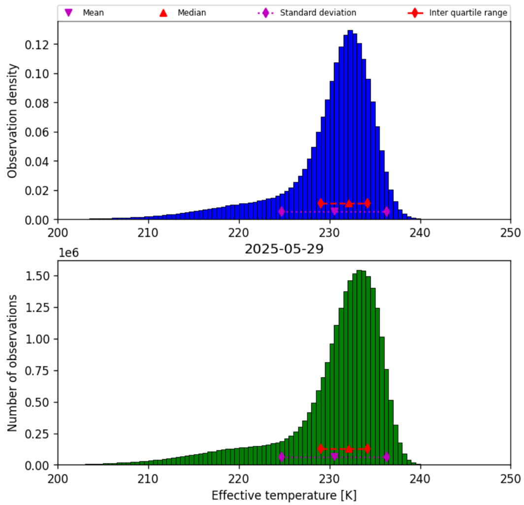
Figure 24: Histogram of “Effective temperature” for 2025-05-28 to 2025-05-30
