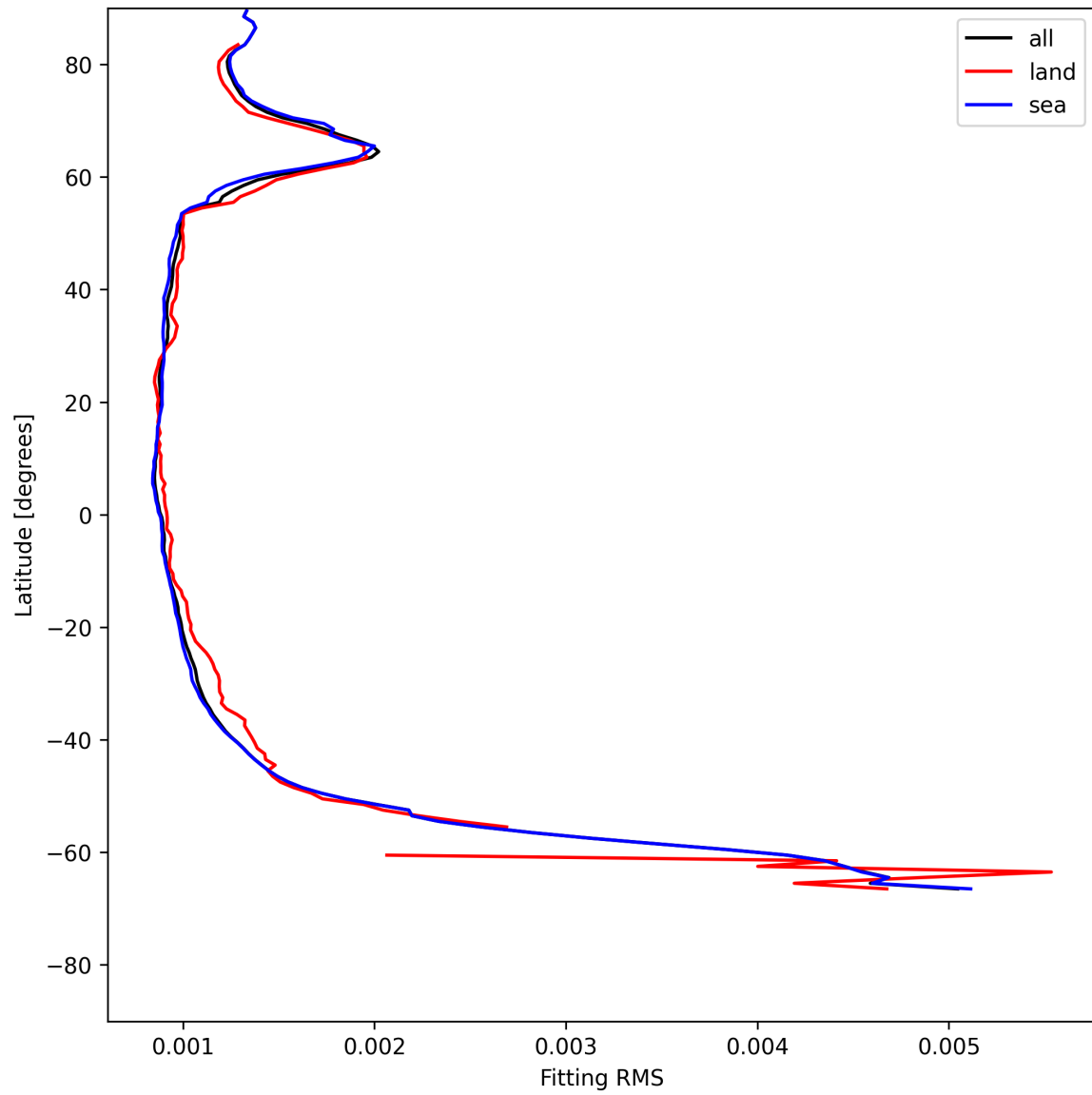
Figure 16: Zonal average of “Fitting RMS” for 2025-05-28 to 2025-05-30.
