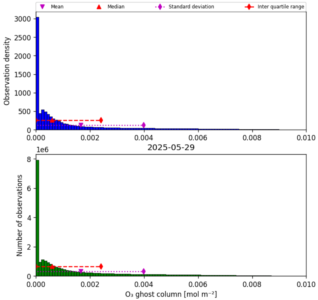
Figure 25: Histogram of “O 3 ghost column” for 2025-05-28 to 2025-05-30
