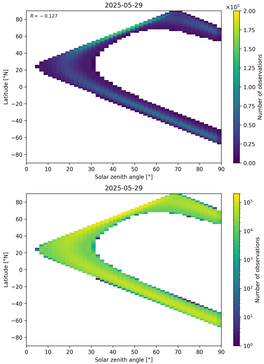
Figure 44: Scatter density plot of “Solar zenith angle” against “Latitude” for 2025-05-28 to 2025-05-30.
