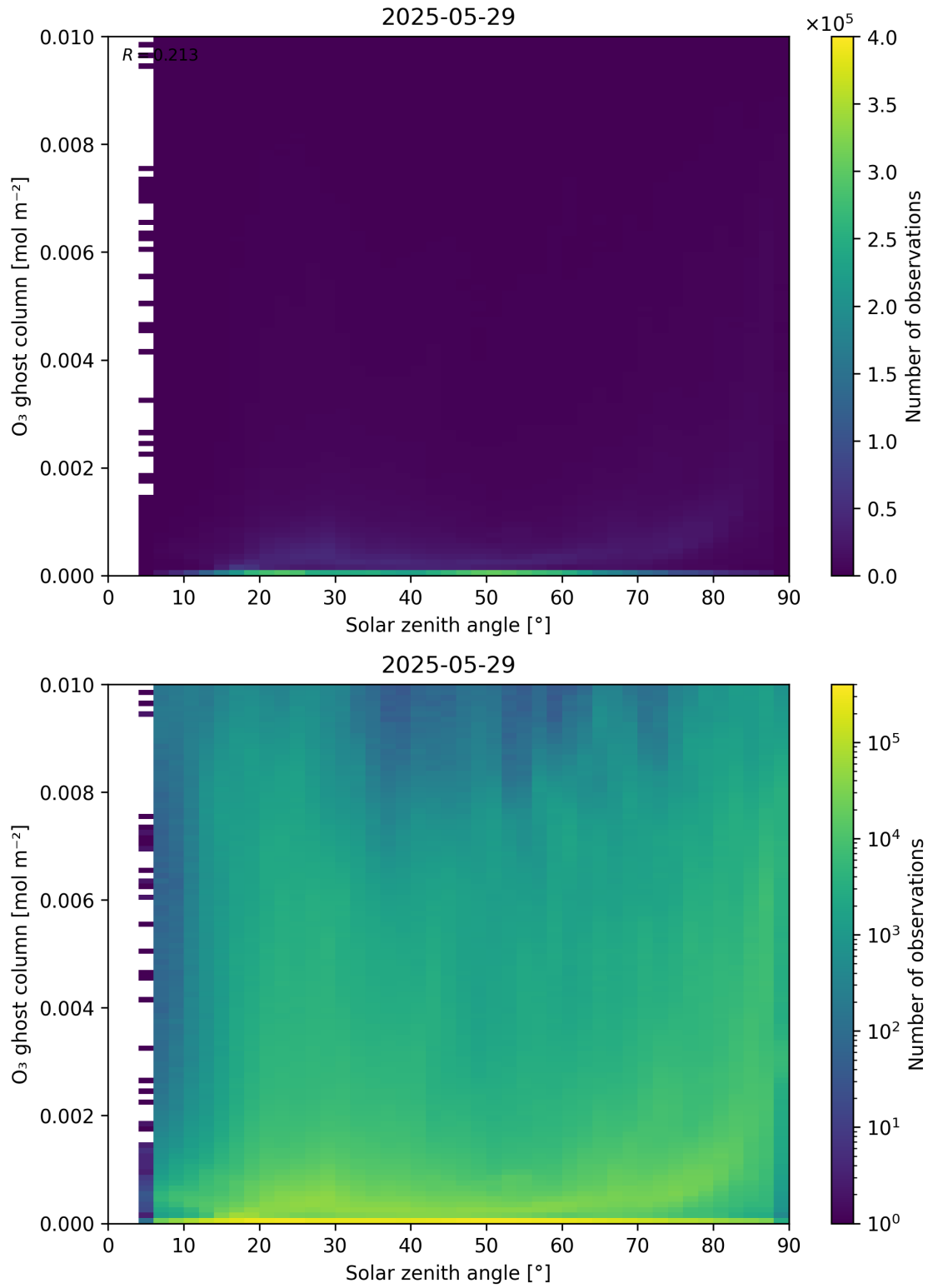
Figure 46: Scatter density plot of “Solar zenith angle” against “O 3 ghost column” for 2025-05-28 to 2025-05-30.
