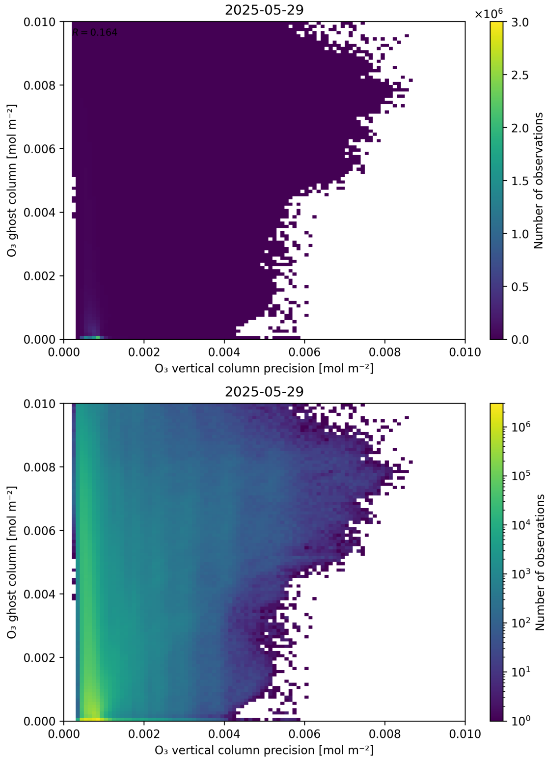
Figure 43: Scatter density plot of “ \text{O}_3 vertical column precision” against “ \text{O}_3 ghost column” for 2025-05-28 to 2025-05-30.
