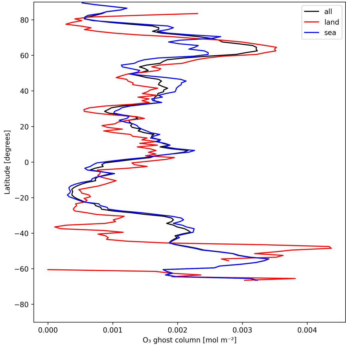
Figure 18: Zonal average of “O 3 ghost column” for 2025-05-28 to 2025-05-30.
