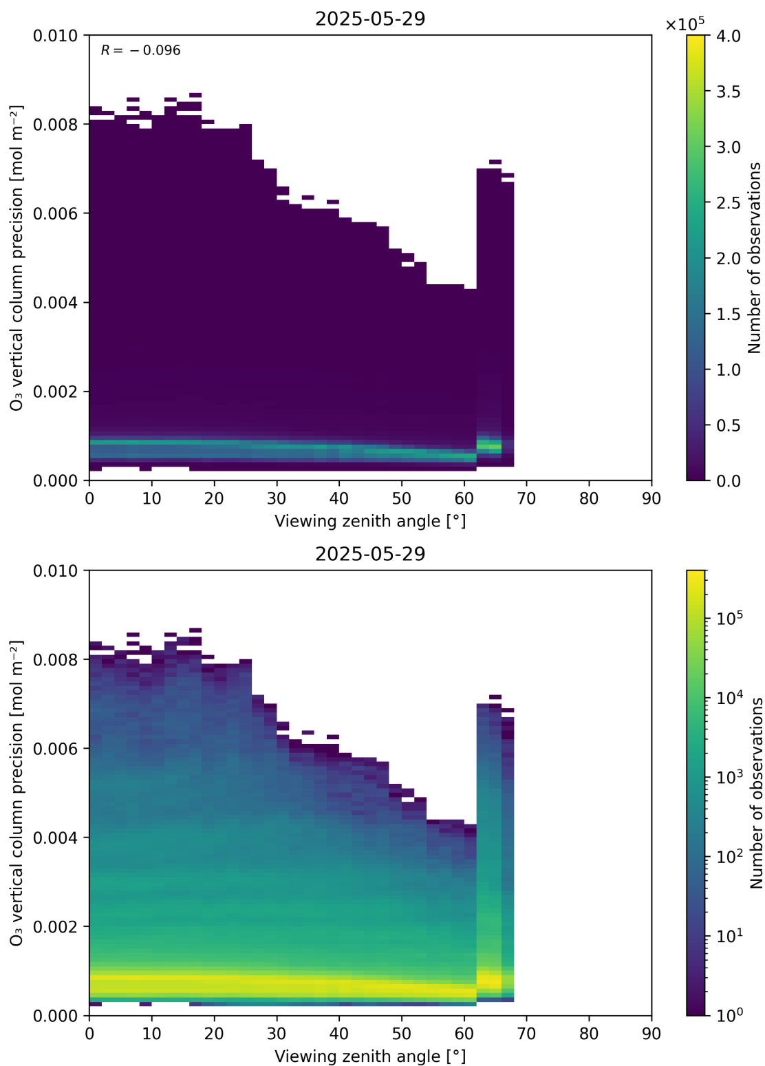
Figure 53: Scatter density plot of “Viewing zenith angle” against “O 3 vertical column precision” for 2025-05-28 to 2025-05-30.
