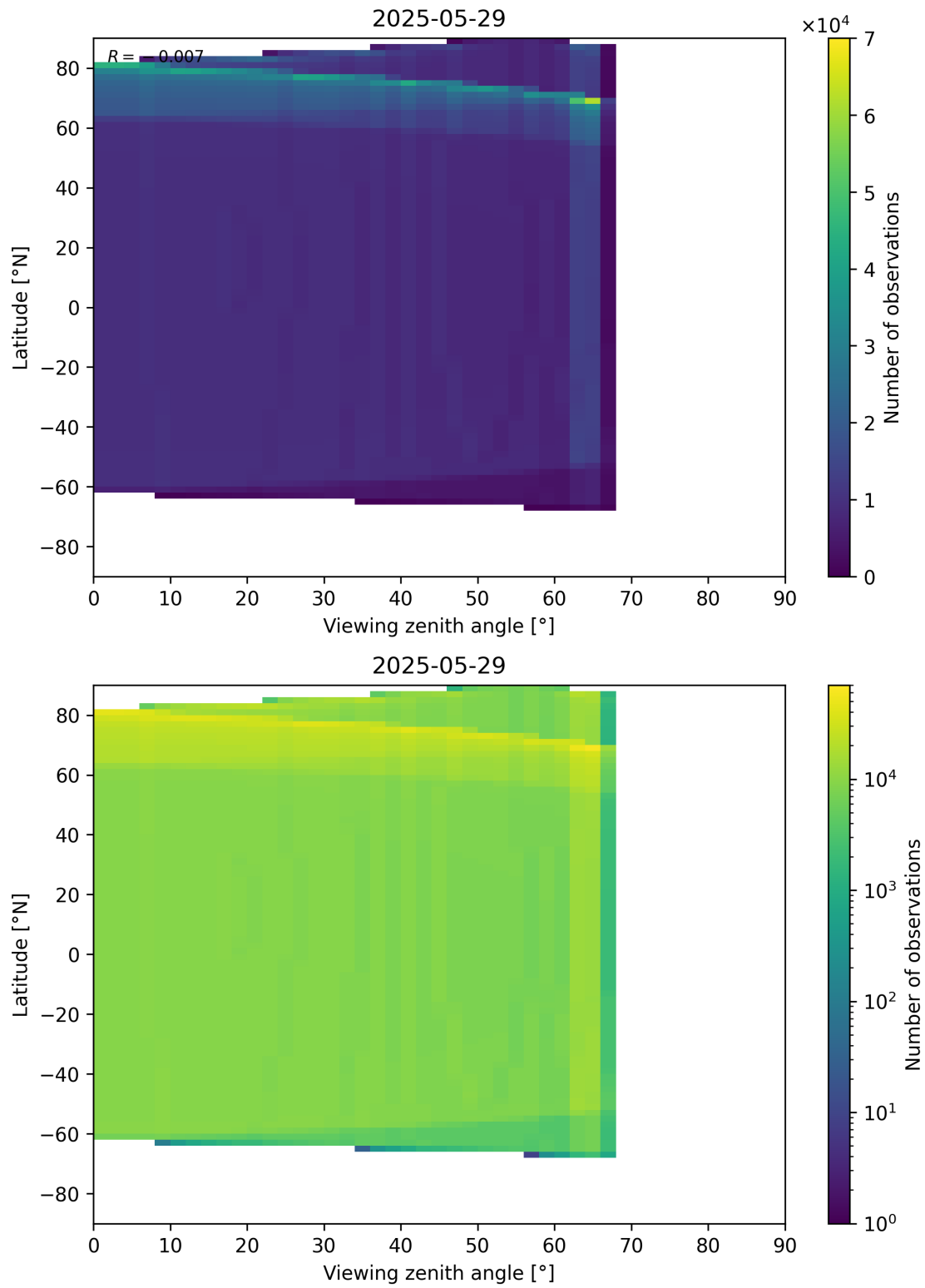
Figure 49: Scatter density plot of “Viewing zenith angle” against “Latitude” for 2025-05-28 to 2025-05-30.
