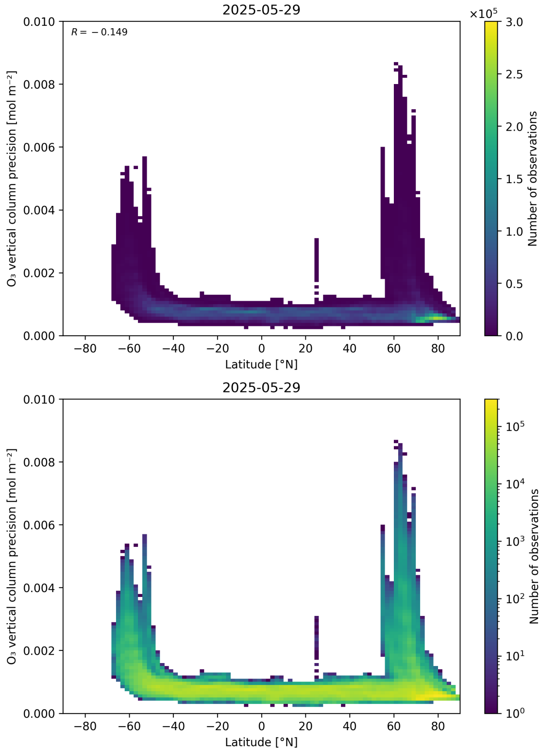
Figure 37: Scatter density plot of “Latitude” against “O 3 vertical column precision” for 2025-05-28 to 2025-05-30.
