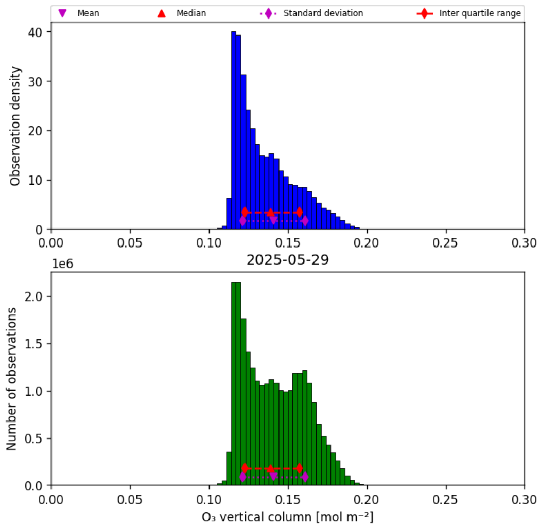
Figure 21: Histogram of “O 3 vertical column” for 2025-05-28 to 2025-05-30
