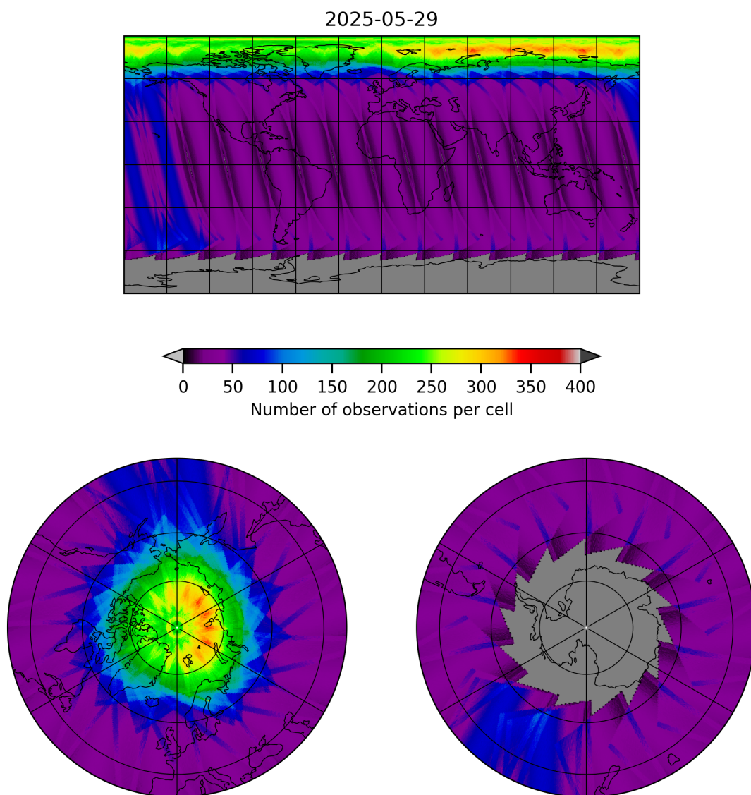
Figure 12: Map of the number of observations for 2025-05-28 to 2025-05-30
