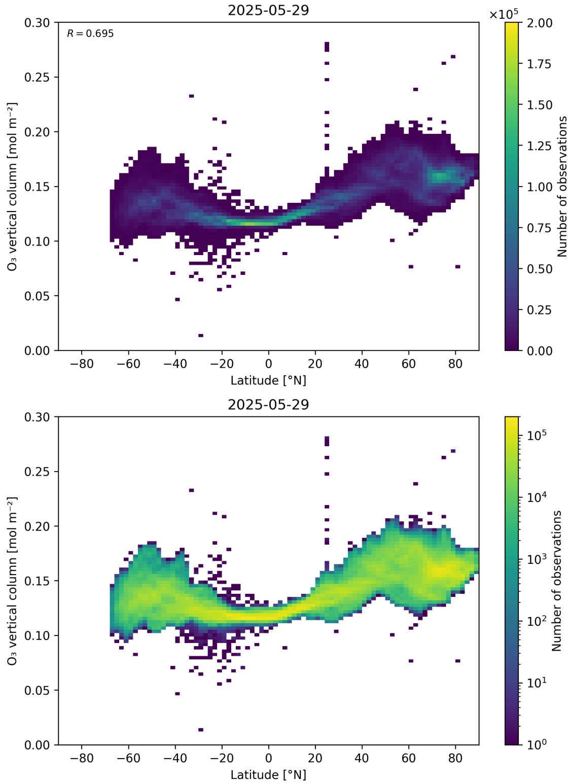
Figure 36: Scatter density plot of “Latitude” against “O 3 vertical column” for 2025-05-28 to 2025-05-30.
