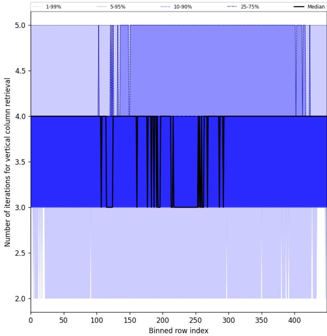
Figure 33: Along track statistics of “Number of iterations for vertical column retrieval” for 2025-05-28 to 2025-05-30
